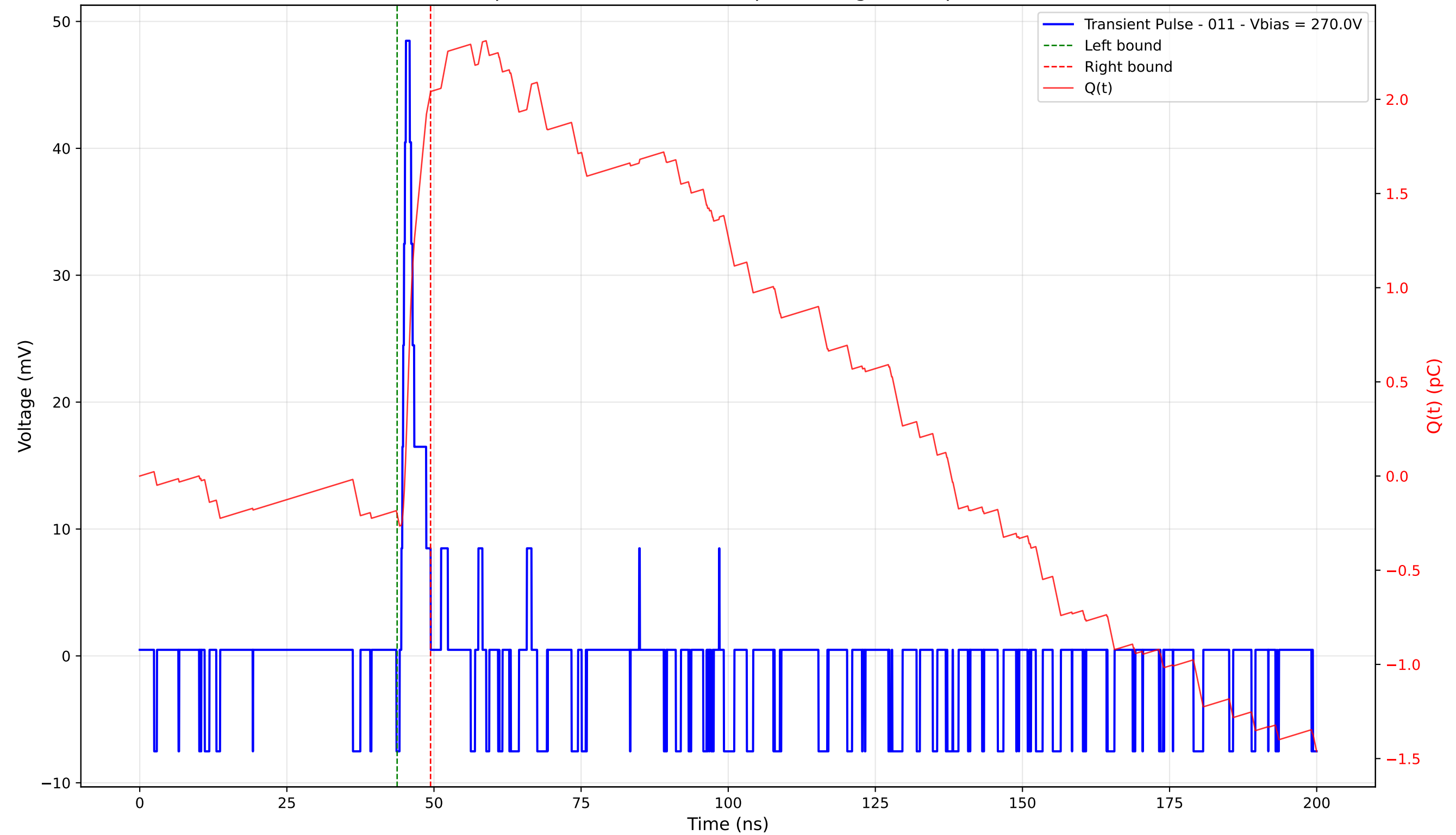
Transient Pulse - Sample: 4003 - Position: 80.0 \mu\text{m} - Charge: 2.24 pC - Rise Time: 0.77 ns
