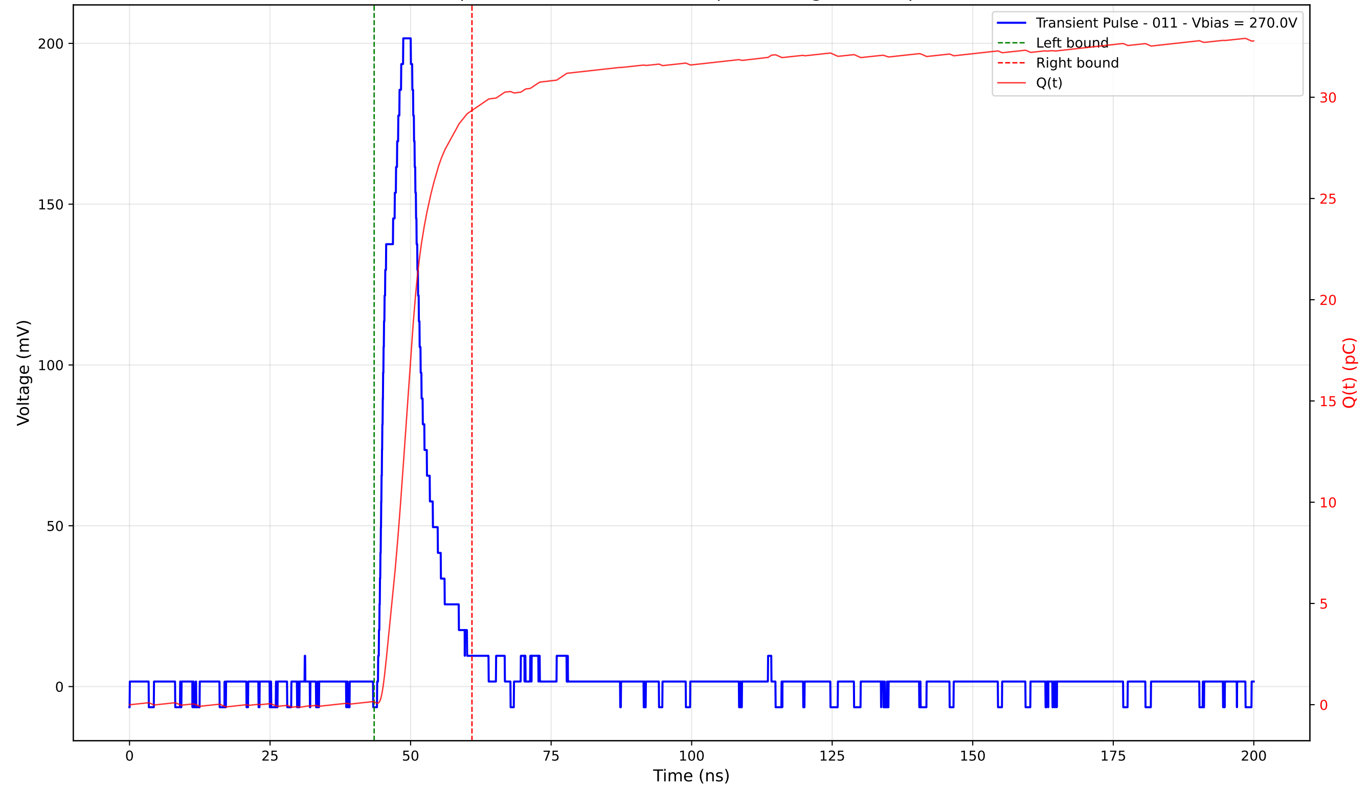
Transient Pulse - Sample: 4003 - Position: 380.0 \mu\text{m} - Charge: 29.22 pC - Rise Time: 3.57 ns
