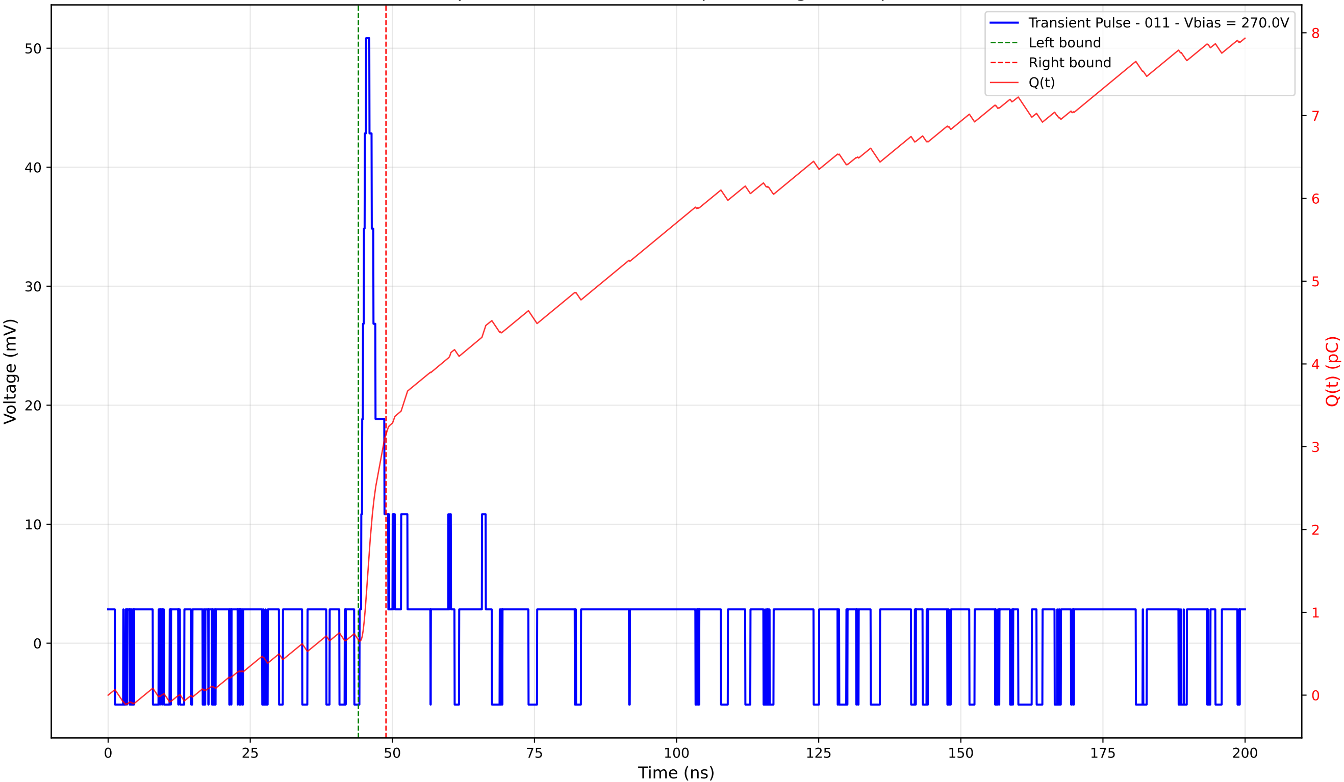
Transient Pulse - Sample: 4003 - Position: 45.0 \mu\text{m} - Charge: 2.48 pC - Rise Time: 0.85 ns
