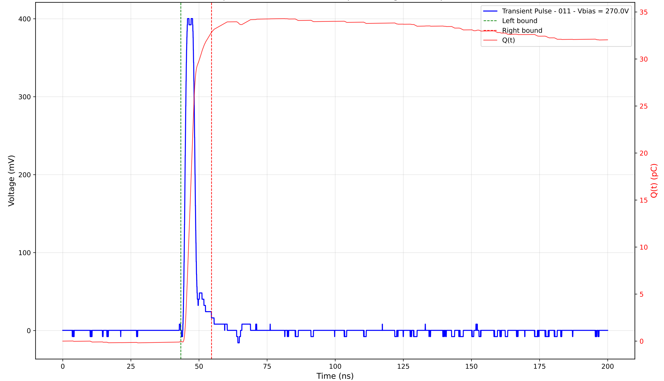
Transient Pulse - Sample: 4003 - Position: 310.0 \mu\text{m} - Charge: 32.89 pC - Rise Time: 1.12 ns
