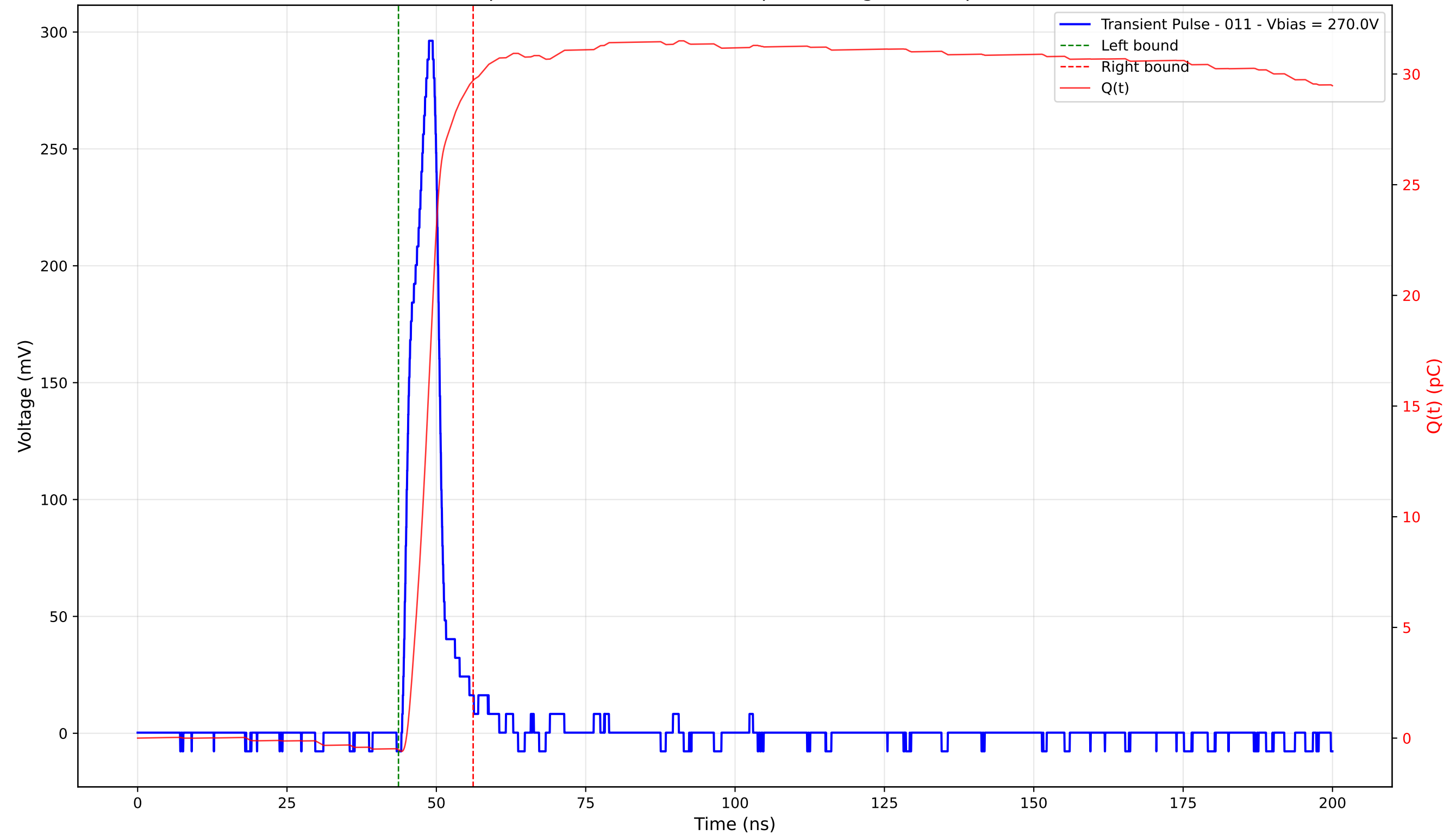
Transient Pulse - Sample: 4003 - Position: 370.0 \mu\text{m} - Charge: 30.24 pC - Rise Time: 3.57 ns
