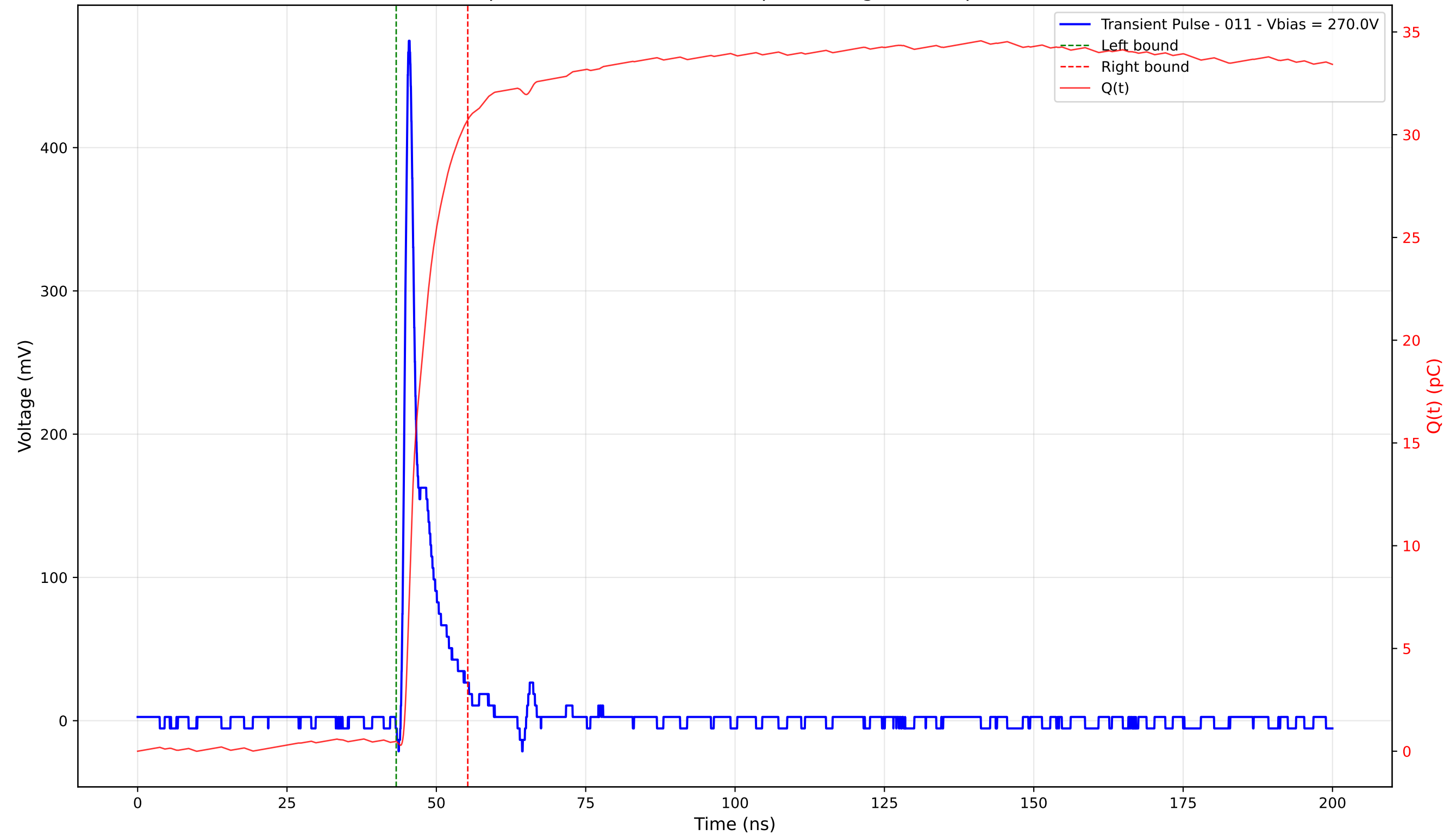
Transient Pulse - Sample: 4003 - Position: 110.0 \mu\text{m} - Charge: 30.26 pC - Rise Time: 0.91 ns
