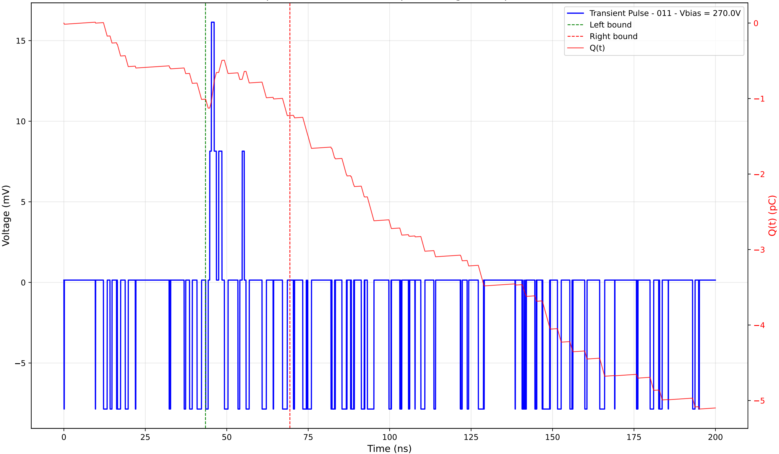
Transient Pulse - Sample: 4003 - Position: 5.0 \mu\text{m} - Charge: 0.22 pC - Rise Time: 0.52 ns
