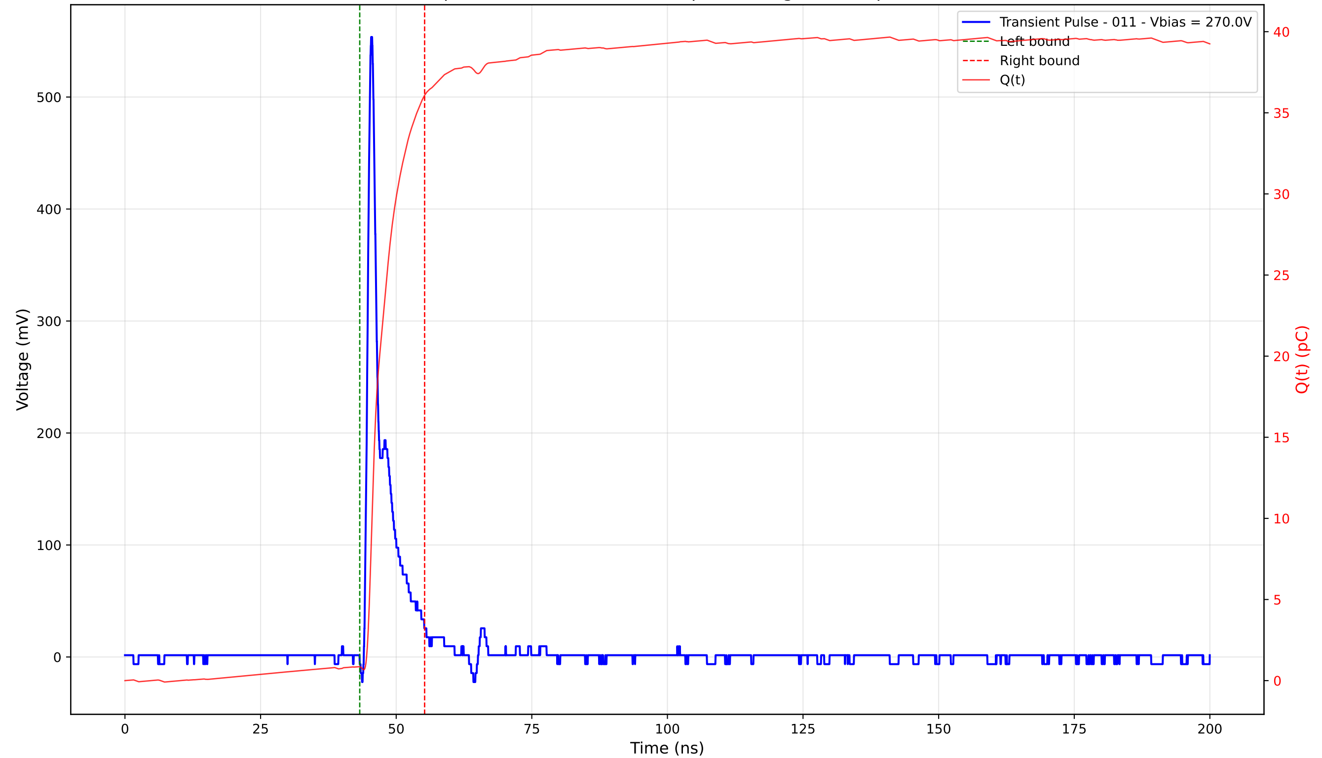
Transient Pulse - Sample: 4003 - Position: 120.0 \mu\text{m} - Charge: 35.22 pC - Rise Time: 0.89 ns
