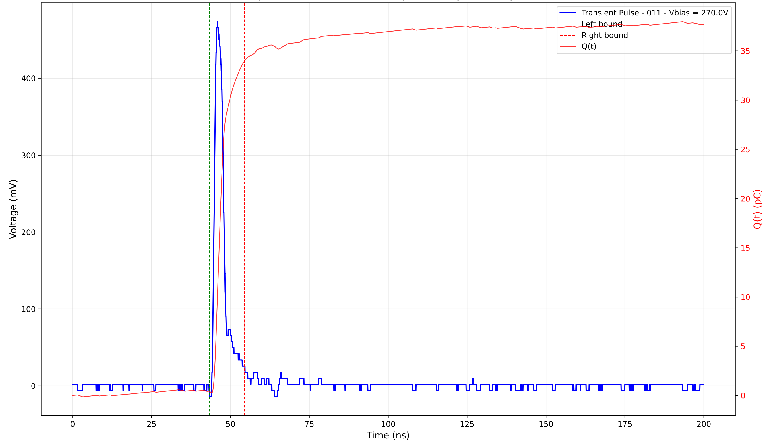
Transient Pulse - Sample: 4003 - Position: 275.0 \mu\text{m} - Charge: 33.56 pC - Rise Time: 1.15 ns
