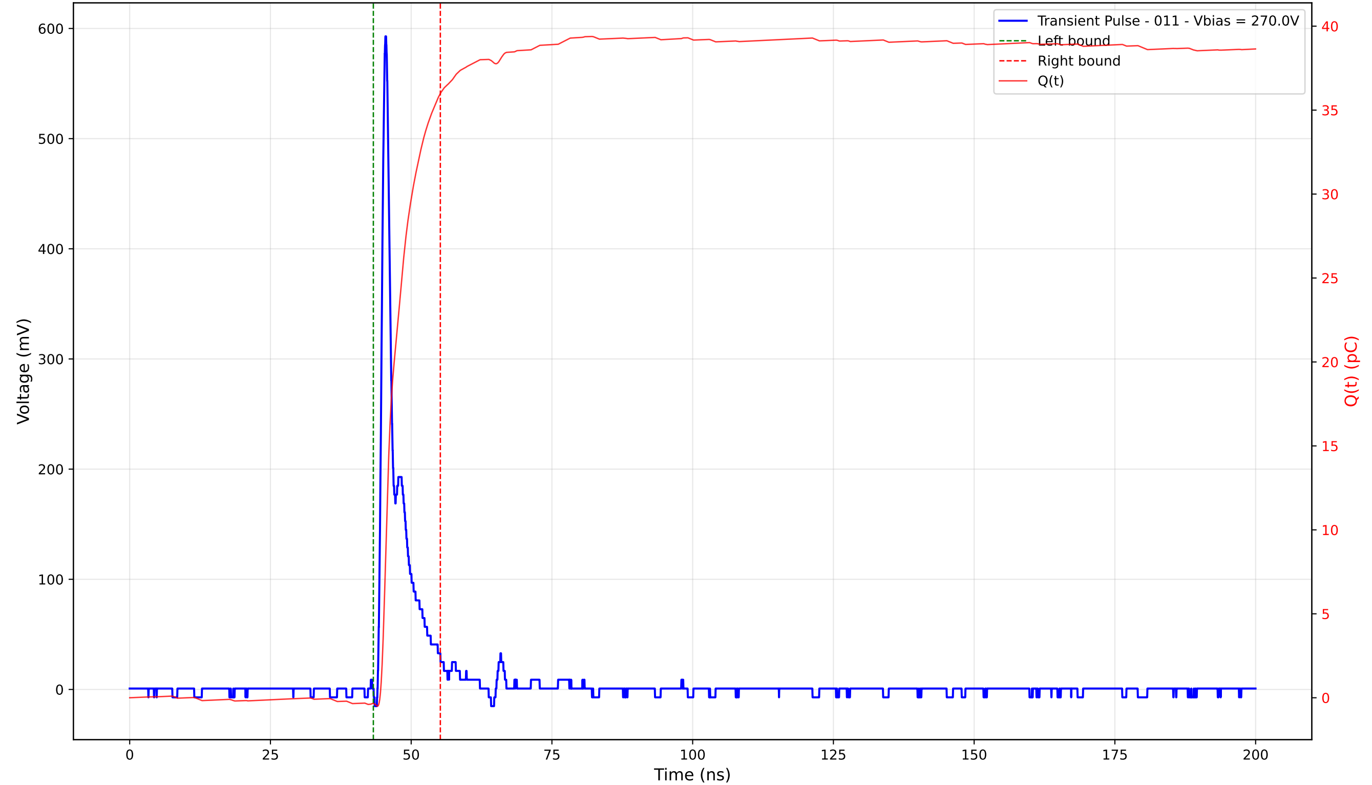
Transient Pulse - Sample: 4003 - Position: 135.0 \mu\text{m} - Charge: 36.34 pC - Rise Time: 0.91 ns
