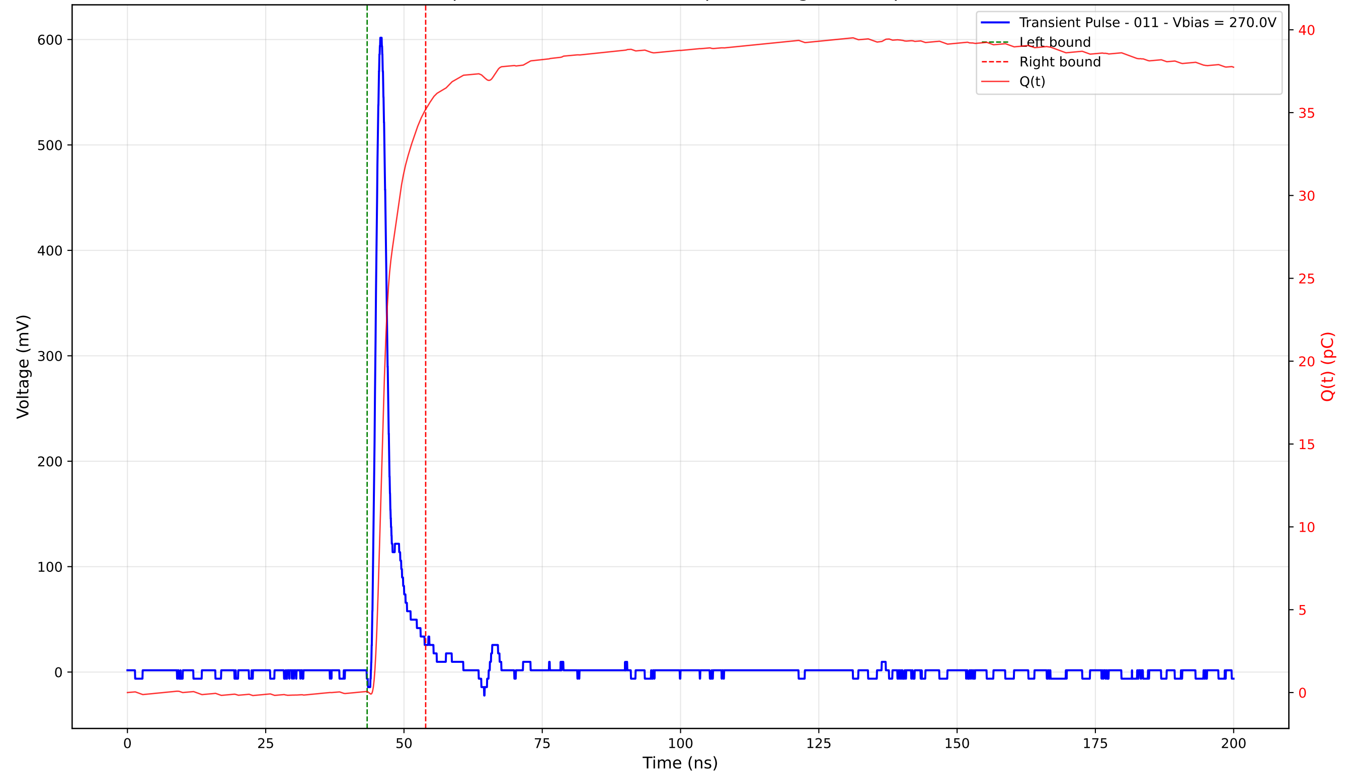
Transient Pulse - Sample: 4003 - Position: 220.0 \mu\text{m} - Charge: 35.13 pC - Rise Time: 1.08 ns
