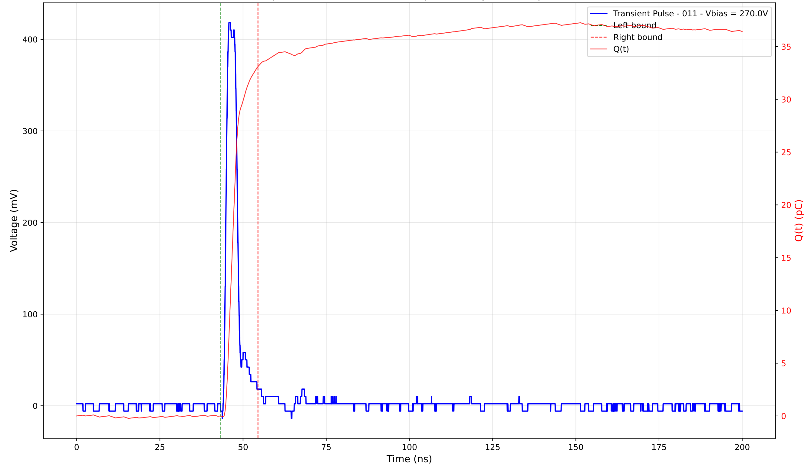
Transient Pulse - Sample: 4003 - Position: 300.0 \mu\text{m} - Charge: 33.11 pC - Rise Time: 1.12 ns
