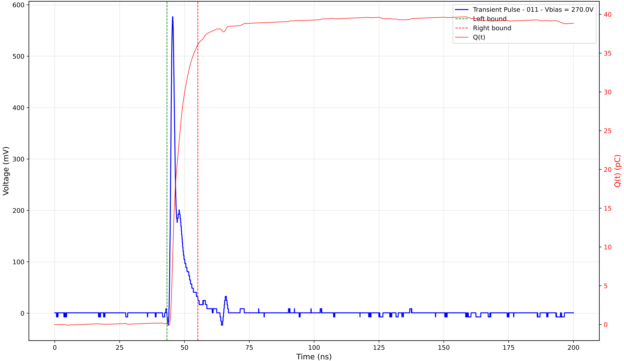
Transient Pulse - Sample: 4003 - Position: 125.0 \mu\text{m} - Charge: 35.99 pC - Rise Time: 0.89 ns
