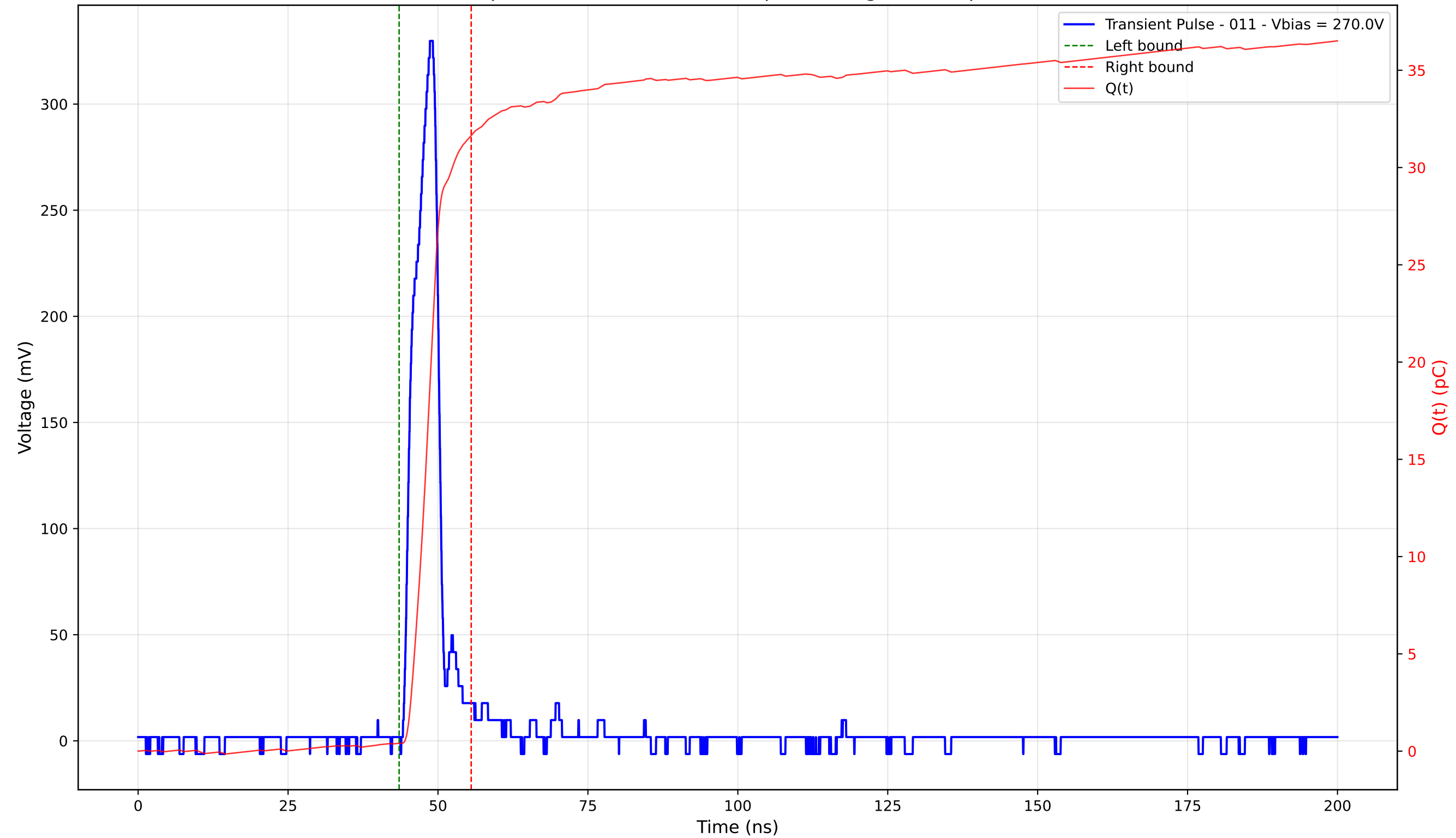
Transient Pulse - Sample: 4003 - Position: 365.0 \mu\text{m} - Charge: 31.24 pC - Rise Time: 3.44 ns
