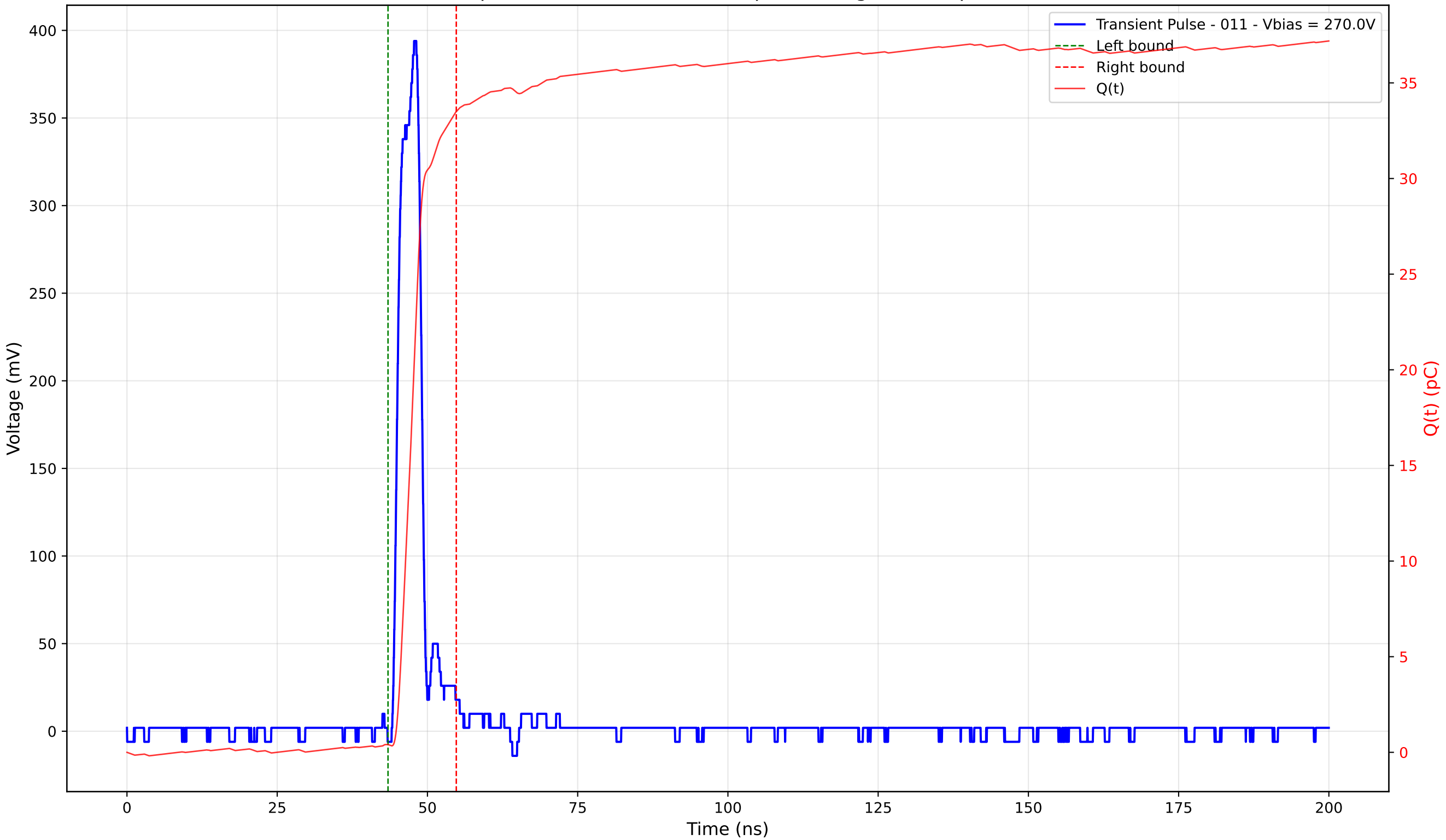
Transient Pulse - Sample: 4003 - Position: 335.0 \mu\text{m} - Charge: 33.09 pC - Rise Time: 2.77 ns
