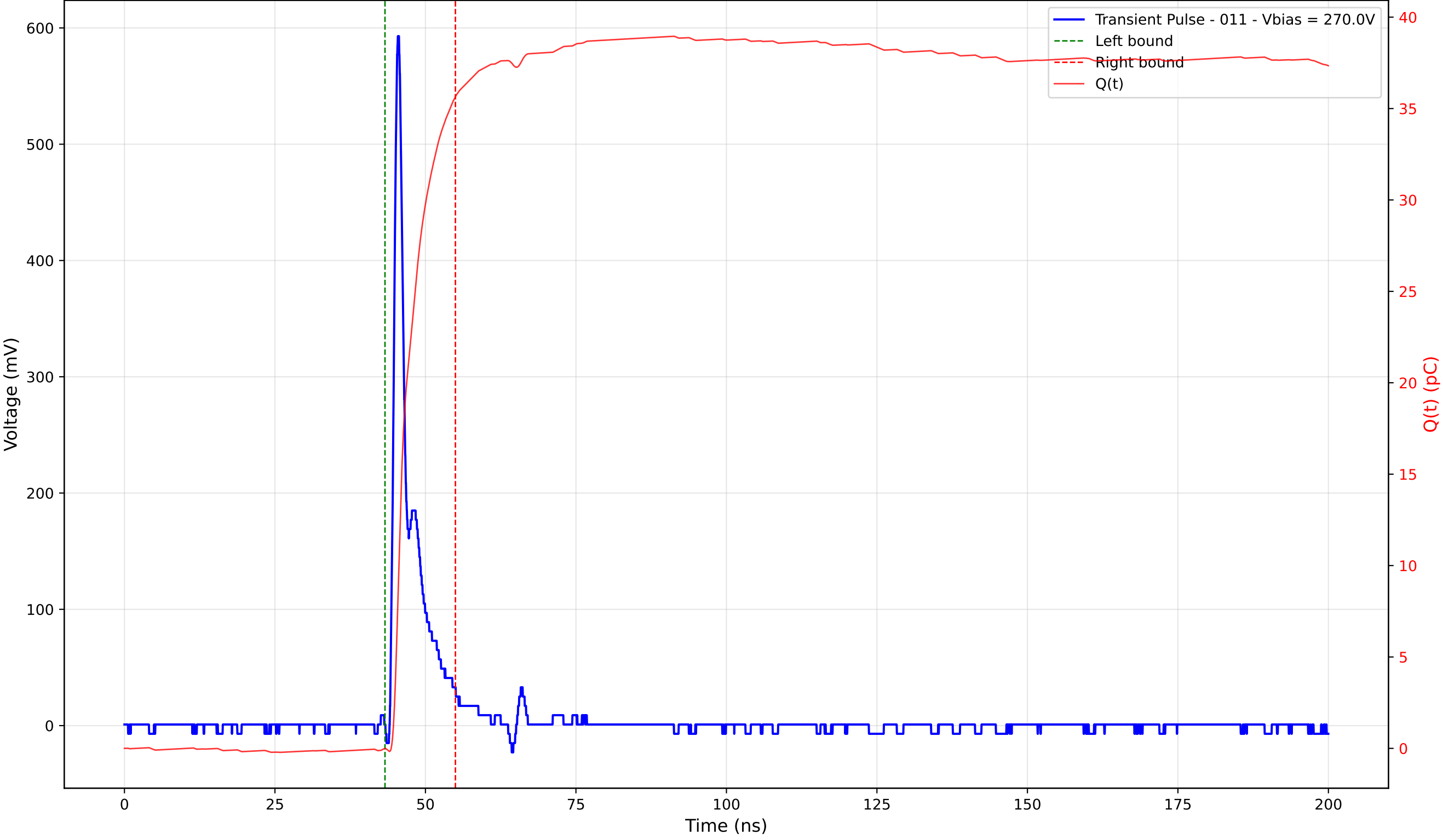
Transient Pulse - Sample: 4003 - Position: 140.0 \mu\text{m} - Charge: 35.66 pC - Rise Time: 0.91 ns
