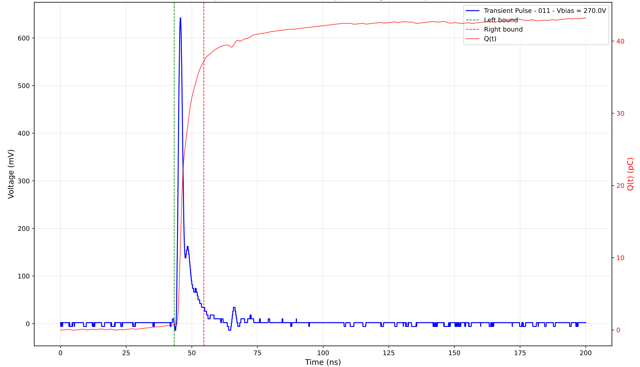
Transient Pulse - Sample: 4003 - Position: 185.0 \mu\text{m} - Charge: 36.47 pC - Rise Time: 1.00 ns
