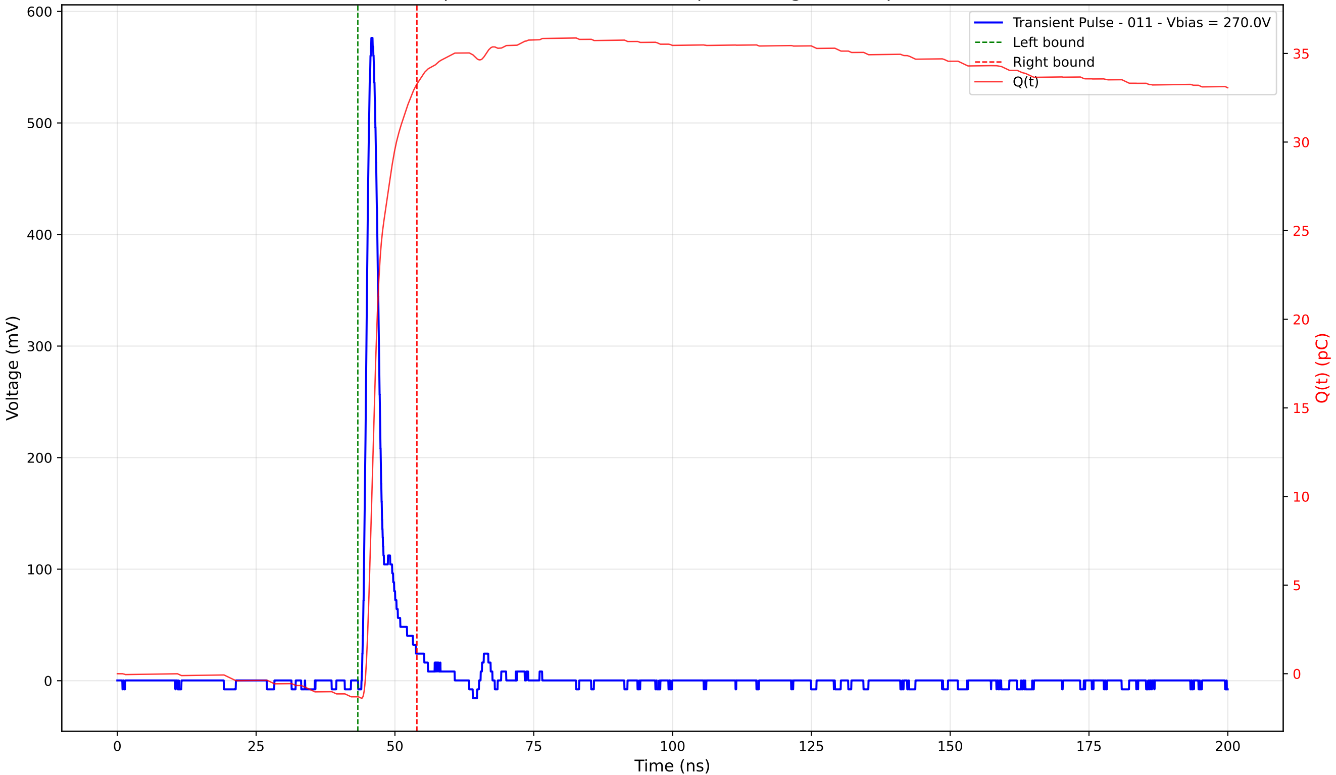
Transient Pulse - Sample: 4003 - Position: 230.0 \mu\text{m} - Charge: 34.57 pC - Rise Time: 1.10 ns
