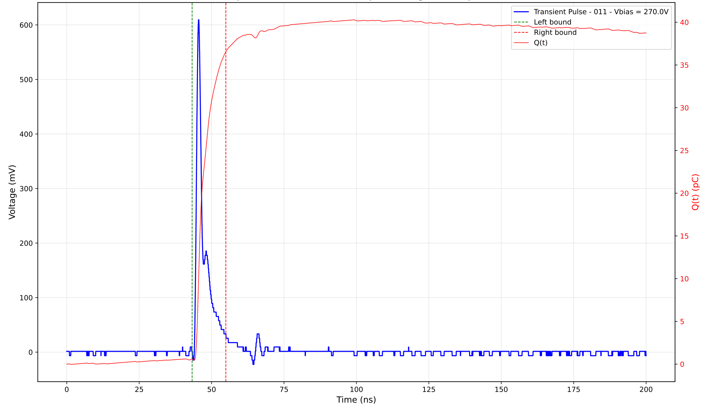
Transient Pulse - Sample: 4003 - Position: 150.0 \mu\text{m} - Charge: 35.95 pC - Rise Time: 0.94 ns
