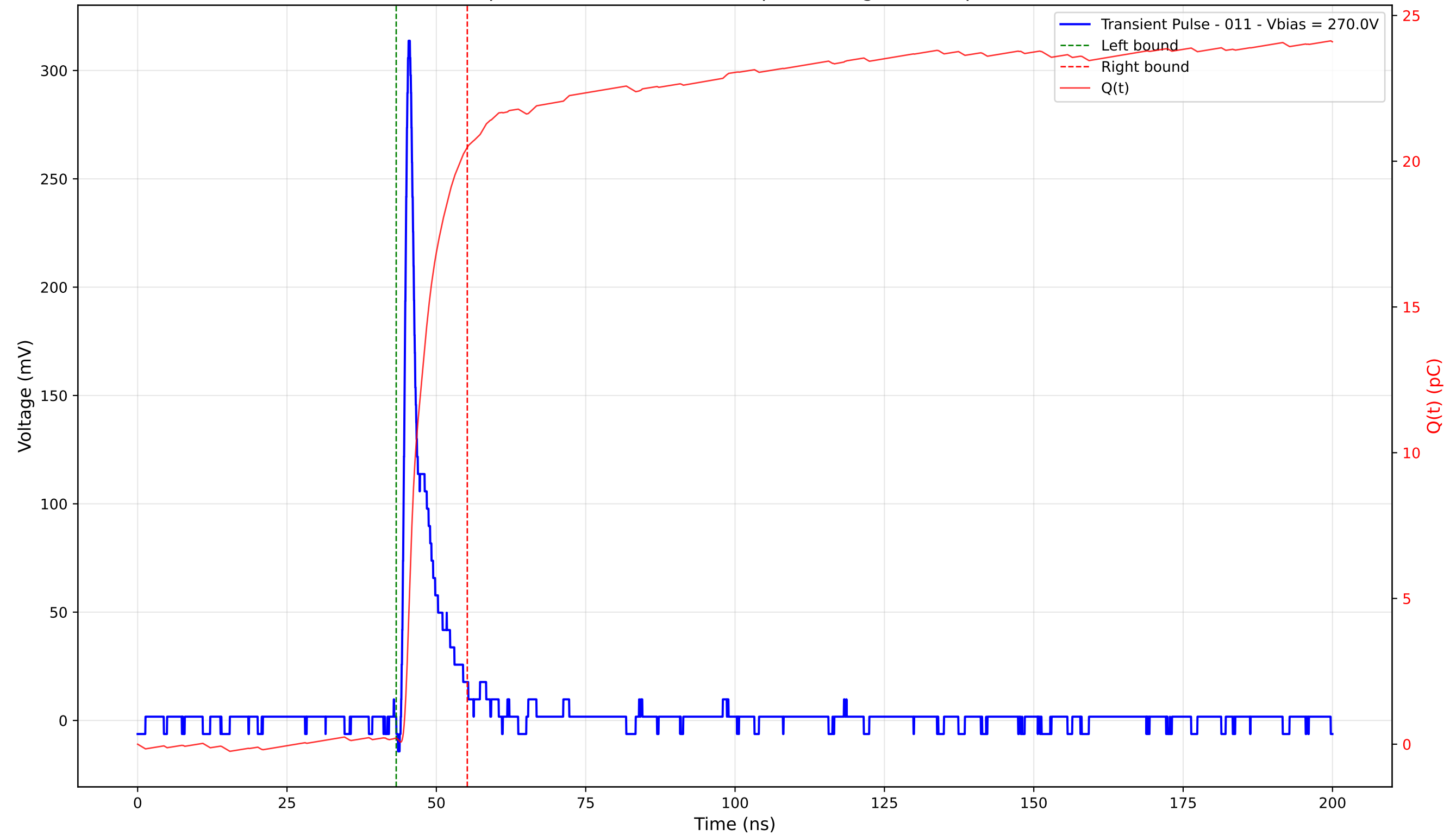
Transient Pulse - Sample: 4003 - Position: 100.0 \mu\text{m} - Charge: 20.27 pC - Rise Time: 0.91 ns
