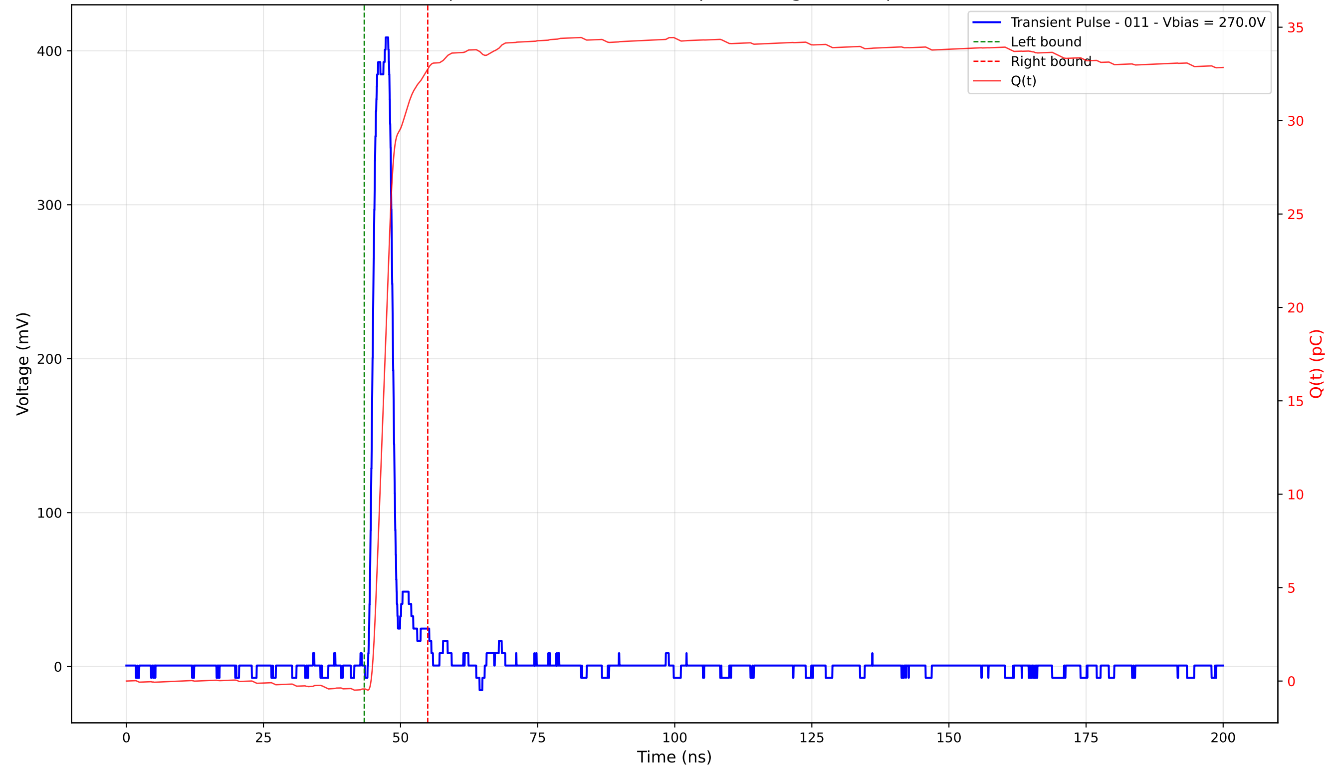
Transient Pulse - Sample: 4003 - Position: 315.0 \mu\text{m} - Charge: 33.19 pC - Rise Time: 1.22 ns
