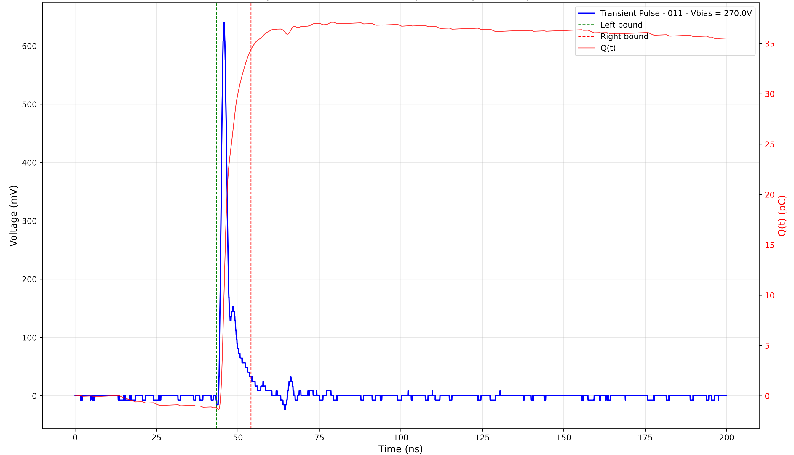
Transient Pulse - Sample: 4003 - Position: 195.0 \mu\text{m} - Charge: 35.58 pC - Rise Time: 1.04 ns
