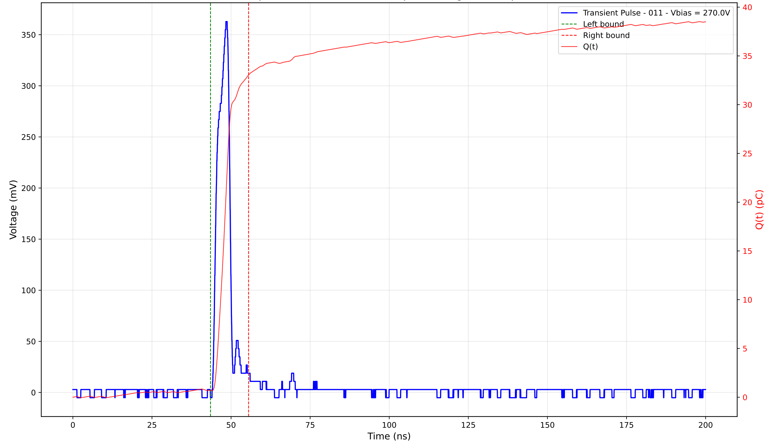
Transient Pulse - Sample: 4003 - Position: 355.0 \mu\text{m} - Charge: 32.33 pC - Rise Time: 3.24 ns
