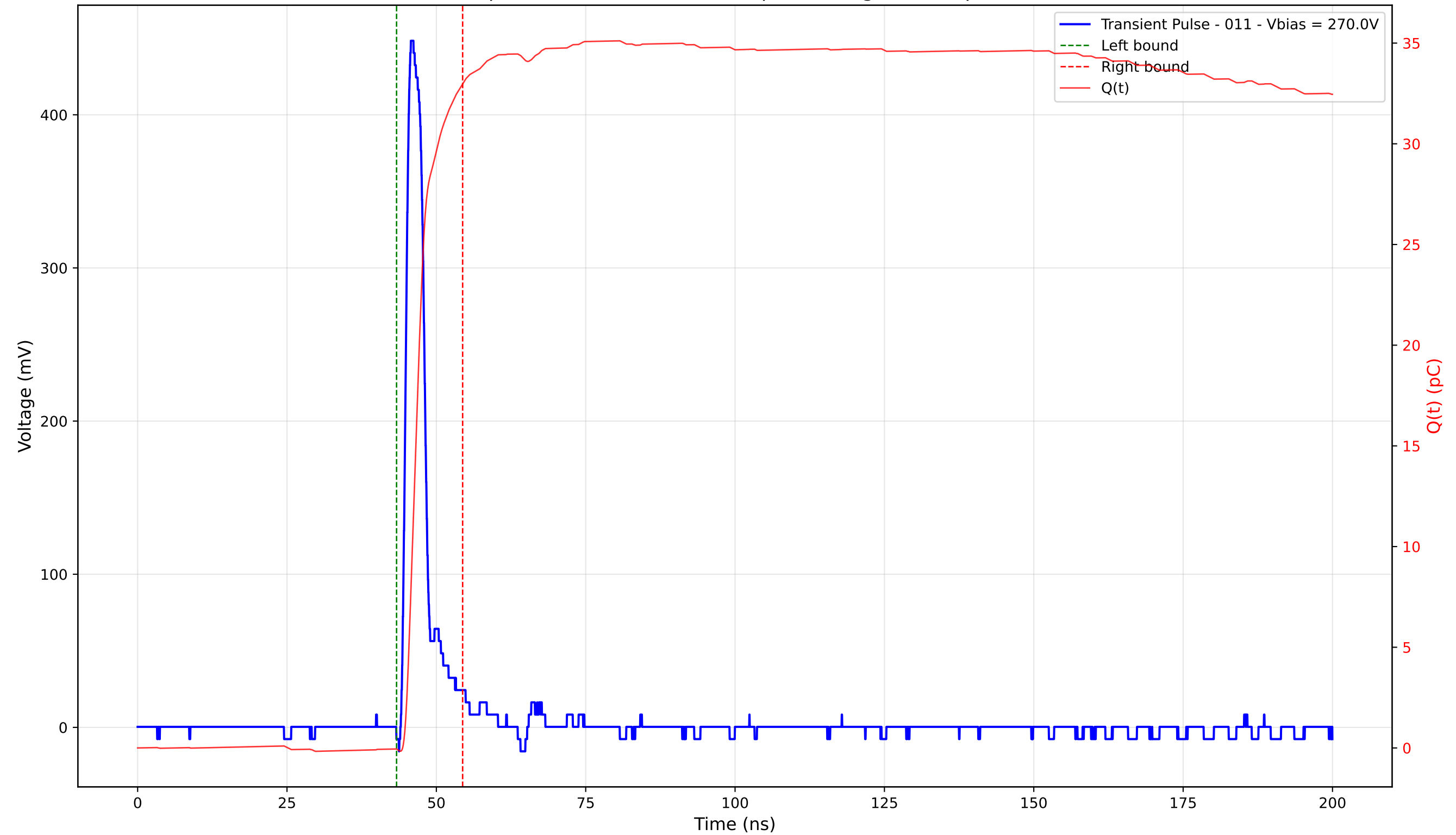
Transient Pulse - Sample: 4003 - Position: 285.0 \mu\text{m} - Charge: 33.03 pC - Rise Time: 1.11 ns
