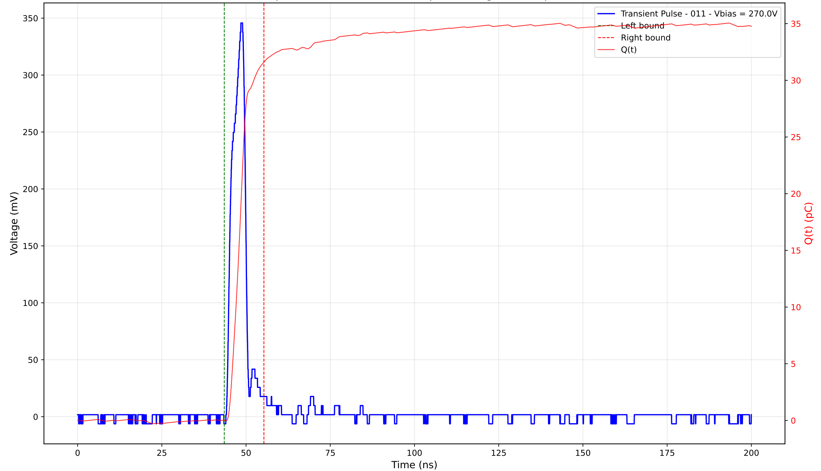
Transient Pulse - Sample: 4003 - Position: 360.0 \mu\text{m} - Charge: 31.58 pC - Rise Time: 3.32 ns
