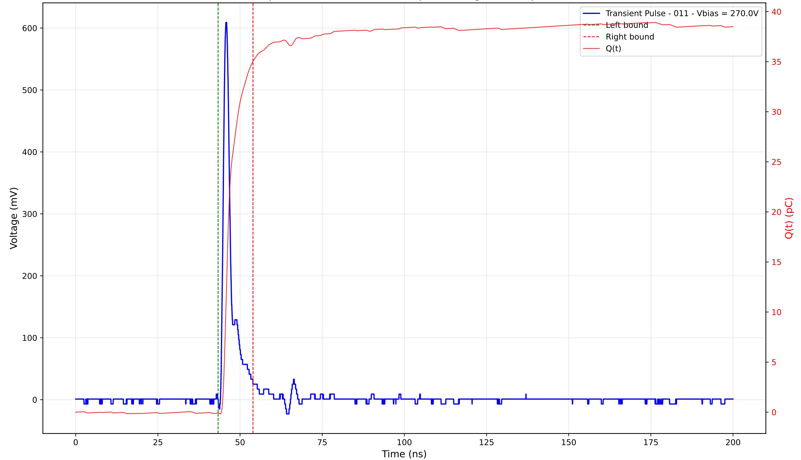
Transient Pulse - Sample: 4003 - Position: 210.0 \mu\text{m} - Charge: 35.11 pC - Rise Time: 1.06 ns
