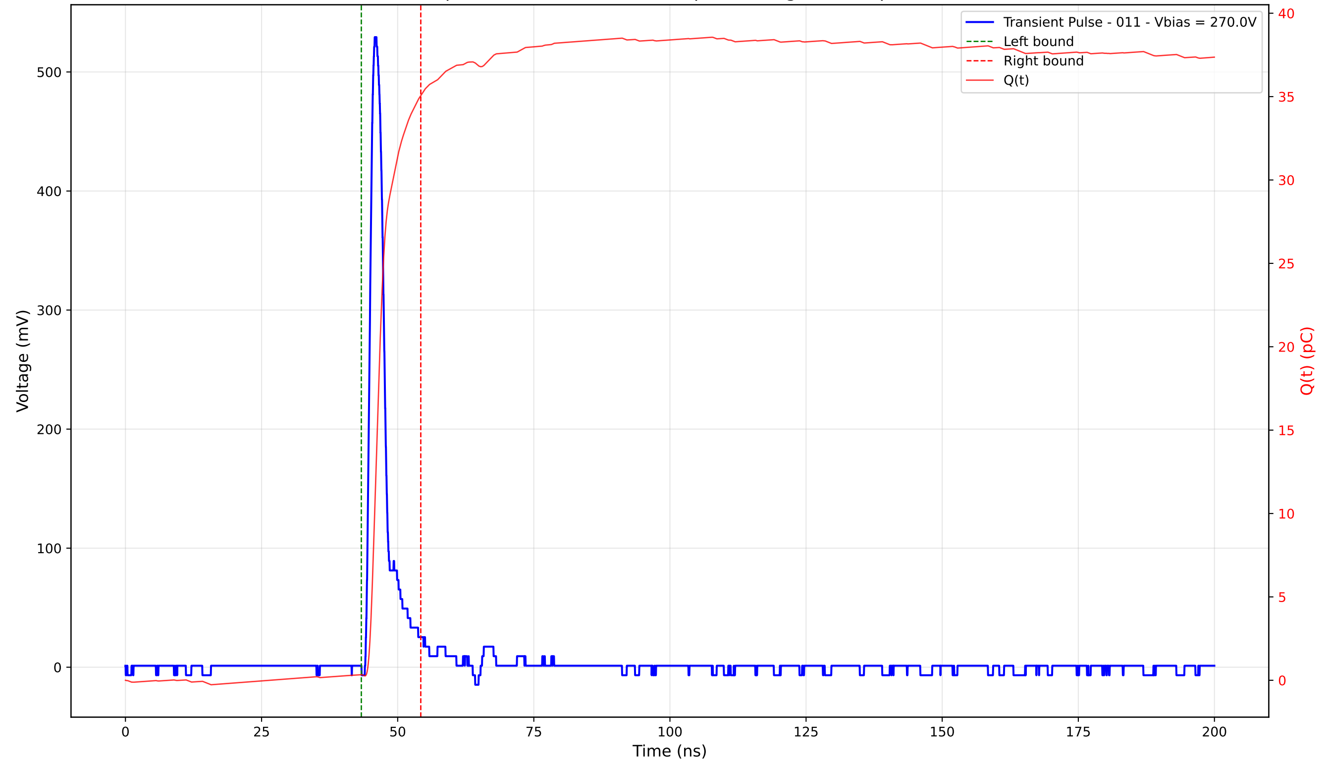
Transient Pulse - Sample: 4003 - Position: 255.0 \mu\text{m} - Charge: 34.72 pC - Rise Time: 1.11 ns
