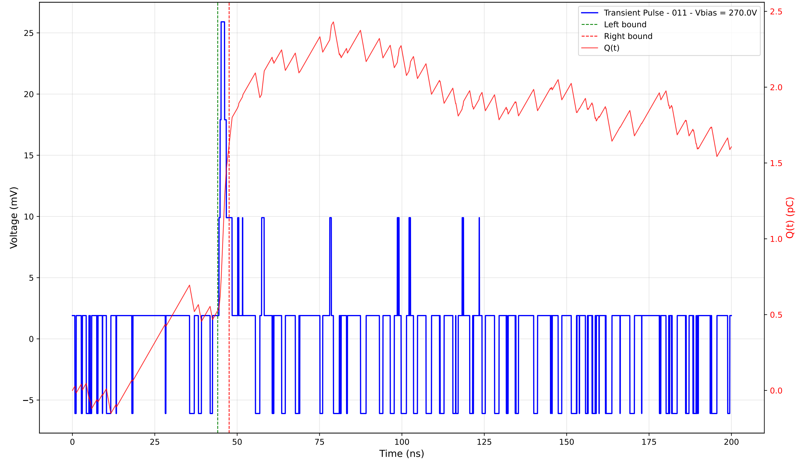
Transient Pulse - Sample: 4003 - Position: 75.0 \mu\text{m} - Charge: 1.10 pC - Rise Time: 0.66 ns
