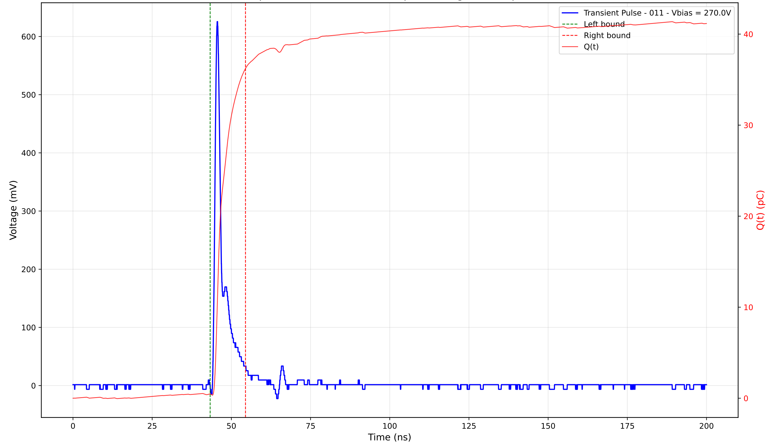
Transient Pulse - Sample: 4003 - Position: 165.0 \mu\text{m} - Charge: 35.75 pC - Rise Time: 0.97 ns
