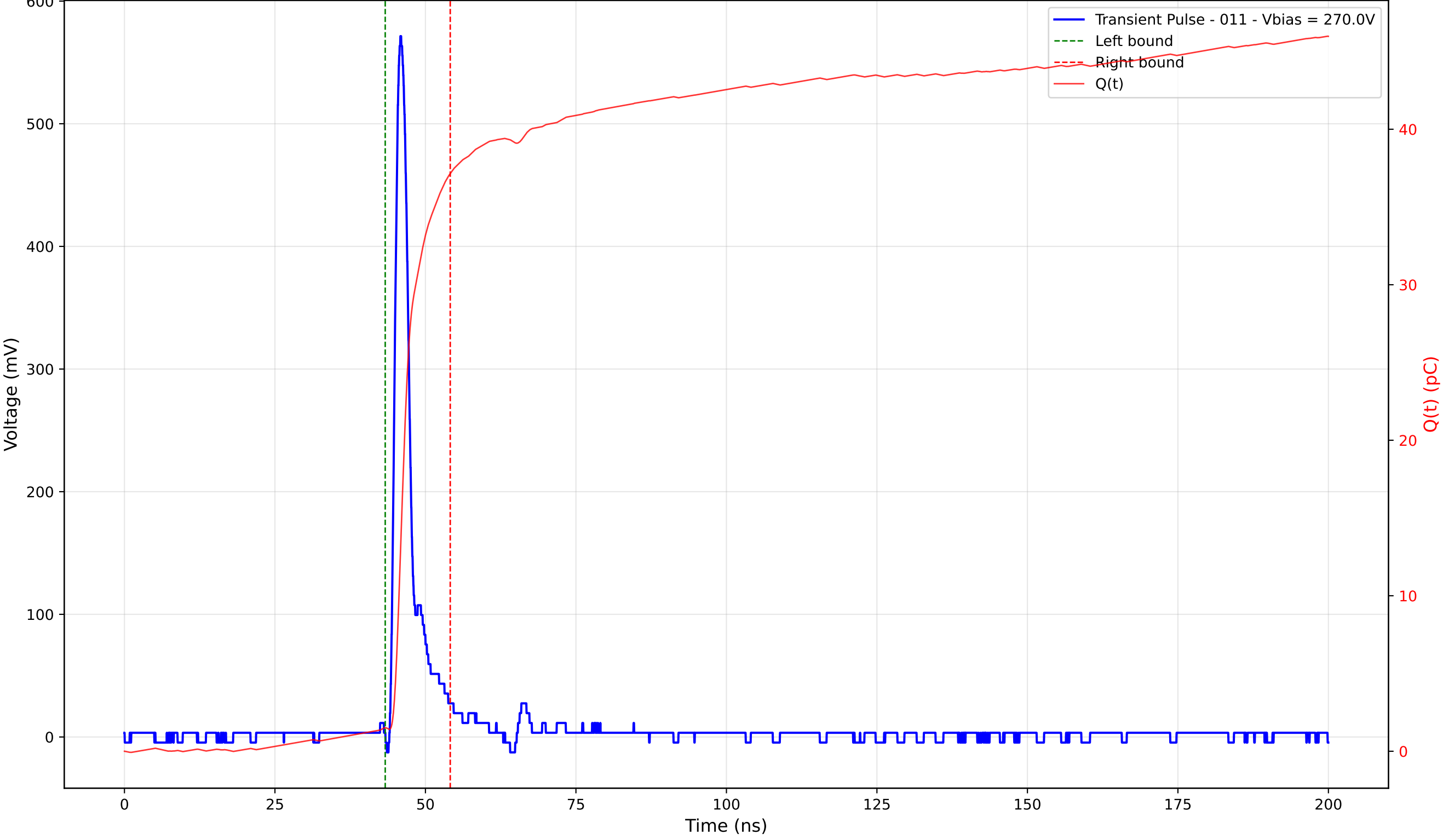
Transient Pulse - Sample: 4003 - Position: 240.0 \mu\text{m} - Charge: 35.64 pC - Rise Time: 1.11 ns
