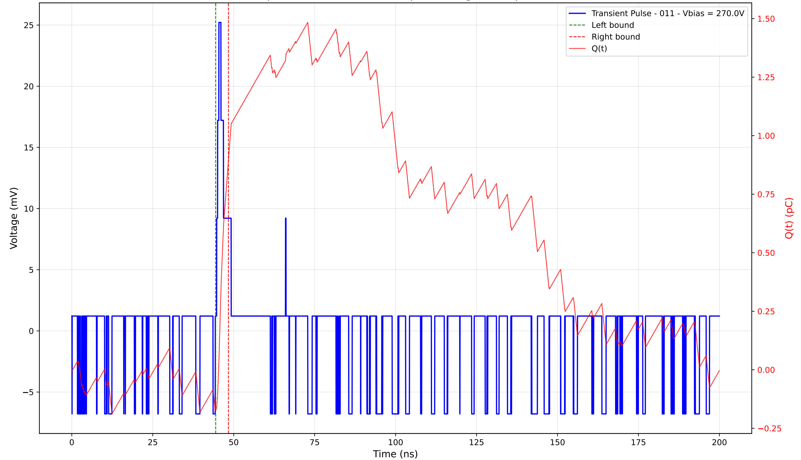
Transient Pulse - Sample: 4003 - Position: 65.0 \mu\text{m} - Charge: 1.07 pC - Rise Time: 0.70 ns
