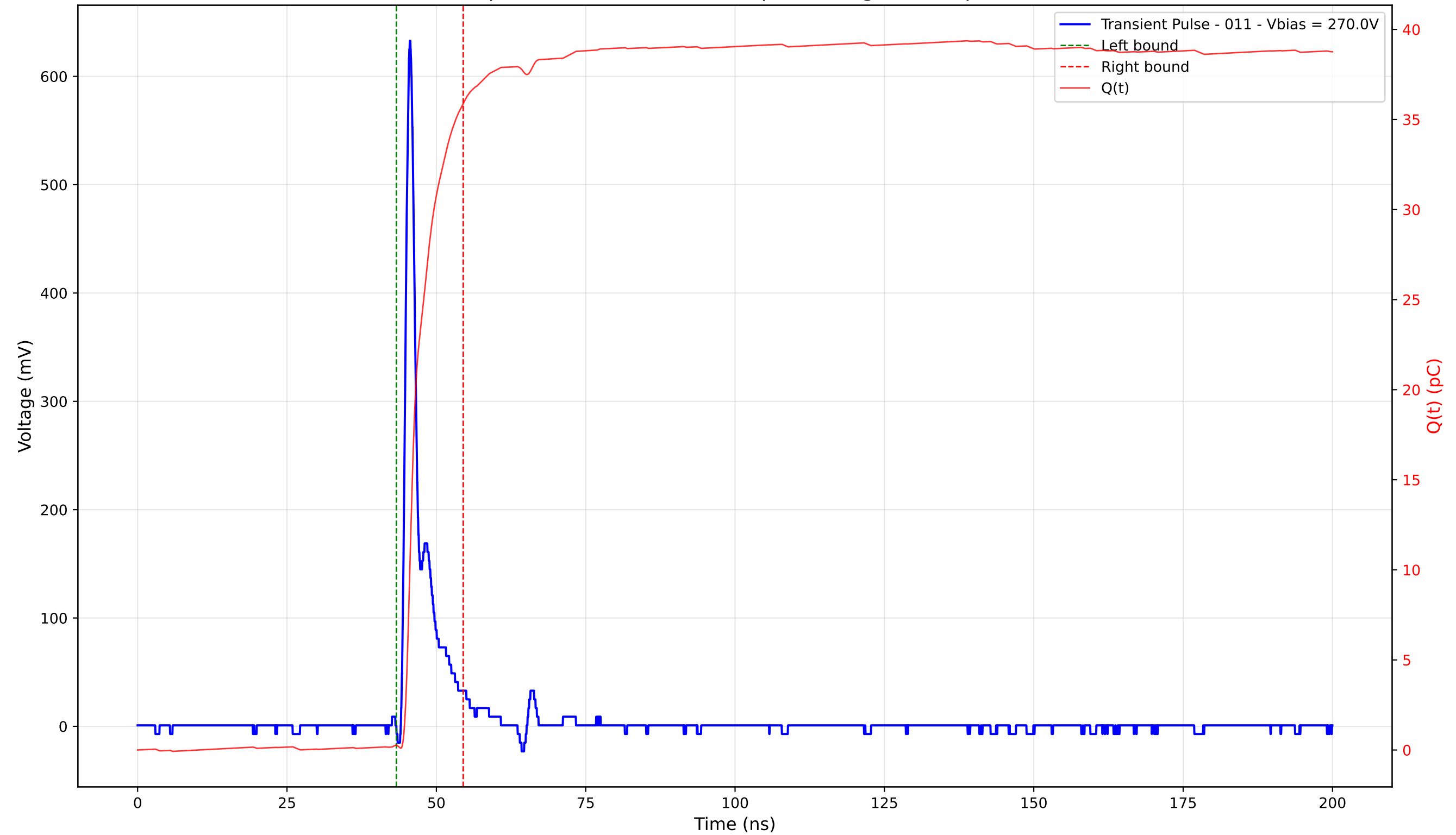
Transient Pulse - Sample: 4003 - Position: 170.0 \mu\text{m} - Charge: 35.62 pC - Rise Time: 0.97 ns
