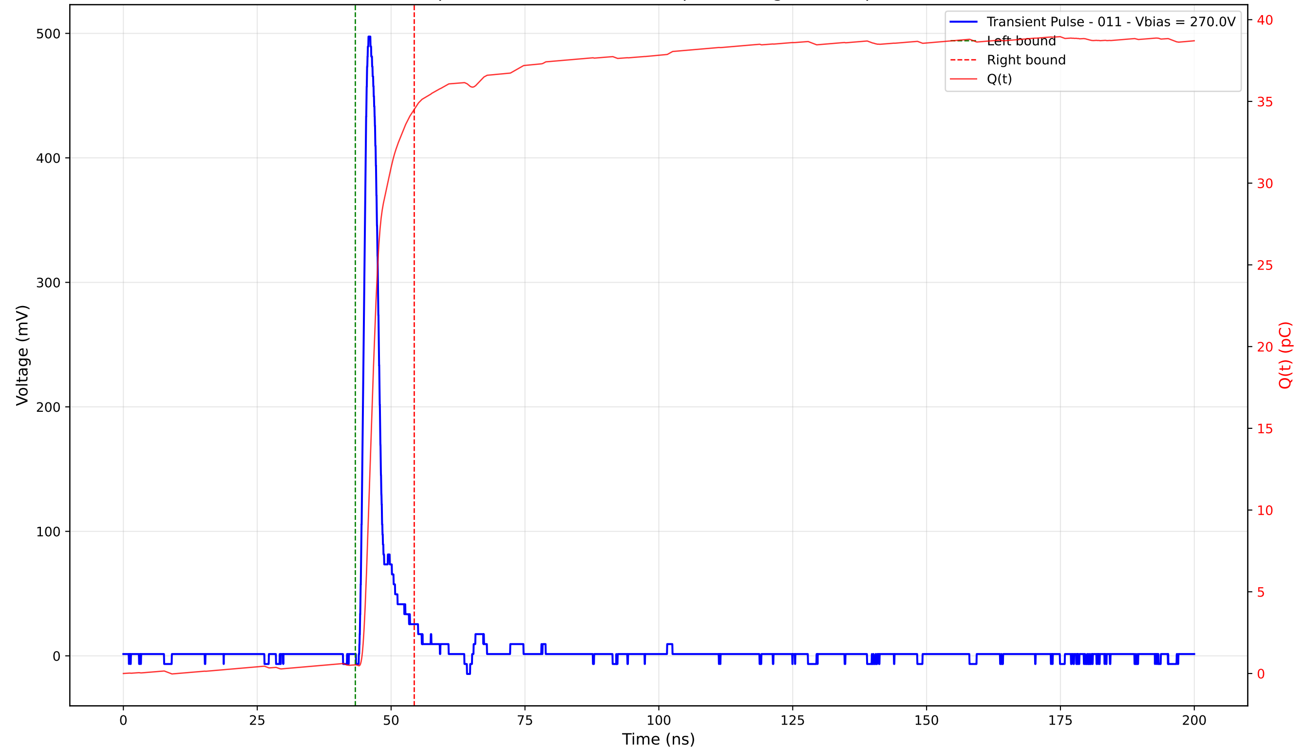
Transient Pulse - Sample: 4003 - Position: 265.0 \mu\text{m} - Charge: 33.98 pC - Rise Time: 1.10 ns
