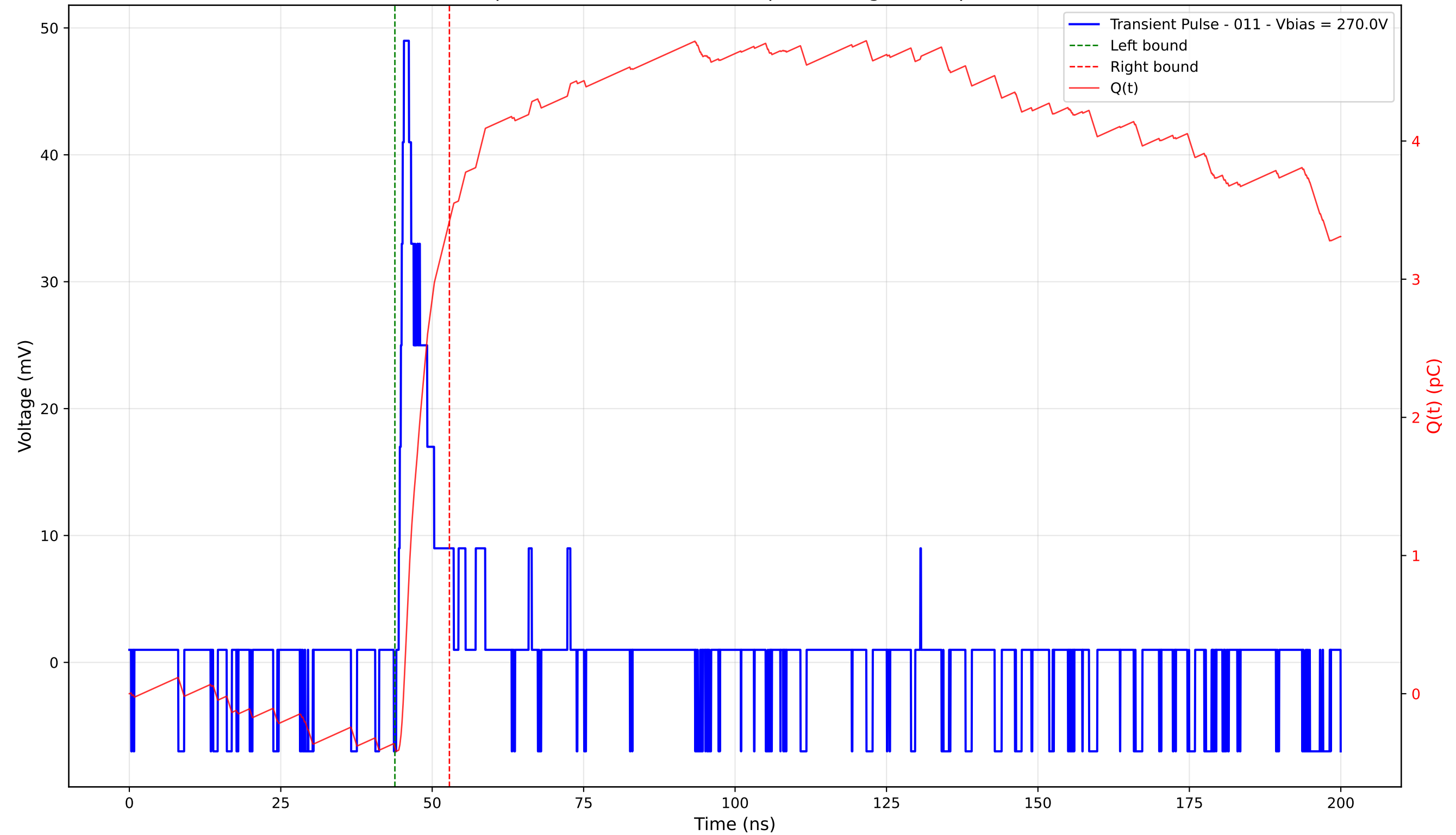
Transient Pulse - Sample: 4003 - Position: 410.0 \mu\text{m} - Charge: 3.81 pC - Rise Time: 0.85 ns
