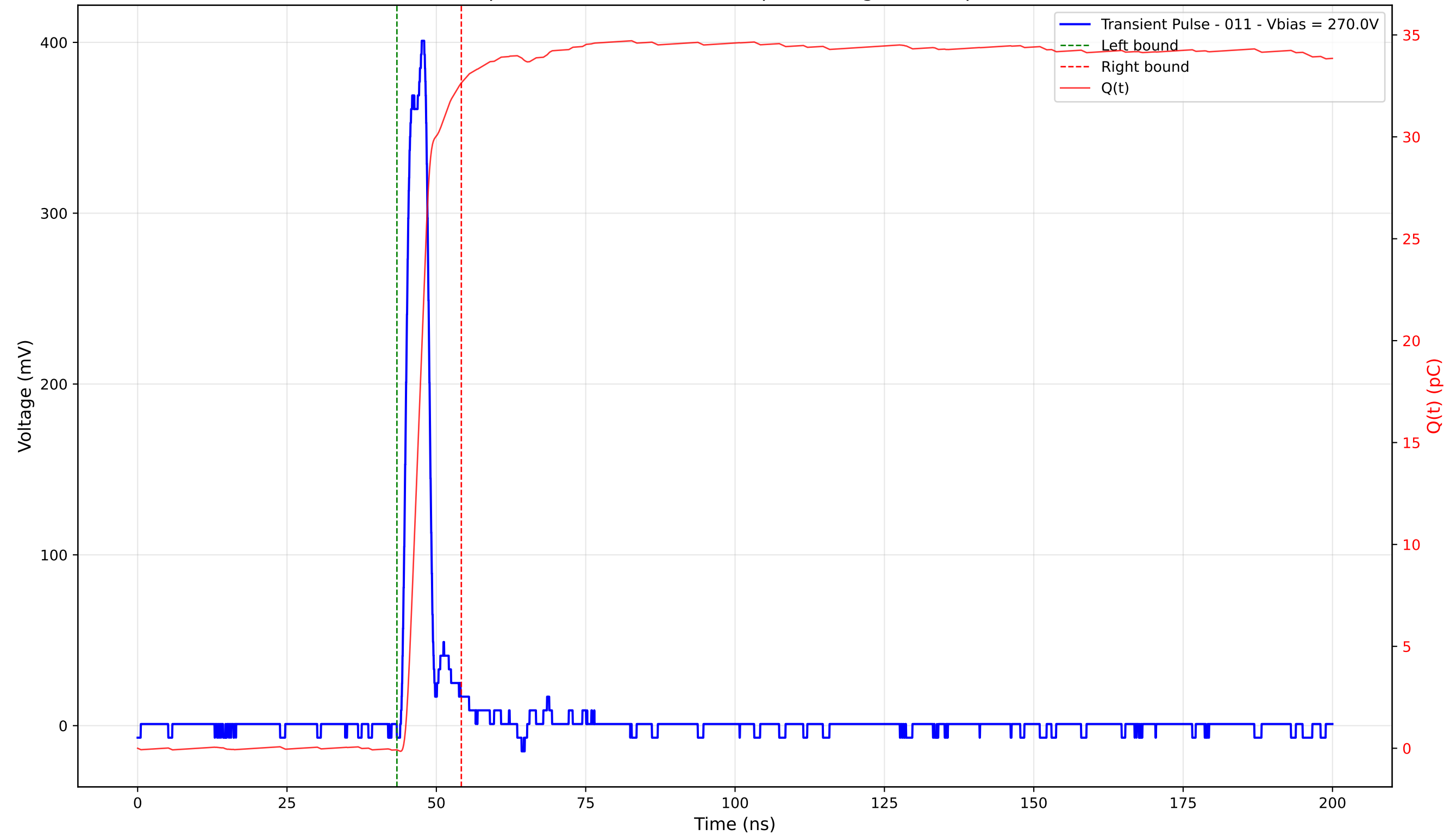
Transient Pulse - Sample: 4003 - Position: 325.0 \mu\text{m} - Charge: 32.72 pC - Rise Time: 1.42 ns
