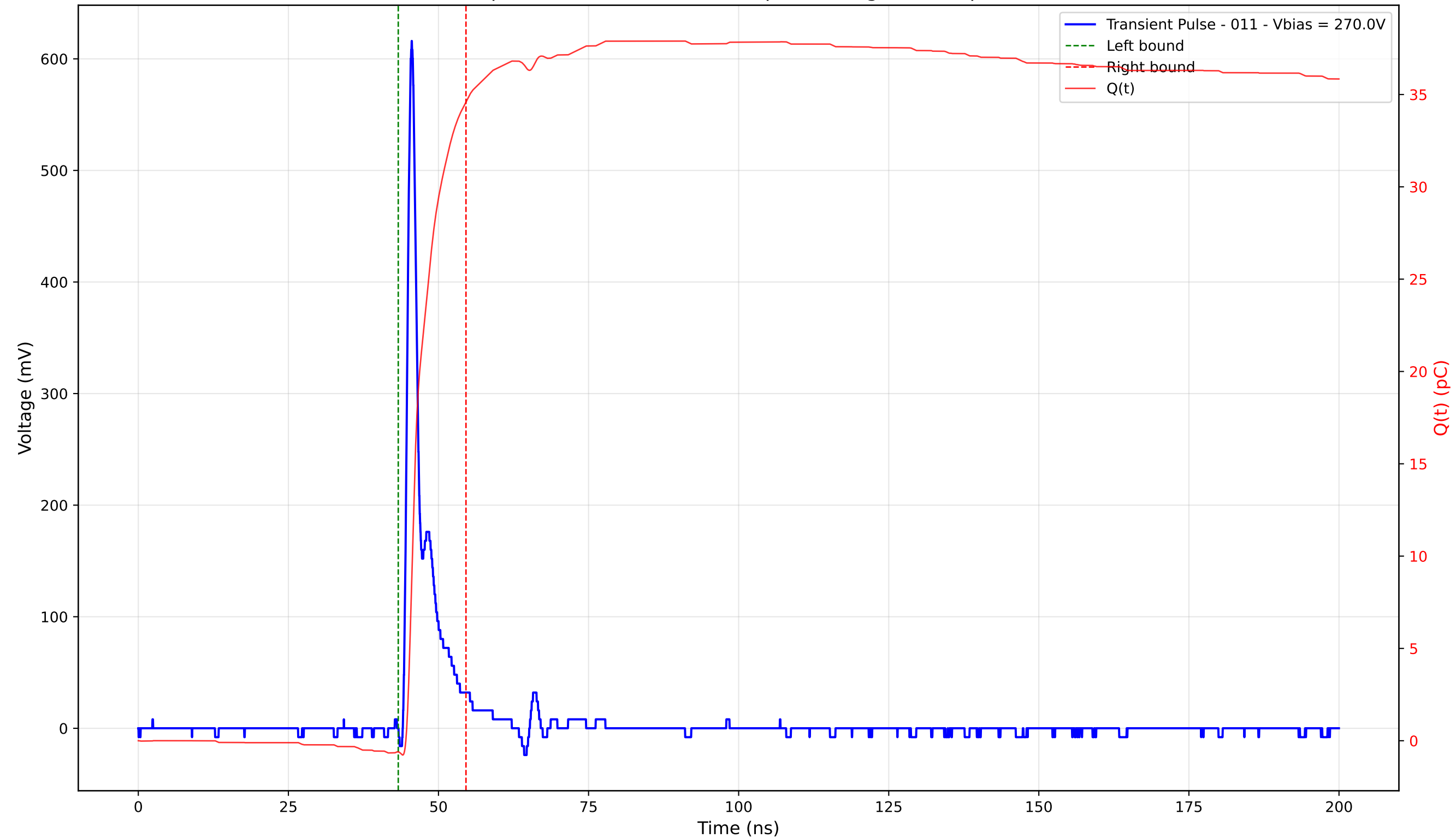
Transient Pulse - Sample: 4003 - Position: 155.0 \mu\text{m} - Charge: 35.20 pC - Rise Time: 0.93 ns
