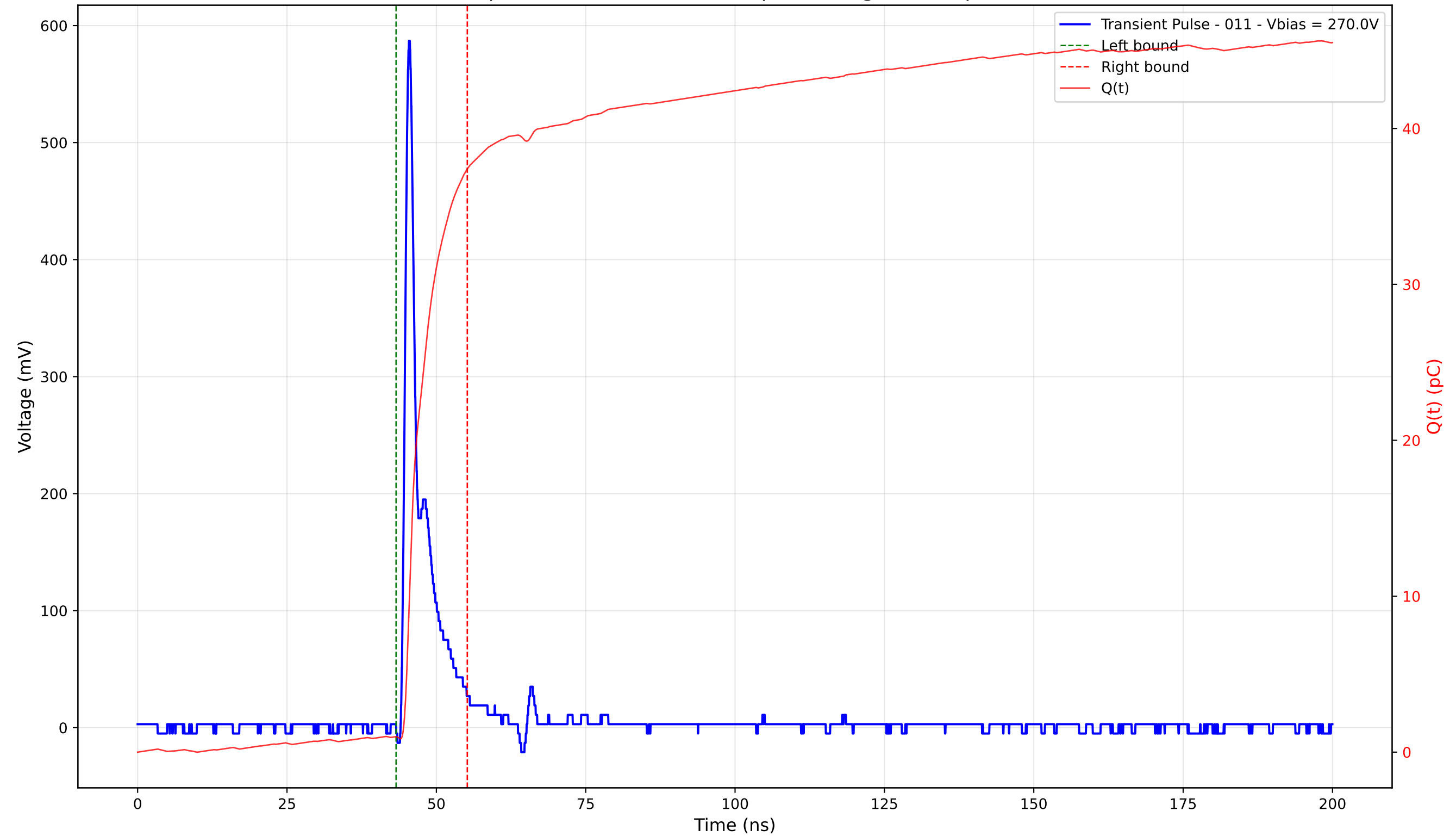
Transient Pulse - Sample: 4003 - Position: 130.0 \mu\text{m} - Charge: 36.41 pC - Rise Time: 0.89 ns
