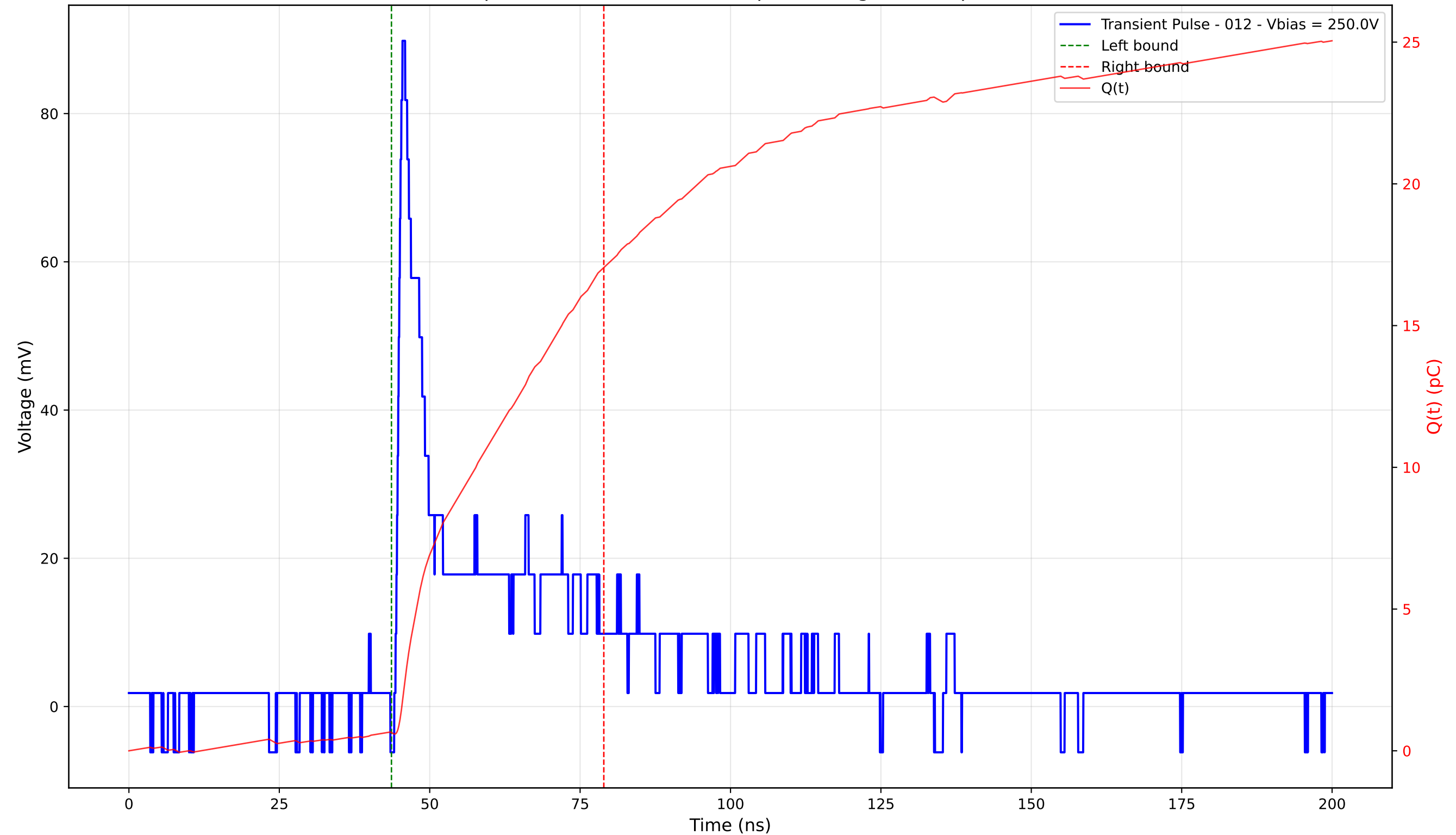
Transient Pulse - Sample: 4003 - Position: 390.0 \mu\text{m} - Charge: 16.41 pC - Rise Time: 0.96 ns
