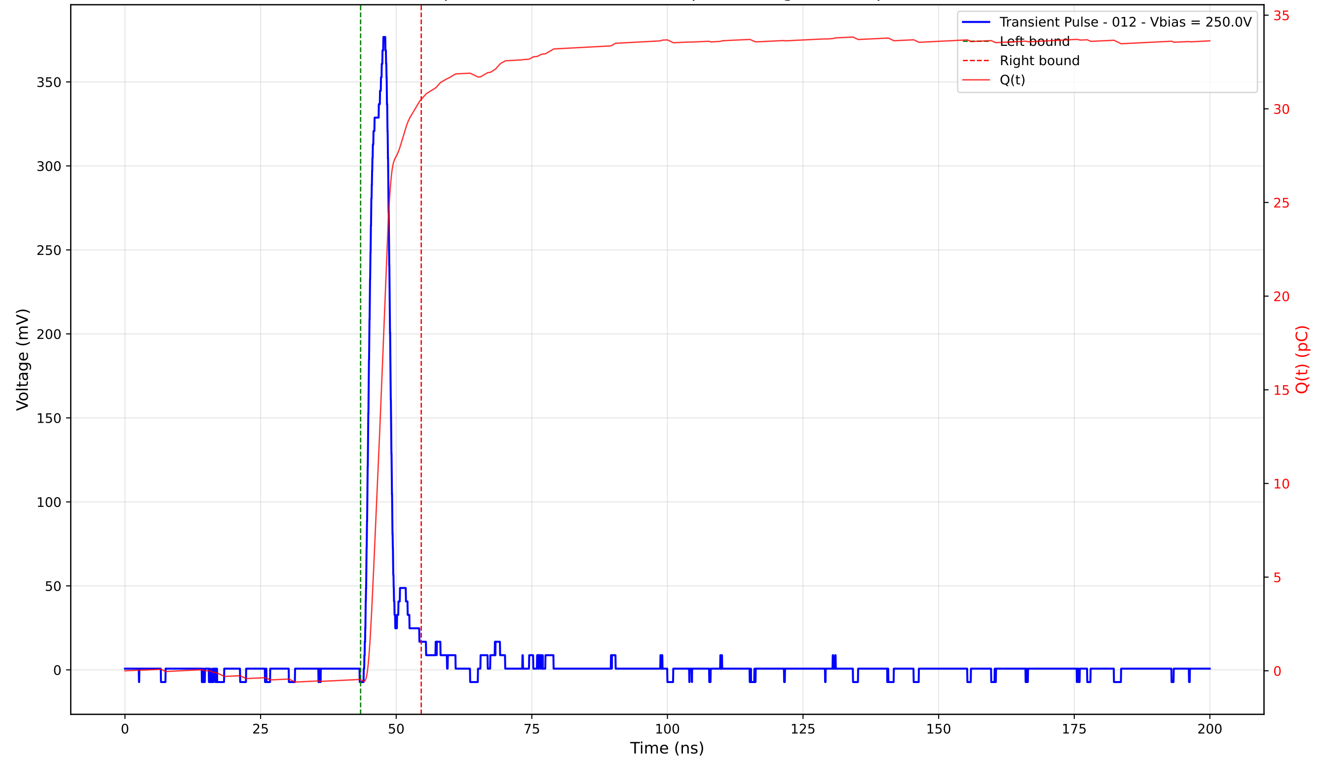
Transient Pulse - Sample: 4003 - Position: 320.0 \mu\text{m} - Charge: 30.99 pC - Rise Time: 2.63 ns
