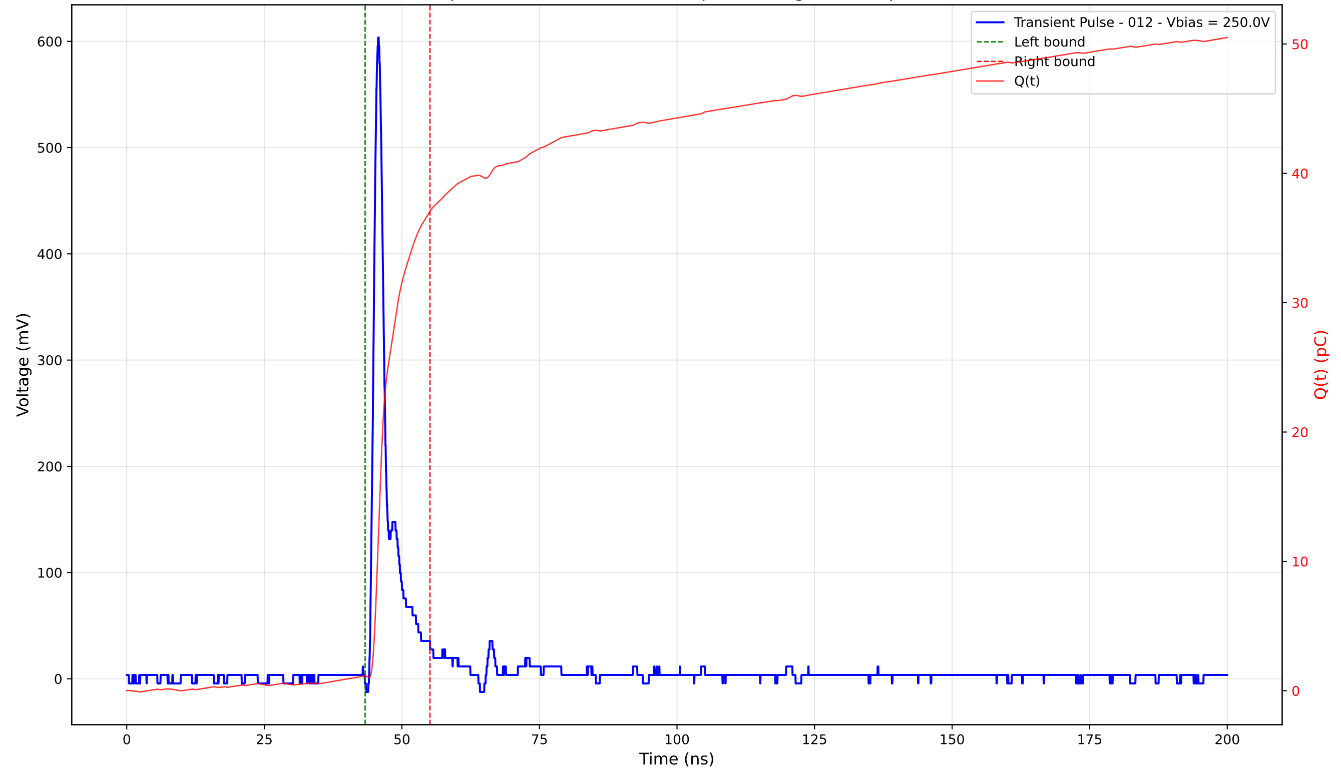
Transient Pulse - Sample: 4003 - Position: 195.0 \mu\text{m} - Charge: 35.94 pC - Rise Time: 1.05 ns
