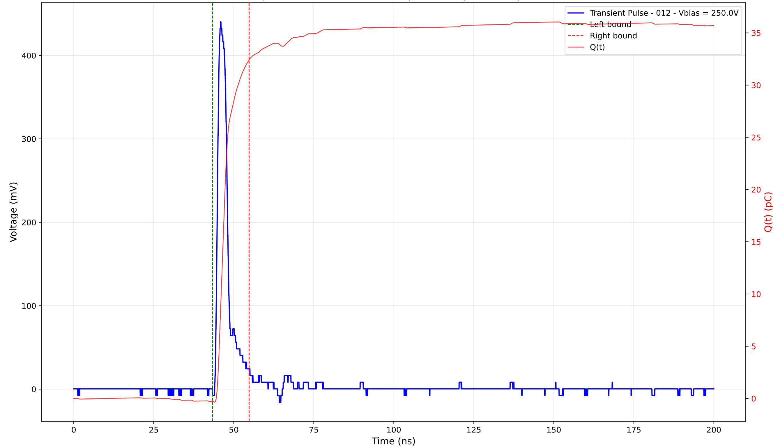
Transient Pulse - Sample: 4003 - Position: 275.0 \mu\text{m} - Charge: 32.68 pC - Rise Time: 1.11 ns
