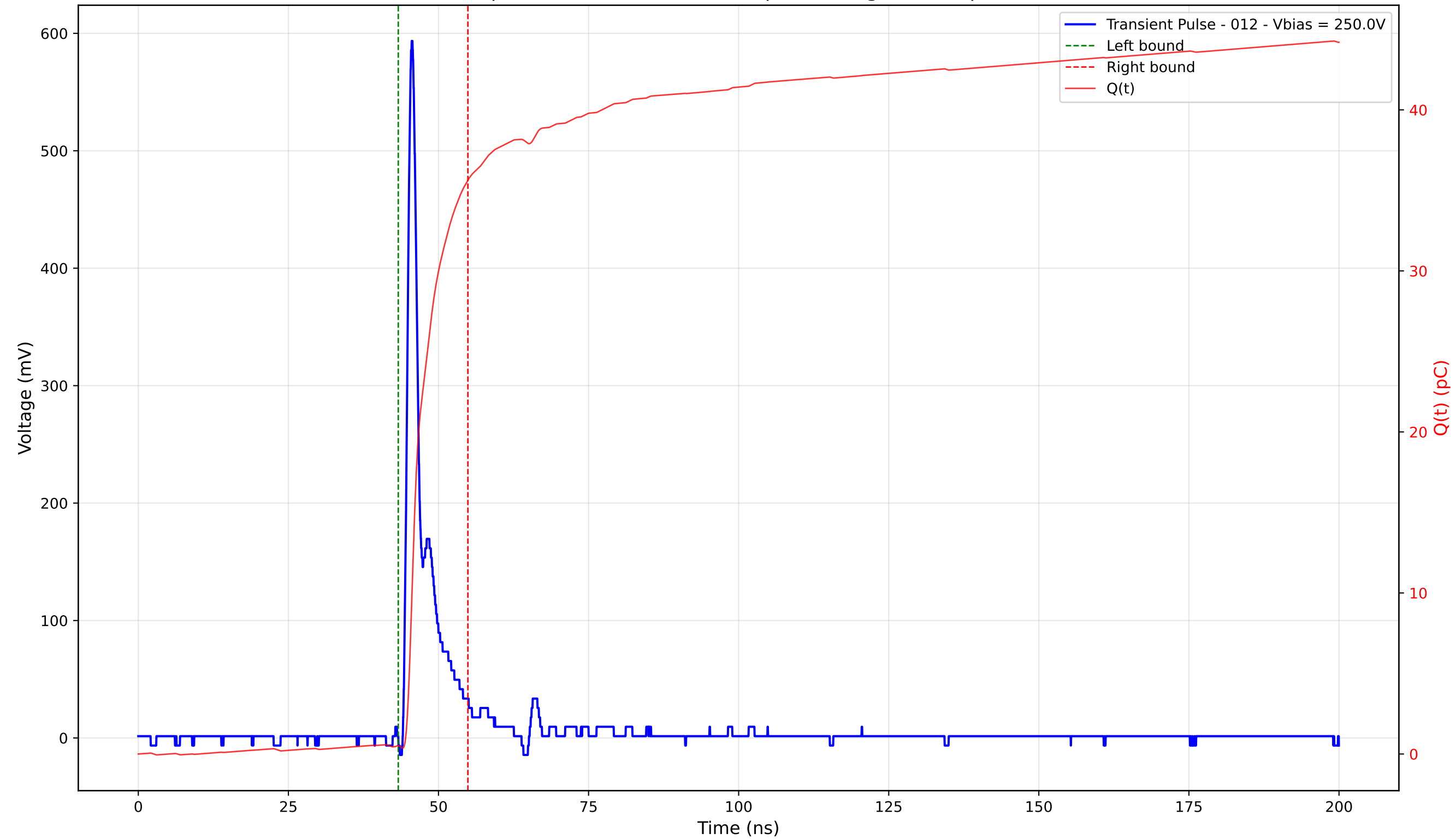
Transient Pulse - Sample: 4003 - Position: 165.0 \mu\text{m} - Charge: 35.12 pC - Rise Time: 0.97 ns
