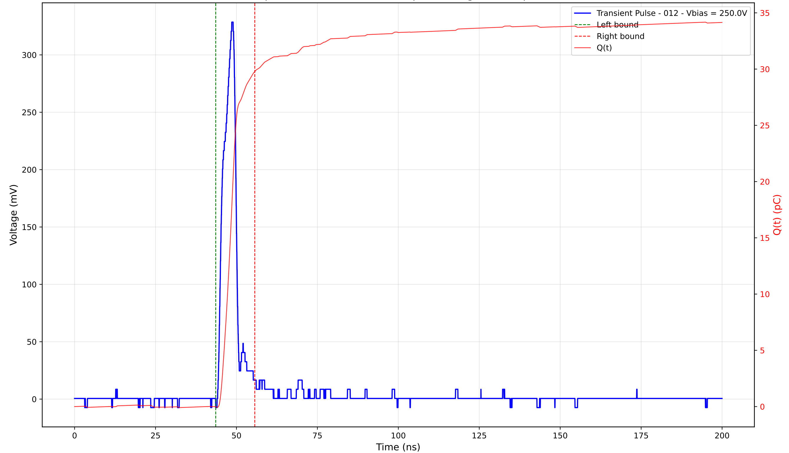
Transient Pulse - Sample: 4003 - Position: 350.0 \mu\text{m} - Charge: 29.79 pC - Rise Time: 3.32 ns
