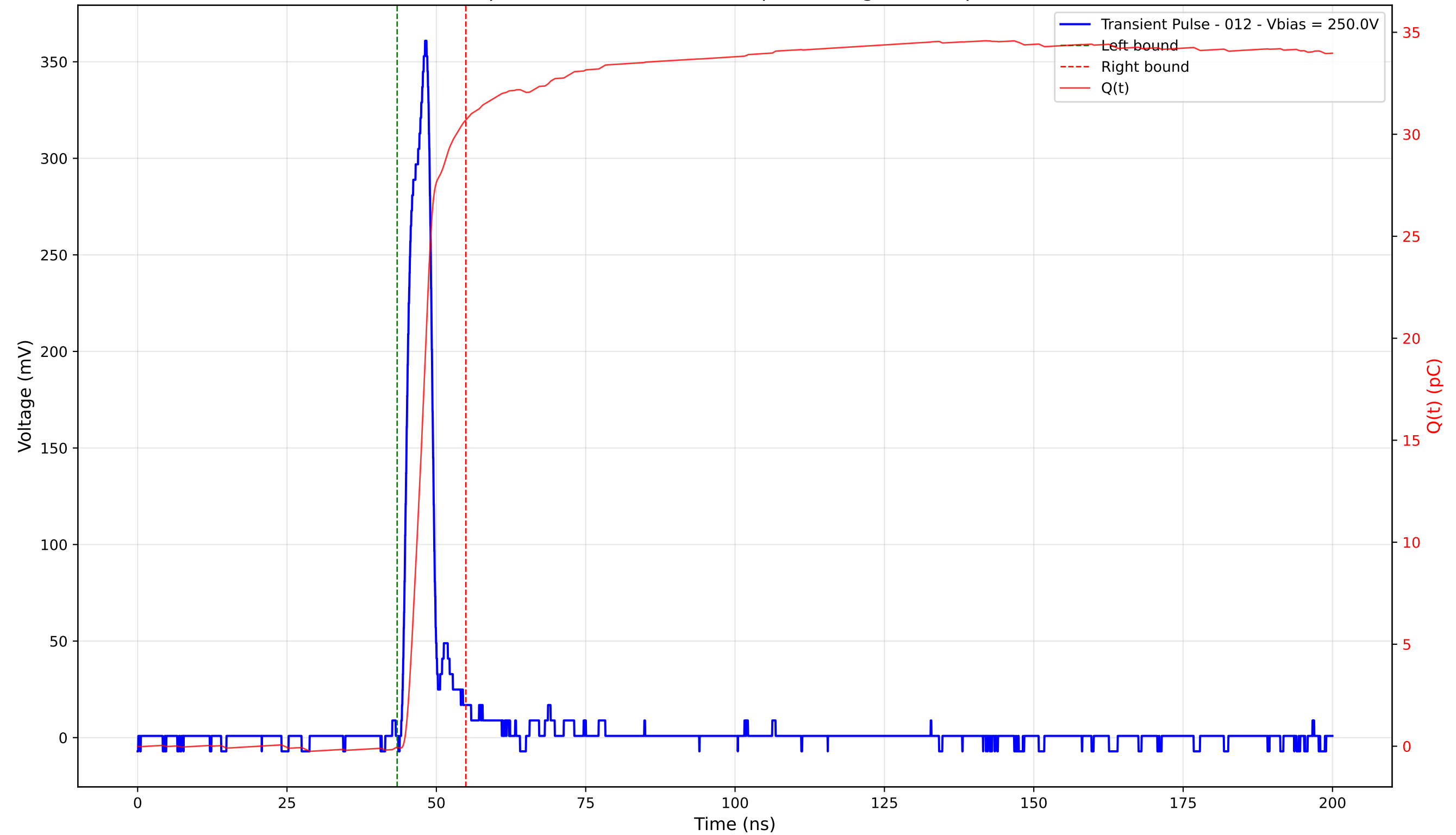
Transient Pulse - Sample: 4003 - Position: 335.0 \mu\text{m} - Charge: 30.77 pC - Rise Time: 3.03 ns
