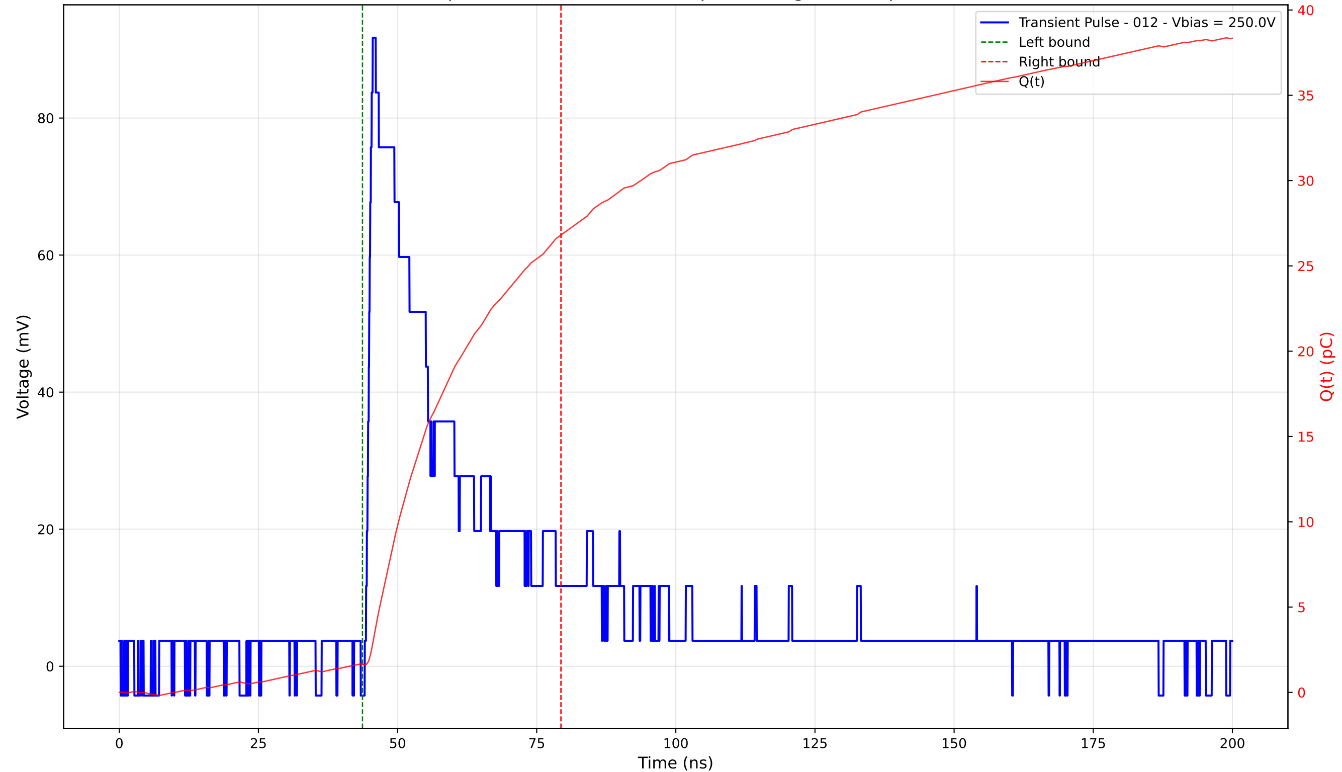
Transient Pulse - Sample: 4003 - Position: 380.0 \mu\text{m} - Charge: 25.16 pC - Rise Time: 1.01 ns
