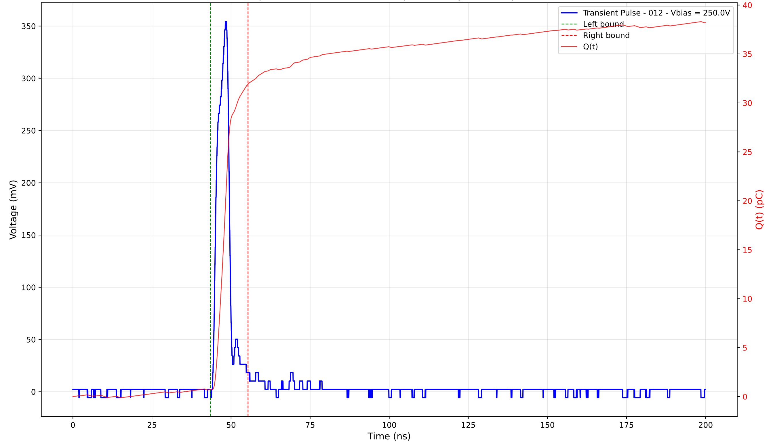
Transient Pulse - Sample: 4003 - Position: 340.0 \mu\text{m} - Charge: 31.20 pC - Rise Time: 3.10 ns
