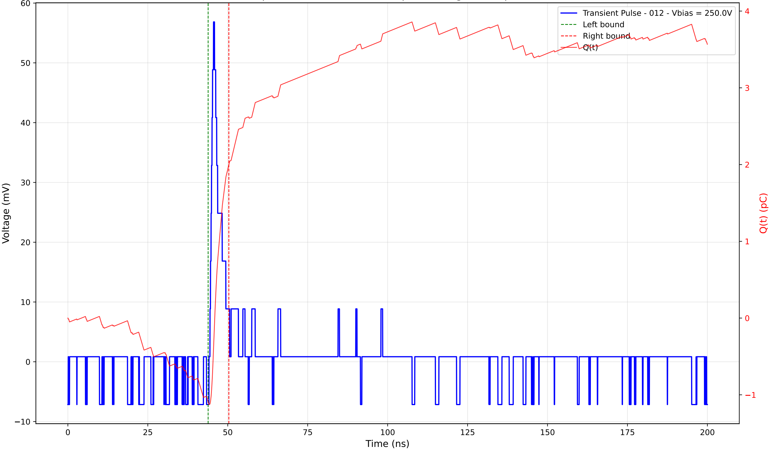
Transient Pulse - Sample: 4003 - Position: 50.0 \mu\text{m} - Charge: 3.09 pC - Rise Time: 1.11 ns
