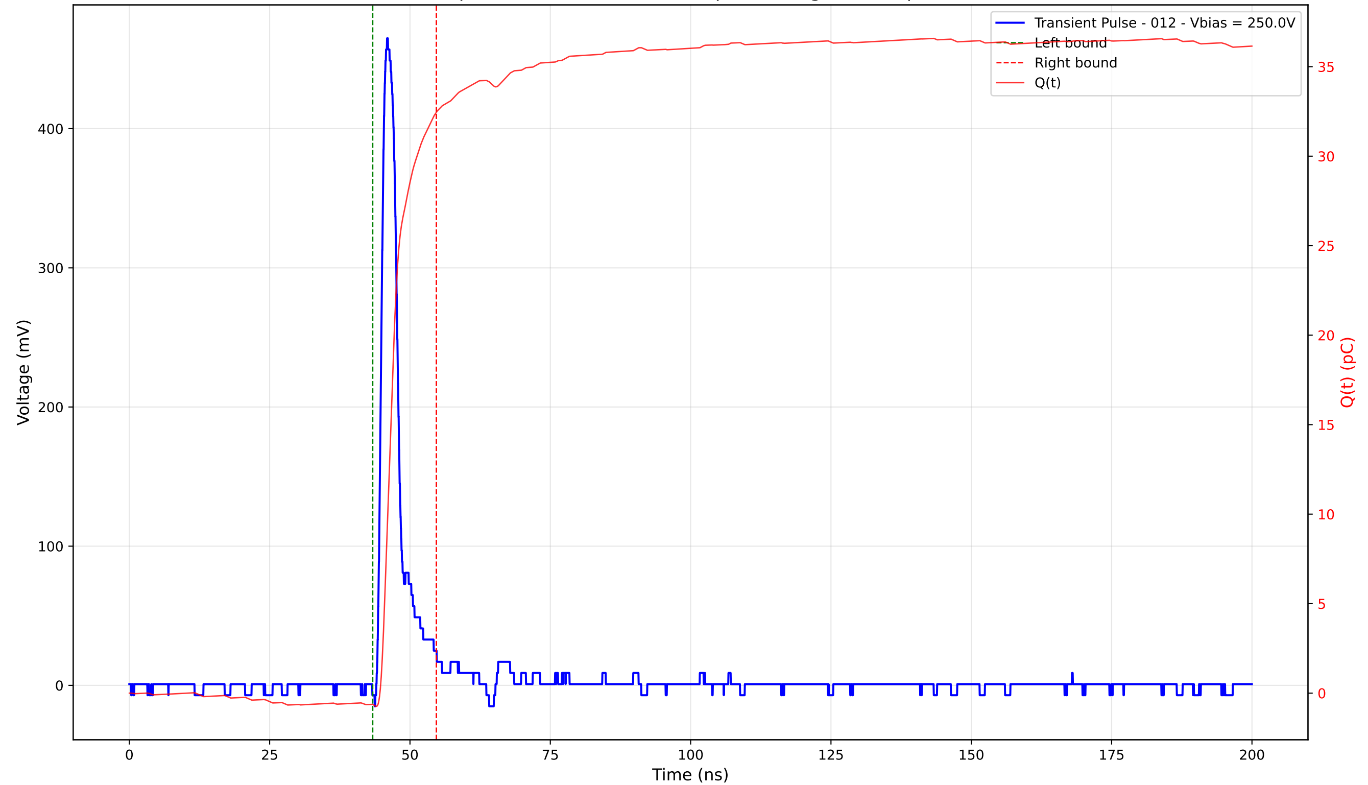
Transient Pulse - Sample: 4003 - Position: 265.0 \mu\text{m} - Charge: 33.10 pC - Rise Time: 1.15 ns
