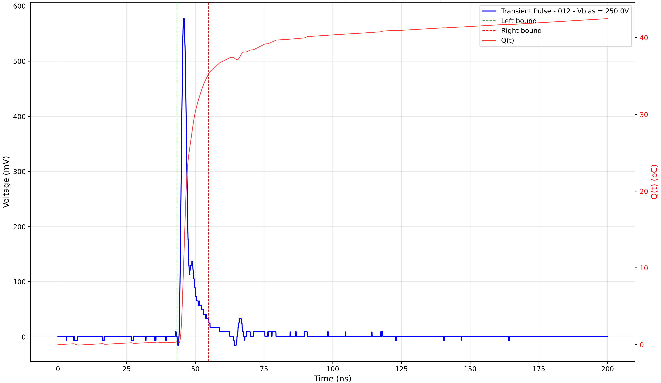
Transient Pulse - Sample: 4003 - Position: 210.0 \mu\text{m} - Charge: 34.82 pC - Rise Time: 1.05 ns
