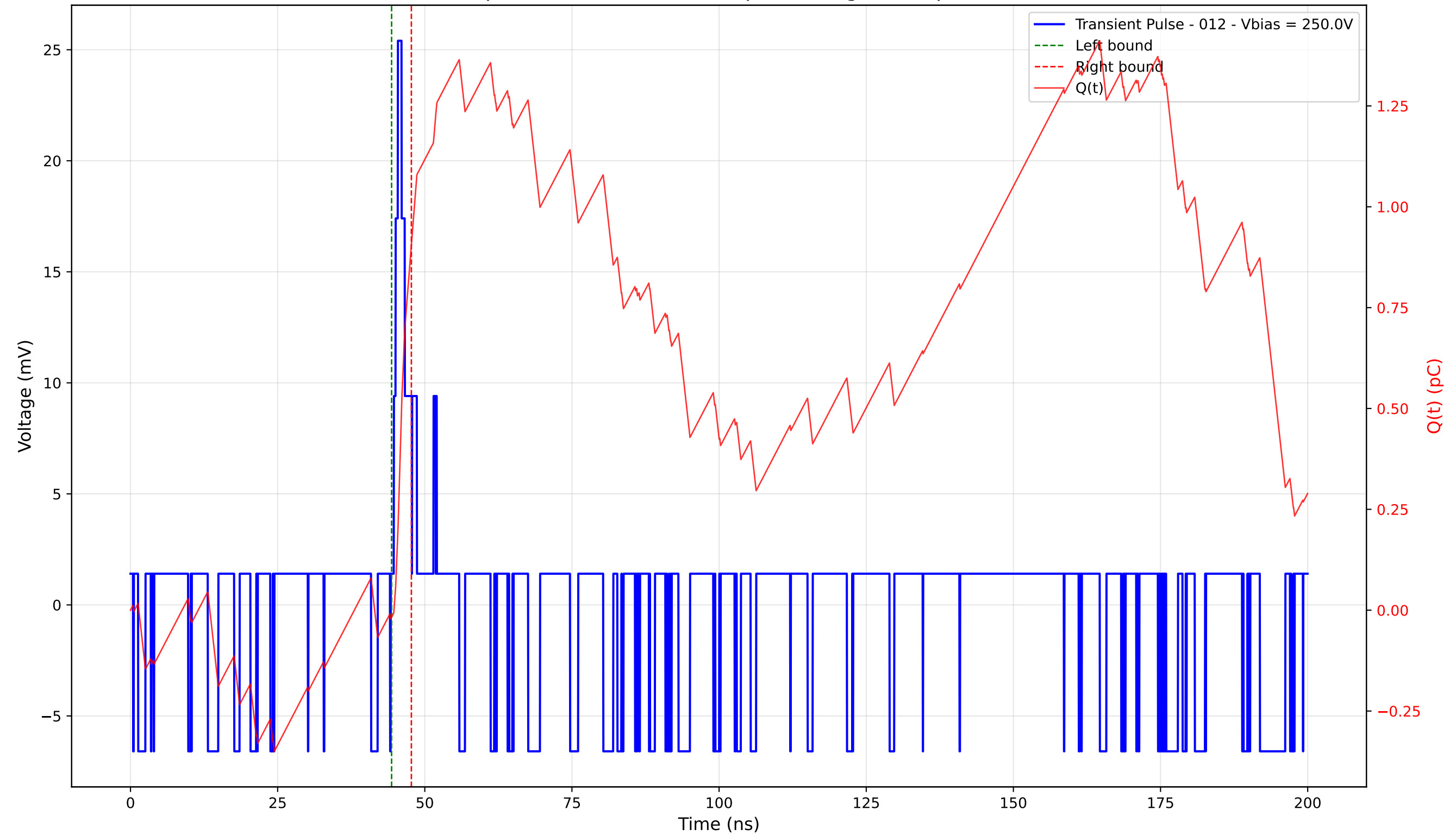
Transient Pulse - Sample: 4003 - Position: 15.0 \mu\text{m} - Charge: 0.92 pC - Rise Time: 0.70 ns
