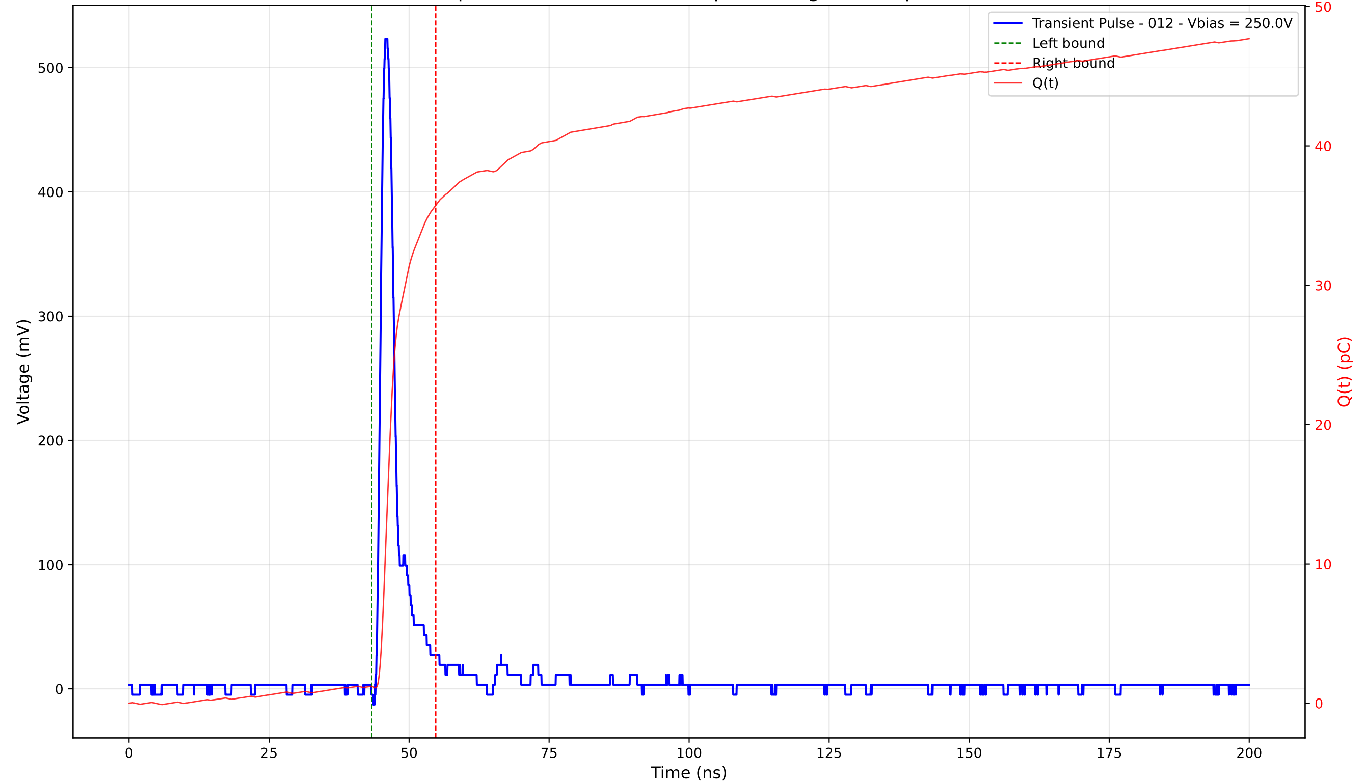
Transient Pulse - Sample: 4003 - Position: 240.0 \mu\text{m} - Charge: 34.53 pC - Rise Time: 1.12 ns
