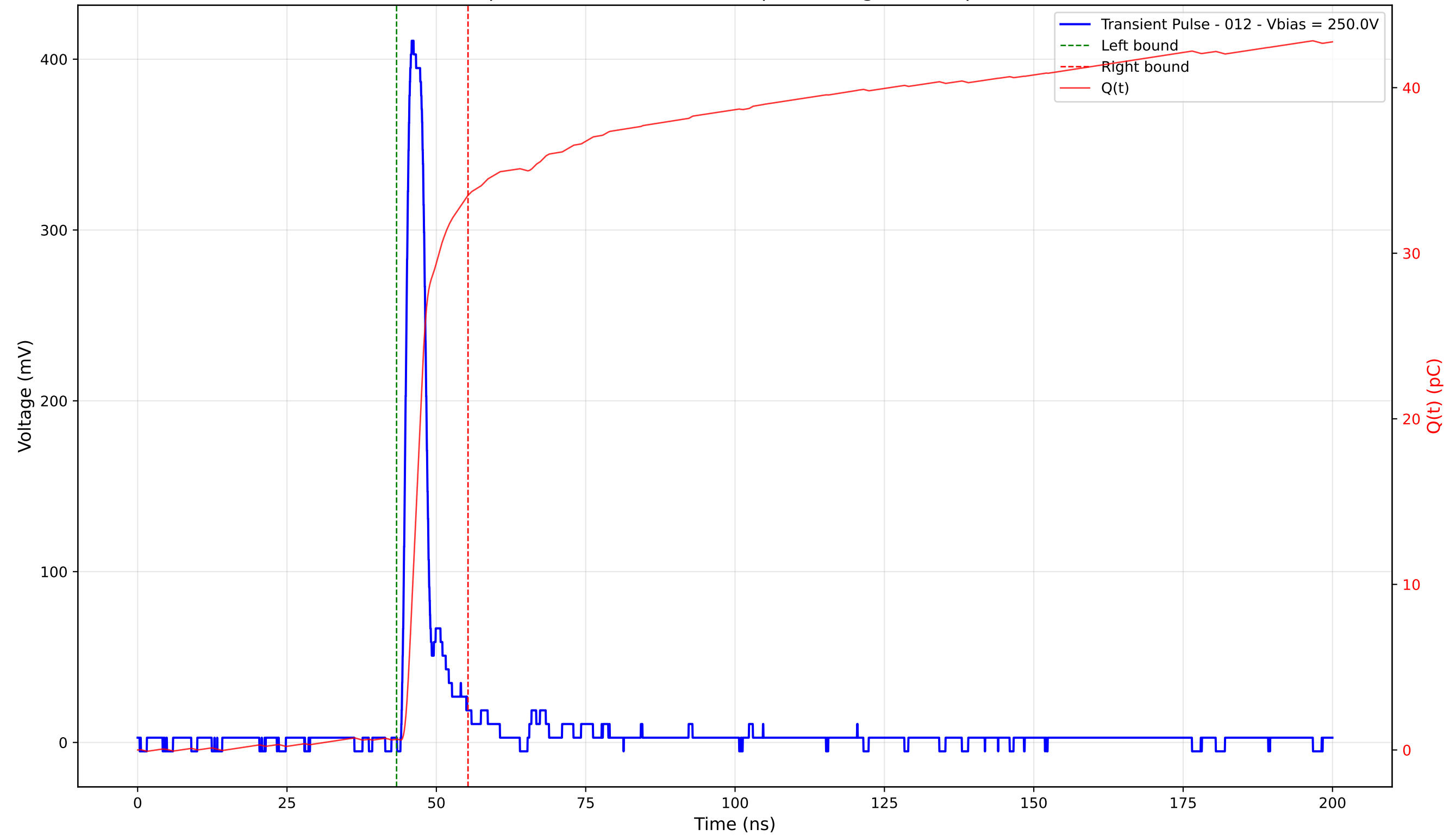
Transient Pulse - Sample: 4003 - Position: 290.0 \mu\text{m} - Charge: 32.84 pC - Rise Time: 1.14 ns
