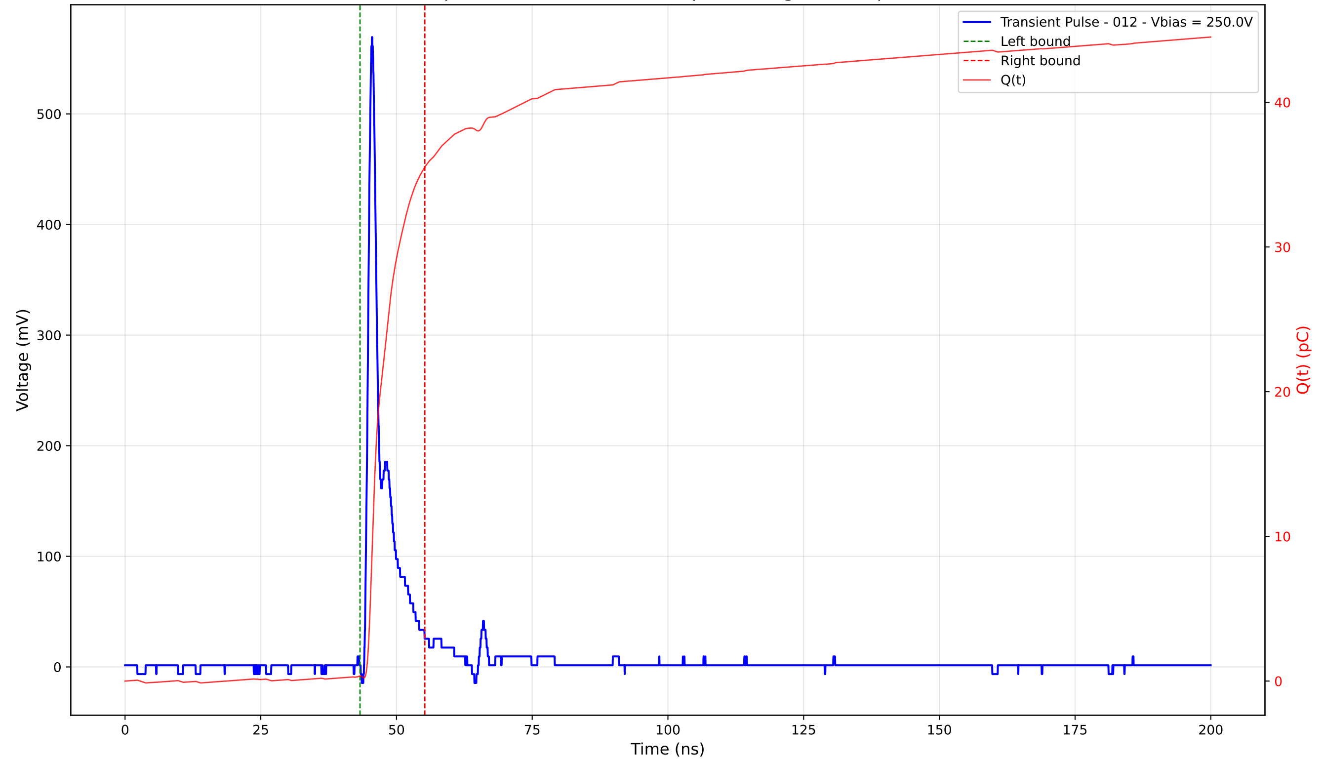
Transient Pulse - Sample: 4003 - Position: 140.0 \mu\text{m} - Charge: 35.19 pC - Rise Time: 0.92 ns
