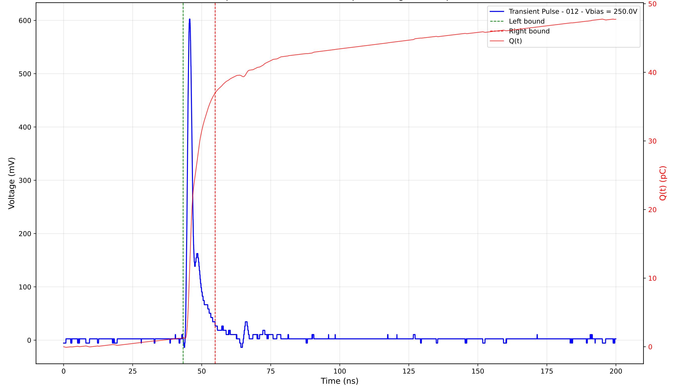
Transient Pulse - Sample: 4003 - Position: 180.0 \mu\text{m} - Charge: 35.70 pC - Rise Time: 1.00 ns
