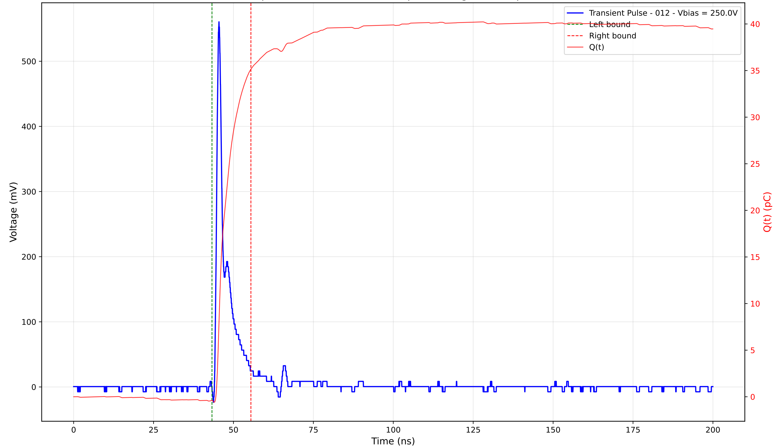
Transient Pulse - Sample: 4003 - Position: 130.0 \mu\text{m} - Charge: 35.53 pC - Rise Time: 0.90 ns
