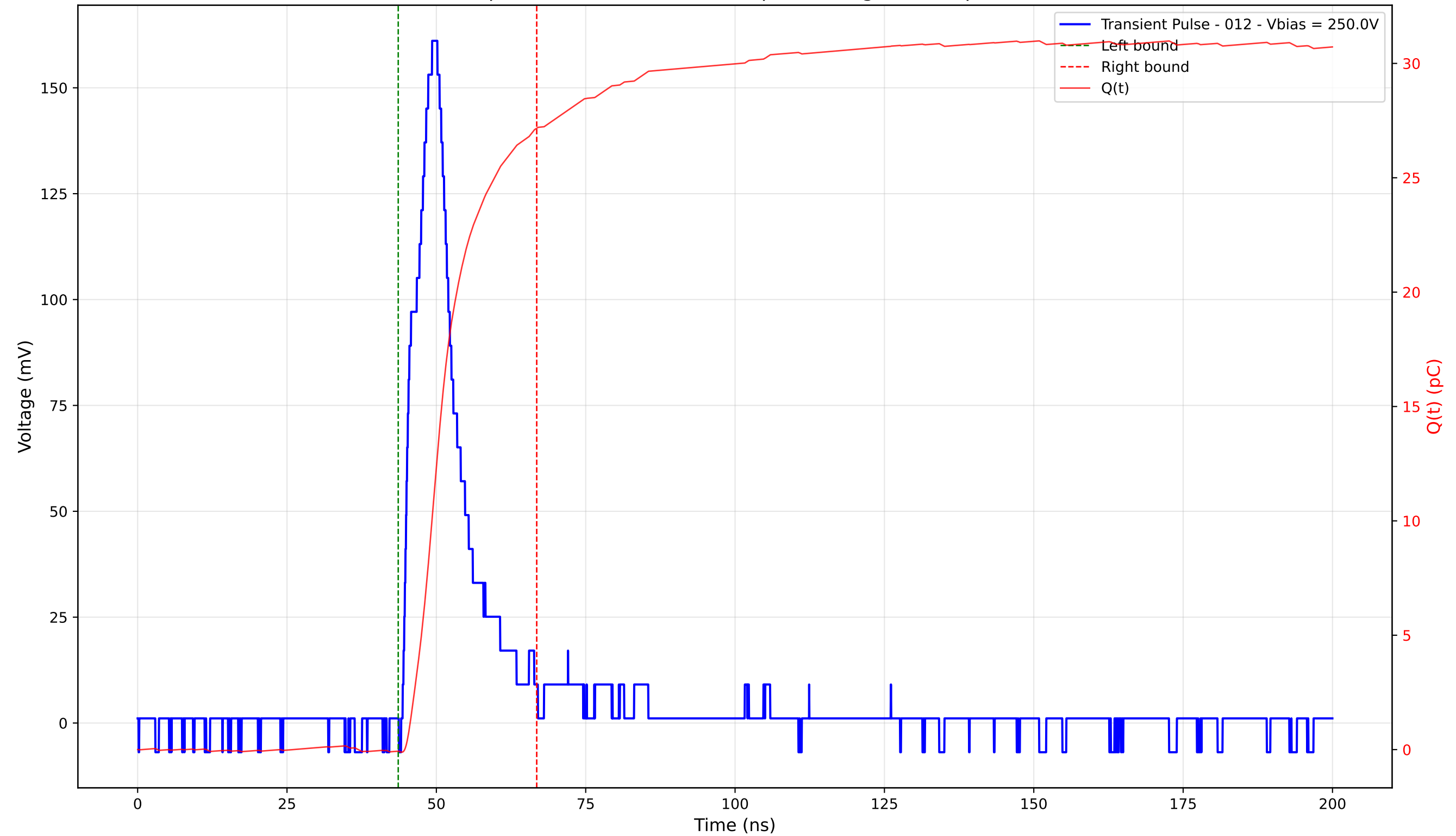
Transient Pulse - Sample: 4003 - Position: 370.0 \mu\text{m} - Charge: 27.24 pC - Rise Time: 3.80 ns
