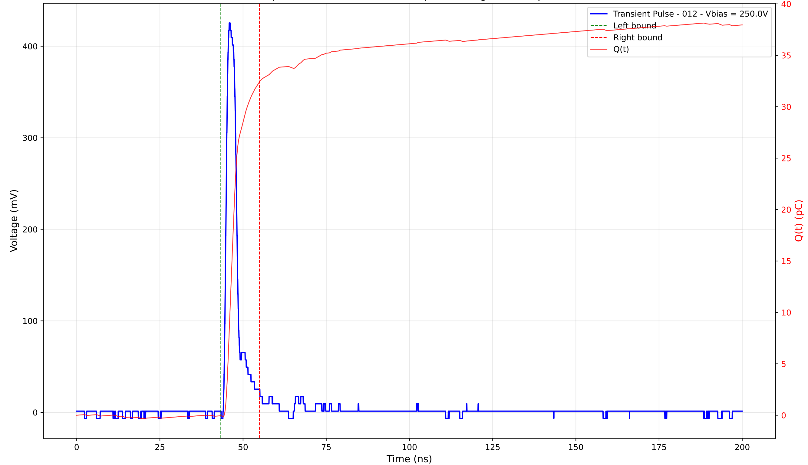
Transient Pulse - Sample: 4003 - Position: 280.0 \mu\text{m} - Charge: 32.47 pC - Rise Time: 1.12 ns
