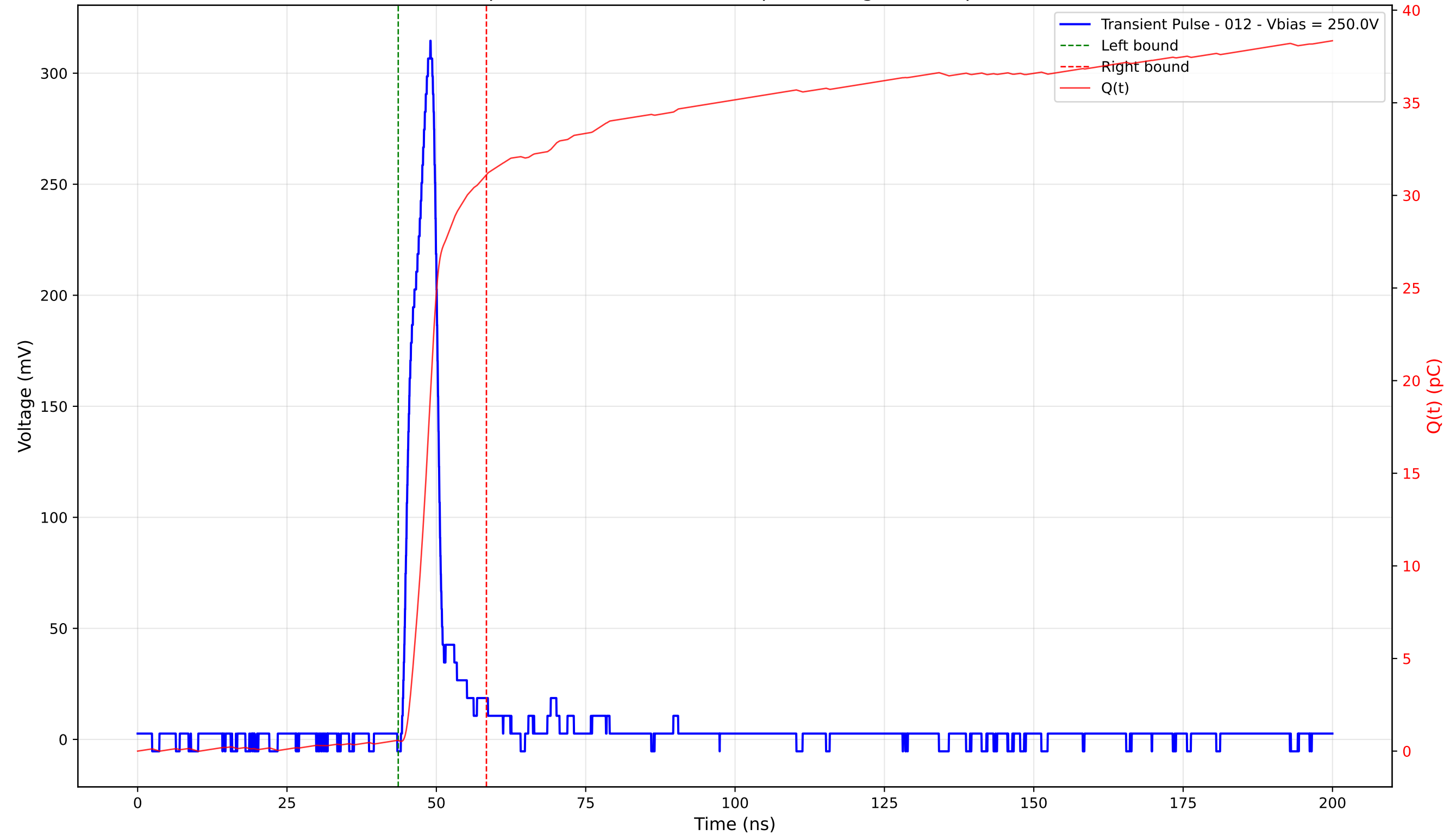
Transient Pulse - Sample: 4003 - Position: 355.0 \mu\text{m} - Charge: 30.55 pC - Rise Time: 3.69 ns
