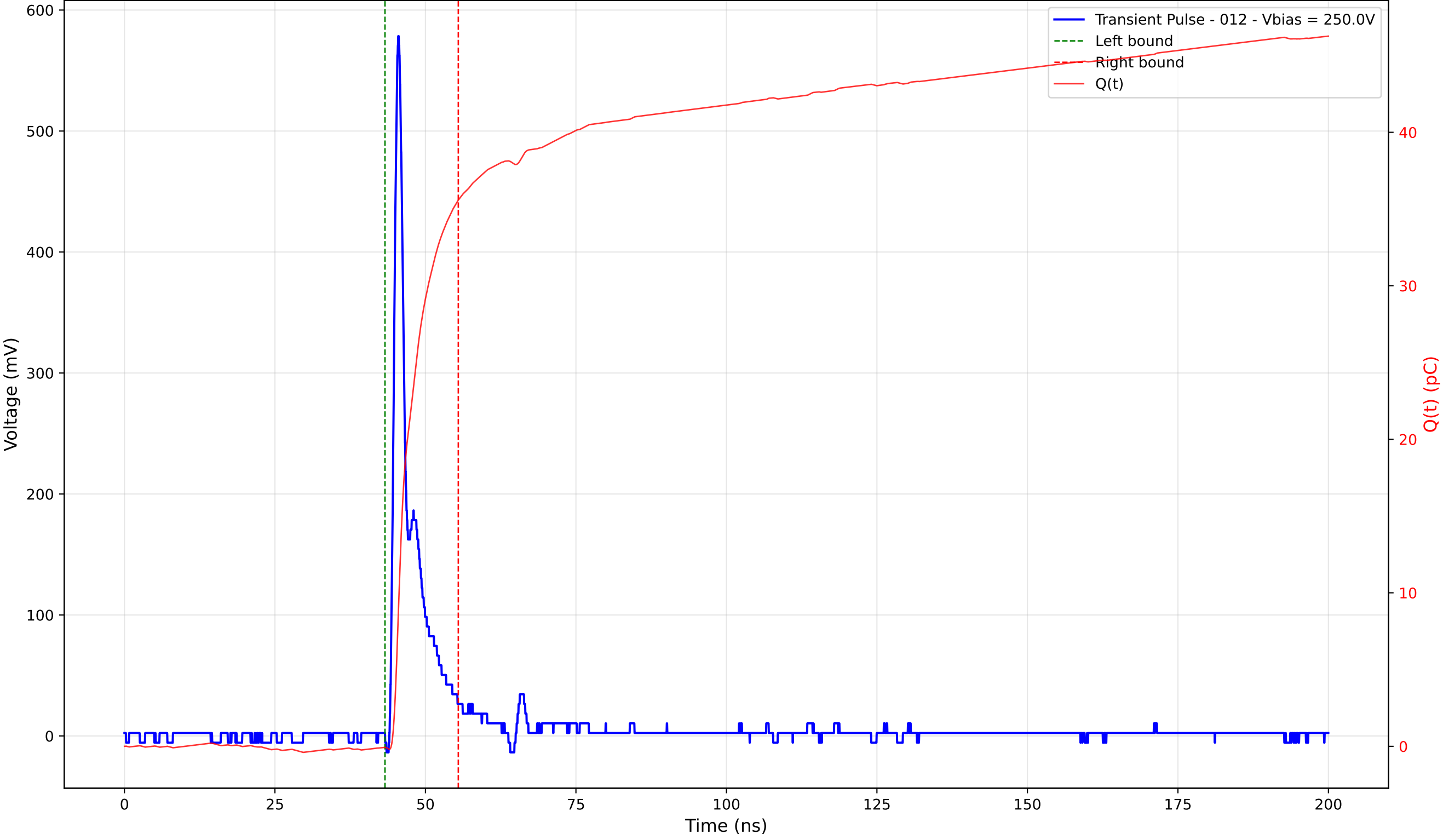
Transient Pulse - Sample: 4003 - Position: 145.0 \mu\text{m} - Charge: 35.65 pC - Rise Time: 0.94 ns
