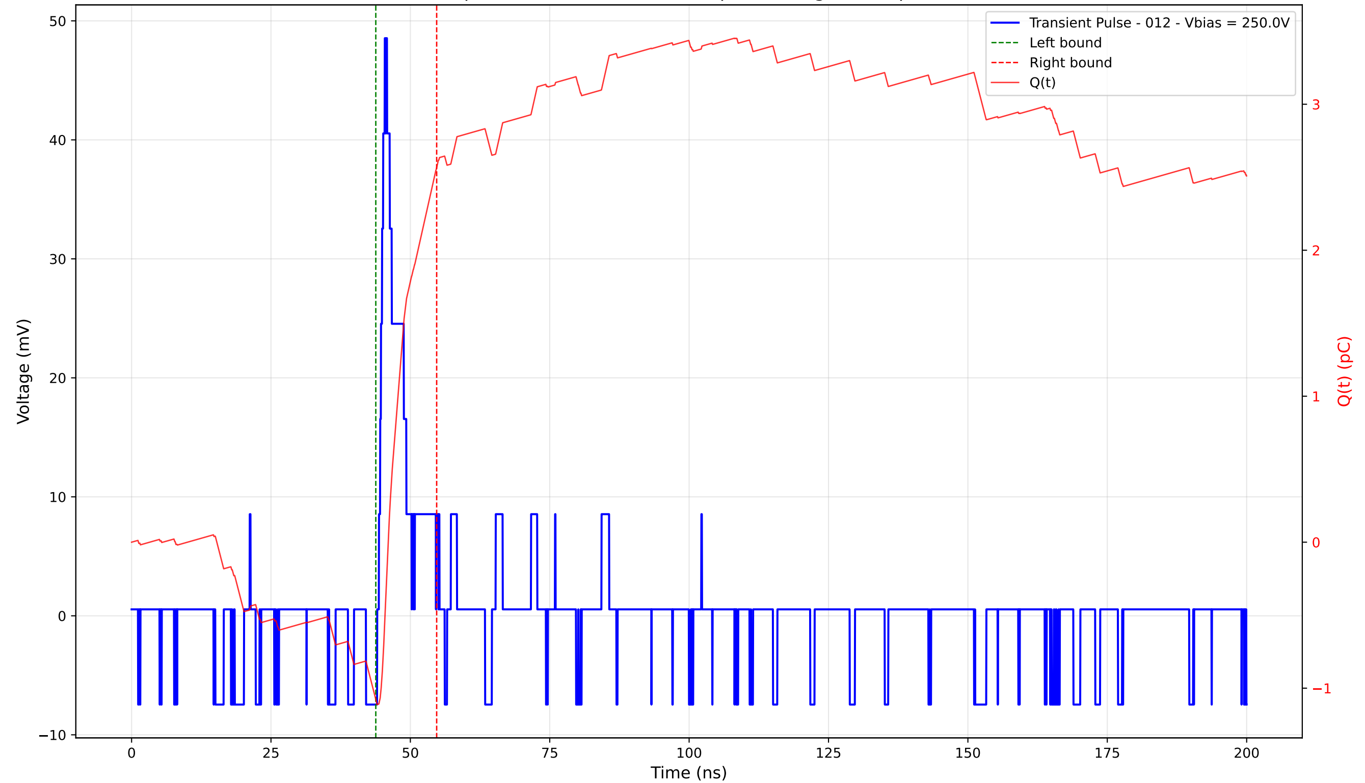
Transient Pulse - Sample: 4003 - Position: 410.0 \mu\text{m} - Charge: 3.64 pC - Rise Time: 1.05 ns
