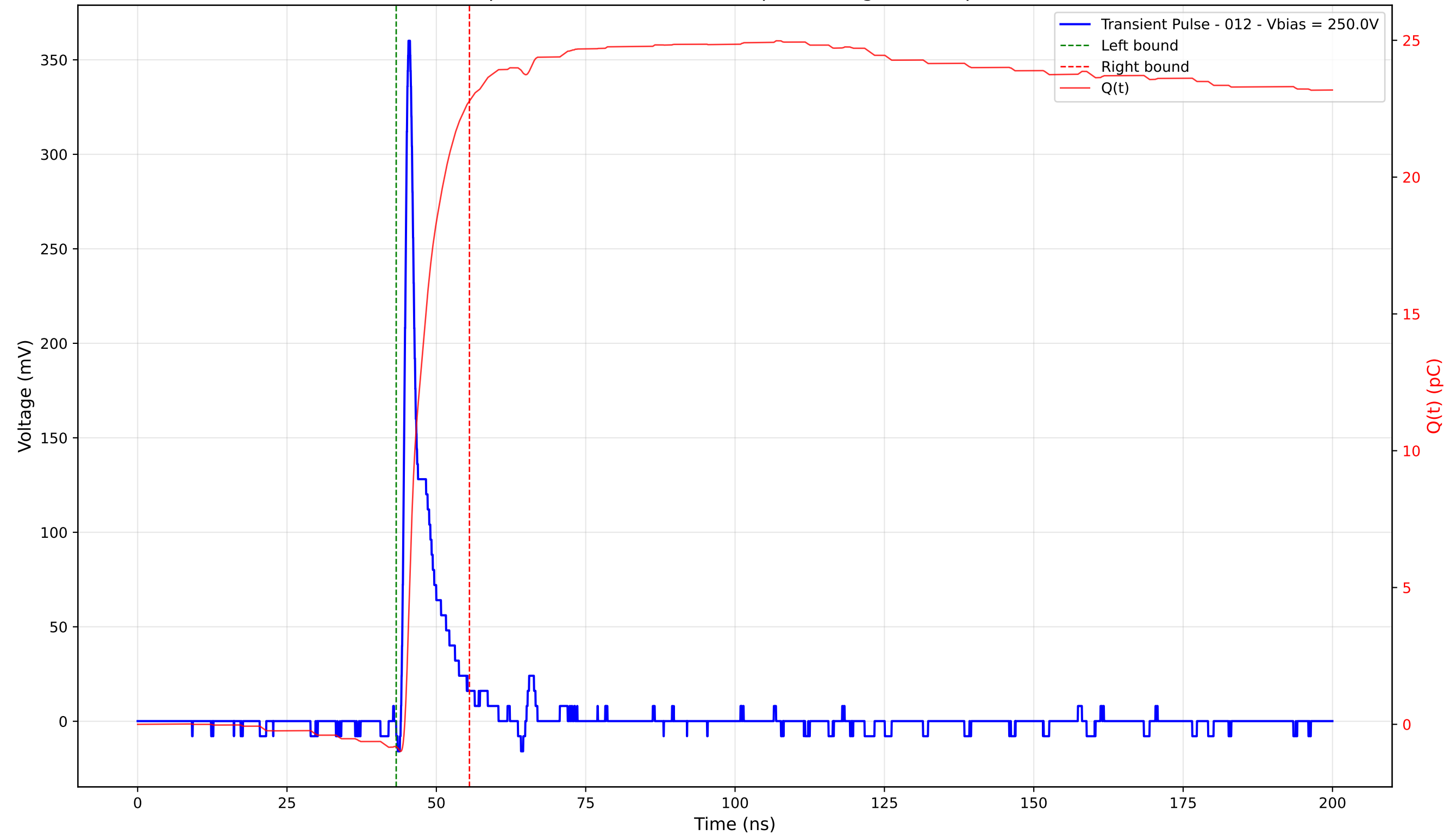
Transient Pulse - Sample: 4003 - Position: 105.0 \mu\text{m} - Charge: 23.60 pC - Rise Time: 0.88 ns
