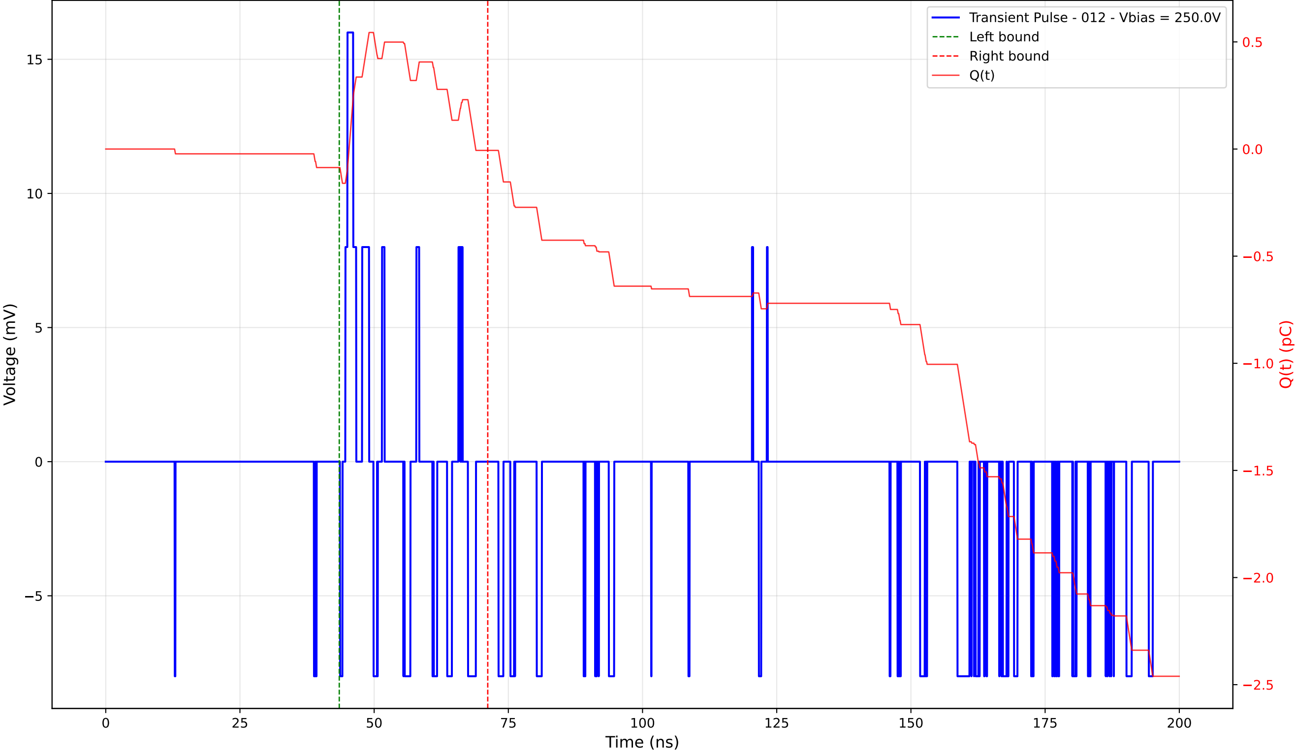
Transient Pulse - Sample: 4003 - Position: 70.0 \mu\text{m} - Charge: 0.08 pC - Rise Time: 0.40 ns
