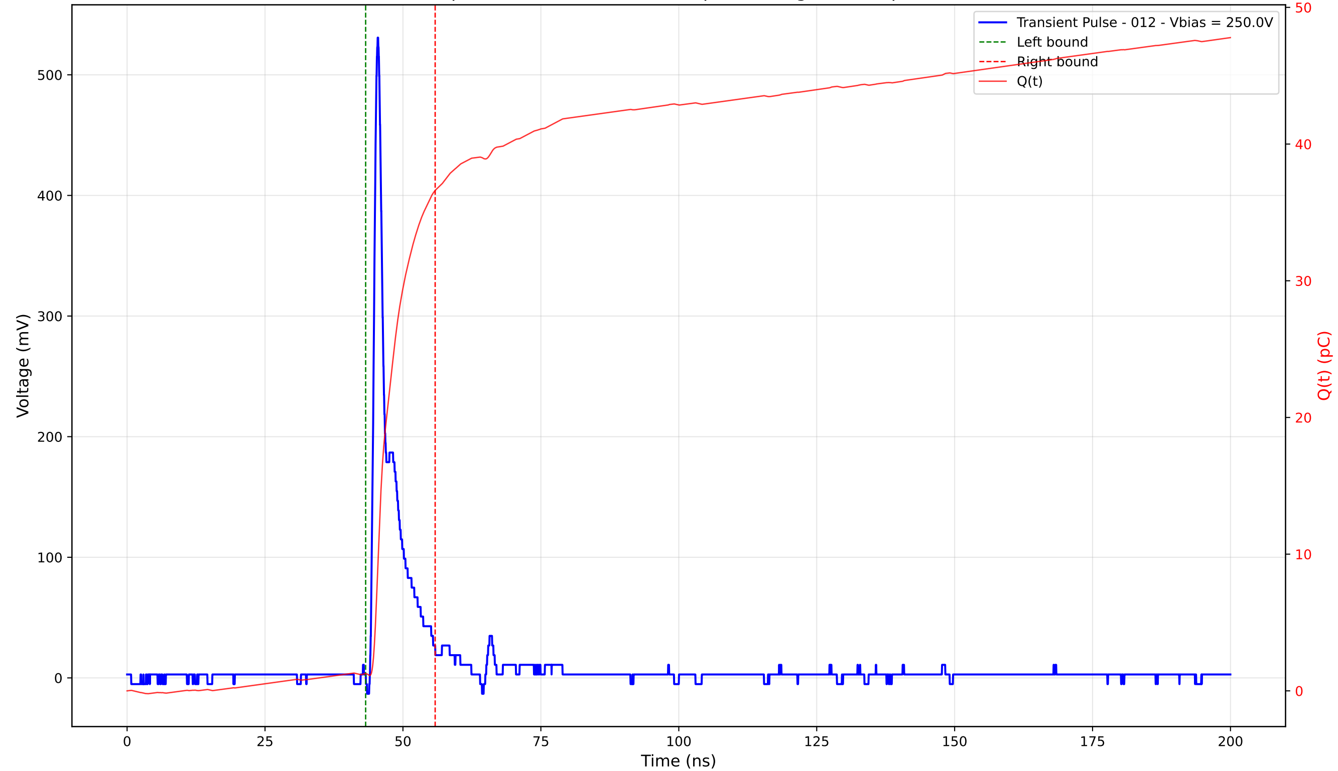
Transient Pulse - Sample: 4003 - Position: 120.0 \mu\text{m} - Charge: 35.35 pC - Rise Time: 0.92 ns
