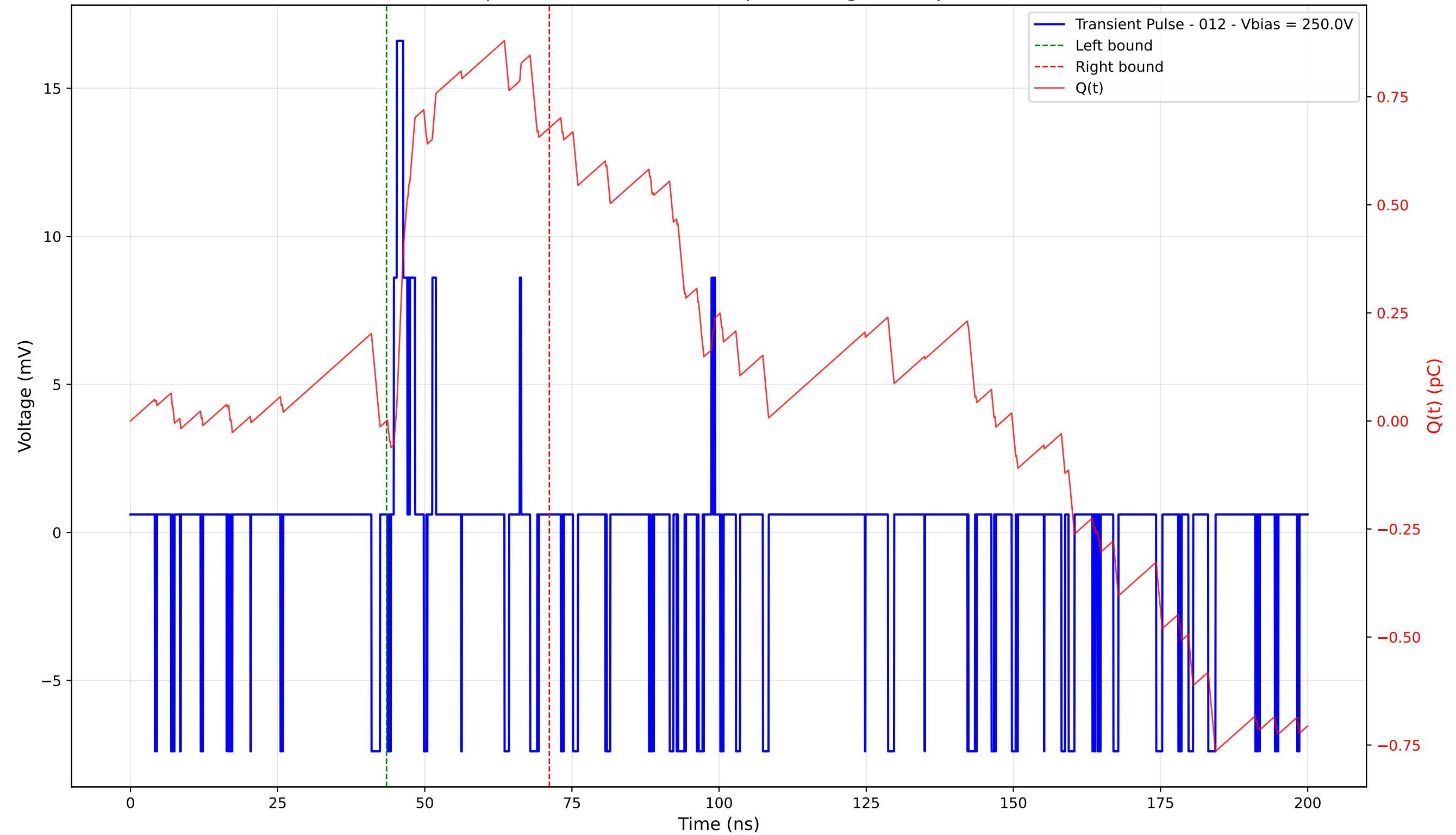
Transient Pulse - Sample: 4003 - Position: 10.0 \mu\text{m} - Charge: 0.68 pC - Rise Time: 0.52 ns
