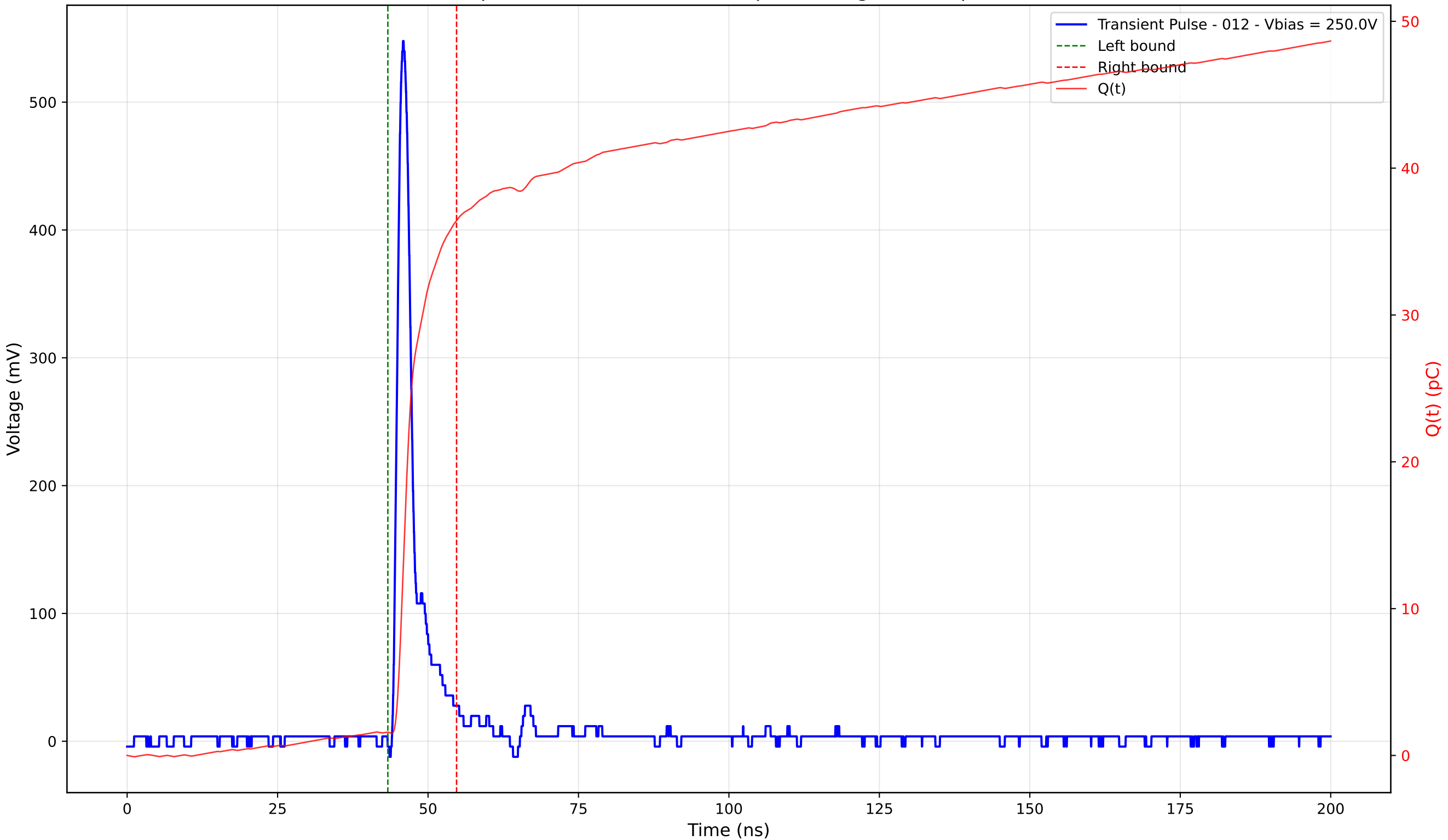
Transient Pulse - Sample: 4003 - Position: 230.0 \mu\text{m} - Charge: 34.85 pC - Rise Time: 1.15 ns
