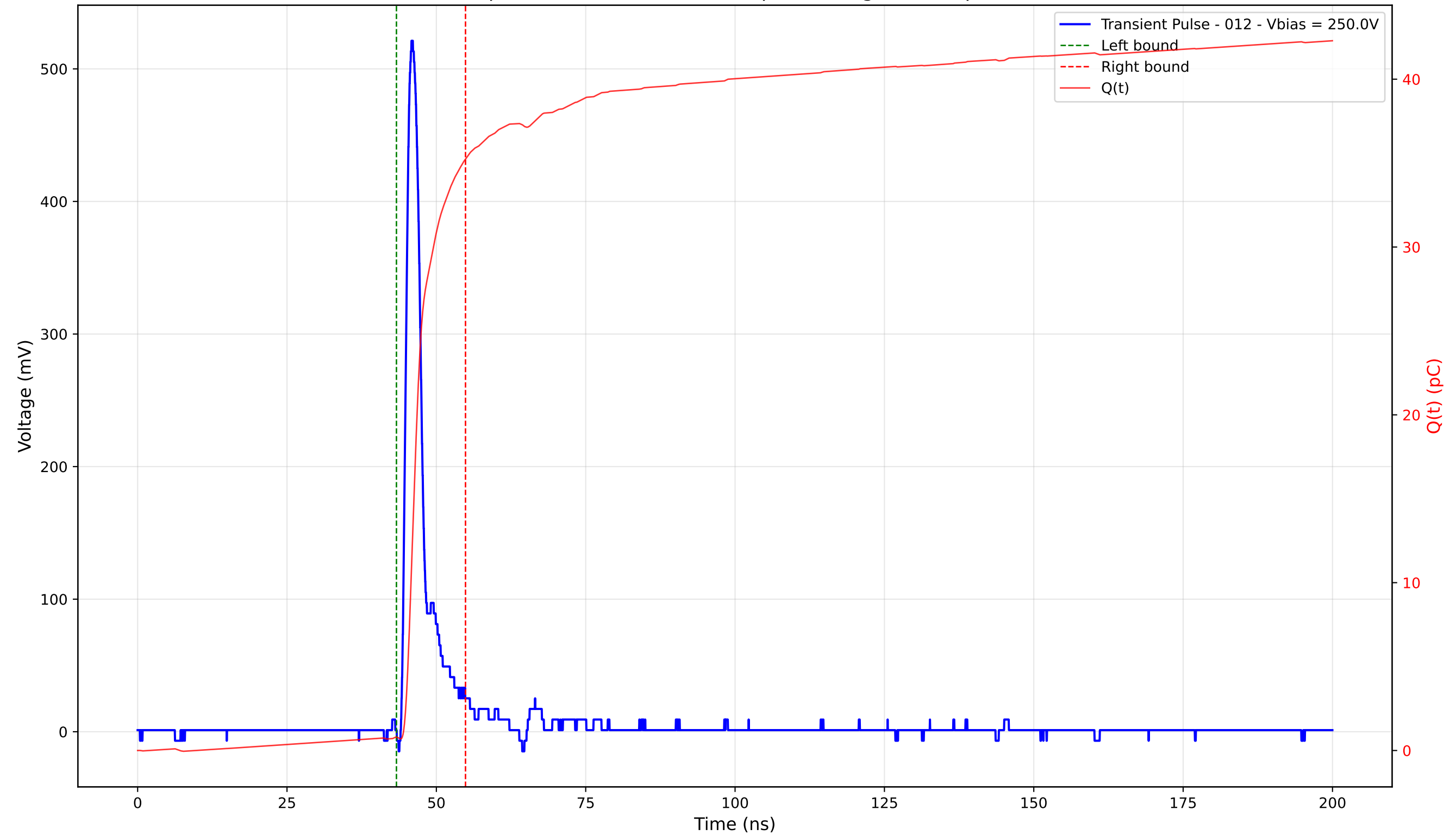
Transient Pulse - Sample: 4003 - Position: 245.0 \mu\text{m} - Charge: 34.45 pC - Rise Time: 1.13 ns
