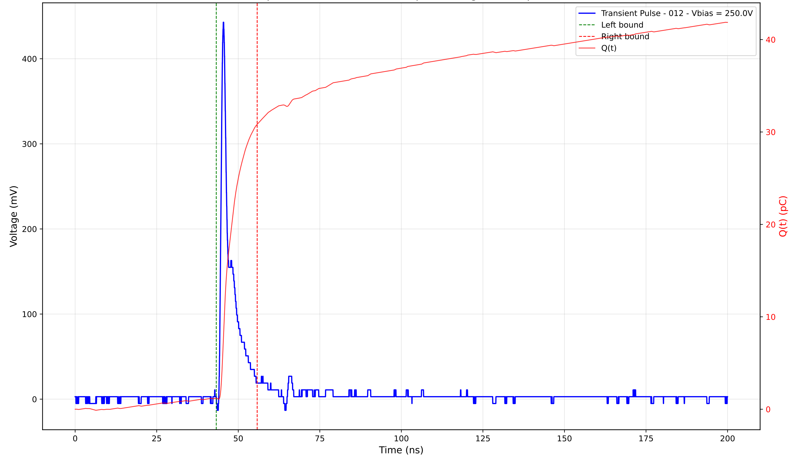
Transient Pulse - Sample: 4003 - Position: 110.0 \mu\text{m} - Charge: 29.63 pC - Rise Time: 0.91 ns
