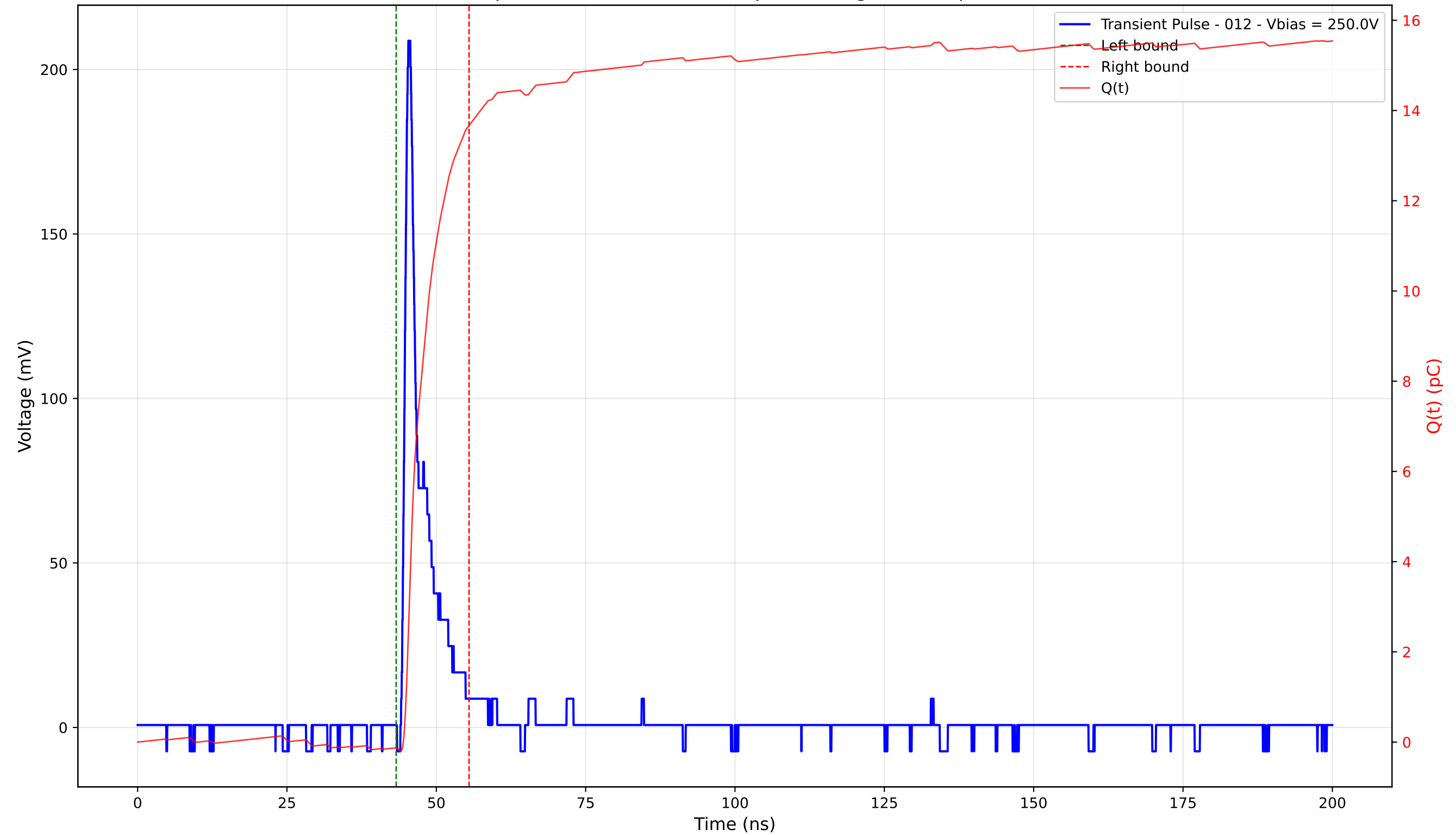
Transient Pulse - Sample: 4003 - Position: 95.0 \mu\text{m} - Charge: 13.79 pC - Rise Time: 0.87 ns
