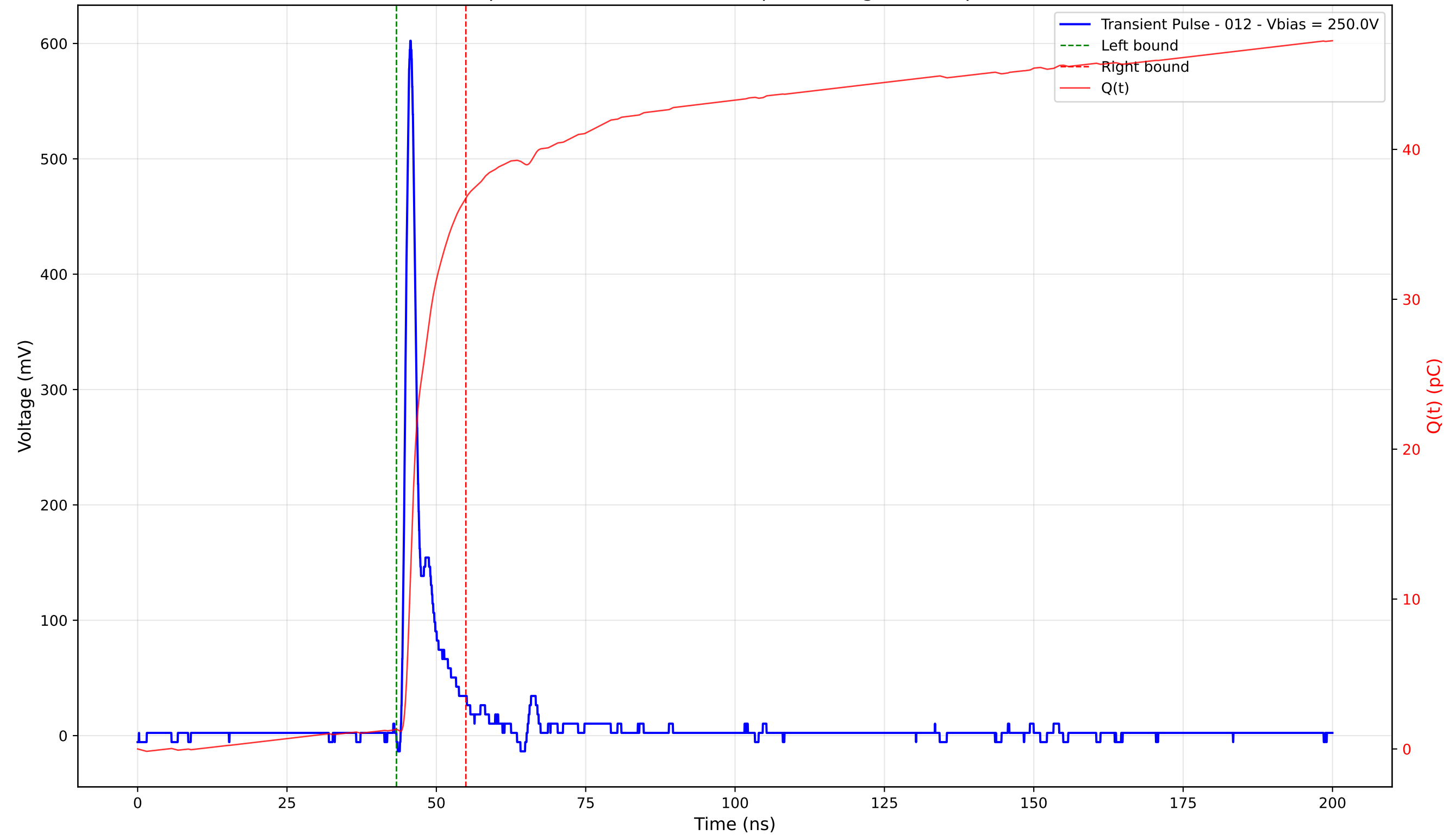
Transient Pulse - Sample: 4003 - Position: 185.0 \mu\text{m} - Charge: 35.45 pC - Rise Time: 1.04 ns
