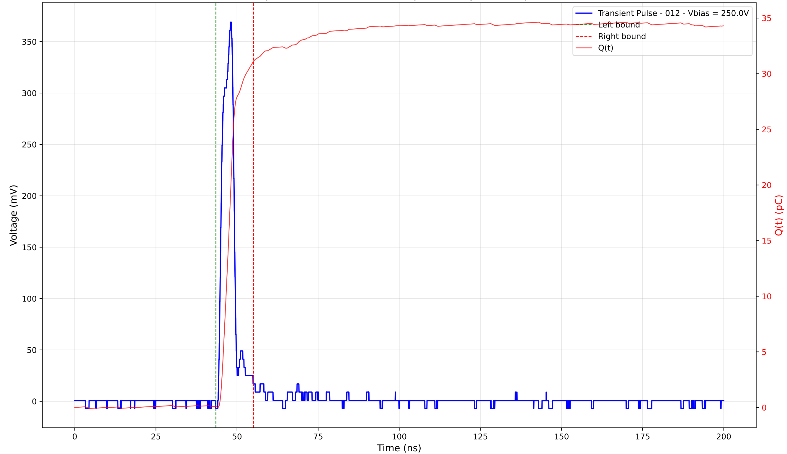
Transient Pulse - Sample: 4003 - Position: 330.0 \mu\text{m} - Charge: 31.03 pC - Rise Time: 2.93 ns
