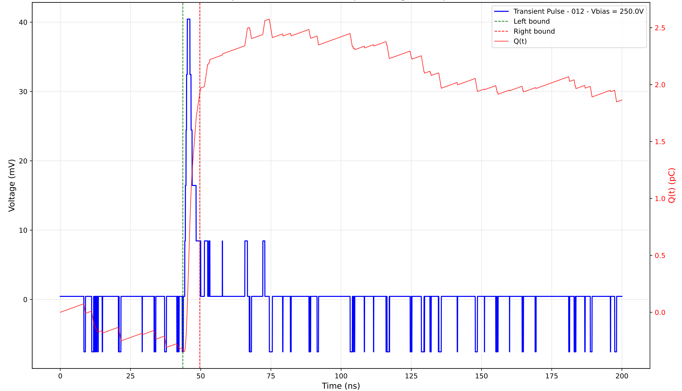
Transient Pulse - Sample: 4003 - Position: 45.0 \mu\text{m} - Charge: 2.25 pC - Rise Time: 0.91 ns
