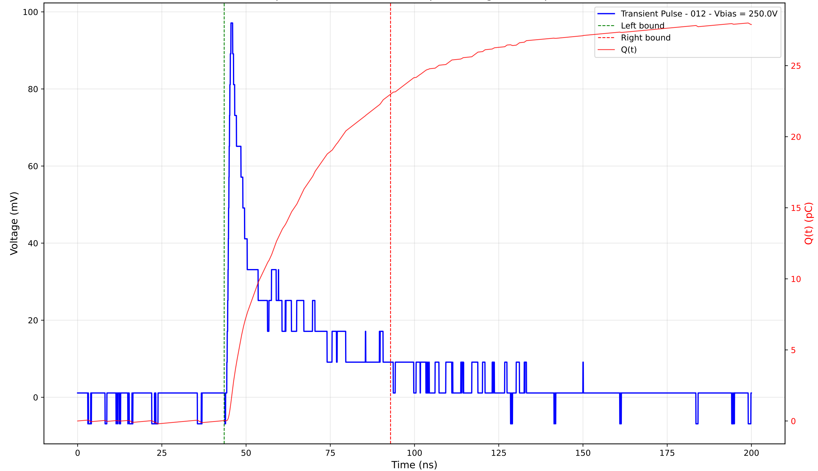
Transient Pulse - Sample: 4003 - Position: 385.0 \mu\text{m} - Charge: 22.96 pC - Rise Time: 0.94 ns
