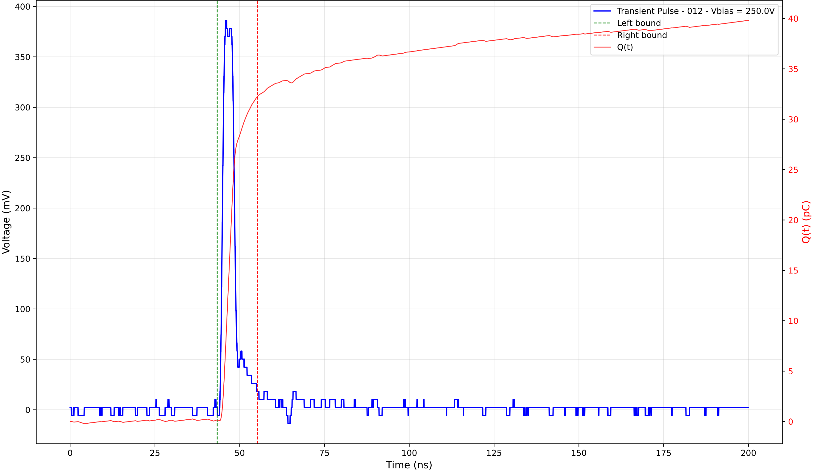
Transient Pulse - Sample: 4003 - Position: 300.0 \mu\text{m} - Charge: 32.09 pC - Rise Time: 1.17 ns
