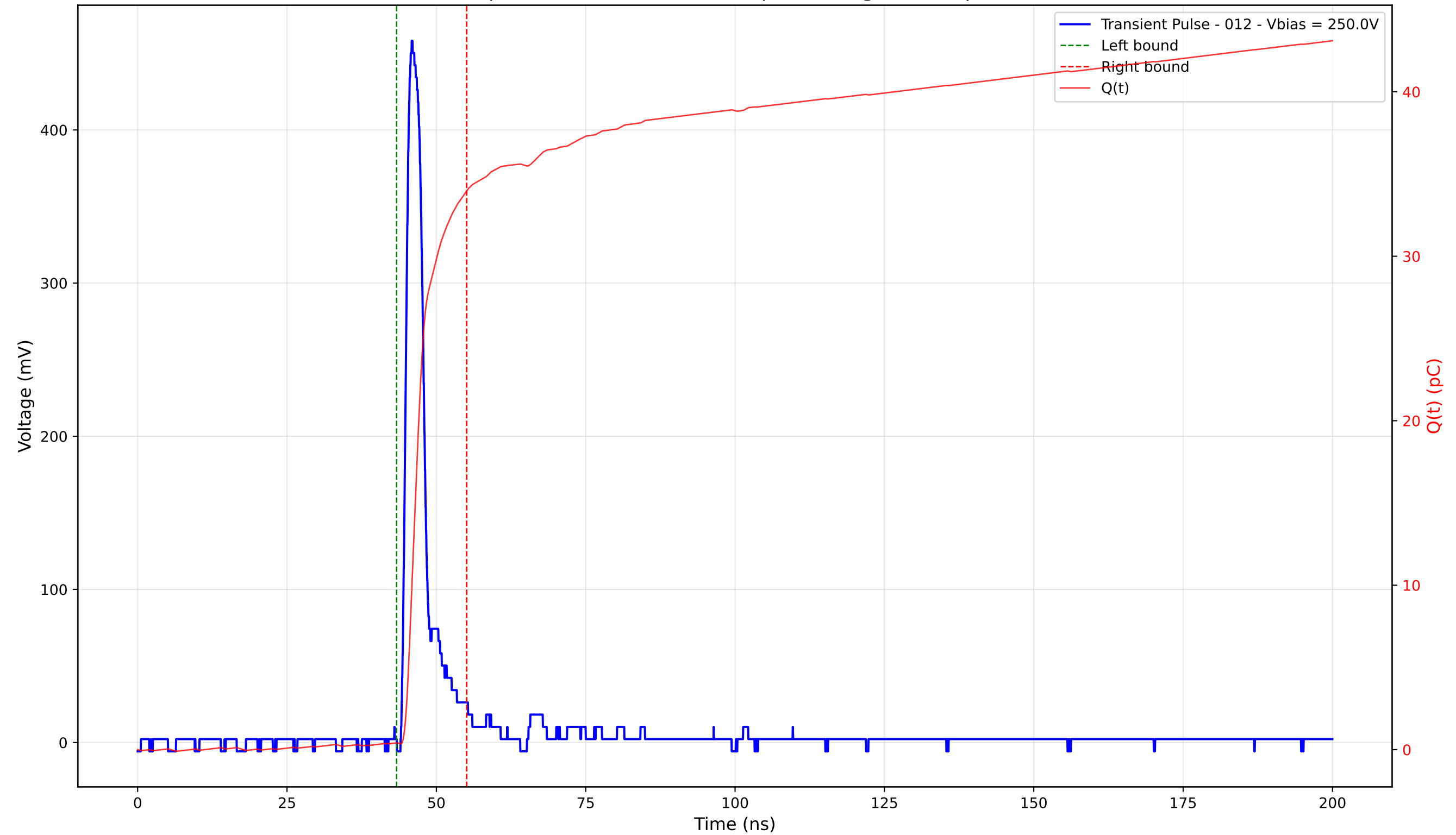
Transient Pulse - Sample: 4003 - Position: 270.0 \mu\text{m} - Charge: 33.55 pC - Rise Time: 1.13 ns
