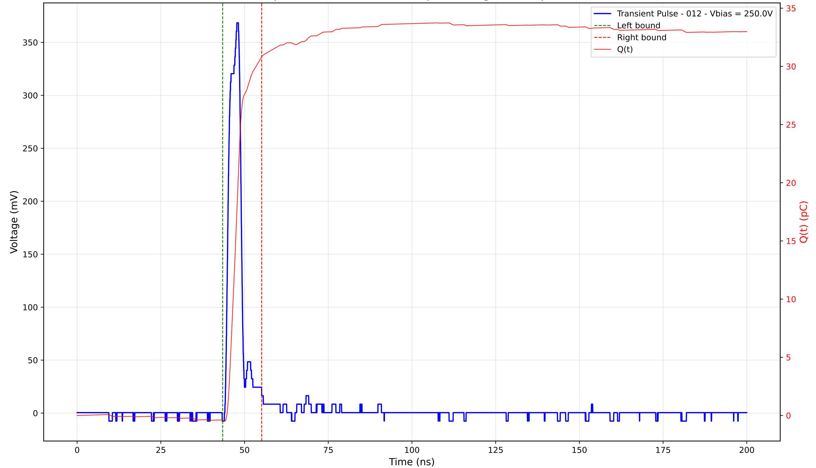
Transient Pulse - Sample: 4003 - Position: 325.0 \mu\text{m} - Charge: 31.23 pC - Rise Time: 2.71 ns
