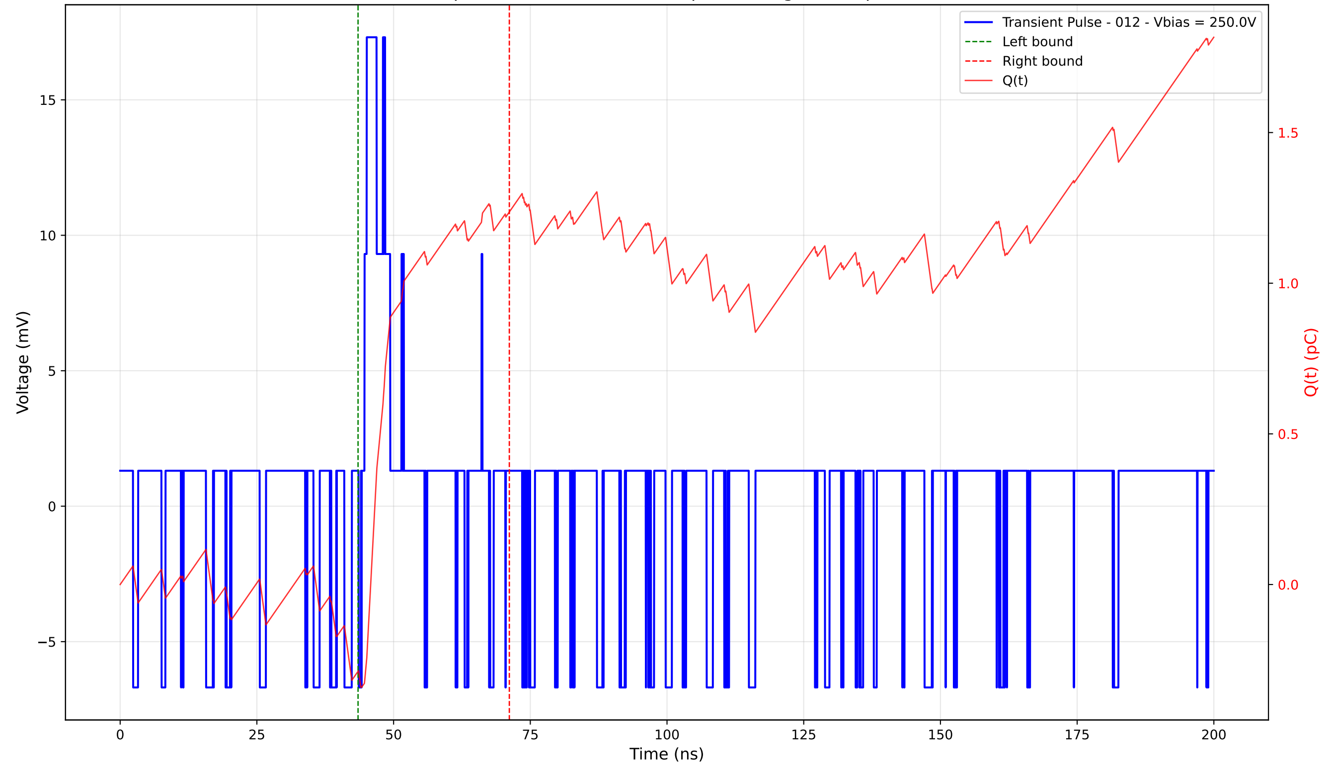
Transient Pulse - Sample: 4003 - Position: 65.0 \mu\text{m} - Charge: 1.52 pC - Rise Time: 0.42 ns
