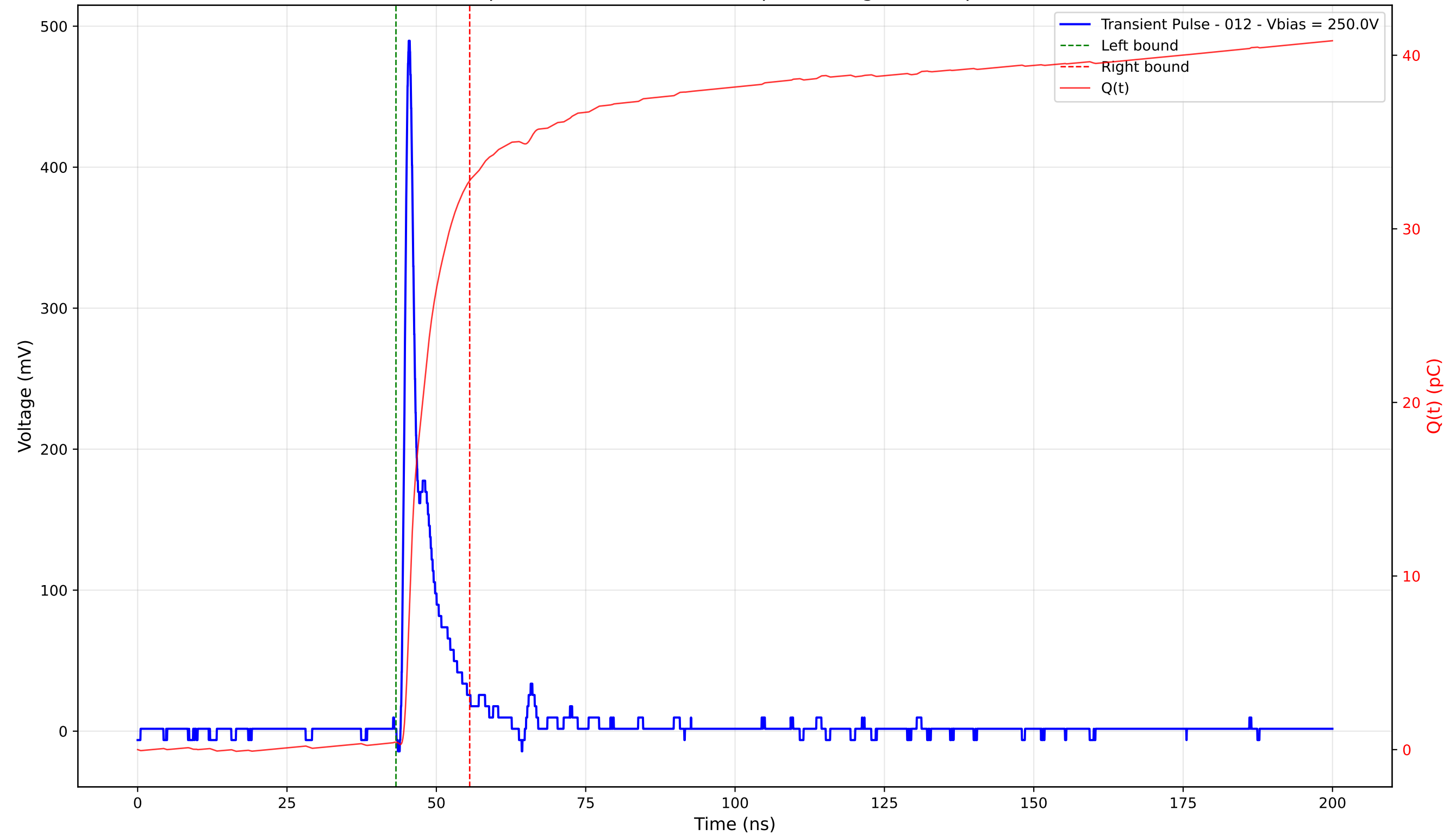
Transient Pulse - Sample: 4003 - Position: 115.0 \mu\text{m} - Charge: 32.35 pC - Rise Time: 0.88 ns
