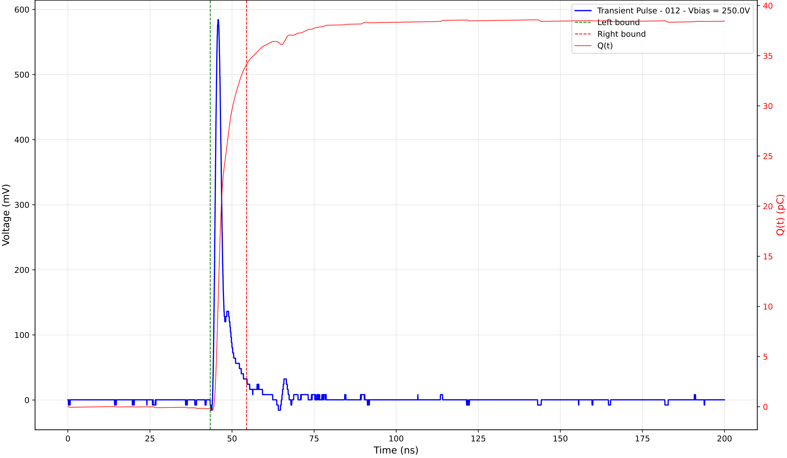
Transient Pulse - Sample: 4003 - Position: 205.0 \mu\text{m} - Charge: 34.33 pC - Rise Time: 1.07 ns
