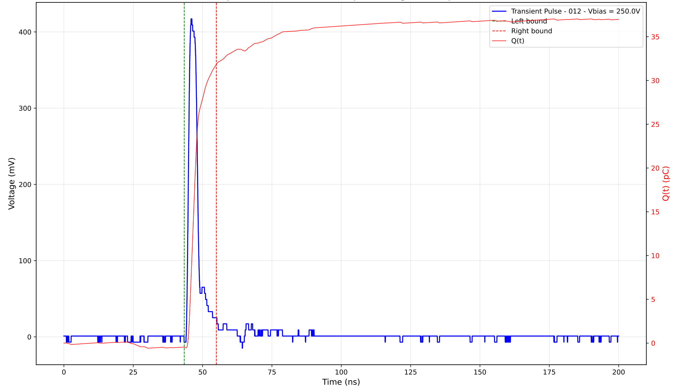
Transient Pulse - Sample: 4003 - Position: 285.0 \mu\text{m} - Charge: 32.30 pC - Rise Time: 1.10 ns
