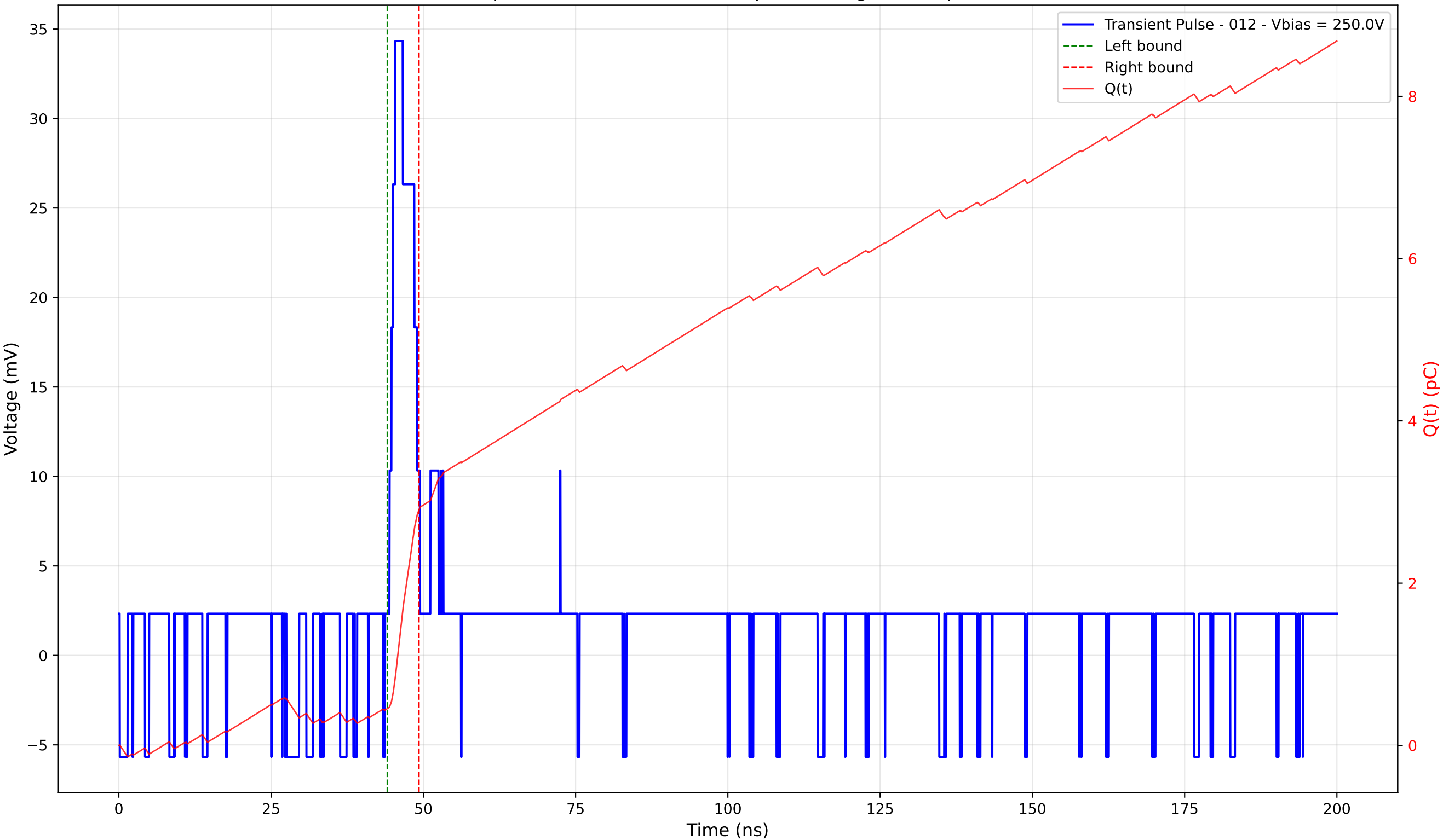
Transient Pulse - Sample: 4003 - Position: 60.0 \mu\text{m} - Charge: 2.45 pC - Rise Time: 0.96 ns
