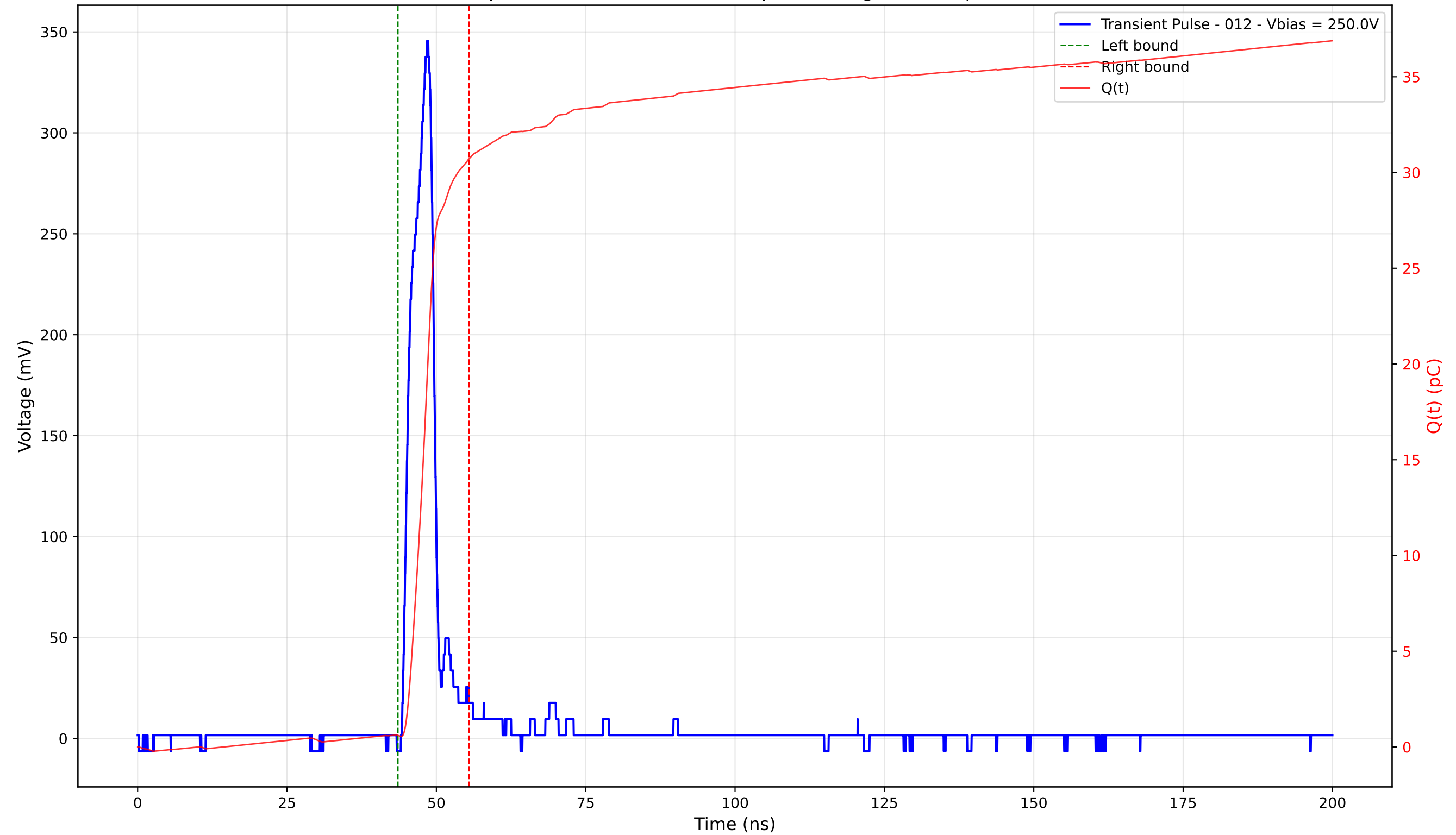
Transient Pulse - Sample: 4003 - Position: 345.0 \mu\text{m} - Charge: 30.11 pC - Rise Time: 3.28 ns
