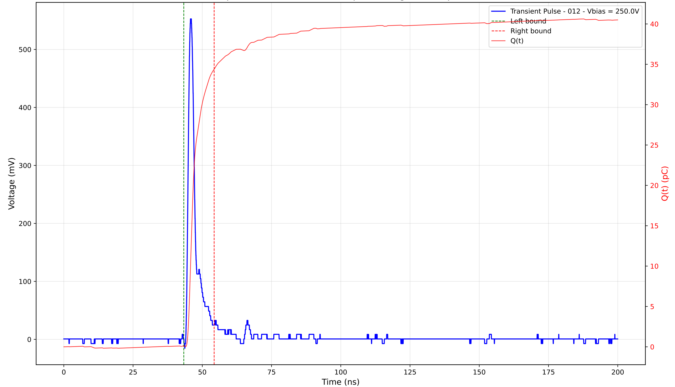
Transient Pulse - Sample: 4003 - Position: 225.0 \mu\text{m} - Charge: 34.26 pC - Rise Time: 1.12 ns
