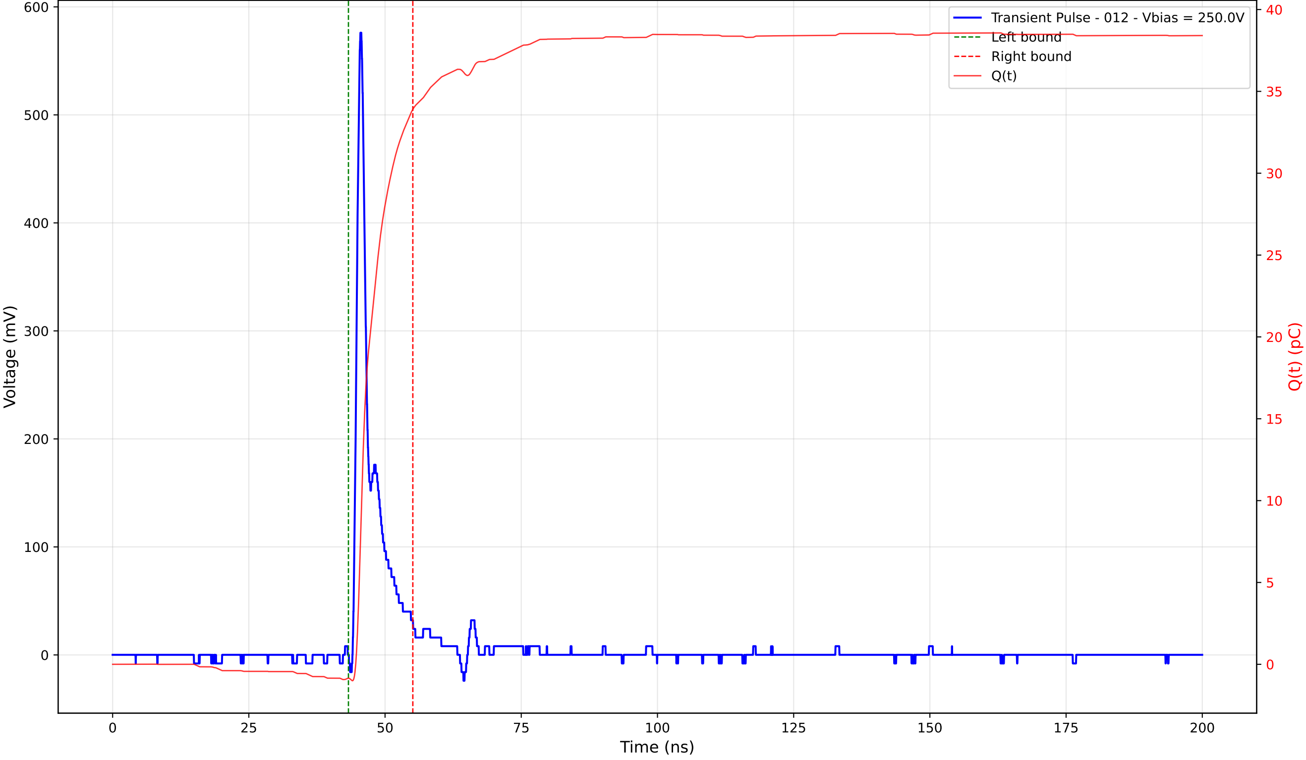
Transient Pulse - Sample: 4003 - Position: 155.0 \mu\text{m} - Charge: 34.76 pC - Rise Time: 0.93 ns
