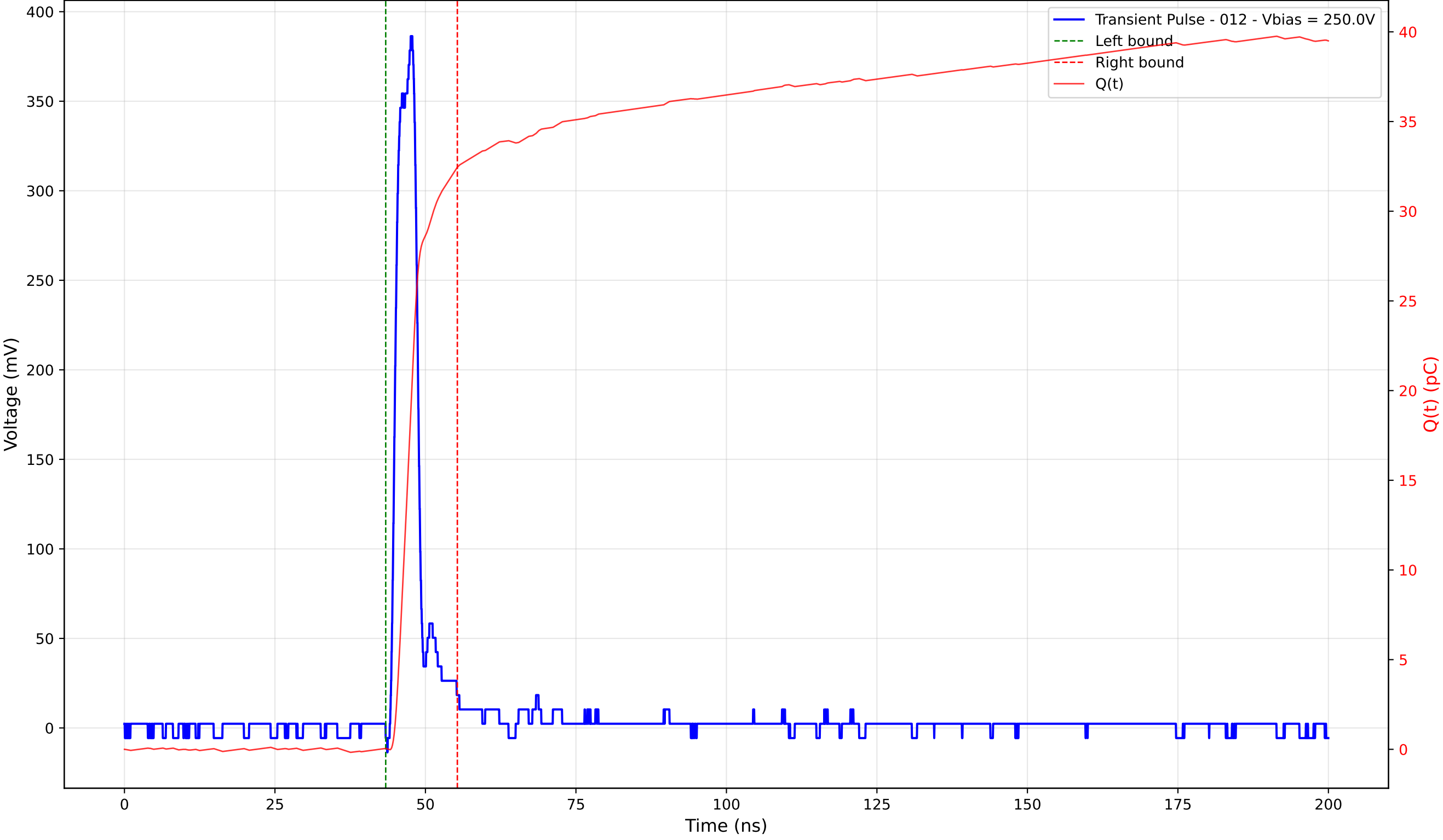
Transient Pulse - Sample: 4003 - Position: 315.0 \mu\text{m} - Charge: 32.40 pC - Rise Time: 1.71 ns
