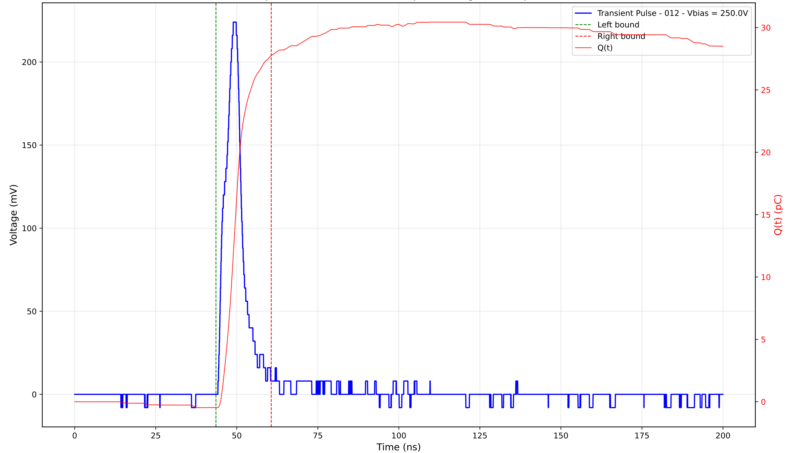
Transient Pulse - Sample: 4003 - Position: 365.0 \mu\text{m} - Charge: 28.23 pC - Rise Time: 3.88 ns
