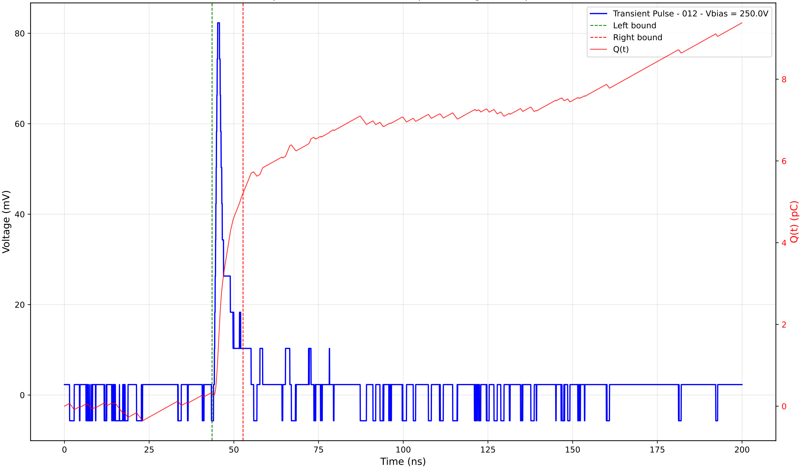
Transient Pulse - Sample: 4003 - Position: 85.0 \mu\text{m} - Charge: 4.90 pC - Rise Time: 0.83 ns
