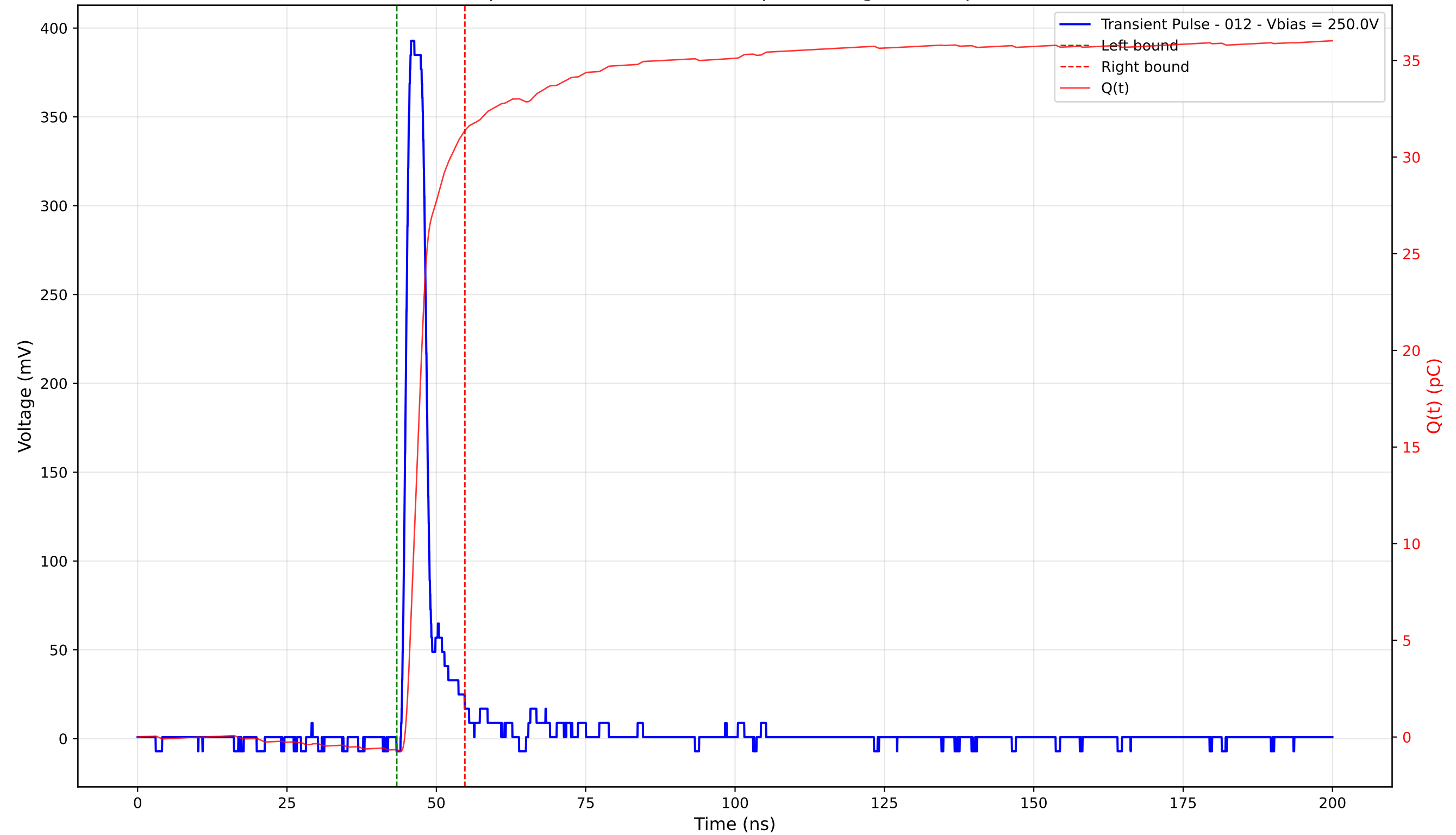
Transient Pulse - Sample: 4003 - Position: 295.0 \mu\text{m} - Charge: 32.04 pC - Rise Time: 1.16 ns
