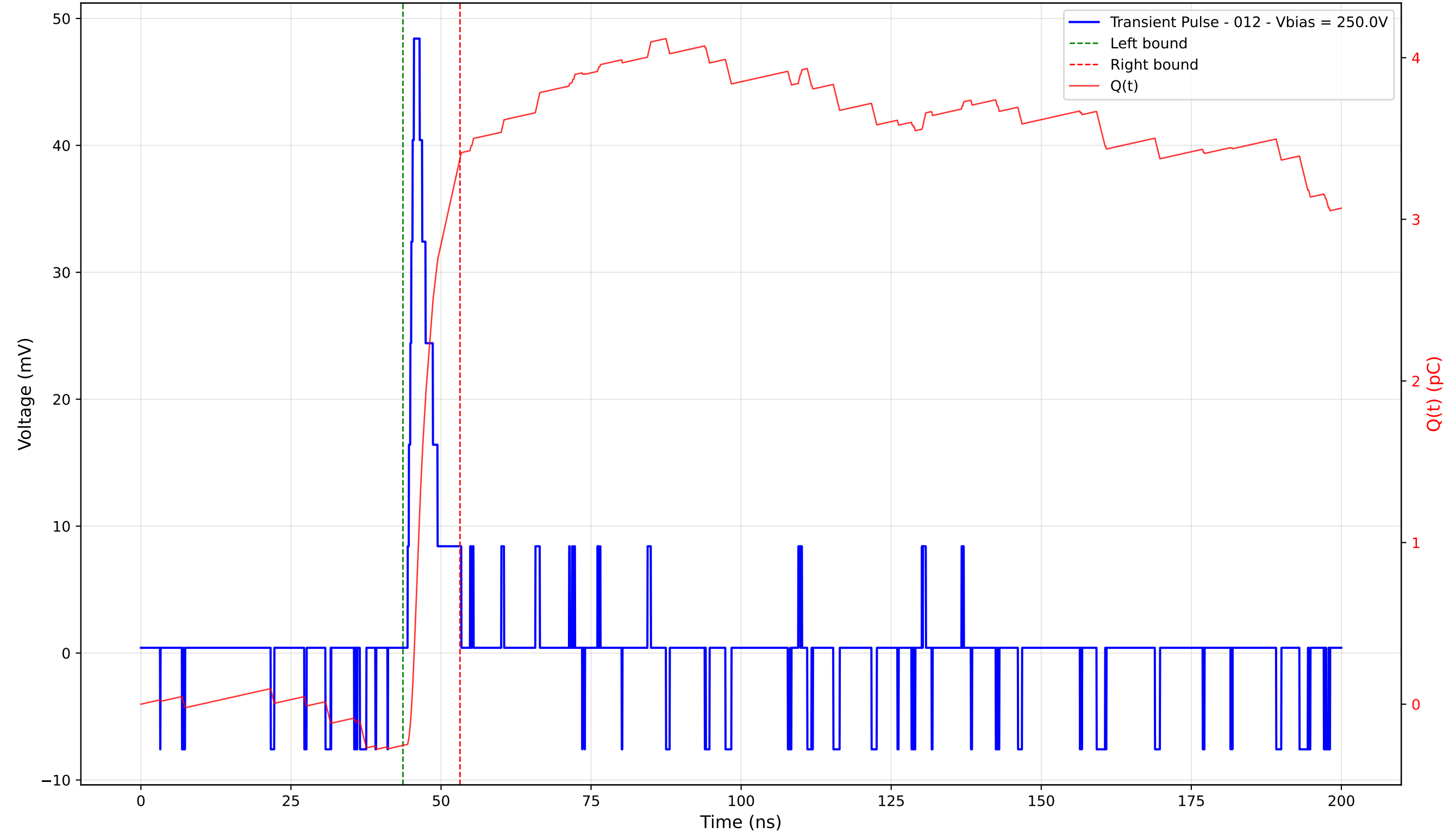
Transient Pulse - Sample: 4003 - Position: 55.0 \mu\text{m} - Charge: 3.63 pC - Rise Time: 1.05 ns
