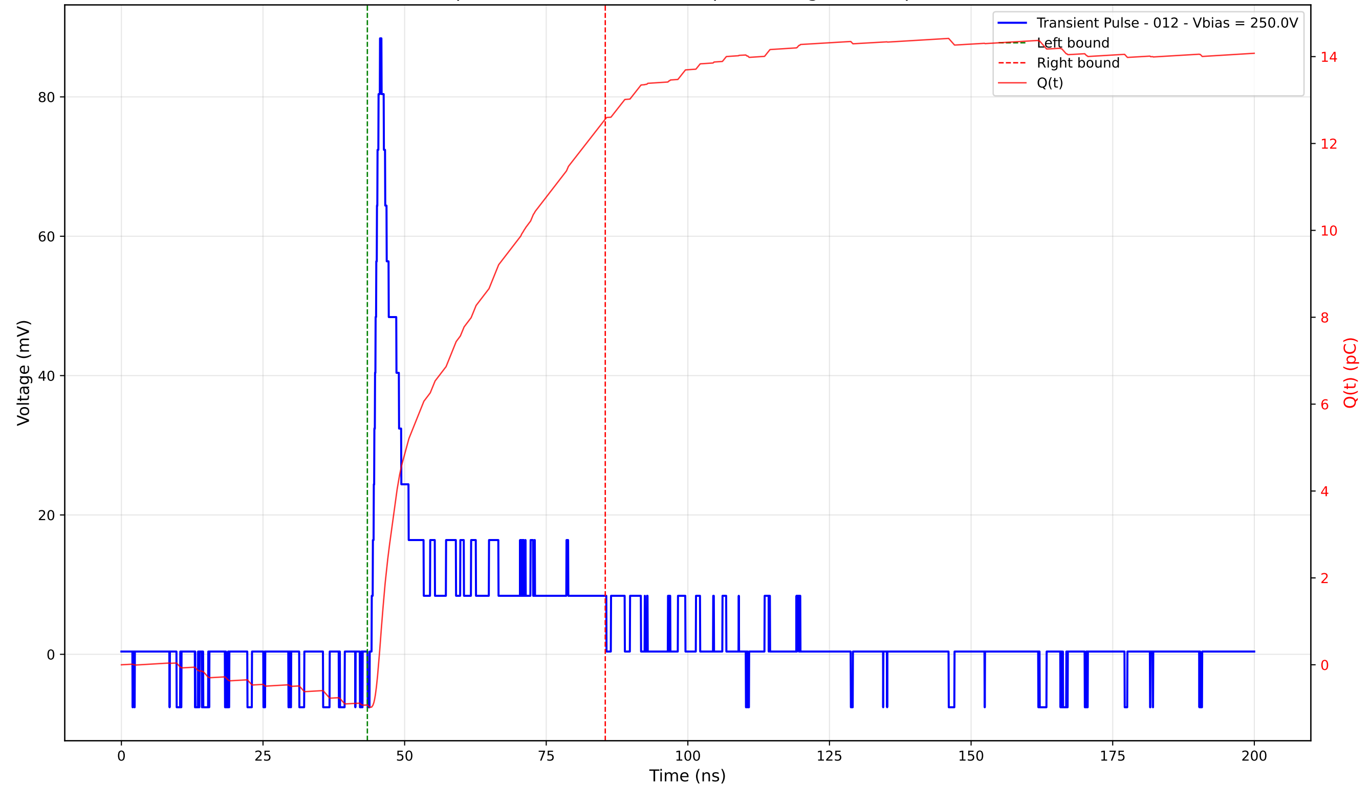
Transient Pulse - Sample: 4003 - Position: 395.0 \mu\text{m} - Charge: 13.49 pC - Rise Time: 1.02 ns
