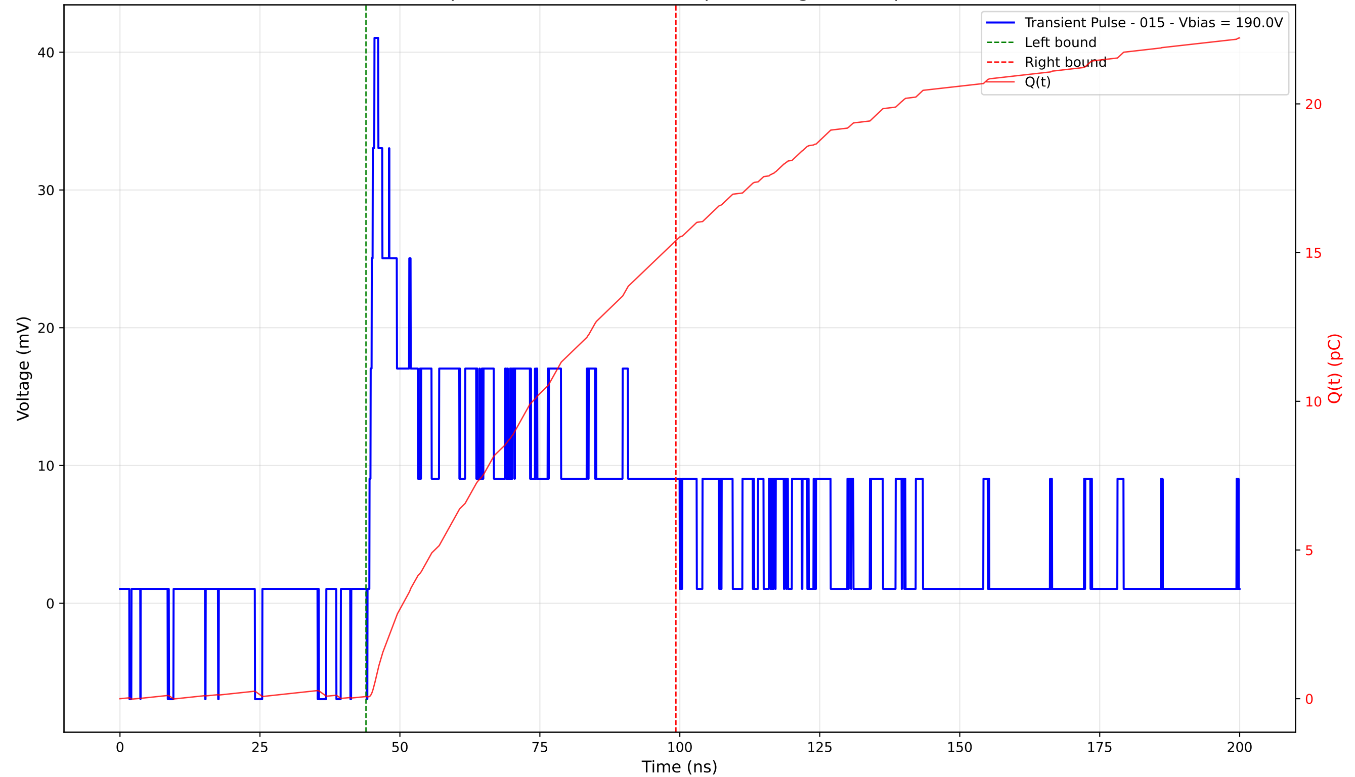
Transient Pulse - Sample: 4003 - Position: 350.0 \mu\text{m} - Charge: 15.33 pC - Rise Time: 0.89 ns
