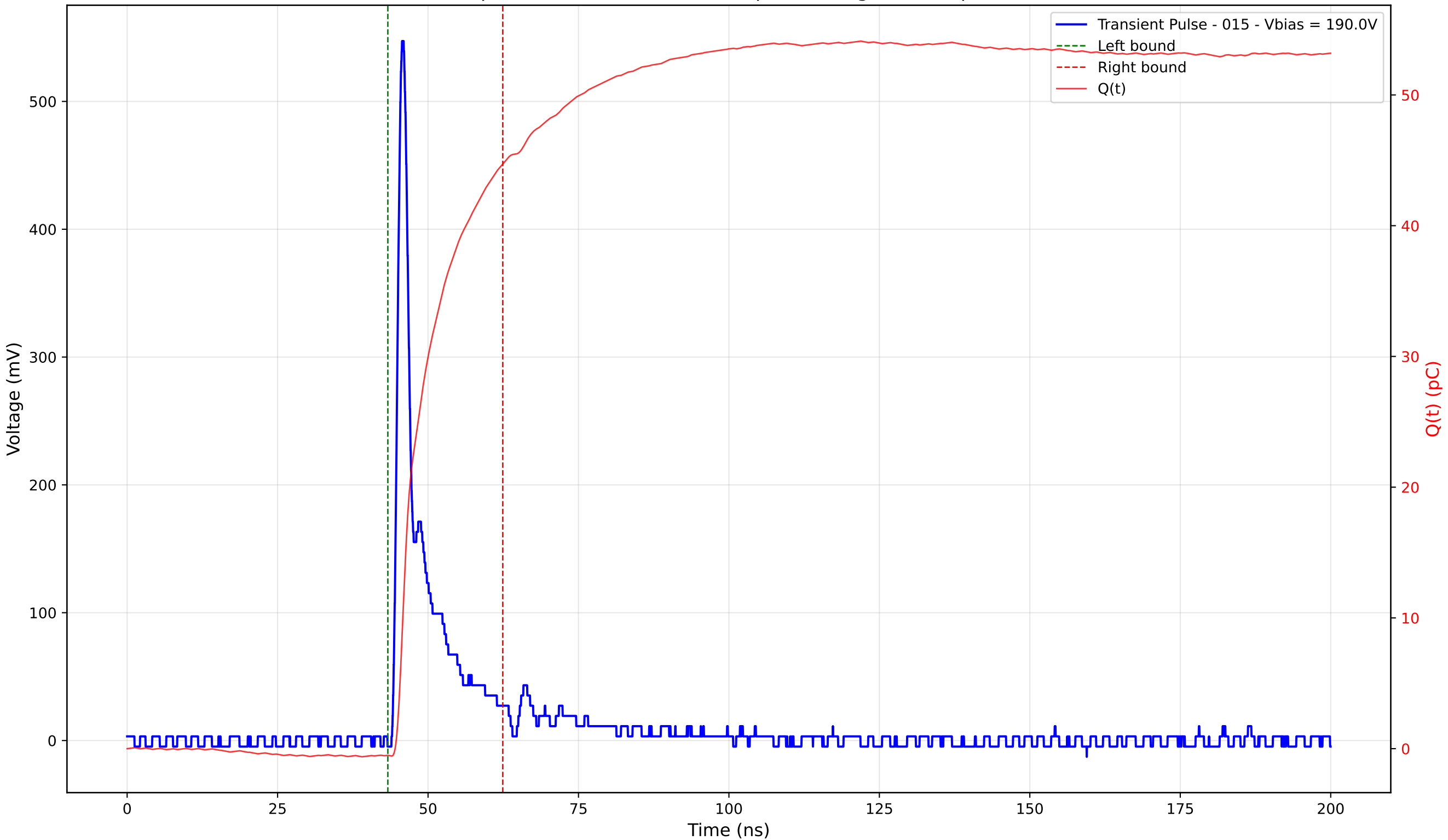
Transient Pulse - Sample: 4003 - Position: 195.0 \mu\text{m} - Charge: 45.24 pC - Rise Time: 1.11 ns
