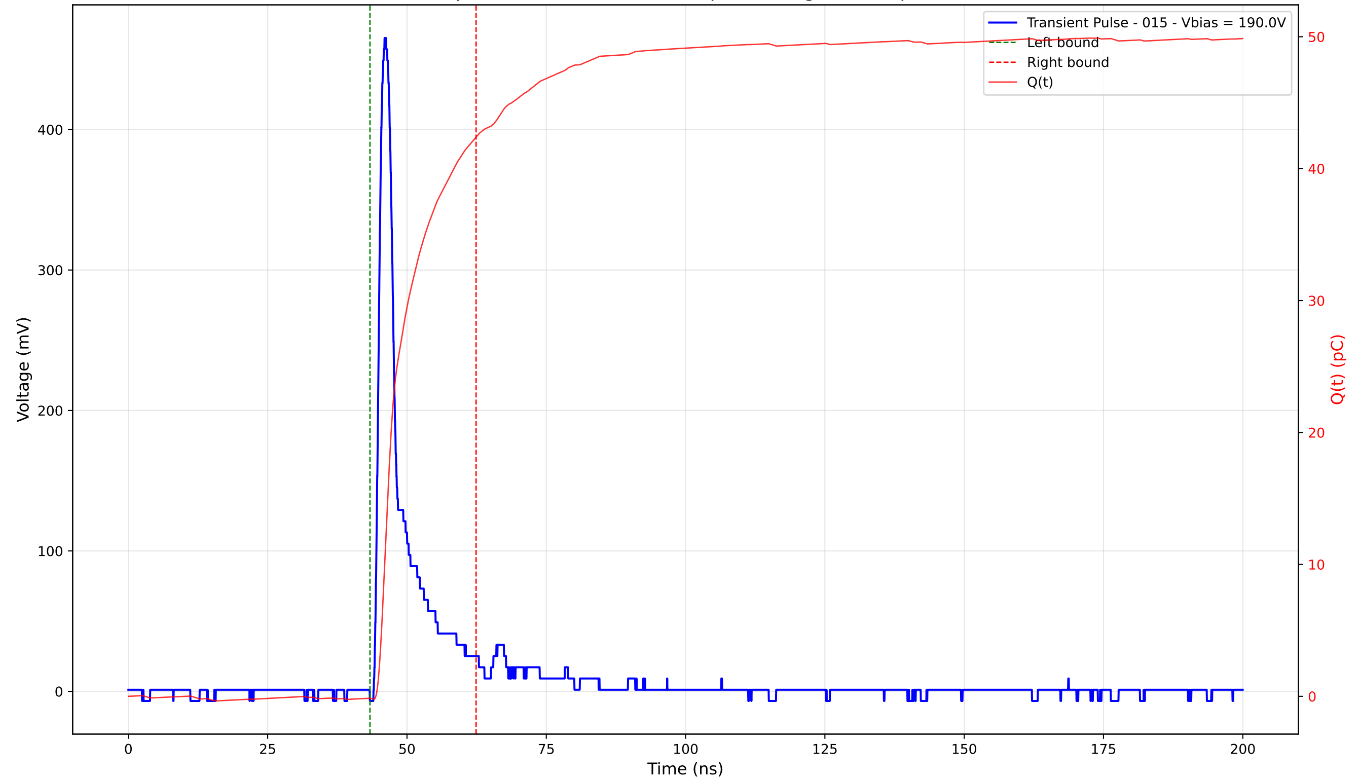
Transient Pulse - Sample: 4003 - Position: 235.0 \mu\text{m} - Charge: 42.55 pC - Rise Time: 1.23 ns
