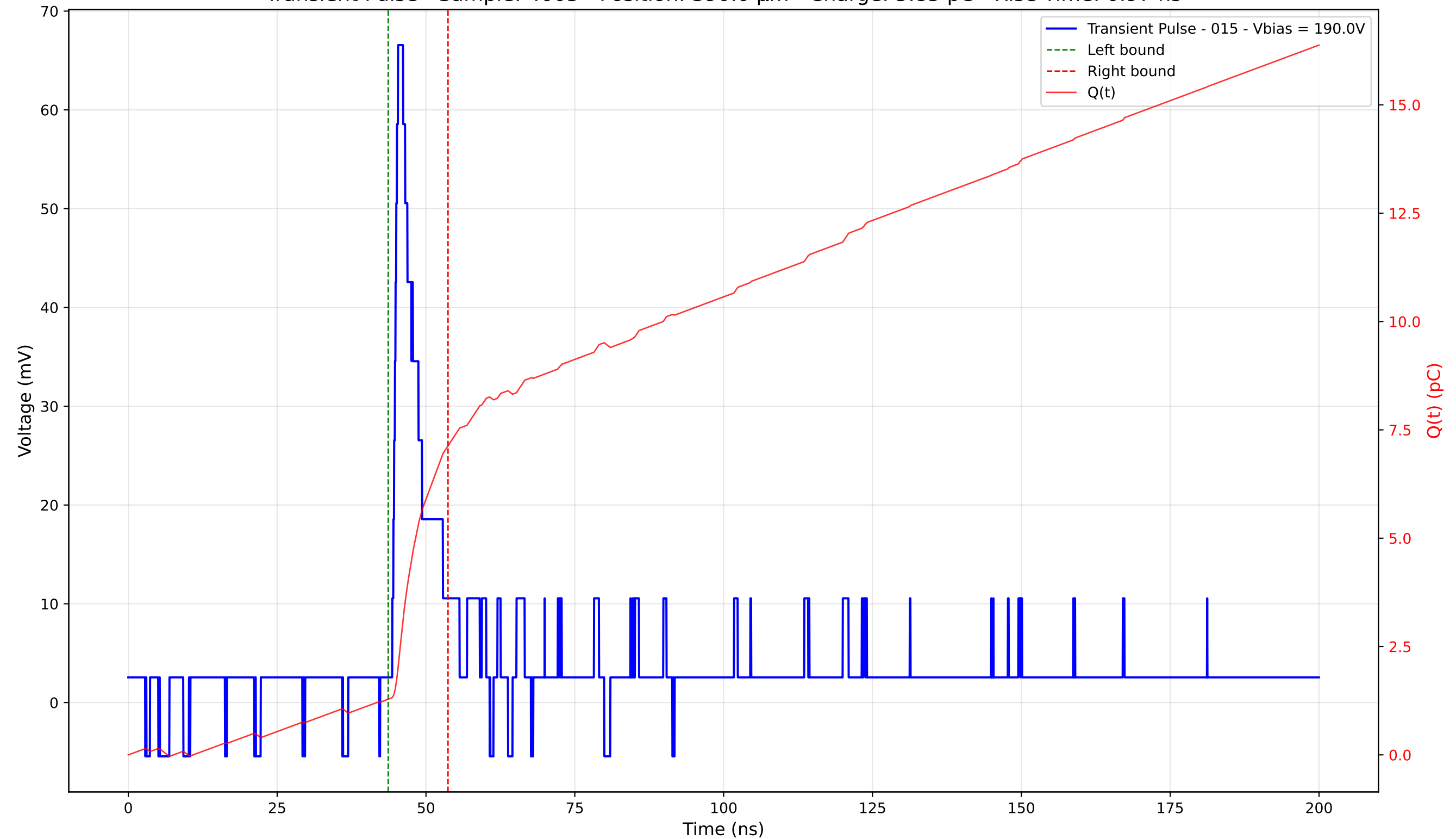
Transient Pulse - Sample: 4003 - Position: 390.0 \mu\text{m} - Charge: 5.85 pC - Rise Time: 0.97 ns
