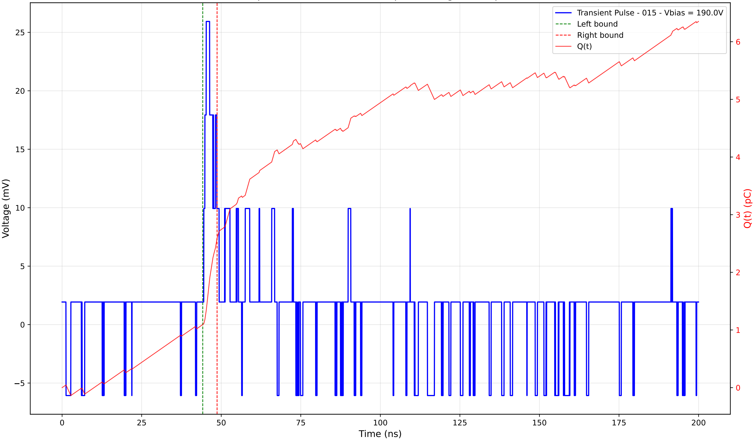
Transient Pulse - Sample: 4003 - Position: 30.0 \mu\text{m} - Charge: 1.50 pC - Rise Time: 0.78 ns
