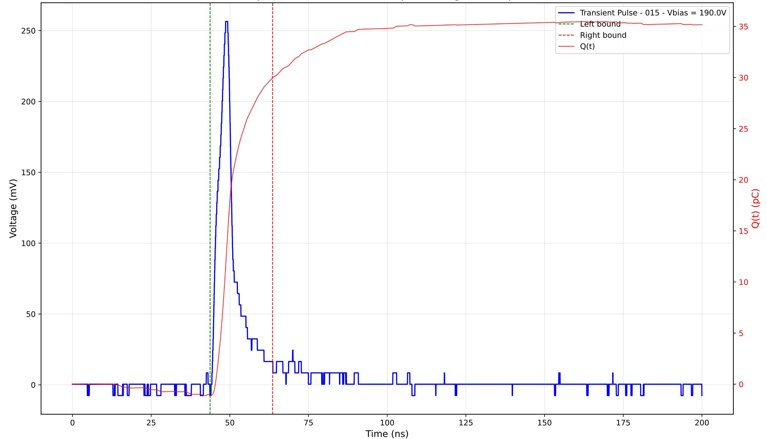
Transient Pulse - Sample: 4003 - Position: 320.0 \mu\text{m} - Charge: 31.00 pC - Rise Time: 3.46 ns
