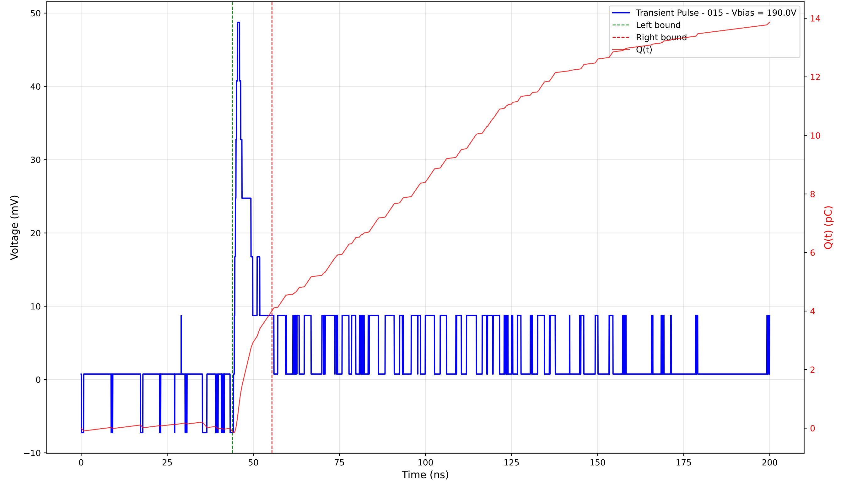
Transient Pulse - Sample: 4003 - Position: 365.0 \mu\text{m} - Charge: 4.12 pC - Rise Time: 0.95 ns
