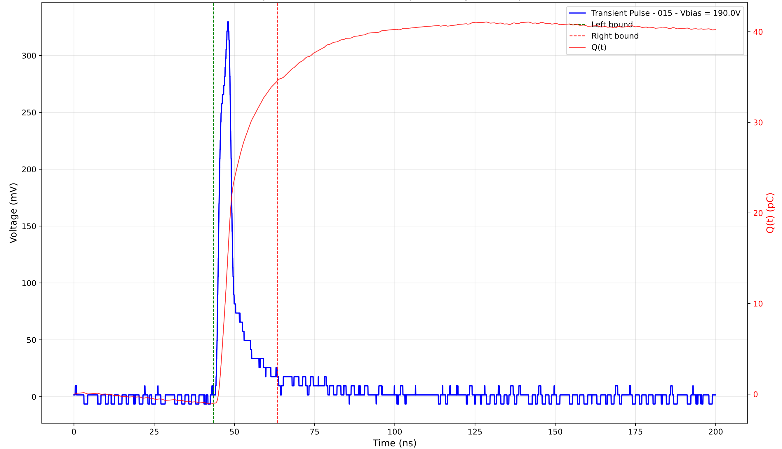
Transient Pulse - Sample: 4003 - Position: 300.0 \mu\text{m} - Charge: 35.59 pC - Rise Time: 2.82 ns
