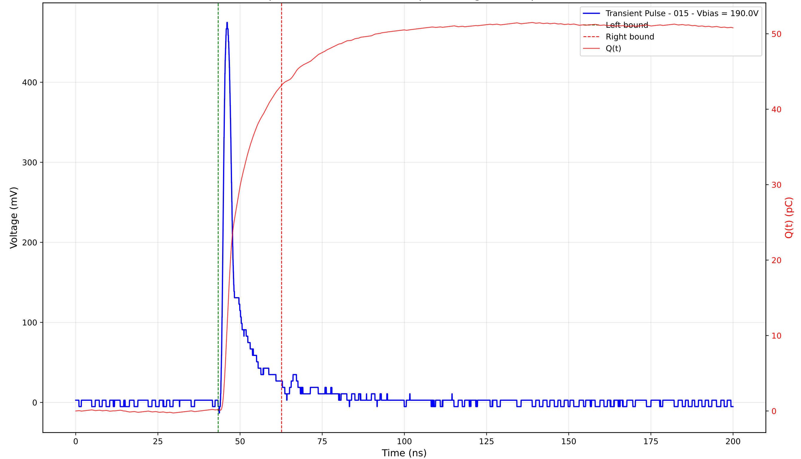
Transient Pulse - Sample: 4003 - Position: 230.0 \mu\text{m} - Charge: 43.01 pC - Rise Time: 1.21 ns
