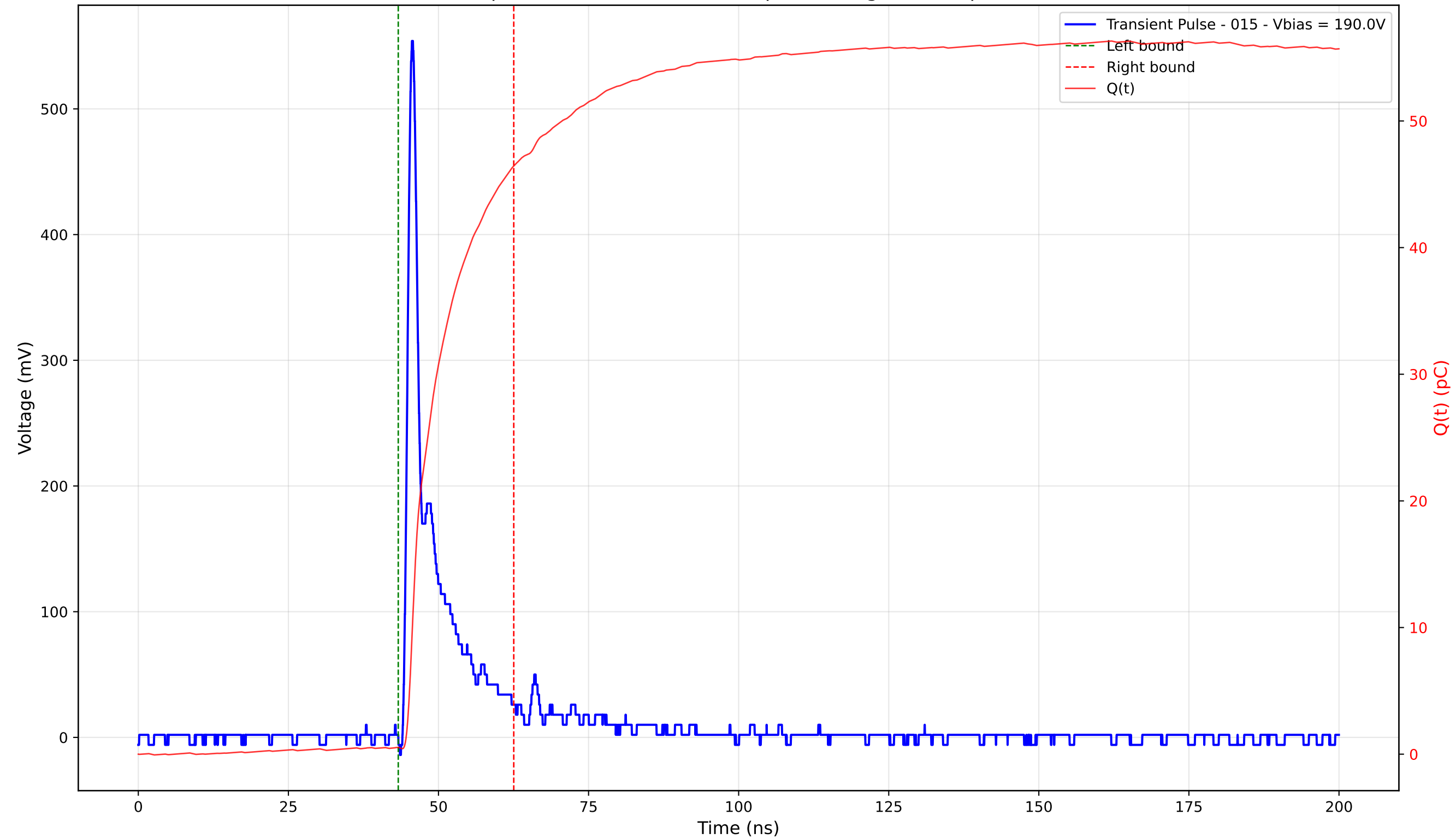
Transient Pulse - Sample: 4003 - Position: 170.0 \mu\text{m} - Charge: 45.91 pC - Rise Time: 1.03 ns
