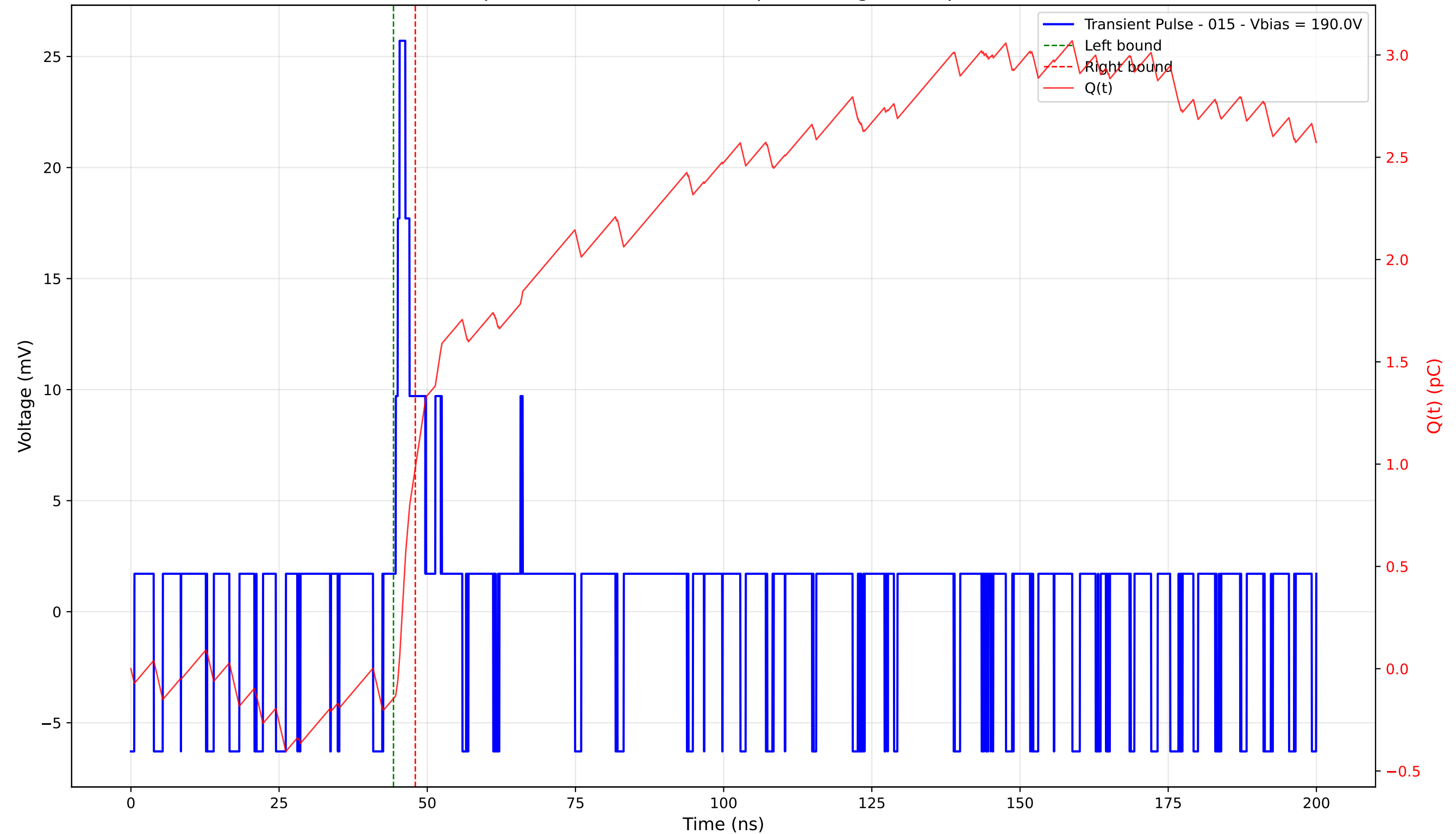
Transient Pulse - Sample: 4003 - Position: 415.0 \mu\text{m} - Charge: 1.13 pC - Rise Time: 0.66 ns
