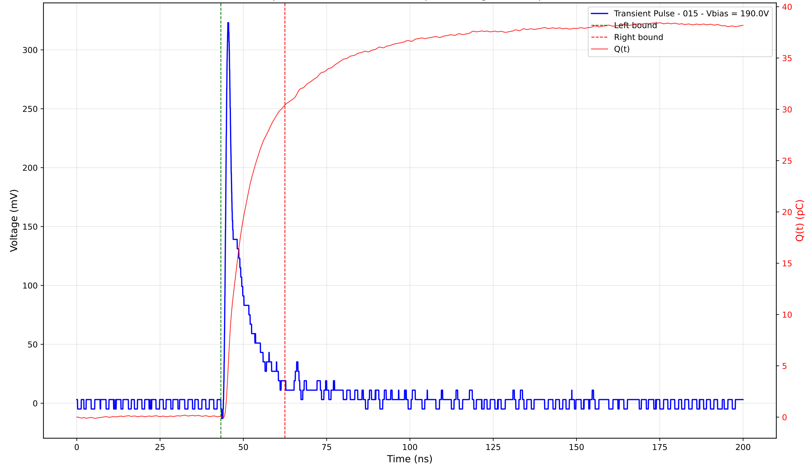
Transient Pulse - Sample: 4003 - Position: 105.0 \mu\text{m} - Charge: 30.33 pC - Rise Time: 0.89 ns
