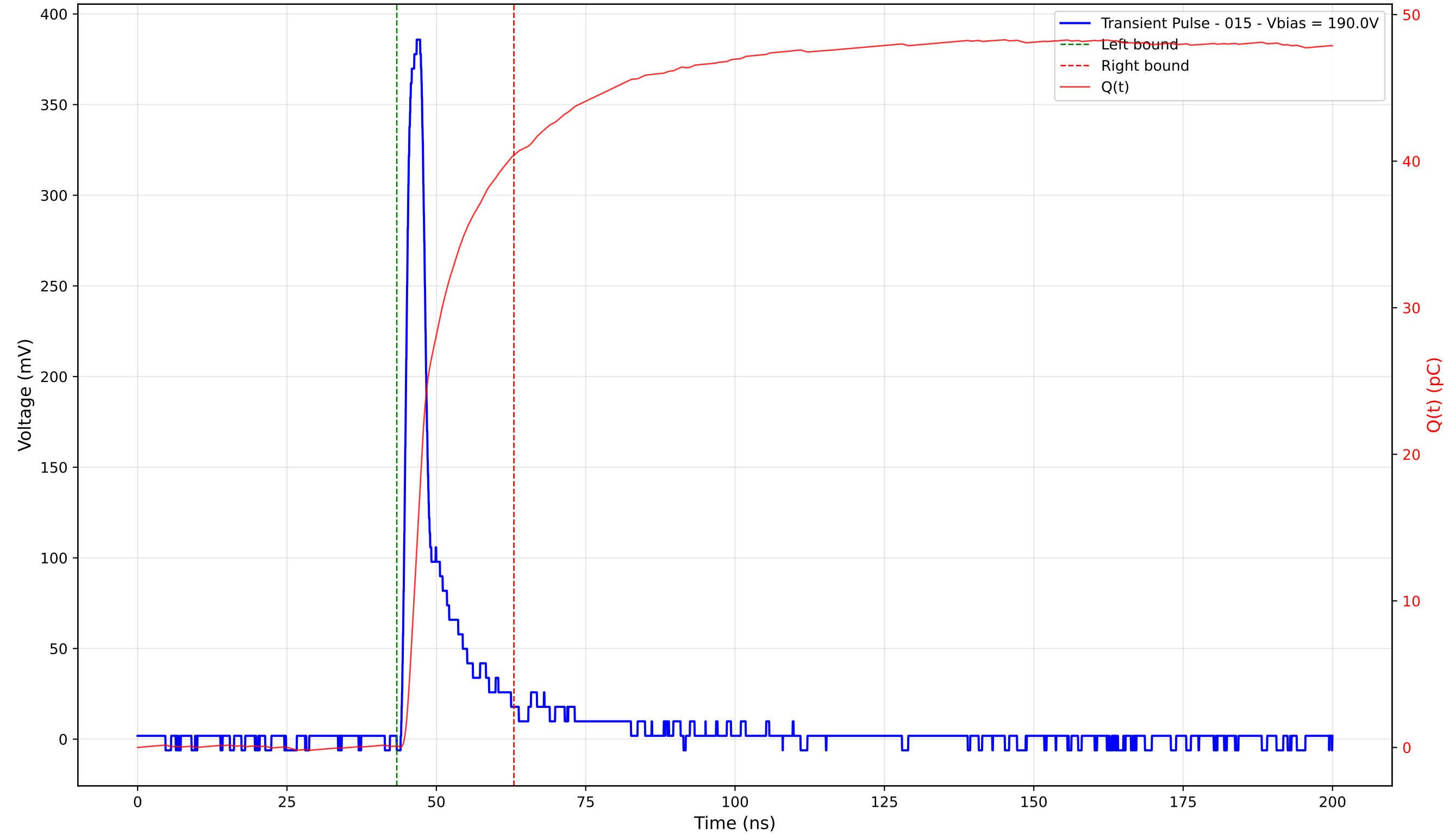
Transient Pulse - Sample: 4003 - Position: 265.0 \mu\text{m} - Charge: 40.31 pC - Rise Time: 1.31 ns
