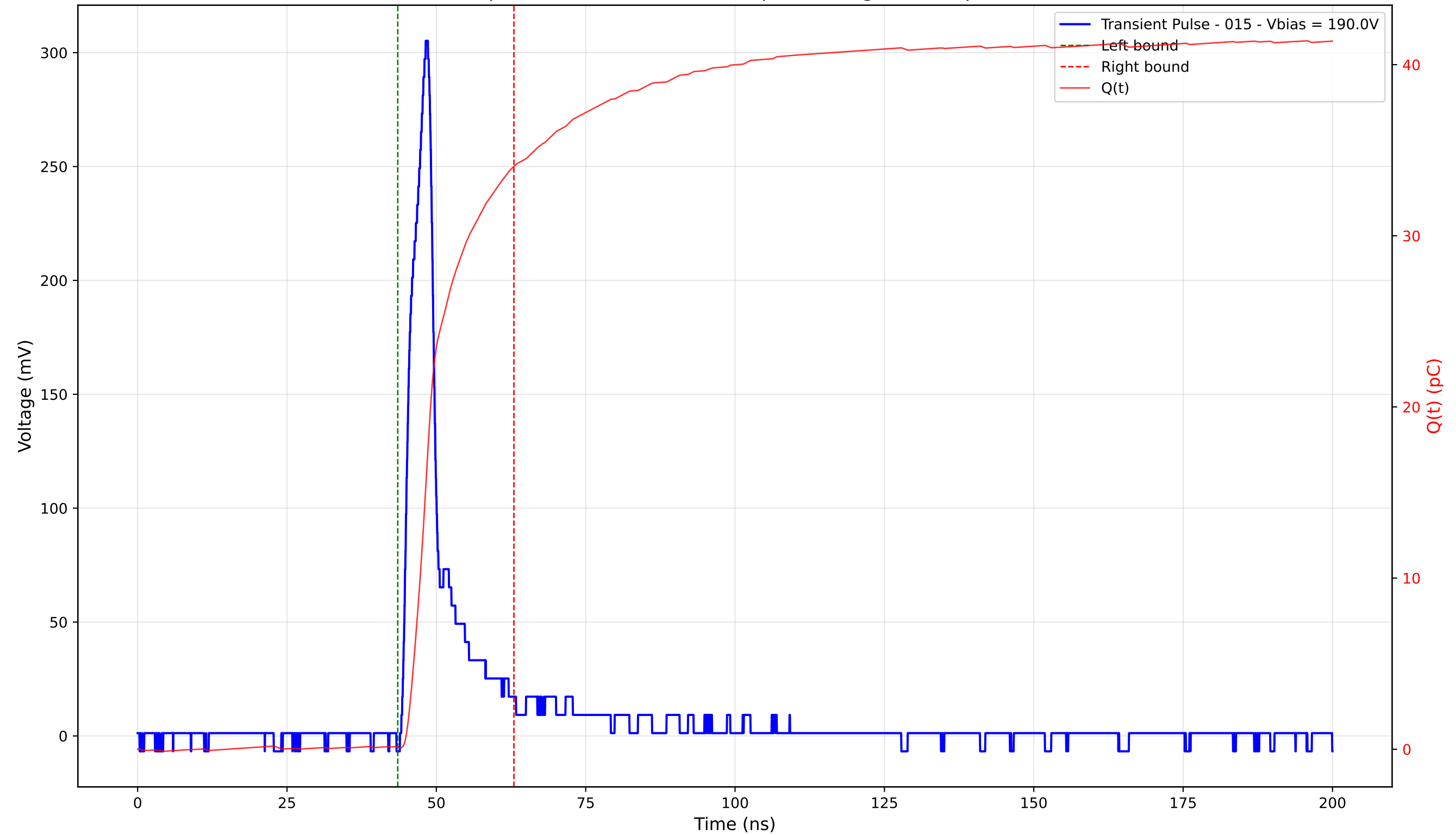
Transient Pulse - Sample: 4003 - Position: 310.0 \mu\text{m} - Charge: 33.94 pC - Rise Time: 3.25 ns
