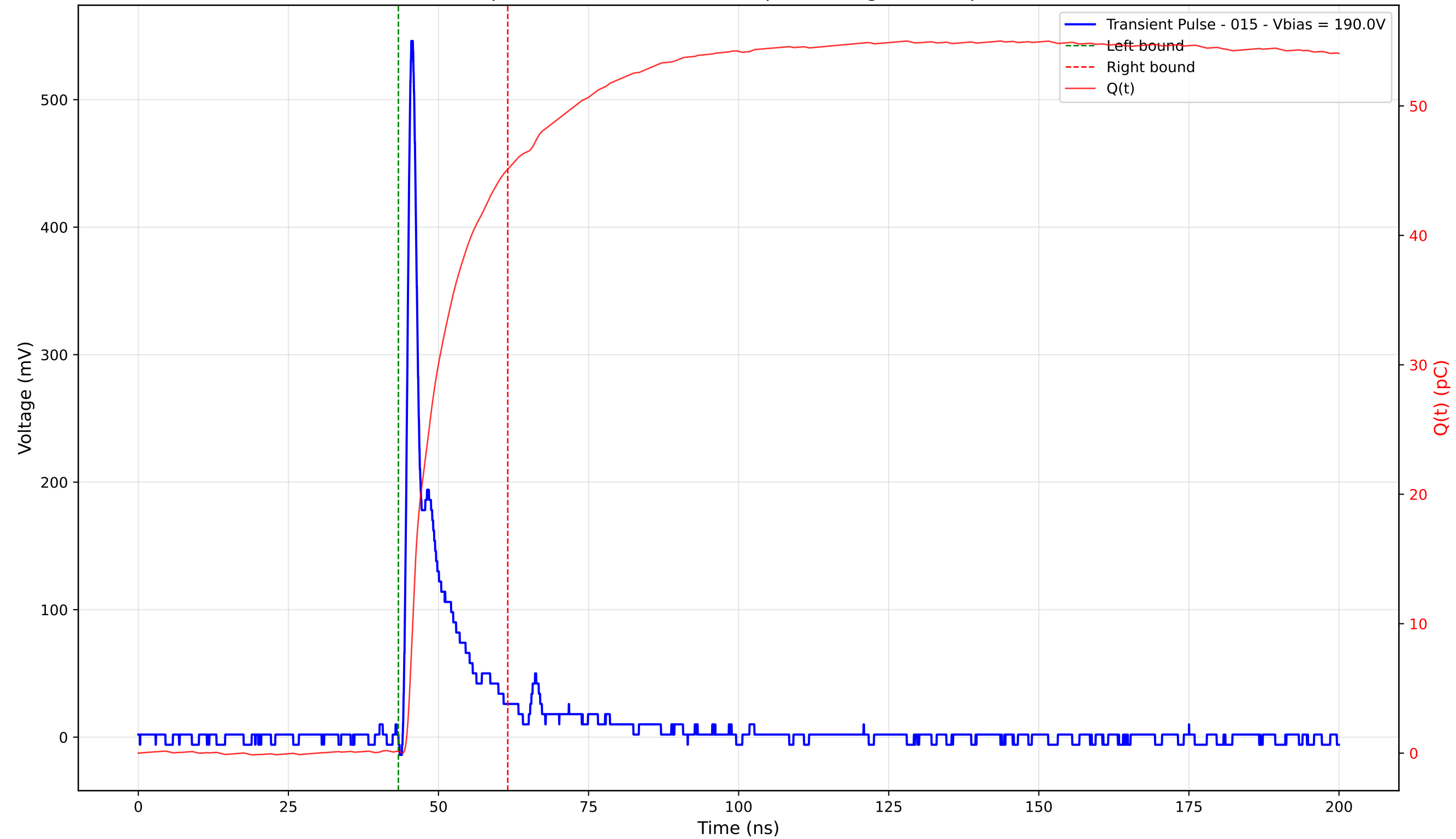
Transient Pulse - Sample: 4003 - Position: 160.0 \mu\text{m} - Charge: 44.96 pC - Rise Time: 0.97 ns
