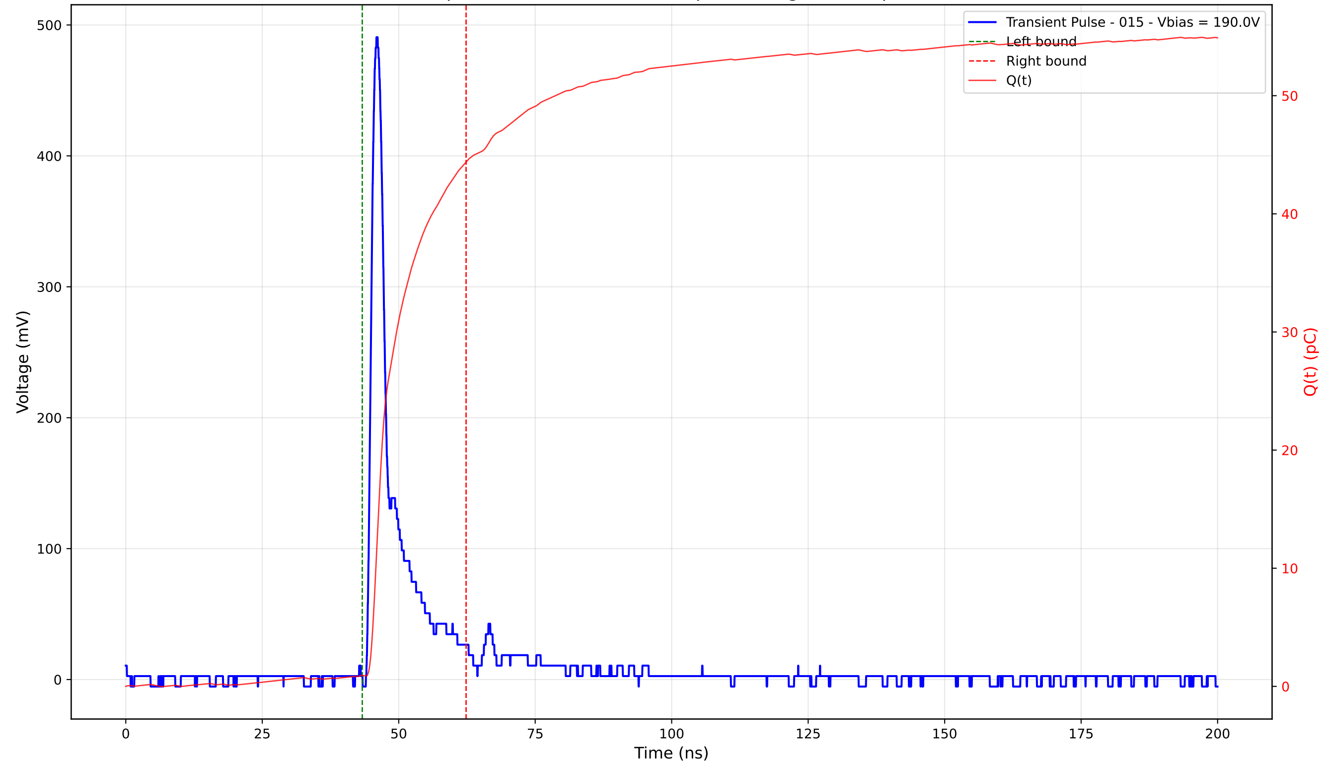
Transient Pulse - Sample: 4003 - Position: 225.0 \mu\text{m} - Charge: 43.46 pC - Rise Time: 1.16 ns
