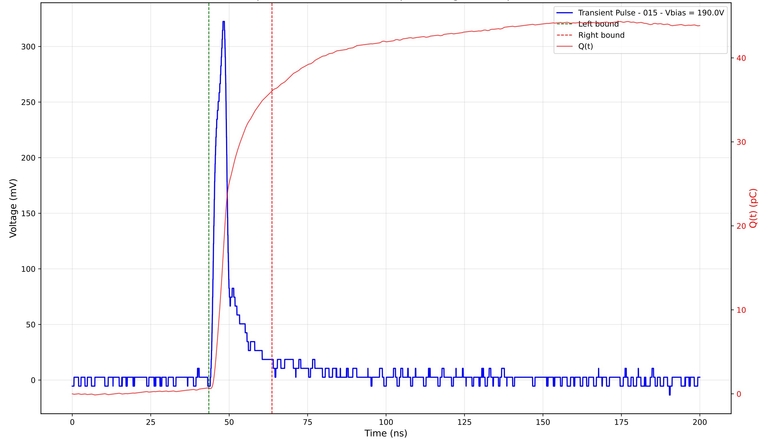
Transient Pulse - Sample: 4003 - Position: 305.0 \mu\text{m} - Charge: 35.40 pC - Rise Time: 3.05 ns
