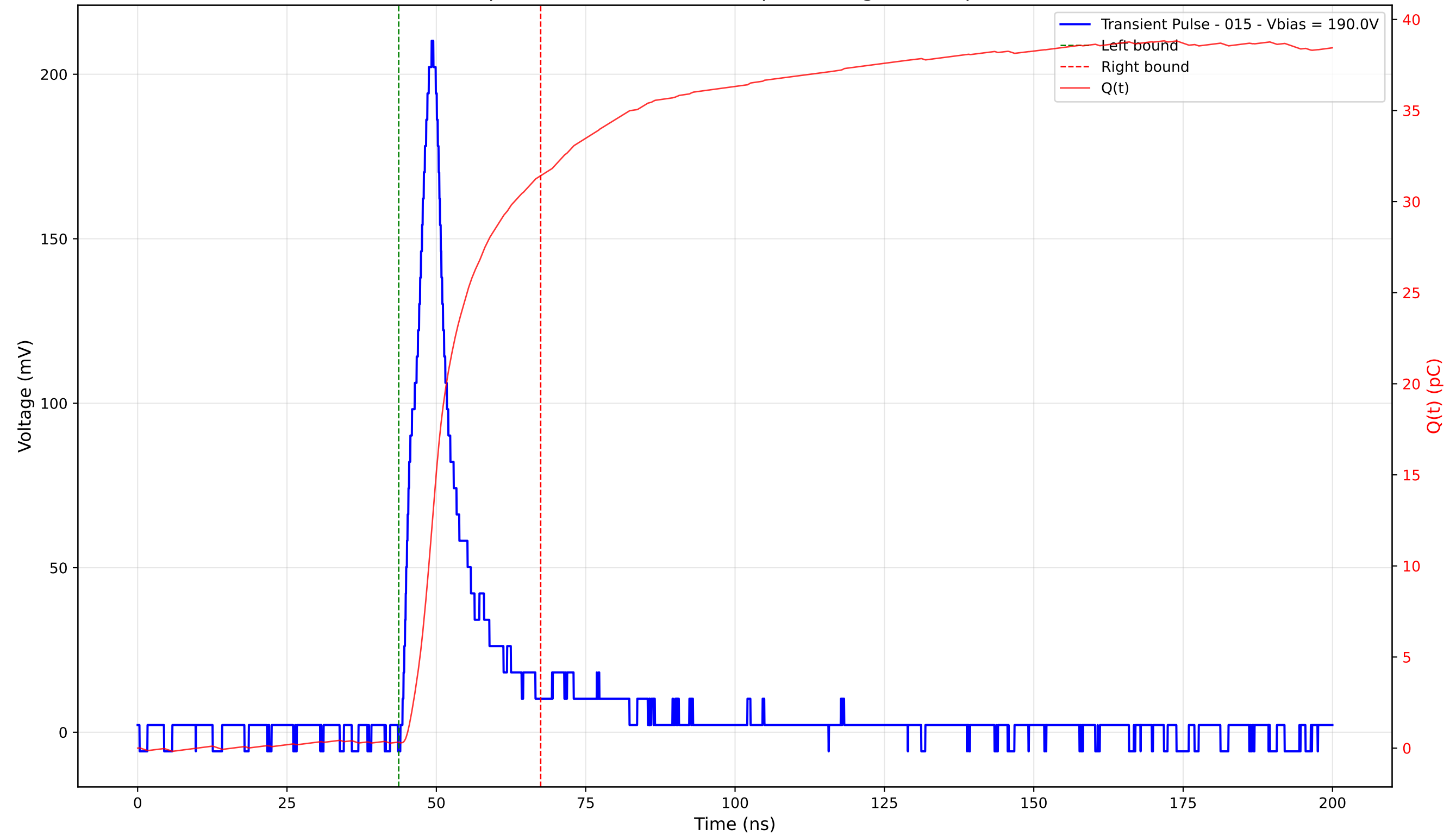
Transient Pulse - Sample: 4003 - Position: 325.0 \mu\text{m} - Charge: 31.10 pC - Rise Time: 3.89 ns
