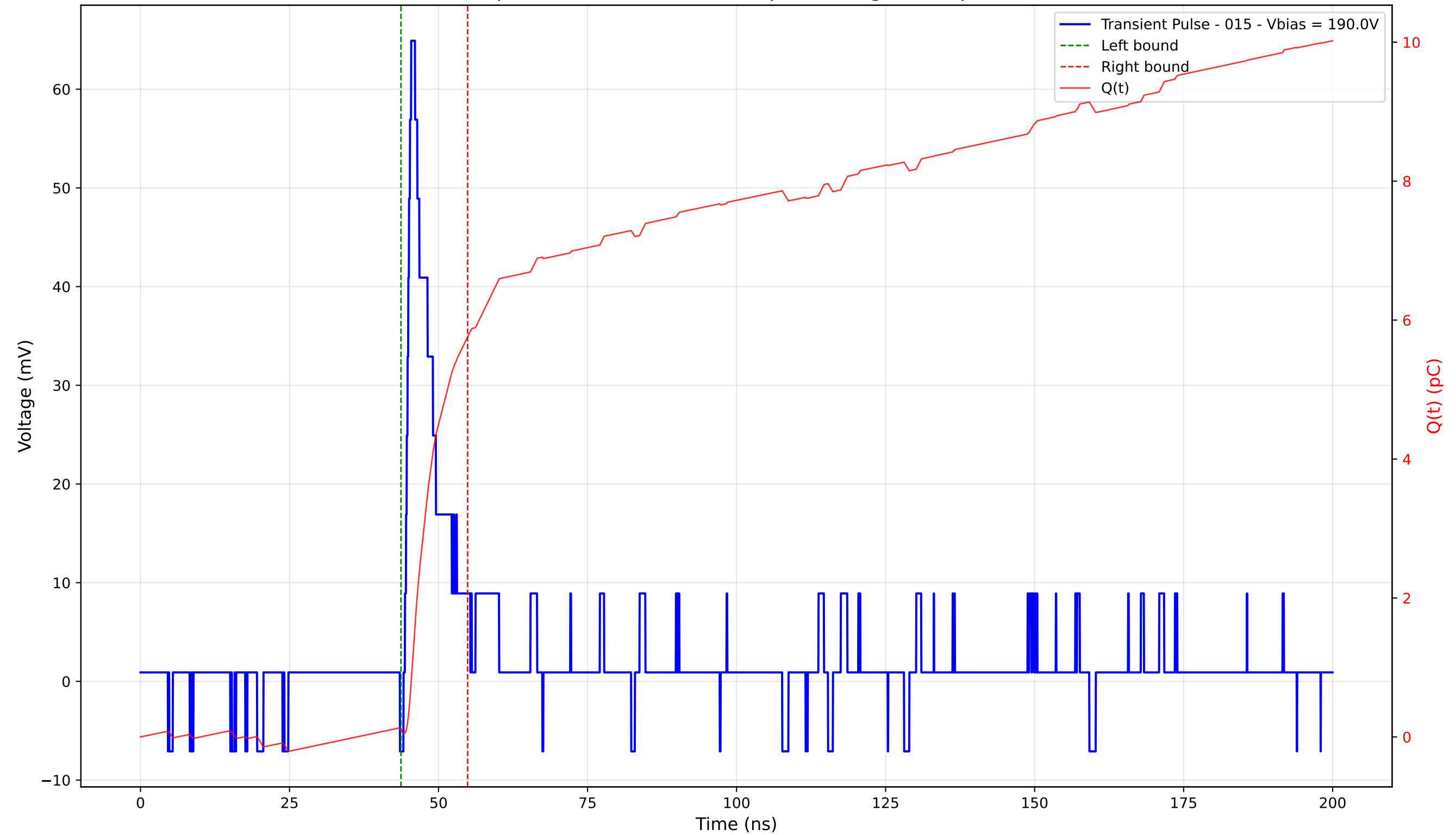
Transient Pulse - Sample: 4003 - Position: 385.0 \mu\text{m} - Charge: 5.66 pC - Rise Time: 1.05 ns
