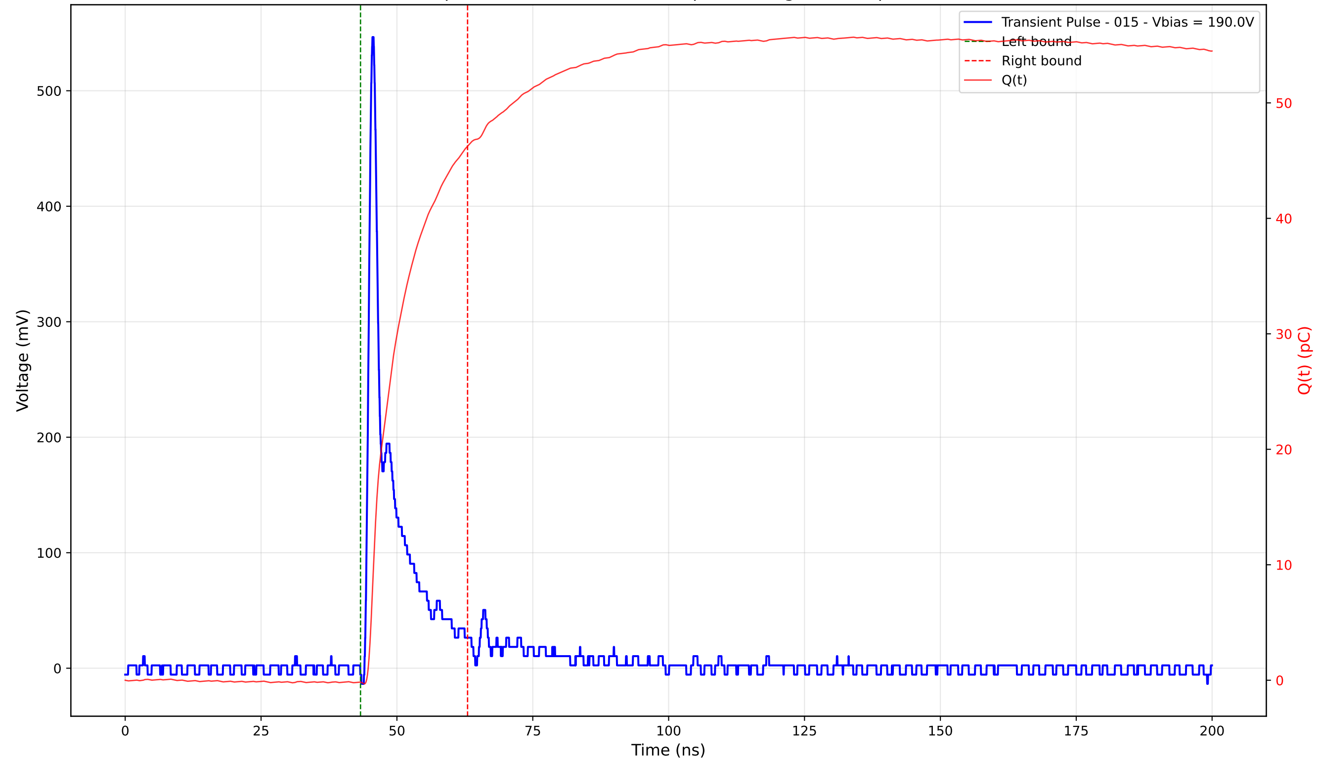
Transient Pulse - Sample: 4003 - Position: 155.0 \mu\text{m} - Charge: 46.42 pC - Rise Time: 0.97 ns
