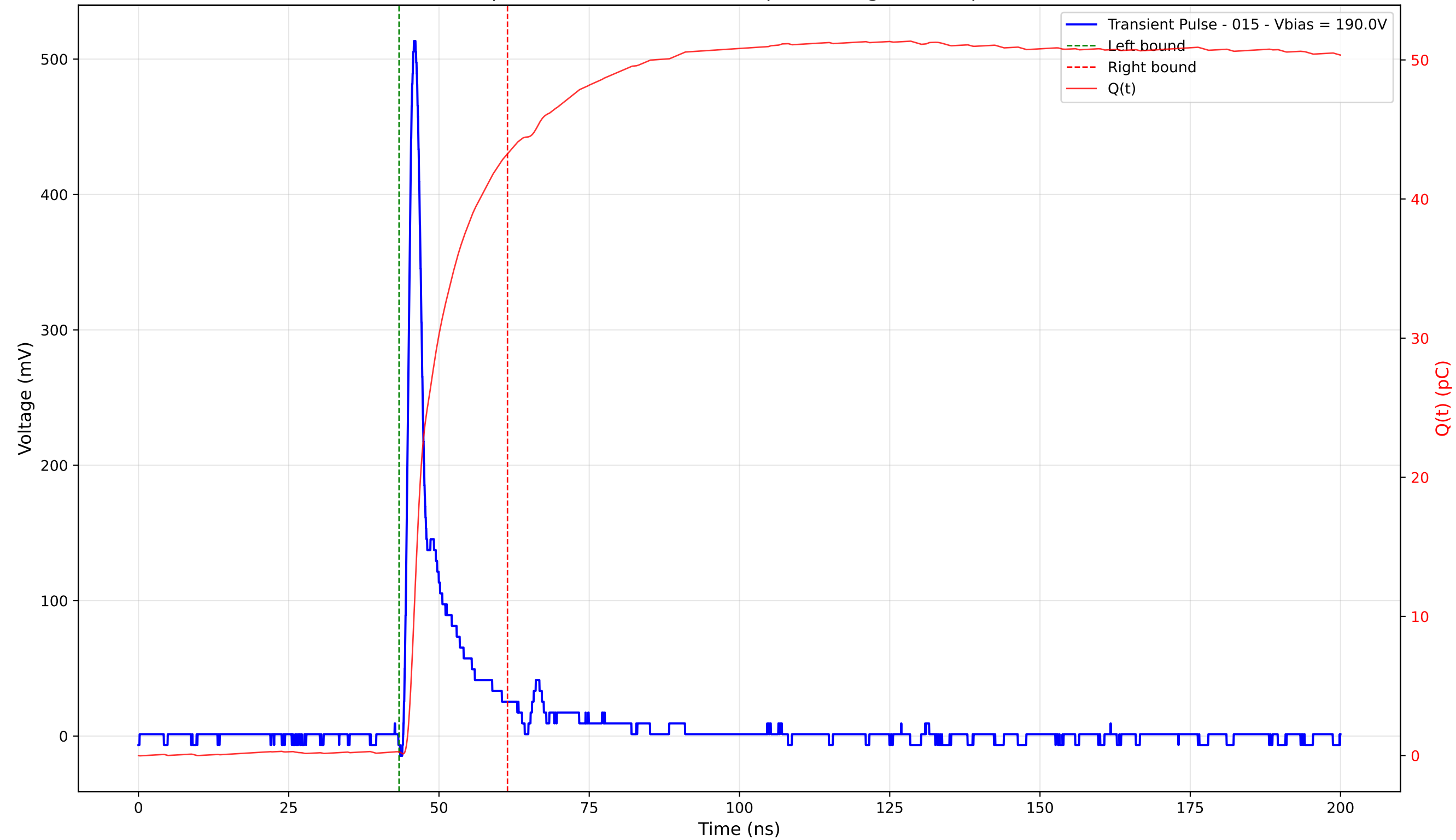
Transient Pulse - Sample: 4003 - Position: 215.0 \mu\text{m} - Charge: 42.99 pC - Rise Time: 1.14 ns
