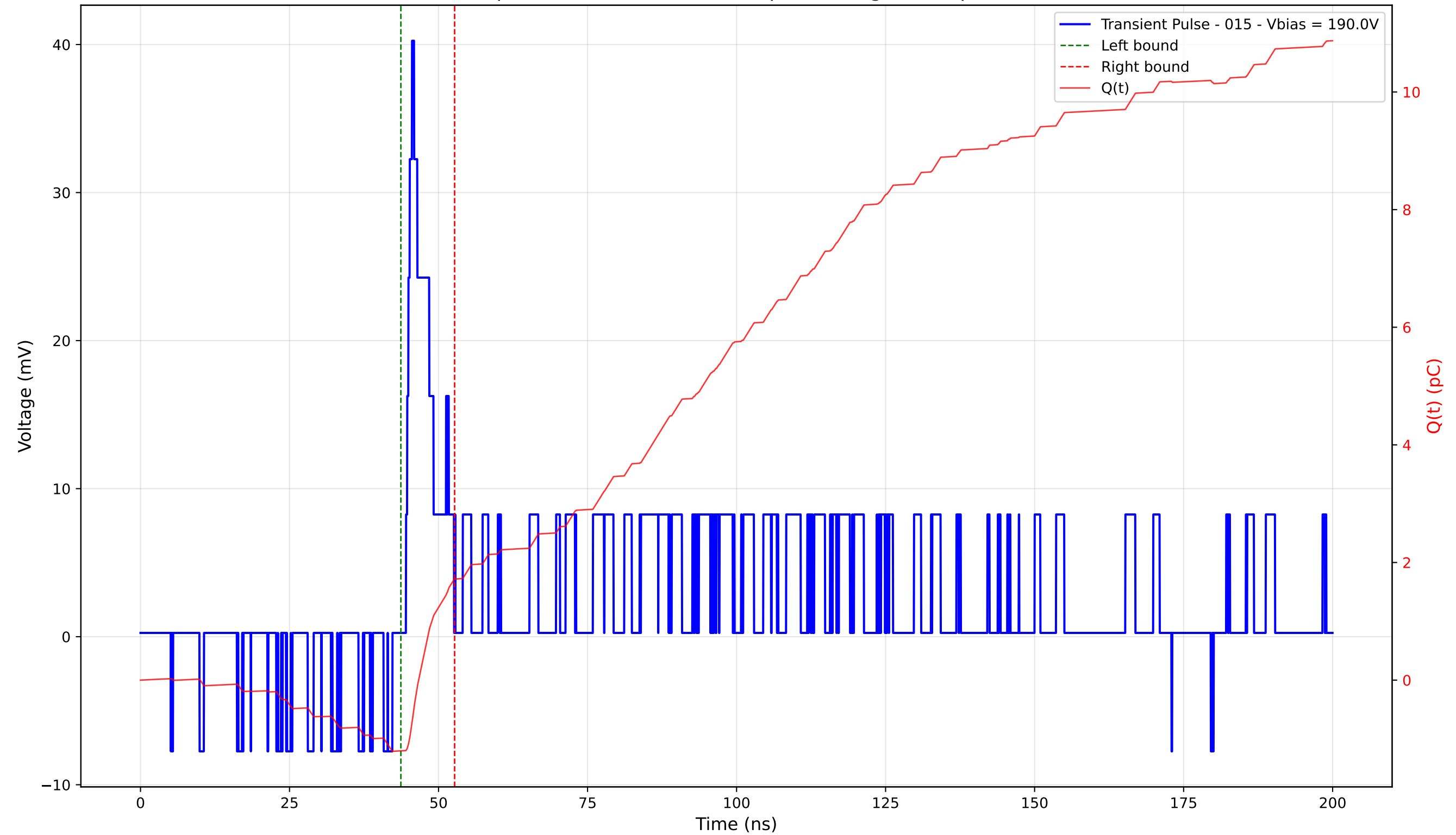
Transient Pulse - Sample: 4003 - Position: 370.0 \mu\text{m} - Charge: 2.92 pC - Rise Time: 1.01 ns
