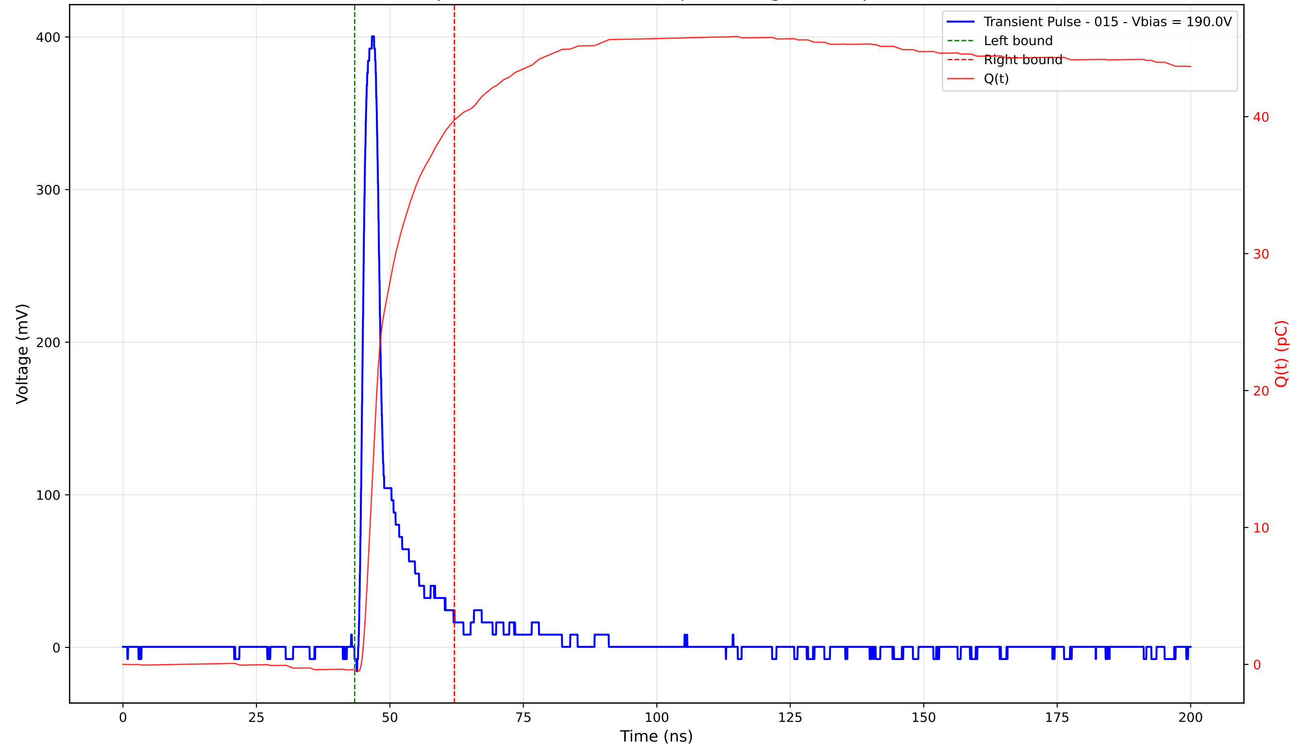
Transient Pulse - Sample: 4003 - Position: 260.0 \mu\text{m} - Charge: 40.16 pC - Rise Time: 1.24 ns
