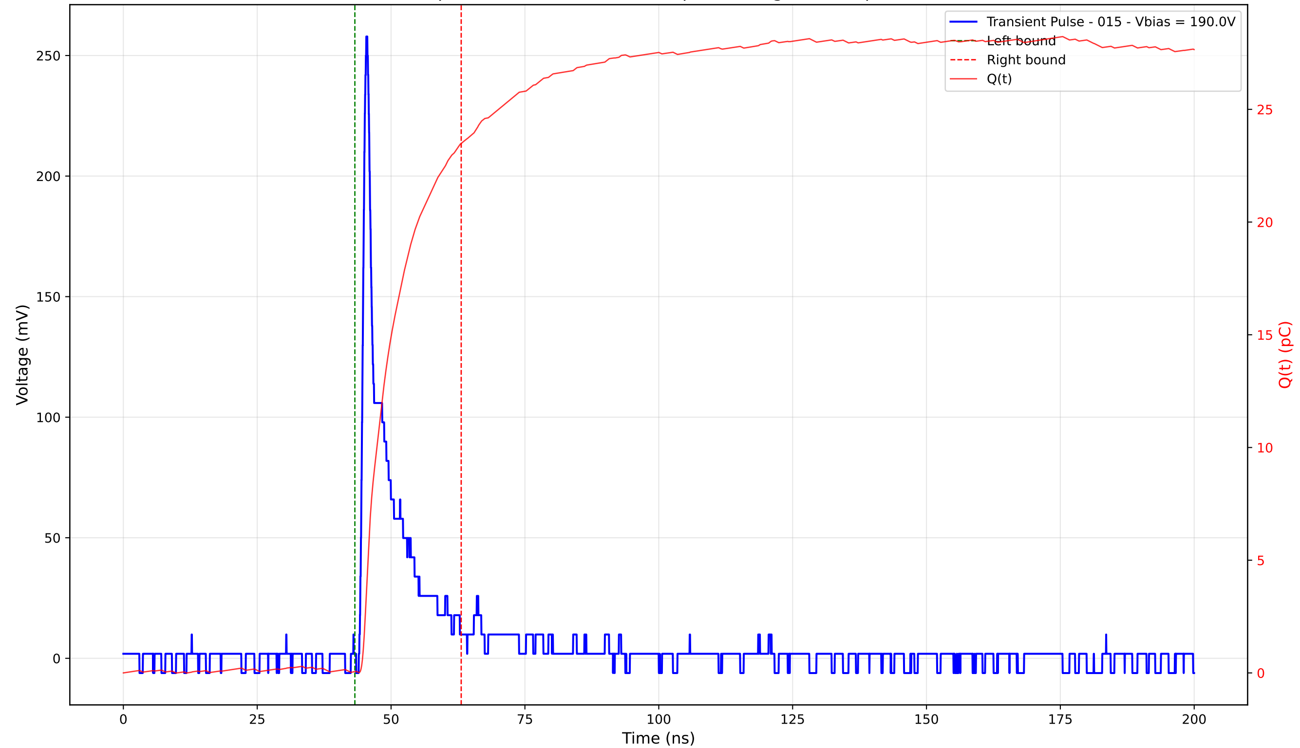
Transient Pulse - Sample: 4003 - Position: 100.0 \mu\text{m} - Charge: 23.43 pC - Rise Time: 0.90 ns
