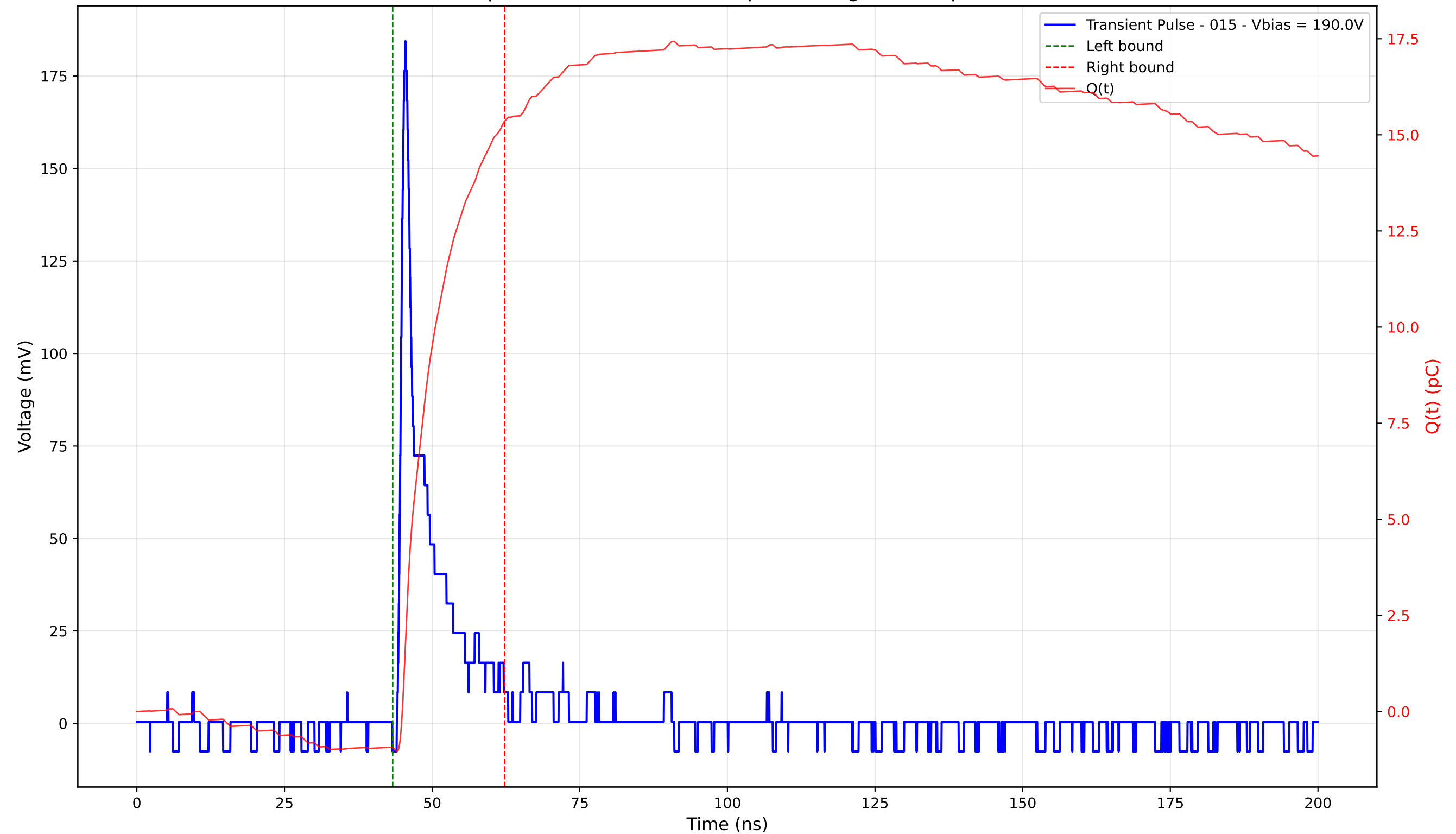
Transient Pulse - Sample: 4003 - Position: 95.0 \mu\text{m} - Charge: 16.30 pC - Rise Time: 0.91 ns
