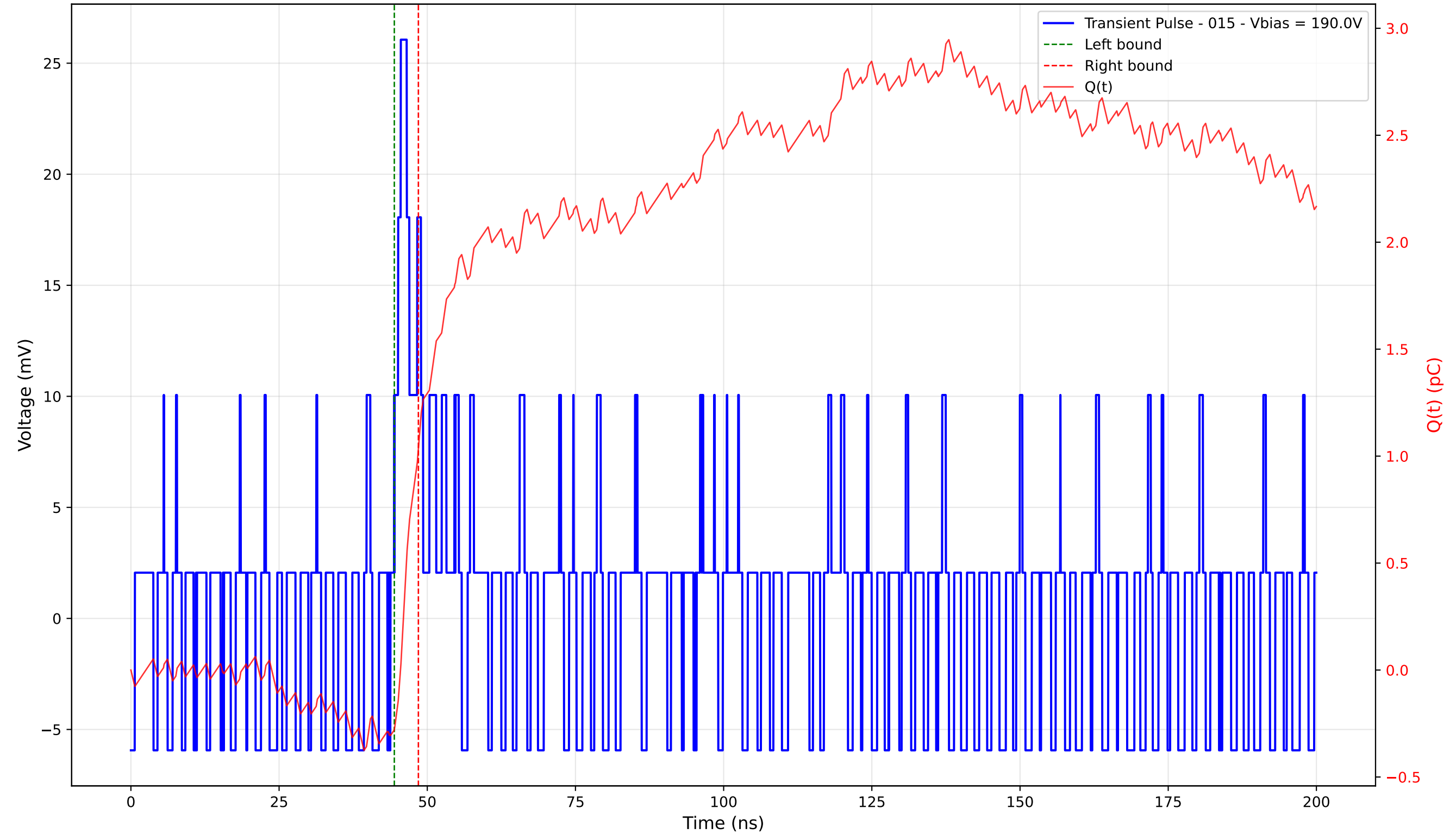
Transient Pulse - Sample: 4003 - Position: 25.0 \mu\text{m} - Charge: 1.31 pC - Rise Time: 1.06 ns
