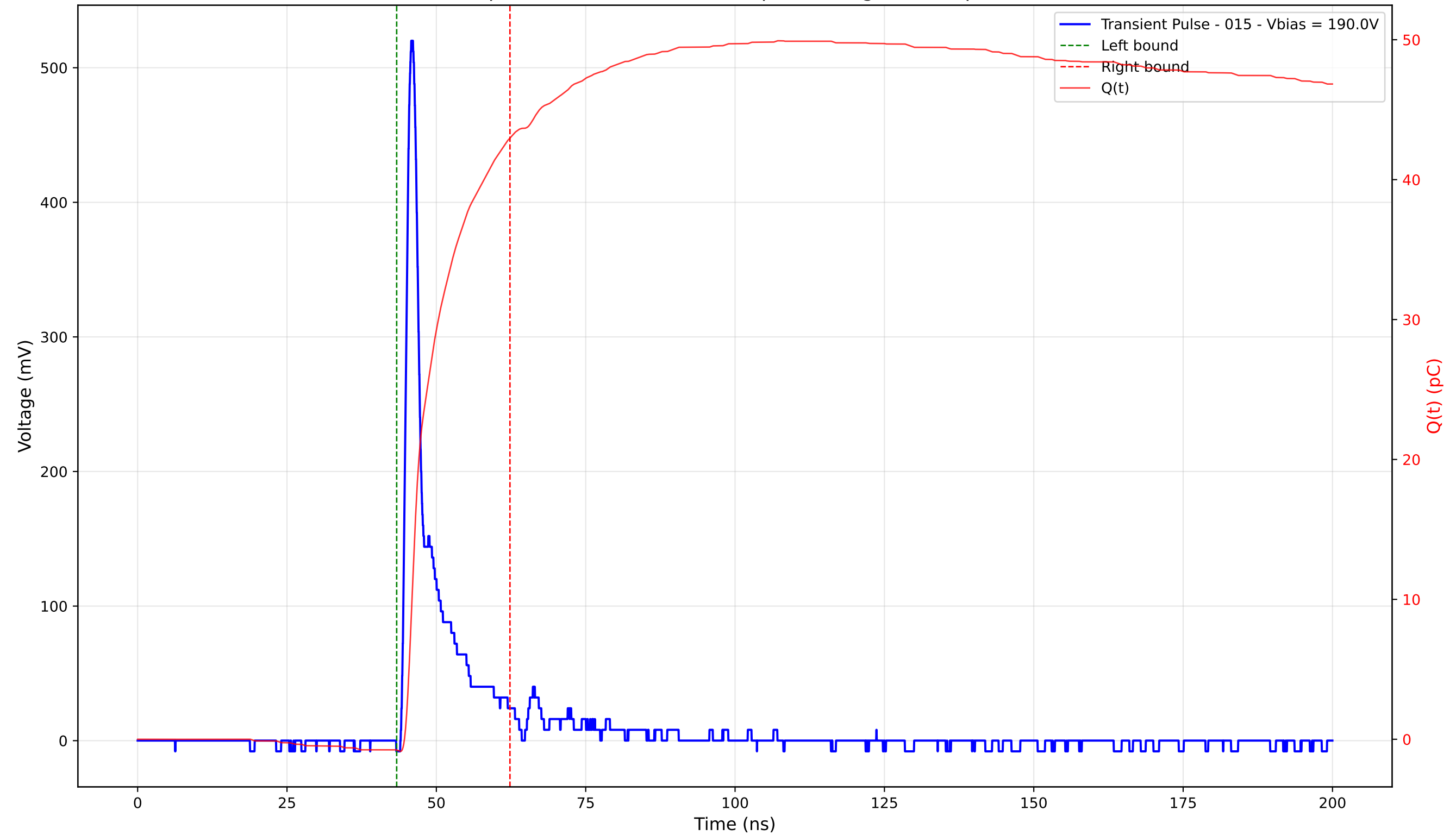
Transient Pulse - Sample: 4003 - Position: 210.0 \mu\text{m} - Charge: 43.74 pC - Rise Time: 1.15 ns
