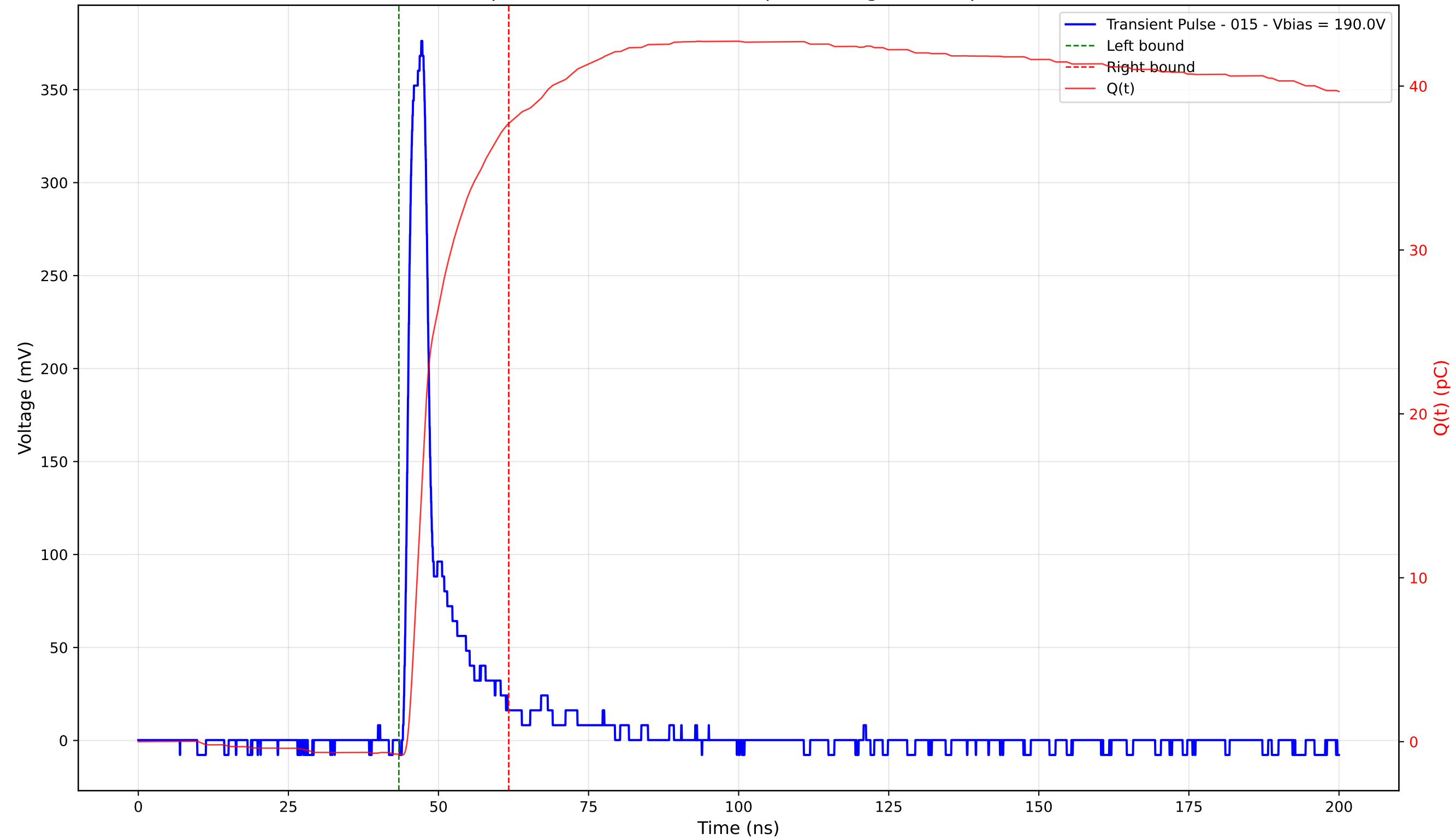
Transient Pulse - Sample: 4003 - Position: 270.0 \mu\text{m} - Charge: 38.47 pC - Rise Time: 1.41 ns
