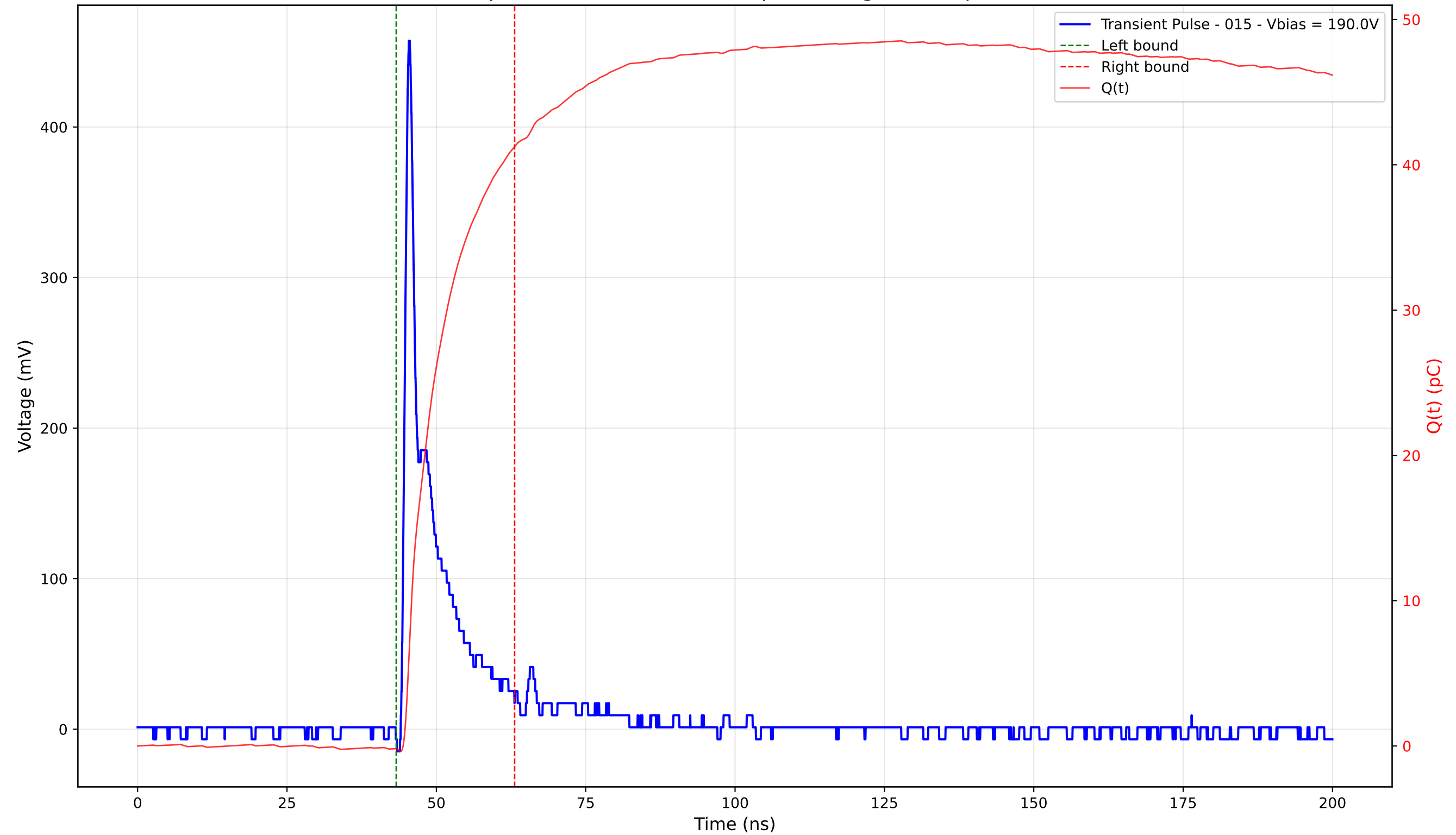
Transient Pulse - Sample: 4003 - Position: 115.0 \mu\text{m} - Charge: 41.44 pC - Rise Time: 0.91 ns
