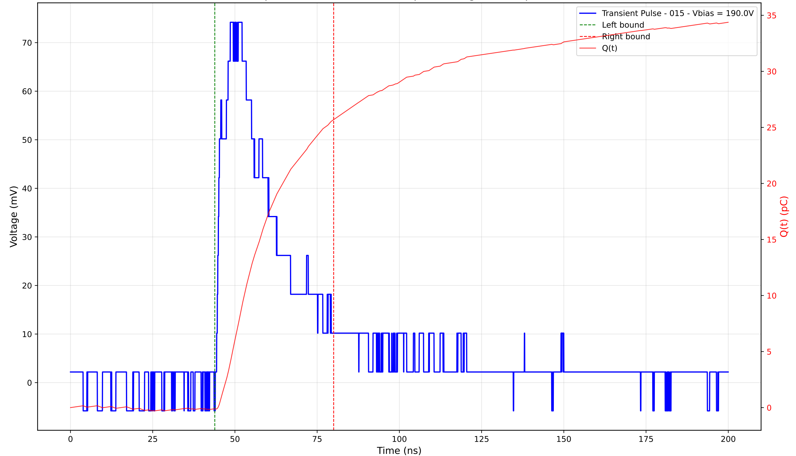
Transient Pulse - Sample: 4003 - Position: 335.0 \mu\text{m} - Charge: 25.81 pC - Rise Time: 4.15 ns
