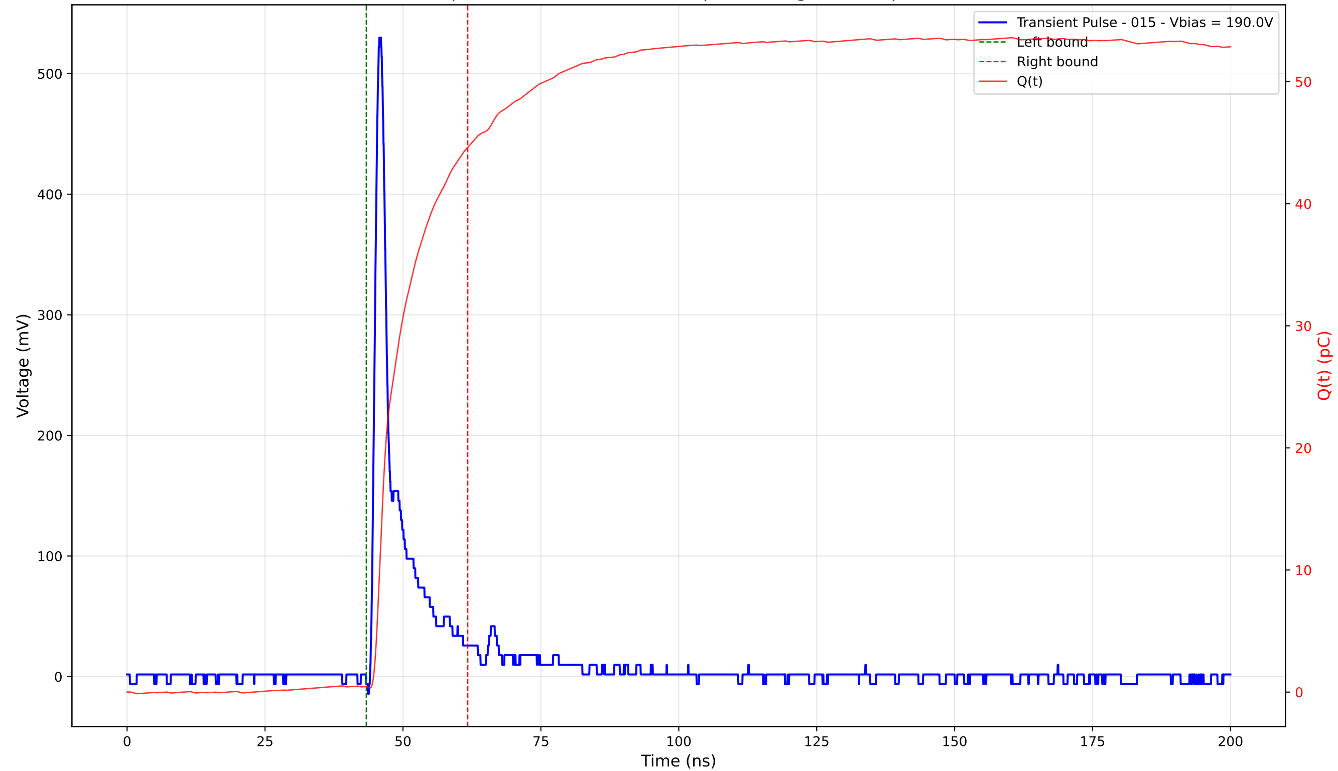
Transient Pulse - Sample: 4003 - Position: 205.0 \mu\text{m} - Charge: 44.16 pC - Rise Time: 1.09 ns
