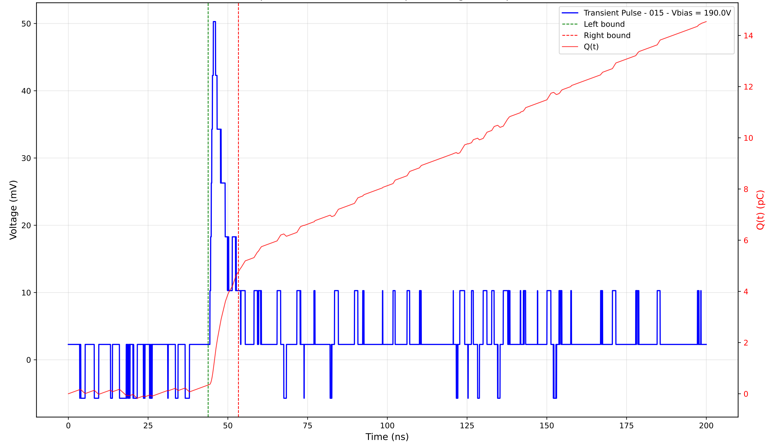
Transient Pulse - Sample: 4003 - Position: 380.0 \mu\text{m} - Charge: 4.43 pC - Rise Time: 1.07 ns
