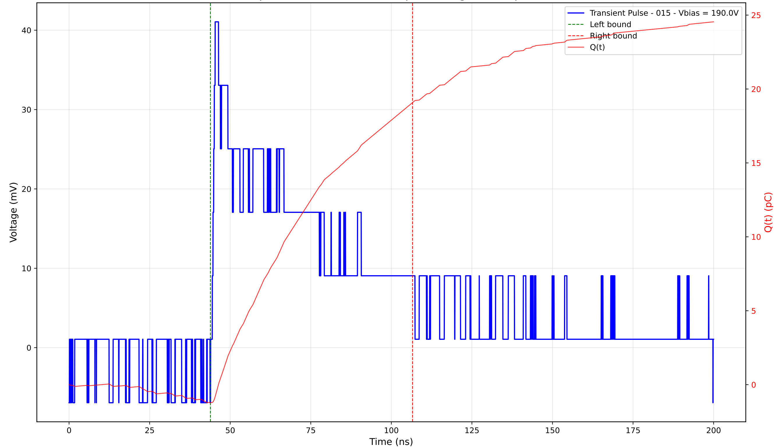
Transient Pulse - Sample: 4003 - Position: 345.0 \mu\text{m} - Charge: 20.30 pC - Rise Time: 0.89 ns
