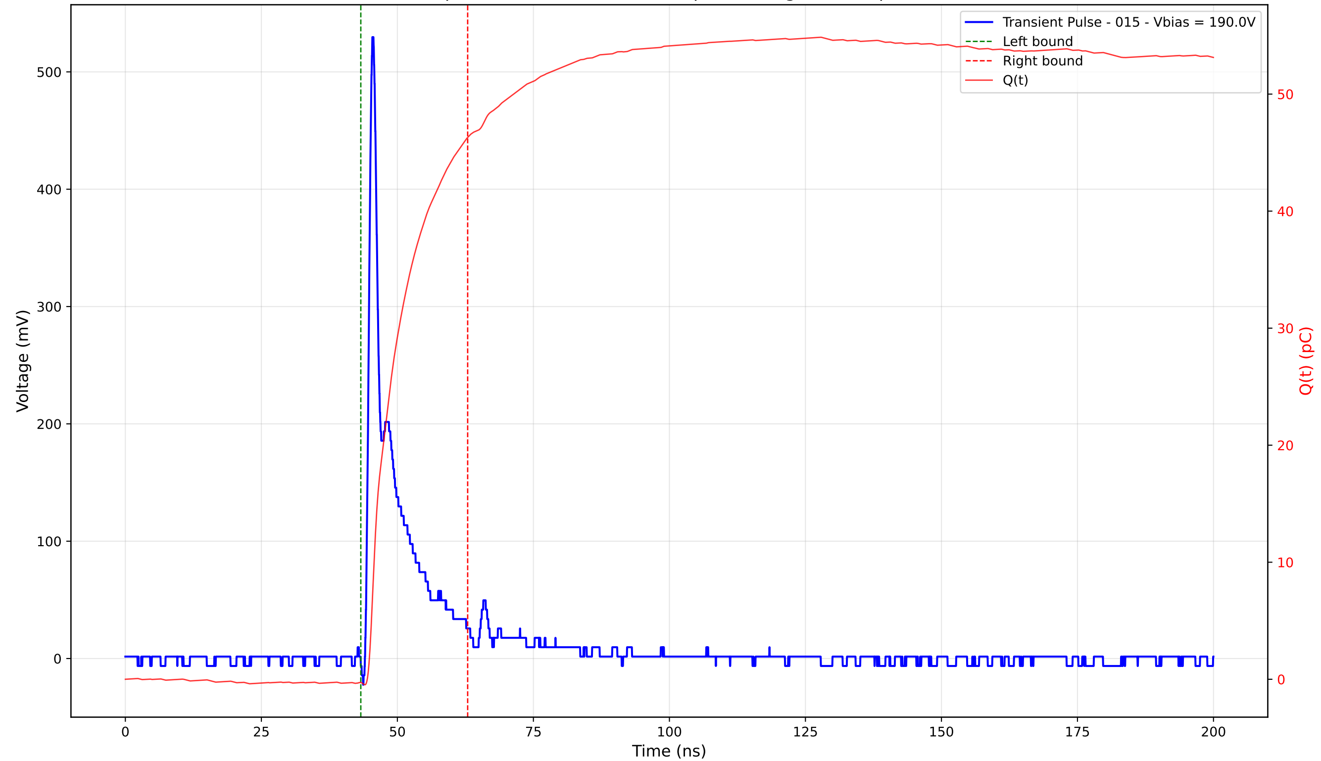
Transient Pulse - Sample: 4003 - Position: 135.0 \mu\text{m} - Charge: 46.58 pC - Rise Time: 0.91 ns
