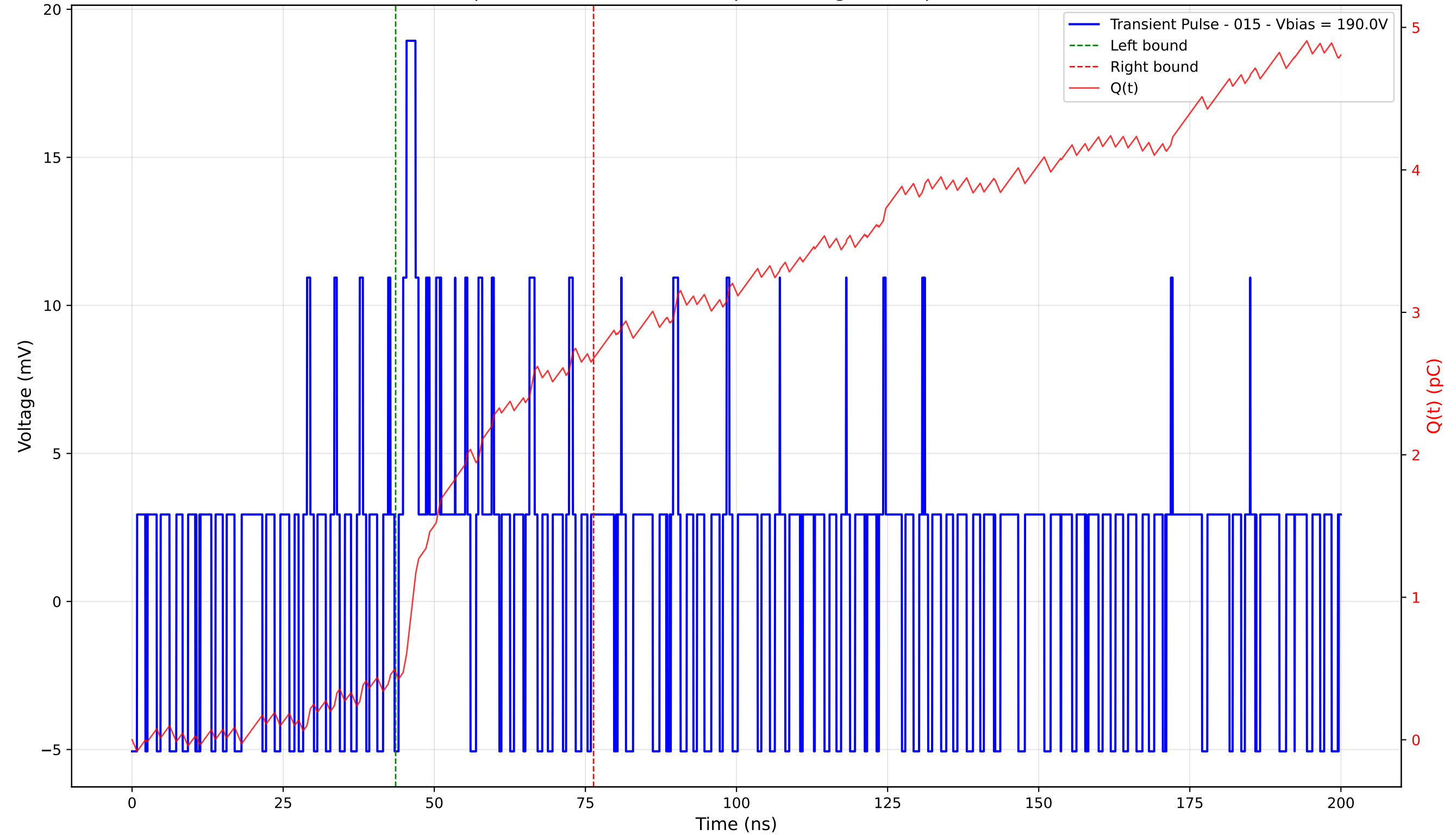
Transient Pulse - Sample: 4003 - Position: 75.0 \mu\text{m} - Charge: 2.20 pC - Rise Time: 0.00 ns (N/A)
