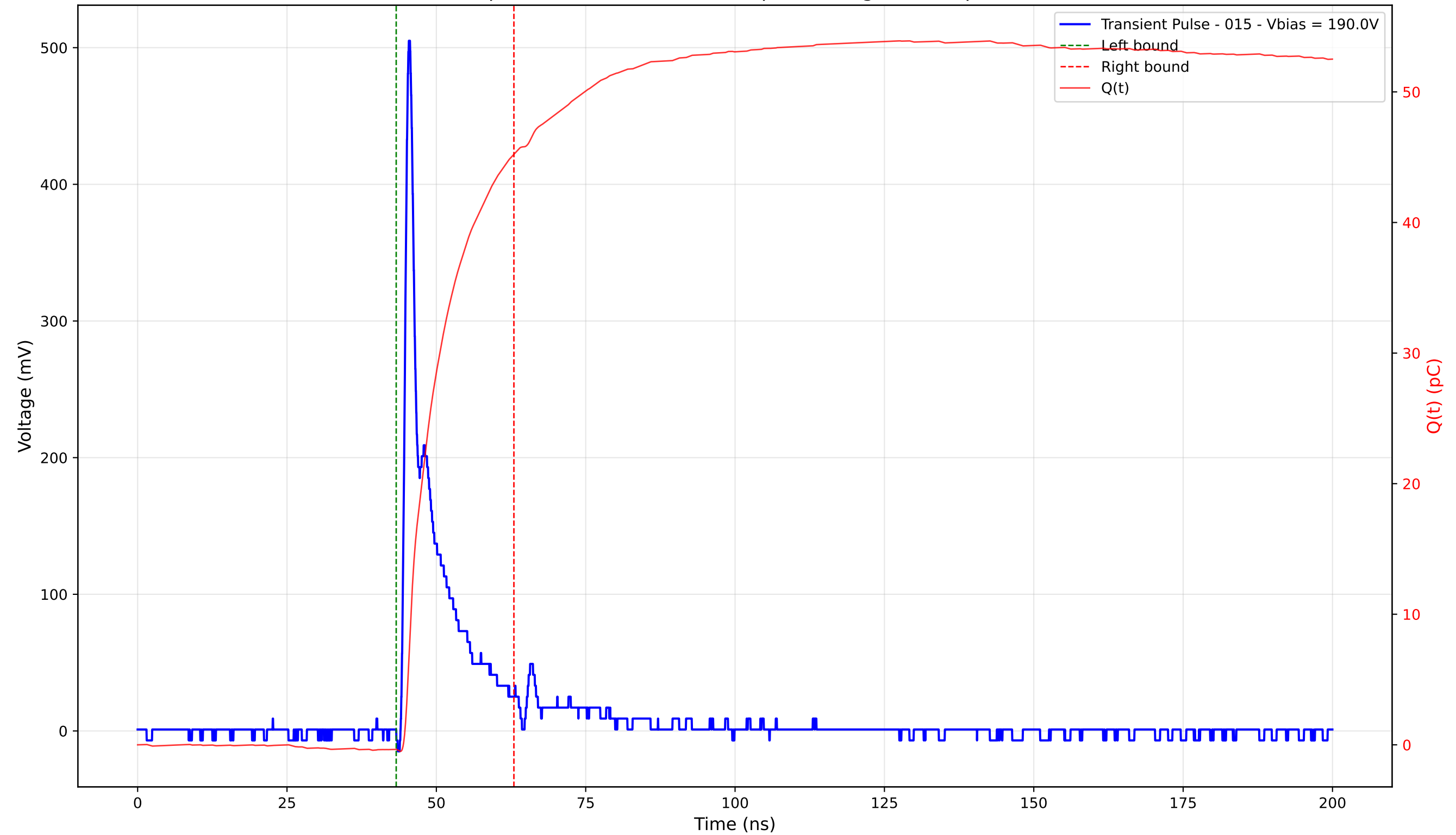
Transient Pulse - Sample: 4003 - Position: 125.0 \mu\text{m} - Charge: 45.57 pC - Rise Time: 0.91 ns
