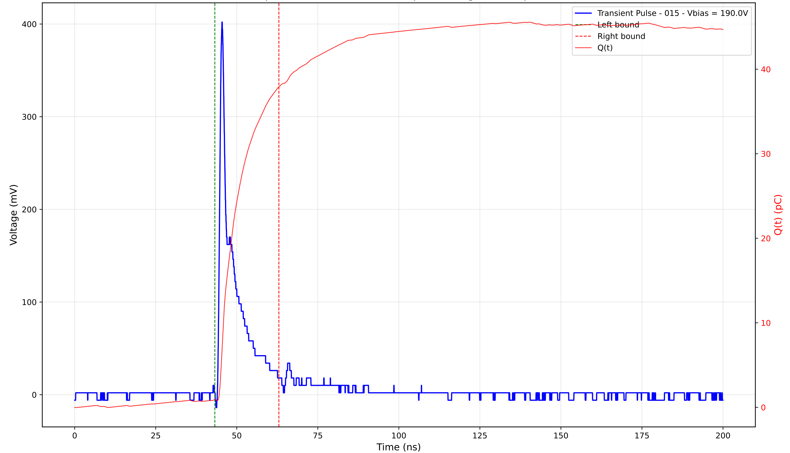
Transient Pulse - Sample: 4003 - Position: 110.0 \mu\text{m} - Charge: 37.01 pC - Rise Time: 0.92 ns
