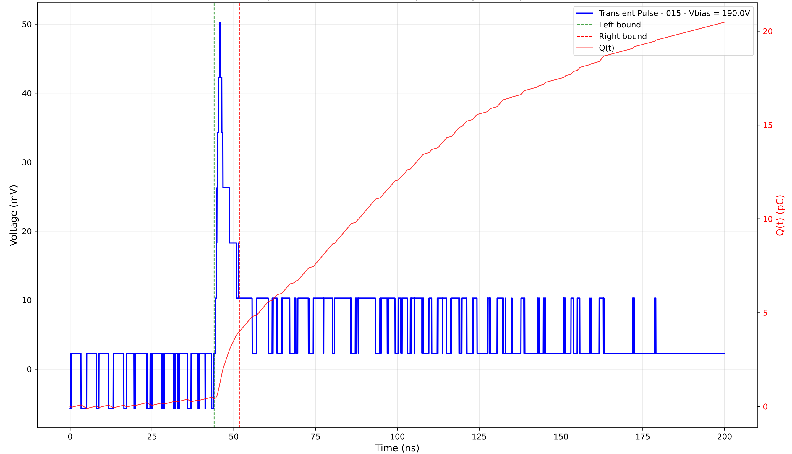
Transient Pulse - Sample: 4003 - Position: 360.0 \mu\text{m} - Charge: 3.57 pC - Rise Time: 1.29 ns
