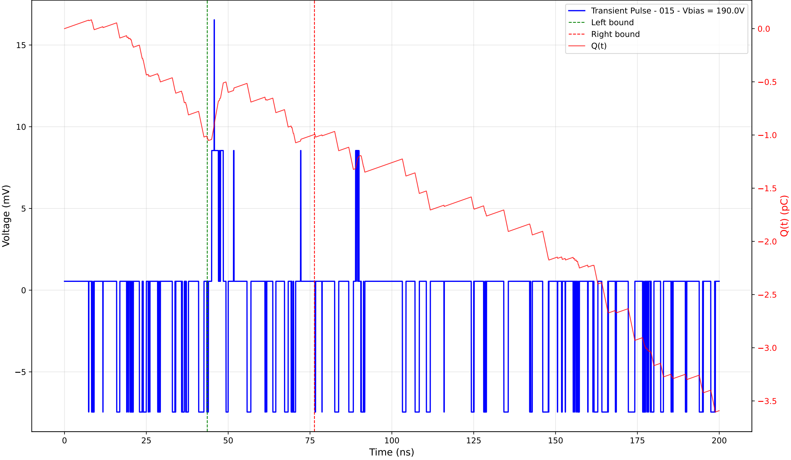
Transient Pulse - Sample: 4003 - Position: 10.0 \mu\text{m} - Charge: 0.04 pC - Rise Time: 0.78 ns
