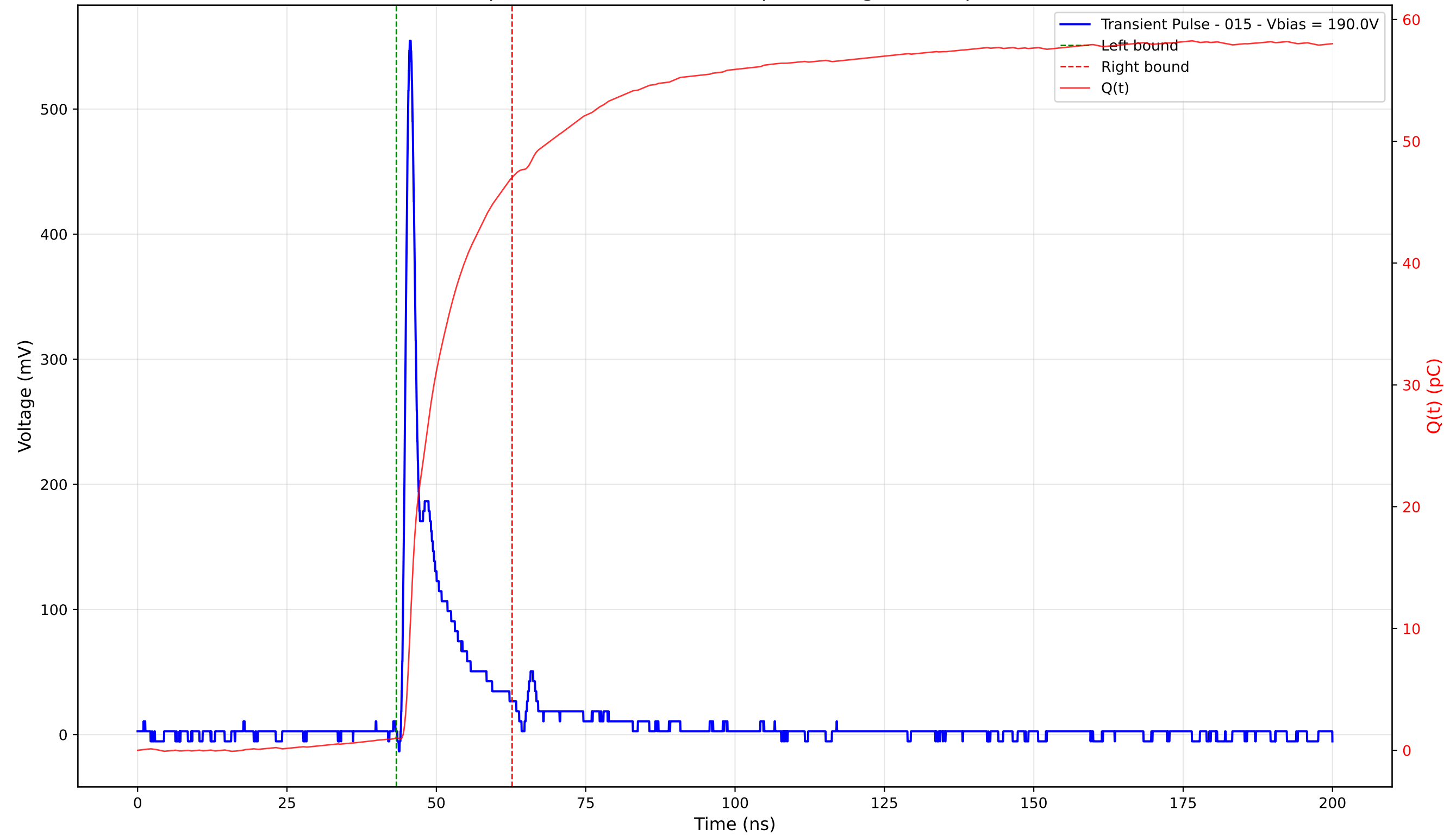
Transient Pulse - Sample: 4003 - Position: 165.0 \mu\text{m} - Charge: 46.01 pC - Rise Time: 0.99 ns
