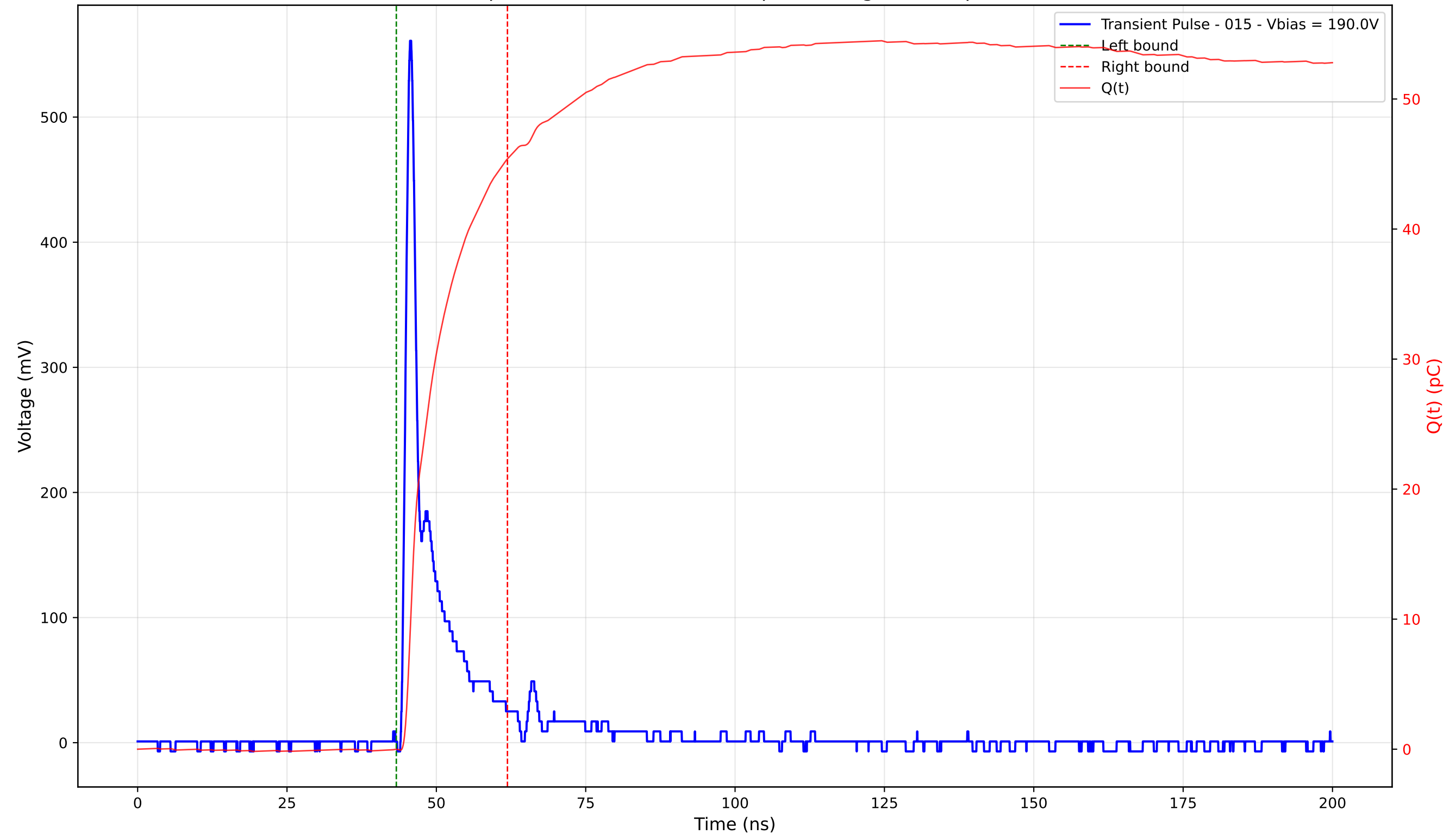
Transient Pulse - Sample: 4003 - Position: 175.0 \mu\text{m} - Charge: 45.40 pC - Rise Time: 1.00 ns
