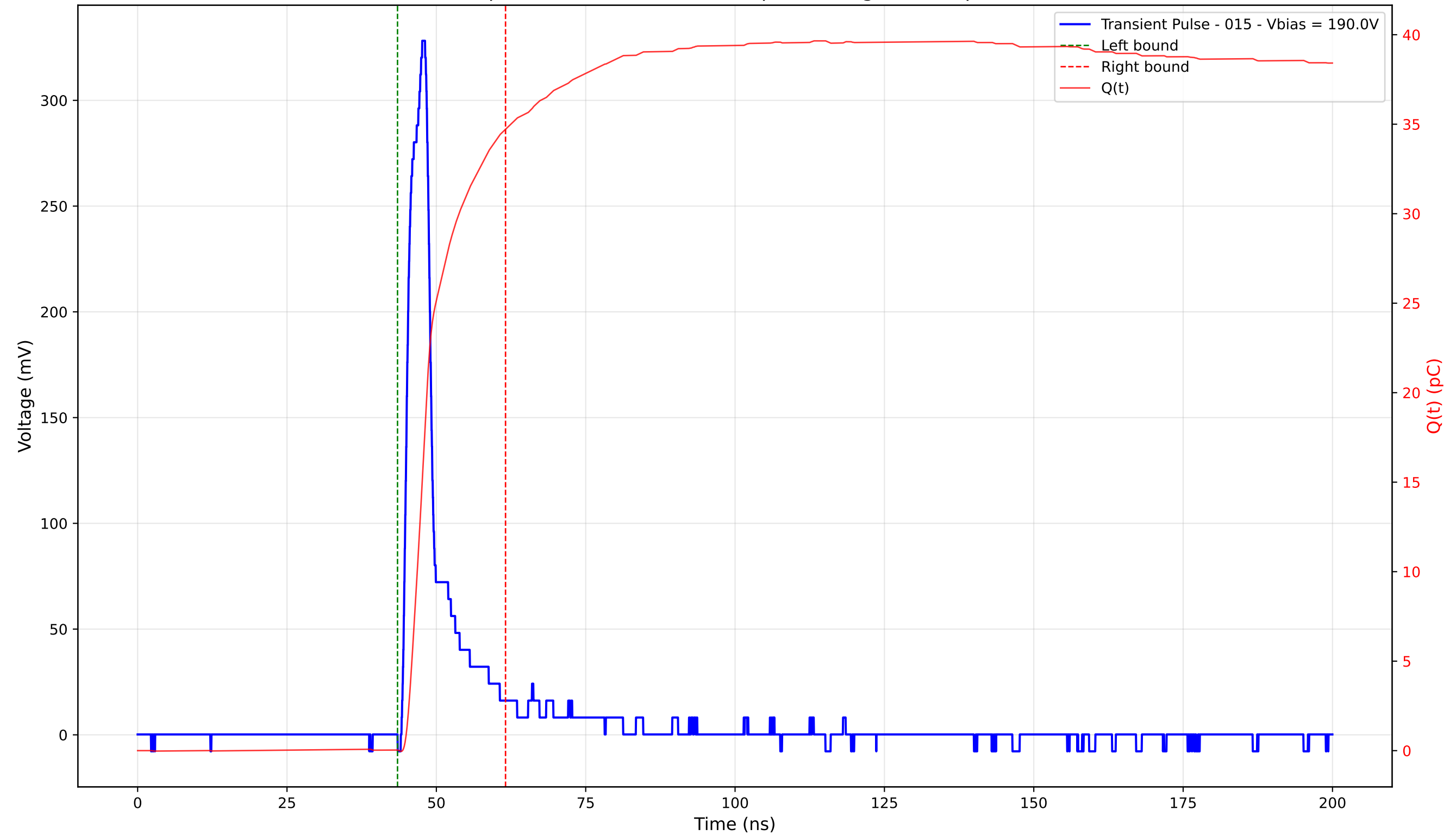
Transient Pulse - Sample: 4003 - Position: 295.0 \mu\text{m} - Charge: 34.68 pC - Rise Time: 2.54 ns
