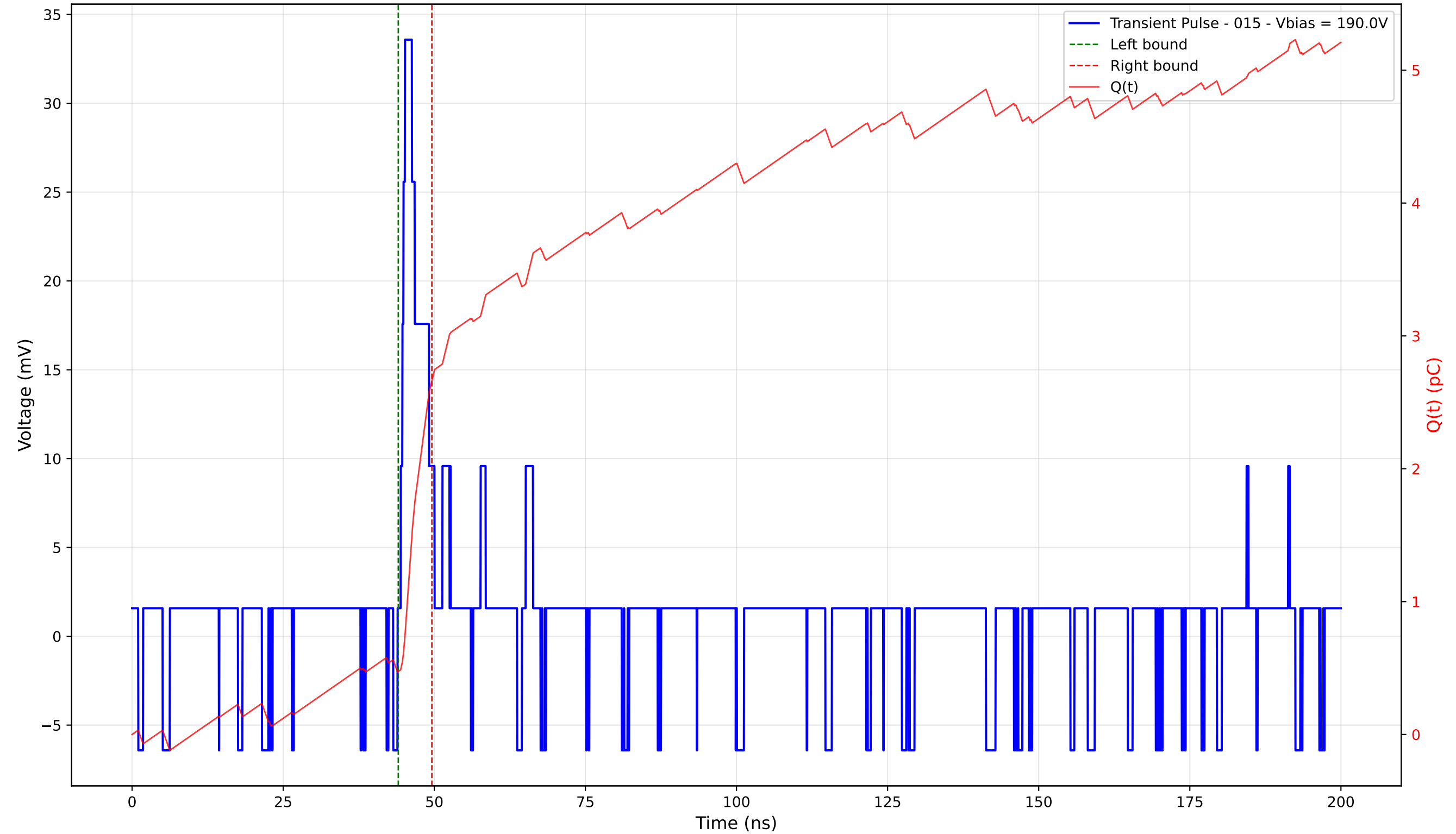
Transient Pulse - Sample: 4003 - Position: 410.0 \mu\text{m} - Charge: 2.19 pC - Rise Time: 0.72 ns
