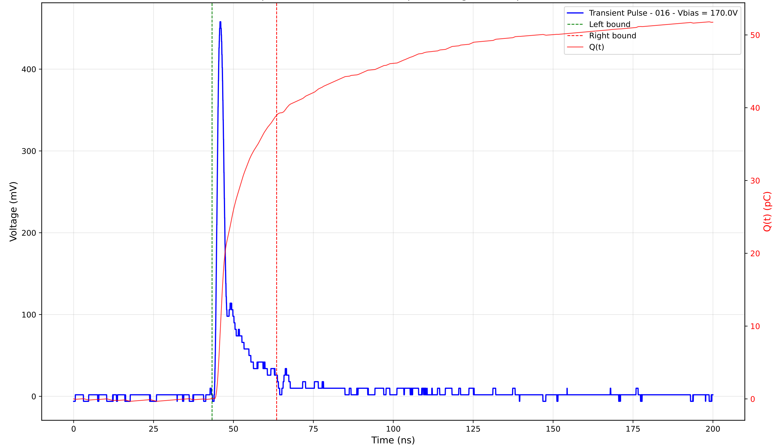
Transient Pulse - Sample: 4003 - Position: 215.0 \mu\text{m} - Charge: 38.91 pC - Rise Time: 1.15 ns
