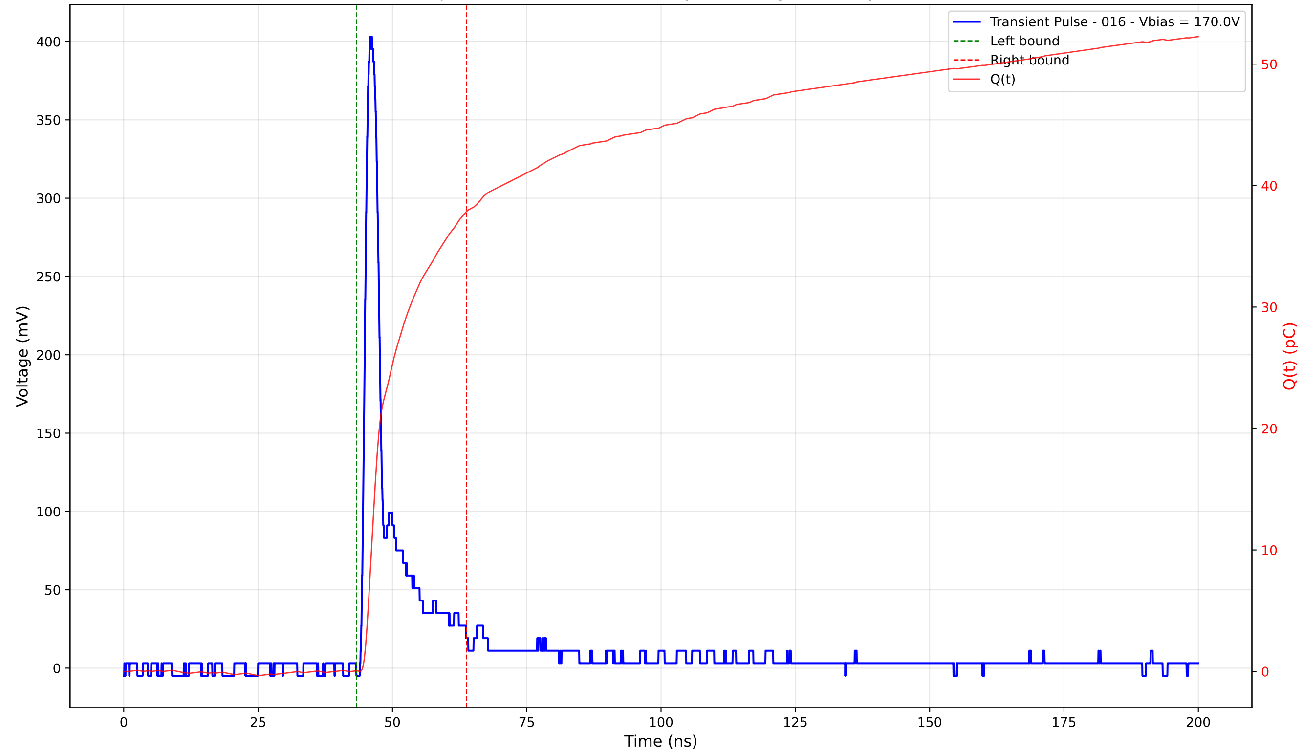
Transient Pulse - Sample: 4003 - Position: 235.0 \mu\text{m} - Charge: 37.81 pC - Rise Time: 1.15 ns
