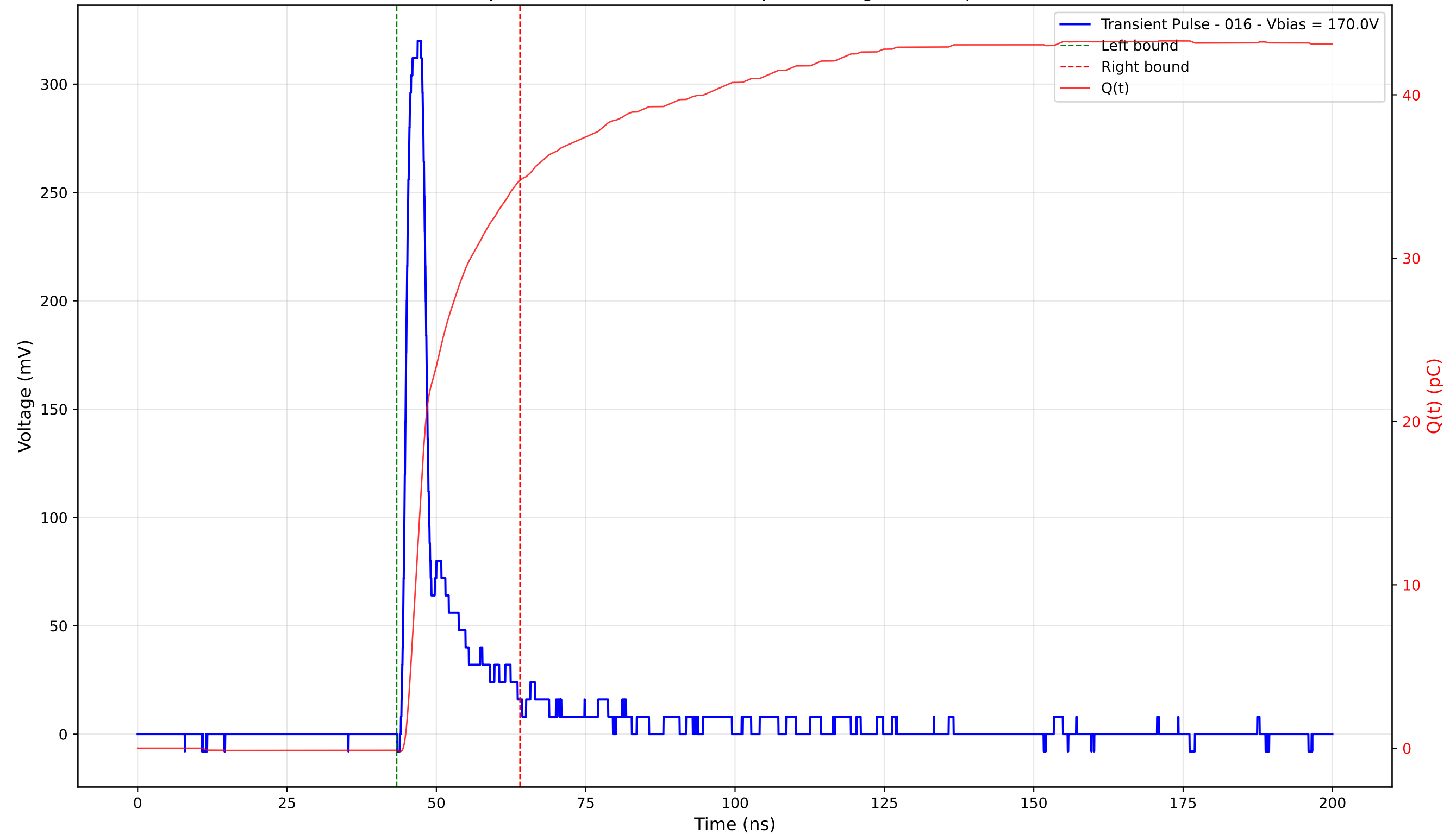
Transient Pulse - Sample: 4003 - Position: 265.0 \mu\text{m} - Charge: 34.88 pC - Rise Time: 1.26 ns
