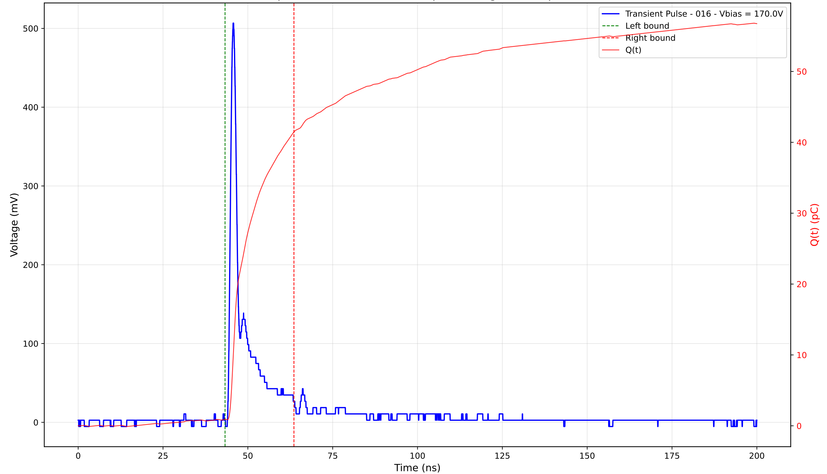
Transient Pulse - Sample: 4003 - Position: 190.0 \mu\text{m} - Charge: 40.55 pC - Rise Time: 1.05 ns
