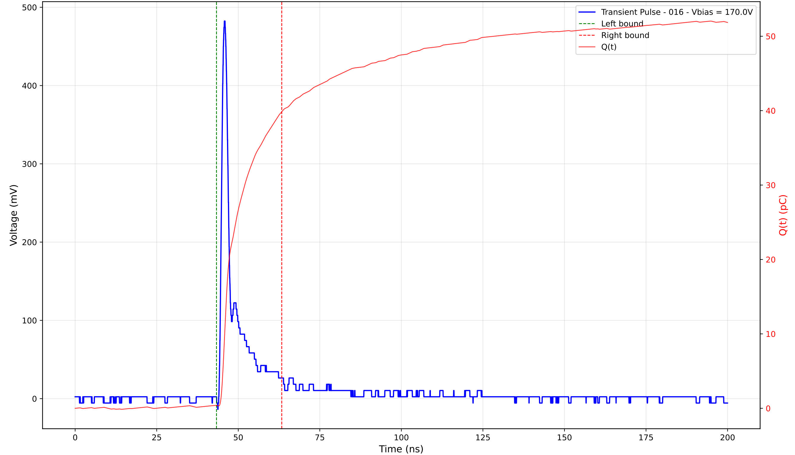
Transient Pulse - Sample: 4003 - Position: 205.0 \mu\text{m} - Charge: 39.46 pC - Rise Time: 1.08 ns
