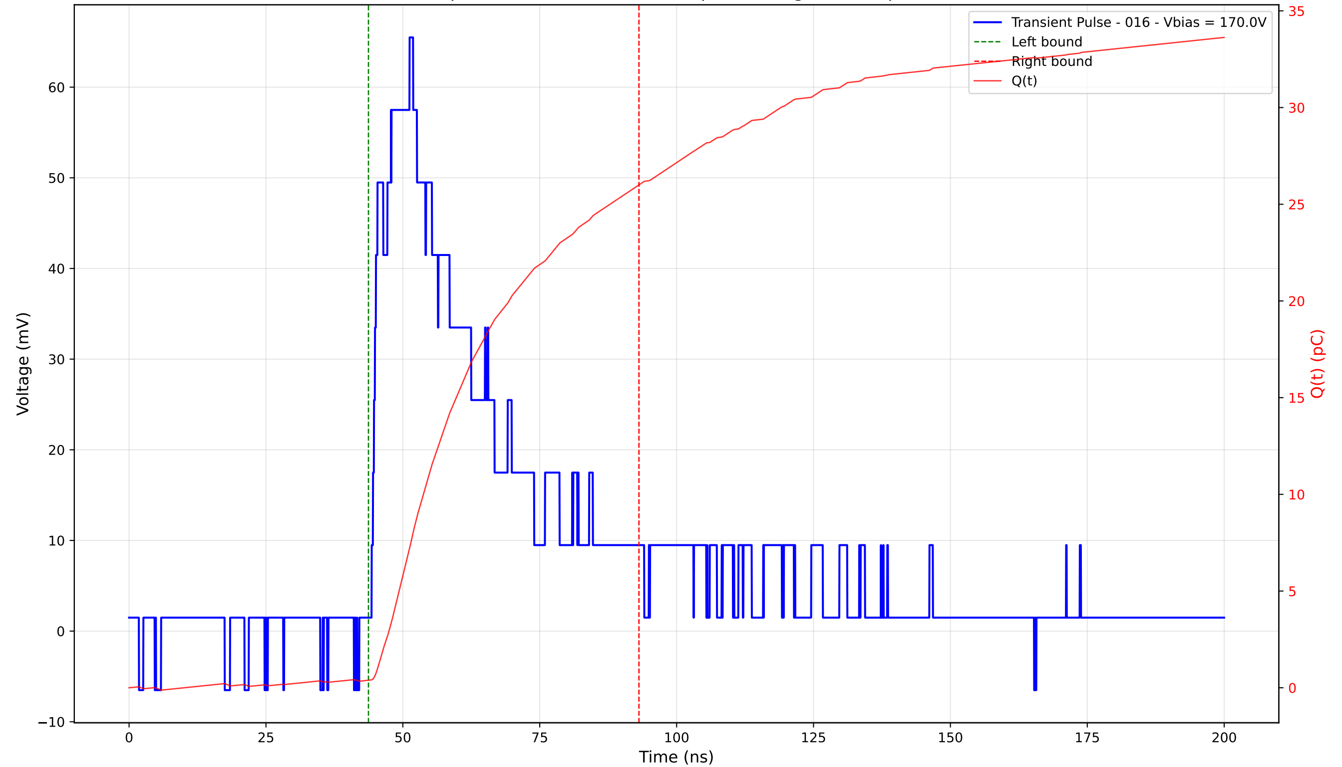
Transient Pulse - Sample: 4003 - Position: 320.0 \mu\text{m} - Charge: 25.62 pC - Rise Time: 6.93 ns
