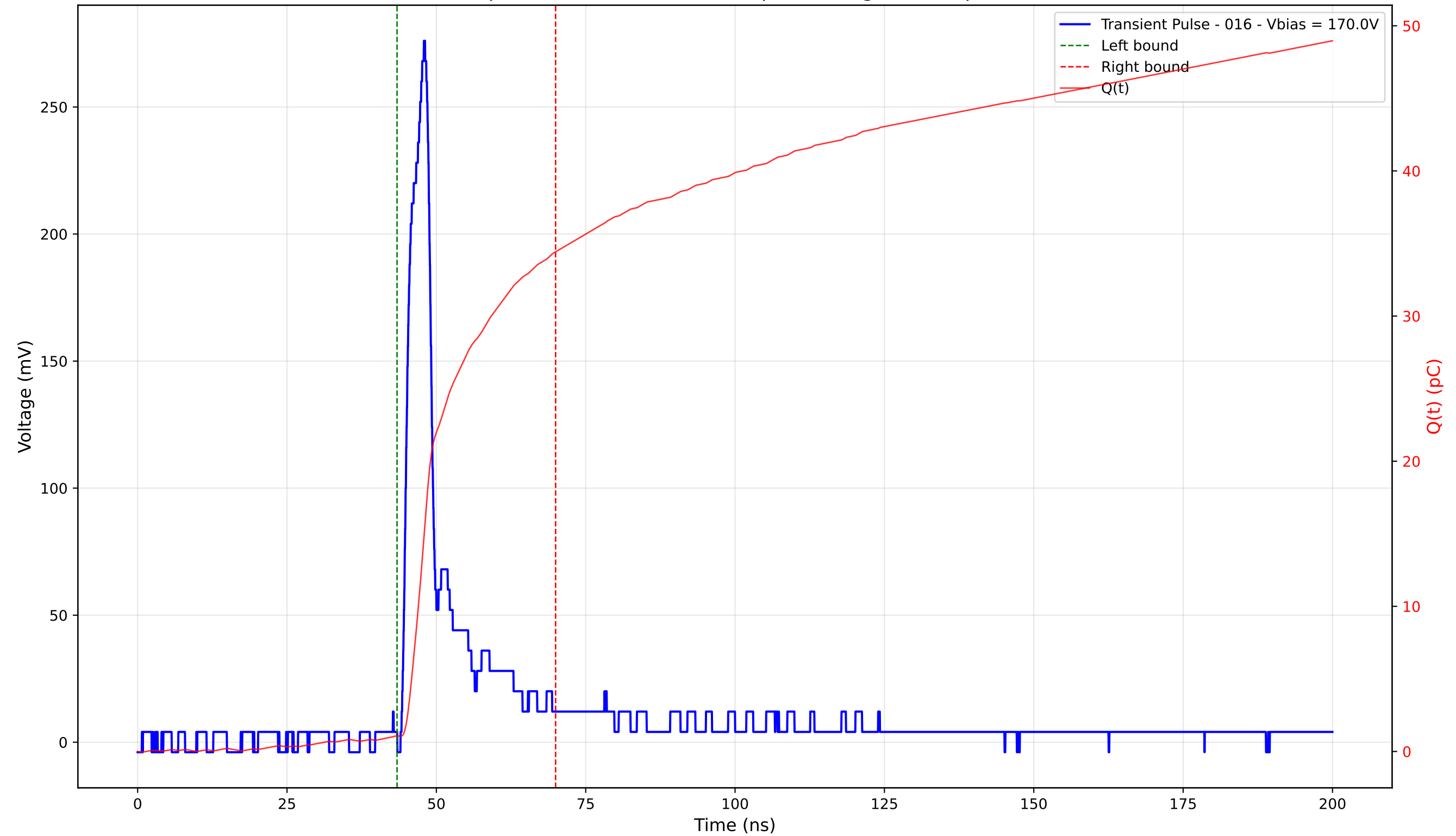
Transient Pulse - Sample: 4003 - Position: 290.0 \mu\text{m} - Charge: 33.34 pC - Rise Time: 2.92 ns
