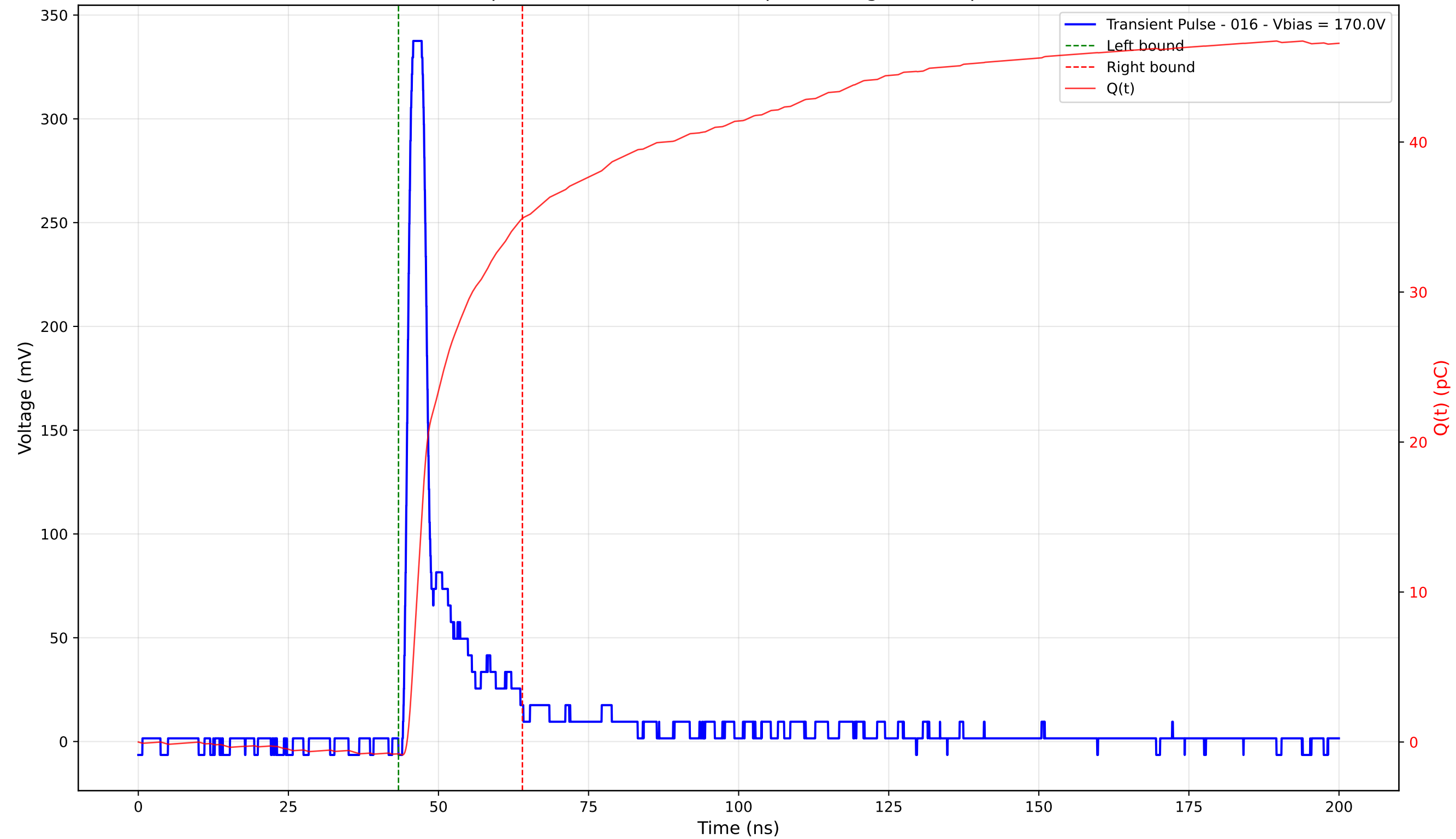
Transient Pulse - Sample: 4003 - Position: 255.0 \mu\text{m} - Charge: 35.69 pC - Rise Time: 1.12 ns
