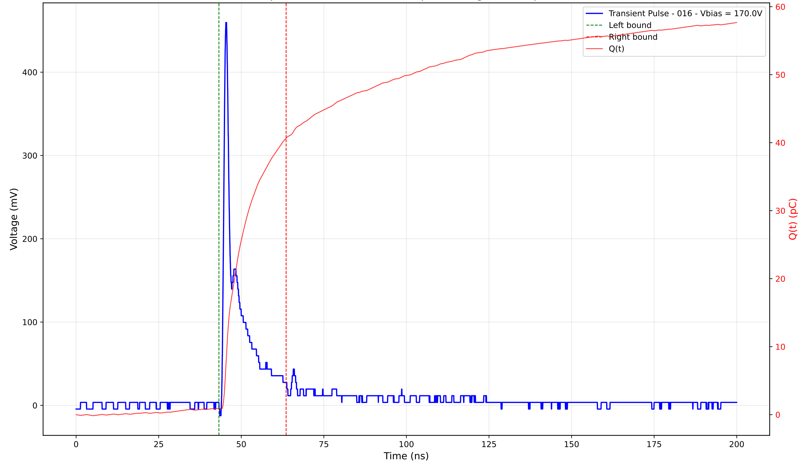
Transient Pulse - Sample: 4003 - Position: 120.0 \mu\text{m} - Charge: 39.71 pC - Rise Time: 0.88 ns
