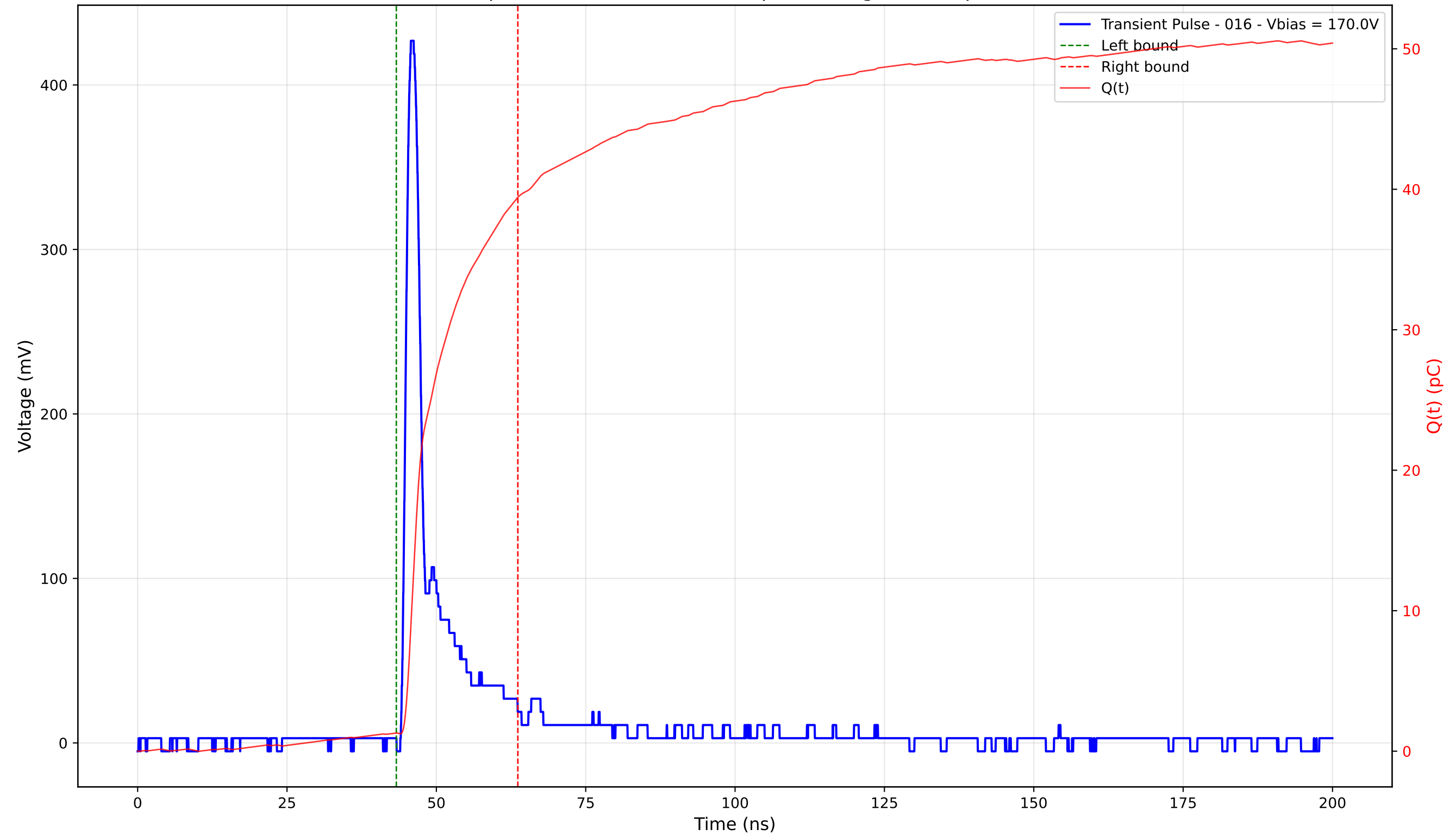
Transient Pulse - Sample: 4003 - Position: 225.0 \mu\text{m} - Charge: 38.14 pC - Rise Time: 1.14 ns
