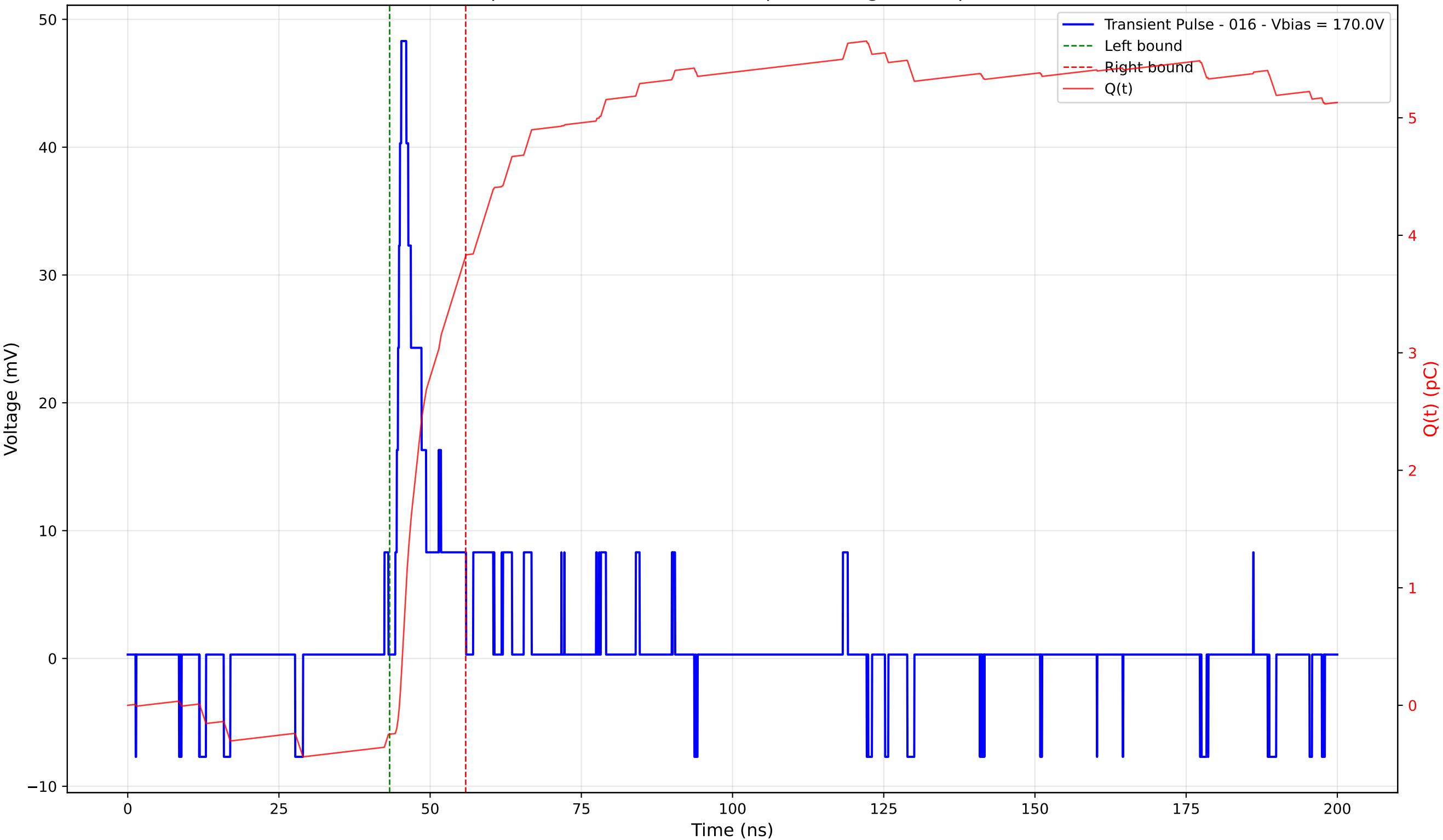
Transient Pulse - Sample: 4003 - Position: 400.0 \mu\text{m} - Charge: 4.07 pC - Rise Time: 0.99 ns
