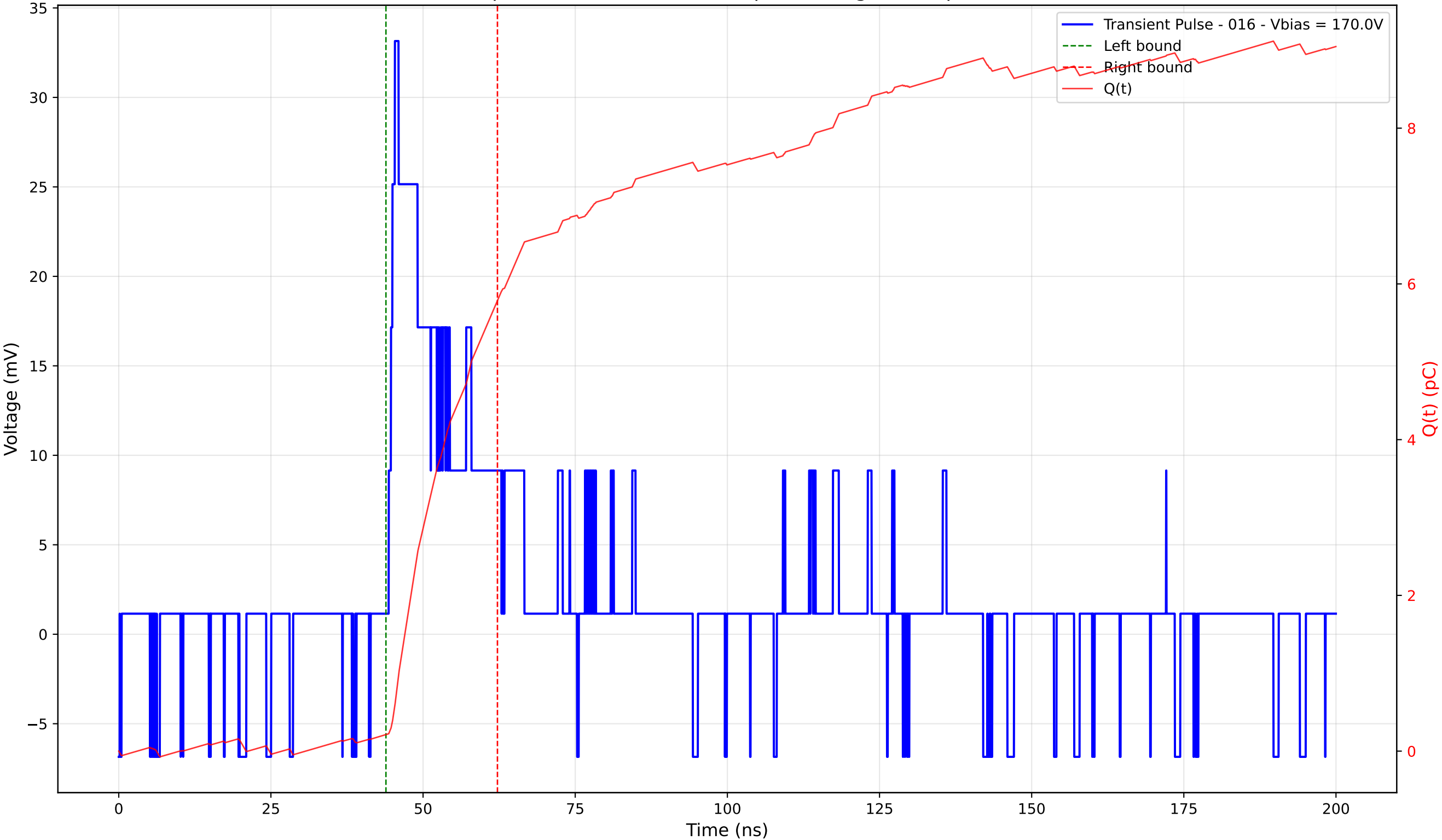
Transient Pulse - Sample: 4003 - Position: 60.0 \mu\text{m} - Charge: 5.58 pC - Rise Time: 1.01 ns
