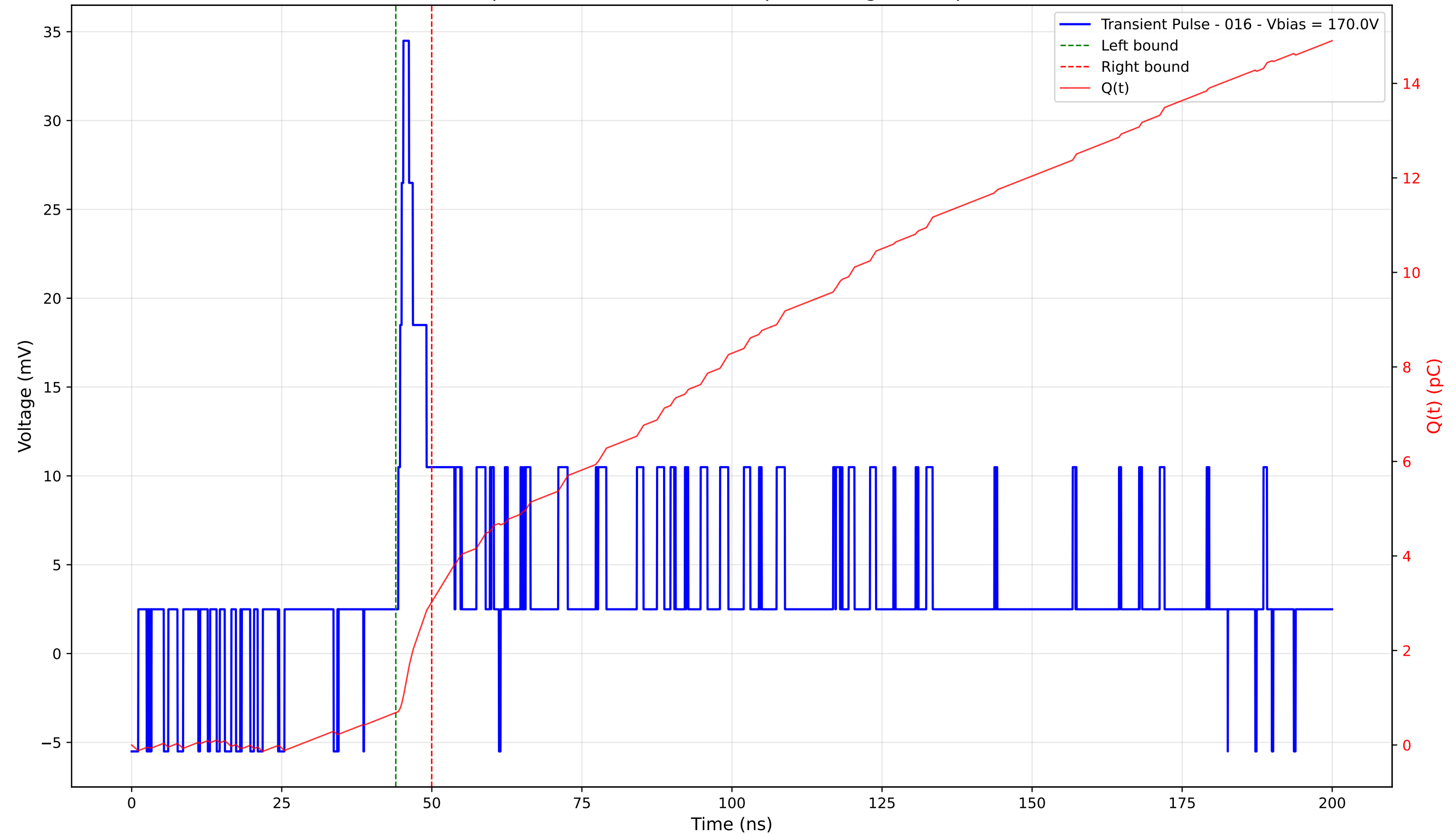
Transient Pulse - Sample: 4003 - Position: 355.0 \mu\text{m} - Charge: 2.34 pC - Rise Time: 0.86 ns
