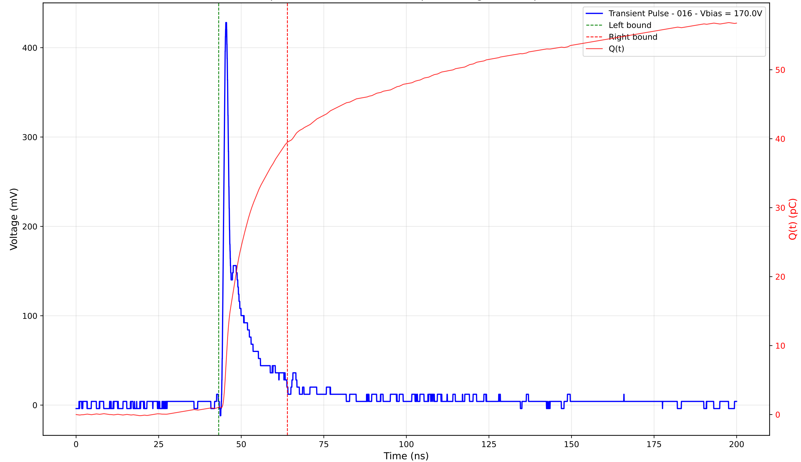
Transient Pulse - Sample: 4003 - Position: 115.0 \mu\text{m} - Charge: 38.42 pC - Rise Time: 0.90 ns
