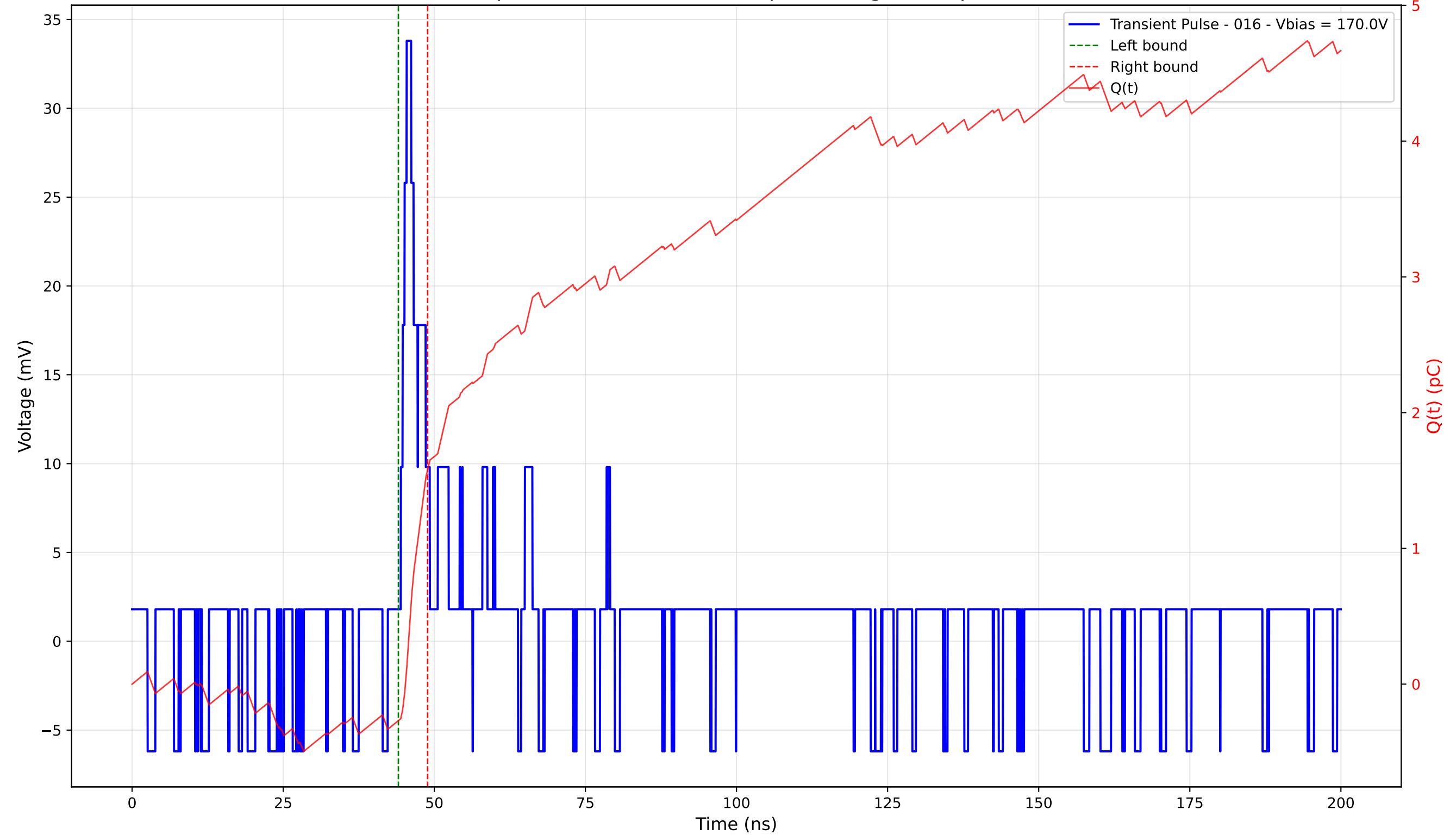
Transient Pulse - Sample: 4003 - Position: 410.0 \mu\text{m} - Charge: 1.85 pC - Rise Time: 0.98 ns
