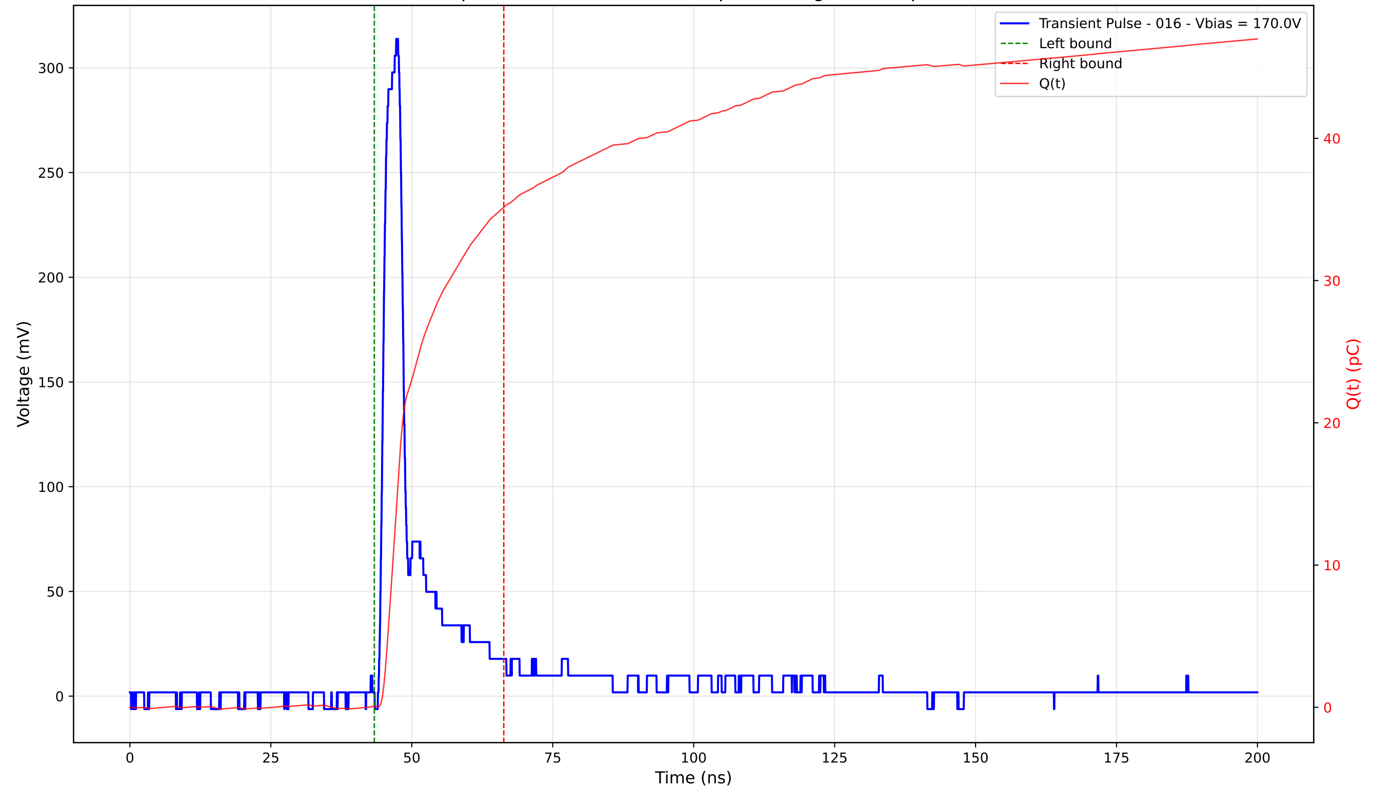
Transient Pulse - Sample: 4003 - Position: 270.0 \mu\text{m} - Charge: 35.07 pC - Rise Time: 1.51 ns
