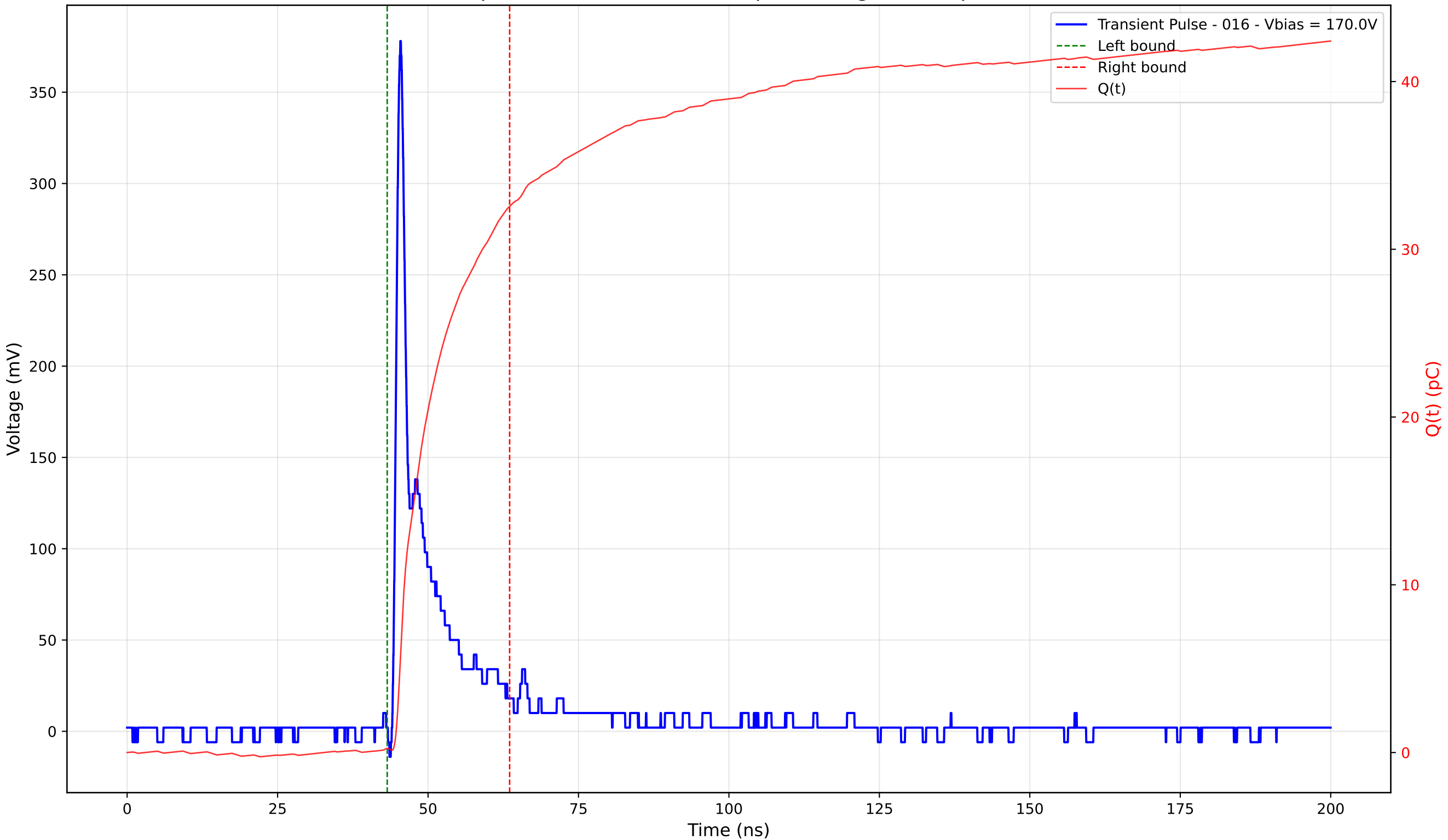
Transient Pulse - Sample: 4003 - Position: 110.0 \mu\text{m} - Charge: 32.32 pC - Rise Time: 0.91 ns
