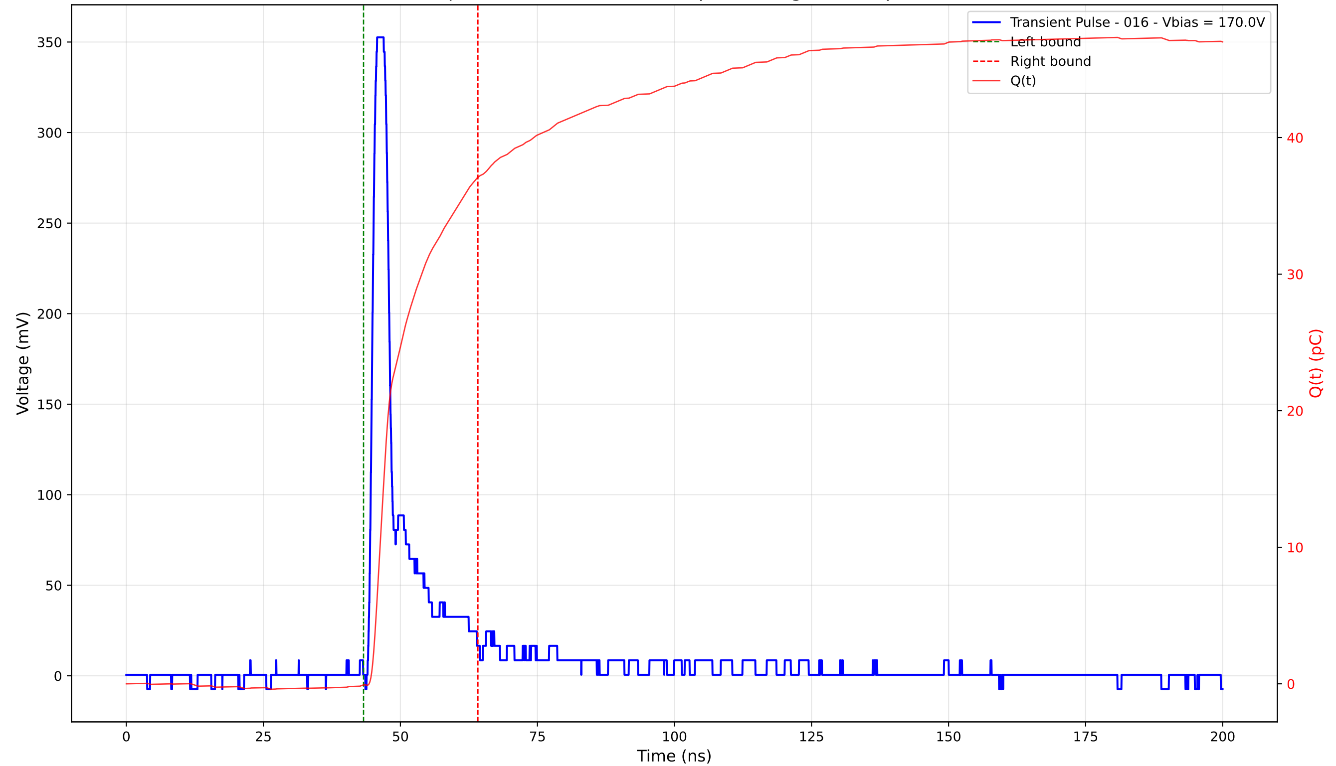
Transient Pulse - Sample: 4003 - Position: 250.0 \mu\text{m} - Charge: 37.16 pC - Rise Time: 1.15 ns
