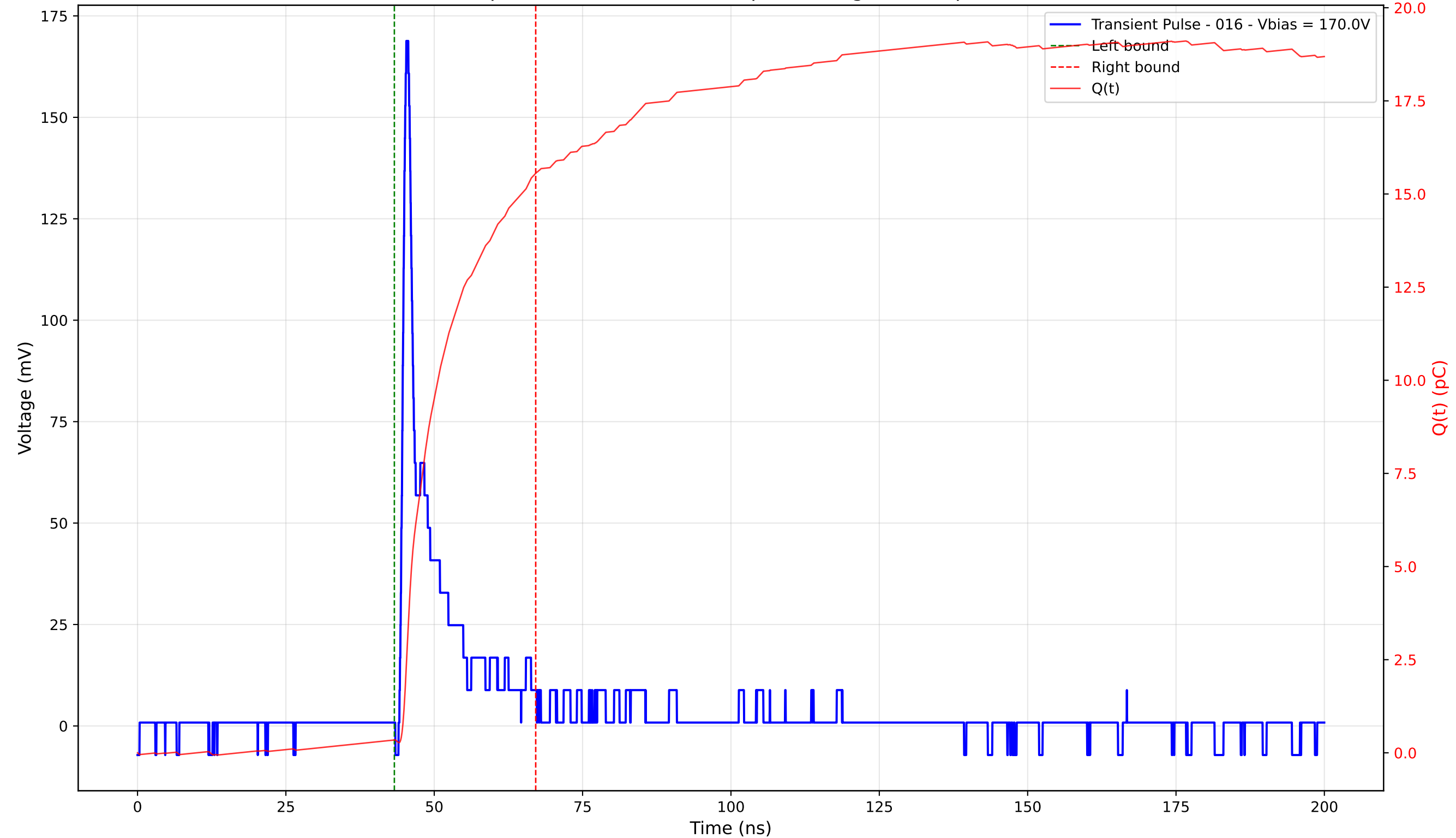
Transient Pulse - Sample: 4003 - Position: 95.0 \mu\text{m} - Charge: 15.21 pC - Rise Time: 0.82 ns
