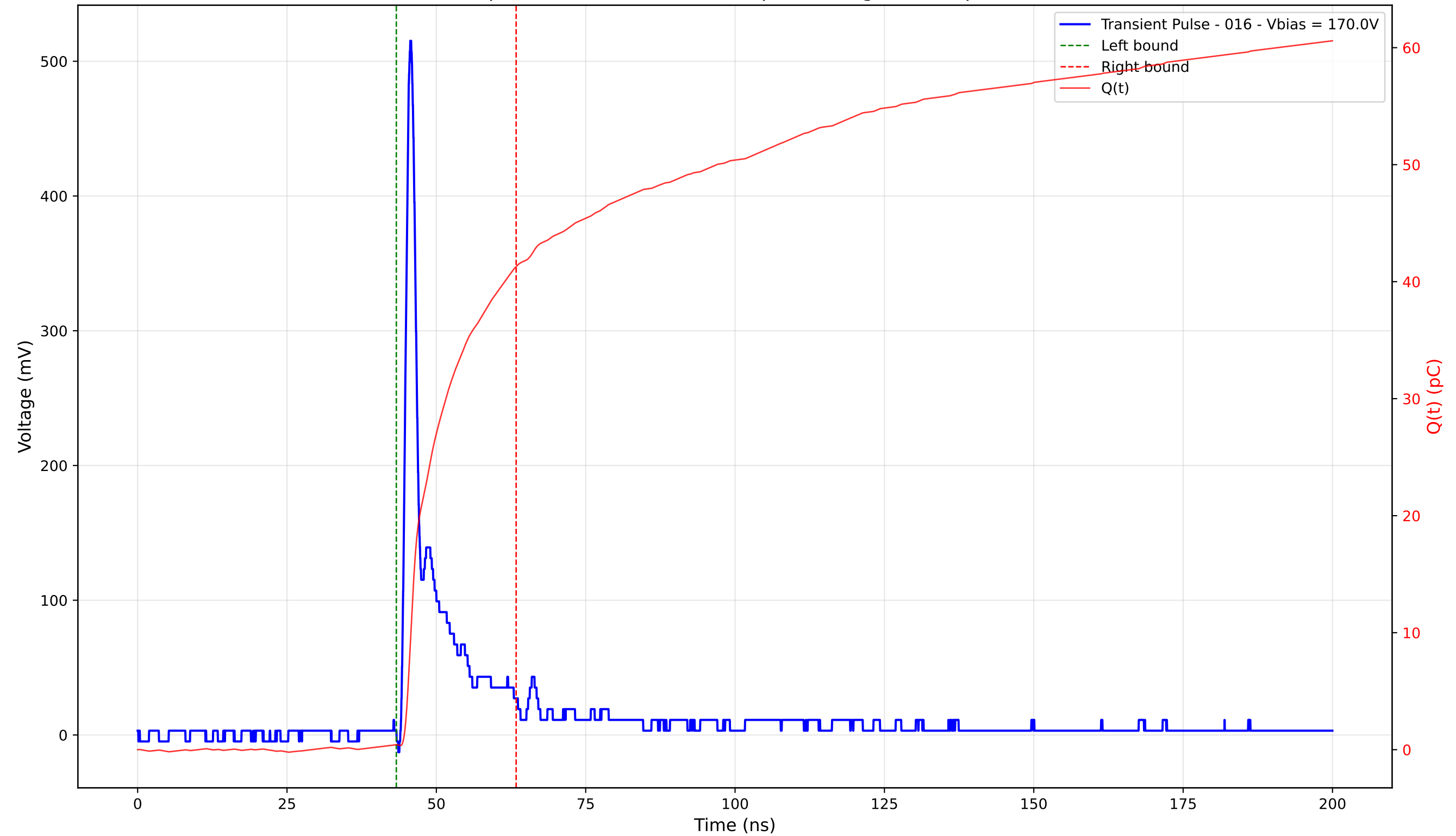
Transient Pulse - Sample: 4003 - Position: 185.0 \mu\text{m} - Charge: 40.85 pC - Rise Time: 1.04 ns
