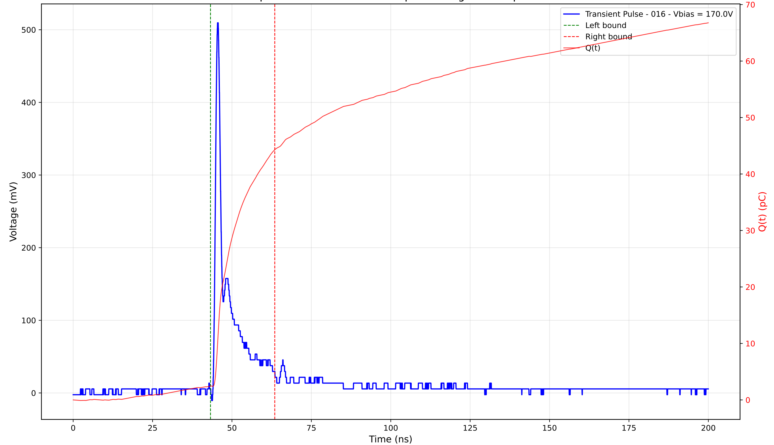
Transient Pulse - Sample: 4003 - Position: 155.0 \mu\text{m} - Charge: 41.84 pC - Rise Time: 0.96 ns
