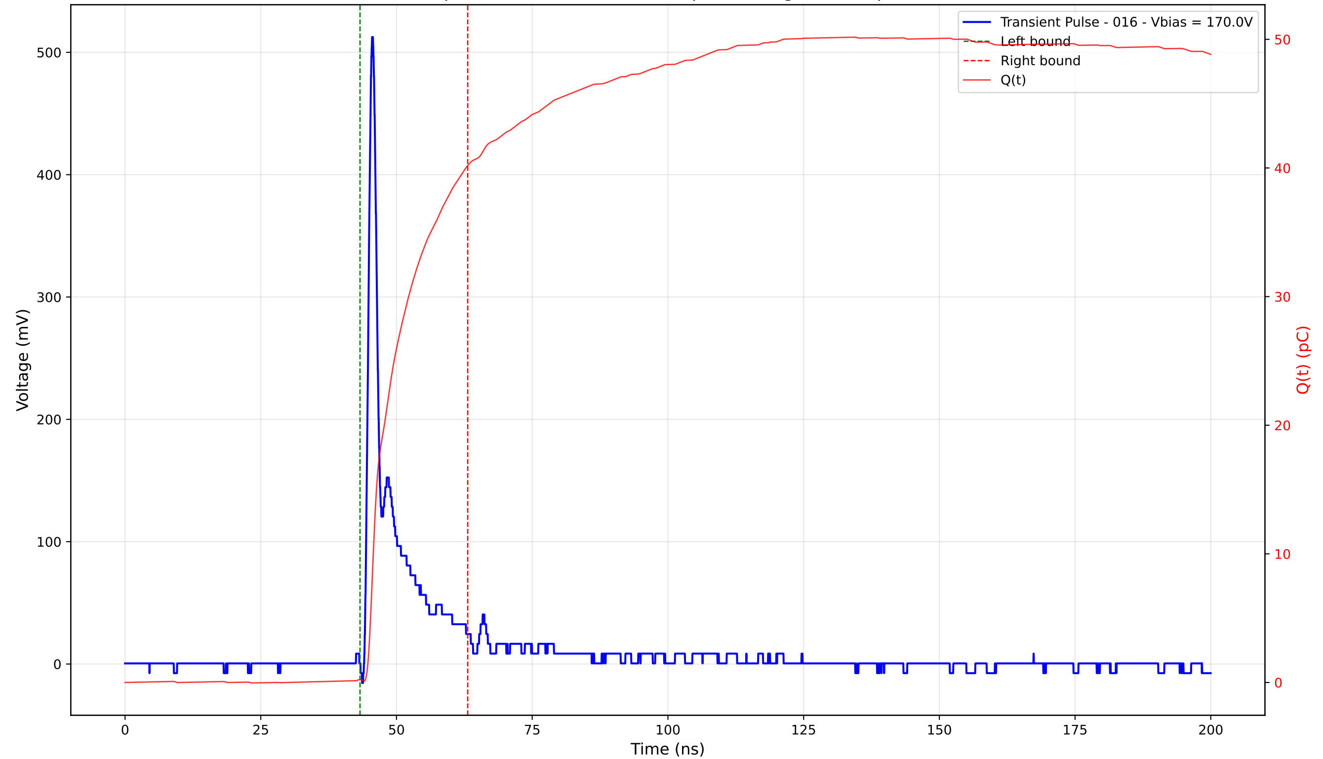
Transient Pulse - Sample: 4003 - Position: 160.0 \mu\text{m} - Charge: 39.96 pC - Rise Time: 0.97 ns
