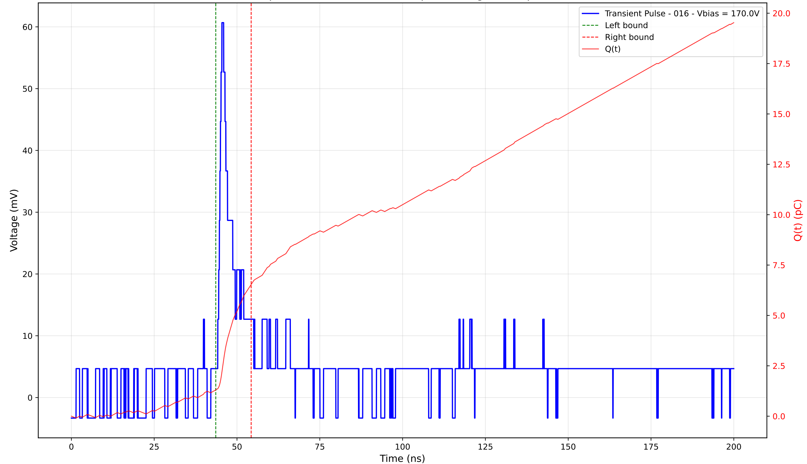
Transient Pulse - Sample: 4003 - Position: 395.0 \mu\text{m} - Charge: 5.24 pC - Rise Time: 1.26 ns
