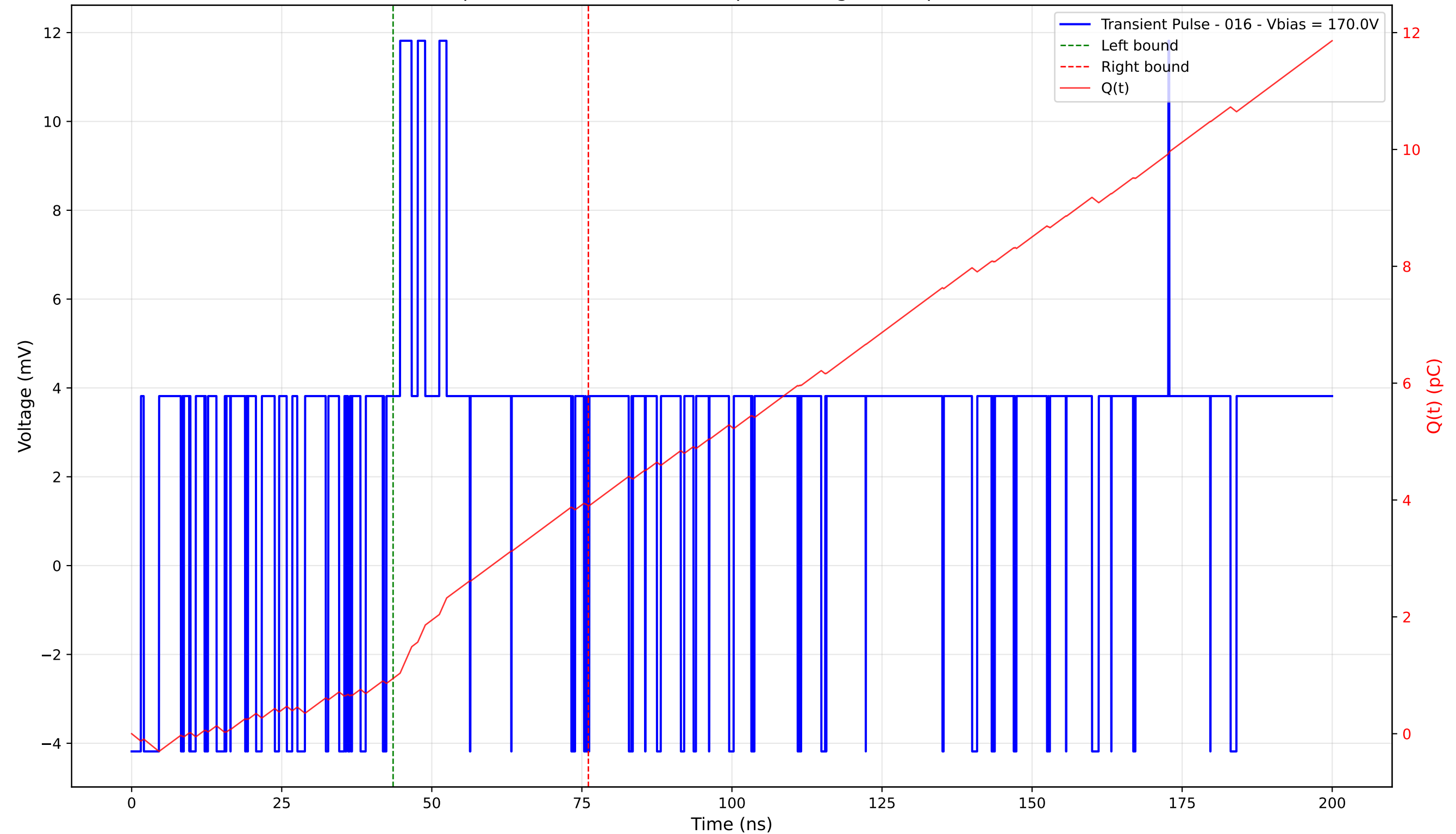
Transient Pulse - Sample: 4003 - Position: 425.0 \mu\text{m} - Charge: 2.97 pC - Rise Time: 0.00 ns (N/A)
