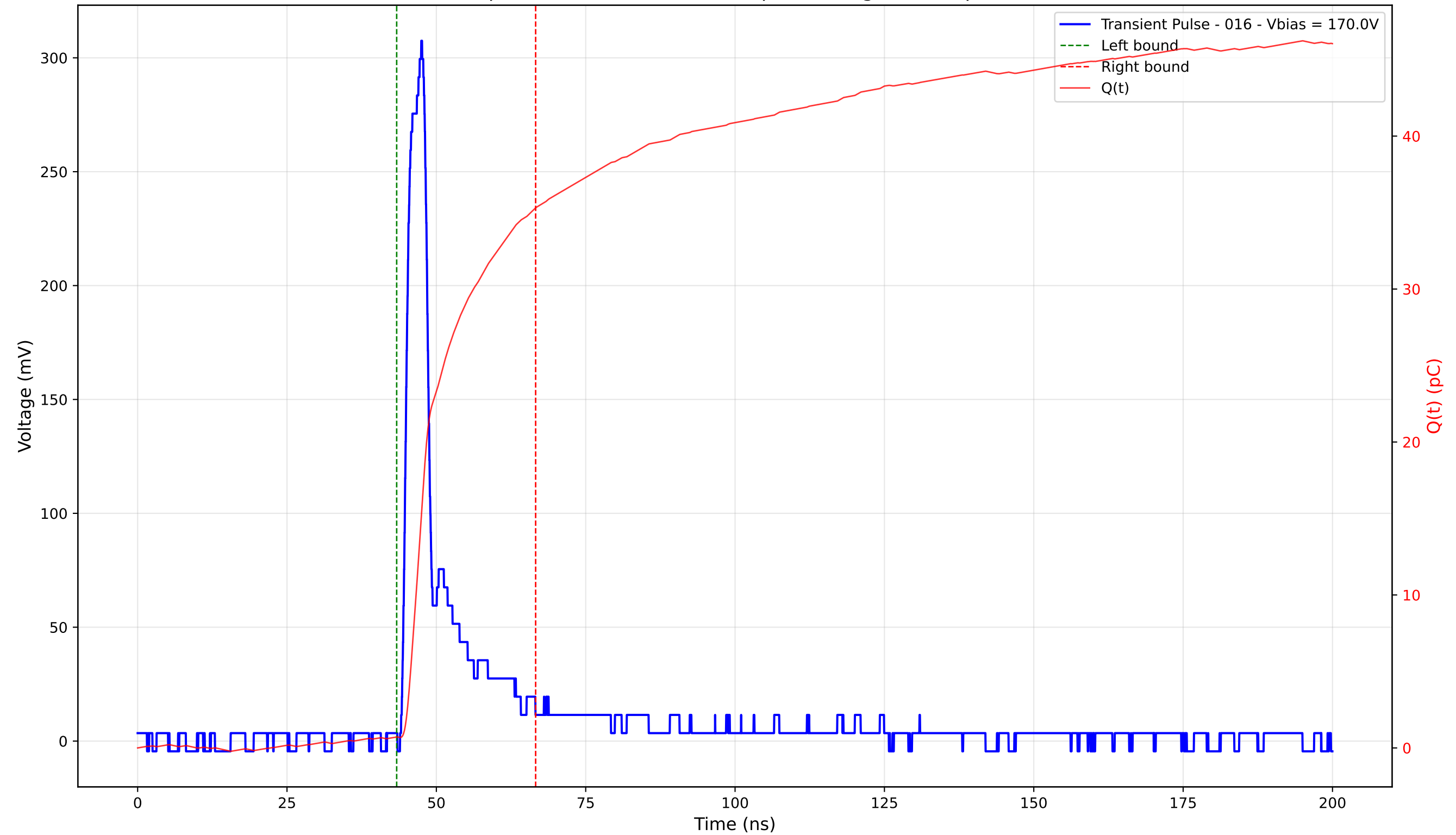
Transient Pulse - Sample: 4003 - Position: 275.0 \mu\text{m} - Charge: 34.60 pC - Rise Time: 2.41 ns
