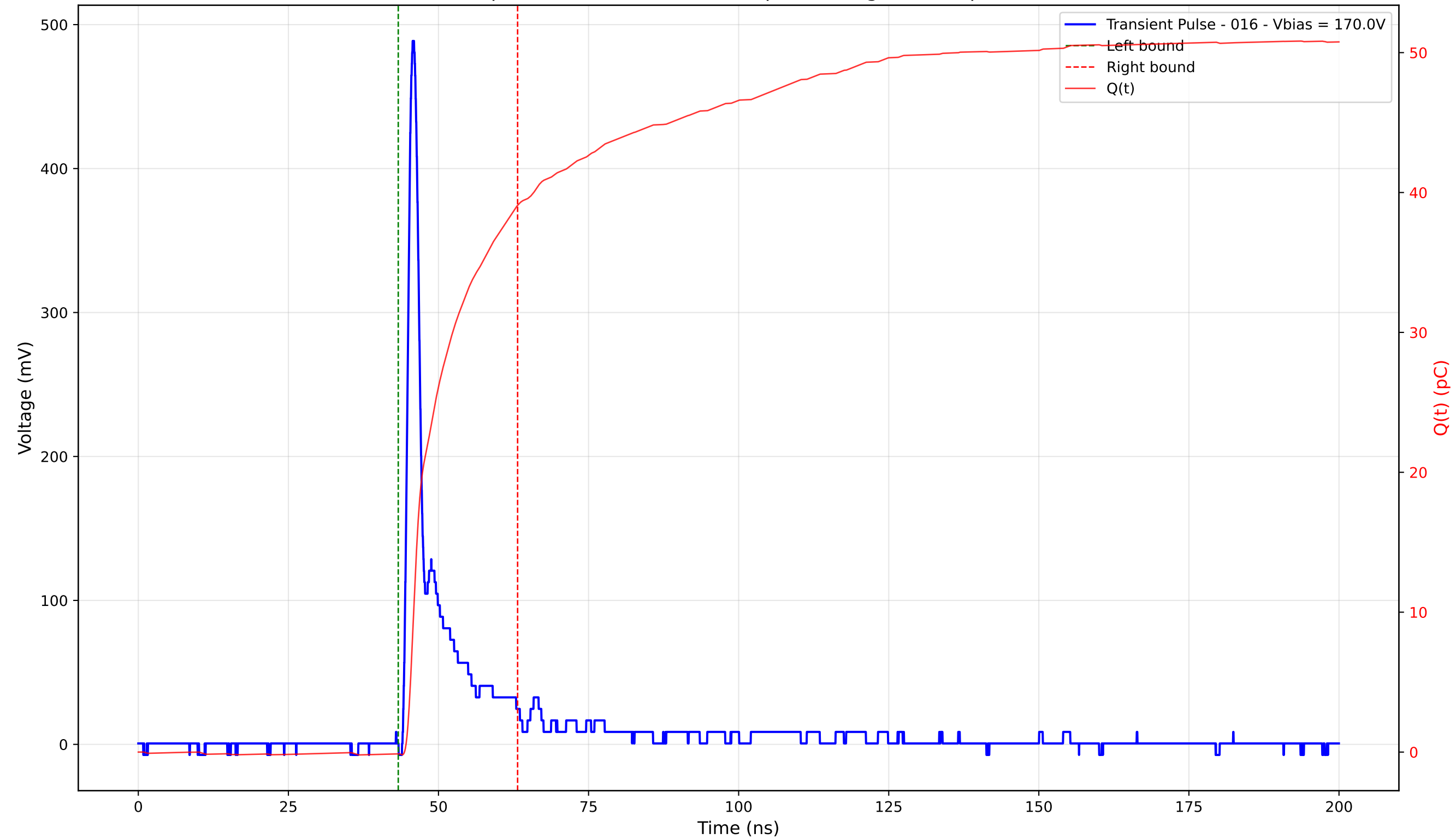
Transient Pulse - Sample: 4003 - Position: 200.0 \mu\text{m} - Charge: 39.19 pC - Rise Time: 1.10 ns
