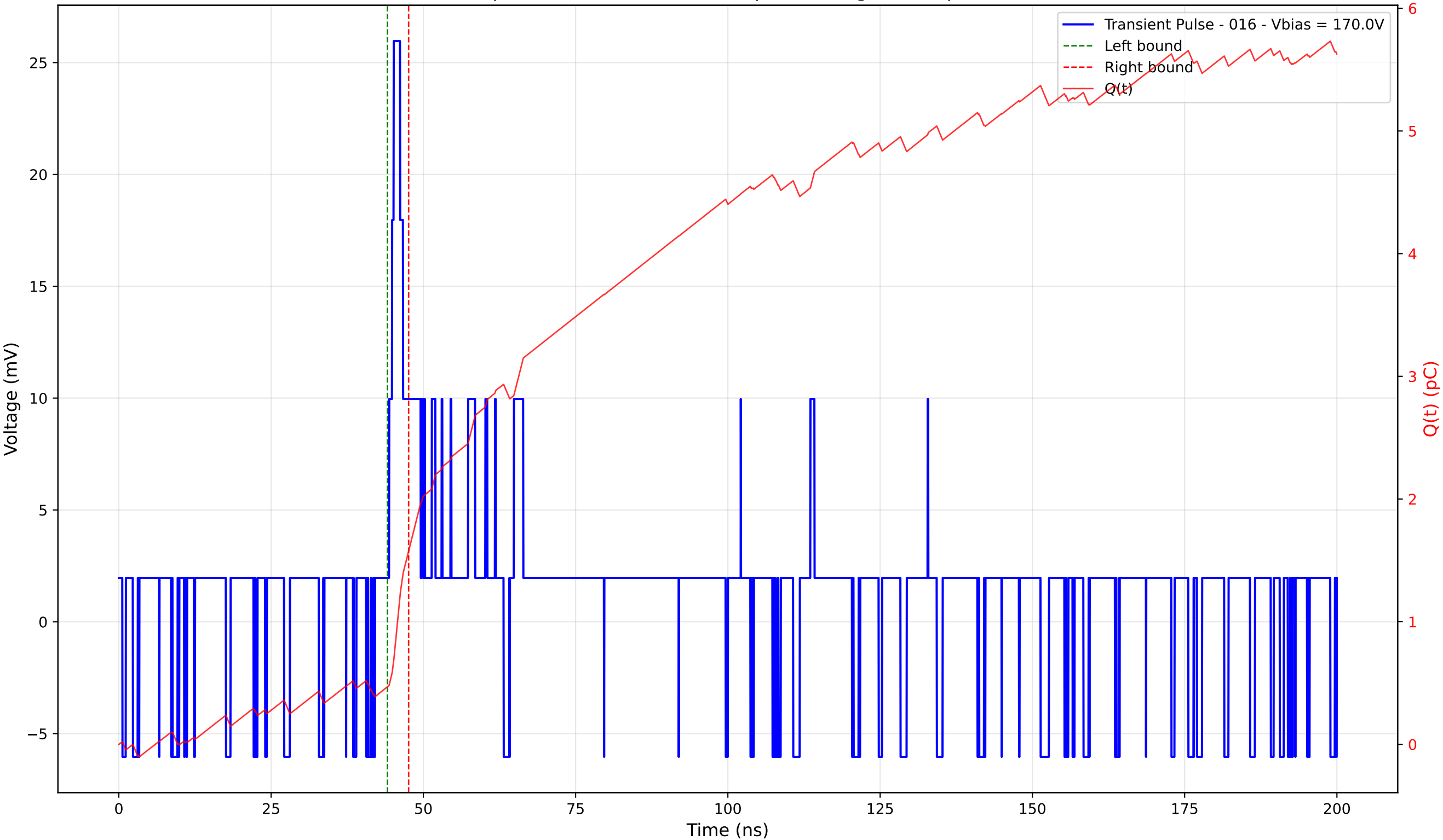
Transient Pulse - Sample: 4003 - Position: 25.0 \mu\text{m} - Charge: 1.11 pC - Rise Time: 0.76 ns
