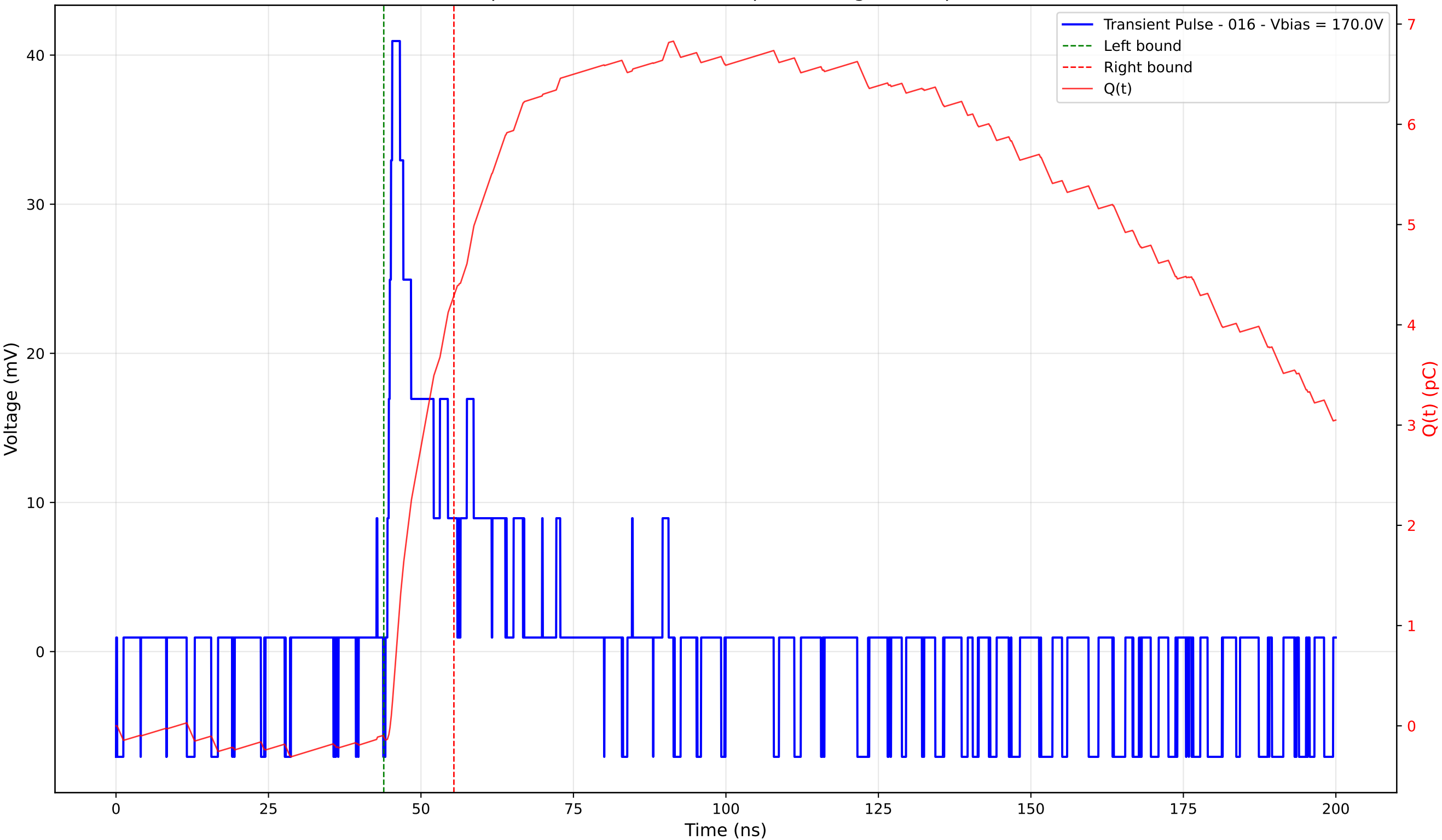
Transient Pulse - Sample: 4003 - Position: 50.0 \mu\text{m} - Charge: 4.40 pC - Rise Time: 0.79 ns
