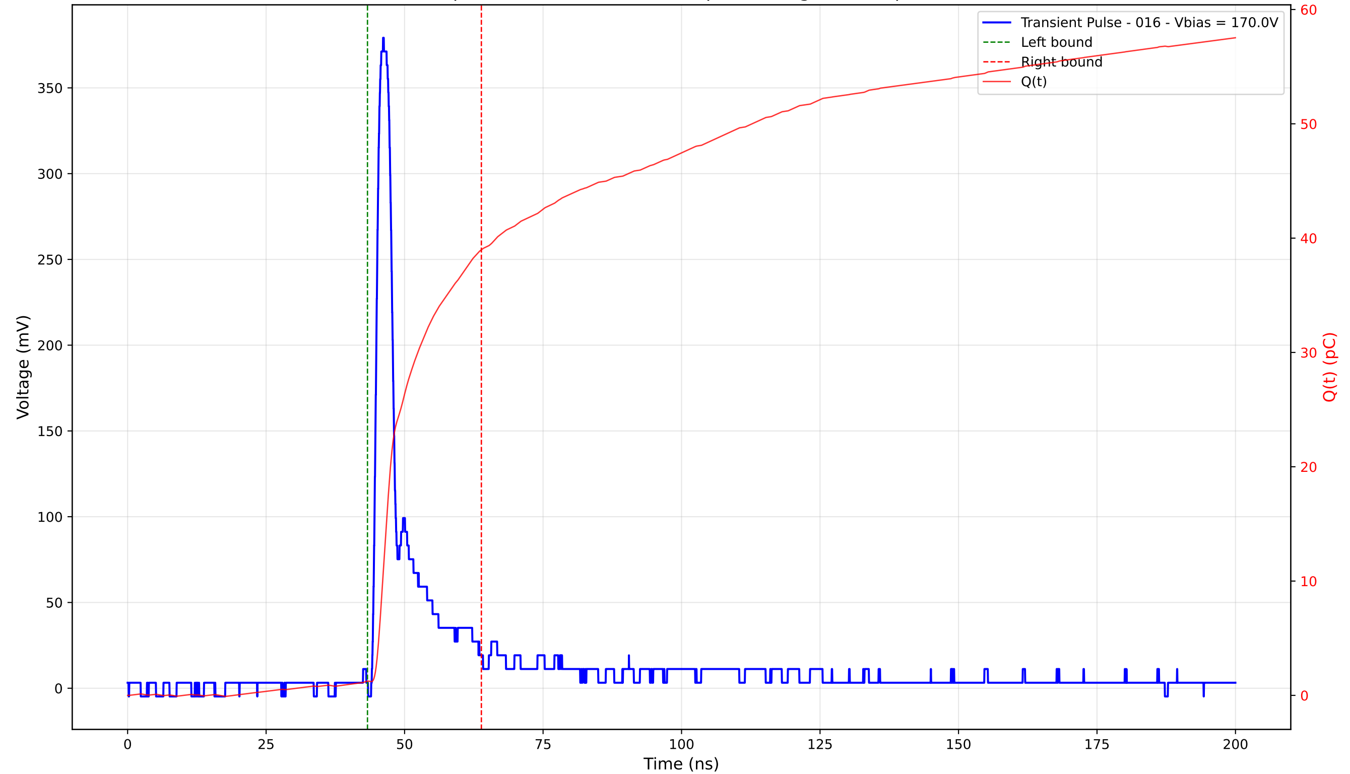
Transient Pulse - Sample: 4003 - Position: 245.0 \mu\text{m} - Charge: 37.73 pC - Rise Time: 1.21 ns
