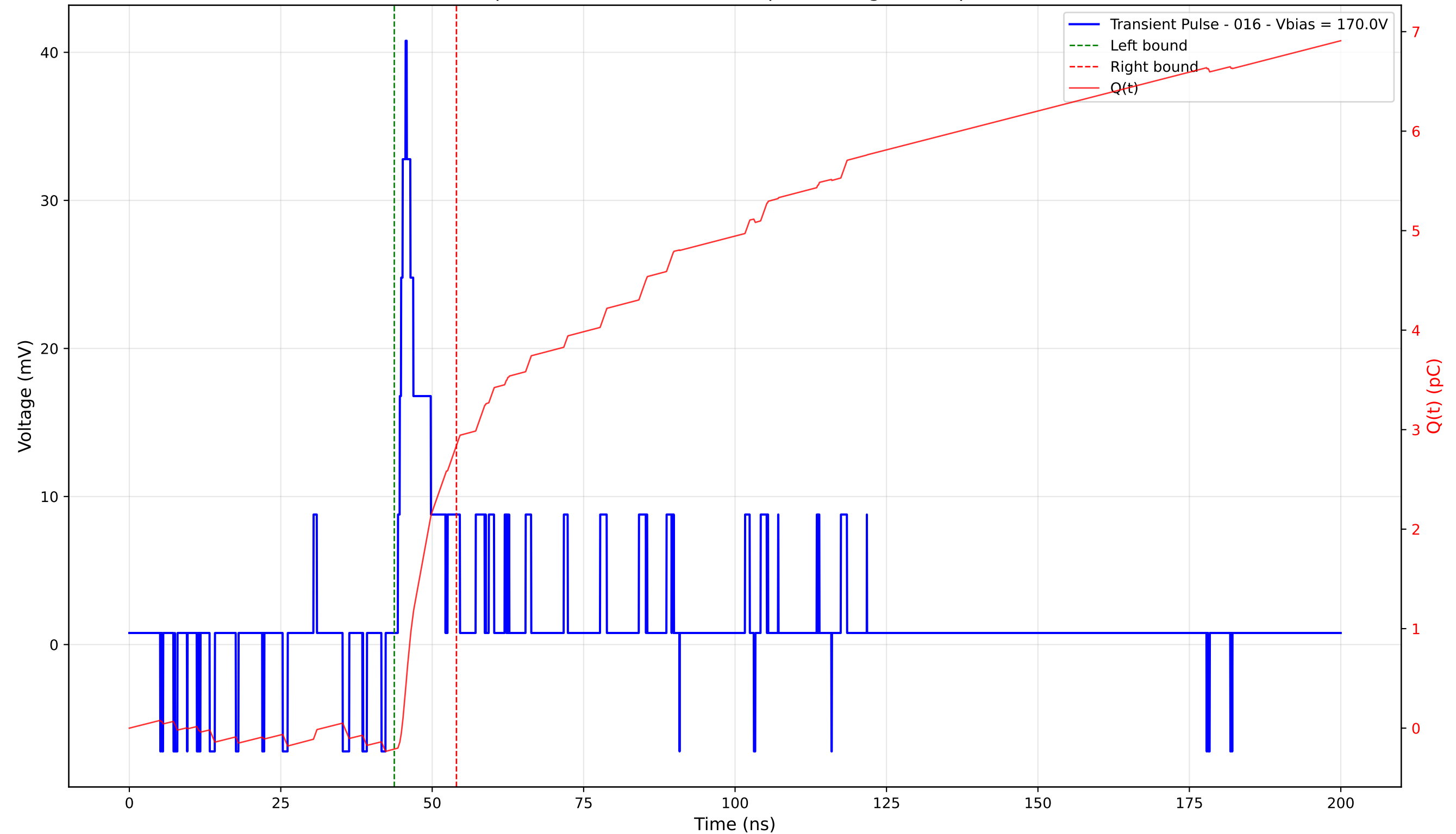
Transient Pulse - Sample: 4003 - Position: 360.0 \mu\text{m} - Charge: 3.05 pC - Rise Time: 1.27 ns
