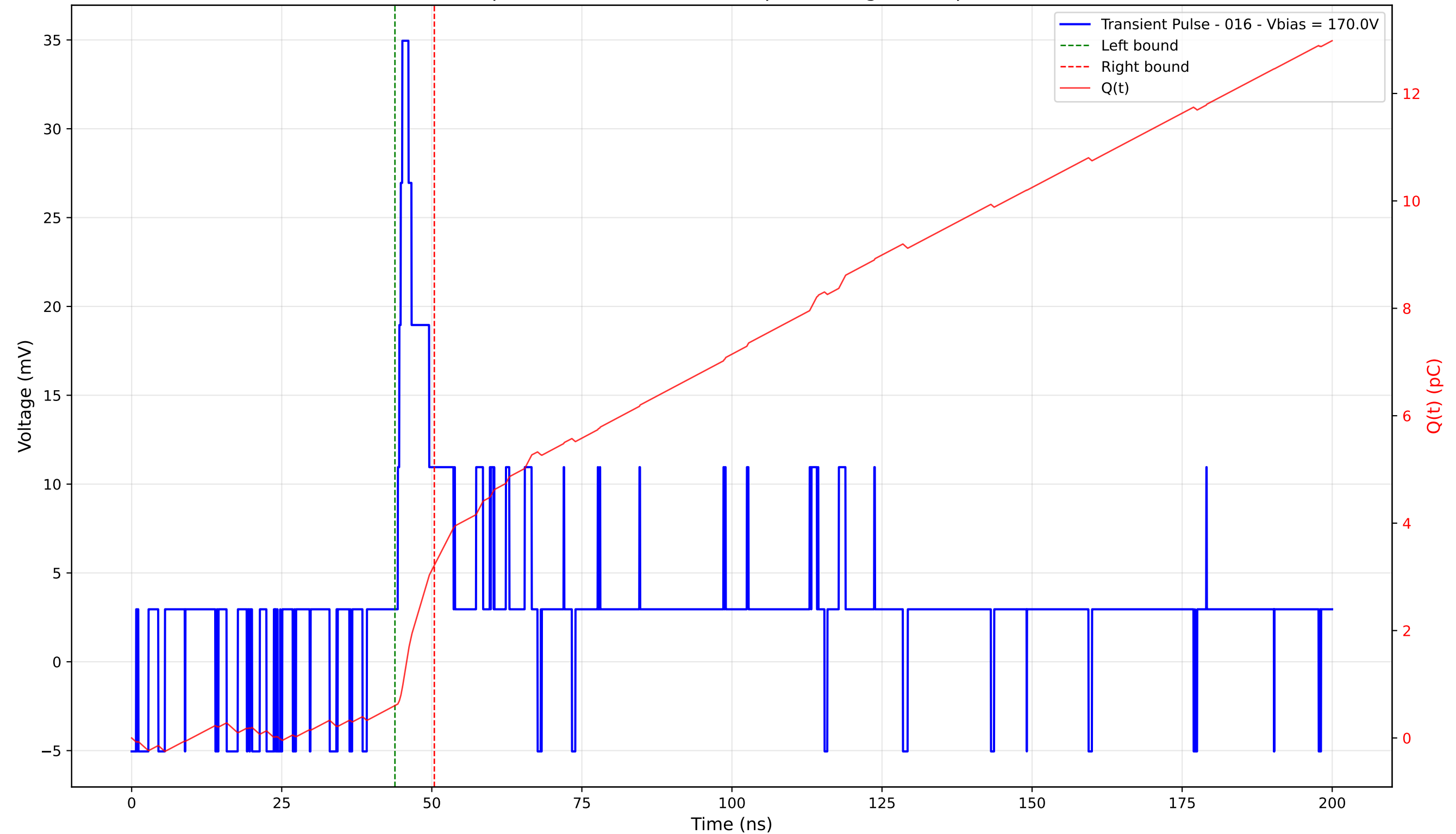
Transient Pulse - Sample: 4003 - Position: 365.0 \mu\text{m} - Charge: 2.61 pC - Rise Time: 0.76 ns
