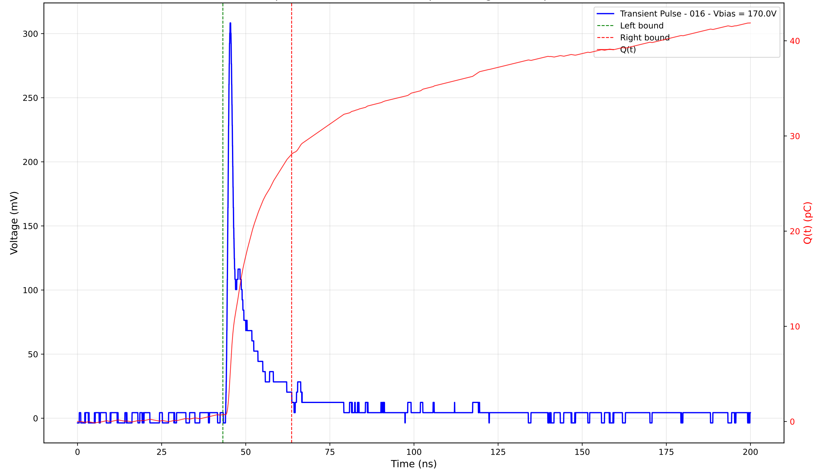
Transient Pulse - Sample: 4003 - Position: 105.0 \mu\text{m} - Charge: 27.36 pC - Rise Time: 0.91 ns
