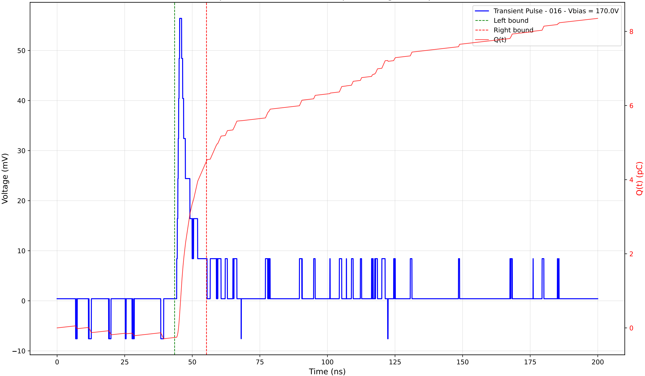
Transient Pulse - Sample: 4003 - Position: 385.0 \mu\text{m} - Charge: 4.77 pC - Rise Time: 1.09 ns
