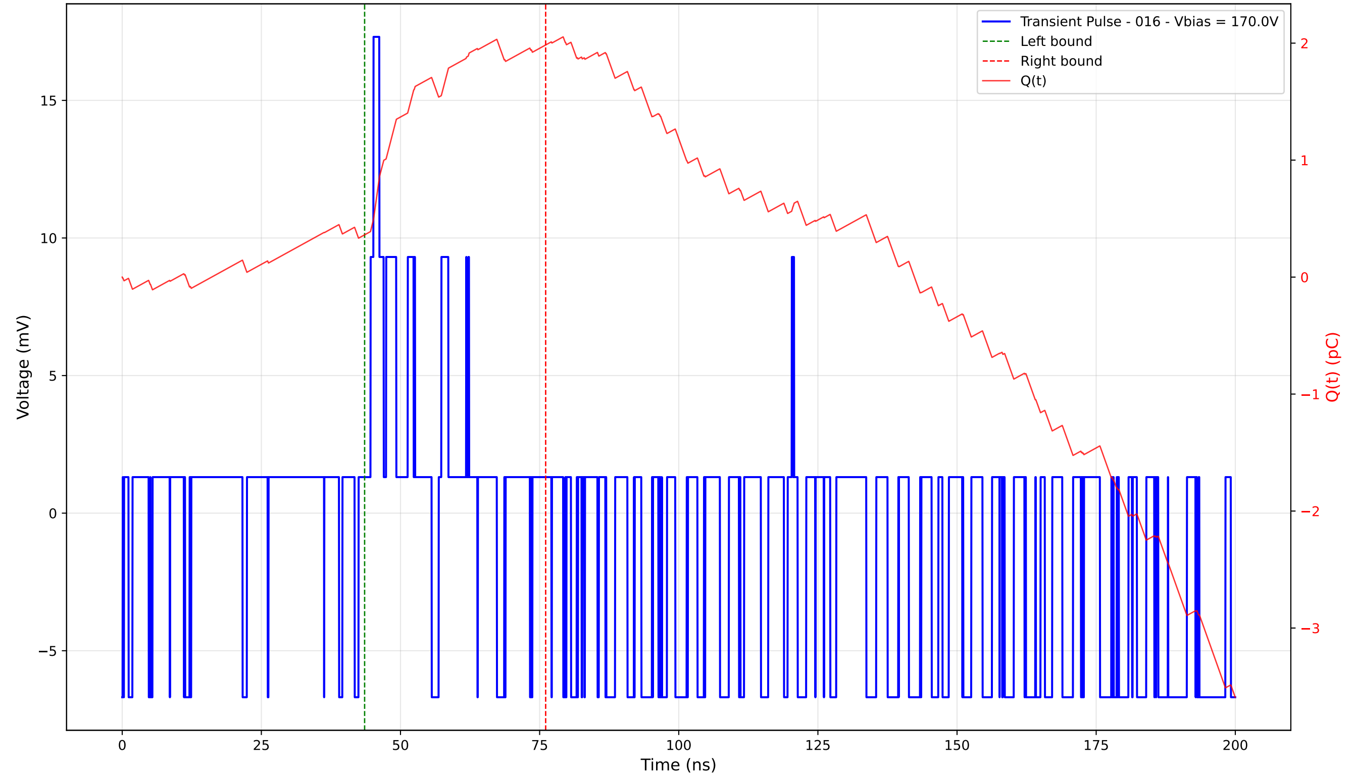
Transient Pulse - Sample: 4003 - Position: 70.0 \mu\text{m} - Charge: 1.62 pC - Rise Time: 0.54 ns
