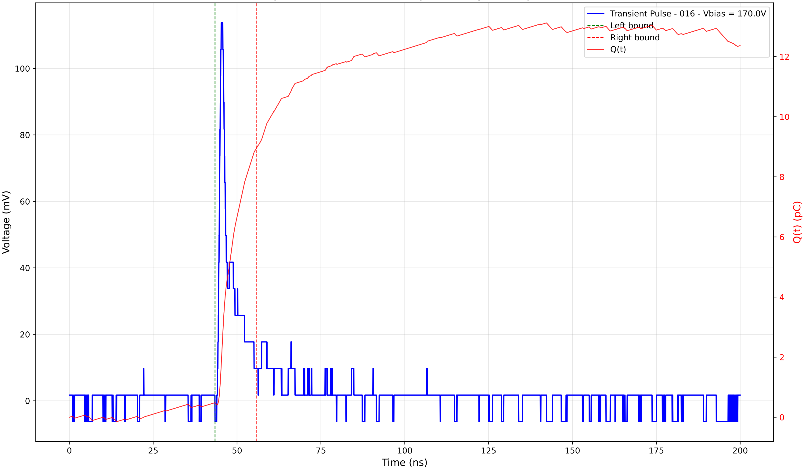
Transient Pulse - Sample: 4003 - Position: 90.0 \mu\text{m} - Charge: 8.50 pC - Rise Time: 0.86 ns
