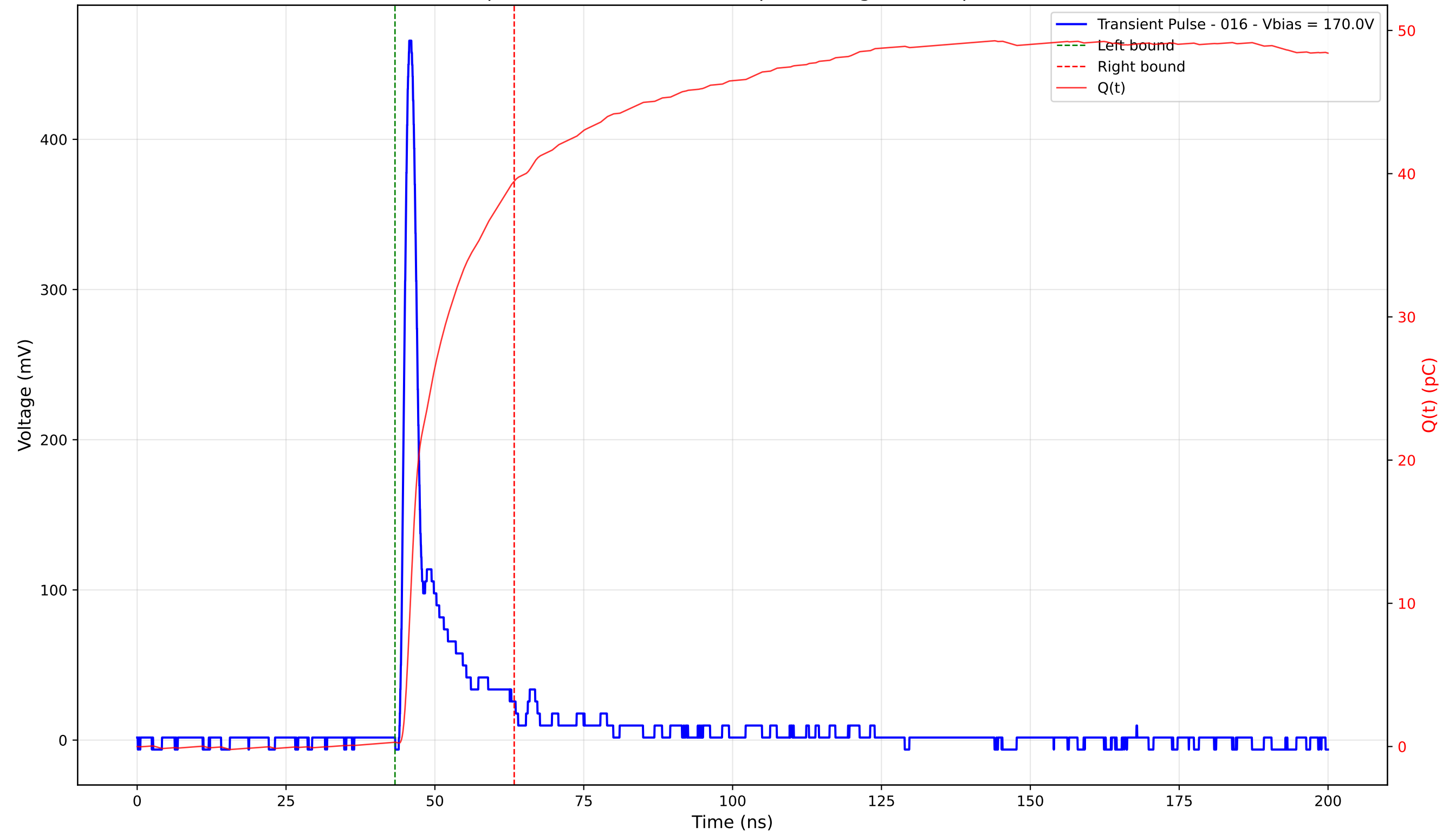
Transient Pulse - Sample: 4003 - Position: 210.0 \mu\text{m} - Charge: 39.17 pC - Rise Time: 1.13 ns
