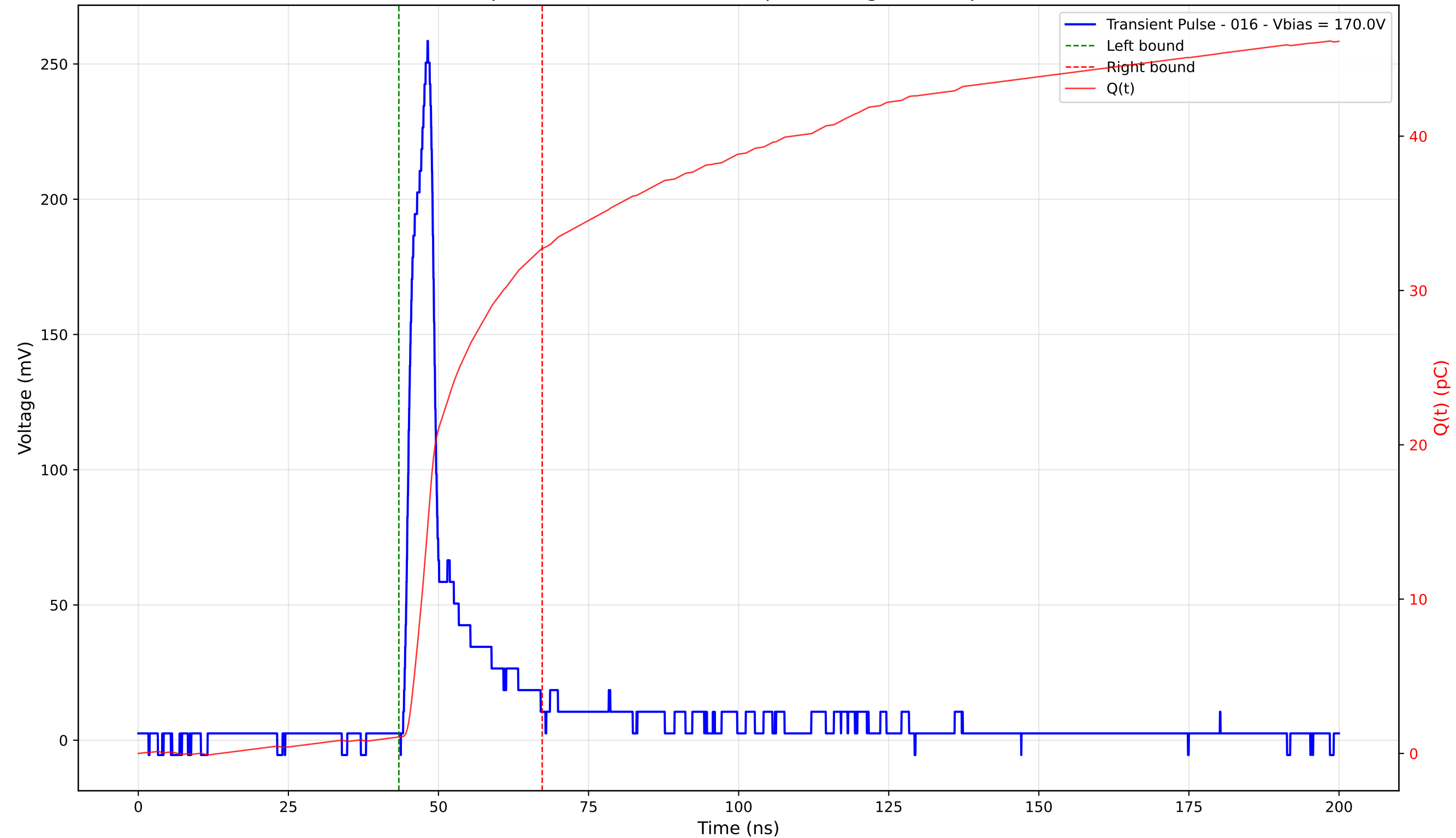
Transient Pulse - Sample: 4003 - Position: 295.0 \mu\text{m} - Charge: 31.65 pC - Rise Time: 3.14 ns
