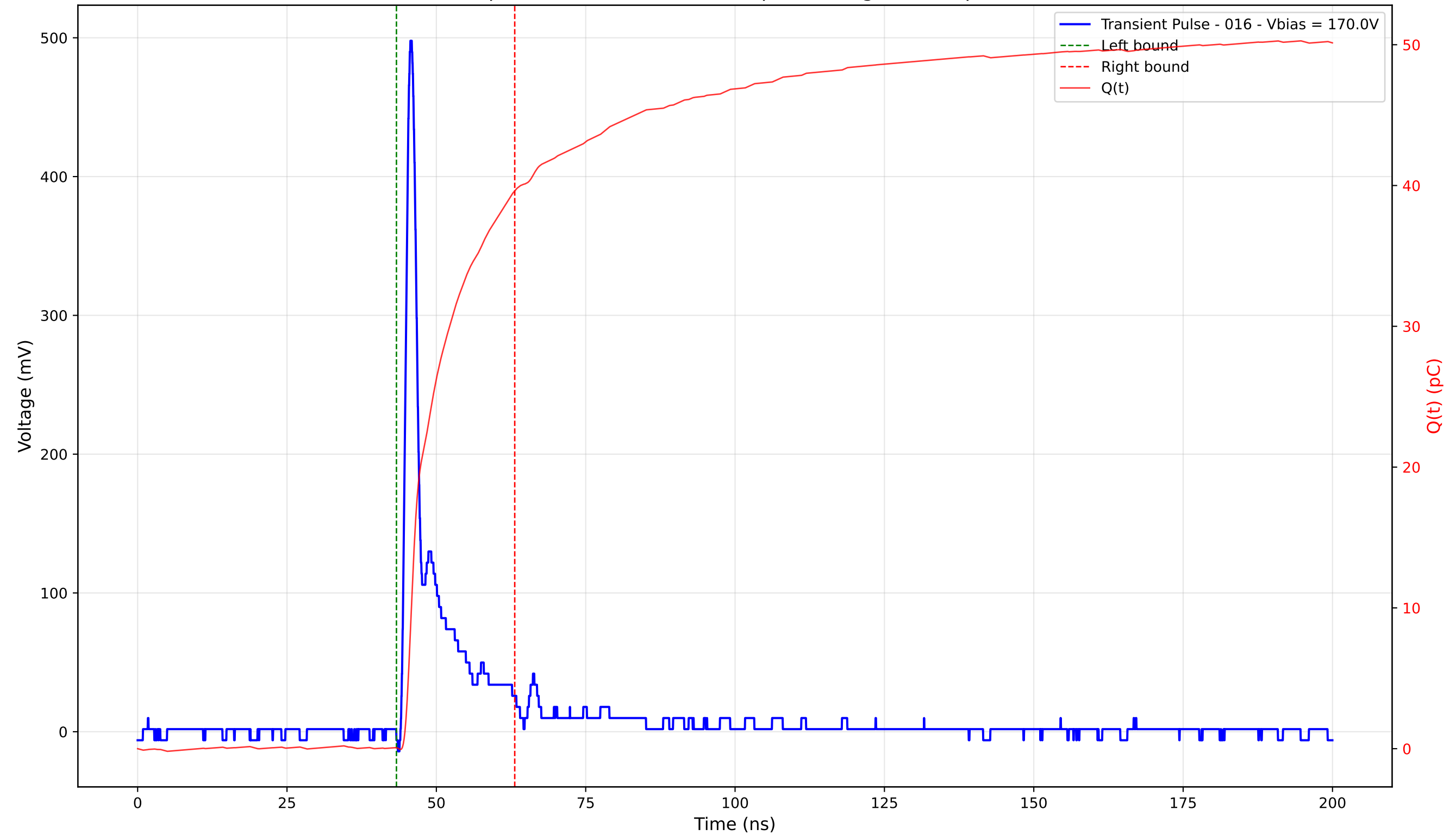
Transient Pulse - Sample: 4003 - Position: 195.0 \mu\text{m} - Charge: 39.55 pC - Rise Time: 1.08 ns
