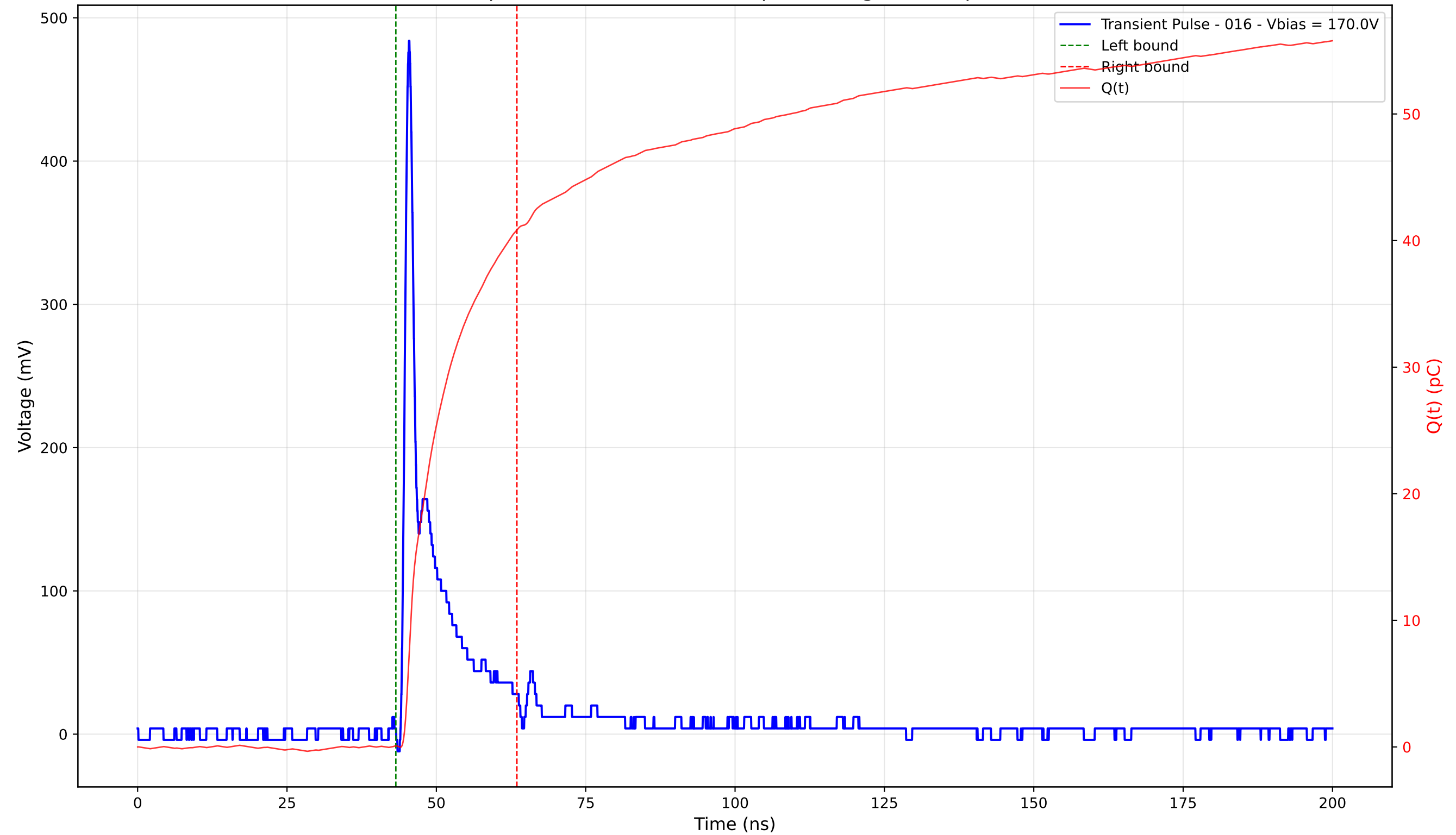
Transient Pulse - Sample: 4003 - Position: 125.0 \mu\text{m} - Charge: 40.75 pC - Rise Time: 0.91 ns
