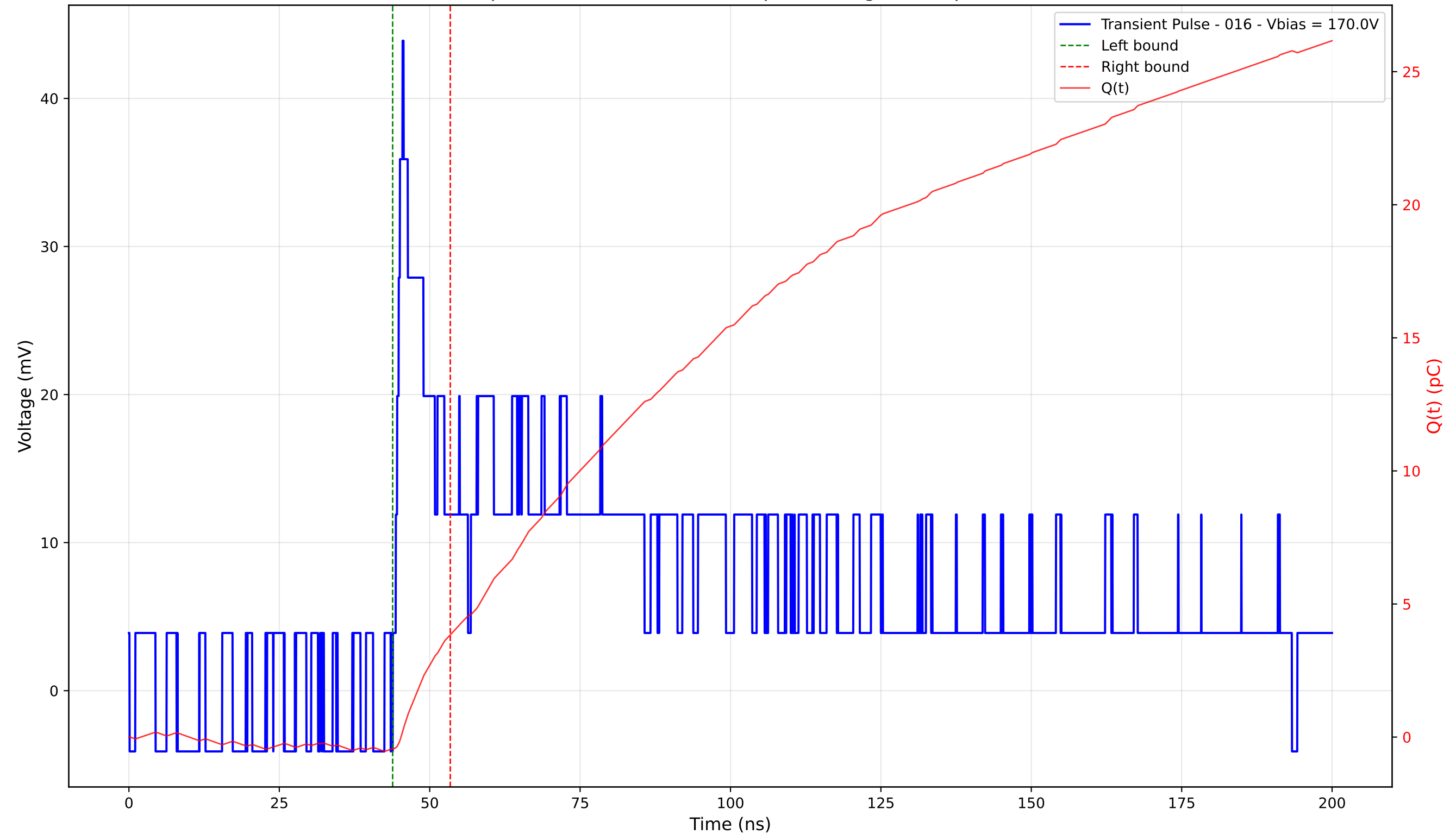
Transient Pulse - Sample: 4003 - Position: 335.0 \mu\text{m} - Charge: 4.29 pC - Rise Time: 1.14 ns
