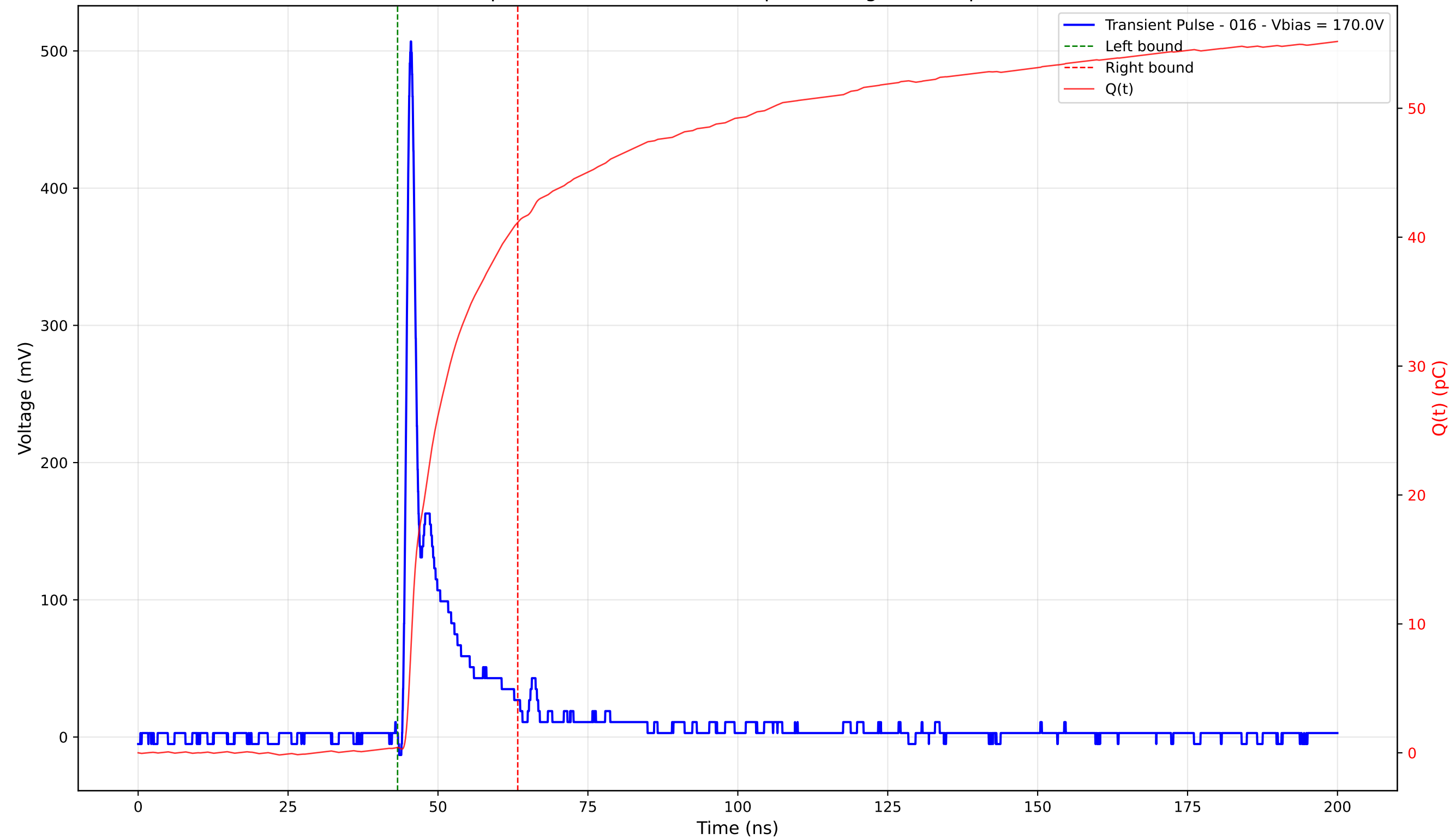
Transient Pulse - Sample: 4003 - Position: 140.0 \mu\text{m} - Charge: 40.74 pC - Rise Time: 0.93 ns
