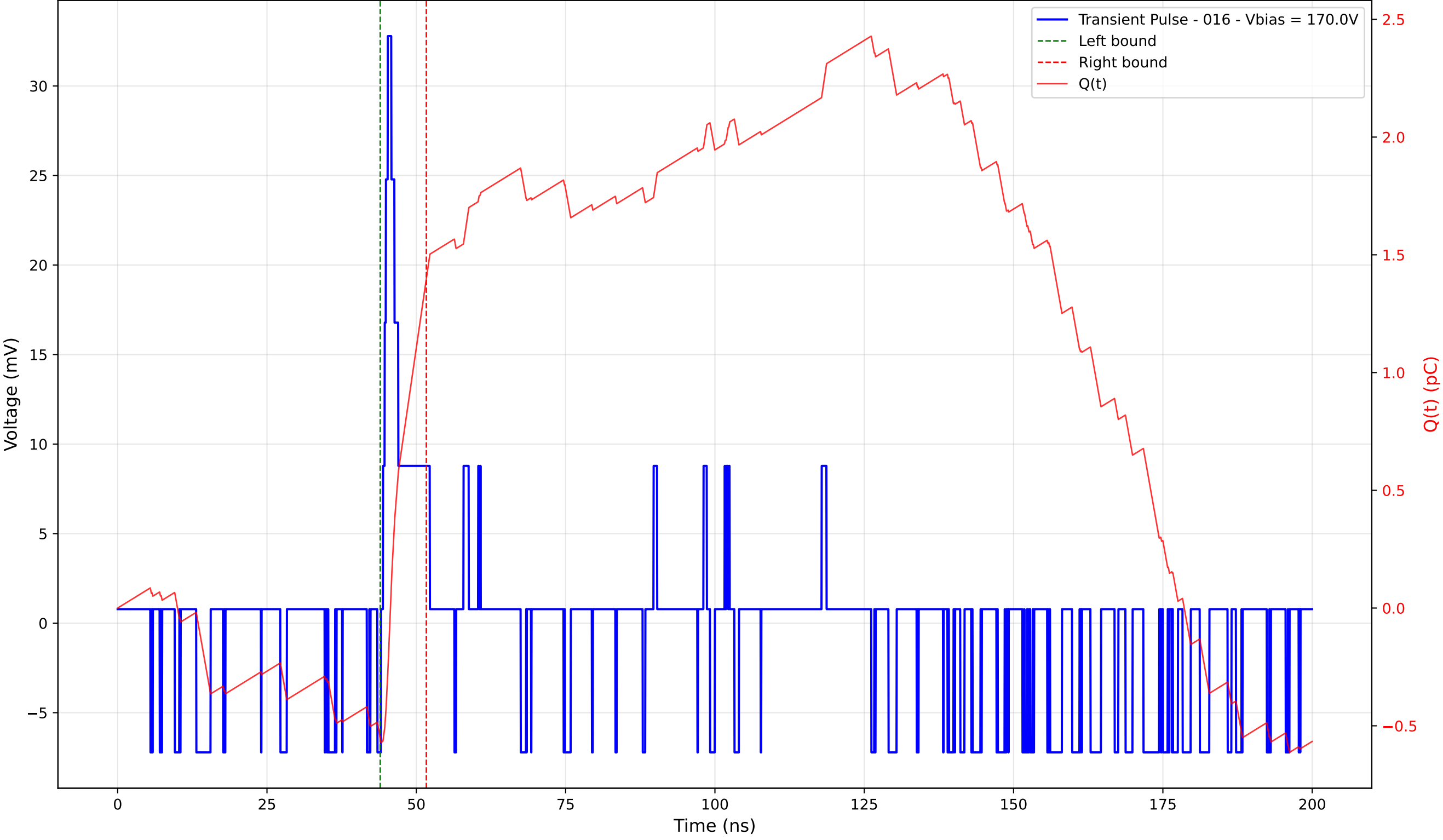
Transient Pulse - Sample: 4003 - Position: 80.0 \mu\text{m} - Charge: 1.96 pC - Rise Time: 0.81 ns
