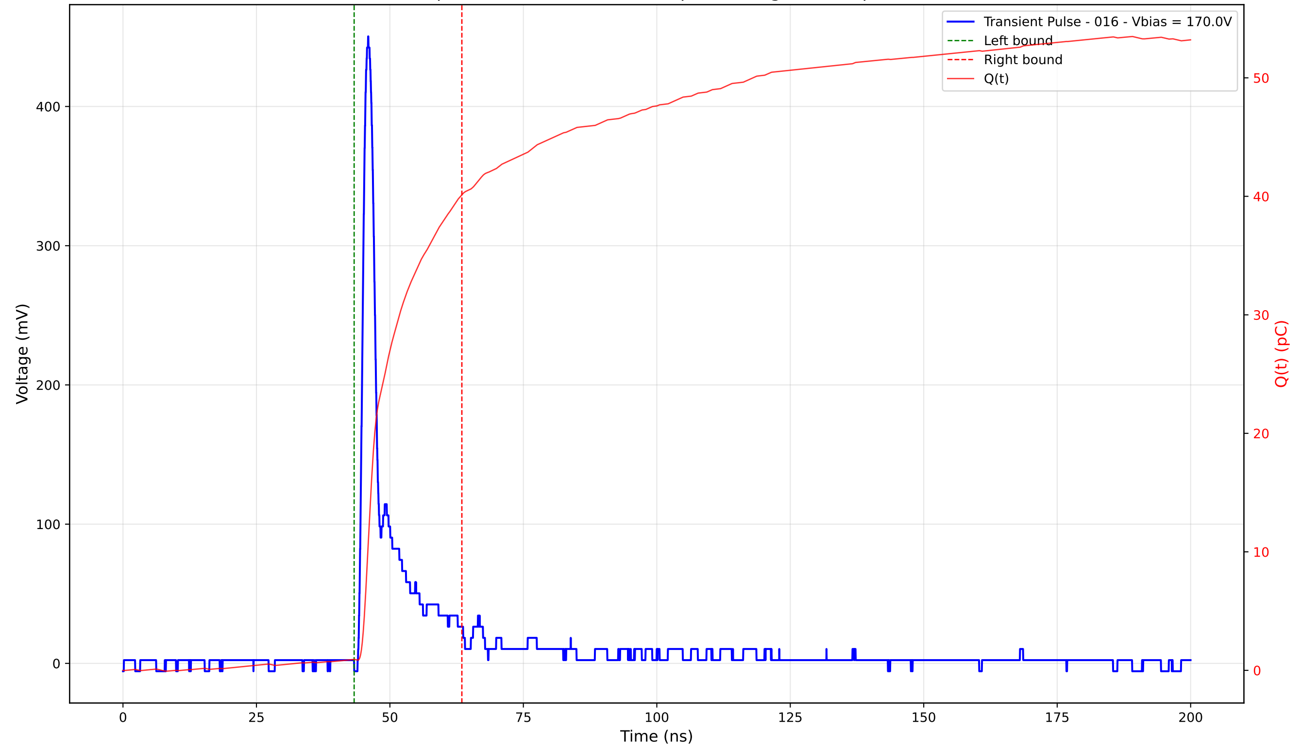
Transient Pulse - Sample: 4003 - Position: 220.0 \mu\text{m} - Charge: 39.20 pC - Rise Time: 1.15 ns
