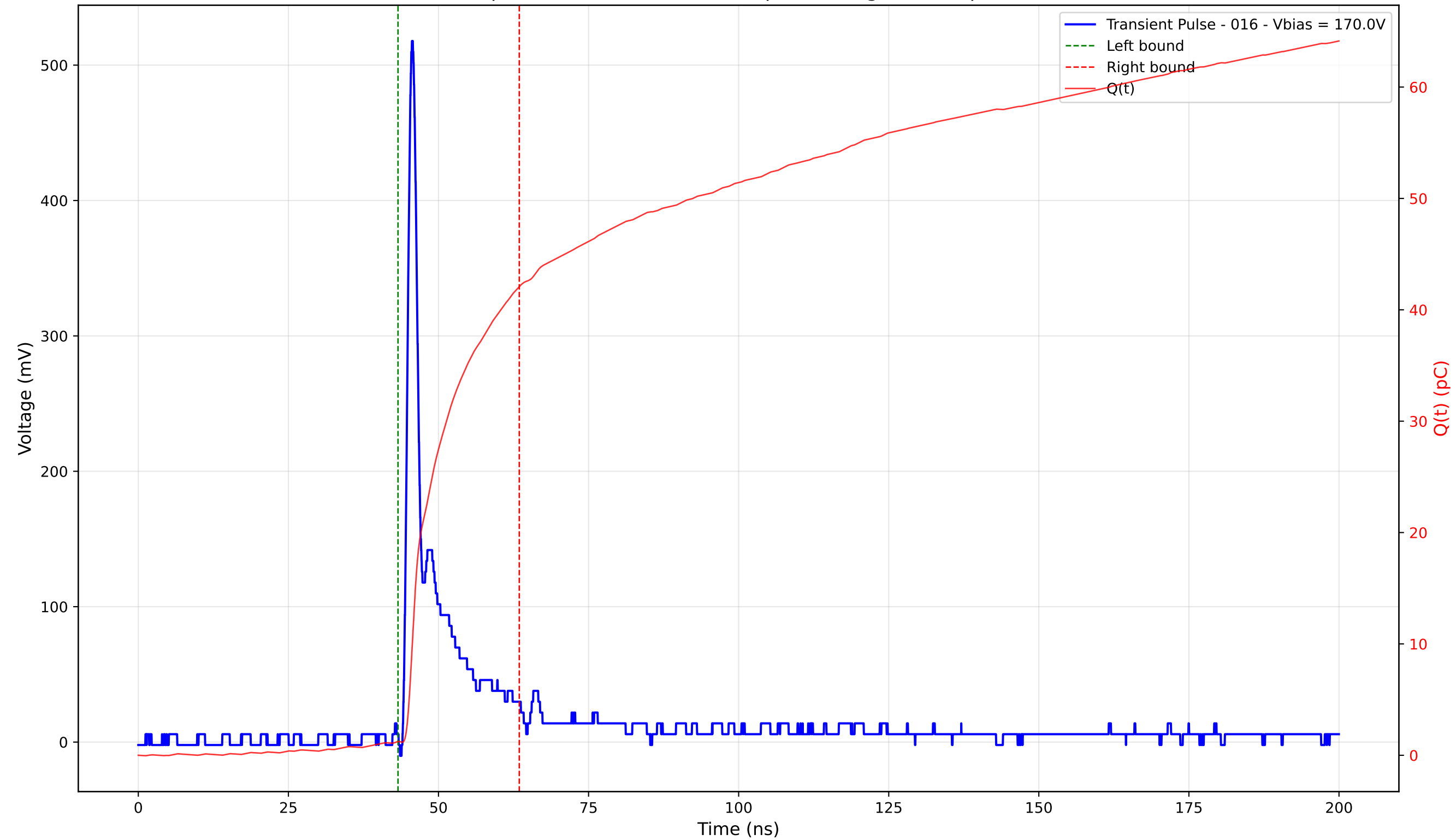
Transient Pulse - Sample: 4003 - Position: 175.0 \mu\text{m} - Charge: 40.86 pC - Rise Time: 1.02 ns
