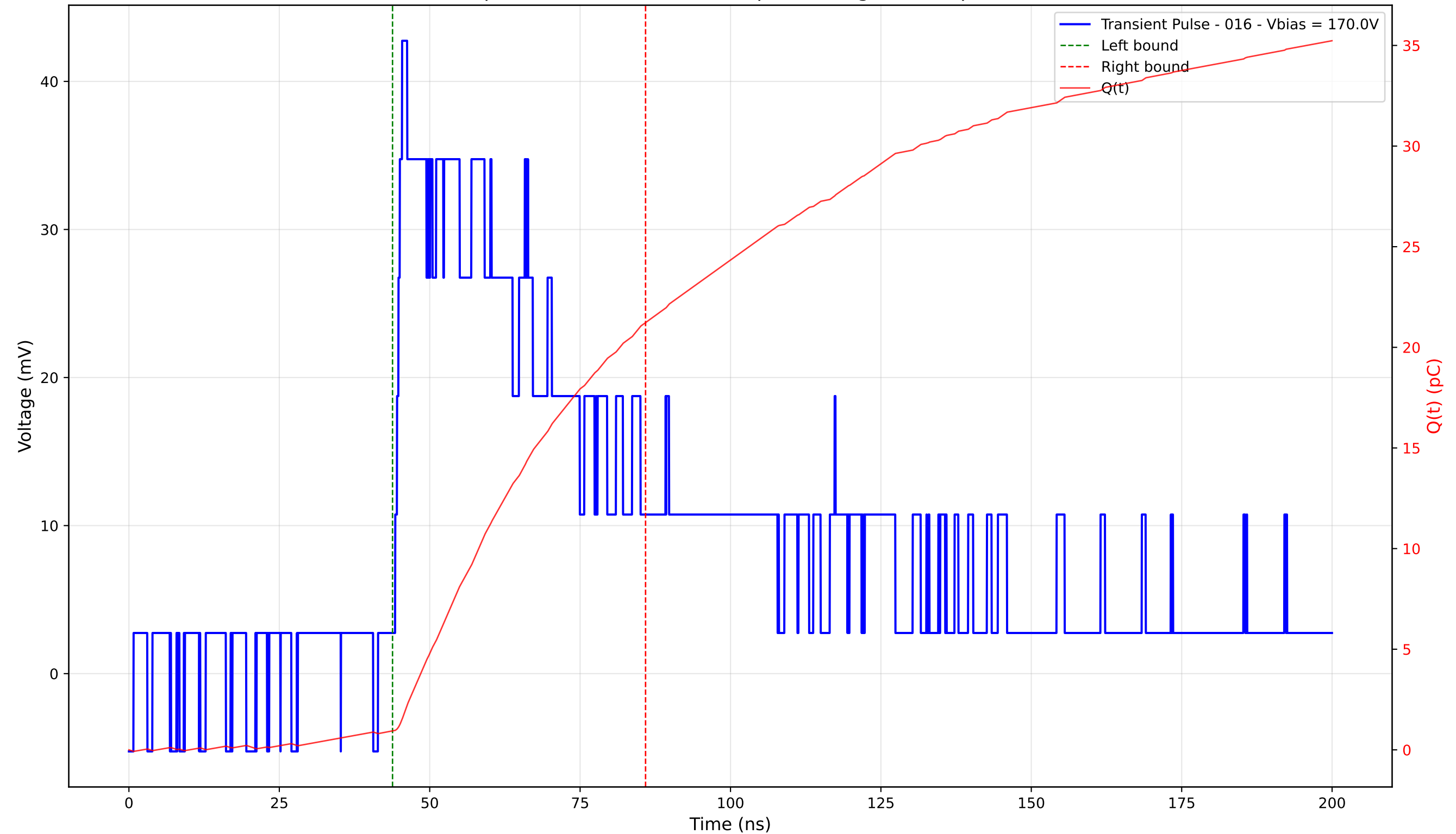
Transient Pulse - Sample: 4003 - Position: 325.0 \mu\text{m} - Charge: 20.29 pC - Rise Time: 1.16 ns
