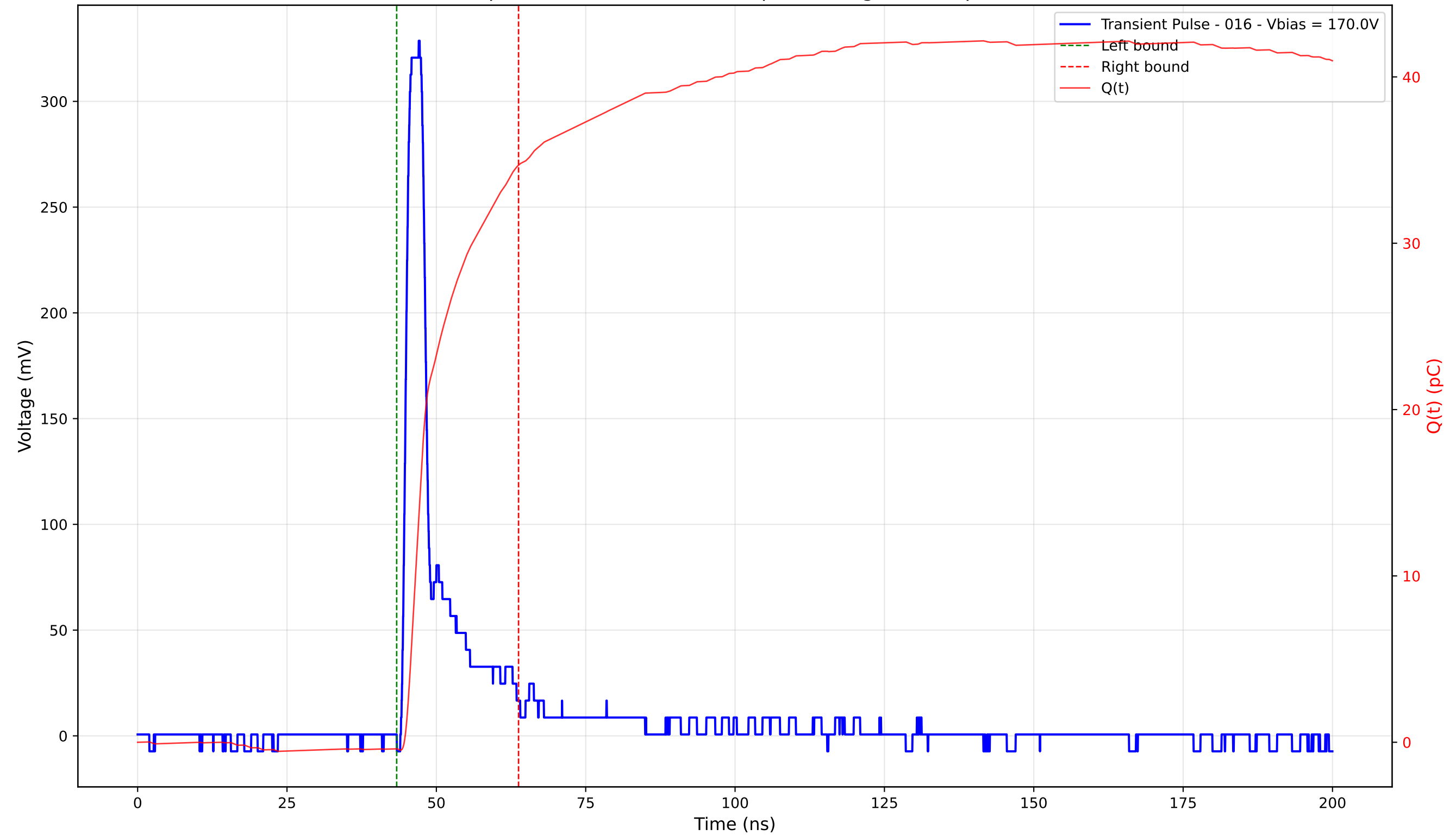
Transient Pulse - Sample: 4003 - Position: 260.0 \mu\text{m} - Charge: 35.08 pC - Rise Time: 1.18 ns
