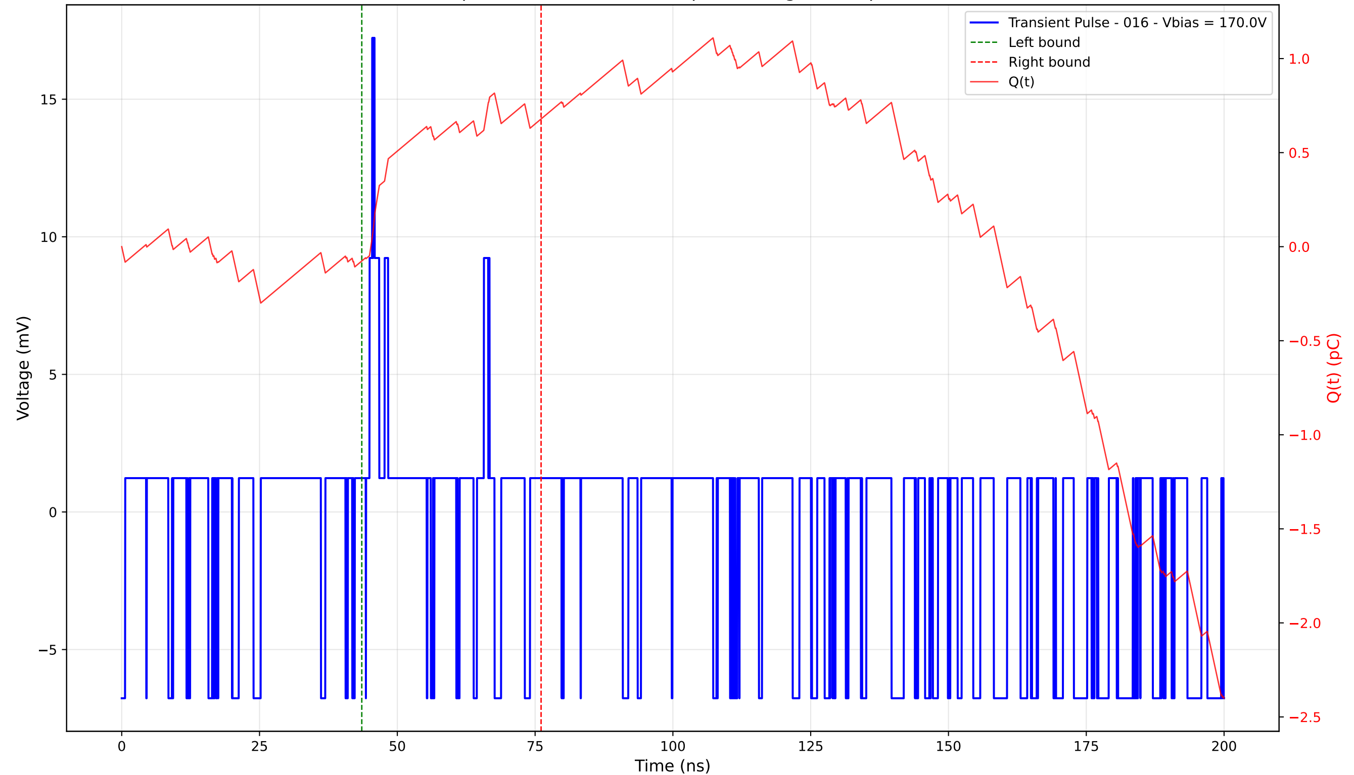
Transient Pulse - Sample: 4003 - Position: 0.0 \mu\text{m} - Charge: 0.75 pC - Rise Time: 0.50 ns
