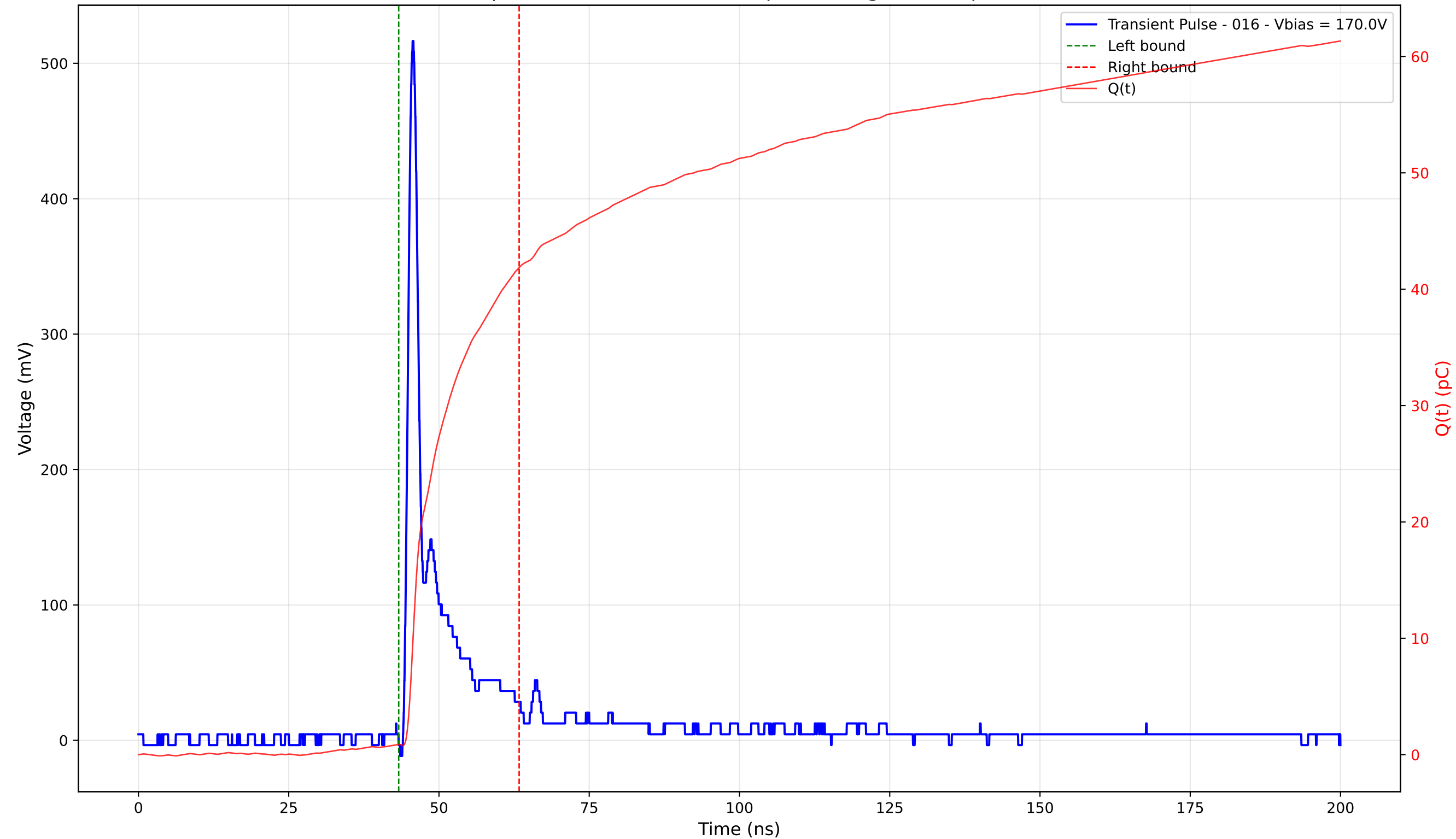
Transient Pulse - Sample: 4003 - Position: 180.0 \mu\text{m} - Charge: 40.97 pC - Rise Time: 1.03 ns
