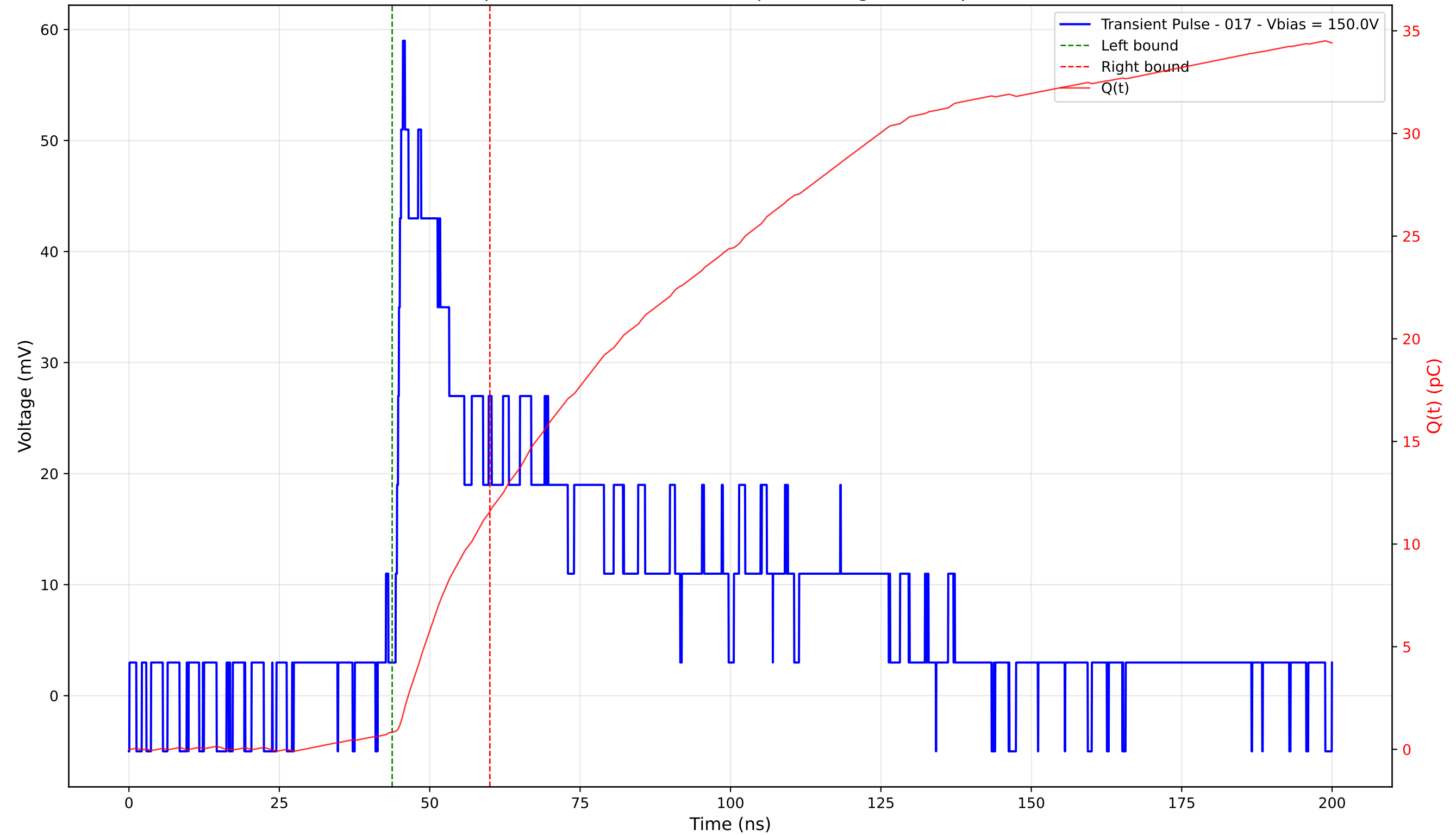
Transient Pulse - Sample: 4003 - Position: 305.0 \mu\text{m} - Charge: 10.76 pC - Rise Time: 1.21 ns
