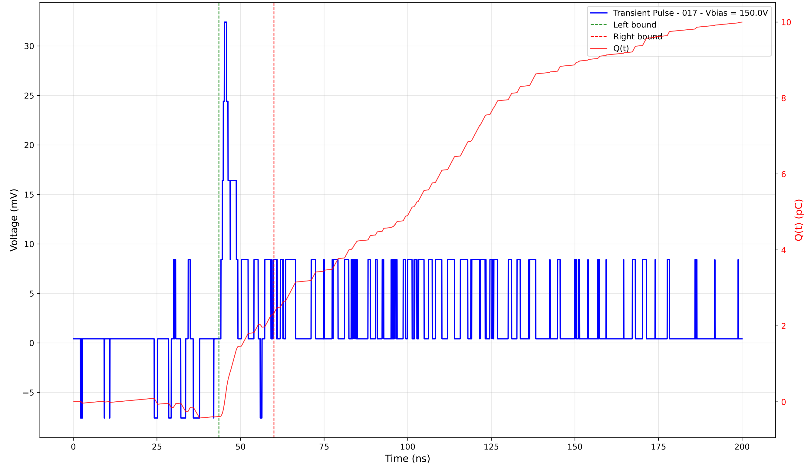
Transient Pulse - Sample: 4003 - Position: 335.0 \mu\text{m} - Charge: 2.72 pC - Rise Time: 1.03 ns
