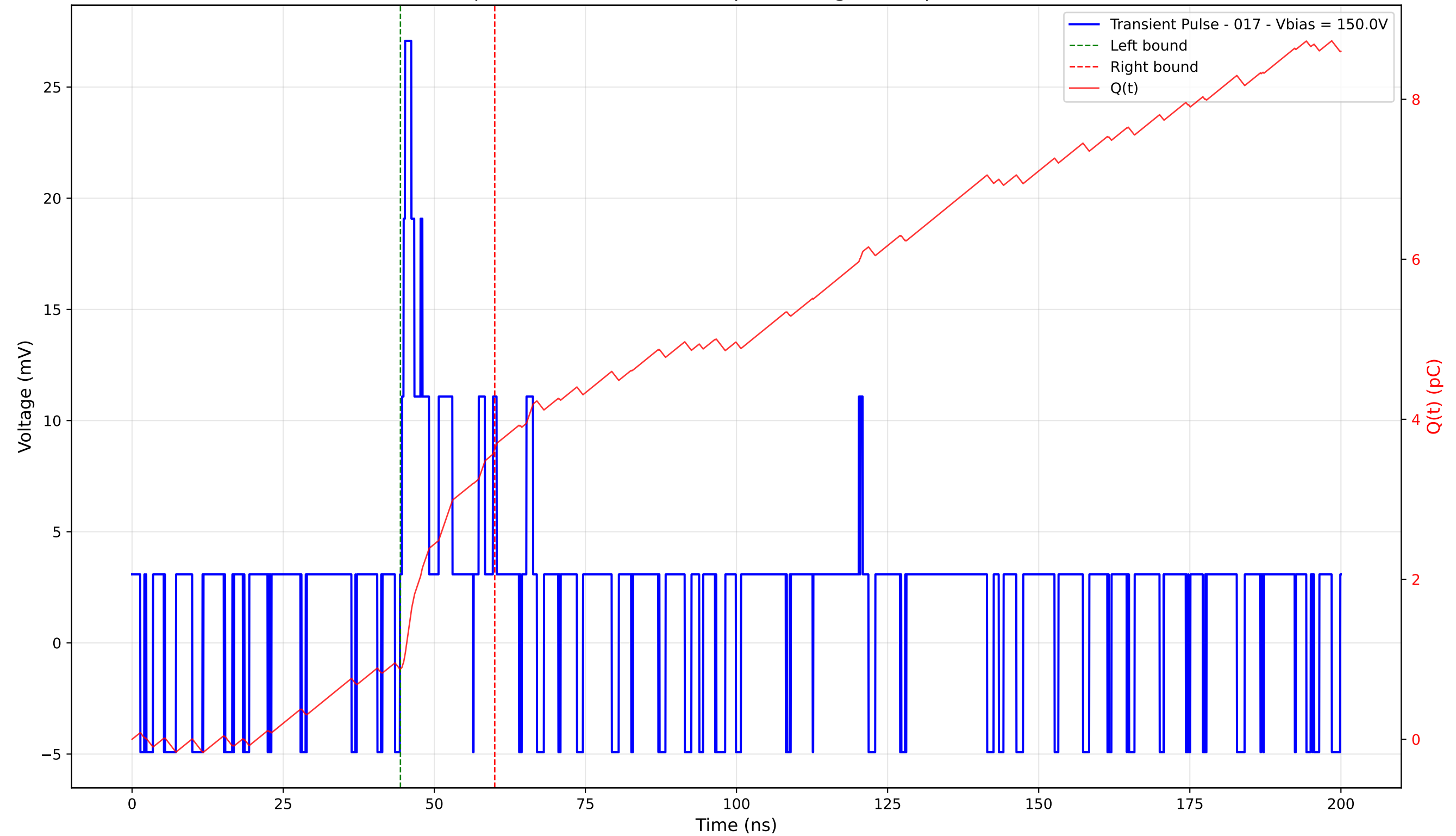
Transient Pulse - Sample: 4003 - Position: 35.0 \mu\text{m} - Charge: 2.75 pC - Rise Time: 0.00 ns (N/A)
