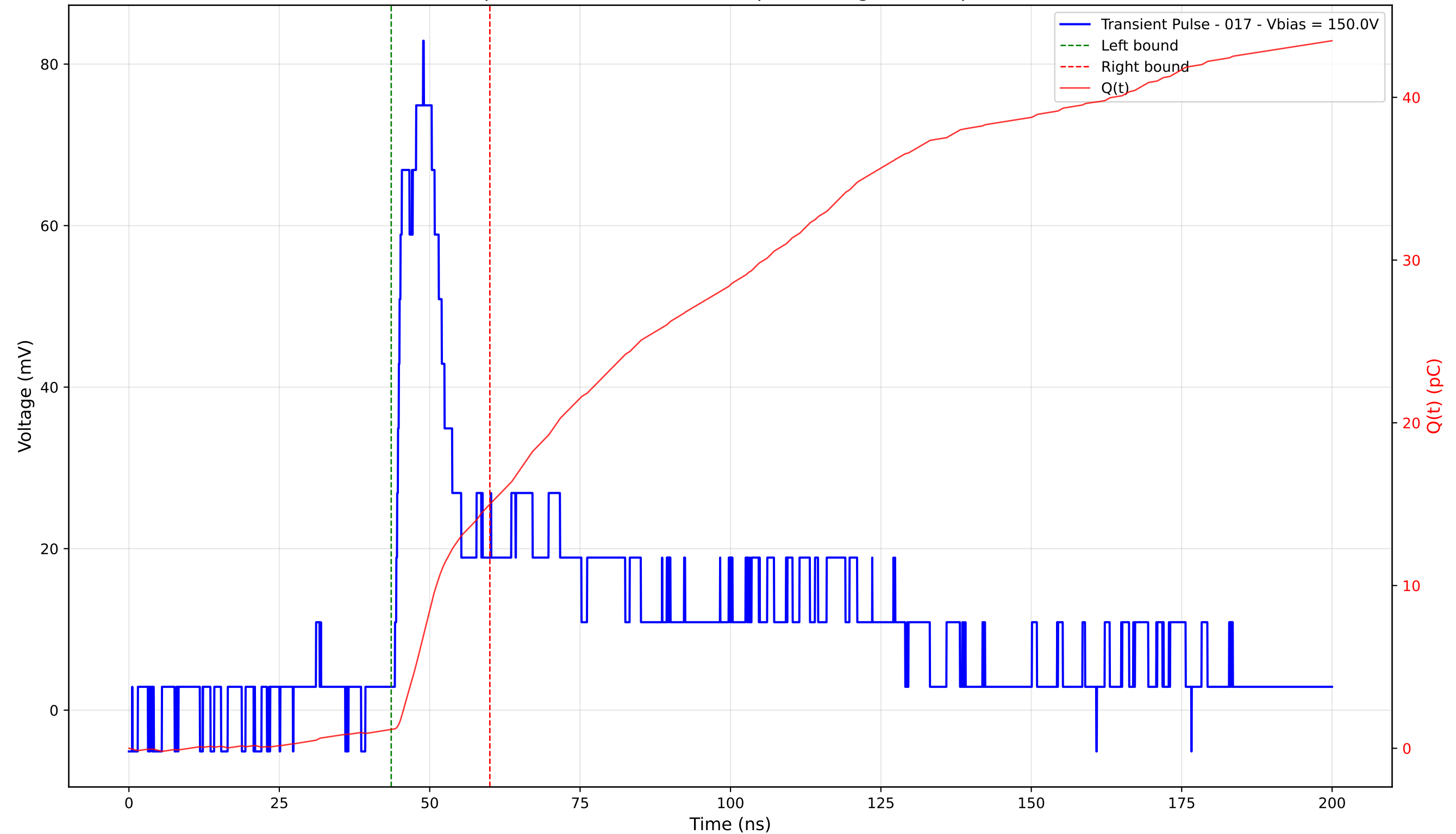
Transient Pulse - Sample: 4003 - Position: 300.0 \mu\text{m} - Charge: 13.84 pC - Rise Time: 3.53 ns
