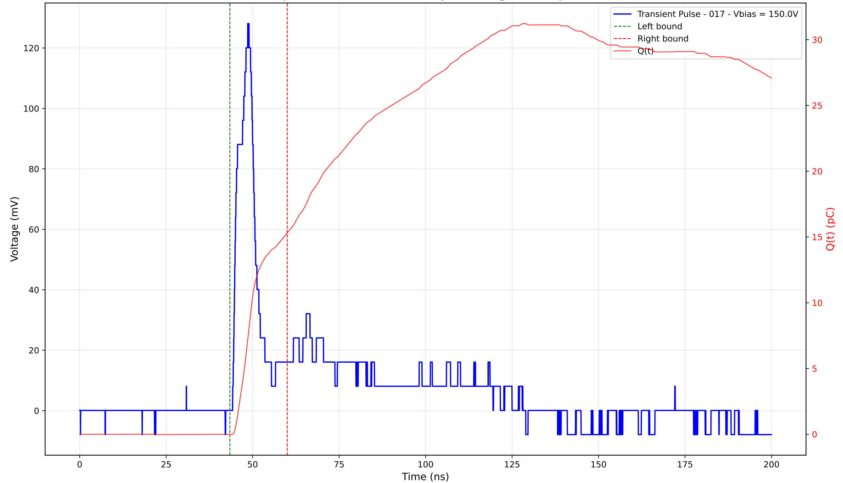
Transient Pulse - Sample: 4003 - Position: 295.0 \mu\text{m} - Charge: 15.31 pC - Rise Time: 3.71 ns
