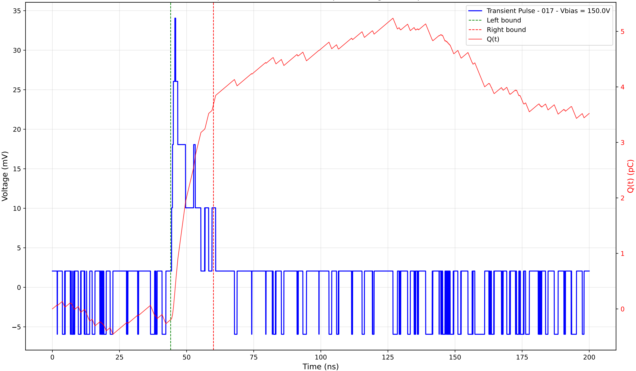
Transient Pulse - Sample: 4003 - Position: 45.0 \mu\text{m} - Charge: 3.88 pC - Rise Time: 1.22 ns
