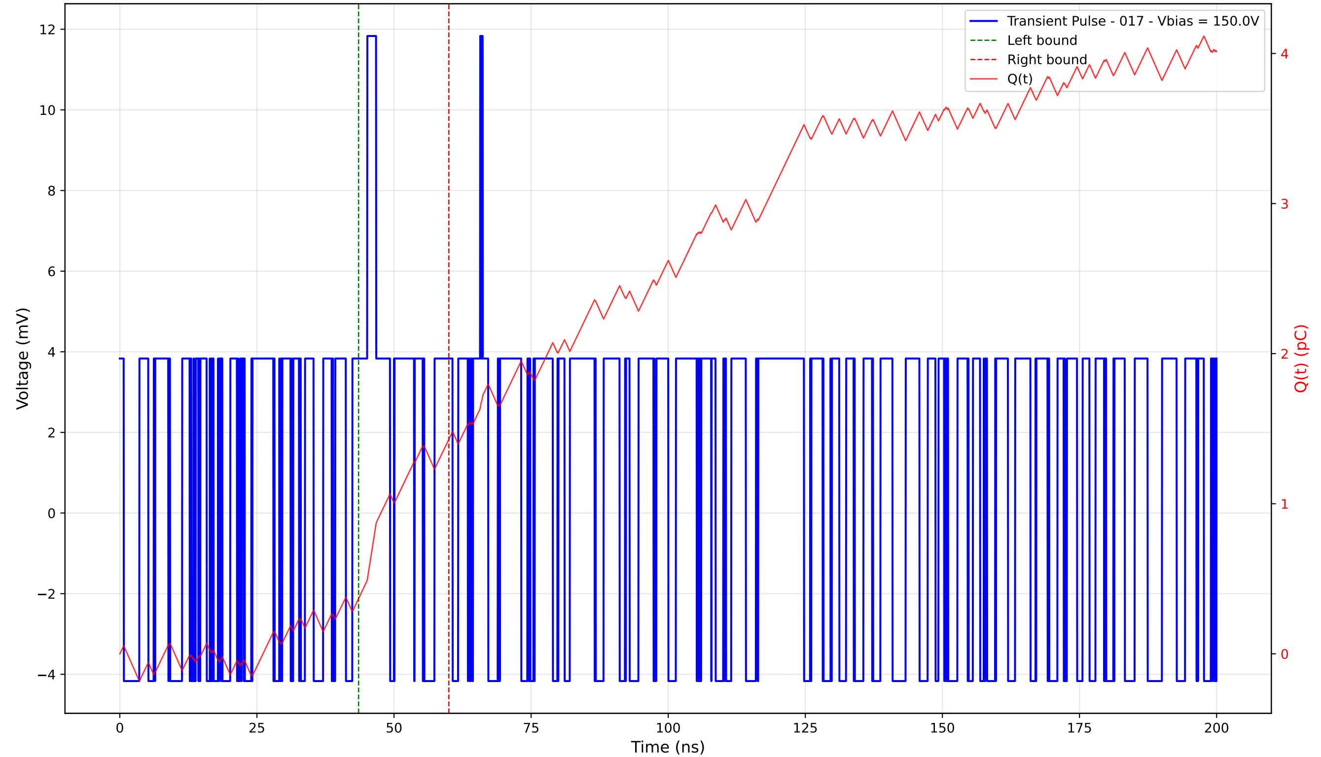
Transient Pulse - Sample: 4003 - Position: 0.0 \mu\text{m} - Charge: 1.06 pC - Rise Time: 0.00 ns (N/A)
