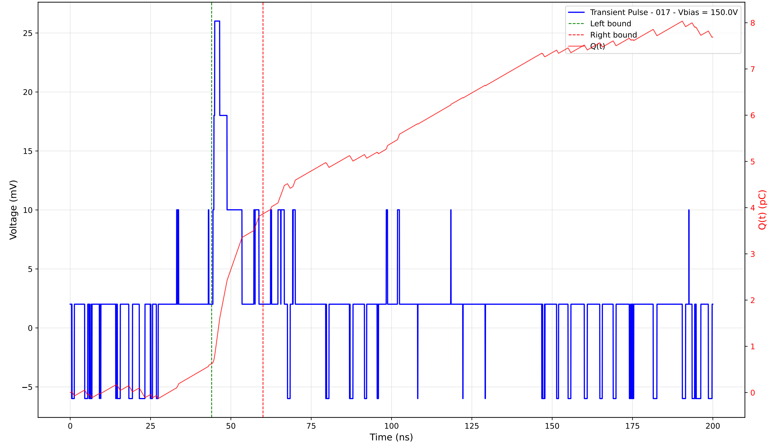
Transient Pulse - Sample: 4003 - Position: 370.0 \mu\text{m} - Charge: 3.24 pC - Rise Time: 0.56 ns
