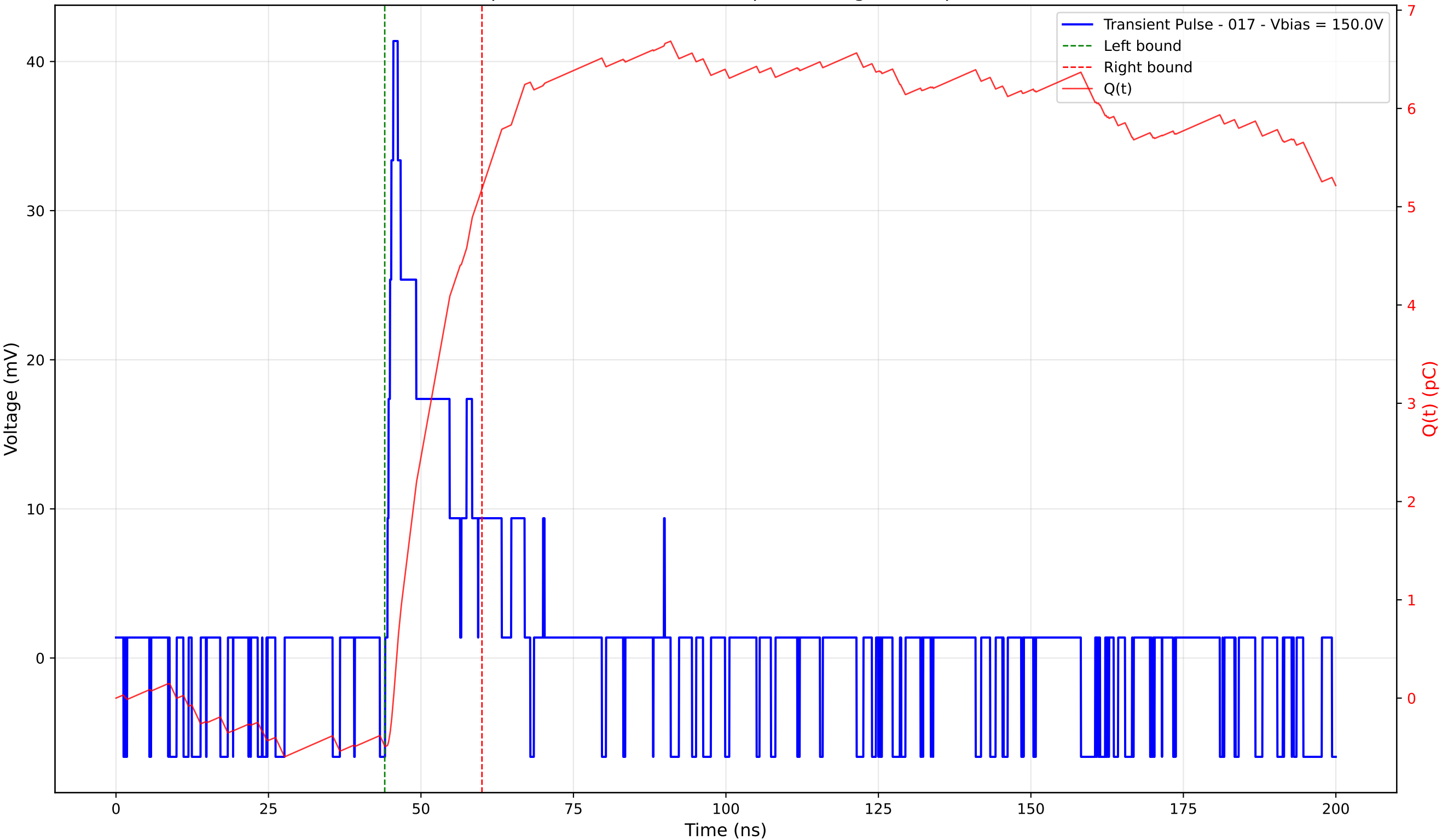
Transient Pulse - Sample: 4003 - Position: 50.0 \mu\text{m} - Charge: 5.67 pC - Rise Time: 0.95 ns
