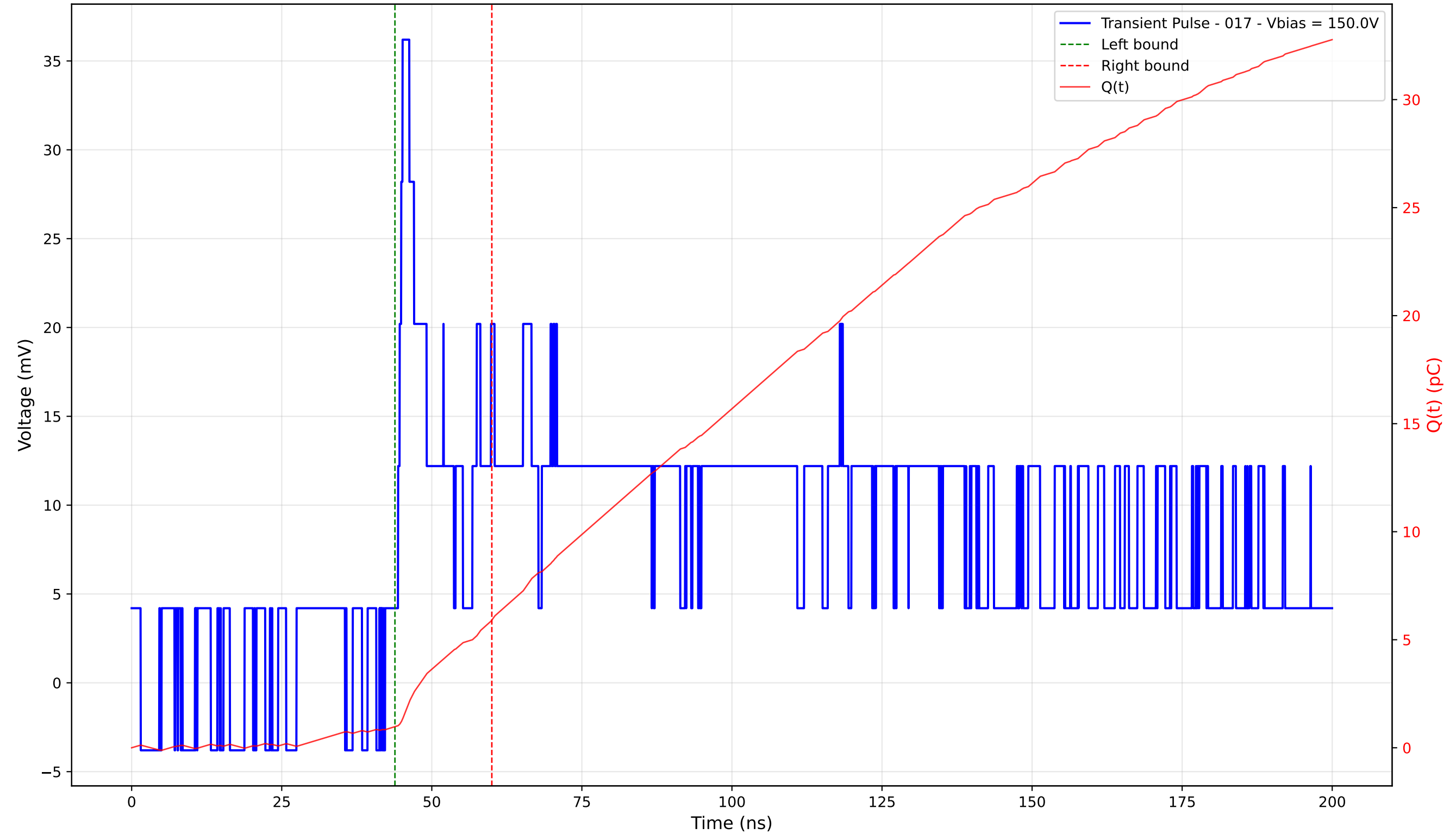
Transient Pulse - Sample: 4003 - Position: 320.0 \mu\text{m} - Charge: 4.94 pC - Rise Time: 0.00 ns (N/A)
