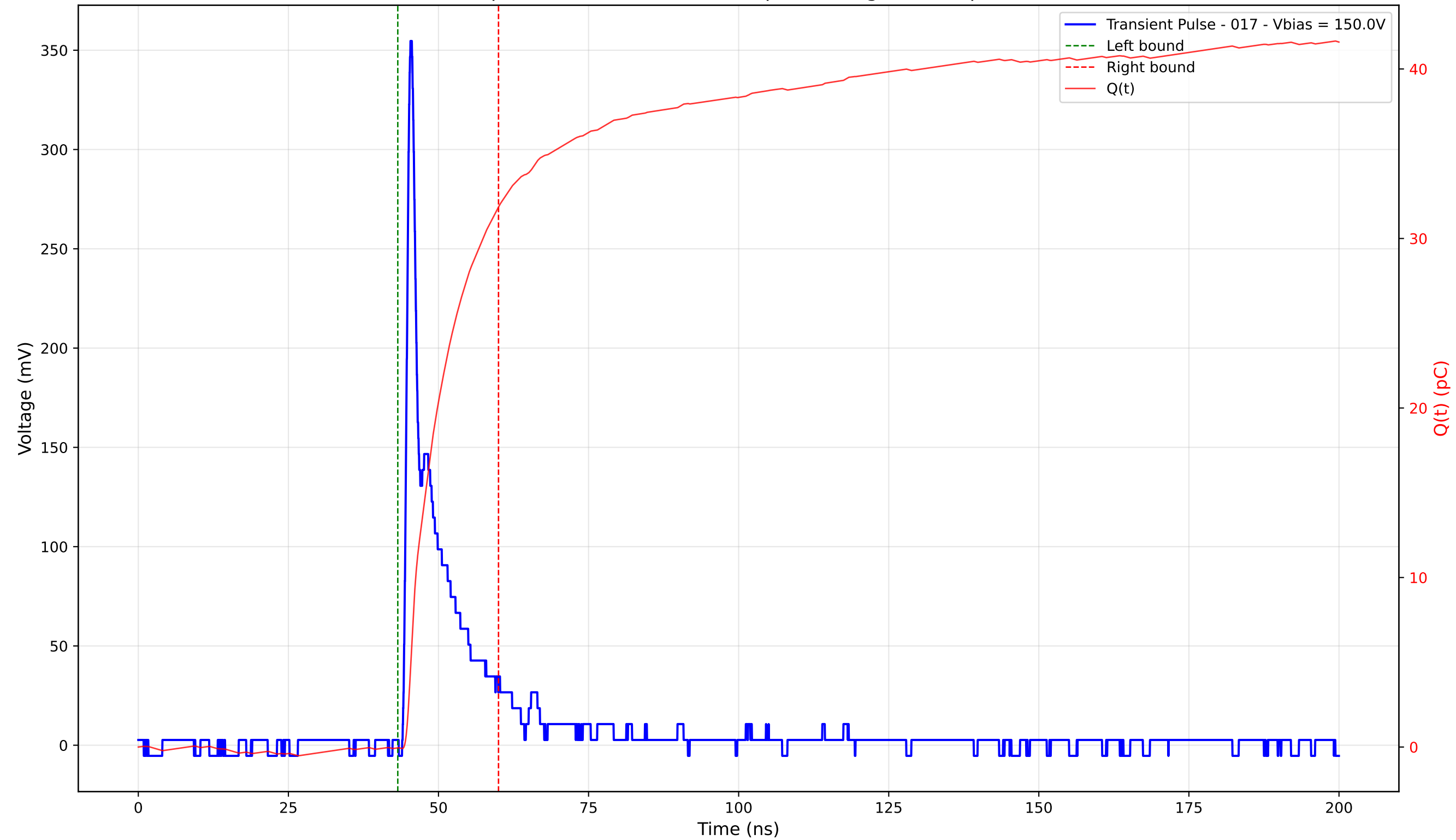
Transient Pulse - Sample: 4003 - Position: 110.0 \mu\text{m} - Charge: 31.90 pC - Rise Time: 0.88 ns
