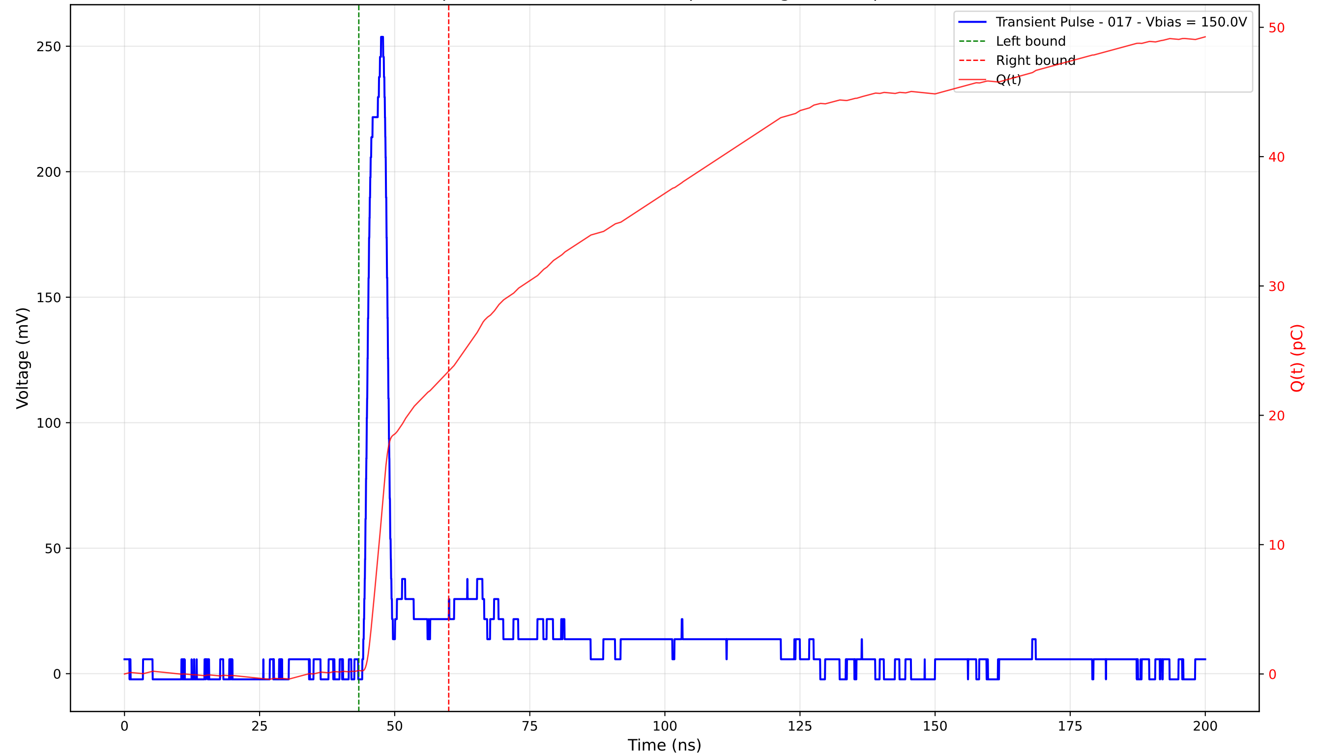
Transient Pulse - Sample: 4003 - Position: 270.0 \mu\text{m} - Charge: 23.14 pC - Rise Time: 2.53 ns
