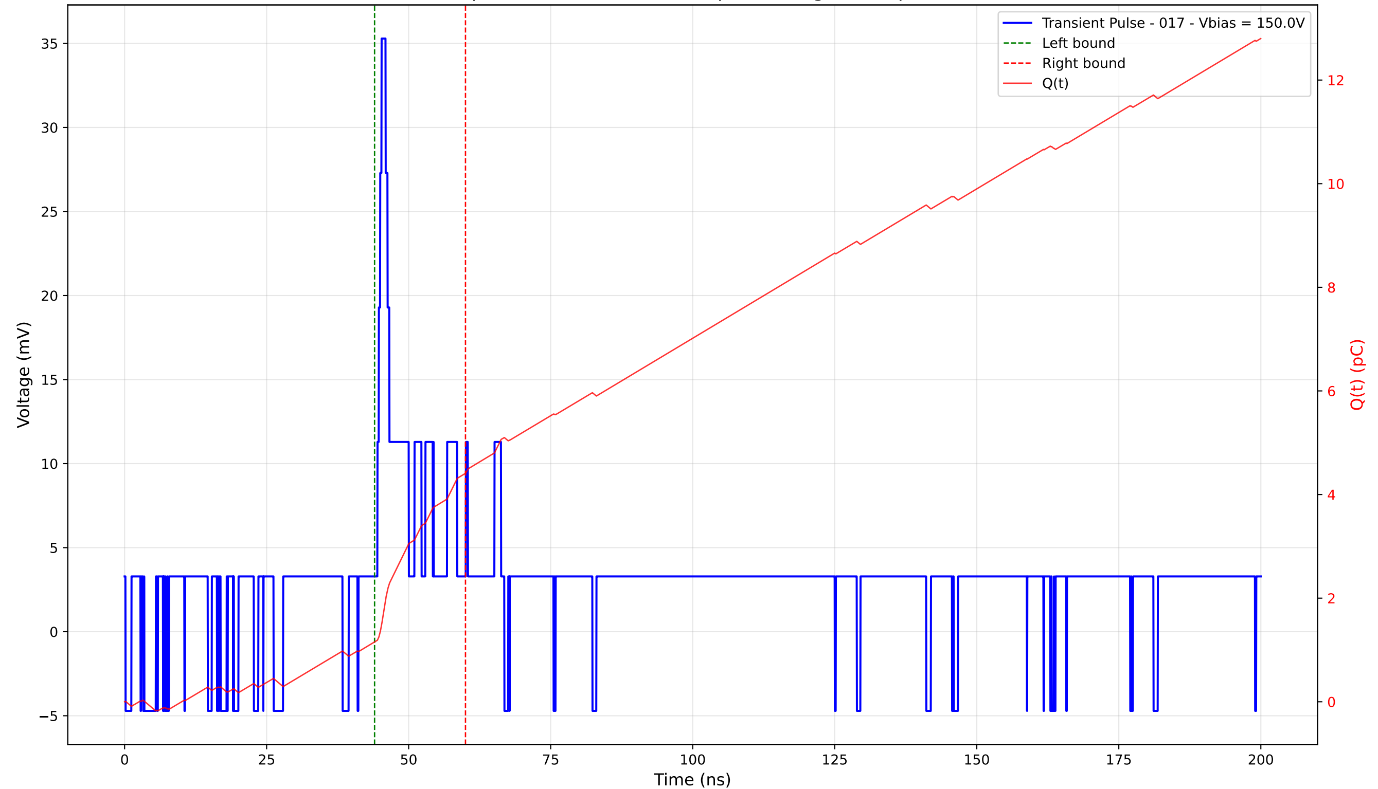
Transient Pulse - Sample: 4003 - Position: 80.0 \mu\text{m} - Charge: 3.25 pC - Rise Time: 0.74 ns
