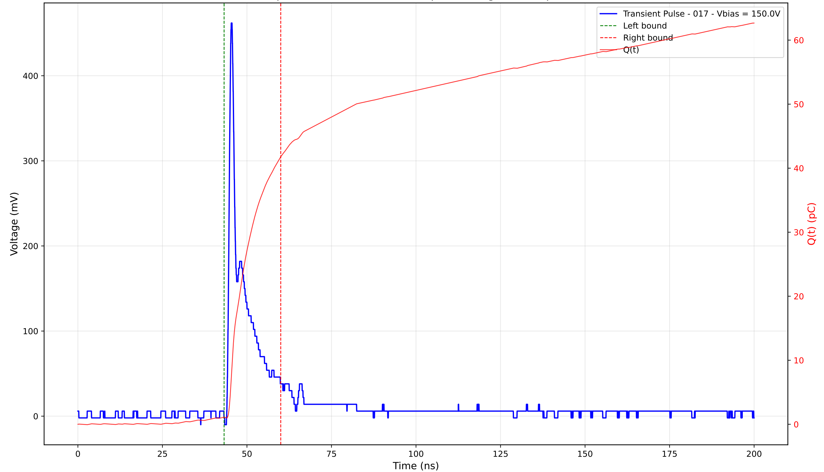
Transient Pulse - Sample: 4003 - Position: 125.0 \mu\text{m} - Charge: 40.68 pC - Rise Time: 0.90 ns
