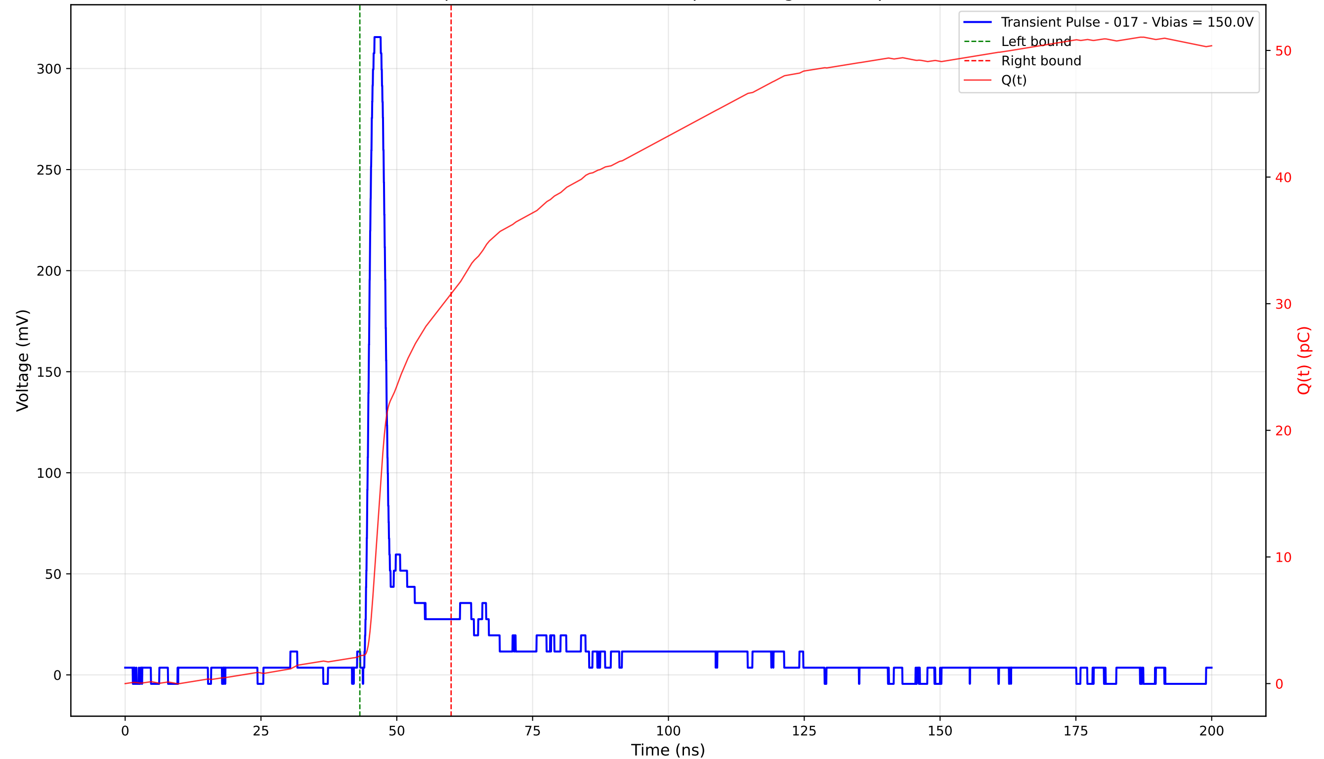
Transient Pulse - Sample: 4003 - Position: 245.0 \mu\text{m} - Charge: 28.58 pC - Rise Time: 1.23 ns
