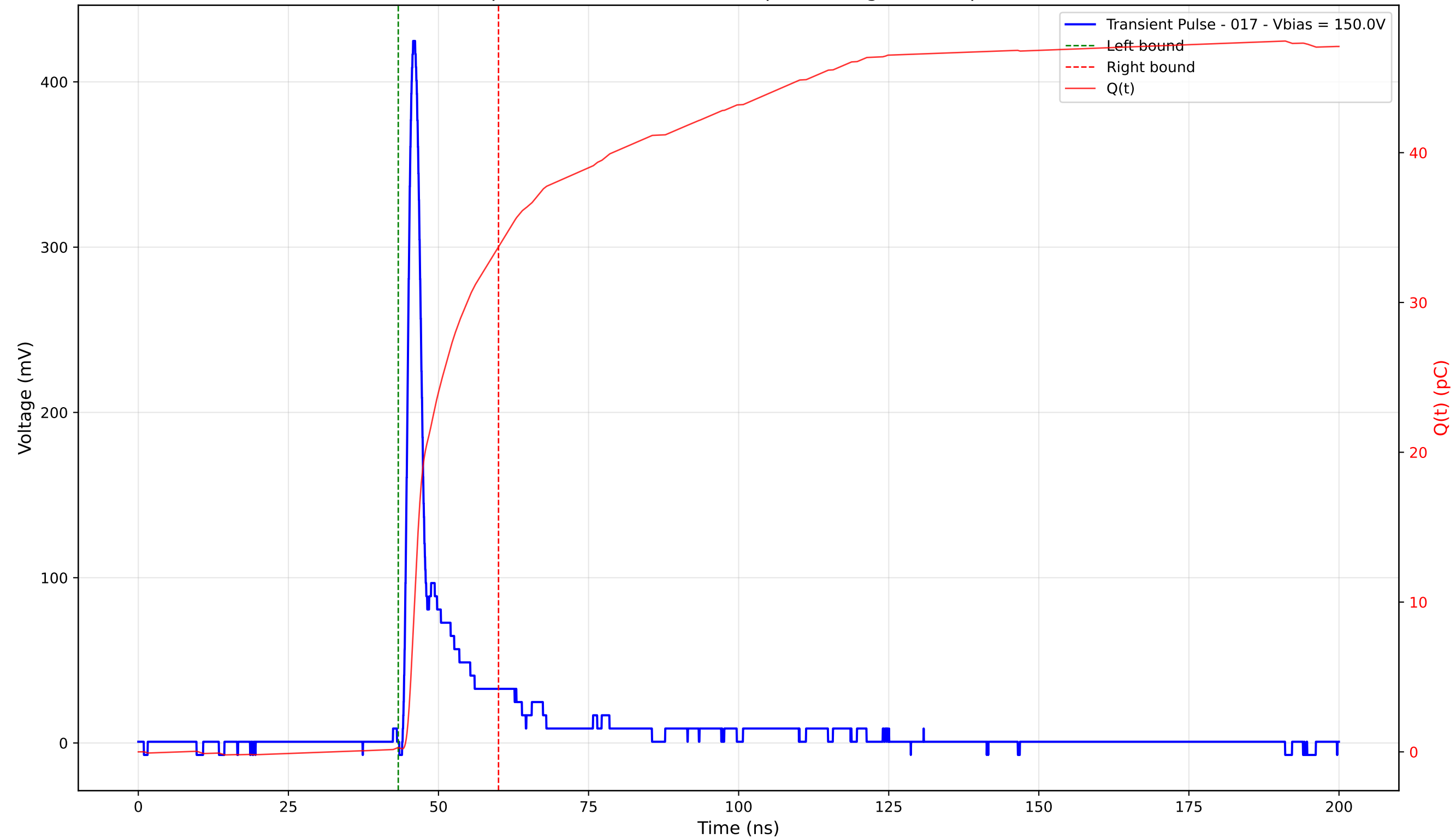
Transient Pulse - Sample: 4003 - Position: 210.0 \mu\text{m} - Charge: 33.46 pC - Rise Time: 1.14 ns
