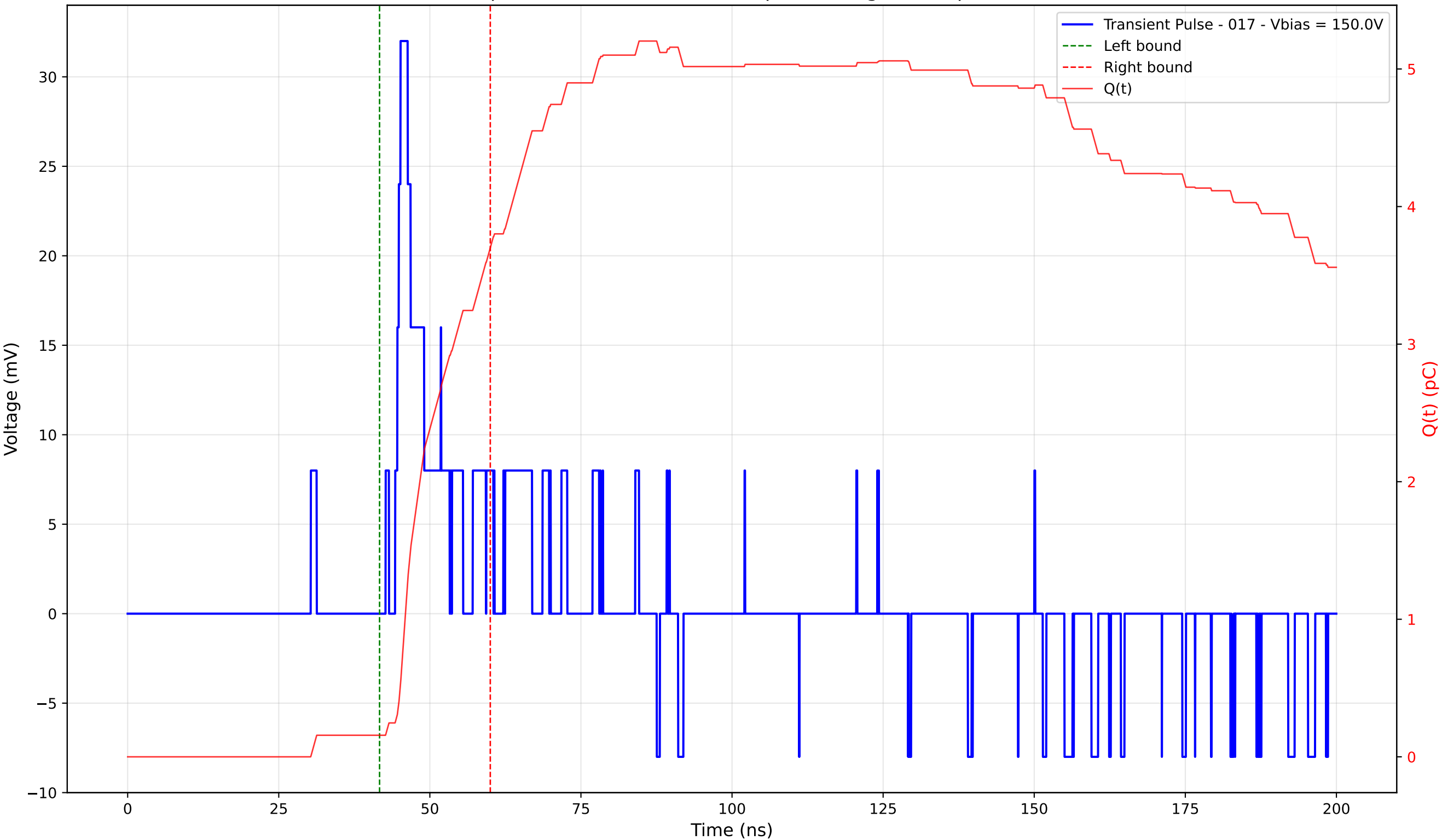
Transient Pulse - Sample: 4003 - Position: 365.0 \mu\text{m} - Charge: 3.54 pC - Rise Time: 0.89 ns
