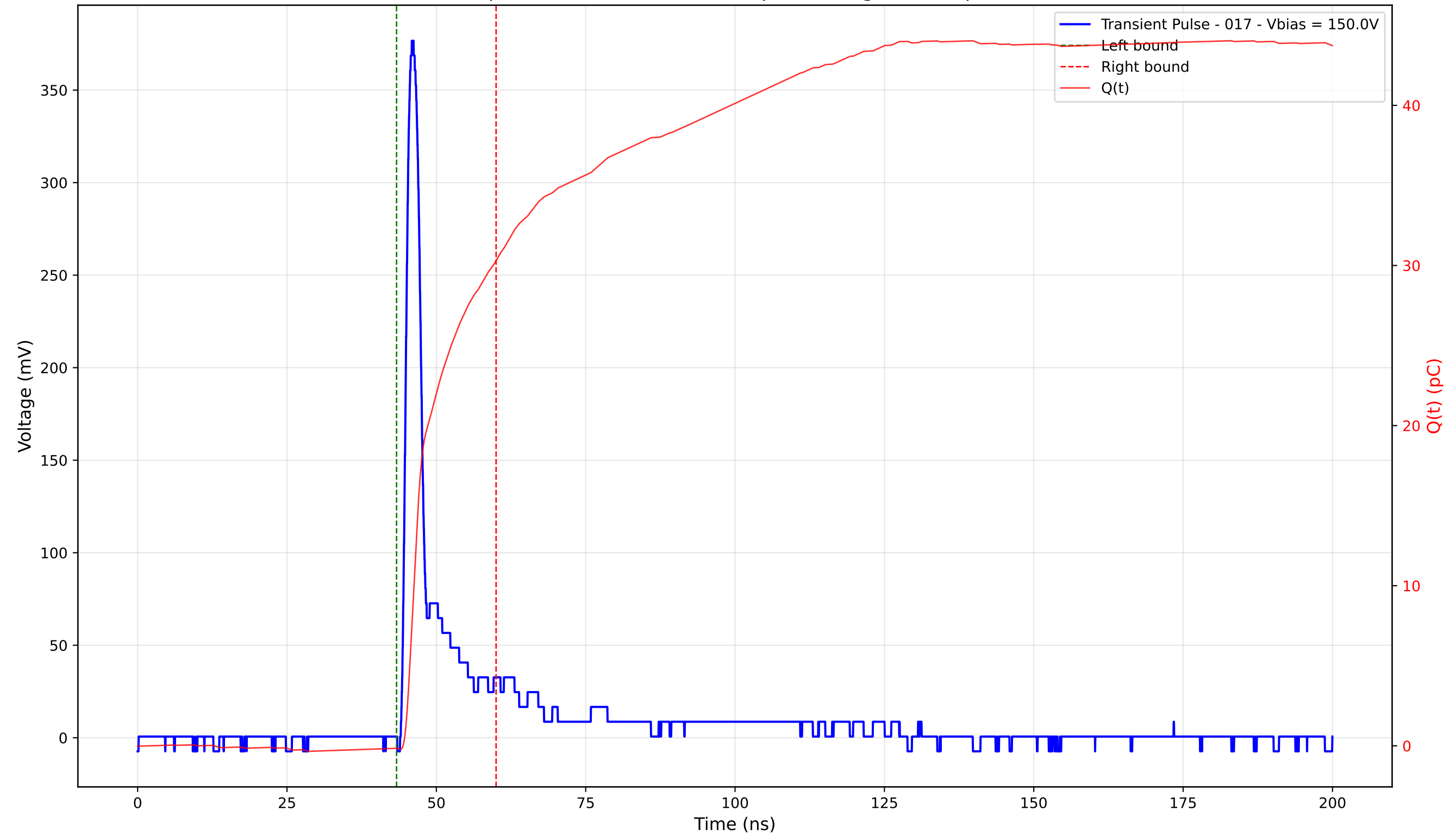
Transient Pulse - Sample: 4003 - Position: 225.0 \mu\text{m} - Charge: 30.46 pC - Rise Time: 1.17 ns
