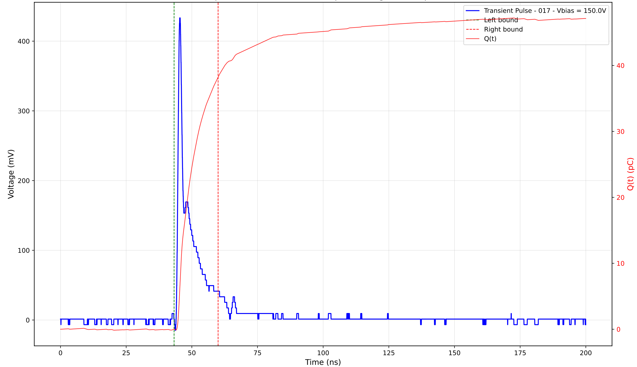
Transient Pulse - Sample: 4003 - Position: 120.0 \mu\text{m} - Charge: 38.21 pC - Rise Time: 0.91 ns
