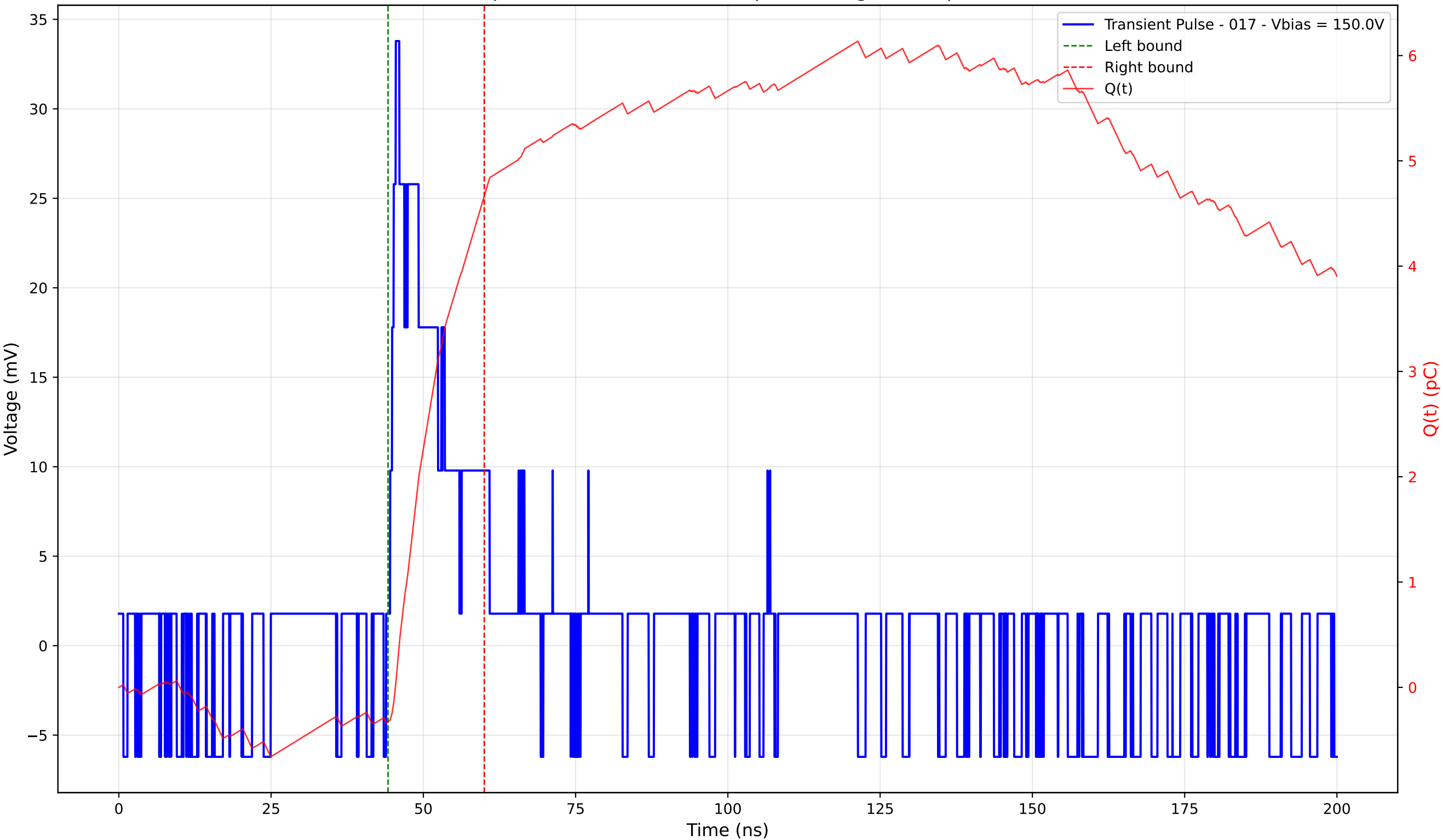
Transient Pulse - Sample: 4003 - Position: 60.0 \mu\text{m} - Charge: 5.00 pC - Rise Time: 0.94 ns
