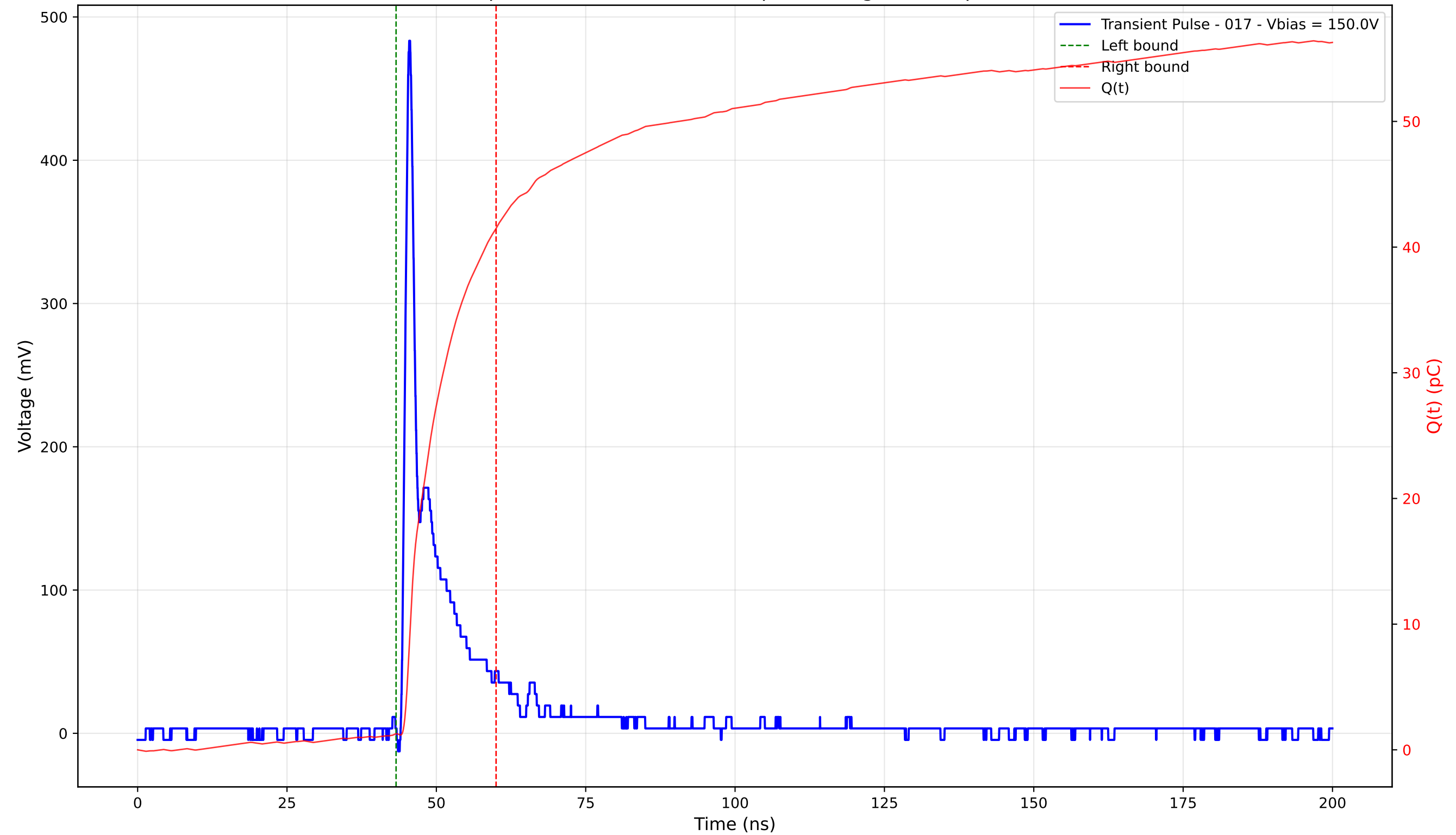
Transient Pulse - Sample: 4003 - Position: 140.0 \mu\text{m} - Charge: 40.21 pC - Rise Time: 0.93 ns
