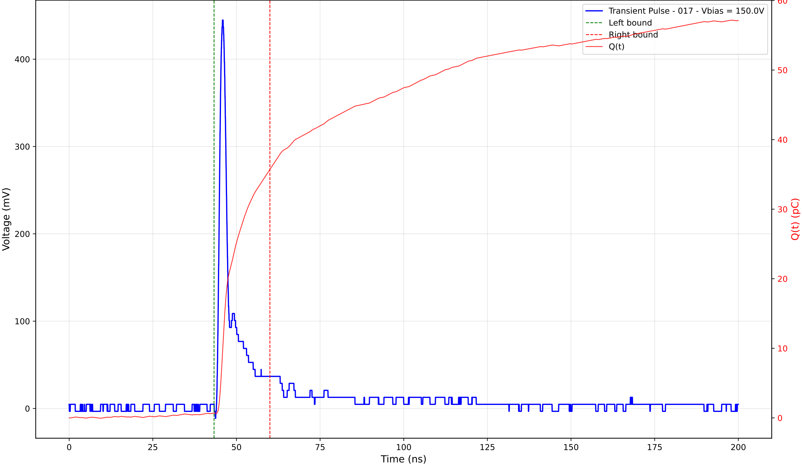
Transient Pulse - Sample: 4003 - Position: 205.0 \mu\text{m} - Charge: 35.02 pC - Rise Time: 1.16 ns
