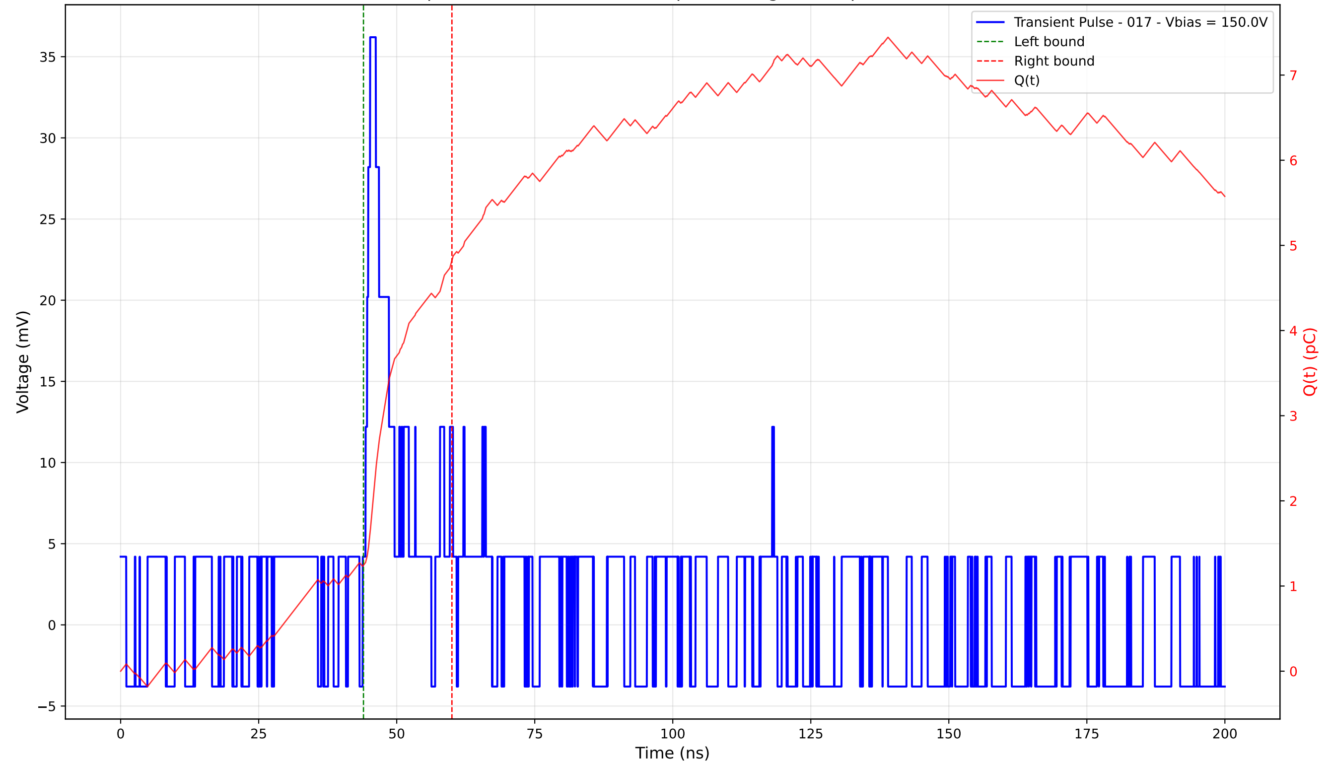
Transient Pulse - Sample: 4003 - Position: 405.0 \mu\text{m} - Charge: 3.58 pC - Rise Time: 0.00 ns (N/A)
