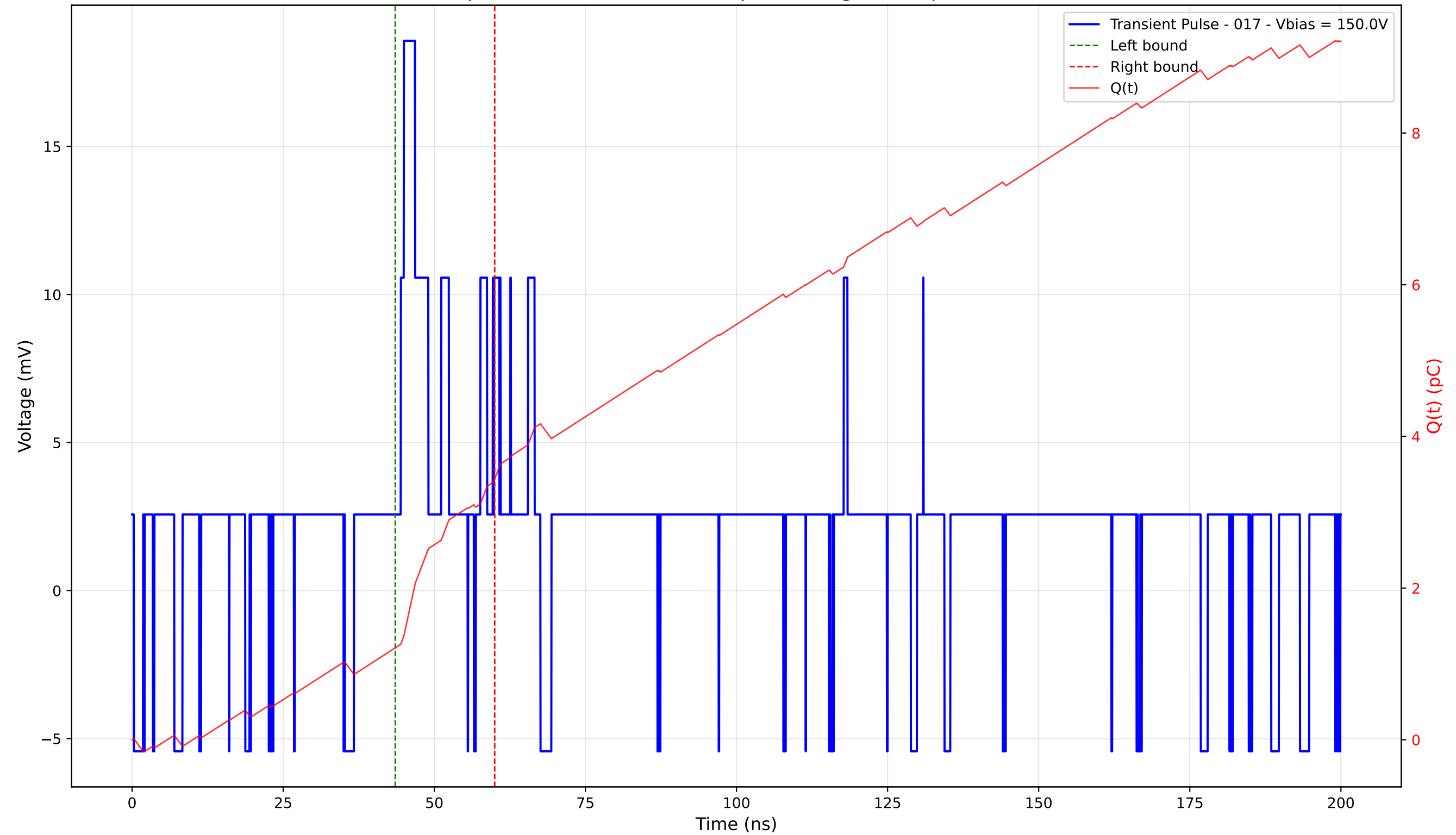
Transient Pulse - Sample: 4003 - Position: 415.0 \mu\text{m} - Charge: 2.23 pC - Rise Time: 0.00 ns (N/A)
