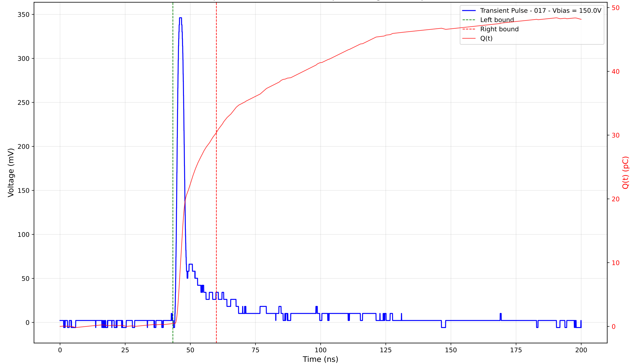
Transient Pulse - Sample: 4003 - Position: 235.0 \mu\text{m} - Charge: 29.91 pC - Rise Time: 1.14 ns
