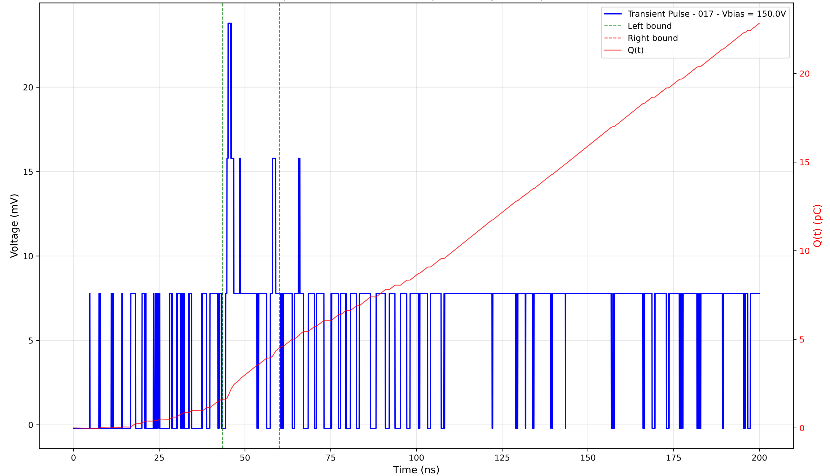
Transient Pulse - Sample: 4003 - Position: 75.0 \mu\text{m} - Charge: 2.88 pC - Rise Time: 0.73 ns
