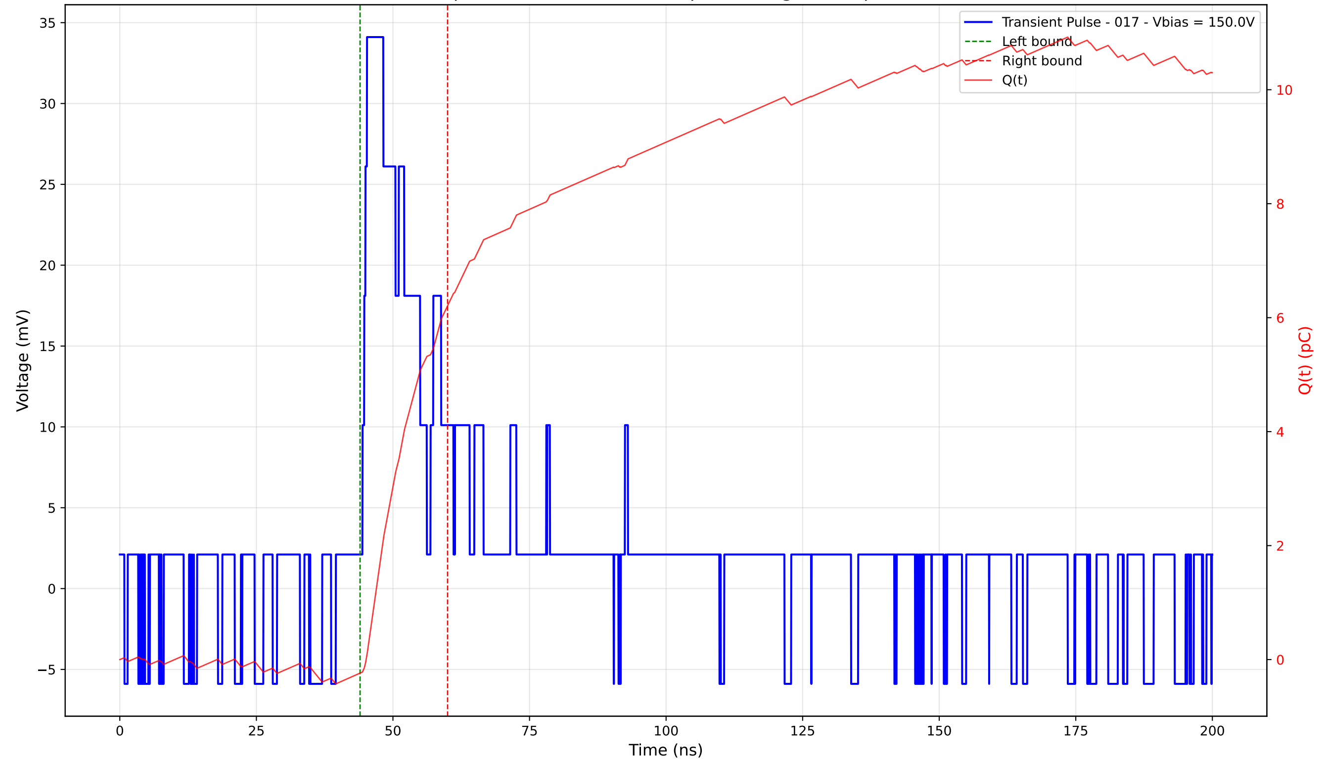
Transient Pulse - Sample: 4003 - Position: 55.0 \mu\text{m} - Charge: 6.45 pC - Rise Time: 0.84 ns
