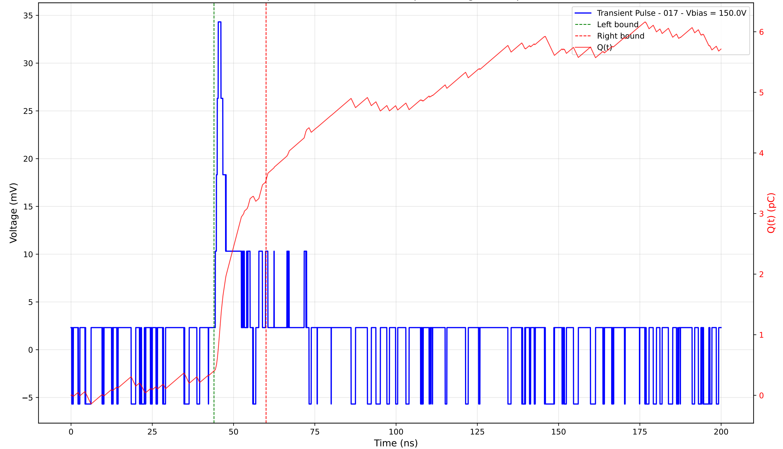
Transient Pulse - Sample: 4003 - Position: 375.0 \mu\text{m} - Charge: 3.15 pC - Rise Time: 0.92 ns
