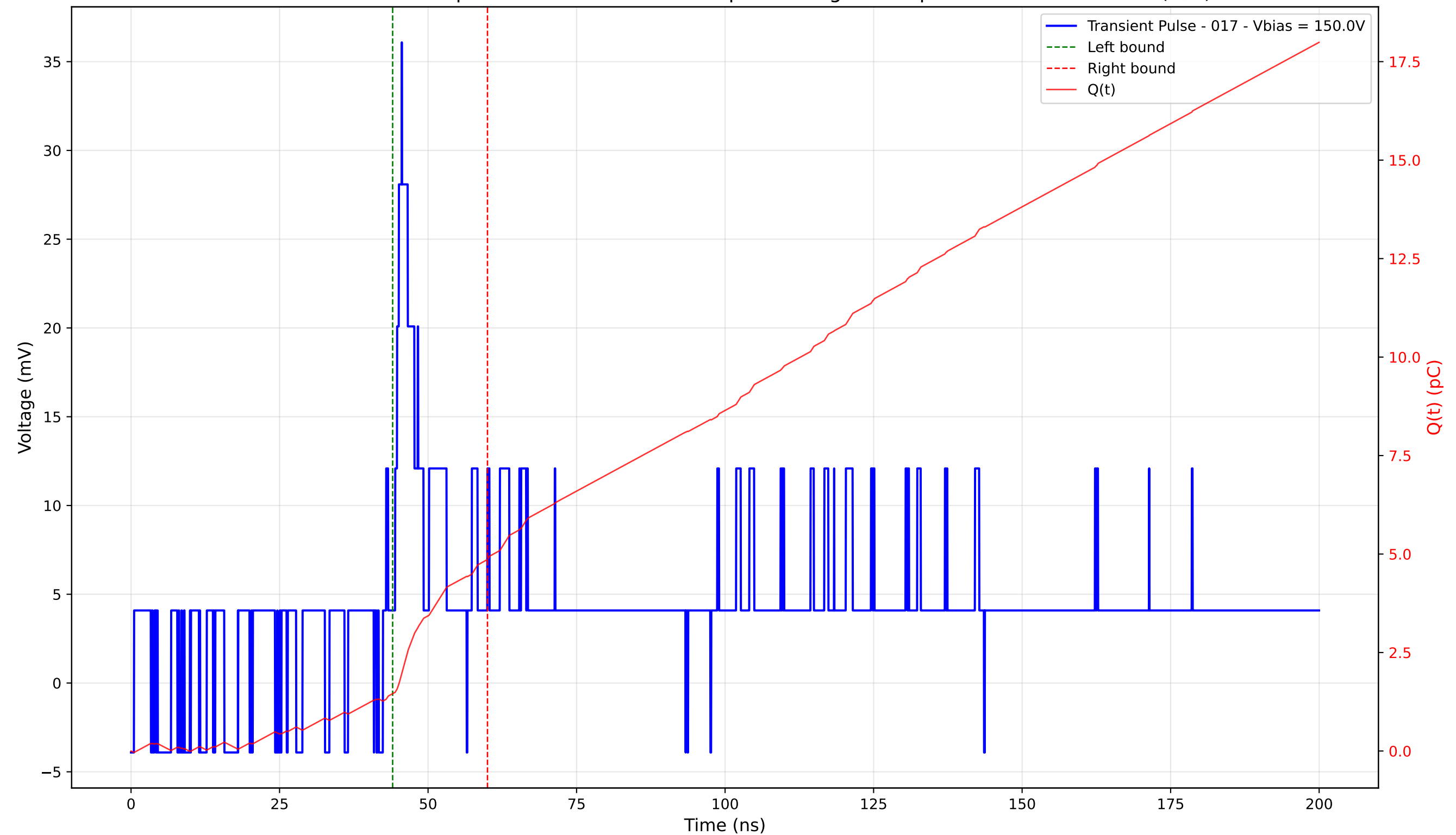
Transient Pulse - Sample: 4003 - Position: 345.0 \mu\text{m} - Charge: 3.41 pC - Rise Time: 0.00 ns (N/A)
