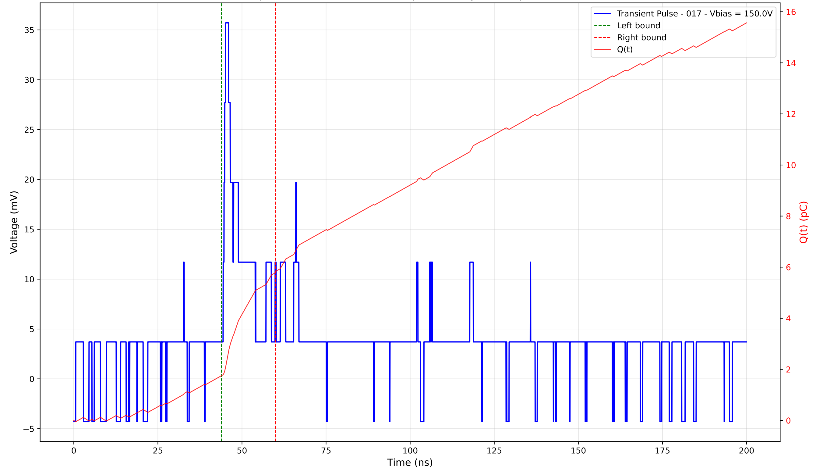
Transient Pulse - Sample: 4003 - Position: 360.0 \mu\text{m} - Charge: 4.06 pC - Rise Time: 0.00 ns (N/A)
