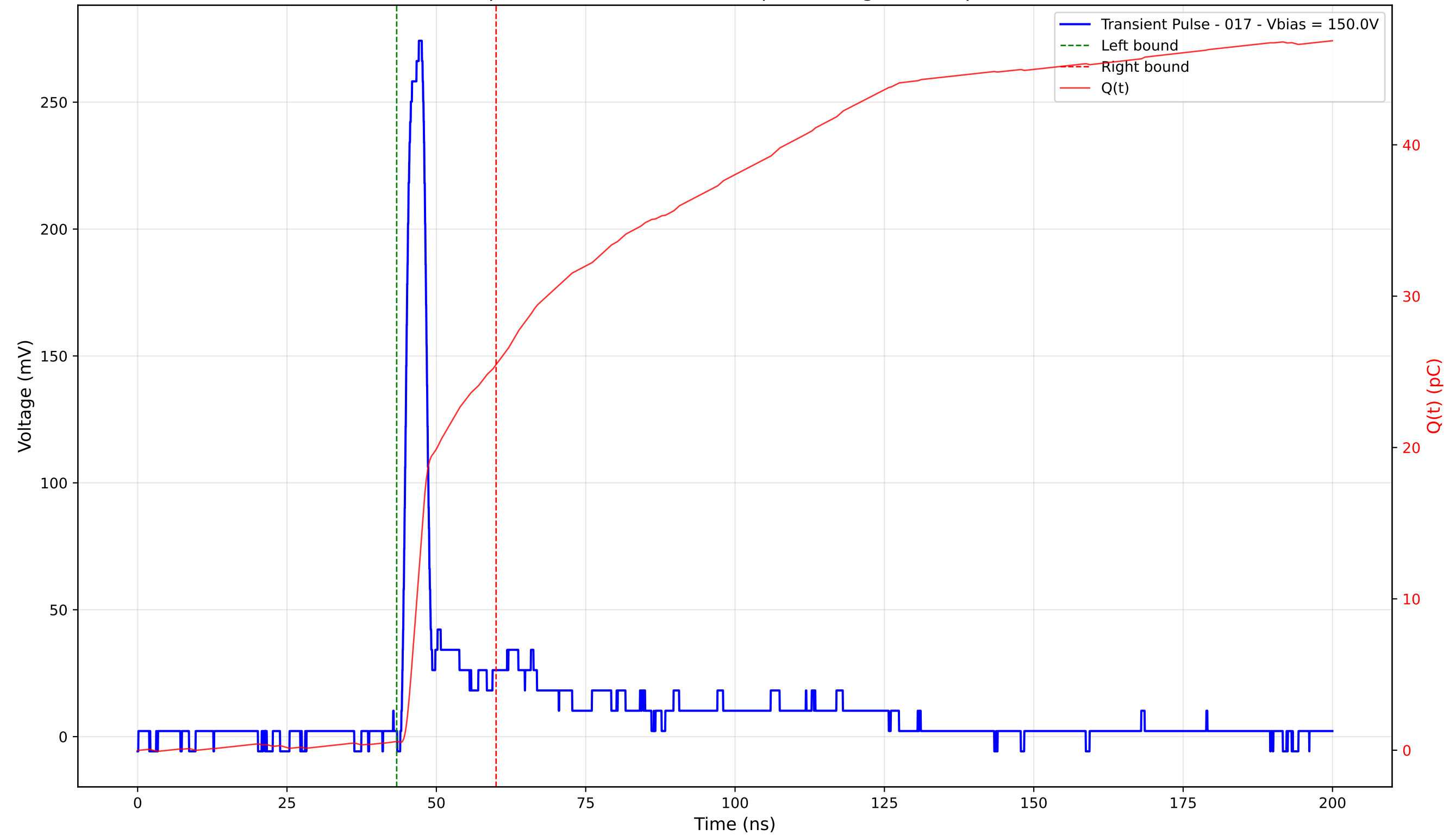
Transient Pulse - Sample: 4003 - Position: 260.0 \mu\text{m} - Charge: 24.90 pC - Rise Time: 1.38 ns
