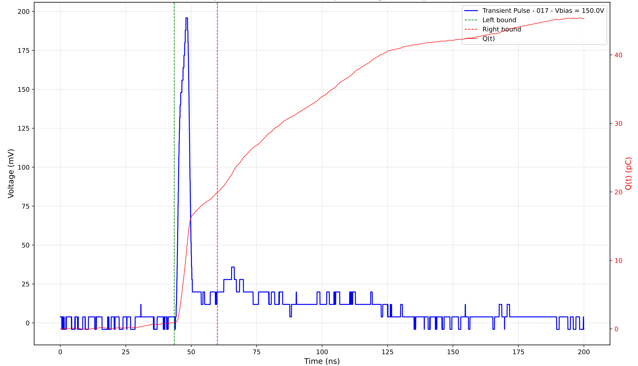
Transient Pulse - Sample: 4003 - Position: 285.0 \mu\text{m} - Charge: 18.91 pC - Rise Time: 3.10 ns
