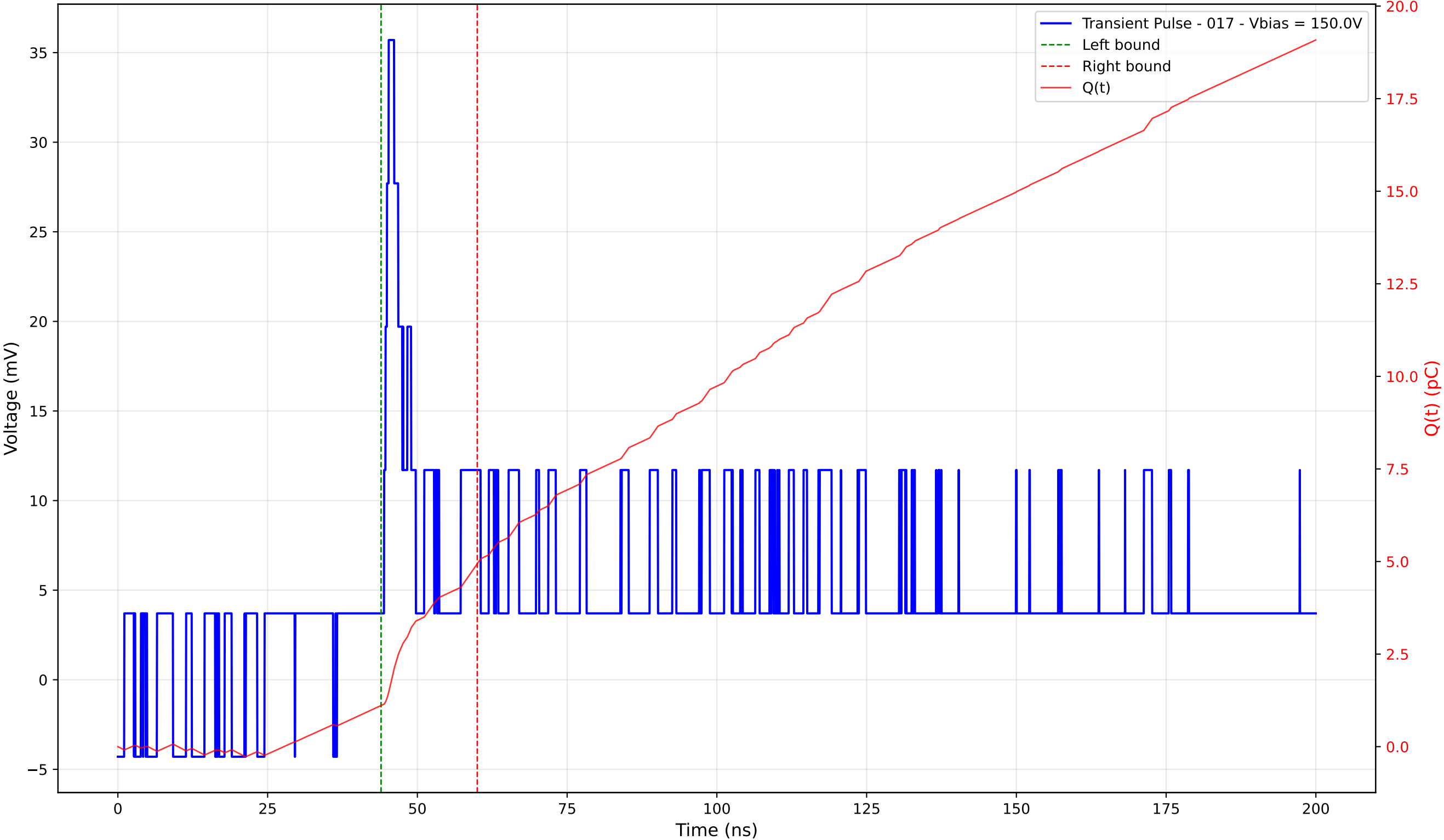
Transient Pulse - Sample: 4003 - Position: 340.0 \mu\text{m} - Charge: 3.84 pC - Rise Time: 0.00 ns (N/A)
