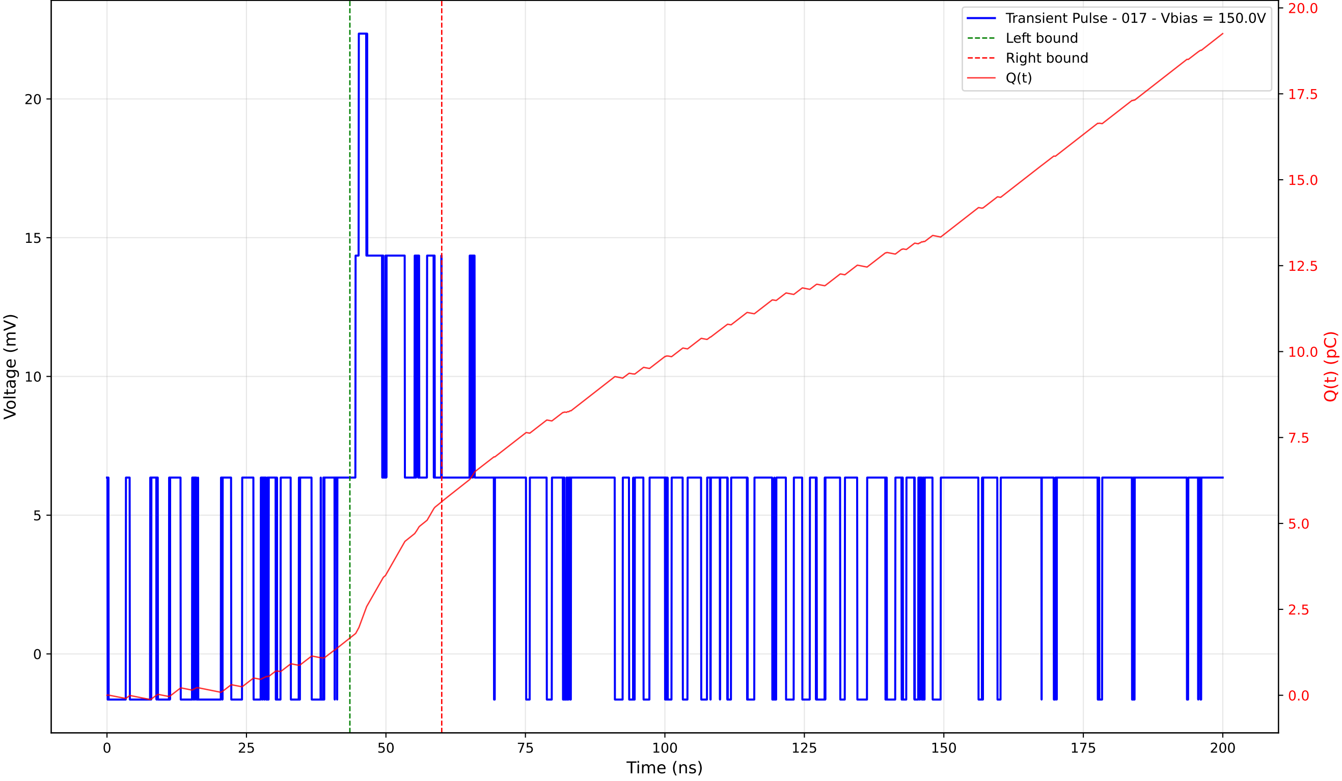
Transient Pulse - Sample: 4003 - Position: 65.0 \mu\text{m} - Charge: 3.98 pC - Rise Time: 3.86 ns
