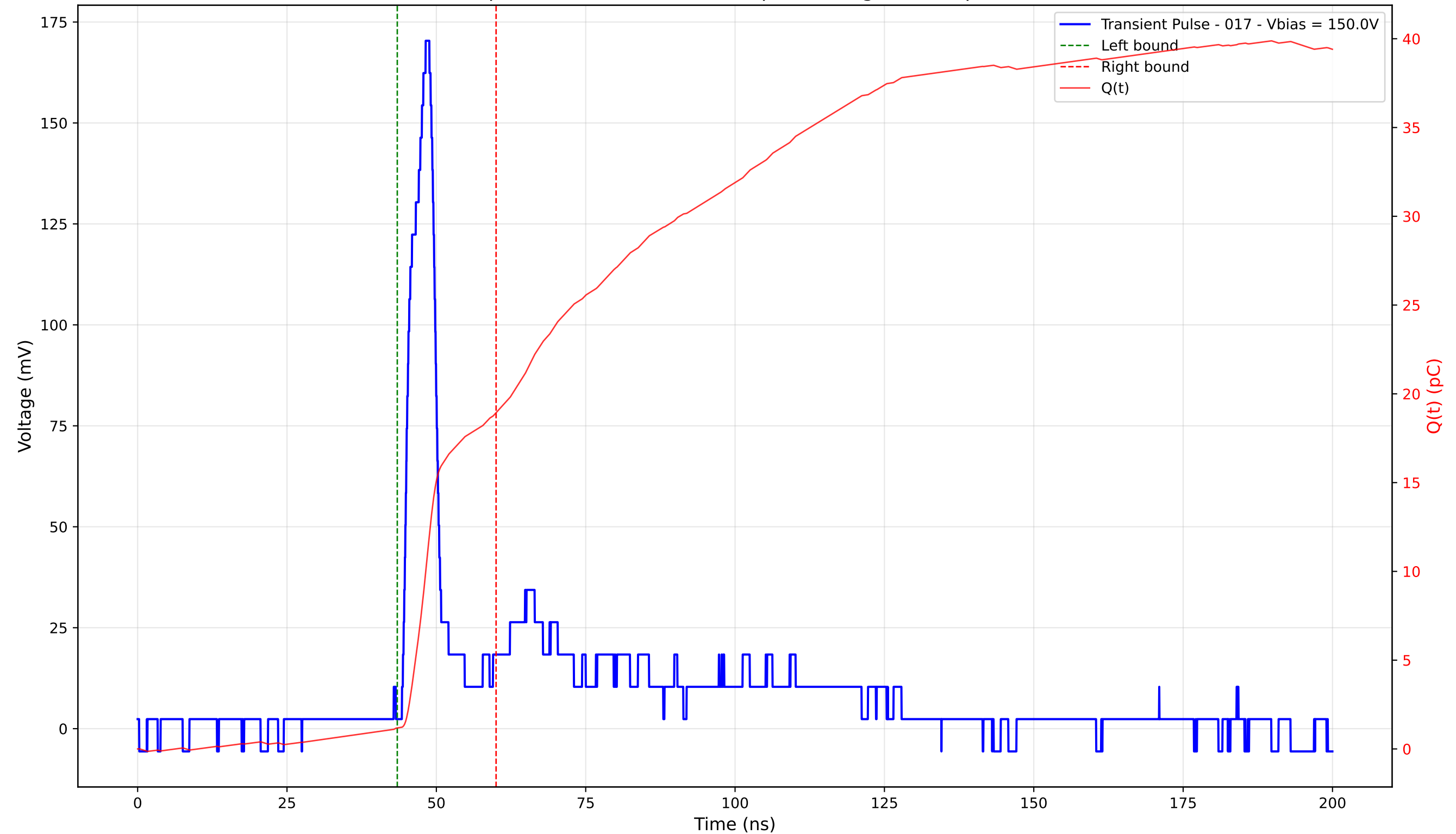
Transient Pulse - Sample: 4003 - Position: 290.0 \mu\text{m} - Charge: 17.75 pC - Rise Time: 3.18 ns
