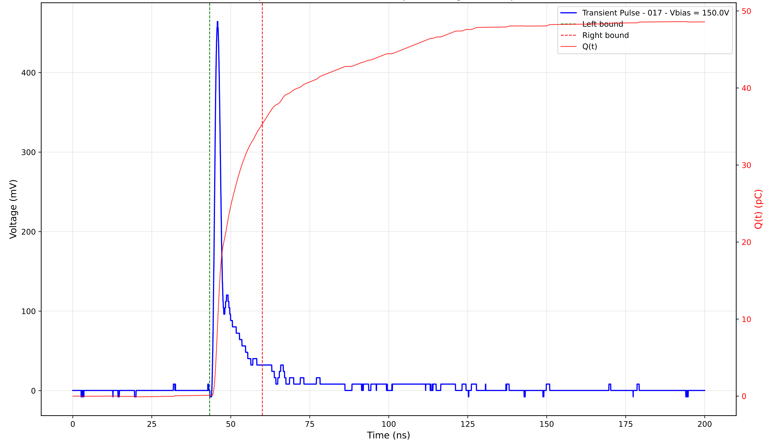
Transient Pulse - Sample: 4003 - Position: 195.0 \mu\text{m} - Charge: 35.20 pC - Rise Time: 1.14 ns
