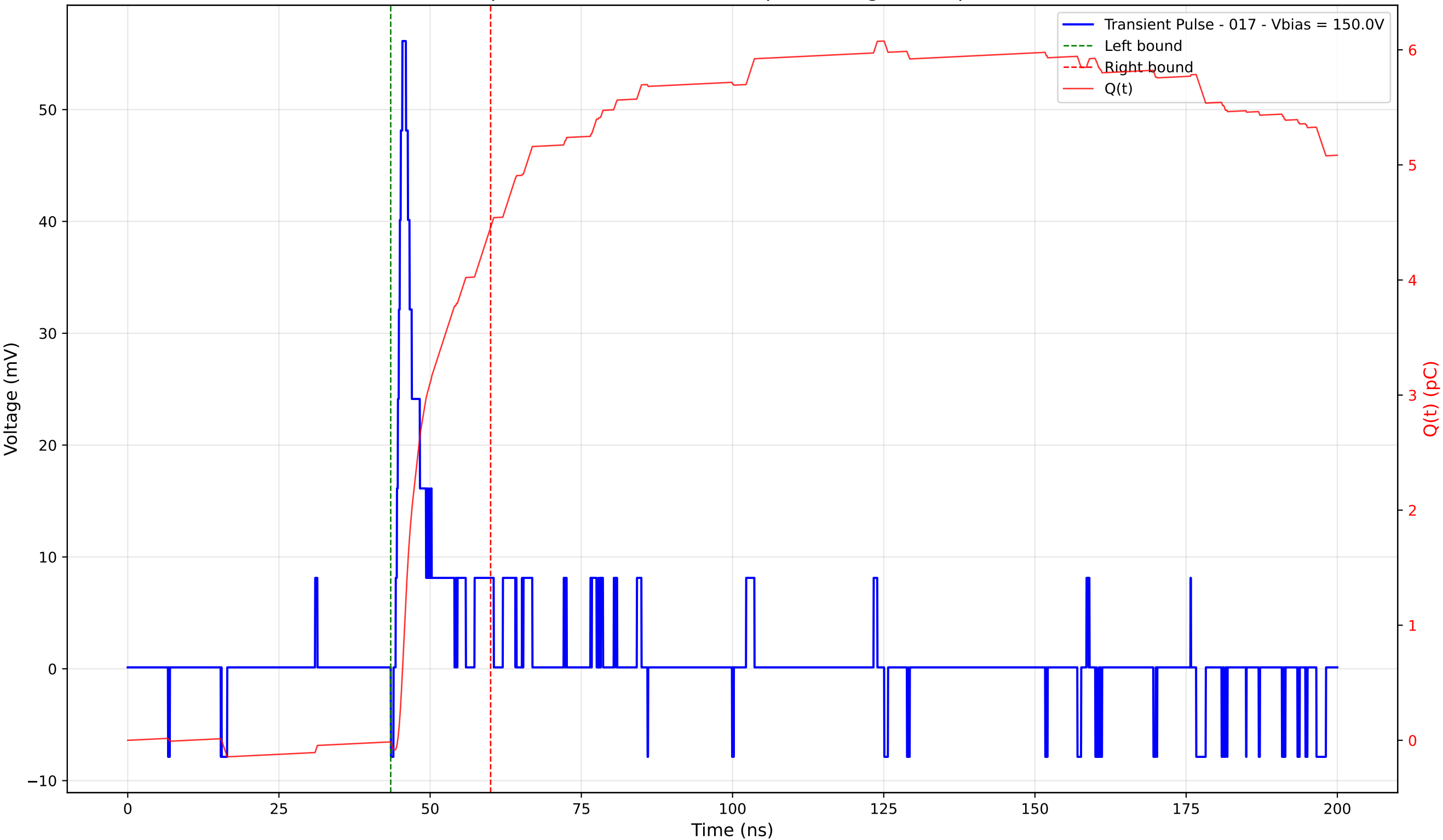
Transient Pulse - Sample: 4003 - Position: 390.0 \mu\text{m} - Charge: 4.47 pC - Rise Time: 1.11 ns
