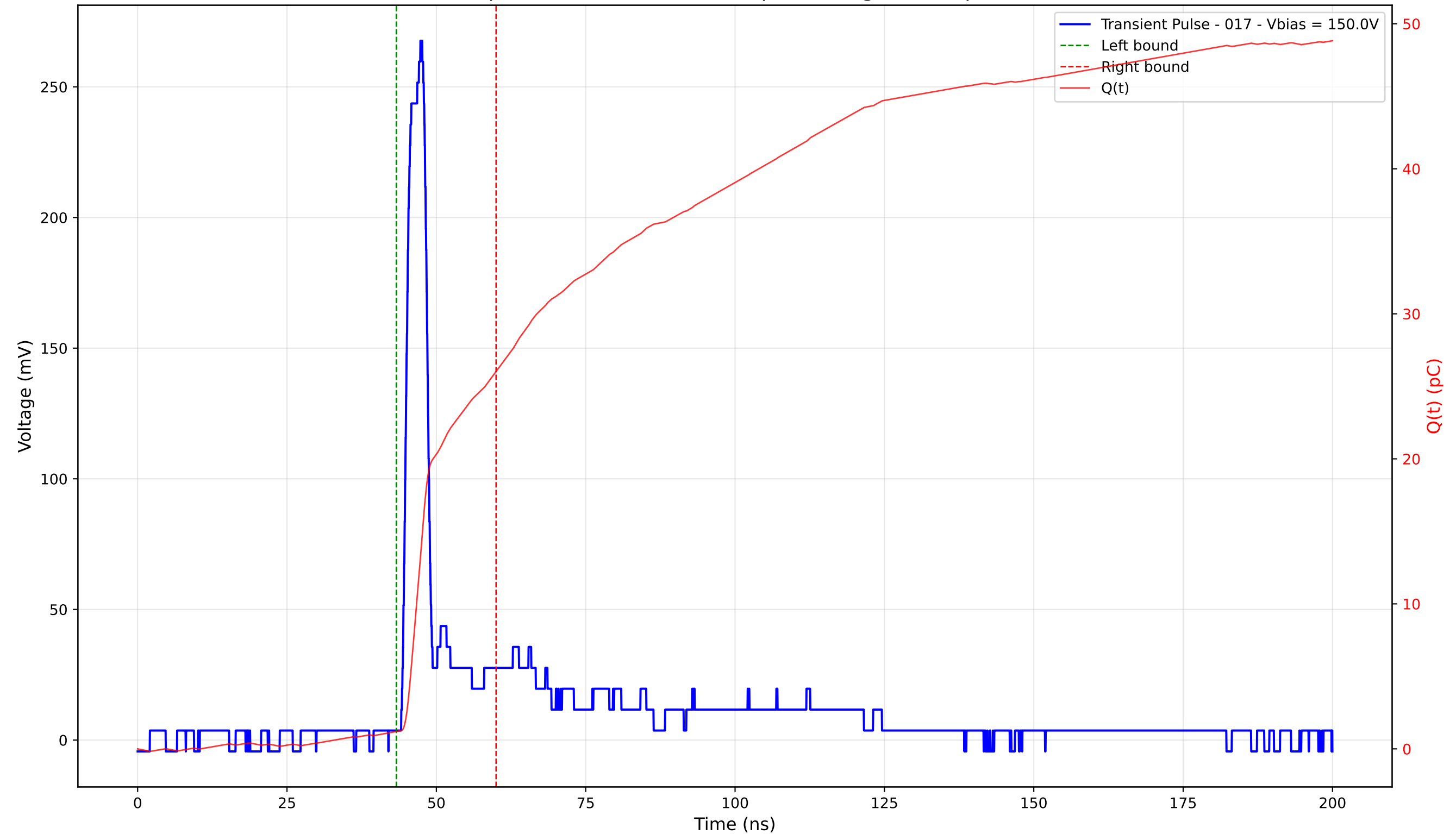
Transient Pulse - Sample: 4003 - Position: 265.0 \mu\text{m} - Charge: 24.83 pC - Rise Time: 1.48 ns
