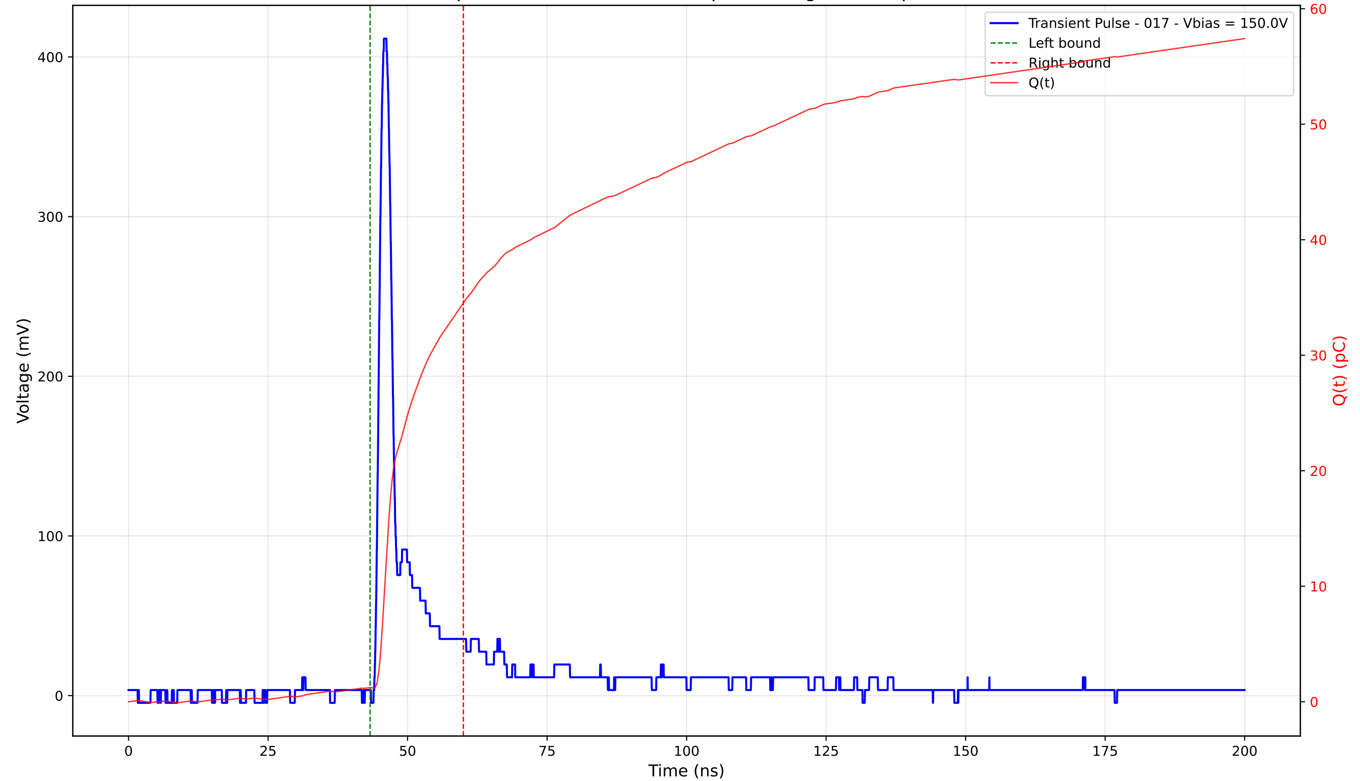
Transient Pulse - Sample: 4003 - Position: 215.0 \mu\text{m} - Charge: 33.32 pC - Rise Time: 1.15 ns
