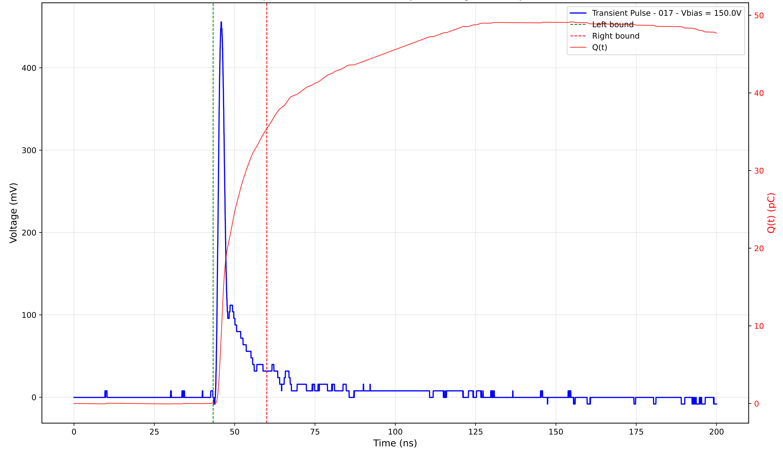
Transient Pulse - Sample: 4003 - Position: 200.0 \mu\text{m} - Charge: 35.29 pC - Rise Time: 1.15 ns
