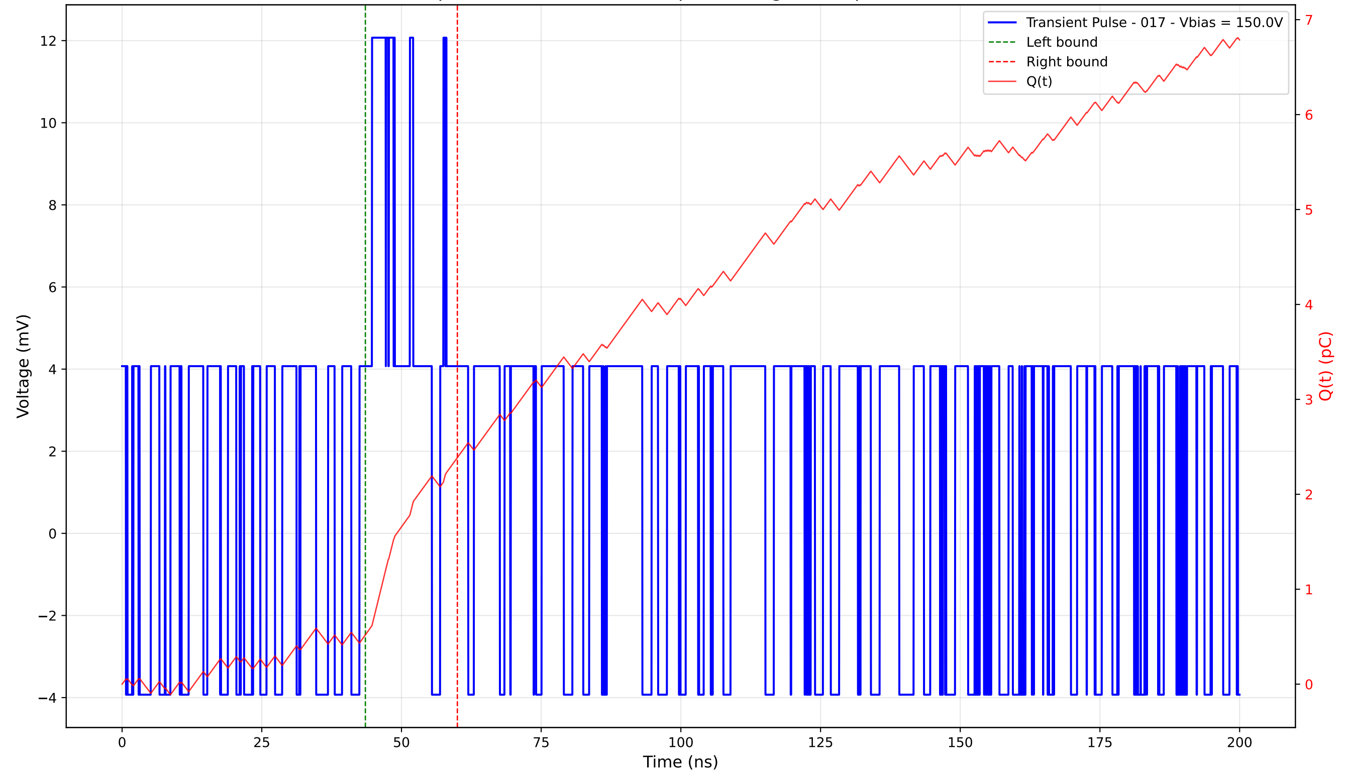
Transient Pulse - Sample: 4003 - Position: 10.0 \mu\text{m} - Charge: 1.87 pC - Rise Time: 0.00 ns (N/A)
