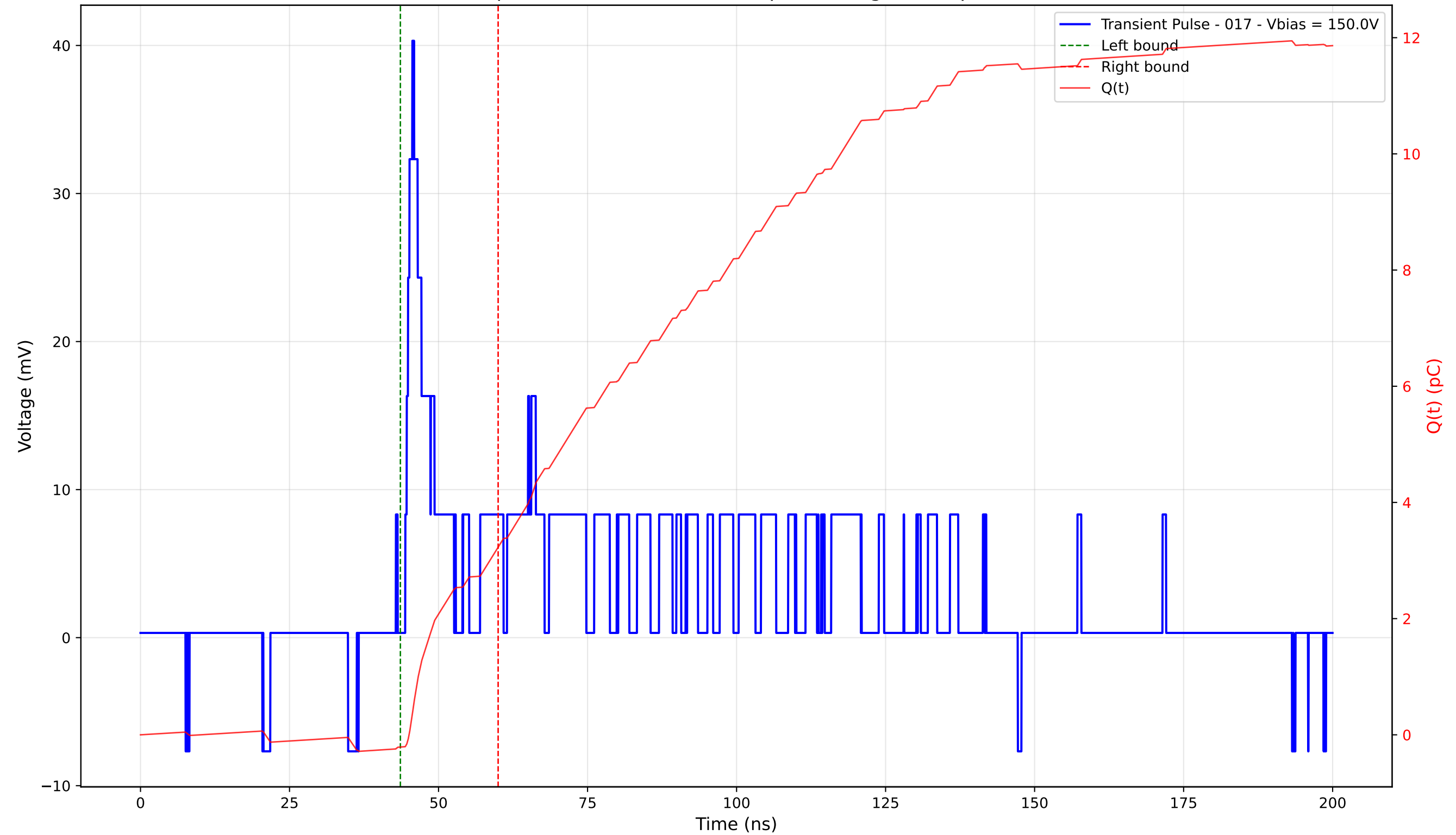
Transient Pulse - Sample: 4003 - Position: 325.0 \mu\text{m} - Charge: 3.44 pC - Rise Time: 1.19 ns
