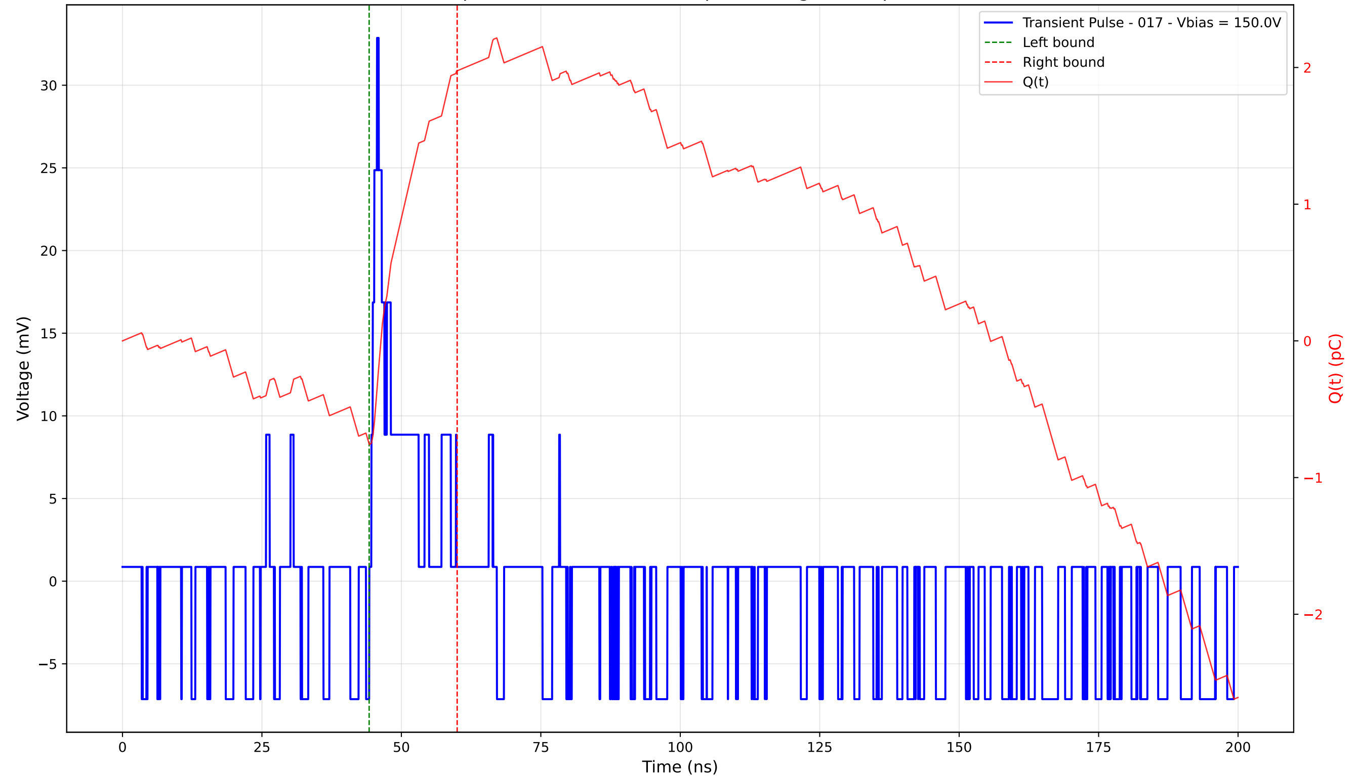
Transient Pulse - Sample: 4003 - Position: 40.0 \mu\text{m} - Charge: 2.73 pC - Rise Time: 1.01 ns
