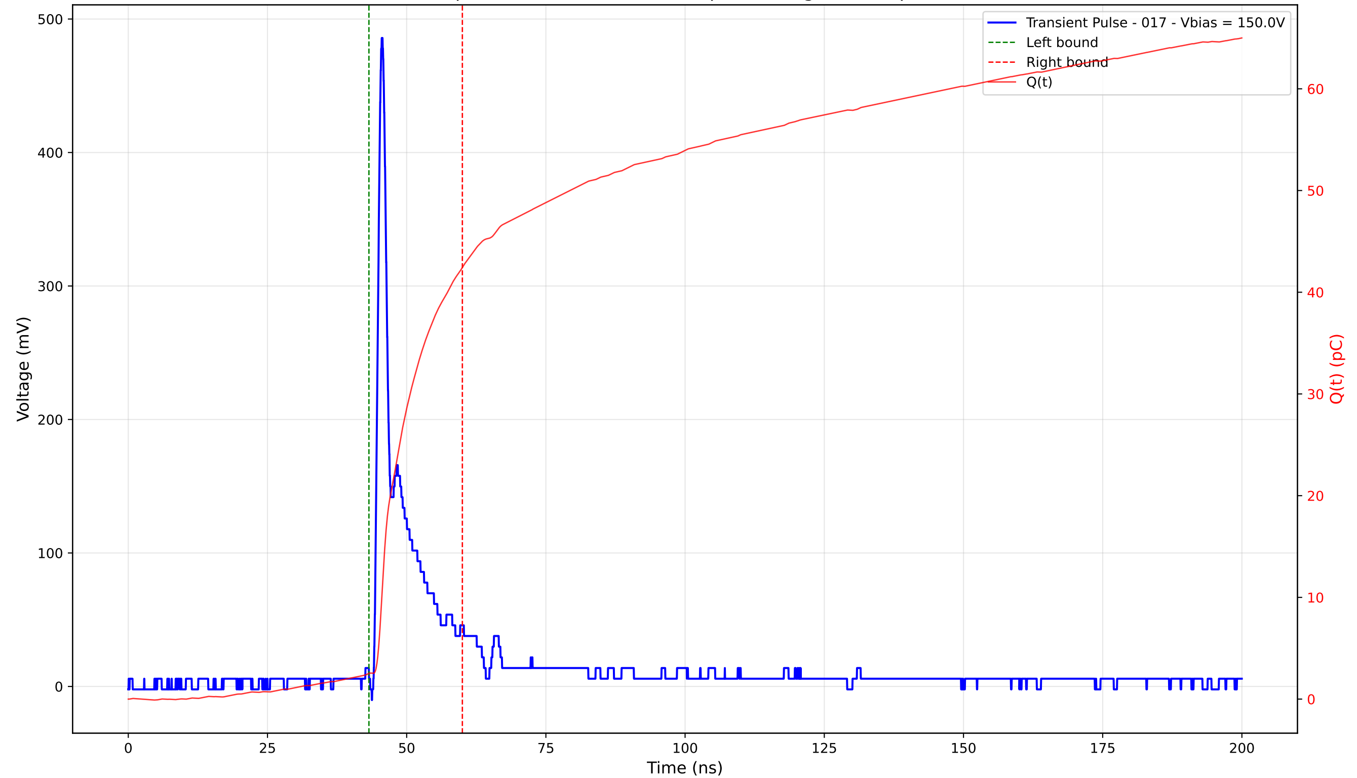
Transient Pulse - Sample: 4003 - Position: 155.0 \mu\text{m} - Charge: 39.90 pC - Rise Time: 0.97 ns
