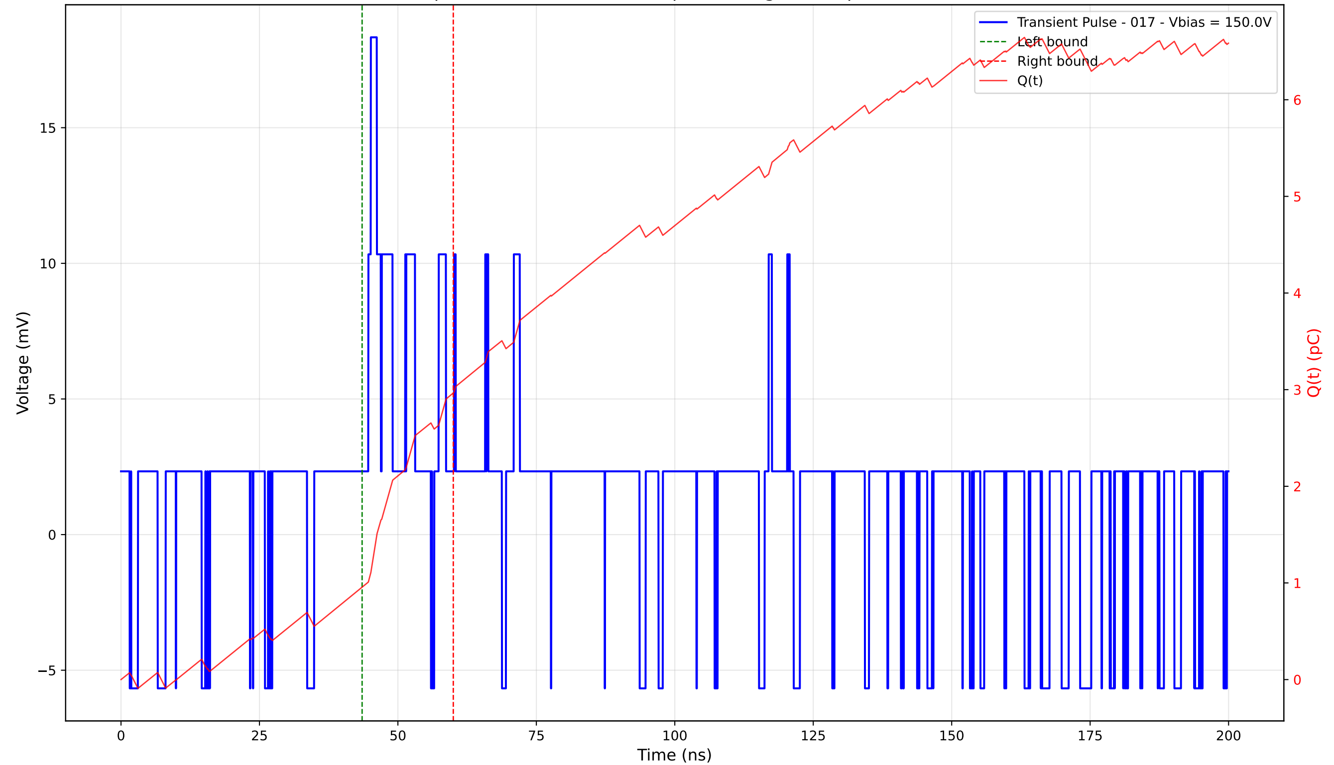
Transient Pulse - Sample: 4003 - Position: 70.0 \mu\text{m} - Charge: 2.01 pC - Rise Time: 0.00 ns (N/A)
