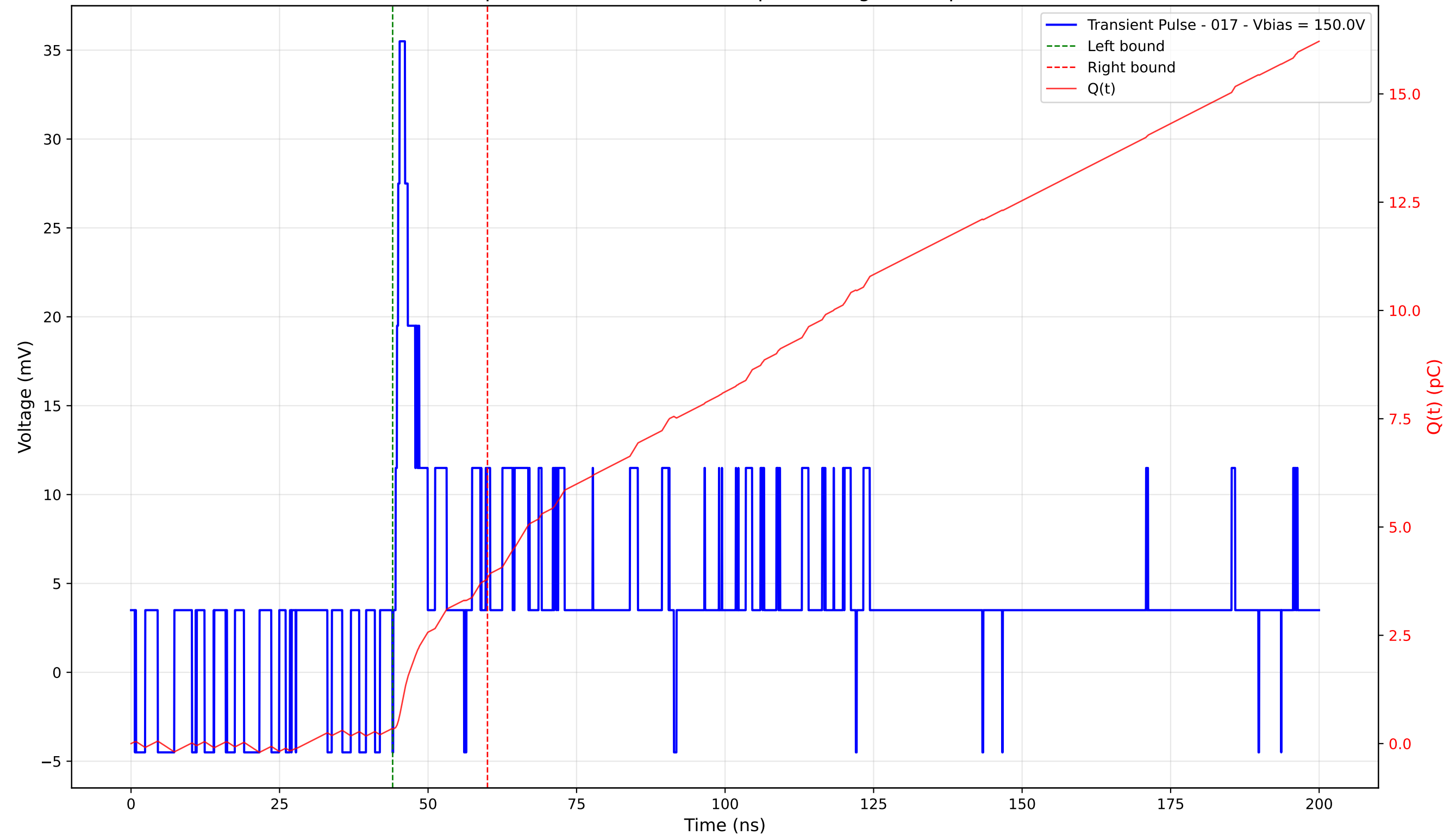
Transient Pulse - Sample: 4003 - Position: 330.0 \mu\text{m} - Charge: 3.48 pC - Rise Time: 0.68 ns
