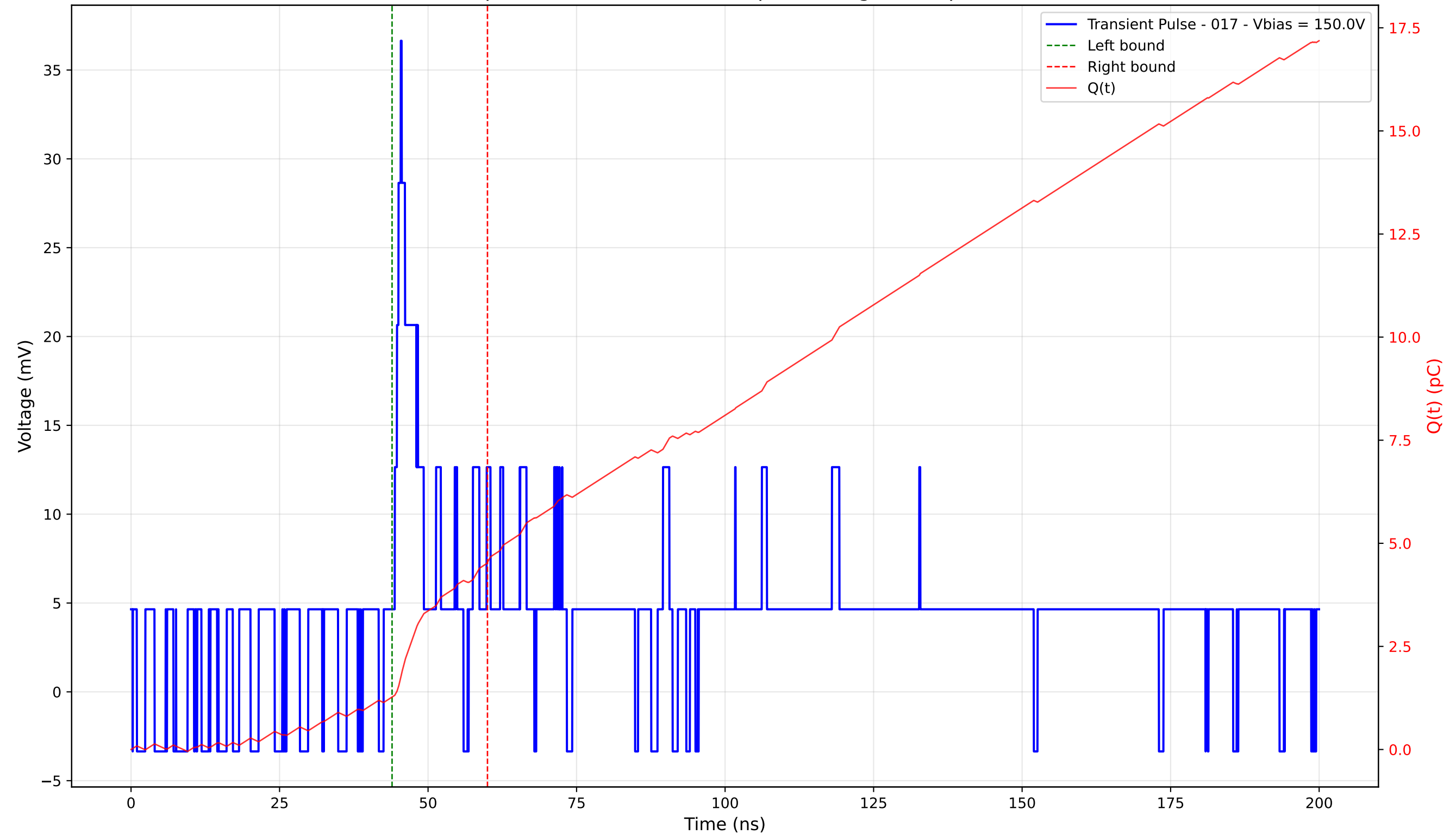
Transient Pulse - Sample: 4003 - Position: 350.0 \mu\text{m} - Charge: 3.27 pC - Rise Time: 2.90 ns
