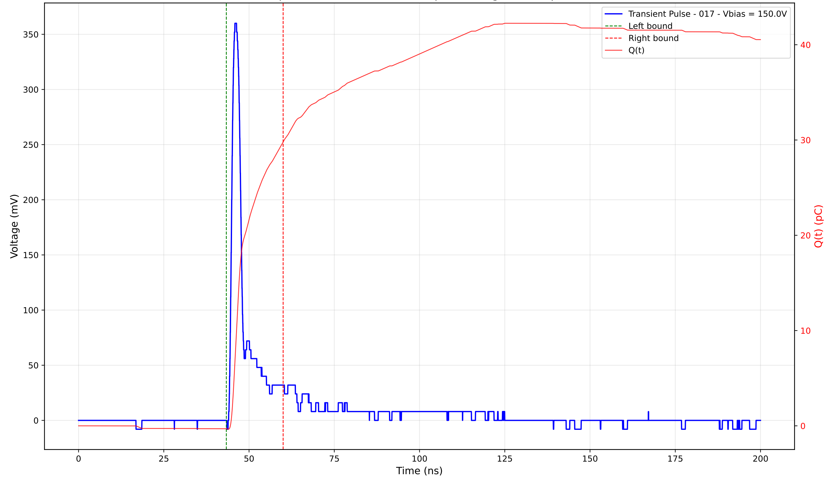
Transient Pulse - Sample: 4003 - Position: 230.0 \mu\text{m} - Charge: 30.11 pC - Rise Time: 1.19 ns
