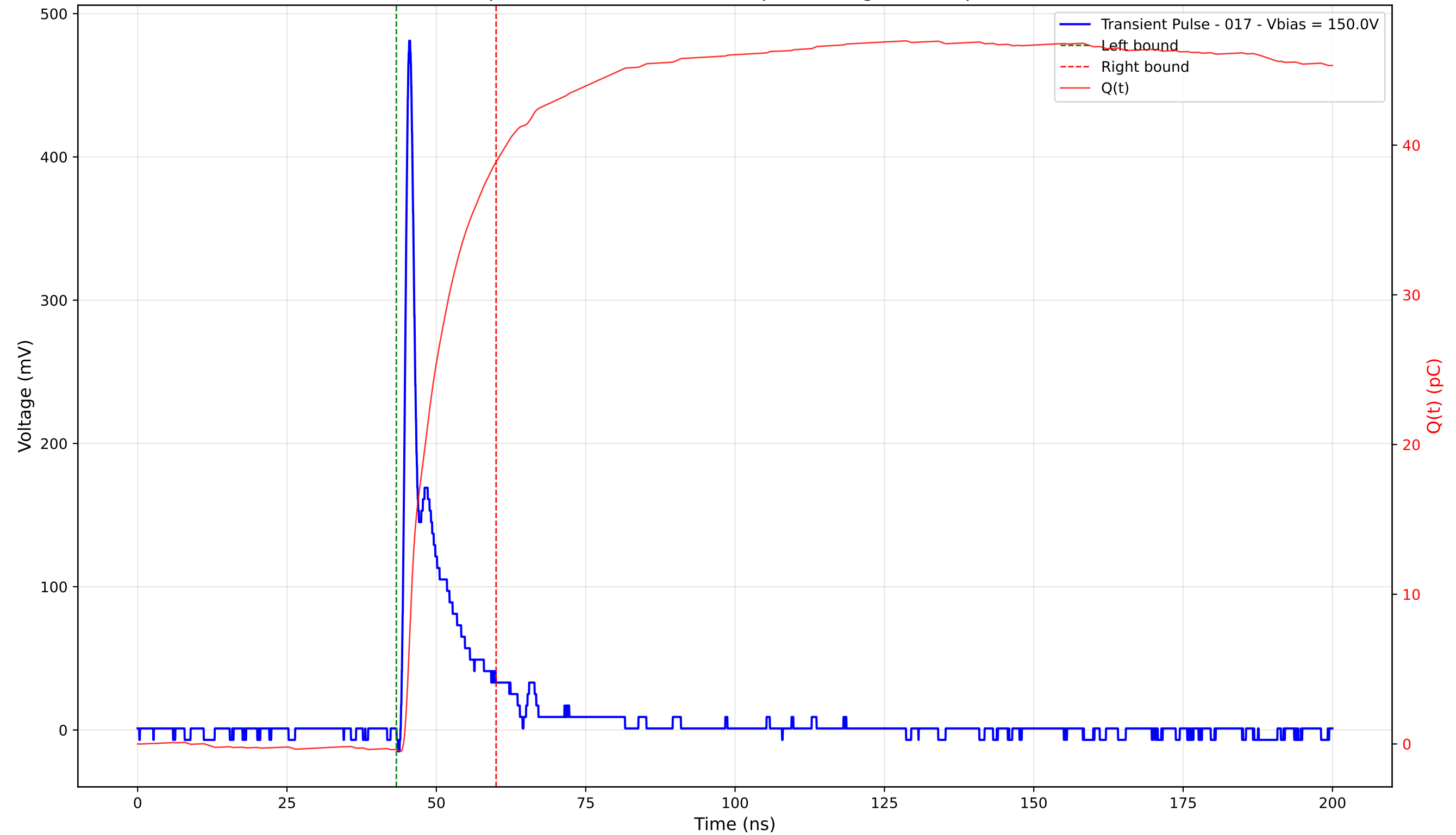
Transient Pulse - Sample: 4003 - Position: 145.0 \mu\text{m} - Charge: 39.25 pC - Rise Time: 0.94 ns
