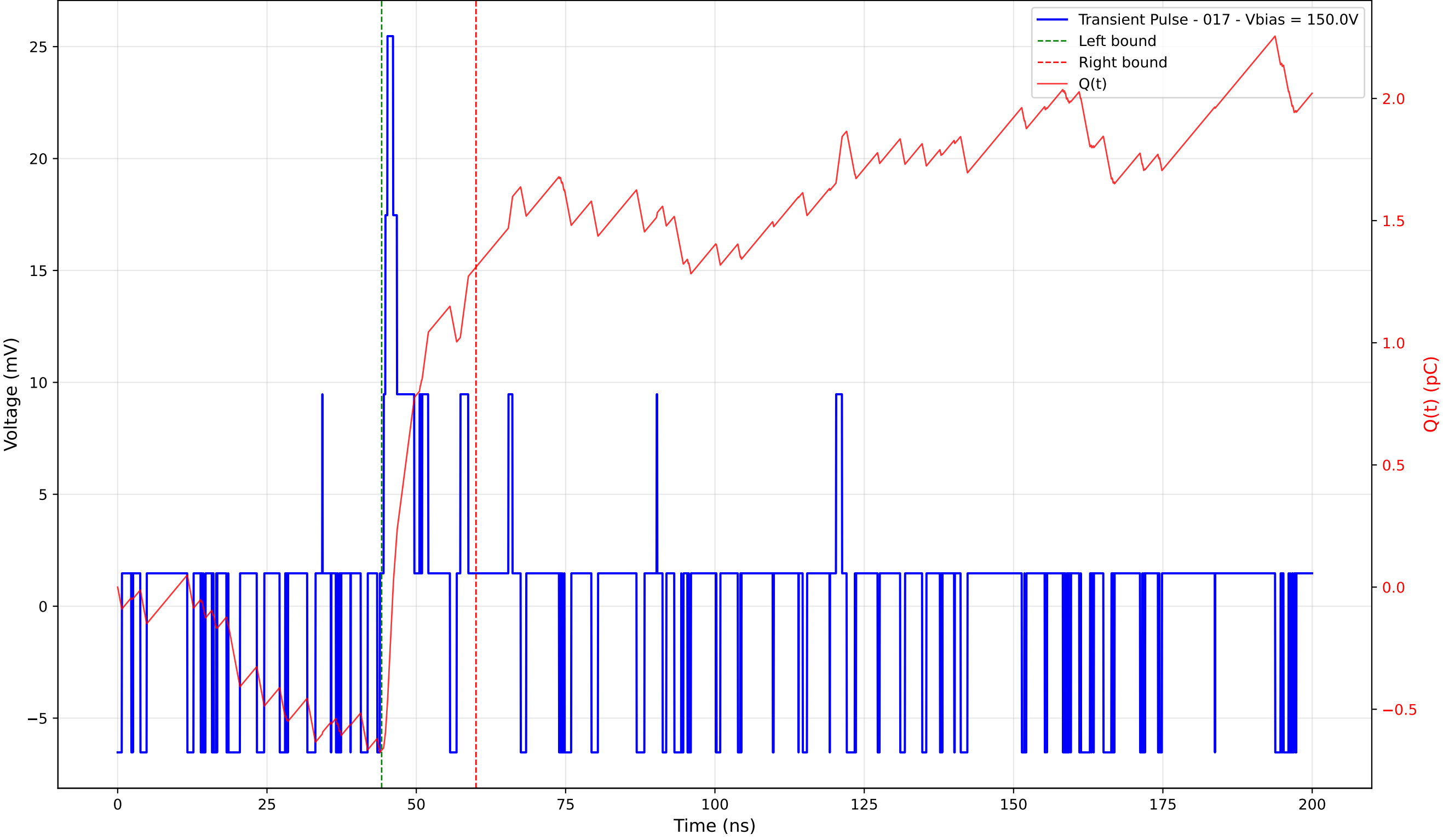
Transient Pulse - Sample: 4003 - Position: 25.0 \mu\text{m} - Charge: 1.98 pC - Rise Time: 0.64 ns
