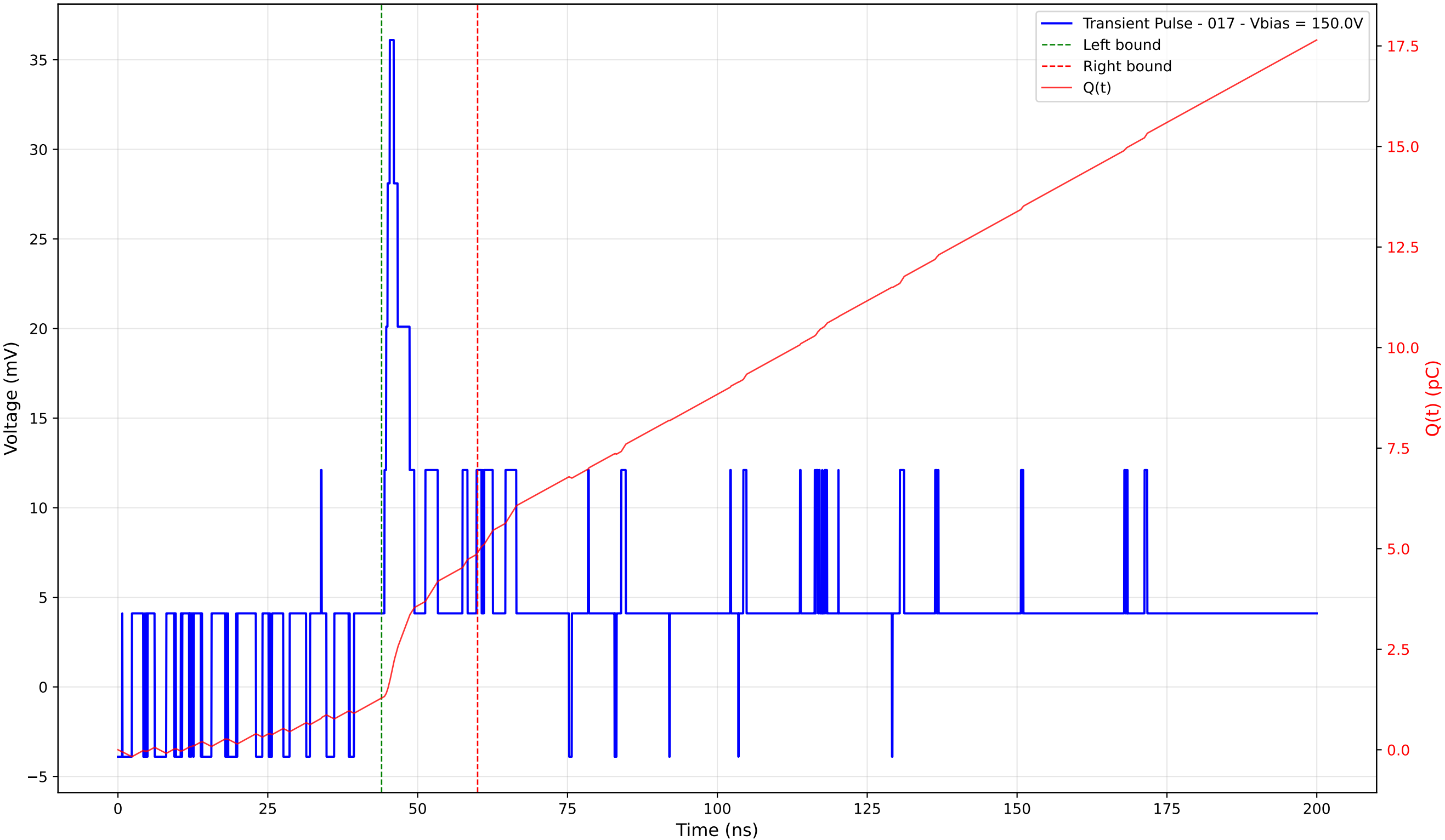
Transient Pulse - Sample: 4003 - Position: 355.0 \mu\text{m} - Charge: 3.61 pC - Rise Time: 0.00 ns (N/A)
