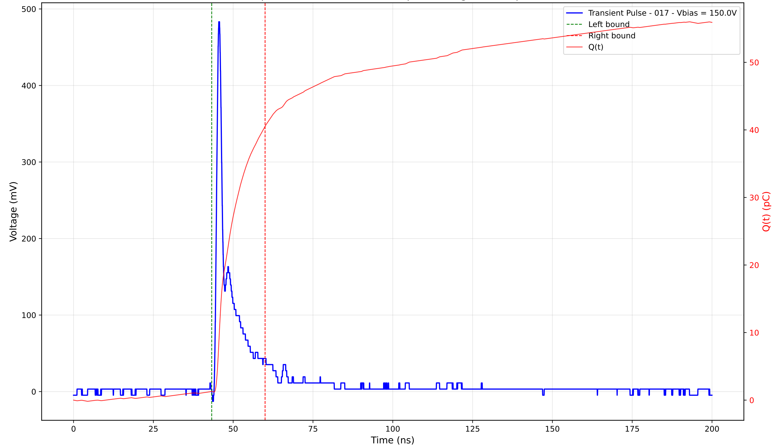
Transient Pulse - Sample: 4003 - Position: 160.0 \mu\text{m} - Charge: 39.22 pC - Rise Time: 0.99 ns
