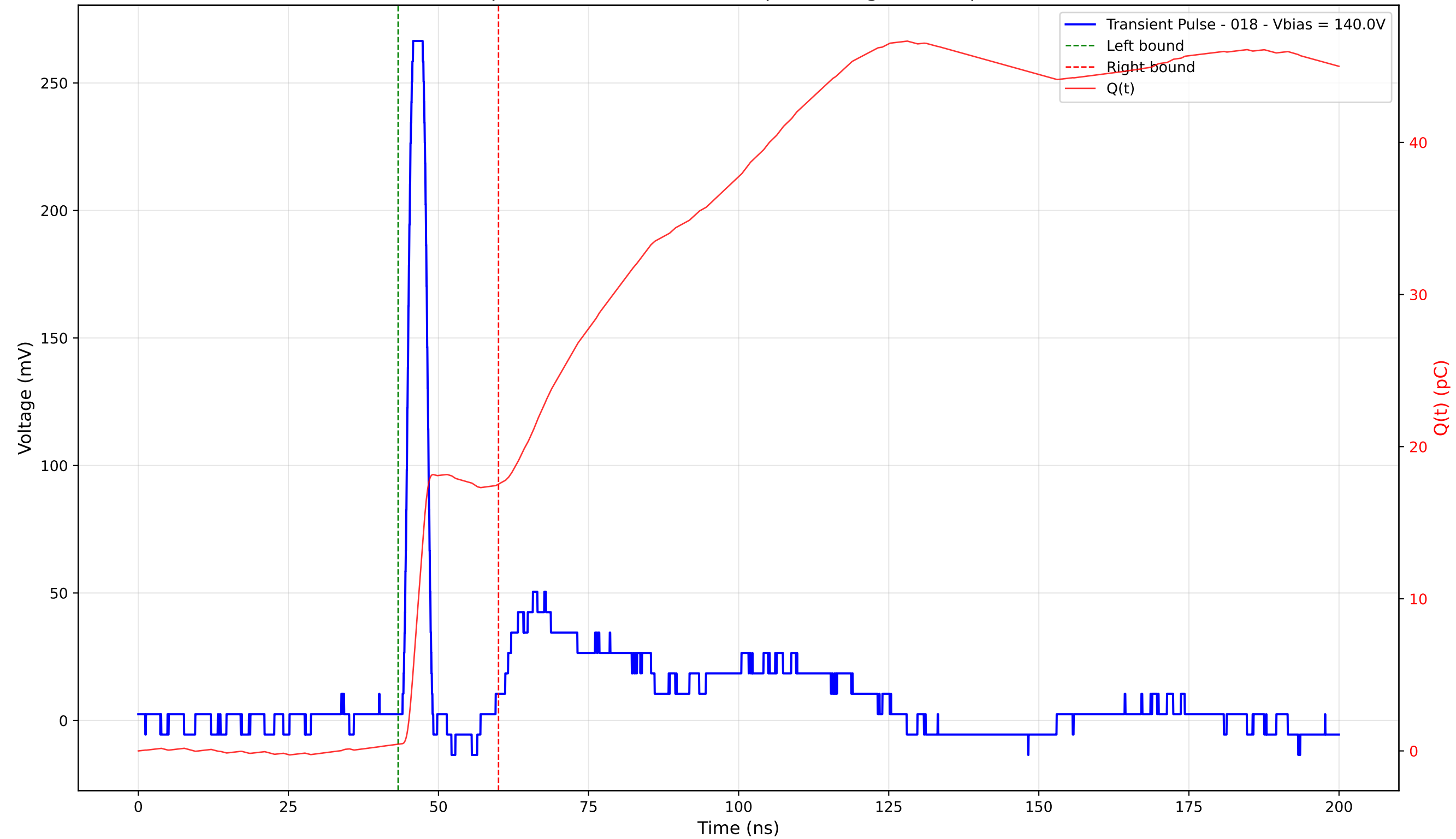
Transient Pulse - Sample: 4003 - Position: 250.0 \mu\text{m} - Charge: 17.10 pC - Rise Time: 1.16 ns
