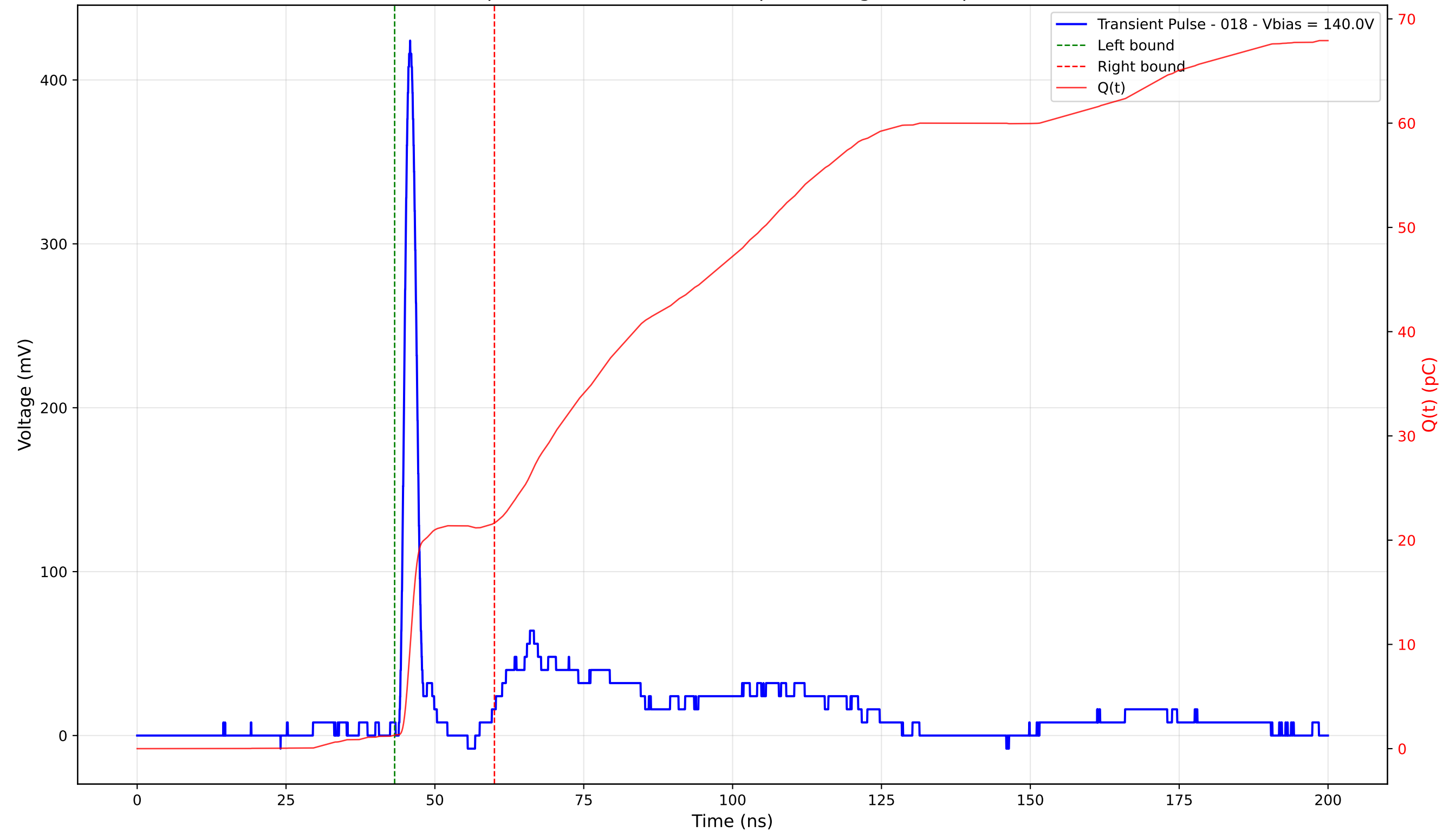
Transient Pulse - Sample: 4003 - Position: 205.0 \mu\text{m} - Charge: 20.34 pC - Rise Time: 1.13 ns
