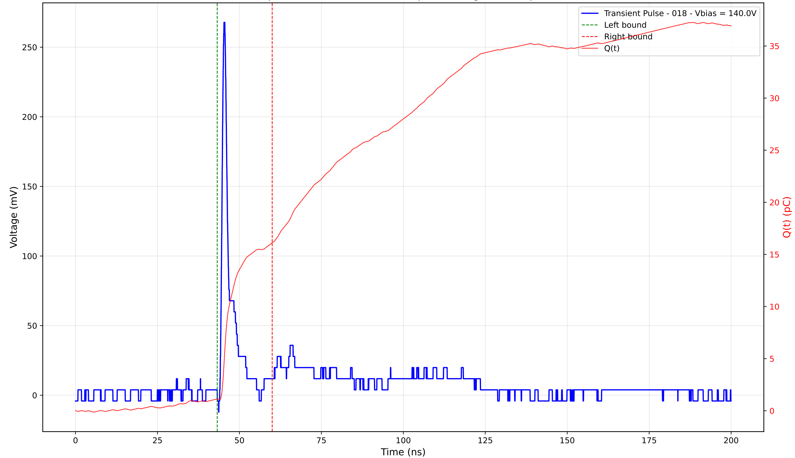
Transient Pulse - Sample: 4003 - Position: 105.0 \mu\text{m} - Charge: 14.97 pC - Rise Time: 0.90 ns
