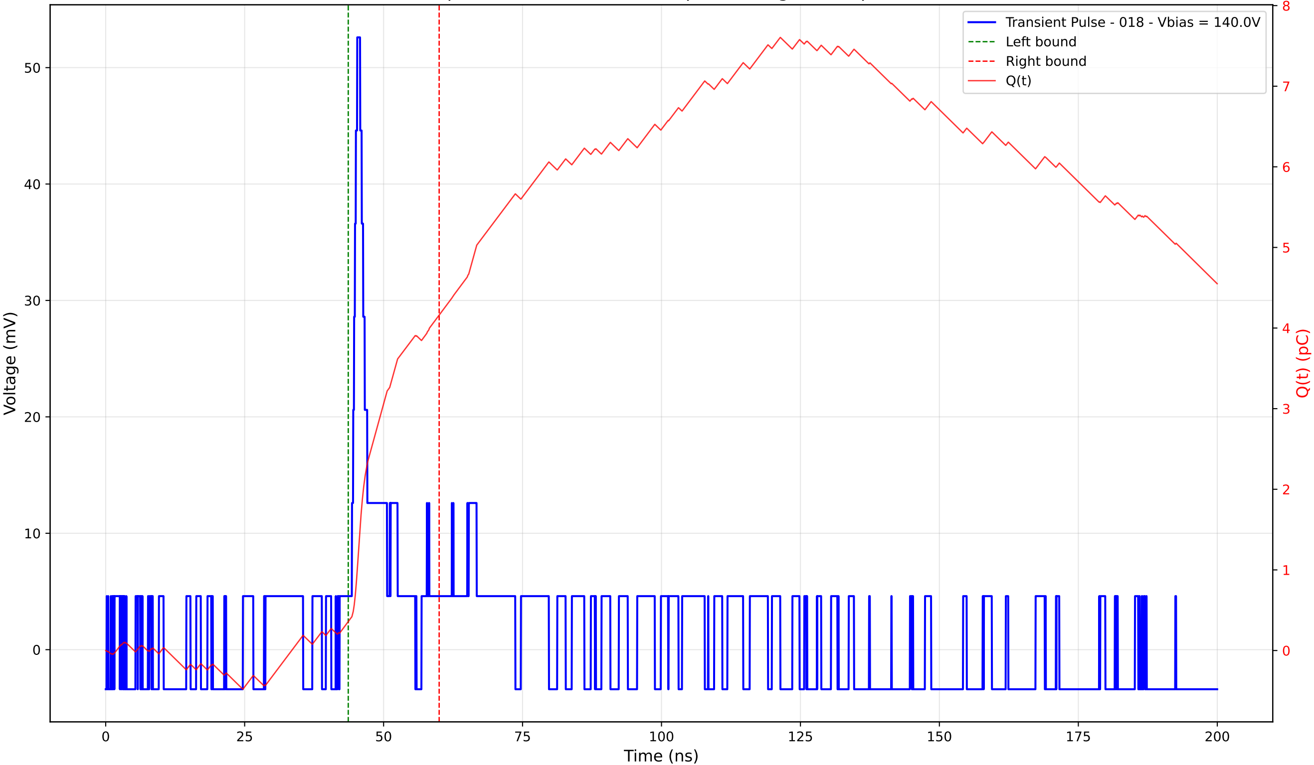
Transient Pulse - Sample: 4003 - Position: 85.0 \mu\text{m} - Charge: 3.80 pC - Rise Time: 0.96 ns
