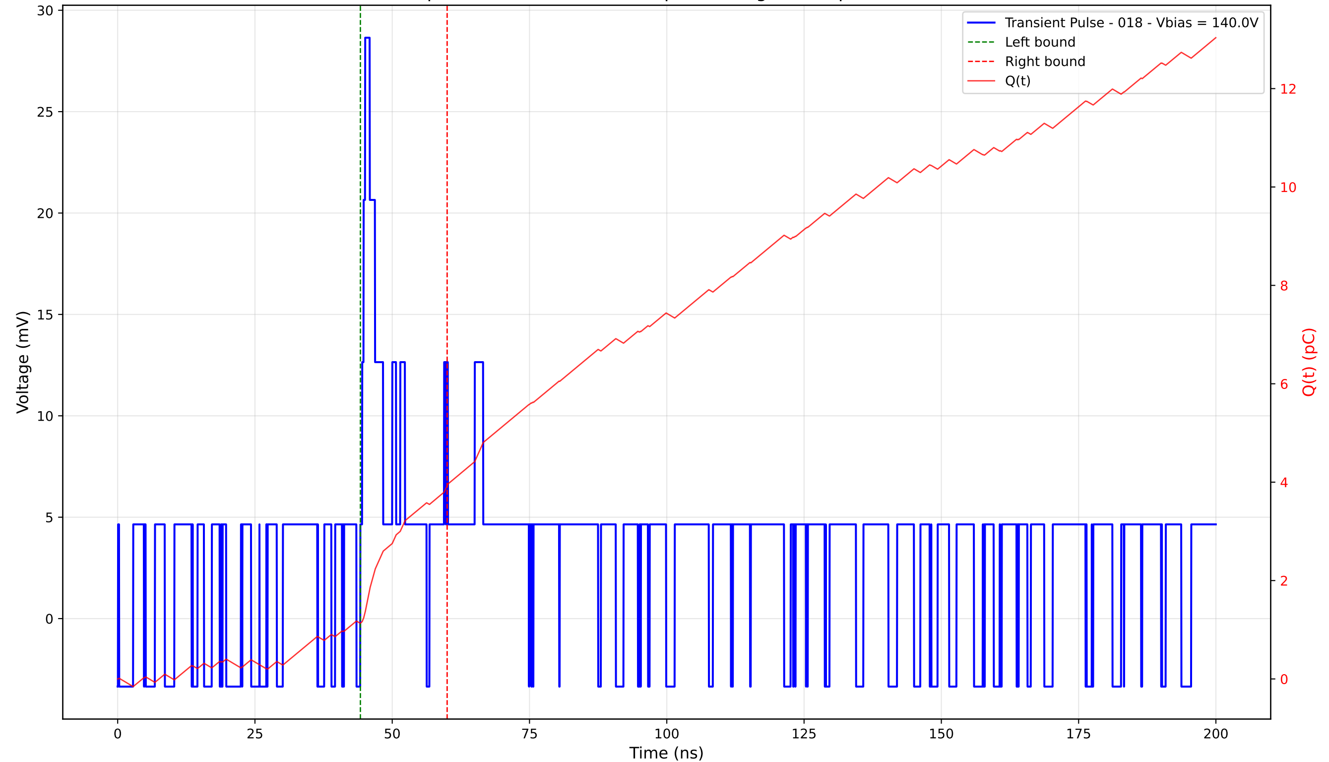
Transient Pulse - Sample: 4003 - Position: 25.0 \mu\text{m} - Charge: 2.79 pC - Rise Time: 0.00 ns (N/A)
