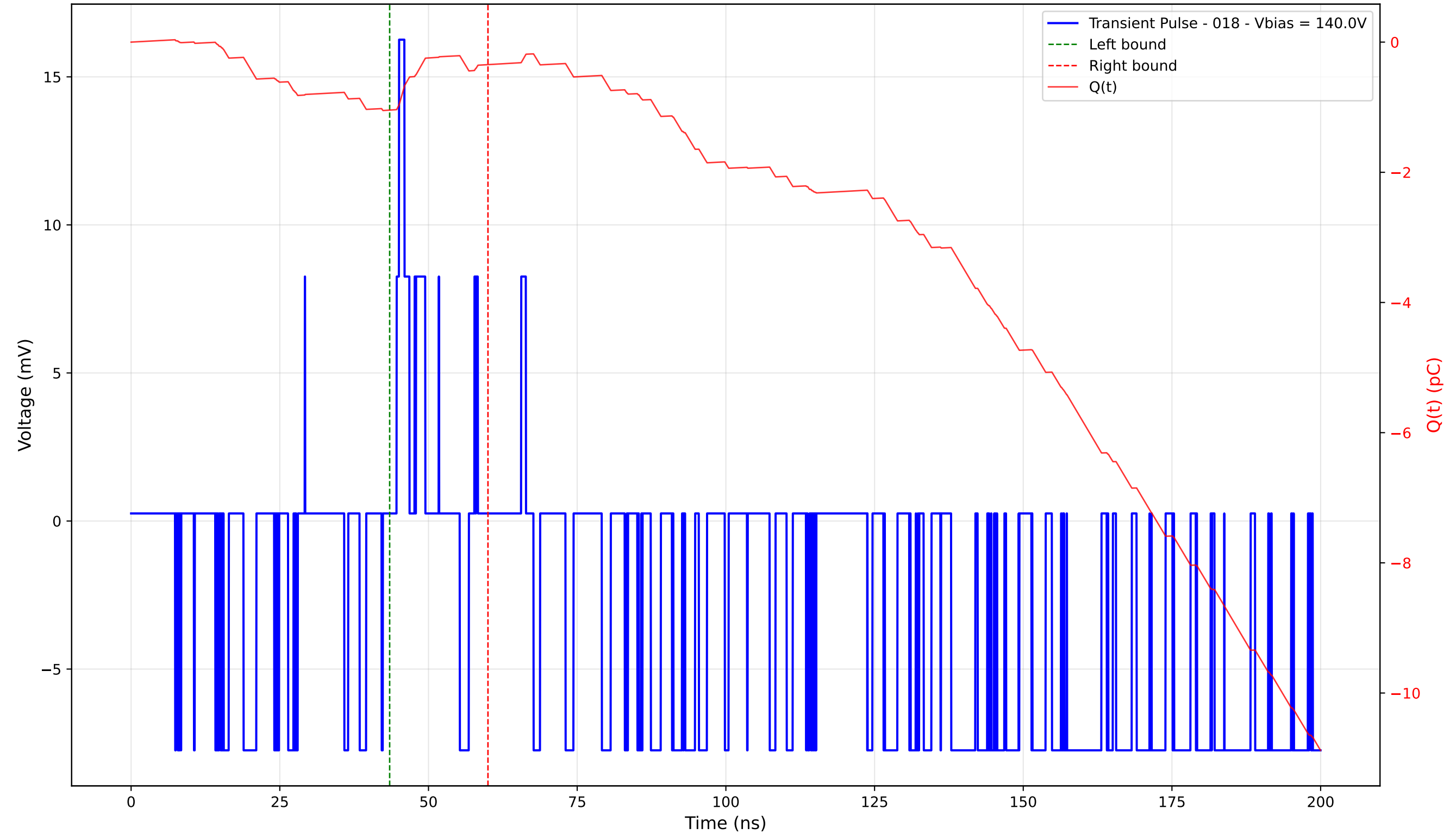
Transient Pulse - Sample: 4003 - Position: 15.0 \mu\text{m} - Charge: 0.70 pC - Rise Time: 0.42 ns
