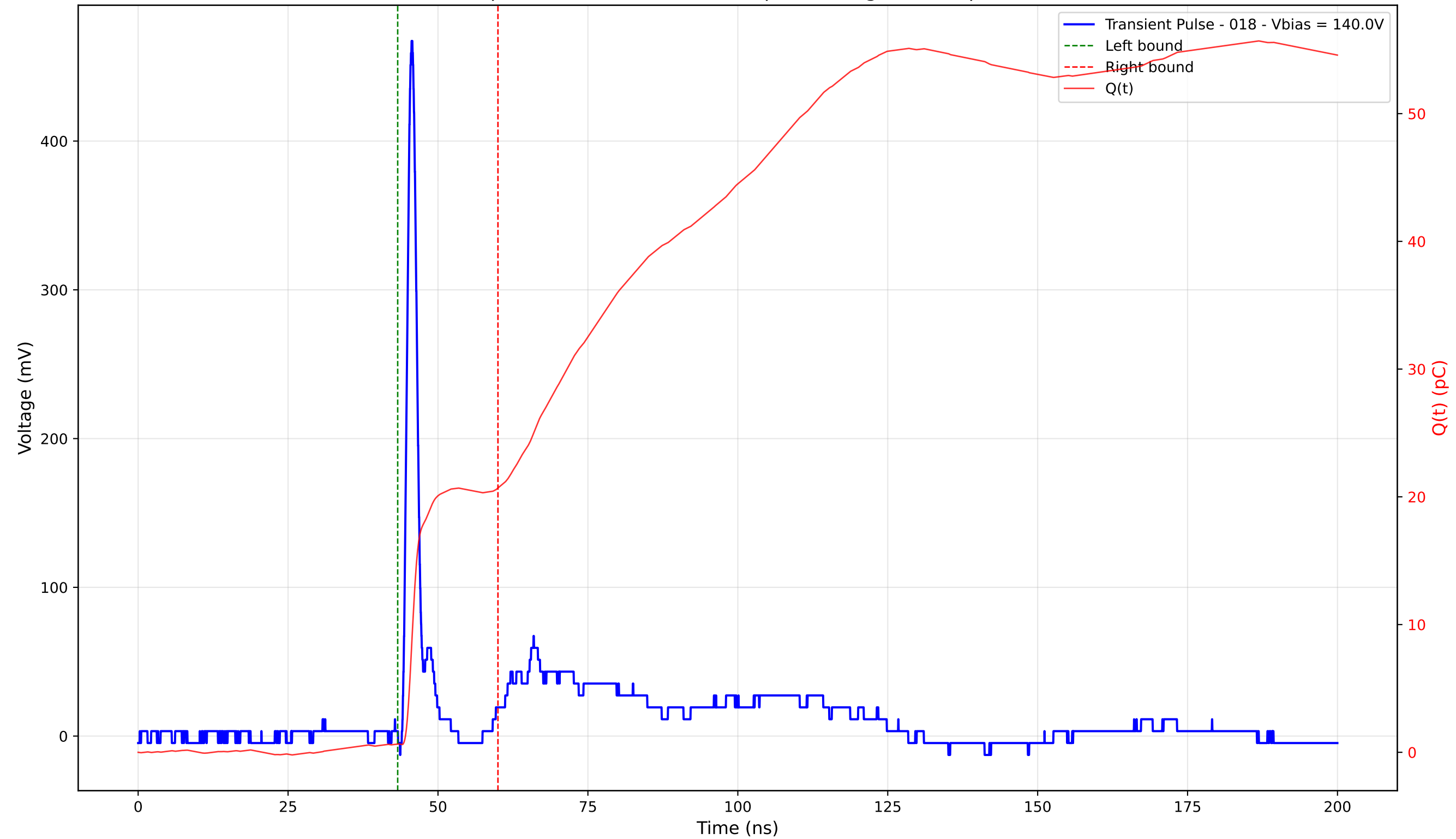
Transient Pulse - Sample: 4003 - Position: 175.0 \mu\text{m} - Charge: 20.03 pC - Rise Time: 1.03 ns
