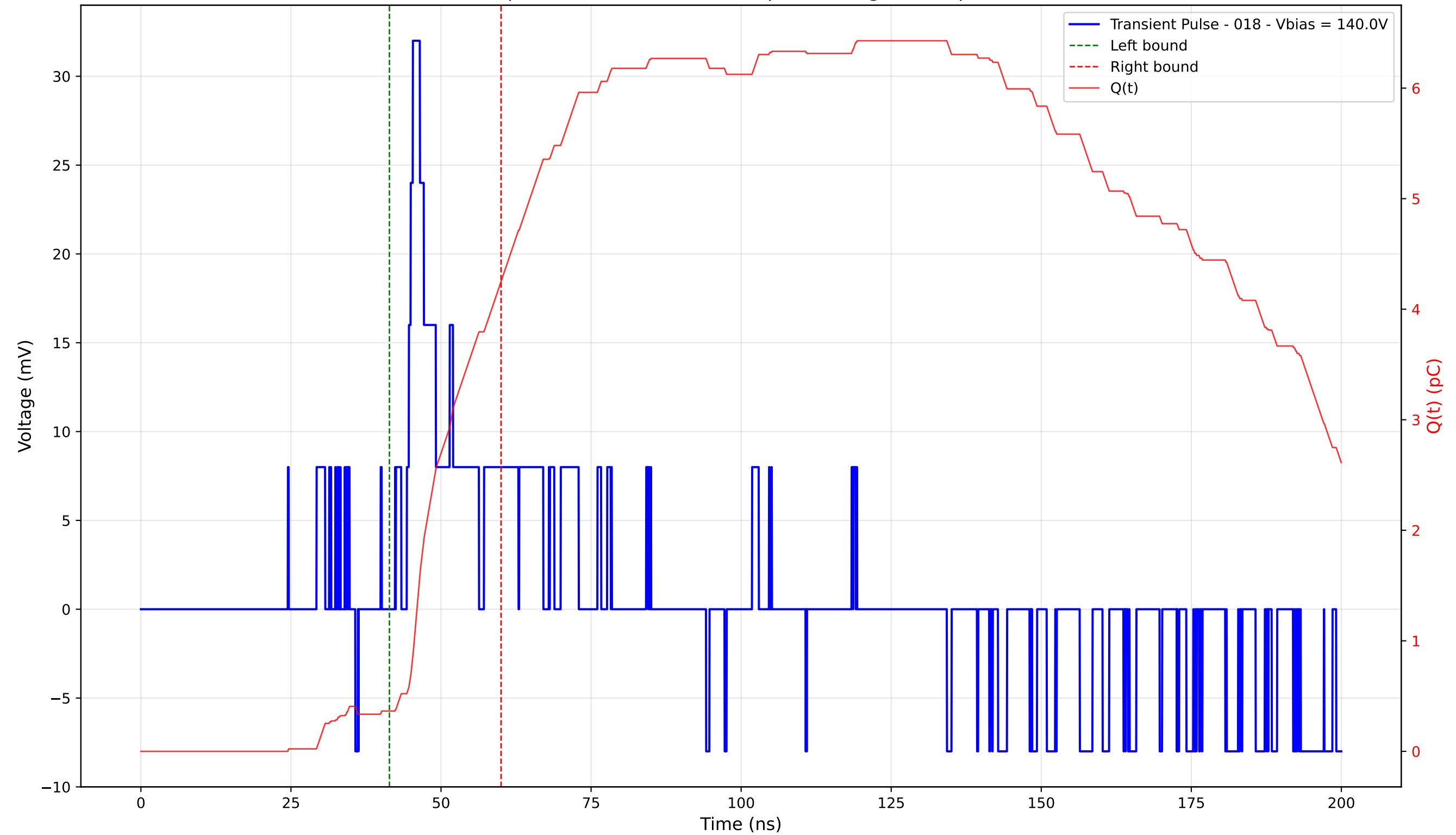
Transient Pulse - Sample: 4003 - Position: 45.0 \mu\text{m} - Charge: 3.89 pC - Rise Time: 1.01 ns
