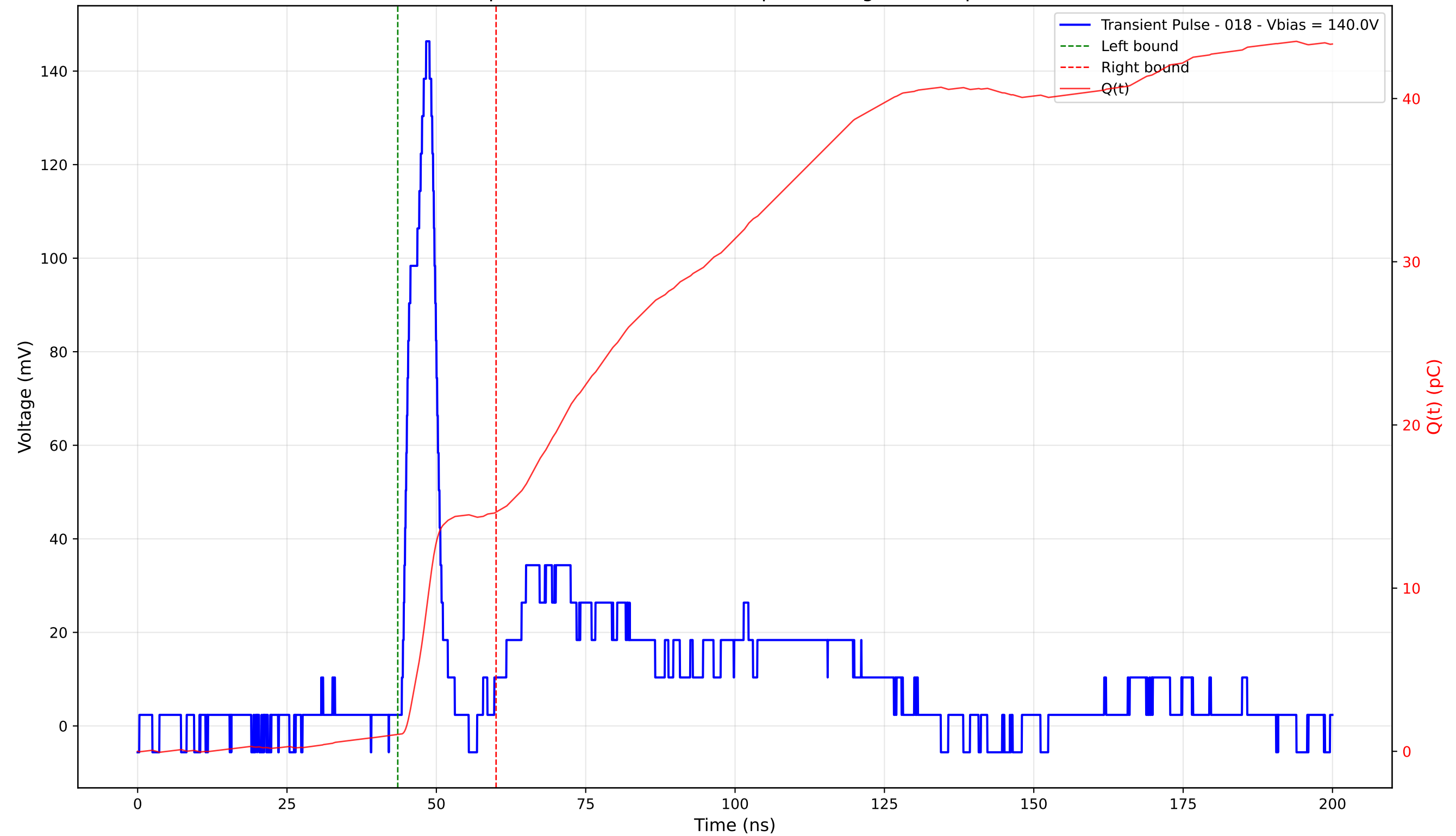
Transient Pulse - Sample: 4003 - Position: 285.0 \mu\text{m} - Charge: 13.63 pC - Rise Time: 3.49 ns
