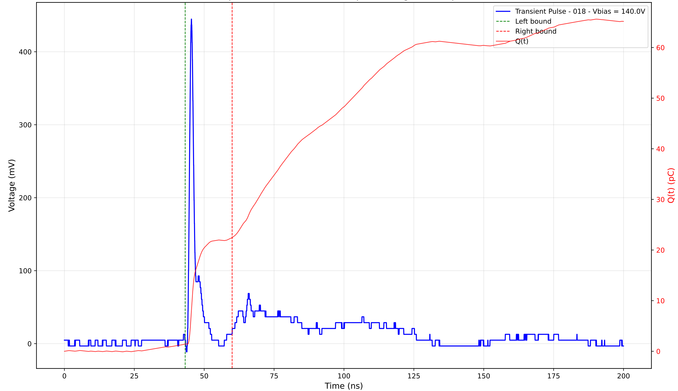
Transient Pulse - Sample: 4003 - Position: 125.0 \mu\text{m} - Charge: 20.99 pC - Rise Time: 0.92 ns
