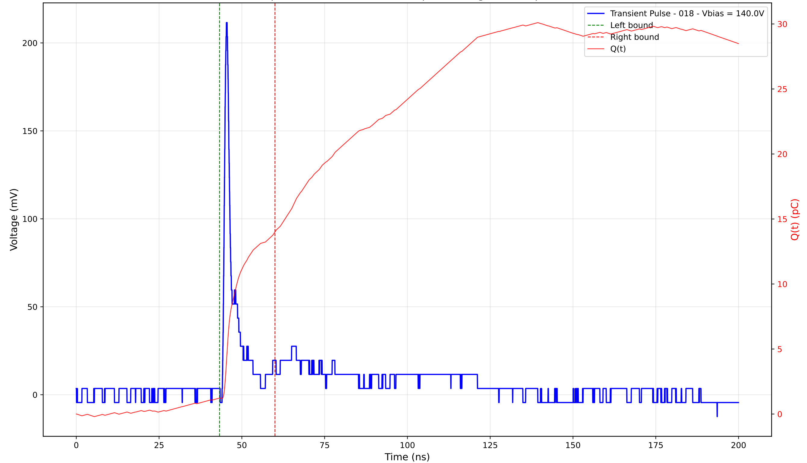
Transient Pulse - Sample: 4003 - Position: 100.0 \mu\text{m} - Charge: 12.78 pC - Rise Time: 0.90 ns
