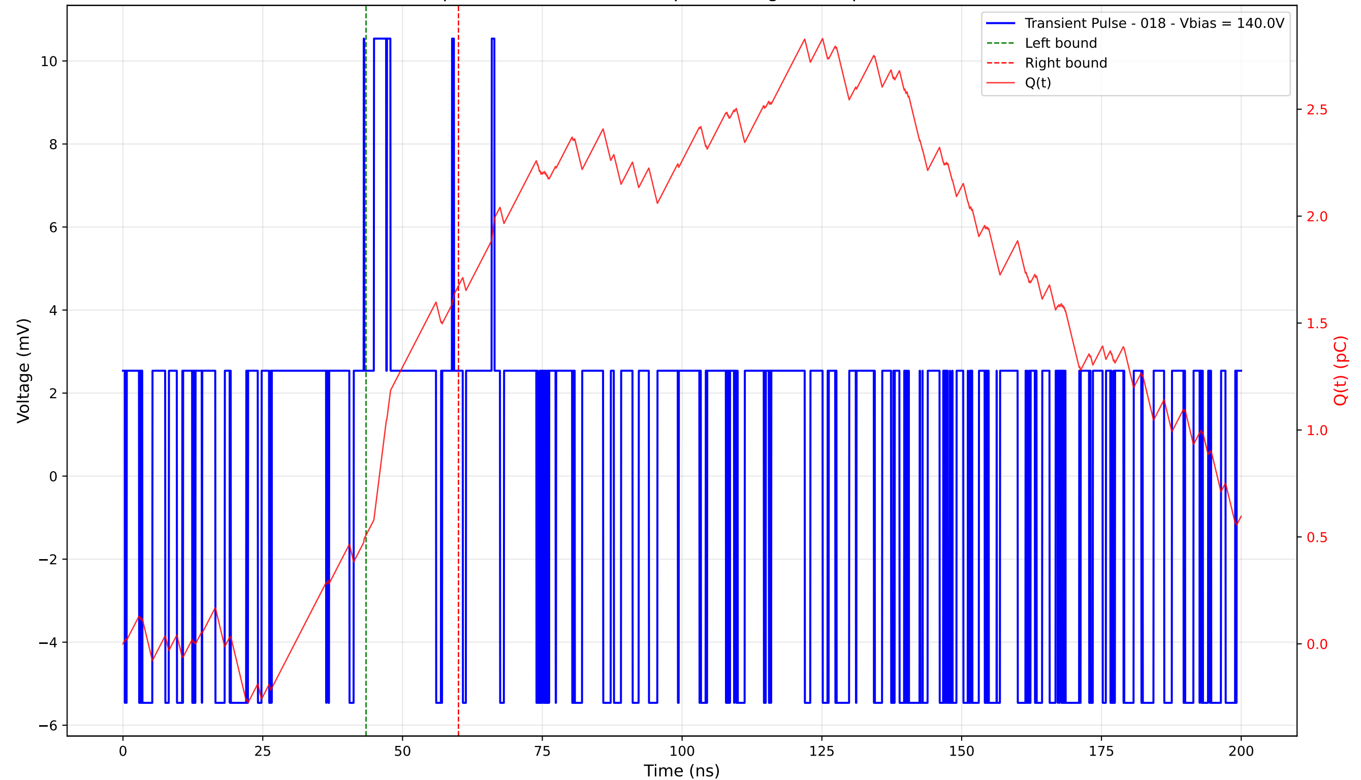
Transient Pulse - Sample: 4003 - Position: 0.0 \mu\text{m} - Charge: 1.17 pC - Rise Time: 0.00 ns (N/A)
