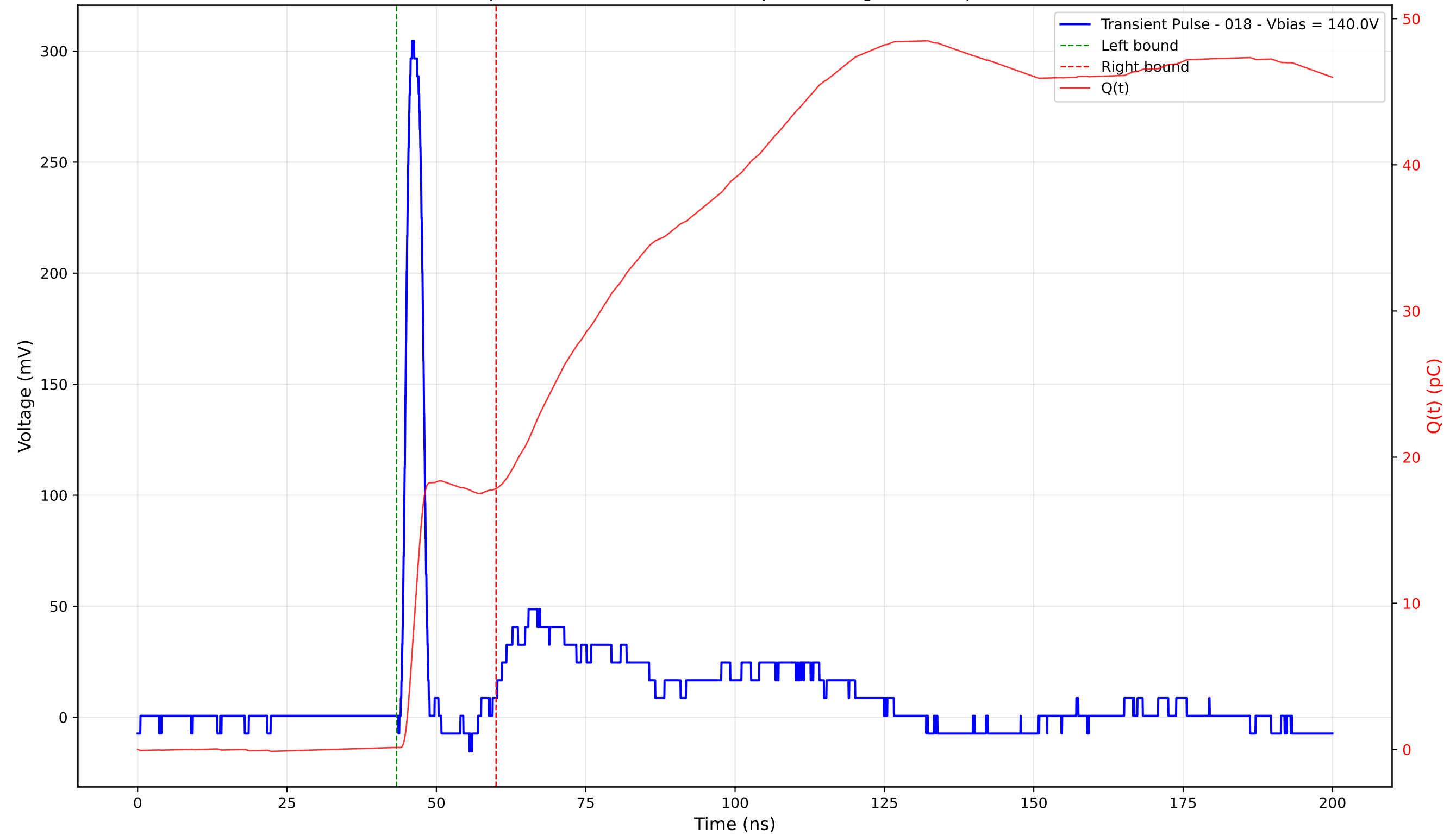
Transient Pulse - Sample: 4003 - Position: 240.0 \mu\text{m} - Charge: 17.70 pC - Rise Time: 1.23 ns
