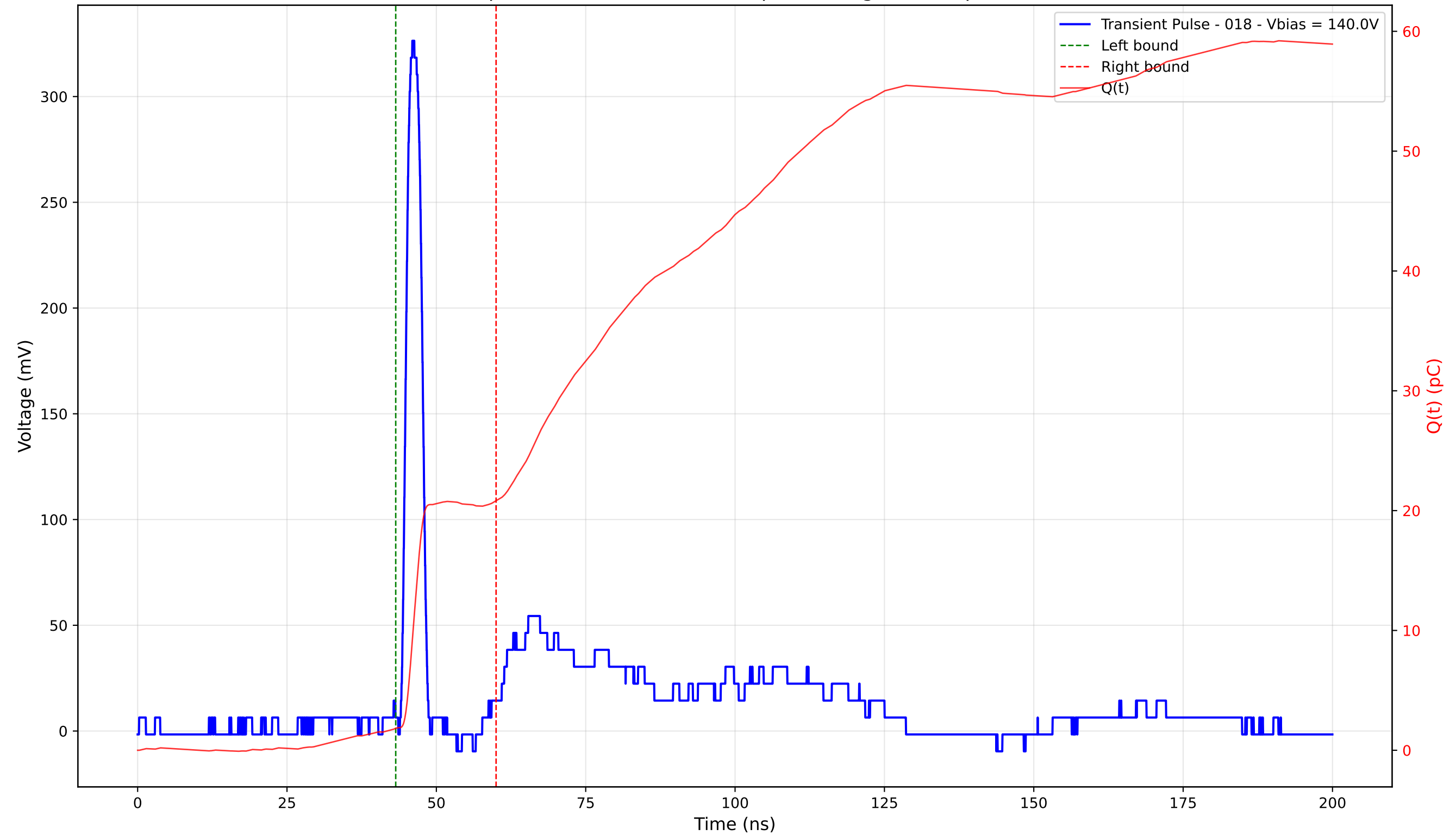
Transient Pulse - Sample: 4003 - Position: 235.0 \mu\text{m} - Charge: 18.98 pC - Rise Time: 1.17 ns
