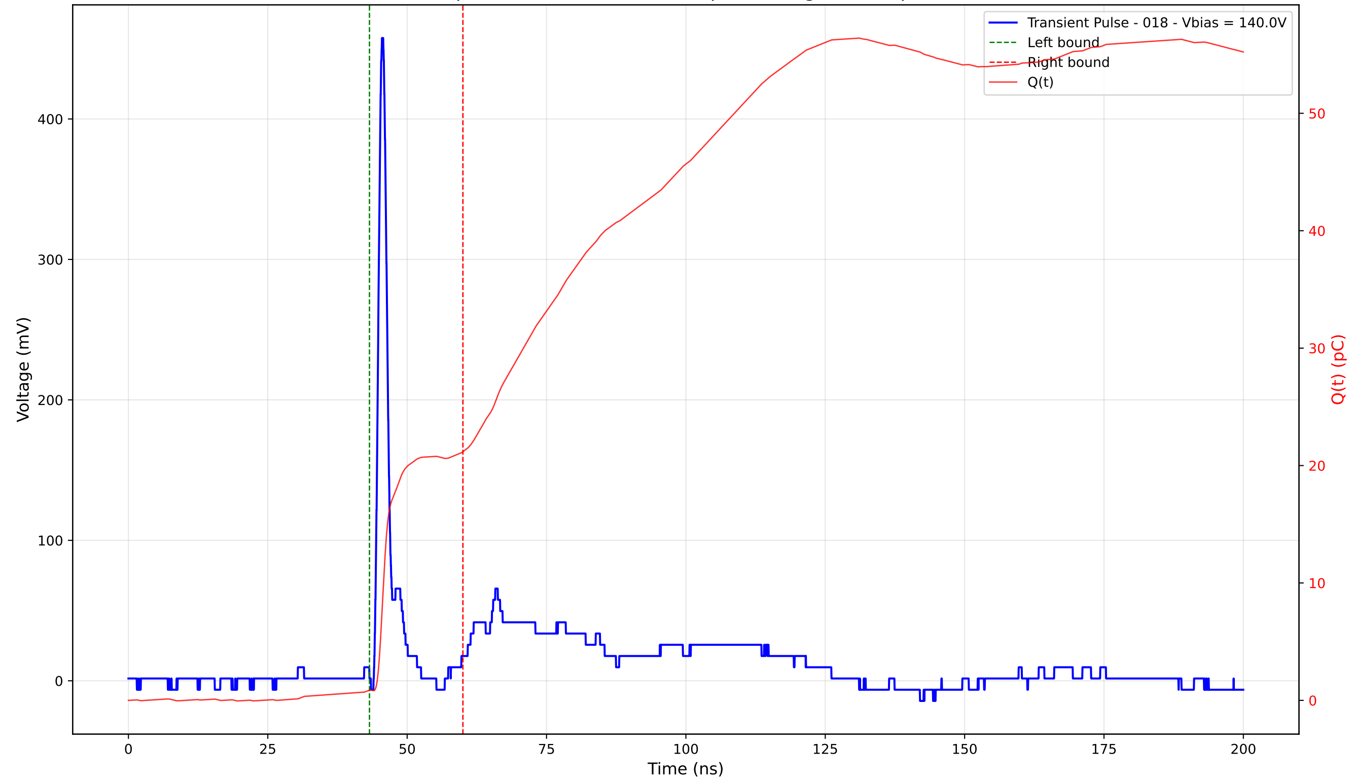
Transient Pulse - Sample: 4003 - Position: 160.0 \mu\text{m} - Charge: 20.30 pC - Rise Time: 0.97 ns
