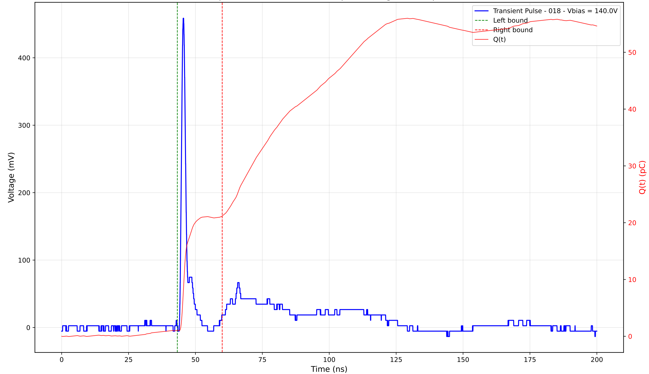
Transient Pulse - Sample: 4003 - Position: 145.0 \mu\text{m} - Charge: 20.14 pC - Rise Time: 0.95 ns
