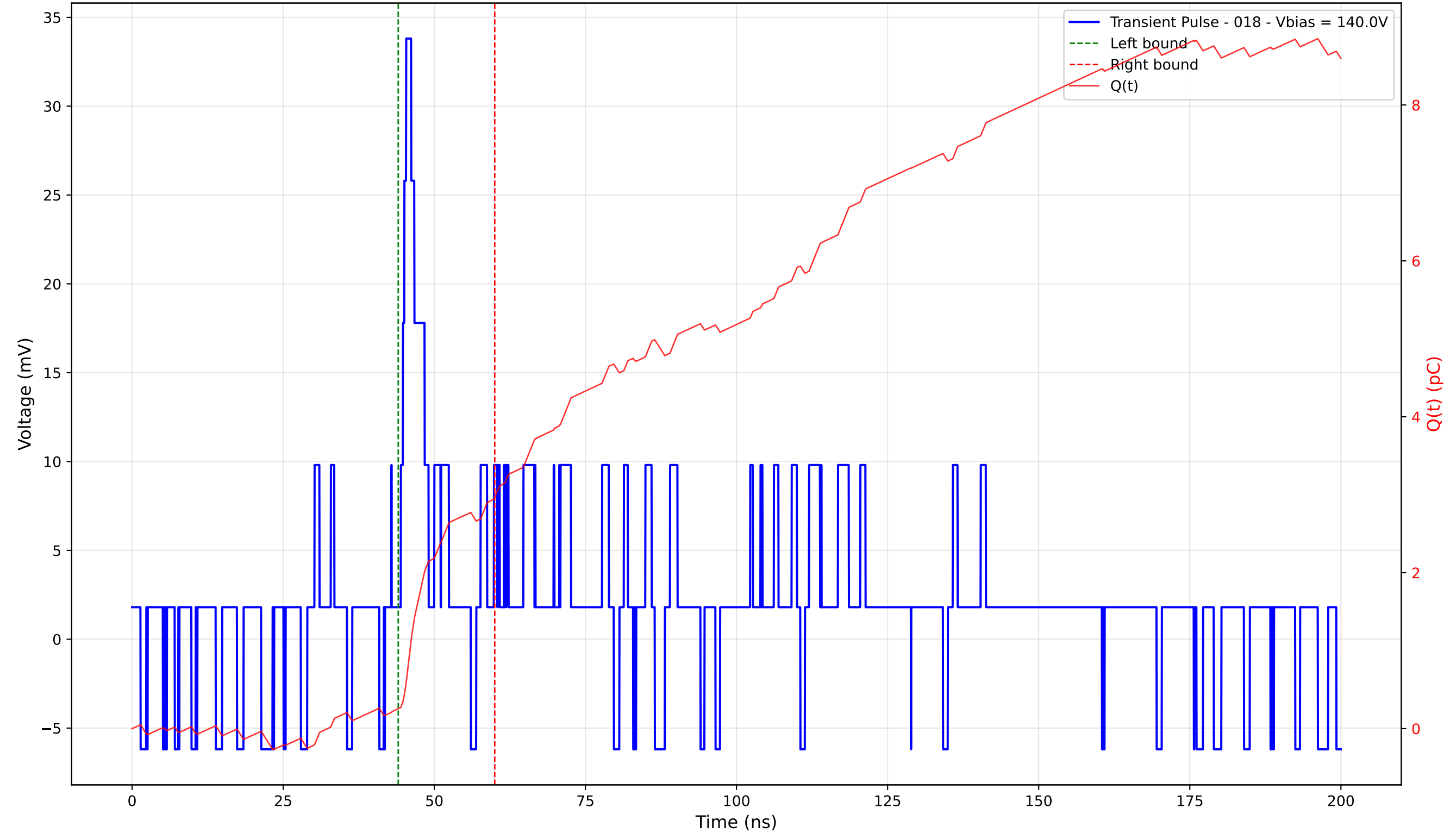
Transient Pulse - Sample: 4003 - Position: 330.0 \mu\text{m} - Charge: 2.72 pC - Rise Time: 0.90 ns
