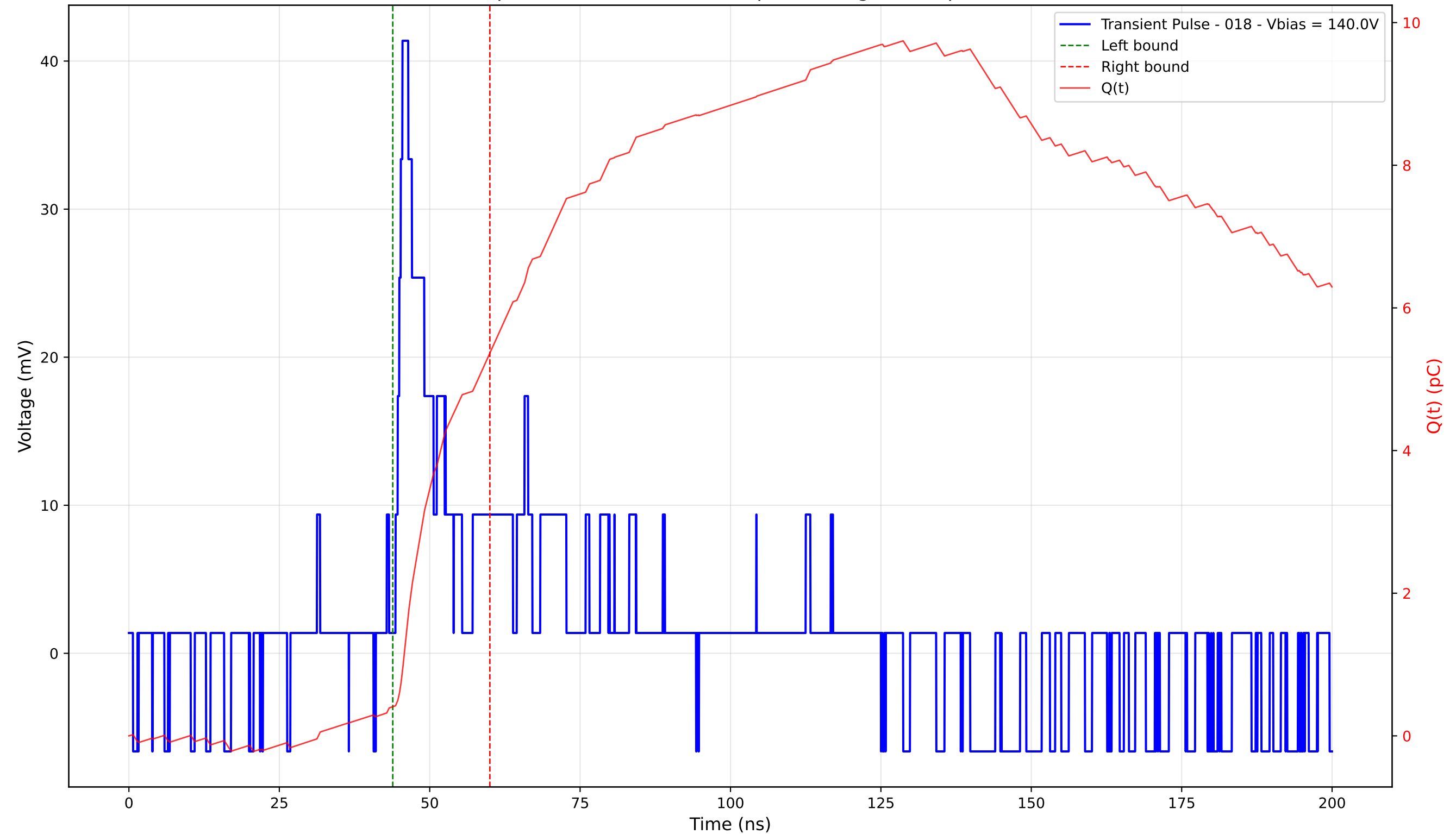
Transient Pulse - Sample: 4003 - Position: 55.0 \mu\text{m} - Charge: 4.96 pC - Rise Time: 1.15 ns
