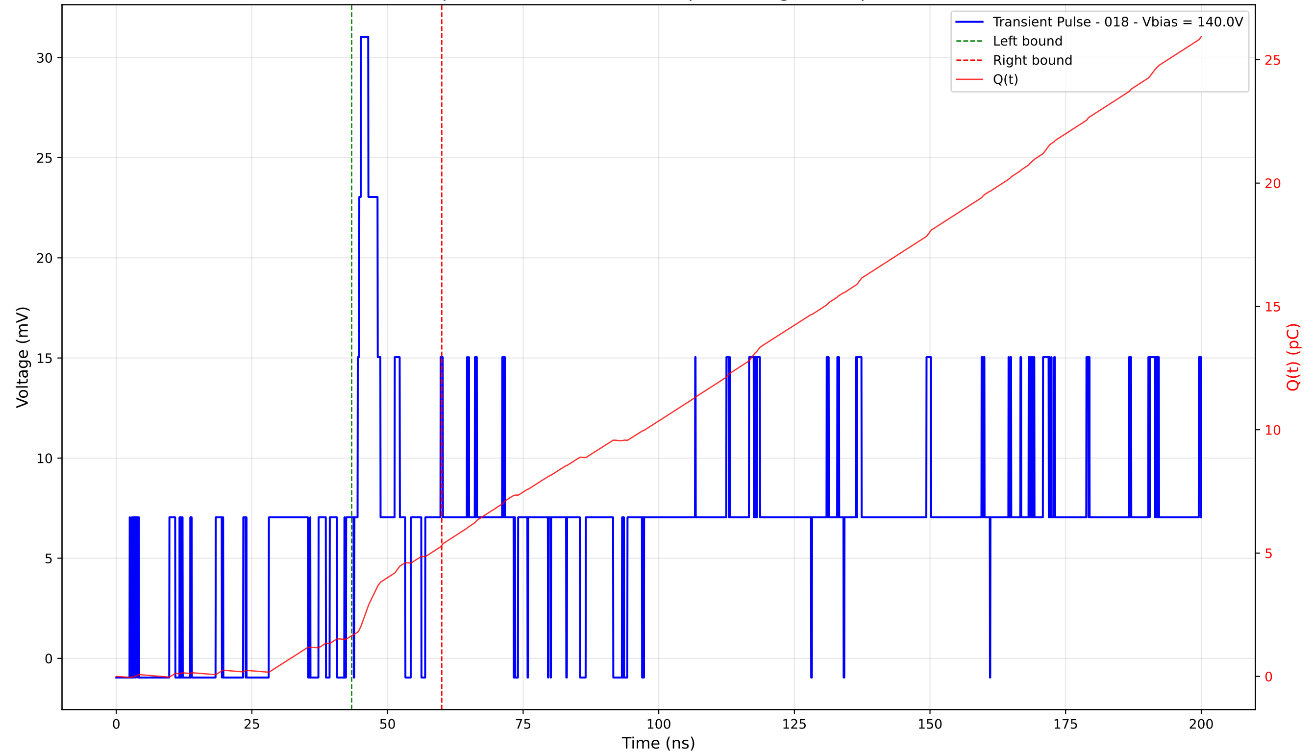
Transient Pulse - Sample: 4003 - Position: 335.0 \mu\text{m} - Charge: 3.66 pC - Rise Time: 1.21 ns
