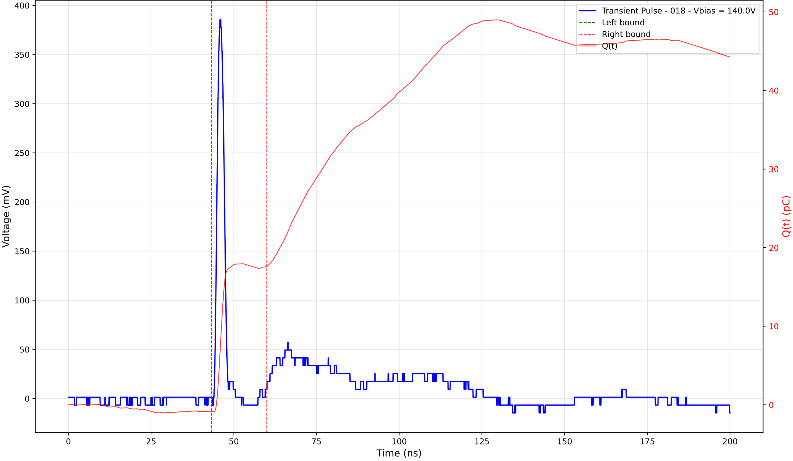
Transient Pulse - Sample: 4003 - Position: 215.0 \mu\text{m} - Charge: 18.48 pC - Rise Time: 1.17 ns
