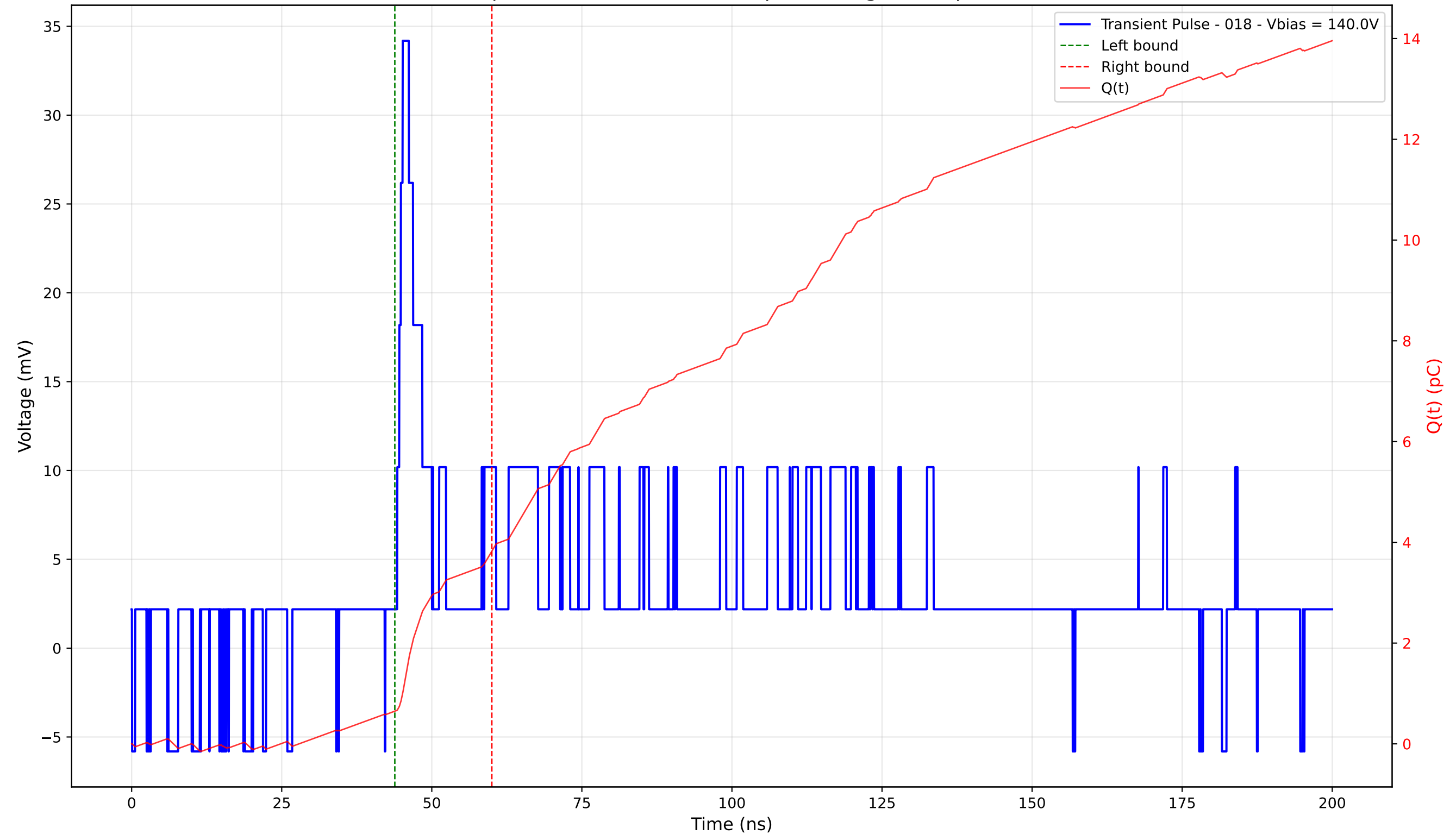
Transient Pulse - Sample: 4003 - Position: 320.0 \mu\text{m} - Charge: 3.18 pC - Rise Time: 0.92 ns
