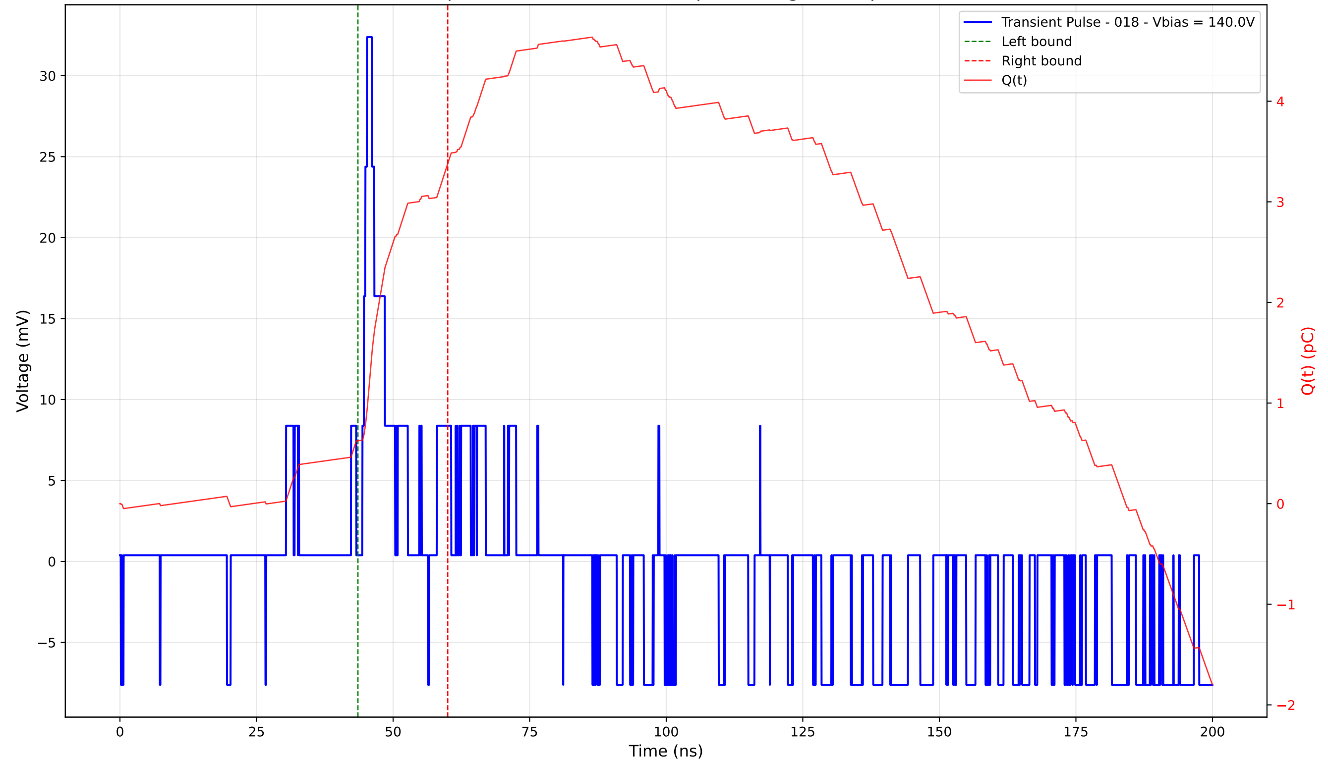
Transient Pulse - Sample: 4003 - Position: 370.0 \mu\text{m} - Charge: 2.75 pC - Rise Time: 0.85 ns
