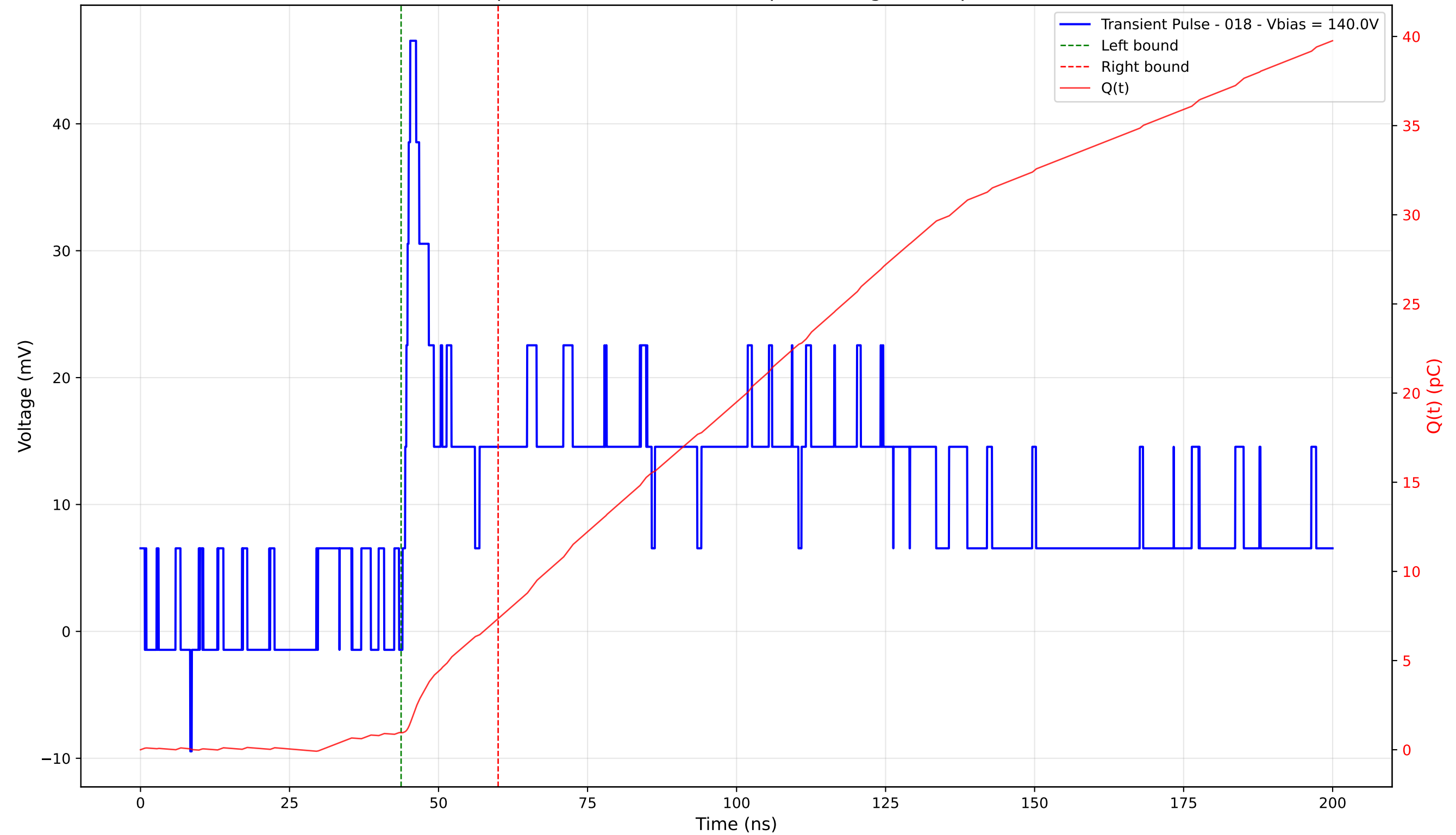
Transient Pulse - Sample: 4003 - Position: 305.0 \mu\text{m} - Charge: 6.39 pC - Rise Time: 1.29 ns
