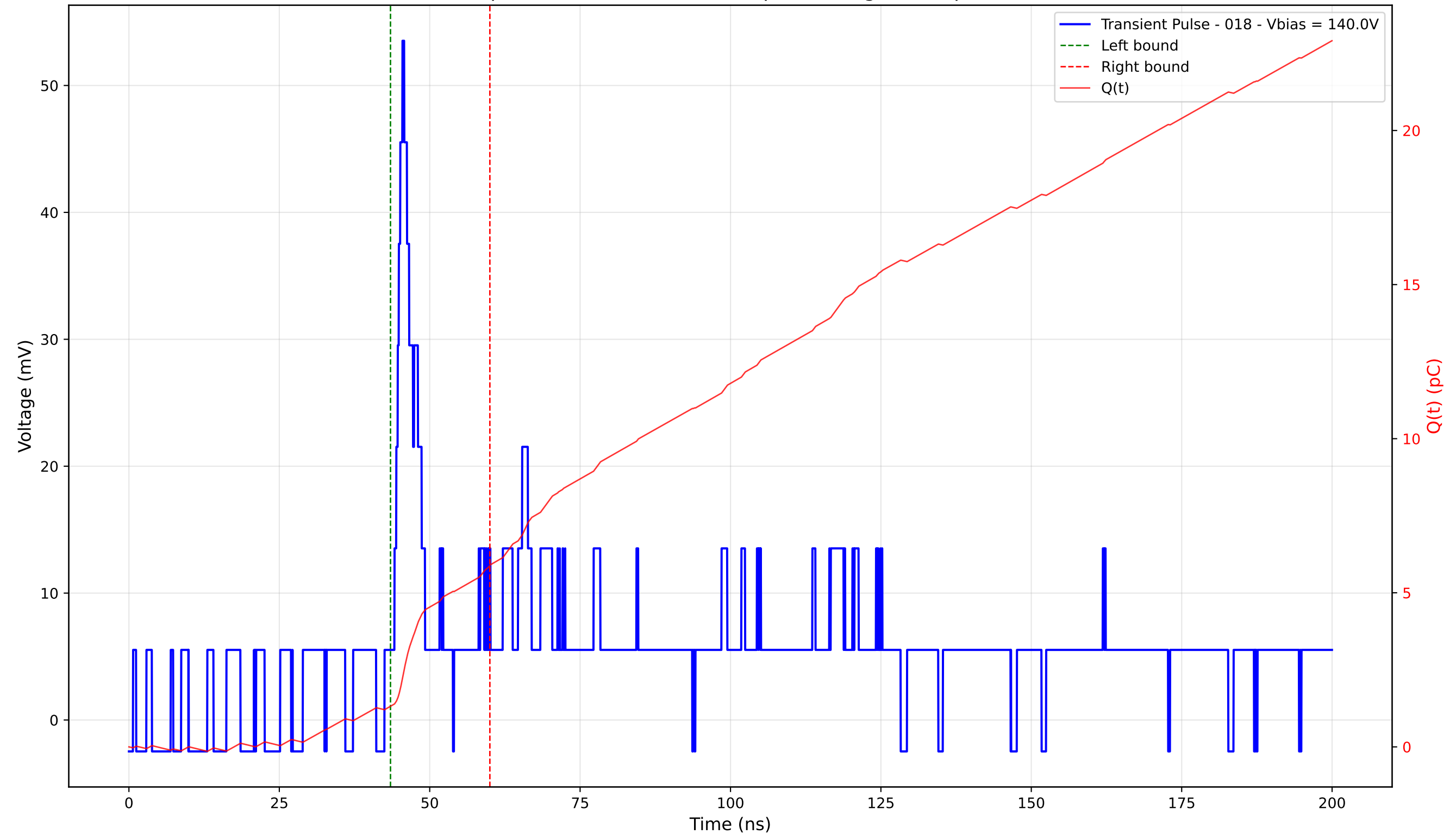
Transient Pulse - Sample: 4003 - Position: 395.0 \mu\text{m} - Charge: 4.57 pC - Rise Time: 2.98 ns
