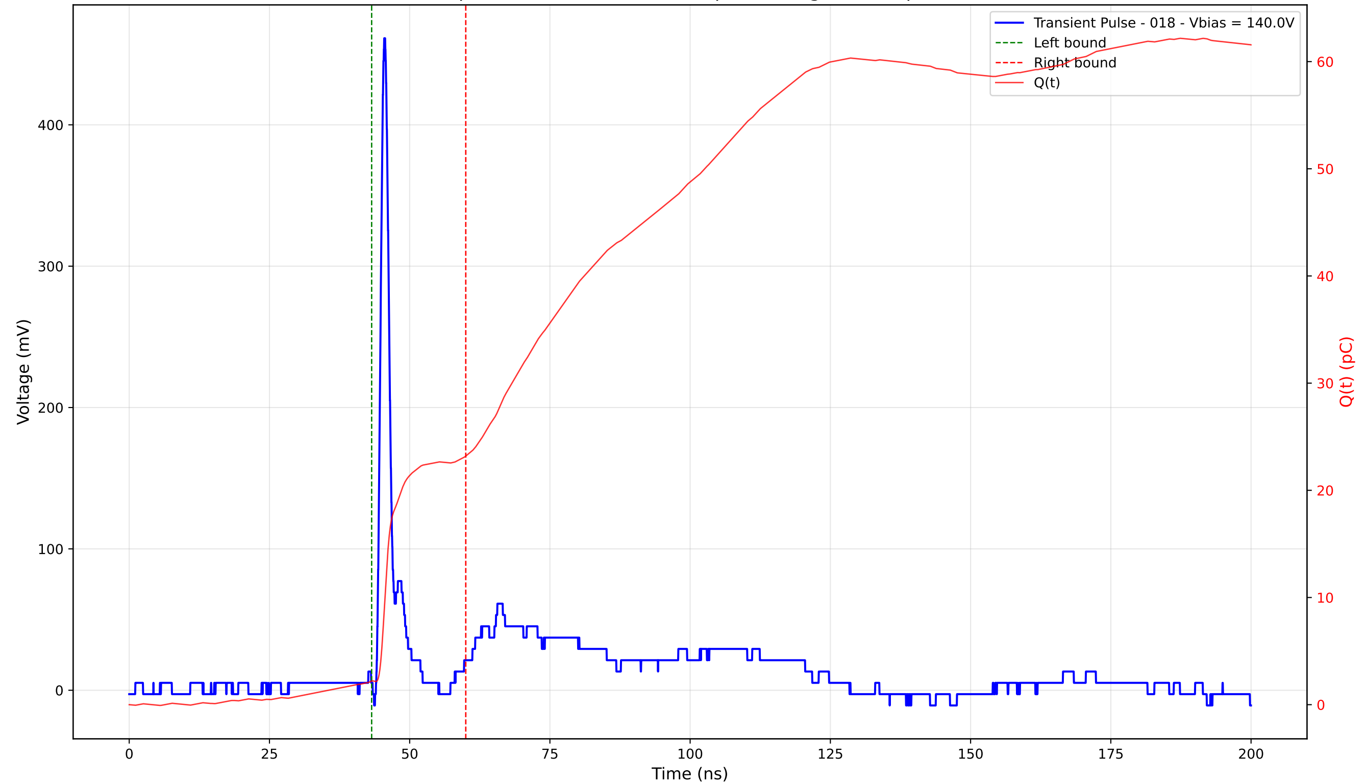
Transient Pulse - Sample: 4003 - Position: 150.0 \mu\text{m} - Charge: 20.99 pC - Rise Time: 0.96 ns
