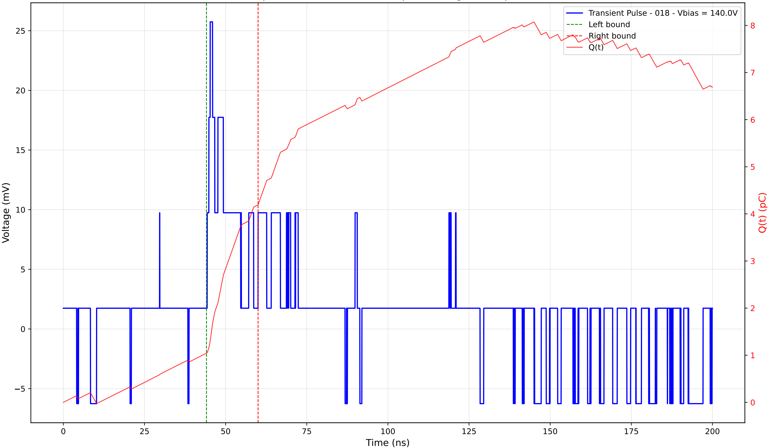
Transient Pulse - Sample: 4003 - Position: 65.0 \mu\text{m} - Charge: 3.15 pC - Rise Time: 0.94 ns
