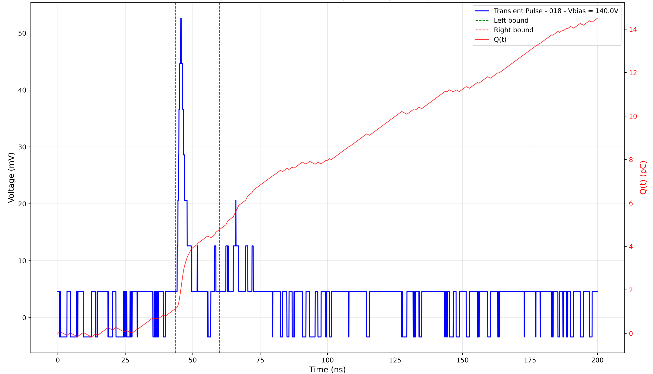
Transient Pulse - Sample: 4003 - Position: 400.0 \mu\text{m} - Charge: 3.64 pC - Rise Time: 1.40 ns
