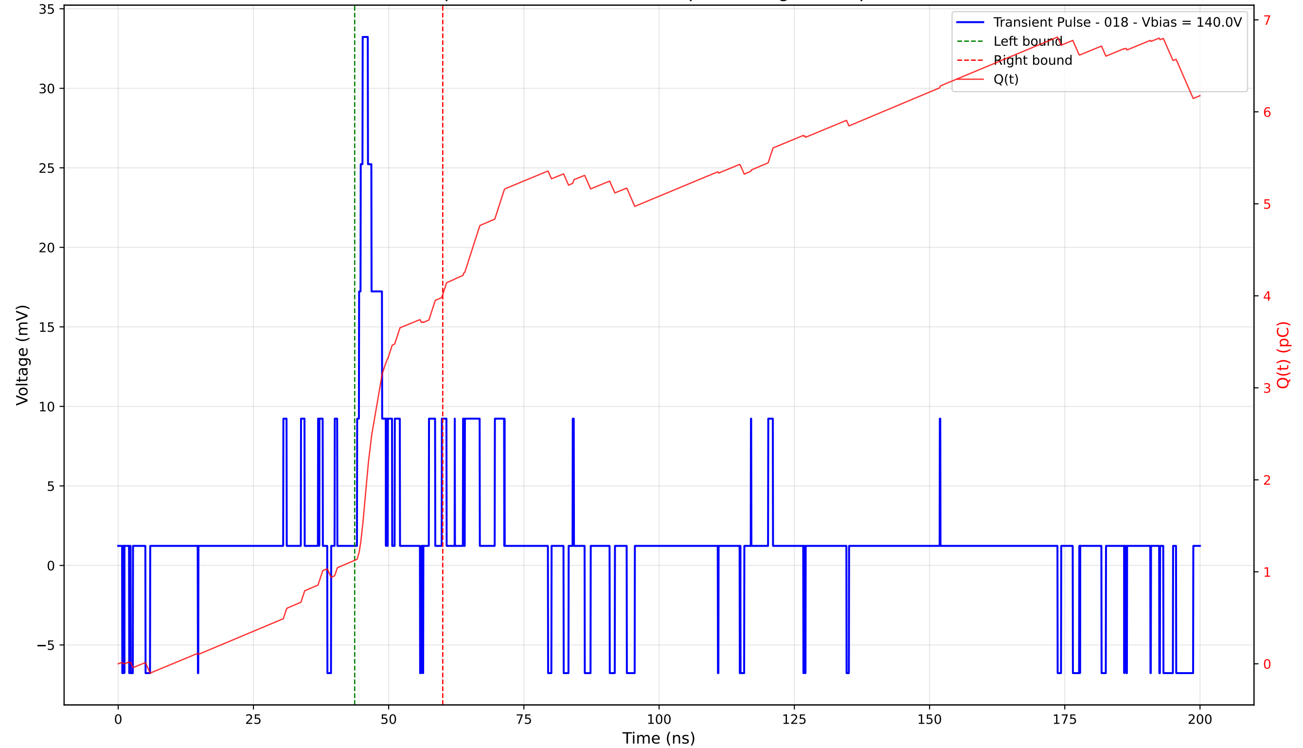
Transient Pulse - Sample: 4003 - Position: 360.0 \mu\text{m} - Charge: 2.89 pC - Rise Time: 1.03 ns
