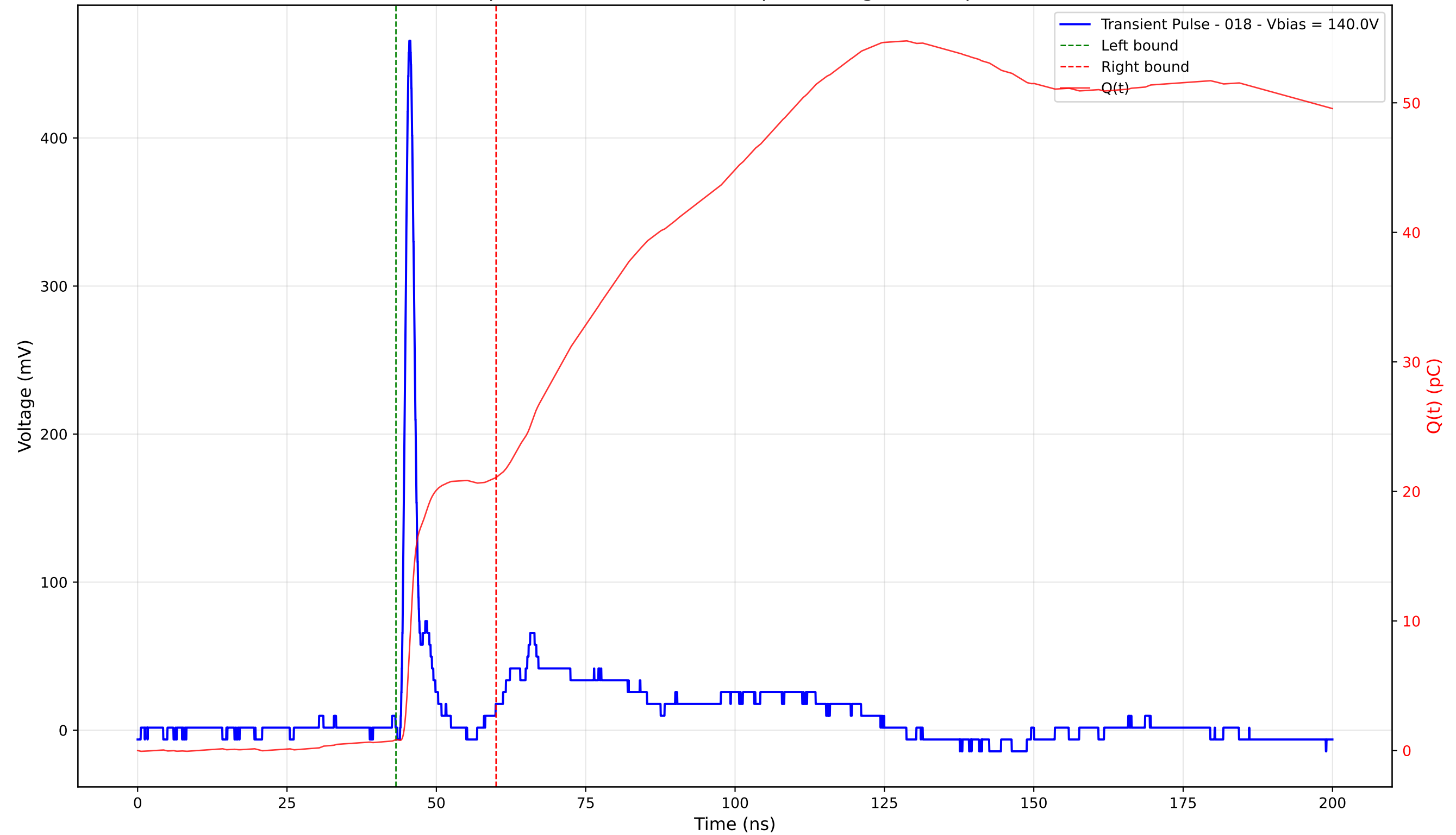
Transient Pulse - Sample: 4003 - Position: 155.0 \mu\text{m} - Charge: 20.24 pC - Rise Time: 0.97 ns
