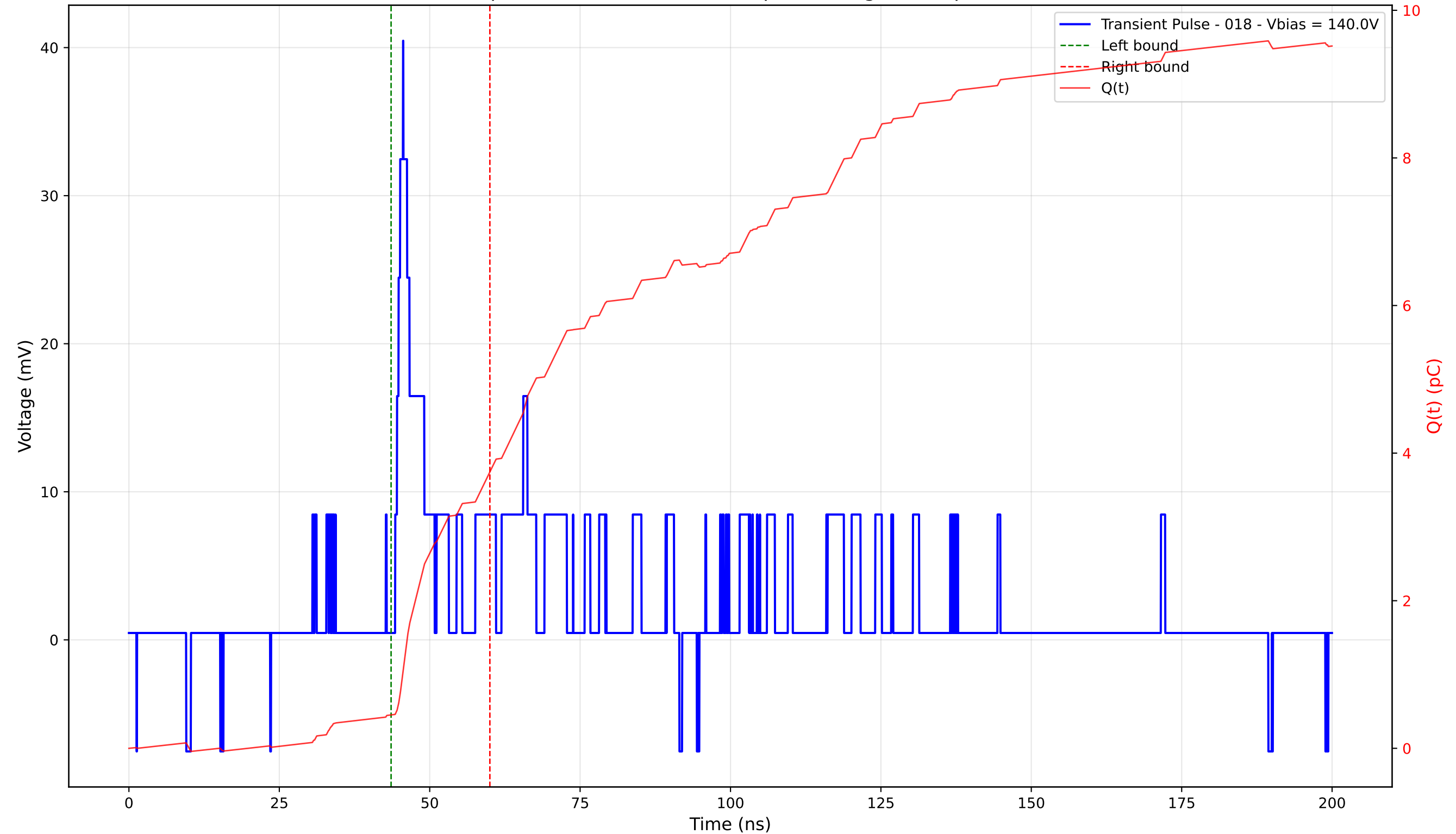
Transient Pulse - Sample: 4003 - Position: 340.0 \mu\text{m} - Charge: 3.30 pC - Rise Time: 1.31 ns
