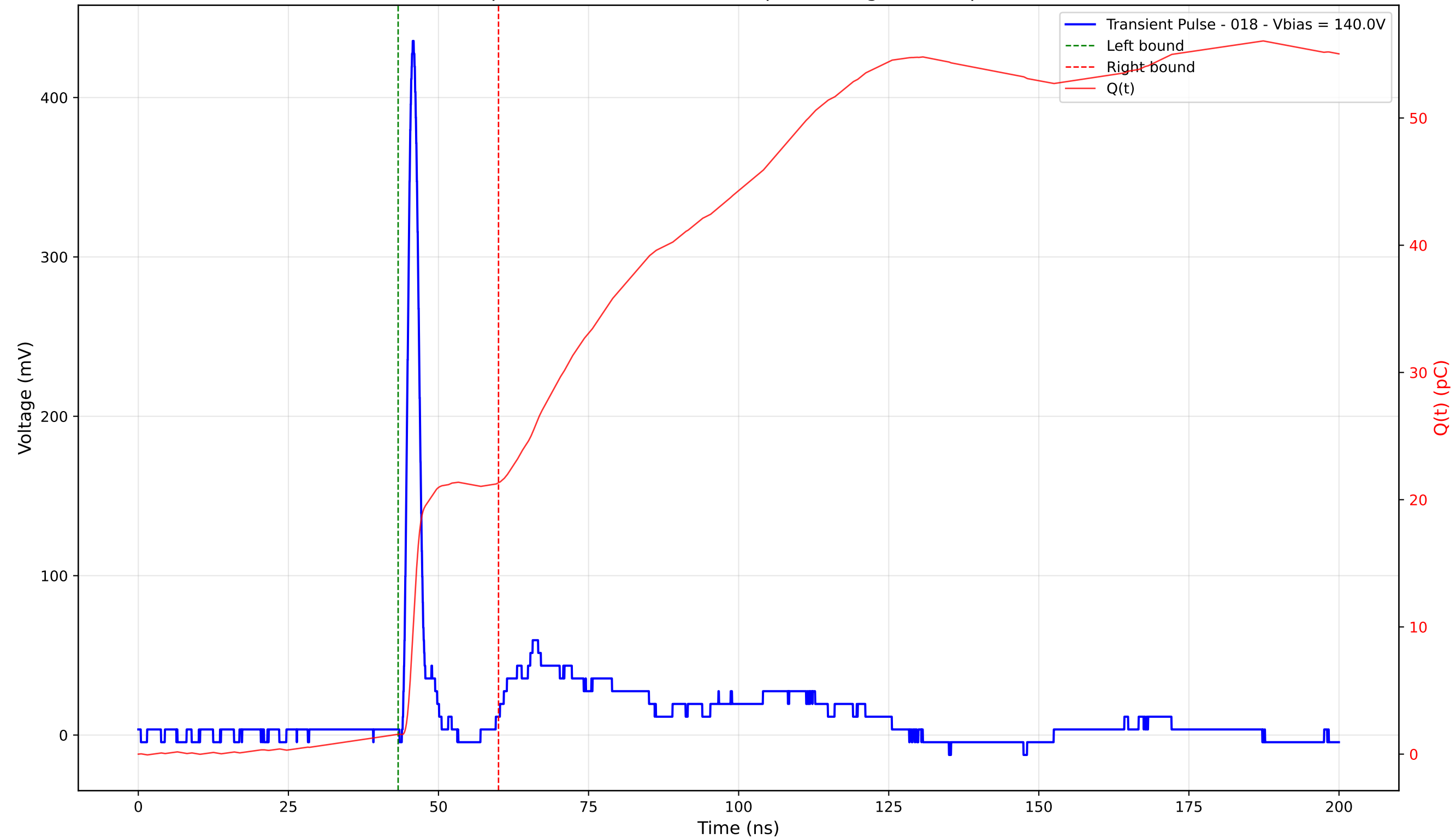
Transient Pulse - Sample: 4003 - Position: 195.0 \mu\text{m} - Charge: 19.77 pC - Rise Time: 1.10 ns
