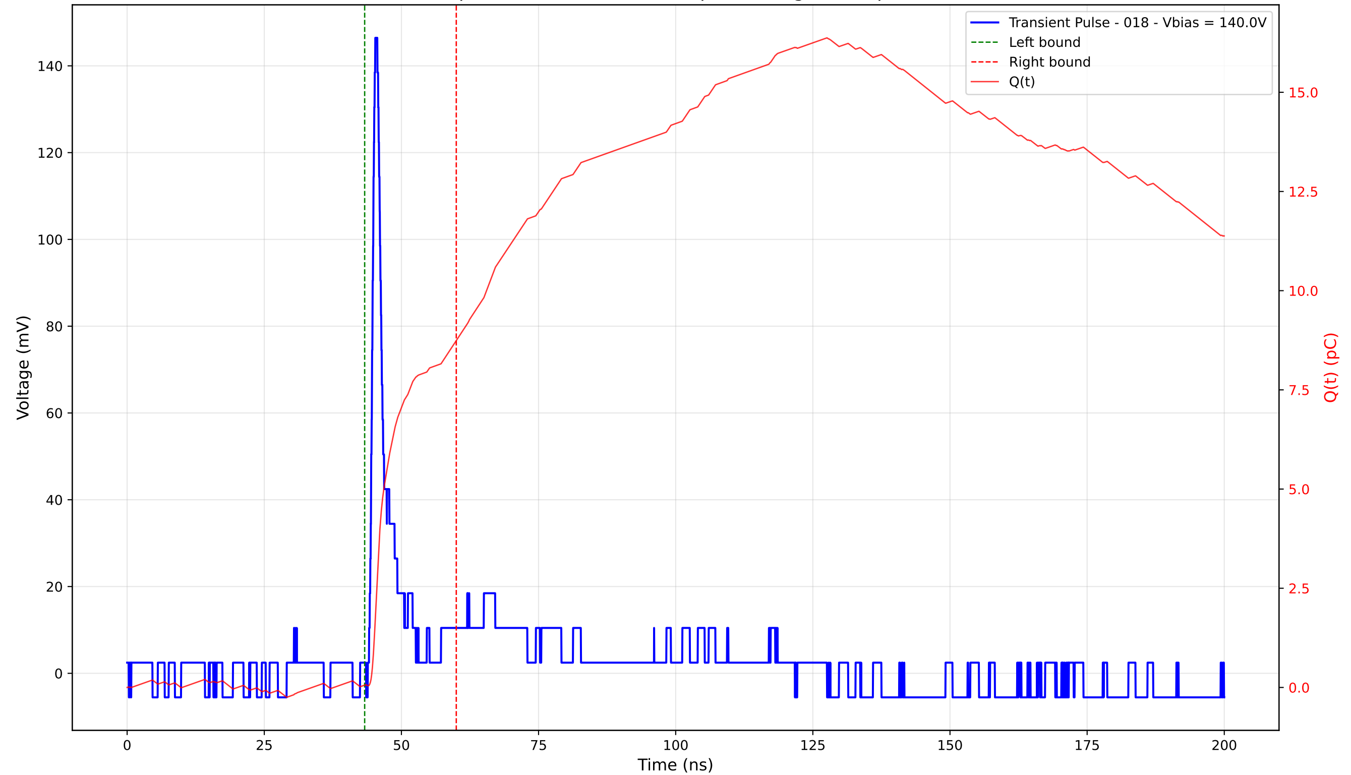
Transient Pulse - Sample: 4003 - Position: 95.0 \mu\text{m} - Charge: 8.68 pC - Rise Time: 0.91 ns
