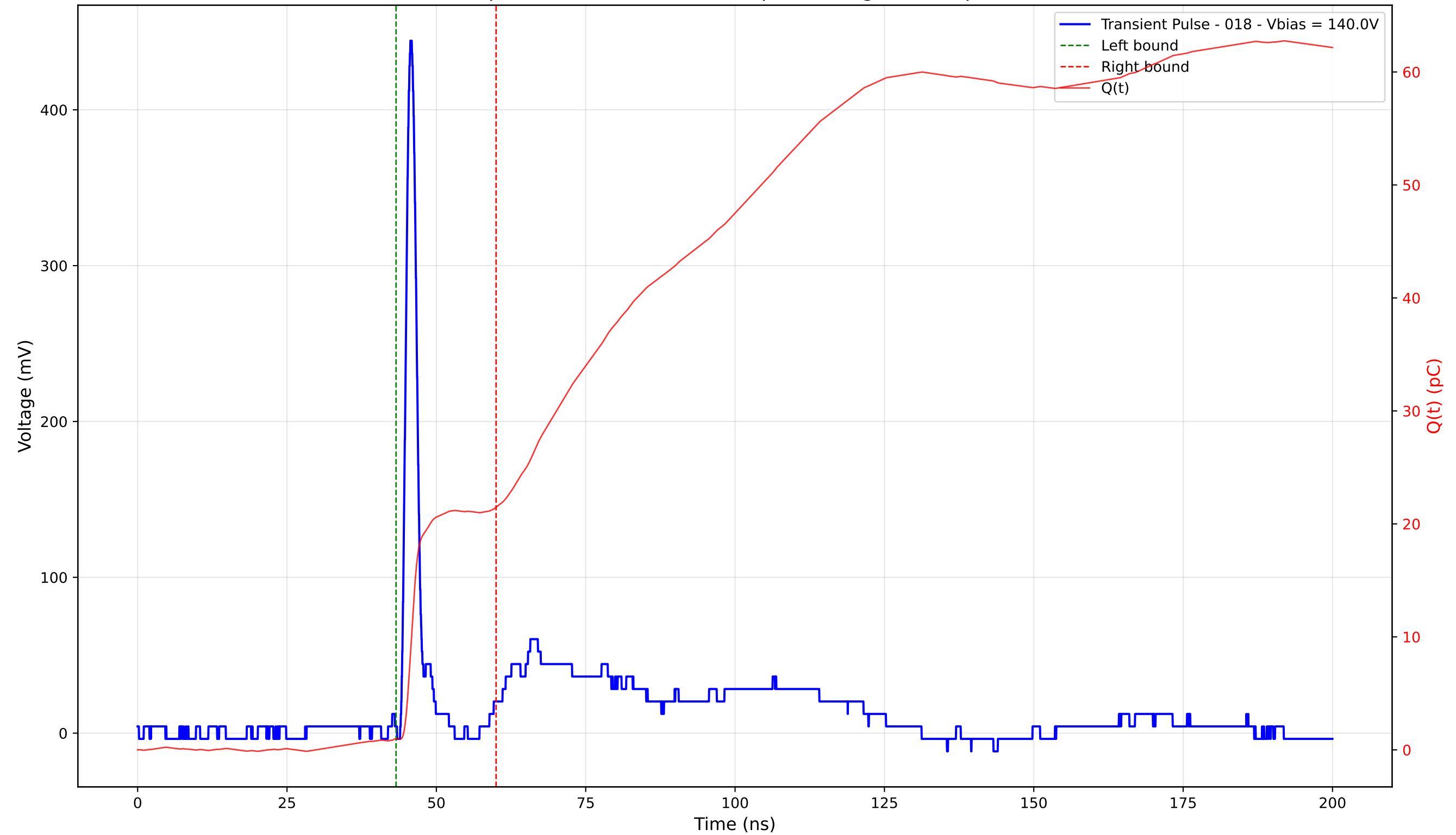
Transient Pulse - Sample: 4003 - Position: 190.0 \mu\text{m} - Charge: 20.49 pC - Rise Time: 1.08 ns
