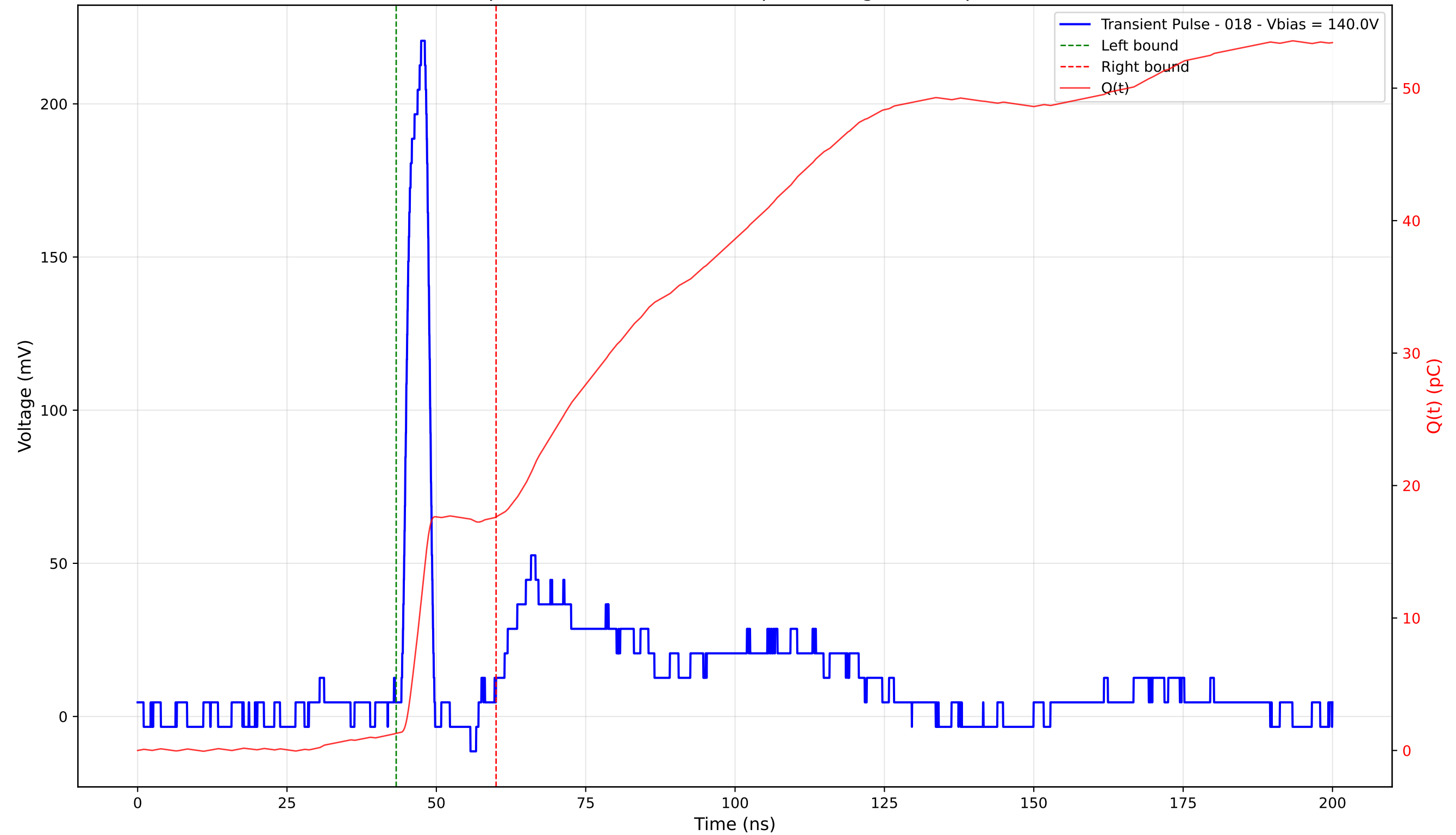
Transient Pulse - Sample: 4003 - Position: 270.0 \mu\text{m} - Charge: 16.33 pC - Rise Time: 2.48 ns
