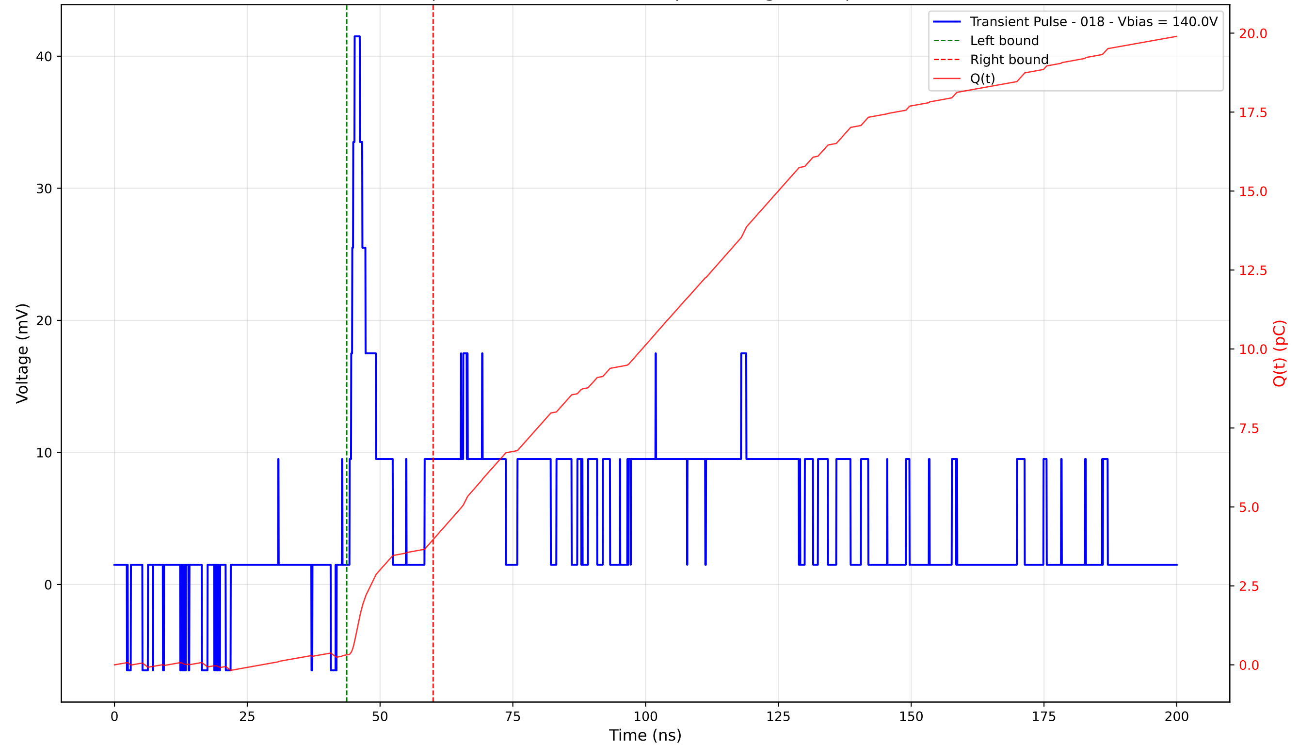
Transient Pulse - Sample: 4003 - Position: 315.0 \mu\text{m} - Charge: 3.65 pC - Rise Time: 0.95 ns
