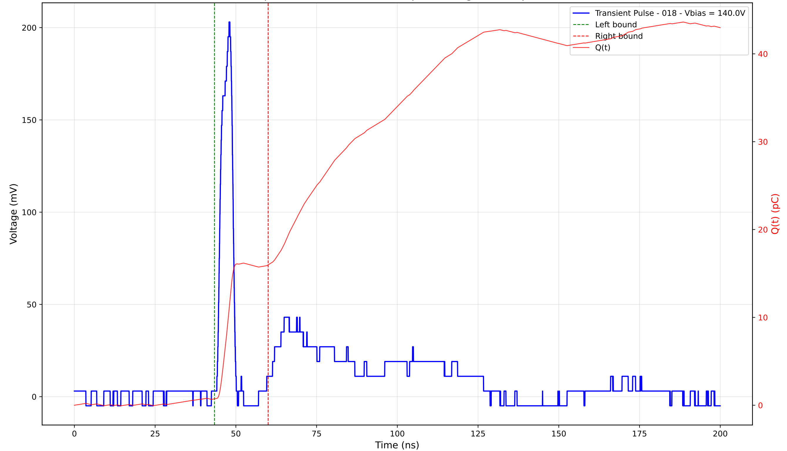
Transient Pulse - Sample: 4003 - Position: 275.0 \mu\text{m} - Charge: 15.26 pC - Rise Time: 2.96 ns
