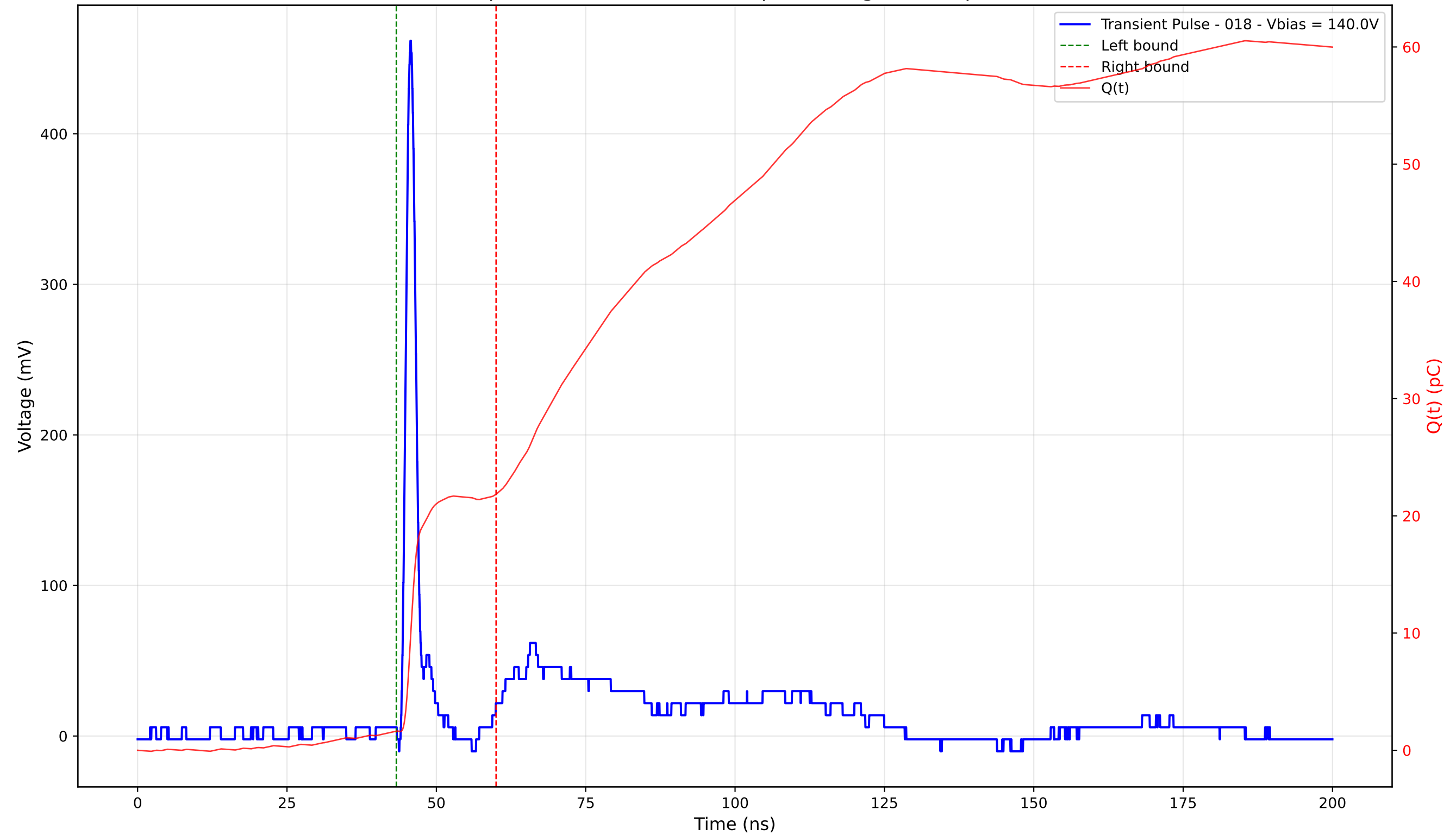
Transient Pulse - Sample: 4003 - Position: 180.0 \mu\text{m} - Charge: 20.19 pC - Rise Time: 1.04 ns
