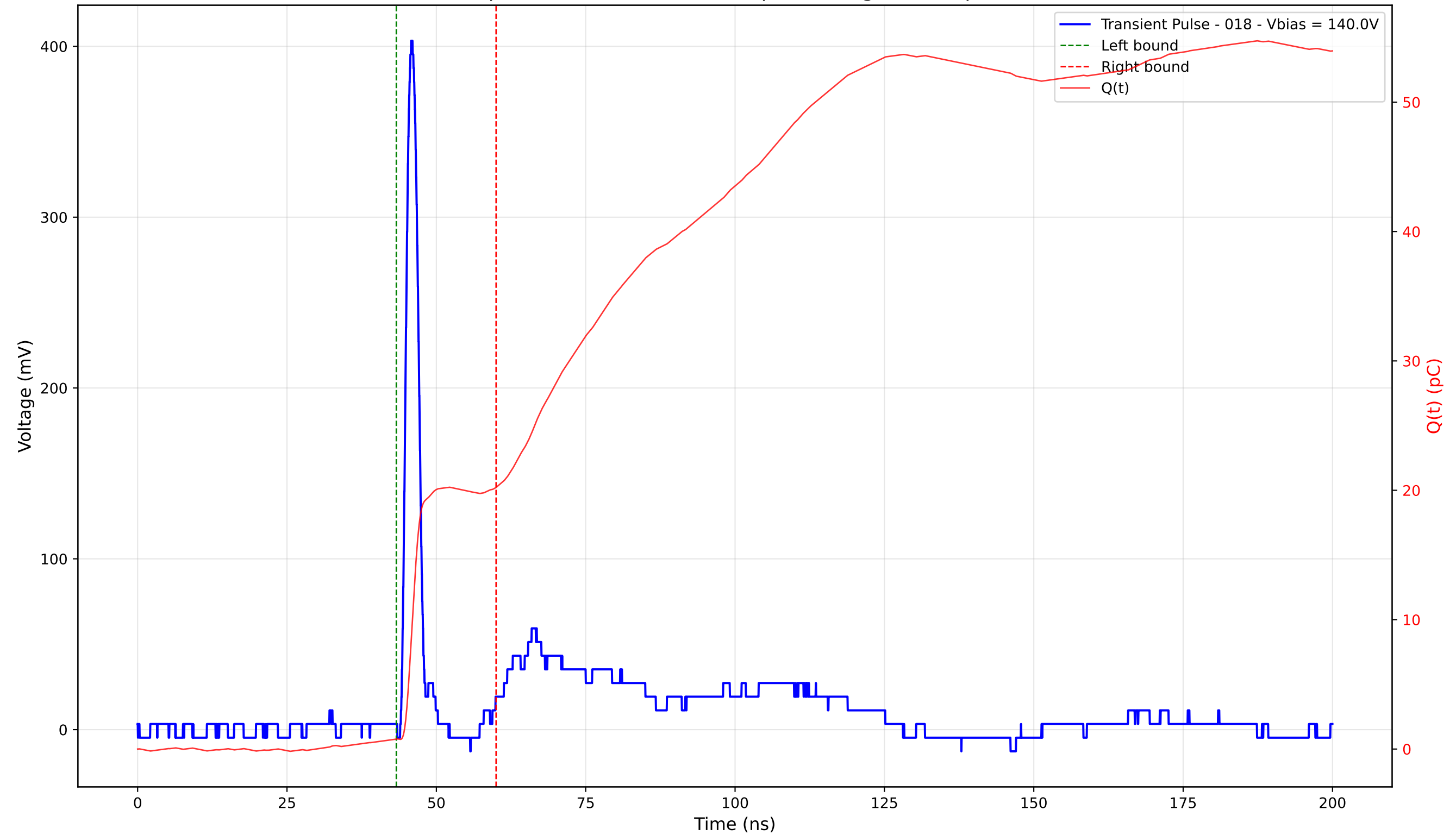
Transient Pulse - Sample: 4003 - Position: 210.0 \mu\text{m} - Charge: 19.44 pC - Rise Time: 1.11 ns
