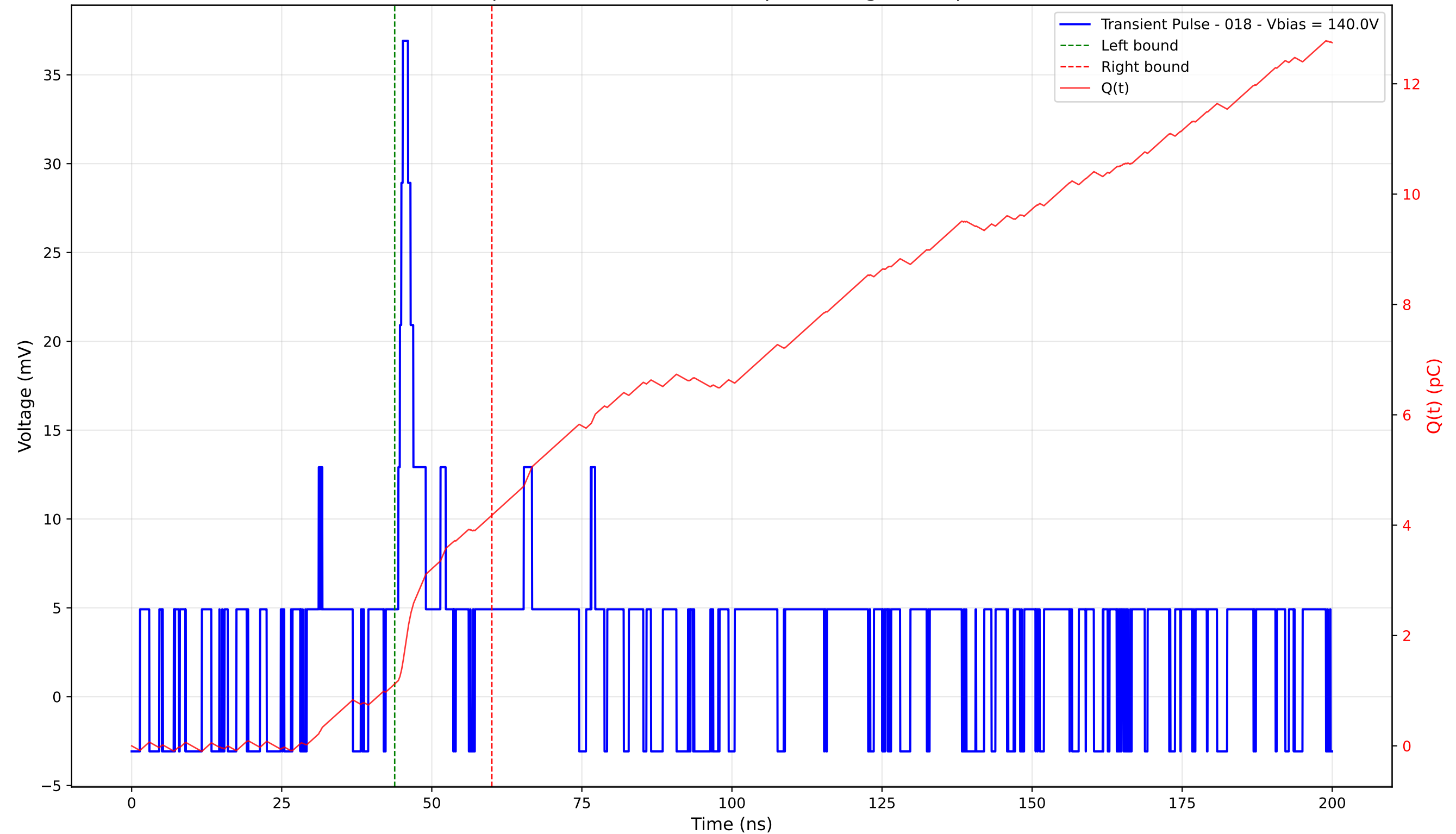
Transient Pulse - Sample: 4003 - Position: 410.0 \mu\text{m} - Charge: 3.06 pC - Rise Time: 2.85 ns
