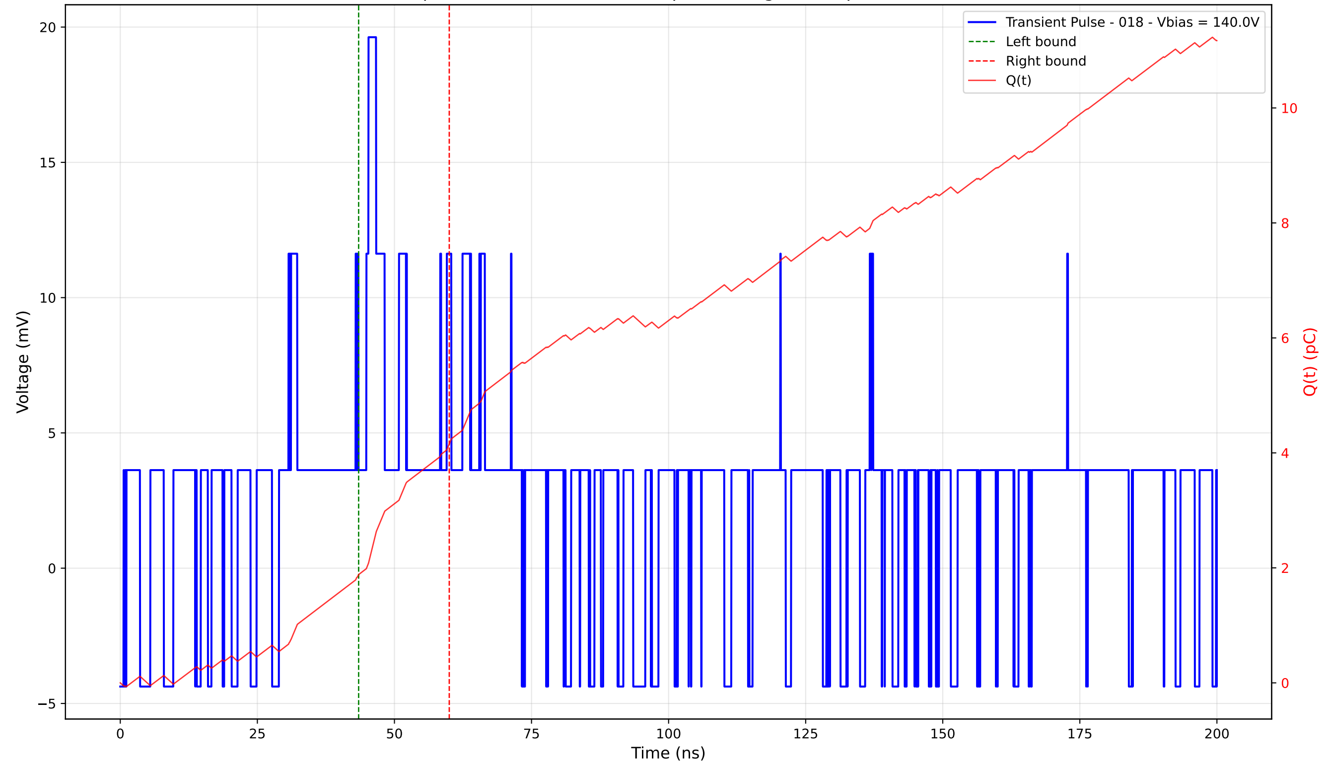
Transient Pulse - Sample: 4003 - Position: 420.0 \mu\text{m} - Charge: 2.27 pC - Rise Time: 0.00 ns (N/A)
