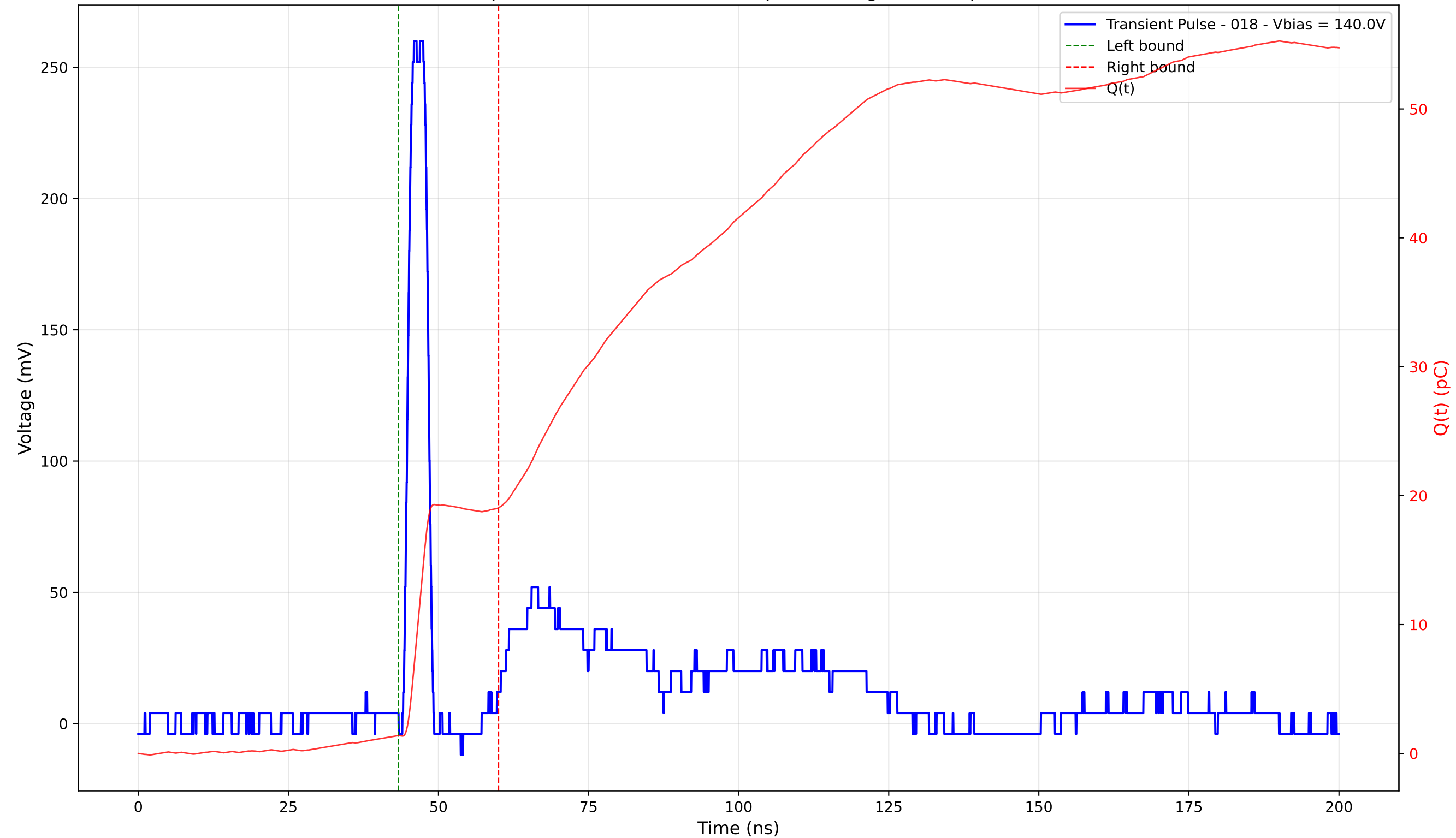
Transient Pulse - Sample: 4003 - Position: 255.0 \mu\text{m} - Charge: 17.67 pC - Rise Time: 1.21 ns
