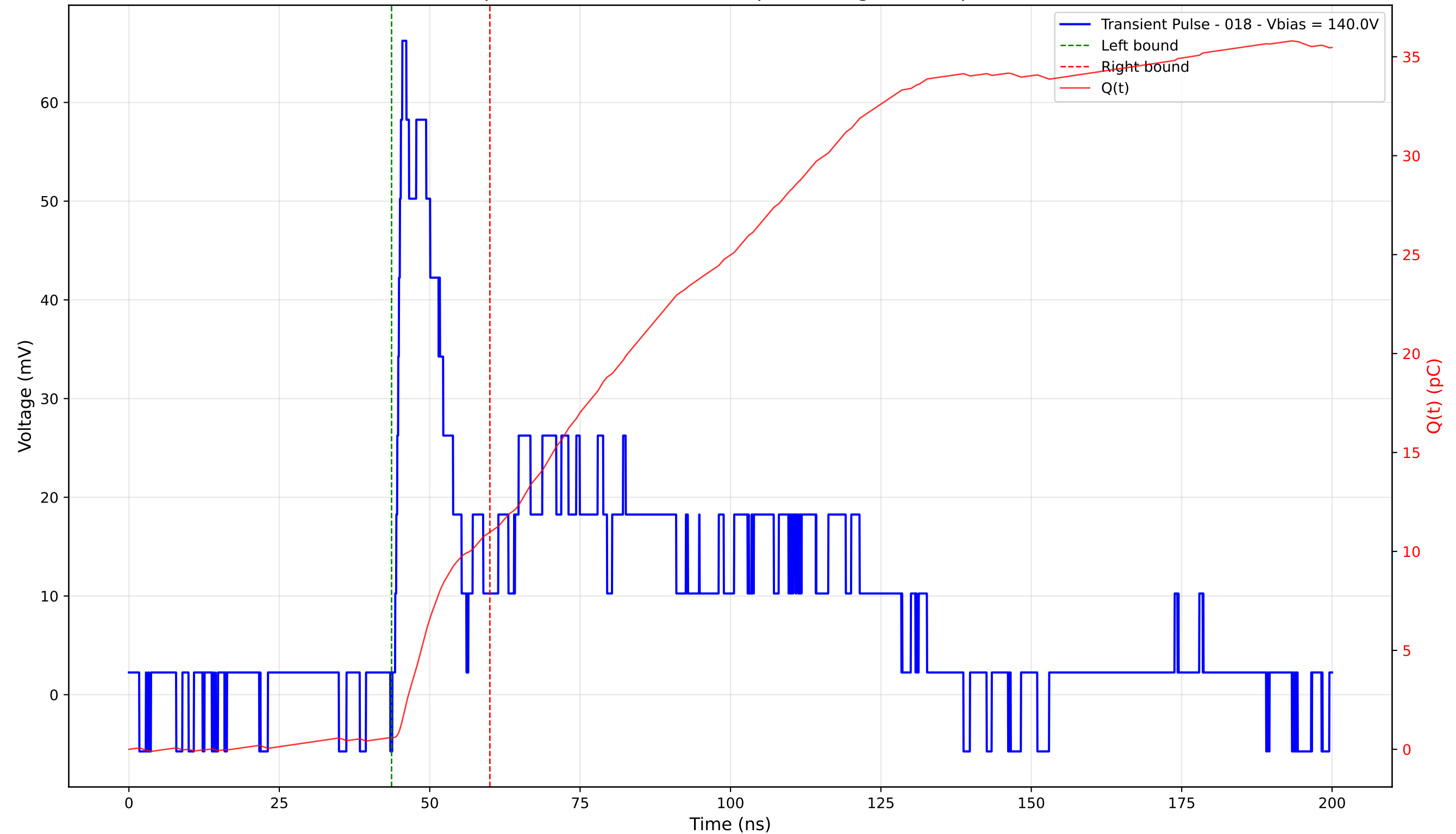
Transient Pulse - Sample: 4003 - Position: 295.0 \mu\text{m} - Charge: 10.37 pC - Rise Time: 1.19 ns
