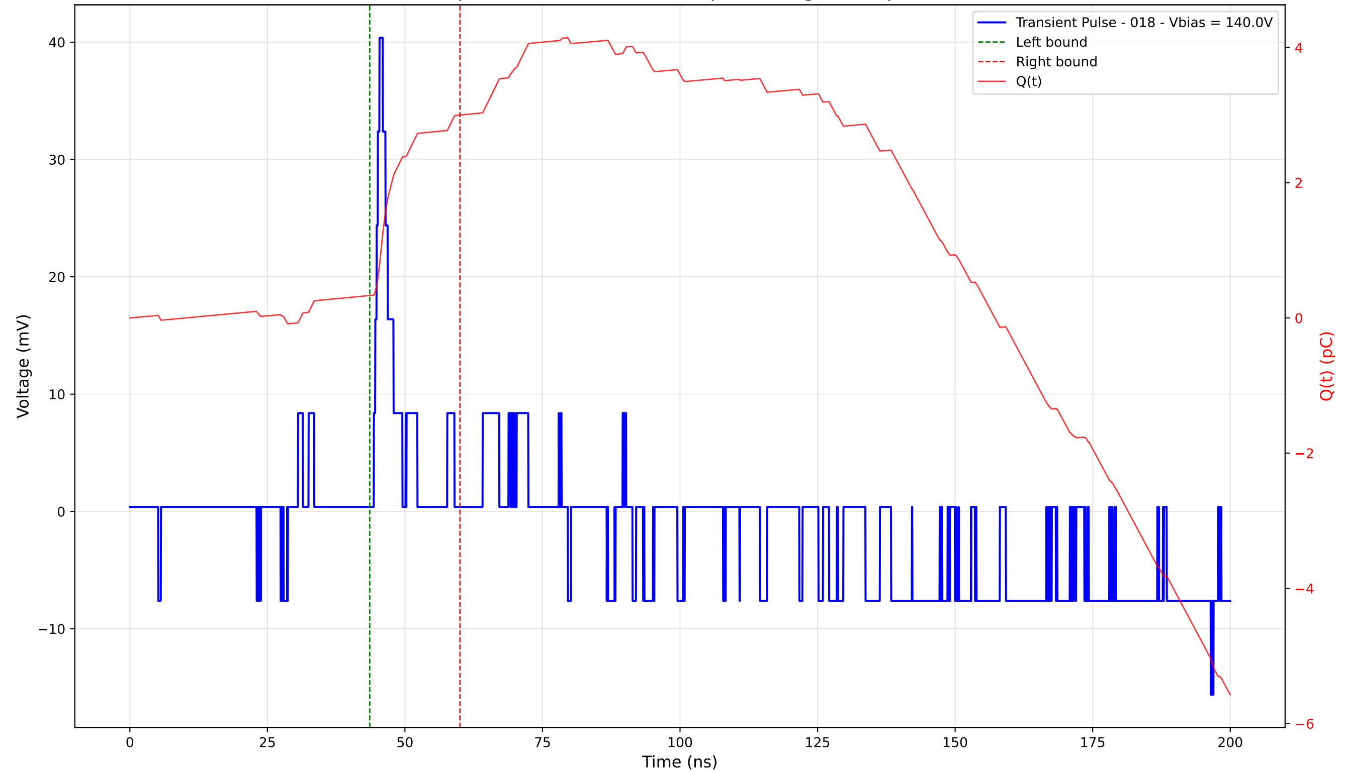
Transient Pulse - Sample: 4003 - Position: 405.0 \mu\text{m} - Charge: 2.67 pC - Rise Time: 1.03 ns
