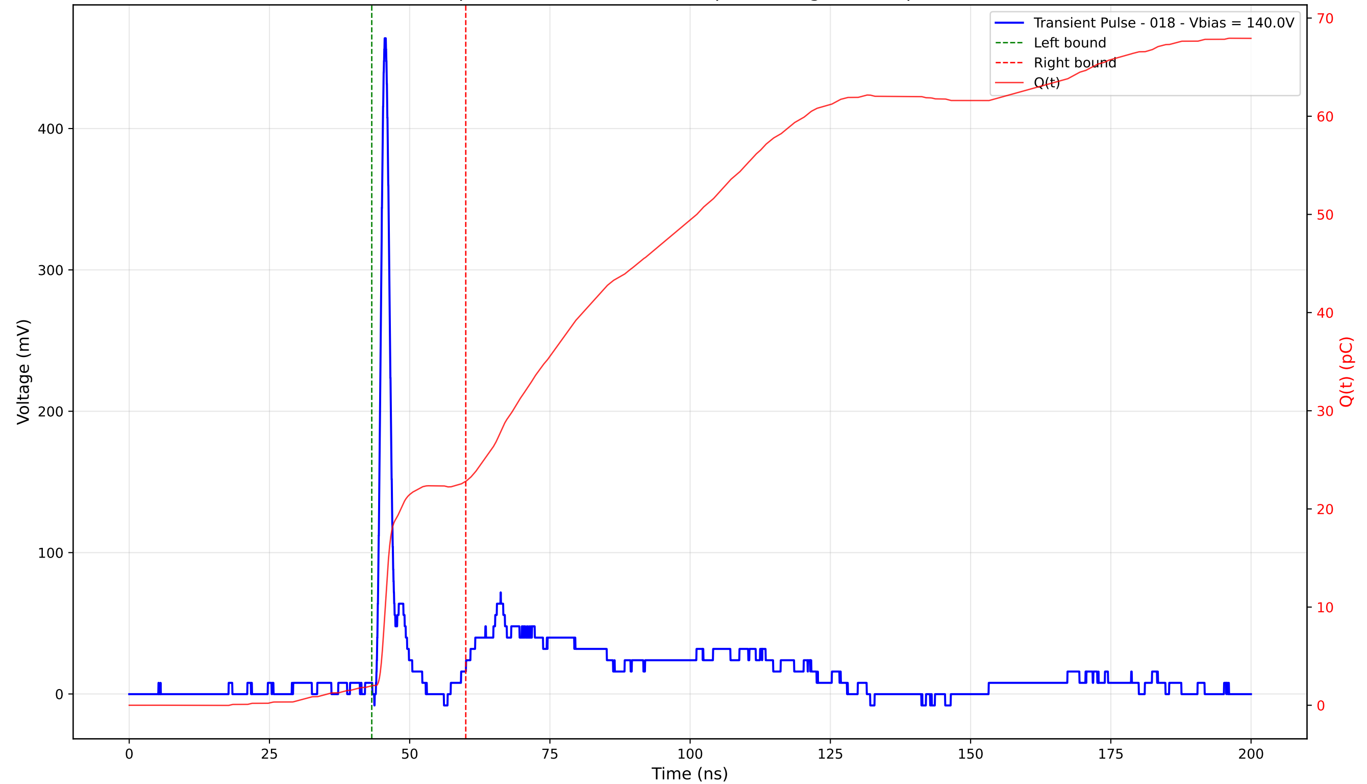
Transient Pulse - Sample: 4003 - Position: 170.0 \mu\text{m} - Charge: 20.81 pC - Rise Time: 1.03 ns
