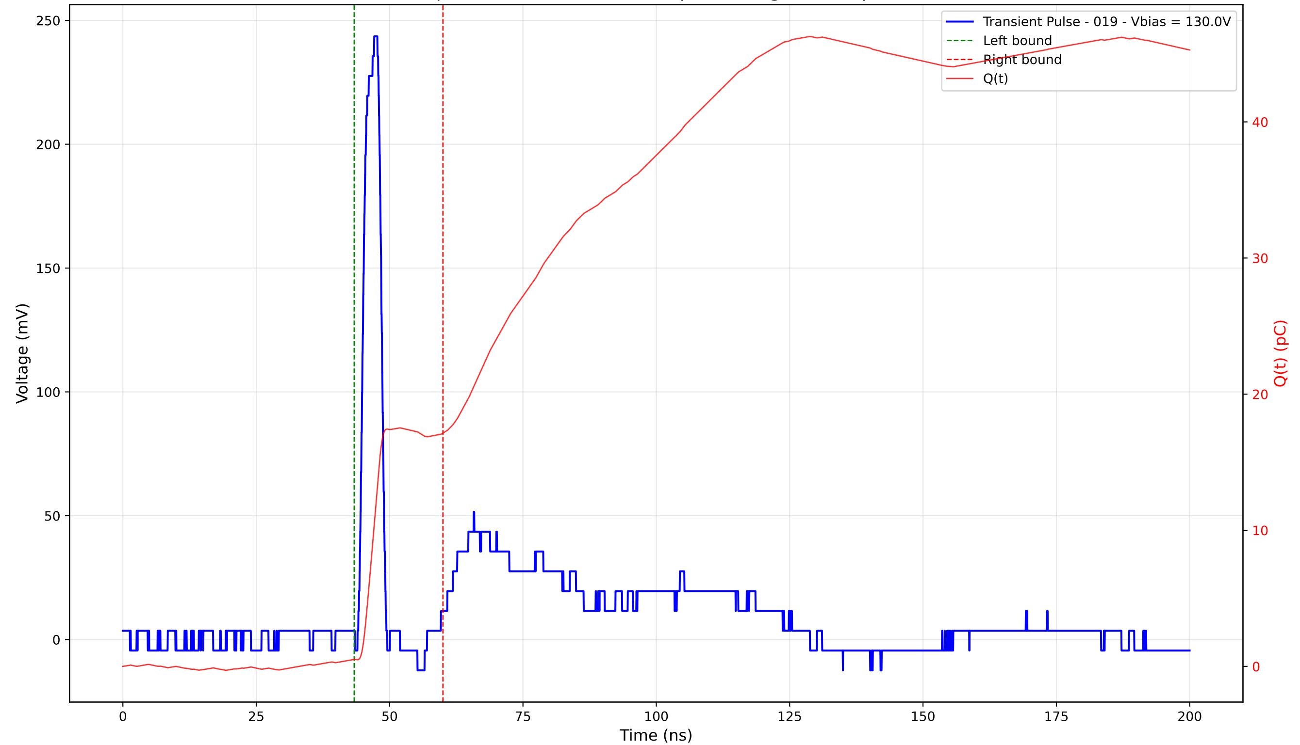
Transient Pulse - Sample: 4003 - Position: 255.0 \mu\text{m} - Charge: 16.62 pC - Rise Time: 1.45 ns
