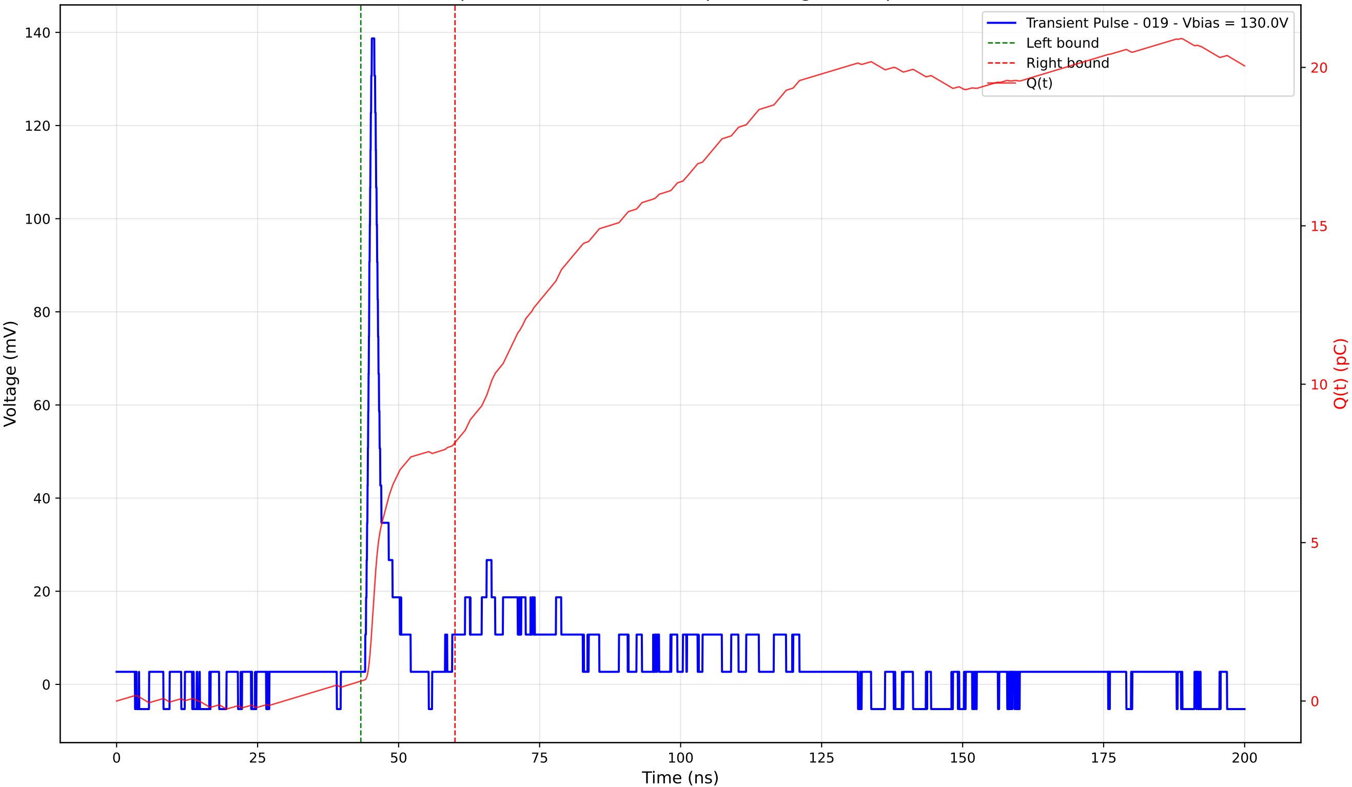
Transient Pulse - Sample: 4003 - Position: 95.0 \mu\text{m} - Charge: 7.53 pC - Rise Time: 0.93 ns
