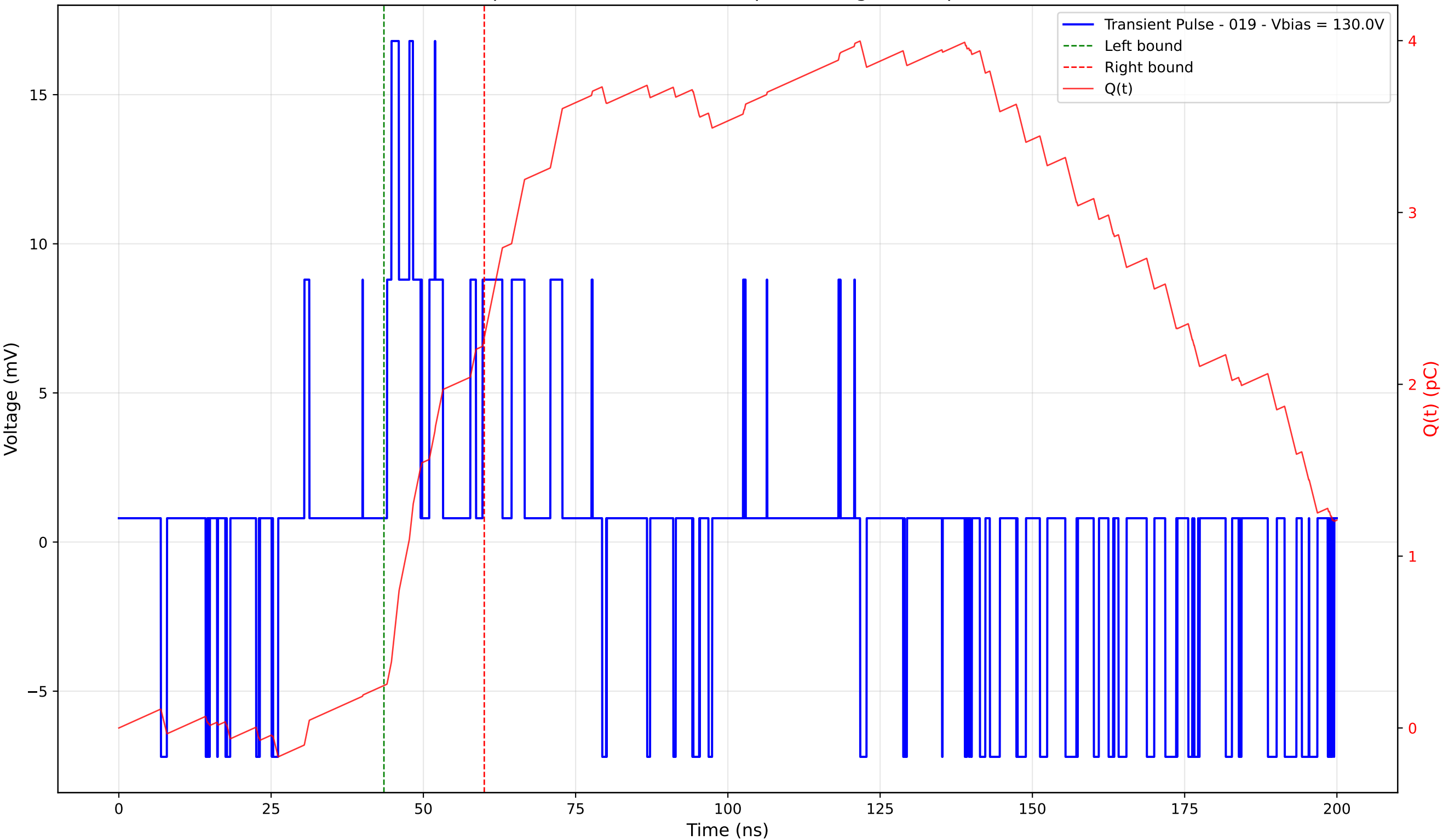
Transient Pulse - Sample: 4003 - Position: 70.0 \mu\text{m} - Charge: 2.02 pC - Rise Time: 0.74 ns
