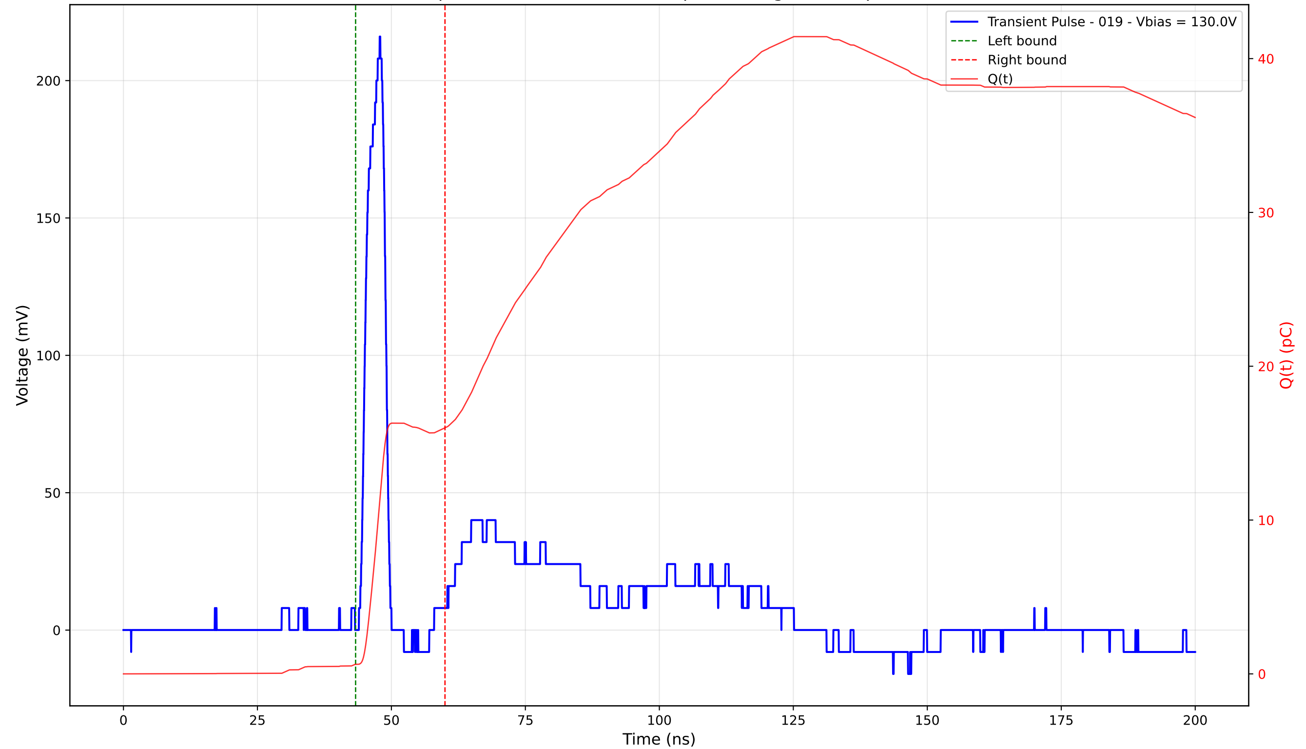
Transient Pulse - Sample: 4003 - Position: 265.0 \mu\text{m} - Charge: 15.37 pC - Rise Time: 2.85 ns
