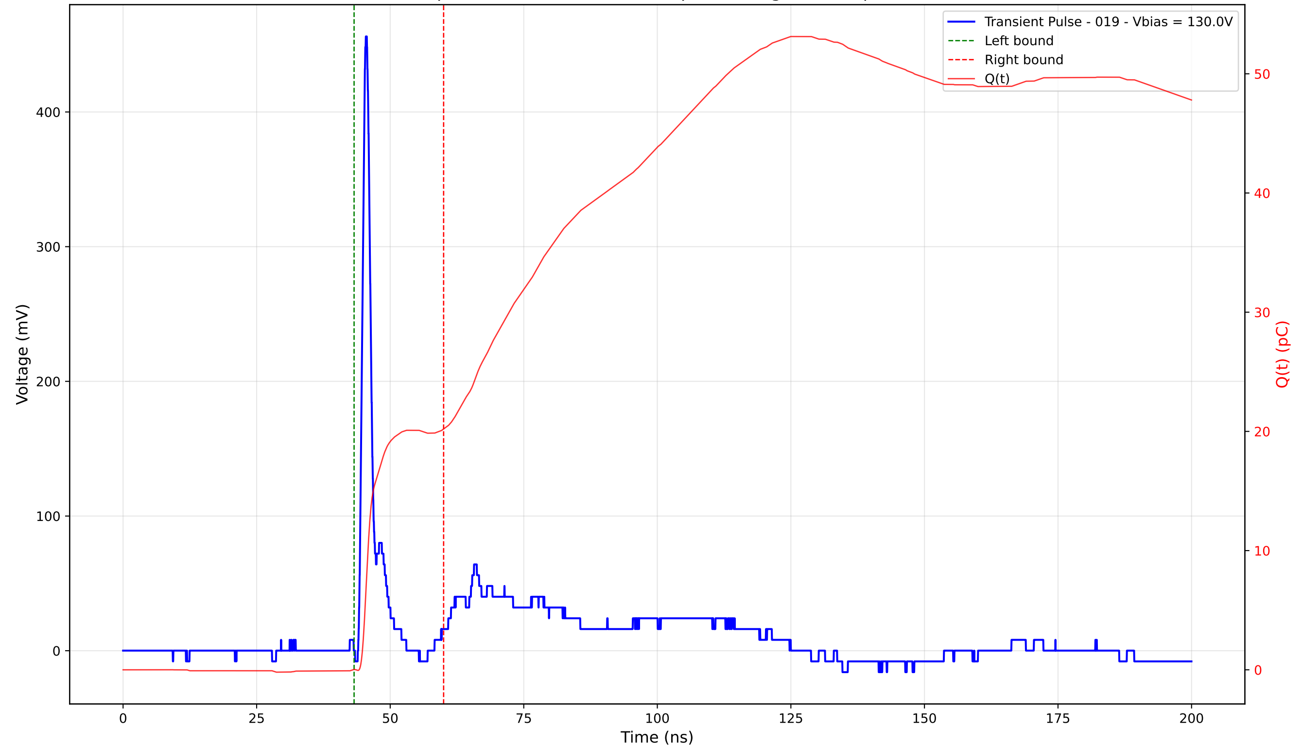
Transient Pulse - Sample: 4003 - Position: 145.0 \mu\text{m} - Charge: 20.17 pC - Rise Time: 0.95 ns
