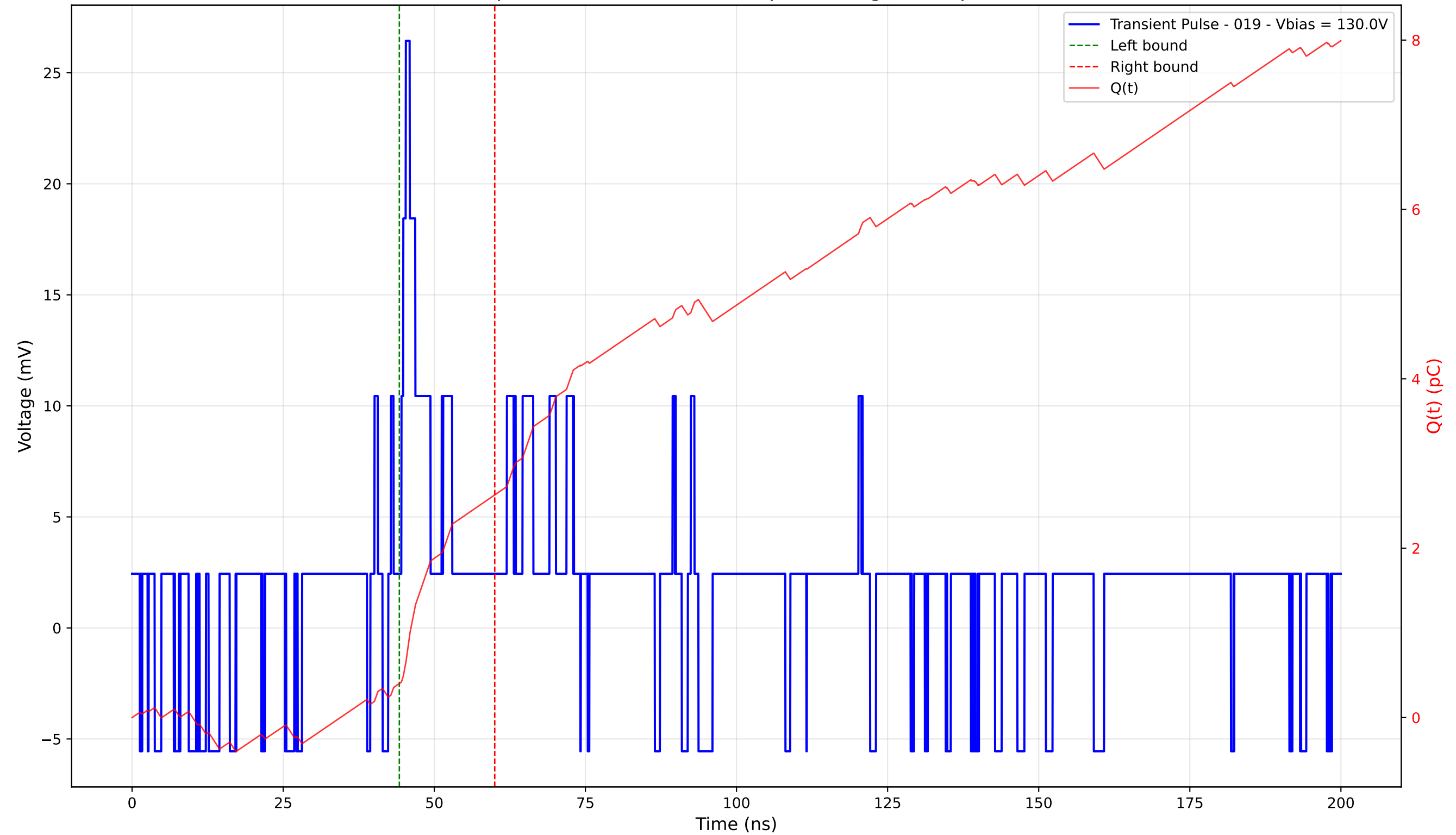
Transient Pulse - Sample: 4003 - Position: 415.0 \mu\text{m} - Charge: 2.23 pC - Rise Time: 0.74 ns
