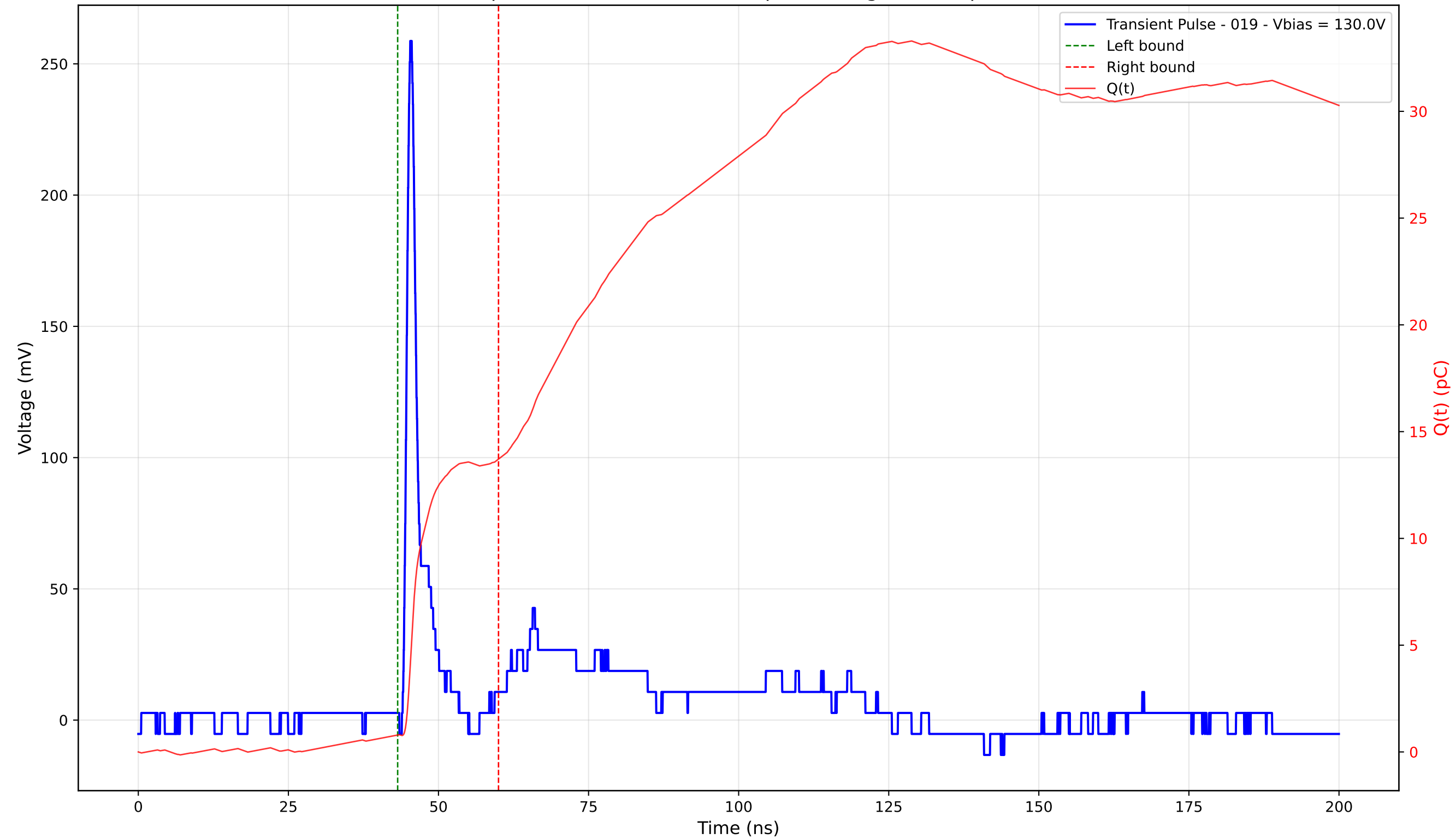
Transient Pulse - Sample: 4003 - Position: 105.0 \mu\text{m} - Charge: 12.92 pC - Rise Time: 0.90 ns
