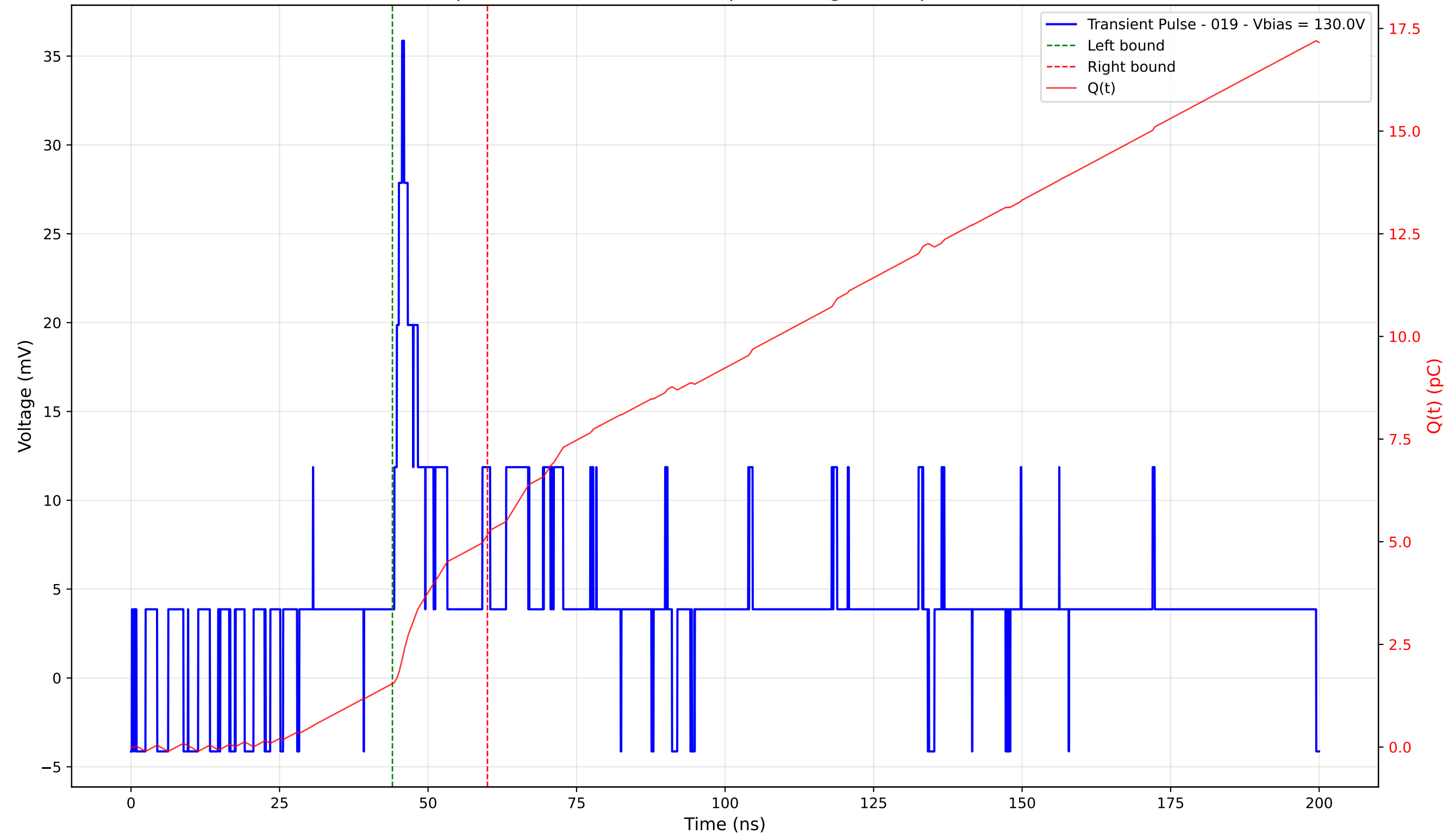
Transient Pulse - Sample: 4003 - Position: 335.0 \mu\text{m} - Charge: 3.63 pC - Rise Time: 0.00 ns (N/A)
