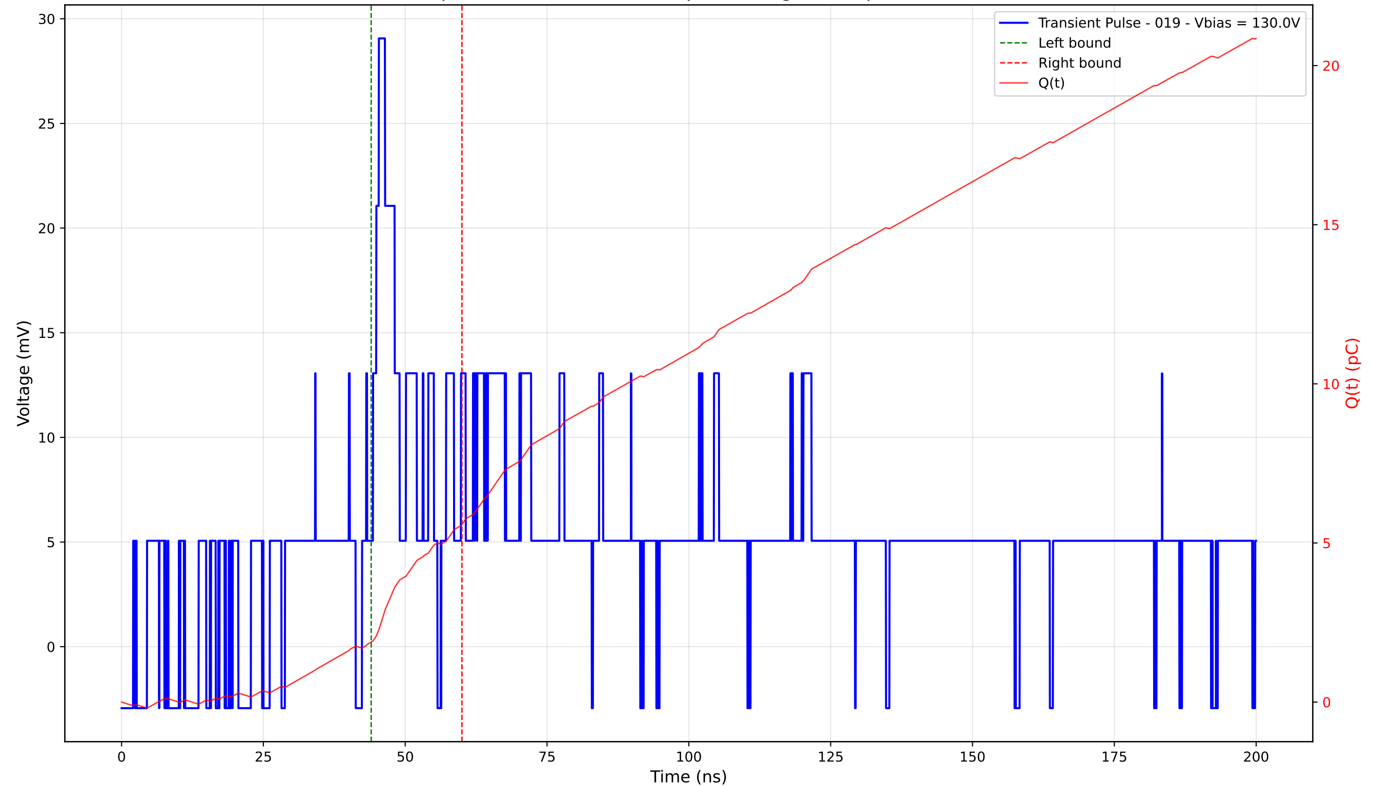
Transient Pulse - Sample: 4003 - Position: 40.0 \mu\text{m} - Charge: 3.70 pC - Rise Time: 0.00 ns (N/A)
