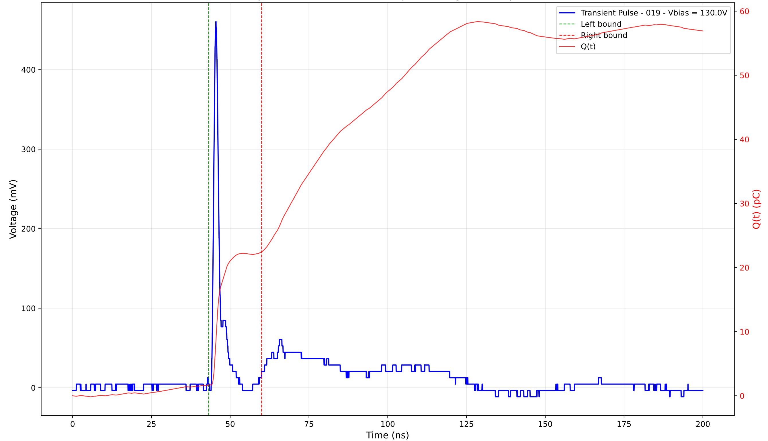
Transient Pulse - Sample: 4003 - Position: 140.0 \mu\text{m} - Charge: 20.76 pC - Rise Time: 0.94 ns
