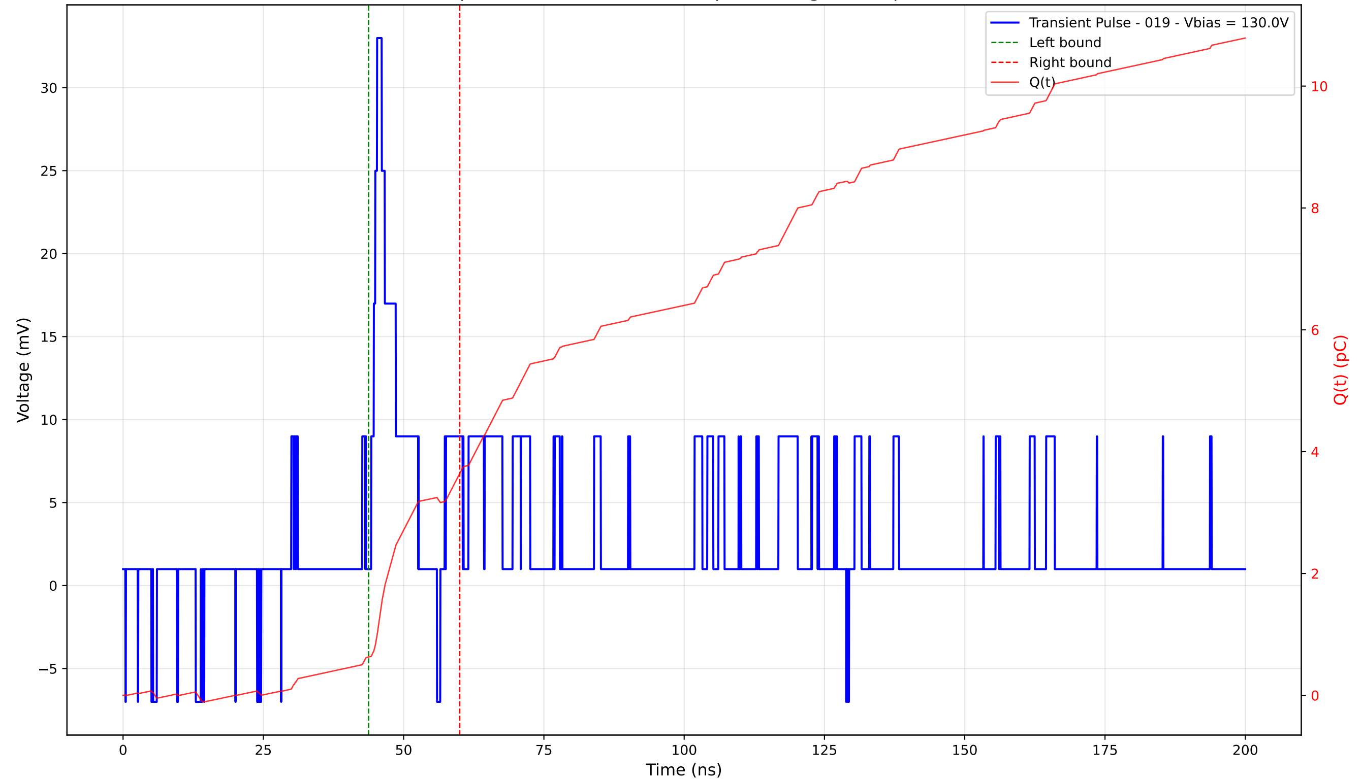
Transient Pulse - Sample: 4003 - Position: 330.0 \mu\text{m} - Charge: 3.01 pC - Rise Time: 1.05 ns
