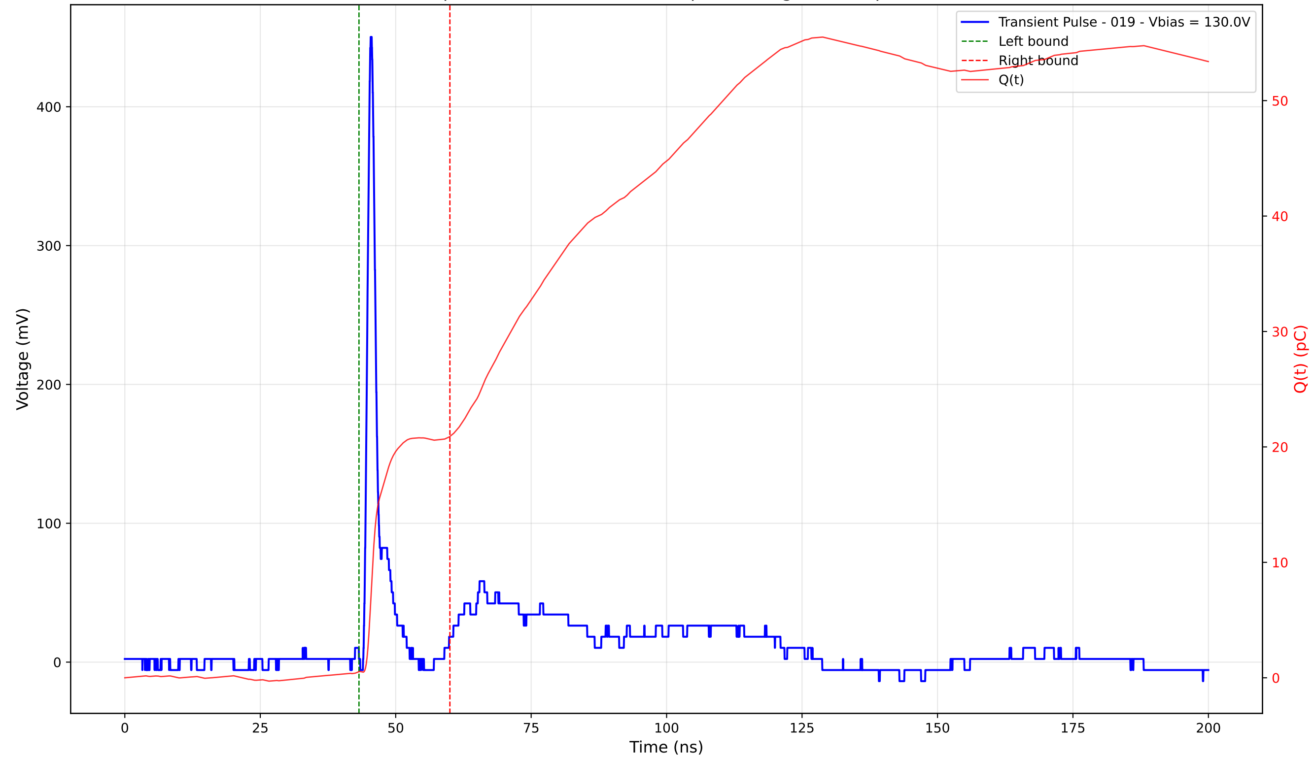
Transient Pulse - Sample: 4003 - Position: 135.0 \mu\text{m} - Charge: 20.37 pC - Rise Time: 0.91 ns
