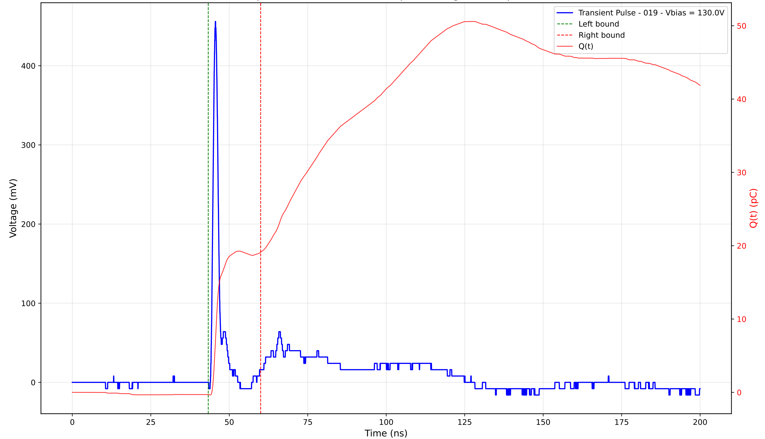
Transient Pulse - Sample: 4003 - Position: 165.0 \mu\text{m} - Charge: 19.40 pC - Rise Time: 1.05 ns
