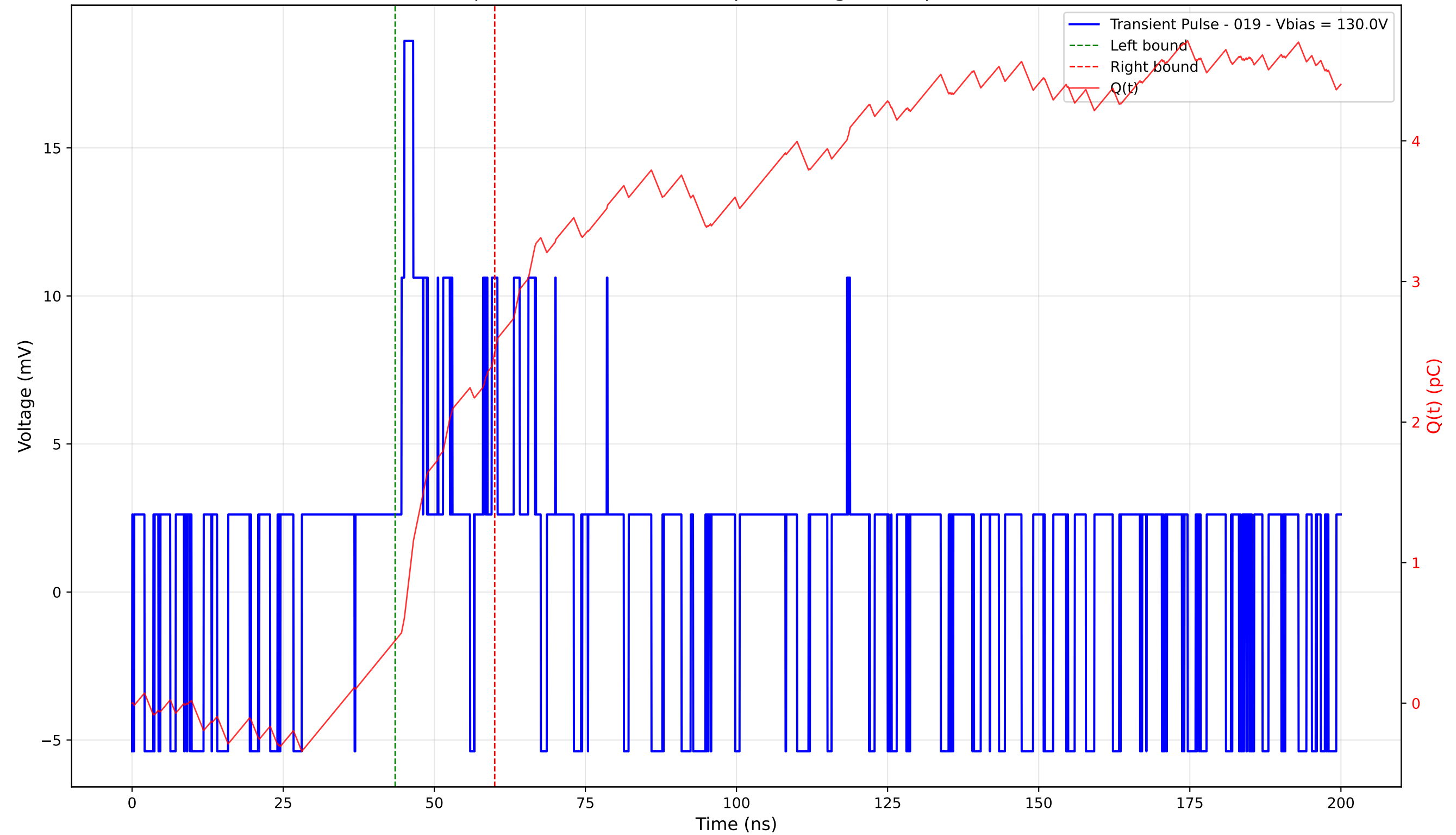
Transient Pulse - Sample: 4003 - Position: 15.0 \mu\text{m} - Charge: 2.05 pC - Rise Time: 0.00 ns (N/A)
