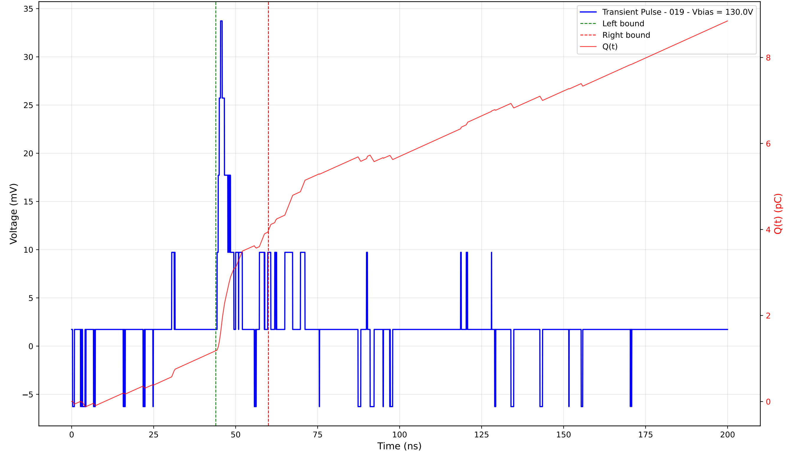
Transient Pulse - Sample: 4003 - Position: 350.0 \mu\text{m} - Charge: 2.80 pC - Rise Time: 1.08 ns
