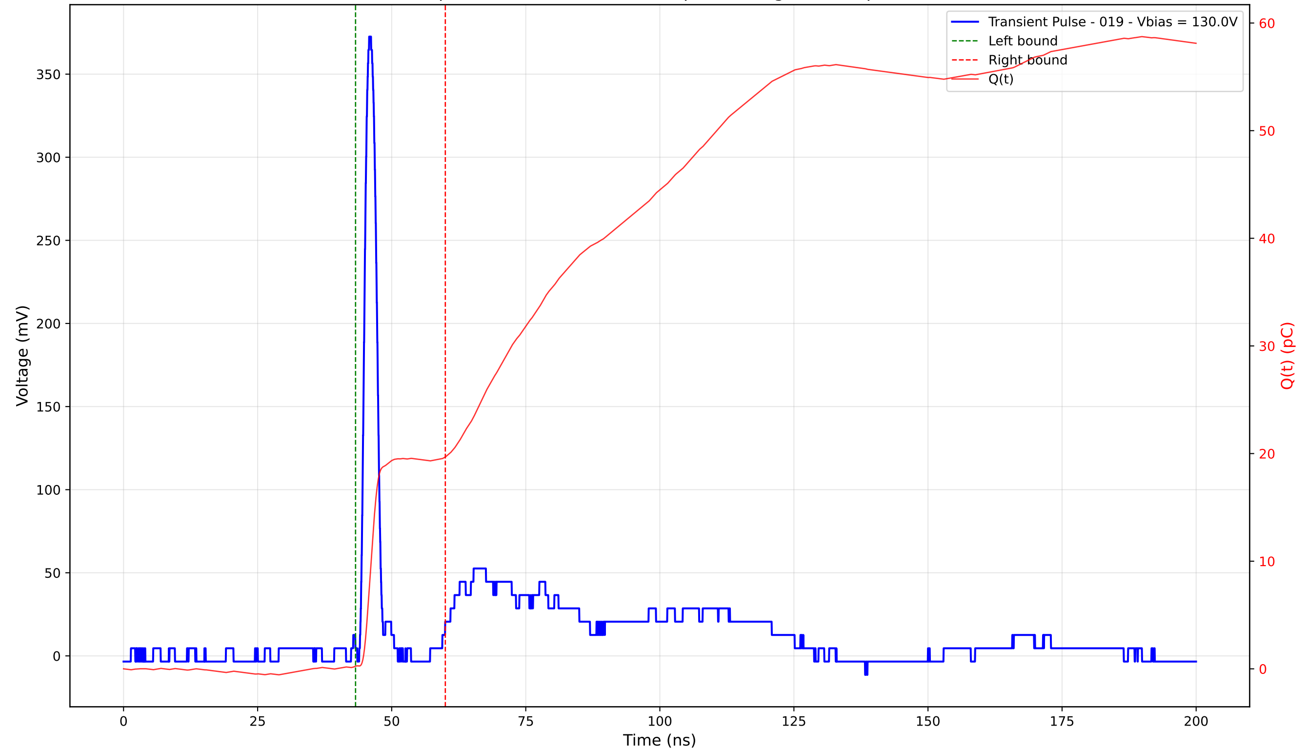
Transient Pulse - Sample: 4003 - Position: 215.0 \mu\text{m} - Charge: 19.42 pC - Rise Time: 1.14 ns
