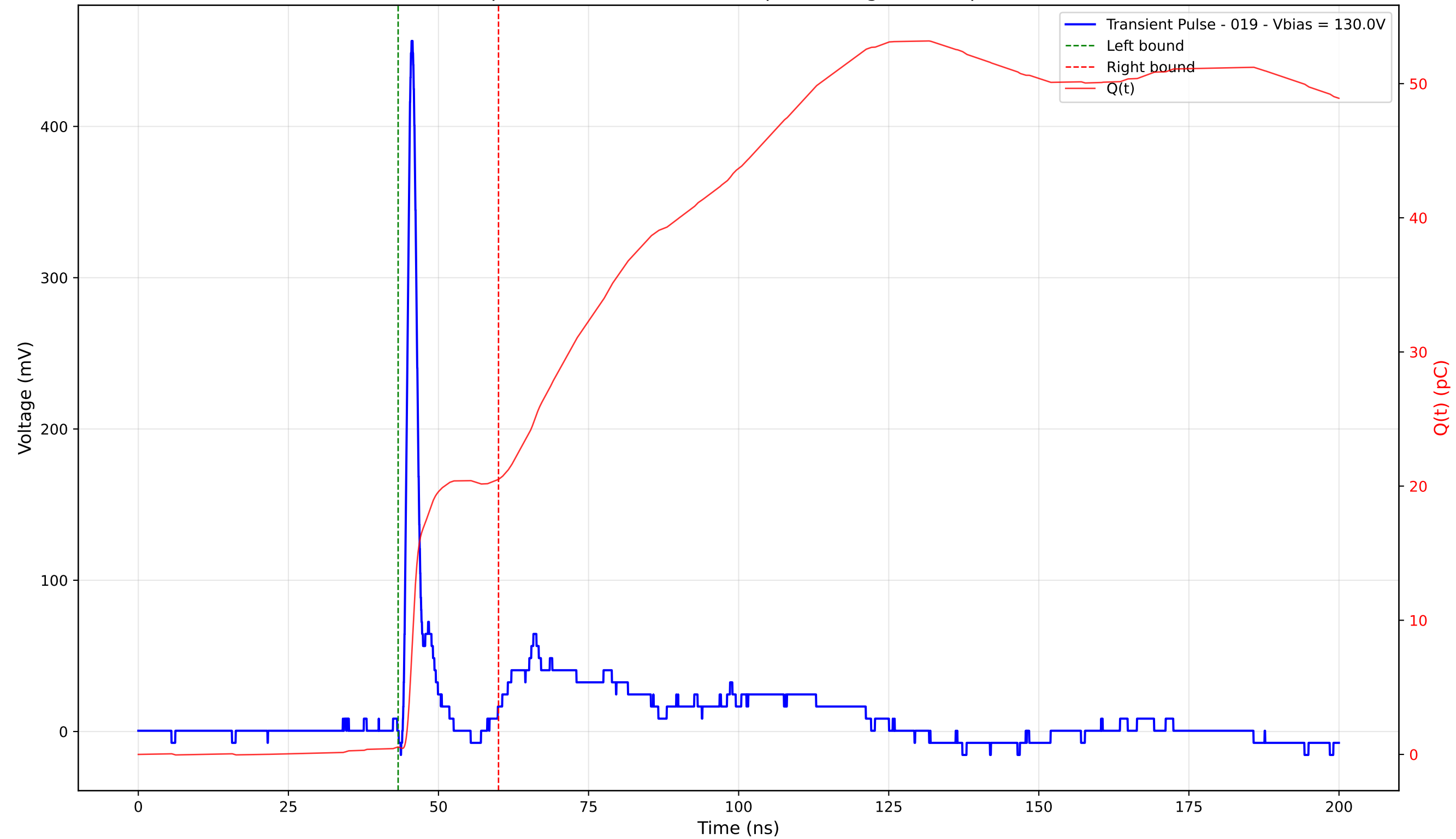
Transient Pulse - Sample: 4003 - Position: 160.0 \mu\text{m} - Charge: 19.95 pC - Rise Time: 0.99 ns
