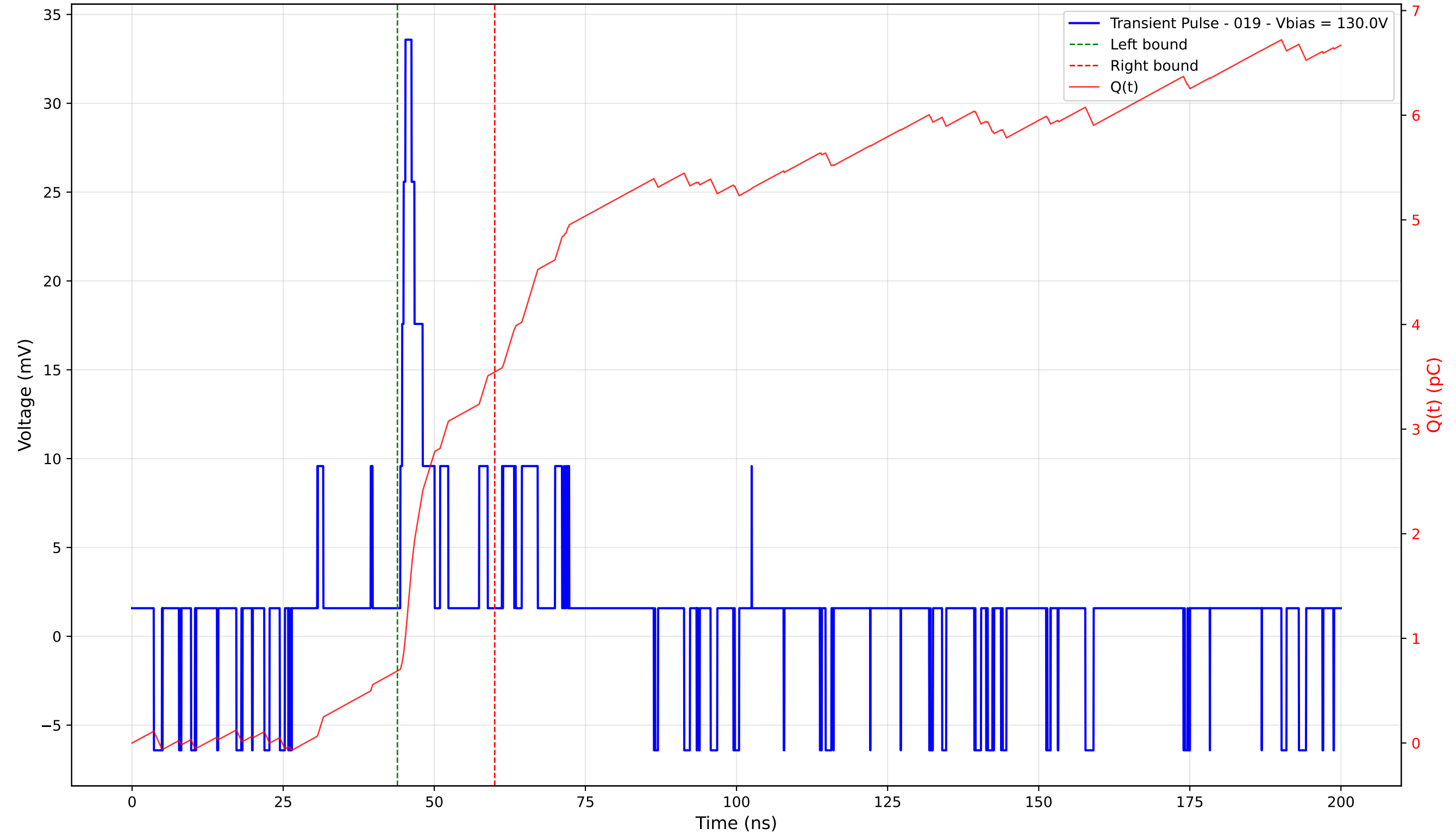
Transient Pulse - Sample: 4003 - Position: 360.0 \mu\text{m} - Charge: 2.86 pC - Rise Time: 0.86 ns
