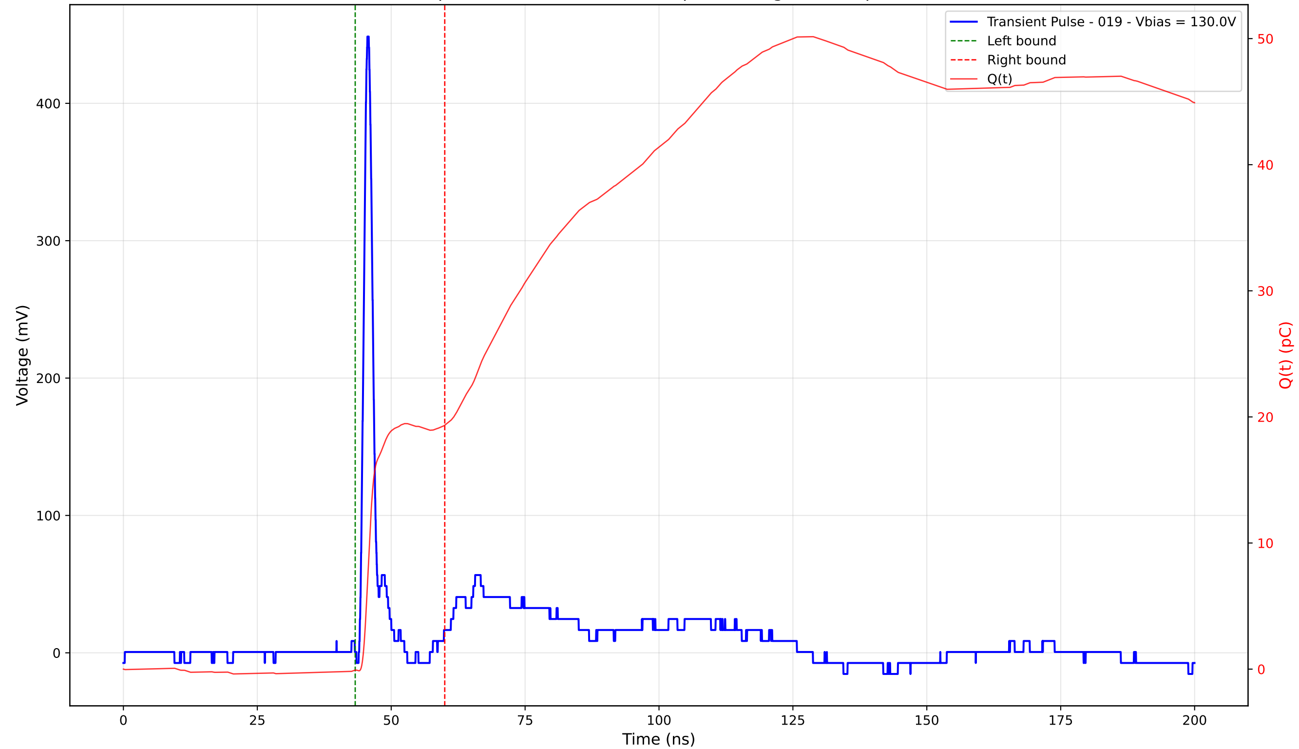
Transient Pulse - Sample: 4003 - Position: 175.0 \mu\text{m} - Charge: 19.42 pC - Rise Time: 1.02 ns
