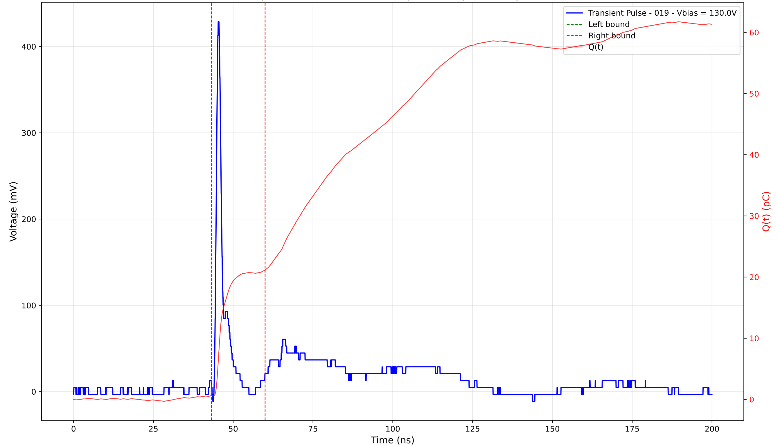
Transient Pulse - Sample: 4003 - Position: 125.0 \mu\text{m} - Charge: 20.47 pC - Rise Time: 0.90 ns
