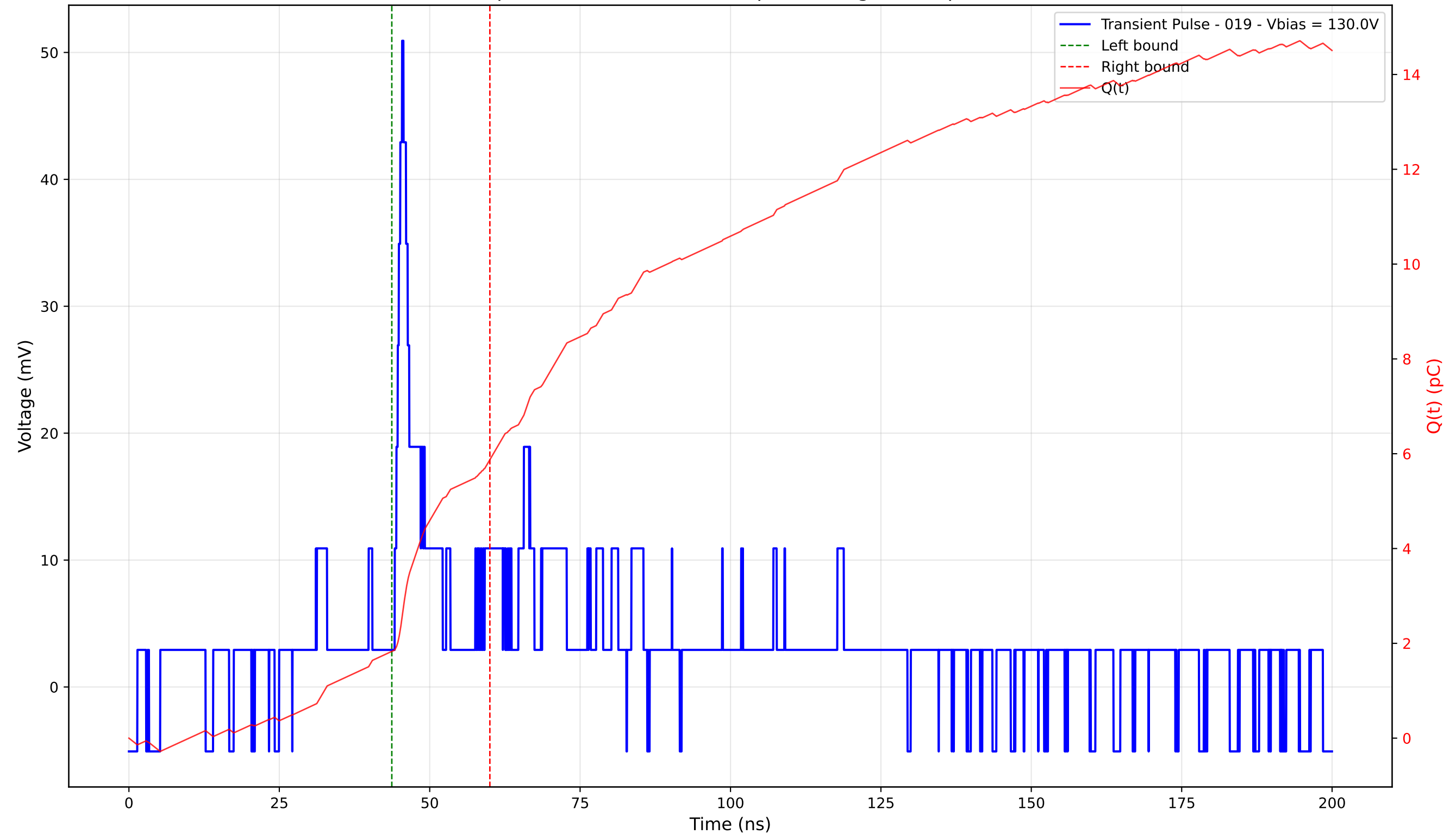
Transient Pulse - Sample: 4003 - Position: 85.0 \mu\text{m} - Charge: 4.05 pC - Rise Time: 1.23 ns
