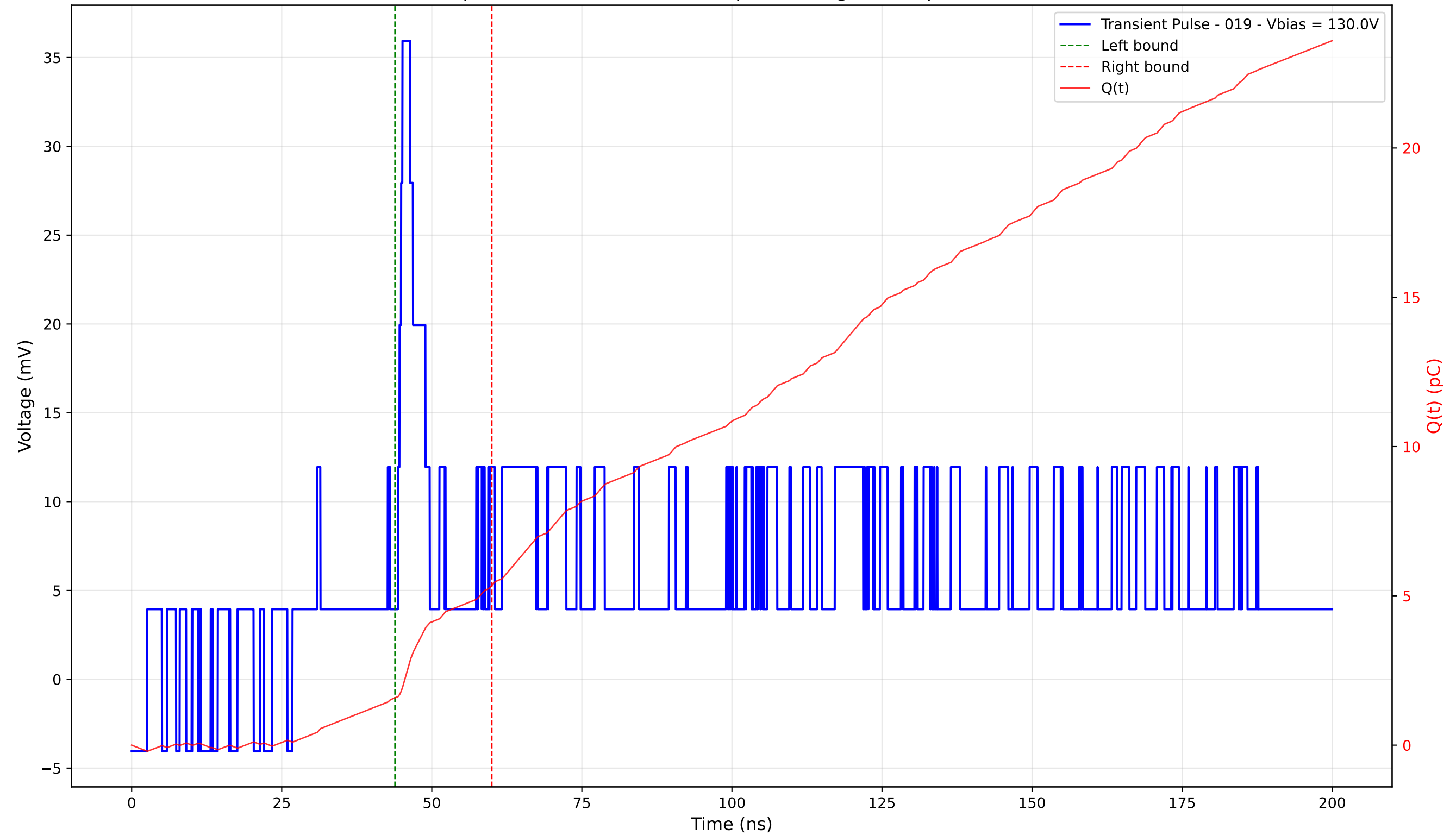
Transient Pulse - Sample: 4003 - Position: 320.0 \mu\text{m} - Charge: 3.77 pC - Rise Time: 0.00 ns (N/A)
