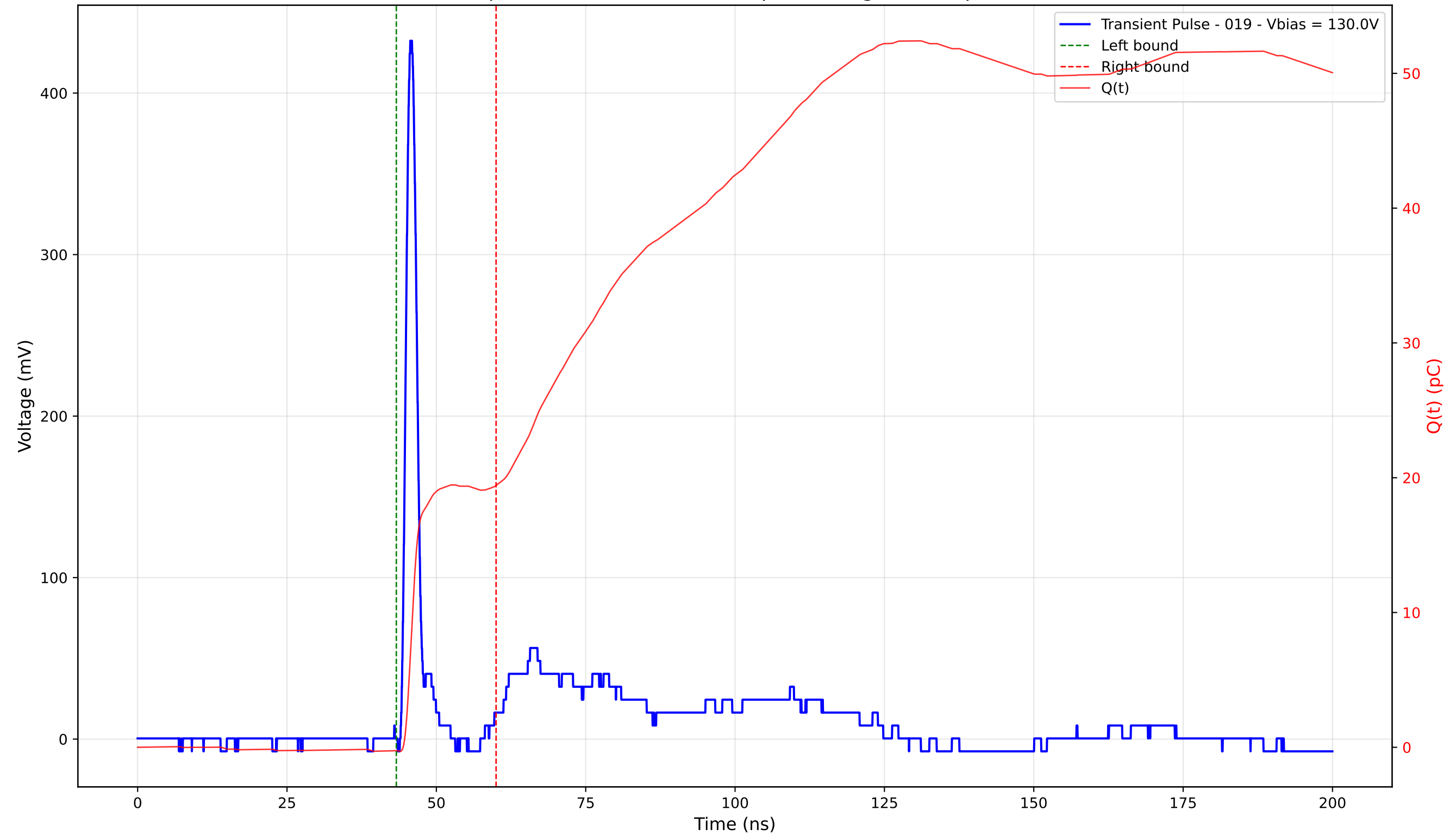
Transient Pulse - Sample: 4003 - Position: 190.0 \mu\text{m} - Charge: 19.68 pC - Rise Time: 1.07 ns
