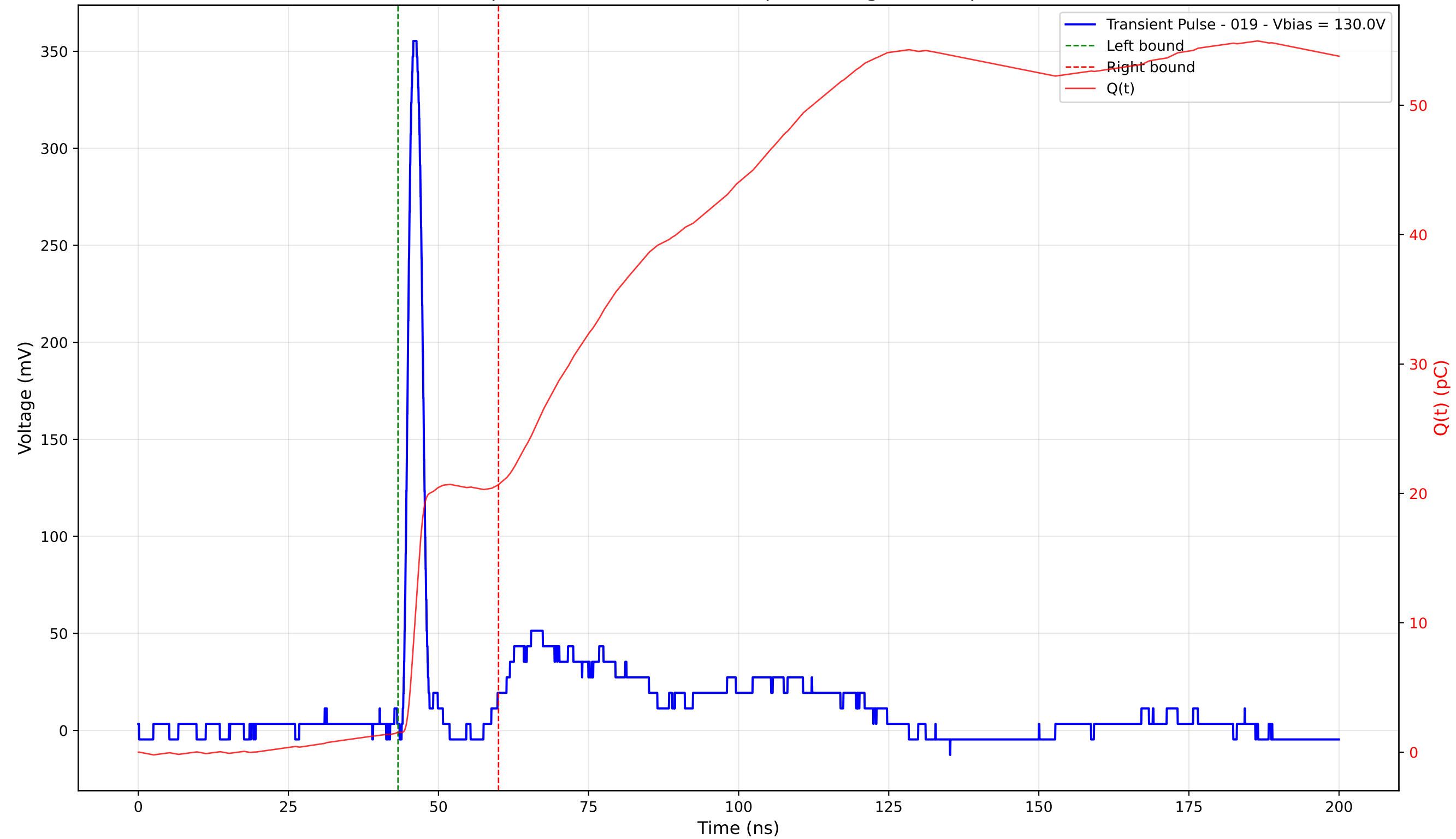
Transient Pulse - Sample: 4003 - Position: 220.0 \mu\text{m} - Charge: 19.15 pC - Rise Time: 1.16 ns
