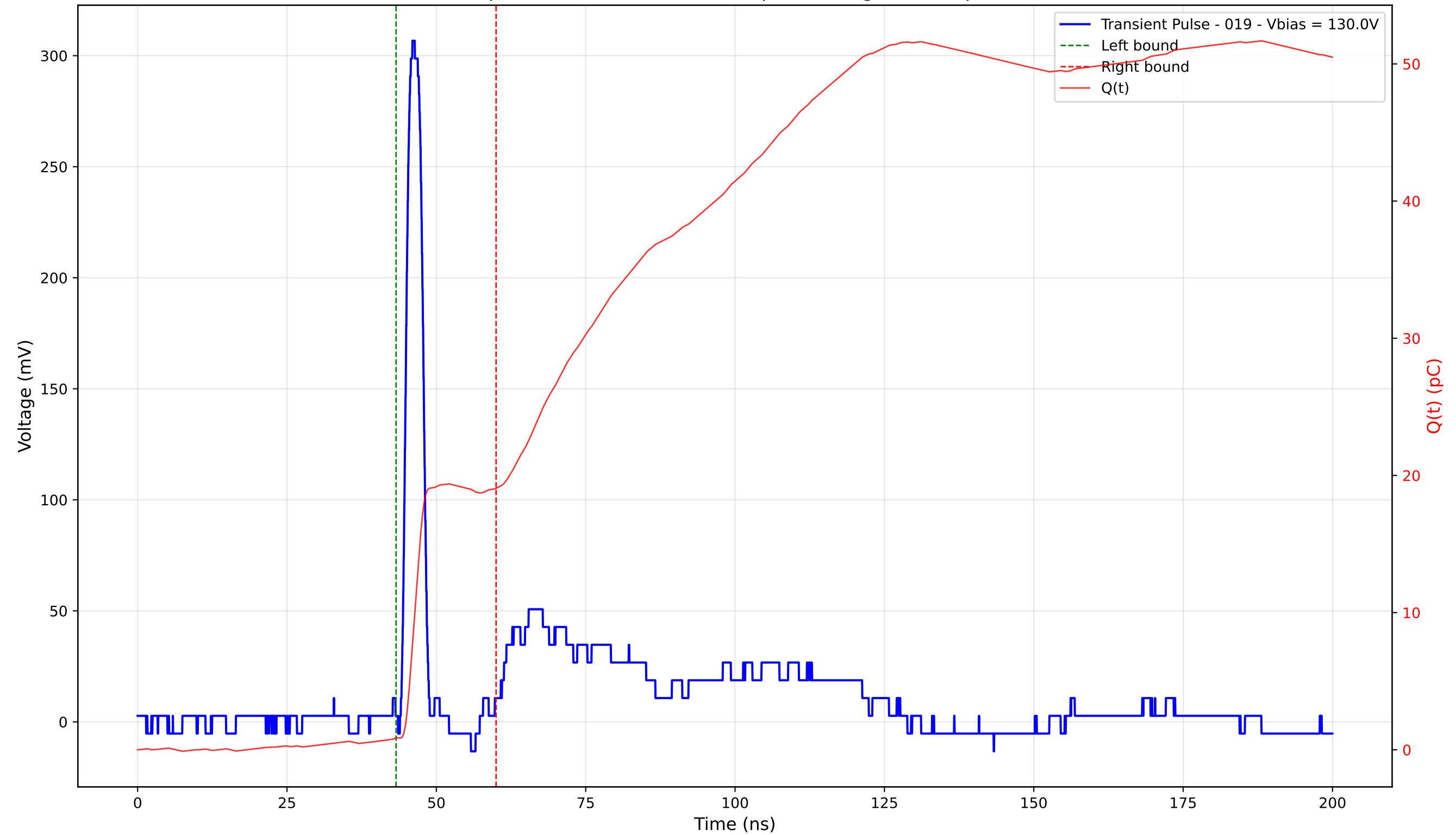
Transient Pulse - Sample: 4003 - Position: 235.0 \mu\text{m} - Charge: 18.19 pC - Rise Time: 1.23 ns
