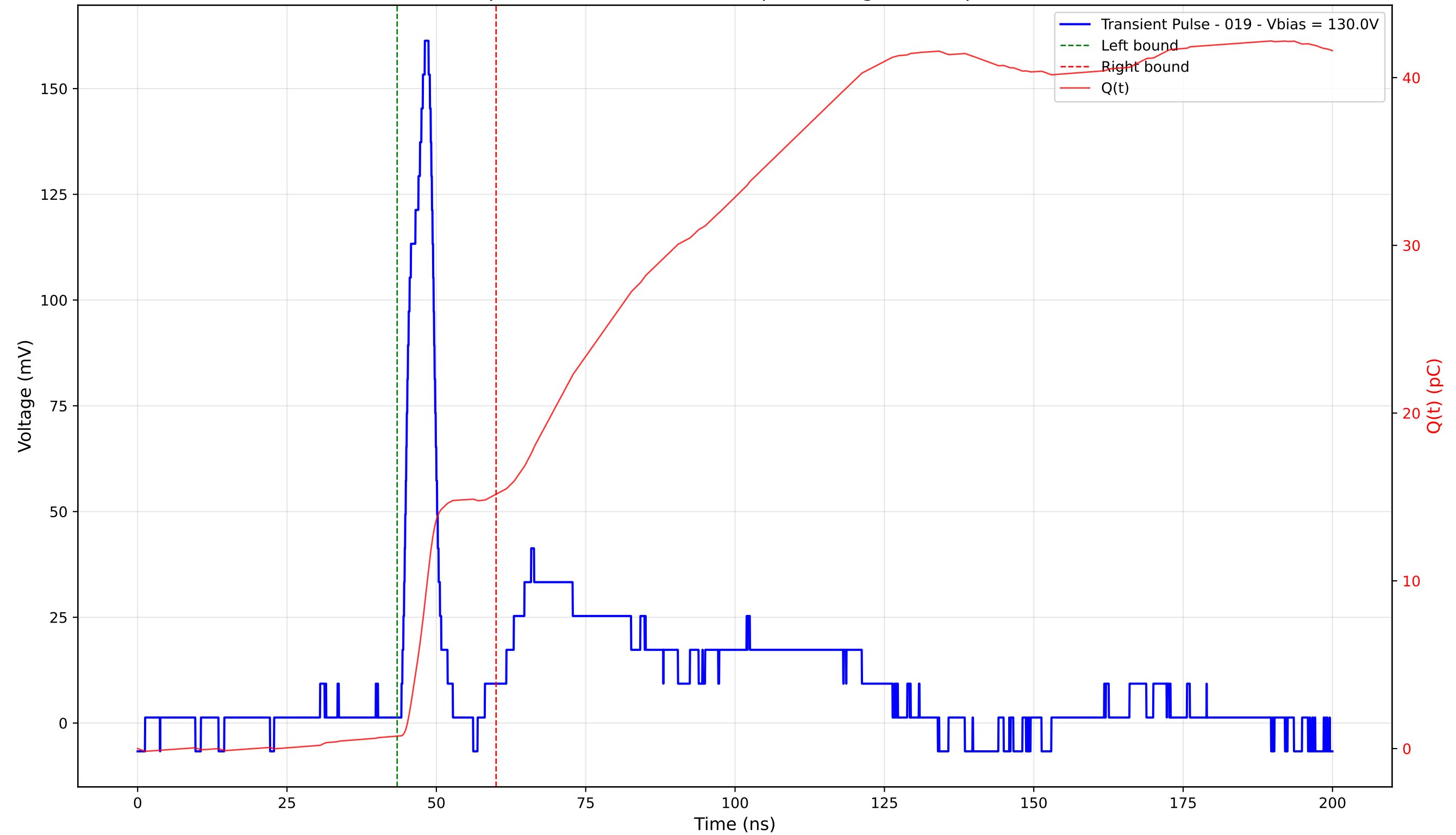
Transient Pulse - Sample: 4003 - Position: 275.0 \mu\text{m} - Charge: 14.43 pC - Rise Time: 3.18 ns
