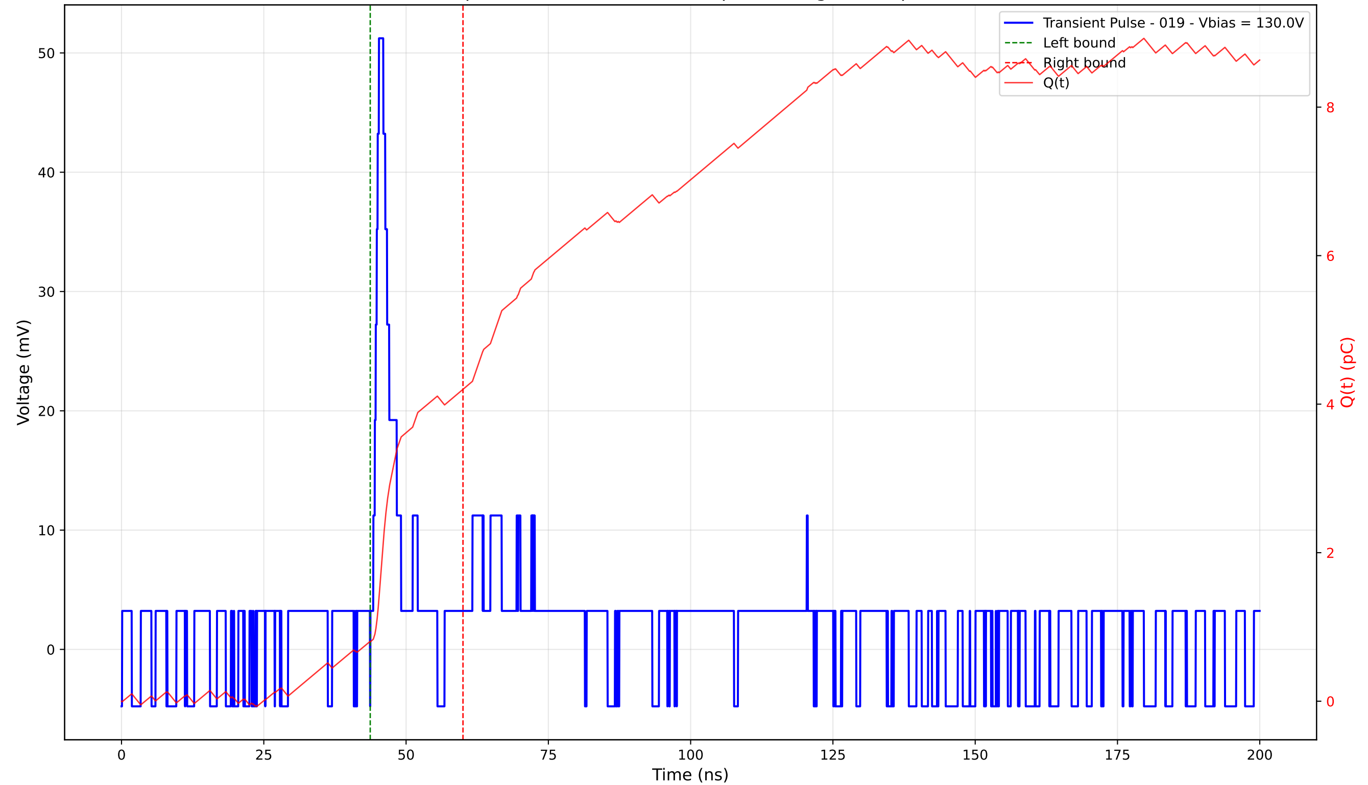
Transient Pulse - Sample: 4003 - Position: 390.0 \mu\text{m} - Charge: 3.40 pC - Rise Time: 1.00 ns
