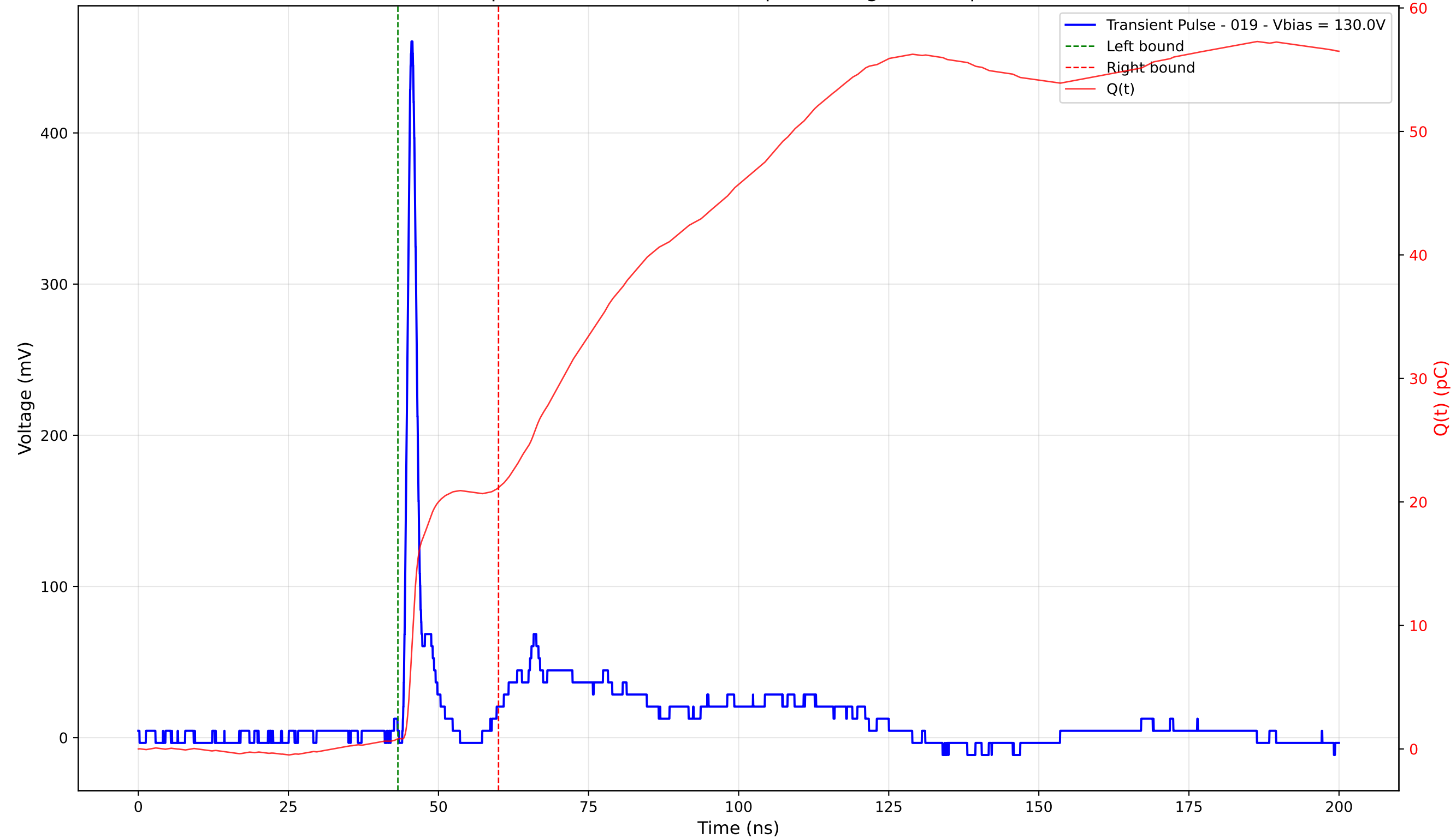
Transient Pulse - Sample: 4003 - Position: 155.0 \mu\text{m} - Charge: 20.34 pC - Rise Time: 0.98 ns
