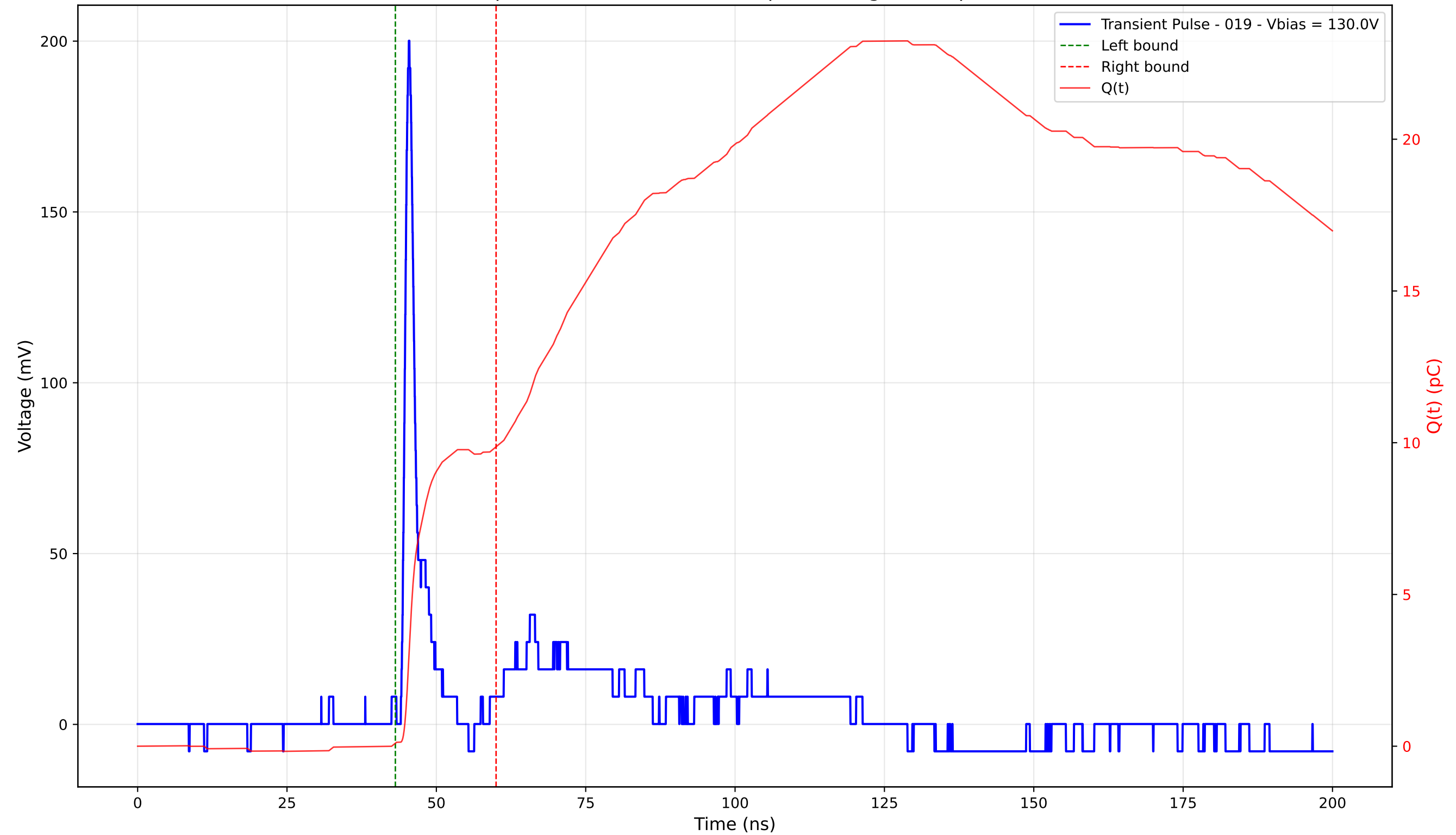
Transient Pulse - Sample: 4003 - Position: 100.0 \mu\text{m} - Charge: 9.76 pC - Rise Time: 0.93 ns
