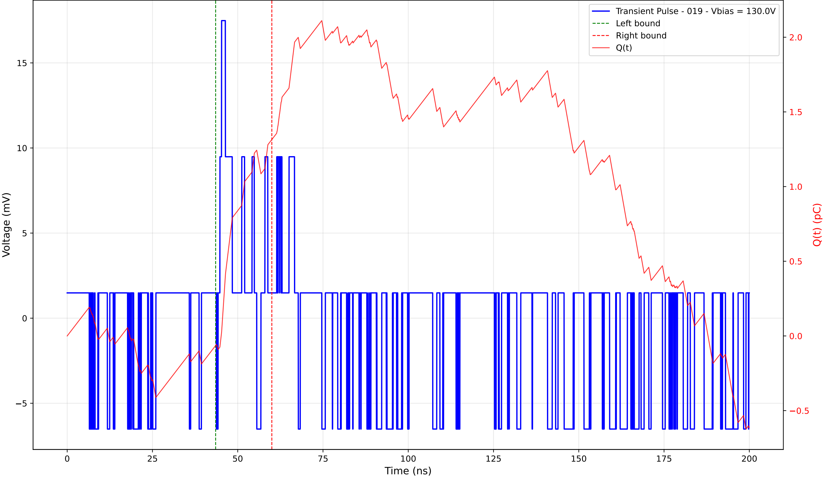
Transient Pulse - Sample: 4003 - Position: 10.0 \mu\text{m} - Charge: 1.38 pC - Rise Time: 0.50 ns
