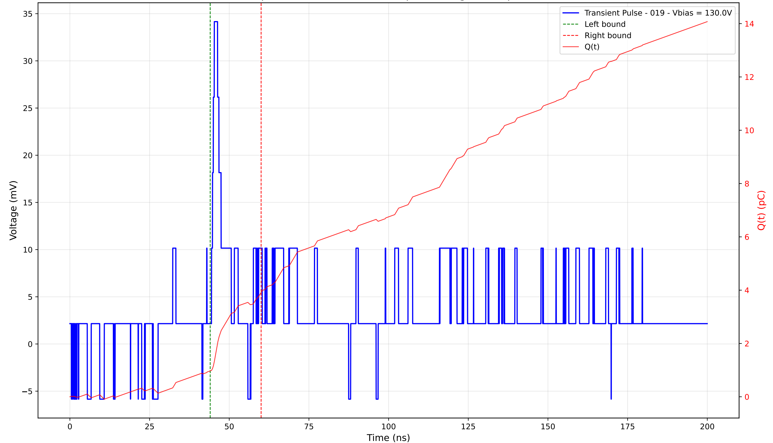
Transient Pulse - Sample: 4003 - Position: 325.0 \mu\text{m} - Charge: 2.95 pC - Rise Time: 0.88 ns
