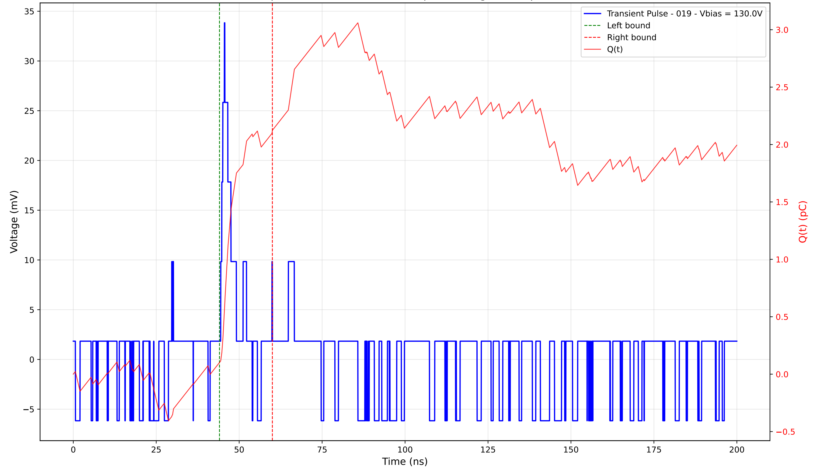
Transient Pulse - Sample: 4003 - Position: 355.0 \mu\text{m} - Charge: 2.02 pC - Rise Time: 1.12 ns
