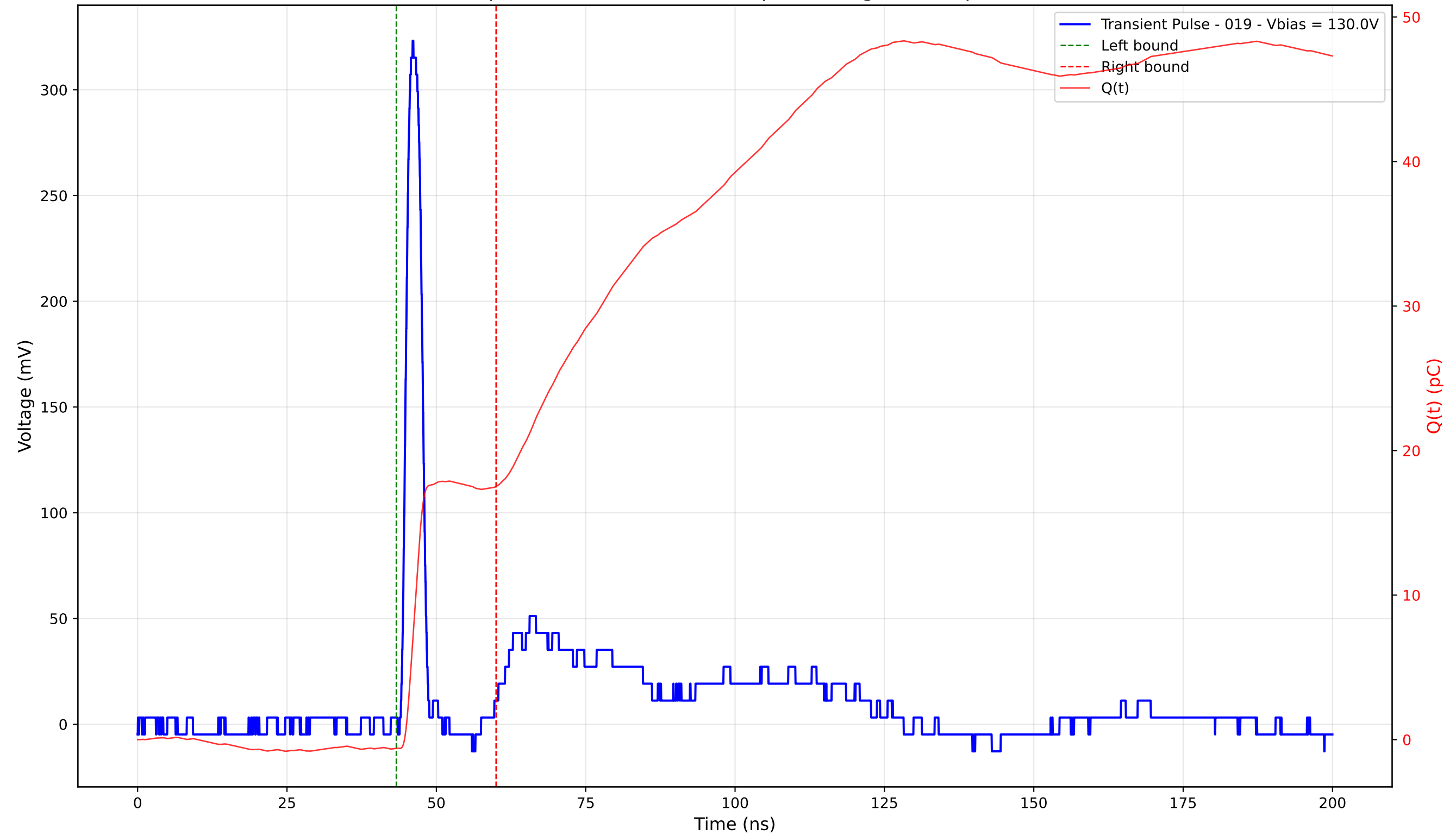
Transient Pulse - Sample: 4003 - Position: 230.0 \mu\text{m} - Charge: 18.11 pC - Rise Time: 1.21 ns
