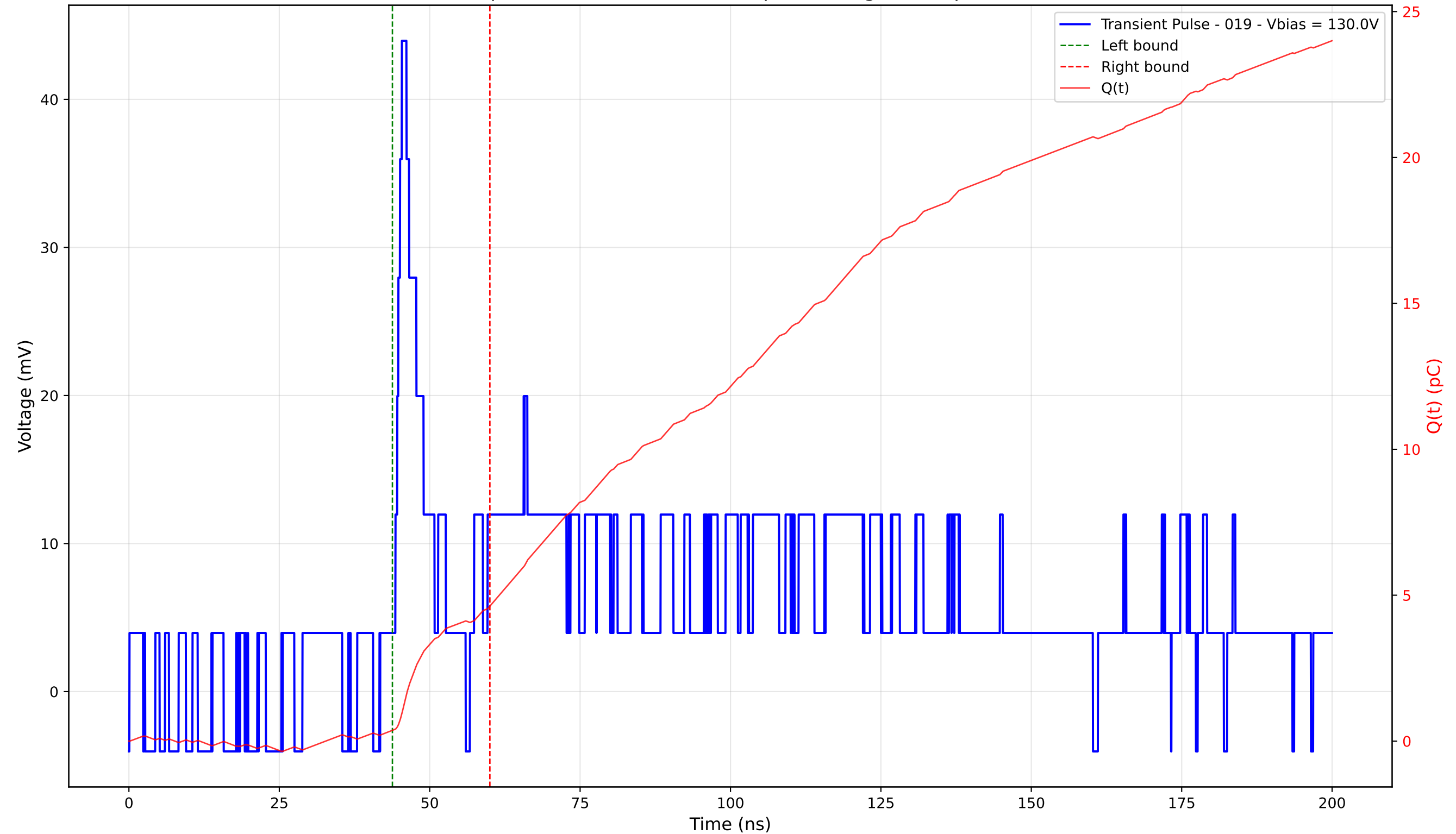
Transient Pulse - Sample: 4003 - Position: 310.0 \mu\text{m} - Charge: 4.26 pC - Rise Time: 1.08 ns
