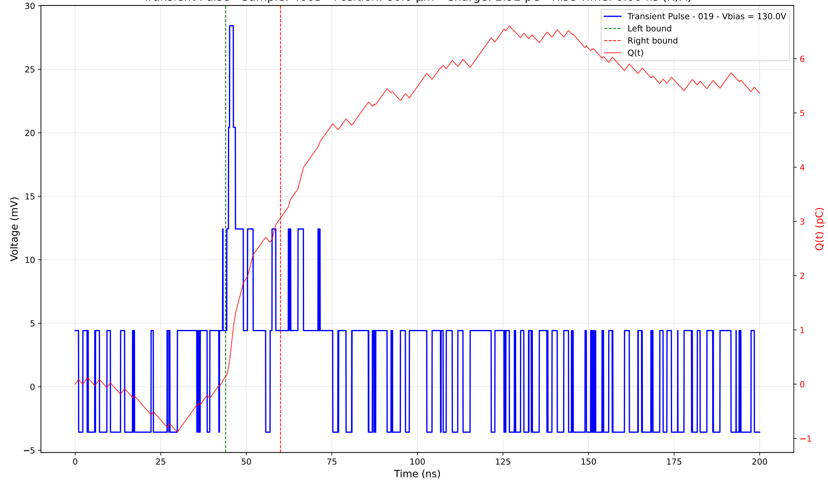
Transient Pulse - Sample: 4003 - Position: 80.0 \mu\text{m} - Charge: 2.92 pC - Rise Time: 0.00 ns (N/A)
