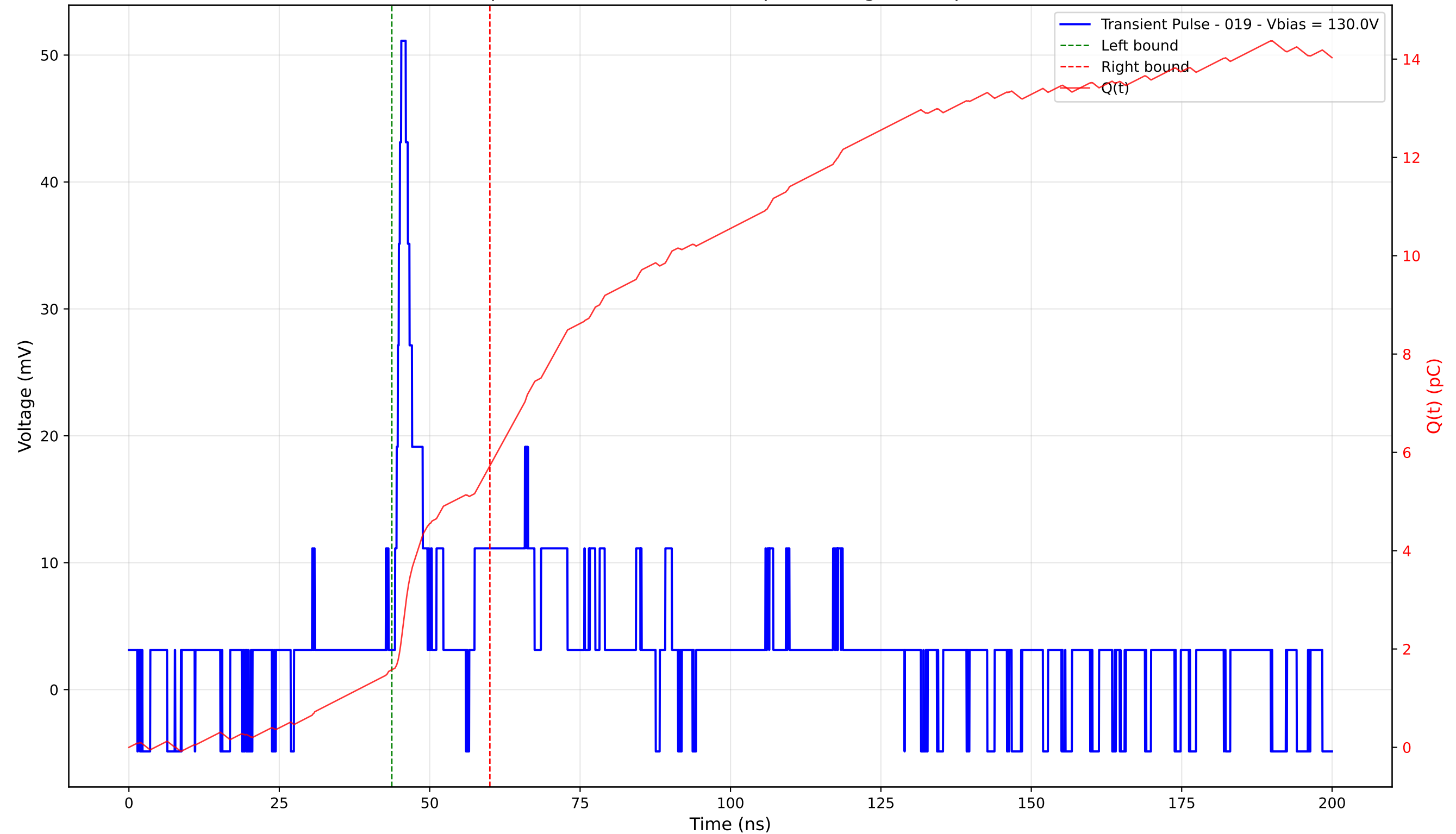
Transient Pulse - Sample: 4003 - Position: 395.0 \mu\text{m} - Charge: 4.15 pC - Rise Time: 1.04 ns
