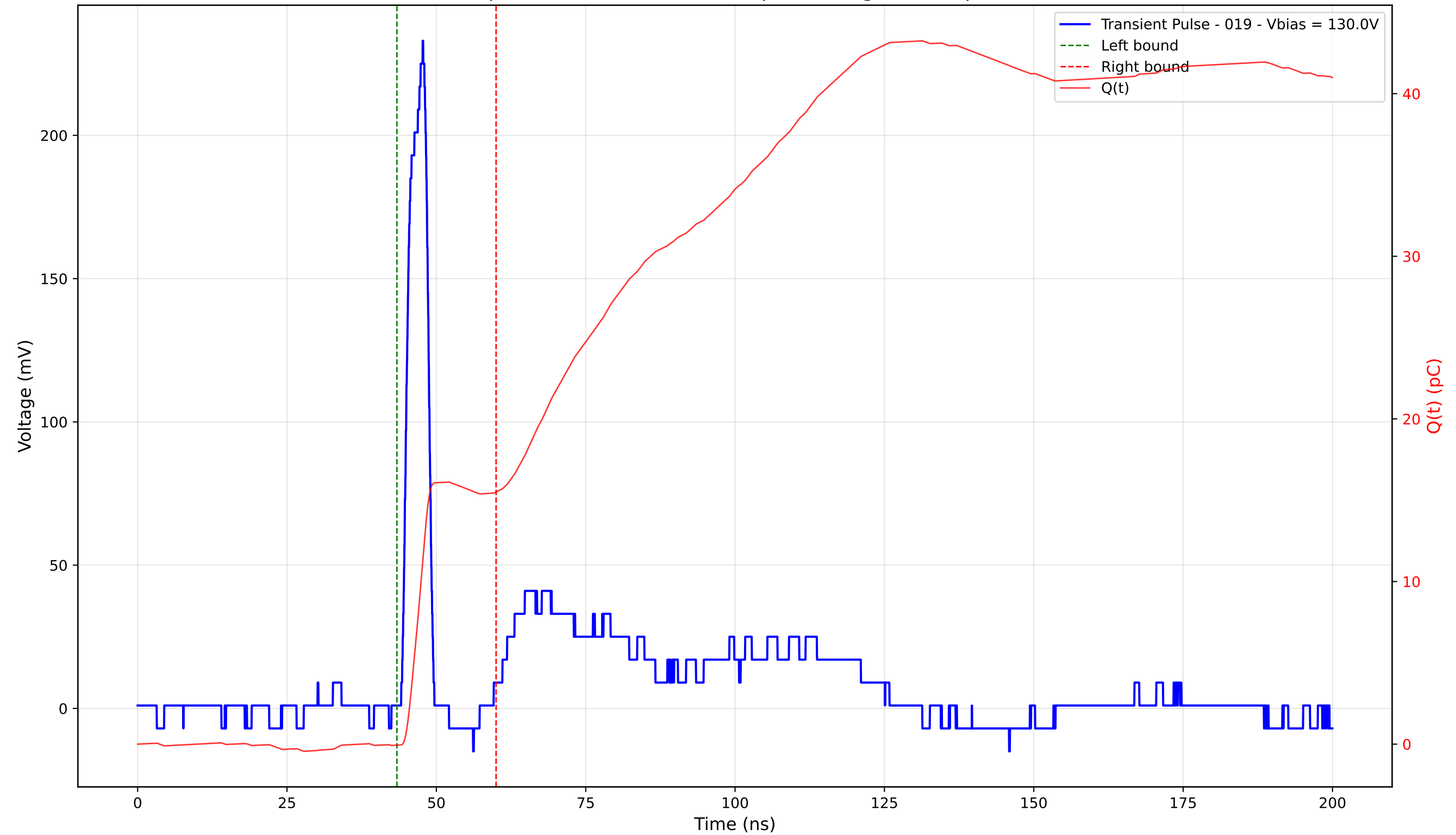
Transient Pulse - Sample: 4003 - Position: 260.0 \mu\text{m} - Charge: 15.57 pC - Rise Time: 2.80 ns
