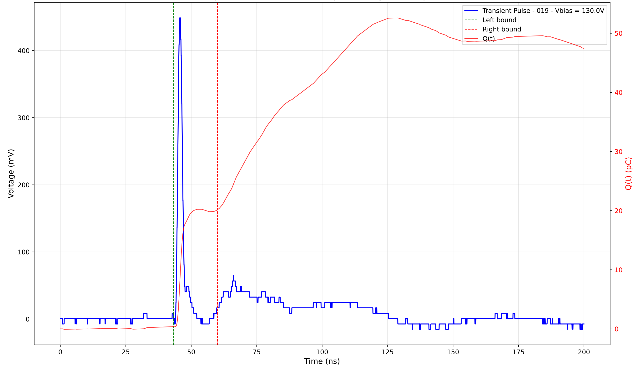
Transient Pulse - Sample: 4003 - Position: 180.0 \mu\text{m} - Charge: 19.68 pC - Rise Time: 1.05 ns
