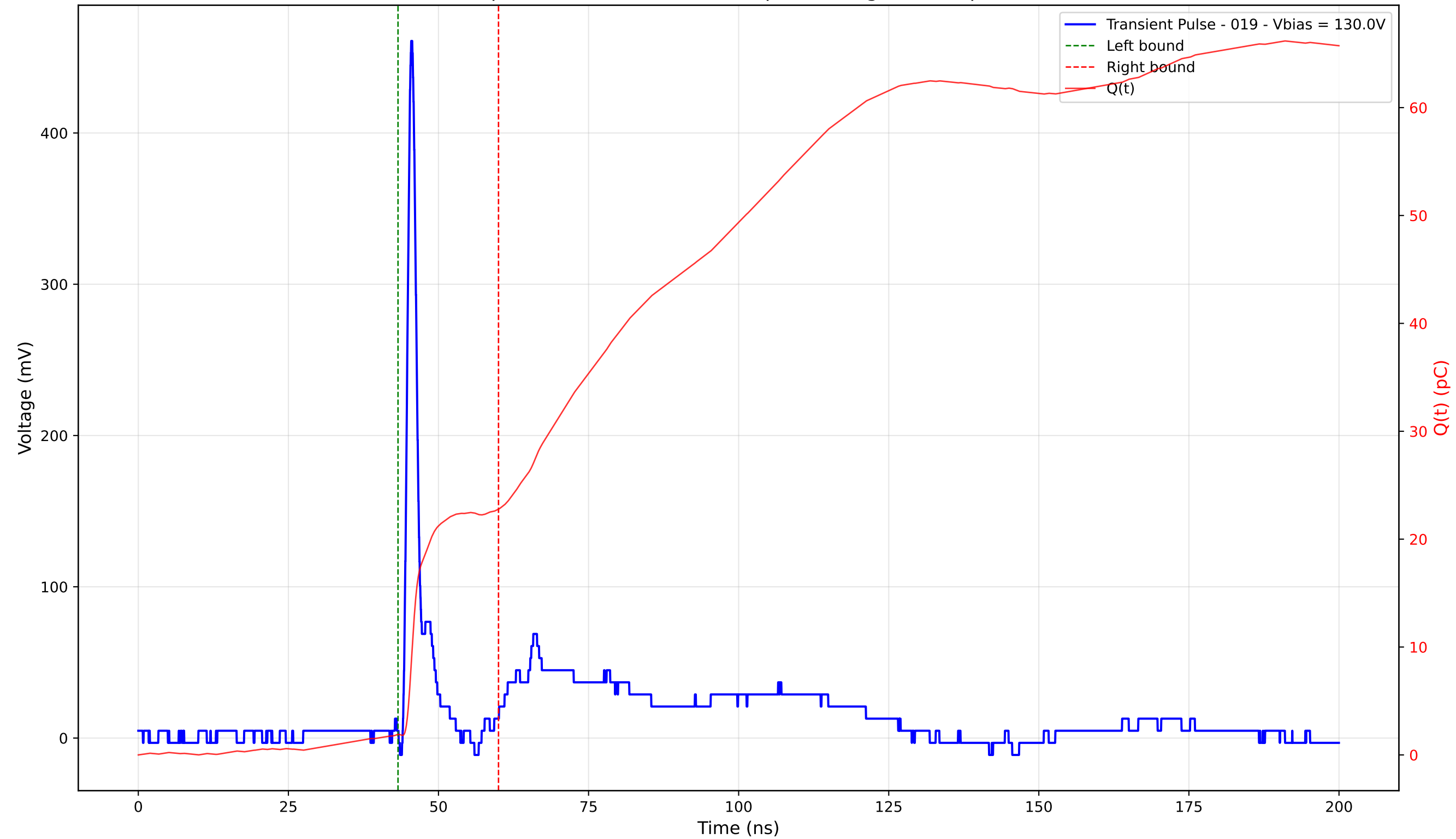
Transient Pulse - Sample: 4003 - Position: 150.0 \mu\text{m} - Charge: 20.87 pC - Rise Time: 0.94 ns
