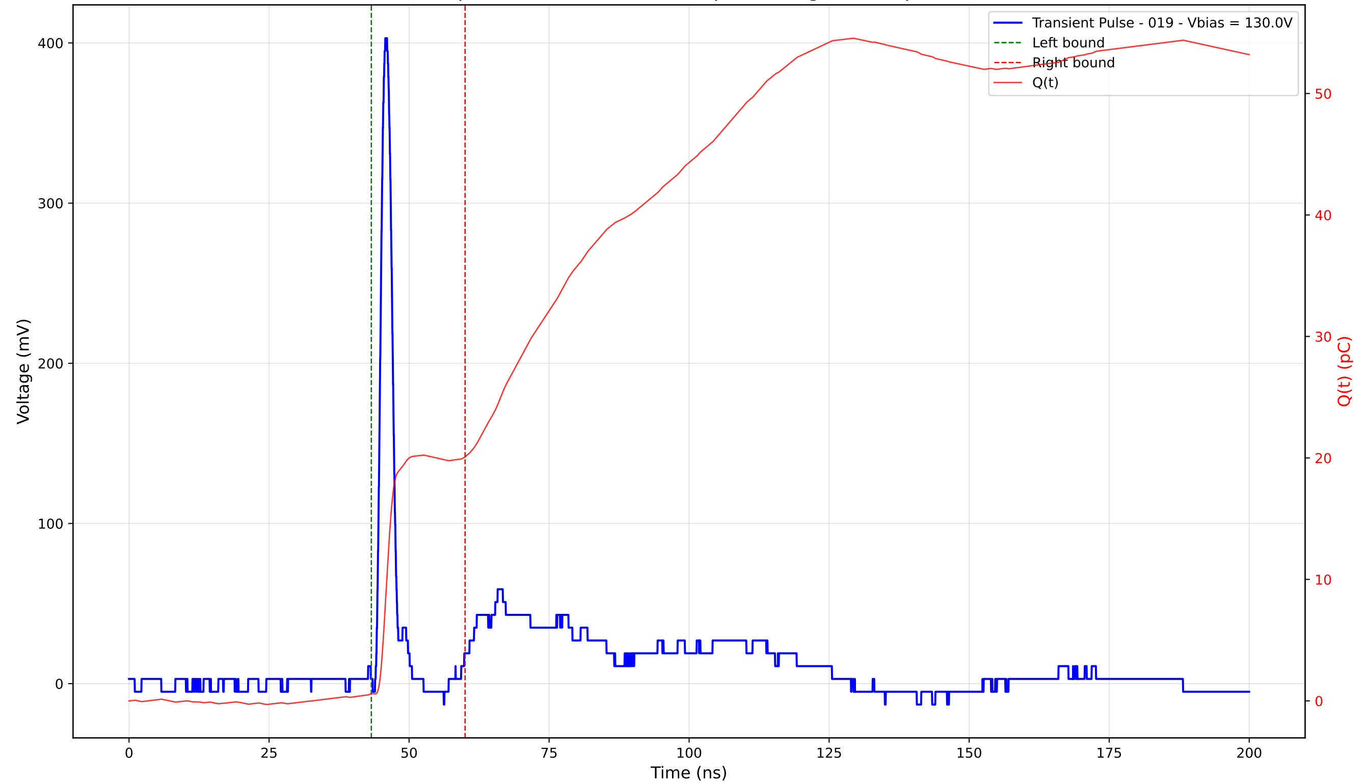
Transient Pulse - Sample: 4003 - Position: 205.0 \mu\text{m} - Charge: 19.50 pC - Rise Time: 1.11 ns
