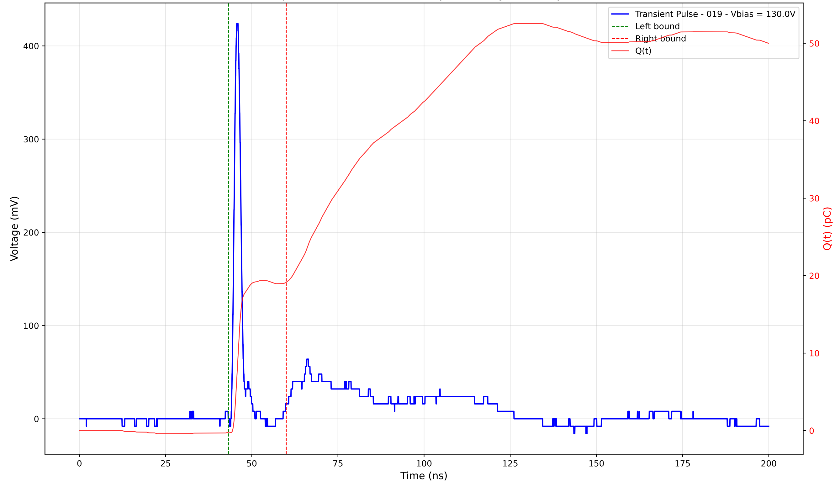
Transient Pulse - Sample: 4003 - Position: 195.0 \mu\text{m} - Charge: 19.35 pC - Rise Time: 1.09 ns
