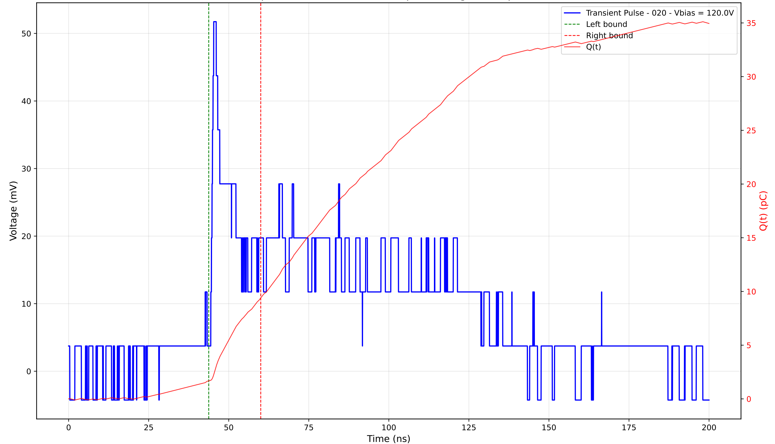
Transient Pulse - Sample: 4003 - Position: 285.0 \mu\text{m} - Charge: 7.73 pC - Rise Time: 0.92 ns
