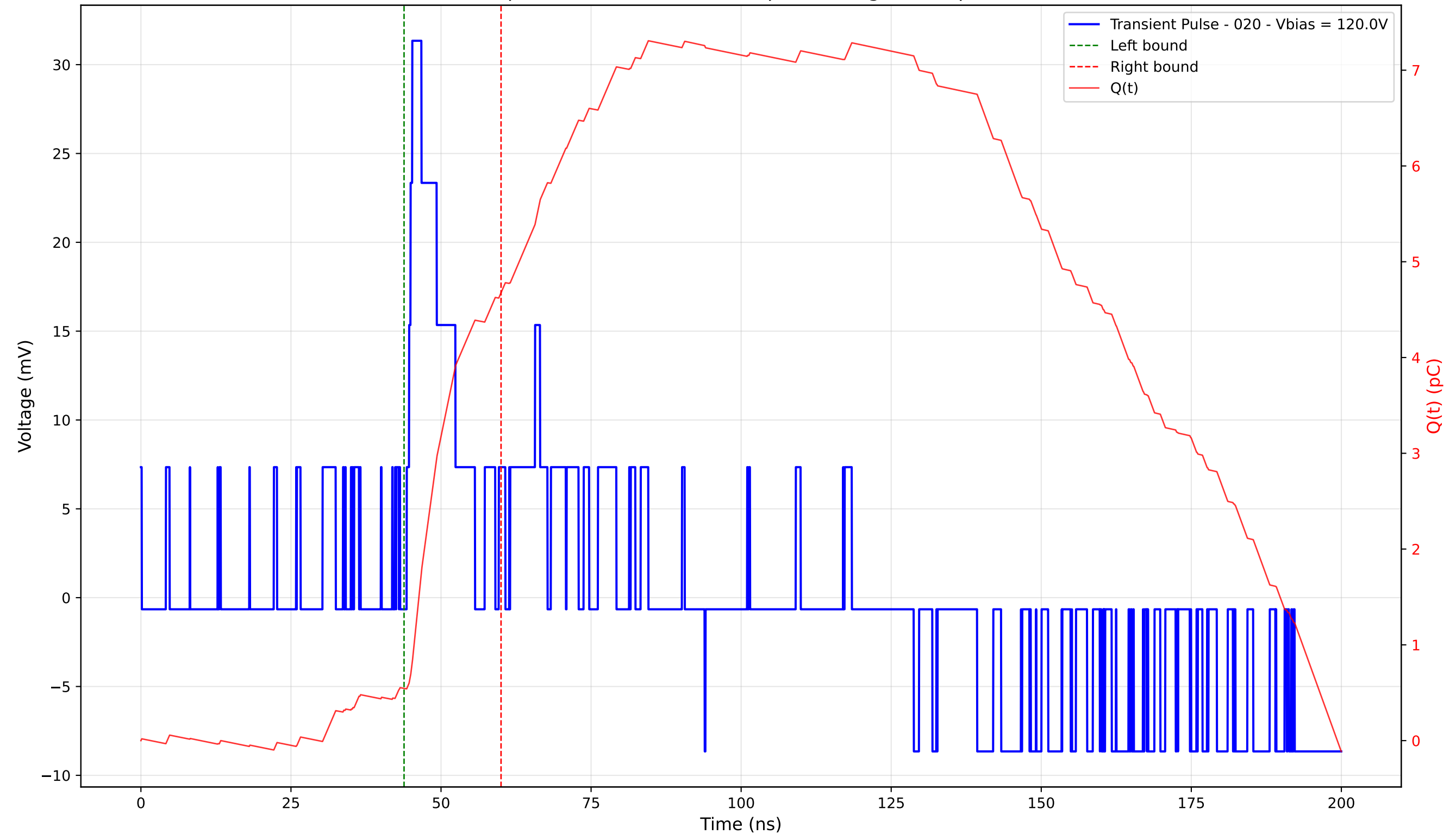
Transient Pulse - Sample: 4003 - Position: 60.0 \mu\text{m} - Charge: 4.13 pC - Rise Time: 0.93 ns
