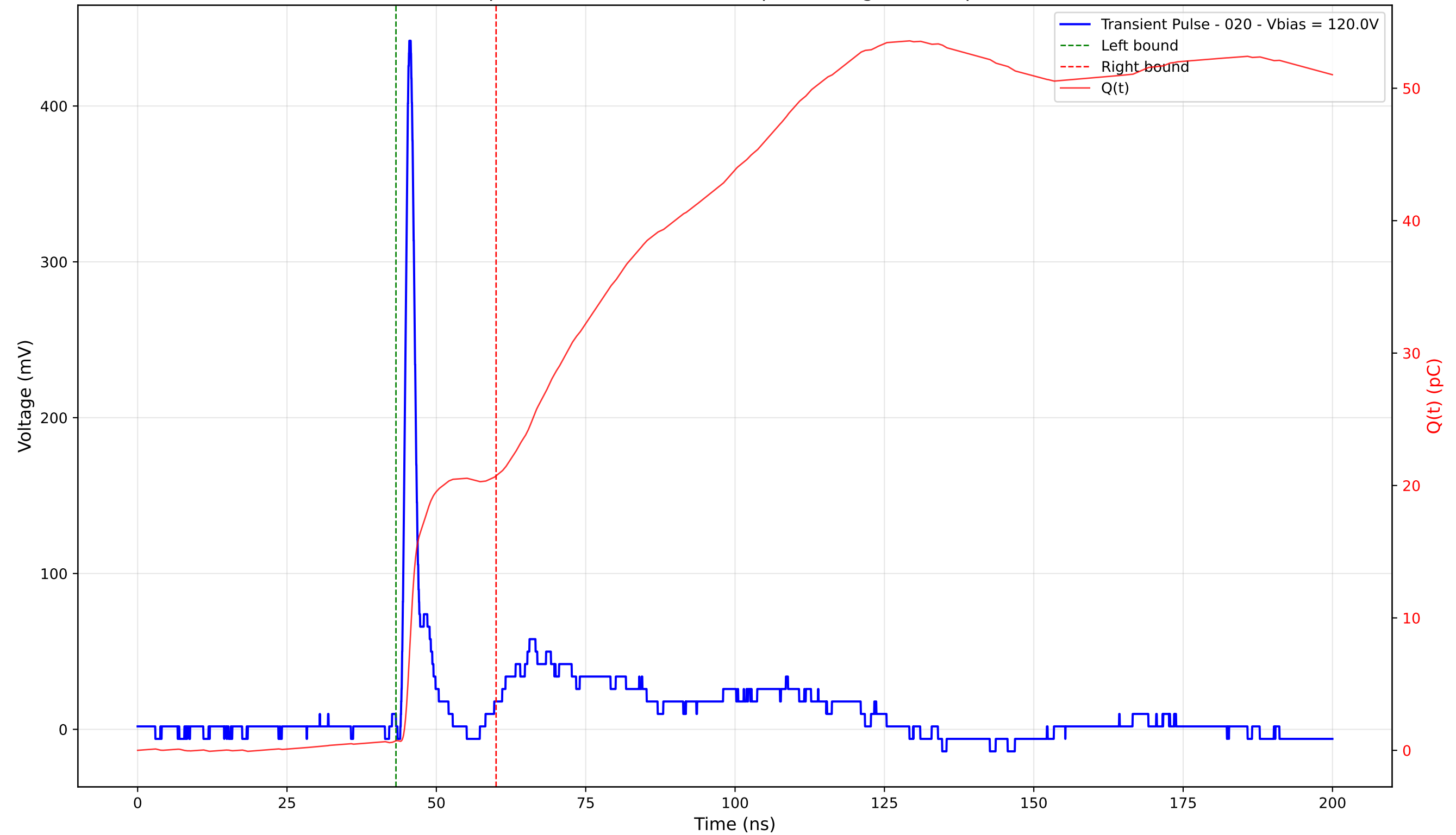
Transient Pulse - Sample: 4003 - Position: 155.0 \mu\text{m} - Charge: 20.00 pC - Rise Time: 0.97 ns
