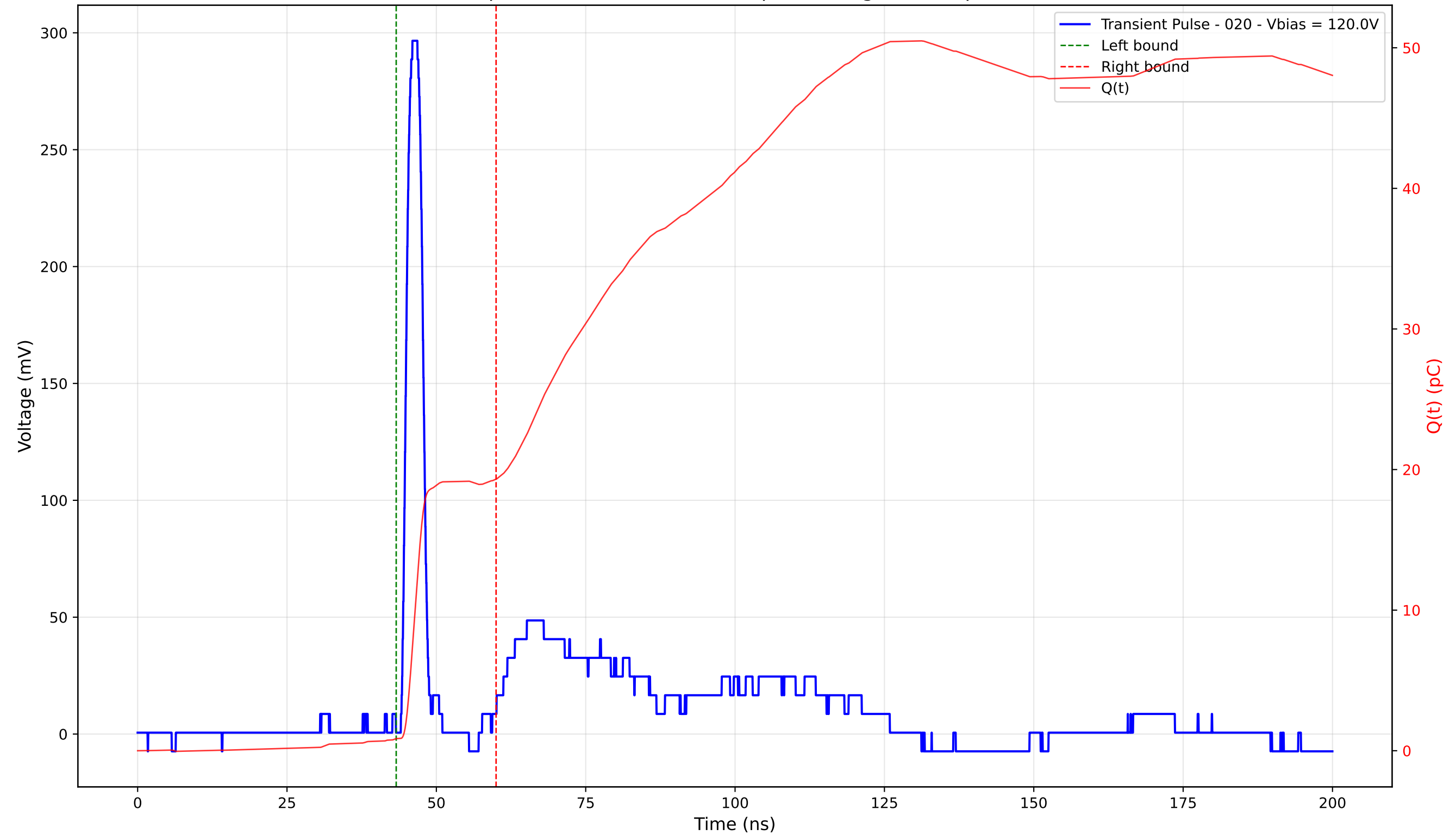
Transient Pulse - Sample: 4003 - Position: 230.0 \mu\text{m} - Charge: 18.45 pC - Rise Time: 1.25 ns
