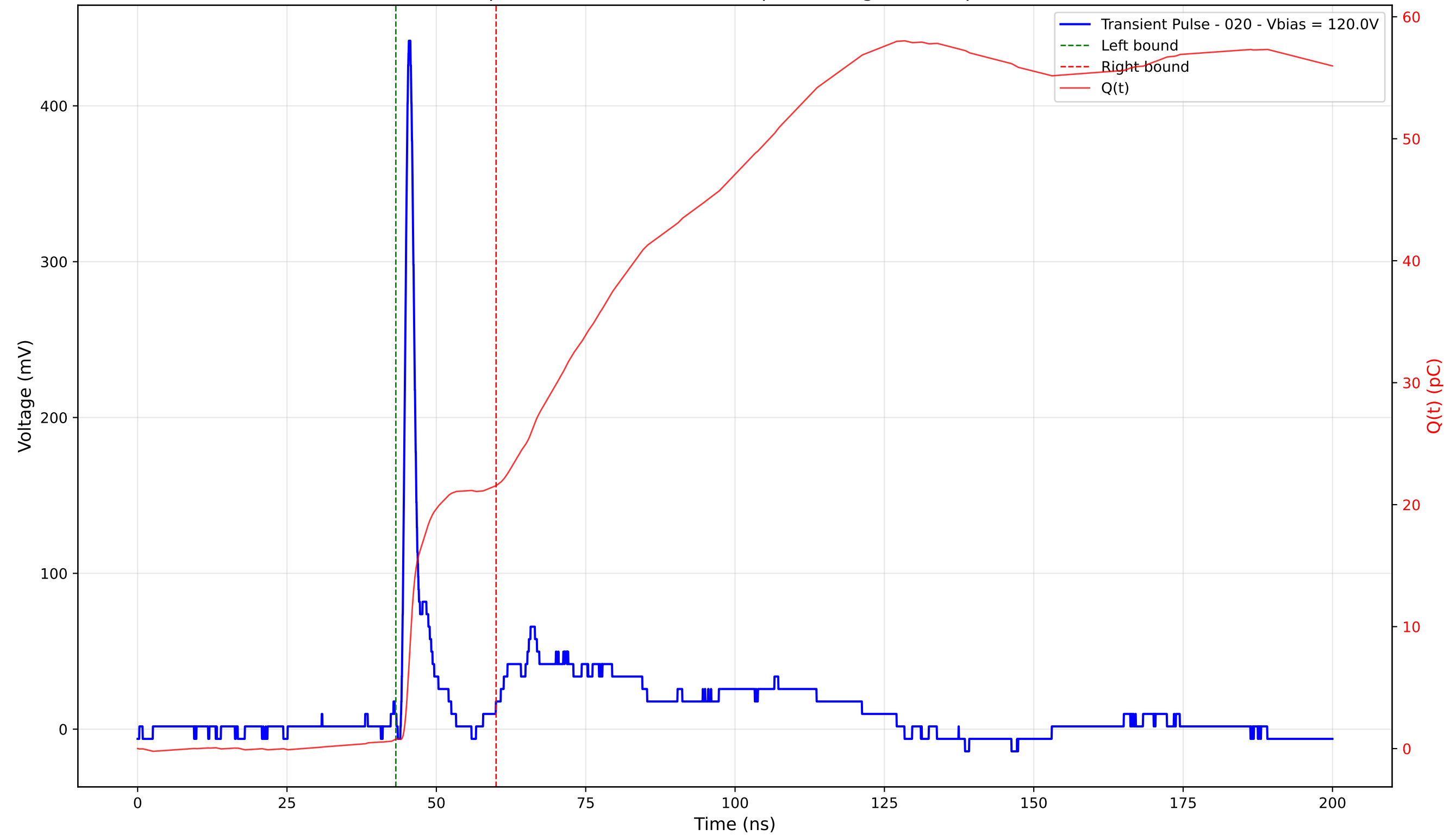
Transient Pulse - Sample: 4003 - Position: 140.0 \mu\text{m} - Charge: 20.78 pC - Rise Time: 0.91 ns
