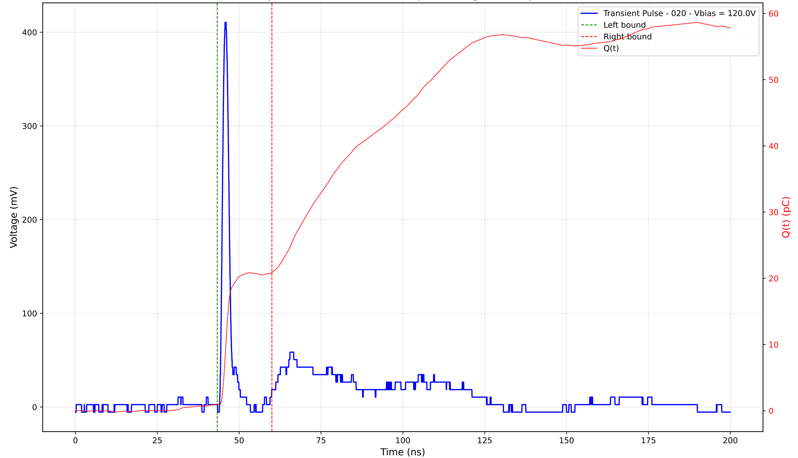
Transient Pulse - Sample: 4003 - Position: 195.0 \mu\text{m} - Charge: 19.91 pC - Rise Time: 1.08 ns
