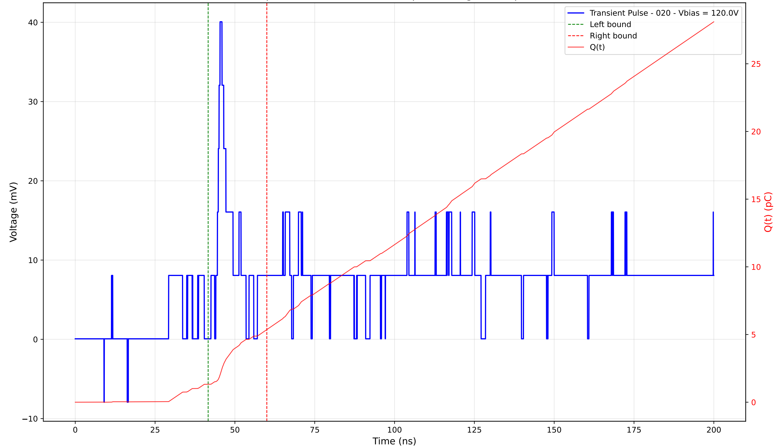
Transient Pulse - Sample: 4003 - Position: 320.0 \mu\text{m} - Charge: 4.04 pC - Rise Time: 1.33 ns
