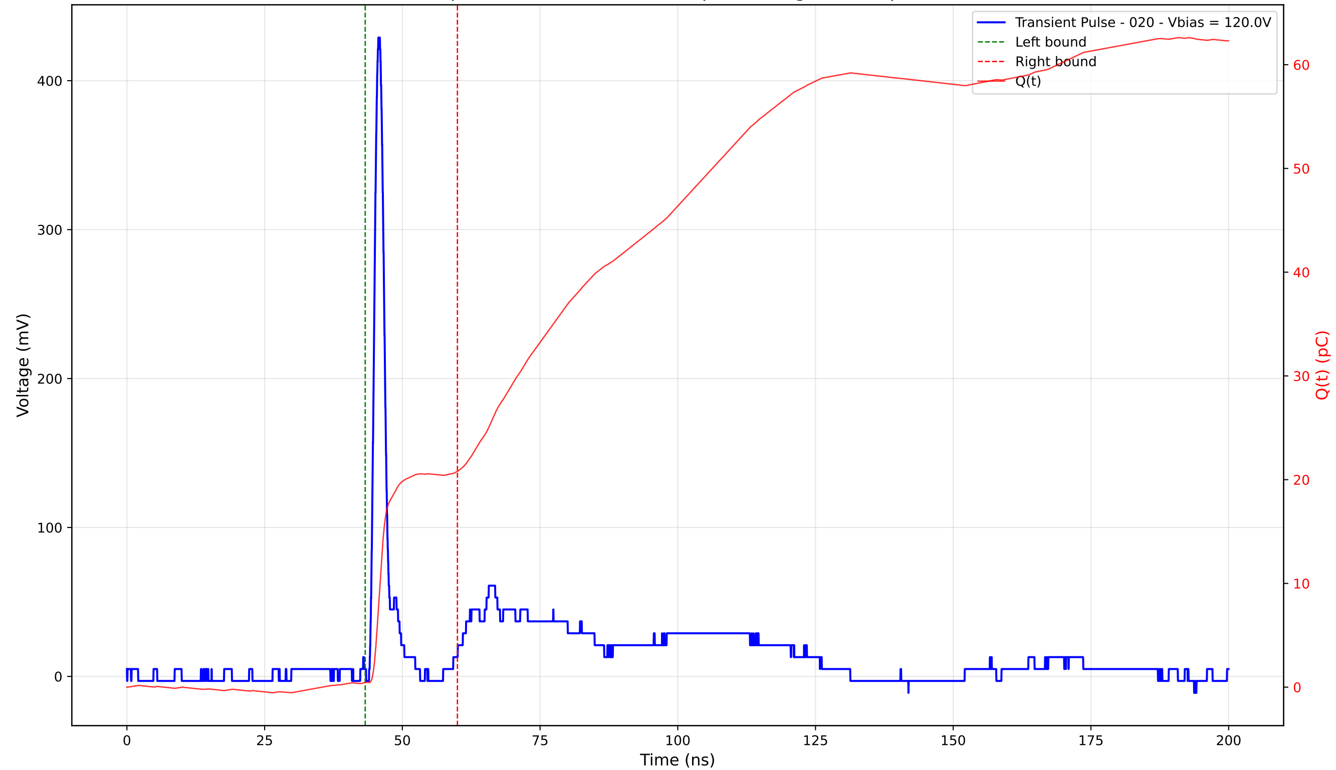
Transient Pulse - Sample: 4003 - Position: 185.0 \mu\text{m} - Charge: 20.33 pC - Rise Time: 1.09 ns
