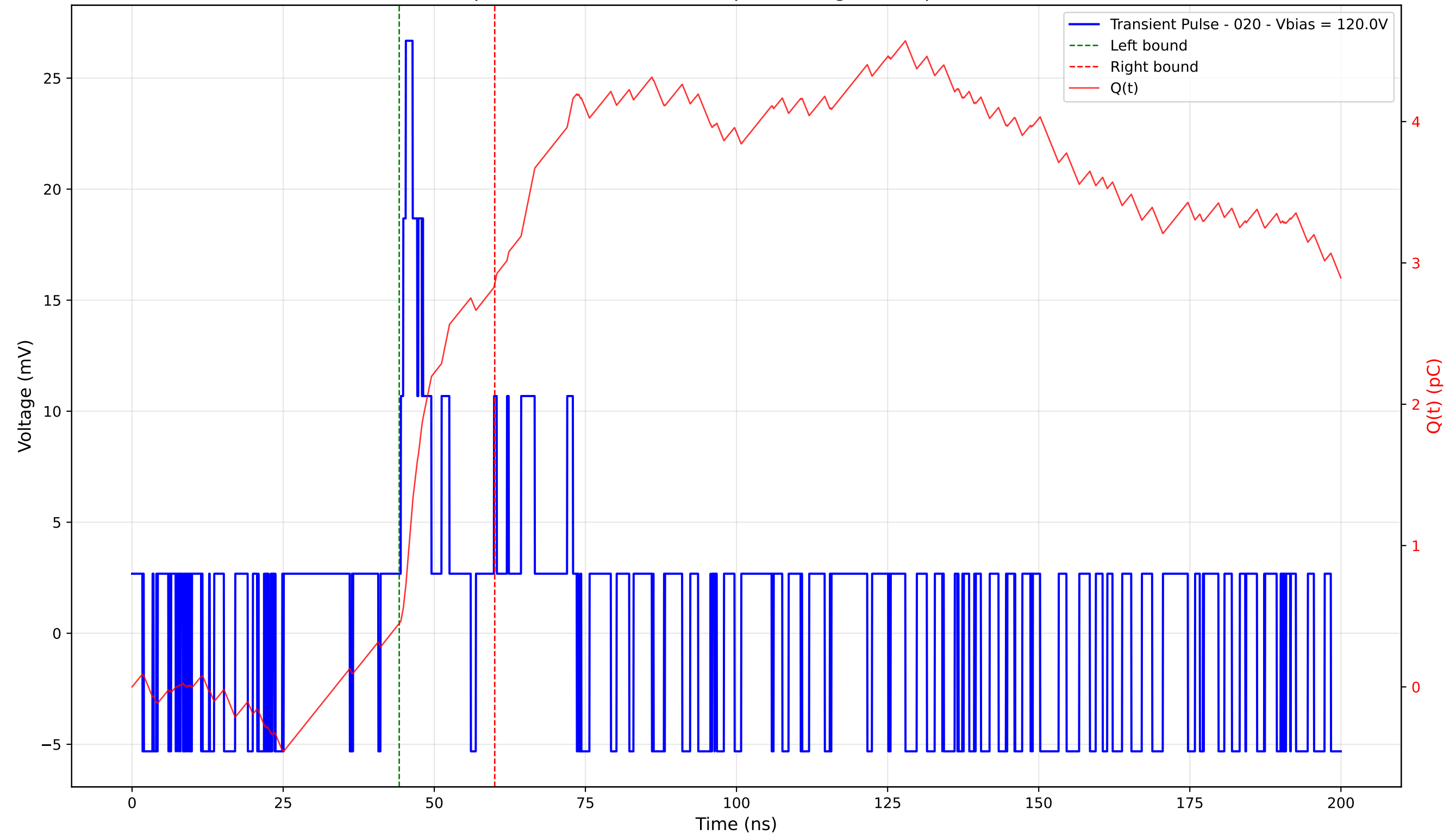
Transient Pulse - Sample: 4003 - Position: 40.0 \mu\text{m} - Charge: 2.40 pC - Rise Time: 0.00 ns (N/A)
