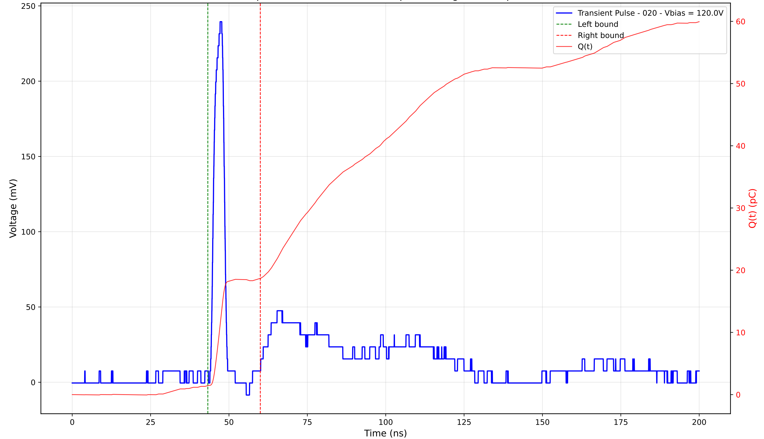
Transient Pulse - Sample: 4003 - Position: 250.0 \mu\text{m} - Charge: 17.22 pC - Rise Time: 2.18 ns
