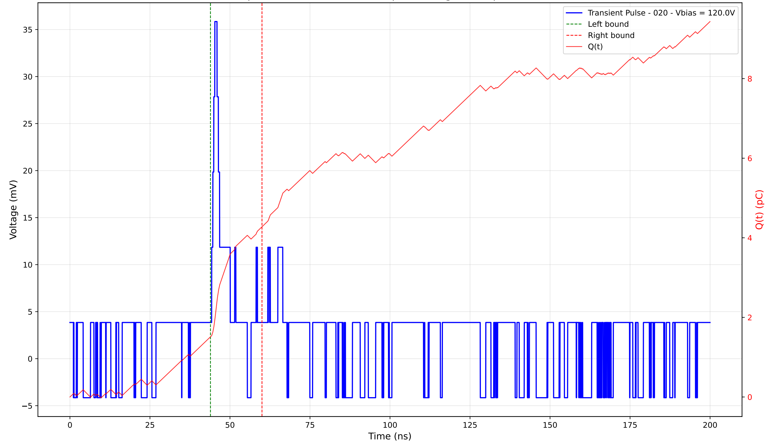
Transient Pulse - Sample: 4003 - Position: 325.0 \mu\text{m} - Charge: 2.77 pC - Rise Time: 0.00 ns (N/A)
