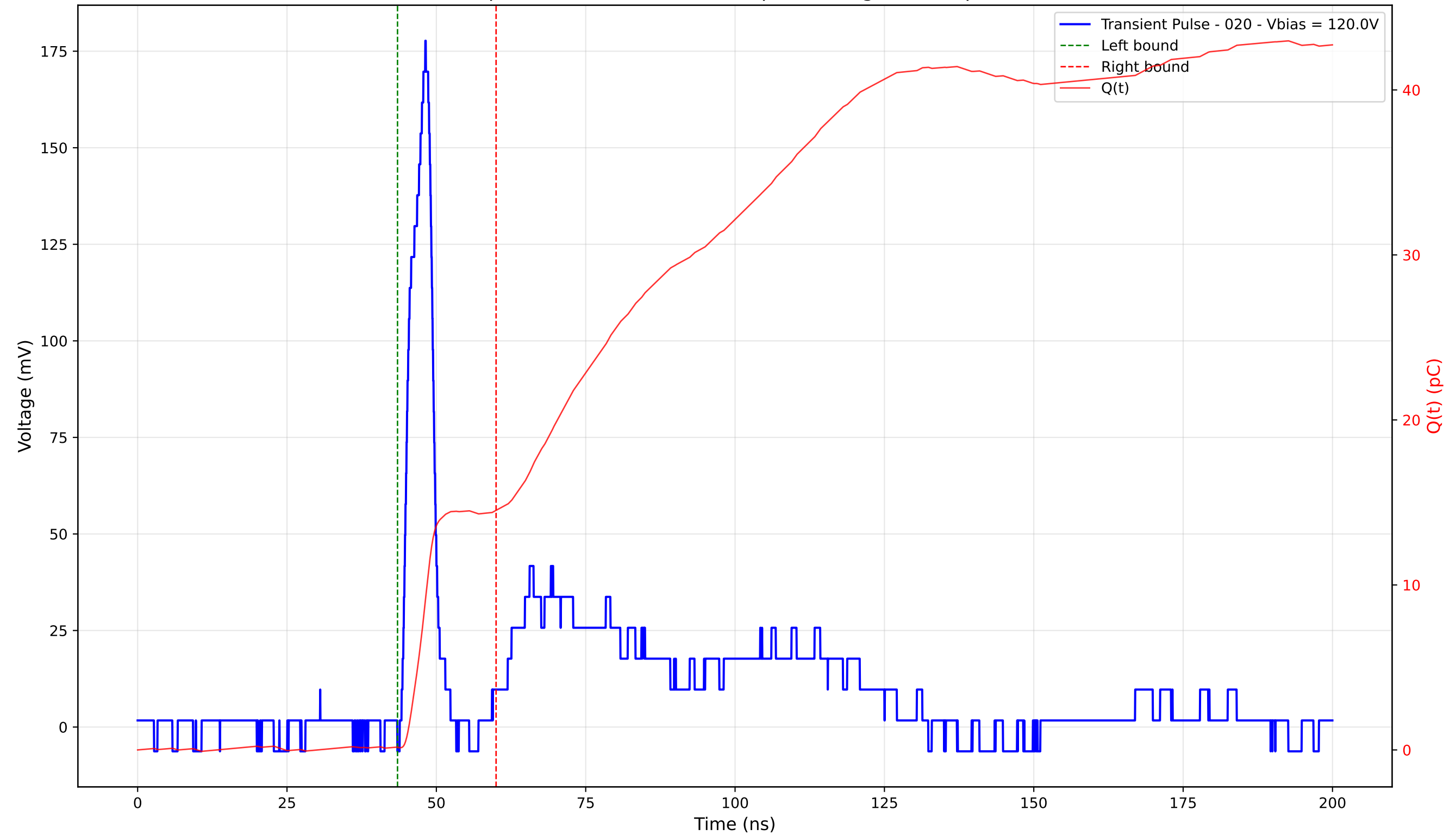
Transient Pulse - Sample: 4003 - Position: 265.0 \mu\text{m} - Charge: 14.34 pC - Rise Time: 3.12 ns
