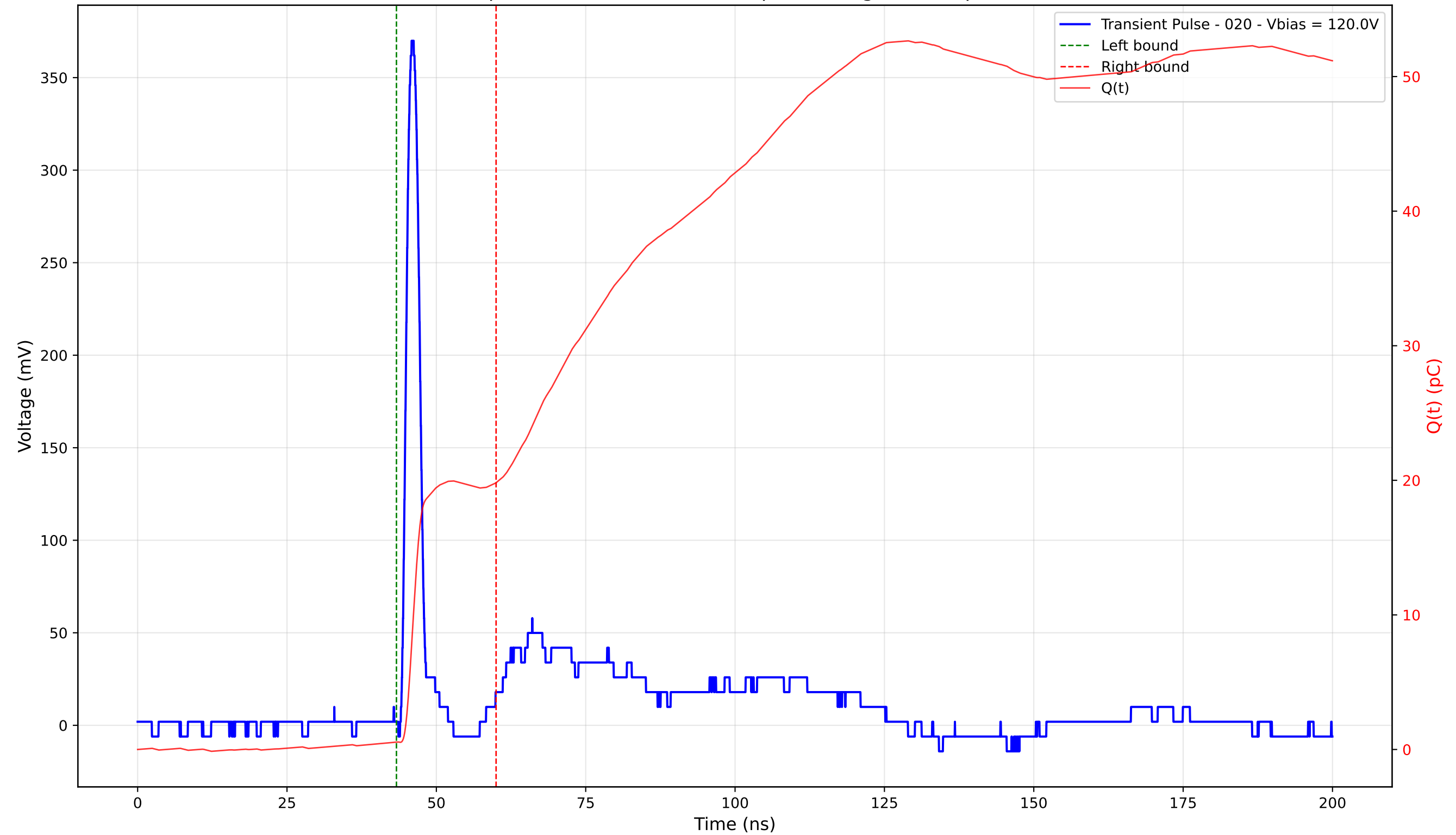
Transient Pulse - Sample: 4003 - Position: 210.0 \mu\text{m} - Charge: 19.27 pC - Rise Time: 1.19 ns
