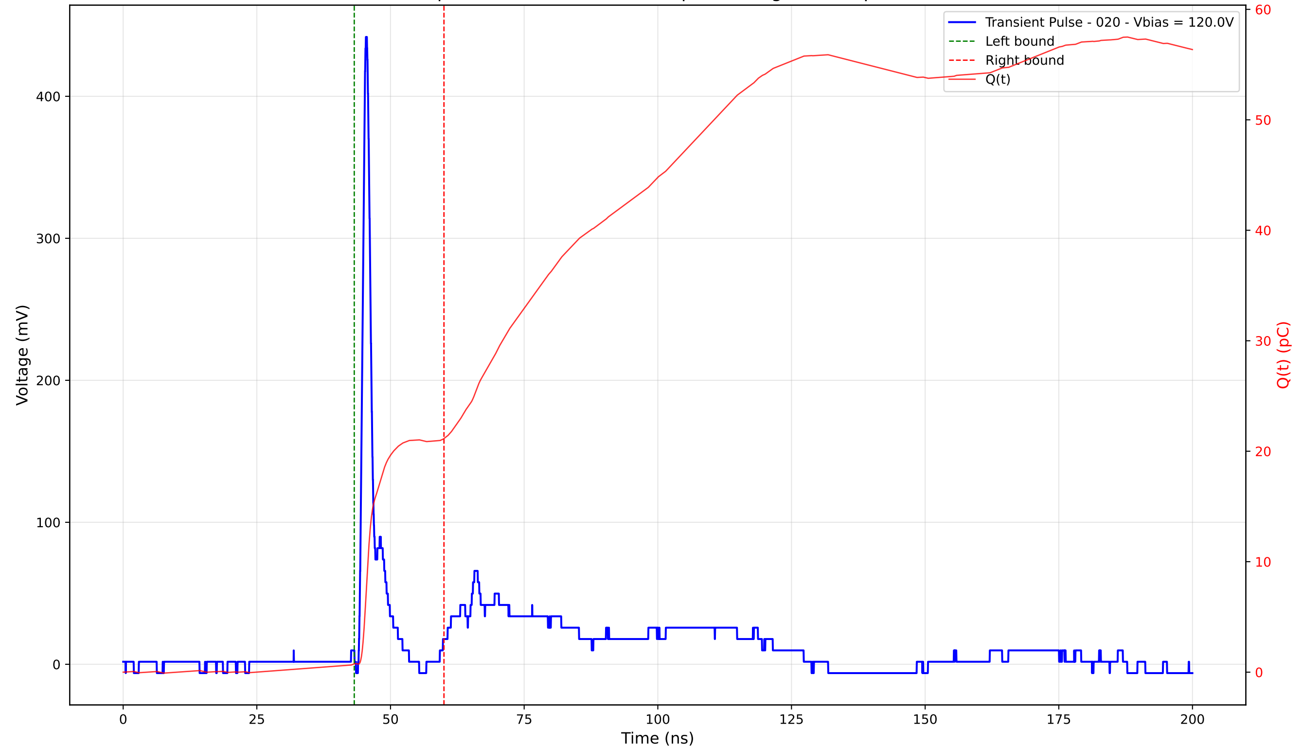
Transient Pulse - Sample: 4003 - Position: 135.0 \mu\text{m} - Charge: 20.39 pC - Rise Time: 0.92 ns
