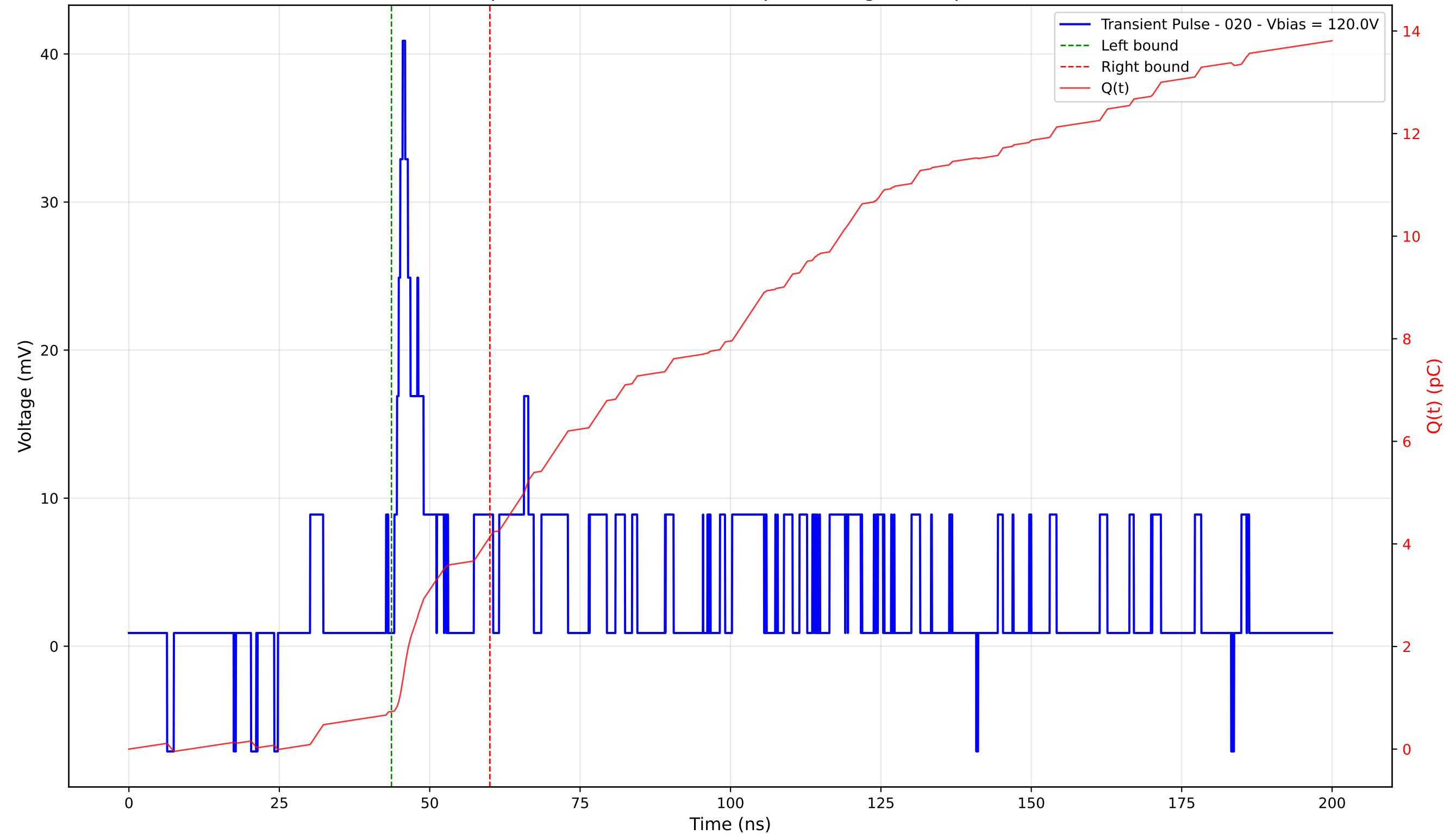
Transient Pulse - Sample: 4003 - Position: 310.0 \mu\text{m} - Charge: 3.41 pC - Rise Time: 1.39 ns
