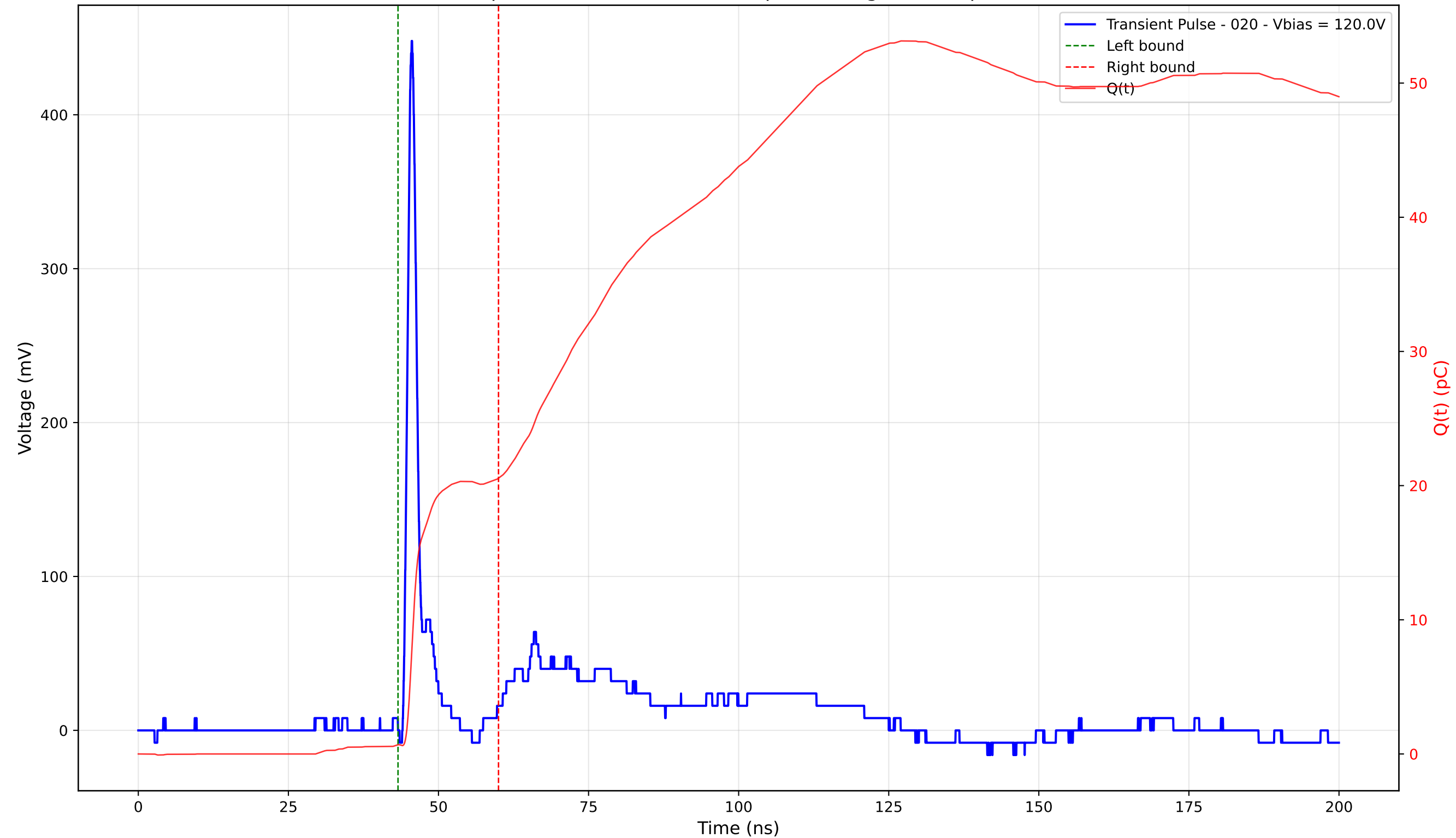
Transient Pulse - Sample: 4003 - Position: 150.0 \mu\text{m} - Charge: 19.86 pC - Rise Time: 0.97 ns
