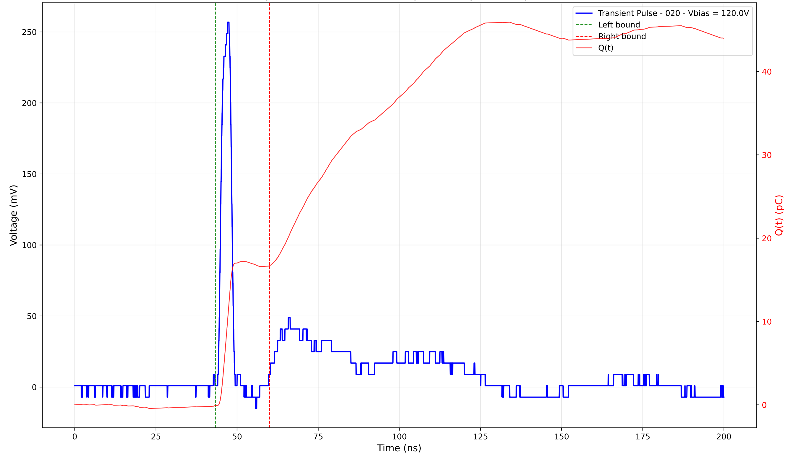
Transient Pulse - Sample: 4003 - Position: 245.0 \mu\text{m} - Charge: 16.78 pC - Rise Time: 1.58 ns
