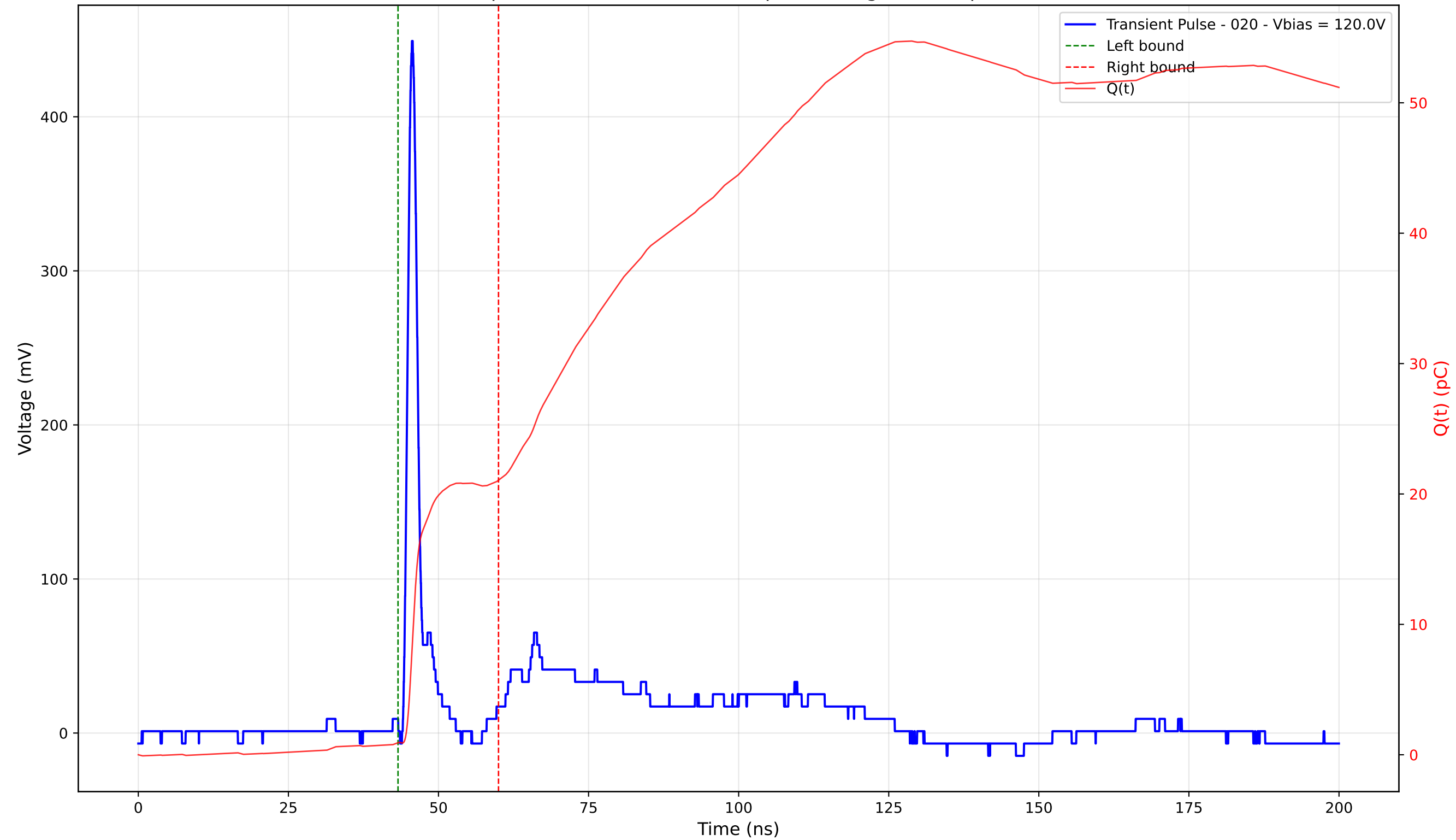
Transient Pulse - Sample: 4003 - Position: 165.0 \mu\text{m} - Charge: 20.12 pC - Rise Time: 1.01 ns
