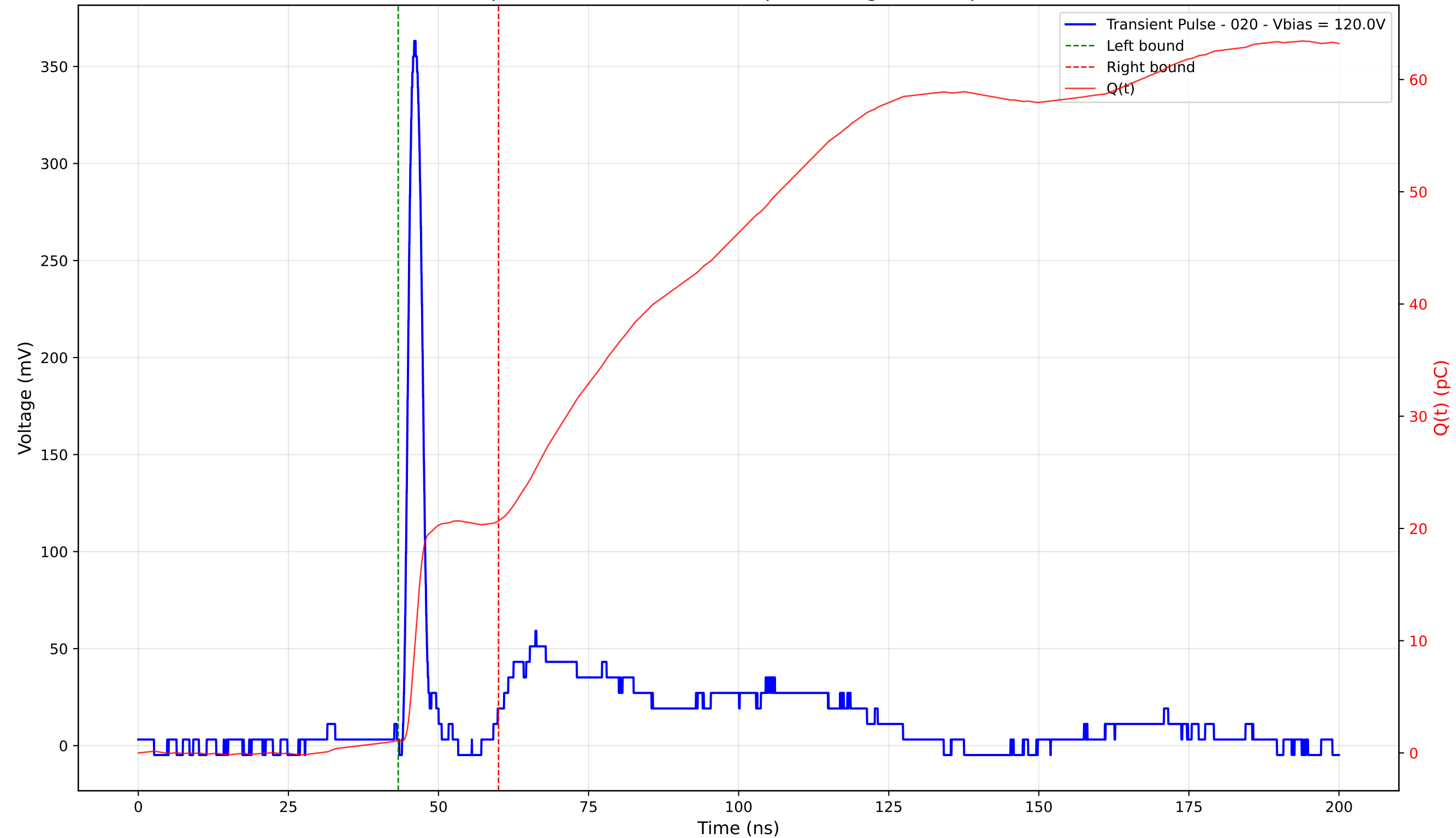
Transient Pulse - Sample: 4003 - Position: 215.0 \mu\text{m} - Charge: 19.56 pC - Rise Time: 1.20 ns
