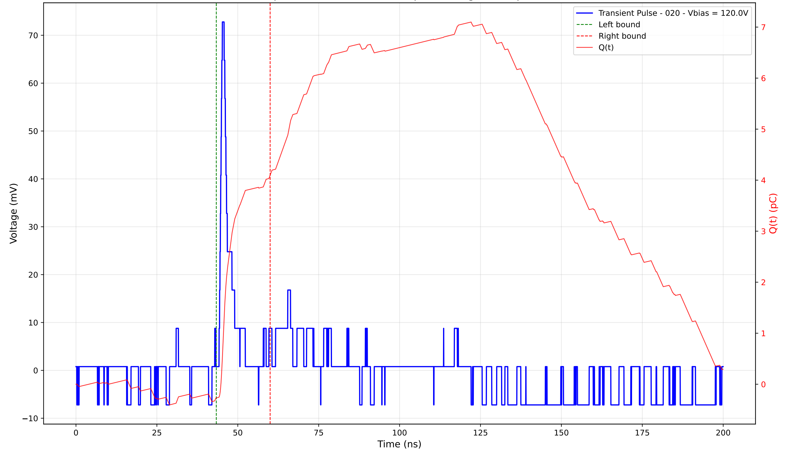
Transient Pulse - Sample: 4003 - Position: 90.0 \mu\text{m} - Charge: 4.37 pC - Rise Time: 1.00 ns
