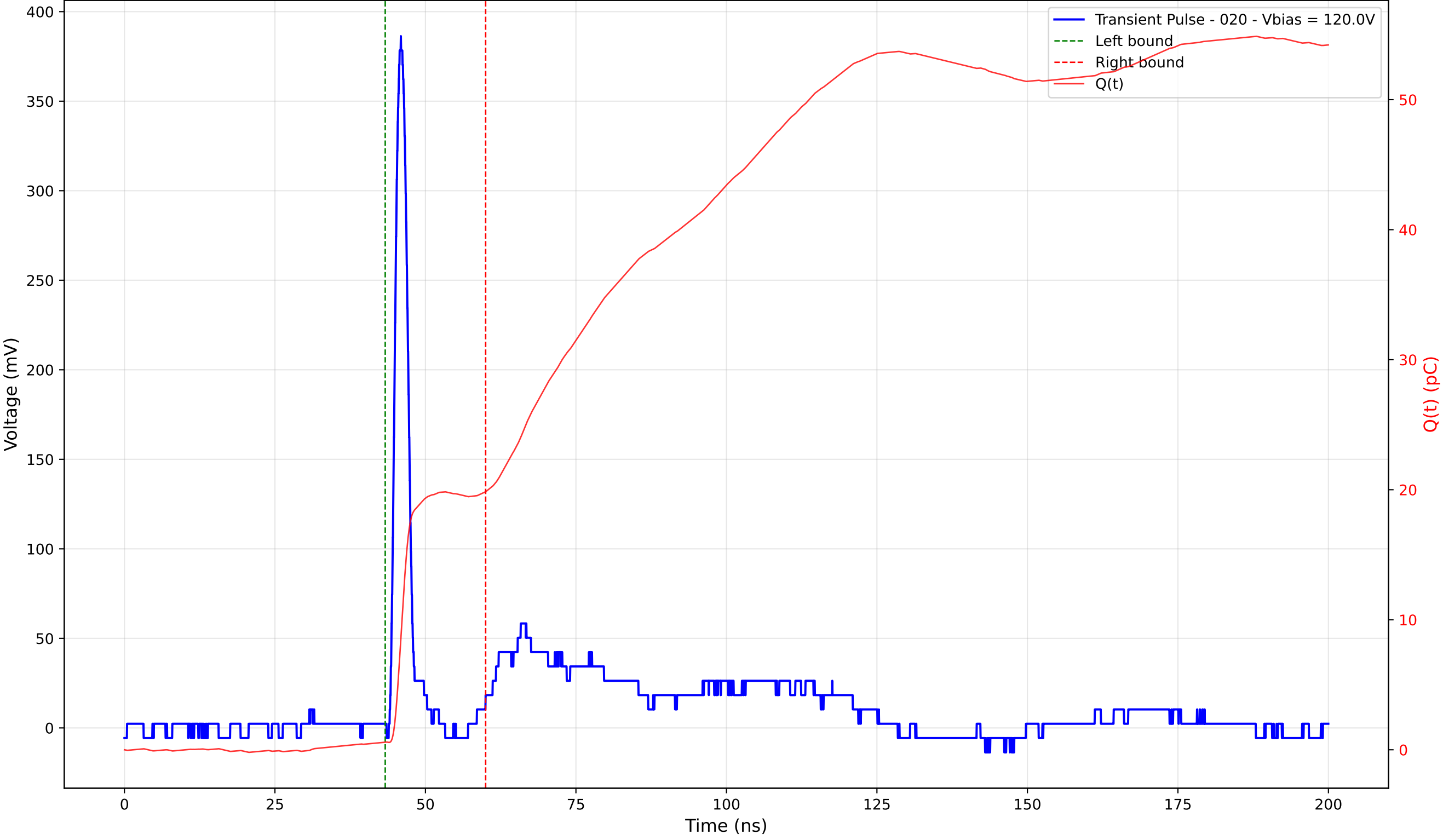
Transient Pulse - Sample: 4003 - Position: 205.0 \mu\text{m} - Charge: 19.25 pC - Rise Time: 1.19 ns
