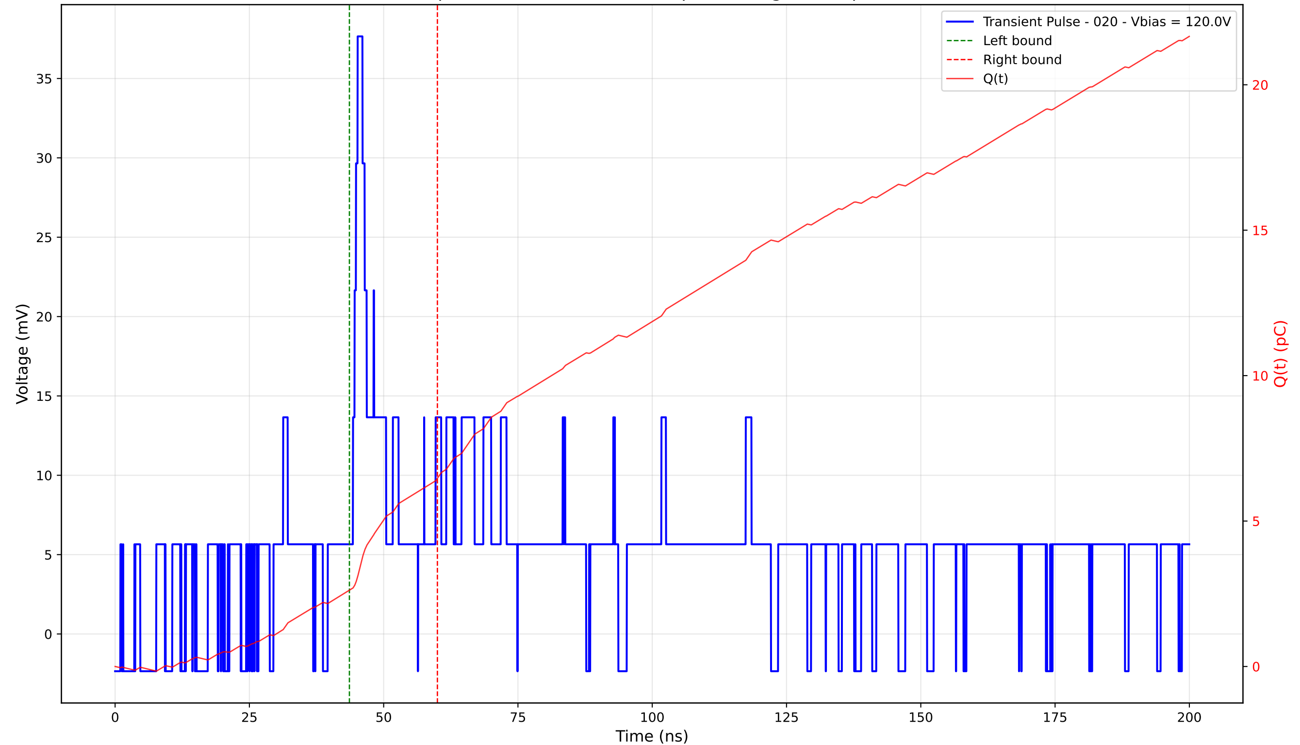
Transient Pulse - Sample: 4003 - Position: 380.0 \mu\text{m} - Charge: 3.85 pC - Rise Time: 5.57 ns
