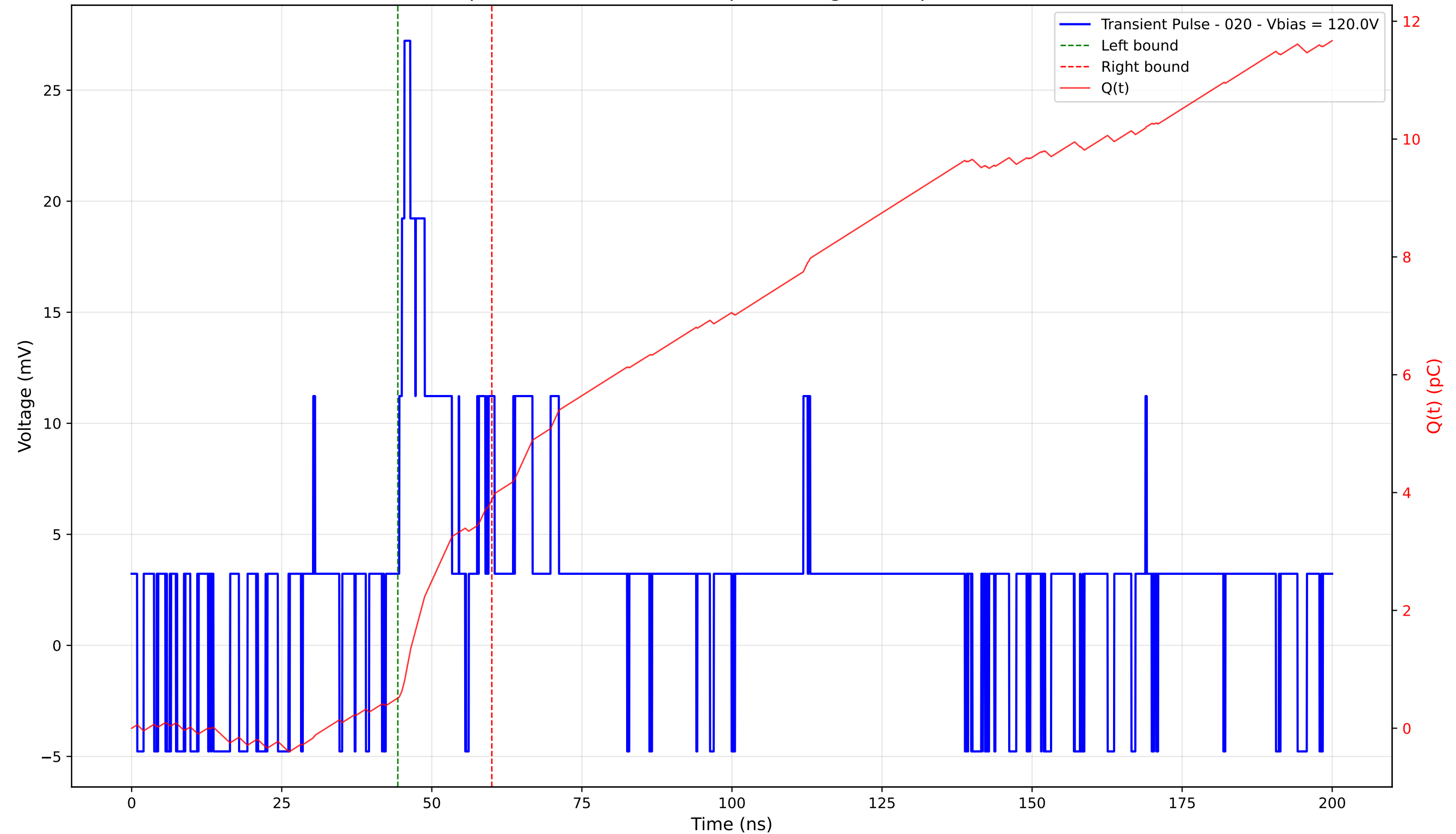
Transient Pulse - Sample: 4003 - Position: 65.0 \mu\text{m} - Charge: 3.37 pC - Rise Time: 0.00 ns (N/A)
