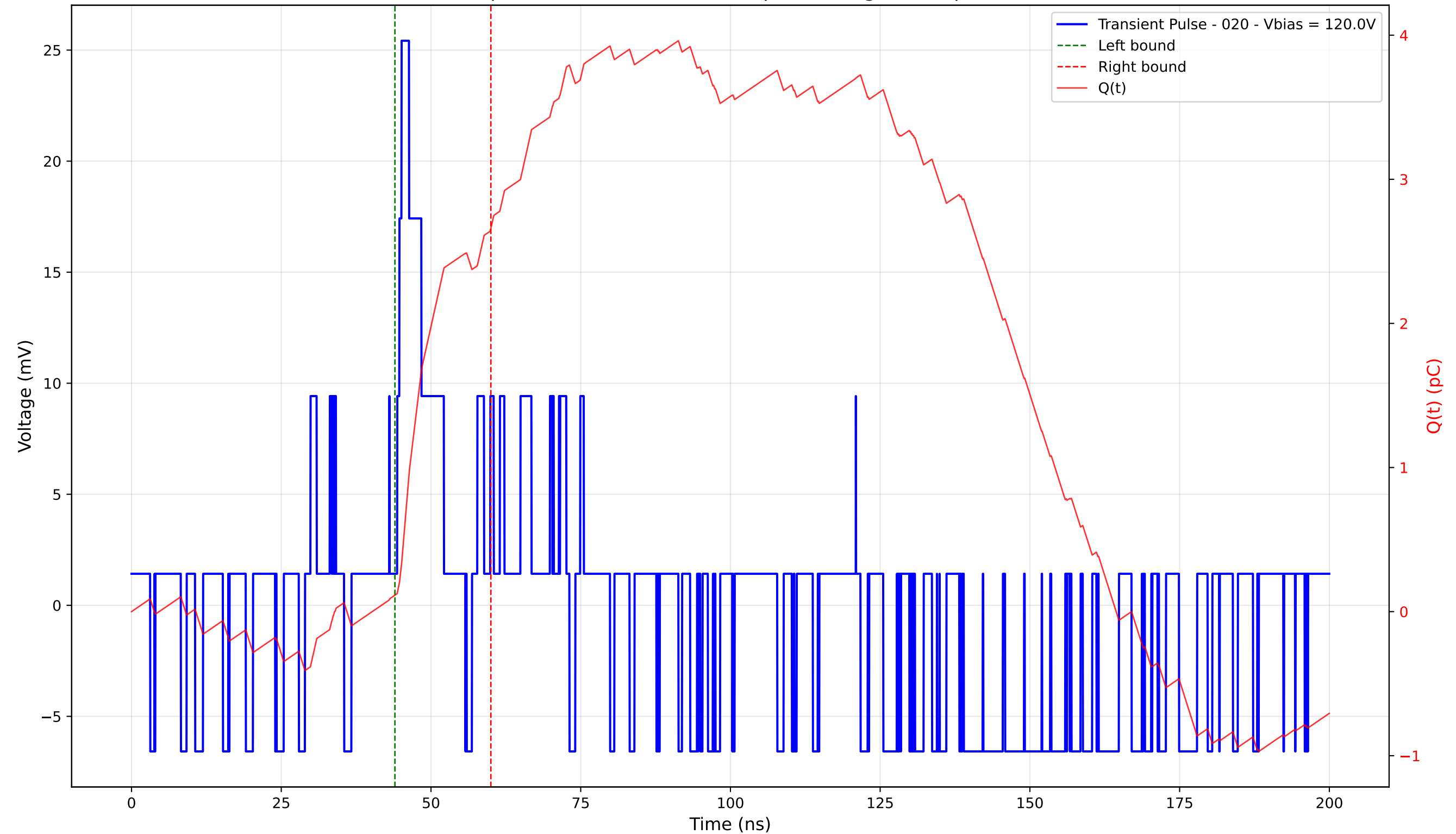
Transient Pulse - Sample: 4003 - Position: 330.0 \mu\text{m} - Charge: 2.55 pC - Rise Time: 0.74 ns
