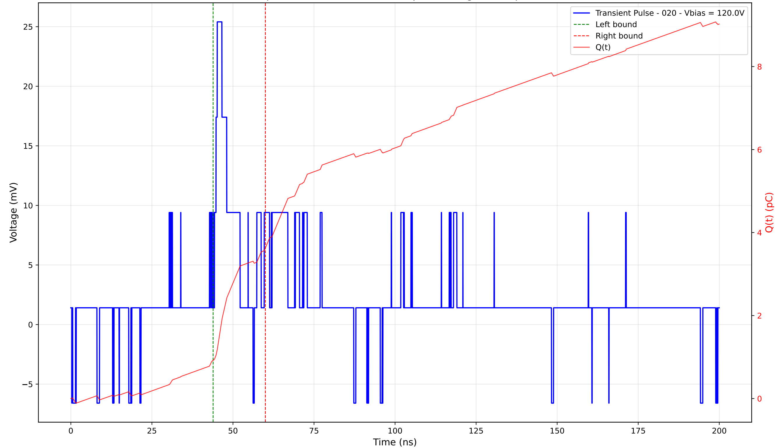
Transient Pulse - Sample: 4003 - Position: 350.0 \mu\text{m} - Charge: 2.71 pC - Rise Time: 0.86 ns
