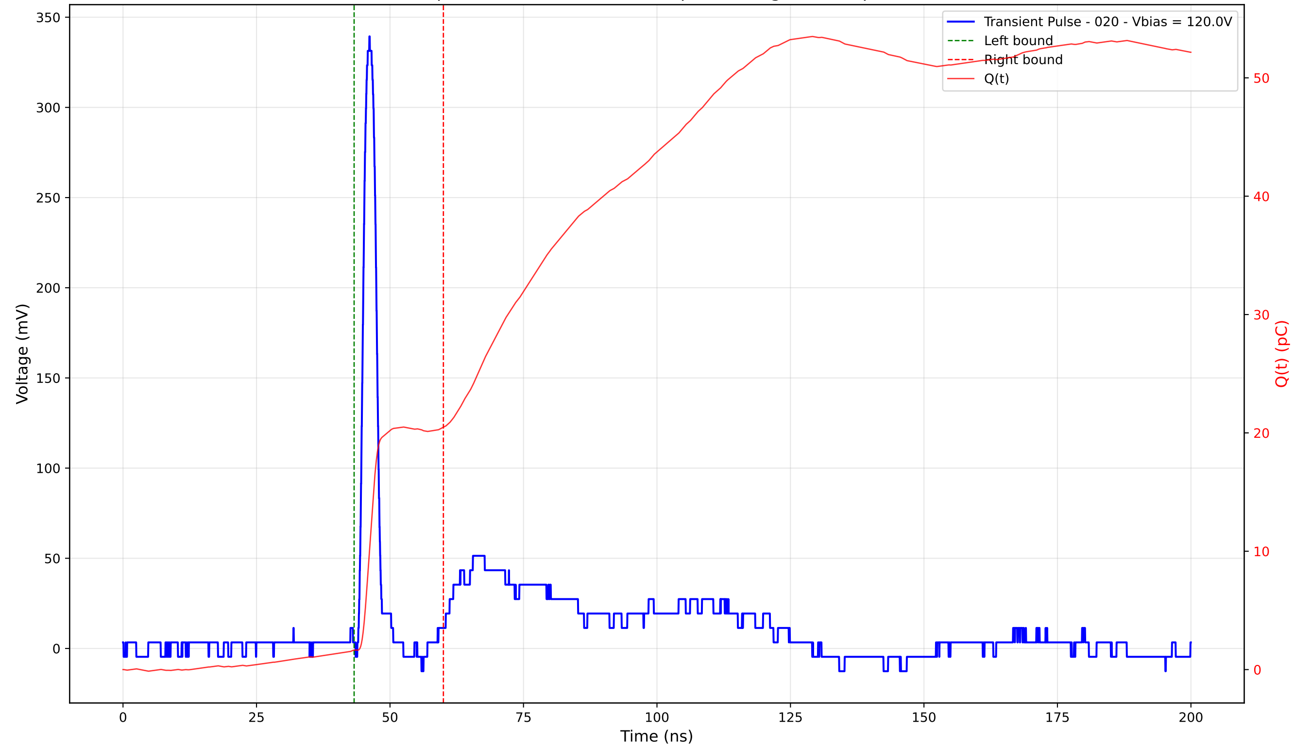
Transient Pulse - Sample: 4003 - Position: 220.0 \mu\text{m} - Charge: 18.83 pC - Rise Time: 1.24 ns
