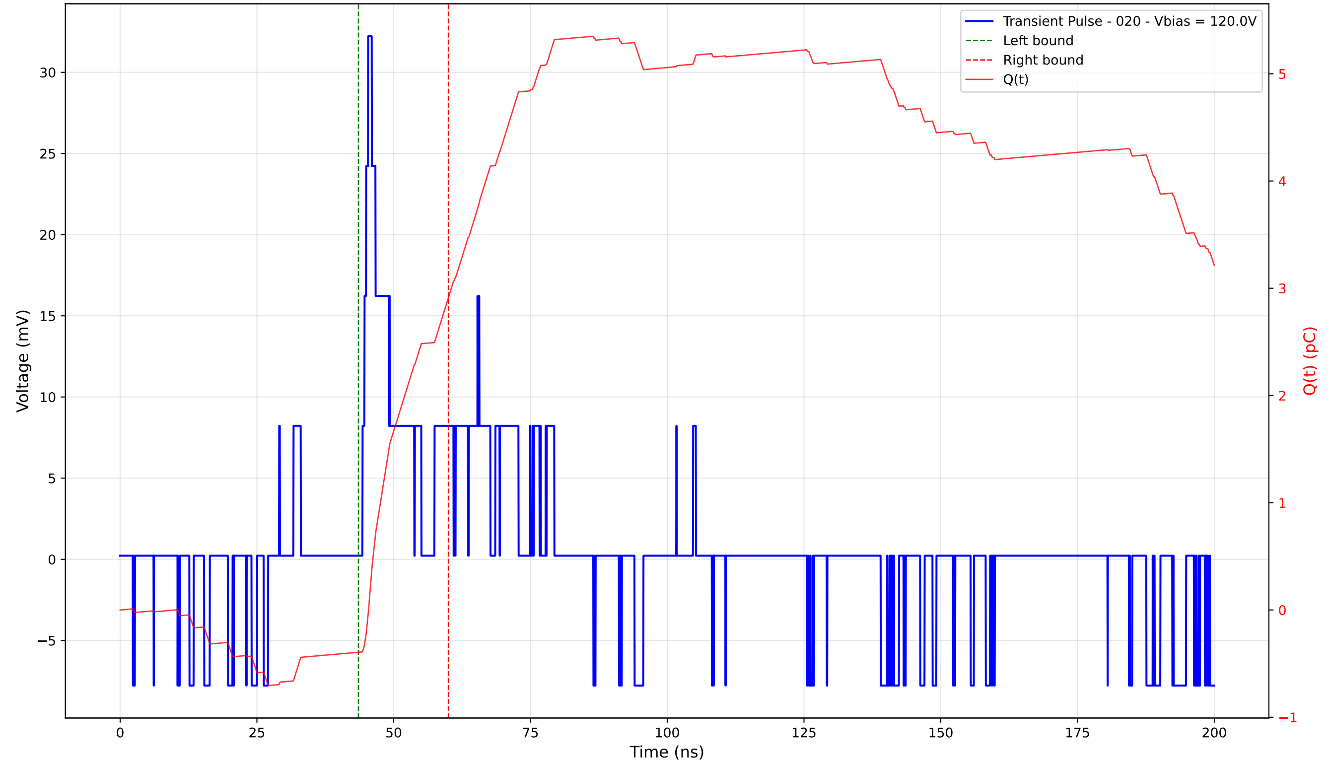
Transient Pulse - Sample: 4003 - Position: 45.0 \mu\text{m} - Charge: 3.31 pC - Rise Time: 1.03 ns
