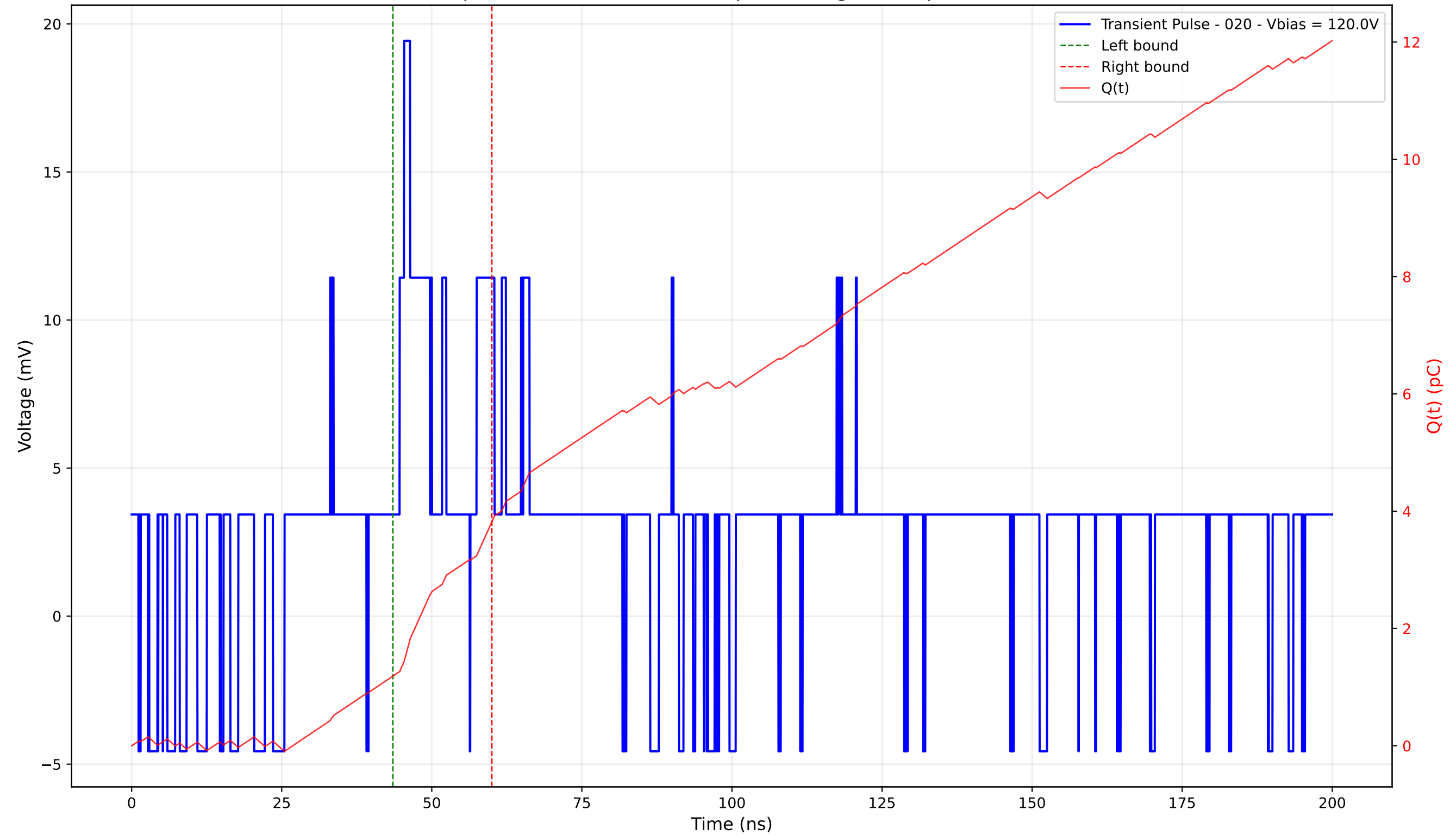
Transient Pulse - Sample: 4003 - Position: 425.0 \mu\text{m} - Charge: 2.64 pC - Rise Time: 0.00 ns (N/A)
