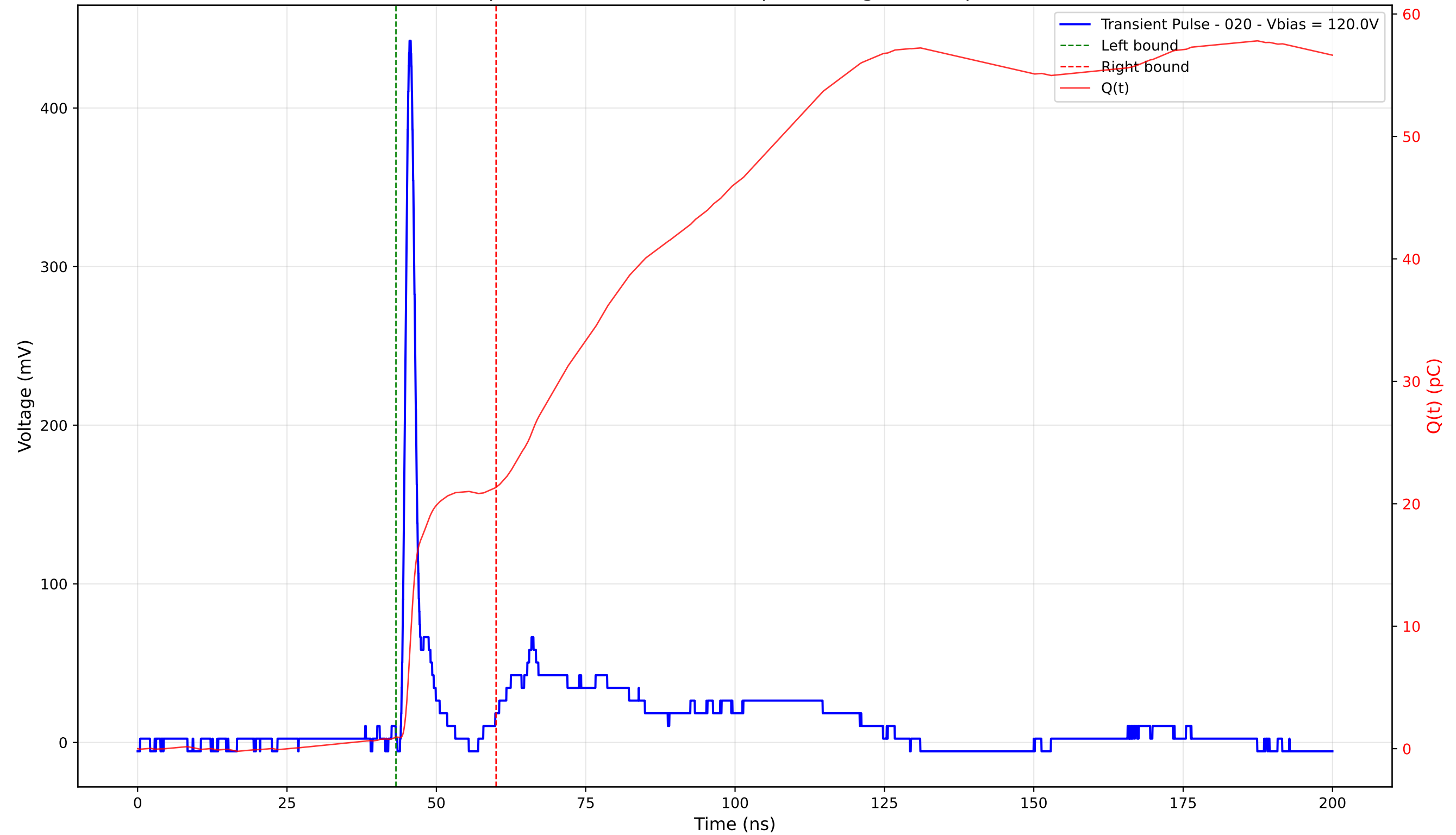
Transient Pulse - Sample: 4003 - Position: 160.0 \mu\text{m} - Charge: 20.41 pC - Rise Time: 1.00 ns
