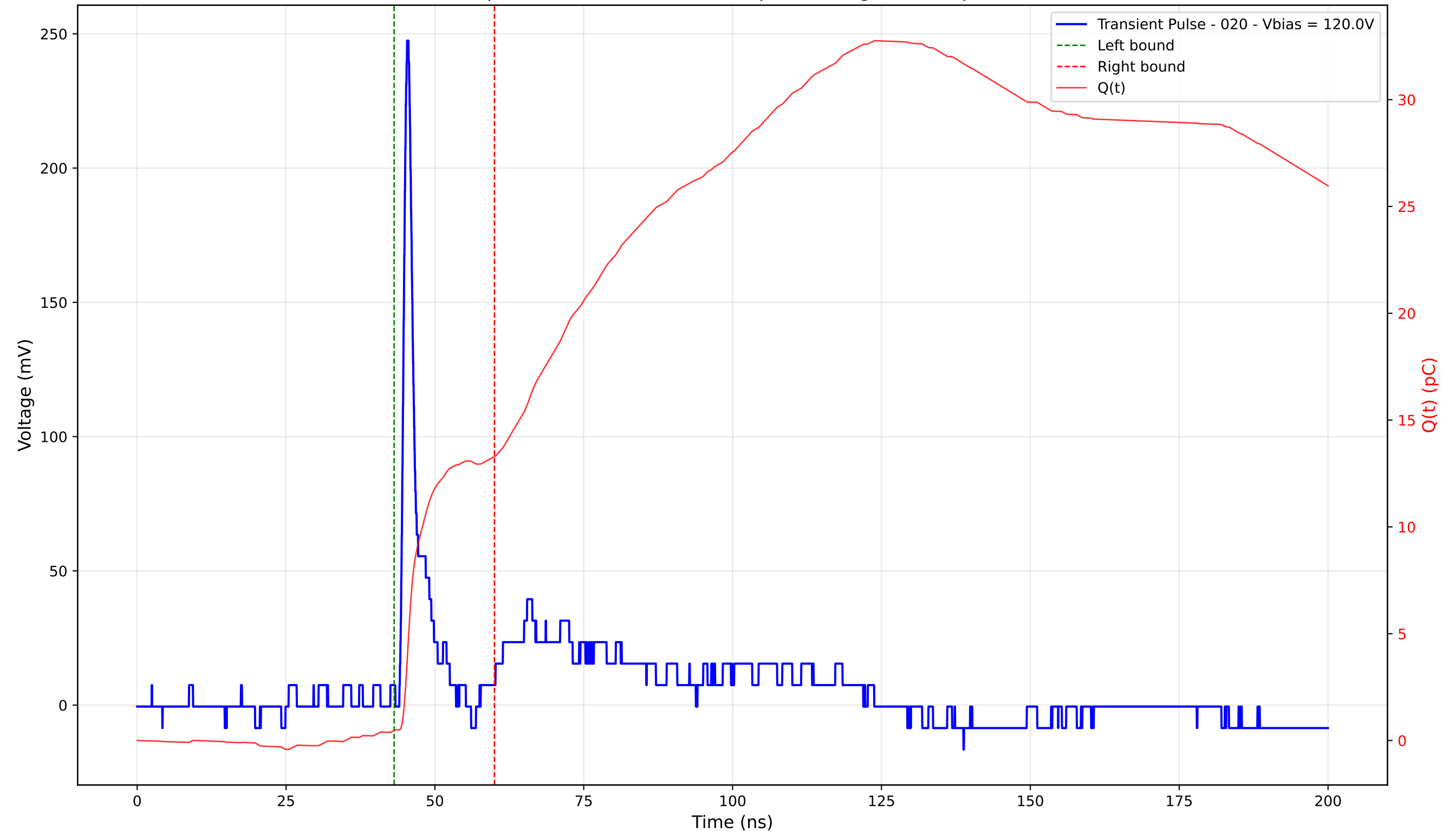
Transient Pulse - Sample: 4003 - Position: 105.0 \mu\text{m} - Charge: 12.81 pC - Rise Time: 0.88 ns
