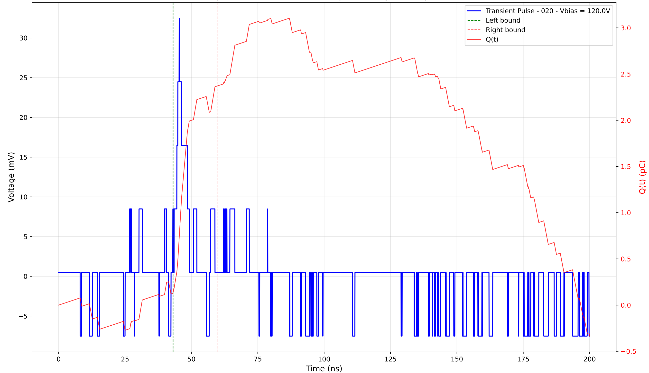
Transient Pulse - Sample: 4003 - Position: 370.0 \mu\text{m} - Charge: 2.23 pC - Rise Time: 1.91 ns
