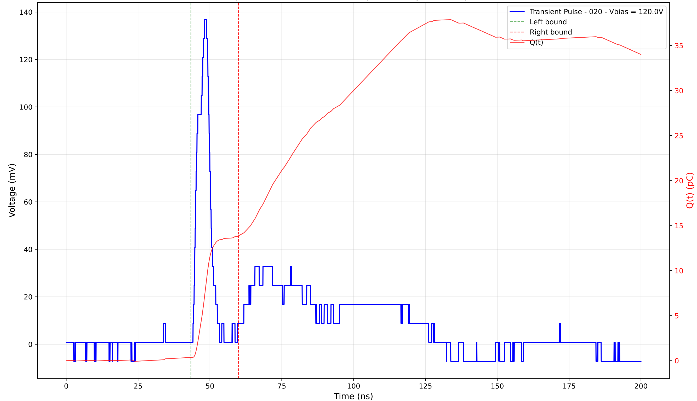
Transient Pulse - Sample: 4003 - Position: 270.0 \mu\text{m} - Charge: 13.52 pC - Rise Time: 3.43 ns
