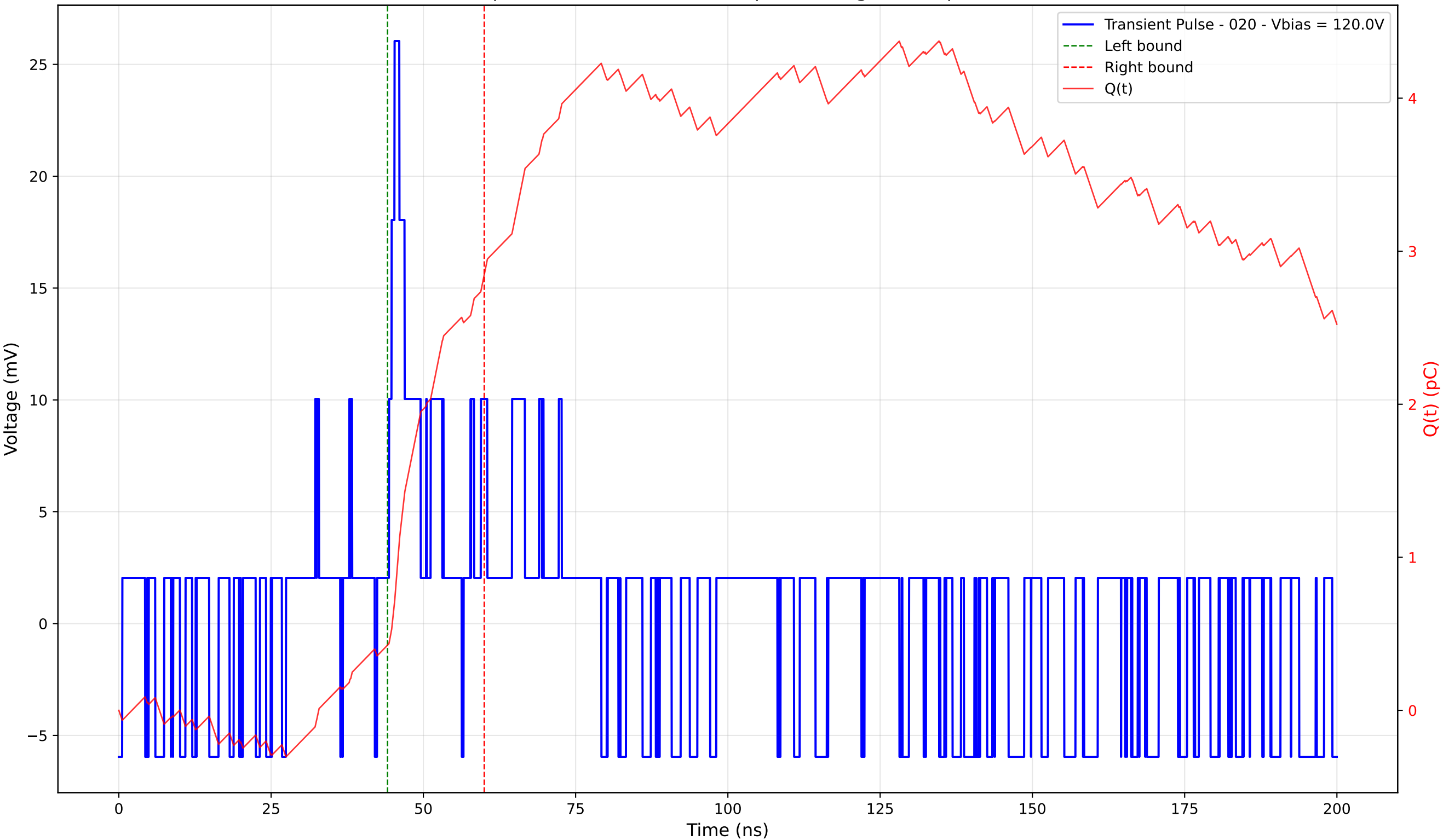
Transient Pulse - Sample: 4003 - Position: 25.0 \mu\text{m} - Charge: 2.42 pC - Rise Time: 0.92 ns
