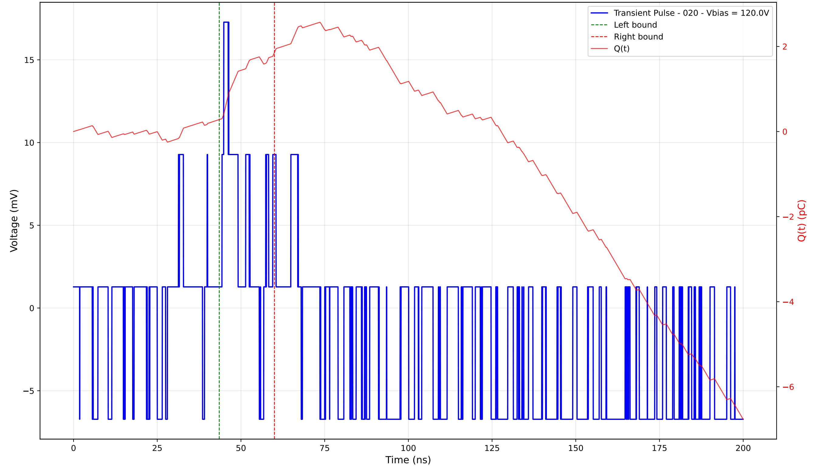
Transient Pulse - Sample: 4003 - Position: 15.0 \mu\text{m} - Charge: 1.58 pC - Rise Time: 0.54 ns
