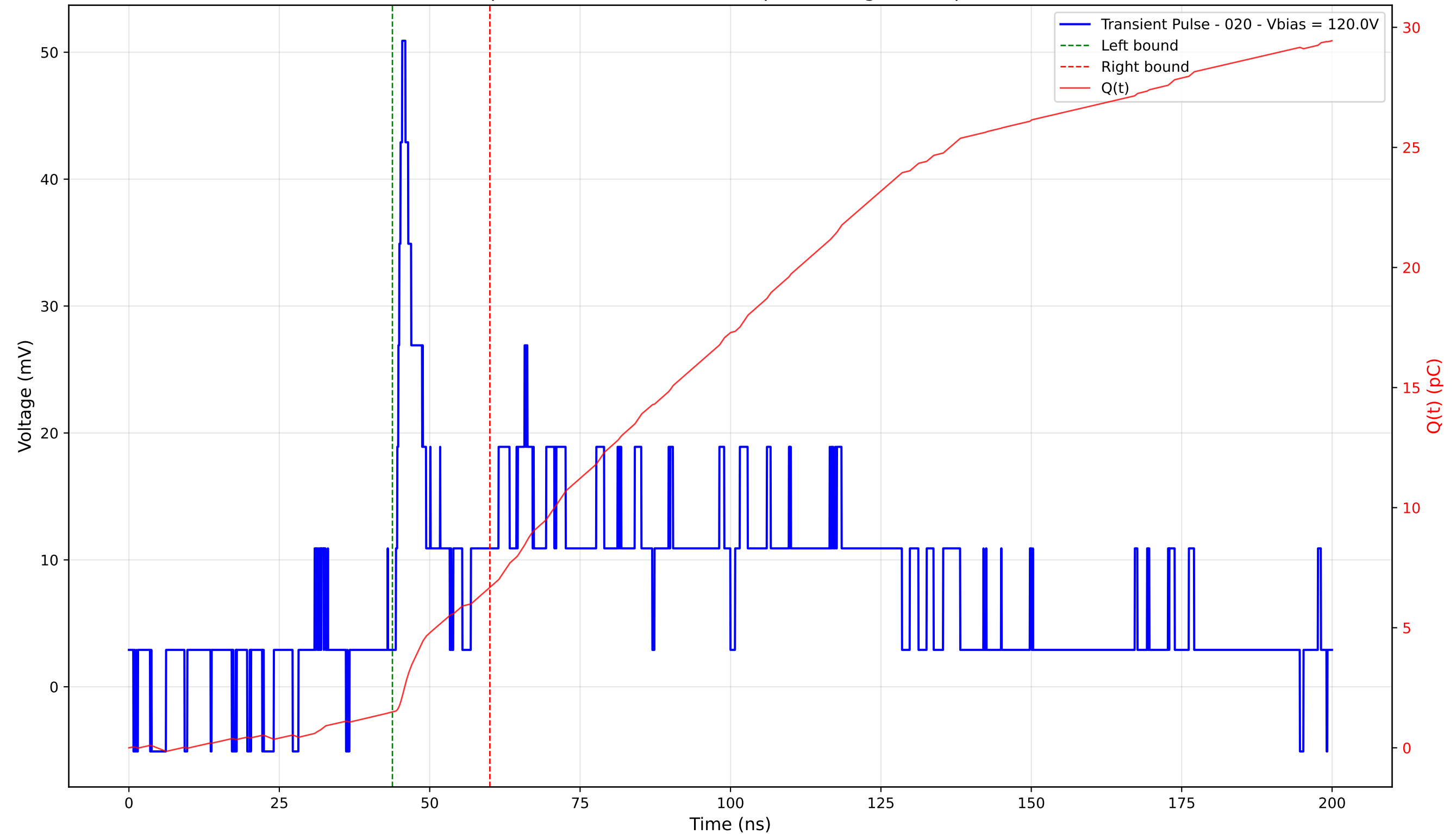
Transient Pulse - Sample: 4003 - Position: 295.0 \mu\text{m} - Charge: 5.18 pC - Rise Time: 1.05 ns
