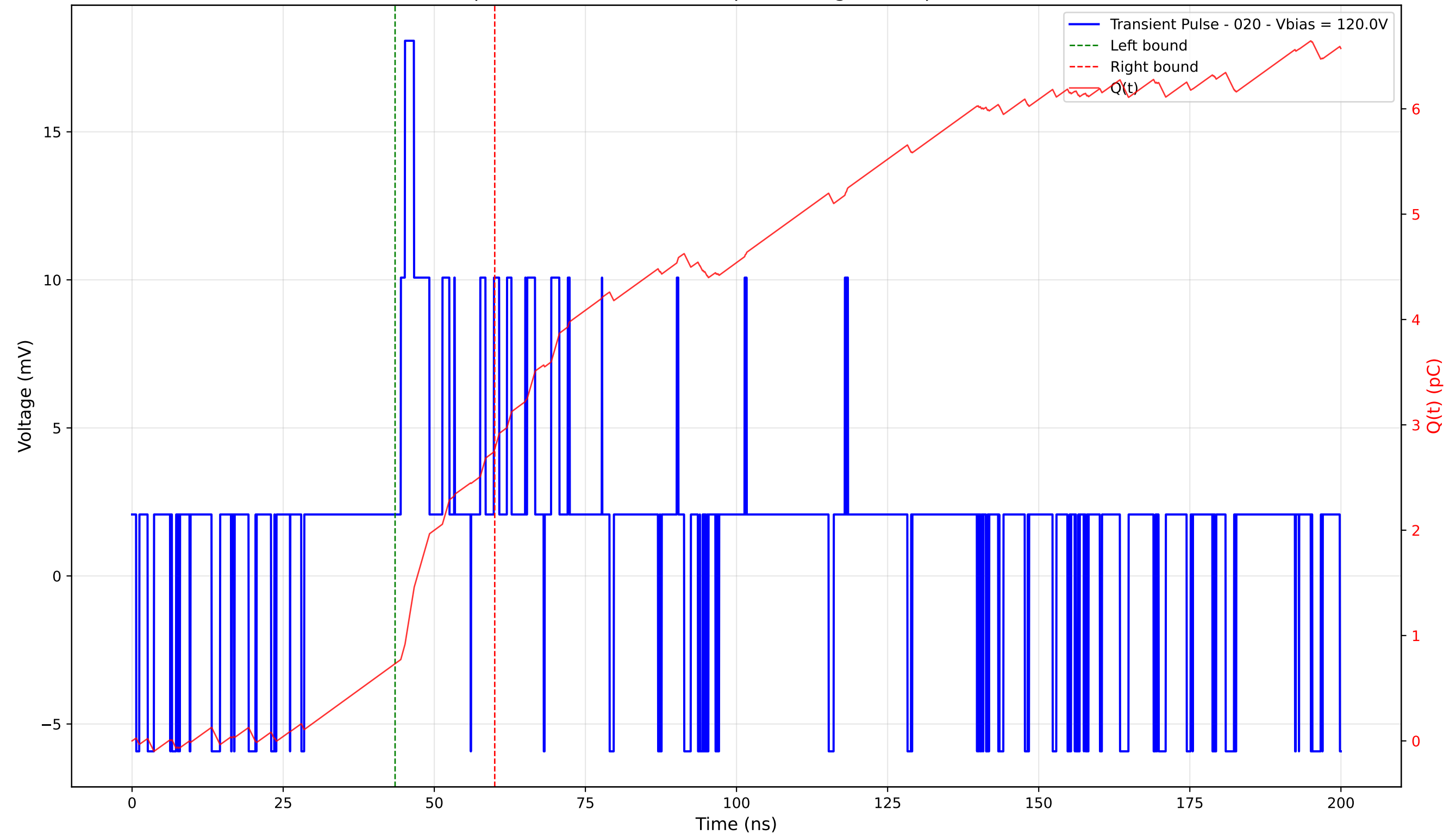
Transient Pulse - Sample: 4003 - Position: 70.0 \mu\text{m} - Charge: 2.04 pC - Rise Time: 0.00 ns (N/A)
