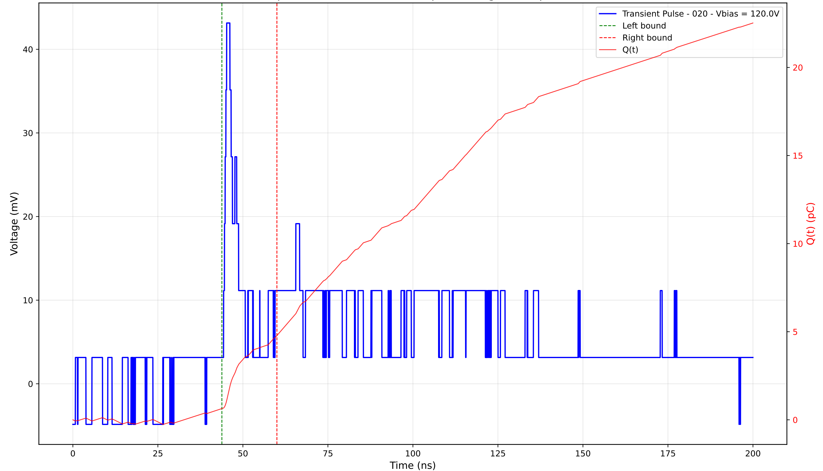
Transient Pulse - Sample: 4003 - Position: 300.0 \mu\text{m} - Charge: 4.15 pC - Rise Time: 0.92 ns
