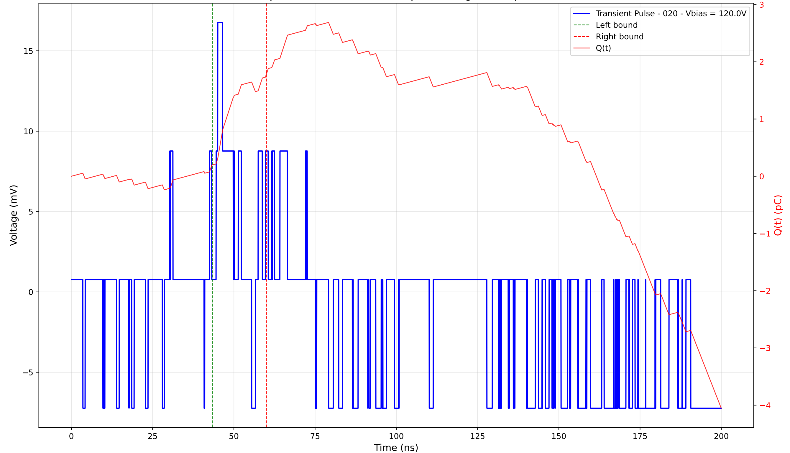
Transient Pulse - Sample: 4003 - Position: 75.0 \mu\text{m} - Charge: 1.58 pC - Rise Time: 0.52 ns
