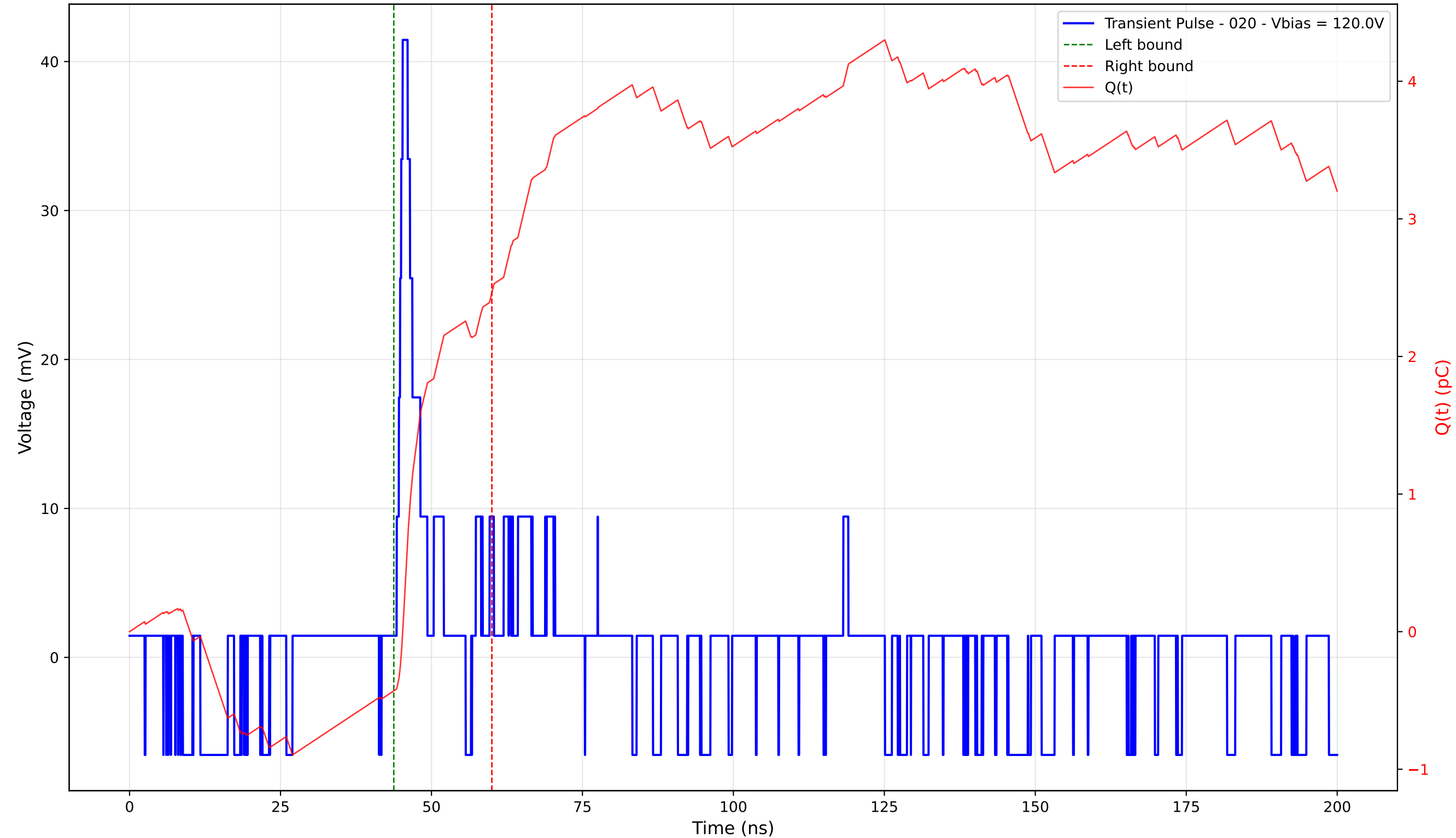
Transient Pulse - Sample: 4003 - Position: 400.0 \mu\text{m} - Charge: 2.90 pC - Rise Time: 0.99 ns
