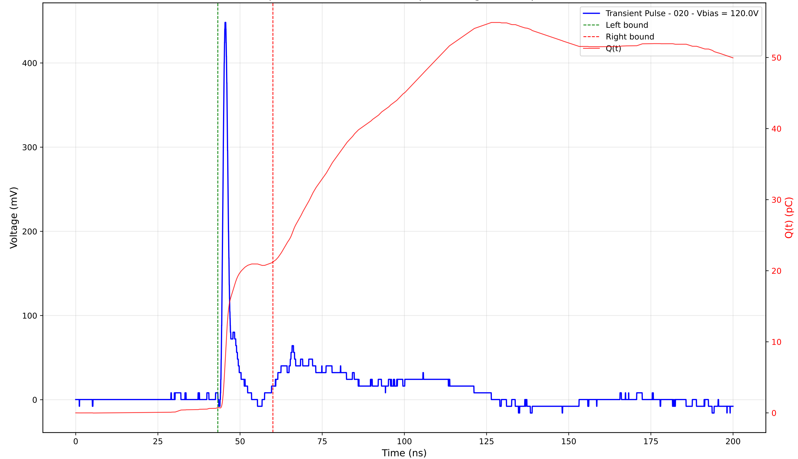
Transient Pulse - Sample: 4003 - Position: 145.0 \mu\text{m} - Charge: 20.49 pC - Rise Time: 0.96 ns
