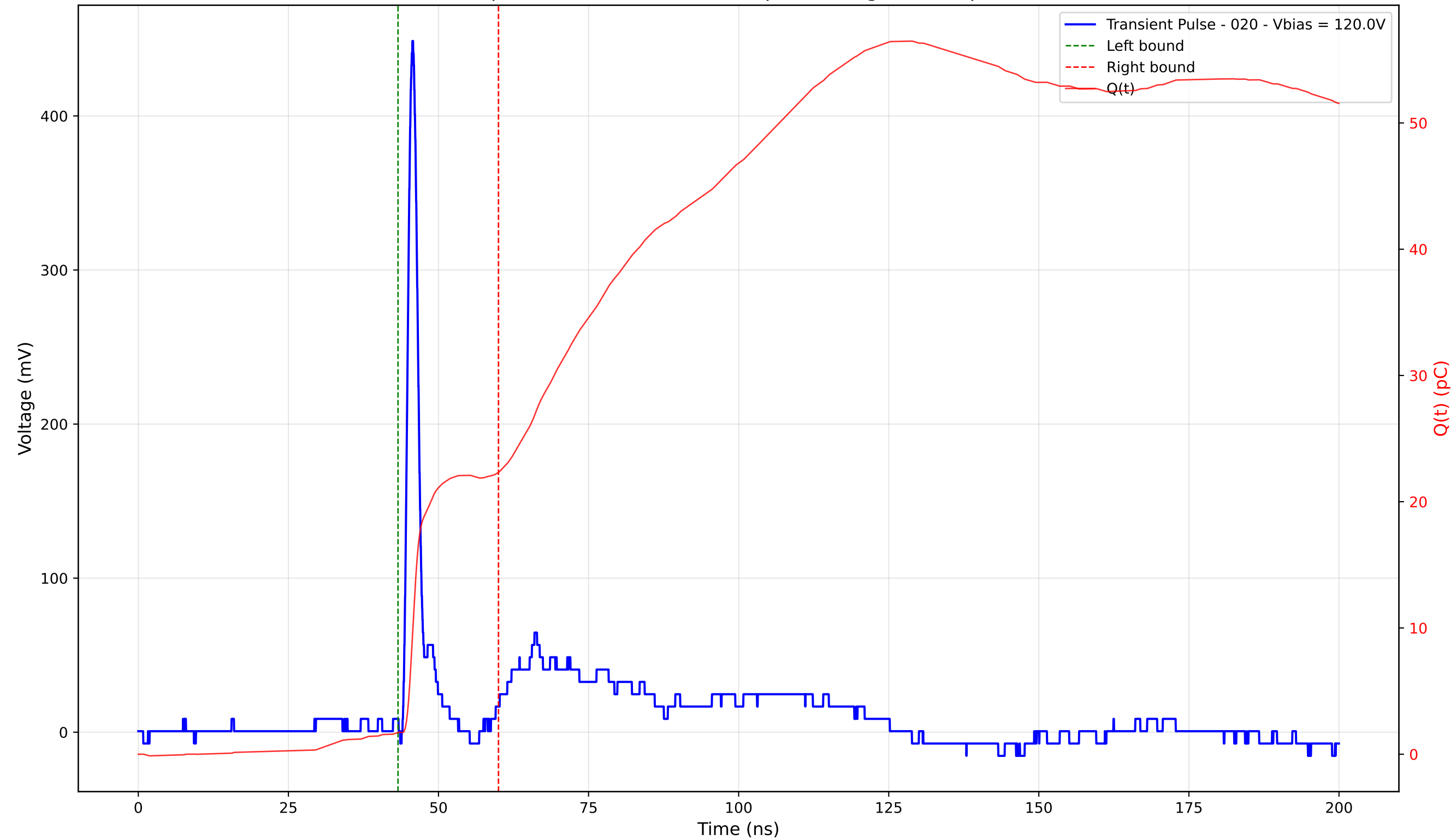
Transient Pulse - Sample: 4003 - Position: 175.0 \mu\text{m} - Charge: 20.60 pC - Rise Time: 1.05 ns
