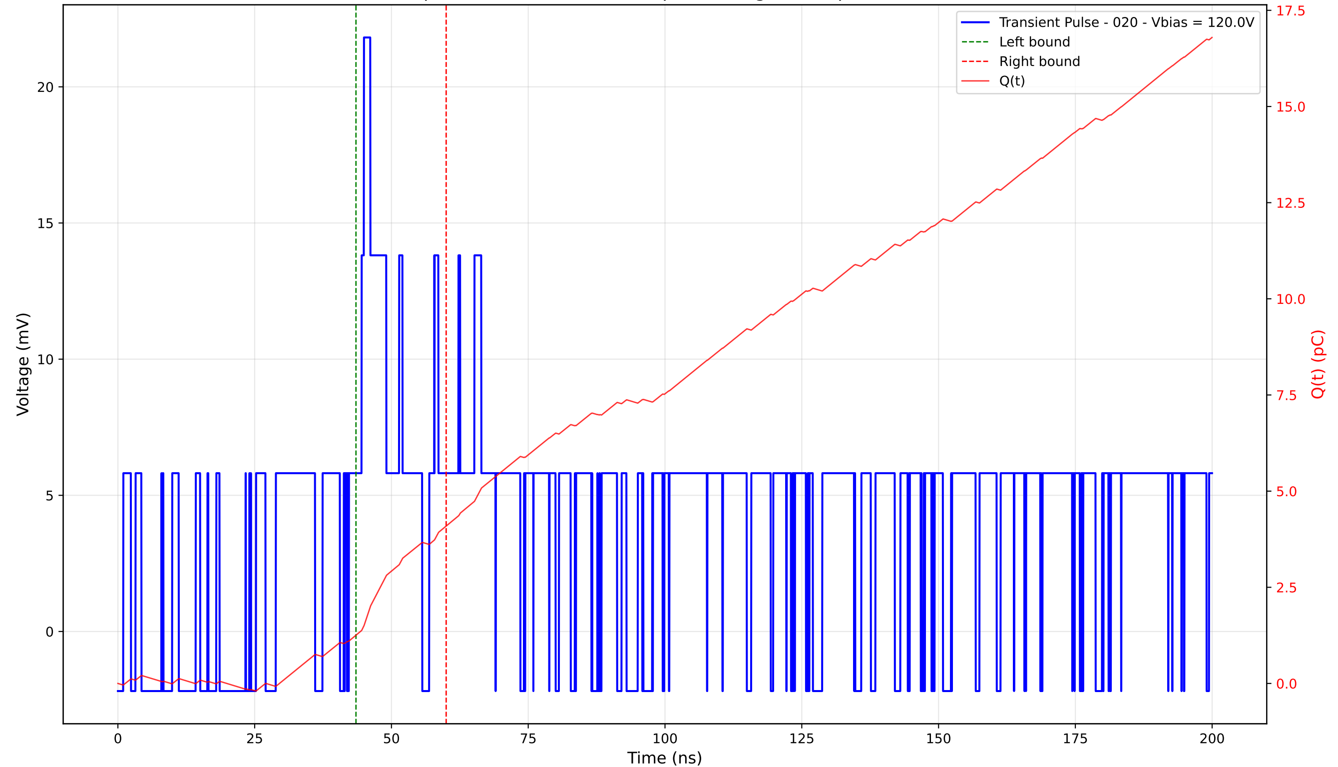
Transient Pulse - Sample: 4003 - Position: 20.0 \mu\text{m} - Charge: 2.84 pC - Rise Time: 0.00 ns (N/A)
