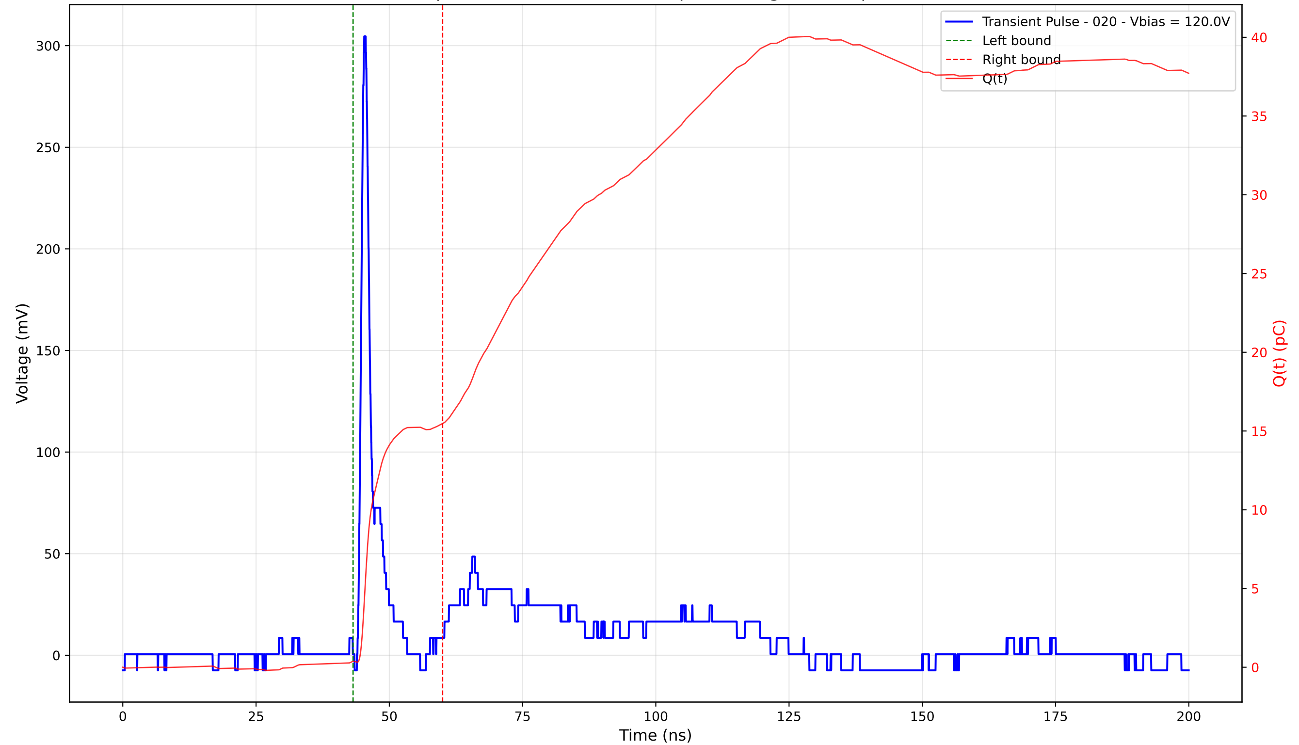
Transient Pulse - Sample: 4003 - Position: 110.0 \mu\text{m} - Charge: 15.09 pC - Rise Time: 0.89 ns
