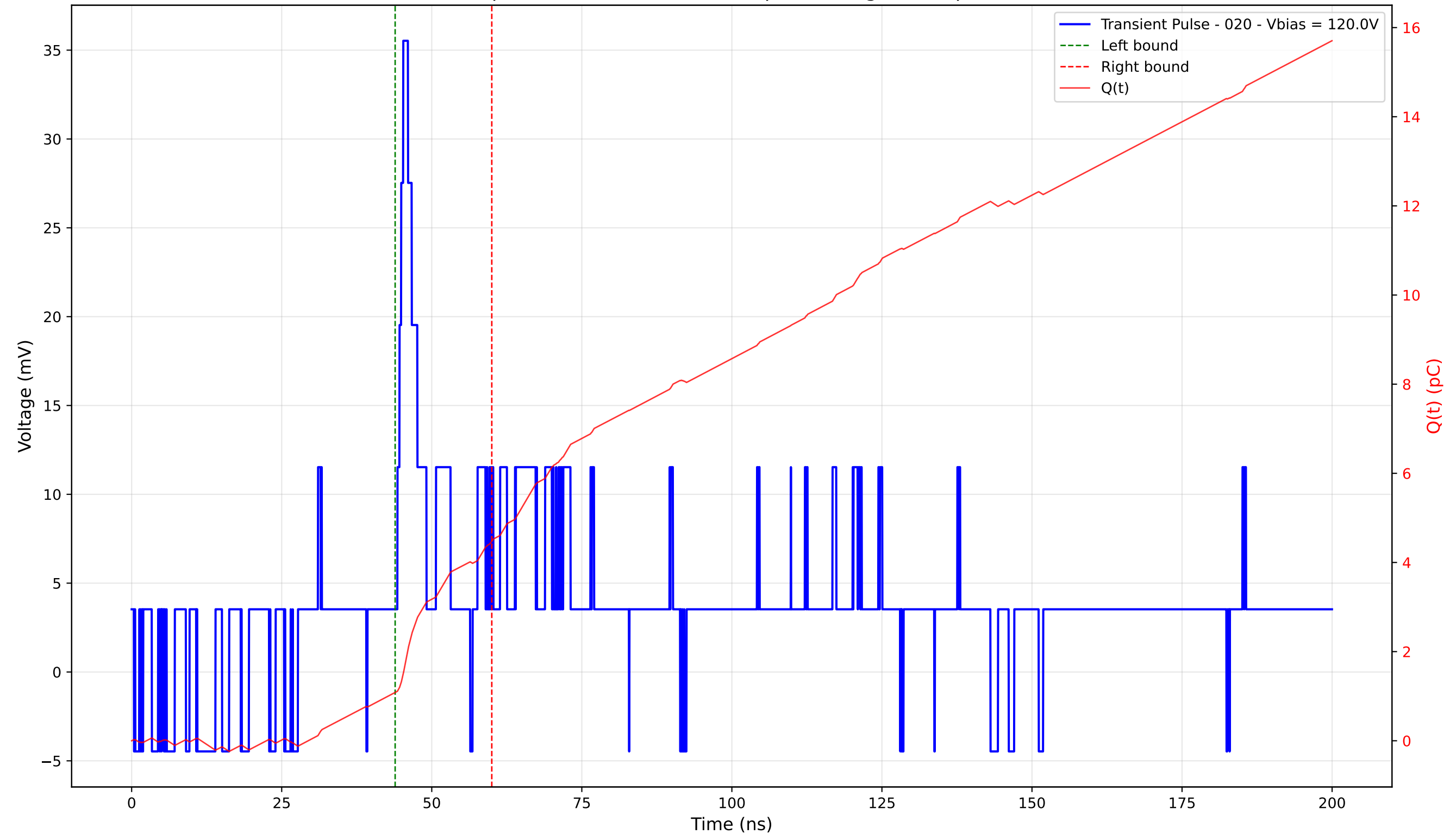
Transient Pulse - Sample: 4003 - Position: 360.0 \mu\text{m} - Charge: 3.40 pC - Rise Time: 0.98 ns
