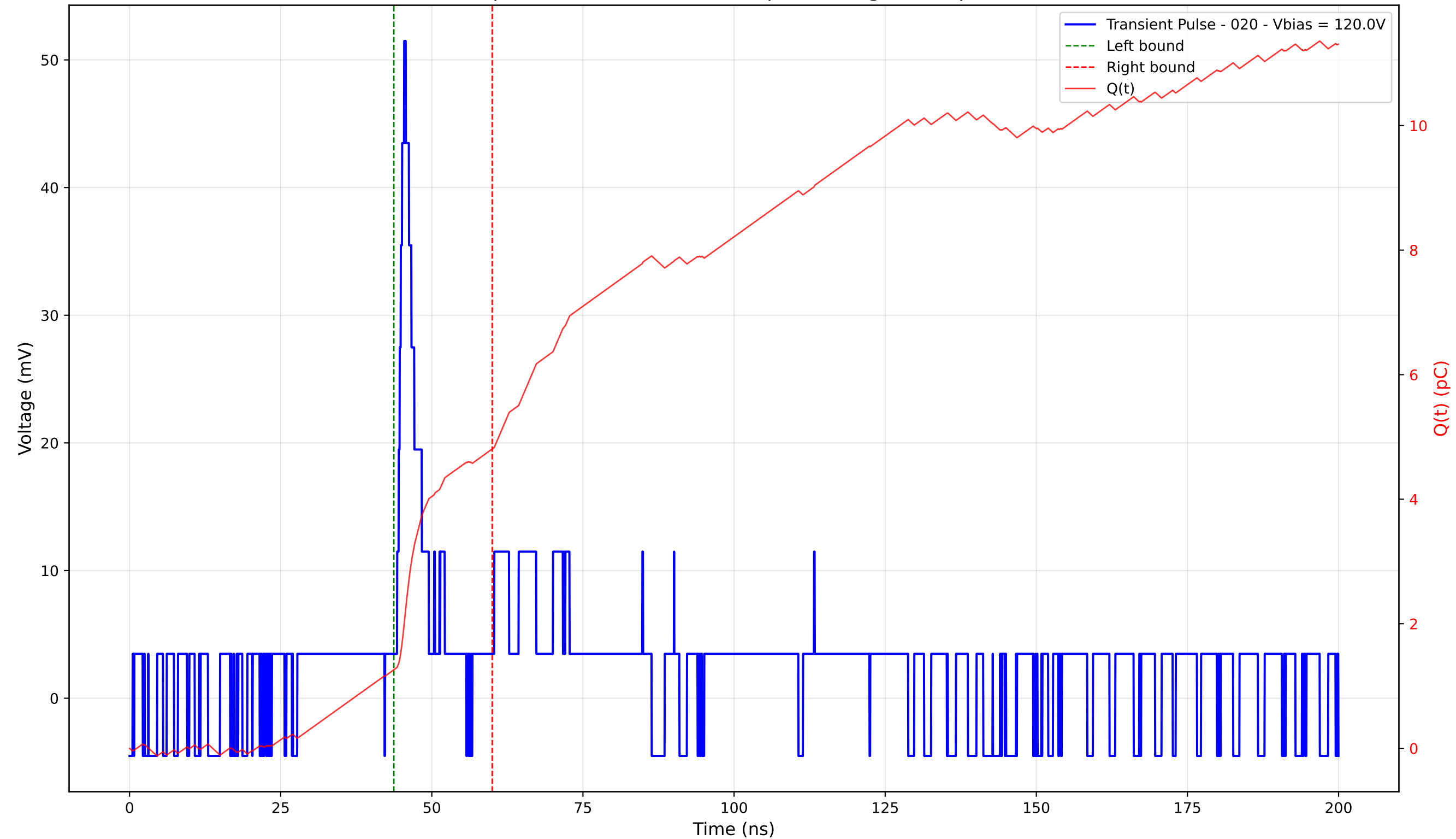
Transient Pulse - Sample: 4003 - Position: 390.0 \mu\text{m} - Charge: 3.55 pC - Rise Time: 1.18 ns
