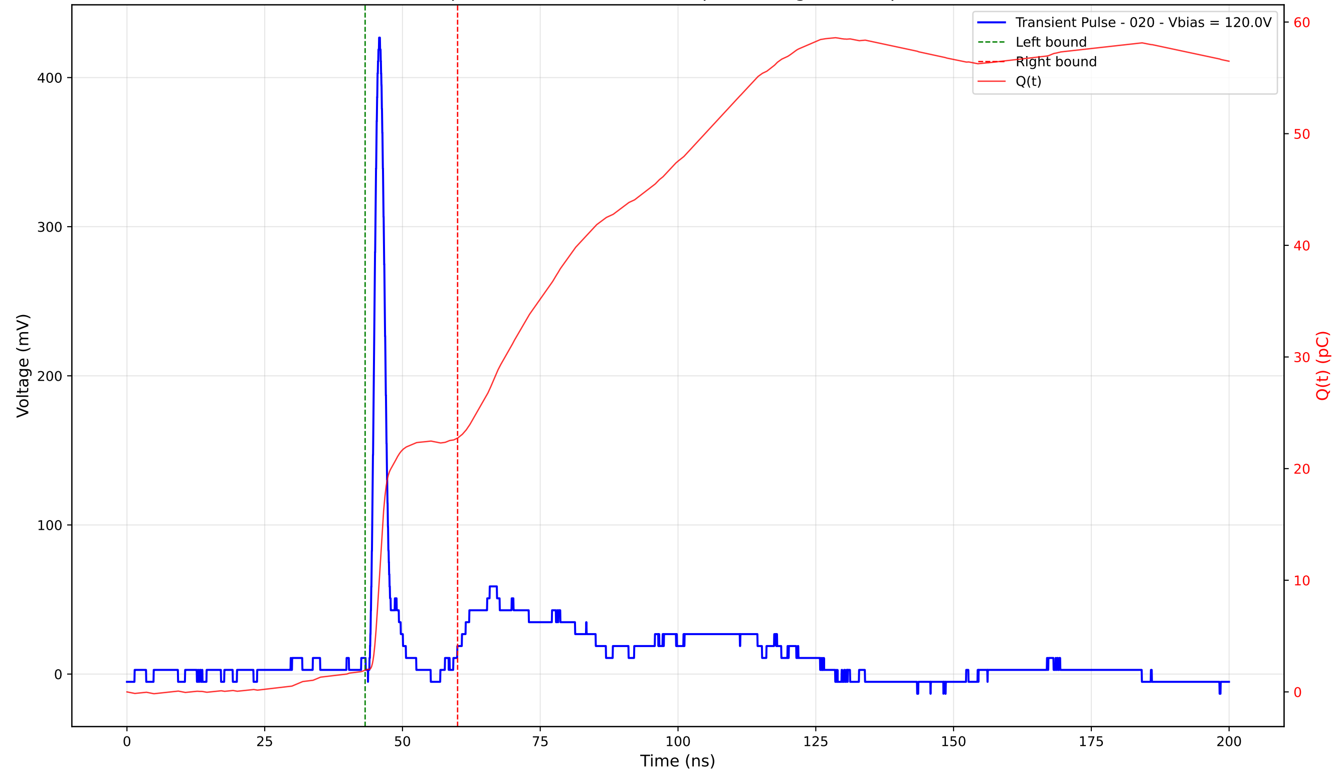
Transient Pulse - Sample: 4003 - Position: 190.0 \mu\text{m} - Charge: 20.77 pC - Rise Time: 1.14 ns
