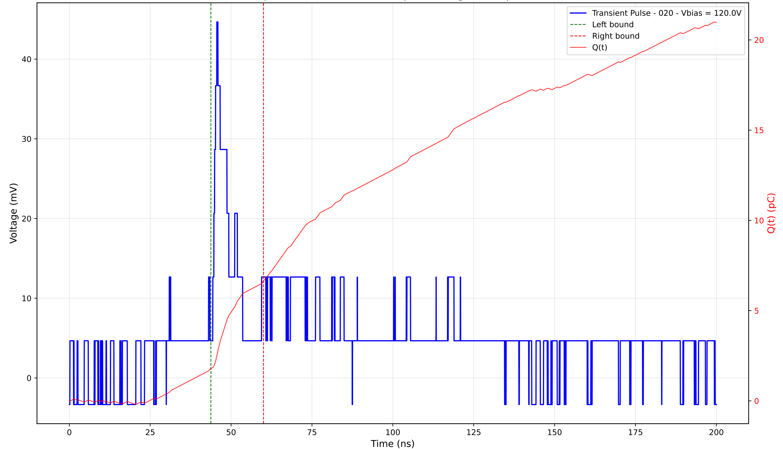
Transient Pulse - Sample: 4003 - Position: 55.0 \mu\text{m} - Charge: 4.85 pC - Rise Time: 15.58 ns
