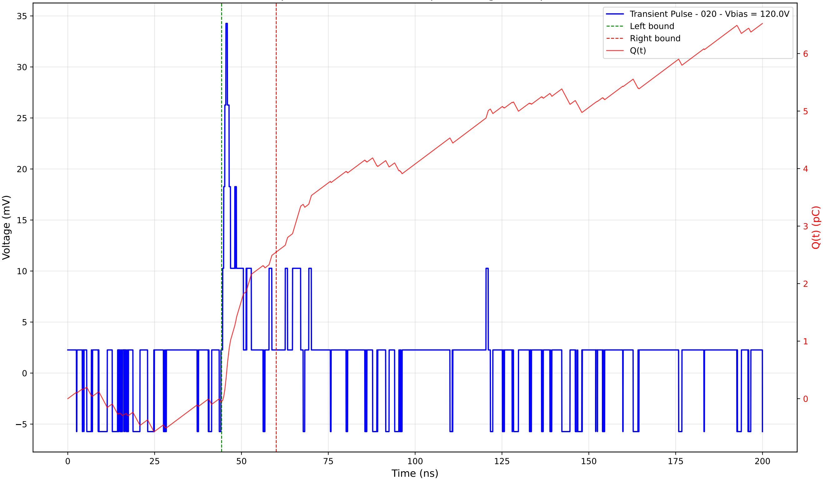
Transient Pulse - Sample: 4003 - Position: 35.0 \mu\text{m} - Charge: 2.59 pC - Rise Time: 0.96 ns
