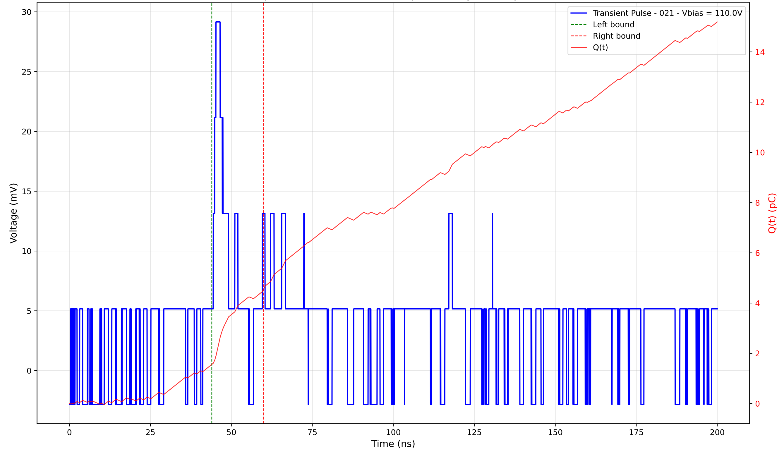
Transient Pulse - Sample: 4003 - Position: 360.0 \mu\text{m} - Charge: 3.02 pC - Rise Time: 4.06 ns
