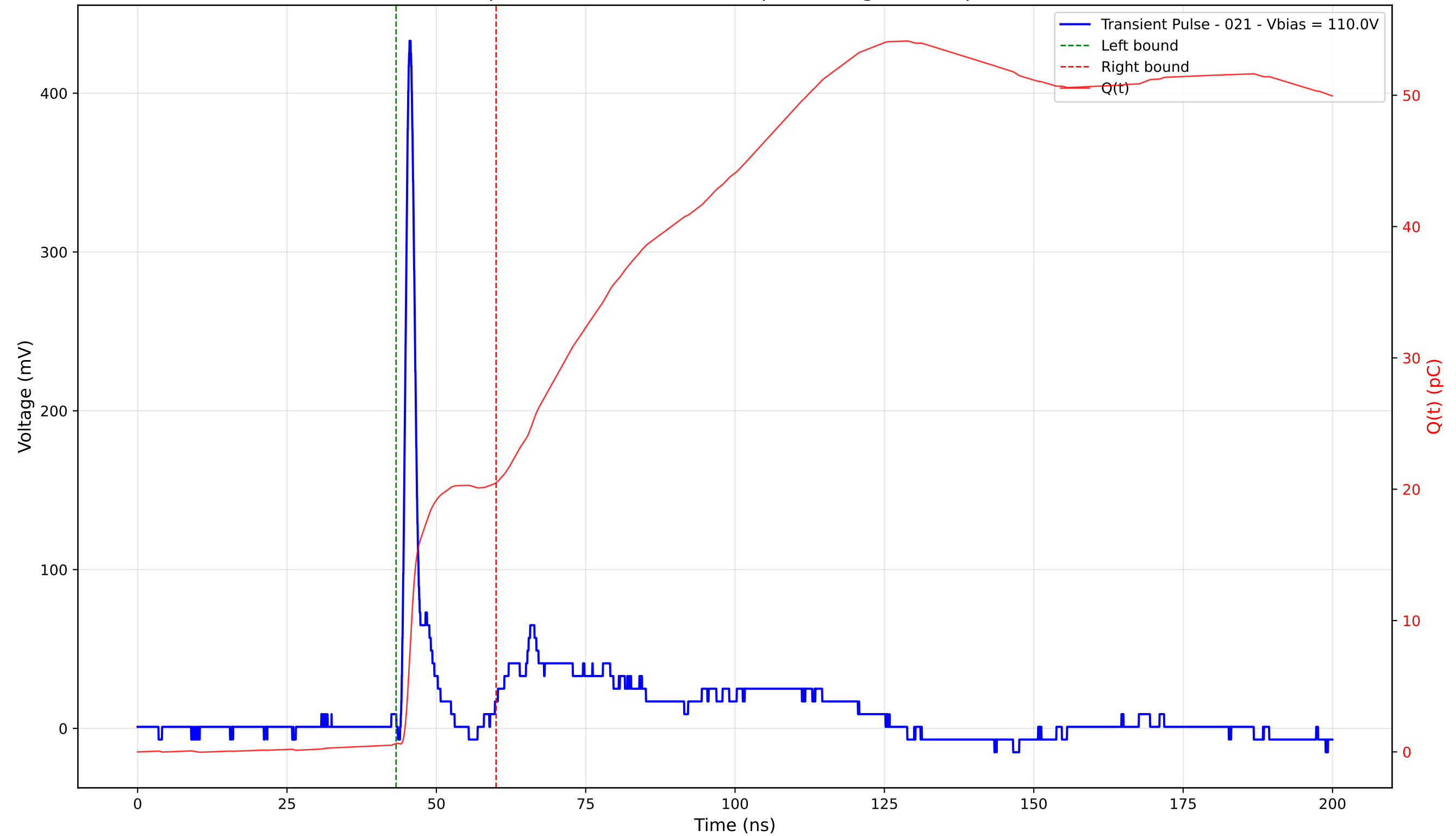
Transient Pulse - Sample: 4003 - Position: 155.0 \mu\text{m} - Charge: 19.85 pC - Rise Time: 0.97 ns
