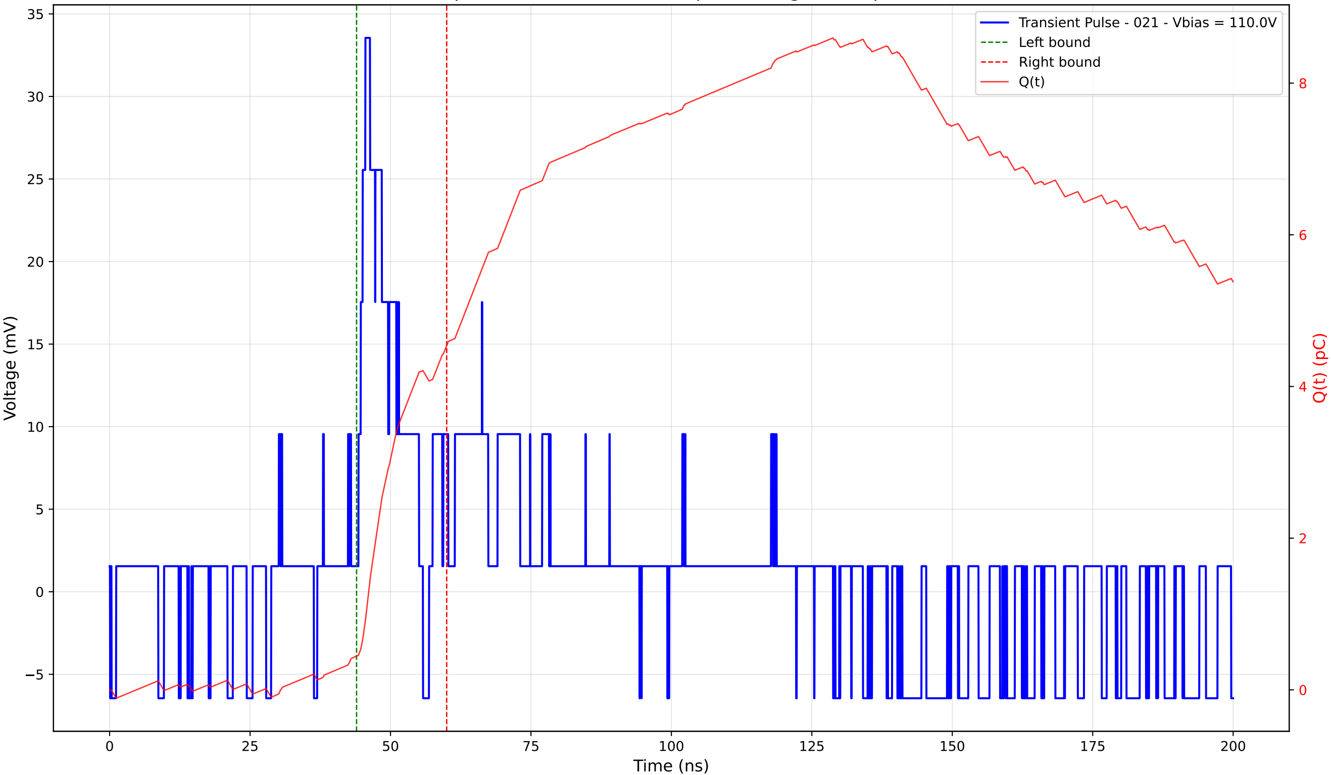
Transient Pulse - Sample: 4003 - Position: 60.0 \mu\text{m} - Charge: 4.10 pC - Rise Time: 1.24 ns
