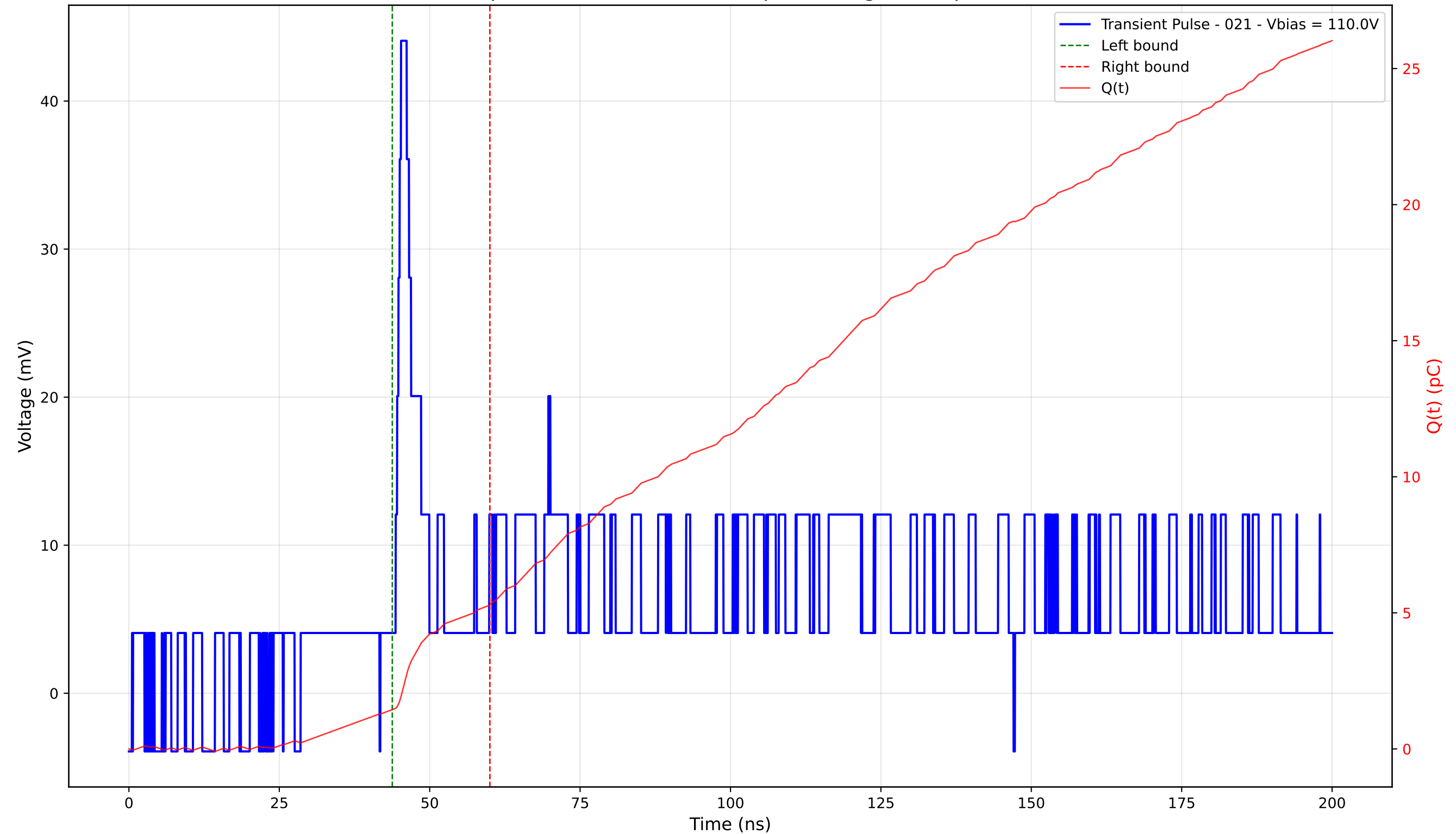
Transient Pulse - Sample: 4003 - Position: 300.0 \mu\text{m} - Charge: 3.85 pC - Rise Time: 0.90 ns
