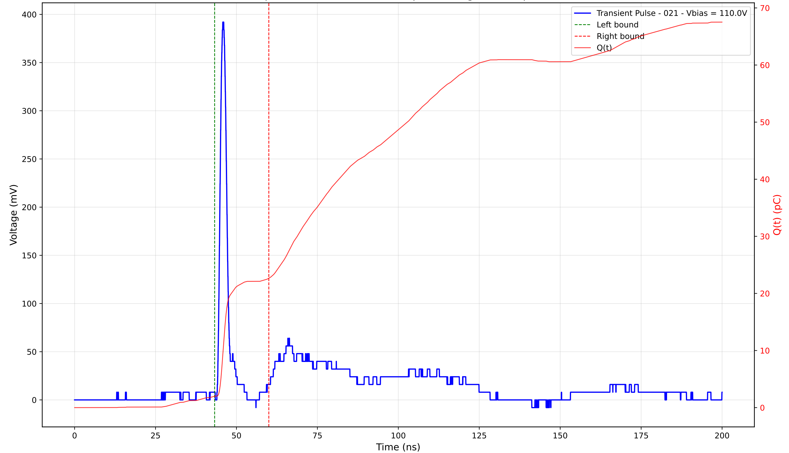
Transient Pulse - Sample: 4003 - Position: 195.0 \mu\text{m} - Charge: 20.67 pC - Rise Time: 1.18 ns
