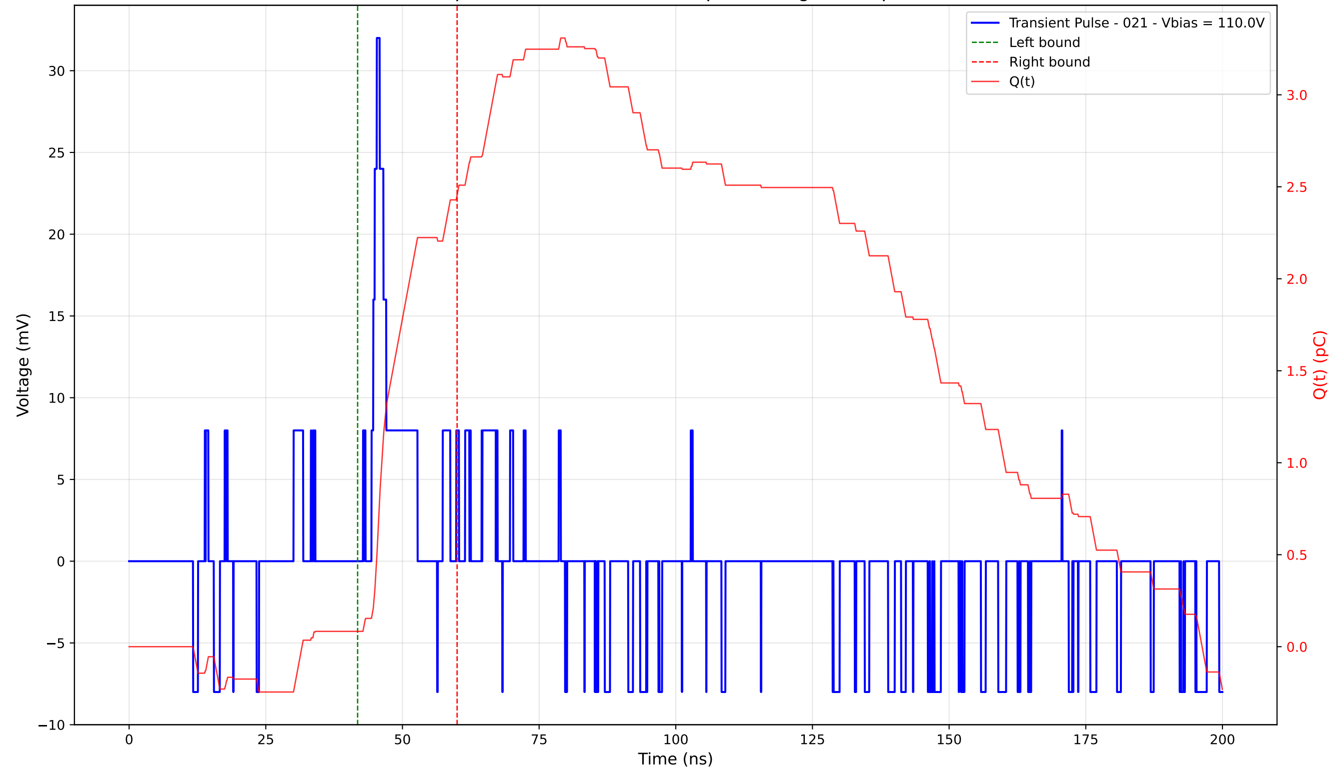
Transient Pulse - Sample: 4003 - Position: 330.0 \mu\text{m} - Charge: 2.37 pC - Rise Time: 0.97 ns
