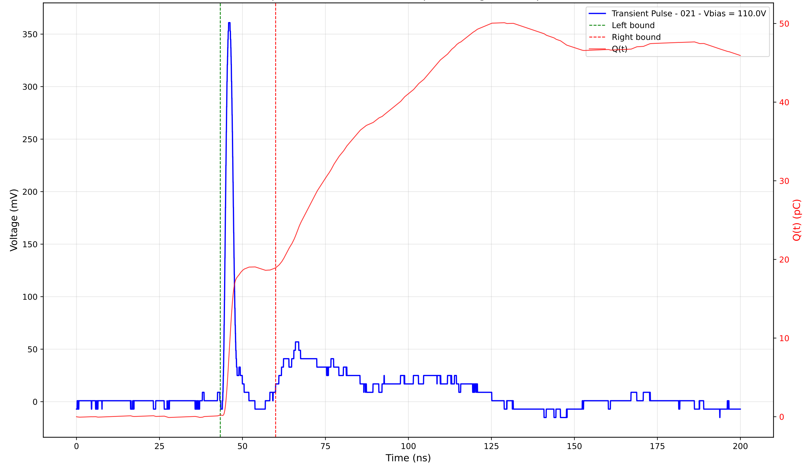
Transient Pulse - Sample: 4003 - Position: 205.0 \mu\text{m} - Charge: 18.72 pC - Rise Time: 1.17 ns
