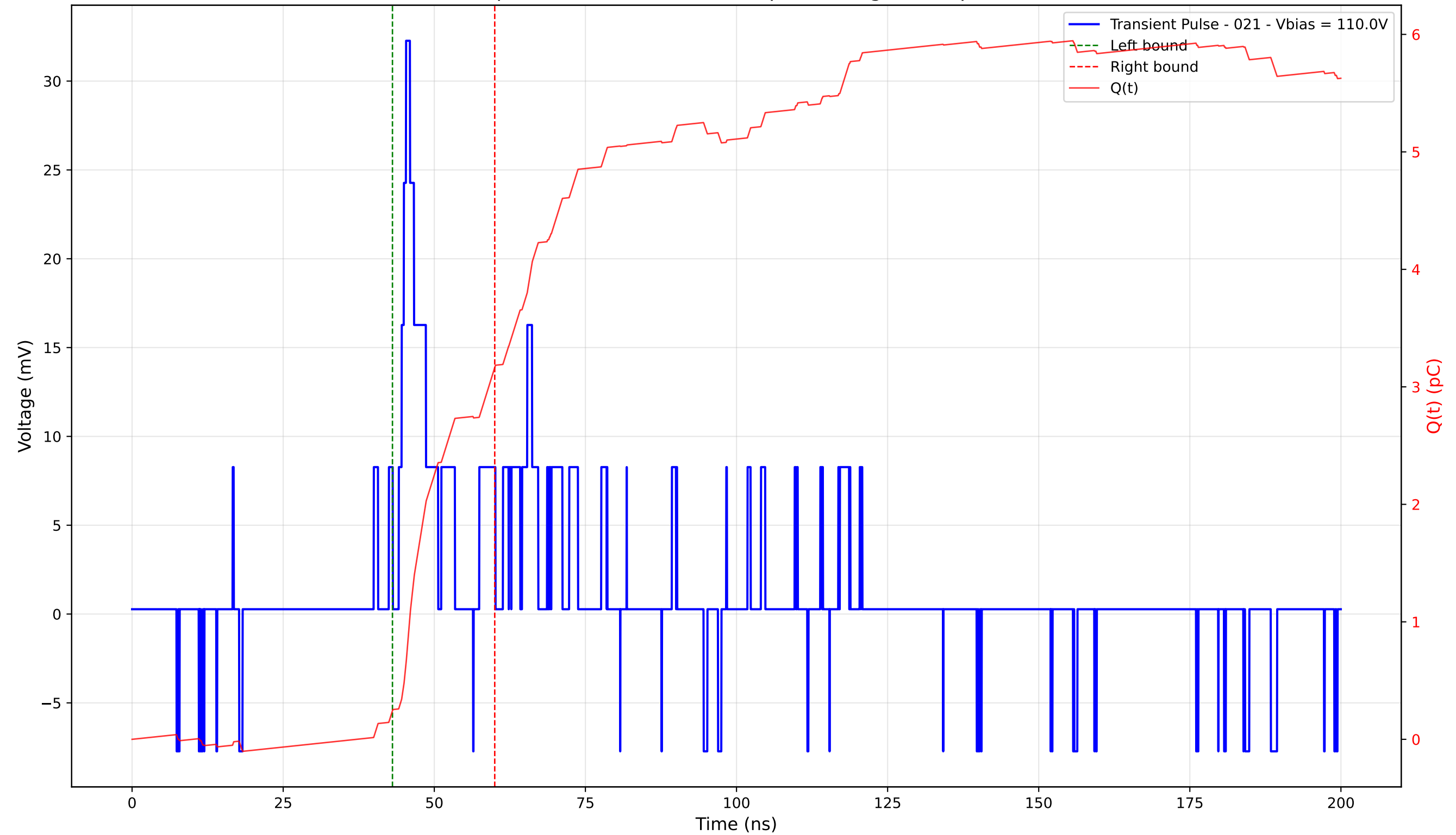
Transient Pulse - Sample: 4003 - Position: 320.0 \mu\text{m} - Charge: 2.92 pC - Rise Time: 1.21 ns
