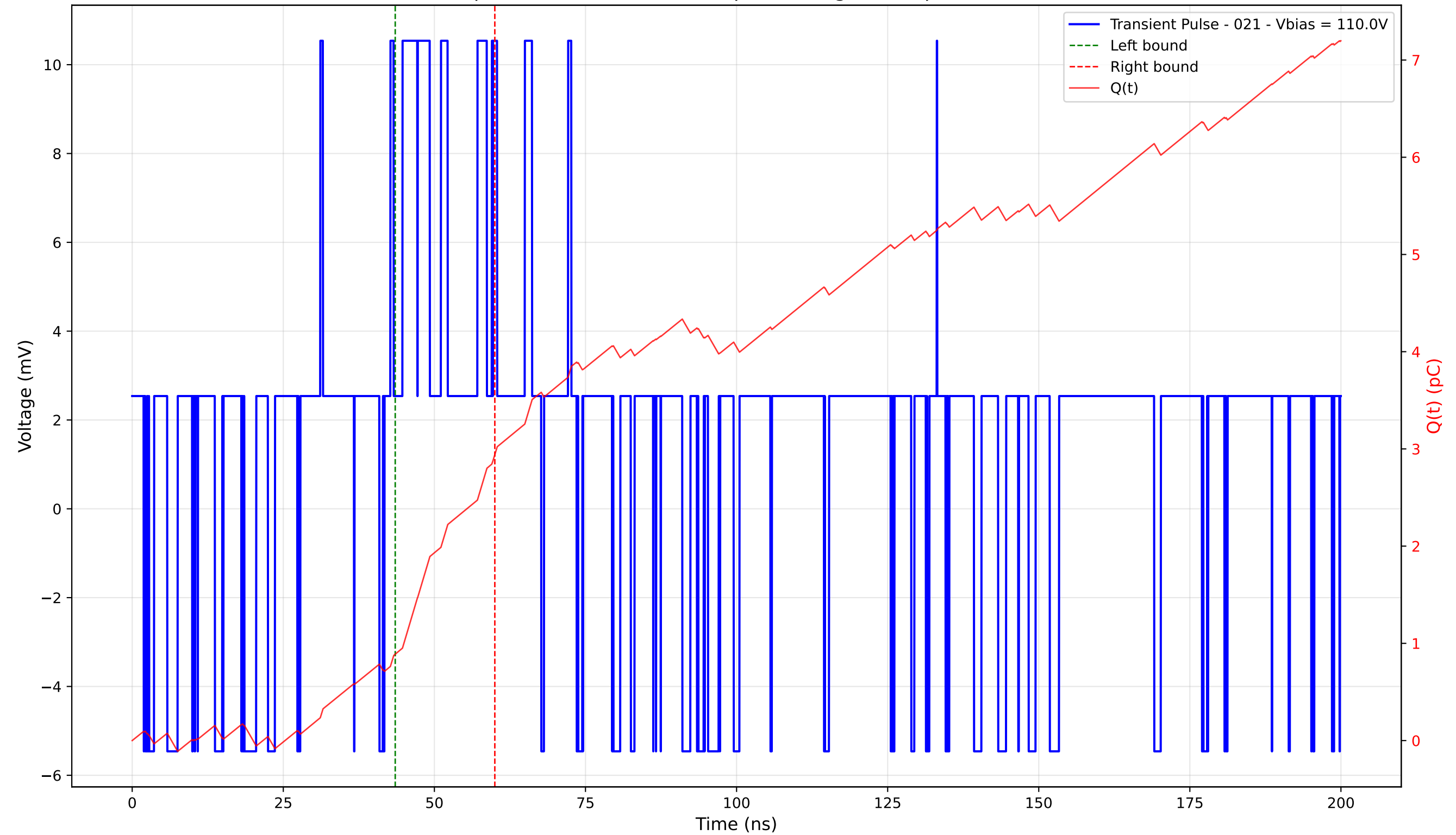
Transient Pulse - Sample: 4003 - Position: 10.0 \mu\text{m} - Charge: 2.05 pC - Rise Time: 0.00 ns (N/A)
