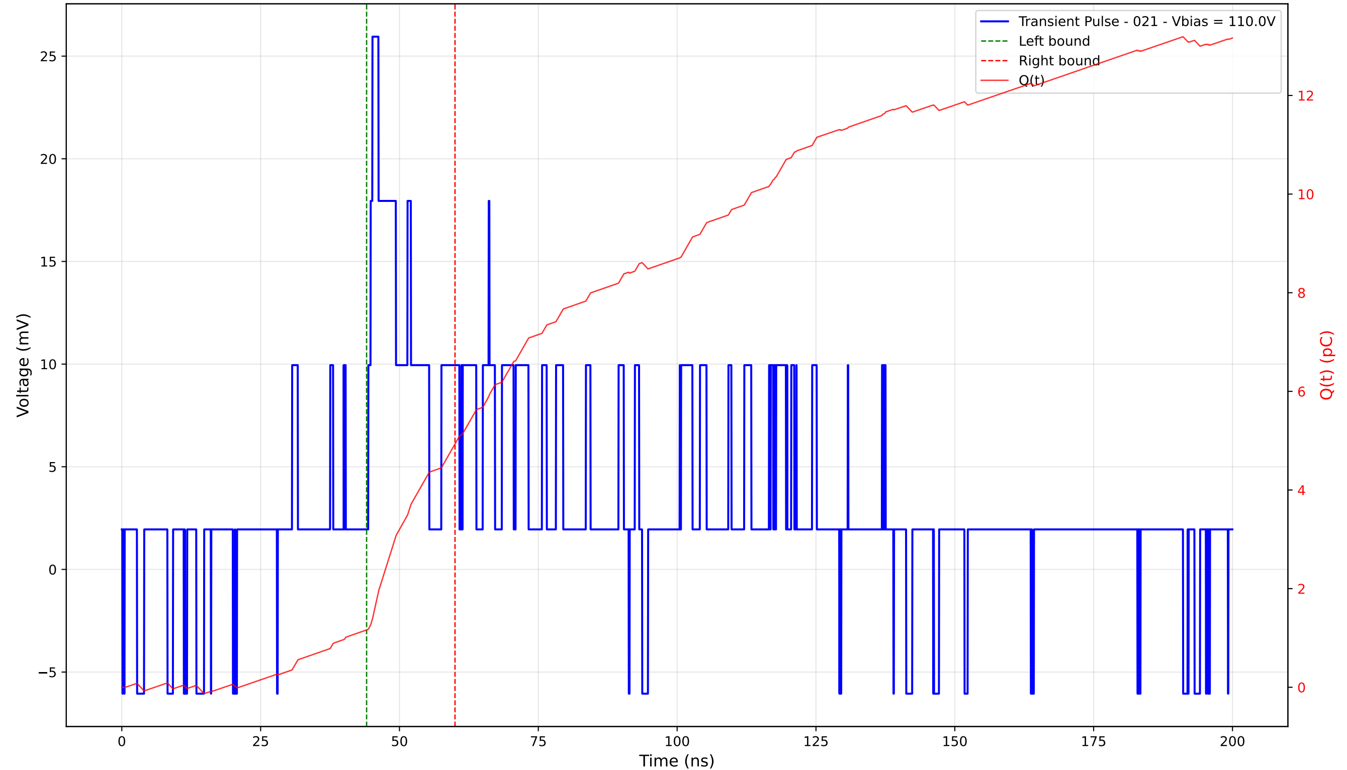
Transient Pulse - Sample: 4003 - Position: 65.0 \mu\text{m} - Charge: 3.78 pC - Rise Time: 0.76 ns
