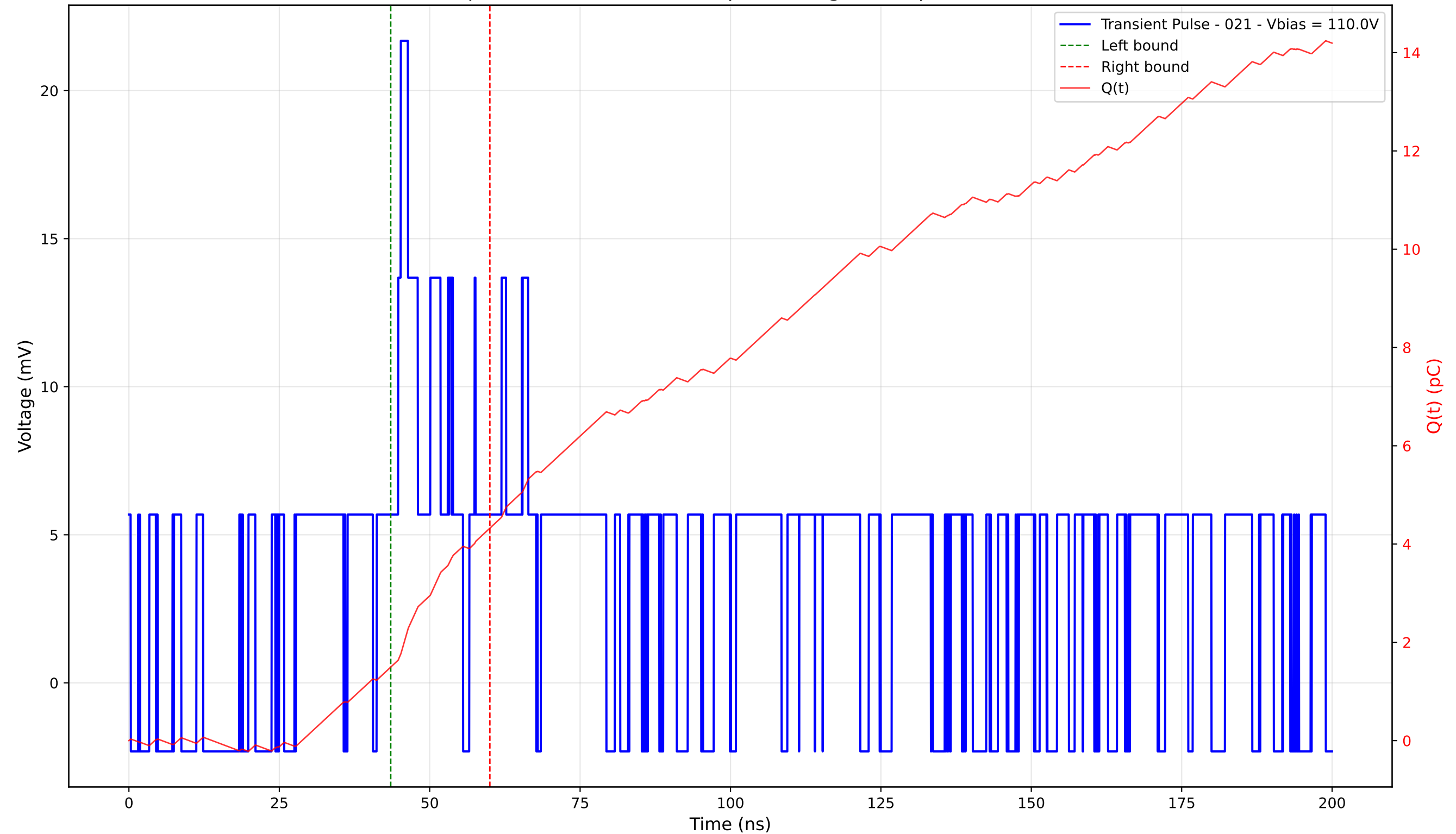
Transient Pulse - Sample: 4003 - Position: 75.0 \mu\text{m} - Charge: 2.82 pC - Rise Time: 0.00 ns (N/A)
