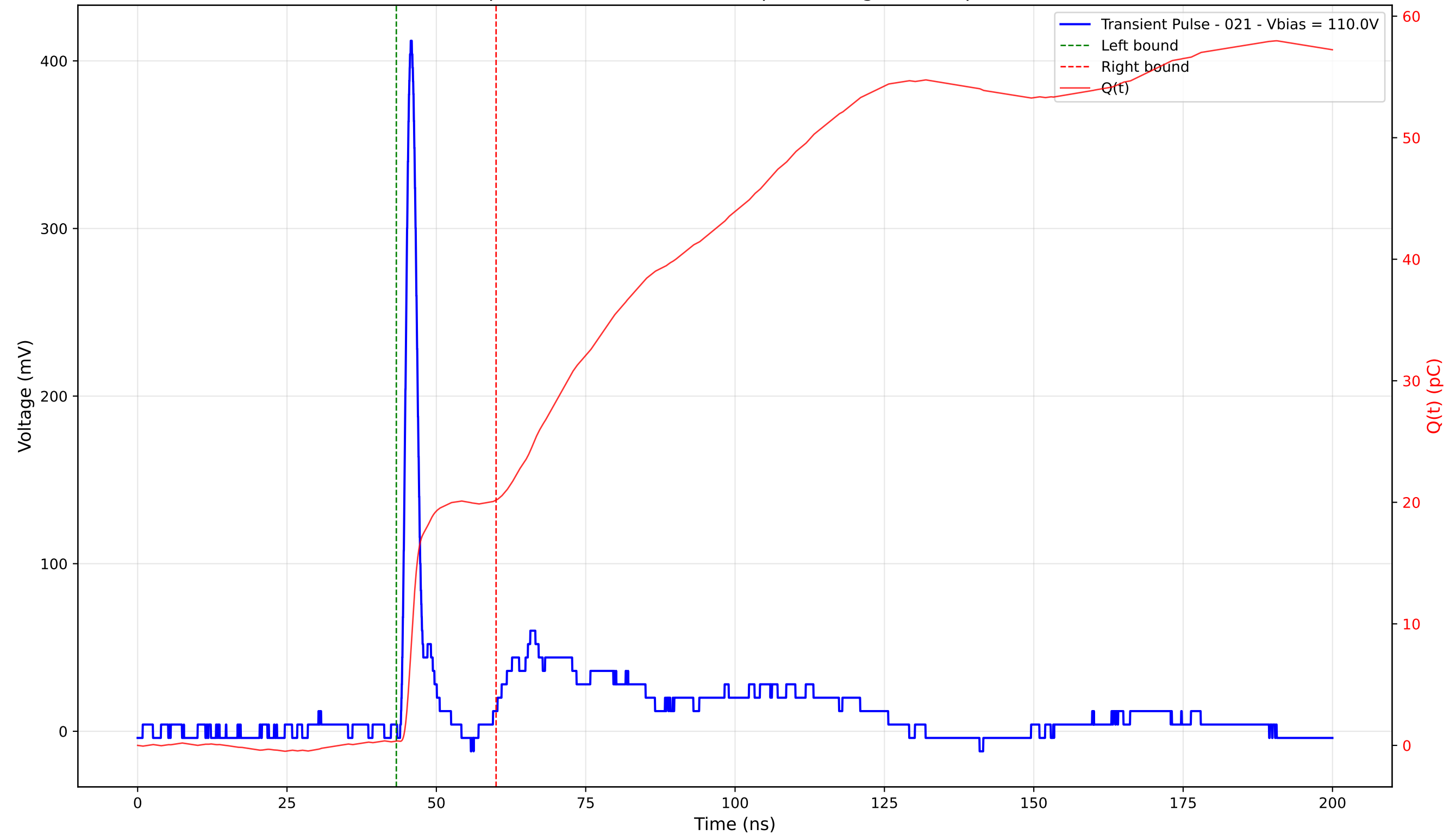
Transient Pulse - Sample: 4003 - Position: 185.0 \mu\text{m} - Charge: 19.82 pC - Rise Time: 1.09 ns
