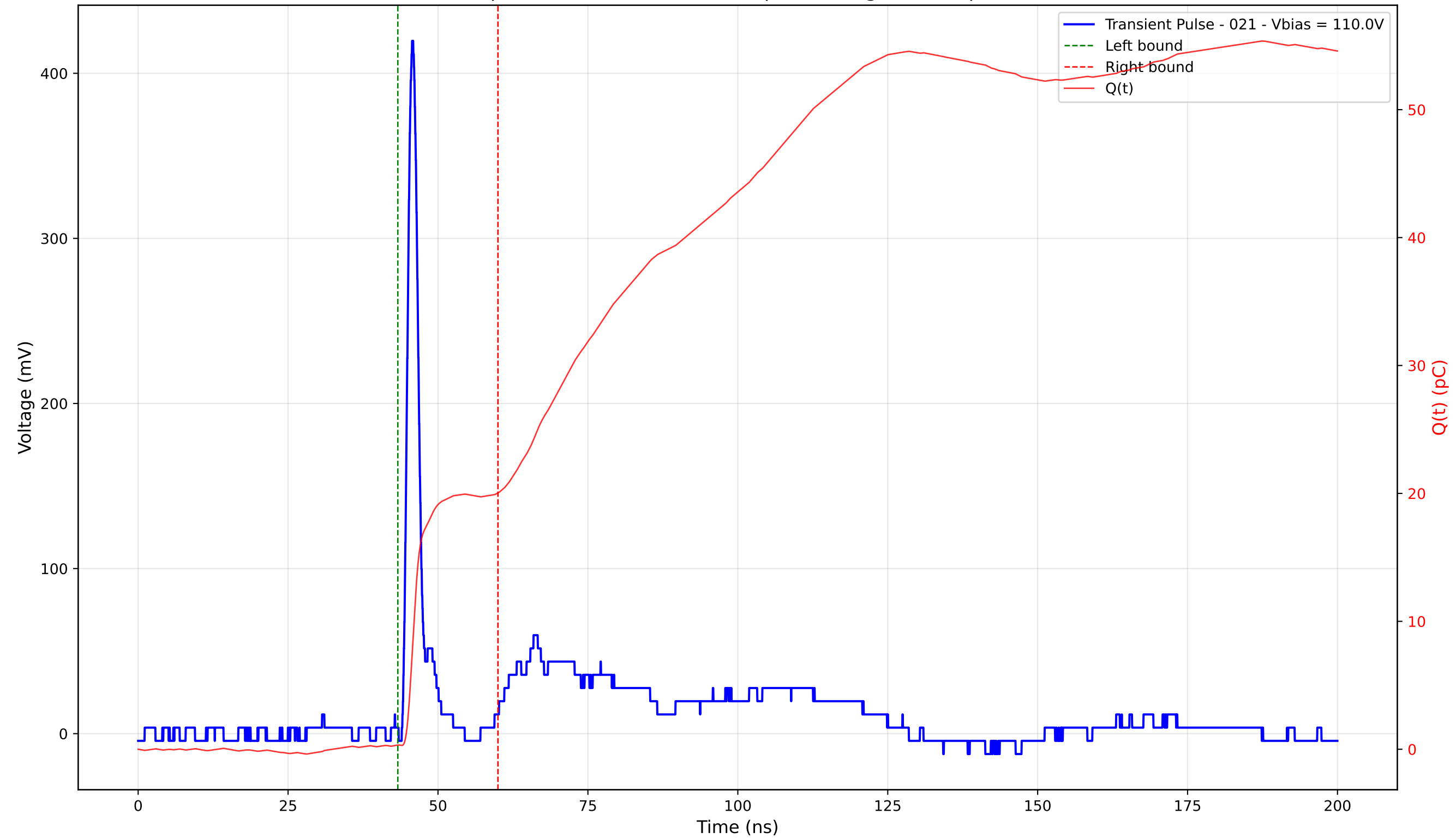
Transient Pulse - Sample: 4003 - Position: 180.0 \mu\text{m} - Charge: 19.70 pC - Rise Time: 1.10 ns
