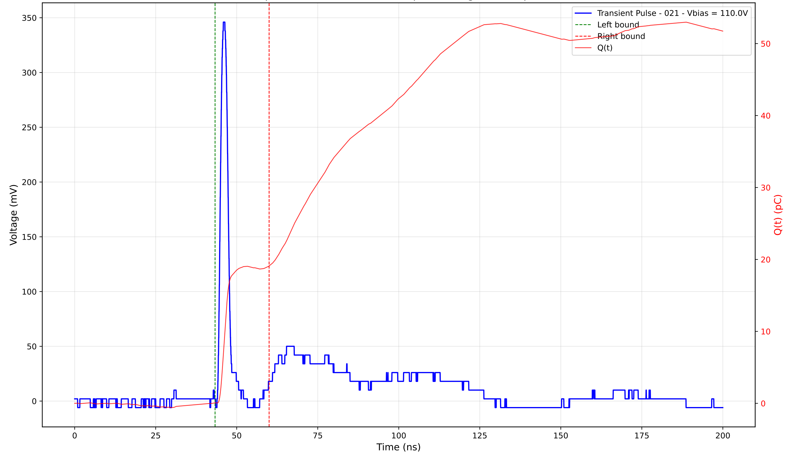
Transient Pulse - Sample: 4003 - Position: 210.0 \mu\text{m} - Charge: 19.02 pC - Rise Time: 1.18 ns
