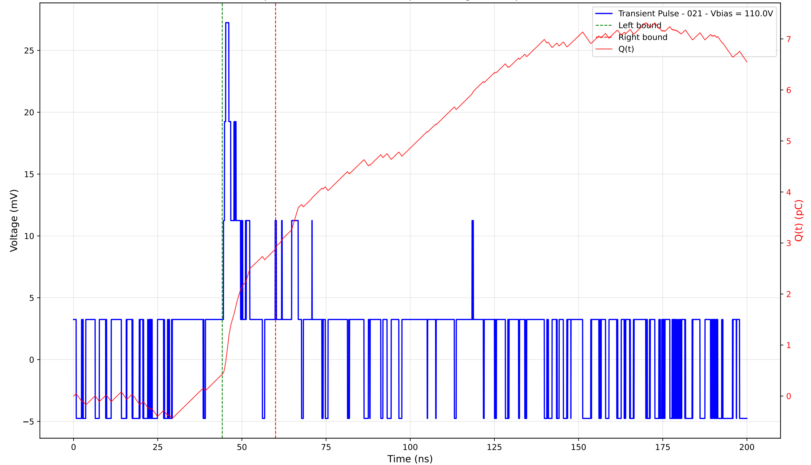
Transient Pulse - Sample: 4003 - Position: 35.0 \mu\text{m} - Charge: 2.47 pC - Rise Time: 0.00 ns (N/A)
