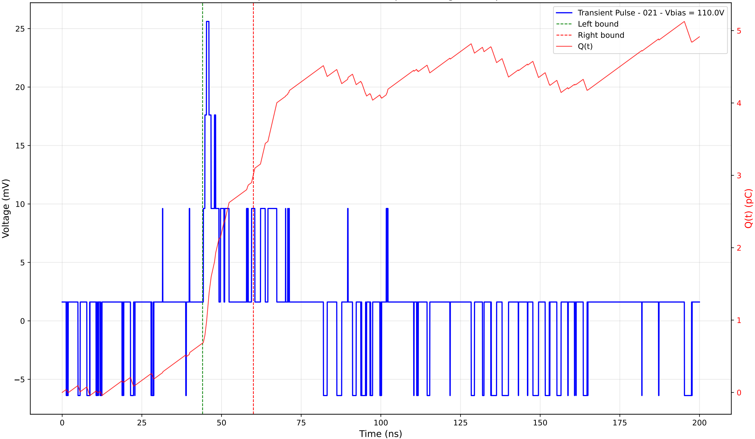
Transient Pulse - Sample: 4003 - Position: 30.0 \mu\text{m} - Charge: 2.33 pC - Rise Time: 1.00 ns
