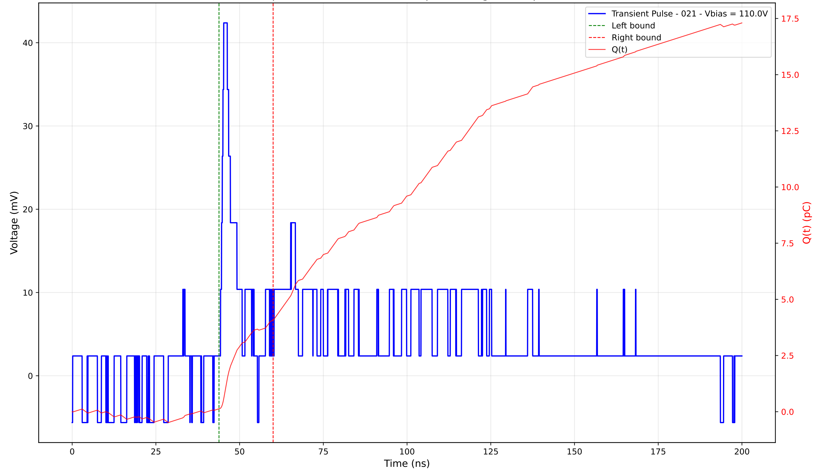
Transient Pulse - Sample: 4003 - Position: 295.0 \mu\text{m} - Charge: 3.96 pC - Rise Time: 0.96 ns
