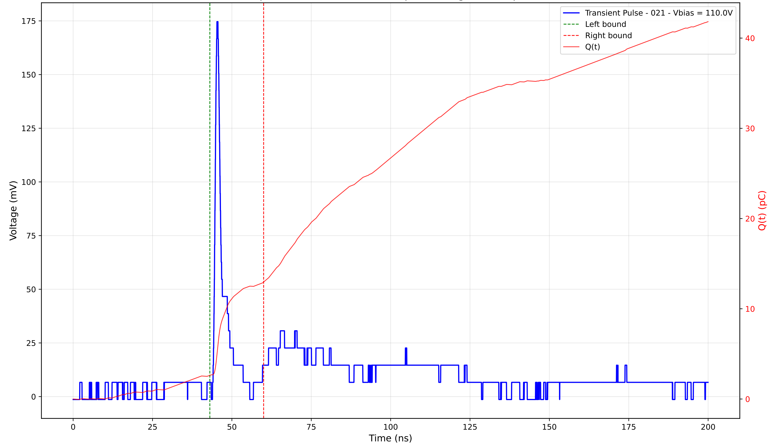
Transient Pulse - Sample: 4003 - Position: 100.0 \mu\text{m} - Charge: 10.34 pC - Rise Time: 0.91 ns
