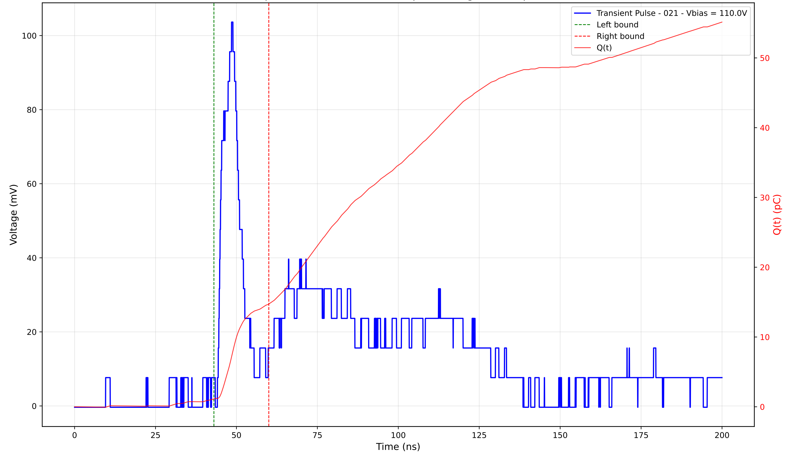
Transient Pulse - Sample: 4003 - Position: 265.0 \mu\text{m} - Charge: 13.59 pC - Rise Time: 3.53 ns
