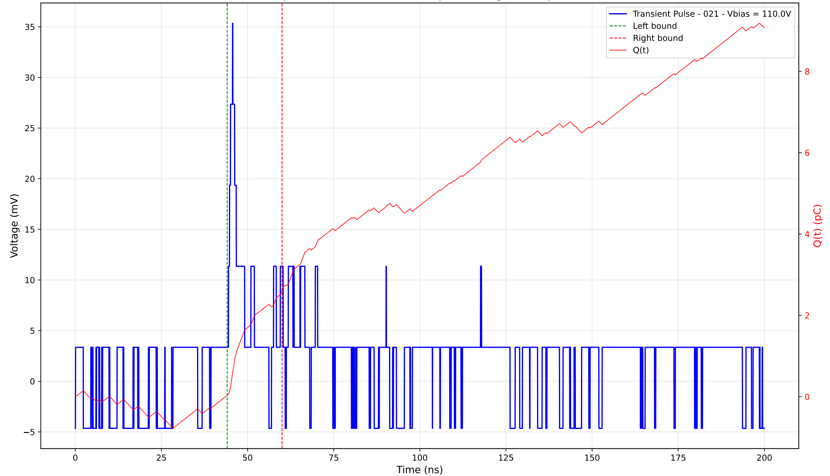
Transient Pulse - Sample: 4003 - Position: 345.0 \mu\text{m} - Charge: 2.59 pC - Rise Time: 1.20 ns
