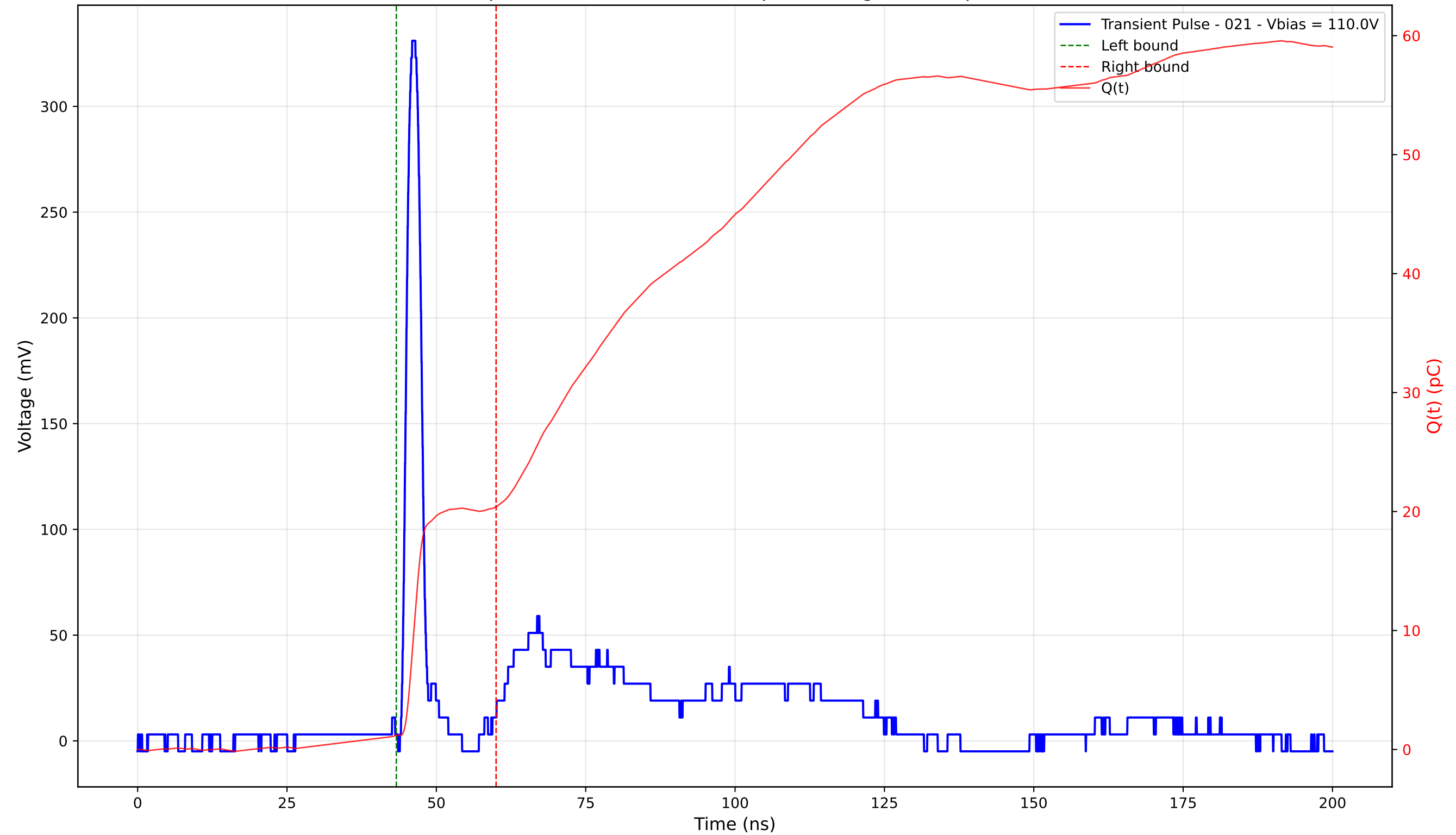
Transient Pulse - Sample: 4003 - Position: 215.0 \mu\text{m} - Charge: 19.19 pC - Rise Time: 1.20 ns
