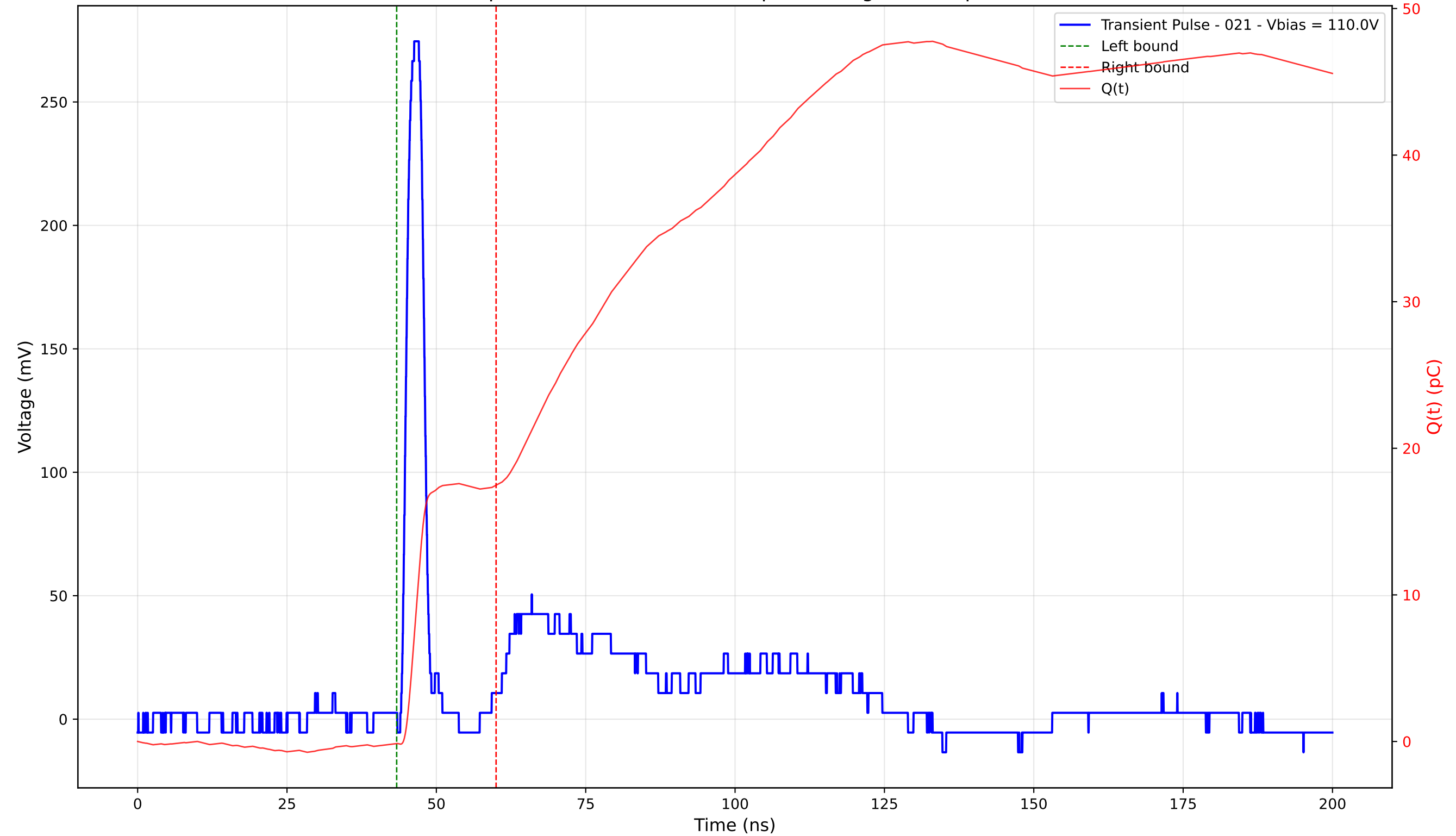
Transient Pulse - Sample: 4003 - Position: 230.0 \mu\text{m} - Charge: 17.62 pC - Rise Time: 1.32 ns
