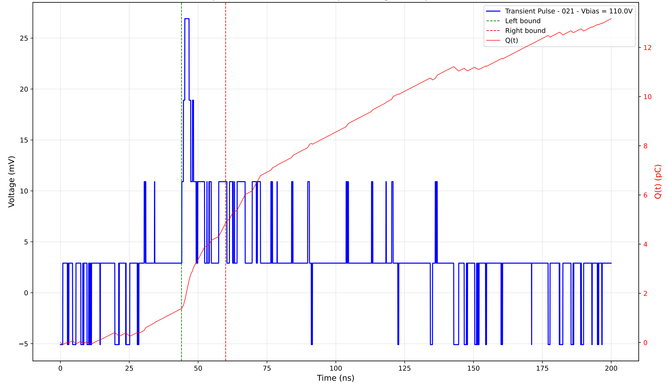
Transient Pulse - Sample: 4003 - Position: 350.0 \mu\text{m} - Charge: 3.48 pC - Rise Time: 0.00 ns (N/A)
