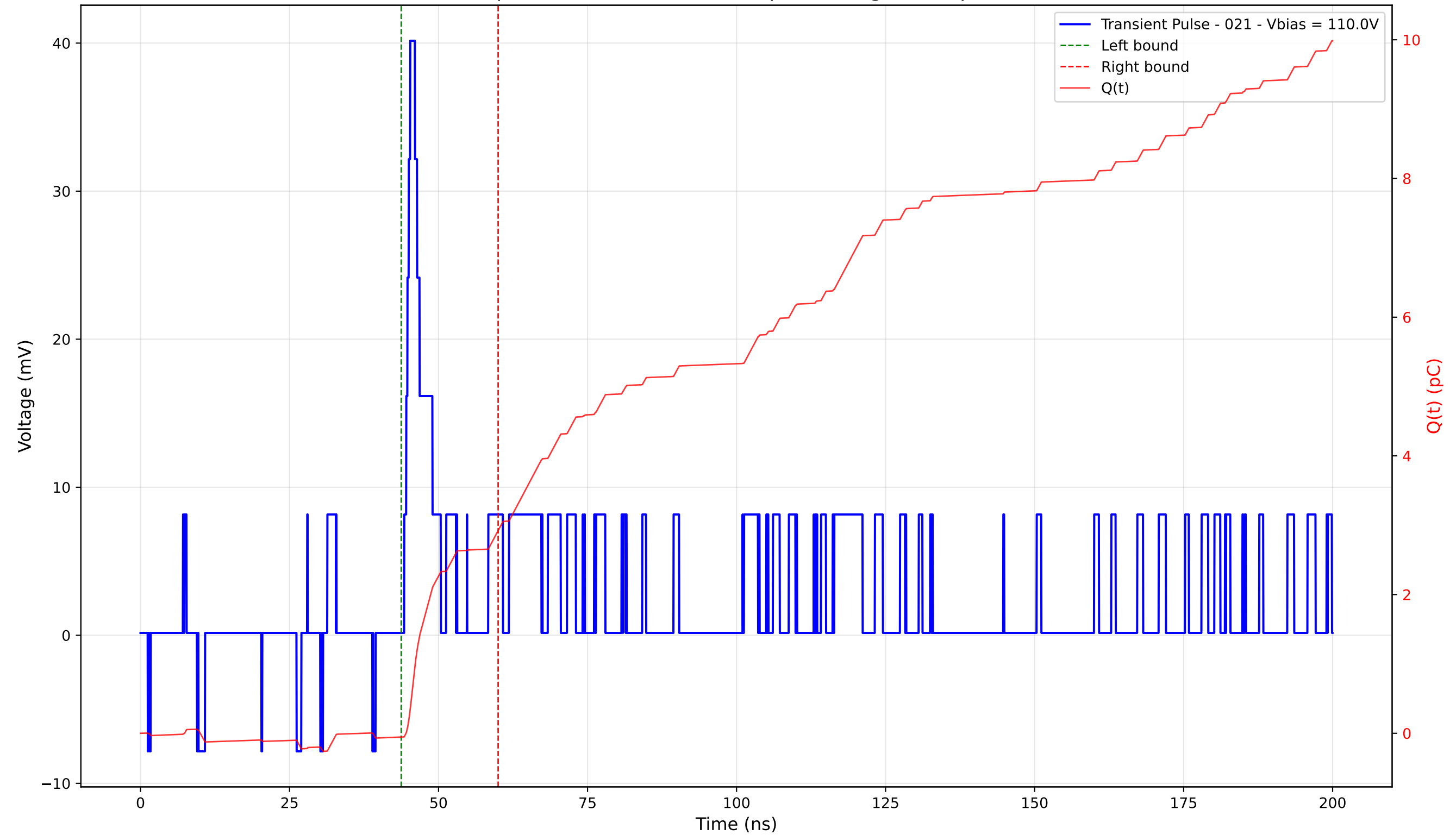
Transient Pulse - Sample: 4003 - Position: 305.0 \mu\text{m} - Charge: 2.98 pC - Rise Time: 1.01 ns
