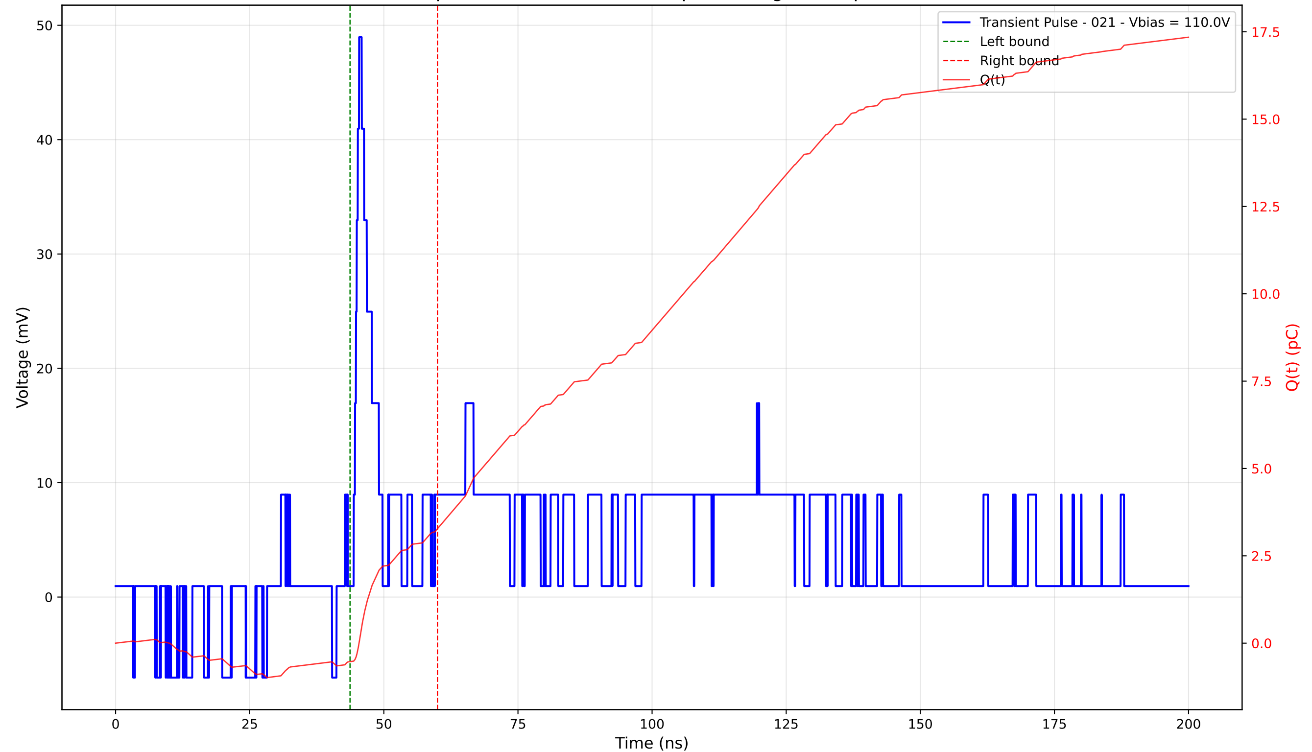
Transient Pulse - Sample: 4003 - Position: 290.0 \mu\text{m} - Charge: 3.81 pC - Rise Time: 1.01 ns
