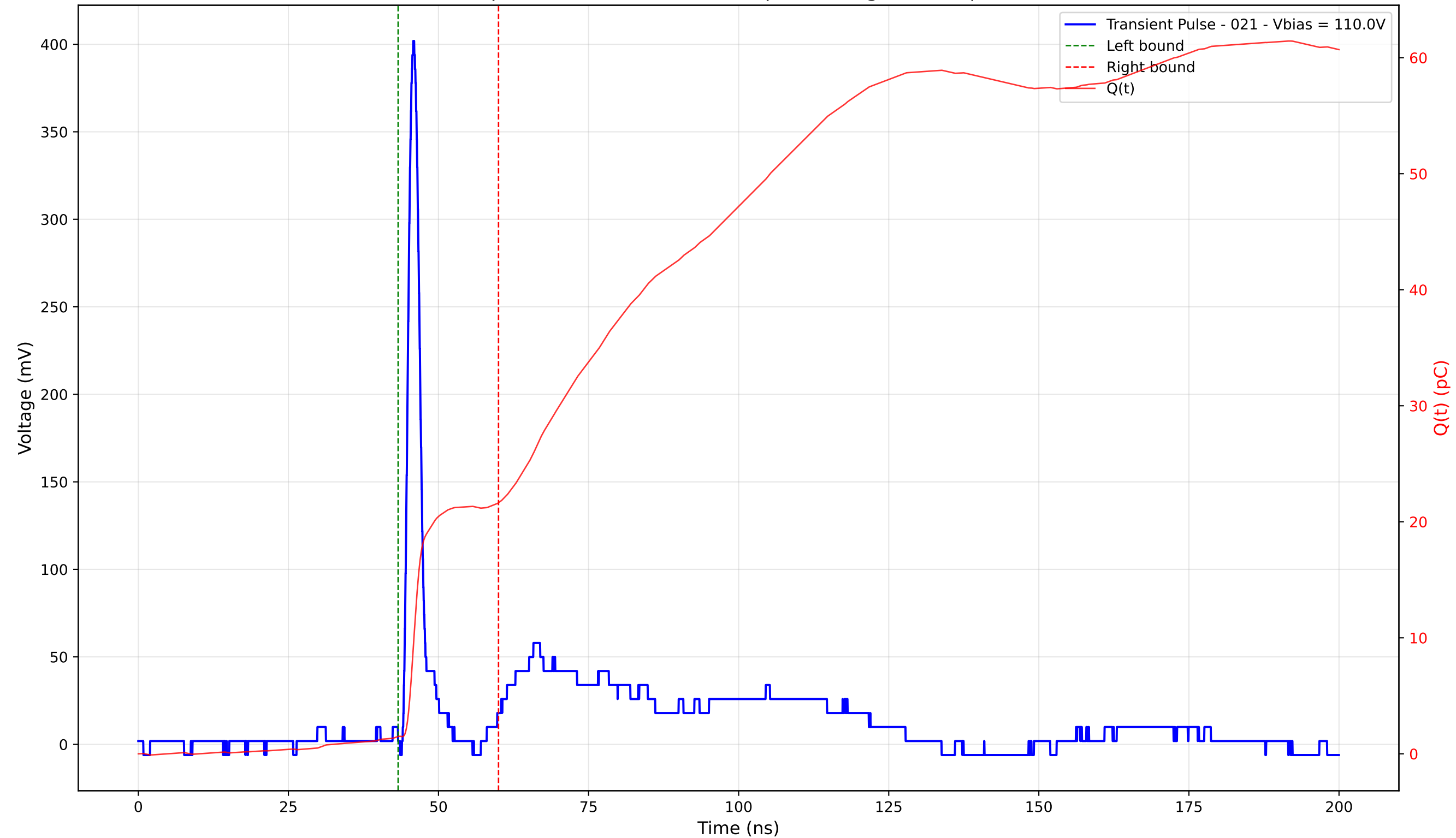
Transient Pulse - Sample: 4003 - Position: 190.0 \mu\text{m} - Charge: 20.14 pC - Rise Time: 1.14 ns
