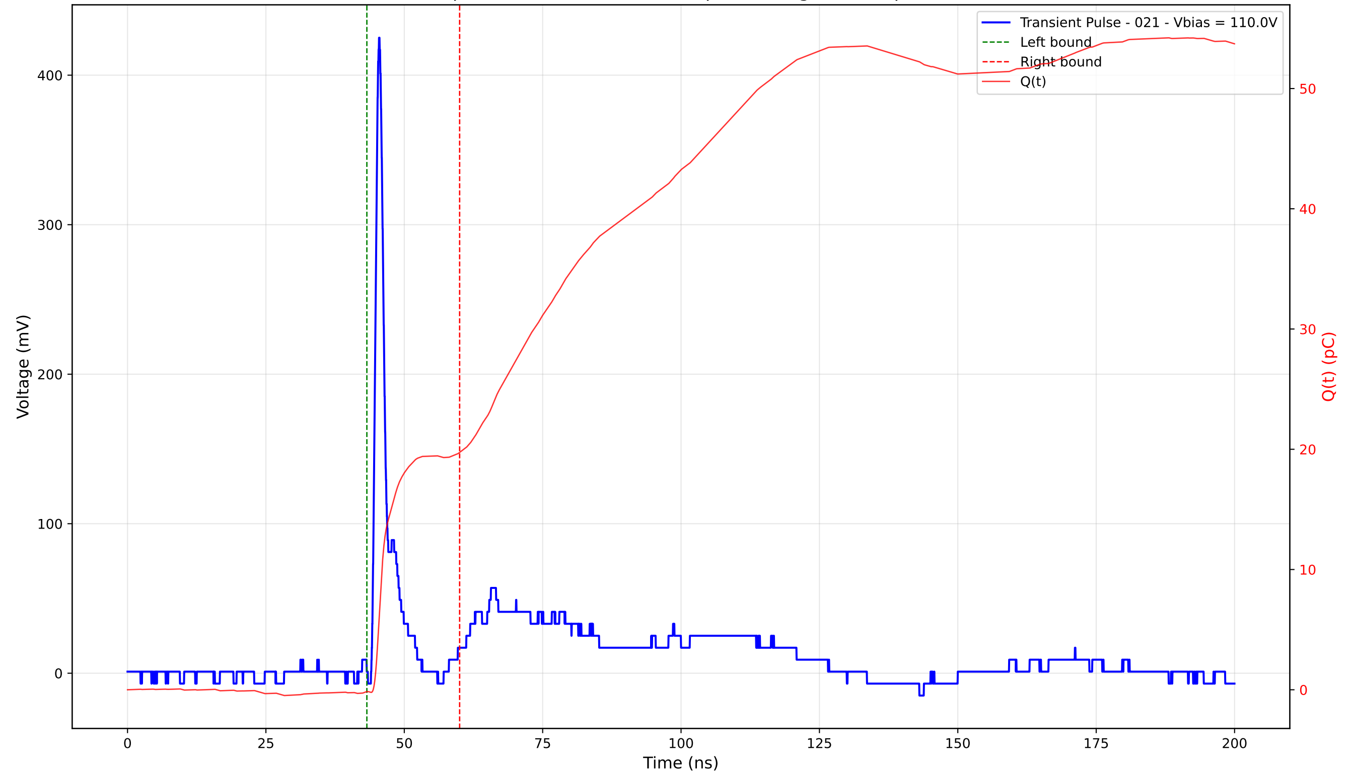
Transient Pulse - Sample: 4003 - Position: 130.0 \mu\text{m} - Charge: 19.89 pC - Rise Time: 0.92 ns
