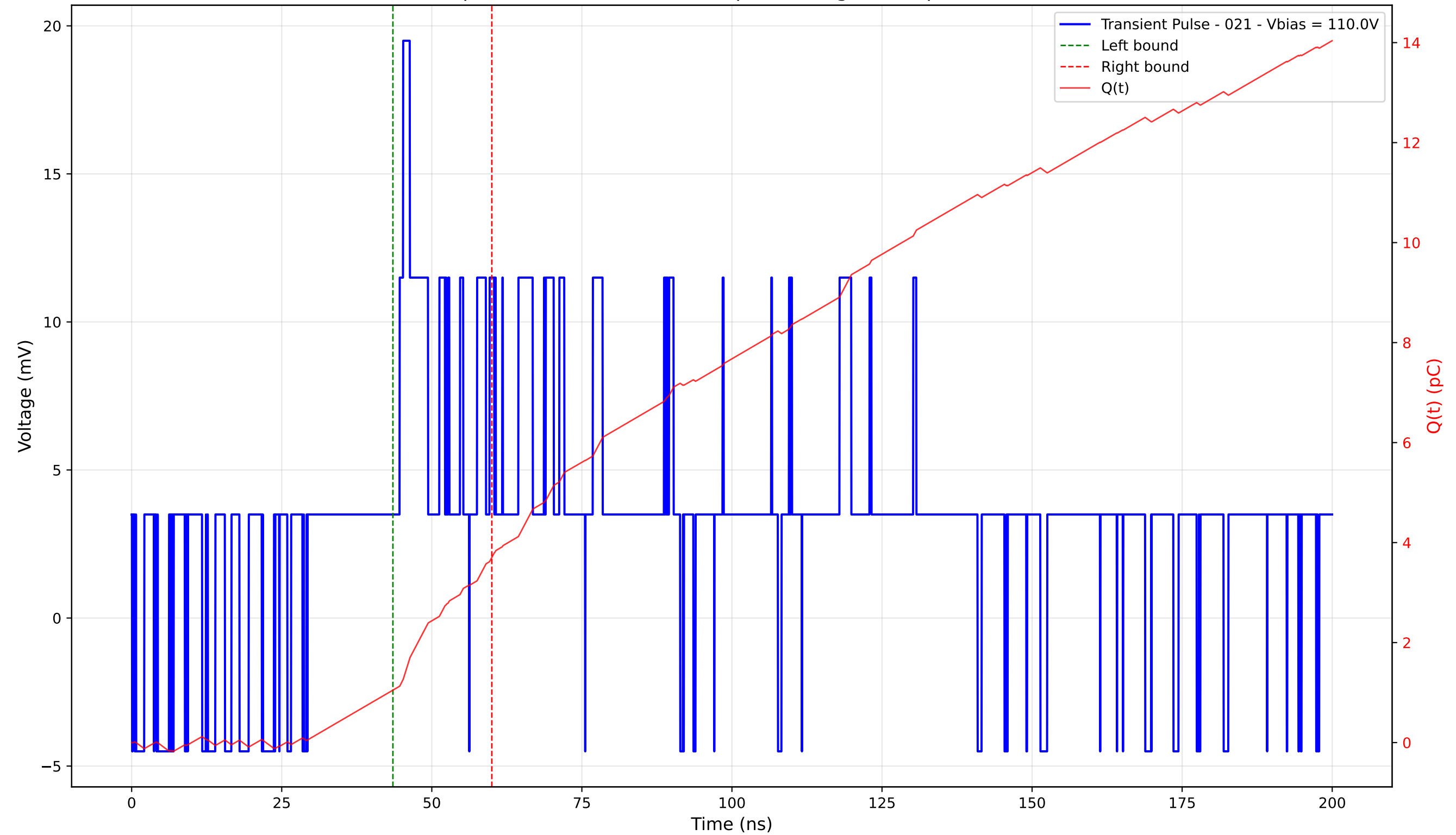
Transient Pulse - Sample: 4003 - Position: 425.0 \mu\text{m} - Charge: 2.66 pC - Rise Time: 0.00 ns (N/A)
