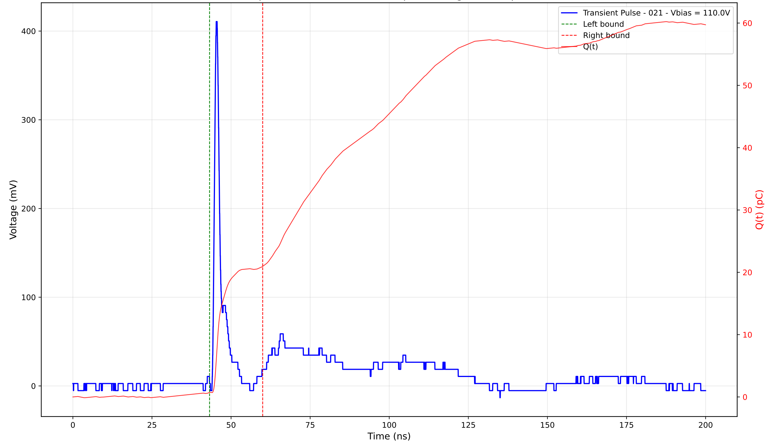
Transient Pulse - Sample: 4003 - Position: 125.0 \mu\text{m} - Charge: 20.22 pC - Rise Time: 0.90 ns
