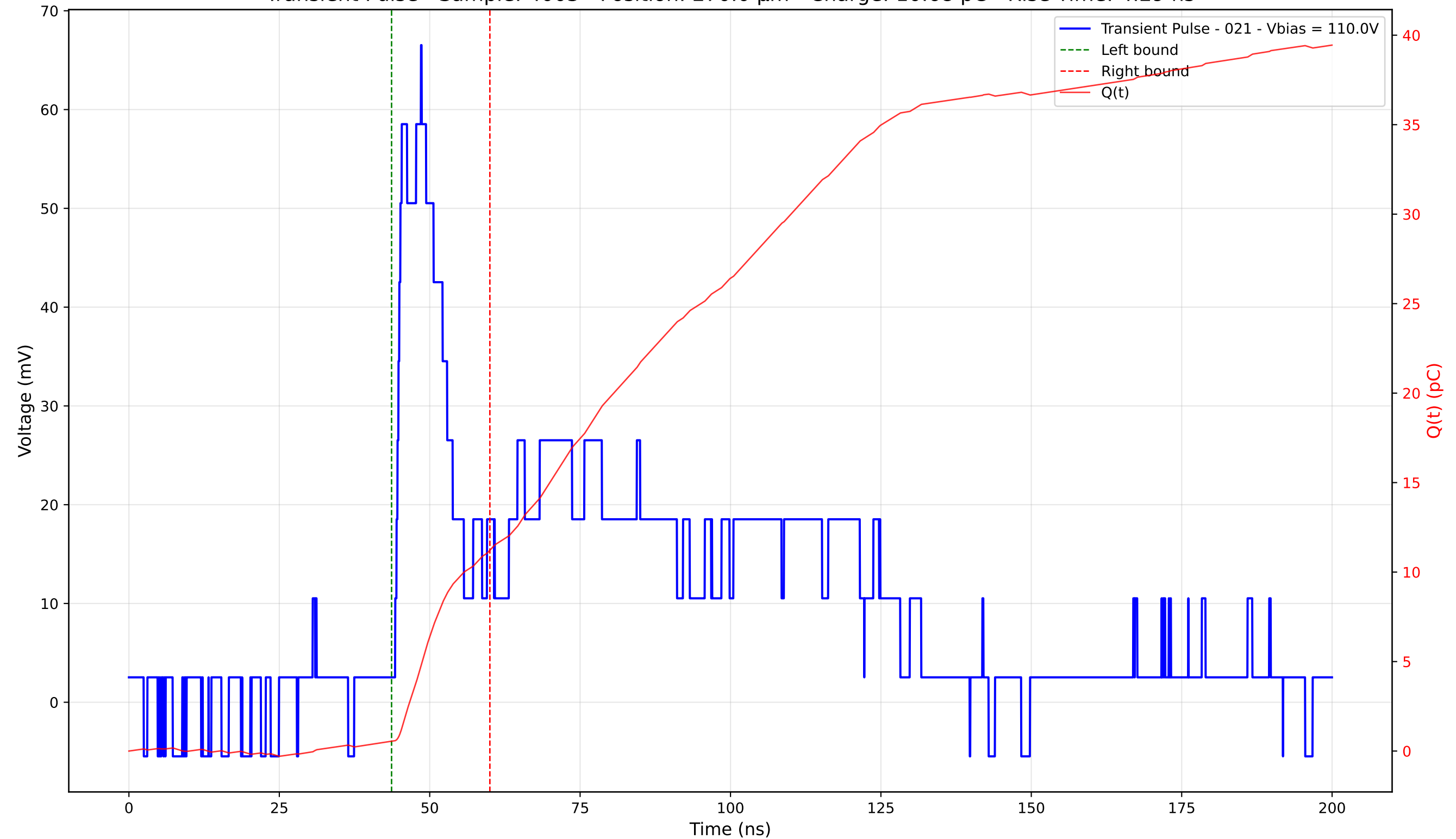
Transient Pulse - Sample: 4003 - Position: 270.0 \mu\text{m} - Charge: 10.68 pC - Rise Time: 4.29 ns
