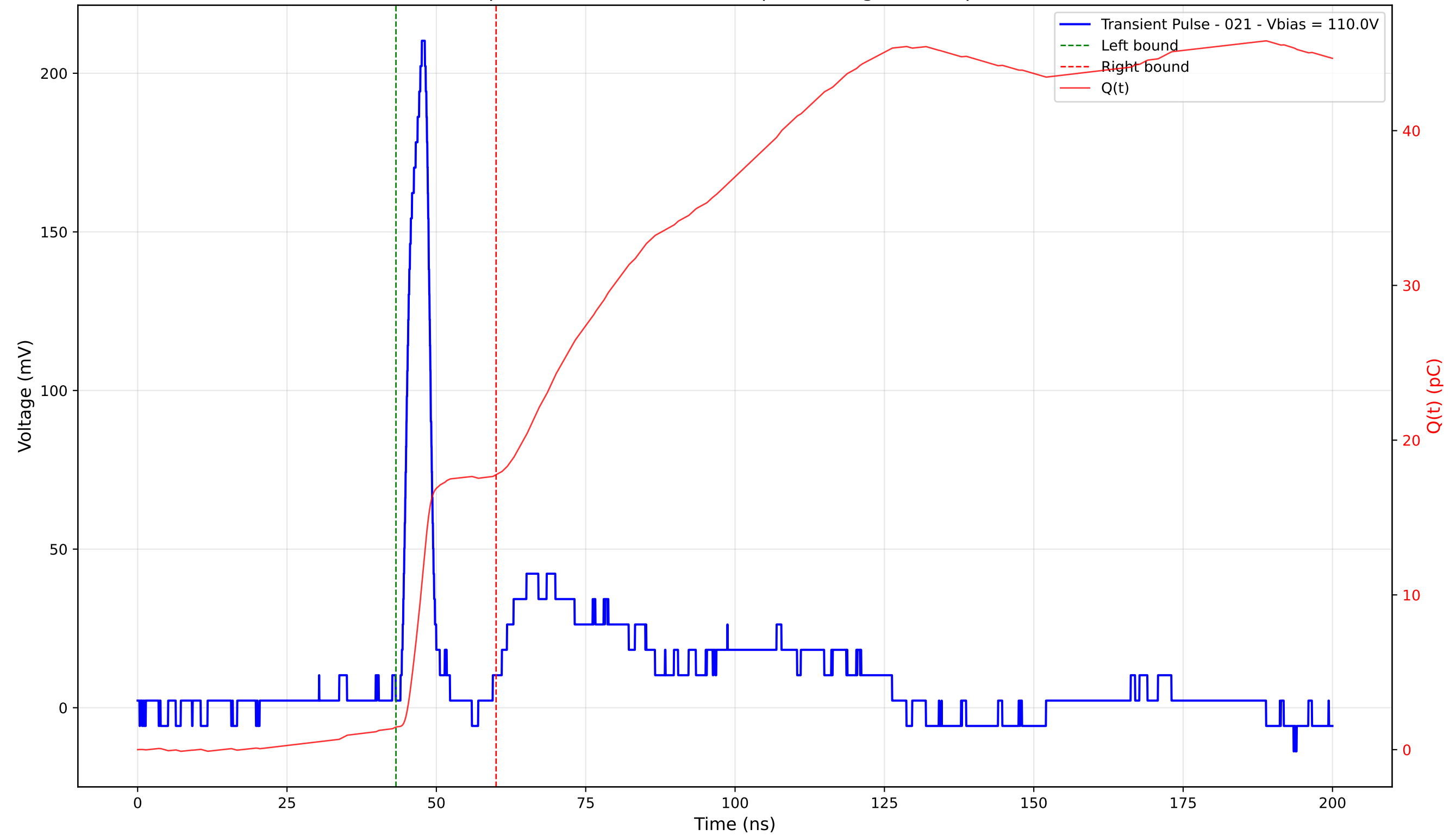
Transient Pulse - Sample: 4003 - Position: 250.0 \mu\text{m} - Charge: 16.30 pC - Rise Time: 2.77 ns
