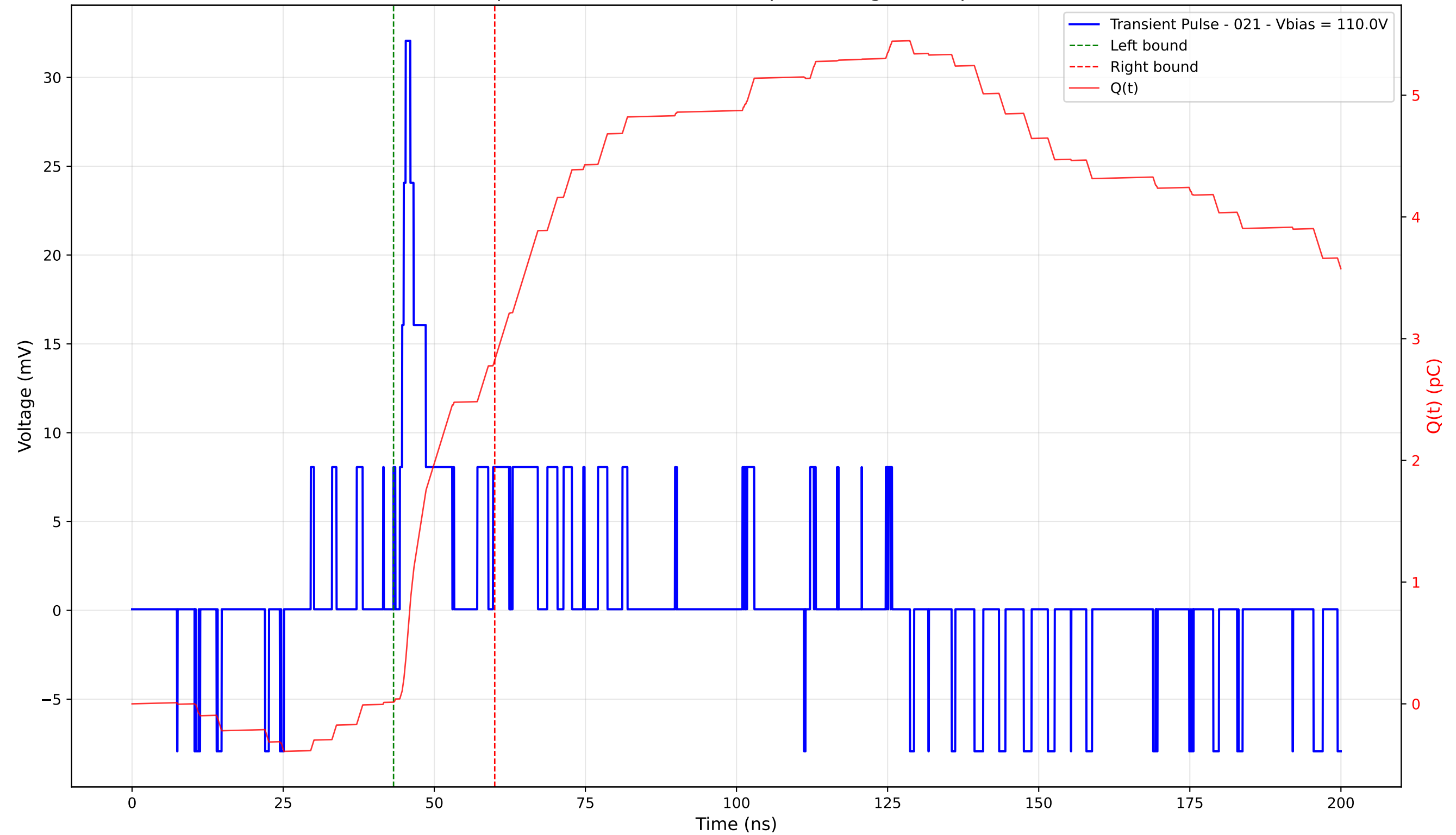
Transient Pulse - Sample: 4003 - Position: 380.0 \mu\text{m} - Charge: 2.81 pC - Rise Time: 0.97 ns
