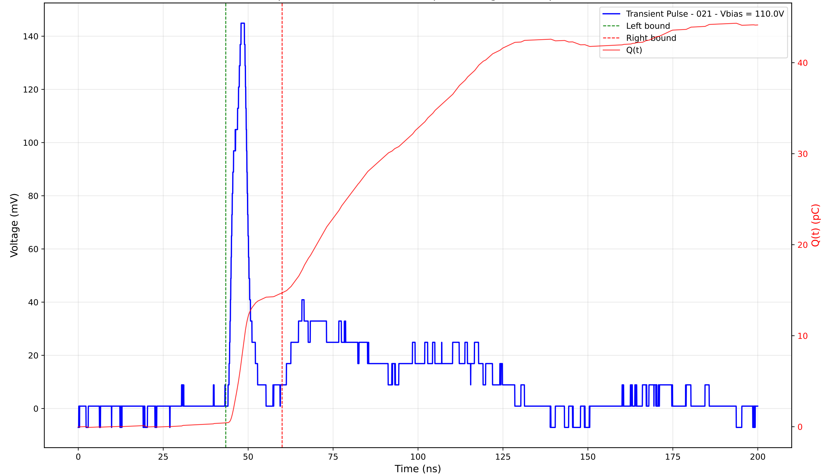
Transient Pulse - Sample: 4003 - Position: 260.0 \mu\text{m} - Charge: 14.28 pC - Rise Time: 3.27 ns
