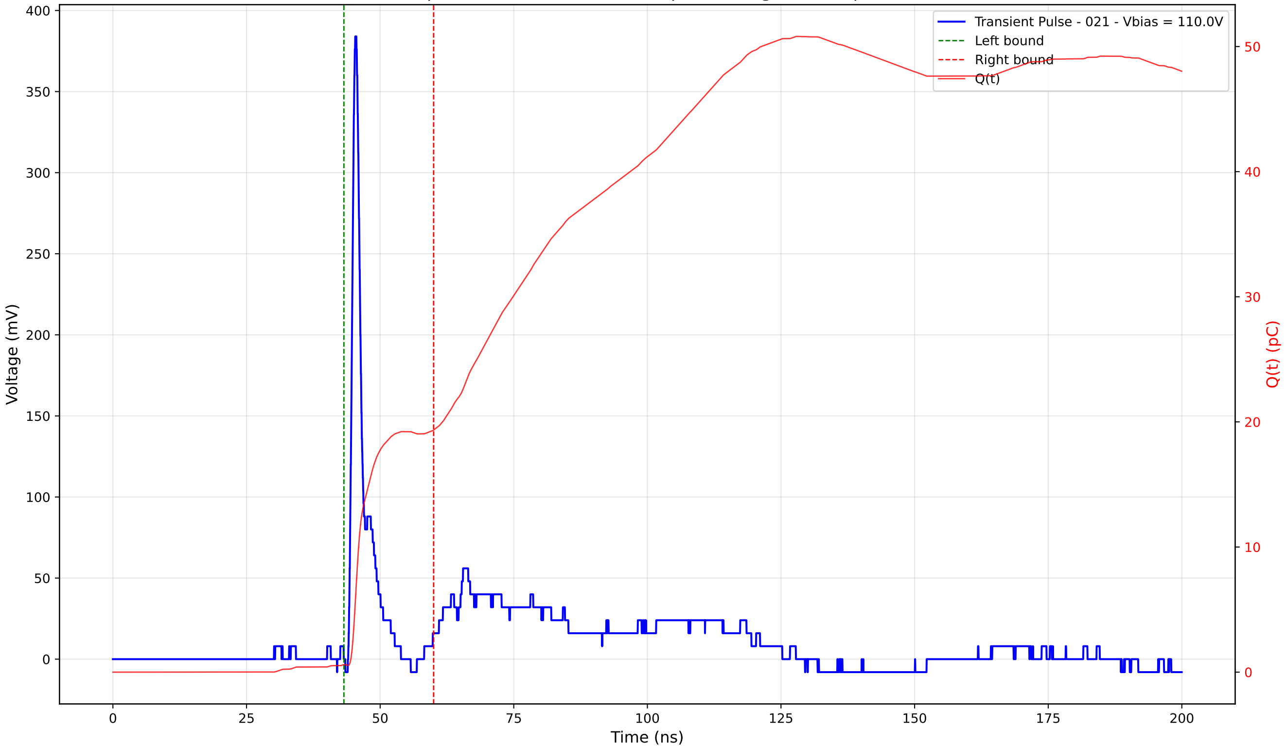
Transient Pulse - Sample: 4003 - Position: 120.0 \mu\text{m} - Charge: 18.74 pC - Rise Time: 0.90 ns
