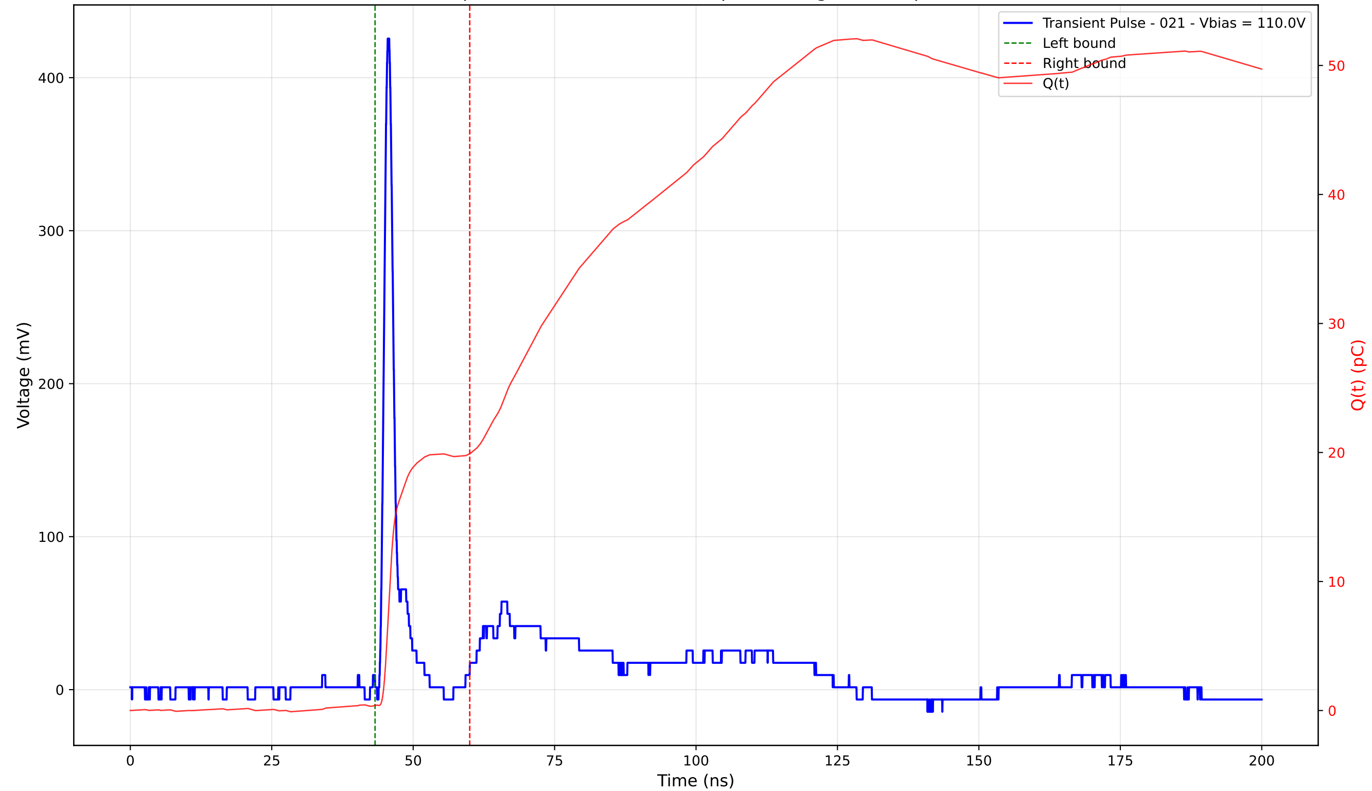
Transient Pulse - Sample: 4003 - Position: 160.0 \mu\text{m} - Charge: 19.48 pC - Rise Time: 0.98 ns
