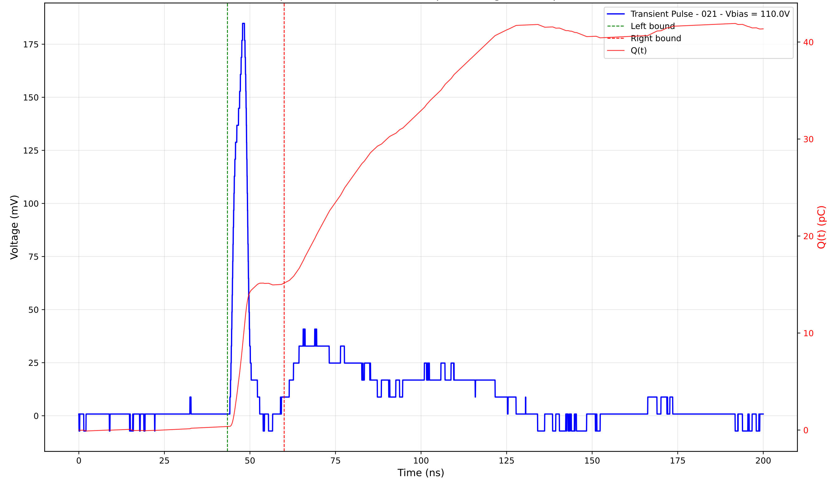
Transient Pulse - Sample: 4003 - Position: 255.0 \mu\text{m} - Charge: 14.79 pC - Rise Time: 3.00 ns
