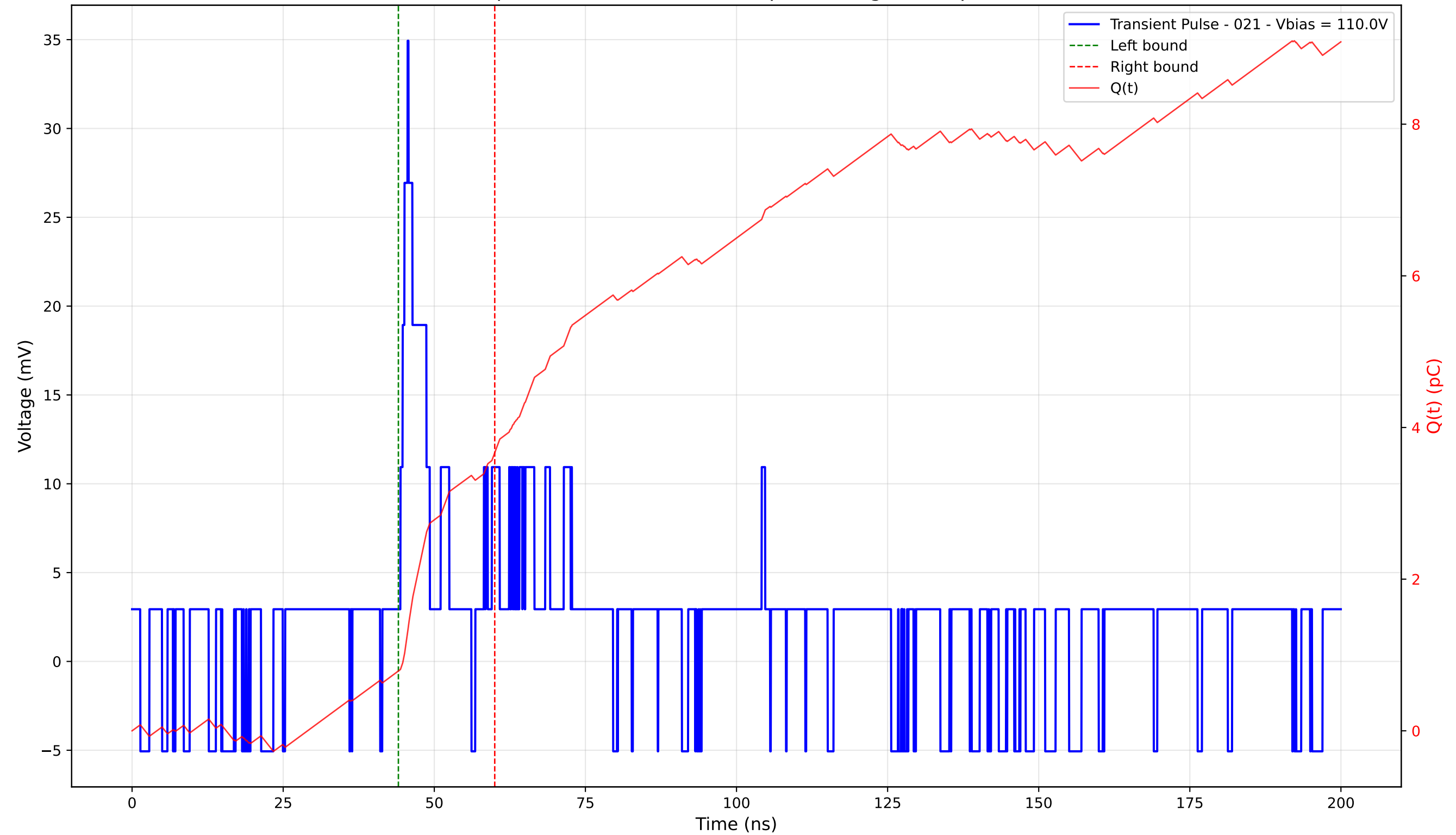
Transient Pulse - Sample: 4003 - Position: 365.0 \mu\text{m} - Charge: 2.88 pC - Rise Time: 1.20 ns
