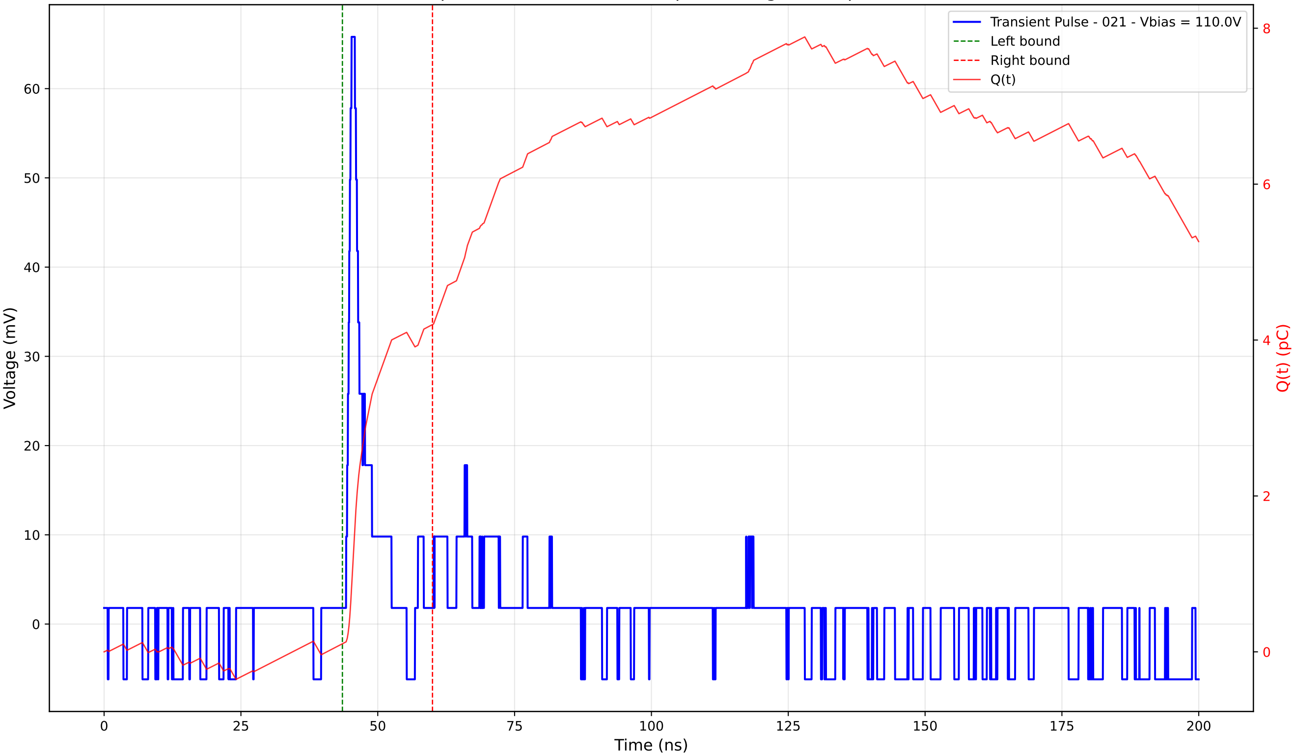
Transient Pulse - Sample: 4003 - Position: 90.0 \mu\text{m} - Charge: 4.09 pC - Rise Time: 0.99 ns
