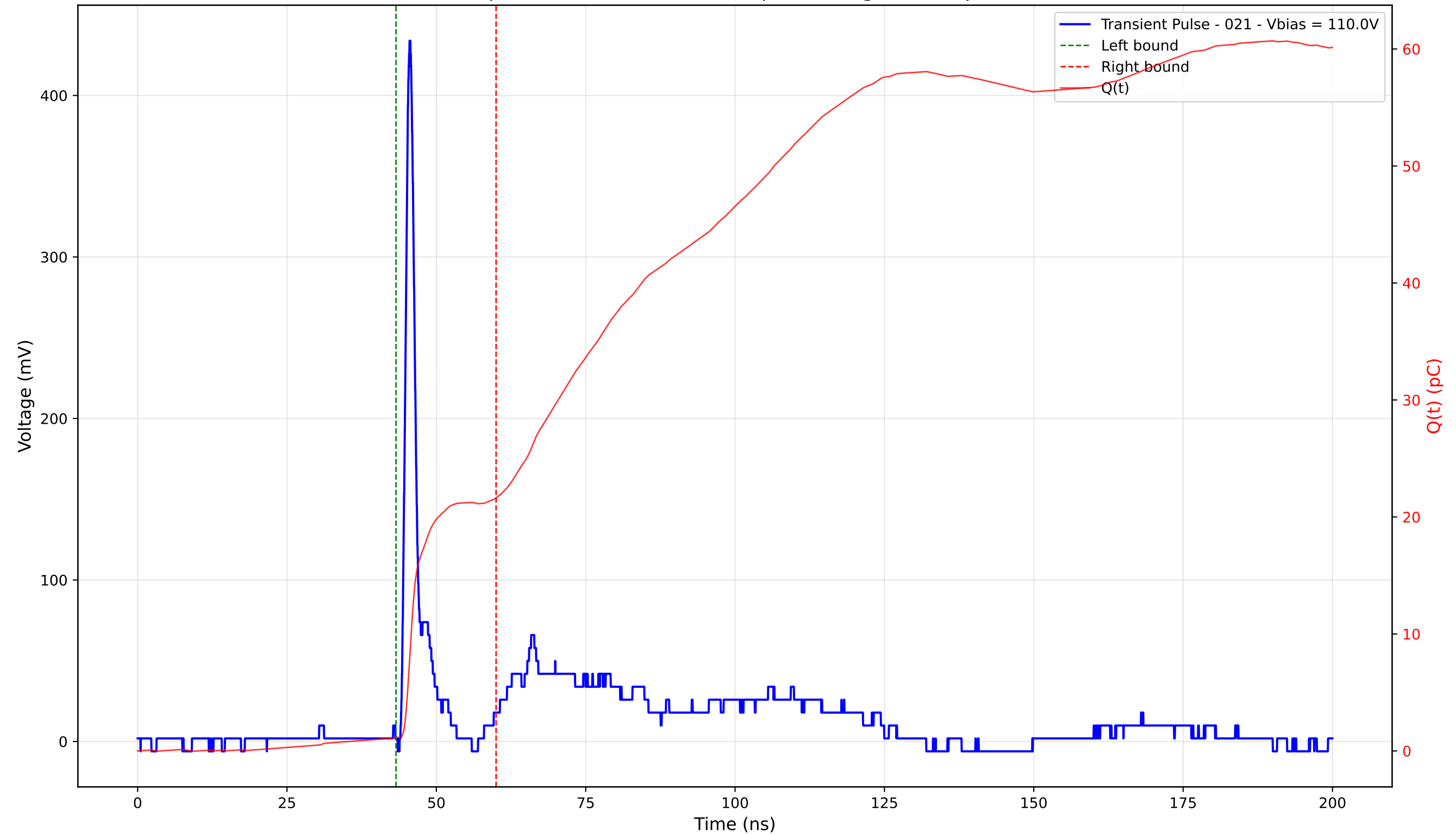
Transient Pulse - Sample: 4003 - Position: 150.0 \mu\text{m} - Charge: 20.47 pC - Rise Time: 0.98 ns
