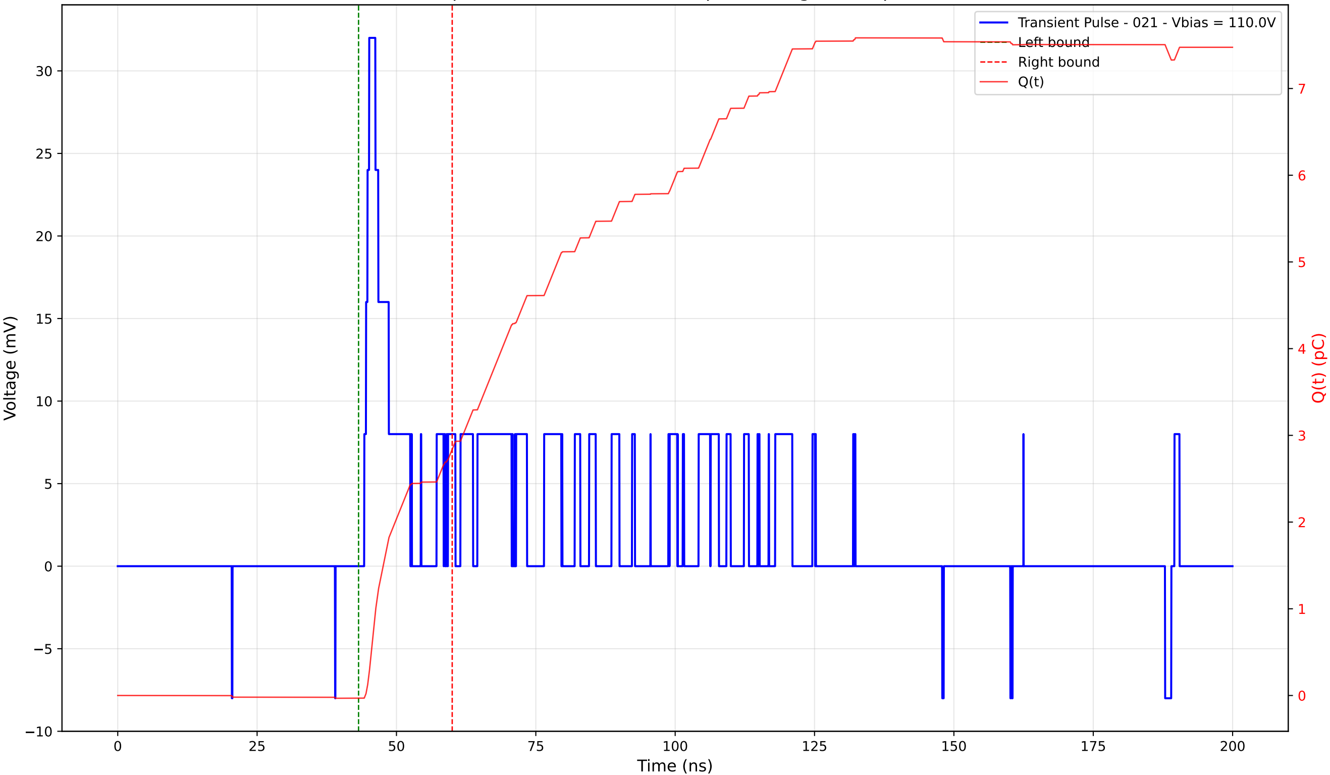
Transient Pulse - Sample: 4003 - Position: 315.0 \mu\text{m} - Charge: 2.87 pC - Rise Time: 0.89 ns
