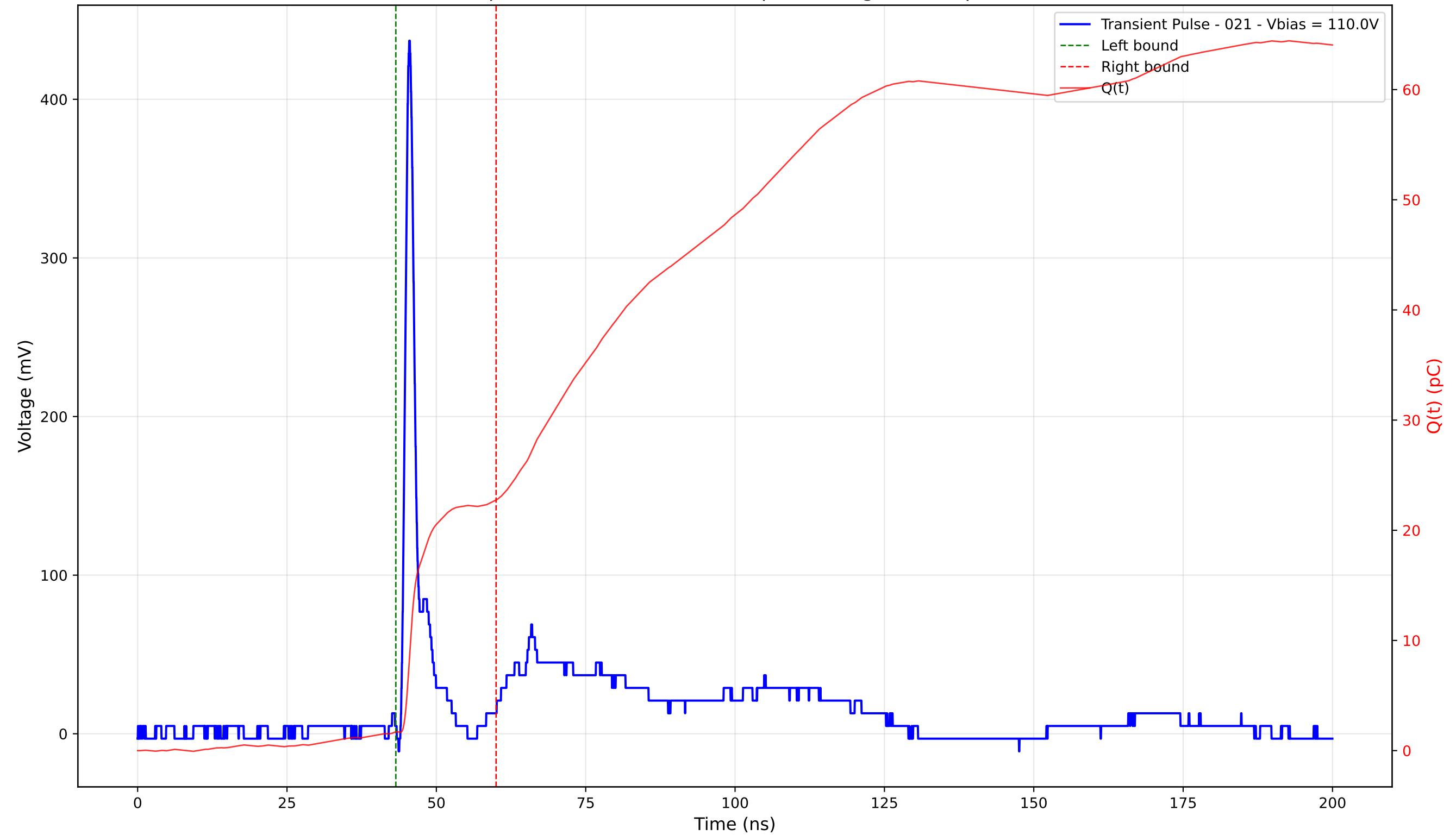
Transient Pulse - Sample: 4003 - Position: 140.0 \mu\text{m} - Charge: 21.03 pC - Rise Time: 0.96 ns
