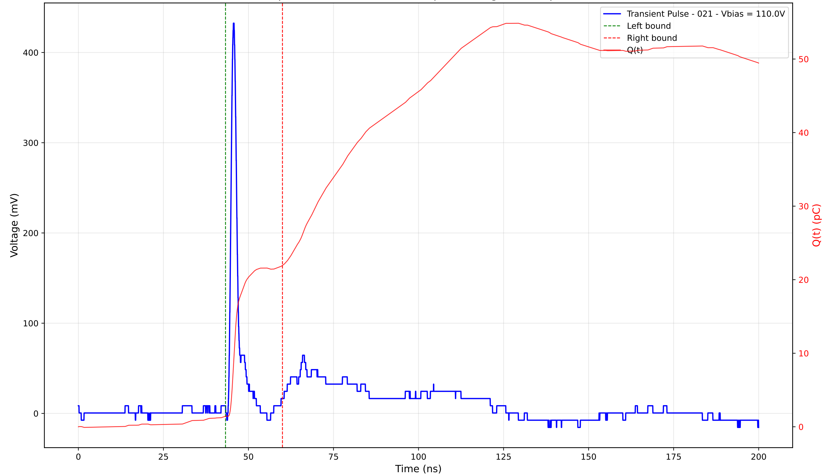
Transient Pulse - Sample: 4003 - Position: 165.0 \mu\text{m} - Charge: 20.49 pC - Rise Time: 1.01 ns
