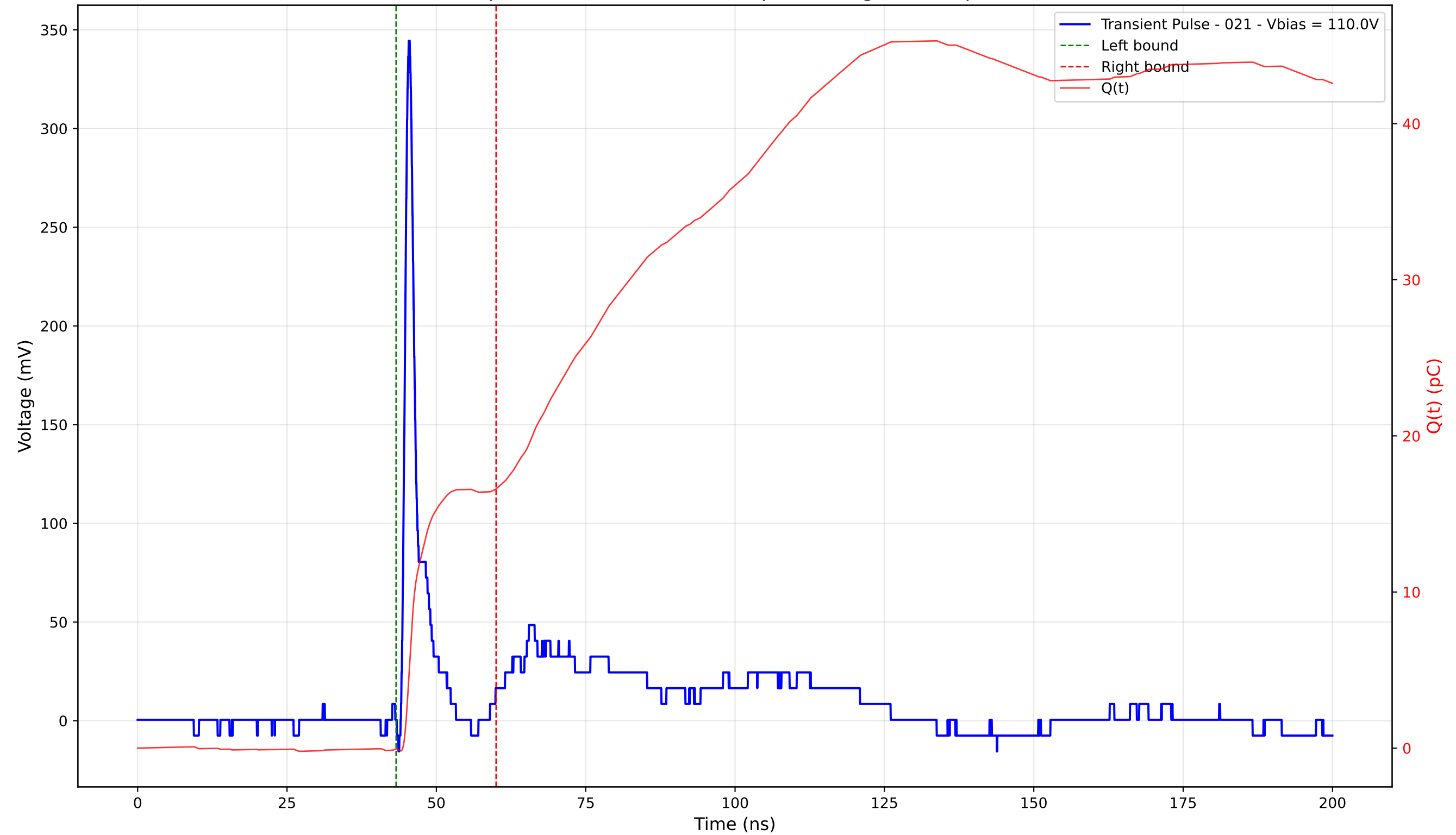
Transient Pulse - Sample: 4003 - Position: 115.0 \mu\text{m} - Charge: 16.66 pC - Rise Time: 0.88 ns
