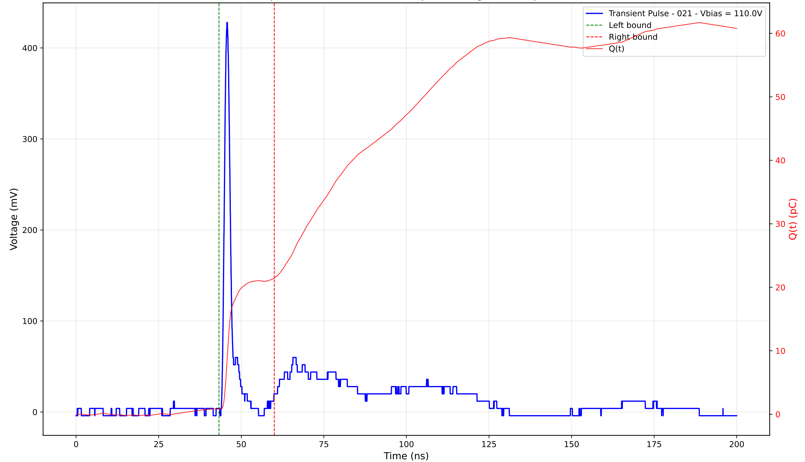
Transient Pulse - Sample: 4003 - Position: 175.0 \mu\text{m} - Charge: 20.58 pC - Rise Time: 1.08 ns
