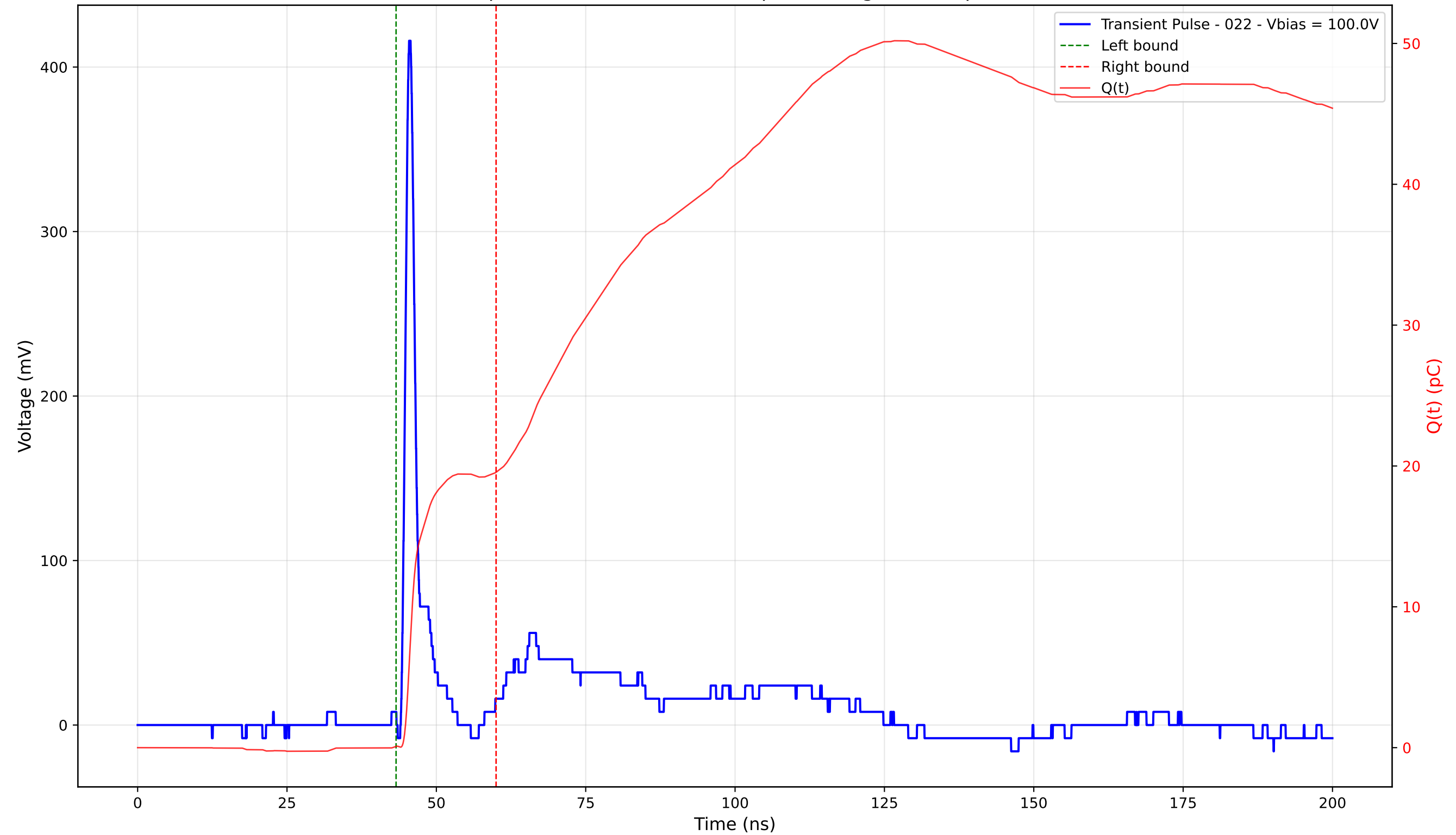
Transient Pulse - Sample: 4003 - Position: 145.0 \mu\text{m} - Charge: 19.45 pC - Rise Time: 0.93 ns
