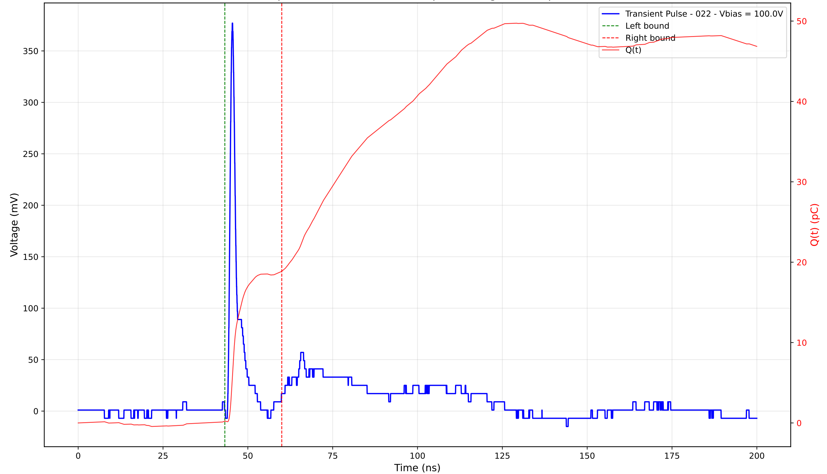
Transient Pulse - Sample: 4003 - Position: 120.0 \mu\text{m} - Charge: 18.65 pC - Rise Time: 0.93 ns
