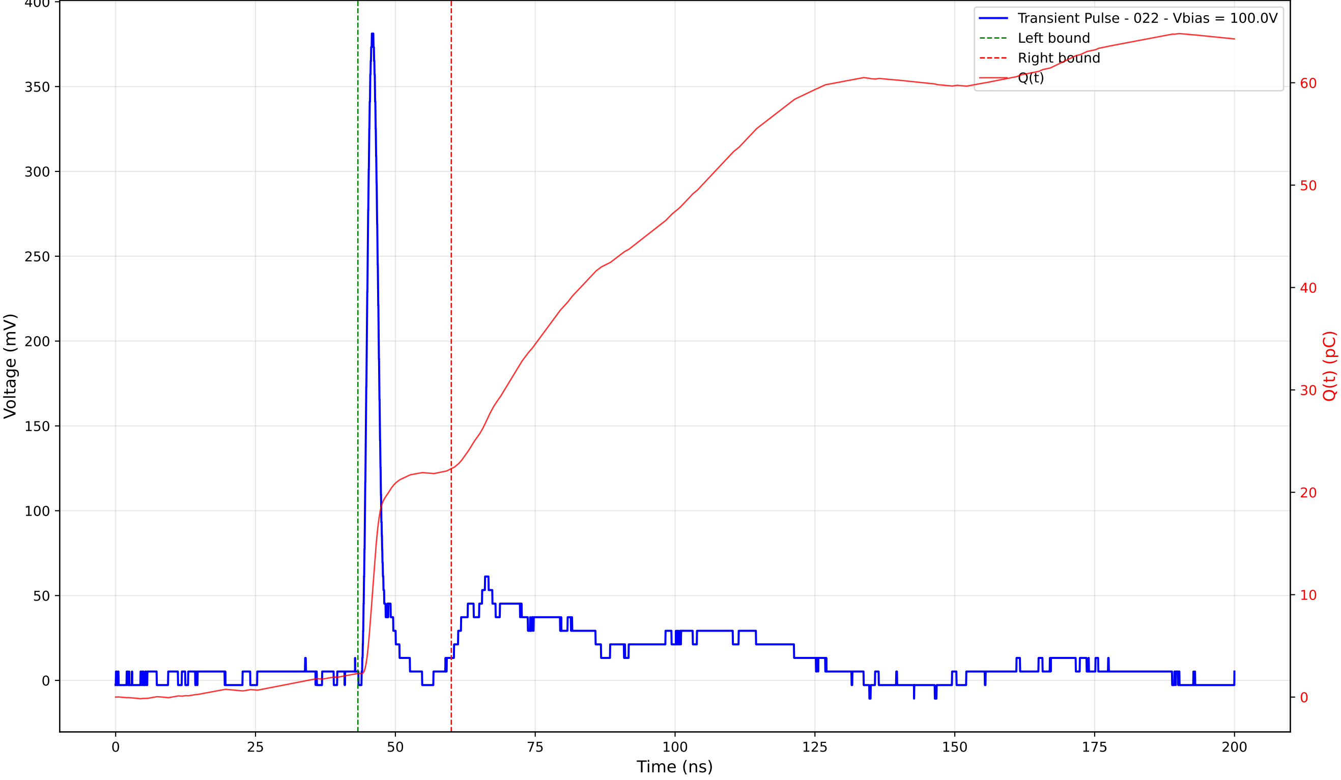
Transient Pulse - Sample: 4003 - Position: 190.0 \mu\text{m} - Charge: 19.99 pC - Rise Time: 1.18 ns
