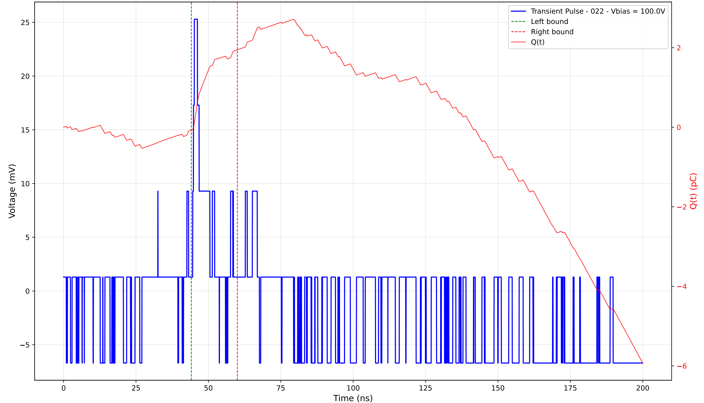
Transient Pulse - Sample: 4003 - Position: 360.0 \mu\text{m} - Charge: 2.02 pC - Rise Time: 0.58 ns
