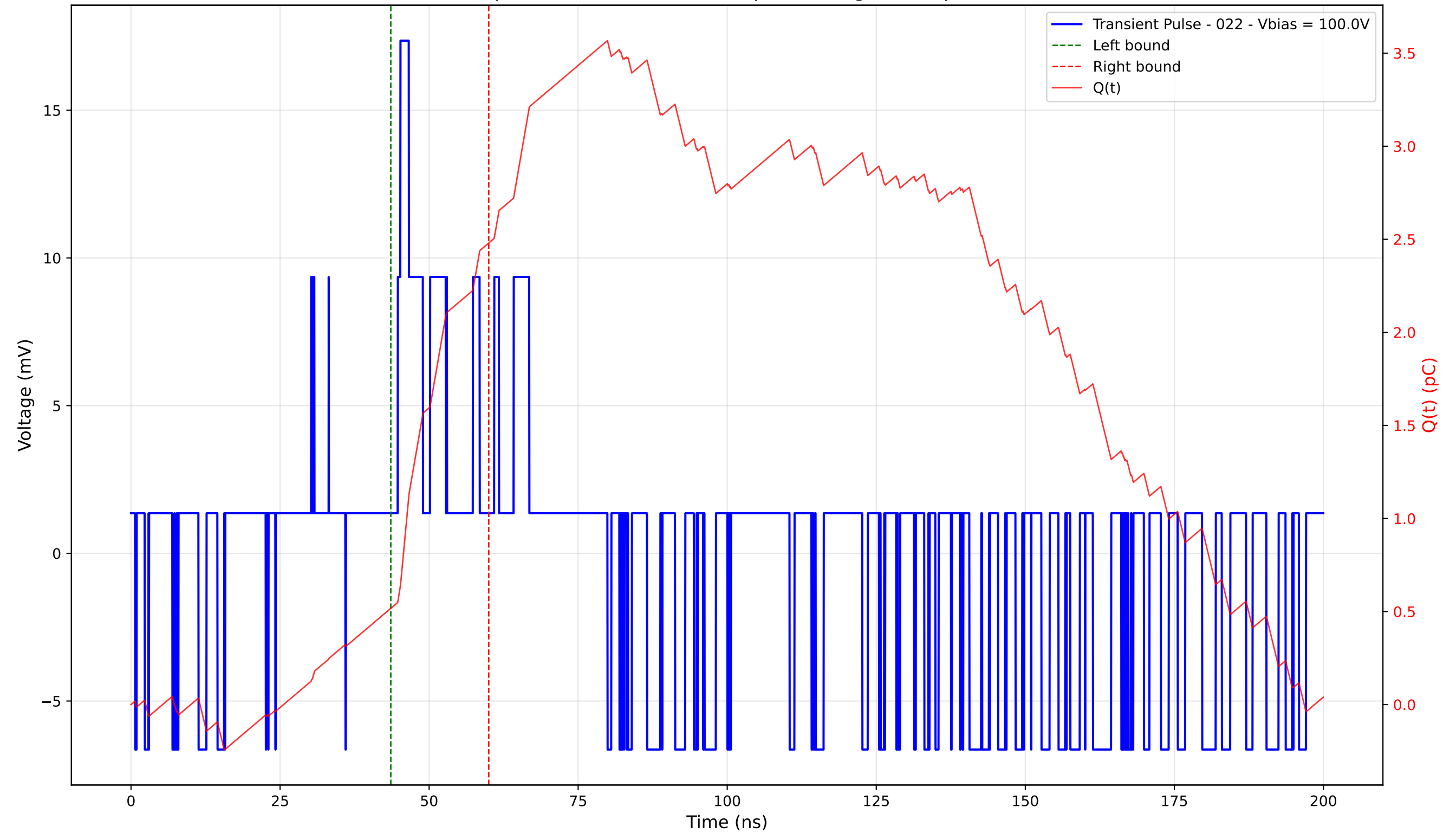
Transient Pulse - Sample: 4003 - Position: 20.0 \mu\text{m} - Charge: 1.96 pC - Rise Time: 0.46 ns
