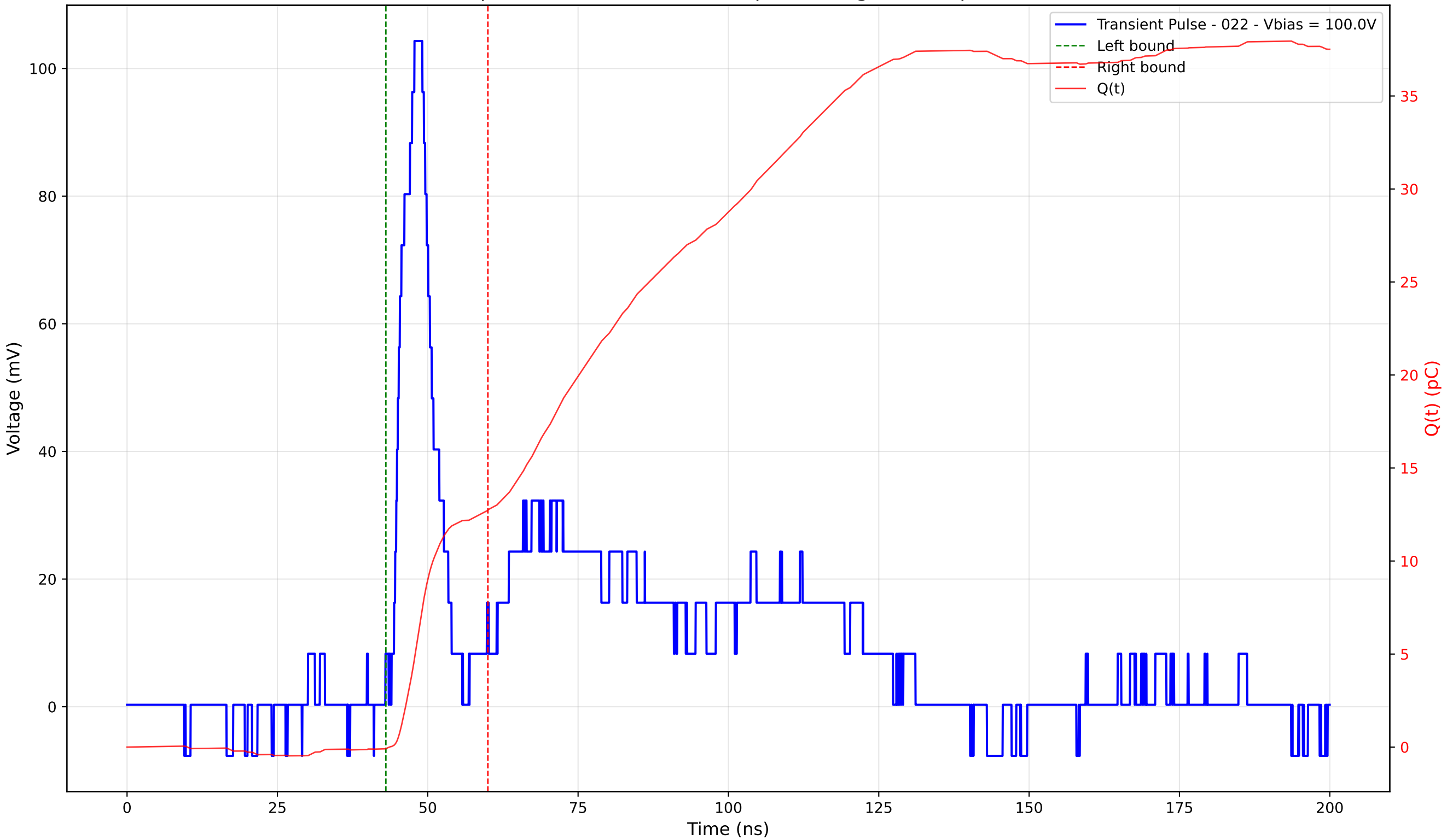
Transient Pulse - Sample: 4003 - Position: 255.0 \mu\text{m} - Charge: 12.82 pC - Rise Time: 3.01 ns
