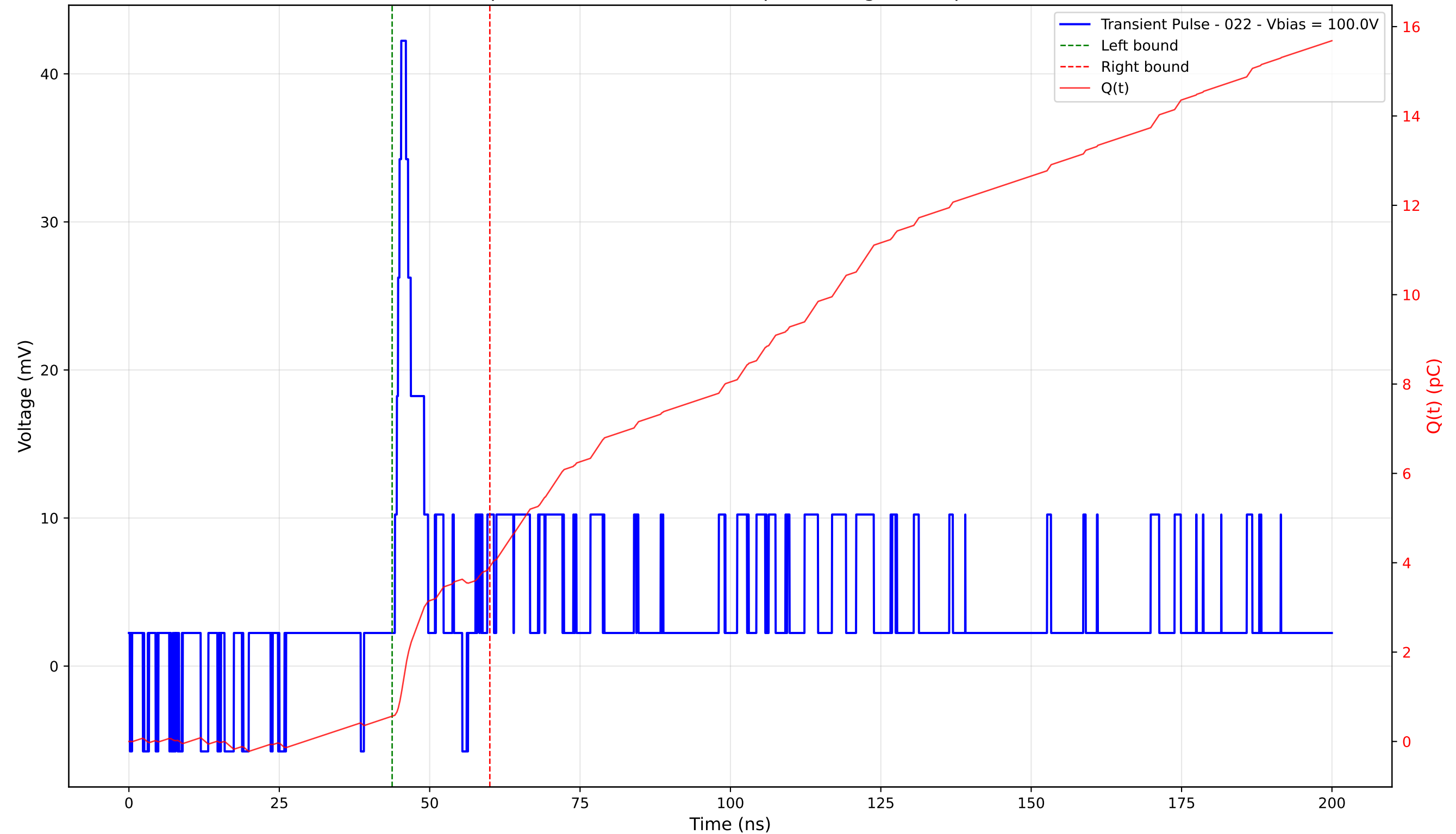
Transient Pulse - Sample: 4003 - Position: 290.0 \mu\text{m} - Charge: 3.35 pC - Rise Time: 1.06 ns
