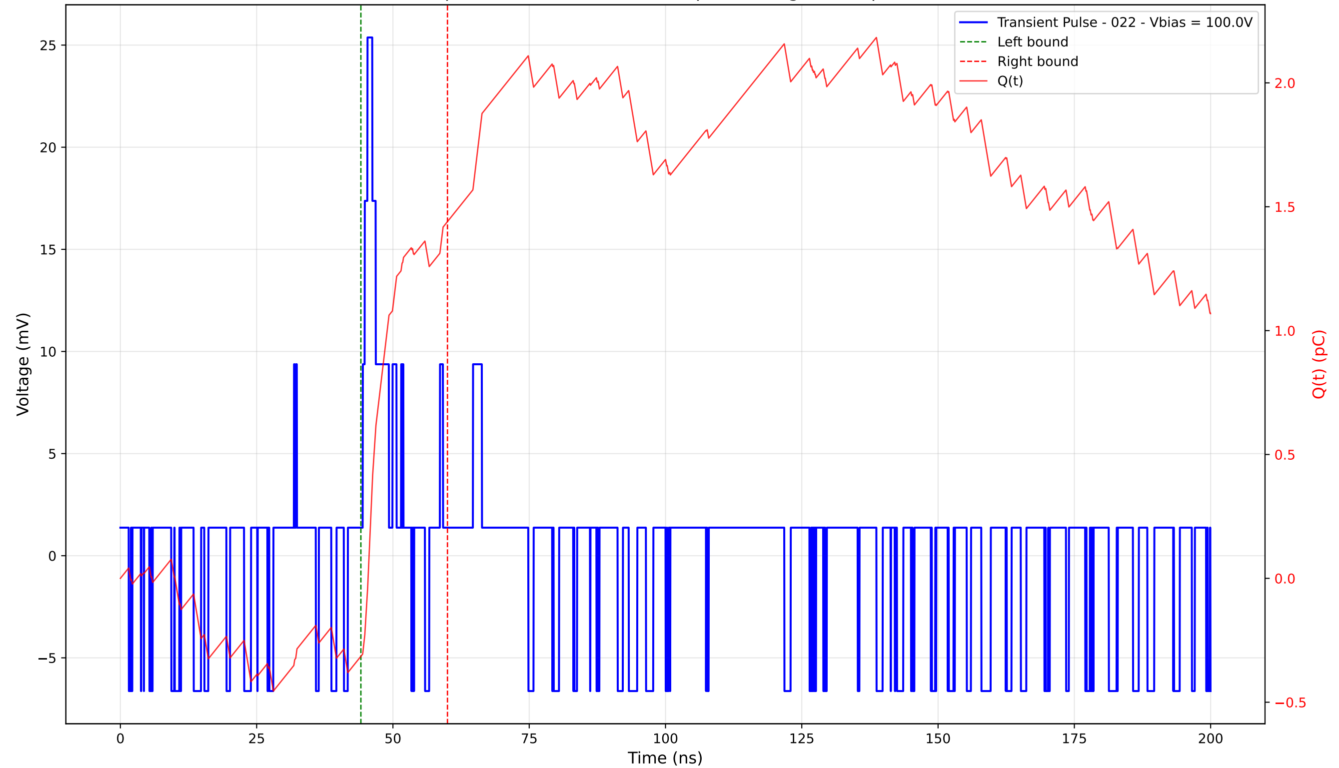
Transient Pulse - Sample: 4003 - Position: 355.0 \mu\text{m} - Charge: 1.75 pC - Rise Time: 0.88 ns
