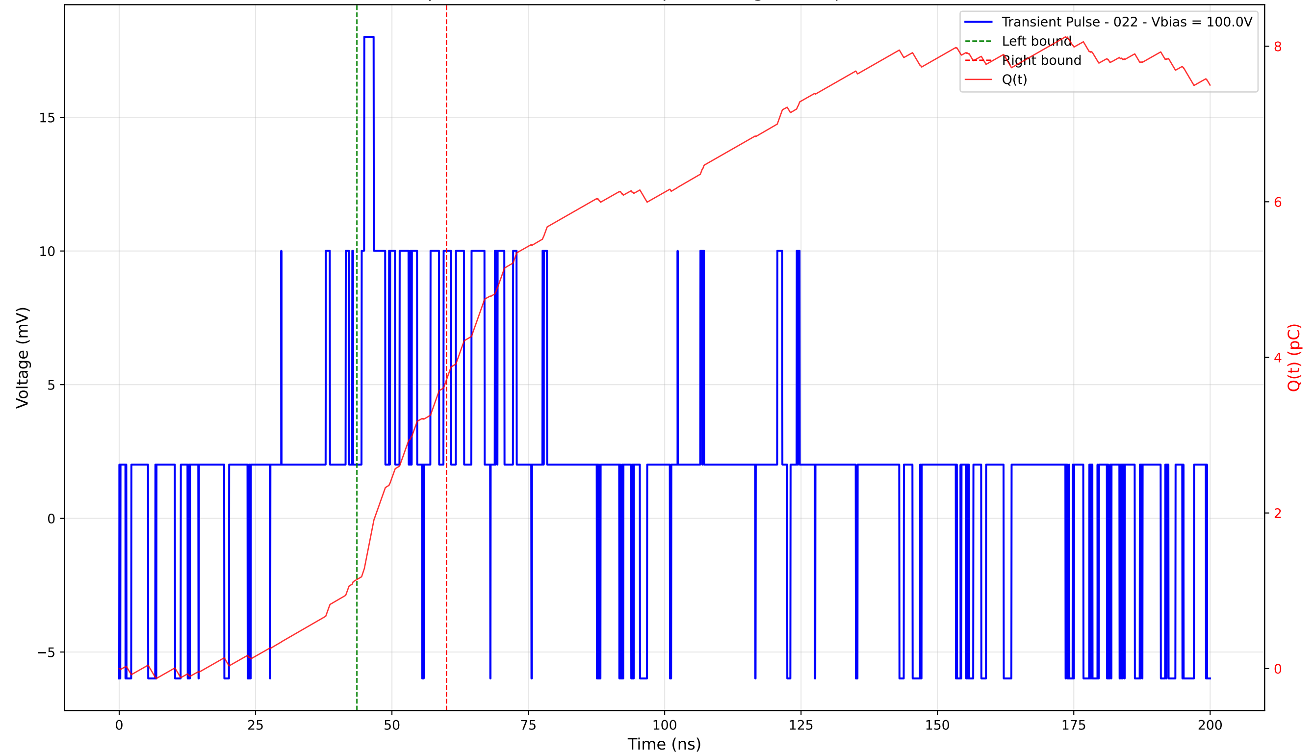
Transient Pulse - Sample: 4003 - Position: 15.0 \mu\text{m} - Charge: 2.57 pC - Rise Time: 0.00 ns (N/A)
