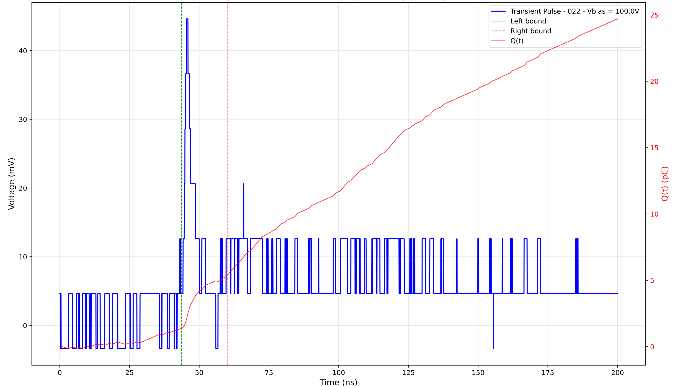
Transient Pulse - Sample: 4003 - Position: 285.0 \mu\text{m} - Charge: 3.95 pC - Rise Time: 3.38 ns
