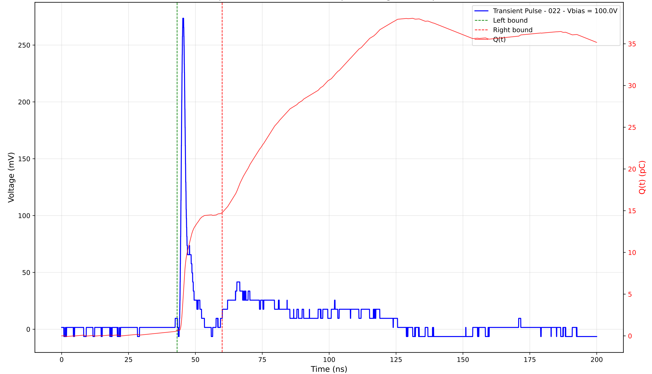
Transient Pulse - Sample: 4003 - Position: 110.0 \mu\text{m} - Charge: 14.11 pC - Rise Time: 0.88 ns
