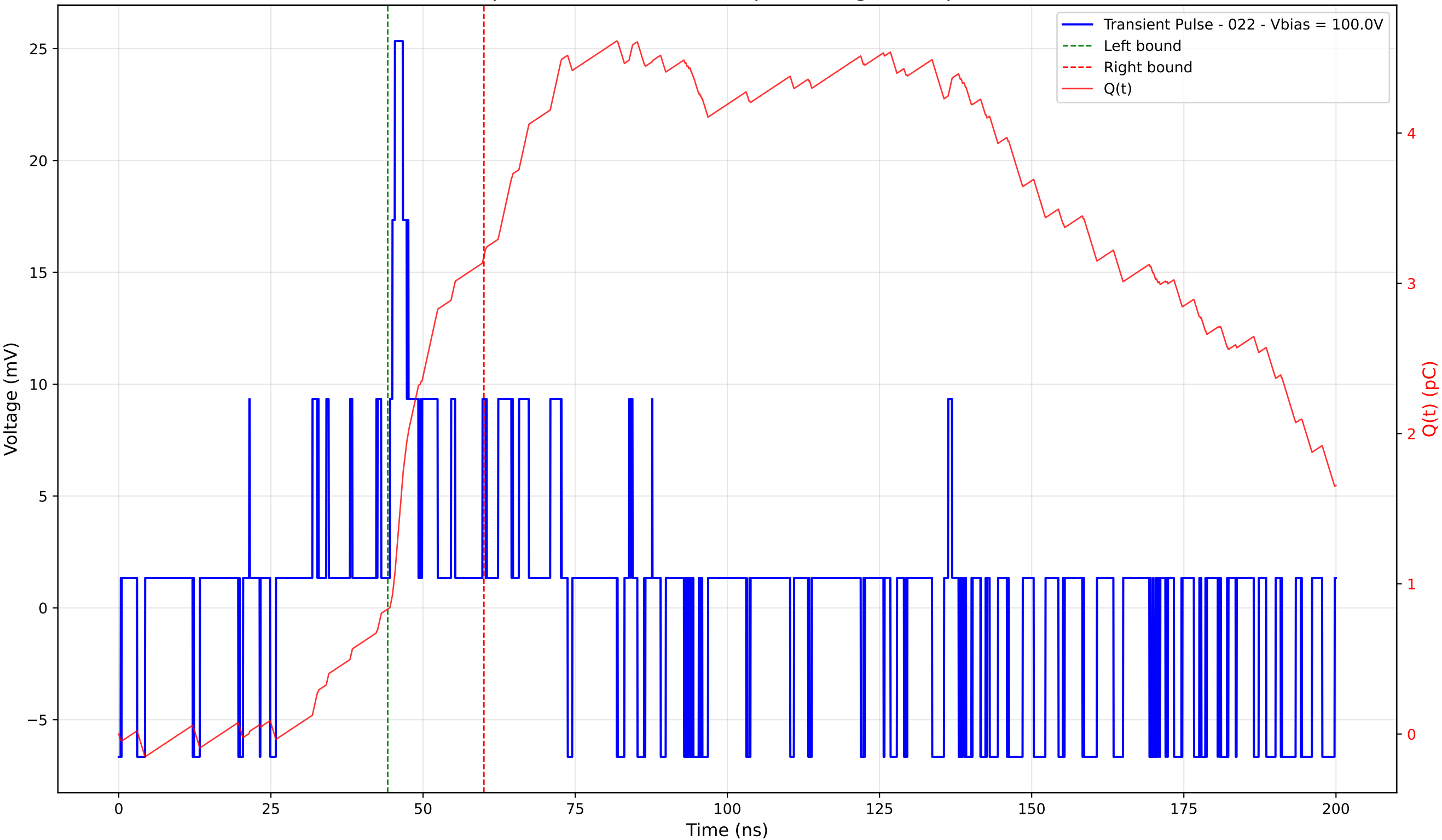
Transient Pulse - Sample: 4003 - Position: 40.0 \mu\text{m} - Charge: 2.35 pC - Rise Time: 0.82 ns
