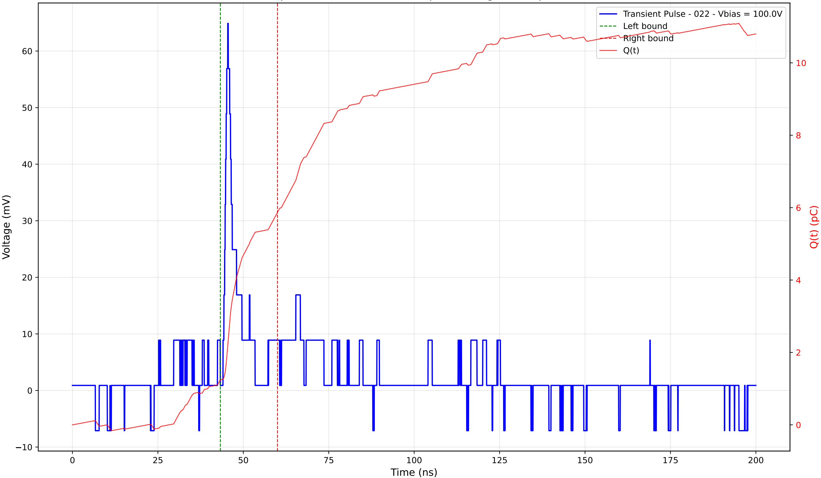
Transient Pulse - Sample: 4003 - Position: 90.0 \mu\text{m} - Charge: 4.63 pC - Rise Time: 1.39 ns
