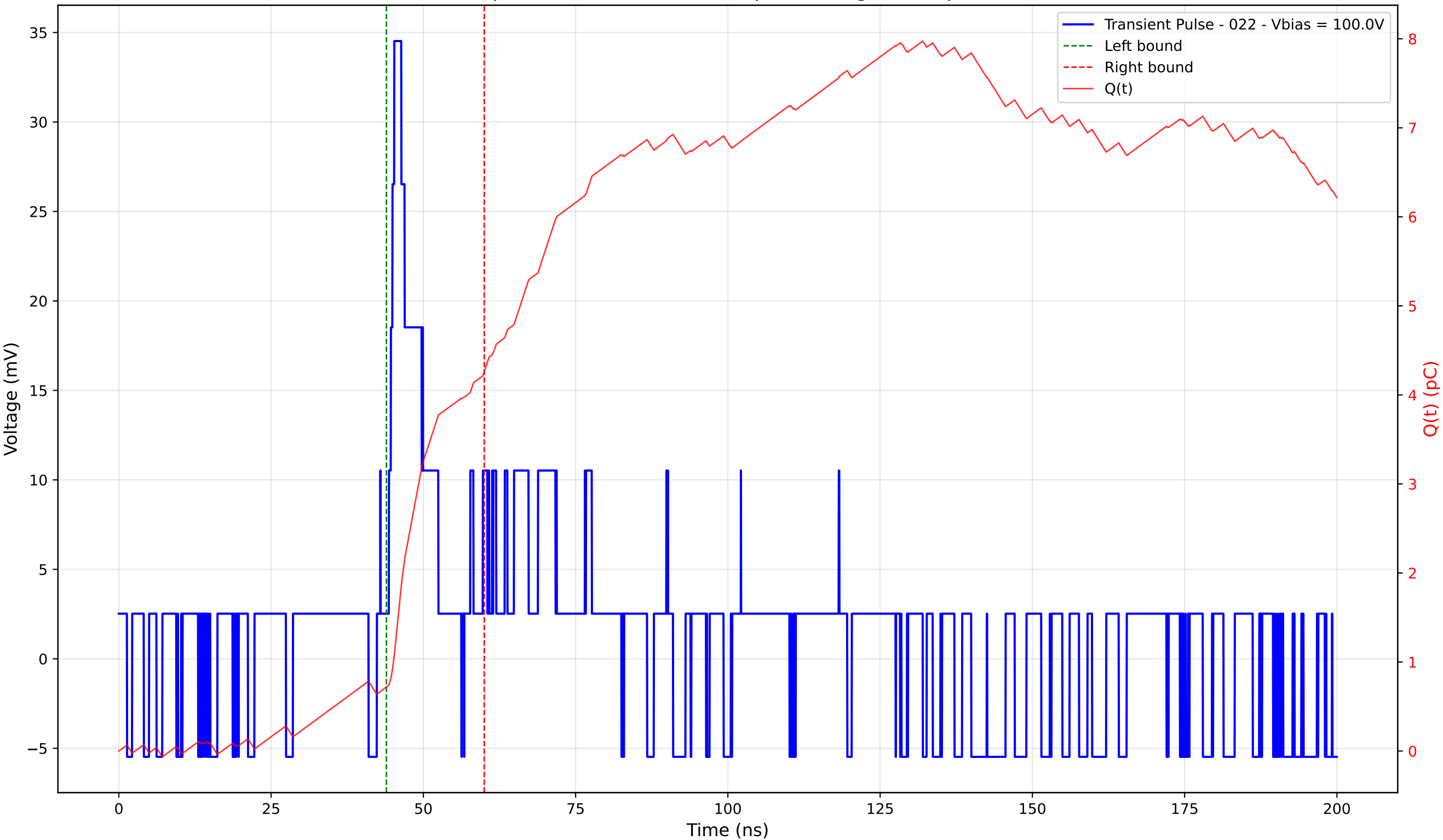
Transient Pulse - Sample: 4003 - Position: 55.0 \mu\text{m} - Charge: 3.54 pC - Rise Time: 0.90 ns
