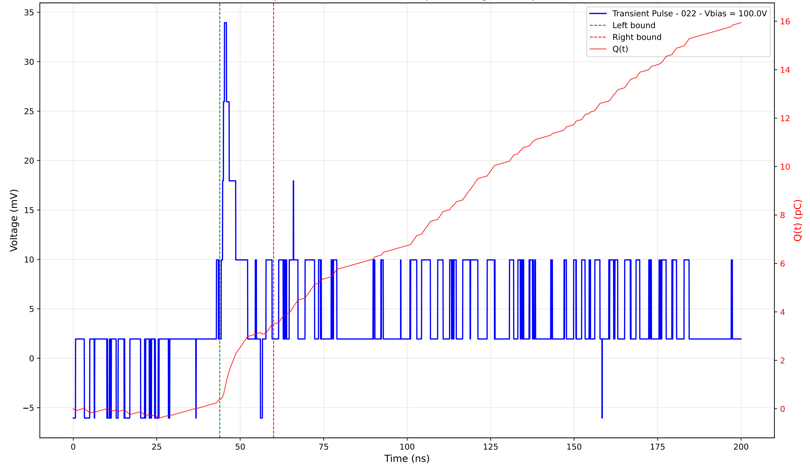
Transient Pulse - Sample: 4003 - Position: 310.0 \mu\text{m} - Charge: 3.11 pC - Rise Time: 1.00 ns
