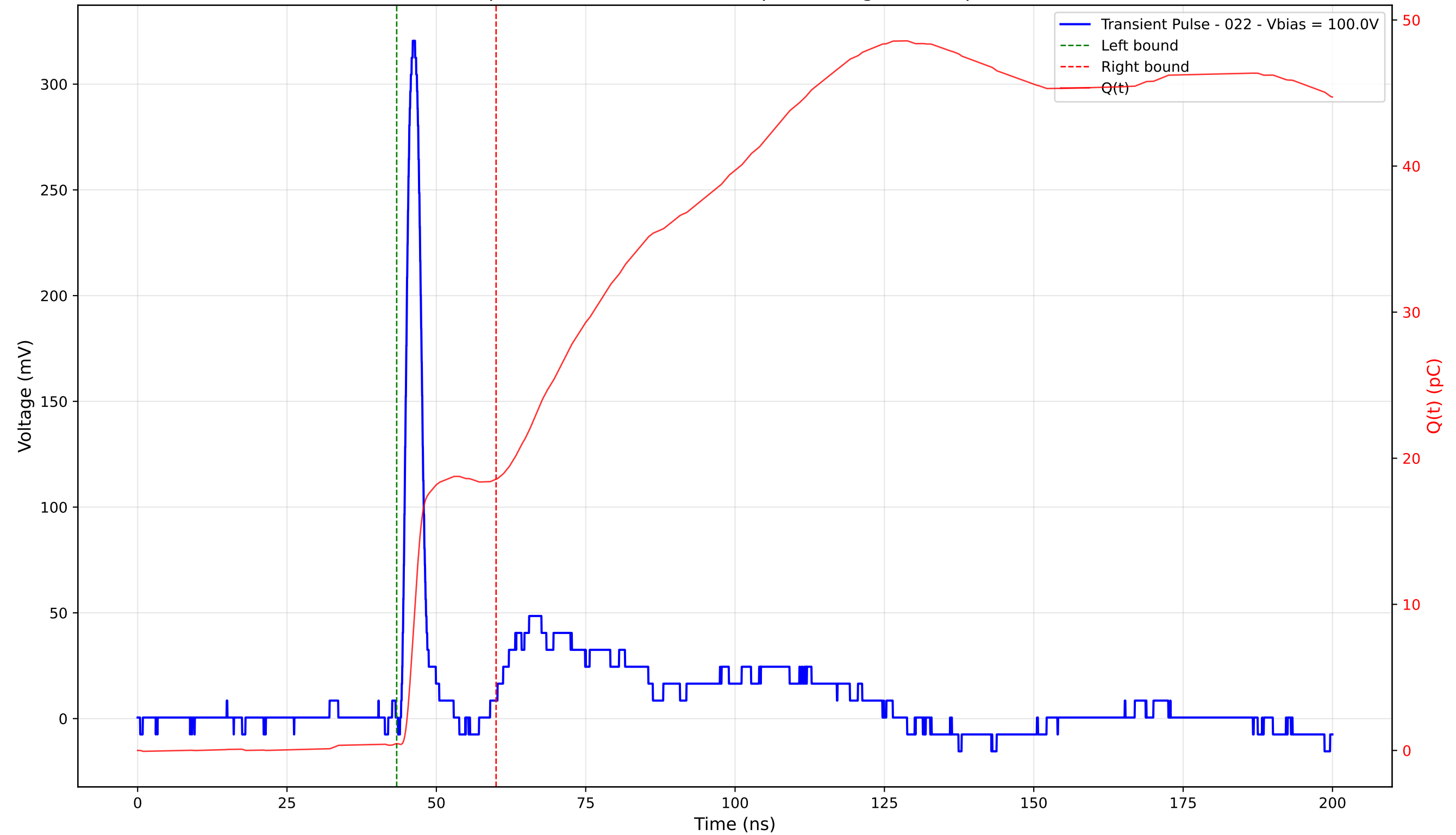
Transient Pulse - Sample: 4003 - Position: 210.0 \mu\text{m} - Charge: 18.10 pC - Rise Time: 1.20 ns
