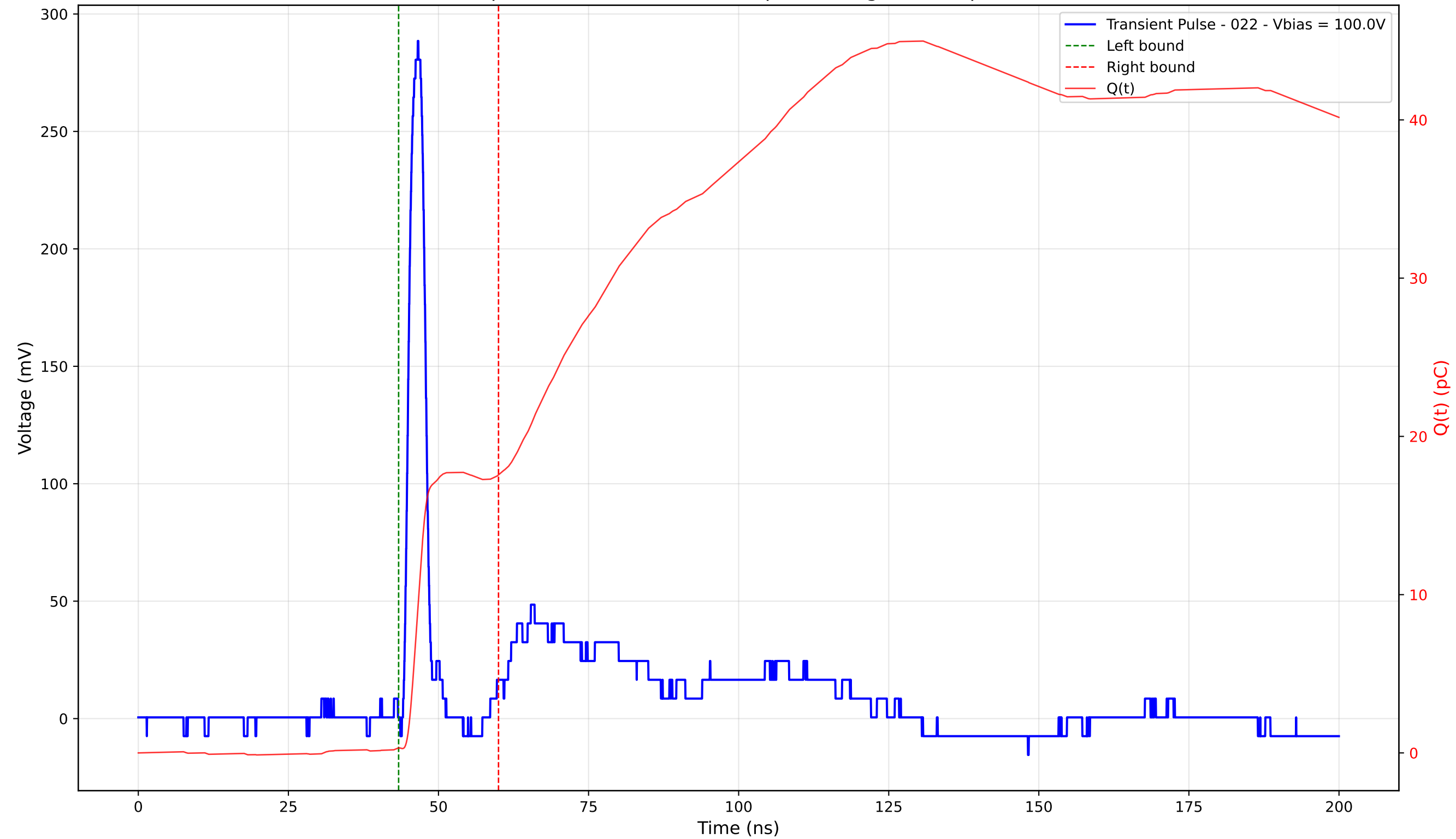
Transient Pulse - Sample: 4003 - Position: 220.0 \mu\text{m} - Charge: 17.26 pC - Rise Time: 1.45 ns
