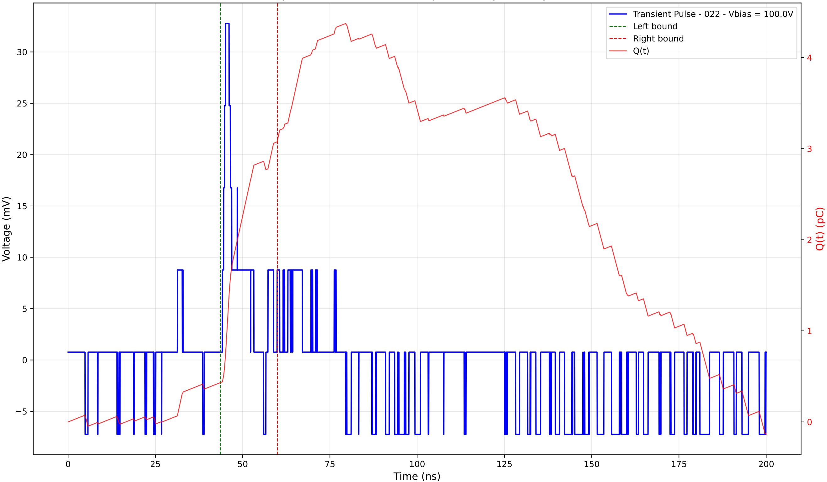
Transient Pulse - Sample: 4003 - Position: 85.0 \mu\text{m} - Charge: 2.66 pC - Rise Time: 0.89 ns
