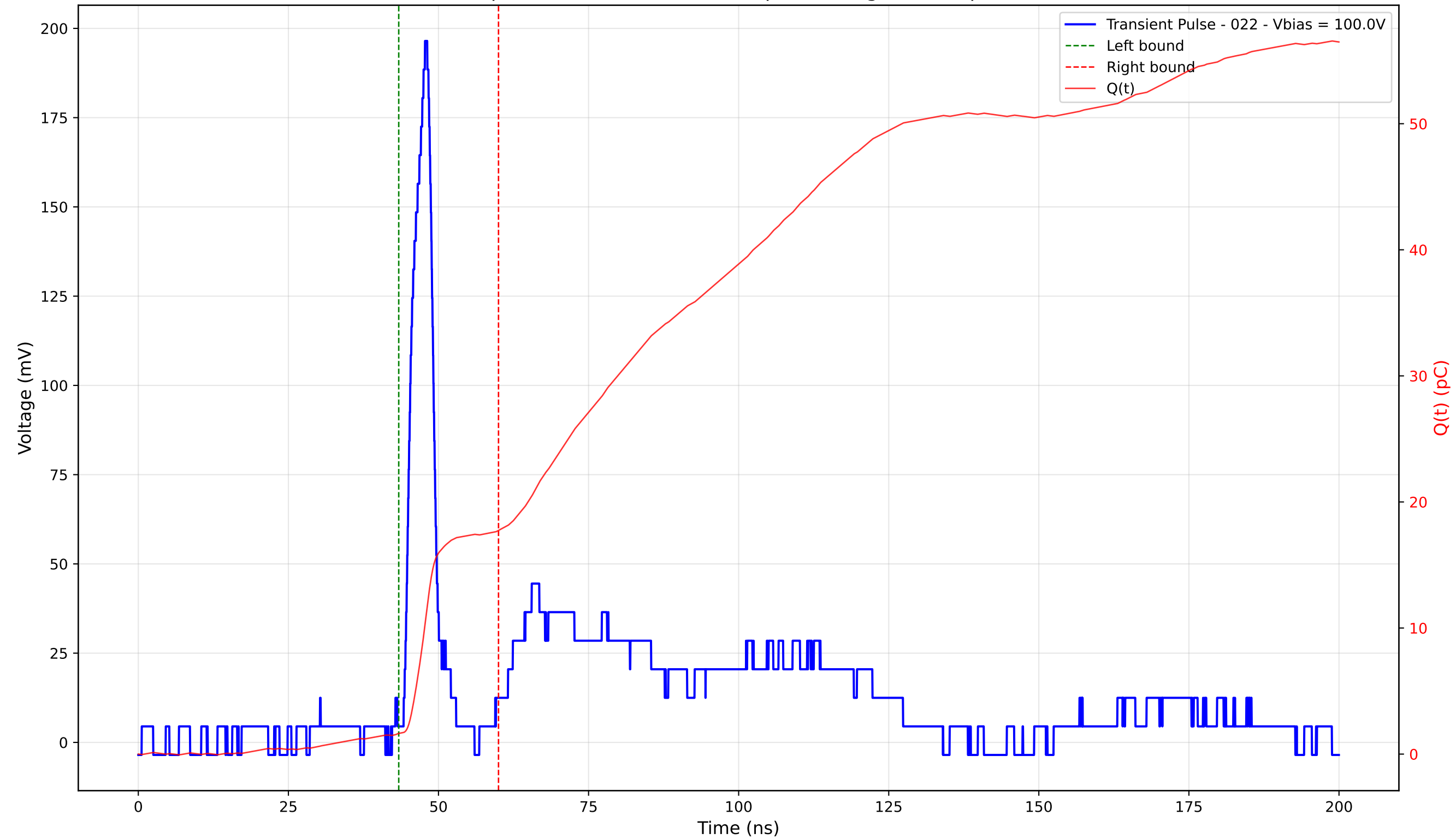
Transient Pulse - Sample: 4003 - Position: 245.0 \mu\text{m} - Charge: 16.10 pC - Rise Time: 2.94 ns
