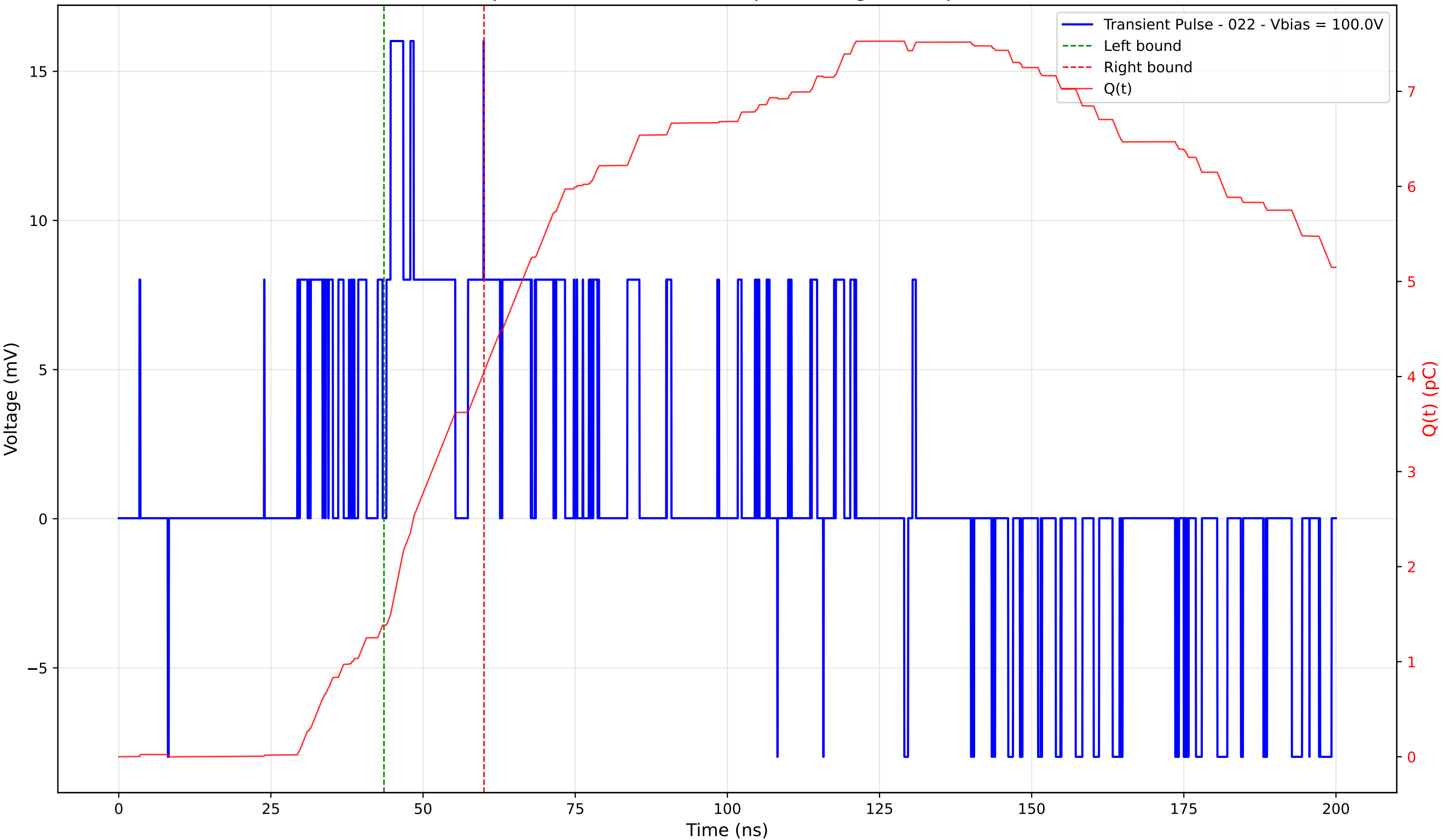
Transient Pulse - Sample: 4003 - Position: 70.0 \mu\text{m} - Charge: 2.67 pC - Rise Time: 0.70 ns
