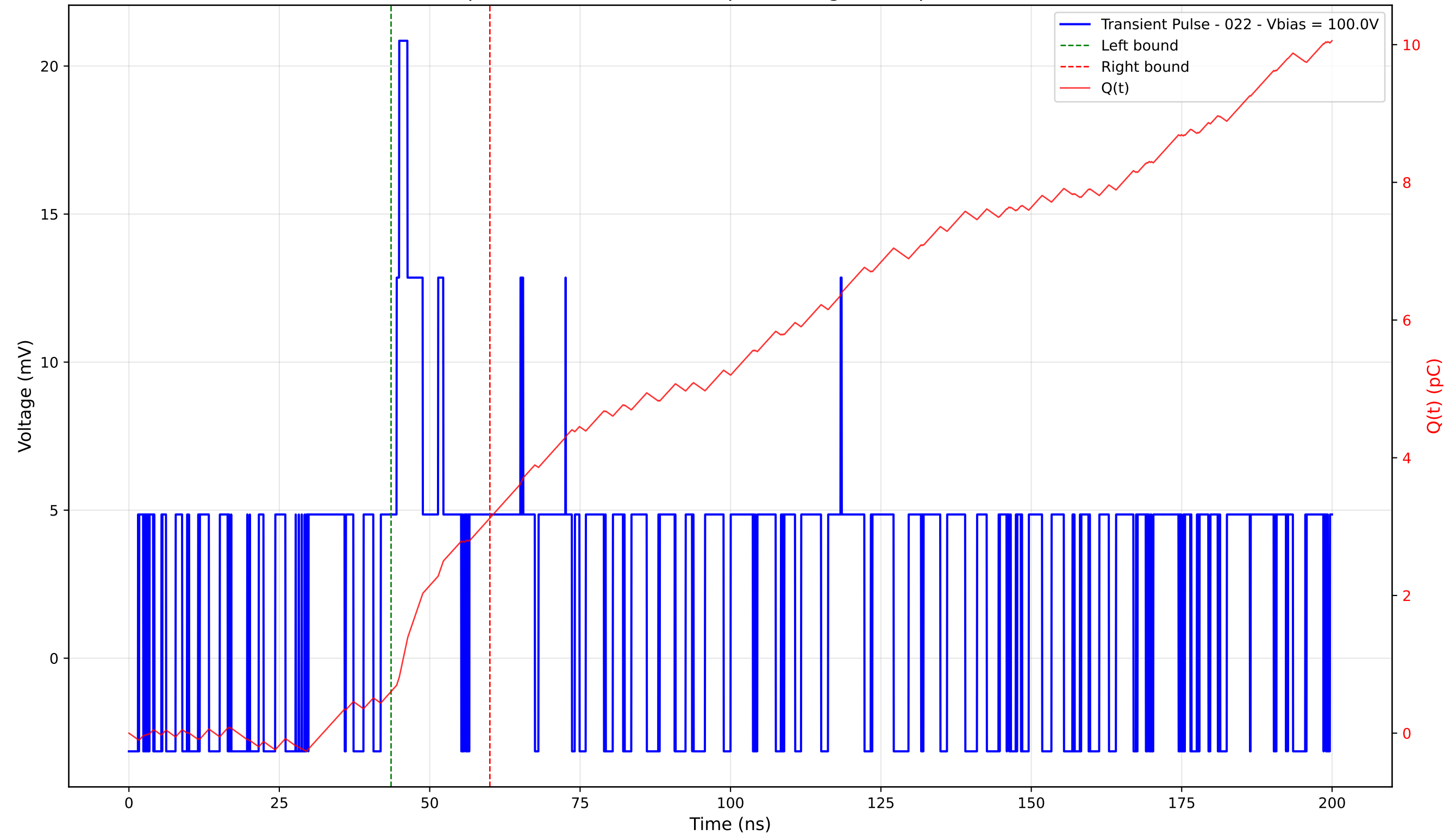
Transient Pulse - Sample: 4003 - Position: 25.0 \mu\text{m} - Charge: 2.52 pC - Rise Time: 0.00 ns (N/A)
