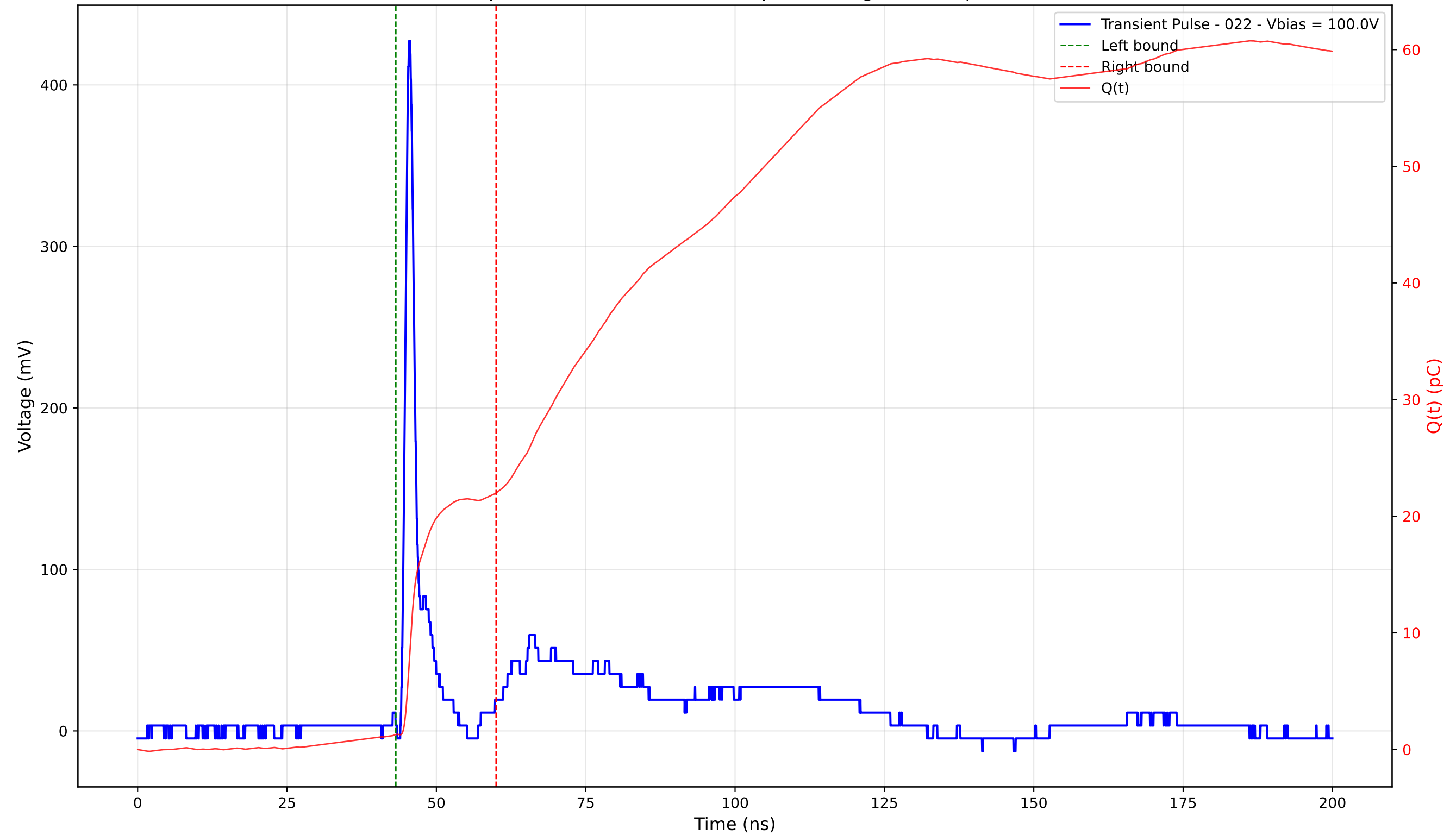
Transient Pulse - Sample: 4003 - Position: 135.0 \mu\text{m} - Charge: 20.70 pC - Rise Time: 0.96 ns
