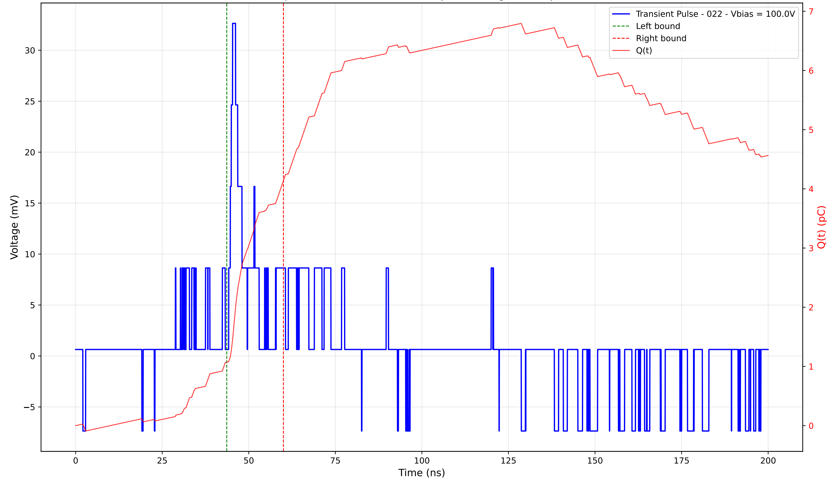
Transient Pulse - Sample: 4003 - Position: 330.0 \mu\text{m} - Charge: 3.07 pC - Rise Time: 1.13 ns
