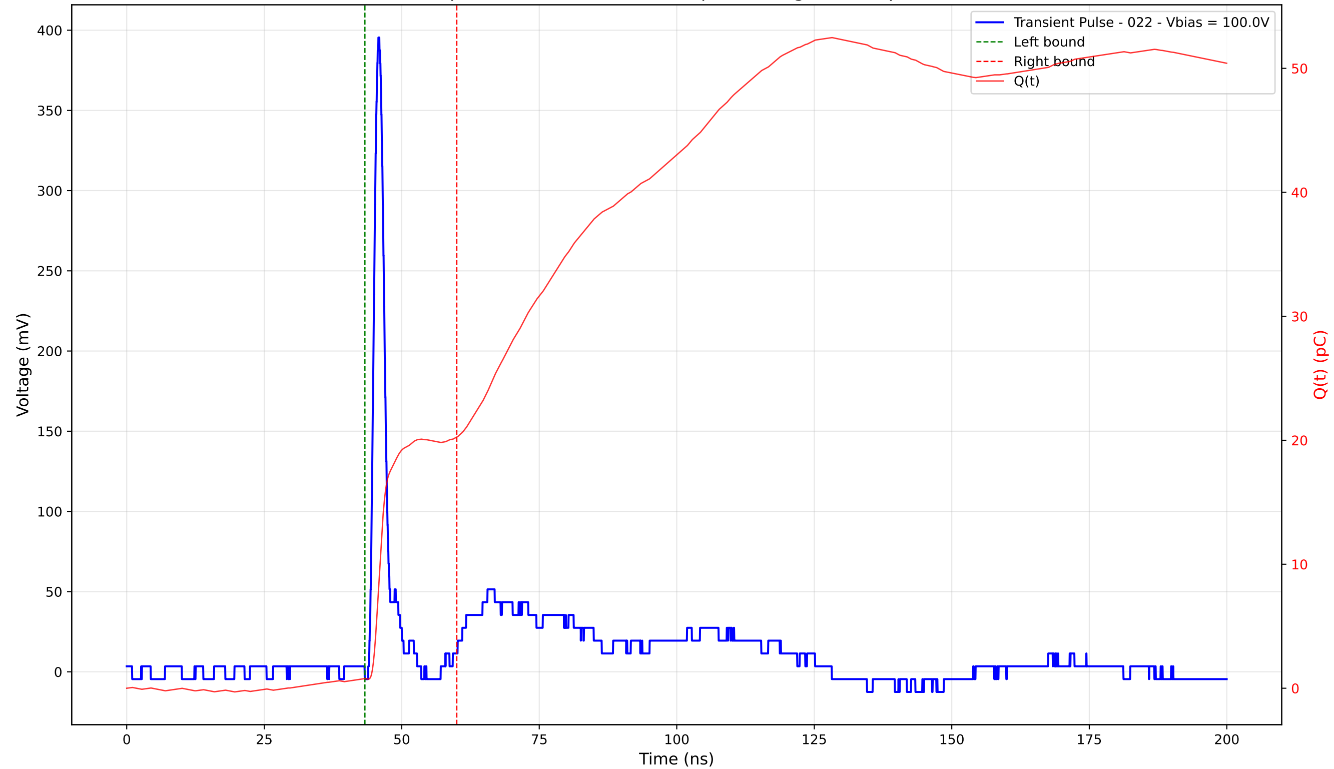
Transient Pulse - Sample: 4003 - Position: 185.0 \mu\text{m} - Charge: 19.47 pC - Rise Time: 1.17 ns
