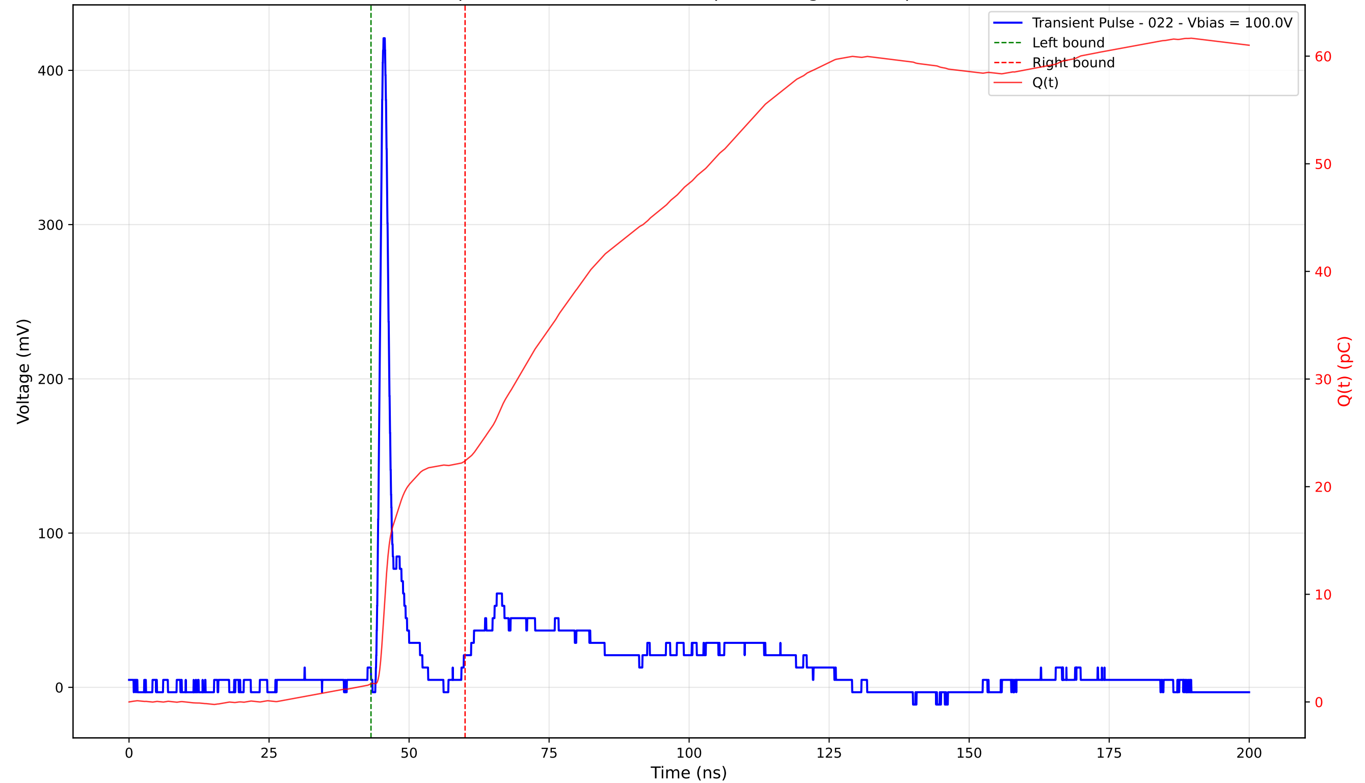
Transient Pulse - Sample: 4003 - Position: 140.0 \mu\text{m} - Charge: 20.70 pC - Rise Time: 0.95 ns
