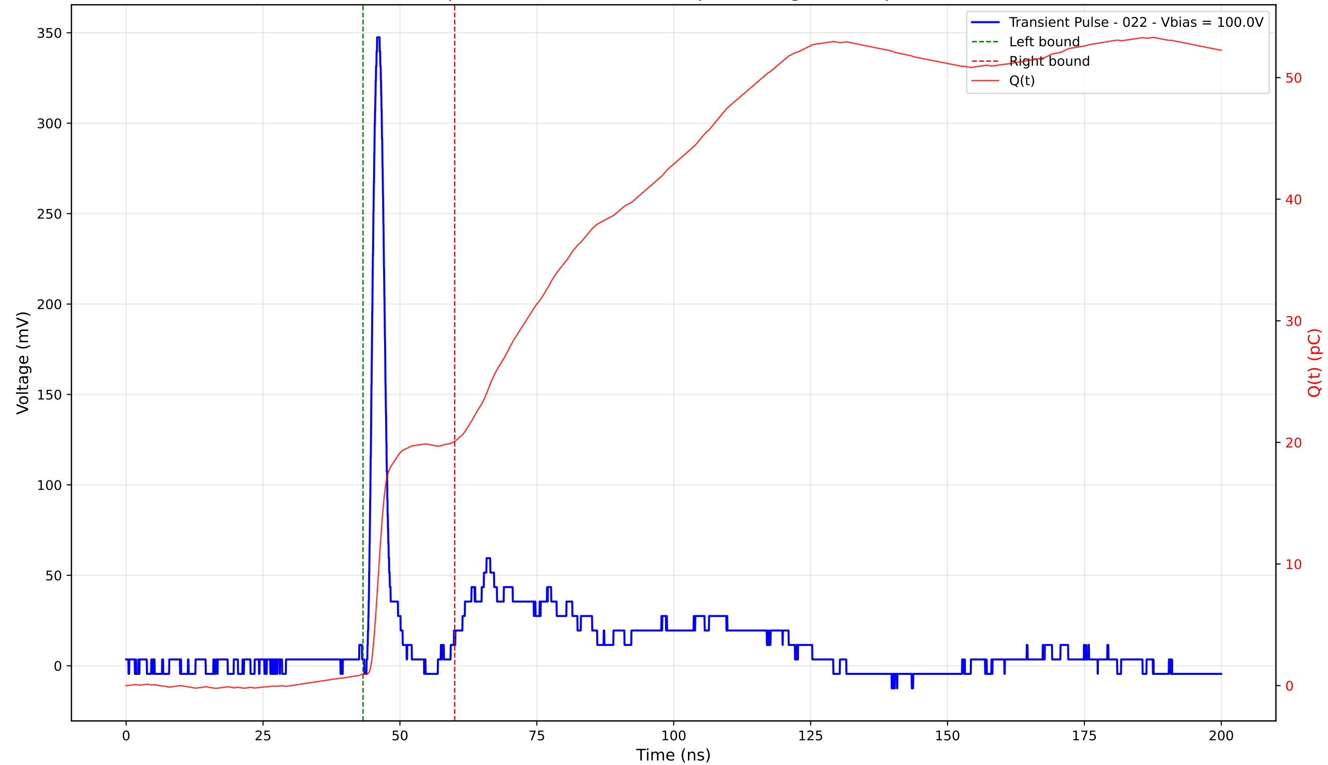
Transient Pulse - Sample: 4003 - Position: 200.0 \mu\text{m} - Charge: 19.13 pC - Rise Time: 1.22 ns
