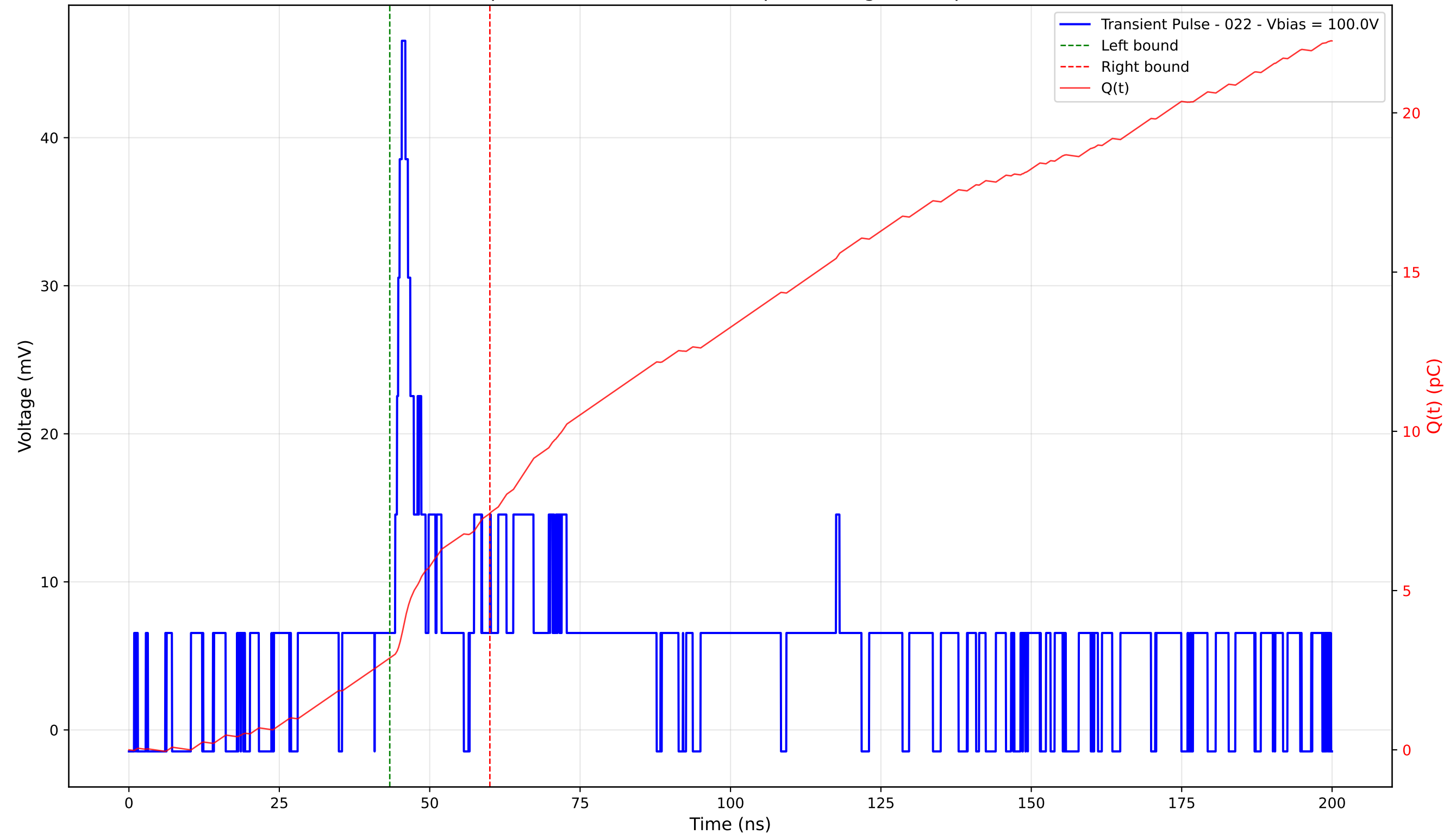
Transient Pulse - Sample: 4003 - Position: 395.0 \mu\text{m} - Charge: 4.54 pC - Rise Time: 4.51 ns
