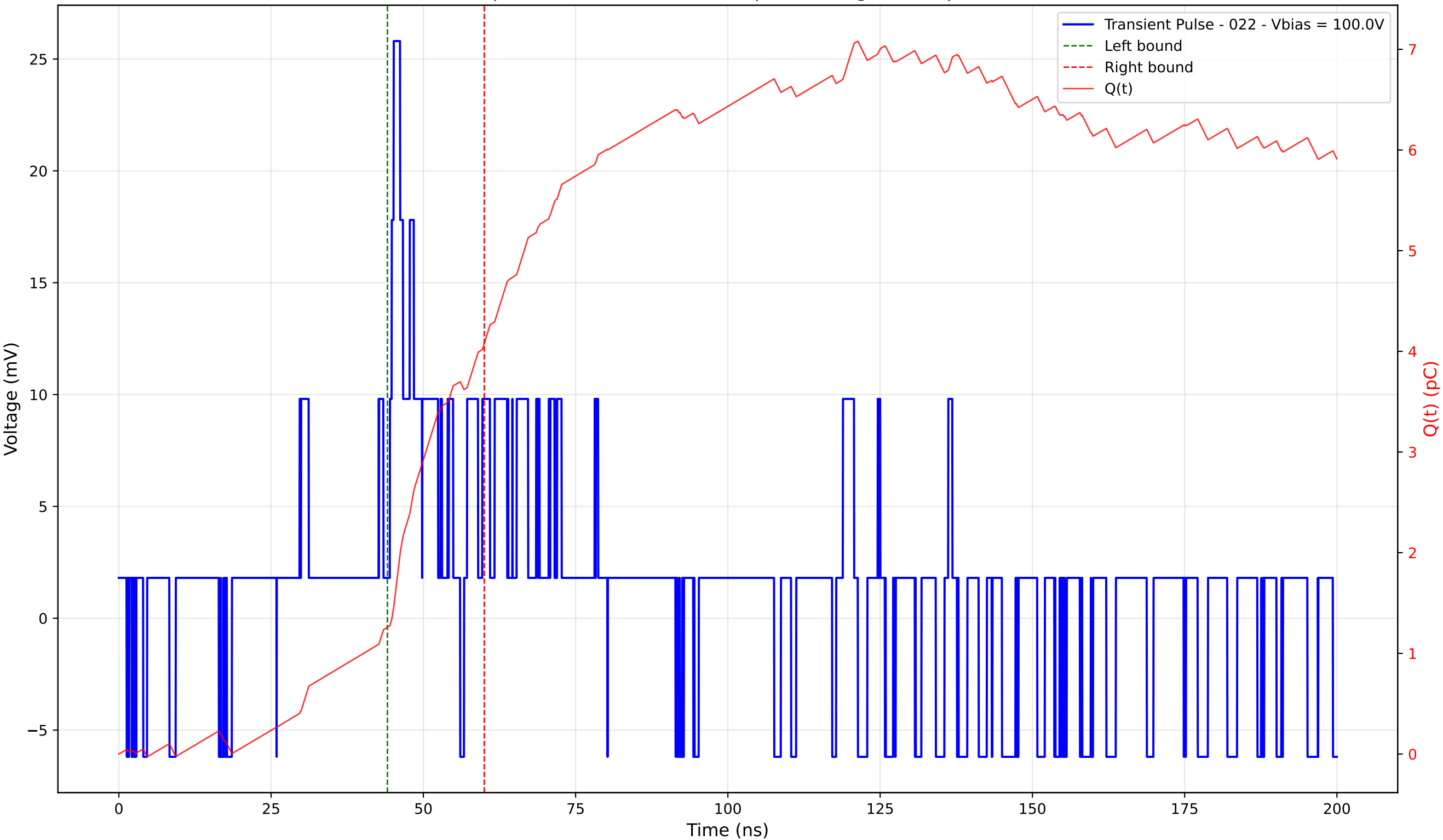
Transient Pulse - Sample: 4003 - Position: 30.0 \mu\text{m} - Charge: 2.82 pC - Rise Time: 0.64 ns
