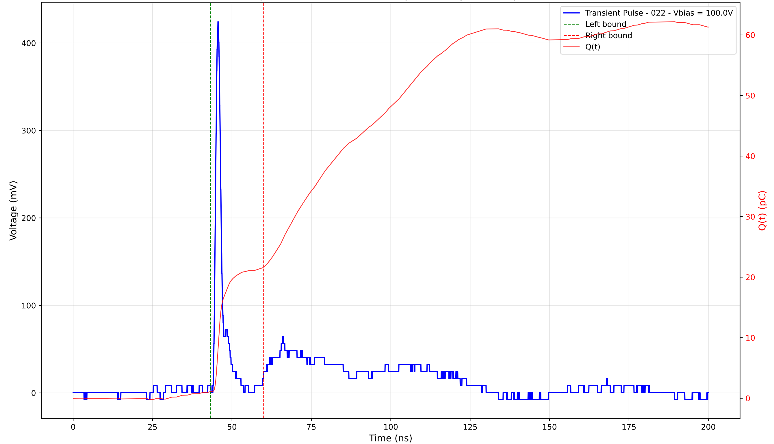
Transient Pulse - Sample: 4003 - Position: 155.0 \mu\text{m} - Charge: 20.55 pC - Rise Time: 0.99 ns
