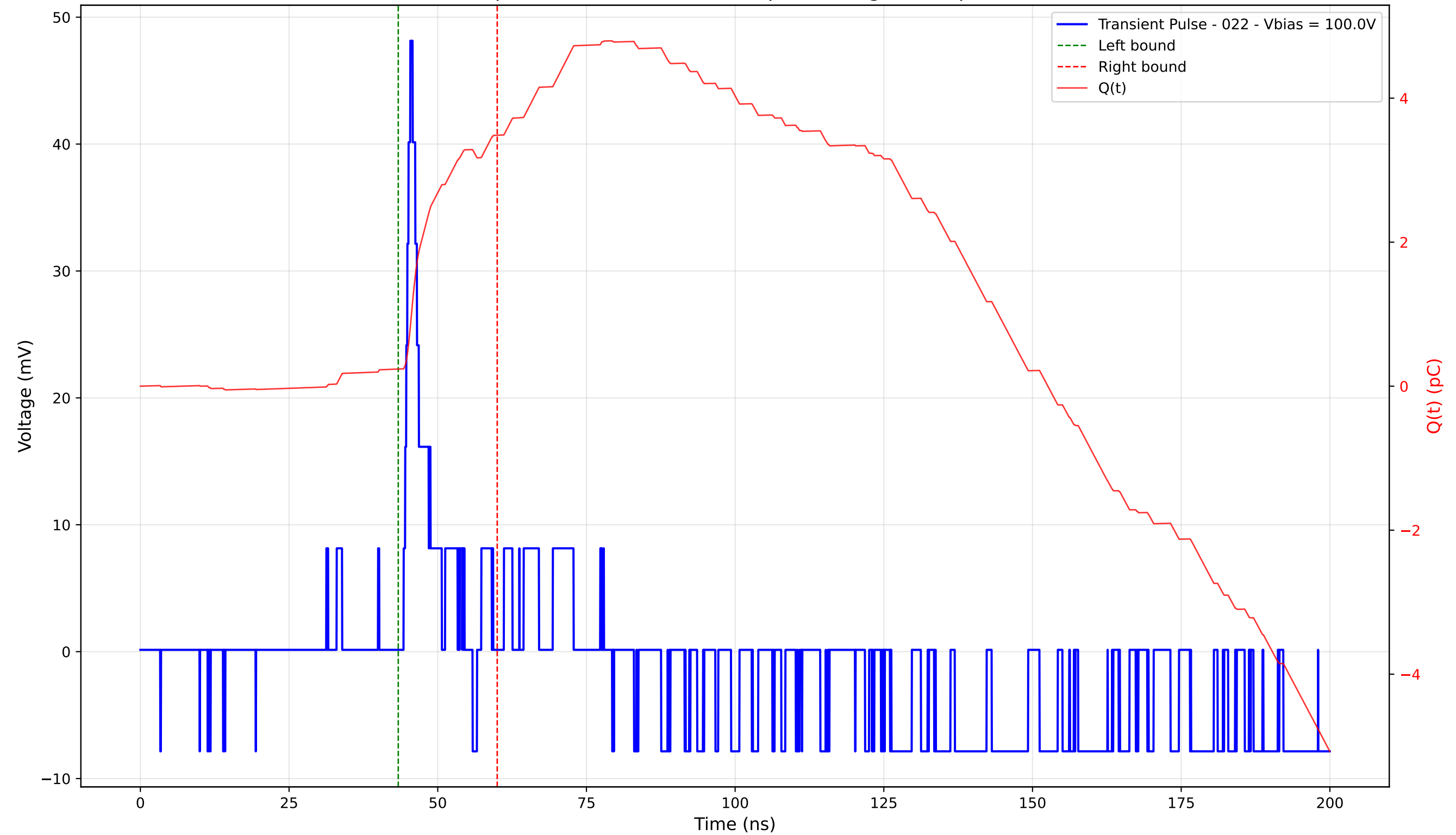
Transient Pulse - Sample: 4003 - Position: 390.0 \mu\text{m} - Charge: 3.25 pC - Rise Time: 1.13 ns
