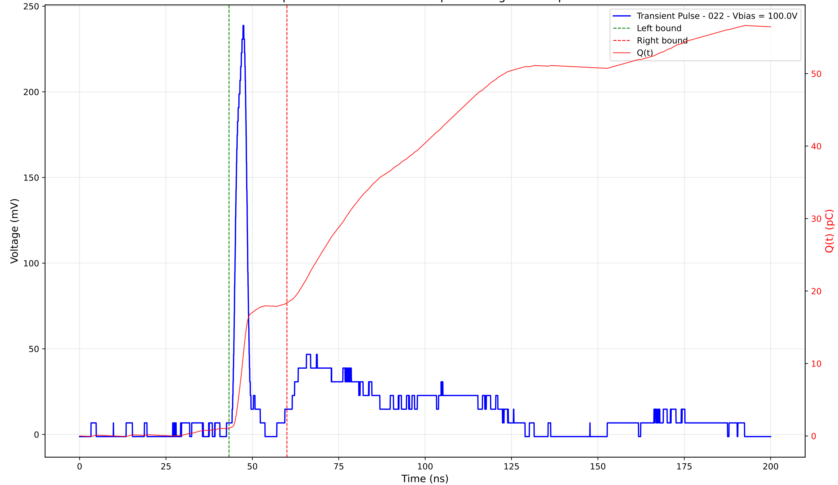
Transient Pulse - Sample: 4003 - Position: 235.0 \mu\text{m} - Charge: 17.26 pC - Rise Time: 2.42 ns
