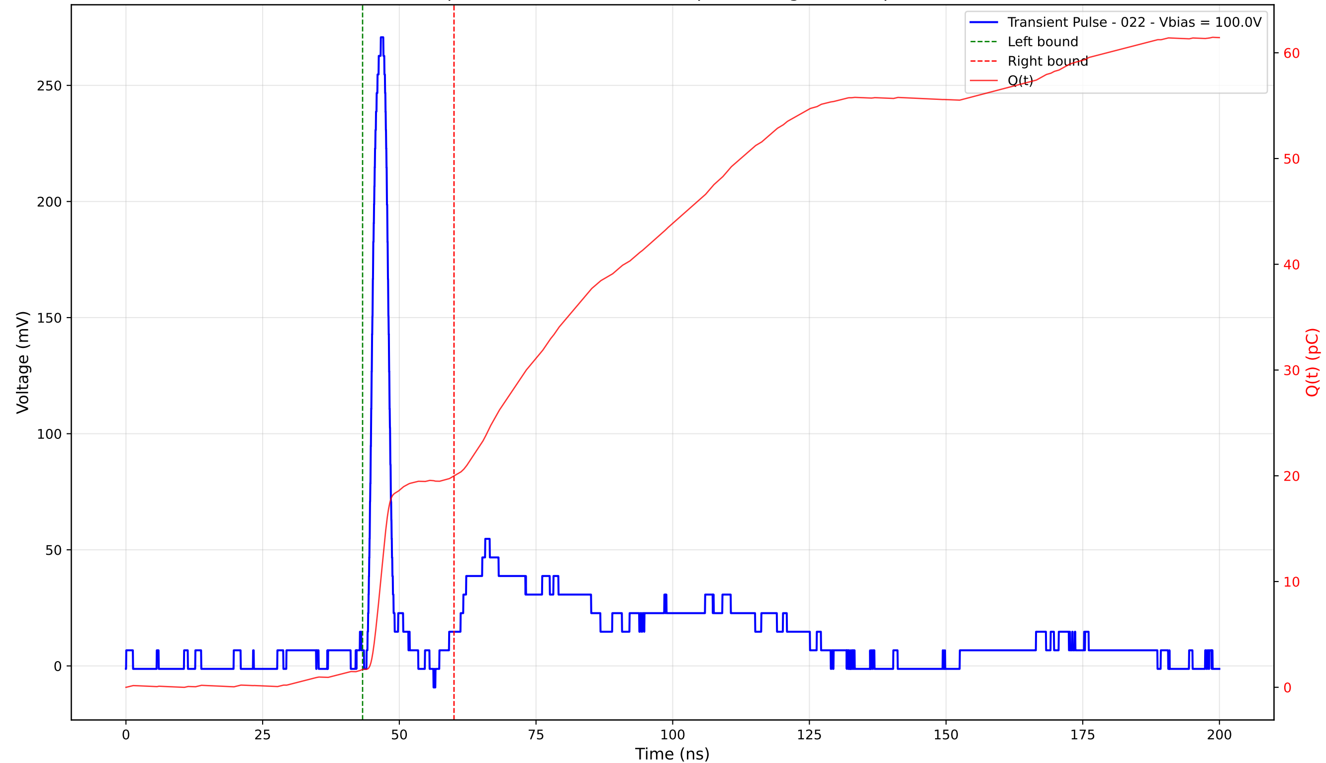
Transient Pulse - Sample: 4003 - Position: 225.0 \mu\text{m} - Charge: 18.30 pC - Rise Time: 1.49 ns
