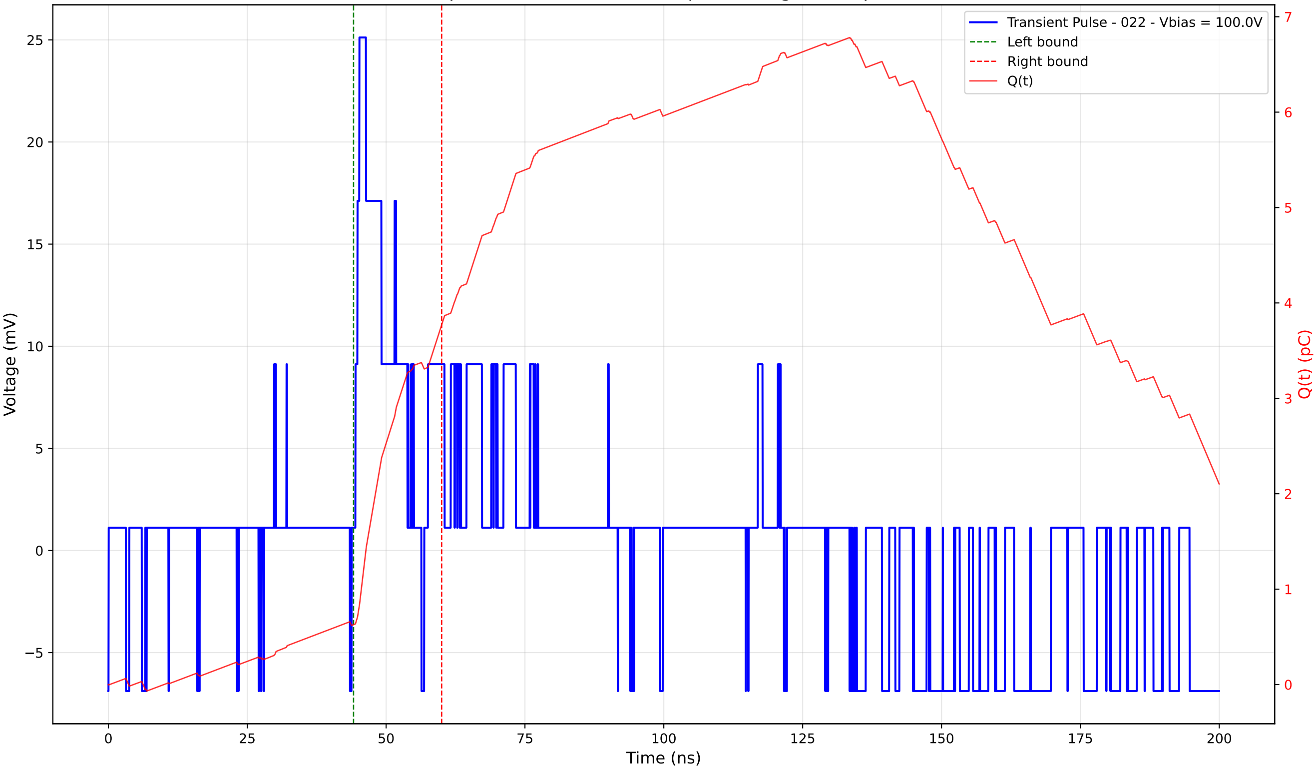
Transient Pulse - Sample: 4003 - Position: 65.0 \mu\text{m} - Charge: 3.15 pC - Rise Time: 0.72 ns
