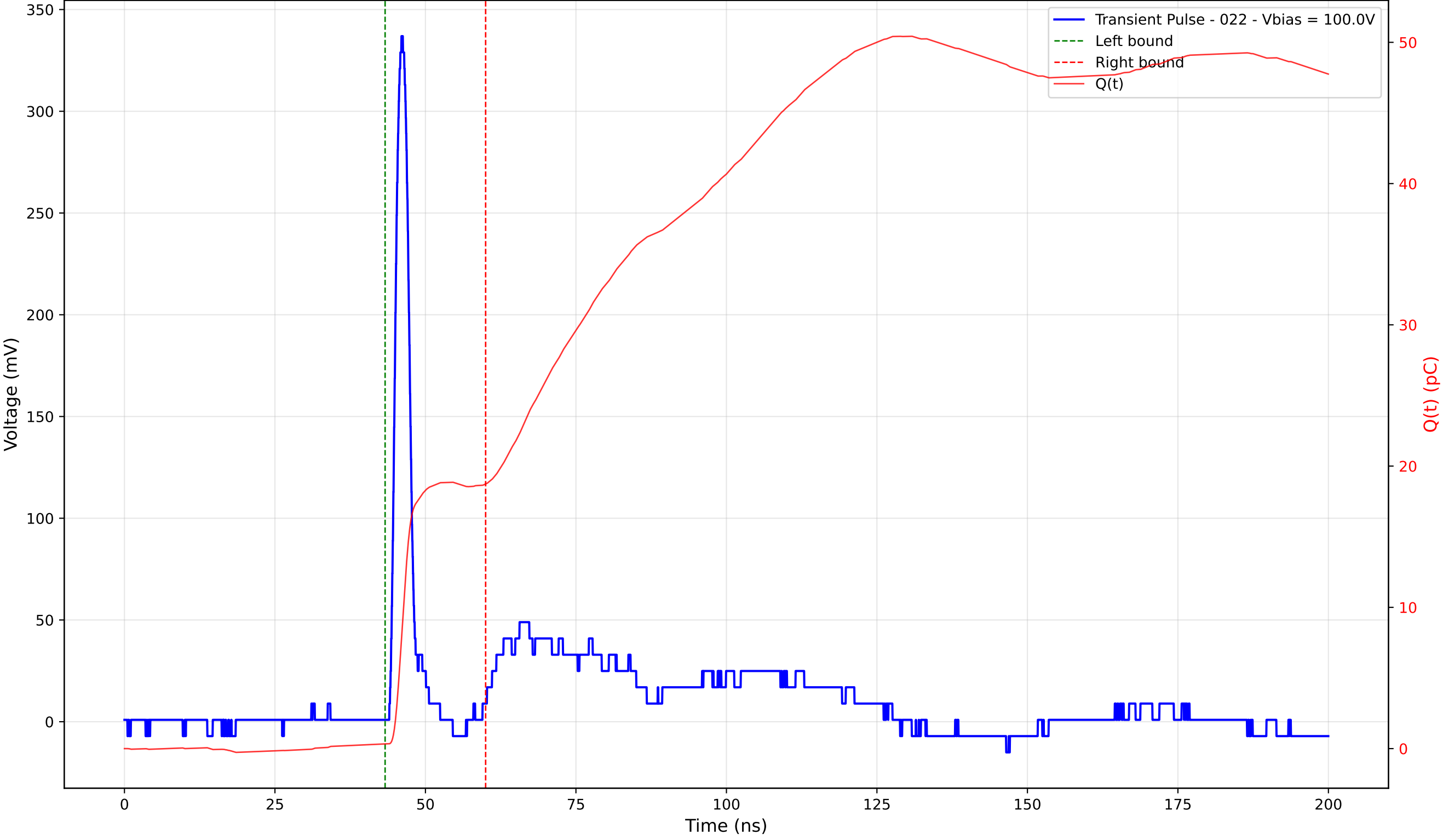
Transient Pulse - Sample: 4003 - Position: 205.0 \mu\text{m} - Charge: 18.41 pC - Rise Time: 1.26 ns
