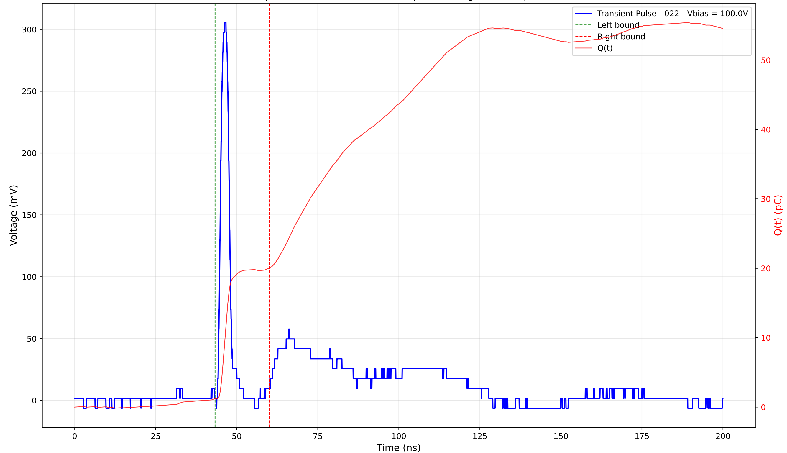
Transient Pulse - Sample: 4003 - Position: 215.0 \mu\text{m} - Charge: 18.80 pC - Rise Time: 1.37 ns
