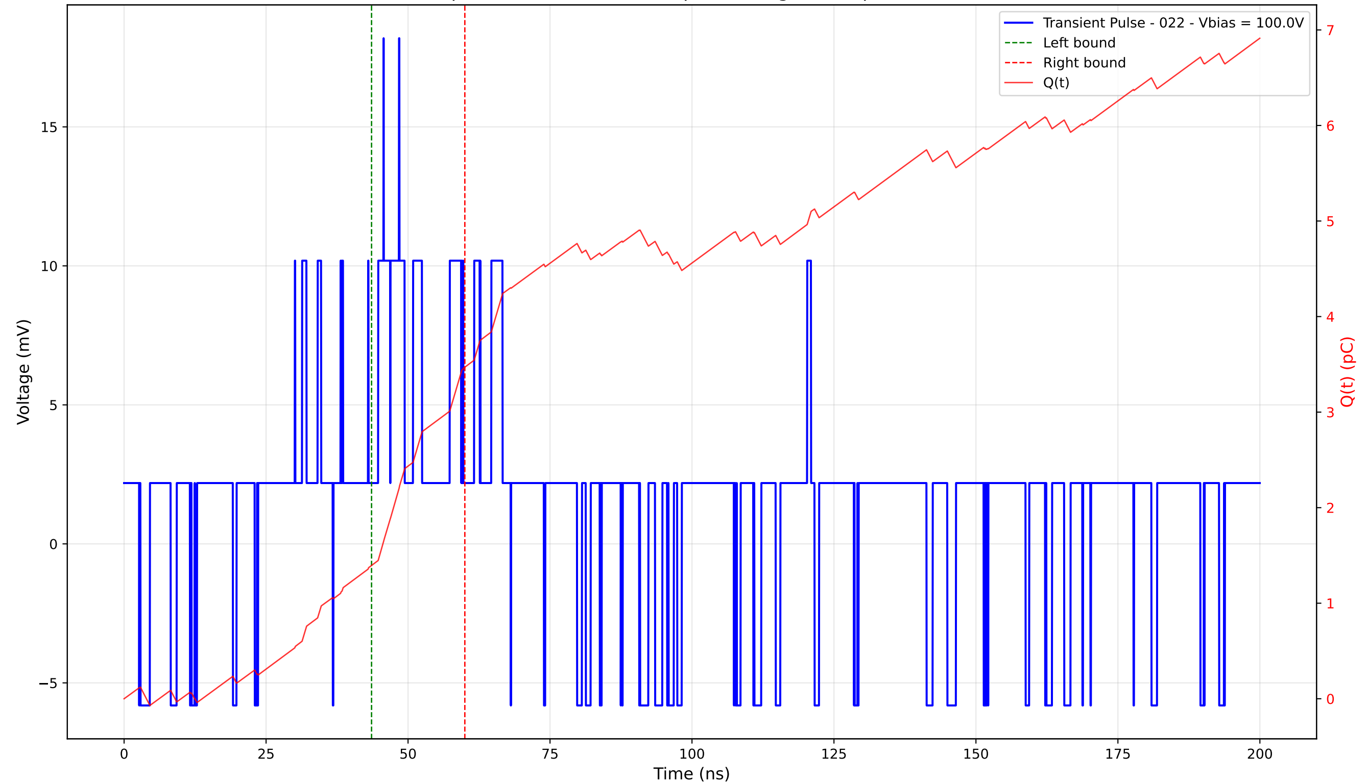
Transient Pulse - Sample: 4003 - Position: 5.0 \mu\text{m} - Charge: 2.08 pC - Rise Time: 0.00 ns (N/A)
