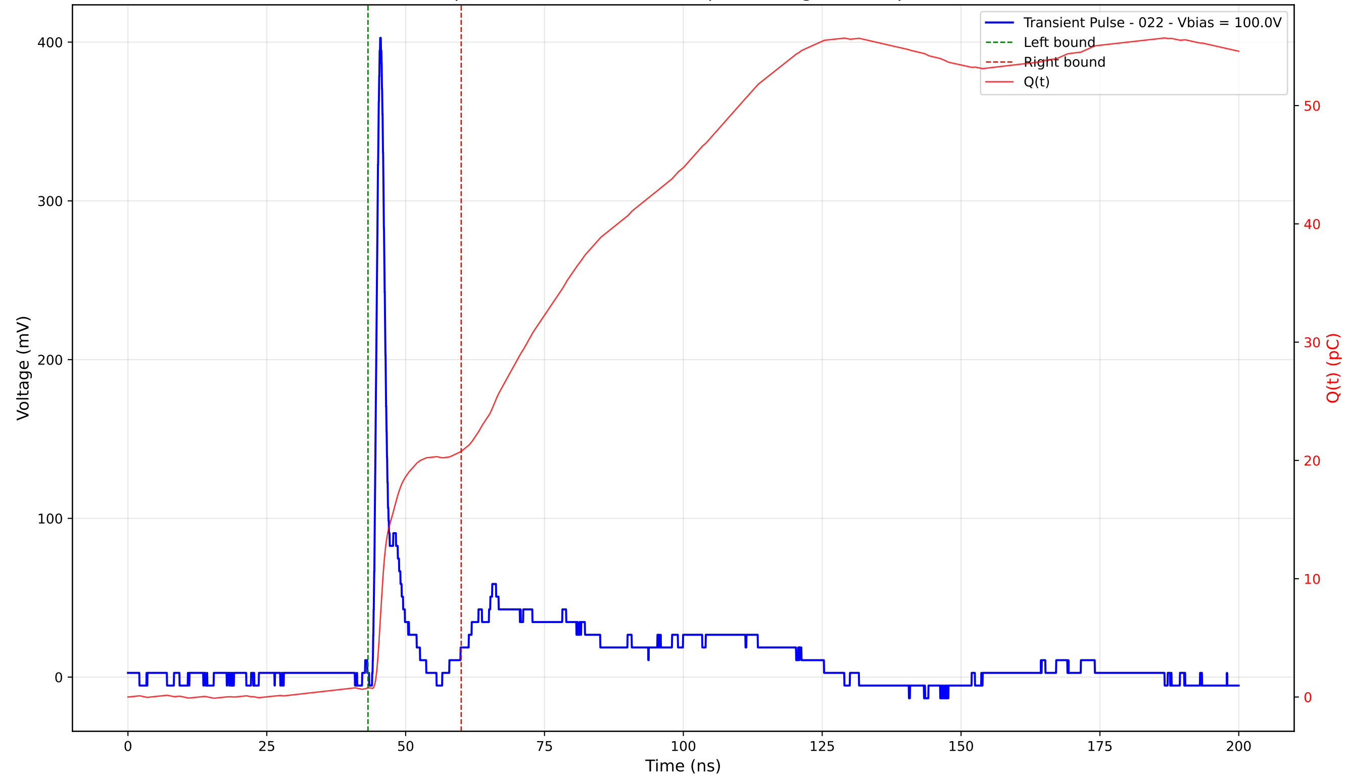
Transient Pulse - Sample: 4003 - Position: 125.0 \mu\text{m} - Charge: 19.99 pC - Rise Time: 0.93 ns
