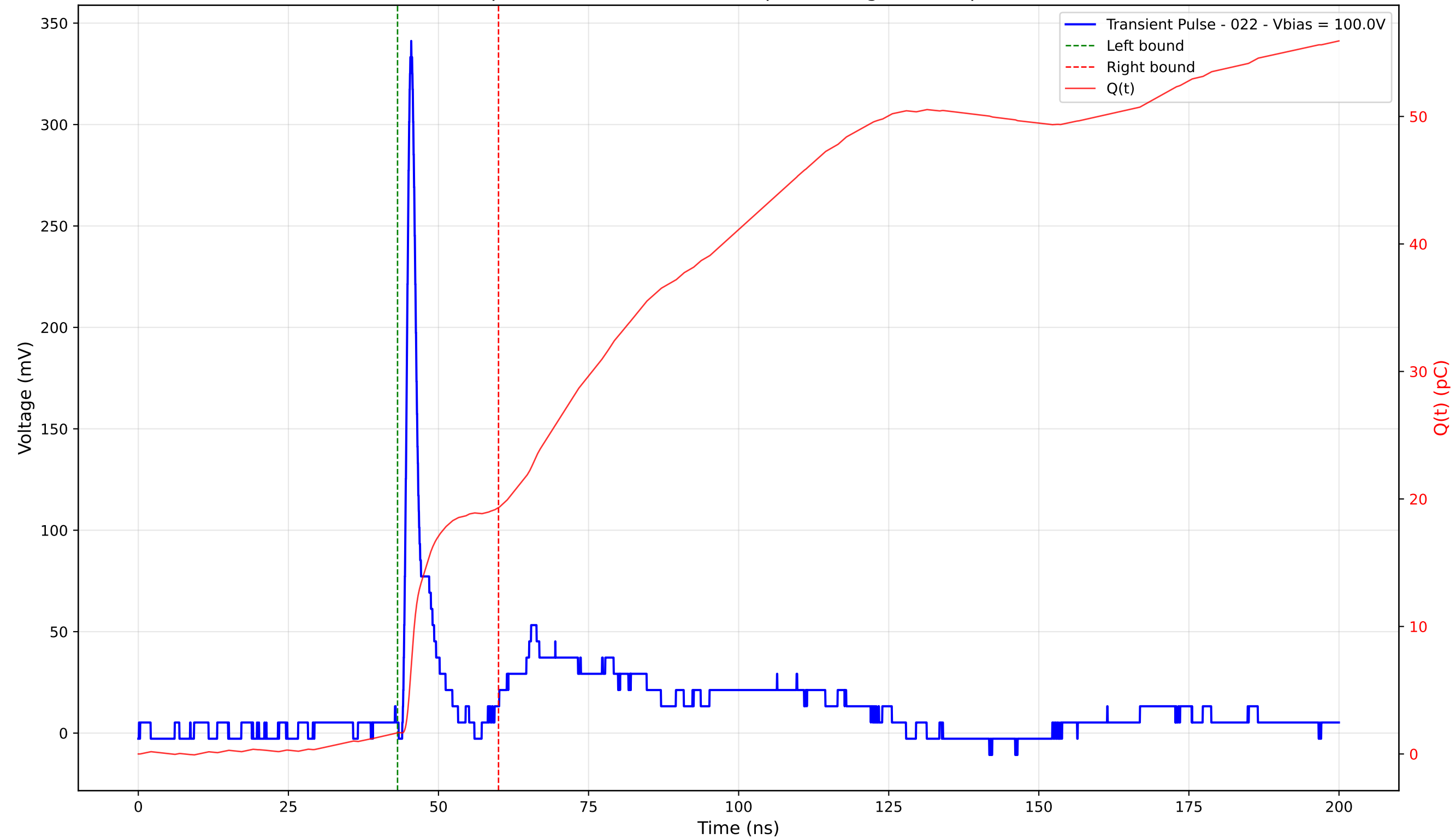
Transient Pulse - Sample: 4003 - Position: 115.0 \mu\text{m} - Charge: 17.65 pC - Rise Time: 0.95 ns
