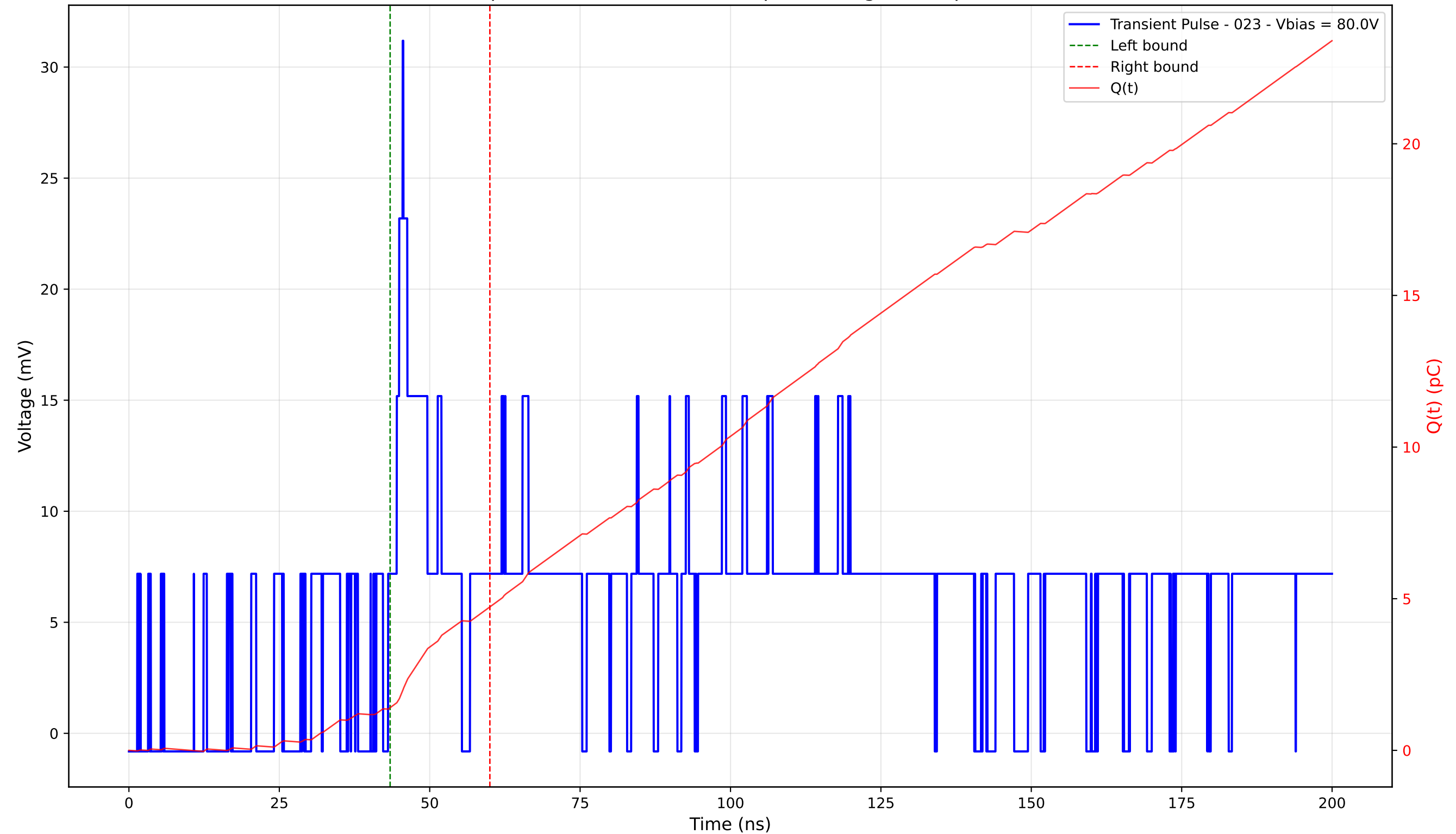
Transient Pulse - Sample: 4003 - Position: 350.0 \mu\text{m} - Charge: 3.32 pC - Rise Time: 2.43 ns
