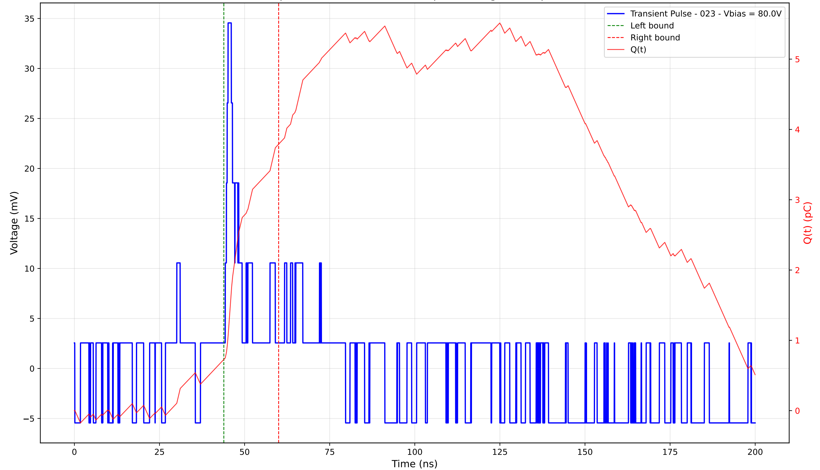
Transient Pulse - Sample: 4003 - Position: 390.0 \mu\text{m} - Charge: 3.06 pC - Rise Time: 0.84 ns
