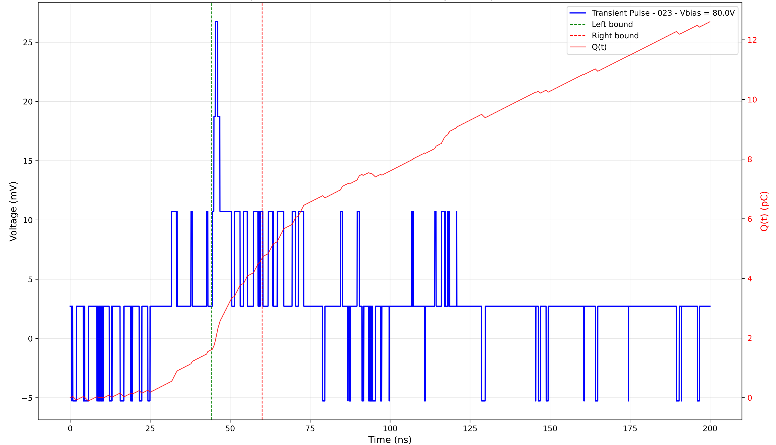
Transient Pulse - Sample: 4003 - Position: 40.0 \mu\text{m} - Charge: 3.07 pC - Rise Time: 0.00 ns (N/A)
