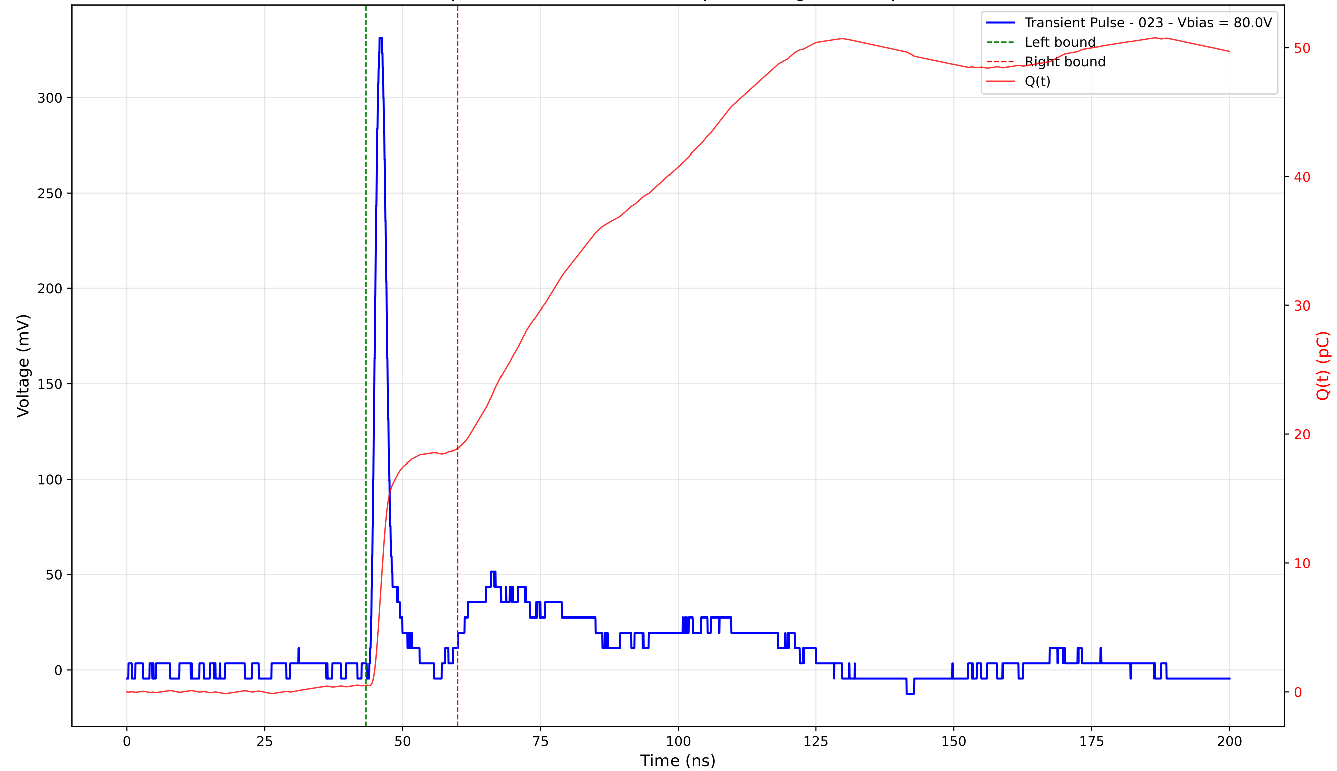
Transient Pulse - Sample: 4003 - Position: 185.0 \mu\text{m} - Charge: 18.35 pC - Rise Time: 1.17 ns
