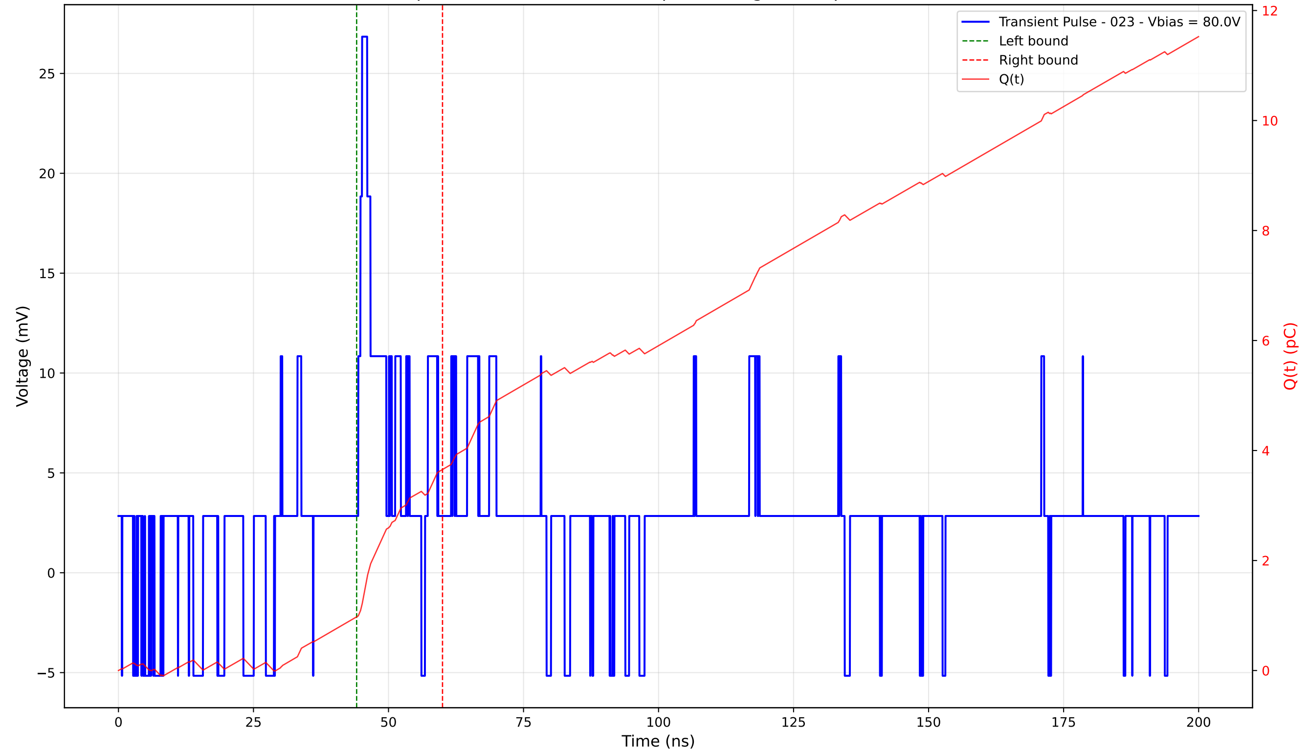
Transient Pulse - Sample: 4003 - Position: 380.0 \mu\text{m} - Charge: 2.68 pC - Rise Time: 0.00 ns (N/A)
