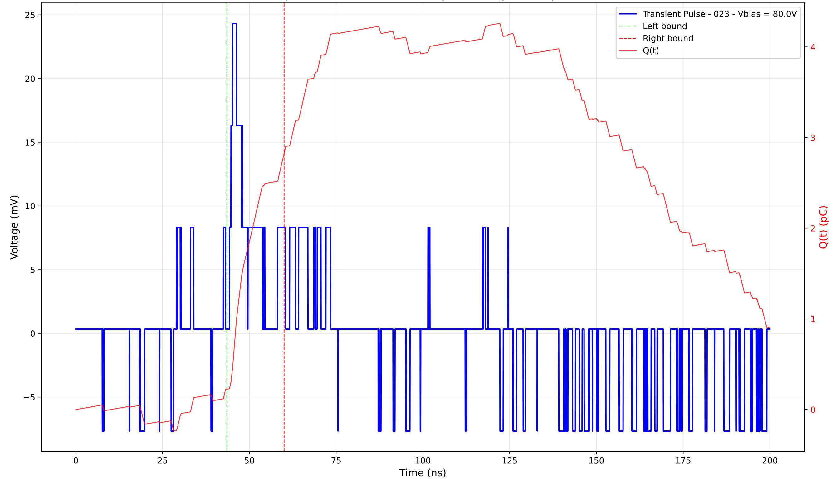
Transient Pulse - Sample: 4003 - Position: 375.0 \mu\text{m} - Charge: 2.60 pC - Rise Time: 0.89 ns
