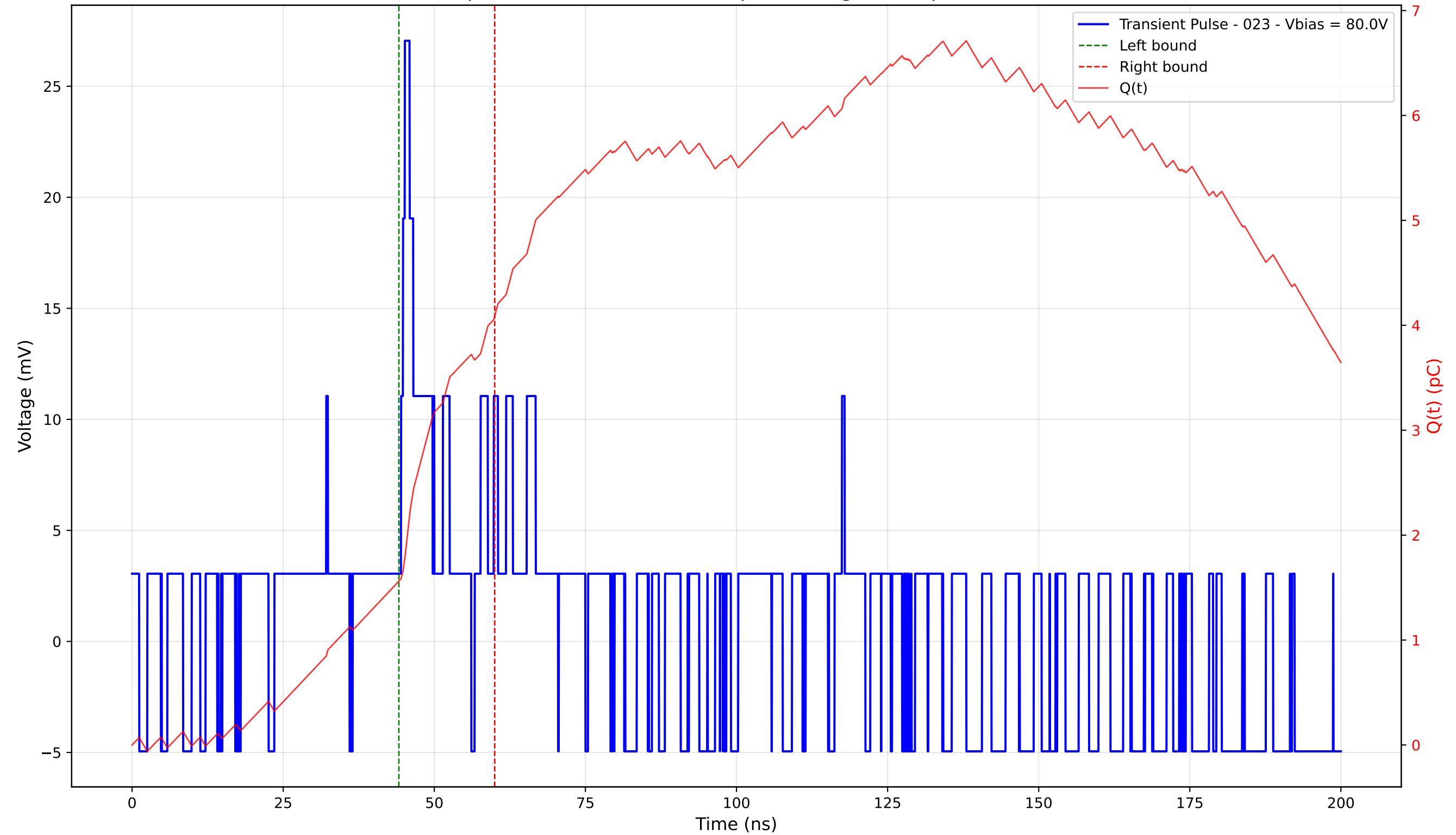
Transient Pulse - Sample: 4003 - Position: 415.0 \mu\text{m} - Charge: 2.53 pC - Rise Time: 0.00 ns (N/A)
