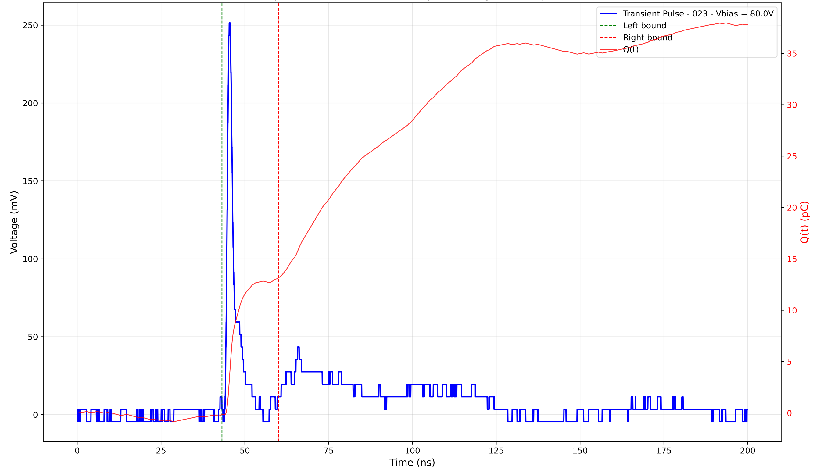
Transient Pulse - Sample: 4003 - Position: 110.0 \mu\text{m} - Charge: 13.28 pC - Rise Time: 0.89 ns
