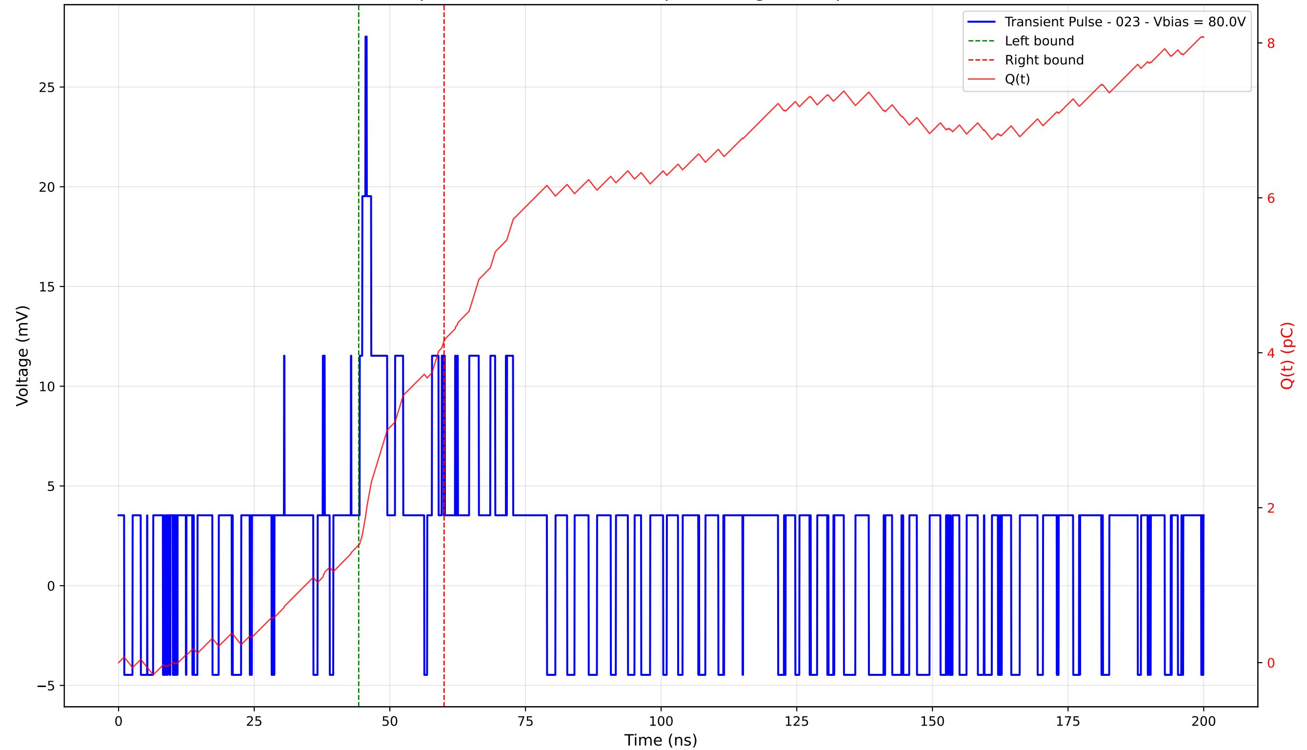
Transient Pulse - Sample: 4003 - Position: 345.0 \mu\text{m} - Charge: 2.63 pC - Rise Time: 0.00 ns (N/A)
