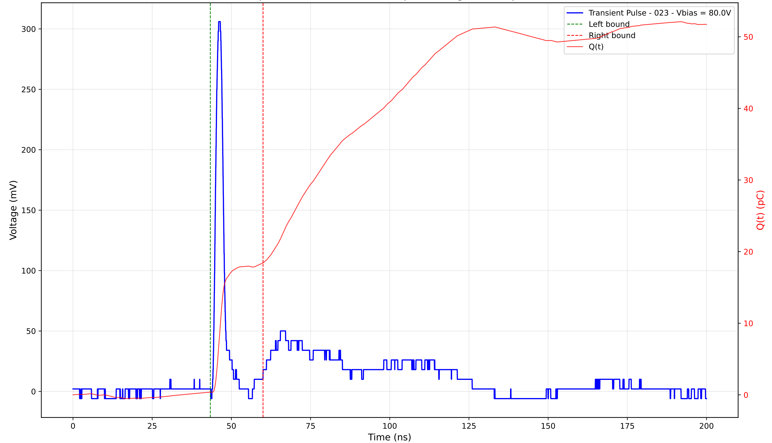
Transient Pulse - Sample: 4003 - Position: 195.0 \mu\text{m} - Charge: 18.02 pC - Rise Time: 1.33 ns
