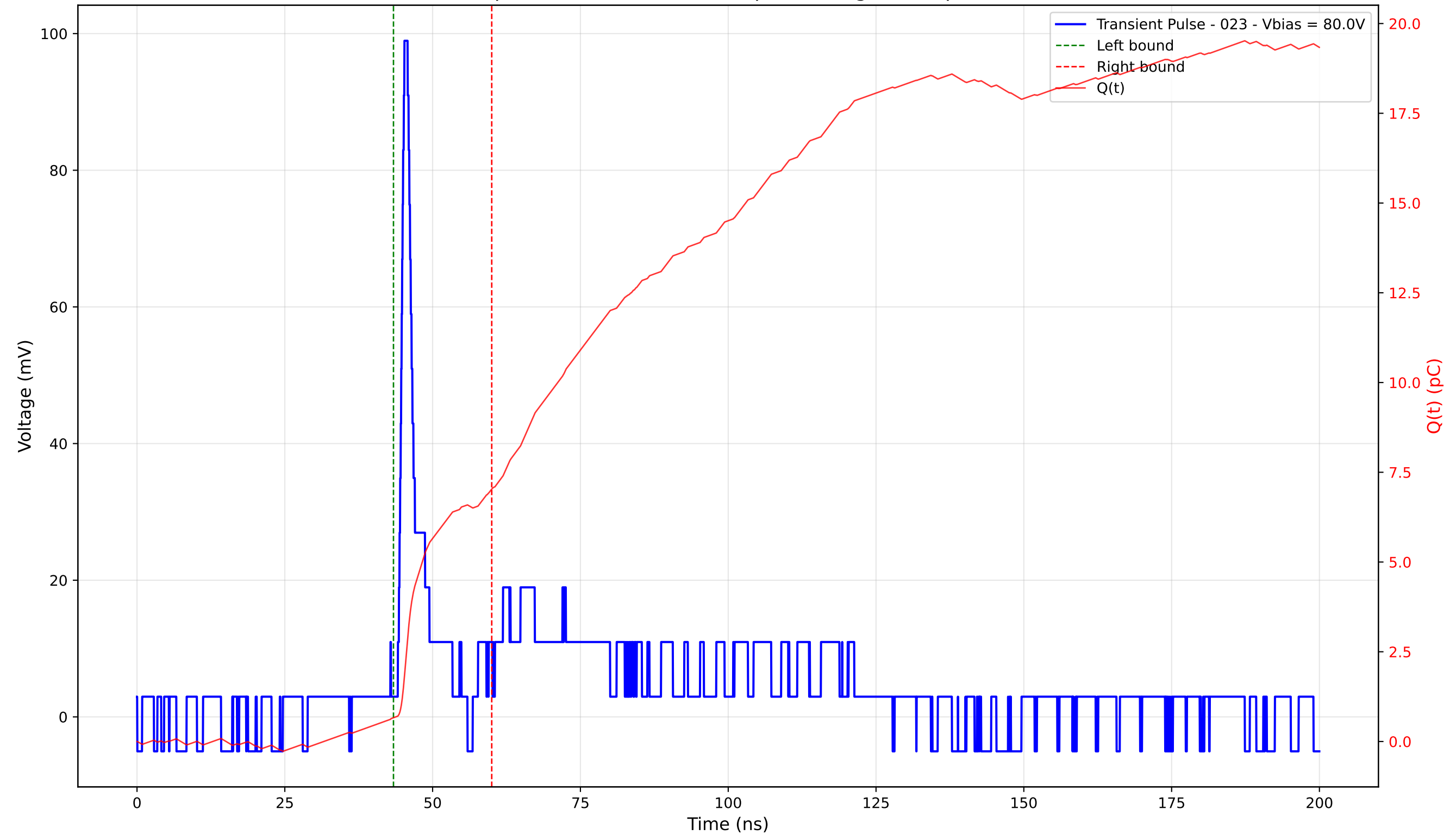
Transient Pulse - Sample: 4003 - Position: 95.0 \mu\text{m} - Charge: 6.37 pC - Rise Time: 1.00 ns
