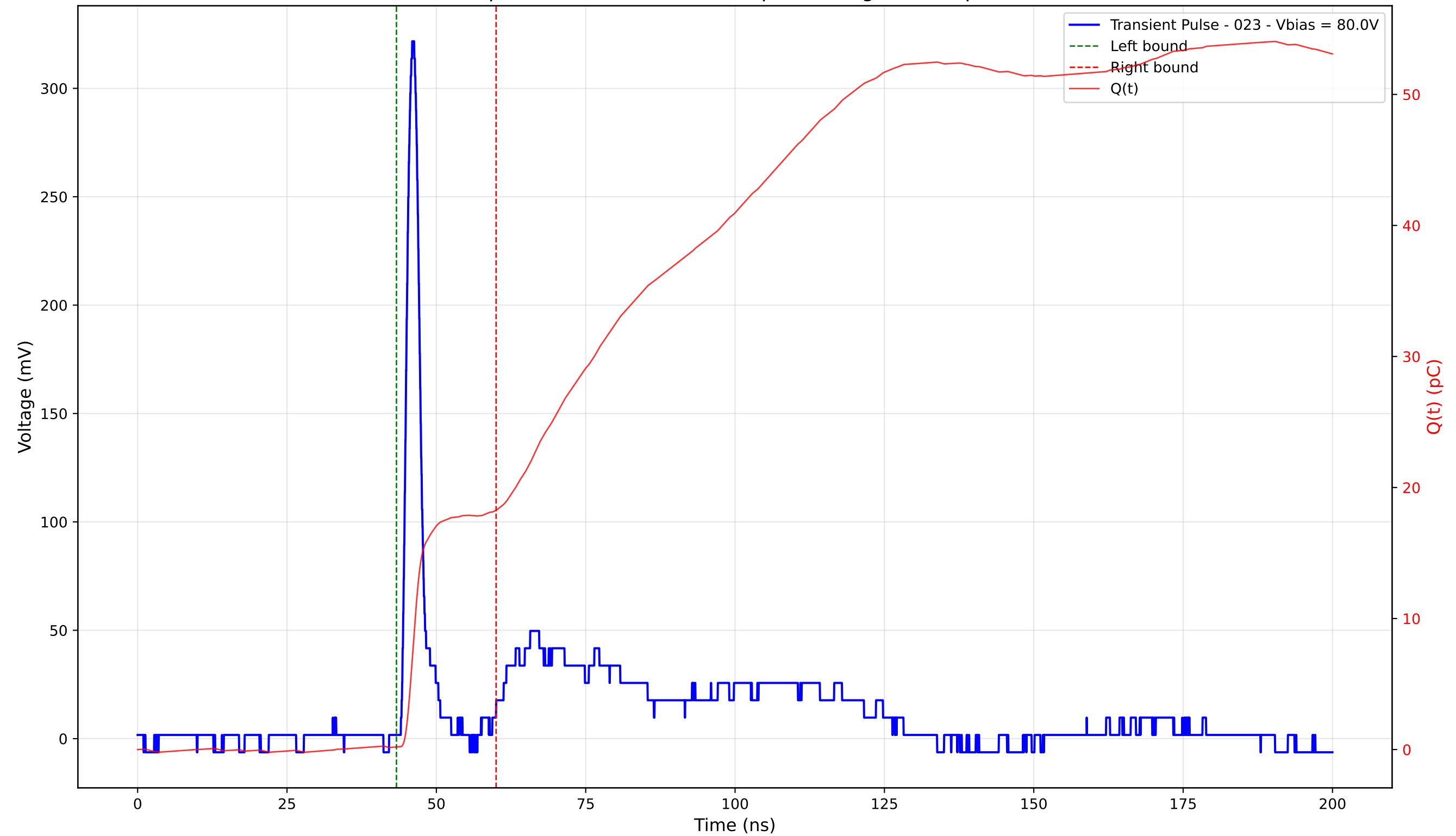
Transient Pulse - Sample: 4003 - Position: 190.0 \mu\text{m} - Charge: 18.06 pC - Rise Time: 1.24 ns
