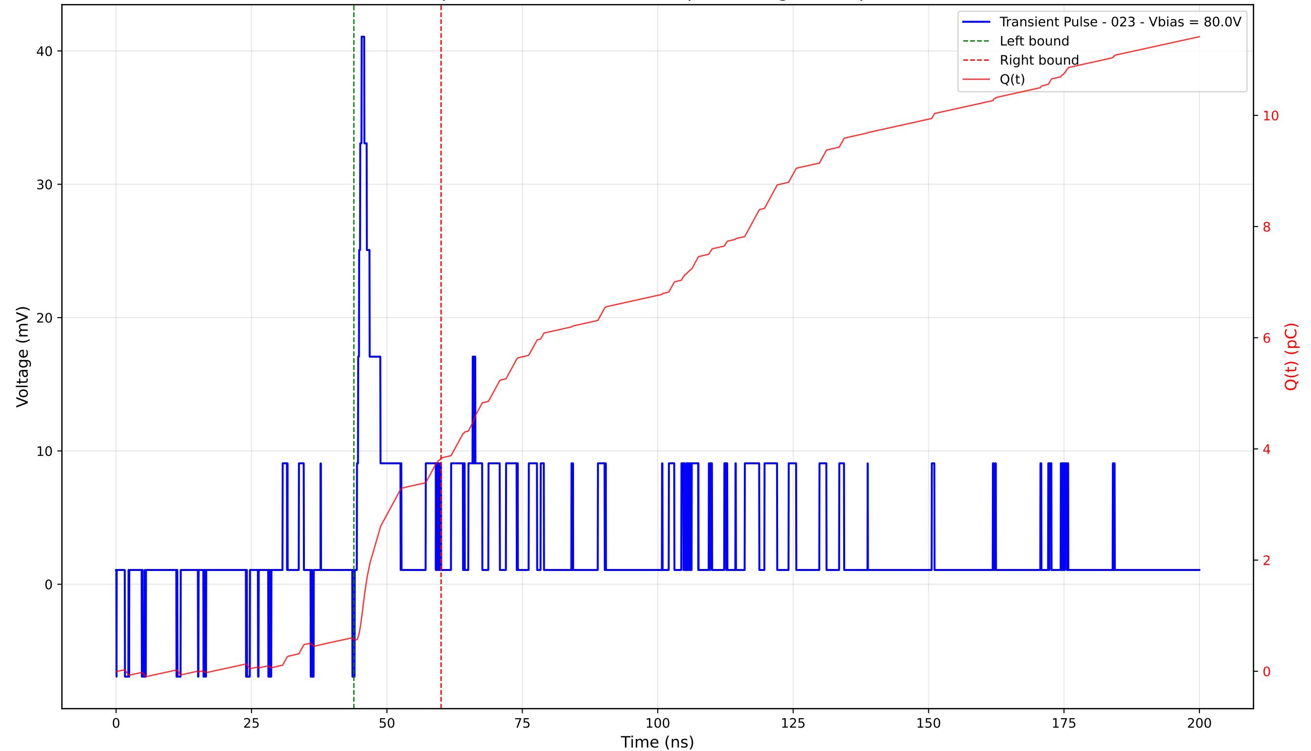
Transient Pulse - Sample: 4003 - Position: 280.0 \mu\text{m} - Charge: 3.26 pC - Rise Time: 0.87 ns
