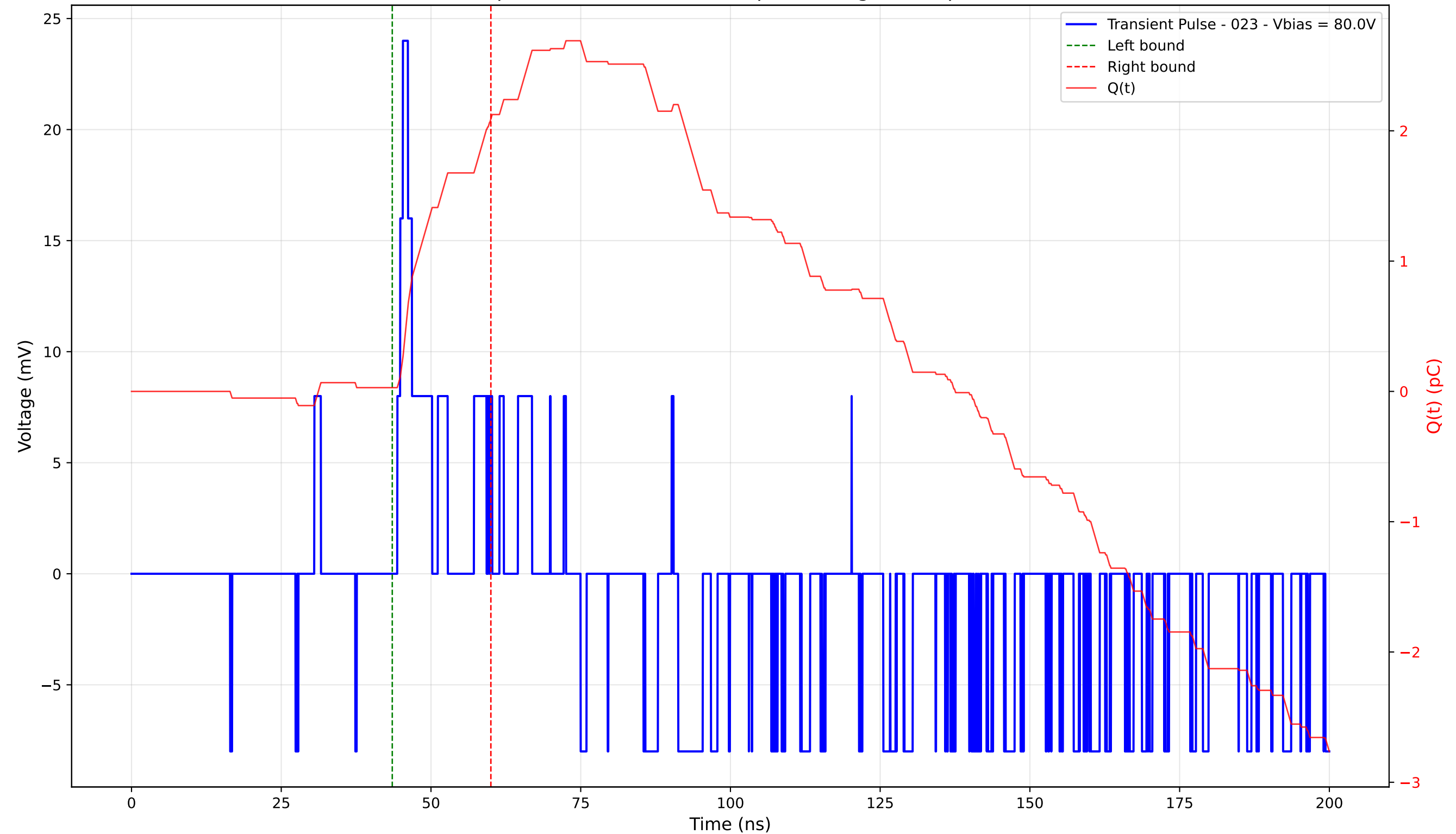
Transient Pulse - Sample: 4003 - Position: 35.0 \mu\text{m} - Charge: 2.06 pC - Rise Time: 0.93 ns
