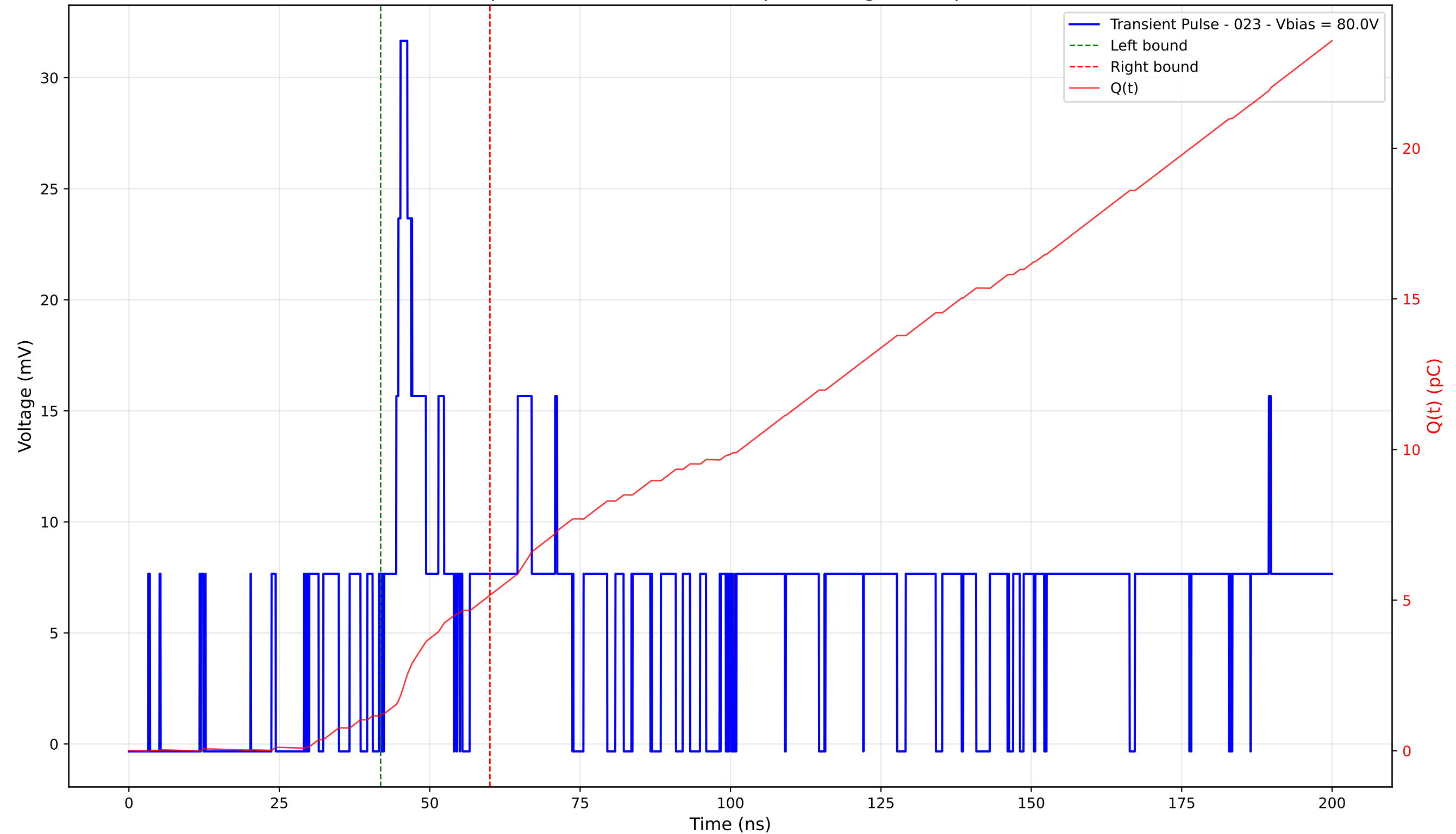
Transient Pulse - Sample: 4003 - Position: 310.0 \mu\text{m} - Charge: 3.96 pC - Rise Time: 2.75 ns
