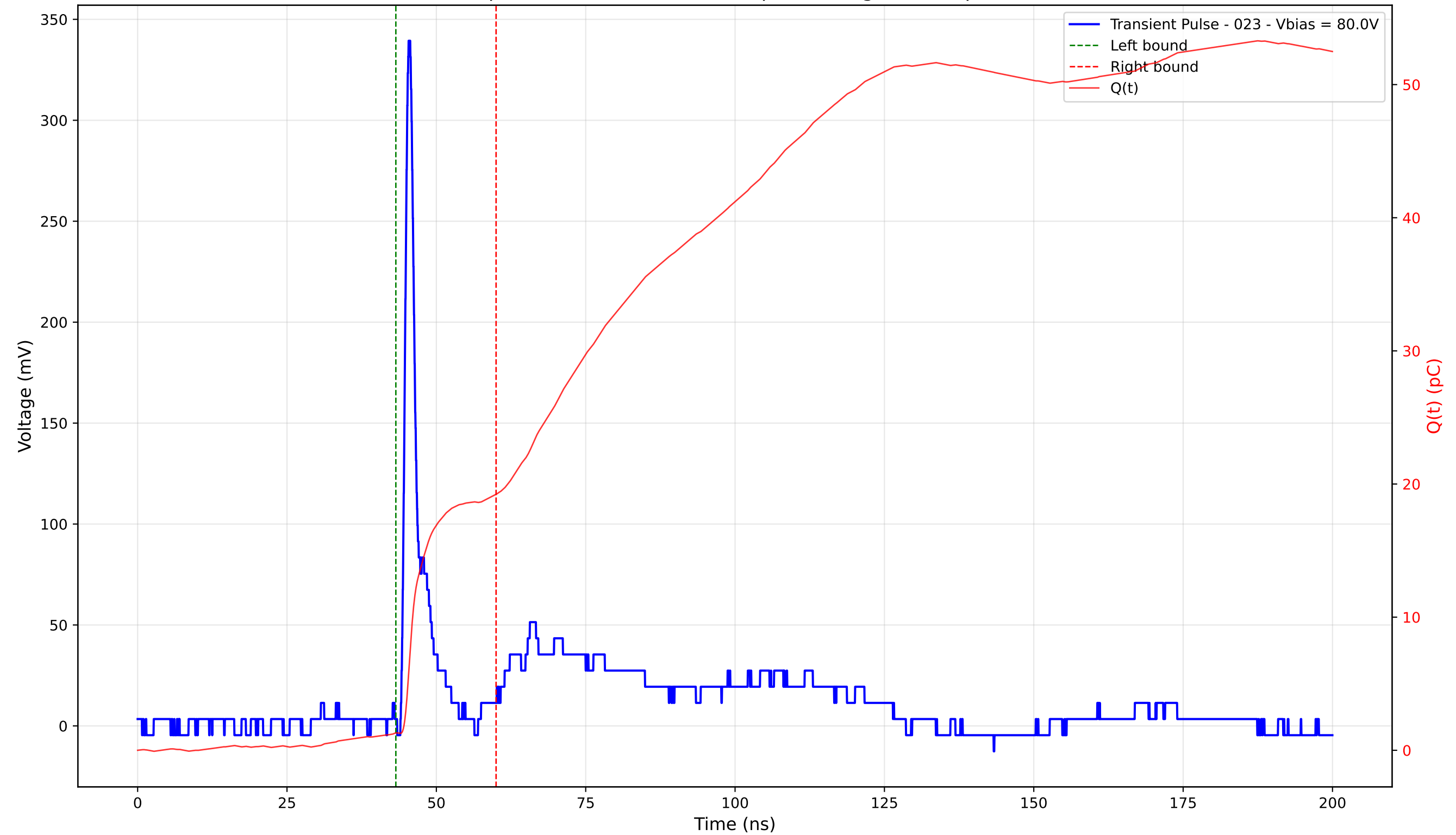
Transient Pulse - Sample: 4003 - Position: 120.0 \mu\text{m} - Charge: 17.92 pC - Rise Time: 0.90 ns
