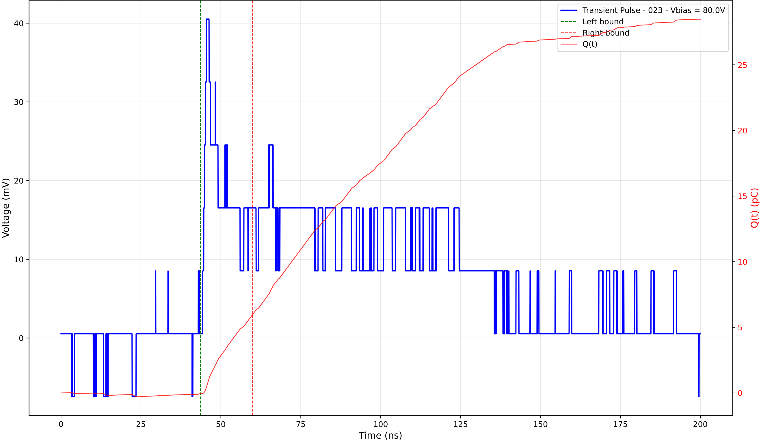
Transient Pulse - Sample: 4003 - Position: 250.0 \mu\text{m} - Charge: 6.05 pC - Rise Time: 1.15 ns
