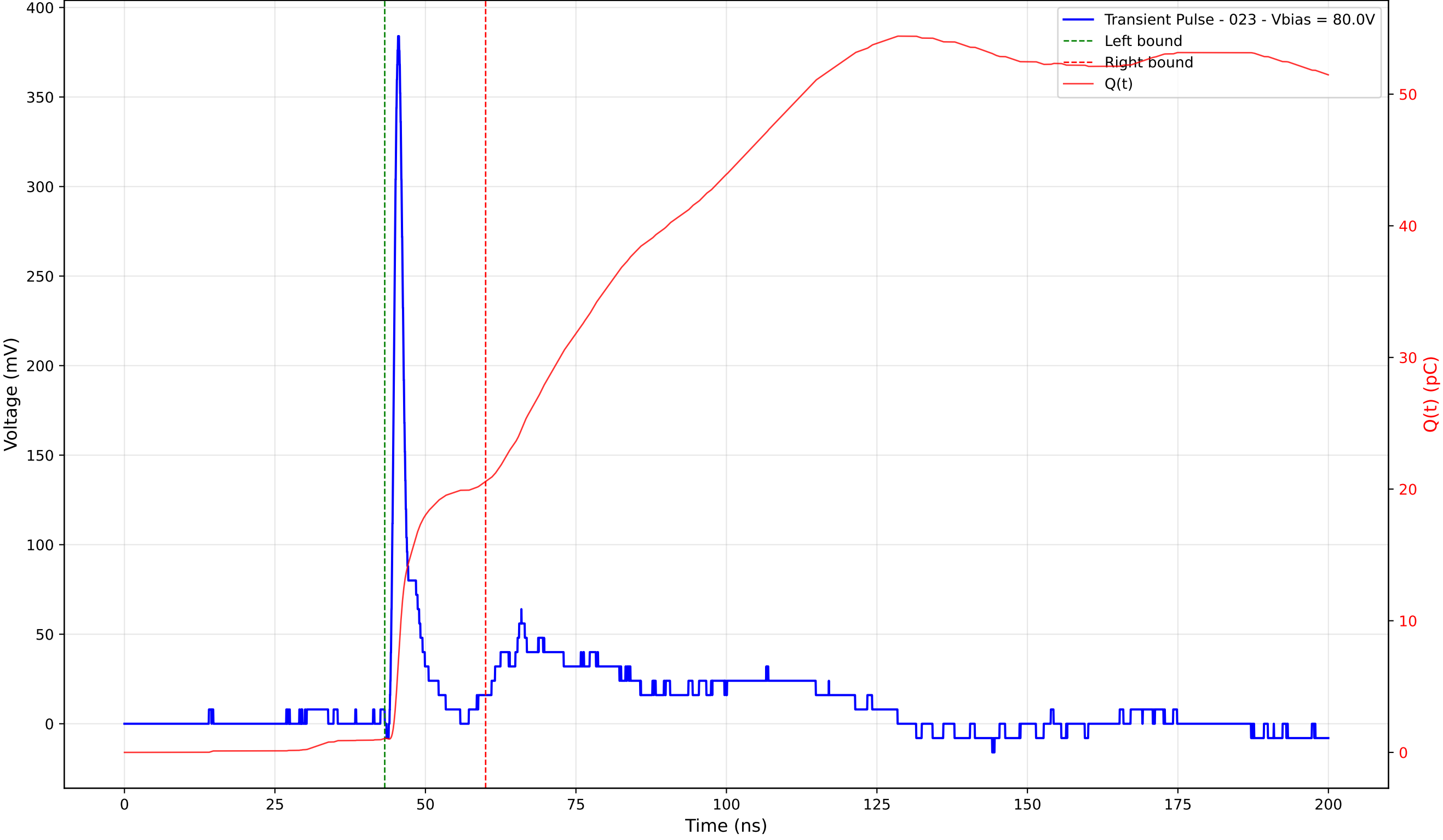
Transient Pulse - Sample: 4003 - Position: 130.0 \mu\text{m} - Charge: 19.50 pC - Rise Time: 0.96 ns
