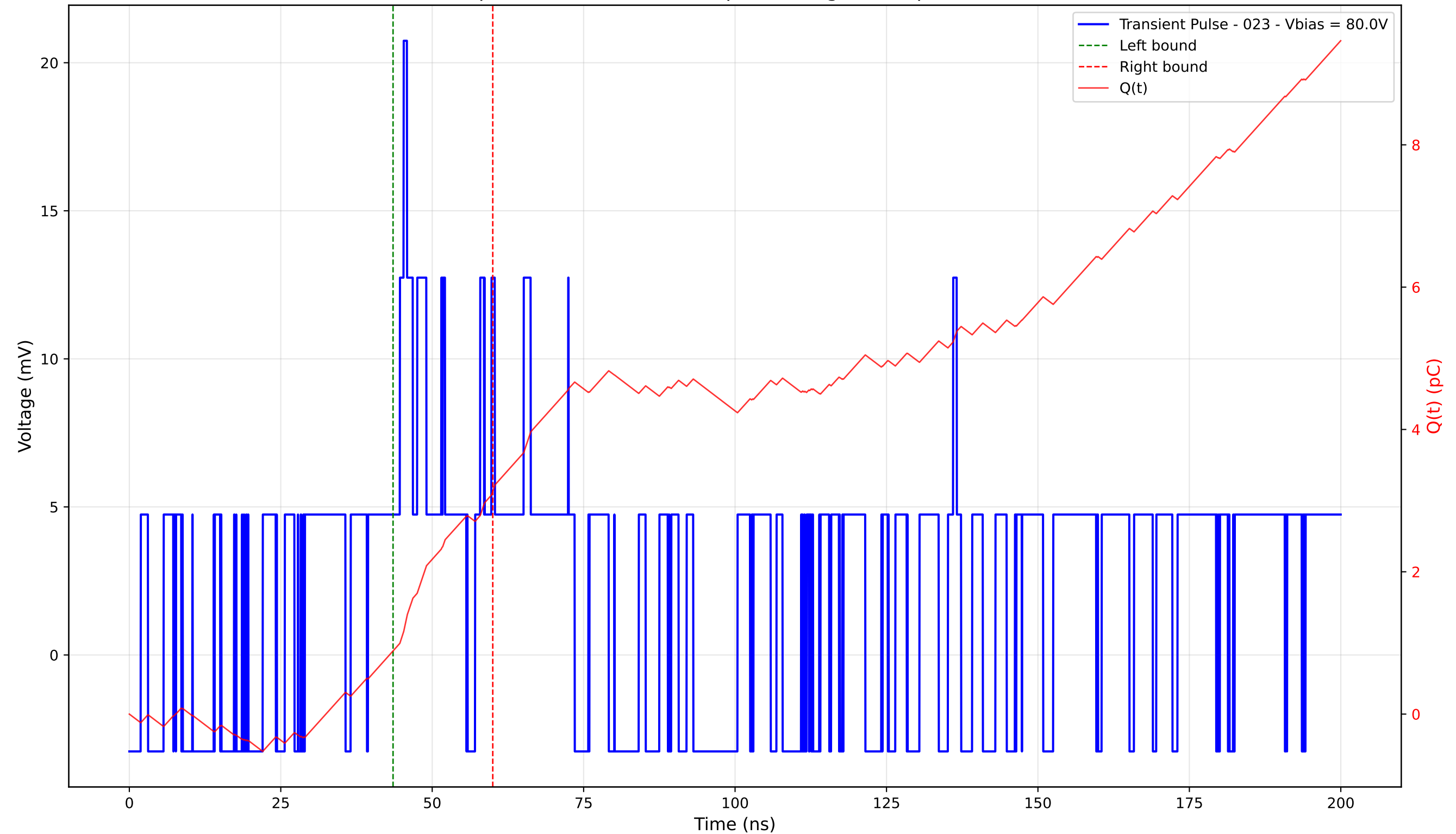
Transient Pulse - Sample: 4003 - Position: 5.0 \mu\text{m} - Charge: 2.25 pC - Rise Time: 0.00 ns (N/A)
