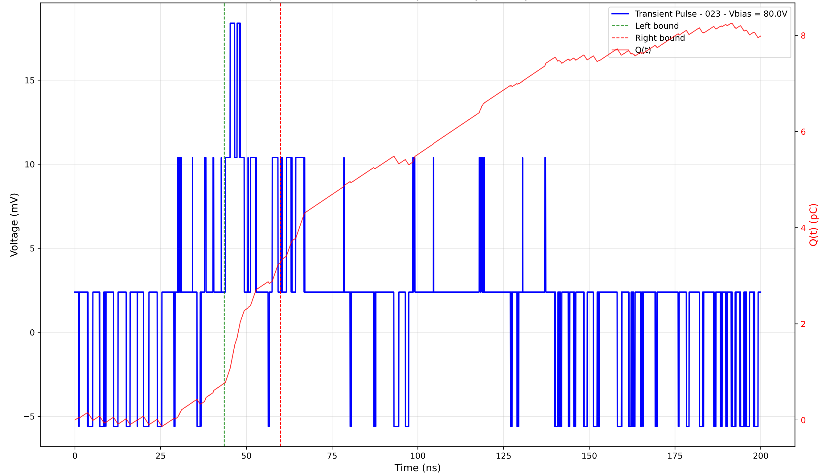
Transient Pulse - Sample: 4003 - Position: 70.0 \mu\text{m} - Charge: 2.51 pC - Rise Time: 0.00 ns (N/A)
