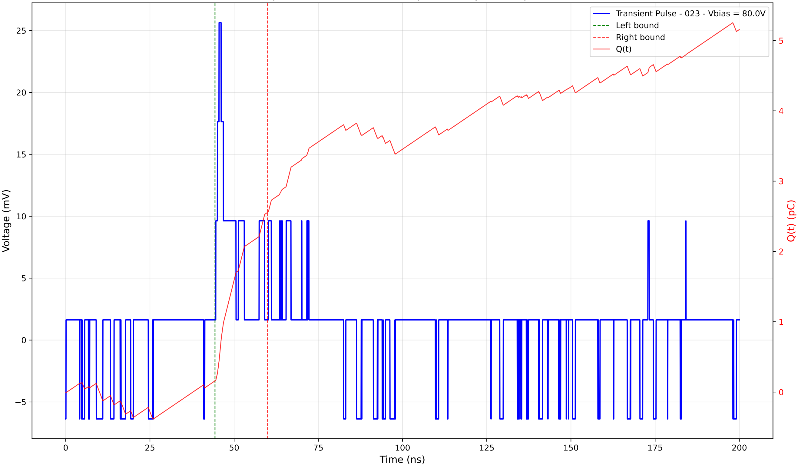
Transient Pulse - Sample: 4003 - Position: 30.0 \mu\text{m} - Charge: 2.40 pC - Rise Time: 0.98 ns
