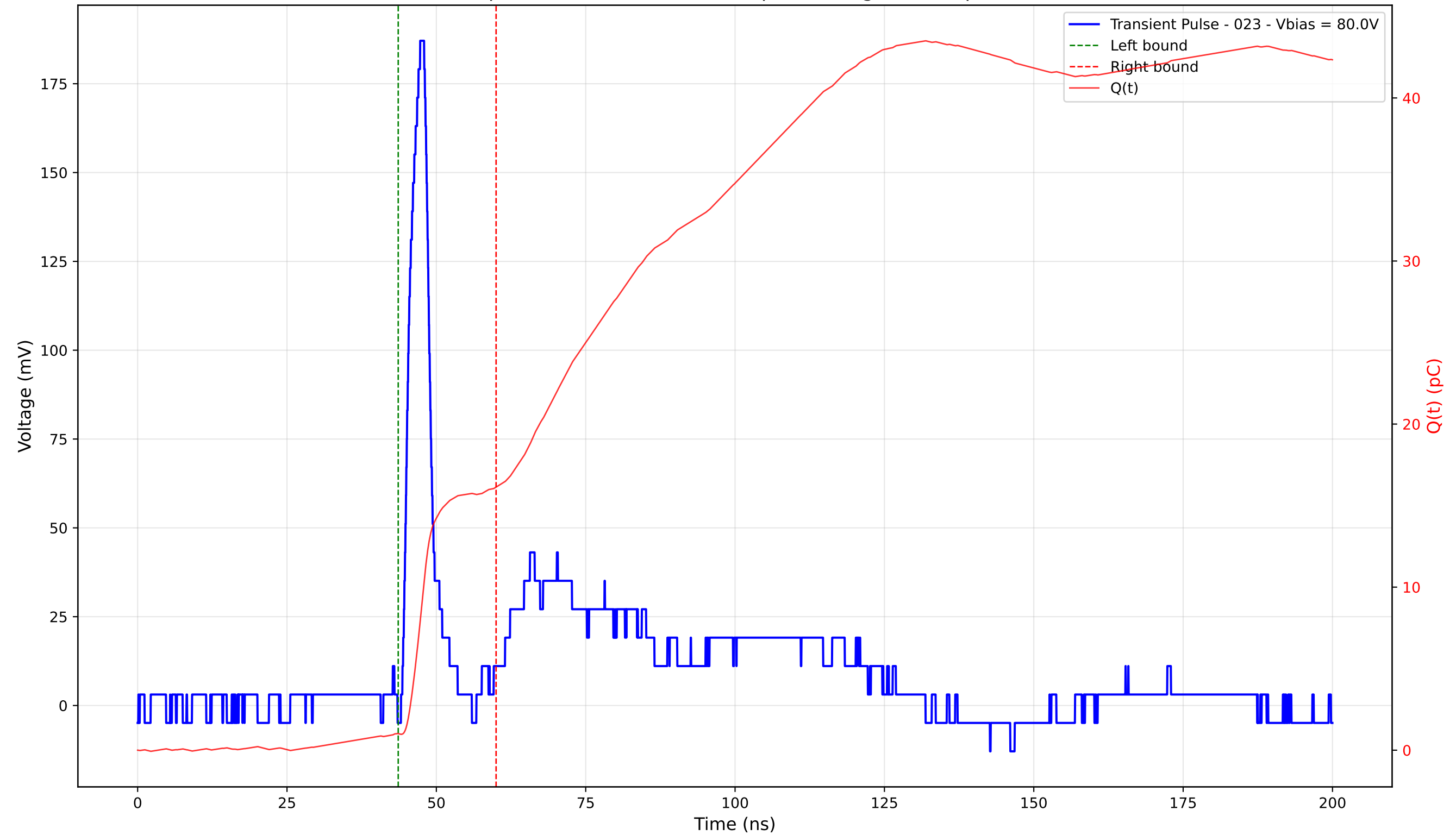
Transient Pulse - Sample: 4003 - Position: 225.0 \mu\text{m} - Charge: 15.12 pC - Rise Time: 2.34 ns
