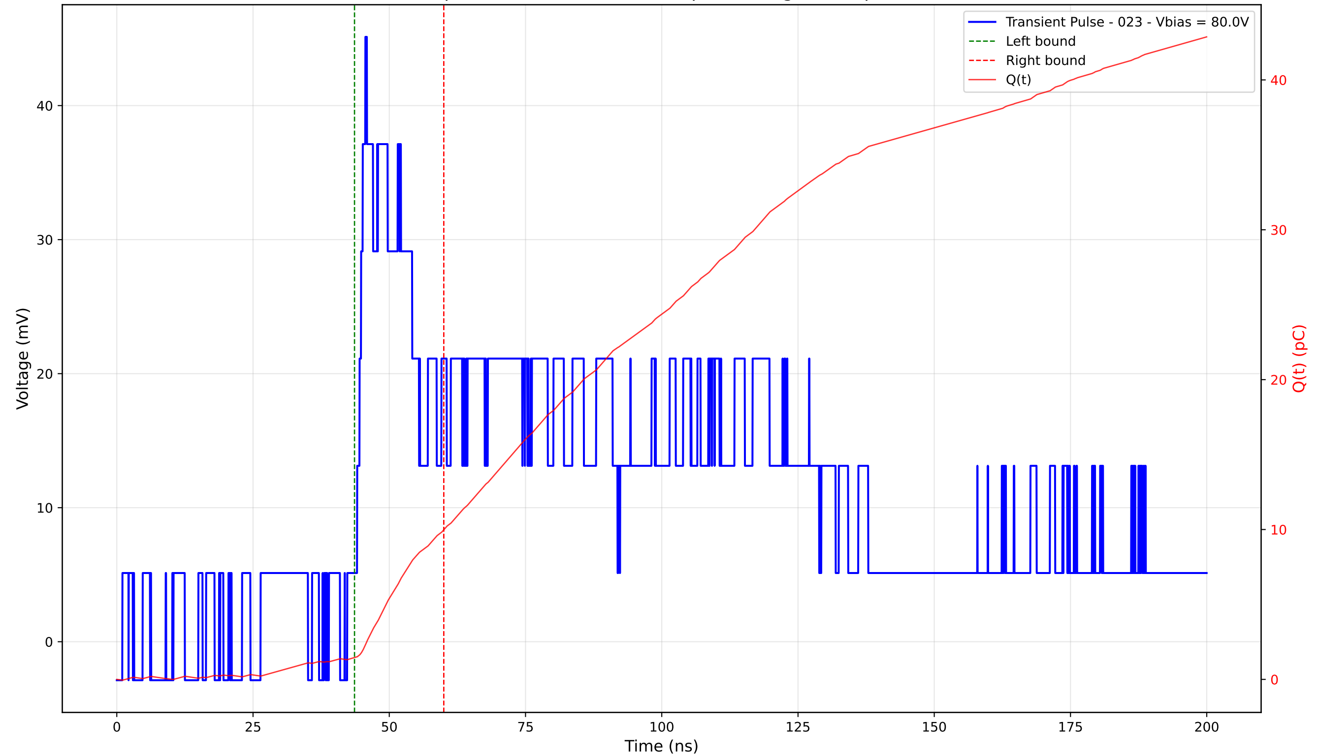
Transient Pulse - Sample: 4003 - Position: 245.0 \mu\text{m} - Charge: 8.53 pC - Rise Time: 3.33 ns
