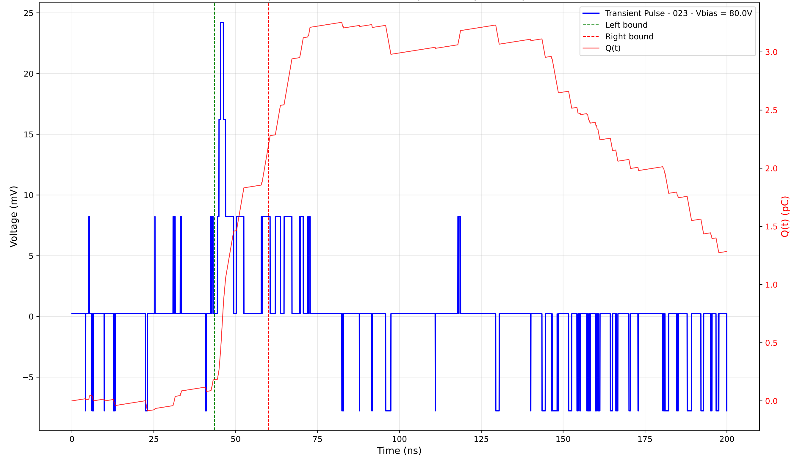
Transient Pulse - Sample: 4003 - Position: 370.0 \mu\text{m} - Charge: 2.01 pC - Rise Time: 0.95 ns
