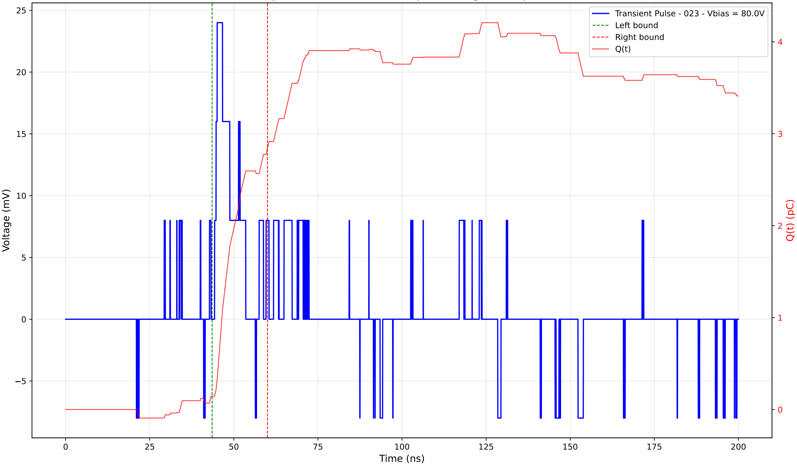
Transient Pulse - Sample: 4003 - Position: 50.0 \mu\text{m} - Charge: 2.70 pC - Rise Time: 0.77 ns
