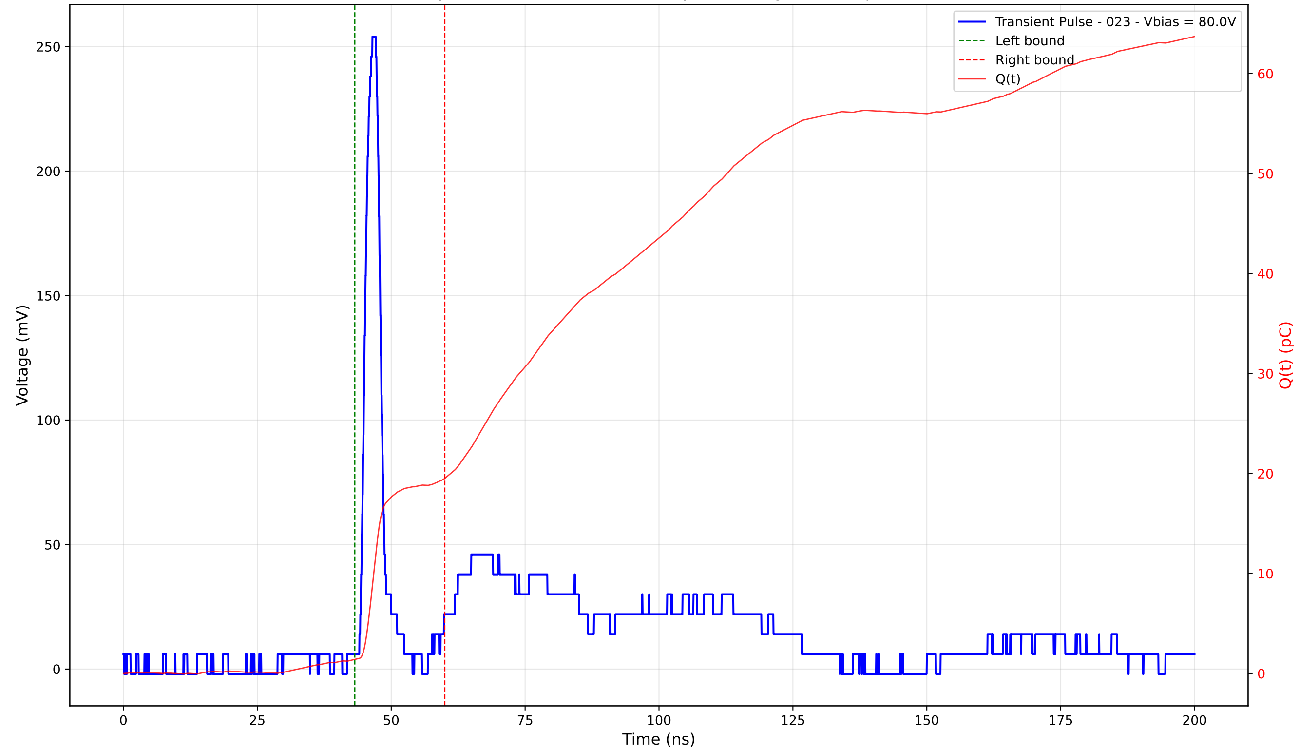
Transient Pulse - Sample: 4003 - Position: 210.0 \mu\text{m} - Charge: 18.11 pC - Rise Time: 1.63 ns
