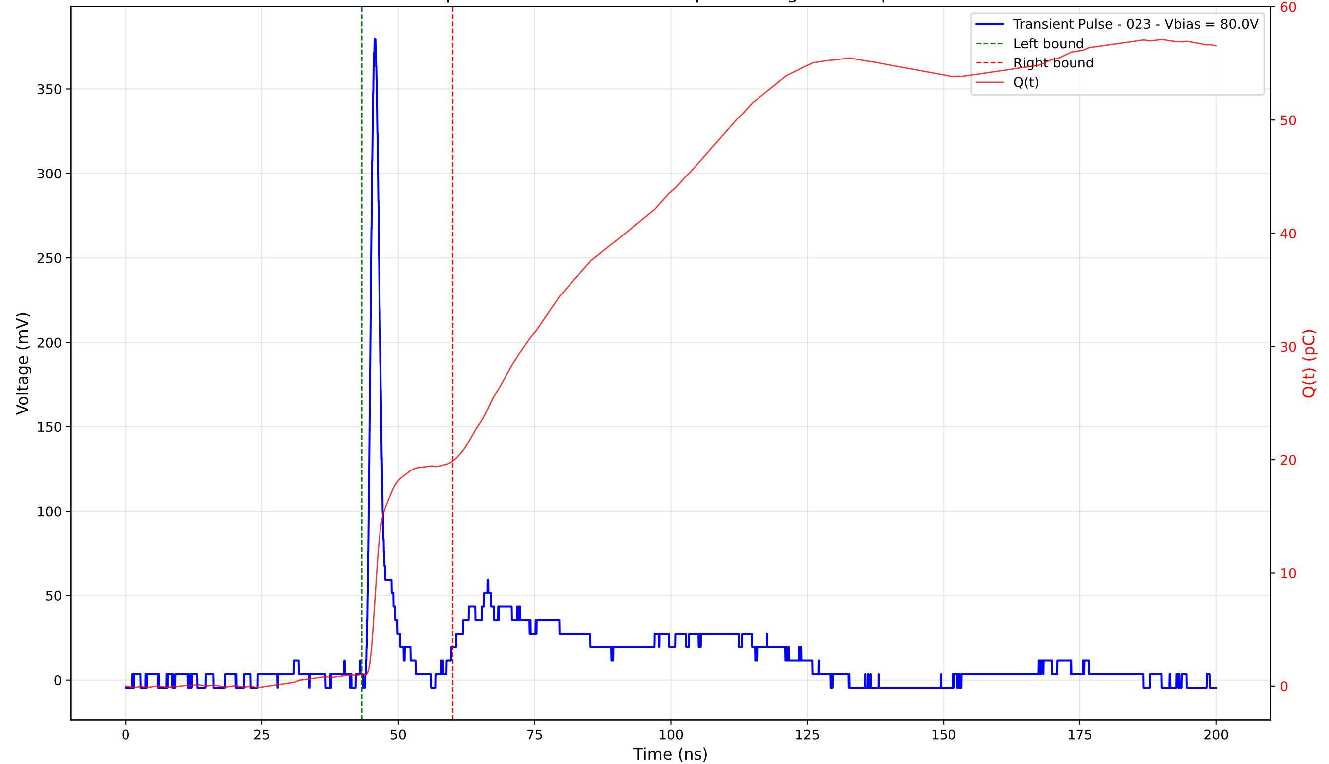
Transient Pulse - Sample: 4003 - Position: 160.0 \mu\text{m} - Charge: 18.85 pC - Rise Time: 1.07 ns
