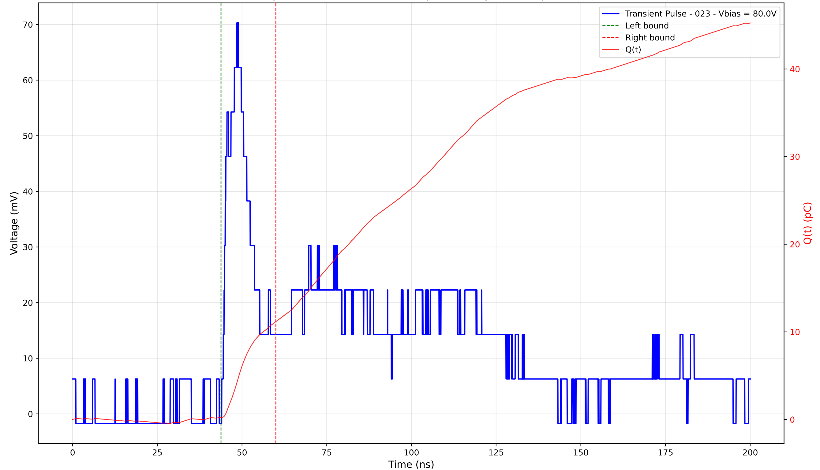
Transient Pulse - Sample: 4003 - Position: 240.0 \mu\text{m} - Charge: 10.94 pC - Rise Time: 4.00 ns
