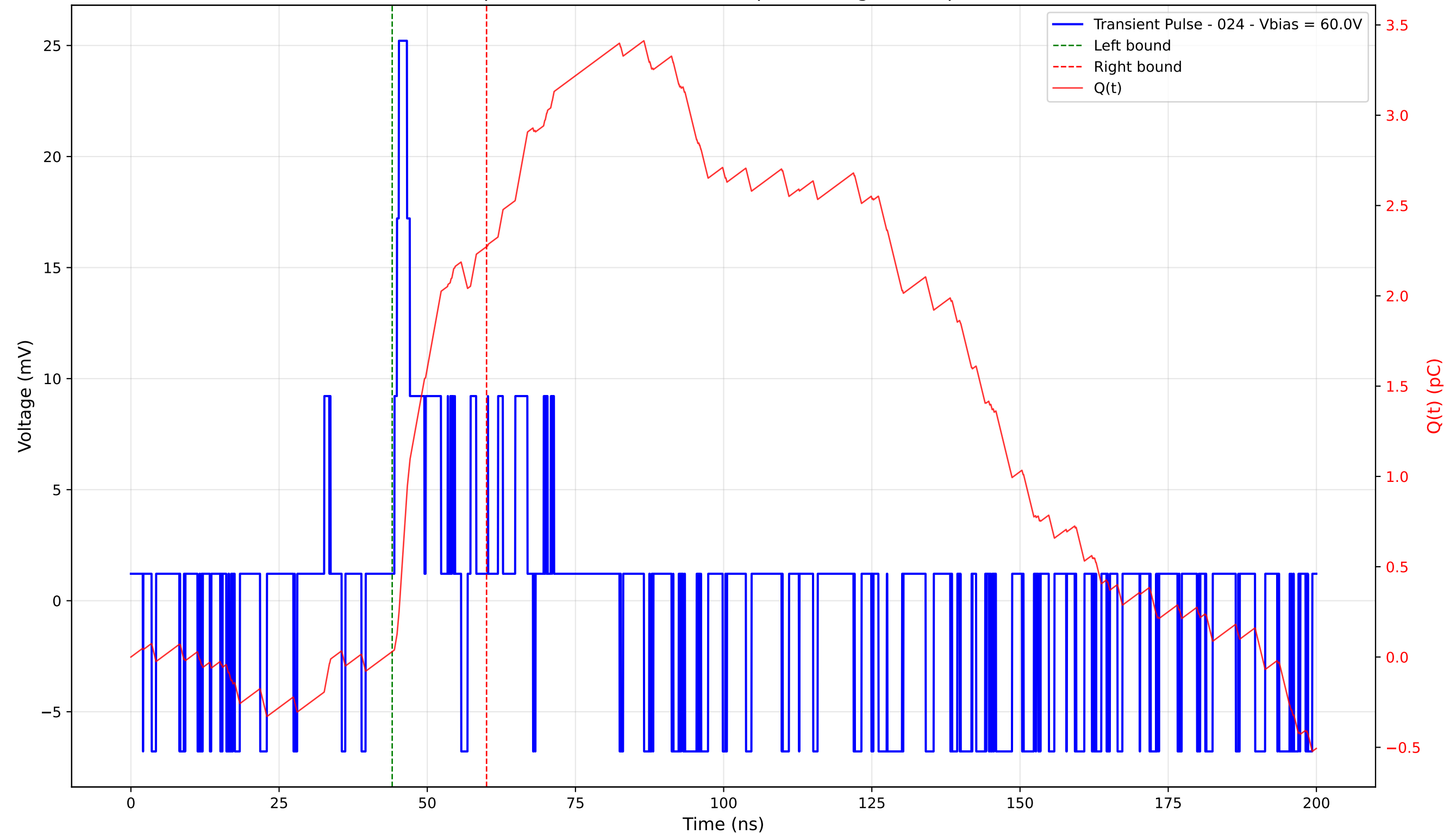
Transient Pulse - Sample: 4003 - Position: 300.0 \mu\text{m} - Charge: 2.24 pC - Rise Time: 0.76 ns
