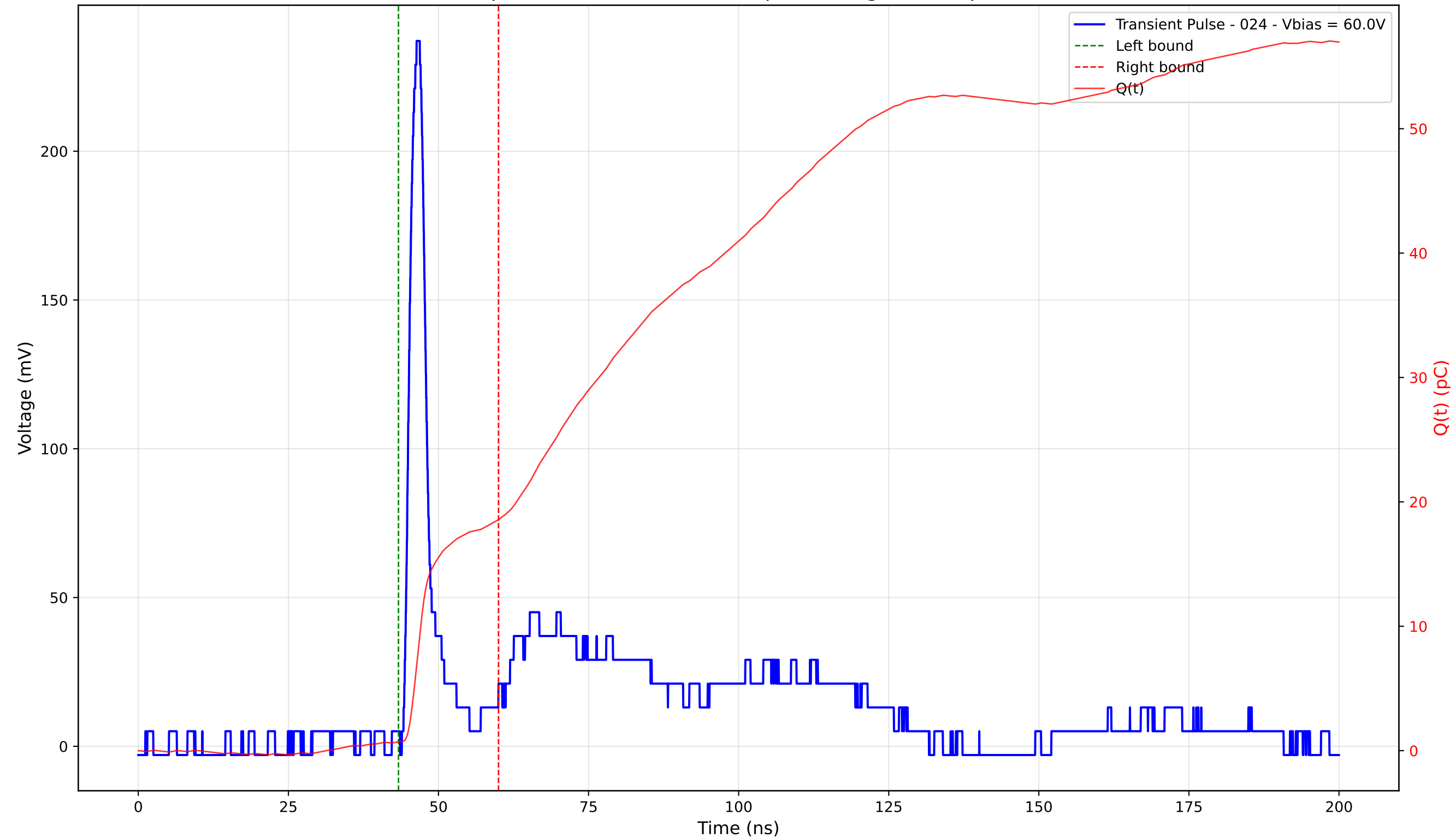
Transient Pulse - Sample: 4003 - Position: 190.0 \mu\text{m} - Charge: 17.83 pC - Rise Time: 1.57 ns
