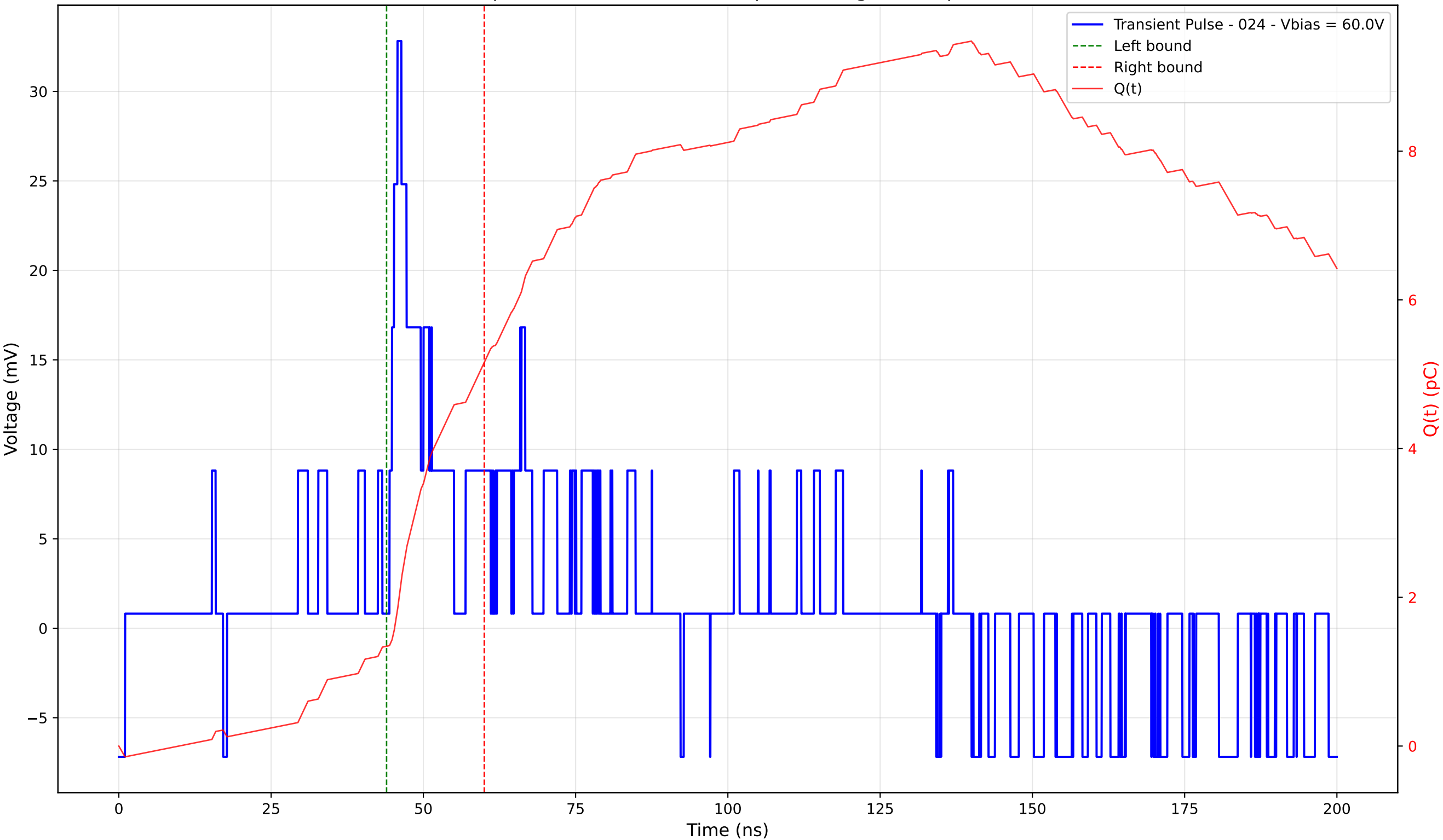
Transient Pulse - Sample: 4003 - Position: 60.0 \mu\text{m} - Charge: 3.82 pC - Rise Time: 1.31 ns
