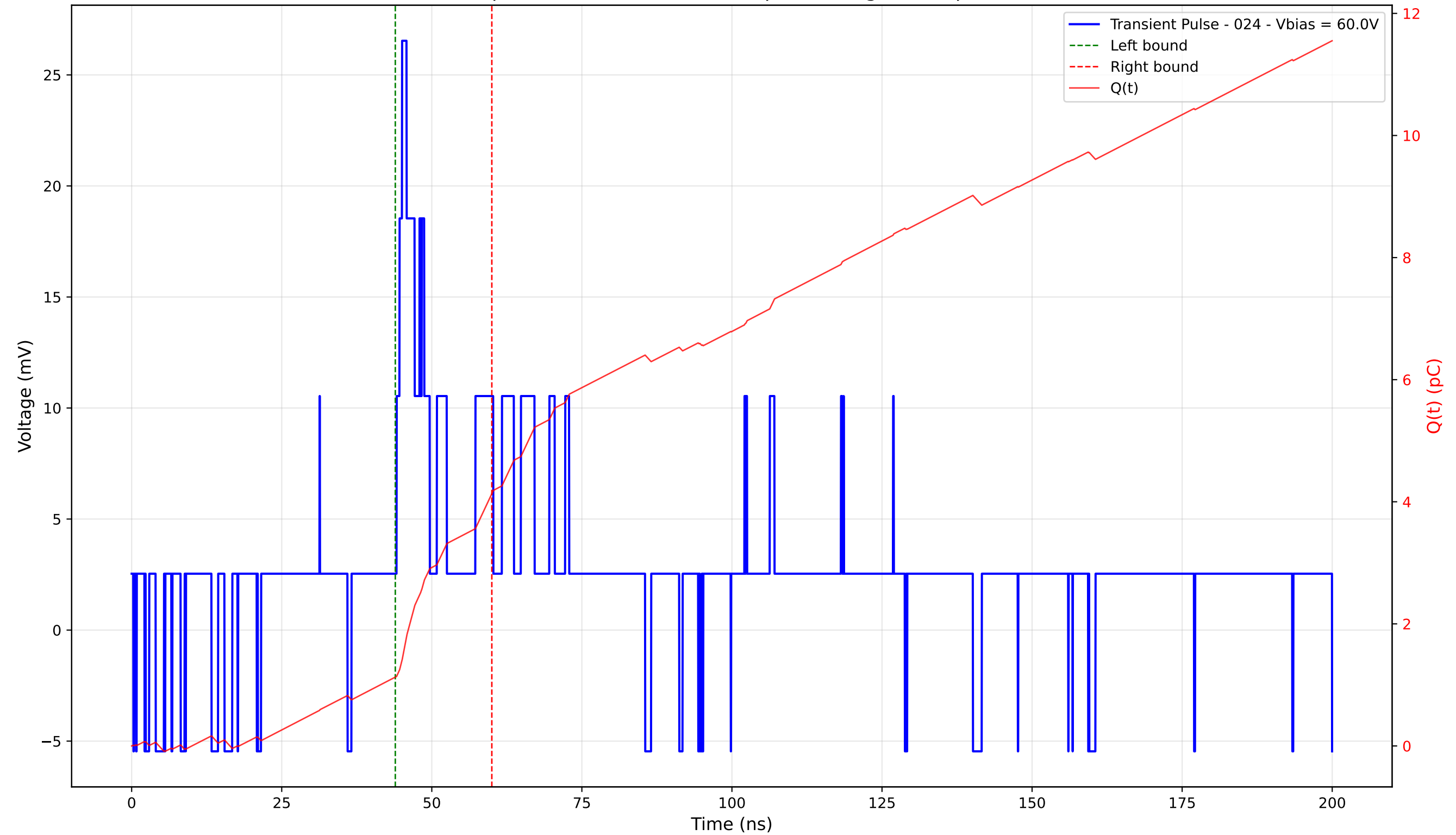
Transient Pulse - Sample: 4003 - Position: 315.0 \mu\text{m} - Charge: 3.01 pC - Rise Time: 0.92 ns
