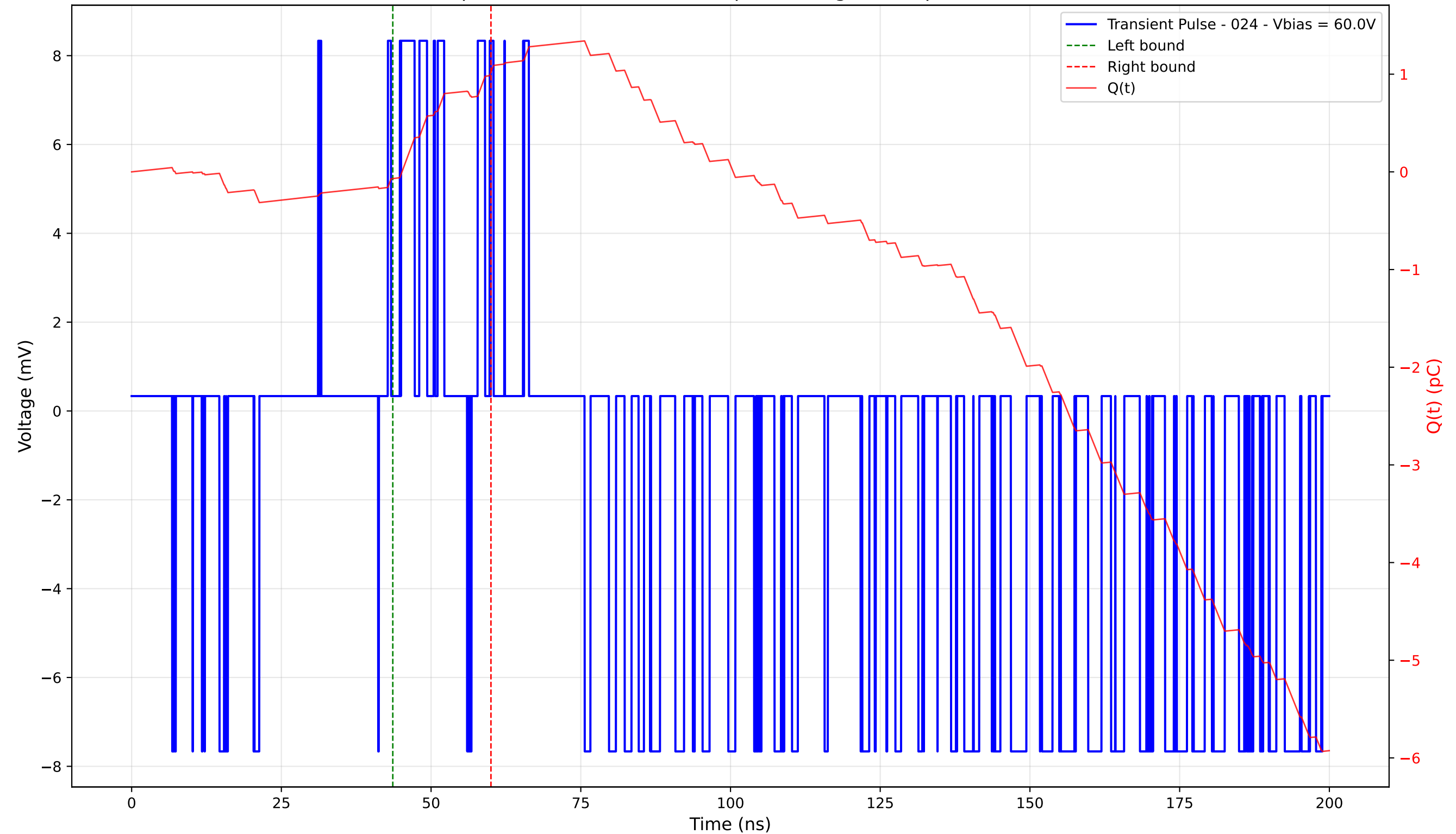
Transient Pulse - Sample: 4003 - Position: 425.0 \mu\text{m} - Charge: 1.09 pC - Rise Time: 0.00 ns (N/A)
