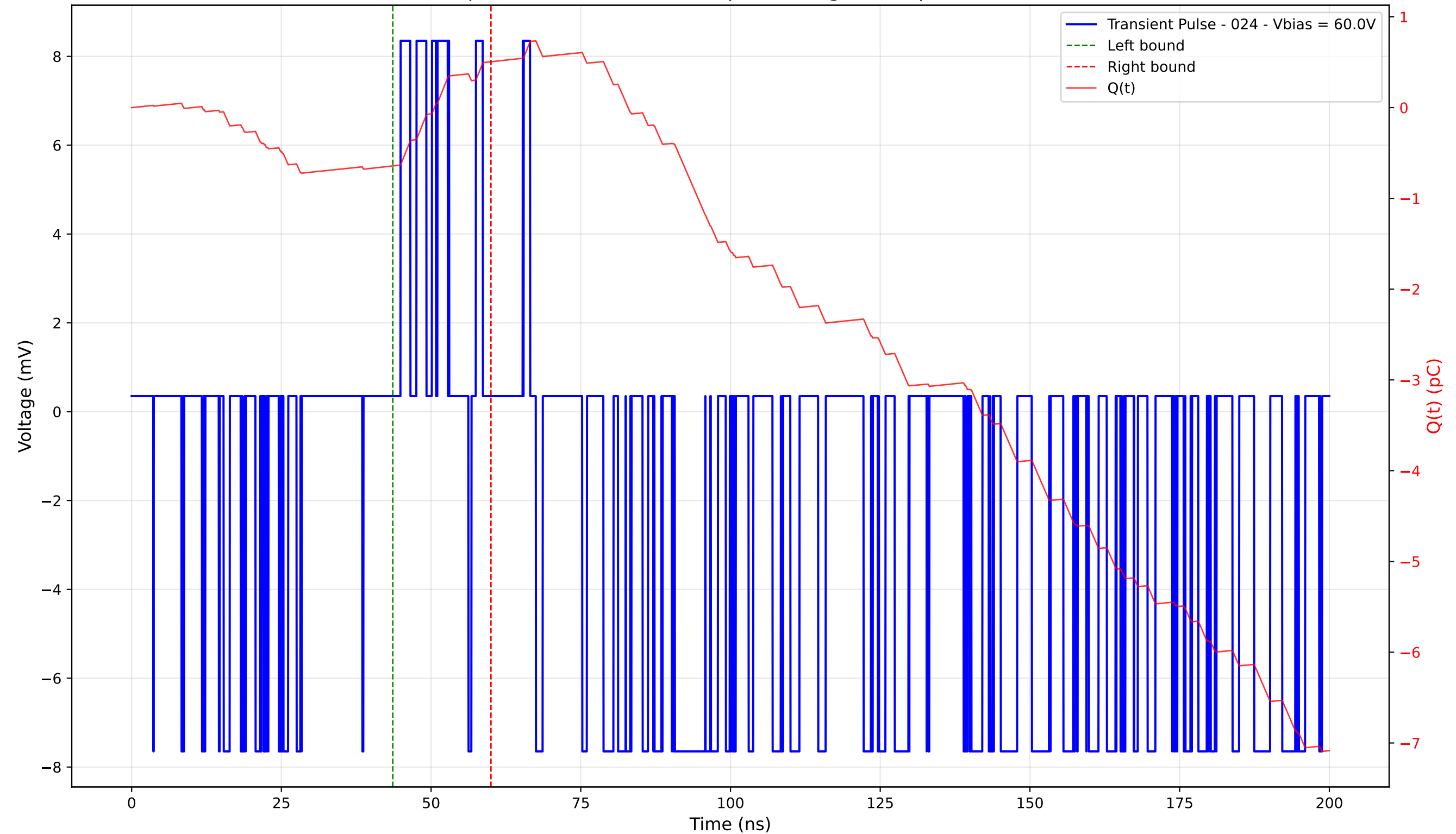
Transient Pulse - Sample: 4003 - Position: 10.0 \mu\text{m} - Charge: 1.15 pC - Rise Time: 0.00 ns (N/A)
