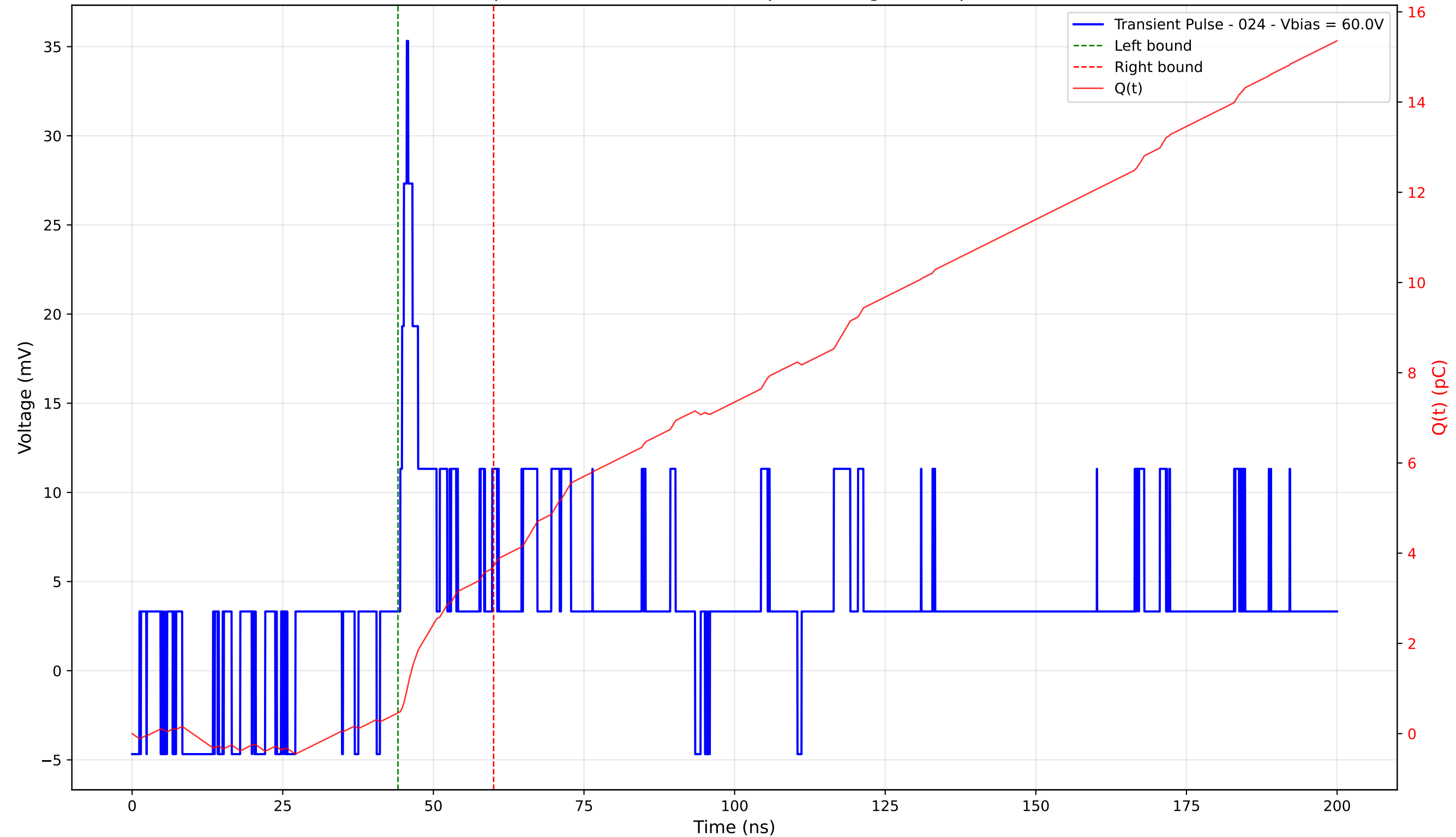
Transient Pulse - Sample: 4003 - Position: 275.0 \mu\text{m} - Charge: 3.25 pC - Rise Time: 1.10 ns
