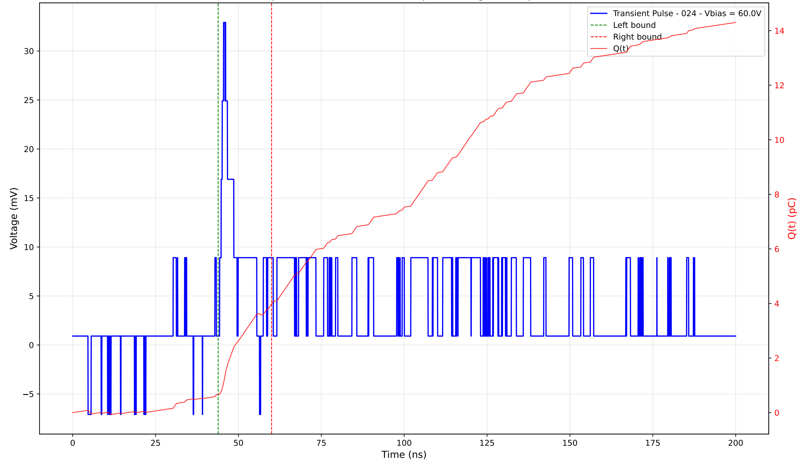
Transient Pulse - Sample: 4003 - Position: 250.0 \mu\text{m} - Charge: 3.32 pC - Rise Time: 1.19 ns
