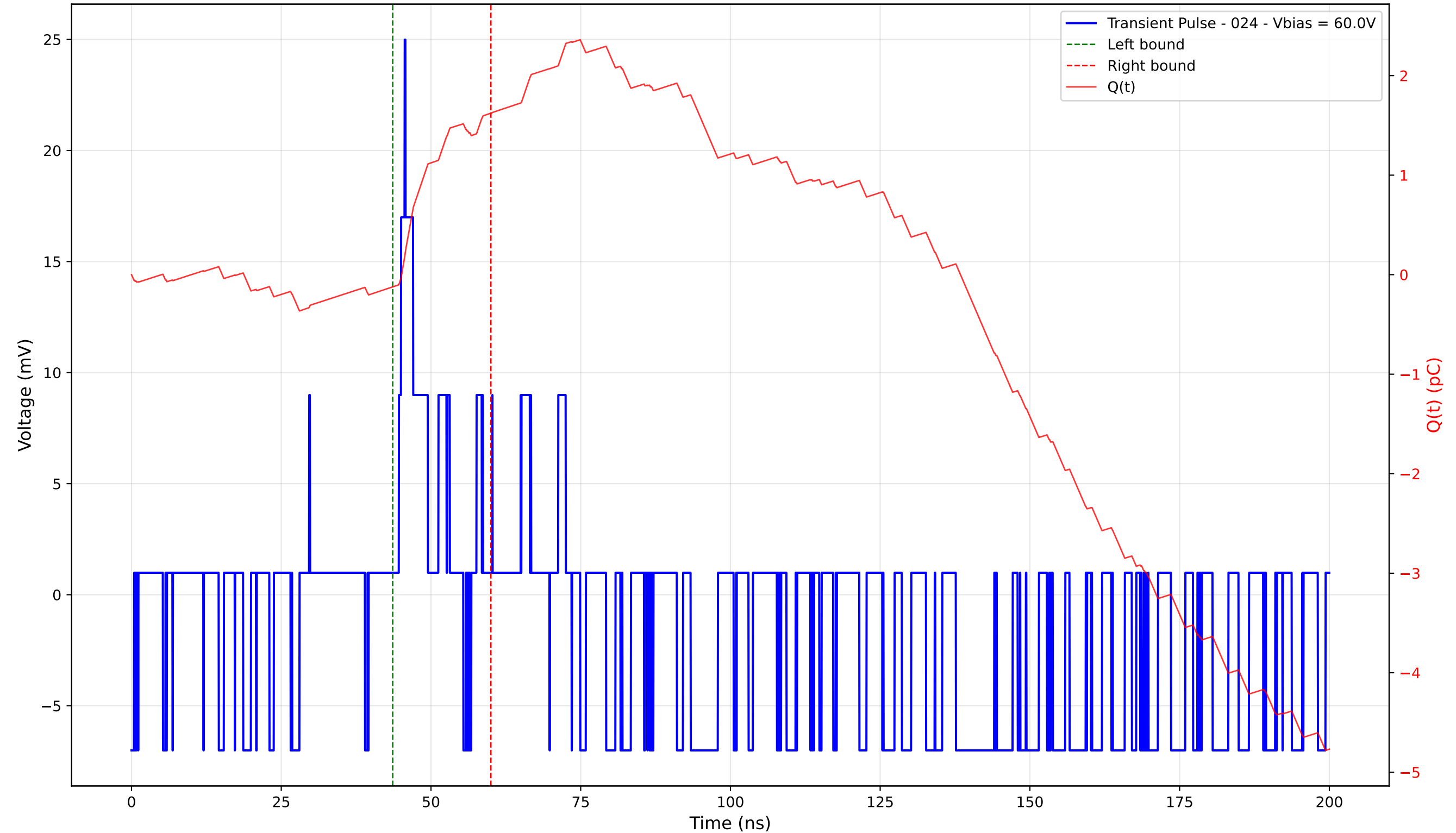
Transient Pulse - Sample: 4003 - Position: 410.0 \mu\text{m} - Charge: 1.75 pC - Rise Time: 0.98 ns
