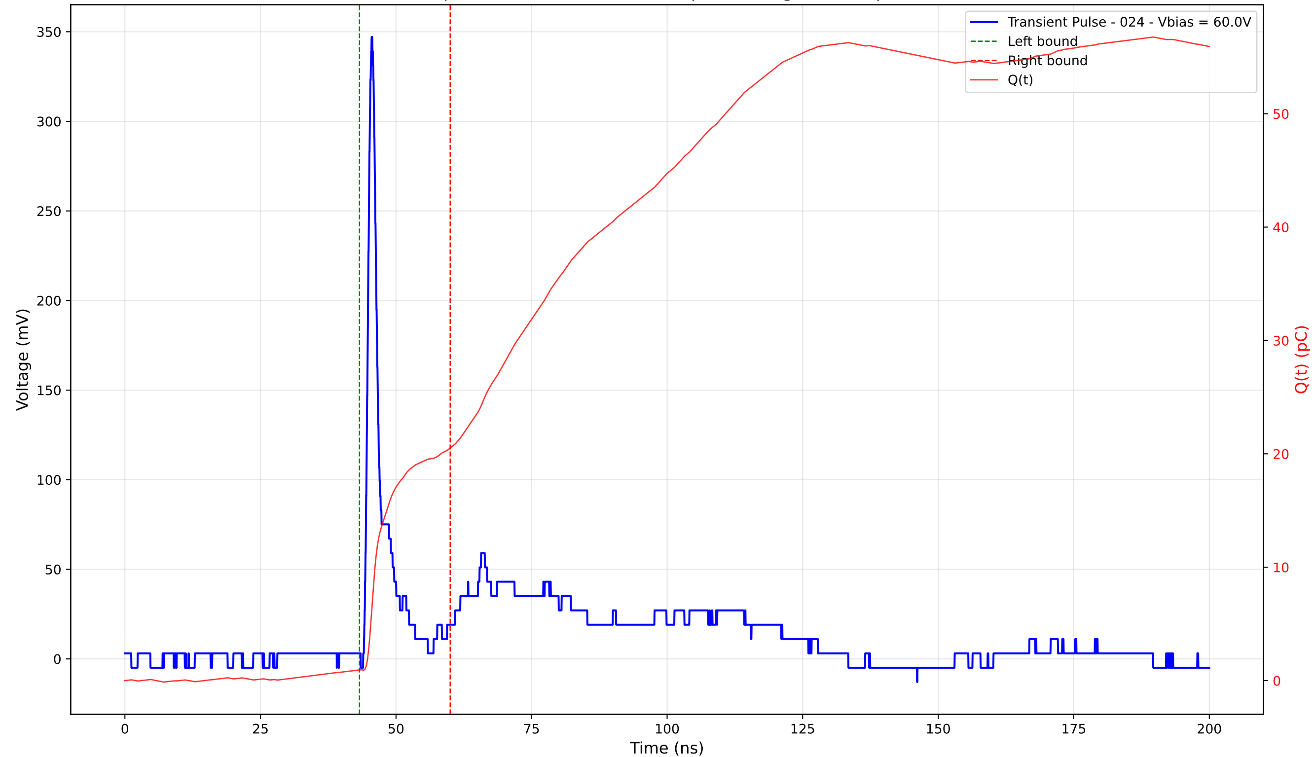
Transient Pulse - Sample: 4003 - Position: 130.0 \mu\text{m} - Charge: 19.56 pC - Rise Time: 0.98 ns
