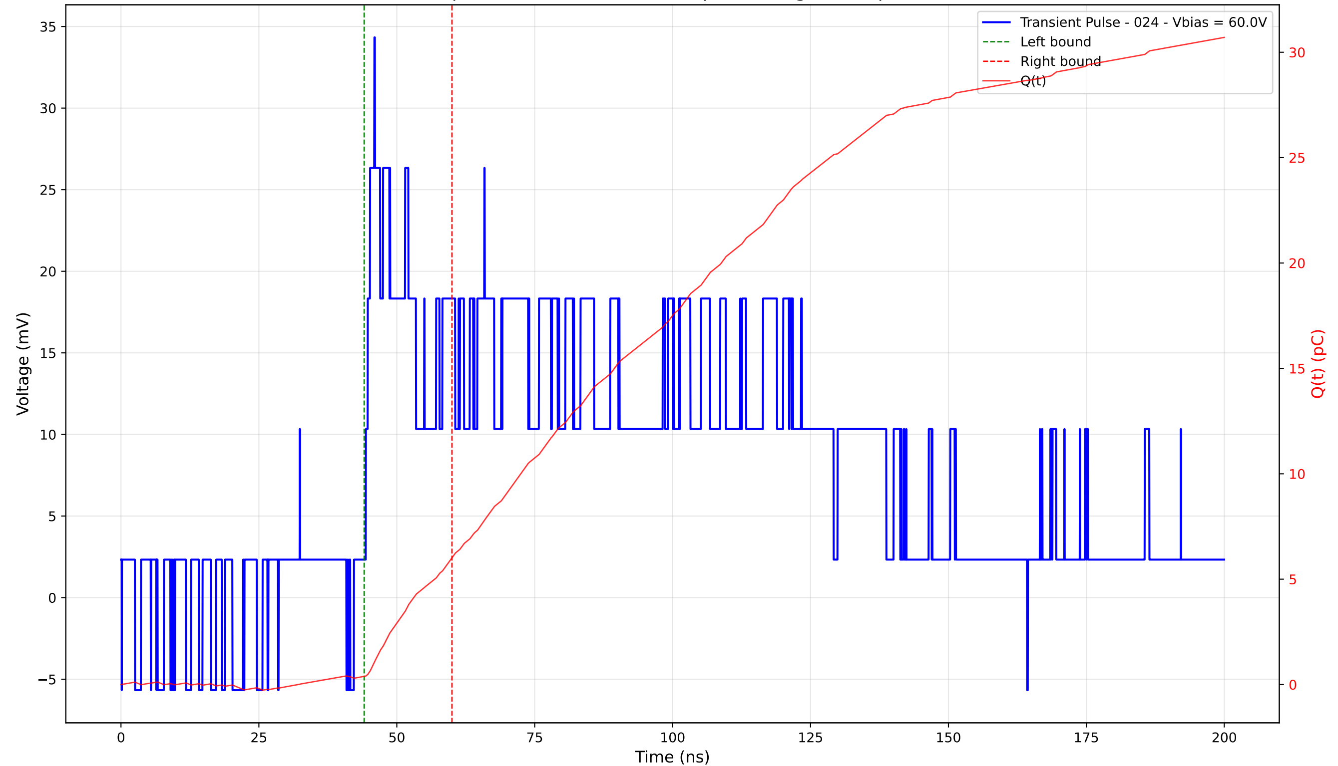
Transient Pulse - Sample: 4003 - Position: 230.0 \mu\text{m} - Charge: 5.64 pC - Rise Time: 1.56 ns
