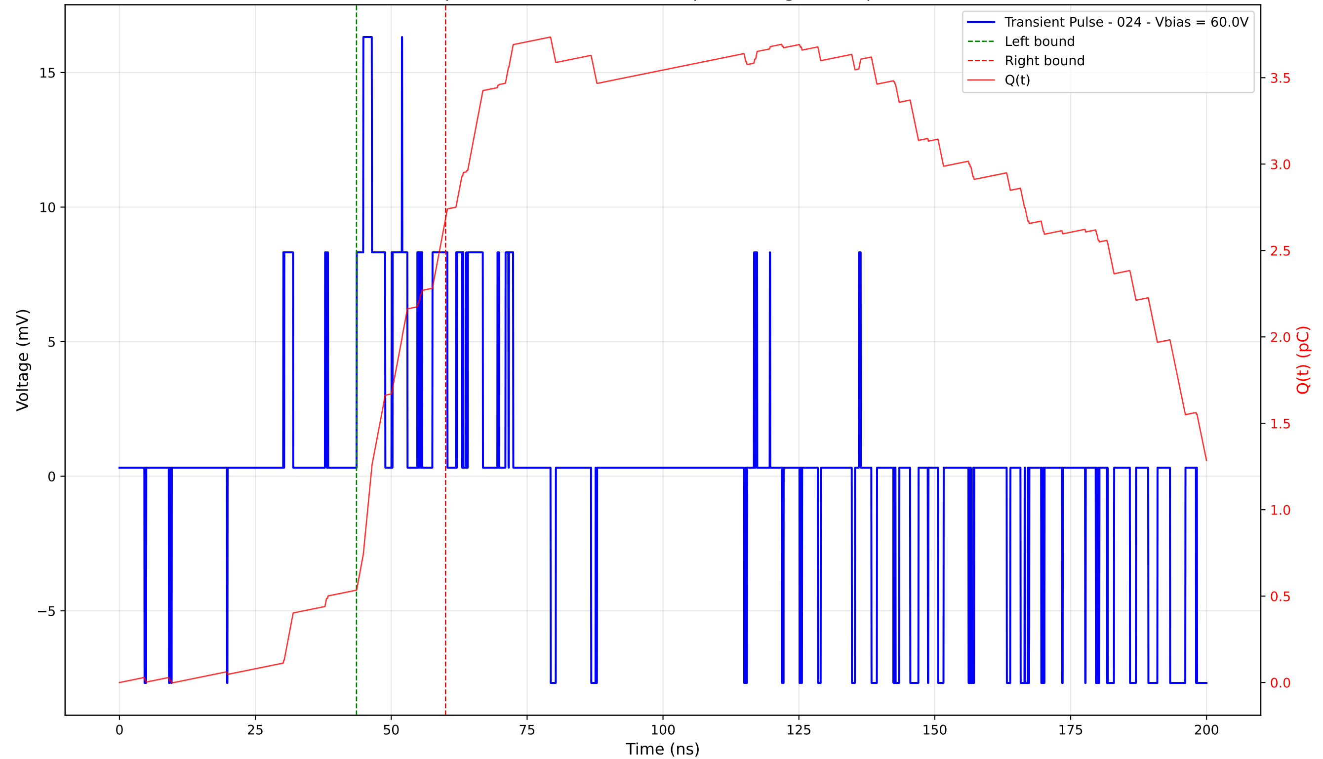
Transient Pulse - Sample: 4003 - Position: 360.0 \mu\text{m} - Charge: 2.15 pC - Rise Time: 1.24 ns
