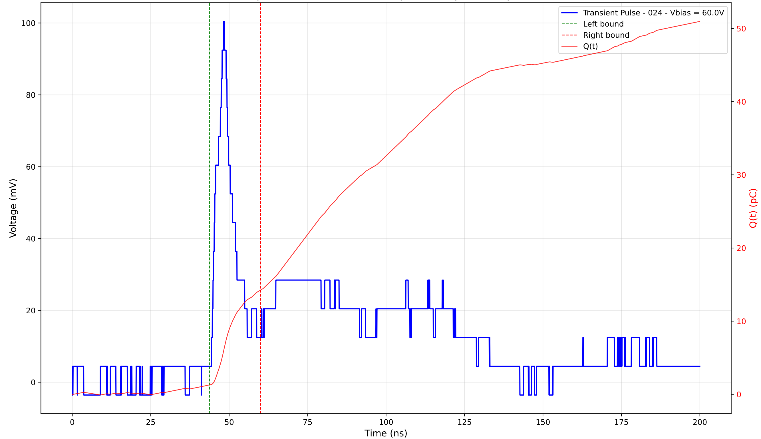
Transient Pulse - Sample: 4003 - Position: 215.0 \mu\text{m} - Charge: 12.96 pC - Rise Time: 3.41 ns
