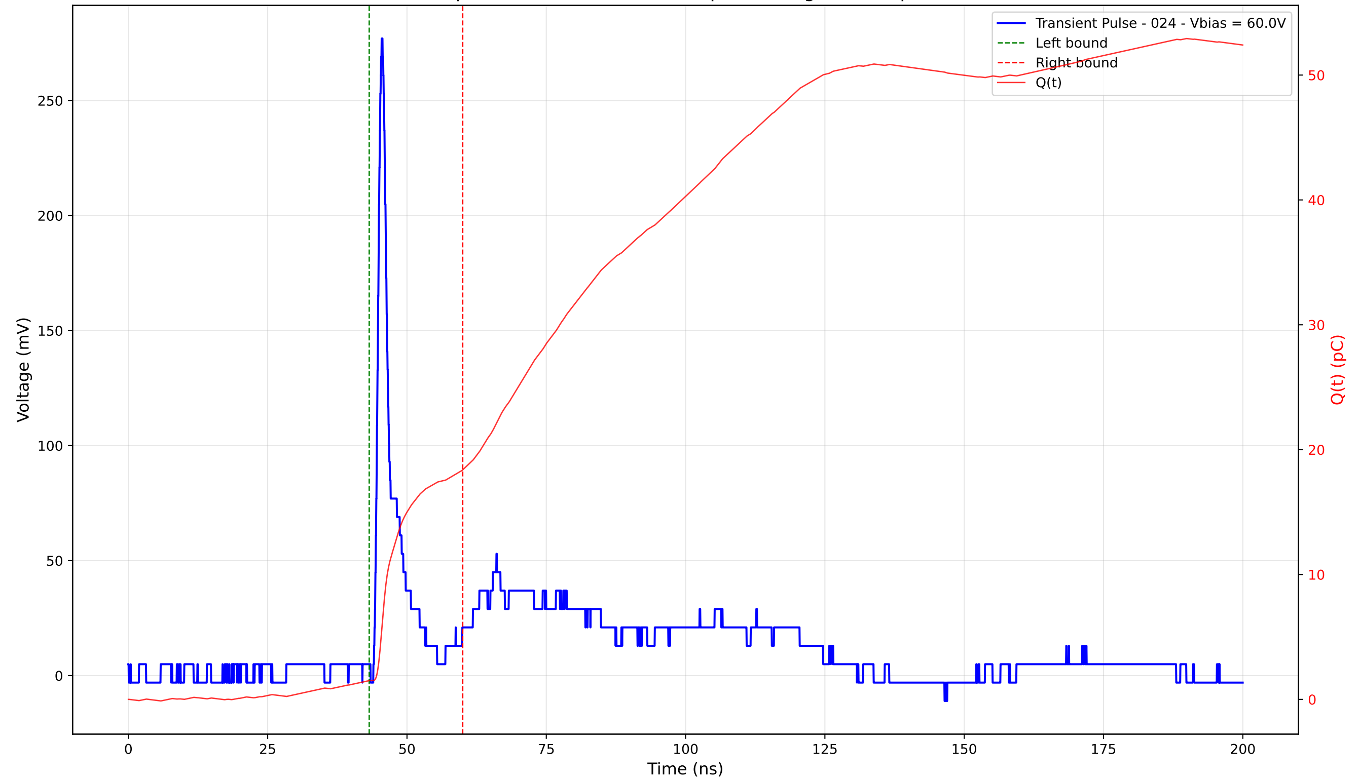
Transient Pulse - Sample: 4003 - Position: 115.0 \mu\text{m} - Charge: 16.87 pC - Rise Time: 0.98 ns
