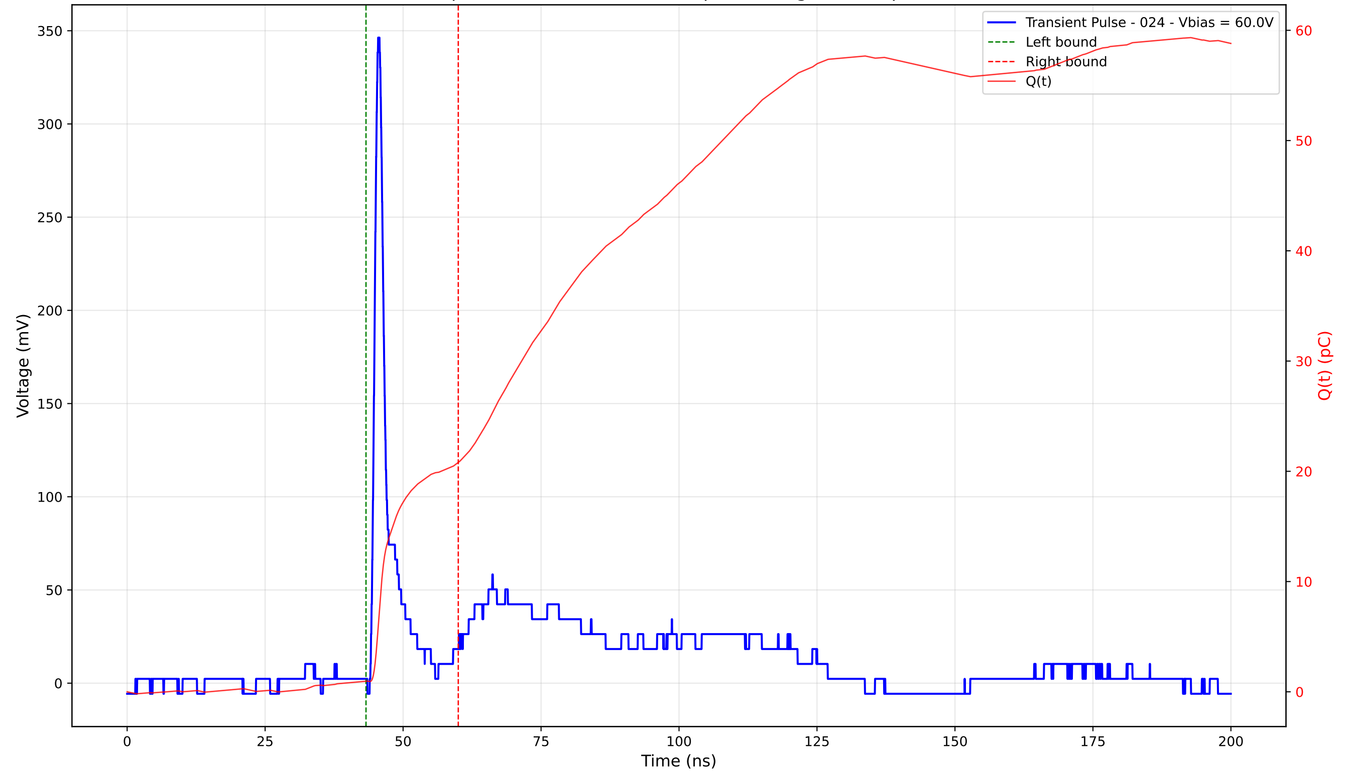
Transient Pulse - Sample: 4003 - Position: 135.0 \mu\text{m} - Charge: 19.83 pC - Rise Time: 0.98 ns
