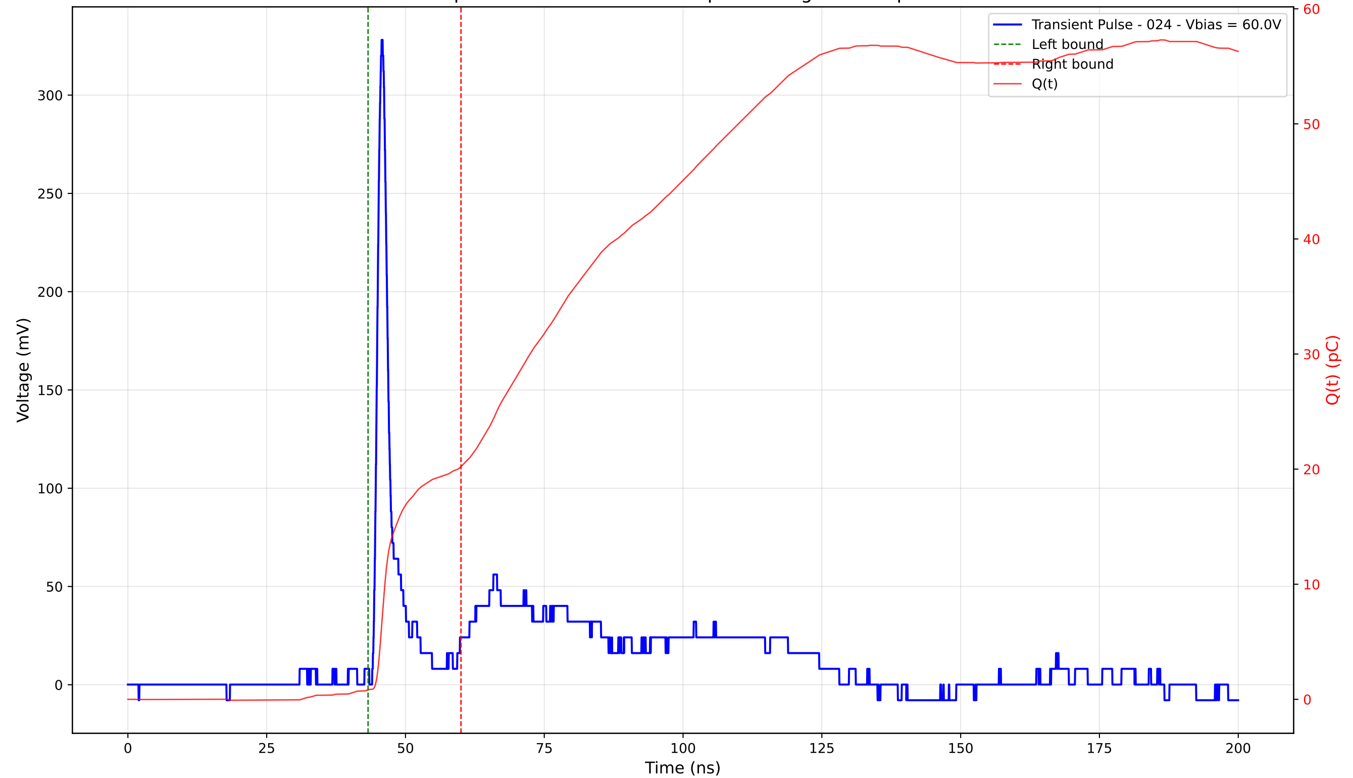
Transient Pulse - Sample: 4003 - Position: 155.0 \mu\text{m} - Charge: 19.39 pC - Rise Time: 1.08 ns
