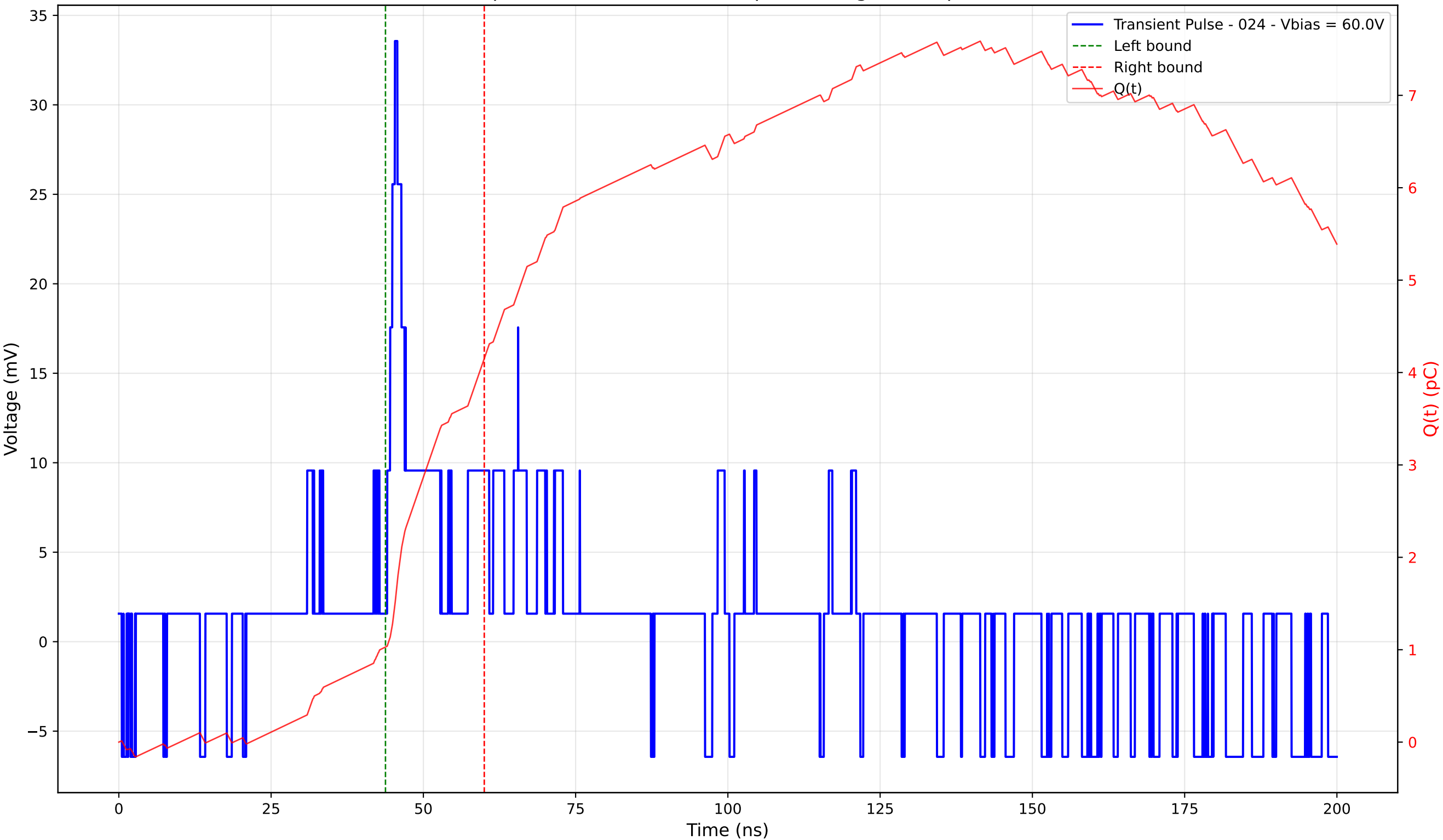
Transient Pulse - Sample: 4003 - Position: 85.0 \mu\text{m} - Charge: 3.13 pC - Rise Time: 1.28 ns
