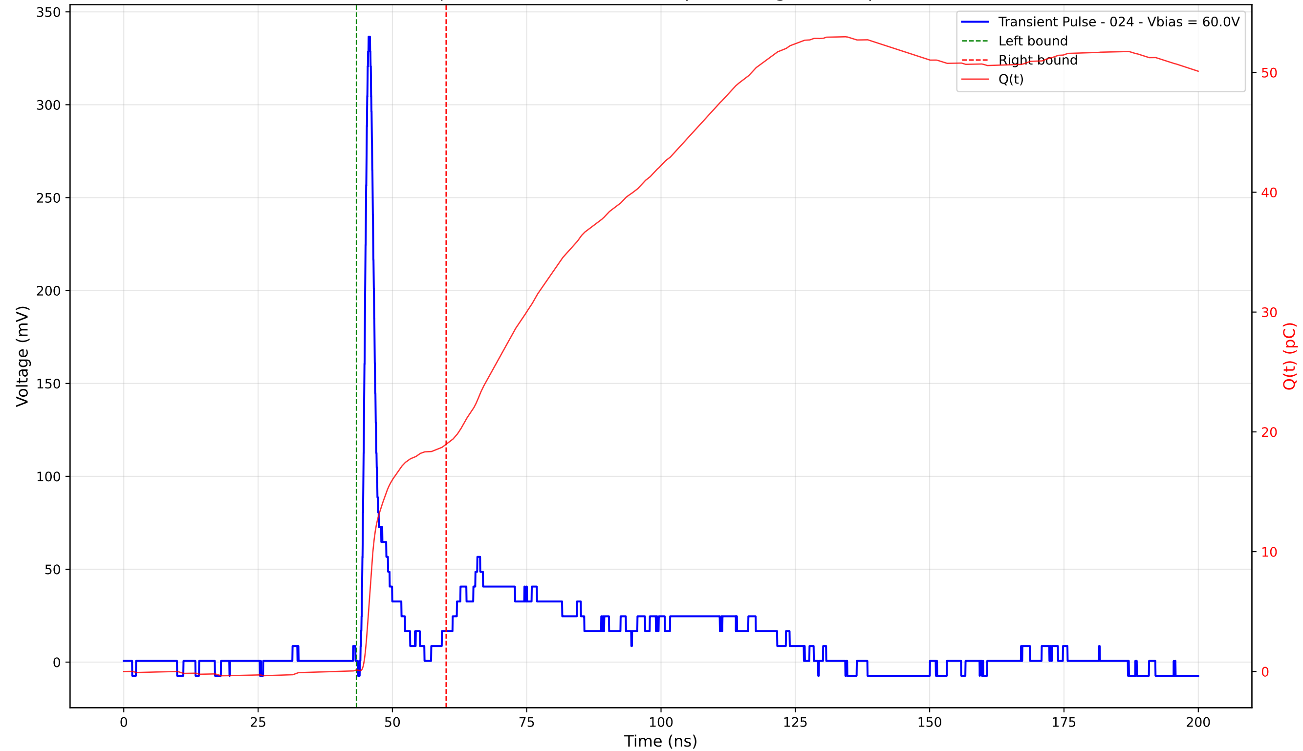
Transient Pulse - Sample: 4003 - Position: 145.0 \mu\text{m} - Charge: 18.85 pC - Rise Time: 1.00 ns
