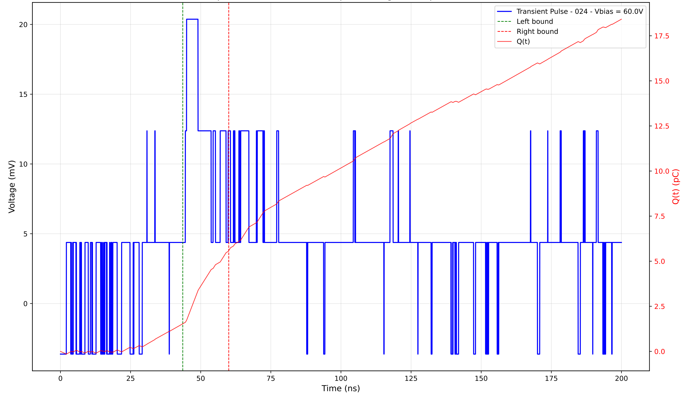
Transient Pulse - Sample: 4003 - Position: 65.0 \mu\text{m} - Charge: 4.07 pC - Rise Time: 0.00 ns (N/A)
