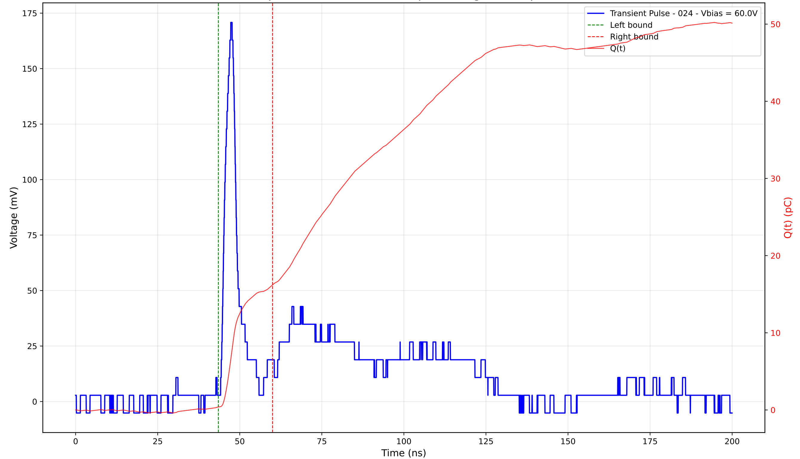
Transient Pulse - Sample: 4003 - Position: 205.0 \mu\text{m} - Charge: 15.84 pC - Rise Time: 2.40 ns
