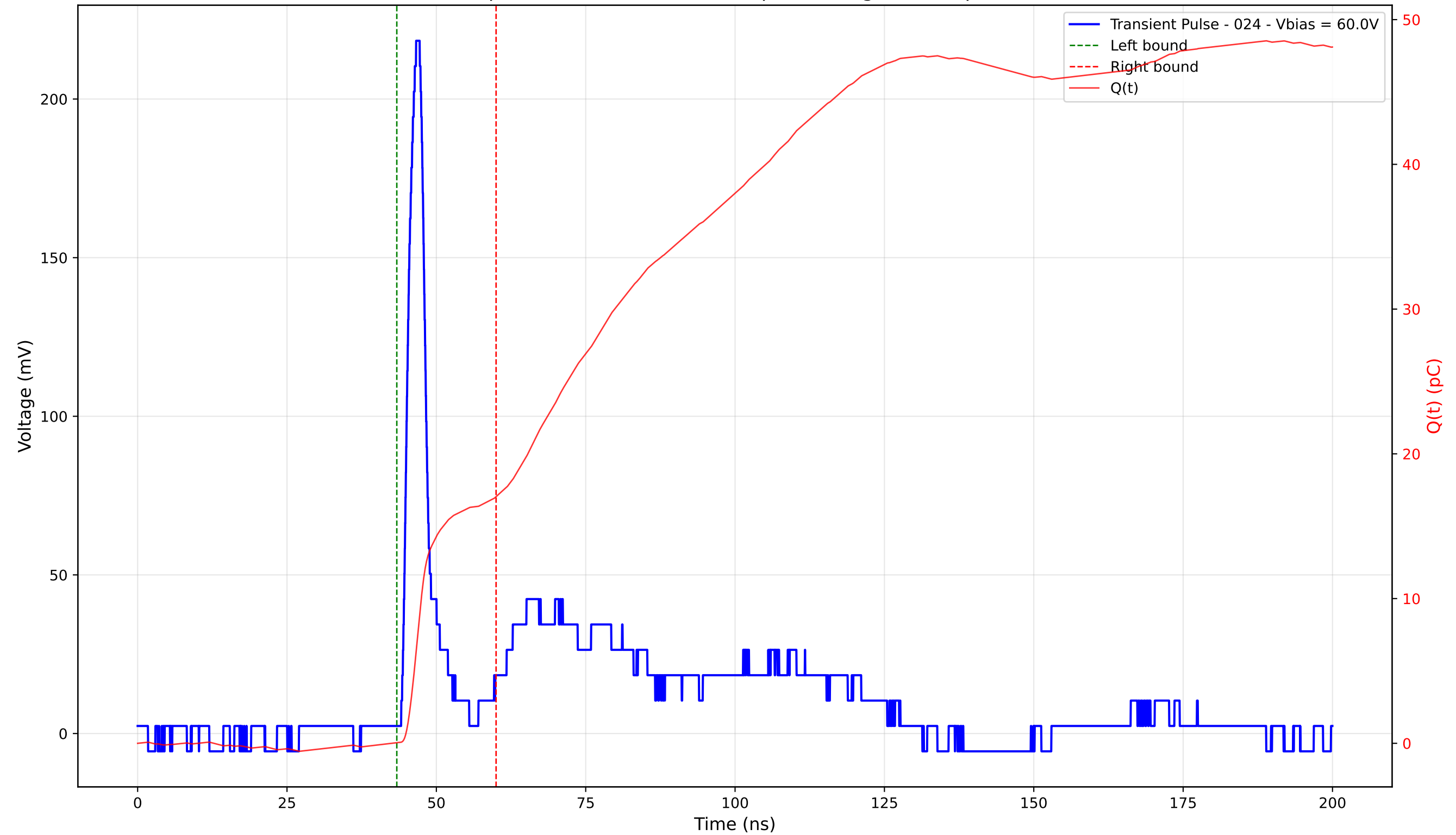
Transient Pulse - Sample: 4003 - Position: 195.0 \mu\text{m} - Charge: 17.00 pC - Rise Time: 1.83 ns
