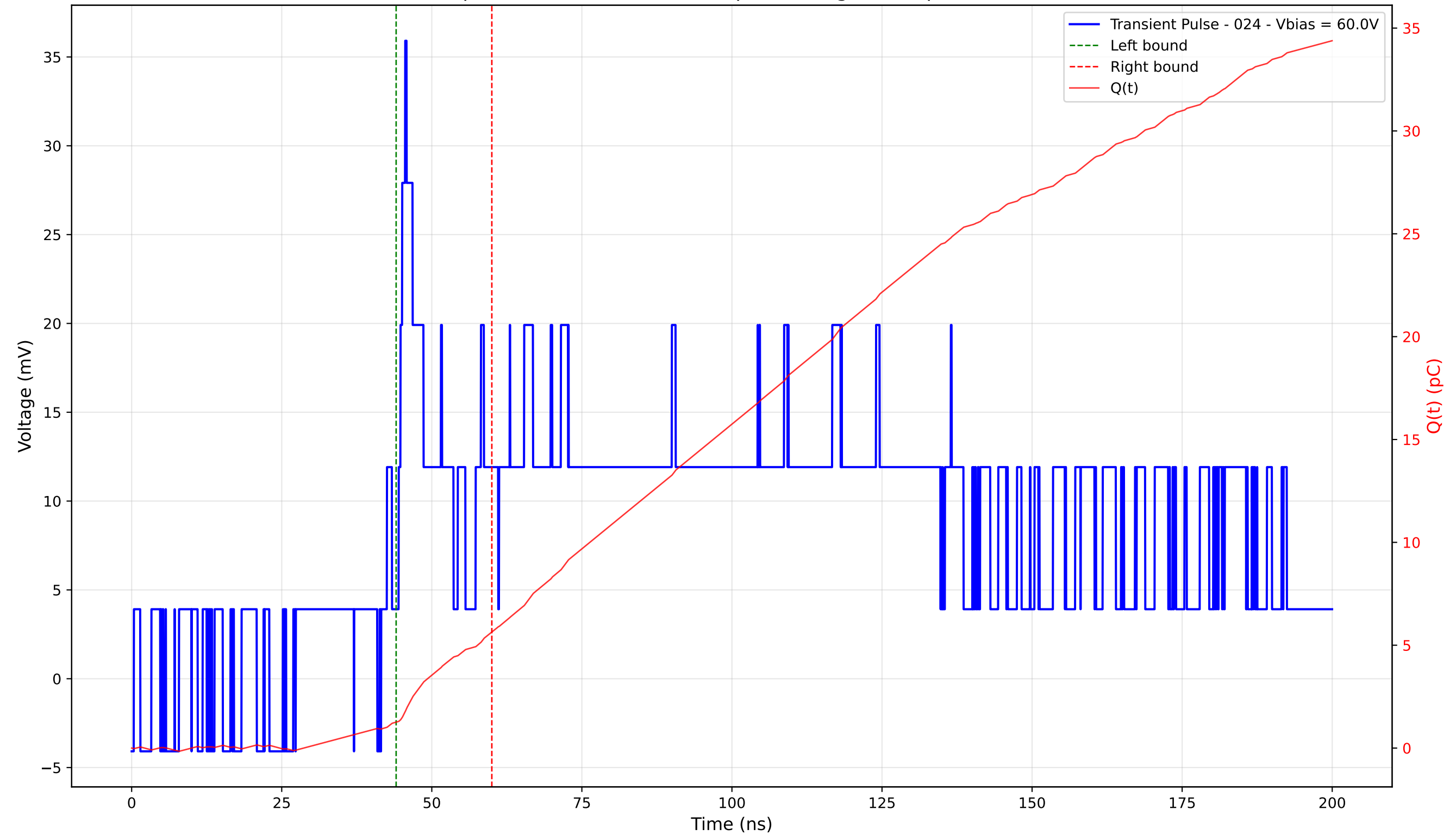
Transient Pulse - Sample: 4003 - Position: 240.0 \mu\text{m} - Charge: 4.39 pC - Rise Time: 0.00 ns (N/A)
