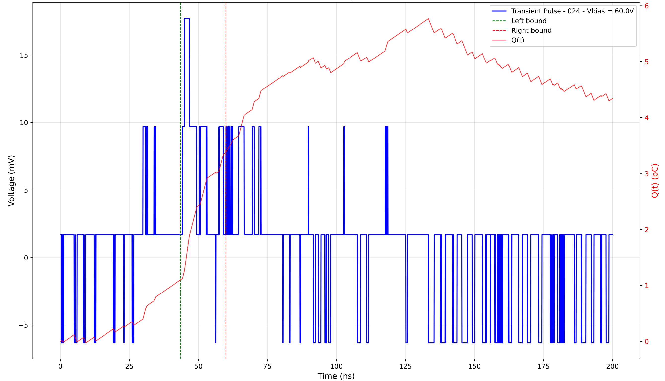
Transient Pulse - Sample: 4003 - Position: 355.0 \mu\text{m} - Charge: 2.27 pC - Rise Time: 0.70 ns
