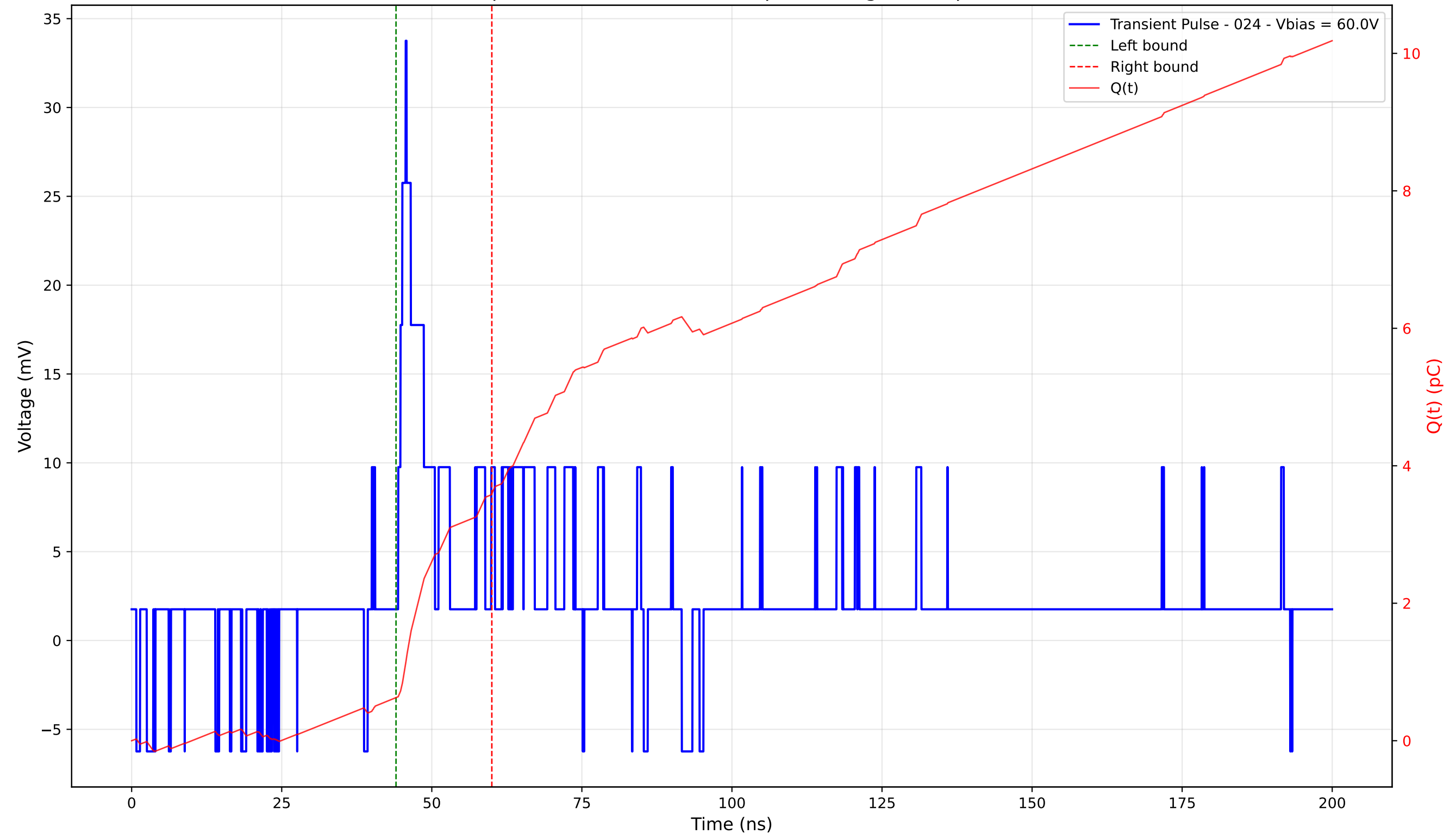
Transient Pulse - Sample: 4003 - Position: 265.0 \mu\text{m} - Charge: 2.97 pC - Rise Time: 1.26 ns
