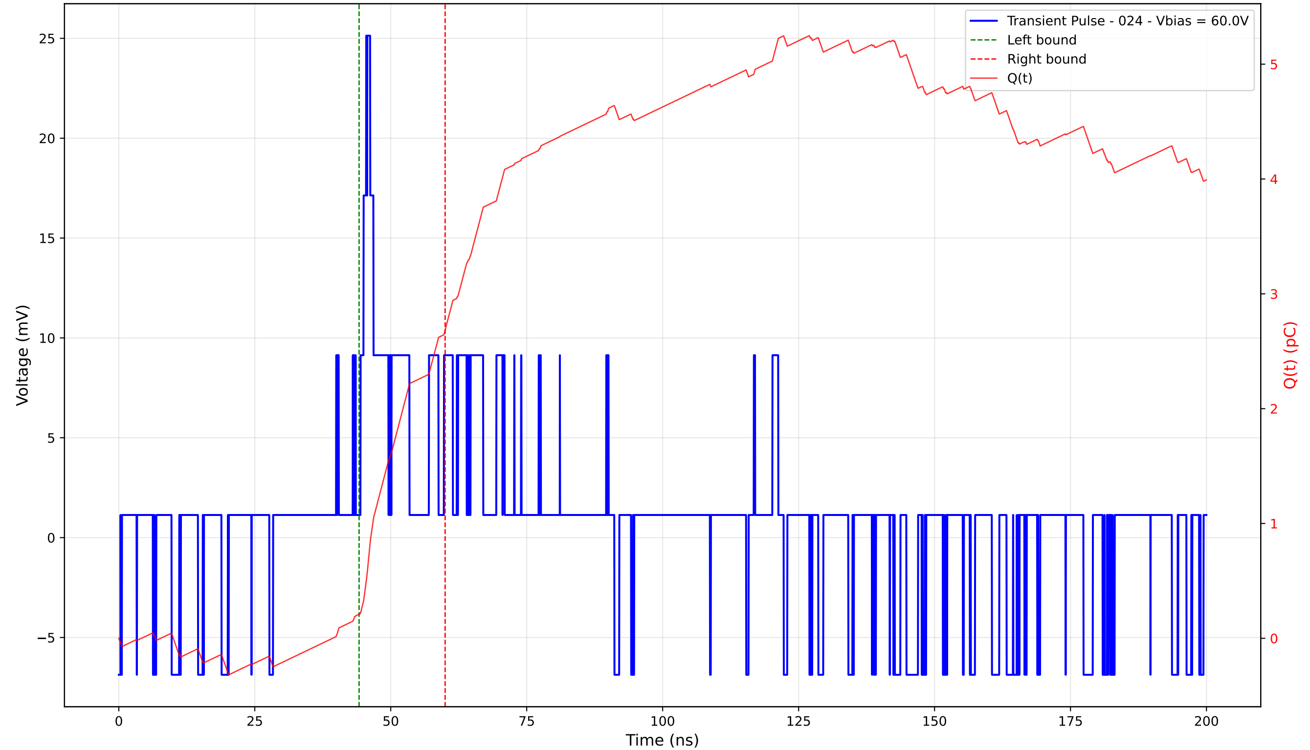
Transient Pulse - Sample: 4003 - Position: 365.0 \mu\text{m} - Charge: 2.48 pC - Rise Time: 1.06 ns
