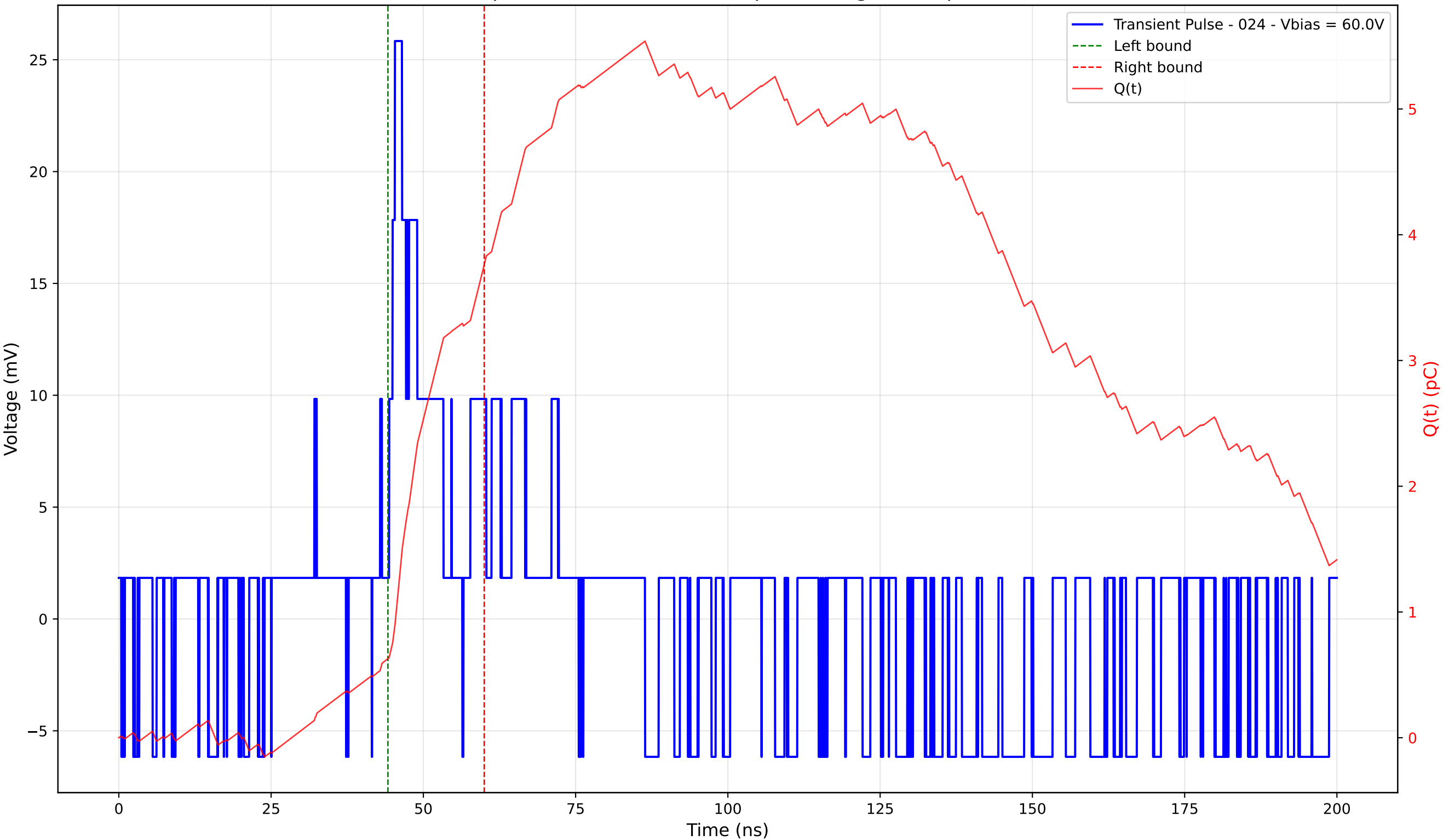
Transient Pulse - Sample: 4003 - Position: 50.0 \mu\text{m} - Charge: 3.14 pC - Rise Time: 0.96 ns
