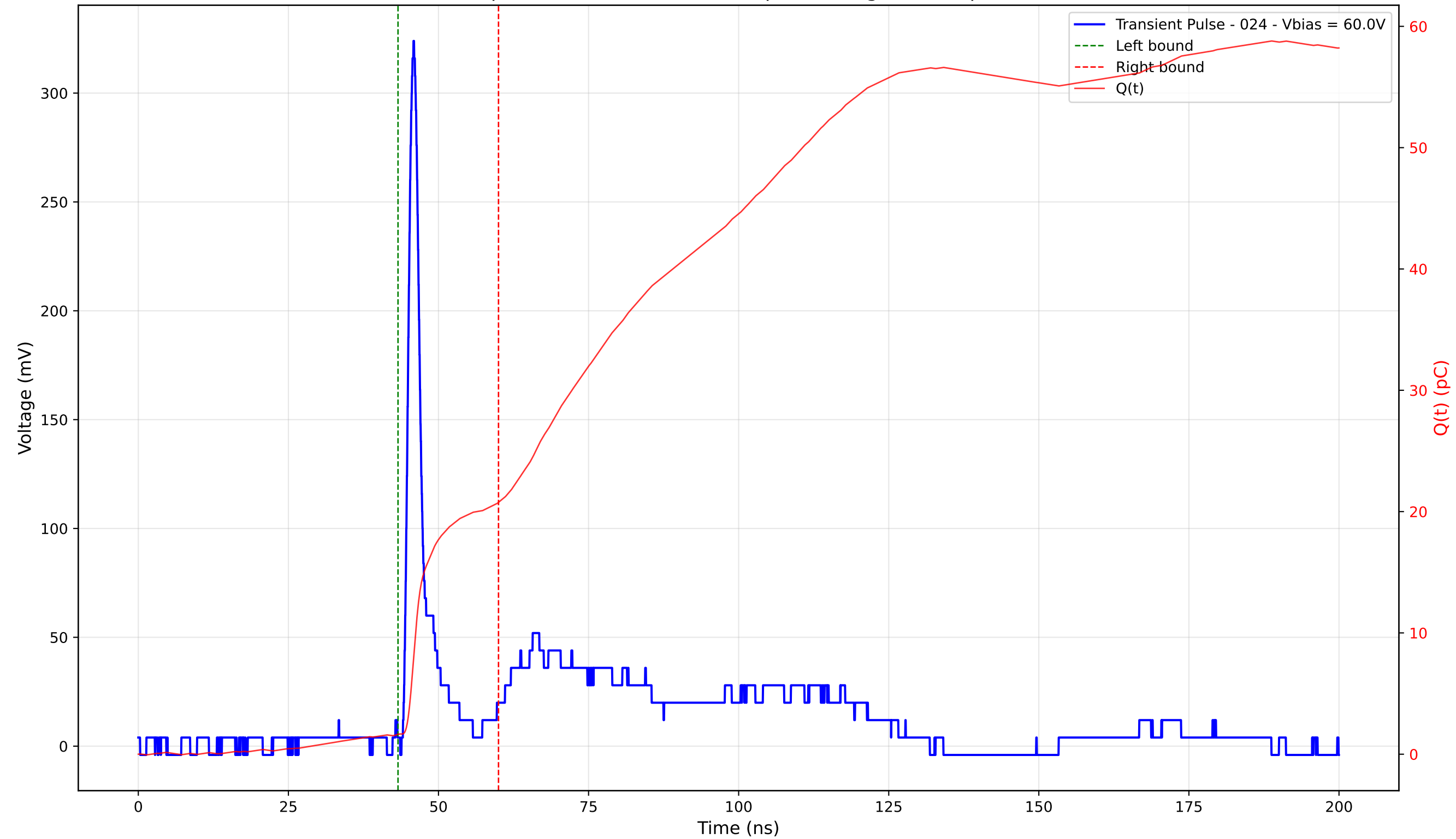
Transient Pulse - Sample: 4003 - Position: 160.0 \mu\text{m} - Charge: 19.11 pC - Rise Time: 1.15 ns
