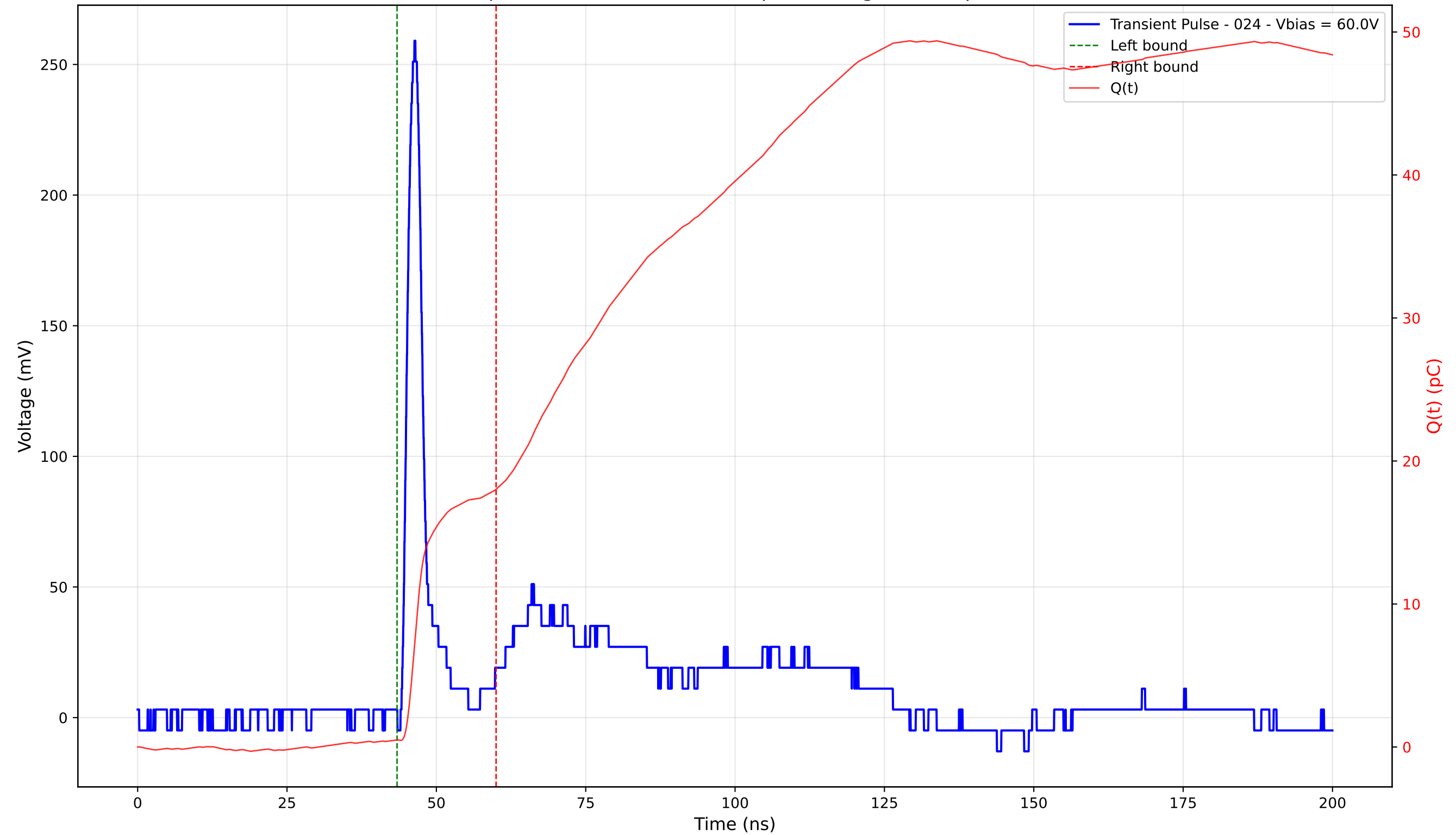
Transient Pulse - Sample: 4003 - Position: 185.0 \mu\text{m} - Charge: 17.51 pC - Rise Time: 1.44 ns
