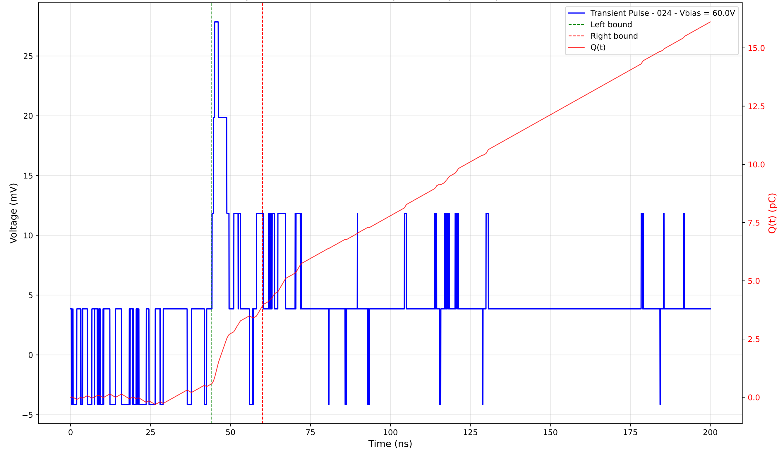
Transient Pulse - Sample: 4003 - Position: 260.0 \mu\text{m} - Charge: 3.37 pC - Rise Time: 0.00 ns (N/A)
