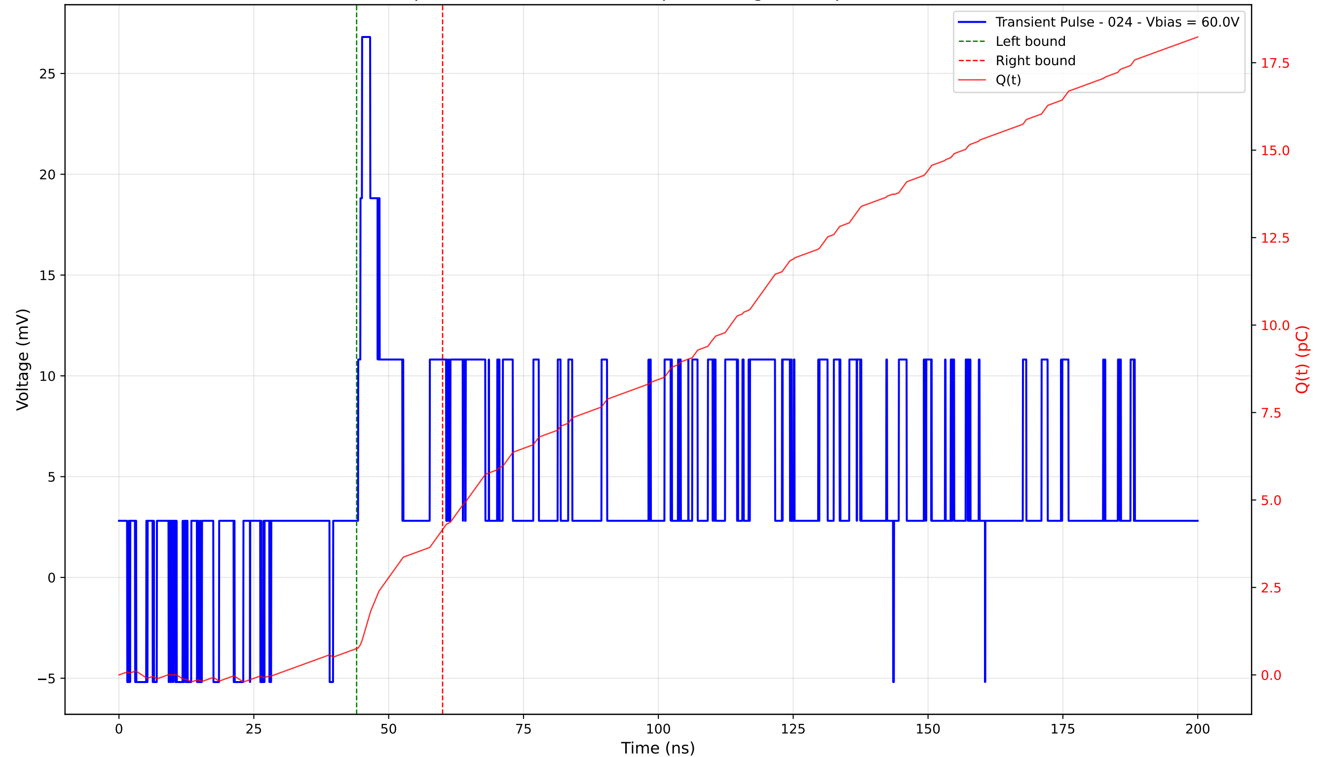
Transient Pulse - Sample: 4003 - Position: 255.0 \mu\text{m} - Charge: 3.41 pC - Rise Time: 0.00 ns (N/A)
