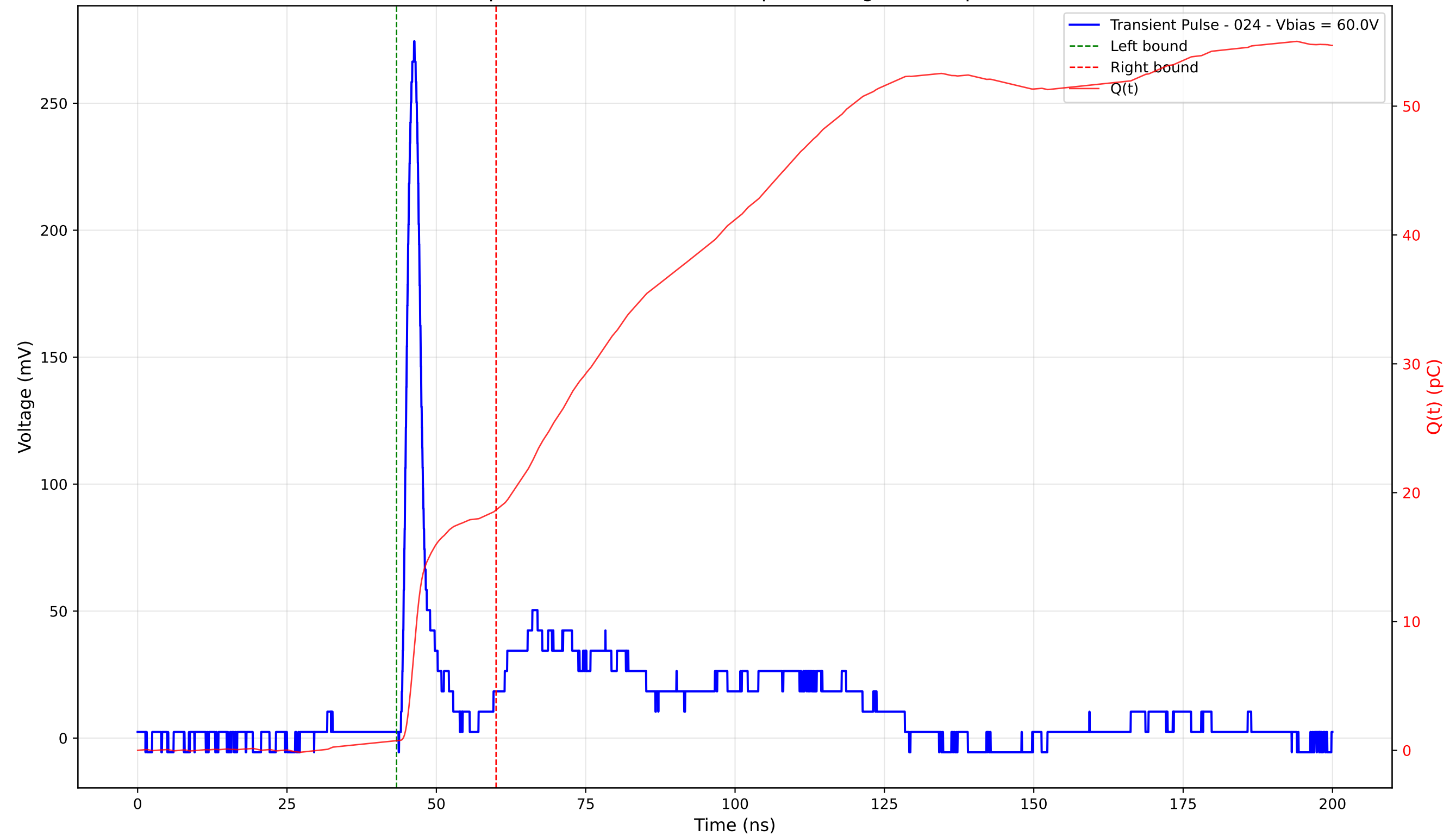
Transient Pulse - Sample: 4003 - Position: 180.0 \mu\text{m} - Charge: 17.89 pC - Rise Time: 1.38 ns
