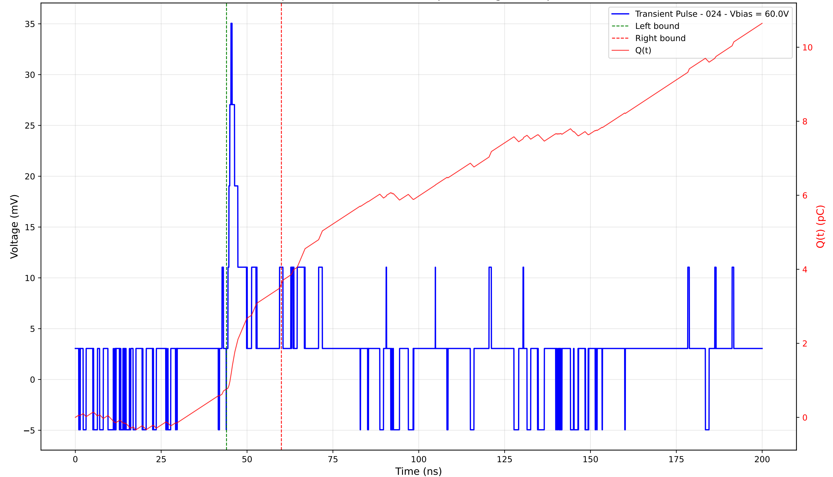
Transient Pulse - Sample: 4003 - Position: 280.0 \mu\text{m} - Charge: 2.85 pC - Rise Time: 0.90 ns
