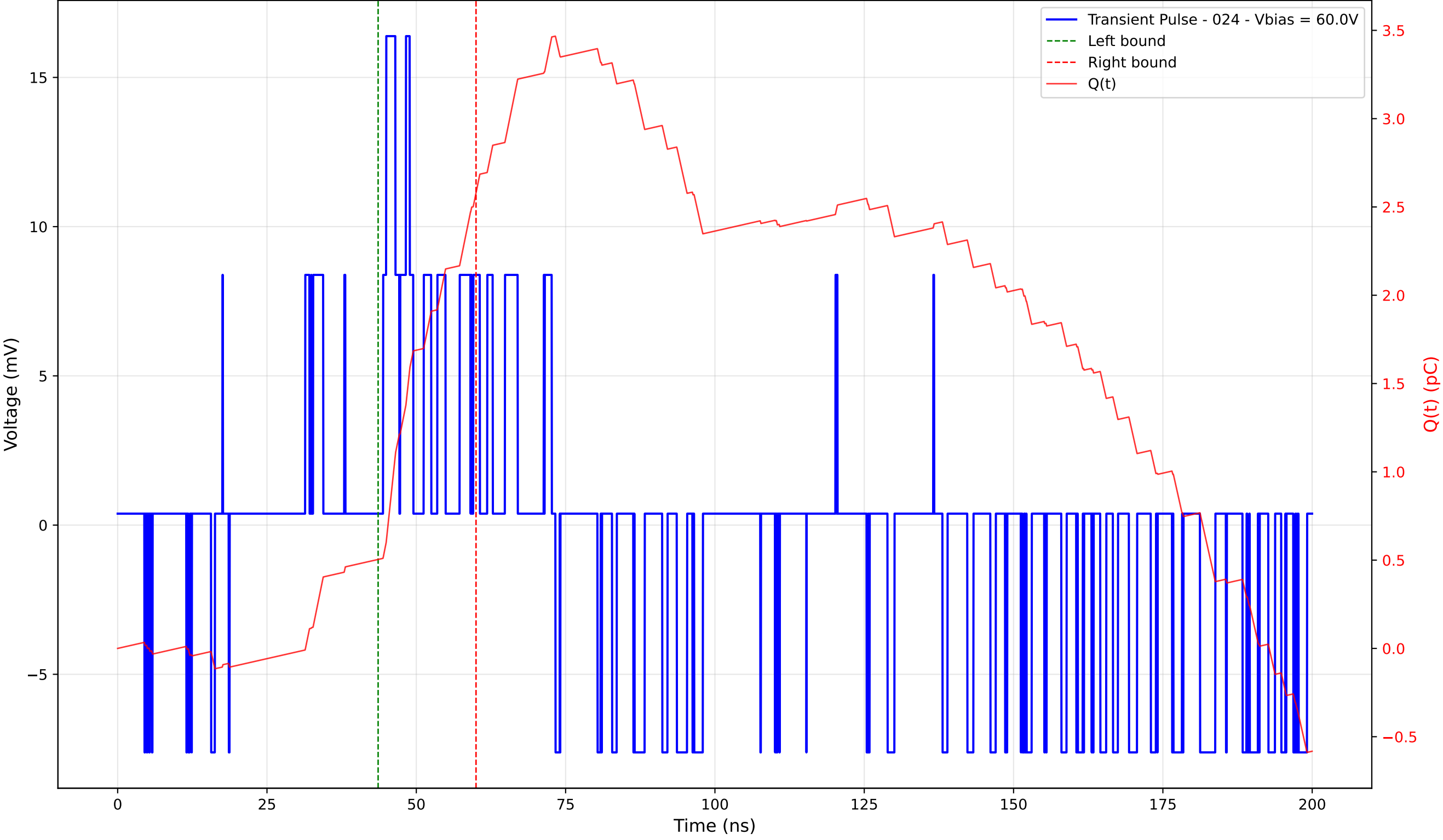
Transient Pulse - Sample: 4003 - Position: 80.0 \mu\text{m} - Charge: 2.08 pC - Rise Time: 0.54 ns
