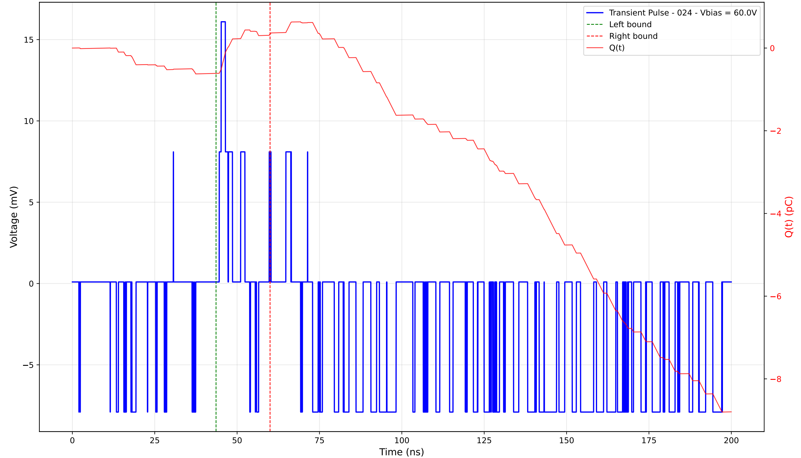
Transient Pulse - Sample: 4003 - Position: 415.0 \mu\text{m} - Charge: 0.96 pC - Rise Time: 0.60 ns
