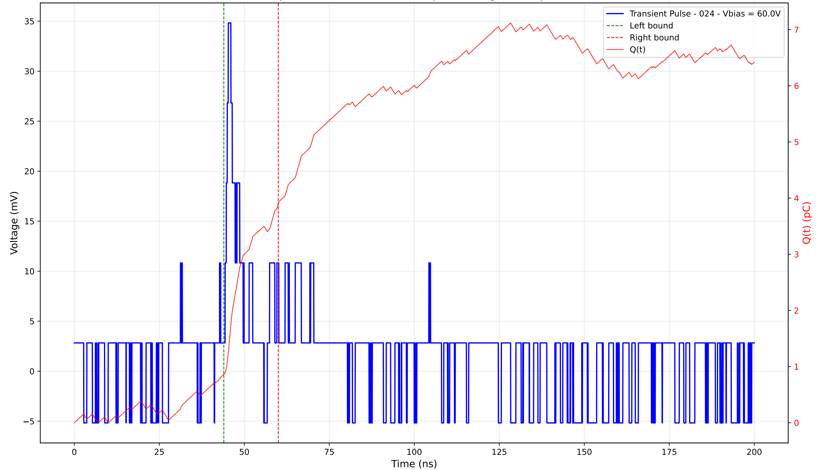
Transient Pulse - Sample: 4003 - Position: 390.0 \mu\text{m} - Charge: 3.04 pC - Rise Time: 0.94 ns
