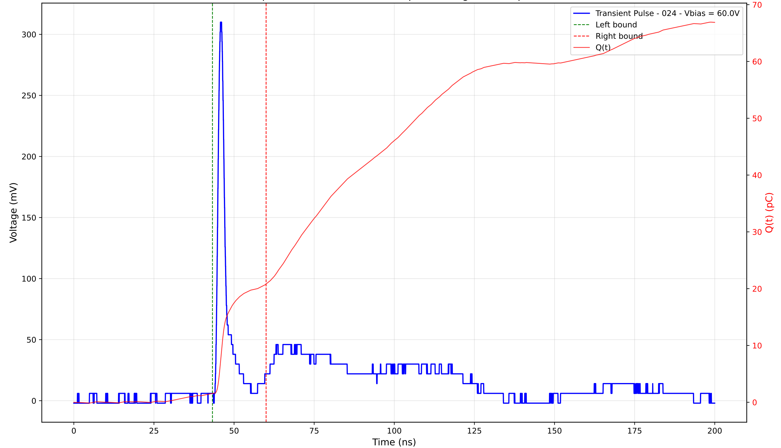
Transient Pulse - Sample: 4003 - Position: 165.0 \mu\text{m} - Charge: 19.26 pC - Rise Time: 1.18 ns
