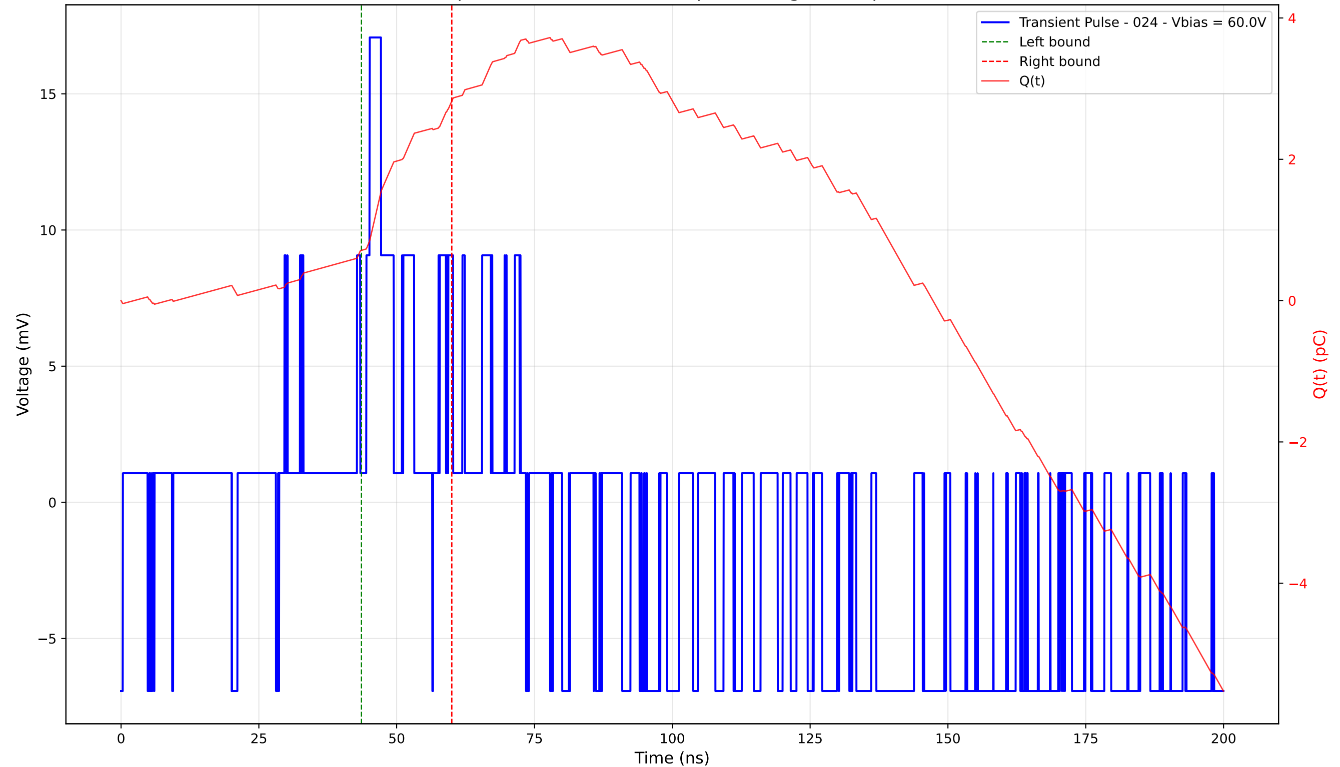
Transient Pulse - Sample: 4003 - Position: 40.0 \mu\text{m} - Charge: 2.12 pC - Rise Time: 0.60 ns
