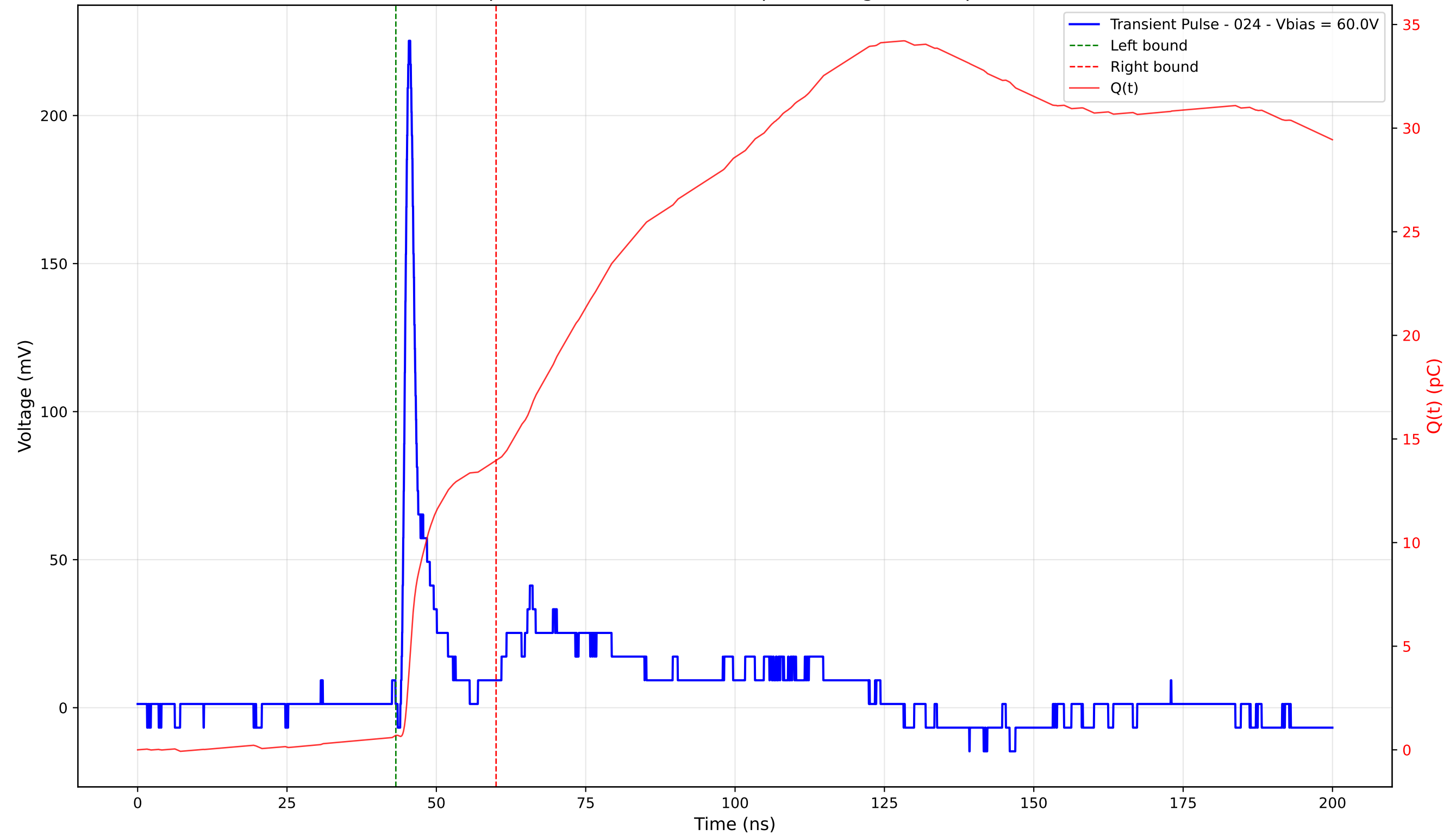
Transient Pulse - Sample: 4003 - Position: 110.0 \mu\text{m} - Charge: 13.26 pC - Rise Time: 0.95 ns
