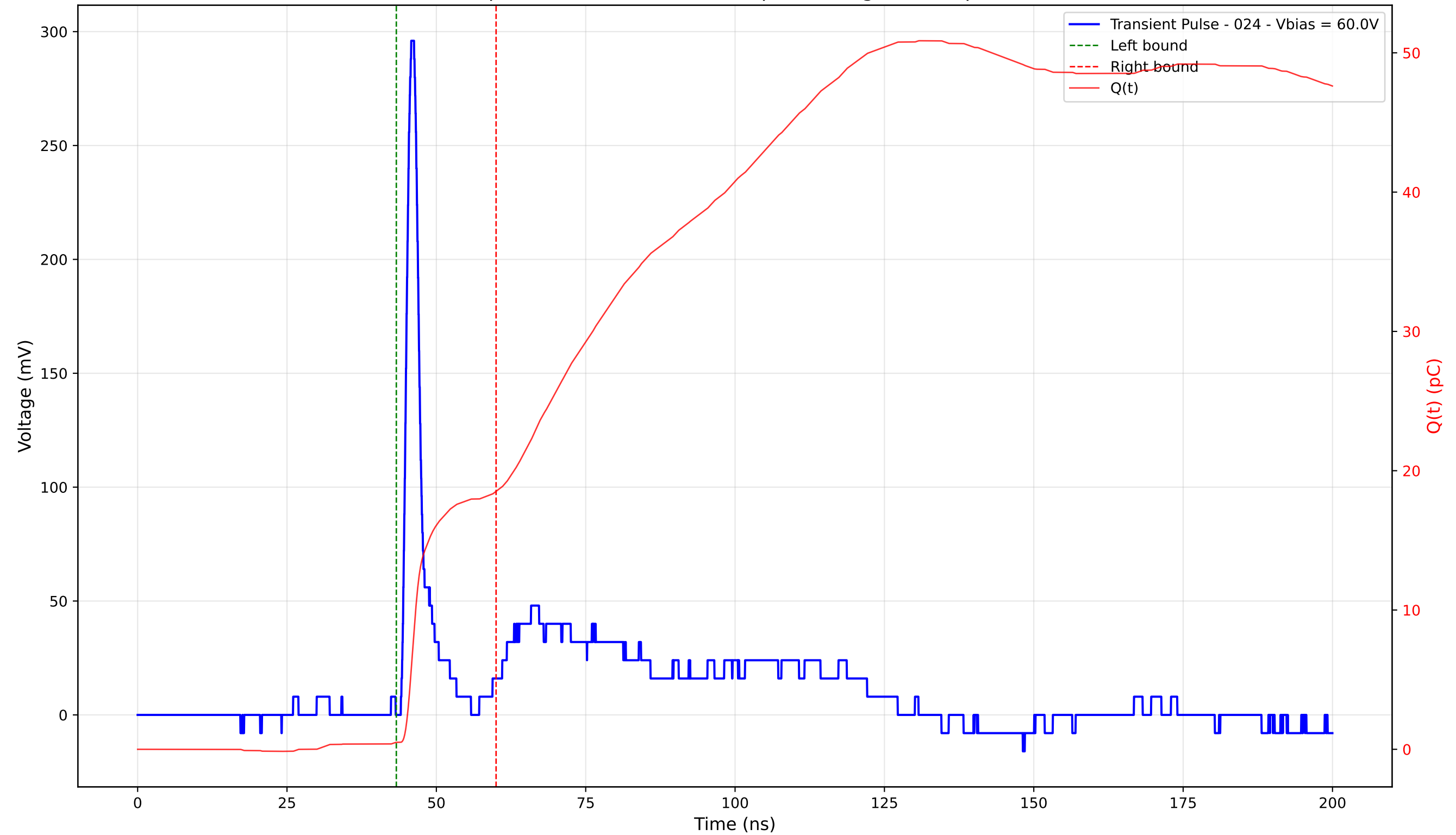
Transient Pulse - Sample: 4003 - Position: 170.0 \mu\text{m} - Charge: 18.02 pC - Rise Time: 1.23 ns
