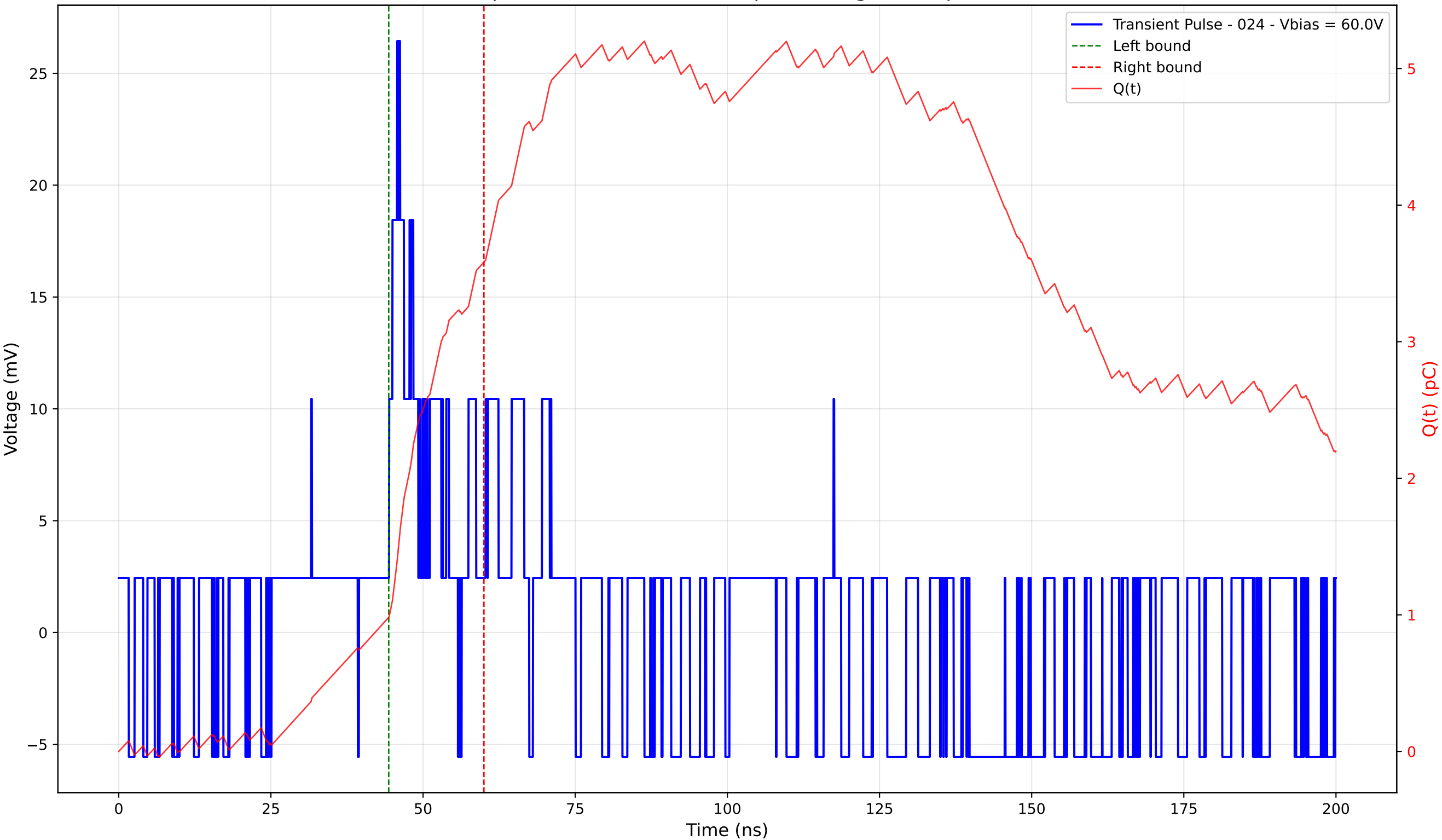
Transient Pulse - Sample: 4003 - Position: 45.0 \mu\text{m} - Charge: 2.60 pC - Rise Time: 1.34 ns
