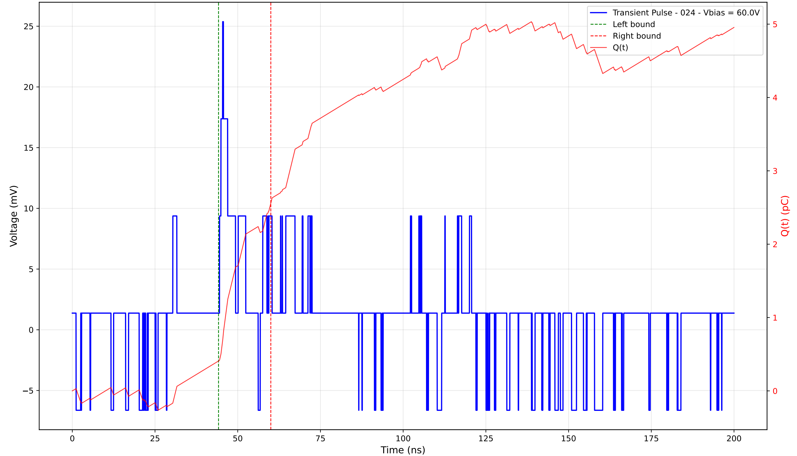
Transient Pulse - Sample: 4003 - Position: 335.0 \mu\text{m} - Charge: 2.15 pC - Rise Time: 0.96 ns
