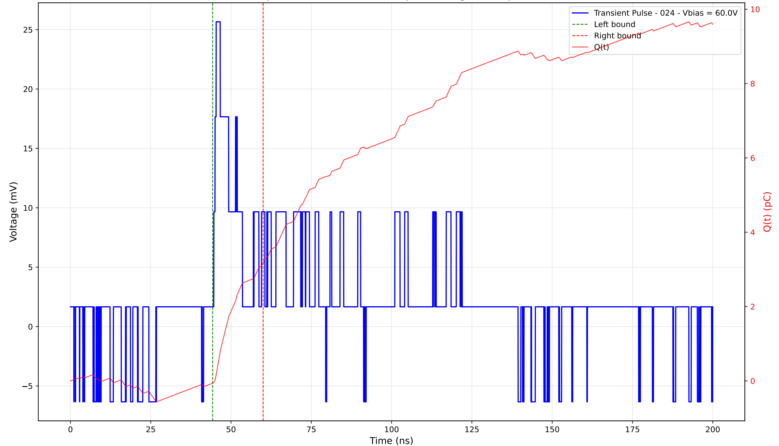
Transient Pulse - Sample: 4003 - Position: 55.0 \mu\text{m} - Charge: 3.24 pC - Rise Time: 0.74 ns
