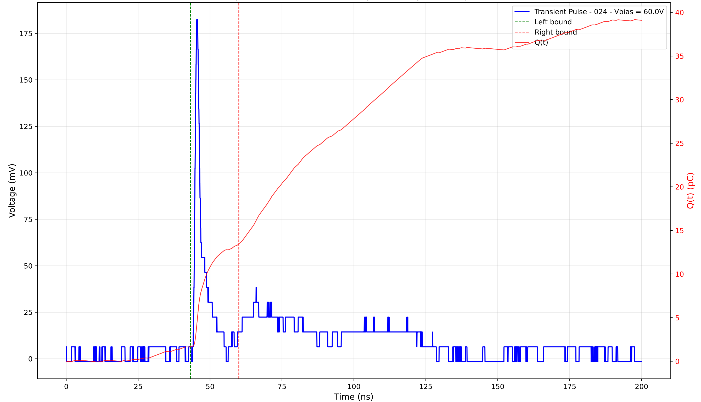
Transient Pulse - Sample: 4003 - Position: 105.0 \mu\text{m} - Charge: 11.76 pC - Rise Time: 0.93 ns
