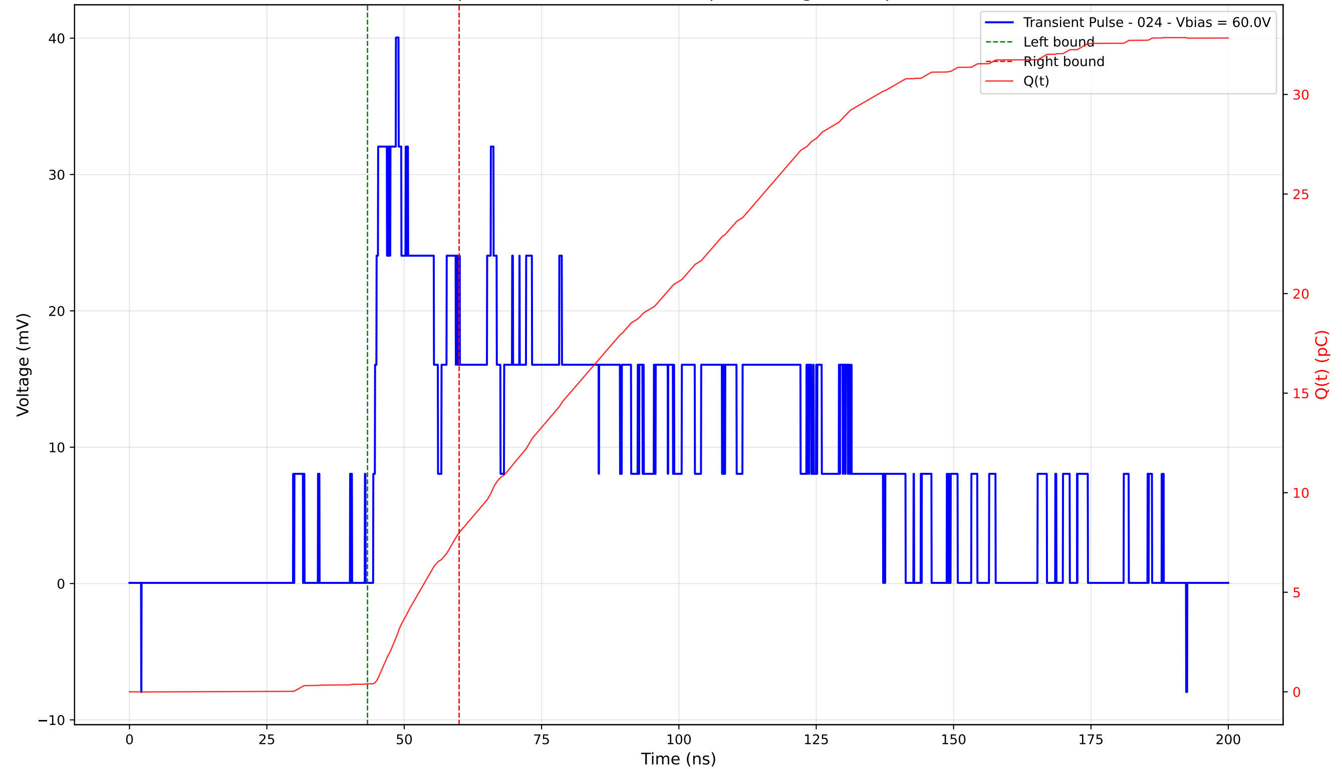
Transient Pulse - Sample: 4003 - Position: 225.0 \mu\text{m} - Charge: 7.58 pC - Rise Time: 4.13 ns
