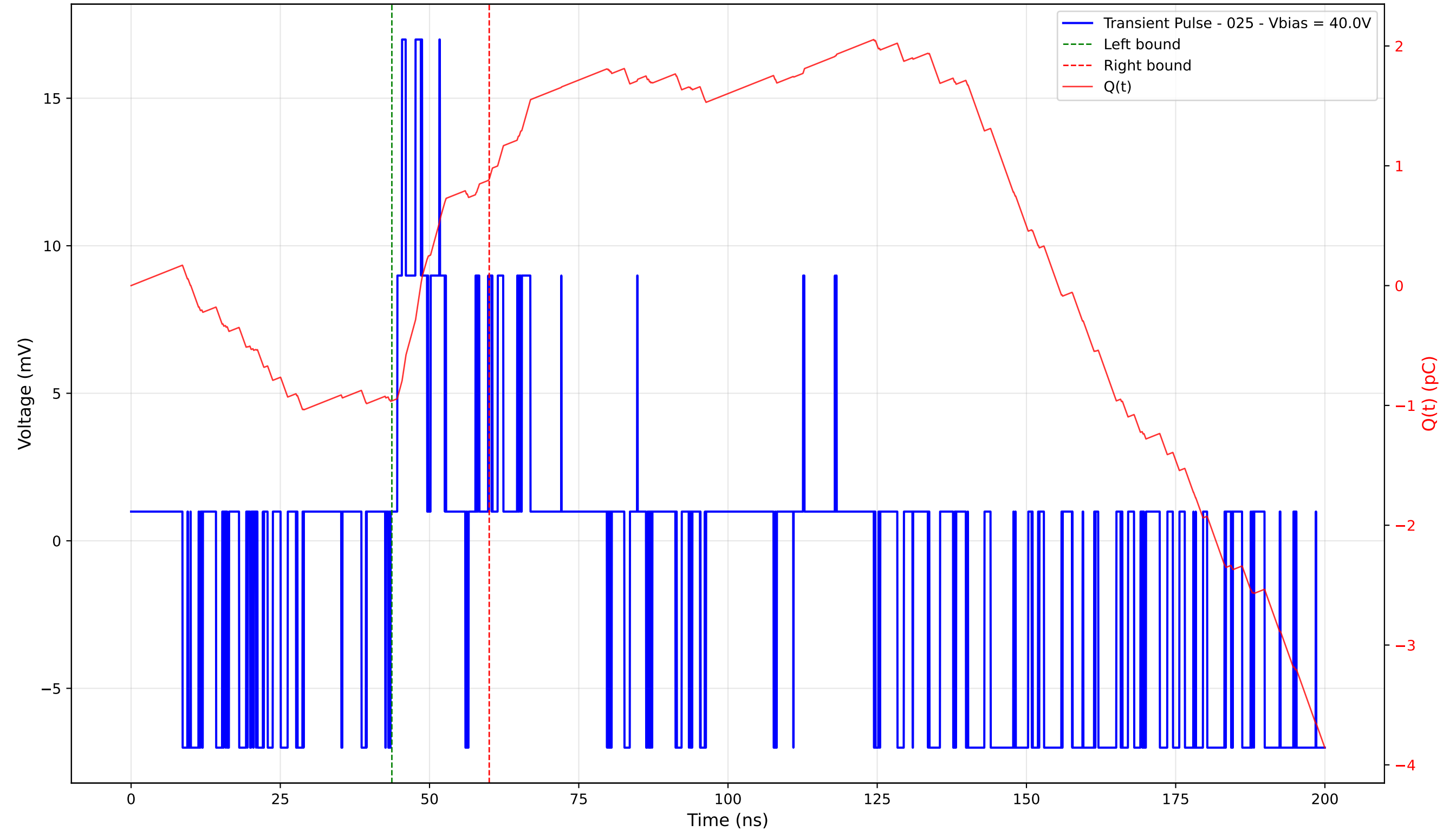
Transient Pulse - Sample: 4003 - Position: 65.0 \mu\text{m} - Charge: 1.85 pC - Rise Time: 0.80 ns
