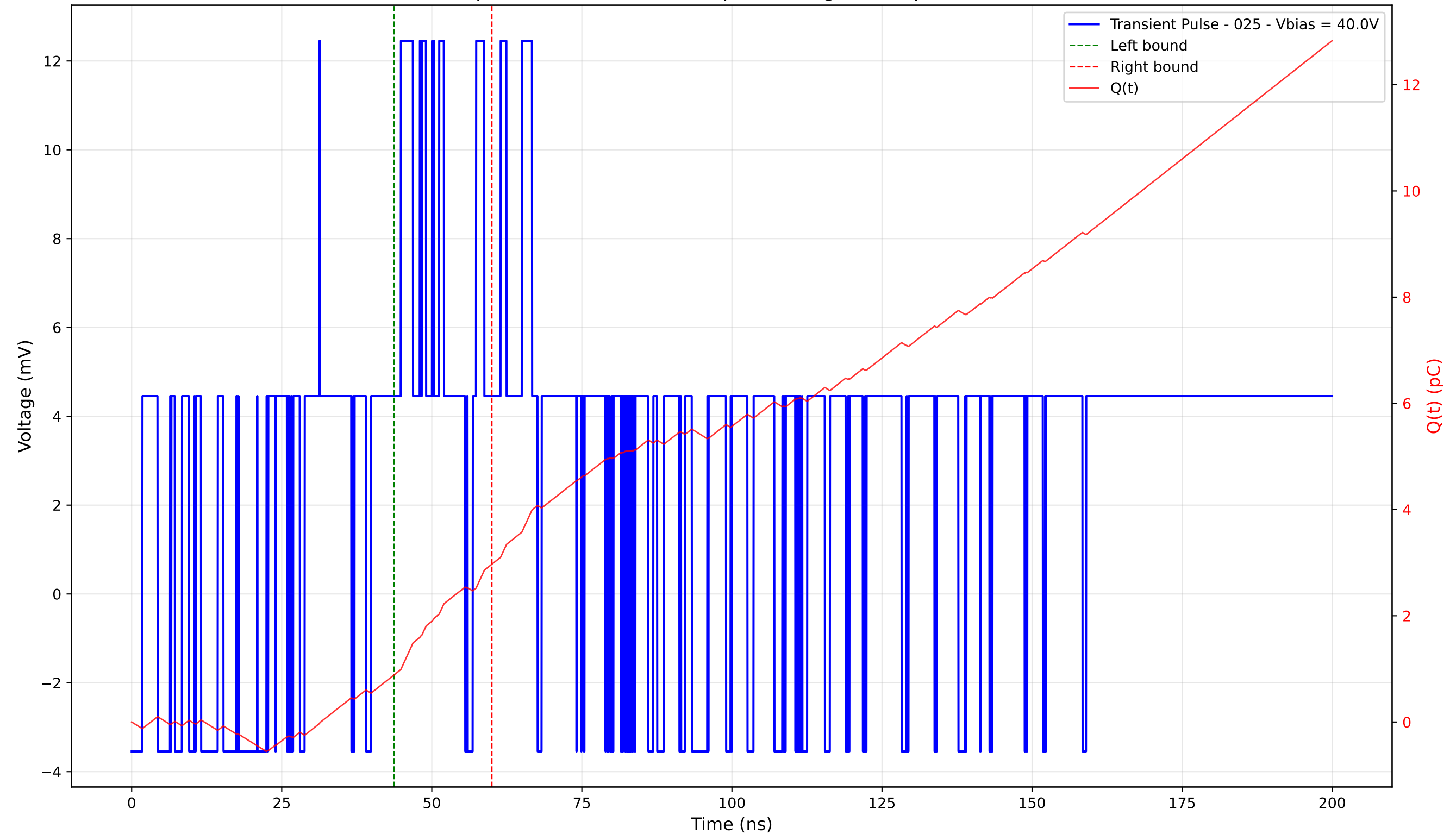
Transient Pulse - Sample: 4003 - Position: 5.0 \mu\text{m} - Charge: 2.09 pC - Rise Time: 0.00 ns (N/A)
