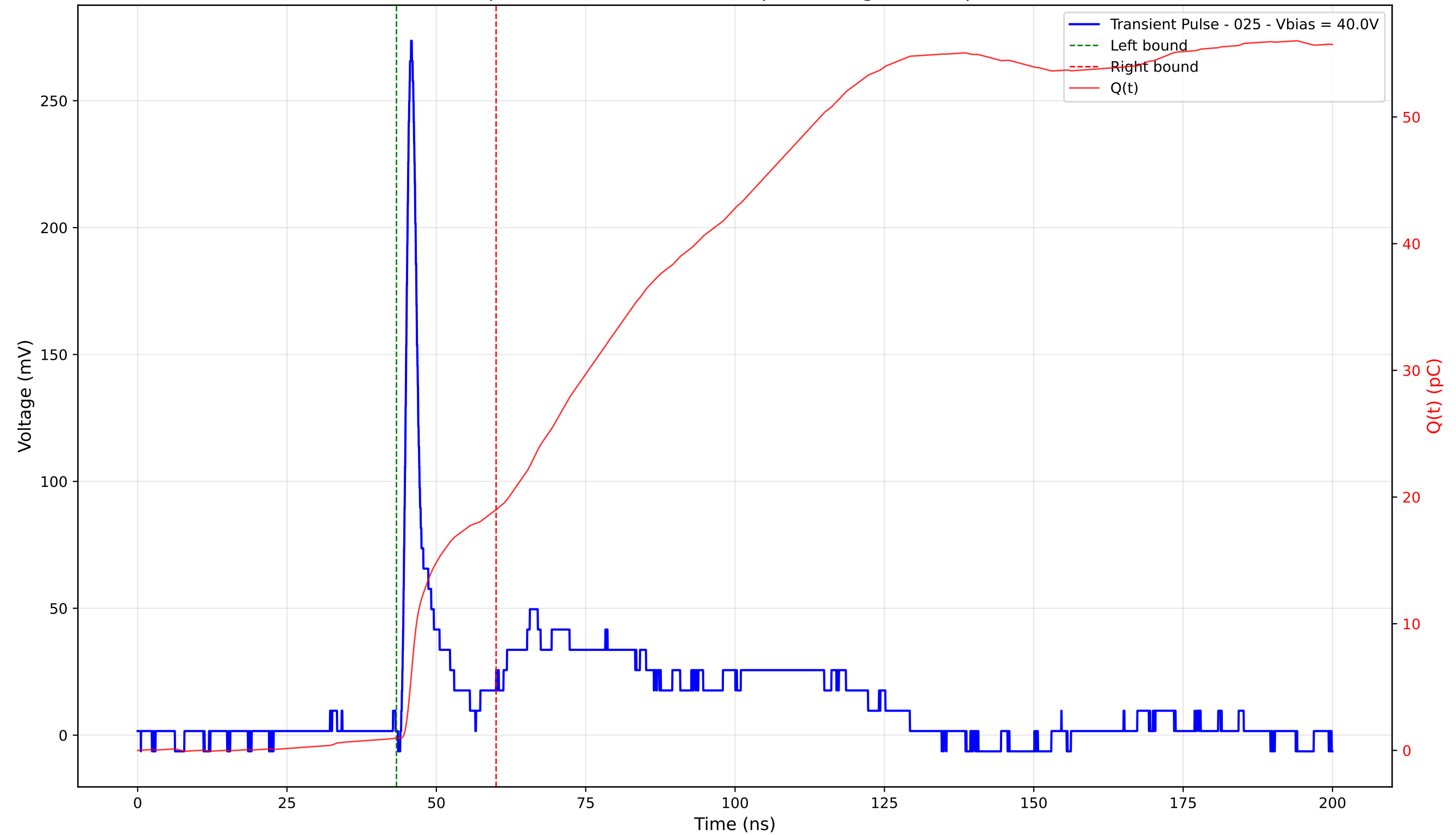
Transient Pulse - Sample: 4003 - Position: 140.0 \mu\text{m} - Charge: 17.99 pC - Rise Time: 1.10 ns
