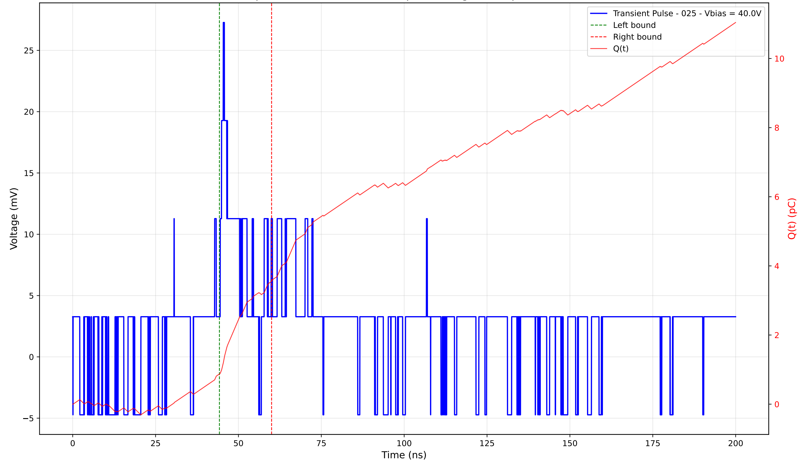
Transient Pulse - Sample: 4003 - Position: 270.0 \mu\text{m} - Charge: 2.69 pC - Rise Time: 0.00 ns (N/A)
