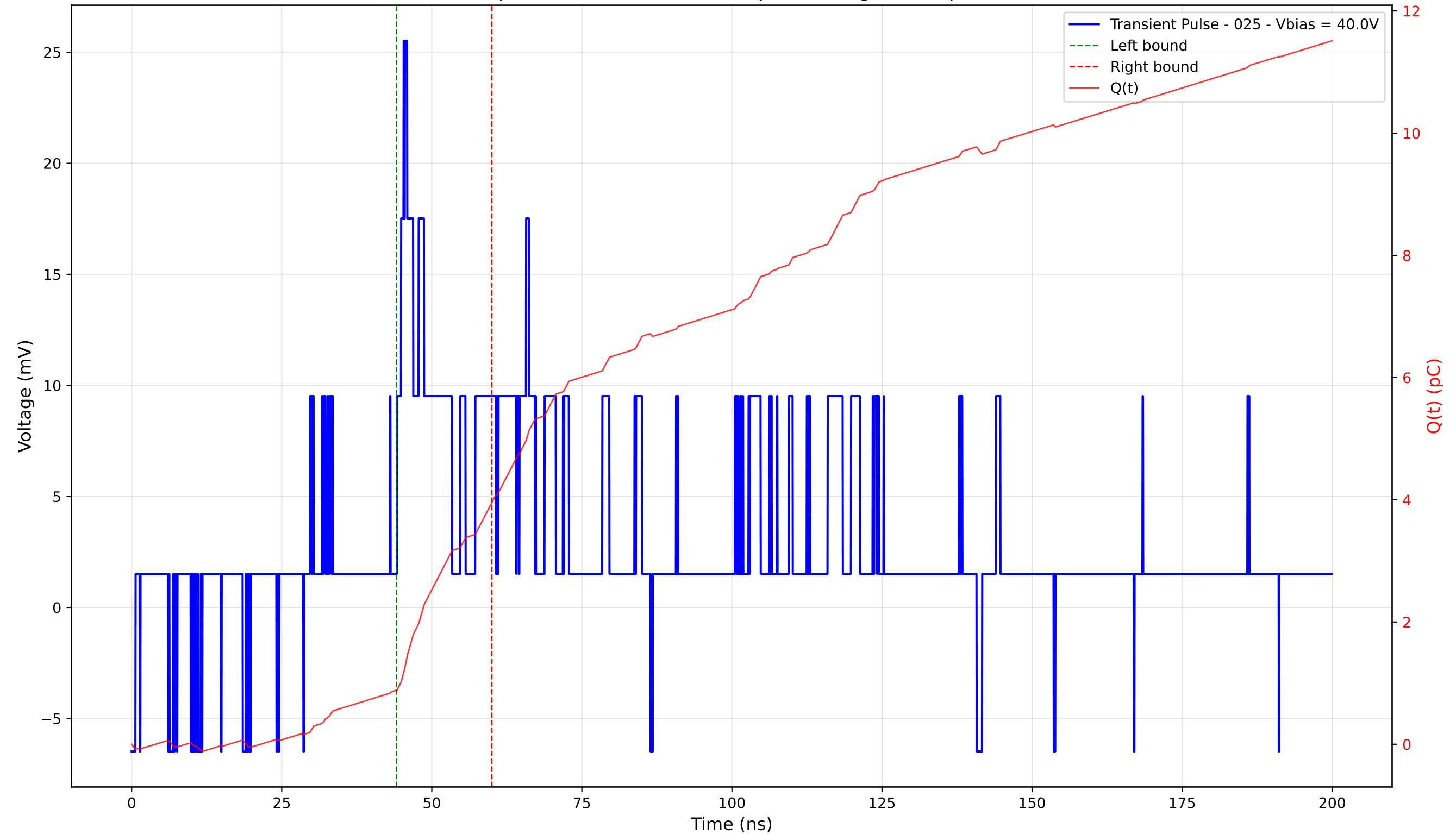
Transient Pulse - Sample: 4003 - Position: 85.0 \mu\text{m} - Charge: 3.08 pC - Rise Time: 1.10 ns
