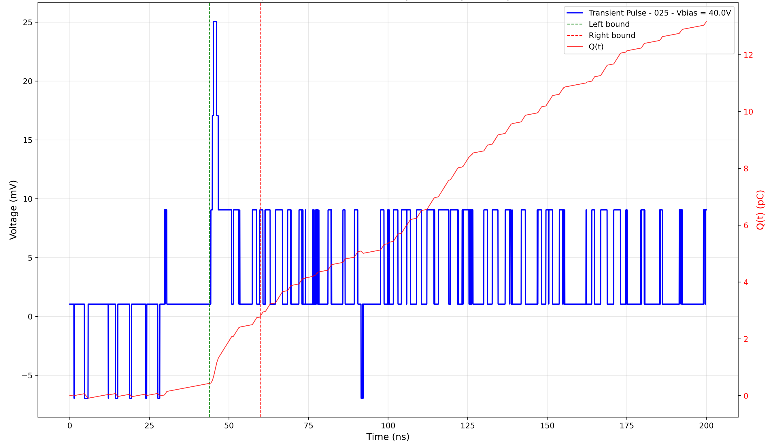
Transient Pulse - Sample: 4003 - Position: 225.0 \mu\text{m} - Charge: 2.39 pC - Rise Time: 0.84 ns
