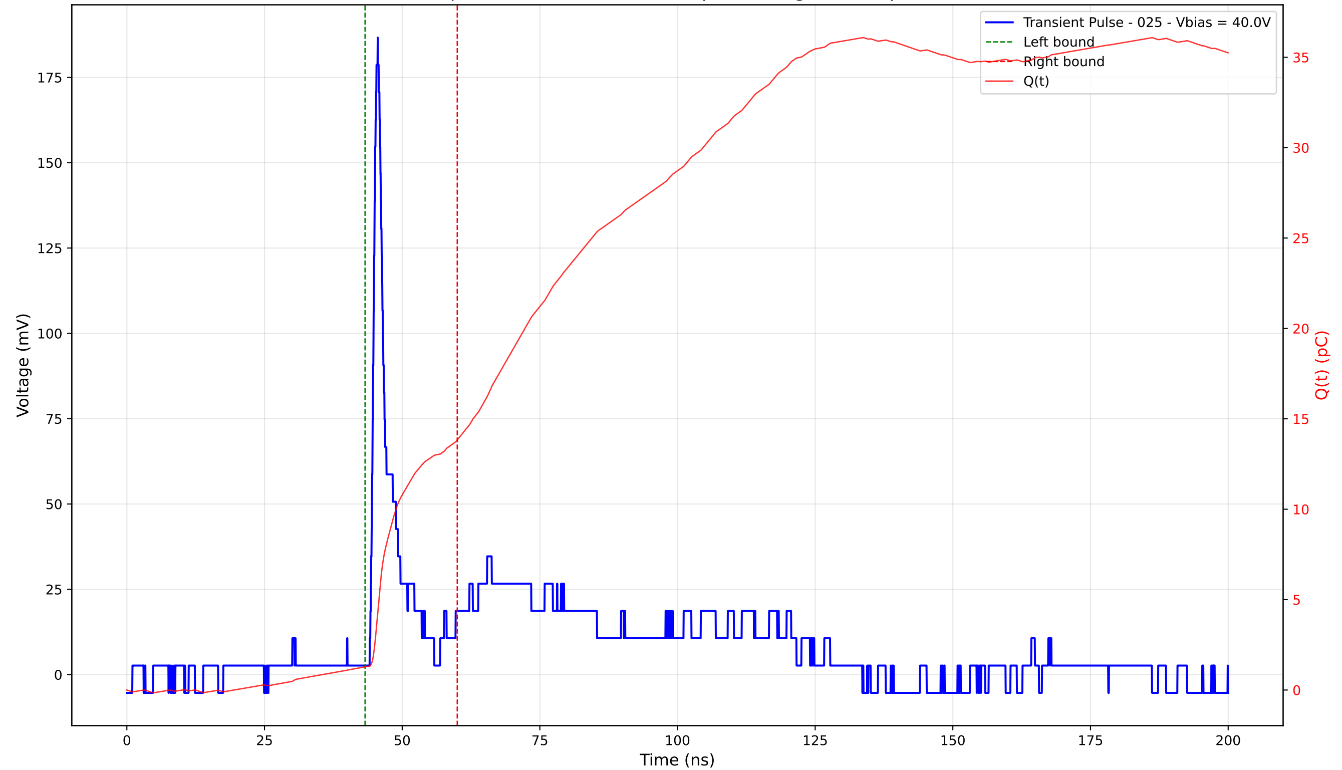
Transient Pulse - Sample: 4003 - Position: 110.0 \mu\text{m} - Charge: 12.56 pC - Rise Time: 0.96 ns
