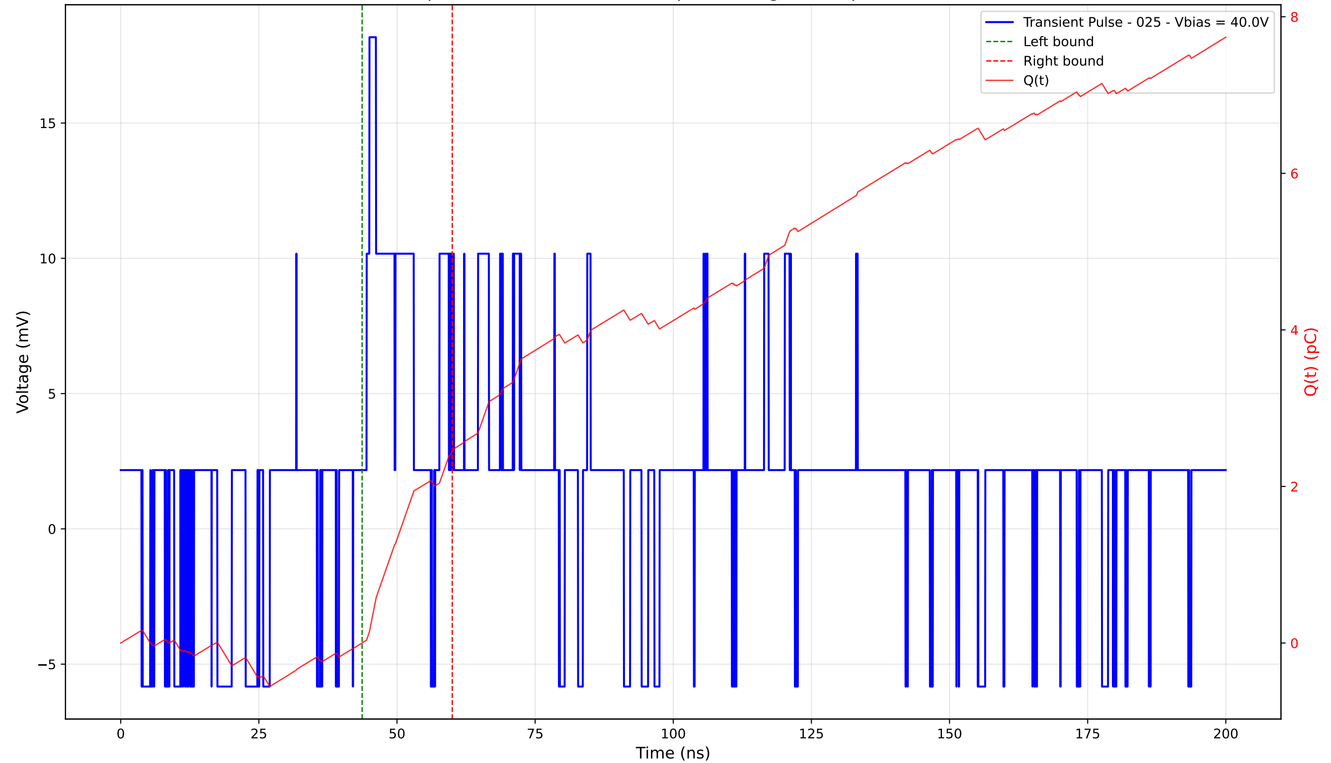
Transient Pulse - Sample: 4003 - Position: 350.0 \mu\text{m} - Charge: 2.45 pC - Rise Time: 0.00 ns (N/A)
