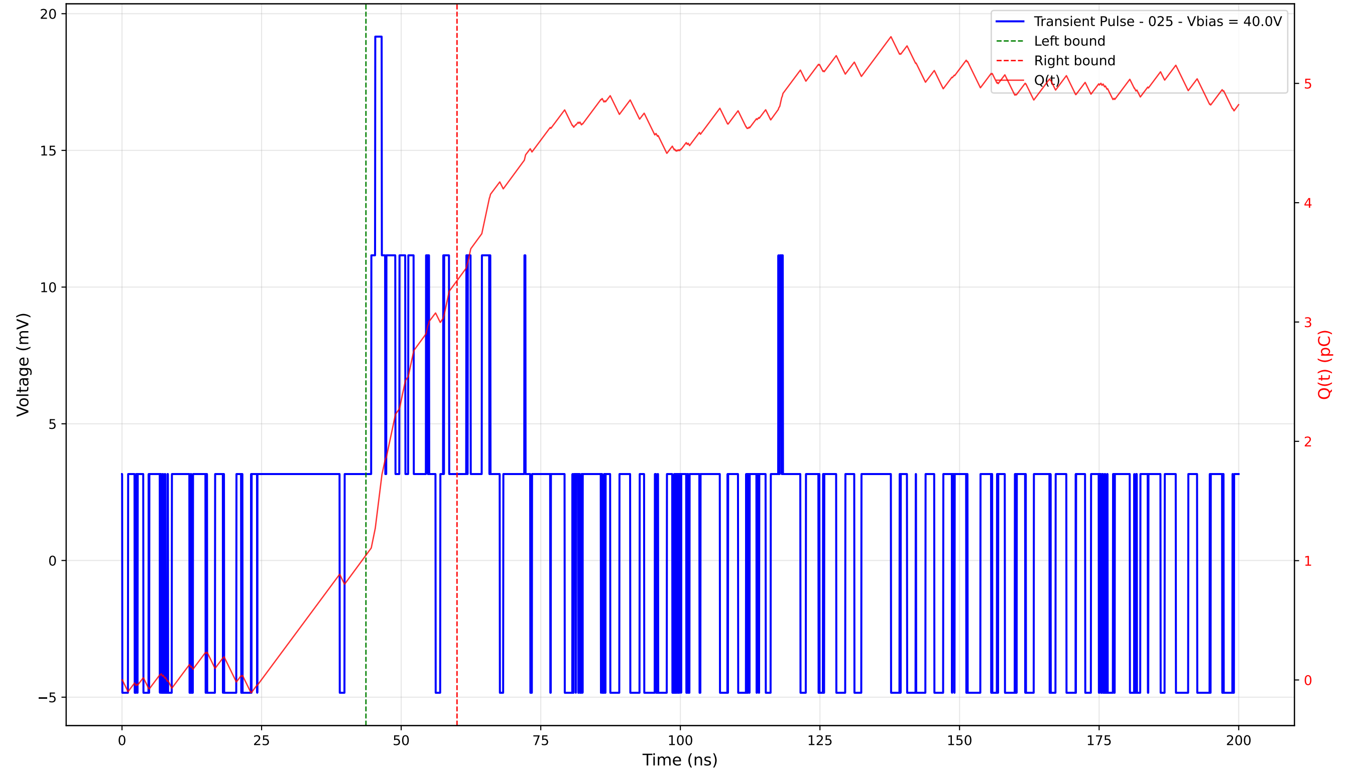
Transient Pulse - Sample: 4003 - Position: 415.0 \mu\text{m} - Charge: 2.30 pC - Rise Time: 0.00 ns (N/A)
