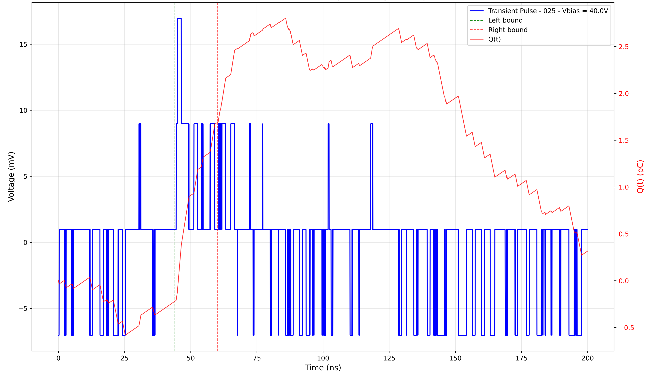
Transient Pulse - Sample: 4003 - Position: 380.0 \mu\text{m} - Charge: 1.91 pC - Rise Time: 0.44 ns
