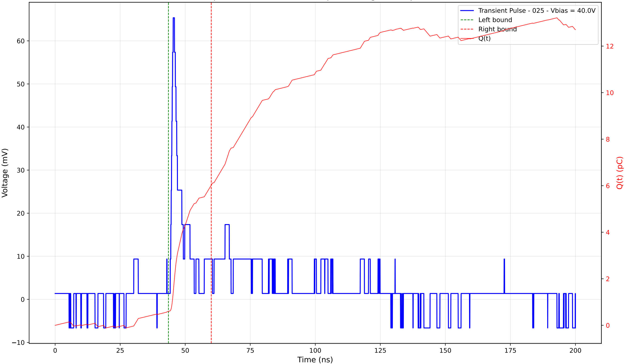
Transient Pulse - Sample: 4003 - Position: 95.0 \mu\text{m} - Charge: 5.42 pC - Rise Time: 1.13 ns
