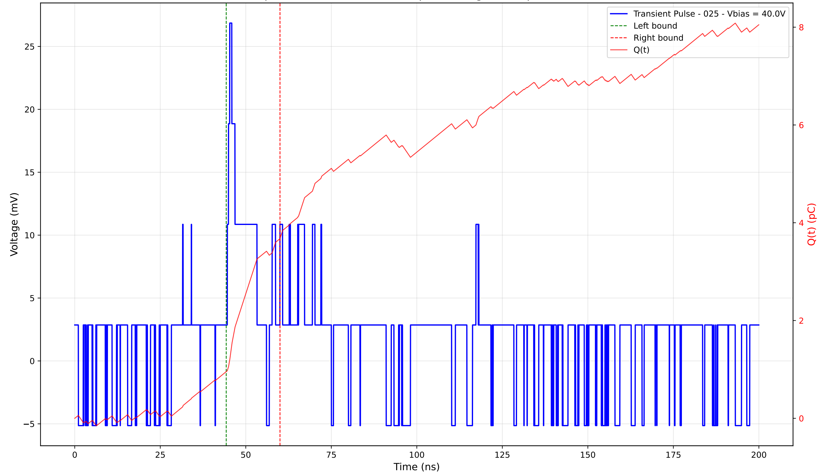
Transient Pulse - Sample: 4003 - Position: 260.0 \mu\text{m} - Charge: 2.72 pC - Rise Time: 0.00 ns (N/A)
