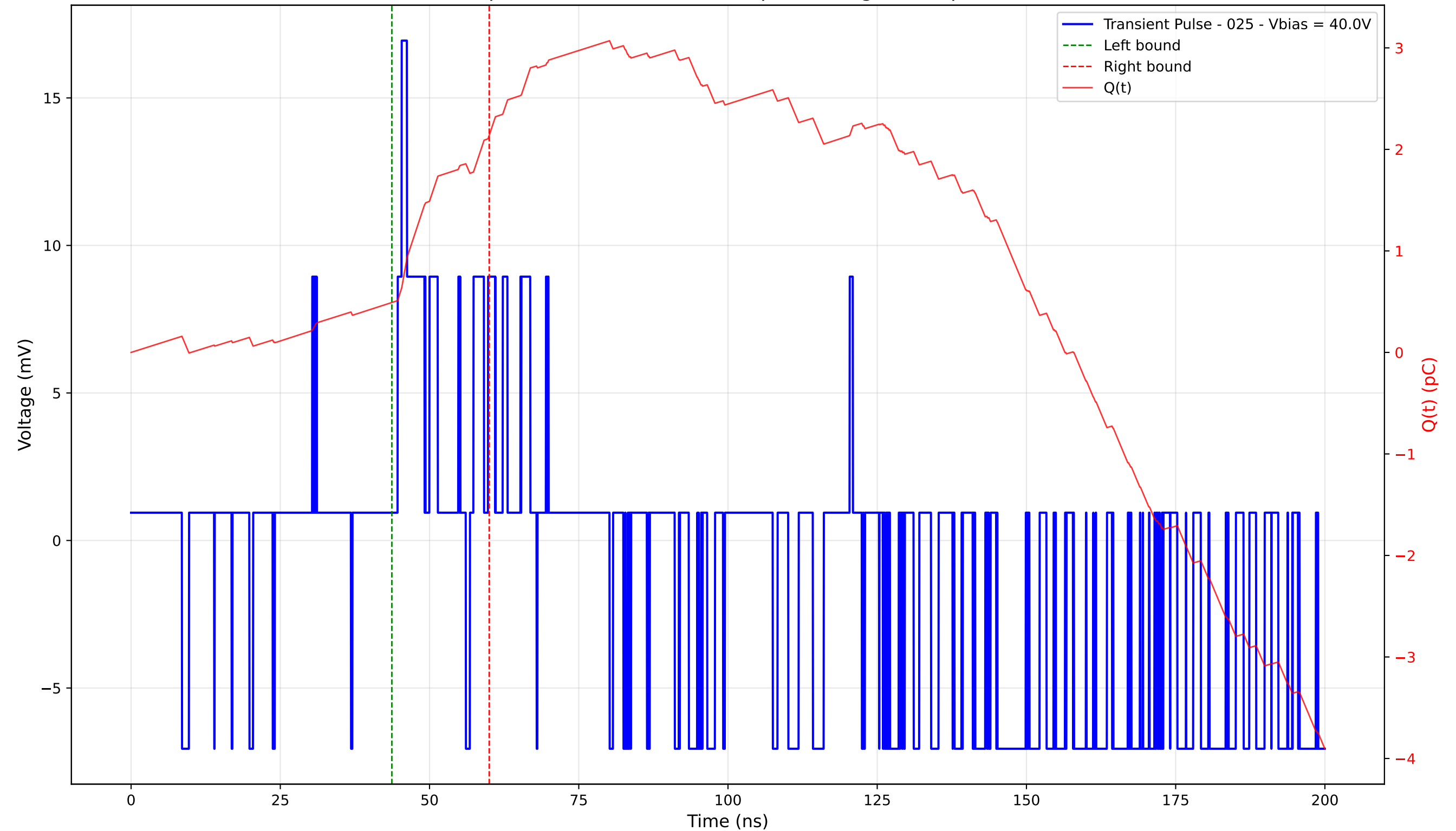
Transient Pulse - Sample: 4003 - Position: 420.0 \mu\text{m} - Charge: 1.65 pC - Rise Time: 0.68 ns
