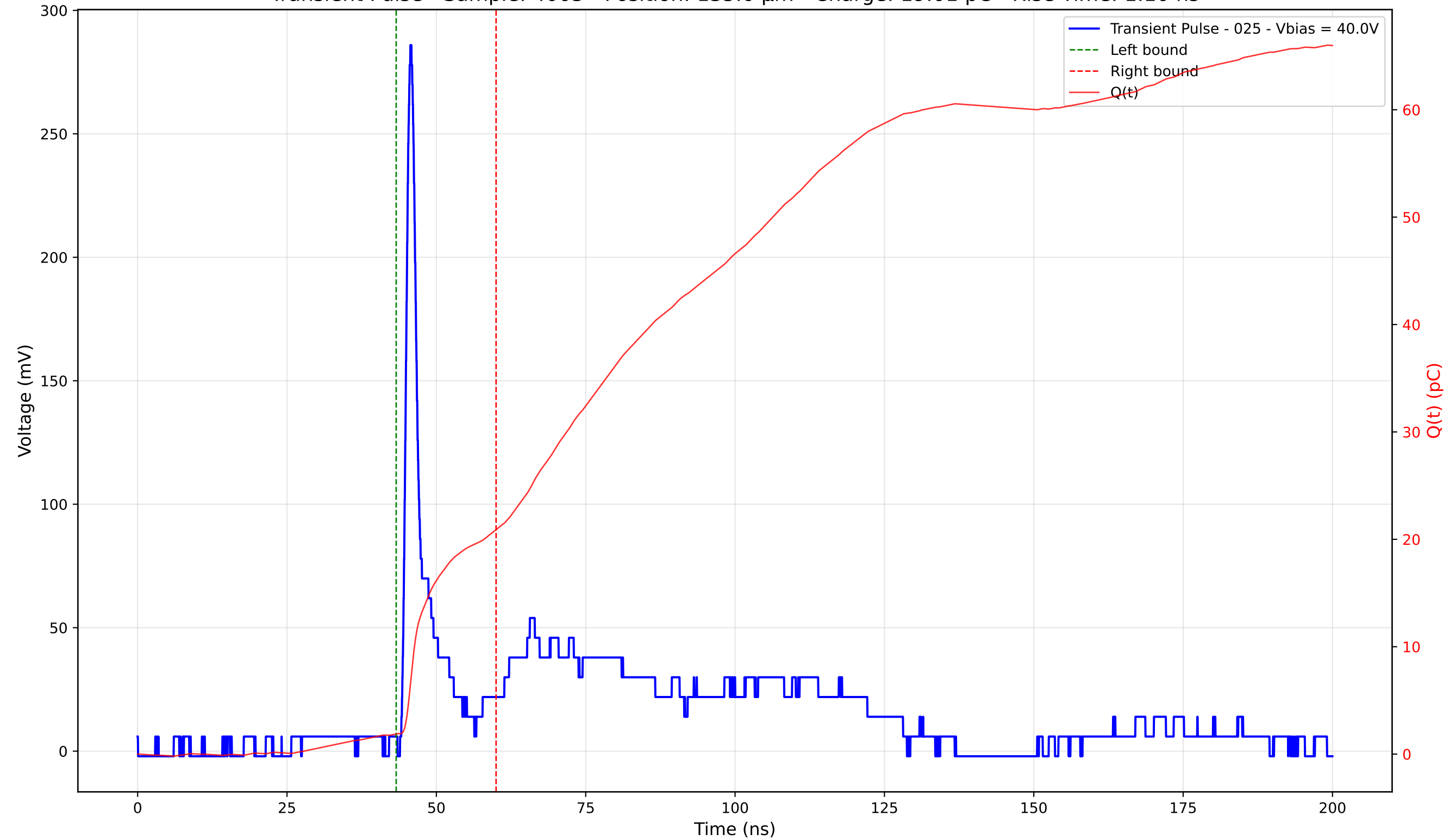
Transient Pulse - Sample: 4003 - Position: 135.0 \mu\text{m} - Charge: 19.01 pC - Rise Time: 1.10 ns
