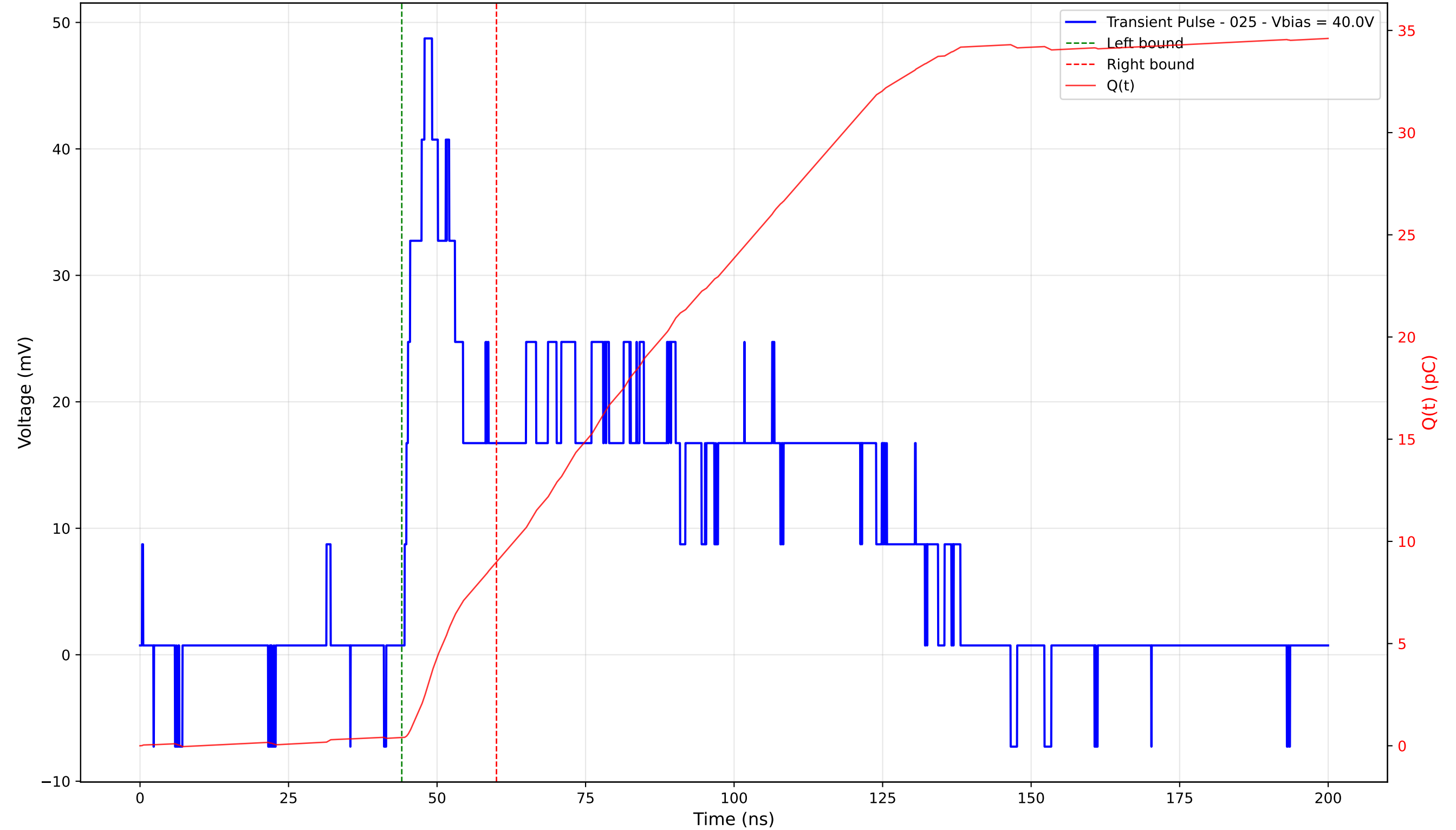
Transient Pulse - Sample: 4003 - Position: 195.0 \mu\text{m} - Charge: 8.59 pC - Rise Time: 3.35 ns
