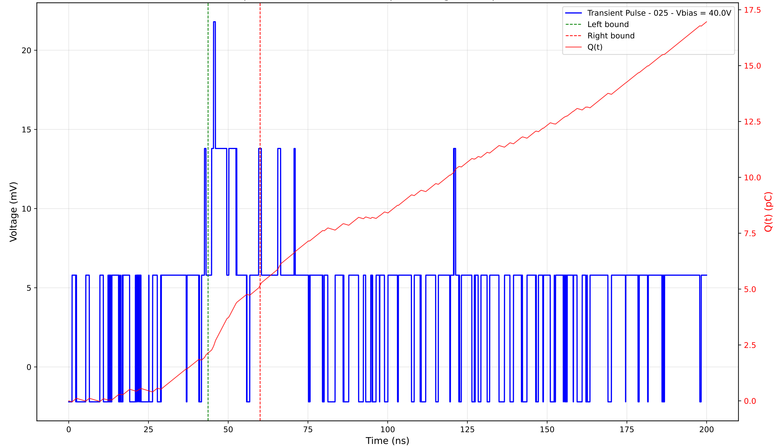
Transient Pulse - Sample: 4003 - Position: 335.0 \mu\text{m} - Charge: 3.03 pC - Rise Time: 0.00 ns (N/A)
