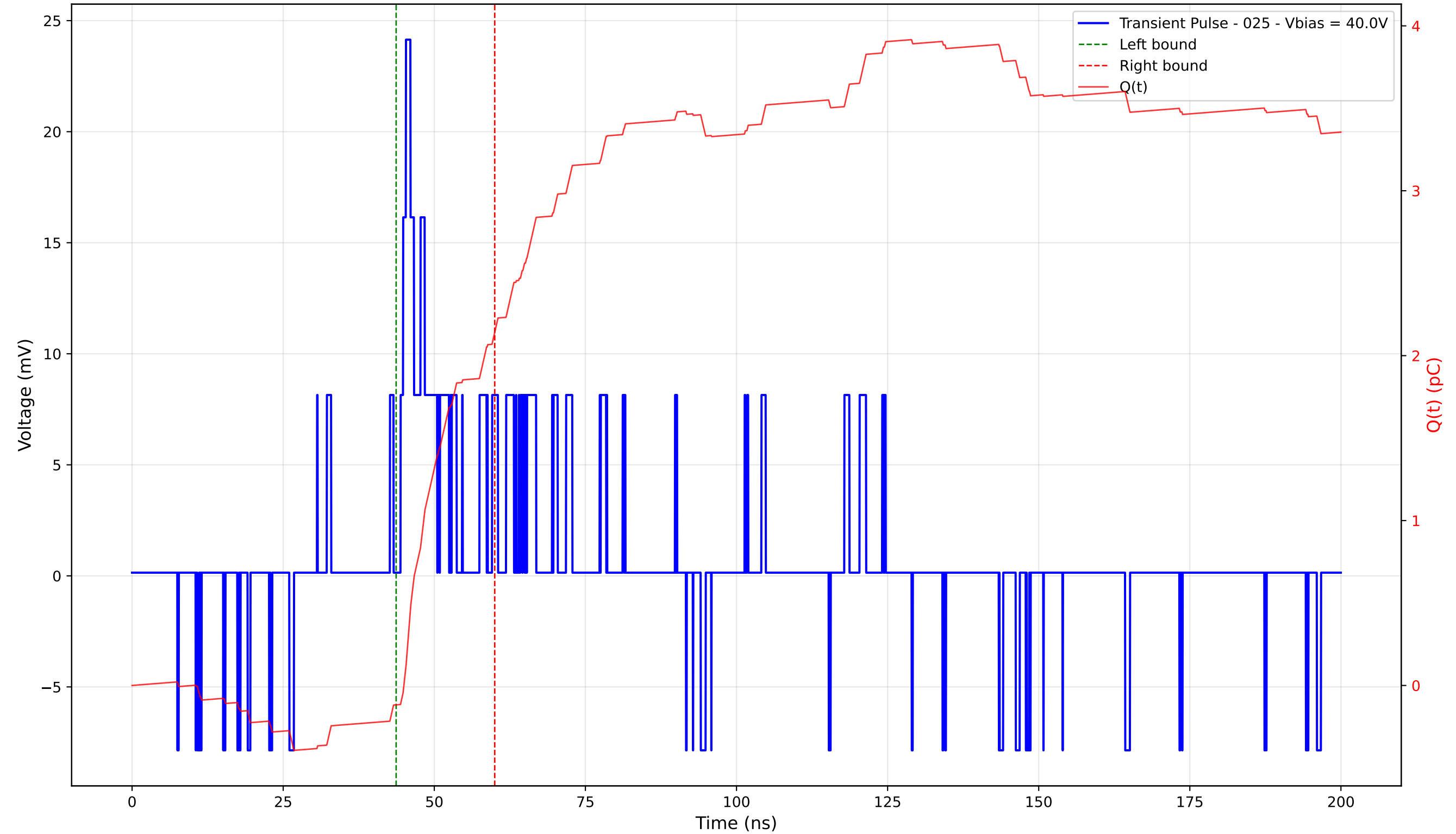
Transient Pulse - Sample: 4003 - Position: 290.0 \mu\text{m} - Charge: 2.26 pC - Rise Time: 0.89 ns
