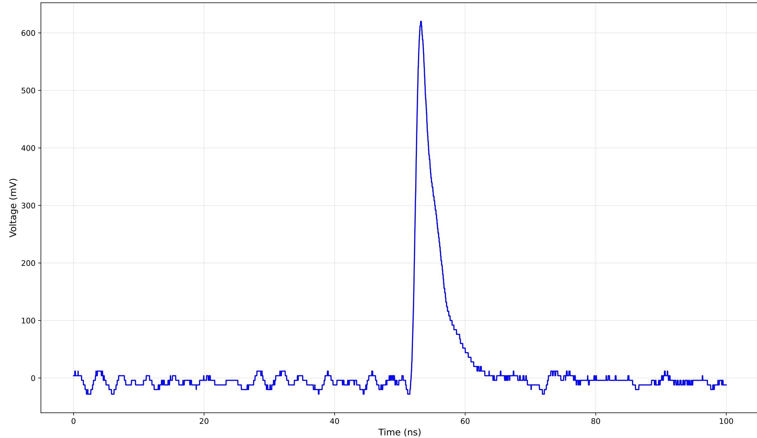
TCT Pulse Waveform - Run 1: 4004 (300.0 V) - Rise Time: 0.95 ns
