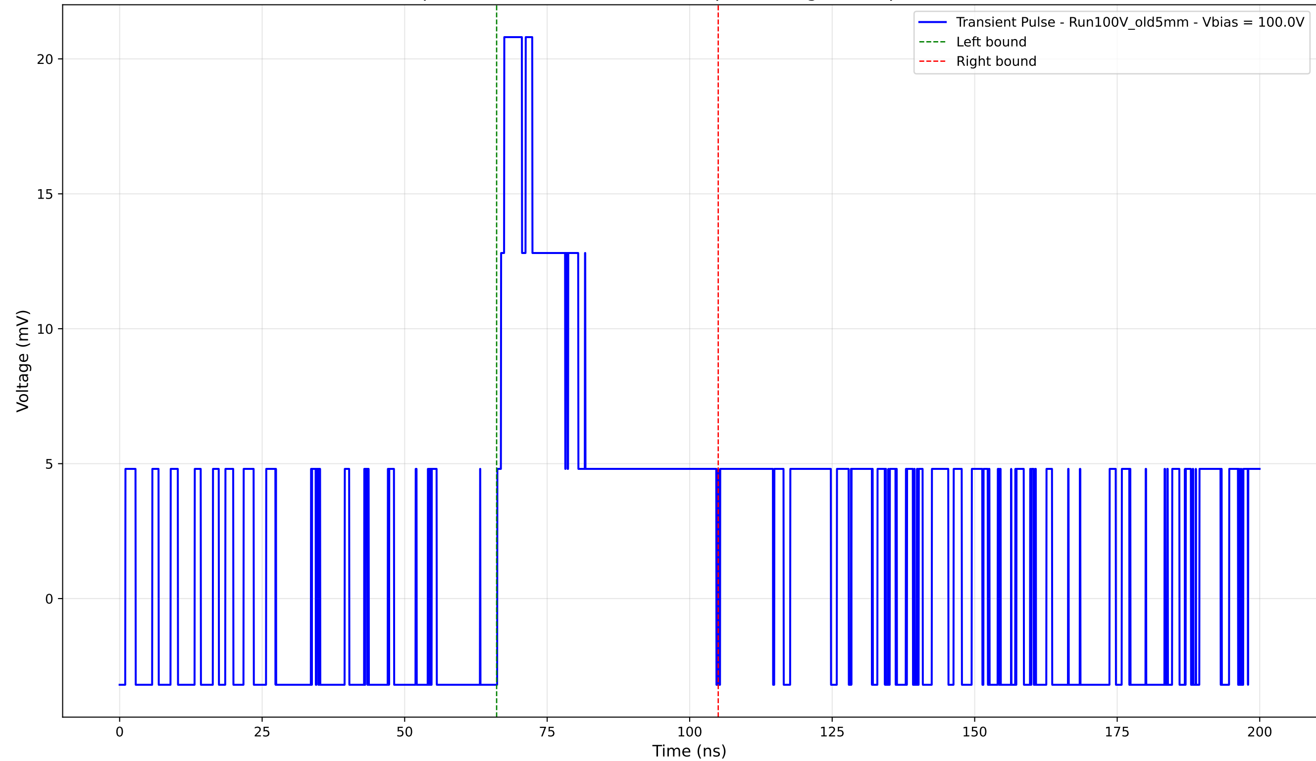
Transient Pulse - Sample: Old5mm - Position: 4555.0 \mu\text{m} - Charge: 6.52 pC - Rise Time: 0.00 ns (N/A)
