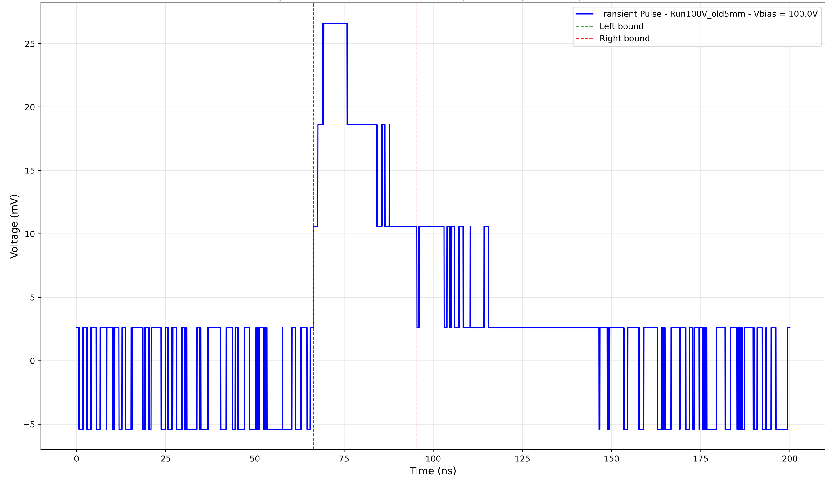
Transient Pulse - Sample: Old5mm - Position: 4985.0 \mu\text{m} - Charge: 10.01 pC - Rise Time: 2.60 ns
