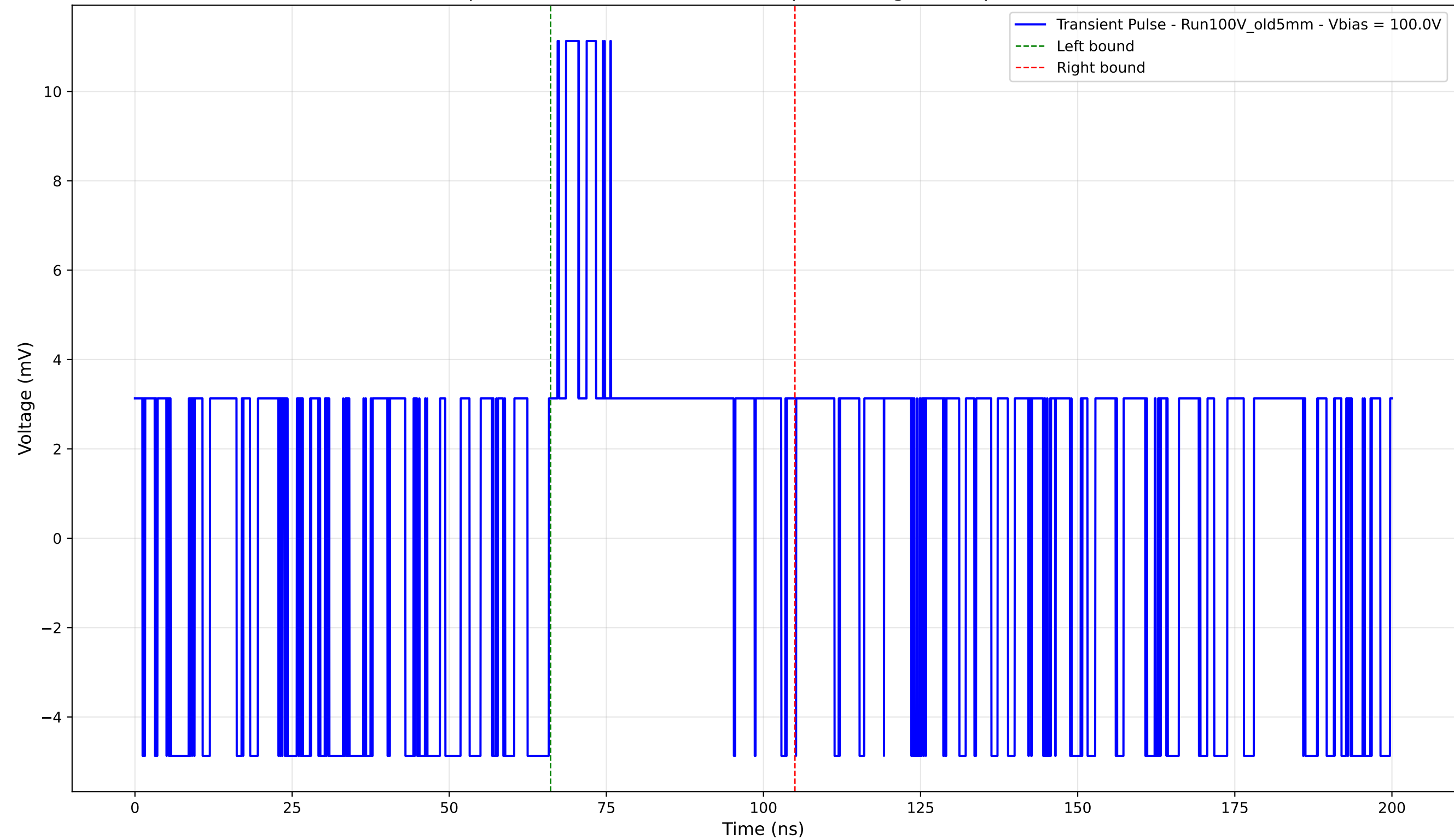
Transient Pulse - Sample: Old5mm - Position: 2750.0 \mu\text{m} - Charge: 2.87 pC - Rise Time: 0.00 ns (N/A)
