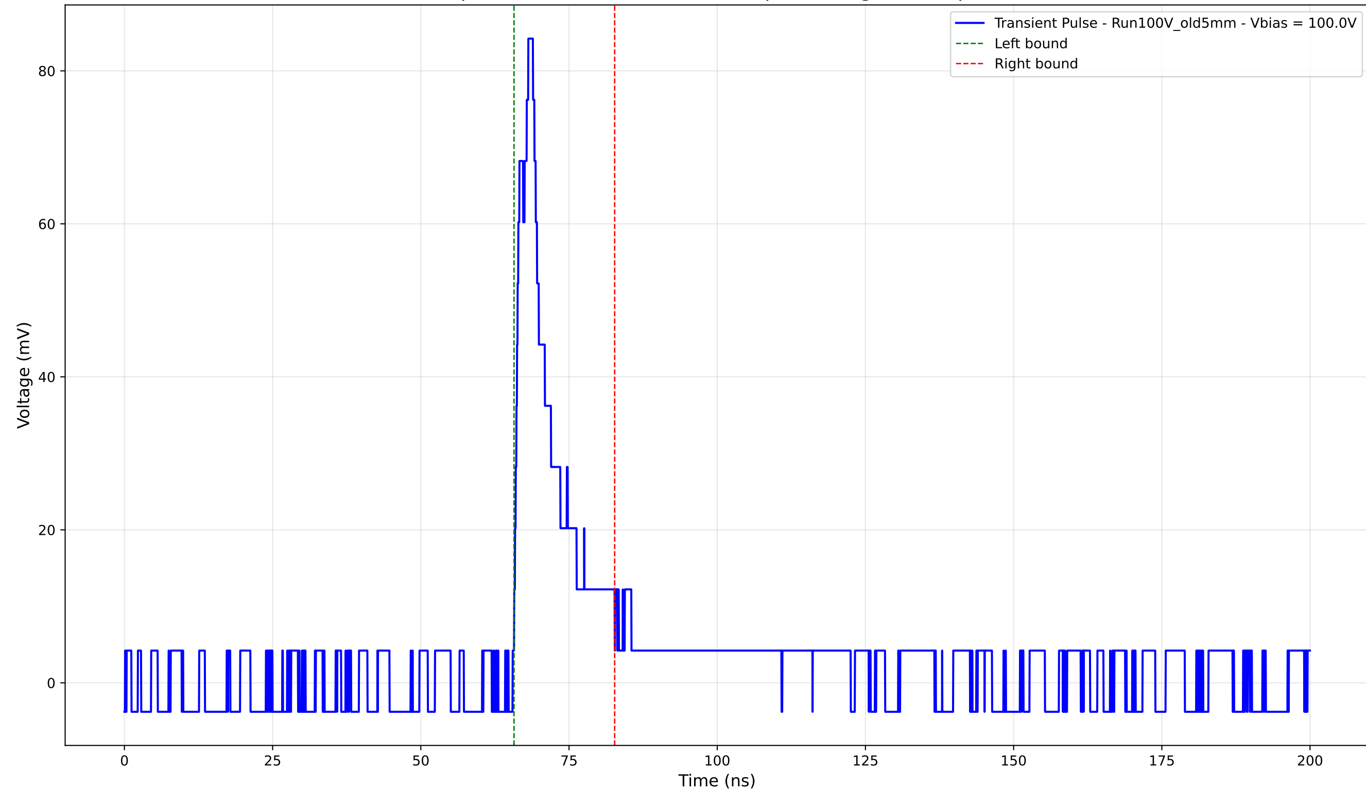
Transient Pulse - Sample: Old5mm - Position: 4090.0 \mu\text{m} - Charge: 10.55 pC - Rise Time: 2.13 ns
