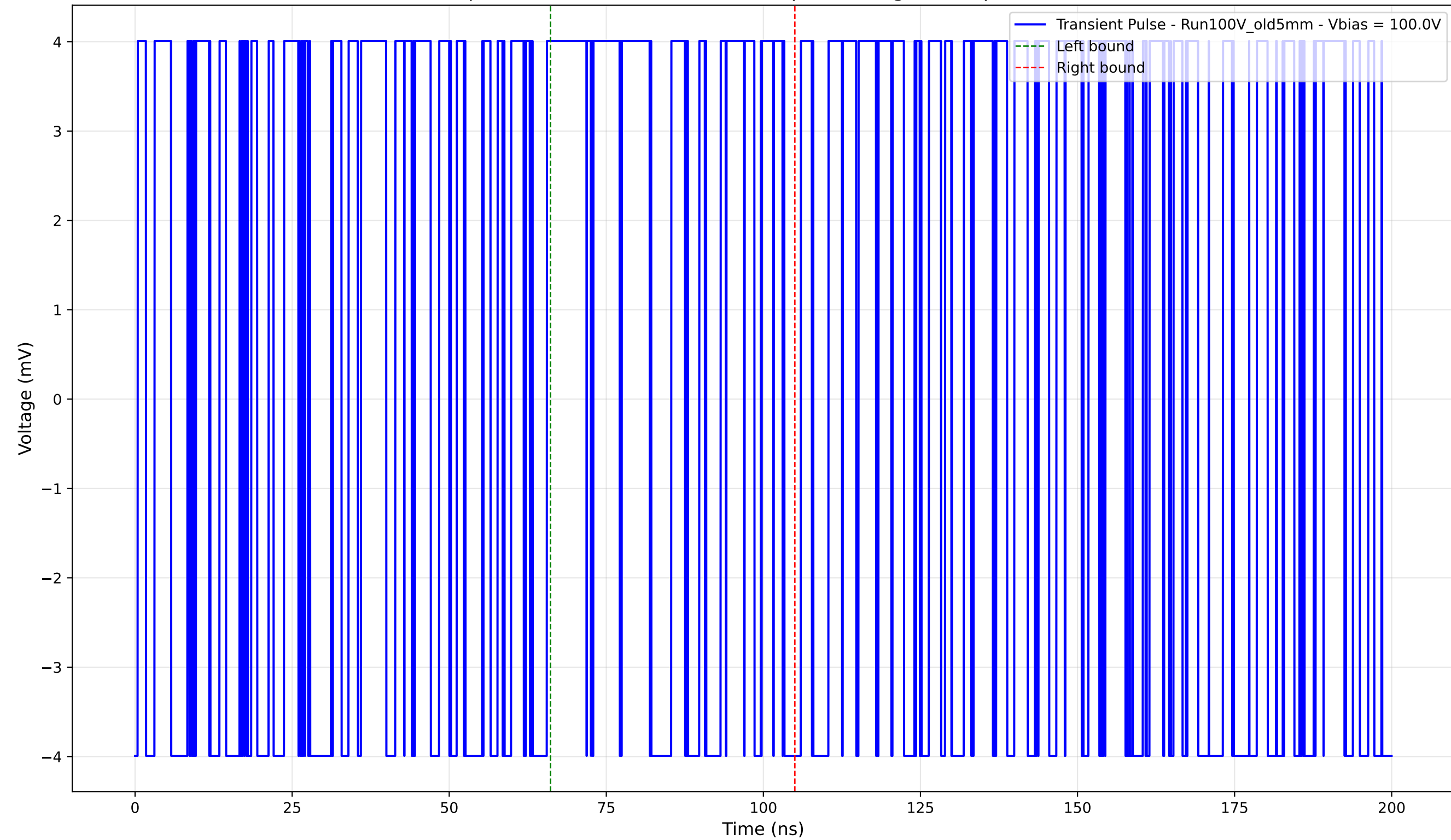
Transient Pulse - Sample: Old5mm - Position: 3080.0 \mu\text{m} - Charge: 1.32 pC - Rise Time: 0.00 ns (N/A)
