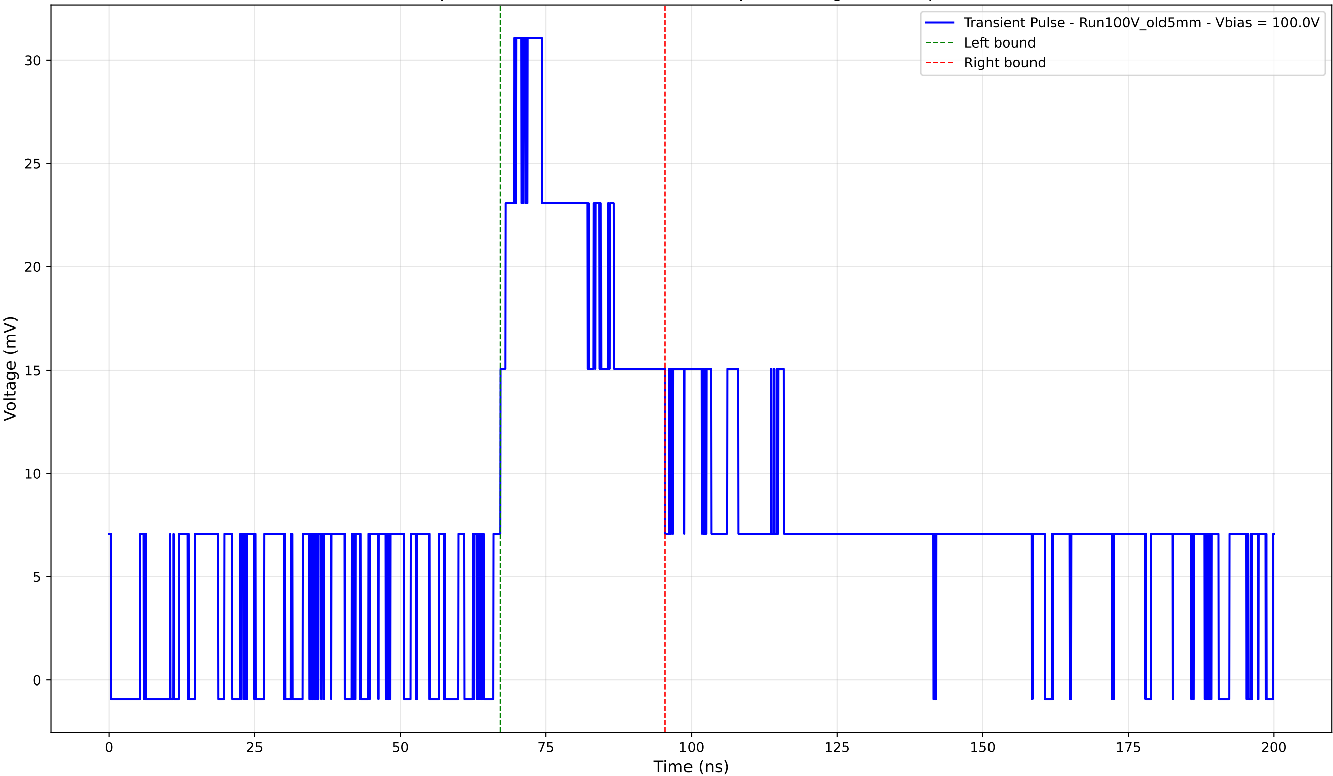
Transient Pulse - Sample: Old5mm - Position: 2445.0 \mu\text{m} - Charge: 11.76 pC - Rise Time: 3.63 ns
