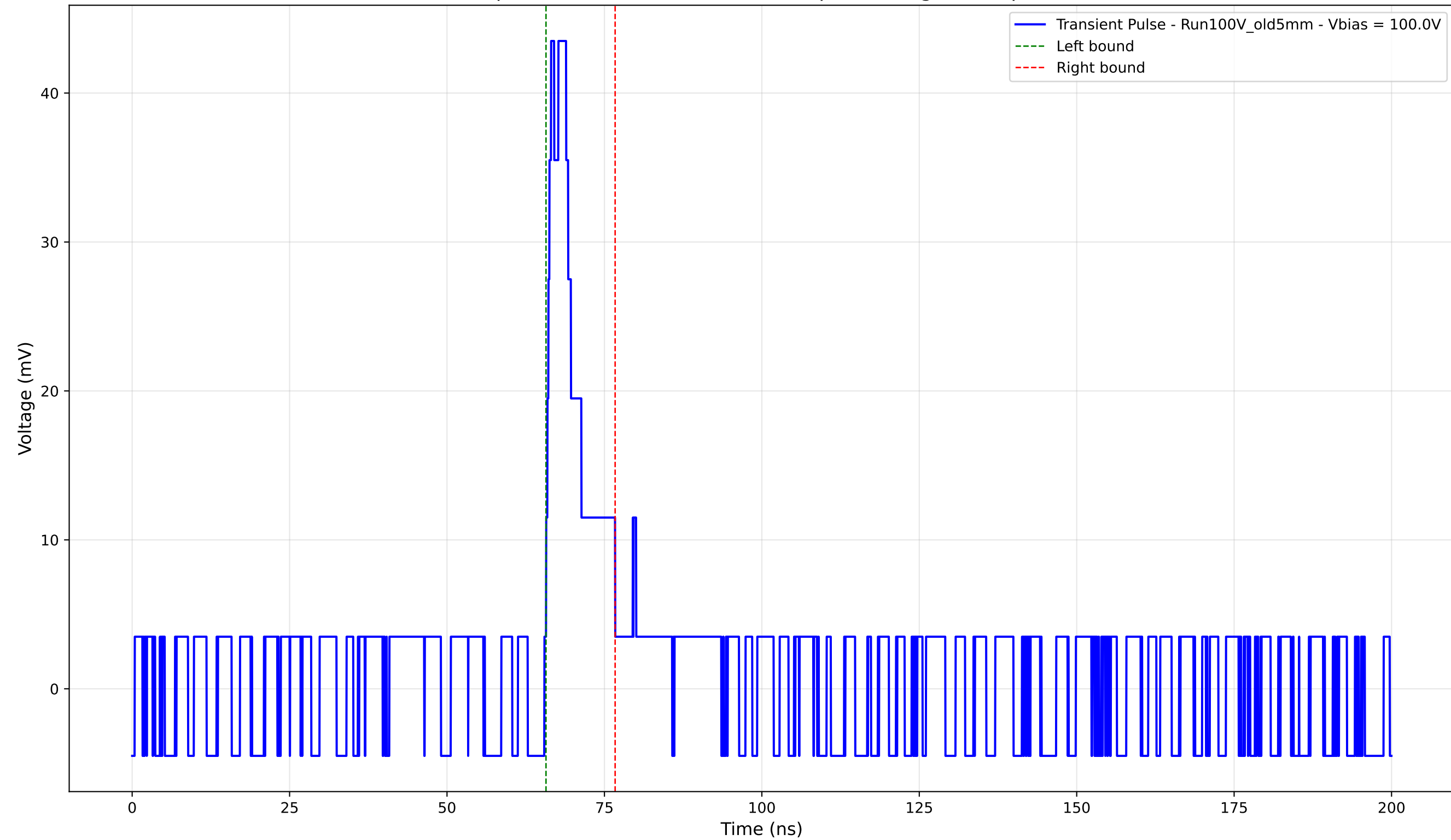
Transient Pulse - Sample: Old5mm - Position: 3960.0 \mu\text{m} - Charge: 4.71 pC - Rise Time: 0.80 ns
