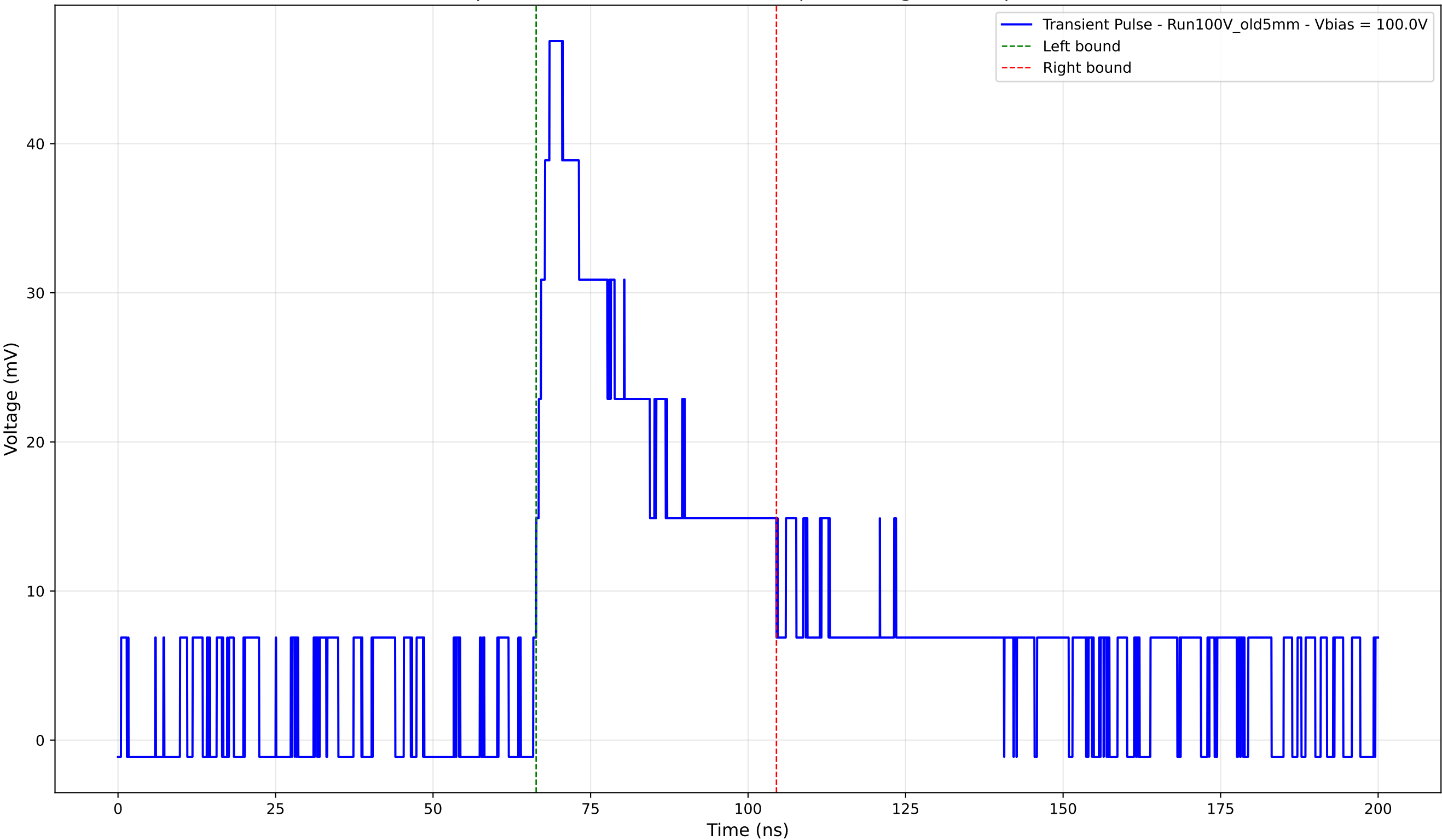
Transient Pulse - Sample: Old5mm - Position: 4730.0 \mu\text{m} - Charge: 17.49 pC - Rise Time: 2.59 ns
