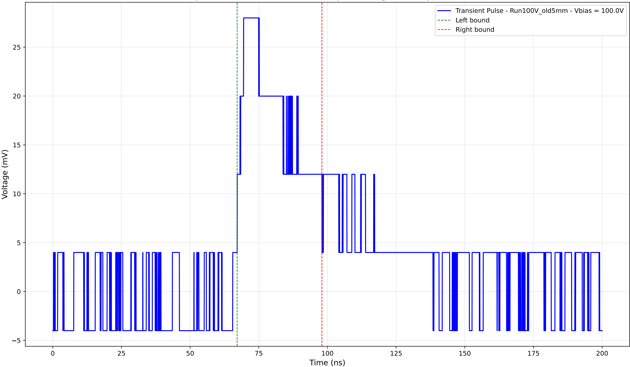
Transient Pulse - Sample: Old5mm - Position: 2410.0 \mu\text{m} - Charge: 10.99 pC - Rise Time: 0.00 ns (N/A)
