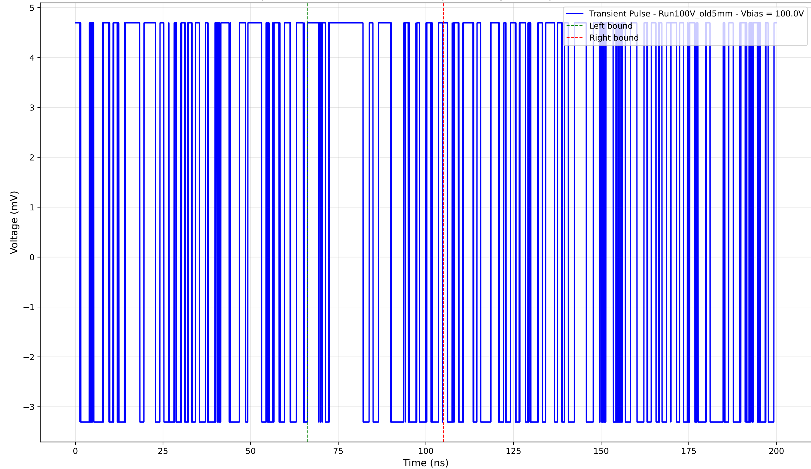
Transient Pulse - Sample: Old5mm - Position: 4620.0 \mu\text{m} - Charge: 1.32 pC - Rise Time: 0.00 ns (N/A)
