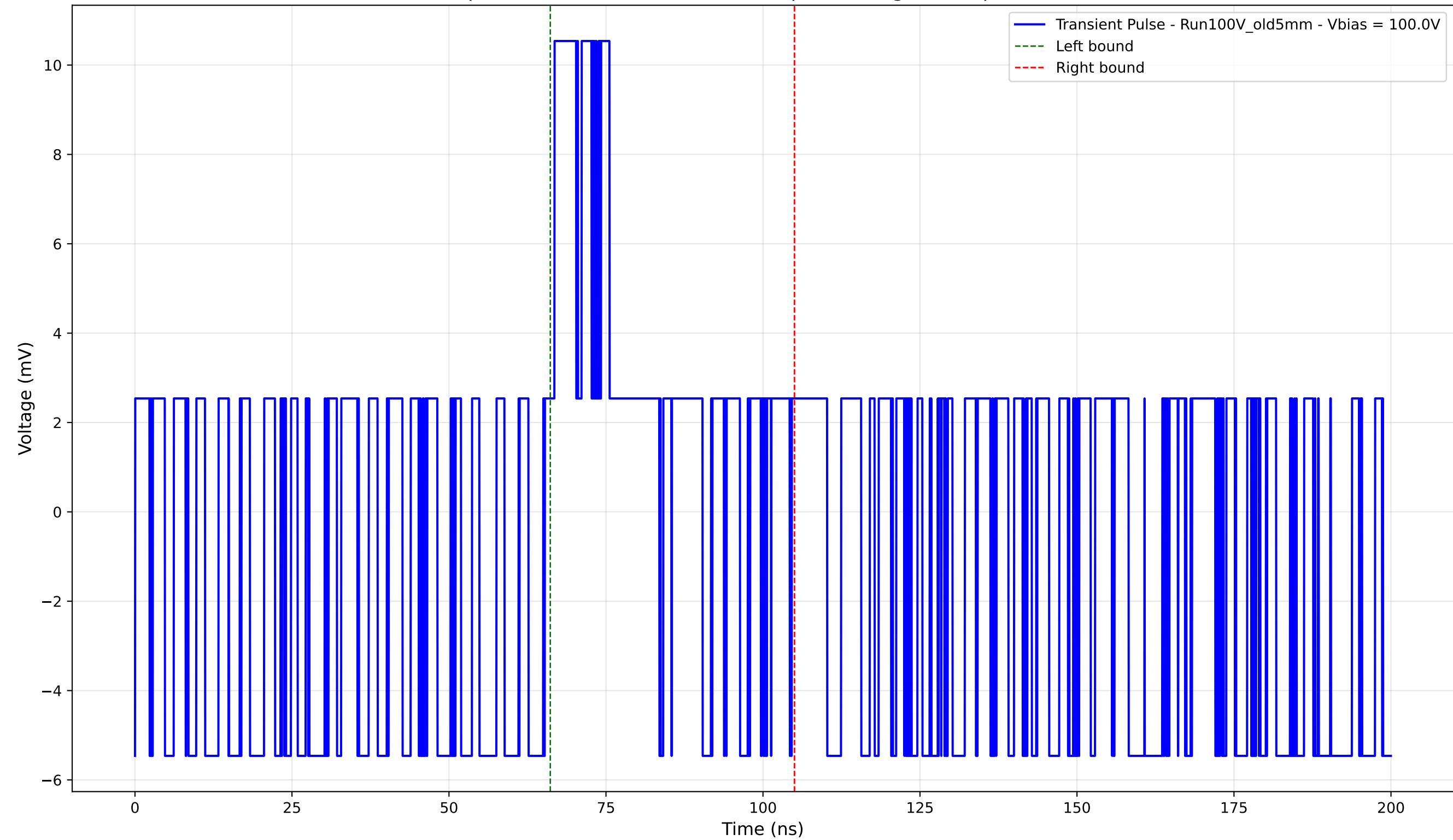
Transient Pulse - Sample: Old5mm - Position: 4355.0 \mu\text{m} - Charge: 2.46 pC - Rise Time: 0.00 ns (N/A)
