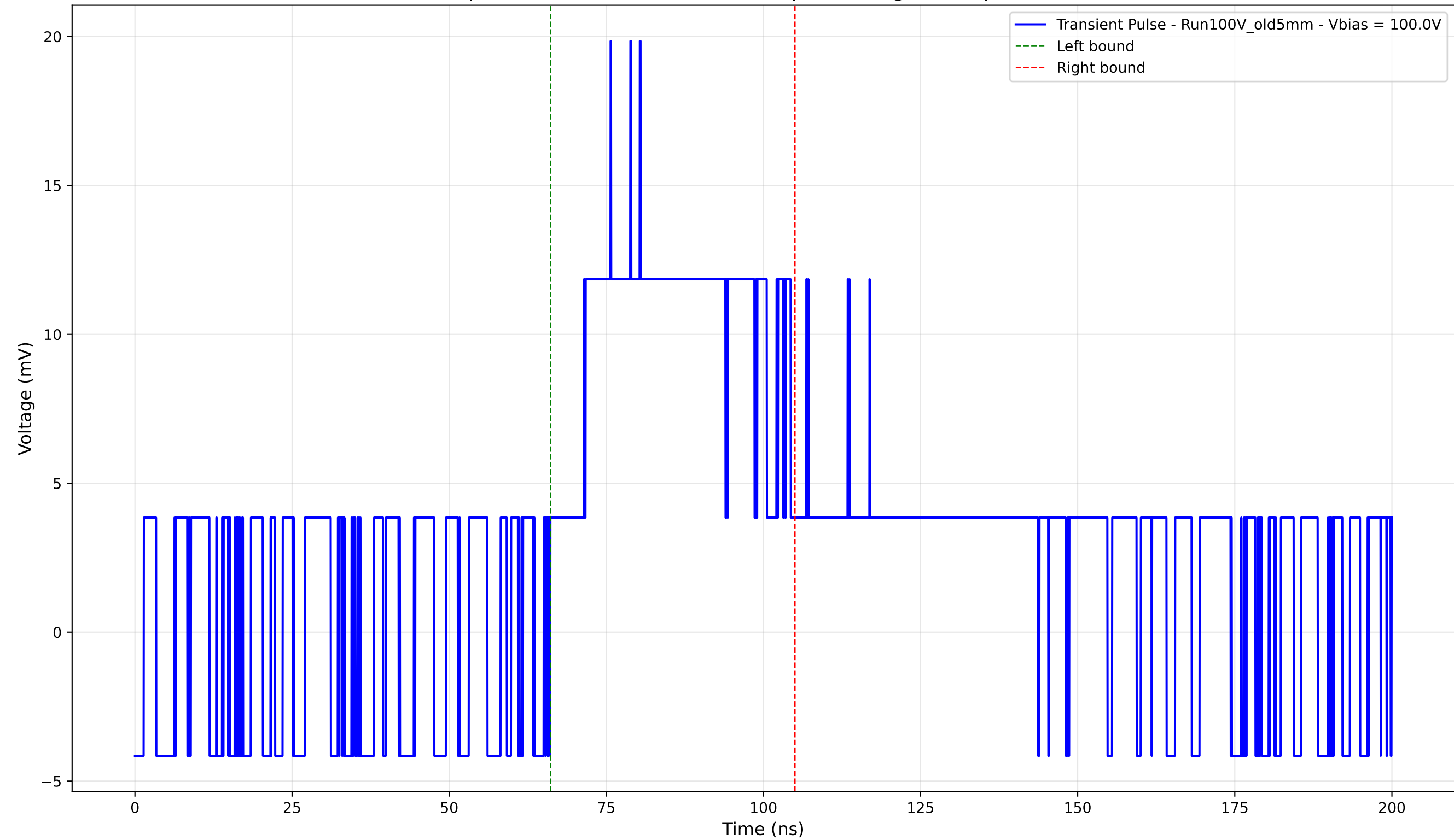
Transient Pulse - Sample: Old5mm - Position: 1185.0 \mu\text{m} - Charge: 7.91 pC - Rise Time: 0.00 ns (N/A)
