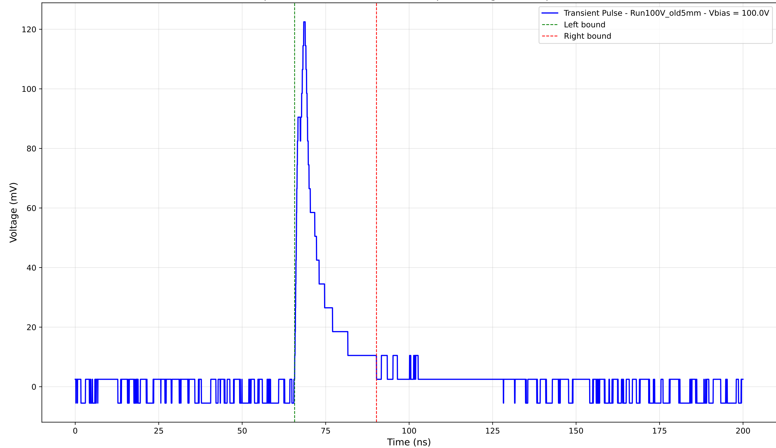
Transient Pulse - Sample: Old5mm - Position: 3270.0 \mu\text{m} - Charge: 16.66 pC - Rise Time: 2.38 ns
