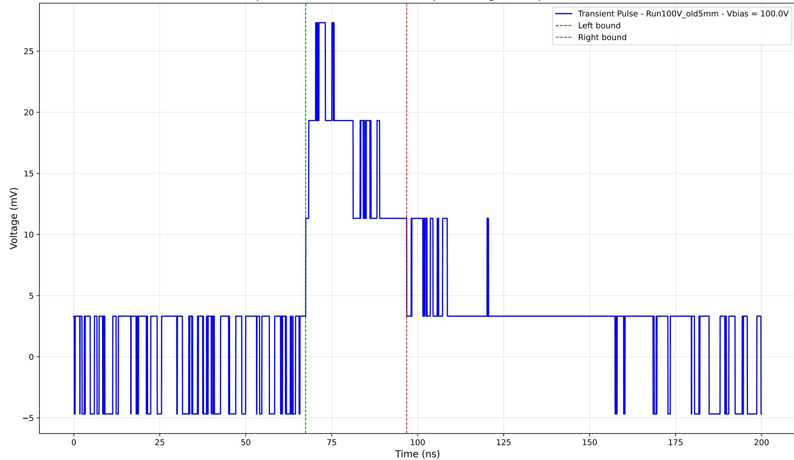
Transient Pulse - Sample: Old5mm - Position: 2450.0 \mu\text{m} - Charge: 9.68 pC - Rise Time: 0.00 ns (N/A)
