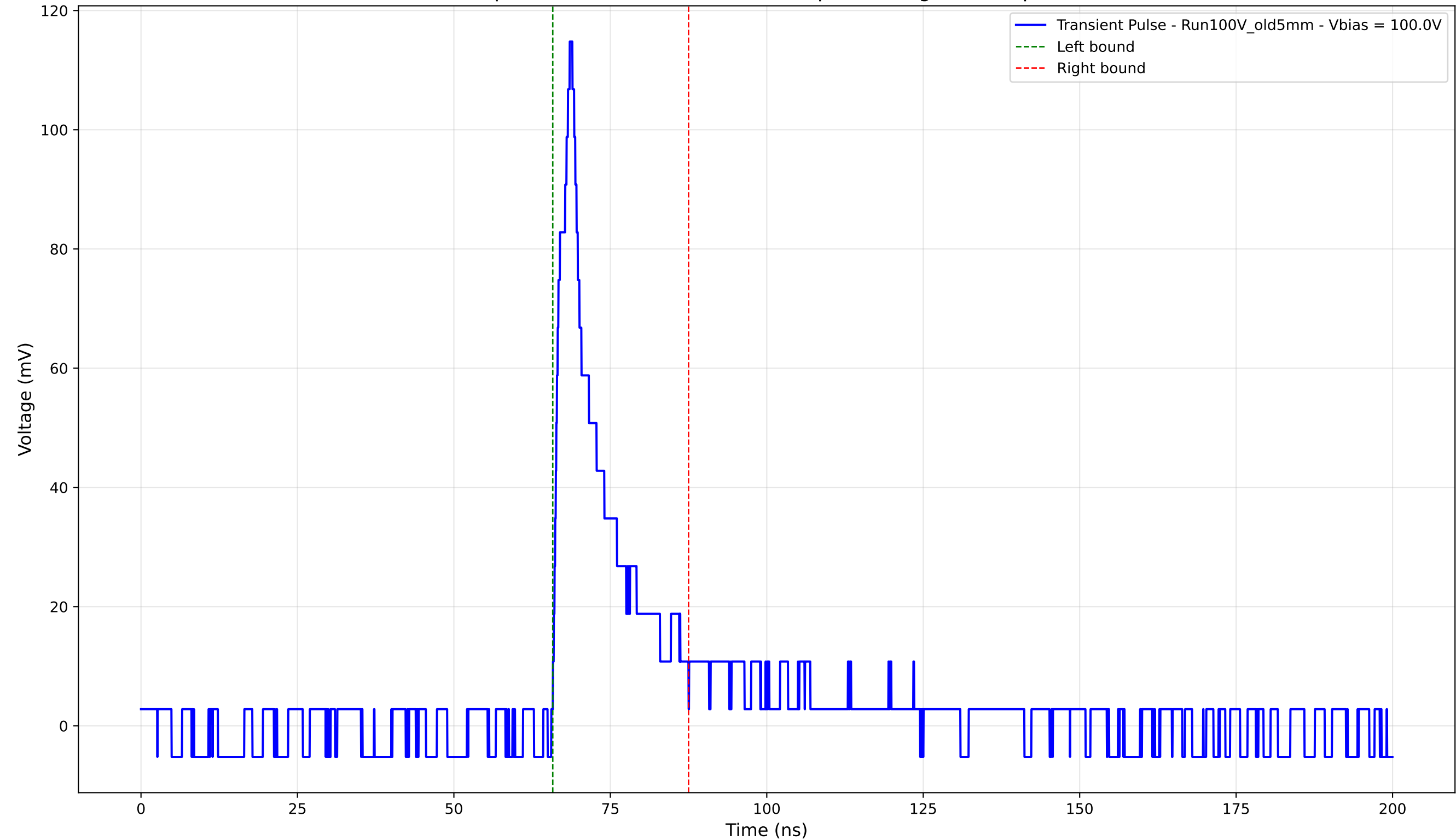
Transient Pulse - Sample: Old5mm - Position: 3225.0 \mu\text{m} - Charge: 16.67 pC - Rise Time: 2.28 ns
