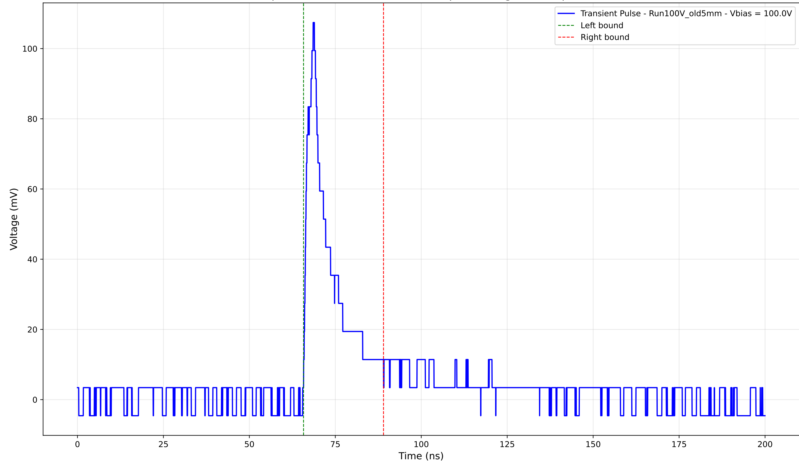
Transient Pulse - Sample: Old5mm - Position: 3215.0 \mu\text{m} - Charge: 16.27 pC - Rise Time: 2.42 ns
