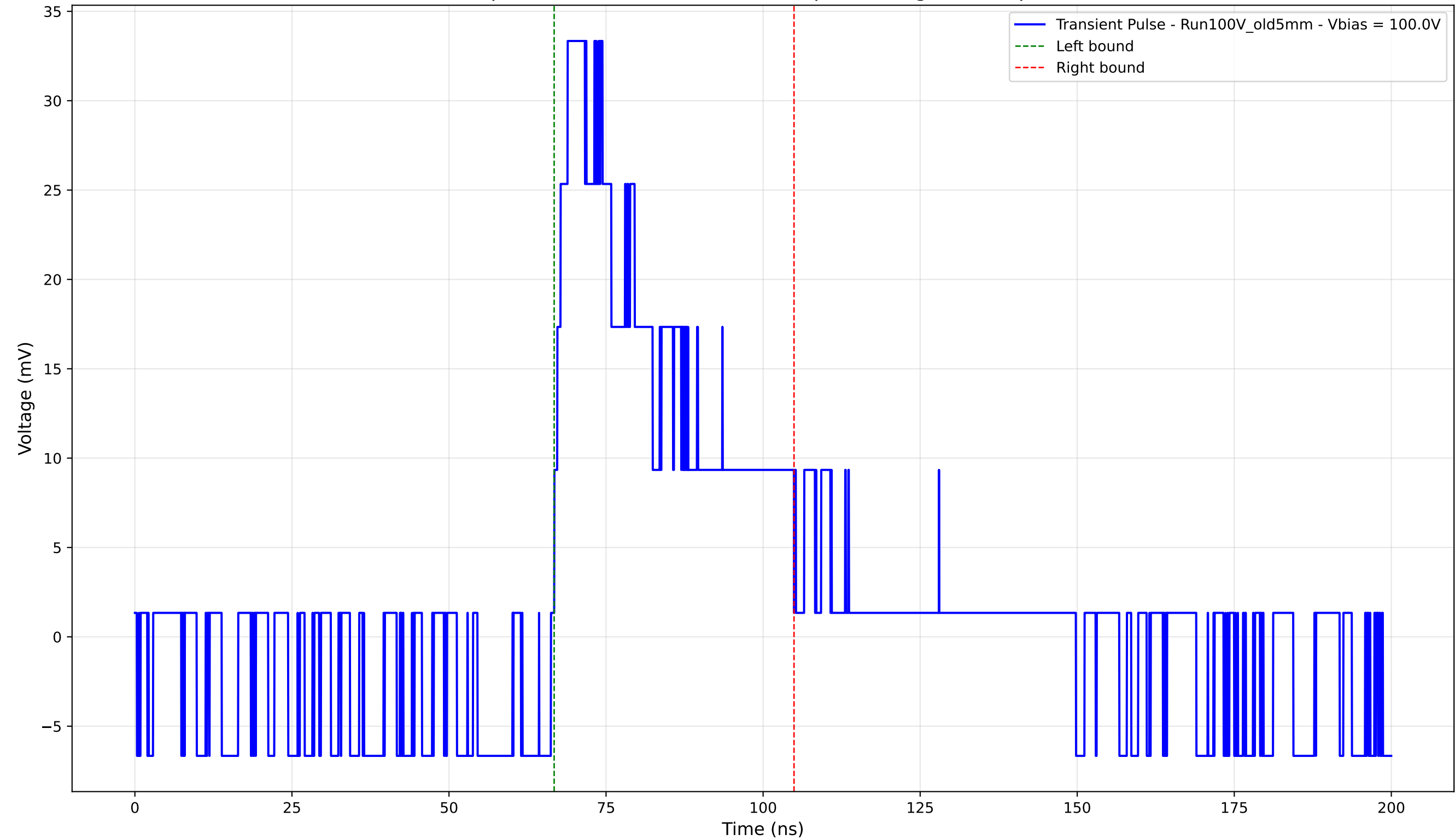
Transient Pulse - Sample: Old5mm - Position: 2620.0 \mu\text{m} - Charge: 12.21 pC - Rise Time: 2.14 ns
