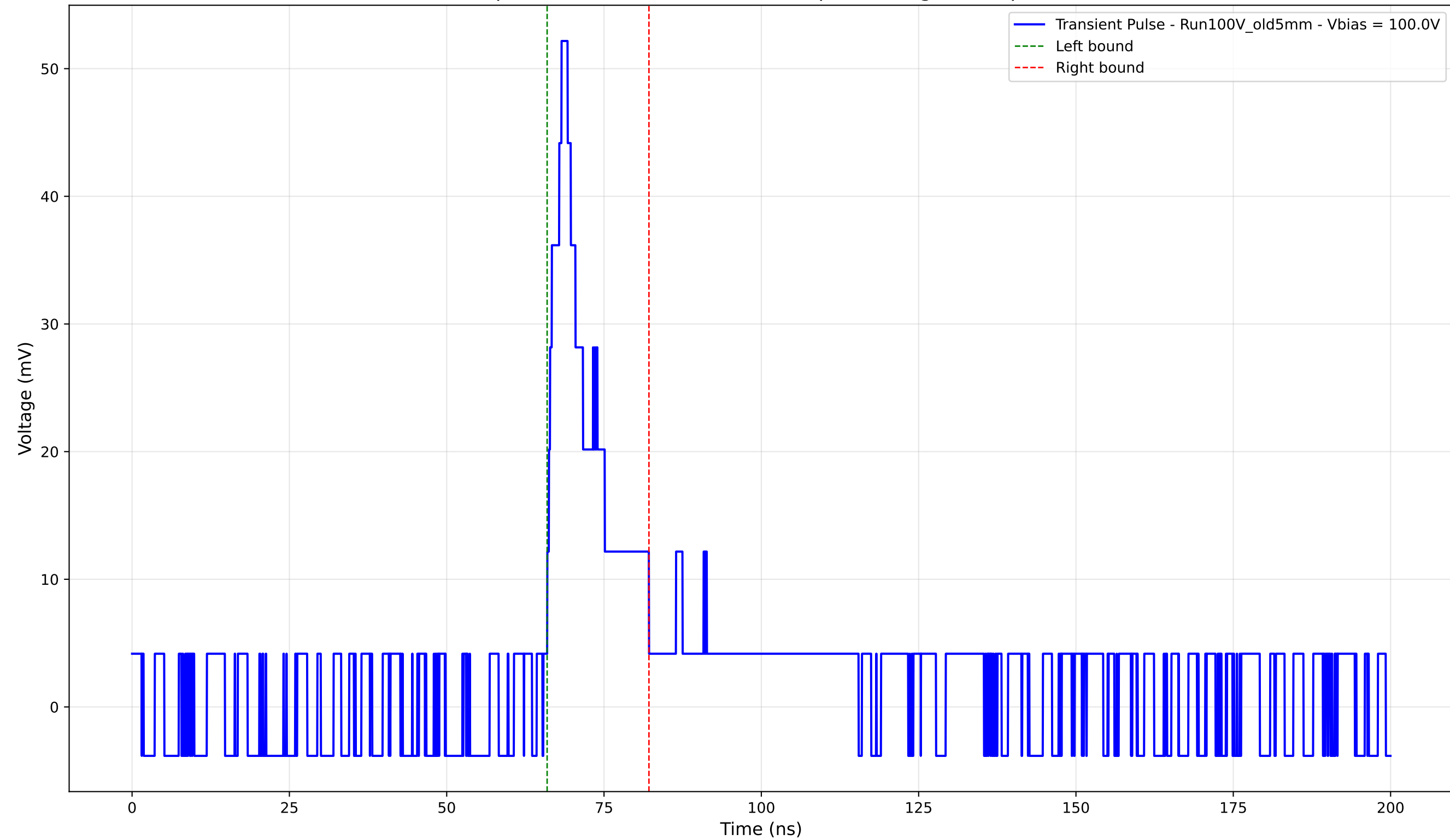
Transient Pulse - Sample: Old5mm - Position: 3170.0 \mu\text{m} - Charge: 7.29 pC - Rise Time: 2.28 ns
