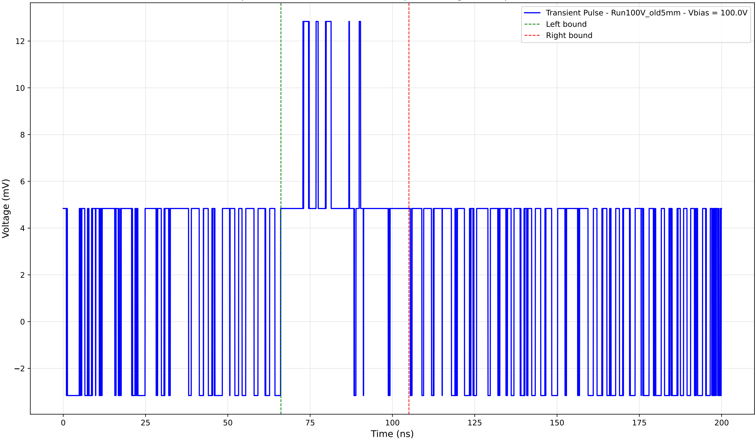
Transient Pulse - Sample: Old5mm - Position: 710.0 \mu\text{m} - Charge: 4.30 pC - Rise Time: 0.00 ns (N/A)
