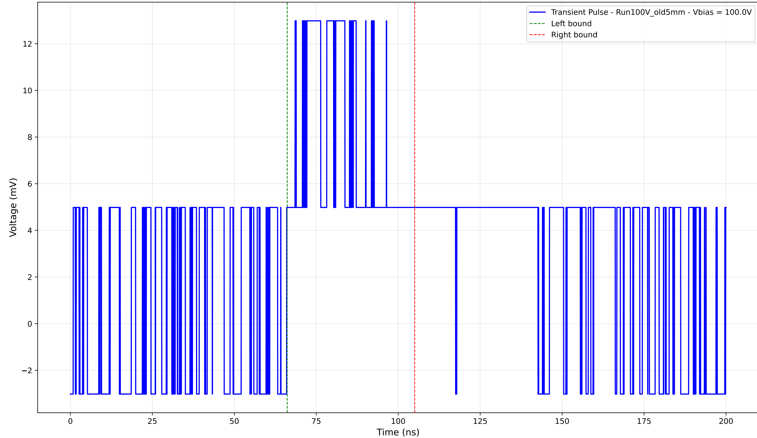
Transient Pulse - Sample: Old5mm - Position: 2075.0 \mu\text{m} - Charge: 5.88 pC - Rise Time: 0.00 ns (N/A)
