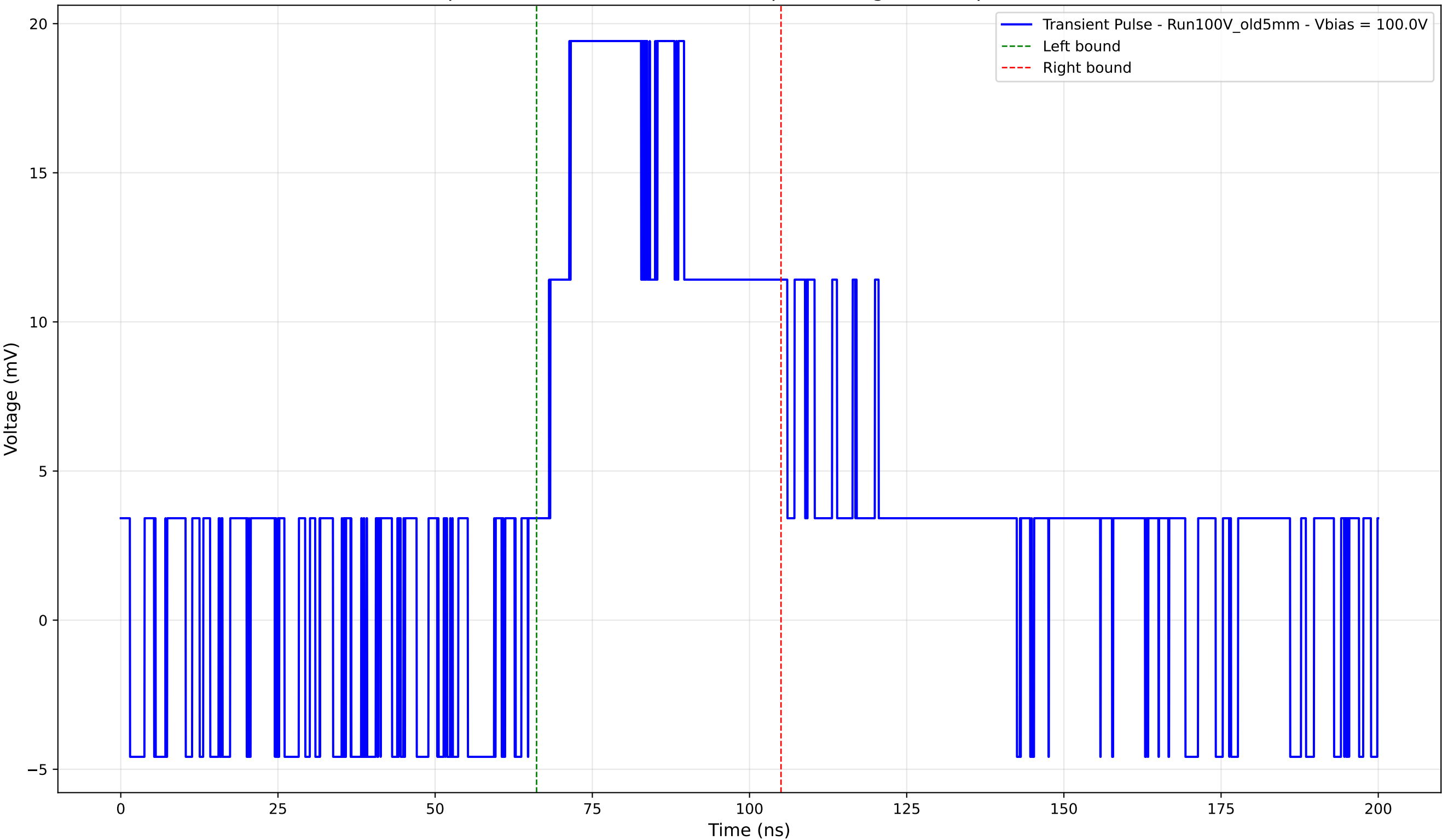
Transient Pulse - Sample: Old5mm - Position: 2015.0 \mu\text{m} - Charge: 11.02 pC - Rise Time: 0.00 ns (N/A)
