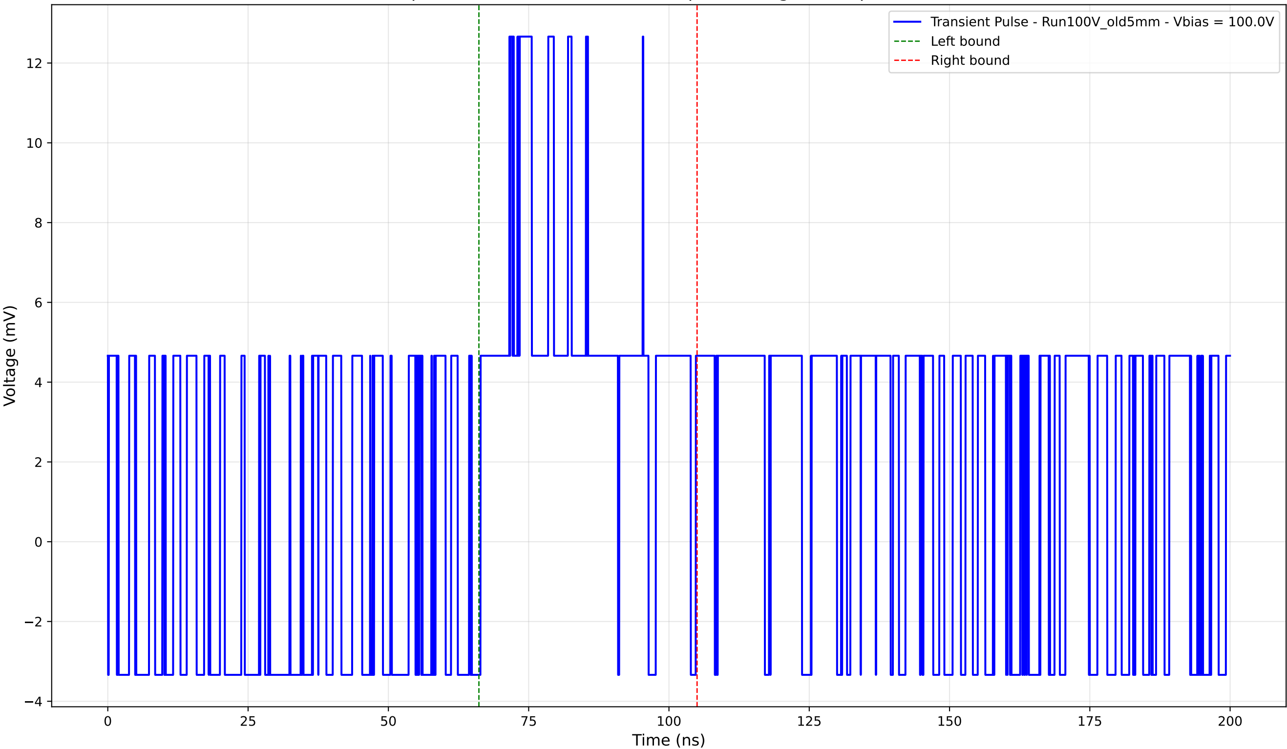
Transient Pulse - Sample: Old5mm - Position: 620.0 \mu\text{m} - Charge: 3.99 pC - Rise Time: 0.00 ns (N/A)
