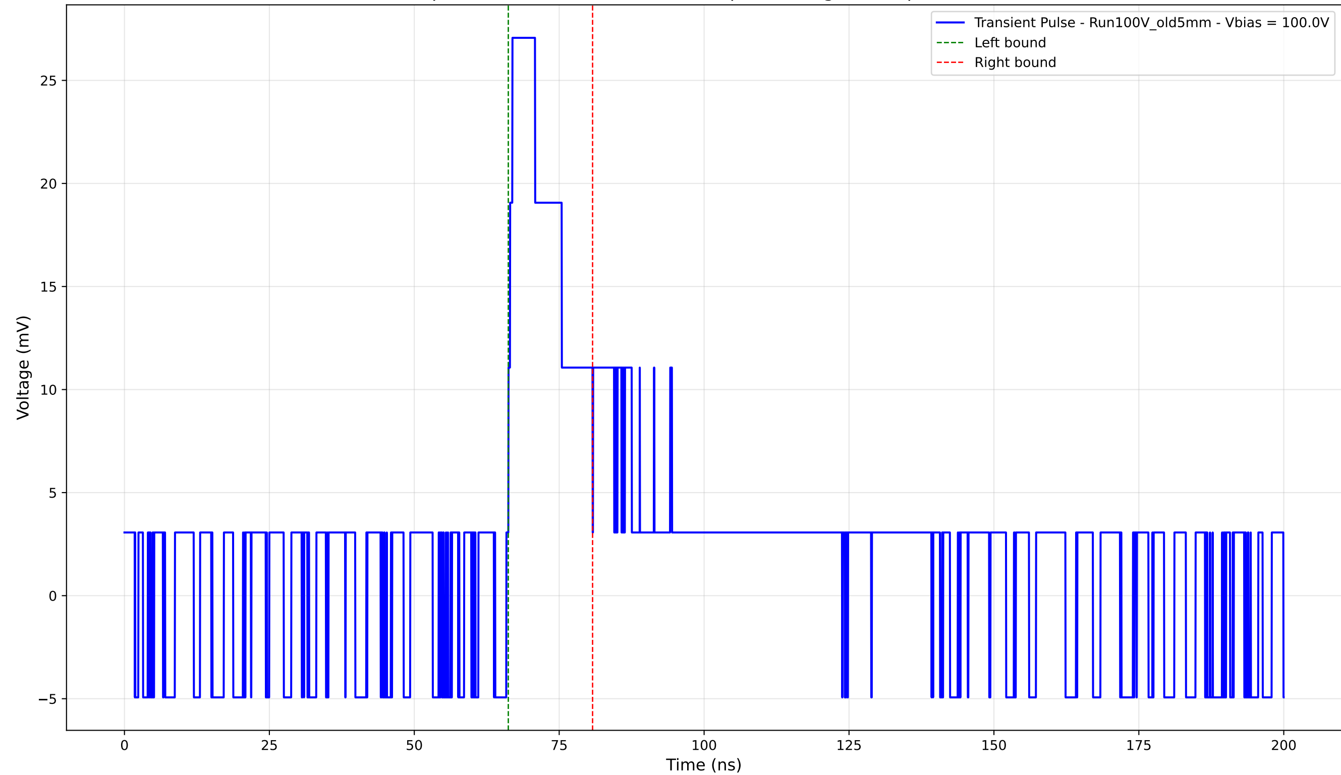
Transient Pulse - Sample: Old5mm - Position: 4375.0 \mu\text{m} - Charge: 5.27 pC - Rise Time: 0.00 ns (N/A)
