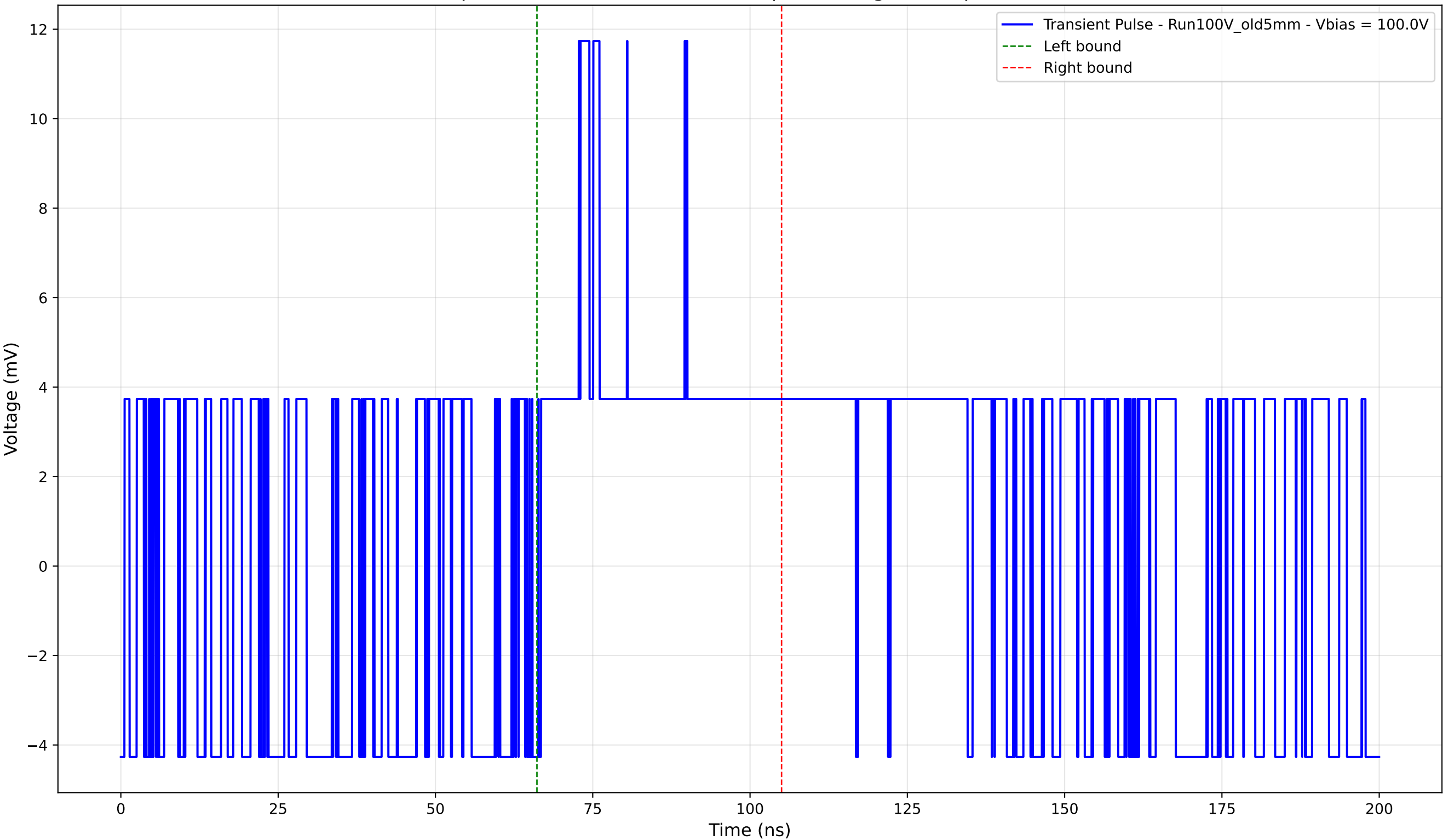
Transient Pulse - Sample: Old5mm - Position: 525.0 \mu\text{m} - Charge: 3.31 pC - Rise Time: 0.00 ns (N/A)
