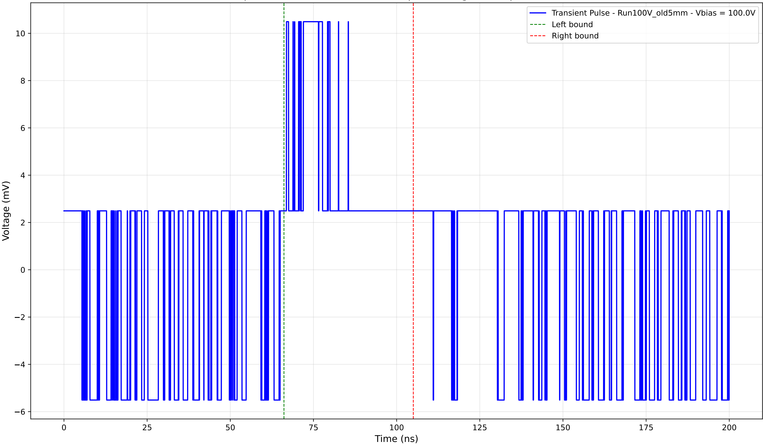
Transient Pulse - Sample: Old5mm - Position: 315.0 \mu\text{m} - Charge: 3.19 pC - Rise Time: 0.00 ns (N/A)
