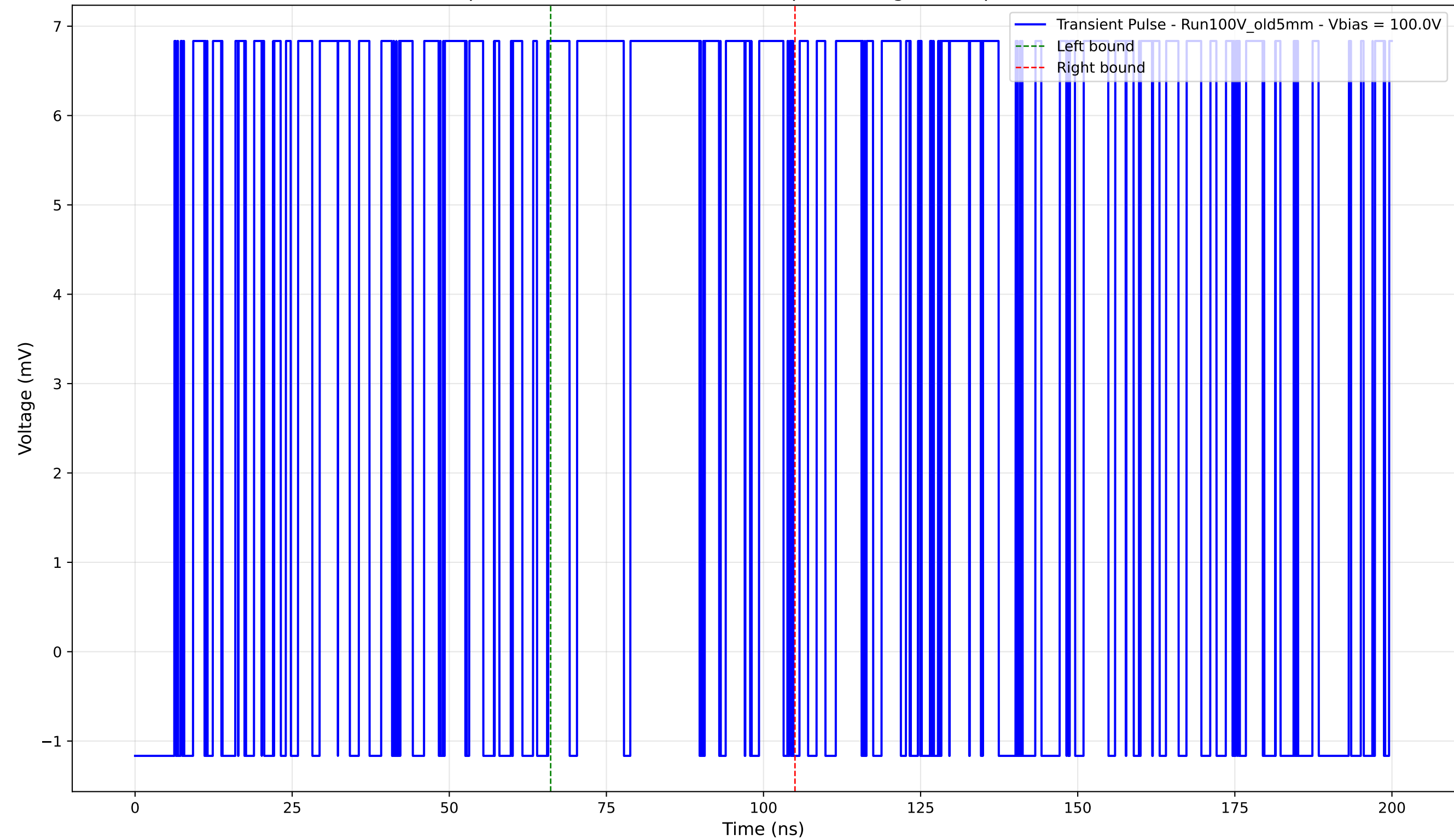
Transient Pulse - Sample: Old5mm - Position: 1910.0 \mu\text{m} - Charge: 4.23 pC - Rise Time: 0.00 ns (N/A)
