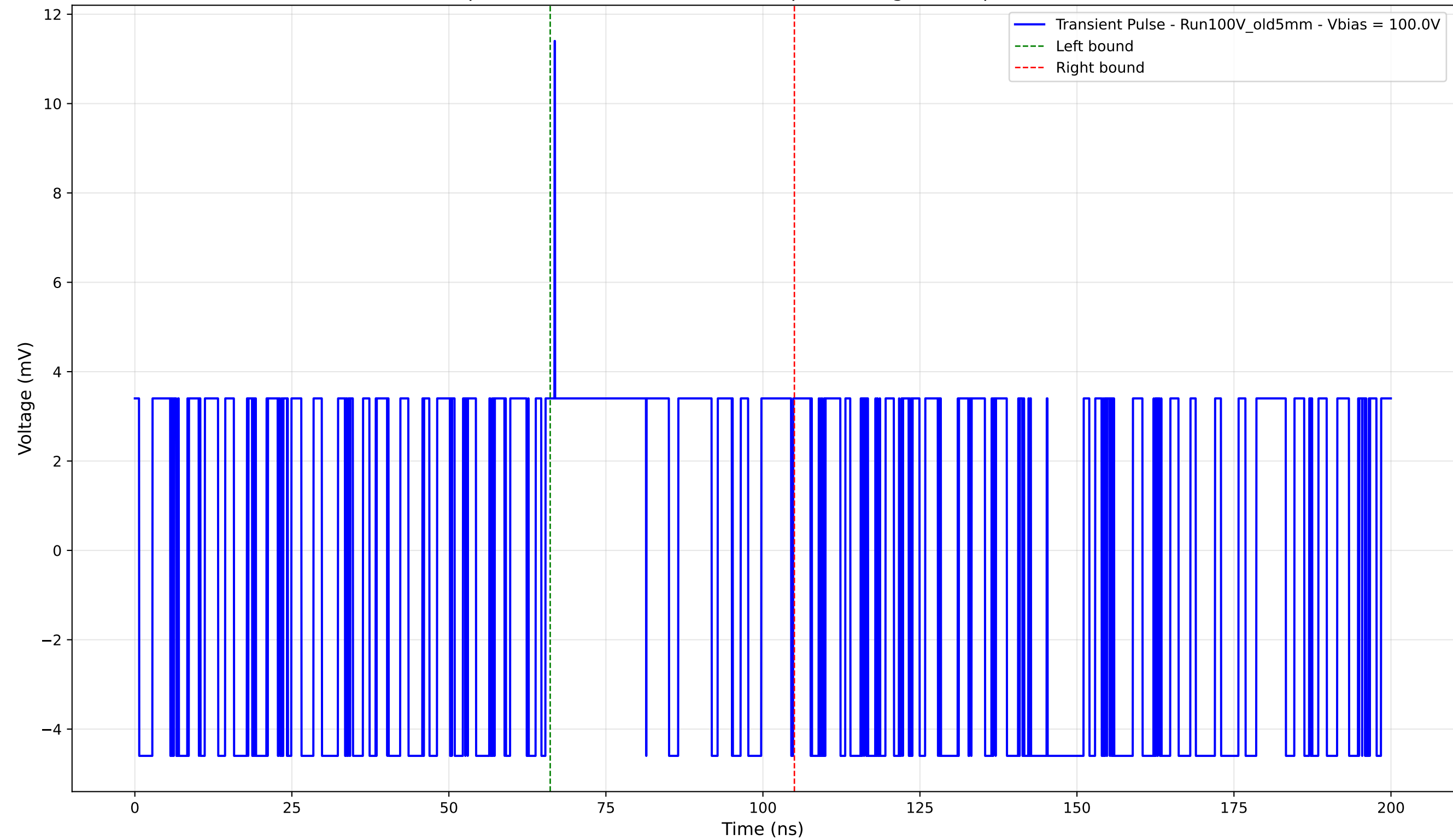
Transient Pulse - Sample: Old5mm - Position: 4030.0 \mu\text{m} - Charge: 1.66 pC - Rise Time: 0.00 ns (N/A)
