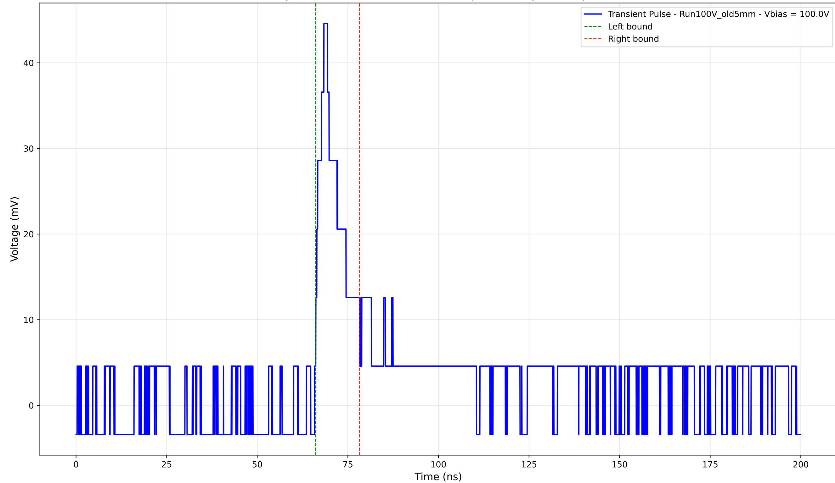
Transient Pulse - Sample: Old5mm - Position: 3165.0 \mu\text{m} - Charge: 5.70 pC - Rise Time: 2.56 ns
