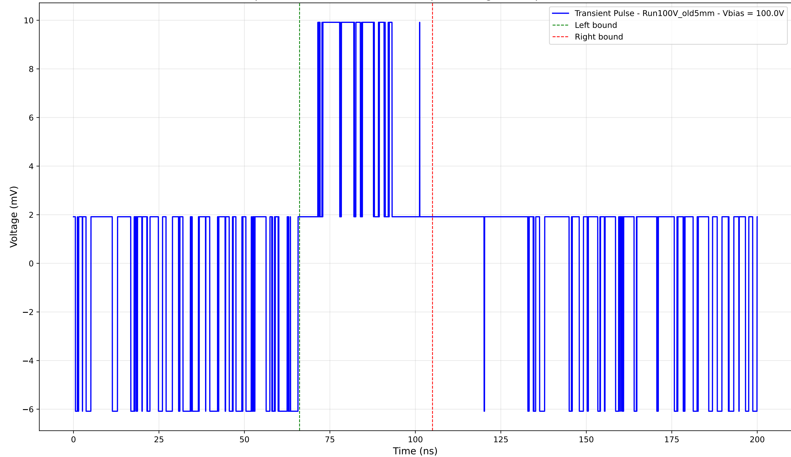
Transient Pulse - Sample: Old5mm - Position: 1460.0 \mu\text{m} - Charge: 4.11 pC - Rise Time: 0.00 ns (N/A)
