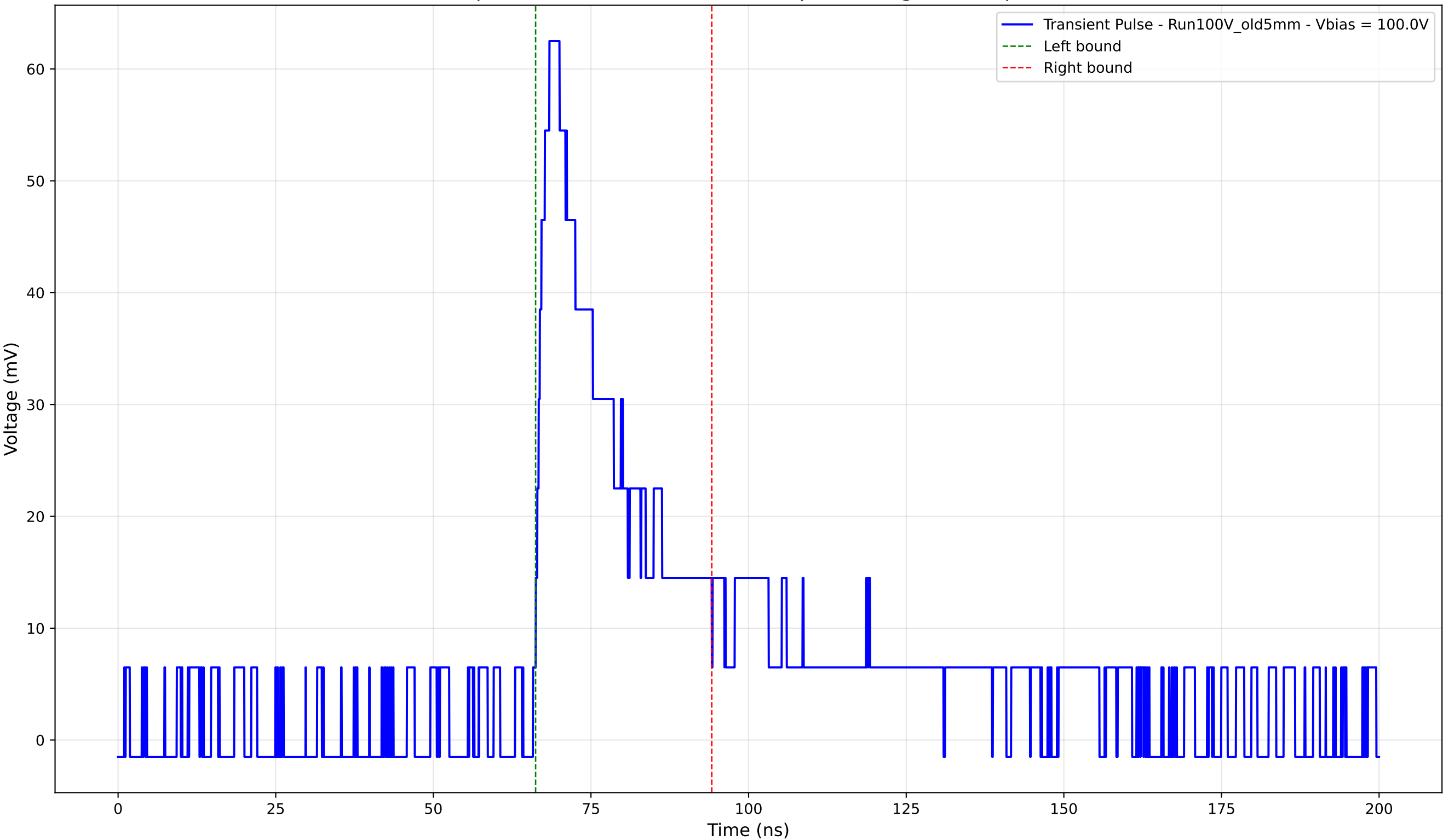
Transient Pulse - Sample: Old5mm - Position: 2935.0 \mu\text{m} - Charge: 15.93 pC - Rise Time: 2.60 ns
