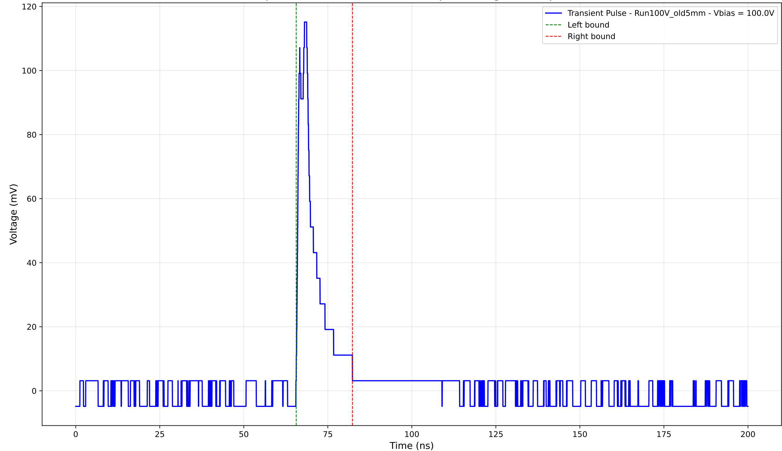
Transient Pulse - Sample: Old5mm - Position: 3490.0 \mu\text{m} - Charge: 12.78 pC - Rise Time: 0.94 ns
