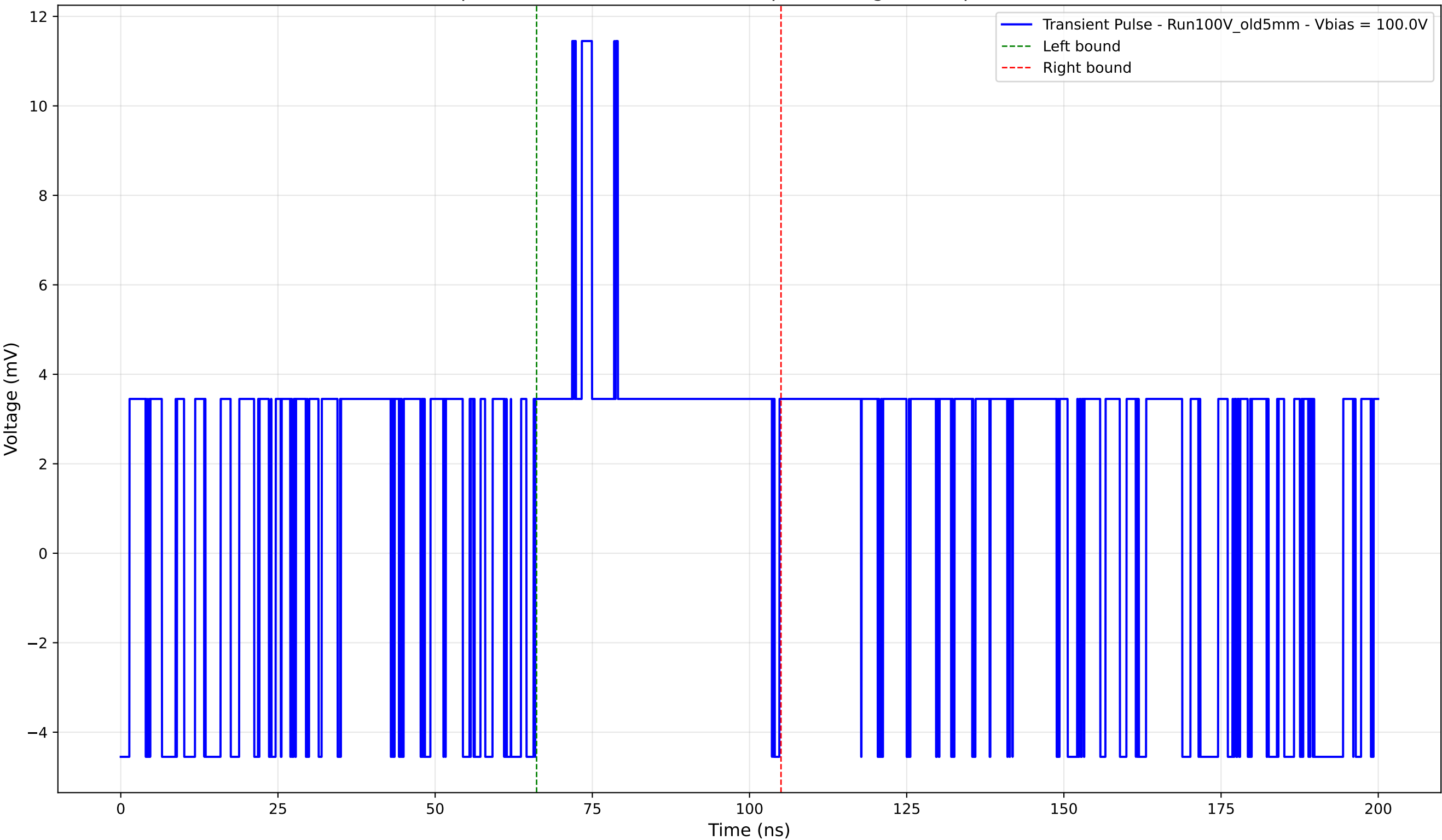
Transient Pulse - Sample: Old5mm - Position: 420.0 \mu\text{m} - Charge: 2.94 pC - Rise Time: 0.00 ns (N/A)
