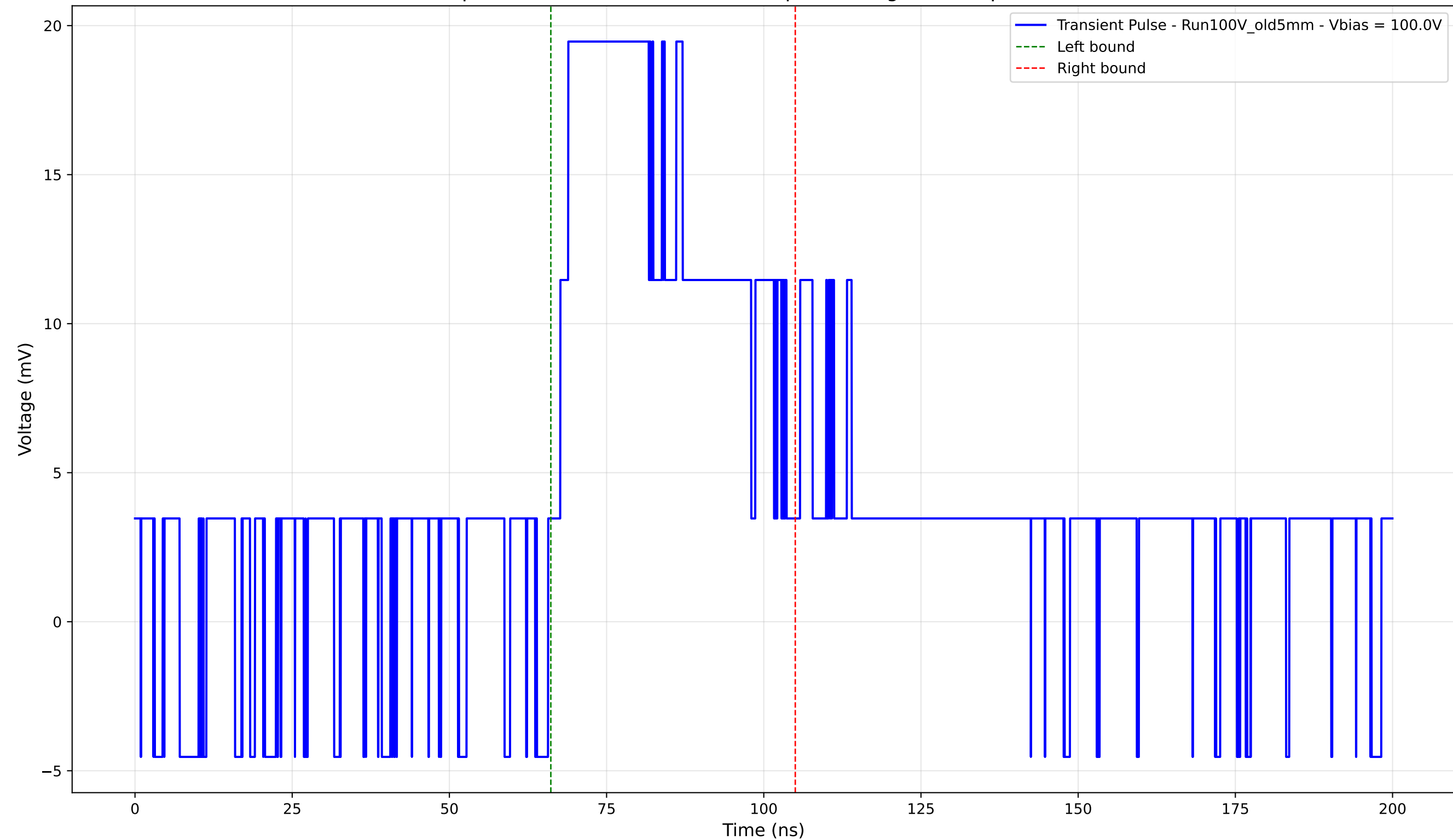
Transient Pulse - Sample: Old5mm - Position: 2380.0 \mu\text{m} - Charge: 10.56 pC - Rise Time: 0.00 ns (N/A)
