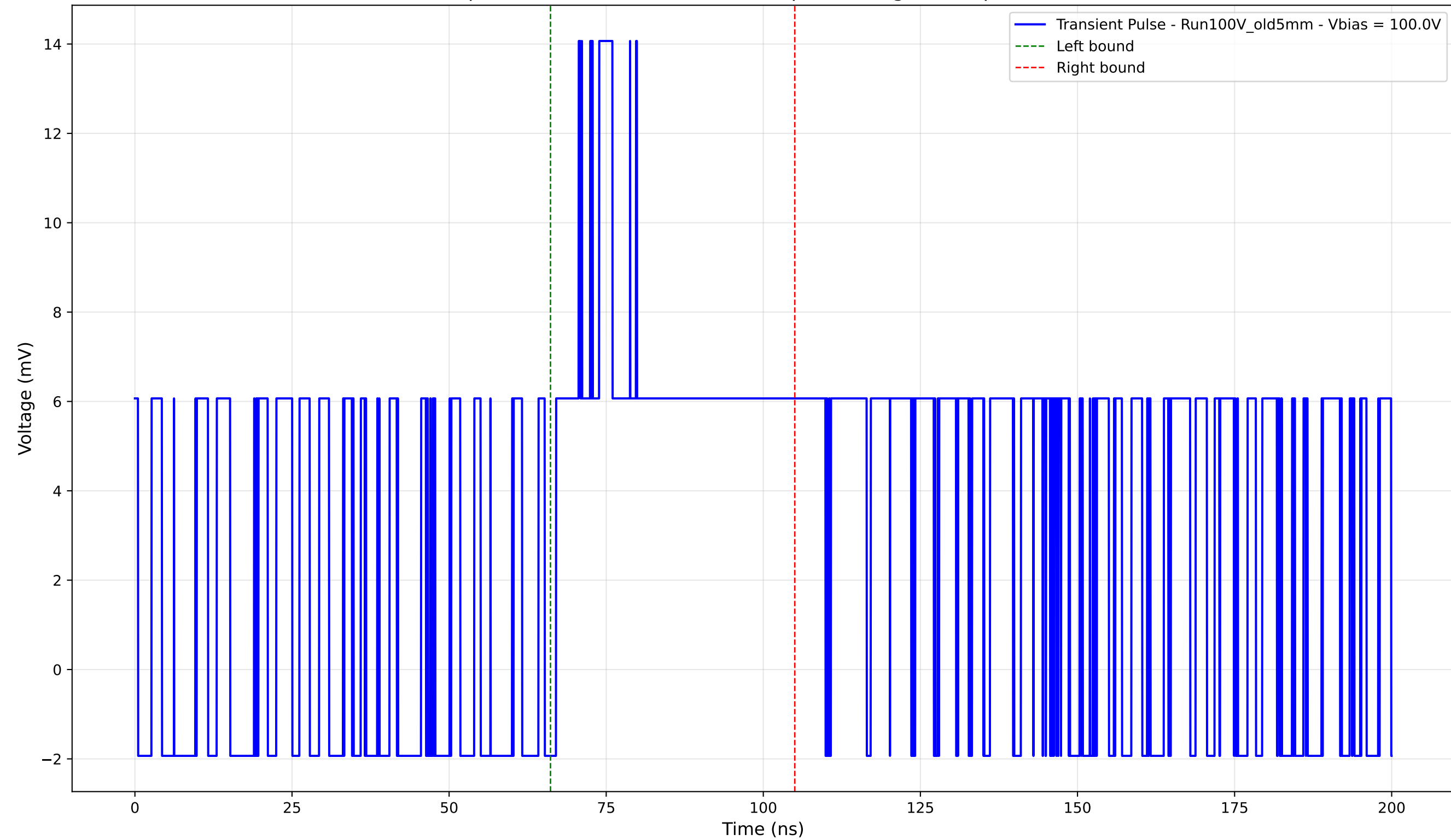
Transient Pulse - Sample: Old5mm - Position: 2290.0 \mu\text{m} - Charge: 5.04 pC - Rise Time: 0.00 ns (N/A)
