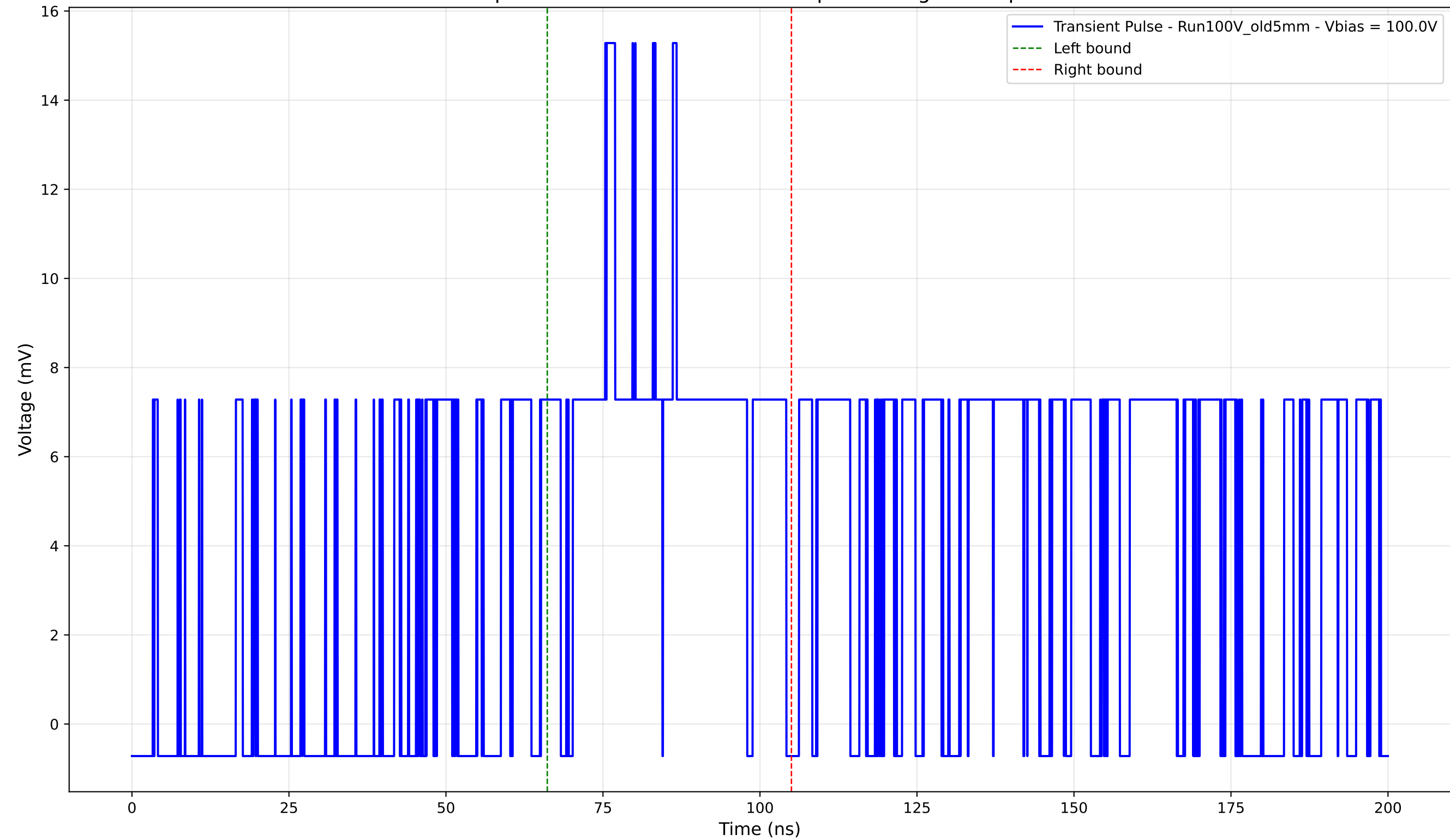
Transient Pulse - Sample: Old5mm - Position: 1025.0 \mu\text{m} - Charge: 5.51 pC - Rise Time: 5.18 ns
