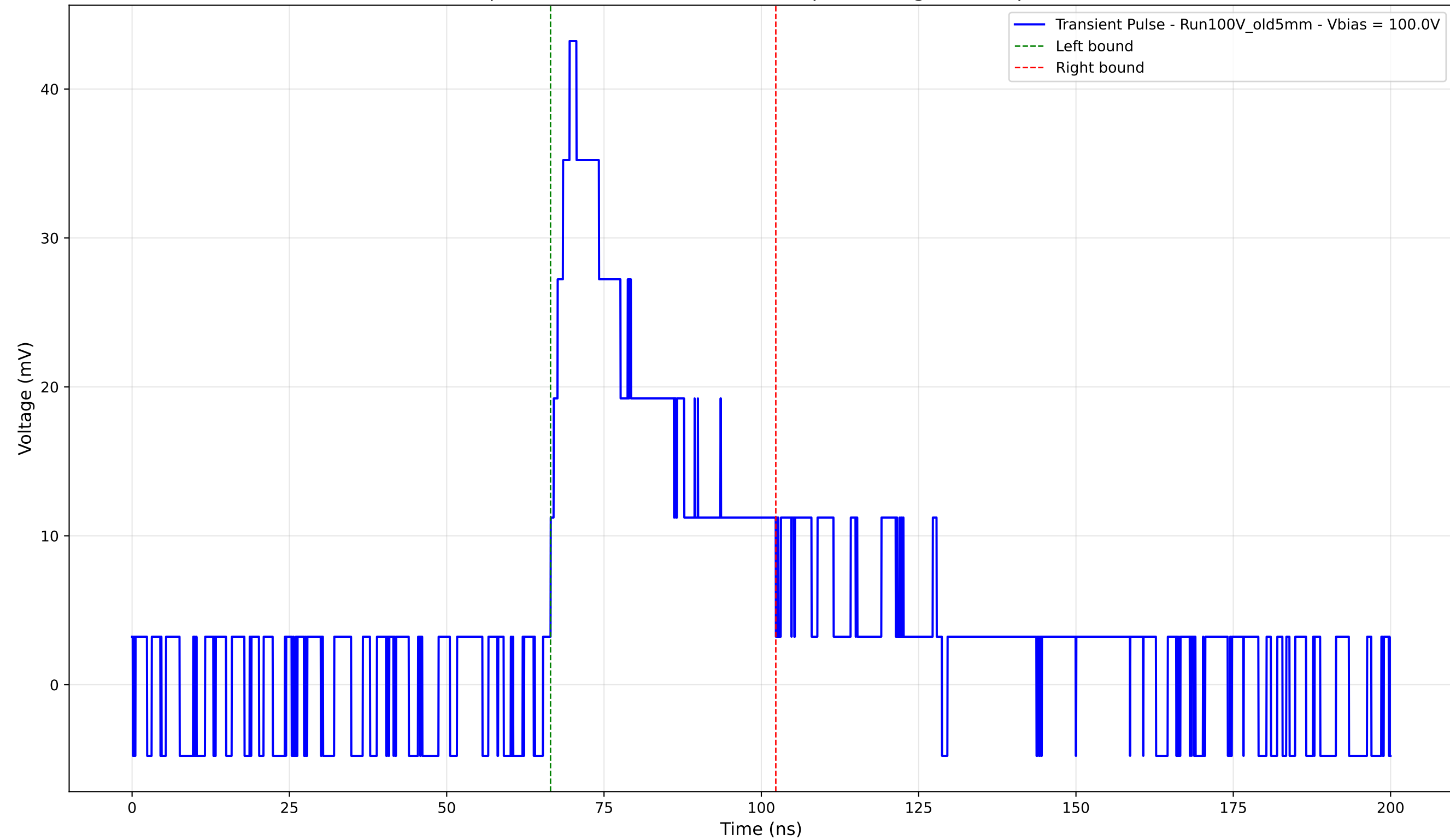
Transient Pulse - Sample: Old5mm - Position: 2640.0 \mu\text{m} - Charge: 14.08 pC - Rise Time: 3.02 ns
