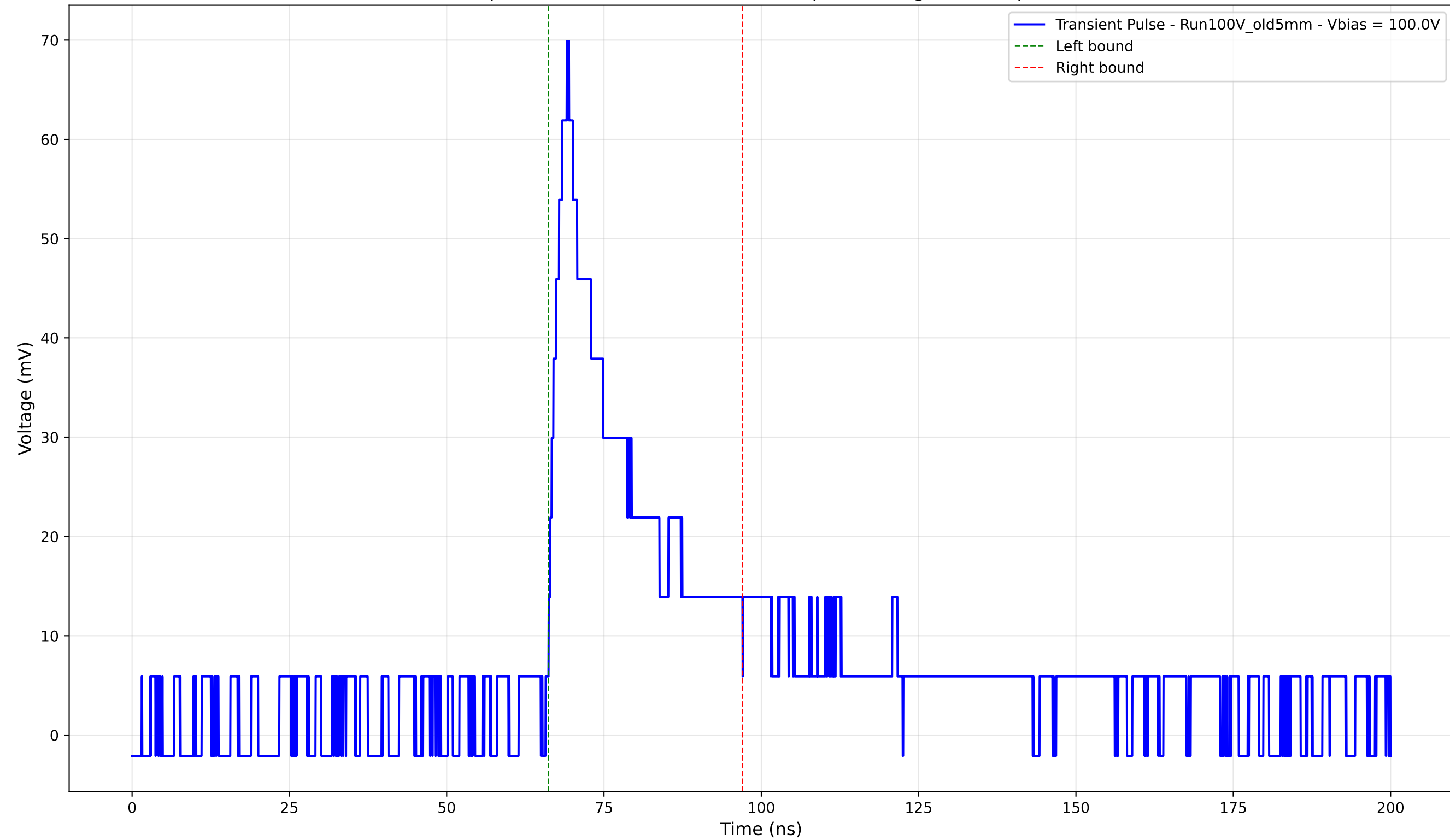
Transient Pulse - Sample: Old5mm - Position: 2925.0 \mu\text{m} - Charge: 16.65 pC - Rise Time: 2.90 ns
