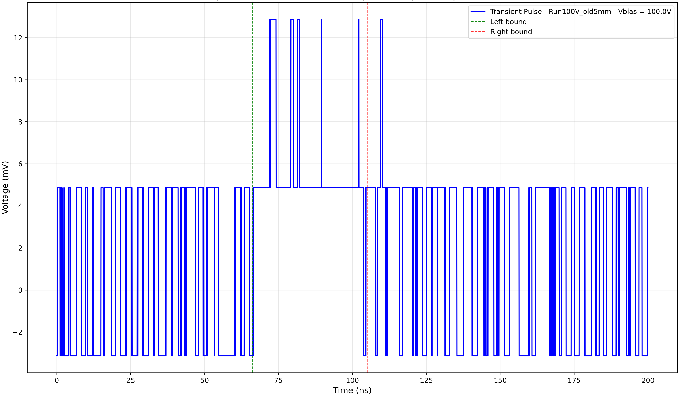
Transient Pulse - Sample: Old5mm - Position: 730.0 \mu\text{m} - Charge: 4.25 pC - Rise Time: 0.00 ns (N/A)
