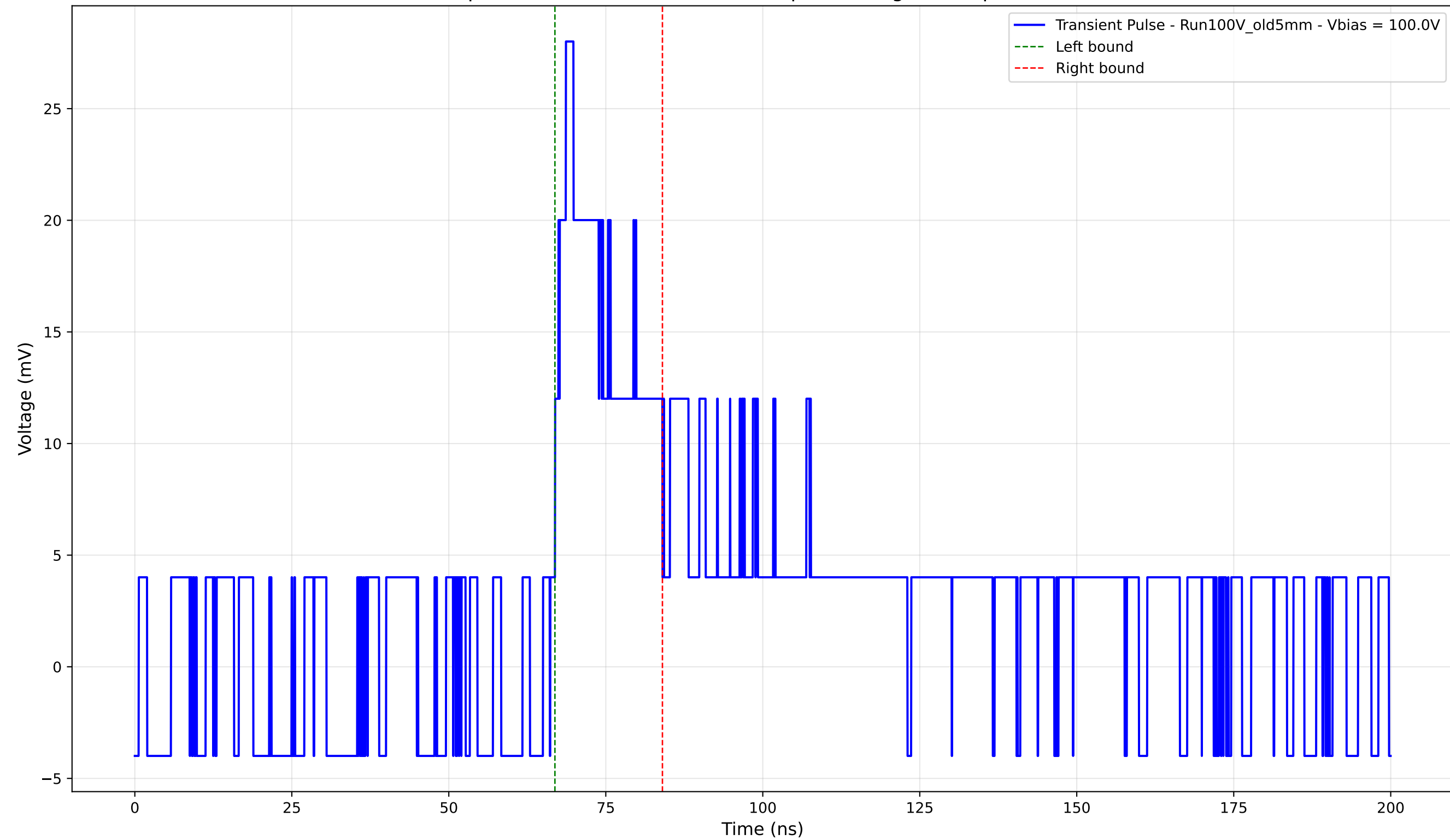
Transient Pulse - Sample: Old5mm - Position: 2725.0 \mu\text{m} - Charge: 5.51 pC - Rise Time: 0.00 ns (N/A)
