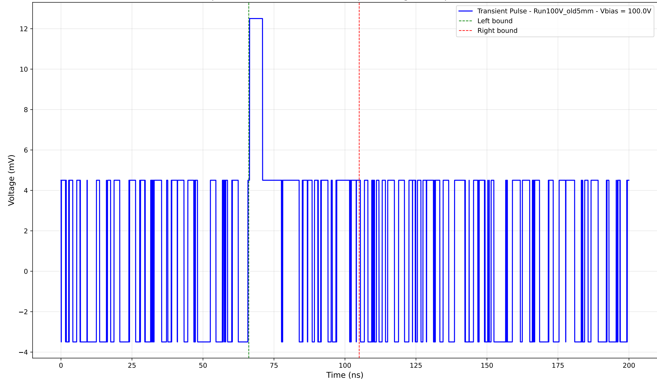
Transient Pulse - Sample: Old5mm - Position: 4040.0 \mu\text{m} - Charge: 3.21 pC - Rise Time: 0.00 ns (N/A)
