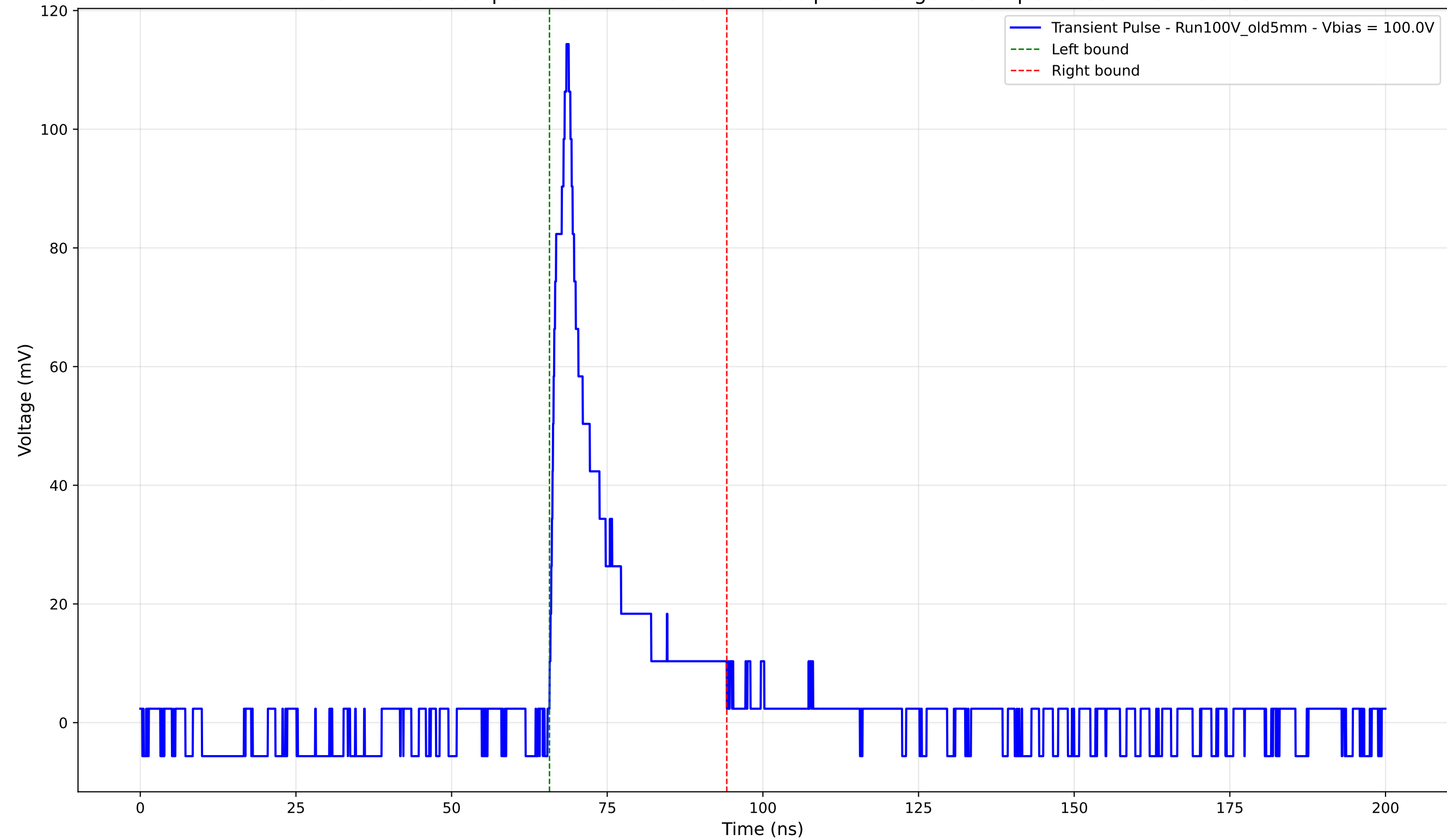
Transient Pulse - Sample: Old5mm - Position: 4165.0 \mu\text{m} - Charge: 16.91 pC - Rise Time: 2.30 ns
