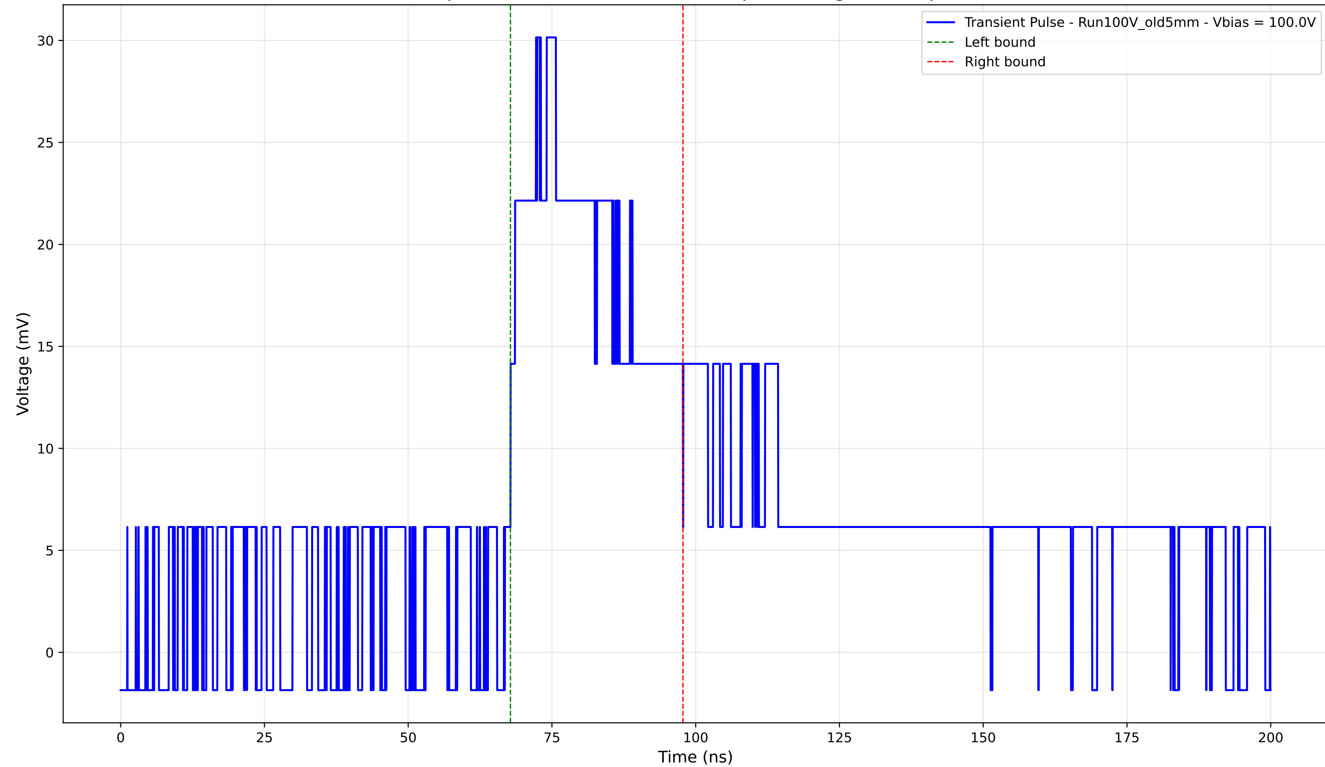
Transient Pulse - Sample: Old5mm - Position: 2195.0 \mu\text{m} - Charge: 11.70 pC - Rise Time: 5.41 ns
