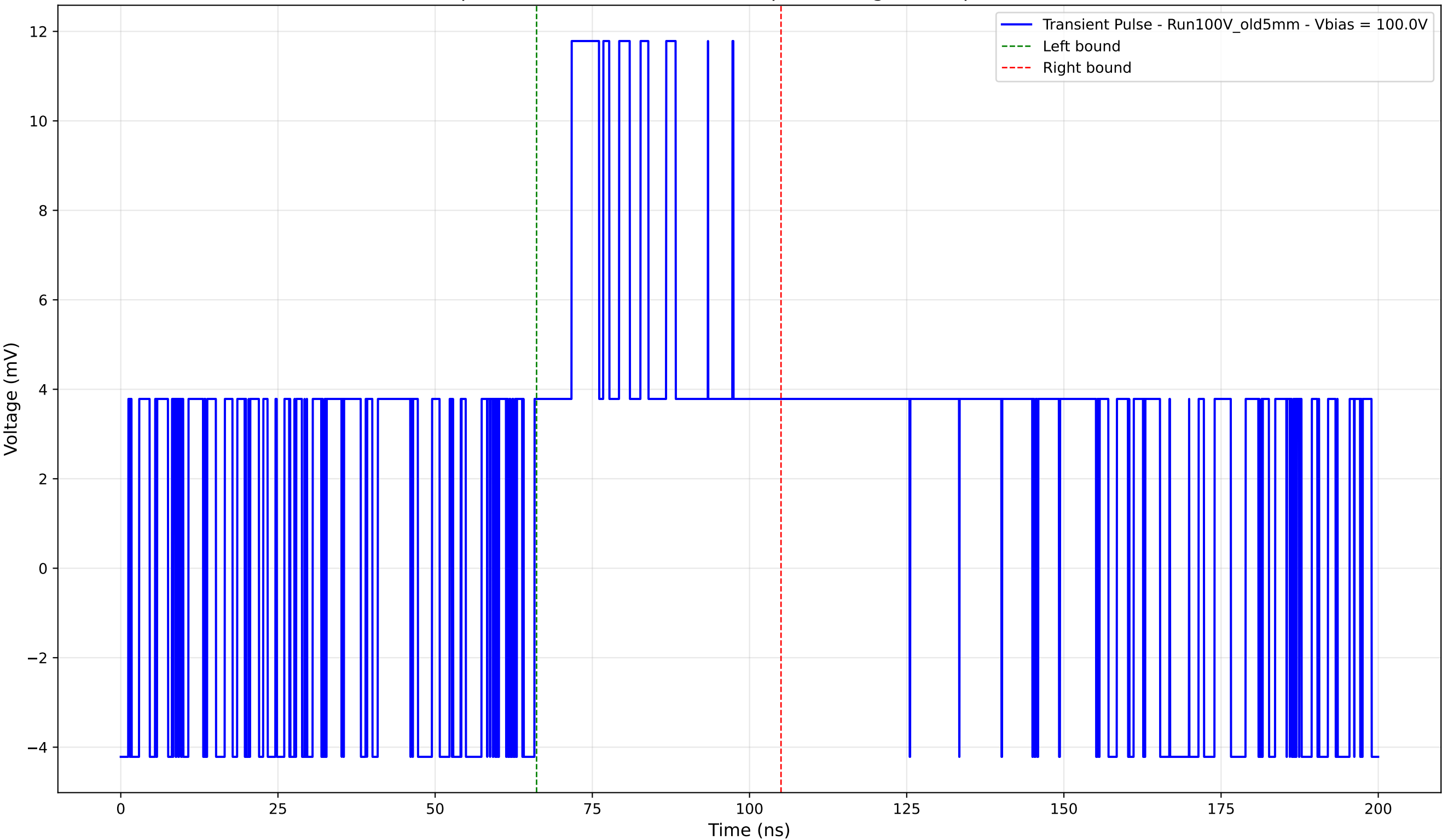
Transient Pulse - Sample: Old5mm - Position: 770.0 \mu\text{m} - Charge: 4.54 pC - Rise Time: 0.00 ns (N/A)
