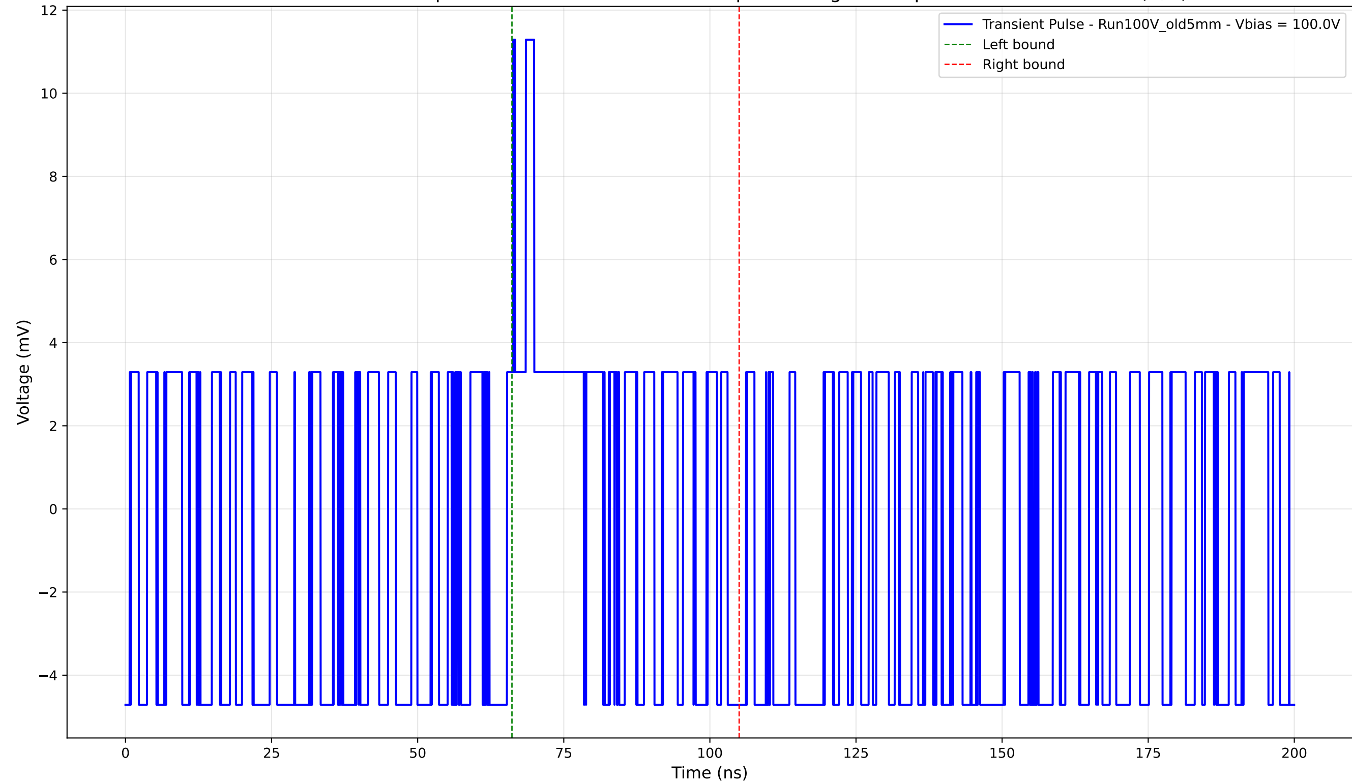
Transient Pulse - Sample: Old5mm - Position: 4035.0 \mu\text{m} - Charge: 1.17 pC - Rise Time: 0.00 ns (N/A)
