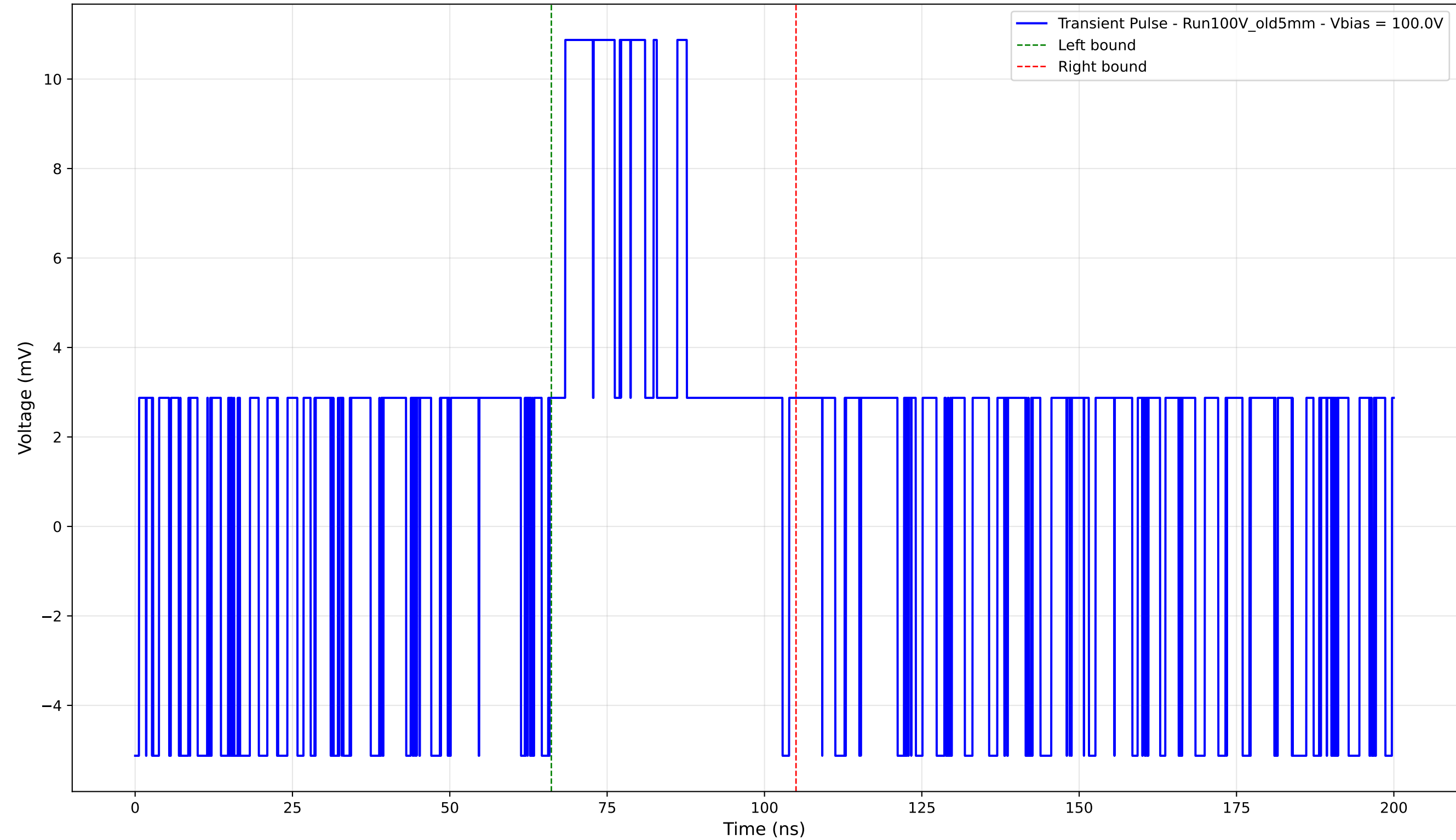
Transient Pulse - Sample: Old5mm - Position: 2490.0 \mu\text{m} - Charge: 4.26 pC - Rise Time: 0.00 ns (N/A)
