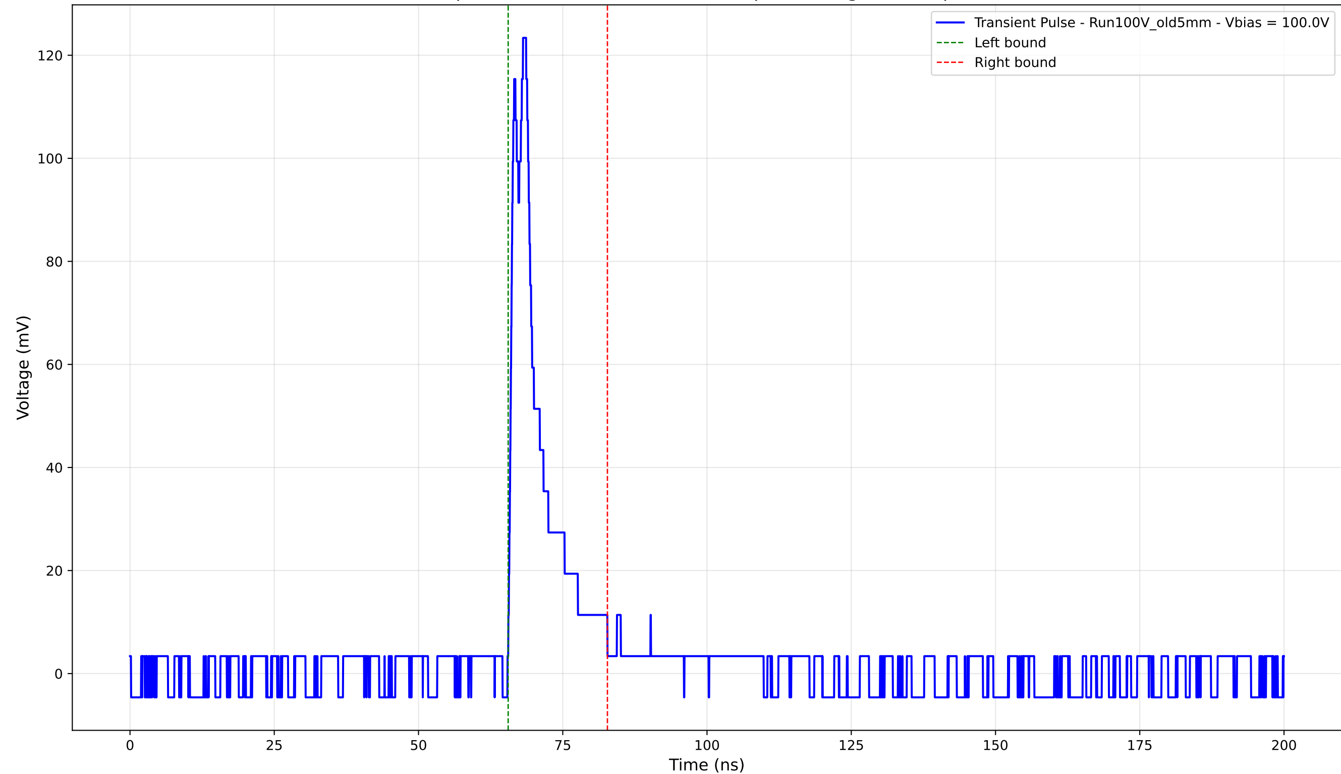
Transient Pulse - Sample: Old5mm - Position: 3925.0 \mu\text{m} - Charge: 13.90 pC - Rise Time: 0.92 ns
