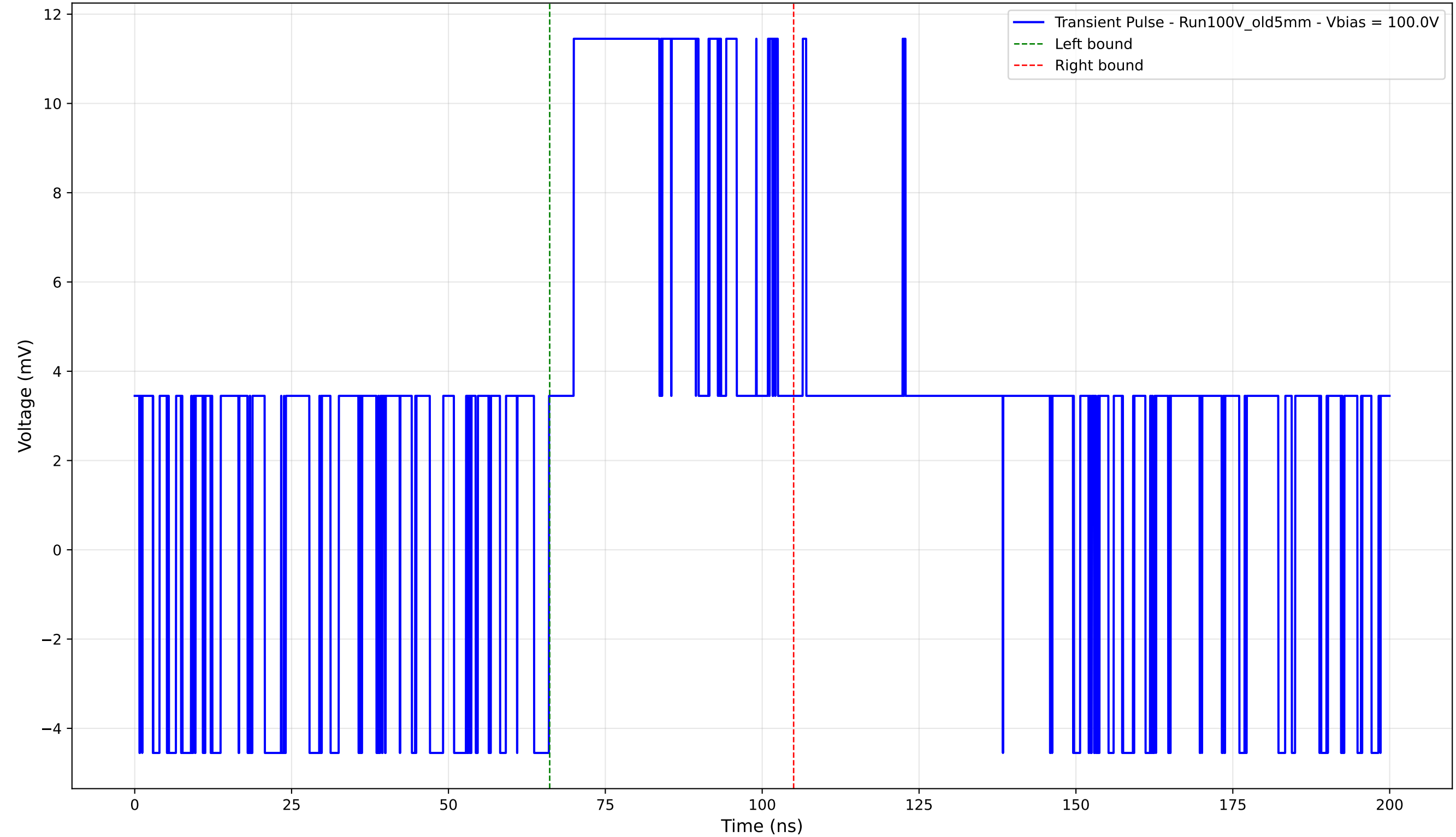
Transient Pulse - Sample: Old5mm - Position: 2070.0 \mu\text{m} - Charge: 6.56 pC - Rise Time: 0.00 ns (N/A)
