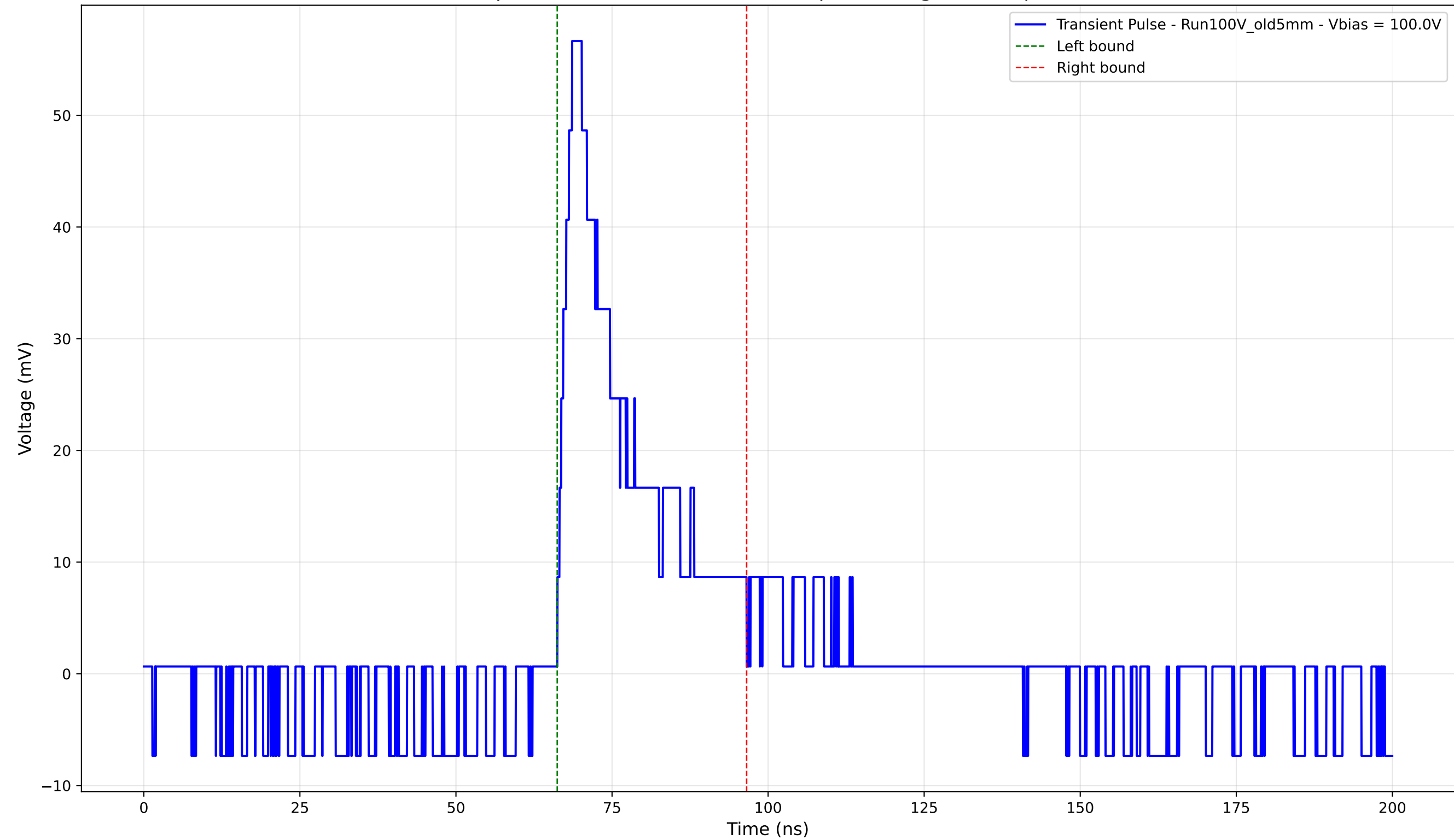
Transient Pulse - Sample: Old5mm - Position: 2910.0 \mu\text{m} - Charge: 12.70 pC - Rise Time: 2.37 ns
