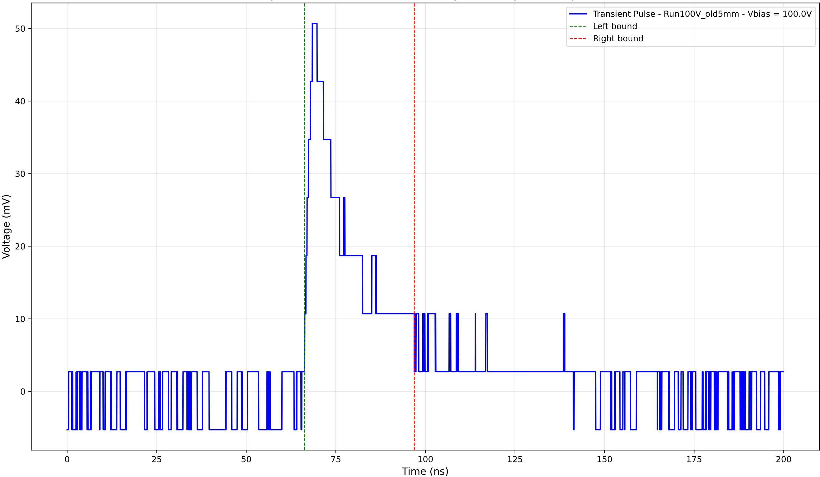
Transient Pulse - Sample: Old5mm - Position: 2895.0 \mu\text{m} - Charge: 12.54 pC - Rise Time: 2.11 ns
