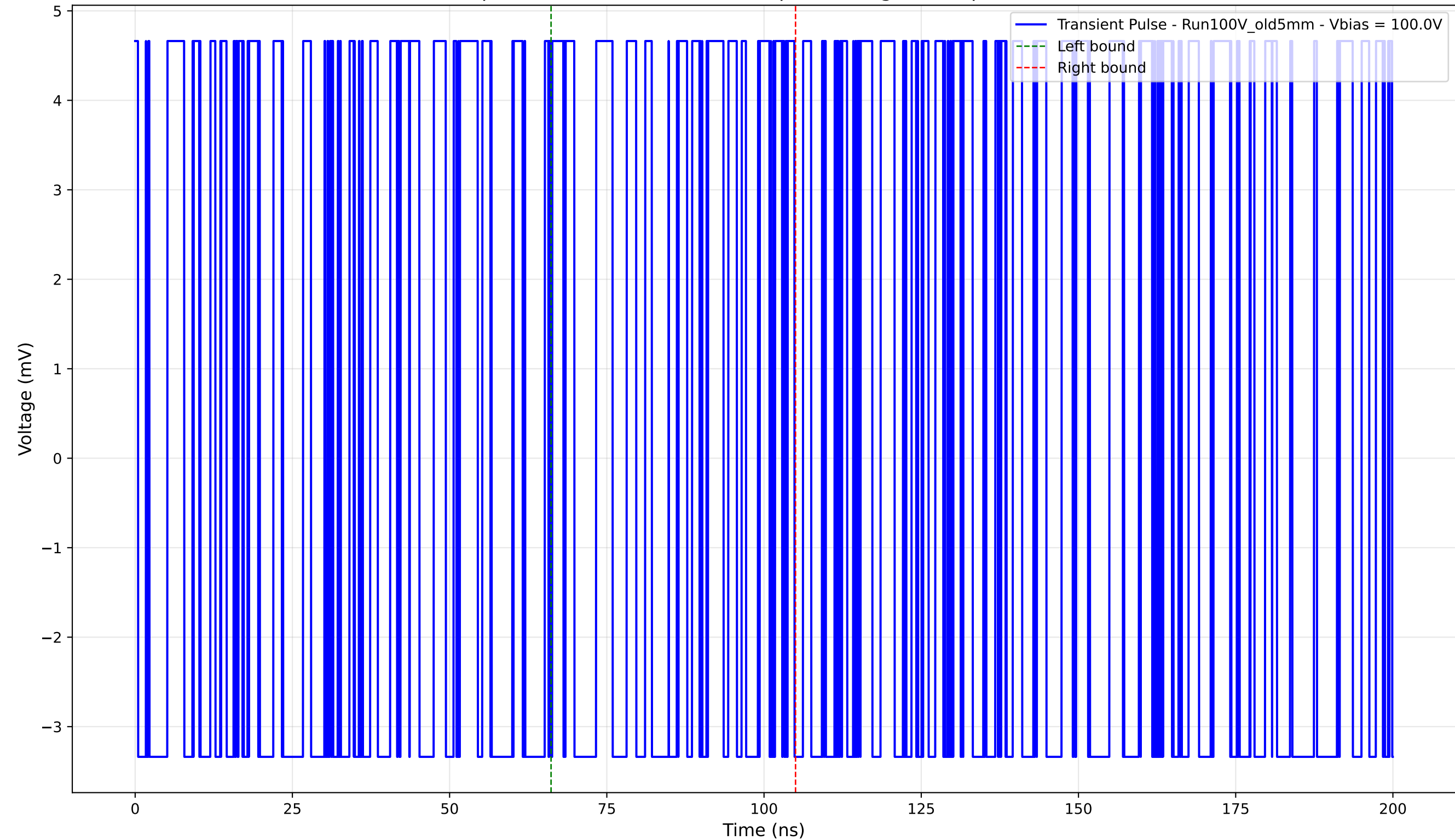
Transient Pulse - Sample: Old5mm - Position: 80.0 \mu\text{m} - Charge: 0.71 pC - Rise Time: 0.00 ns (N/A)
