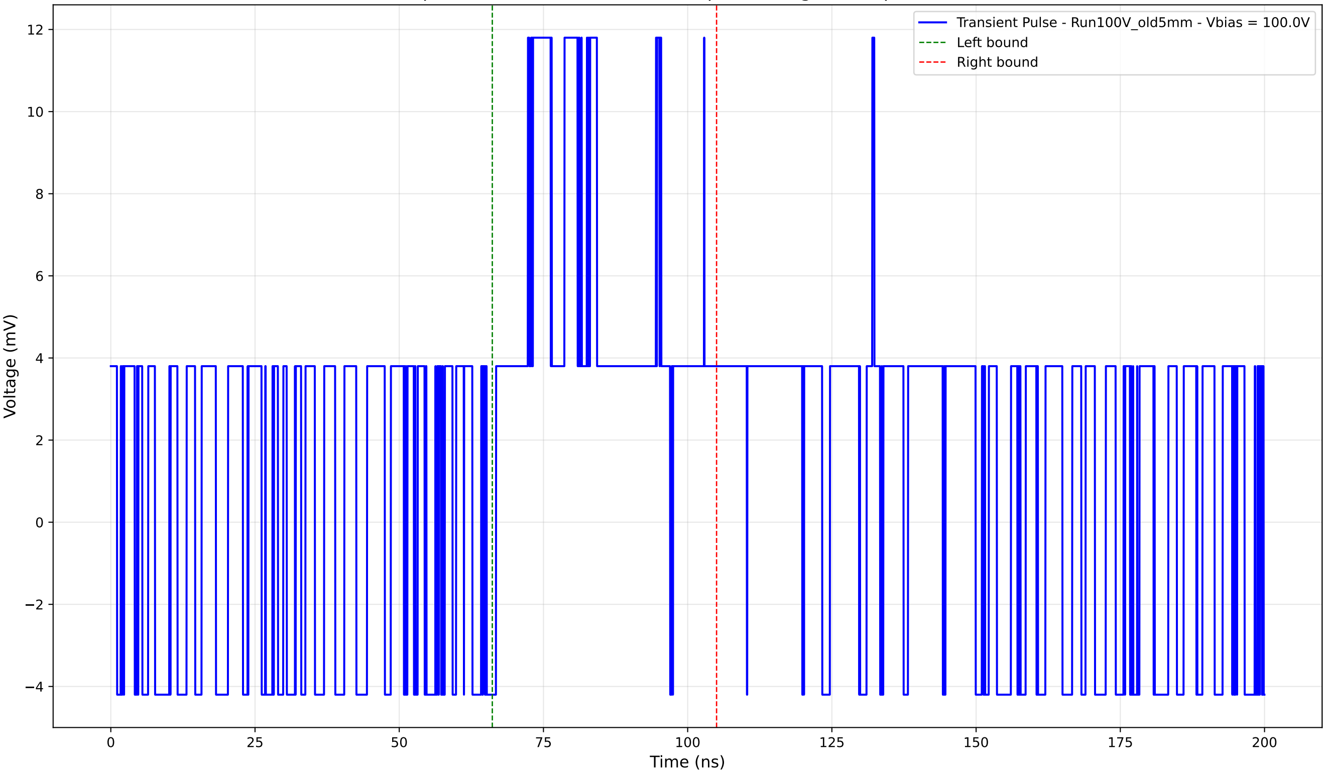
Transient Pulse - Sample: Old5mm - Position: 645.0 \mu\text{m} - Charge: 4.14 pC - Rise Time: 0.00 ns (N/A)
