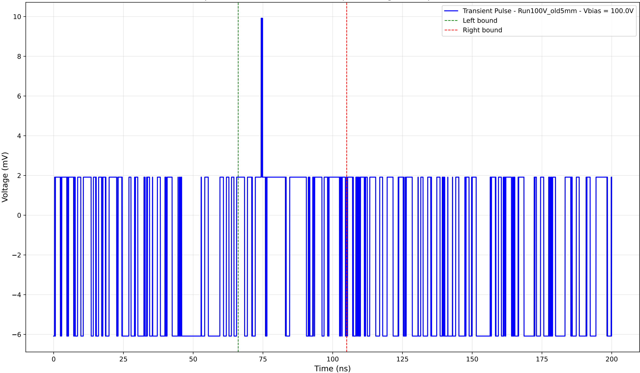
Transient Pulse - Sample: Old5mm - Position: 275.0 \mu\text{m} - Charge: 0.35 pC - Rise Time: 0.00 ns (N/A)
