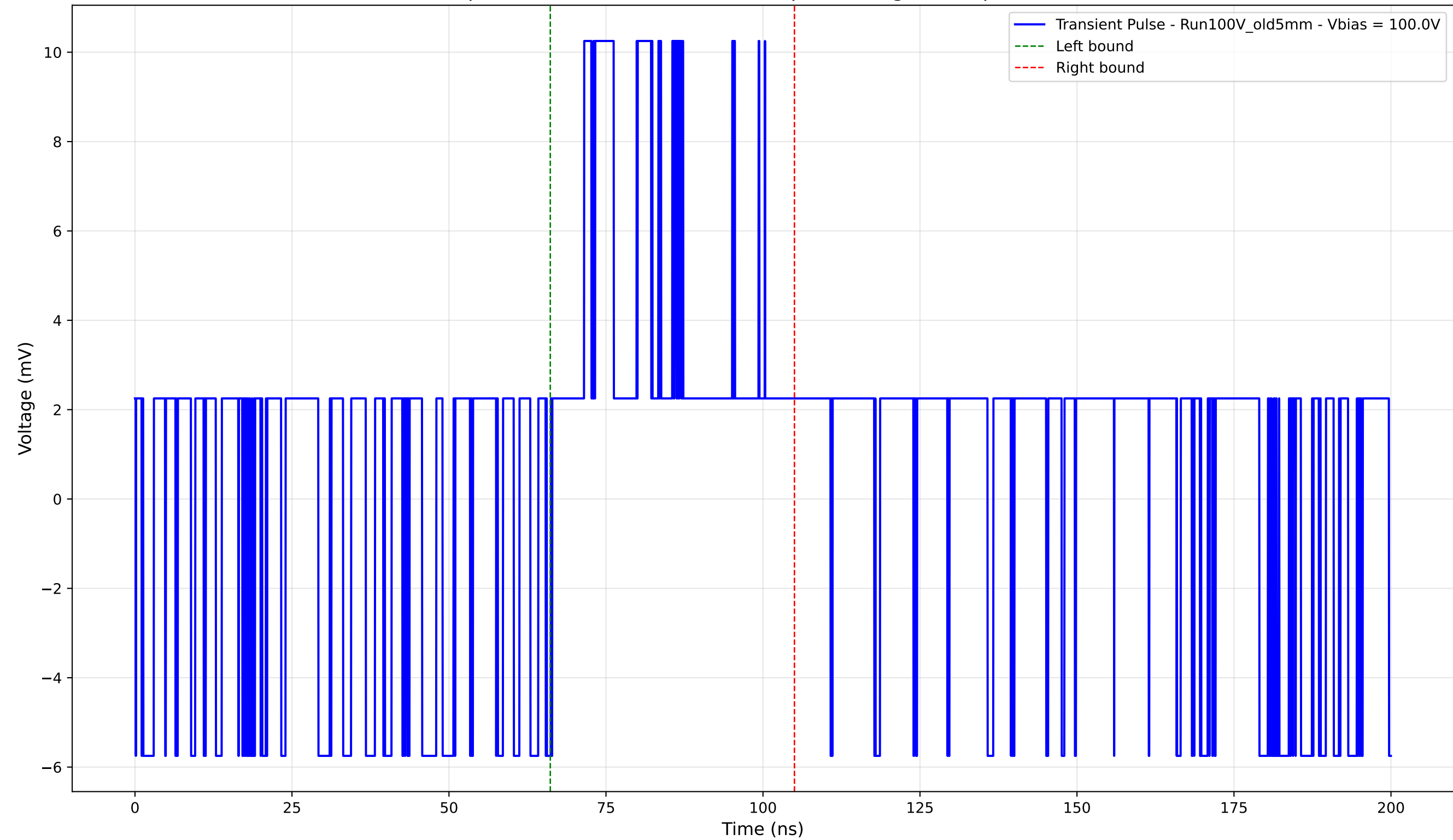
Transient Pulse - Sample: Old5mm - Position: 1145.0 \mu\text{m} - Charge: 3.07 pC - Rise Time: 0.00 ns (N/A)
