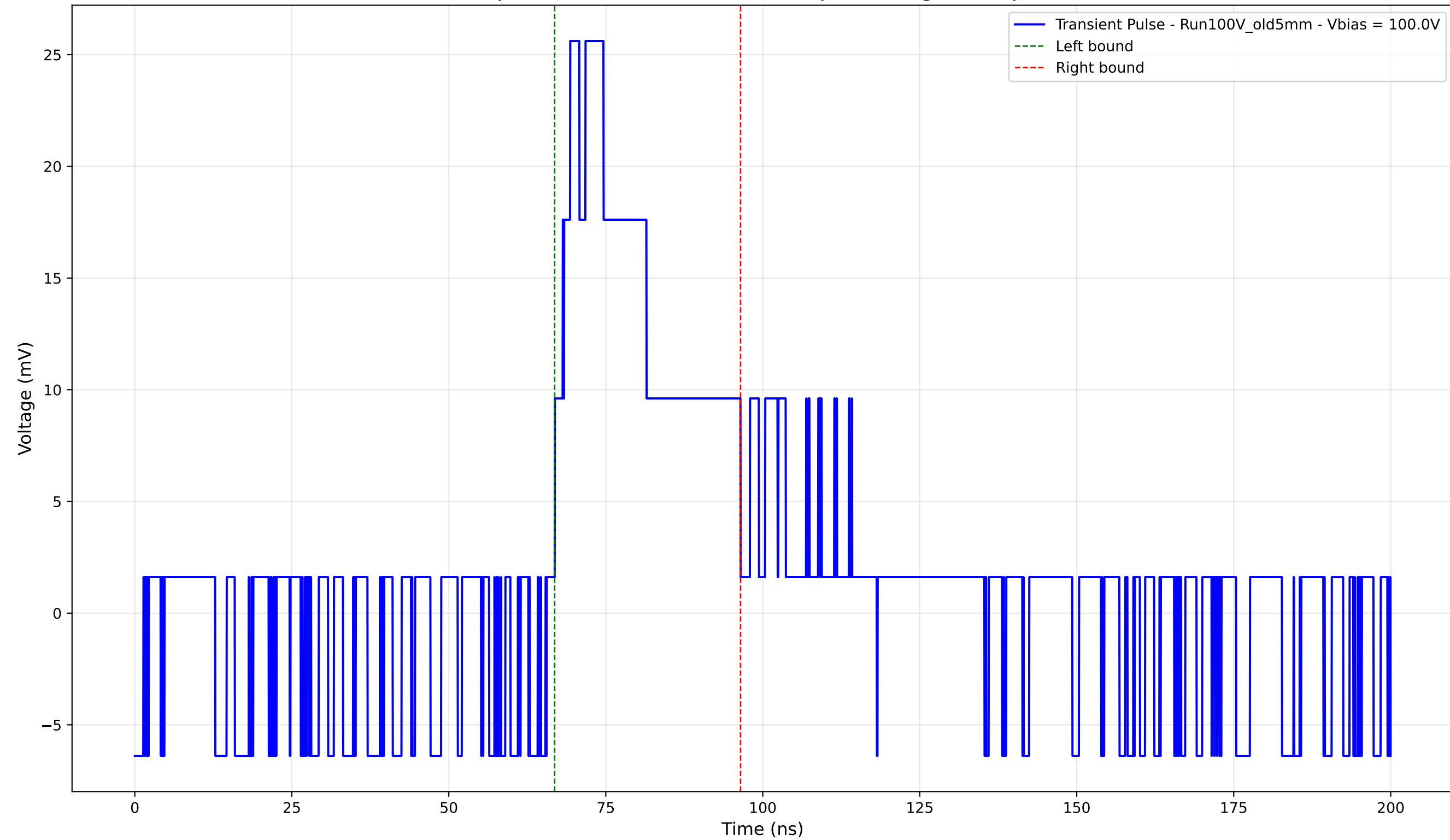
Transient Pulse - Sample: Old5mm - Position: 2580.0 \mu\text{m} - Charge: 8.50 pC - Rise Time: 2.46 ns
