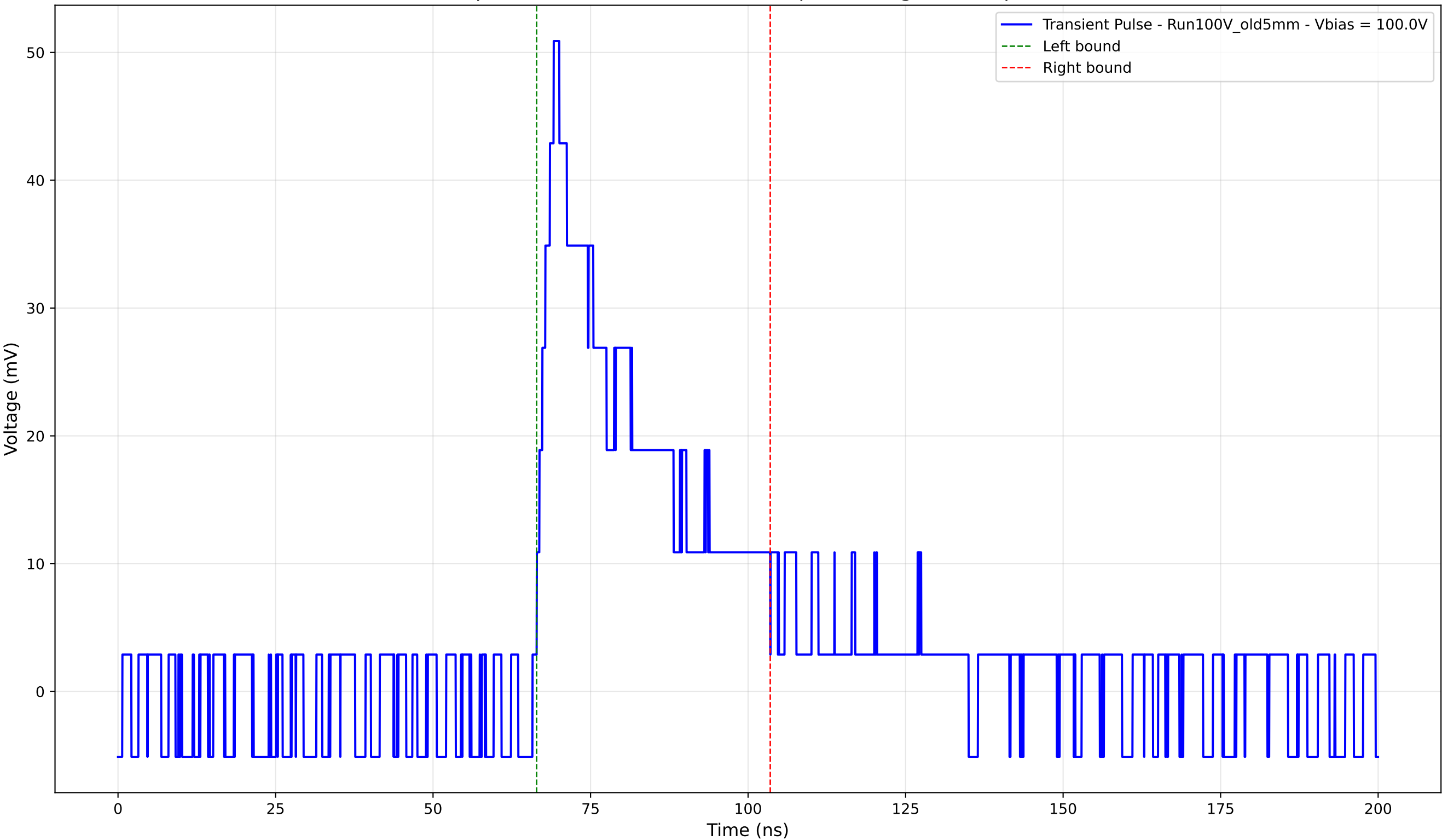
Transient Pulse - Sample: Old5mm - Position: 4760.0 \mu\text{m} - Charge: 15.54 pC - Rise Time: 2.69 ns
