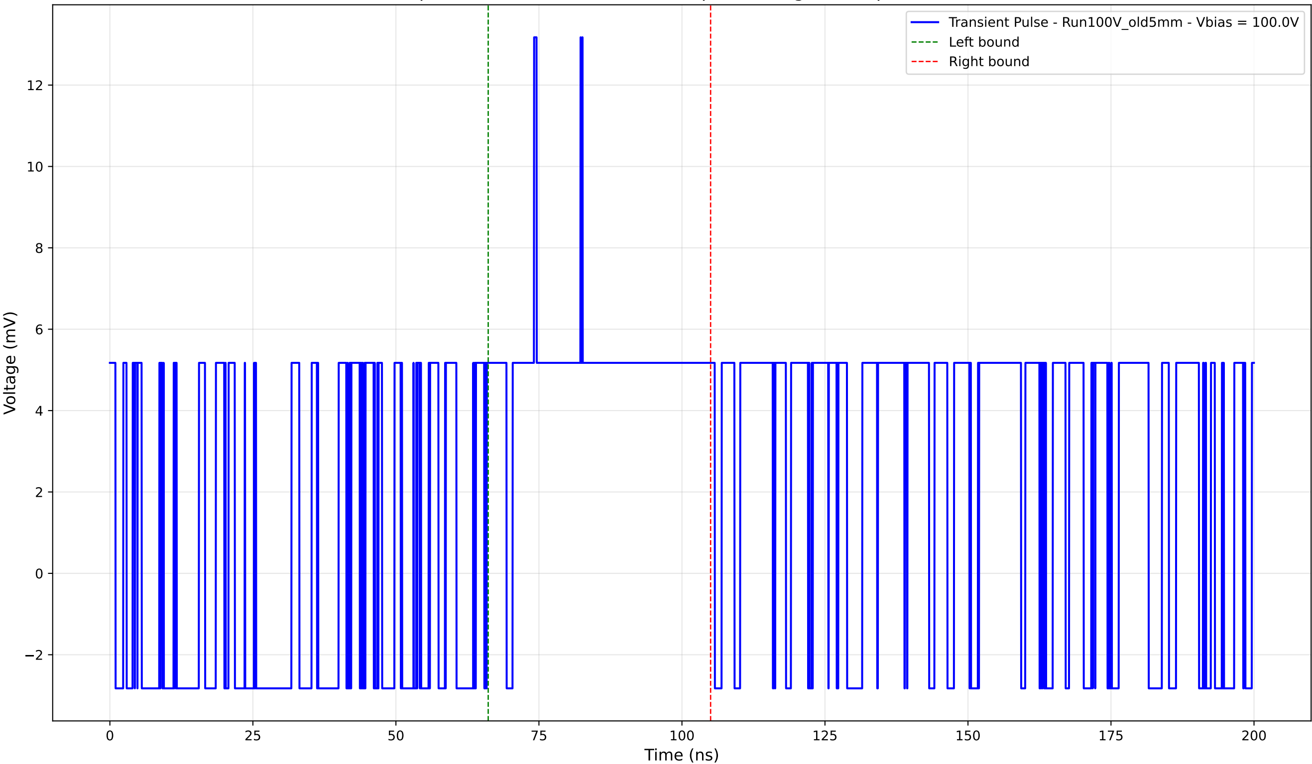
Transient Pulse - Sample: Old5mm - Position: 830.0 \mu\text{m} - Charge: 3.95 pC - Rise Time: 0.00 ns (N/A)
