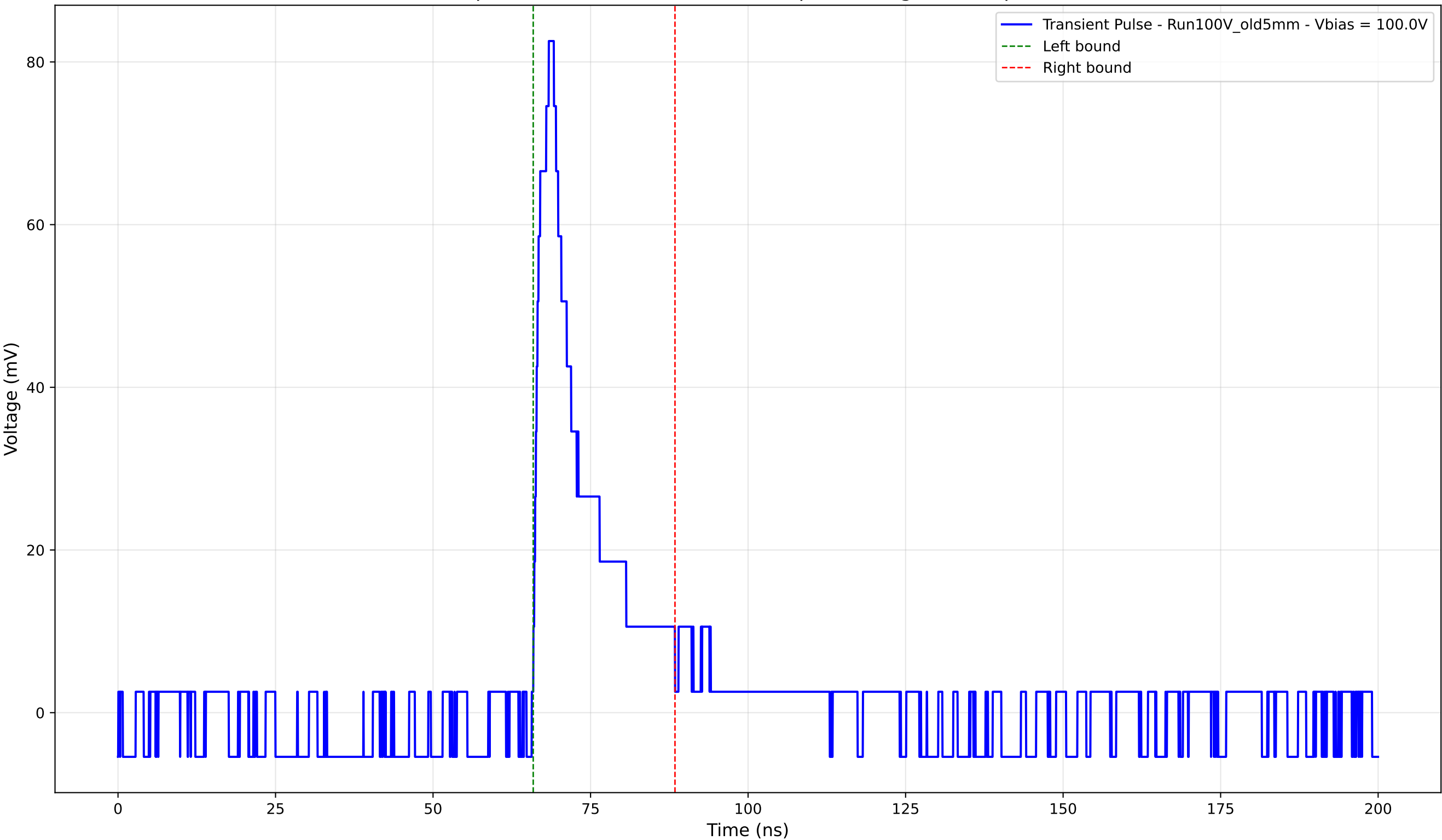
Transient Pulse - Sample: Old5mm - Position: 4210.0 \mu\text{m} - Charge: 12.83 pC - Rise Time: 2.05 ns
