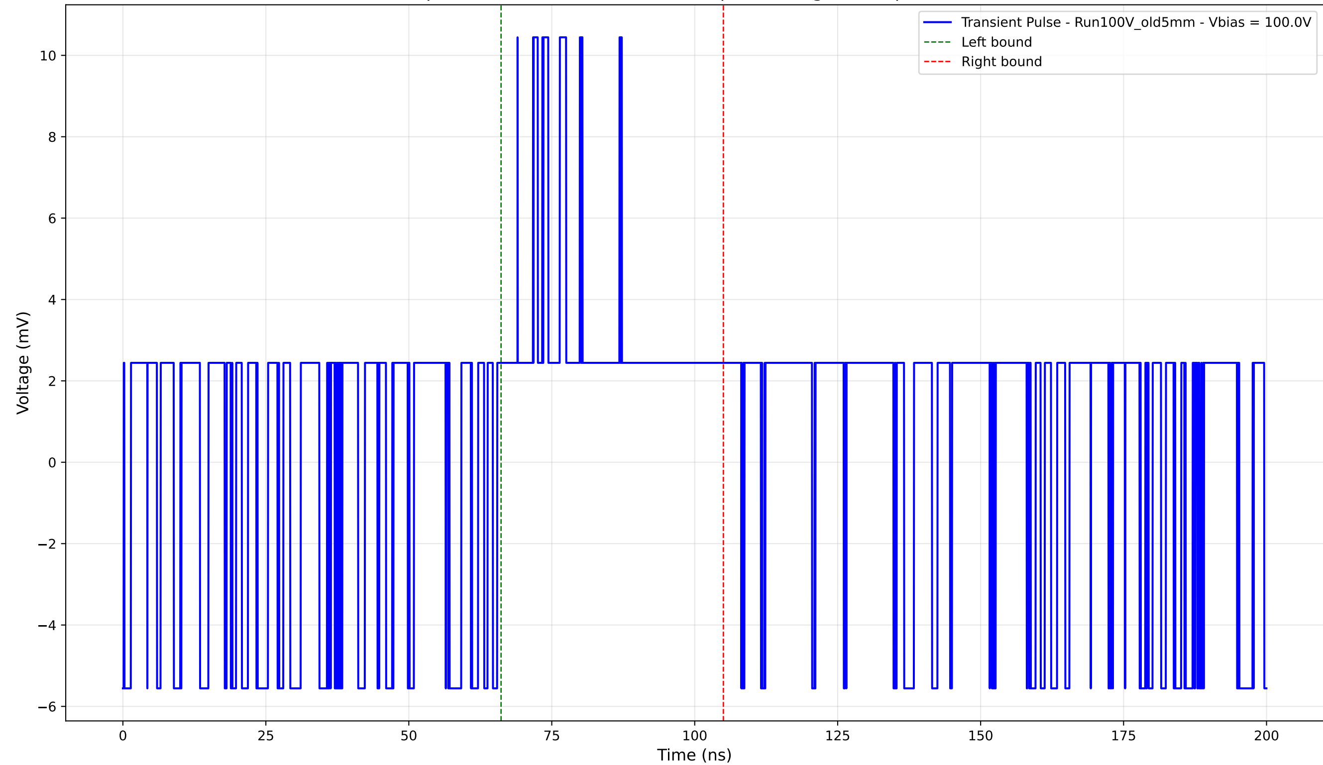
Transient Pulse - Sample: Old5mm - Position: 2295.0 \mu\text{m} - Charge: 2.47 pC - Rise Time: 0.00 ns (N/A)
