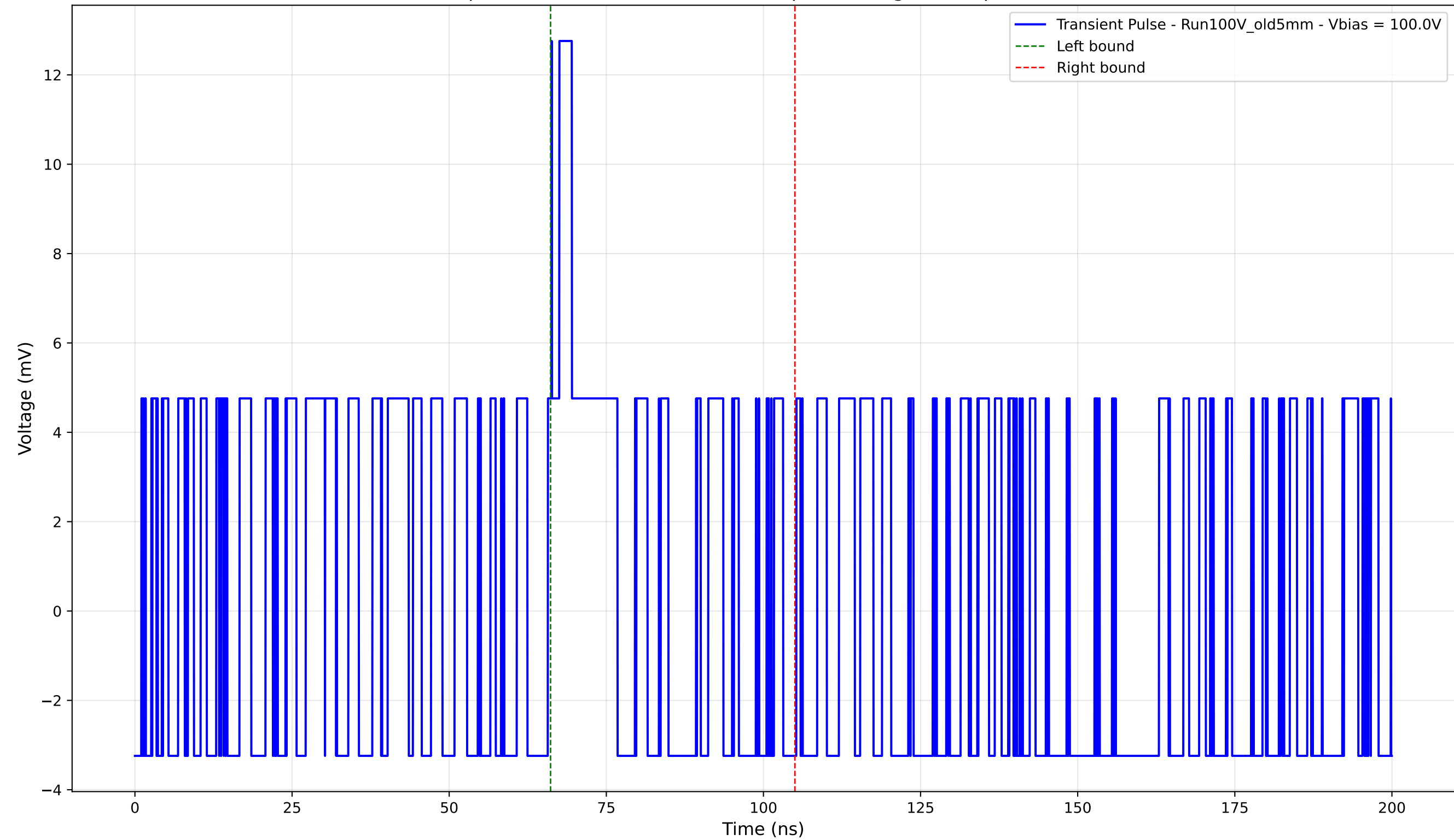
Transient Pulse - Sample: Old5mm - Position: 3725.0 \mu\text{m} - Charge: 0.94 pC - Rise Time: 0.00 ns (N/A)
