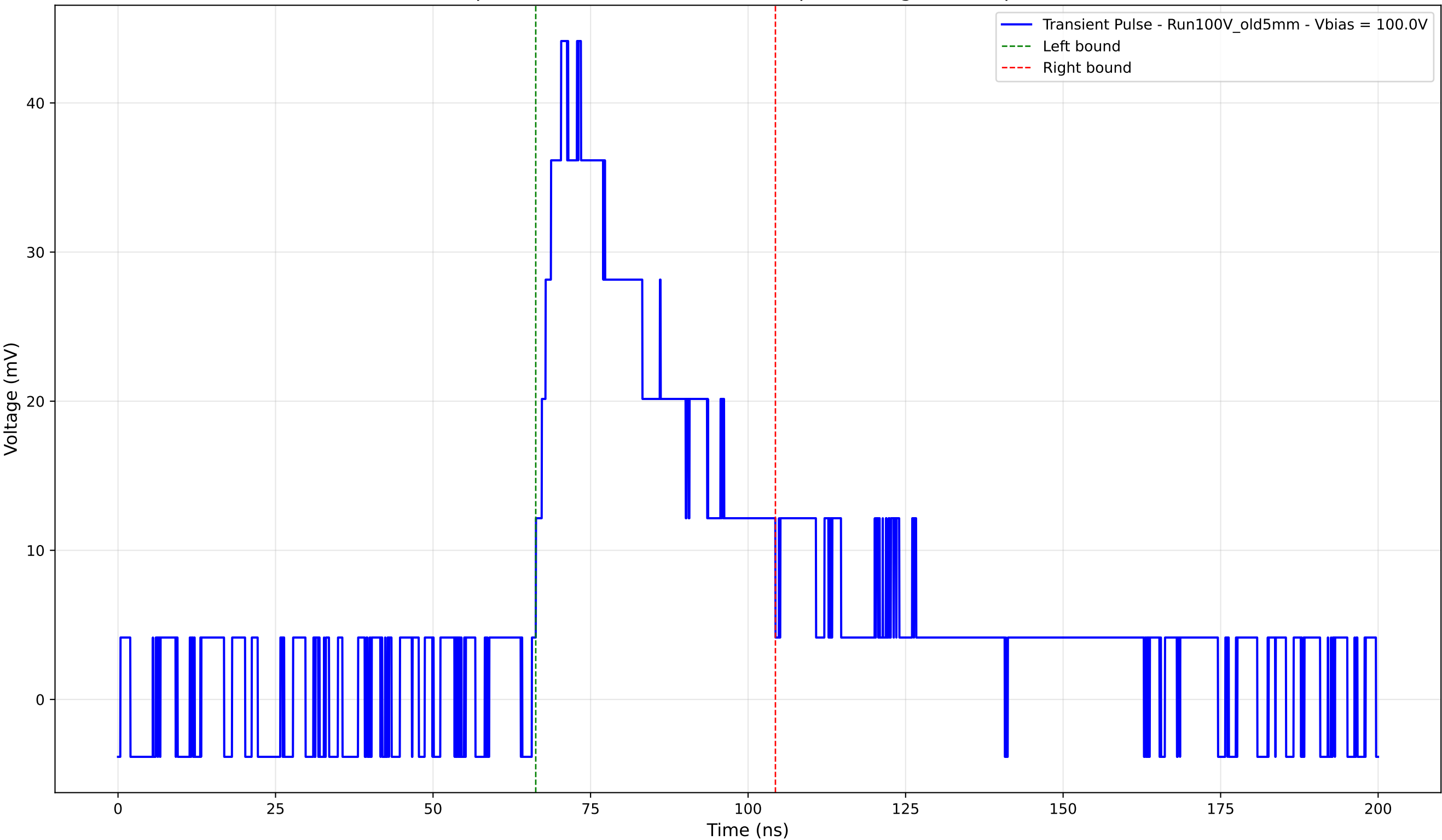
Transient Pulse - Sample: Old5mm - Position: 4920.0 \mu\text{m} - Charge: 17.57 pC - Rise Time: 4.02 ns
