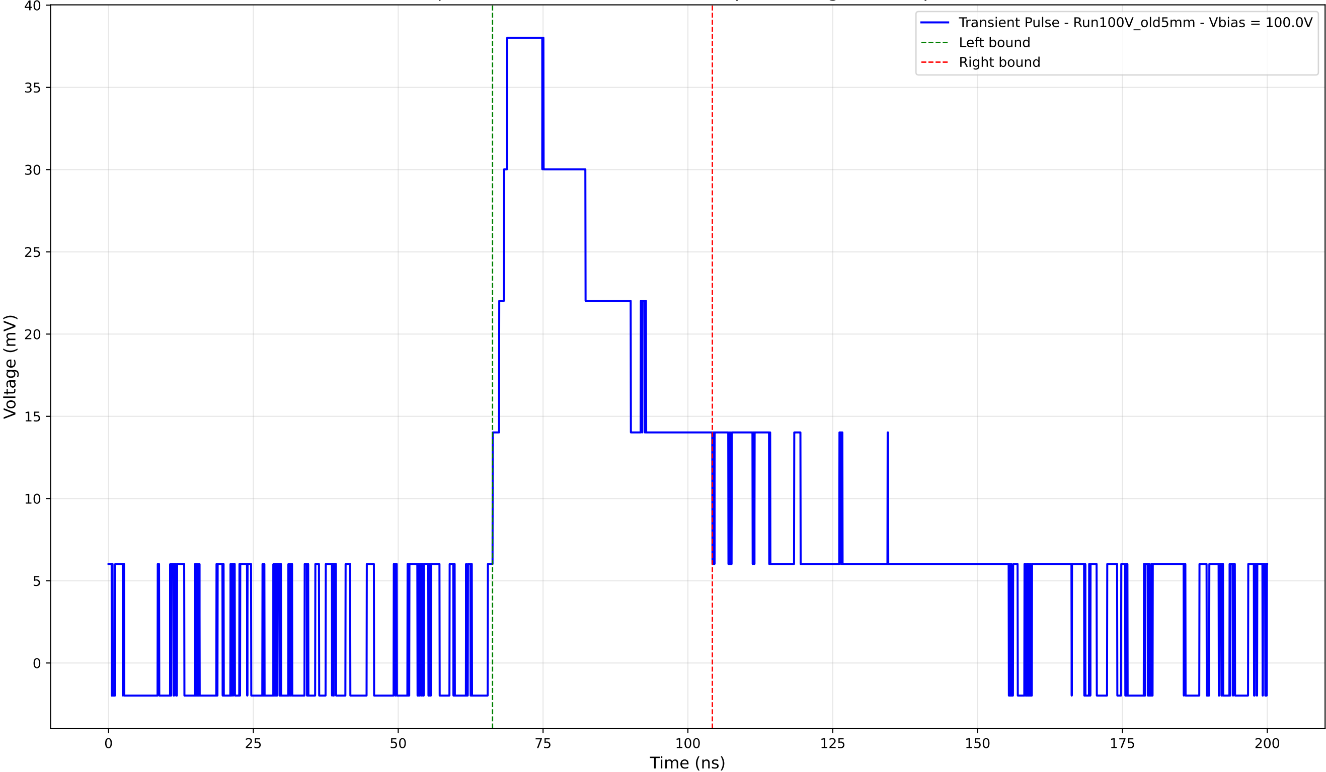
Transient Pulse - Sample: Old5mm - Position: 4945.0 \mu\text{m} - Charge: 17.64 pC - Rise Time: 3.35 ns
