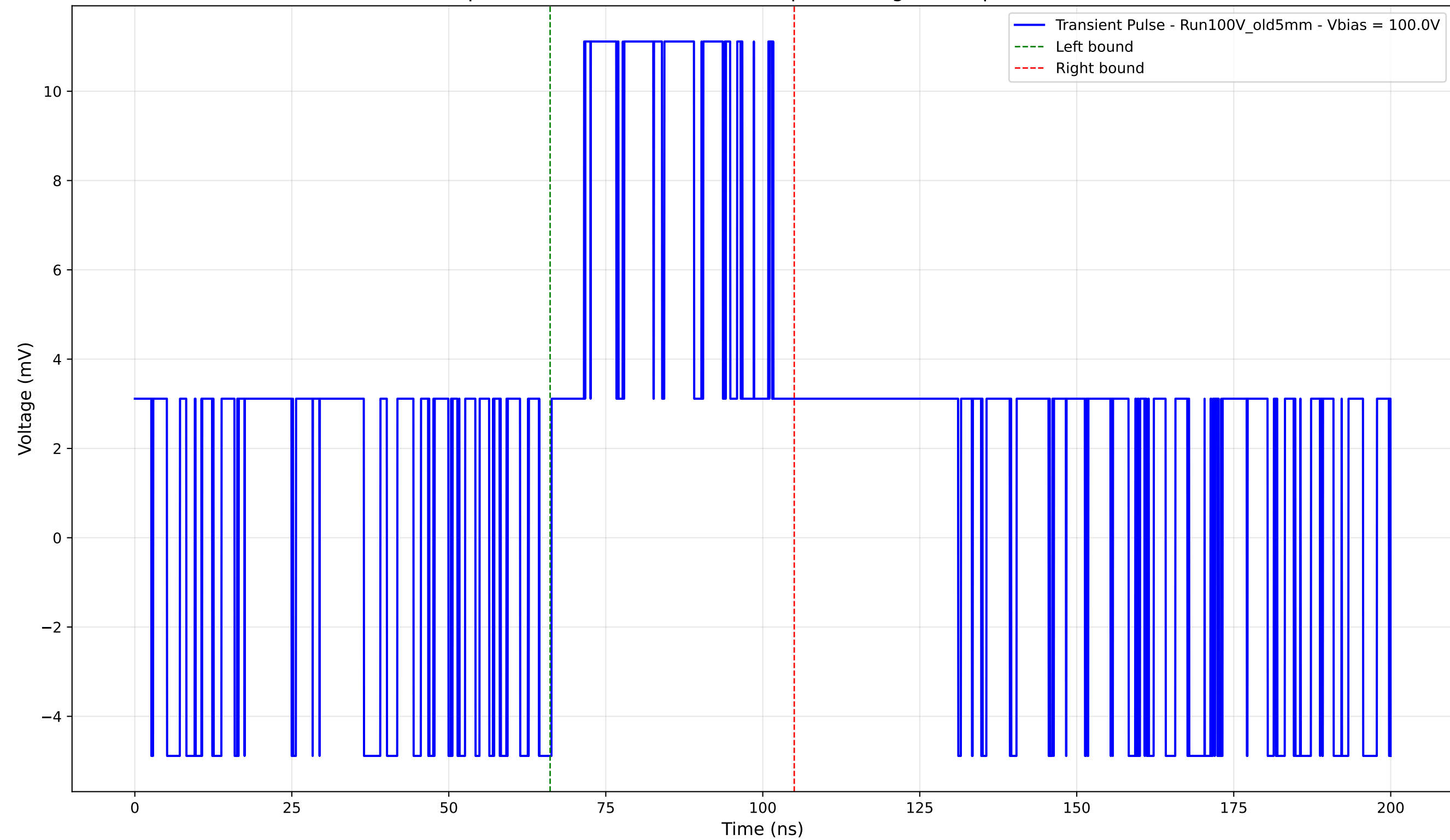
Transient Pulse - Sample: Old5mm - Position: 1365.0 \mu\text{m} - Charge: 5.78 pC - Rise Time: 0.00 ns (N/A)
