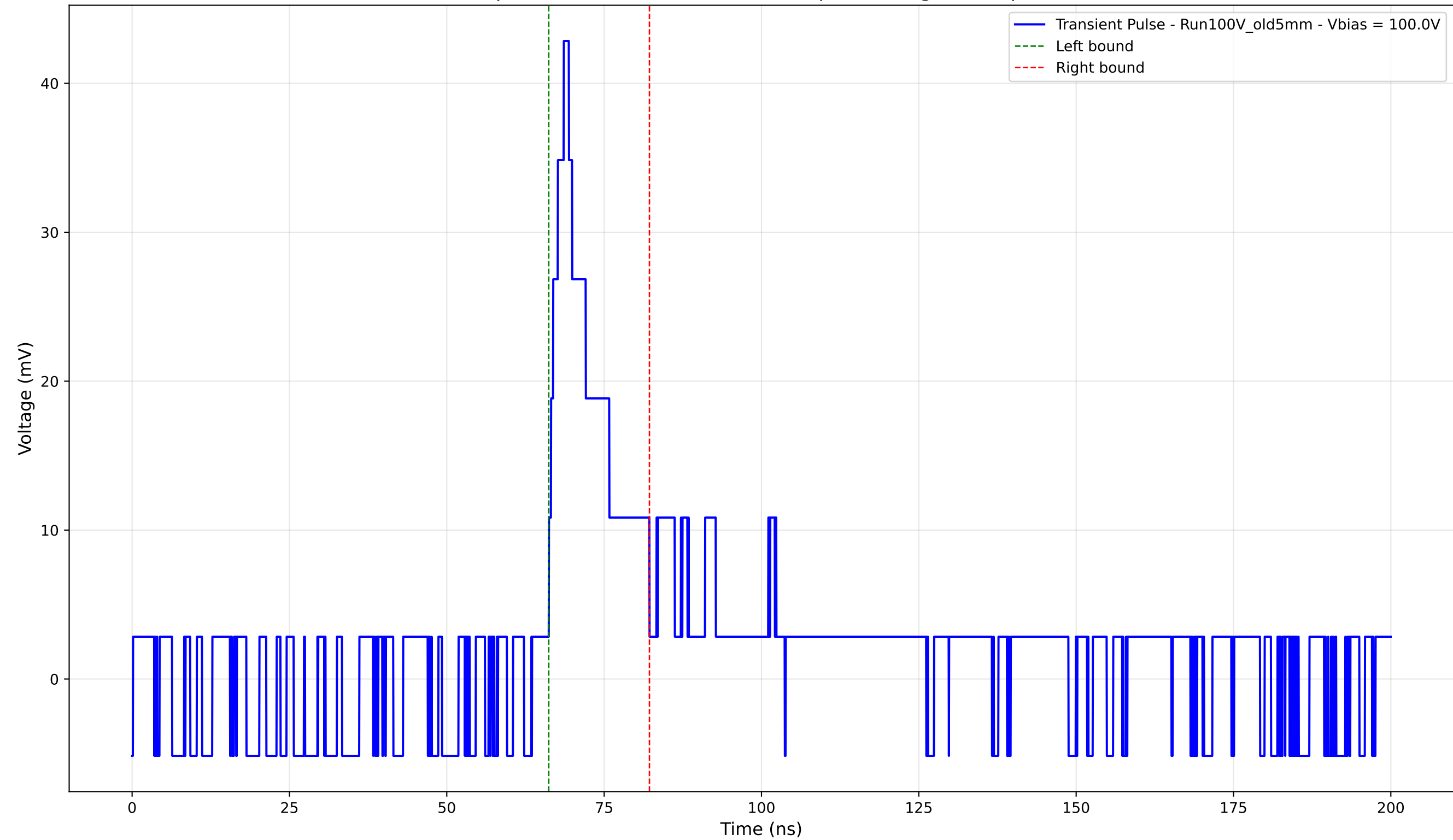
Transient Pulse - Sample: Old5mm - Position: 3030.0 \mu\text{m} - Charge: 6.27 pC - Rise Time: 2.38 ns
