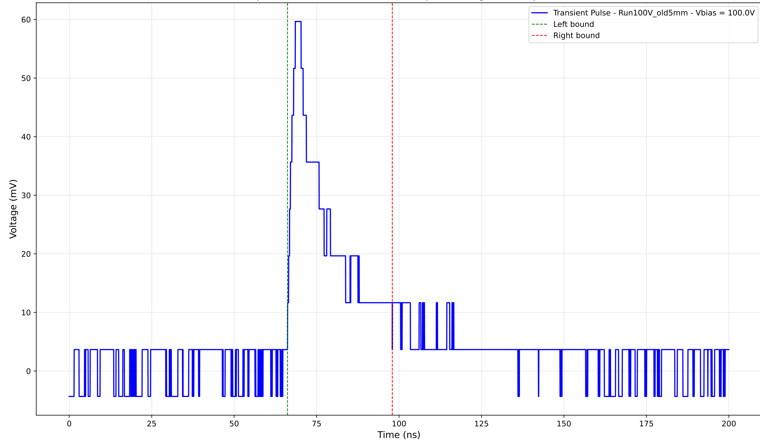
Transient Pulse - Sample: Old5mm - Position: 4510.0 \mu\text{m} - Charge: 15.25 pC - Rise Time: 2.35 ns
