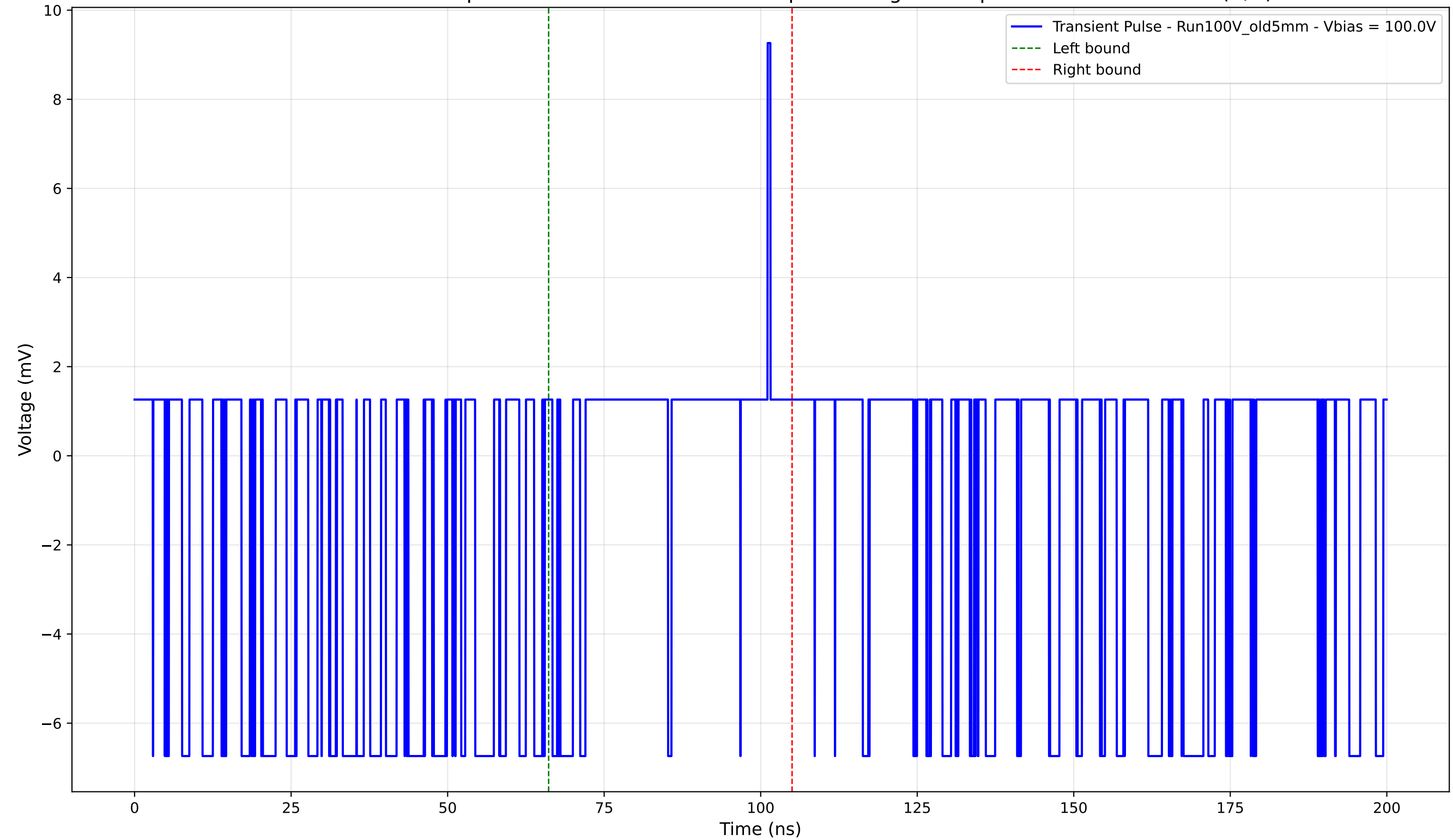
Transient Pulse - Sample: Old5mm - Position: 1320.0 \mu\text{m} - Charge: 0.34 pC - Rise Time: 0.00 ns (N/A)
