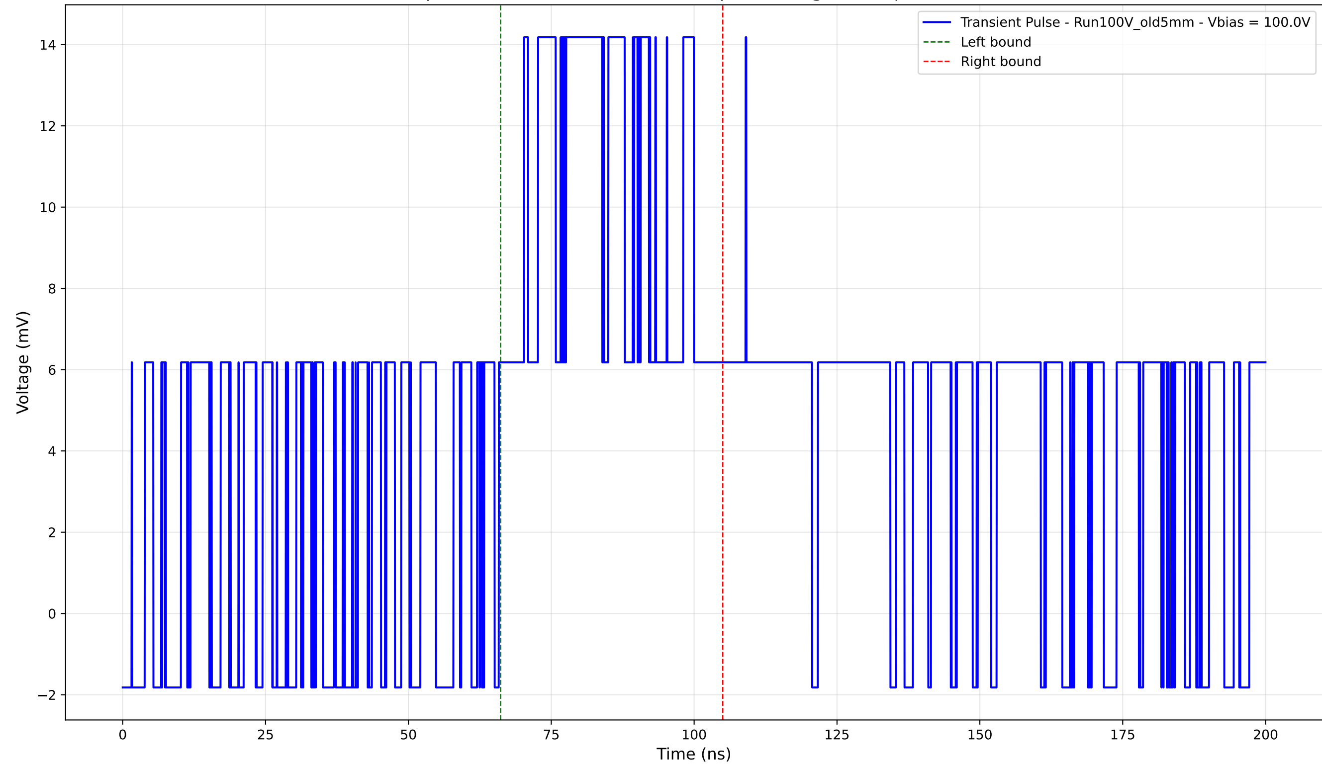
Transient Pulse - Sample: Old5mm - Position: 1760.0 \mu\text{m} - Charge: 7.73 pC - Rise Time: 0.00 ns (N/A)
