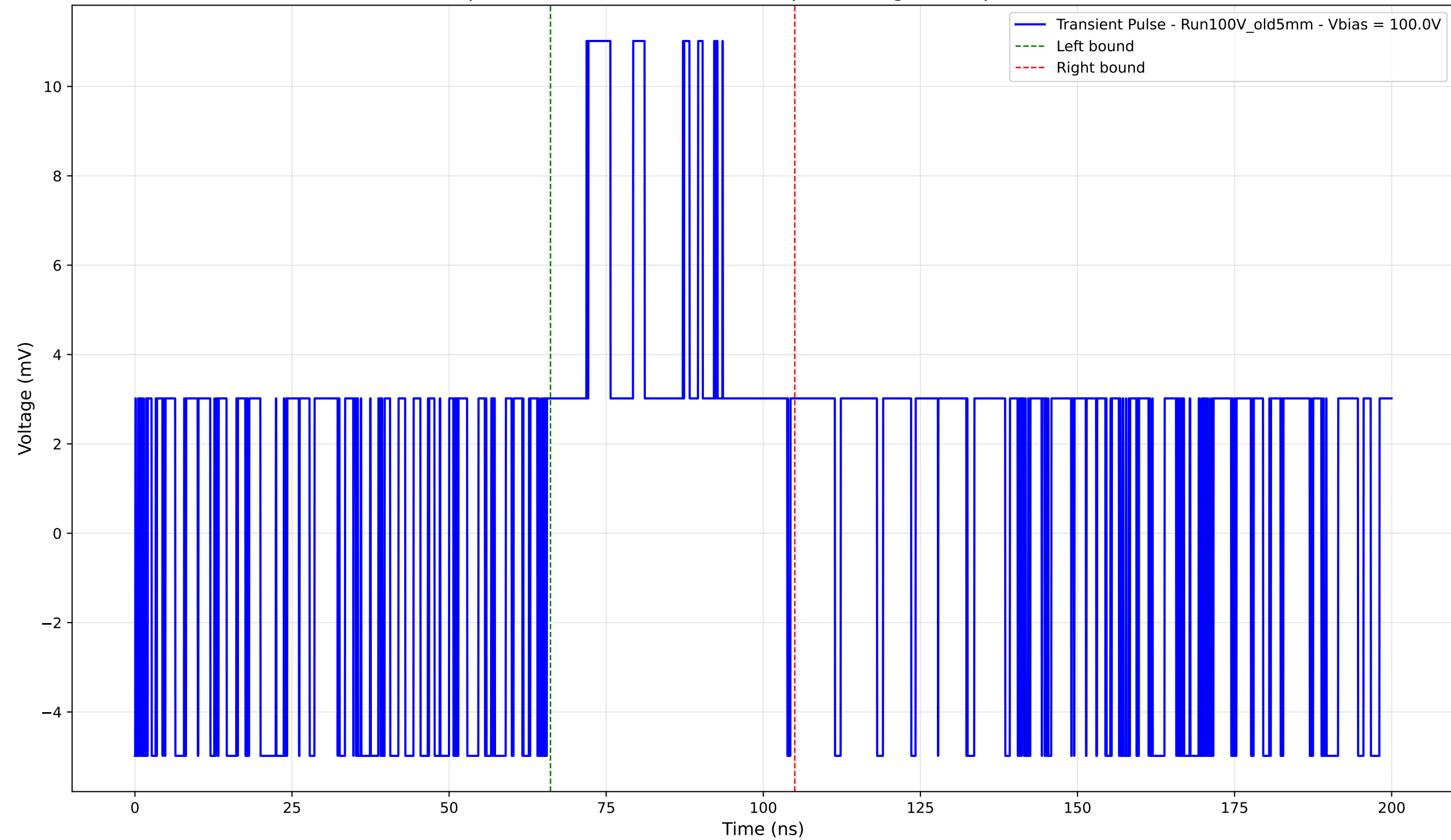
Transient Pulse - Sample: Old5mm - Position: 1045.0 \mu\text{m} - Charge: 3.49 pC - Rise Time: 0.00 ns (N/A)
