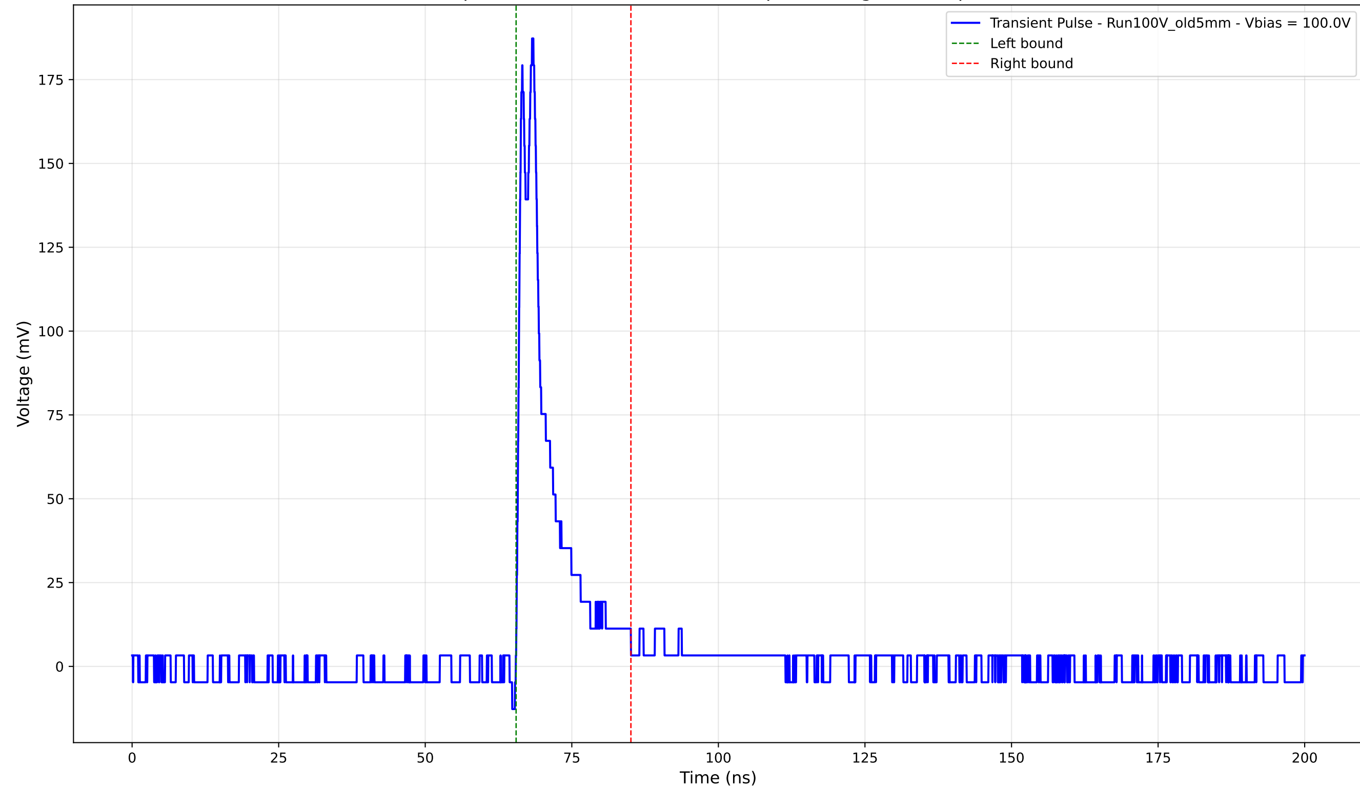
Transient Pulse - Sample: Old5mm - Position: 3545.0 \mu\text{m} - Charge: 20.13 pC - Rise Time: 0.80 ns
