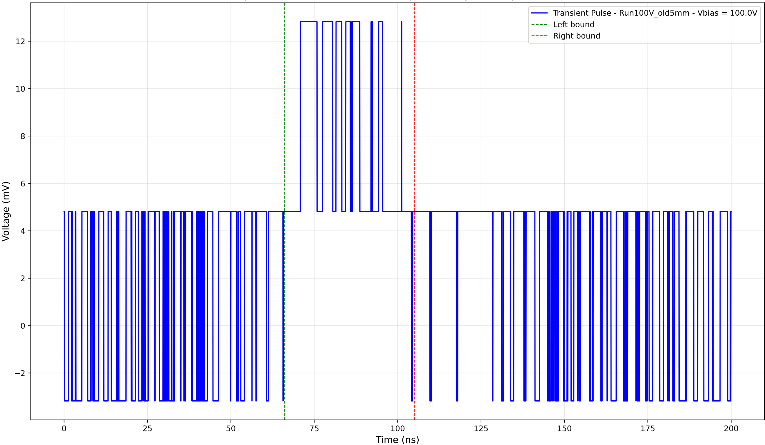
Transient Pulse - Sample: Old5mm - Position: 785.0 \mu\text{m} - Charge: 6.11 pC - Rise Time: 0.00 ns (N/A)
