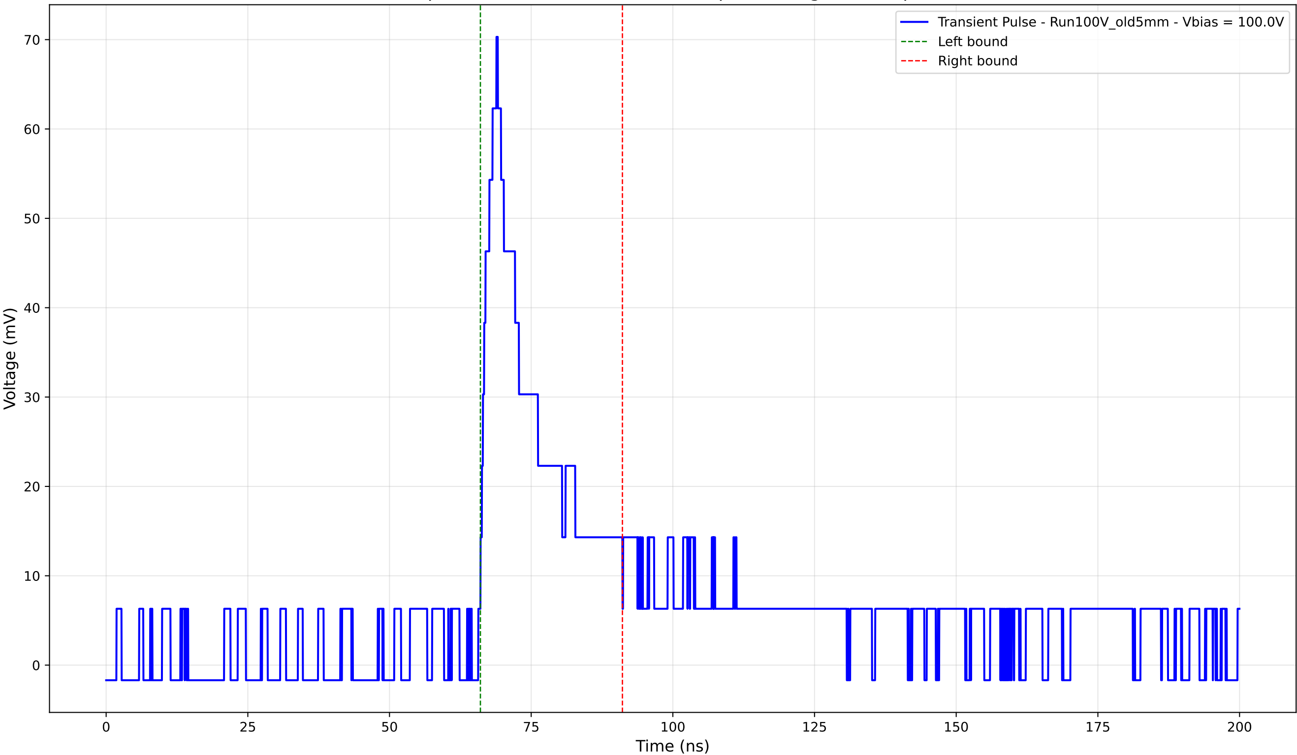
Transient Pulse - Sample: Old5mm - Position: 4410.0 \mu\text{m} - Charge: 13.77 pC - Rise Time: 2.82 ns
