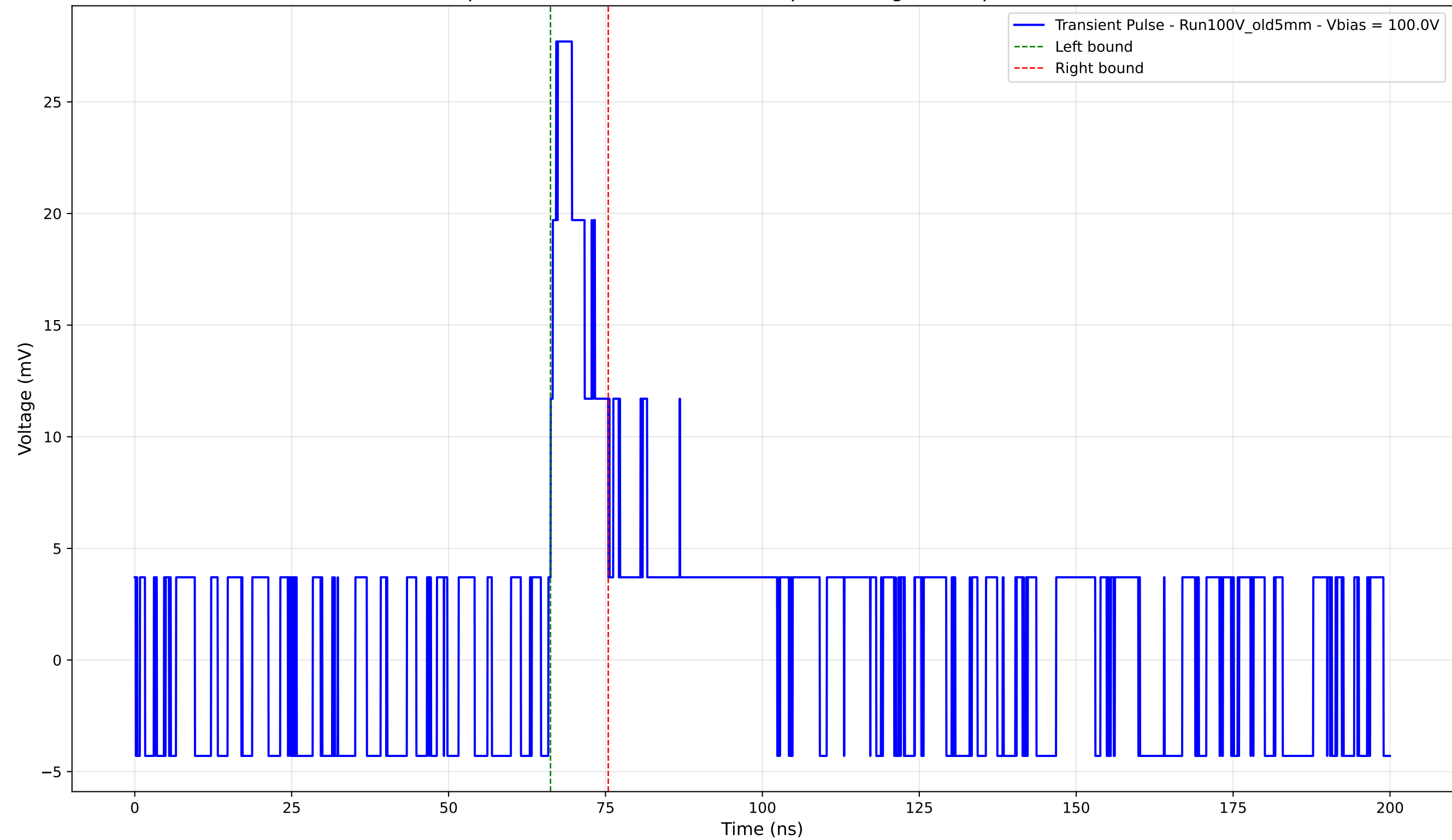
Transient Pulse - Sample: Old5mm - Position: 4250.0 \mu\text{m} - Charge: 3.39 pC - Rise Time: 0.00 ns (N/A)
