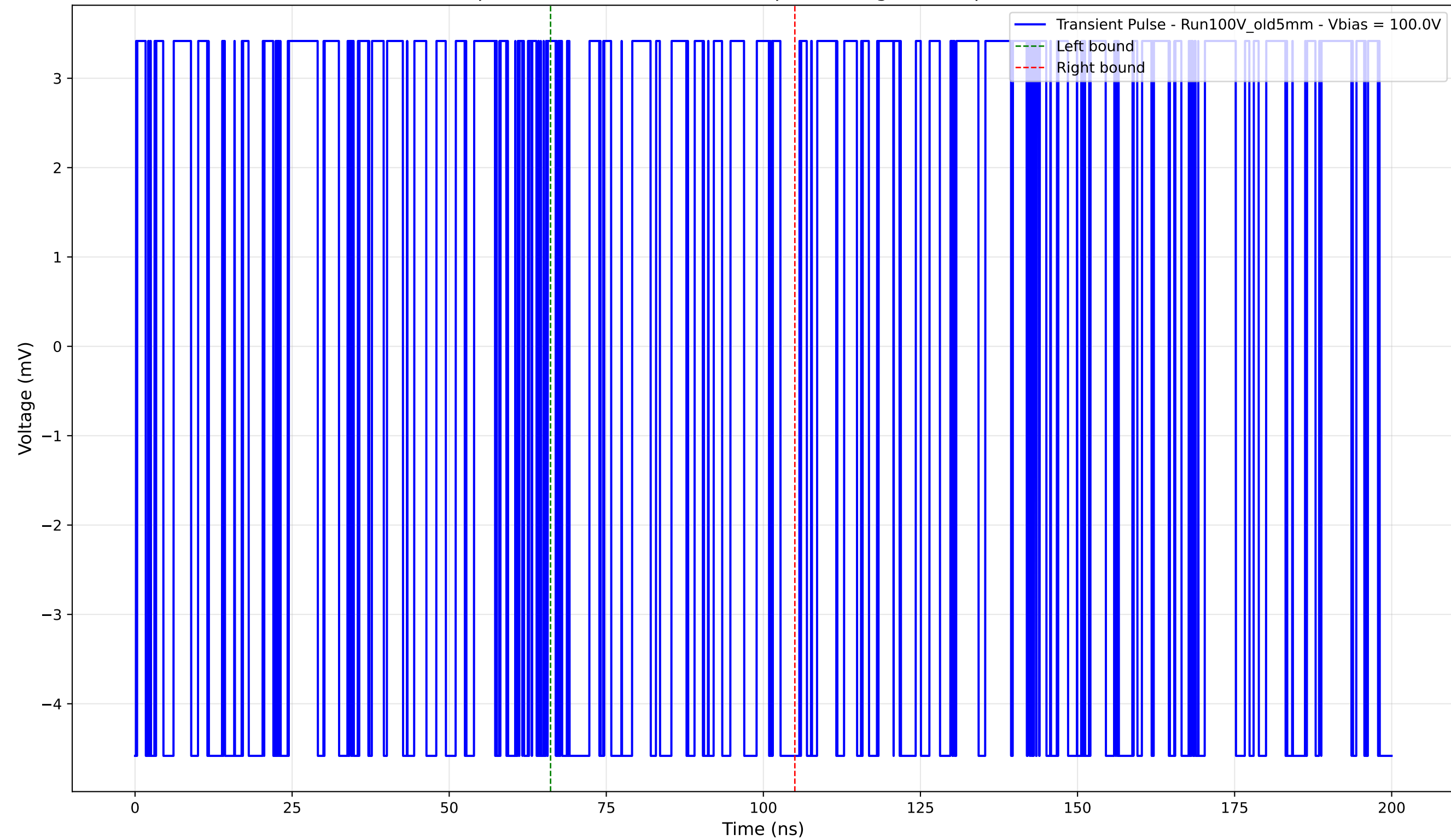
Transient Pulse - Sample: Old5mm - Position: 85.0 \mu\text{m} - Charge: -0.53 pC - Rise Time: 0.00 ns (N/A)
