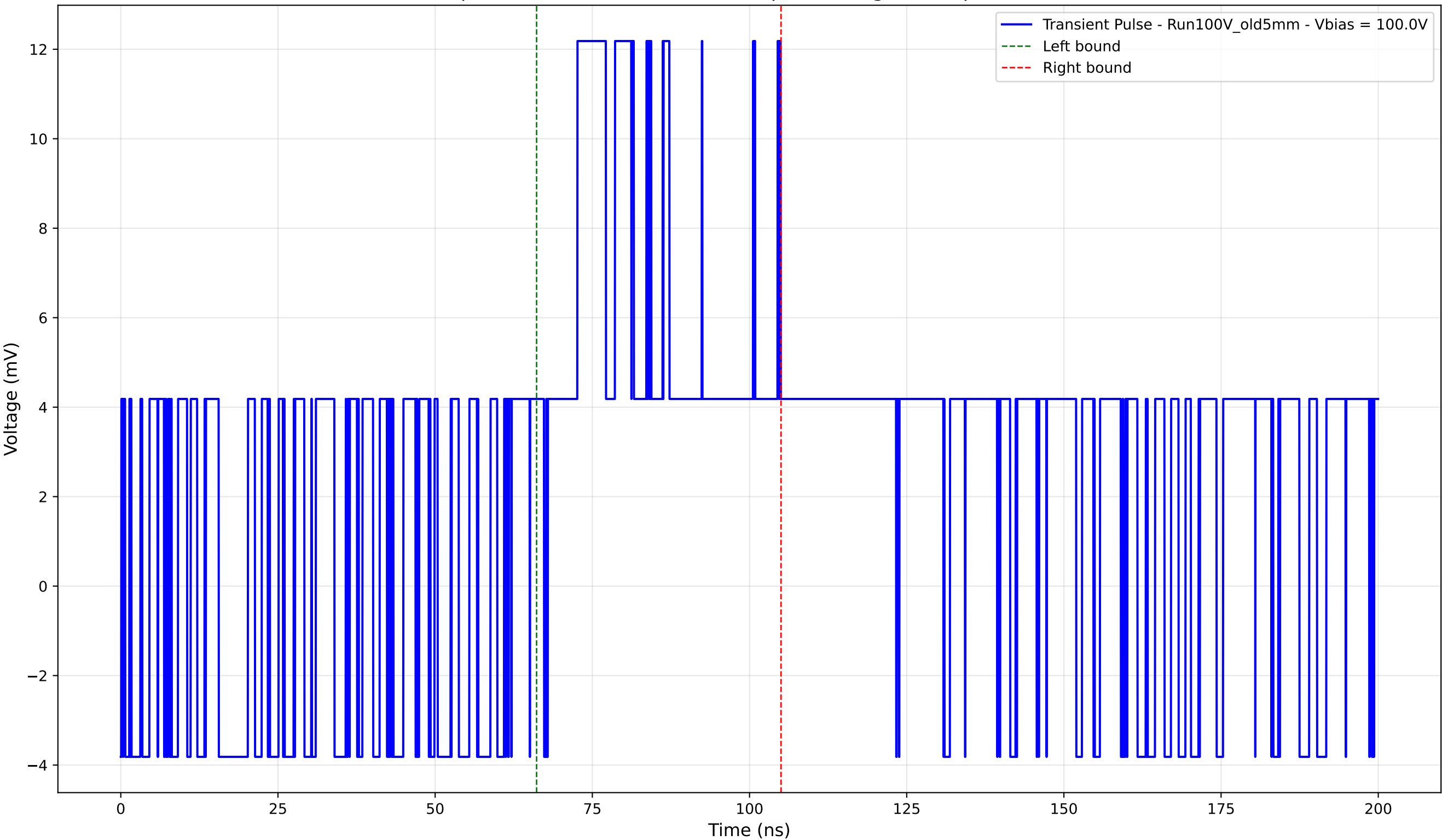
Transient Pulse - Sample: Old5mm - Position: 955.0 \mu\text{m} - Charge: 4.73 pC - Rise Time: 0.00 ns (N/A)
