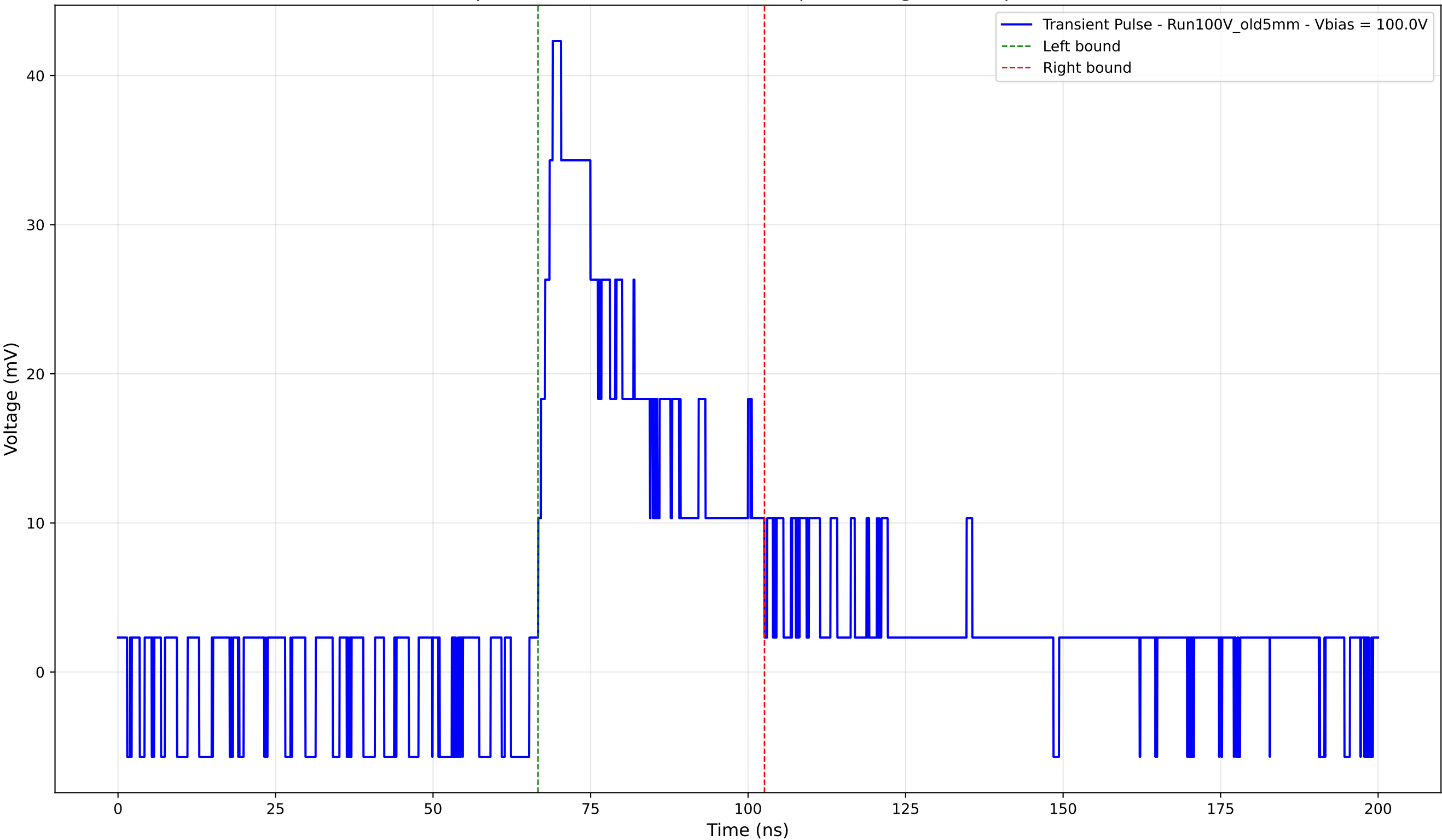
Transient Pulse - Sample: Old5mm - Position: 2625.0 \mu\text{m} - Charge: 14.06 pC - Rise Time: 2.32 ns
