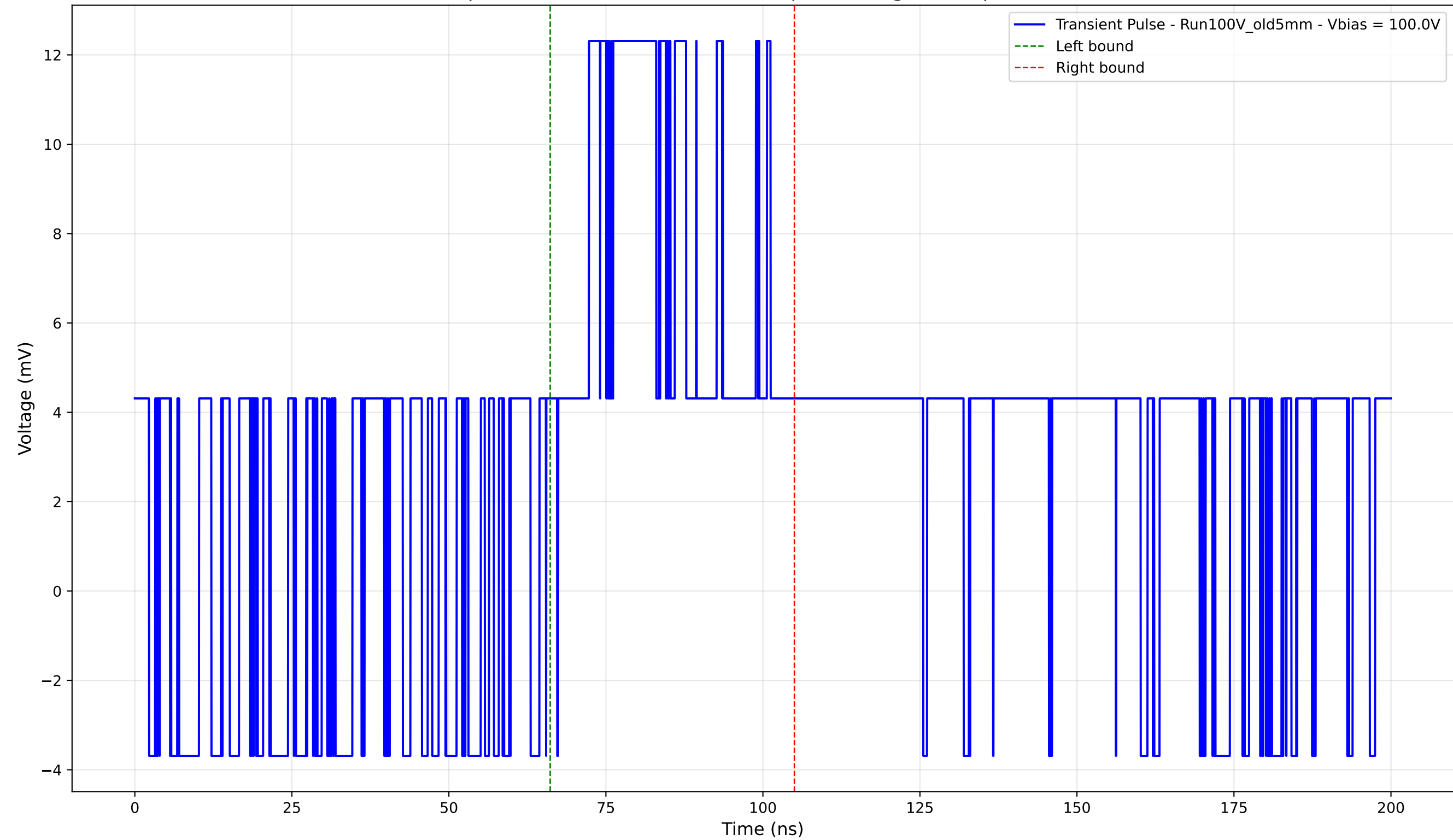
Transient Pulse - Sample: Old5mm - Position: 1155.0 \mu\text{m} - Charge: 5.78 pC - Rise Time: 0.00 ns (N/A)
