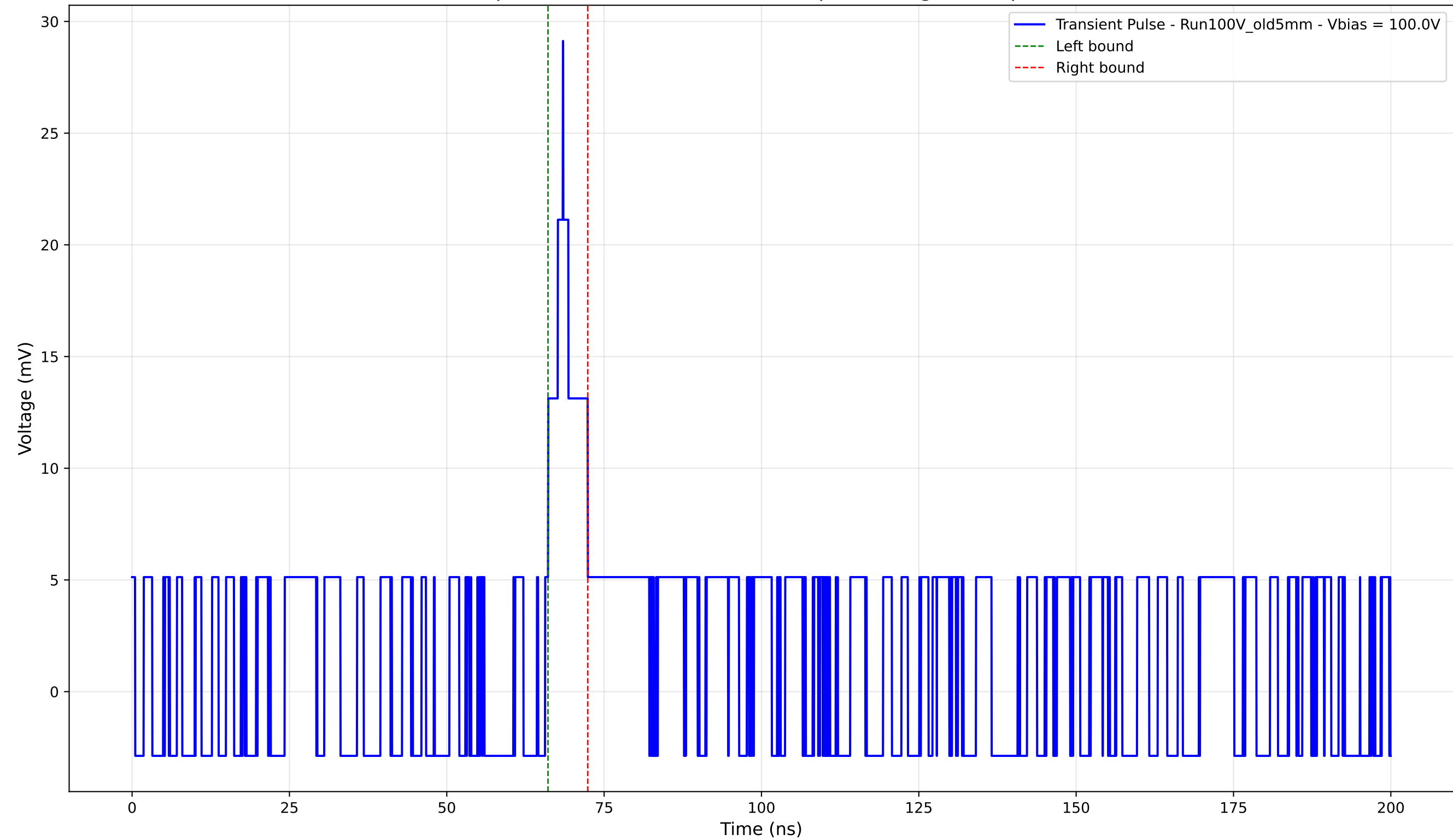
Transient Pulse - Sample: Old5mm - Position: 4050.0 \mu\text{m} - Charge: 1.93 pC - Rise Time: 2.84 ns
