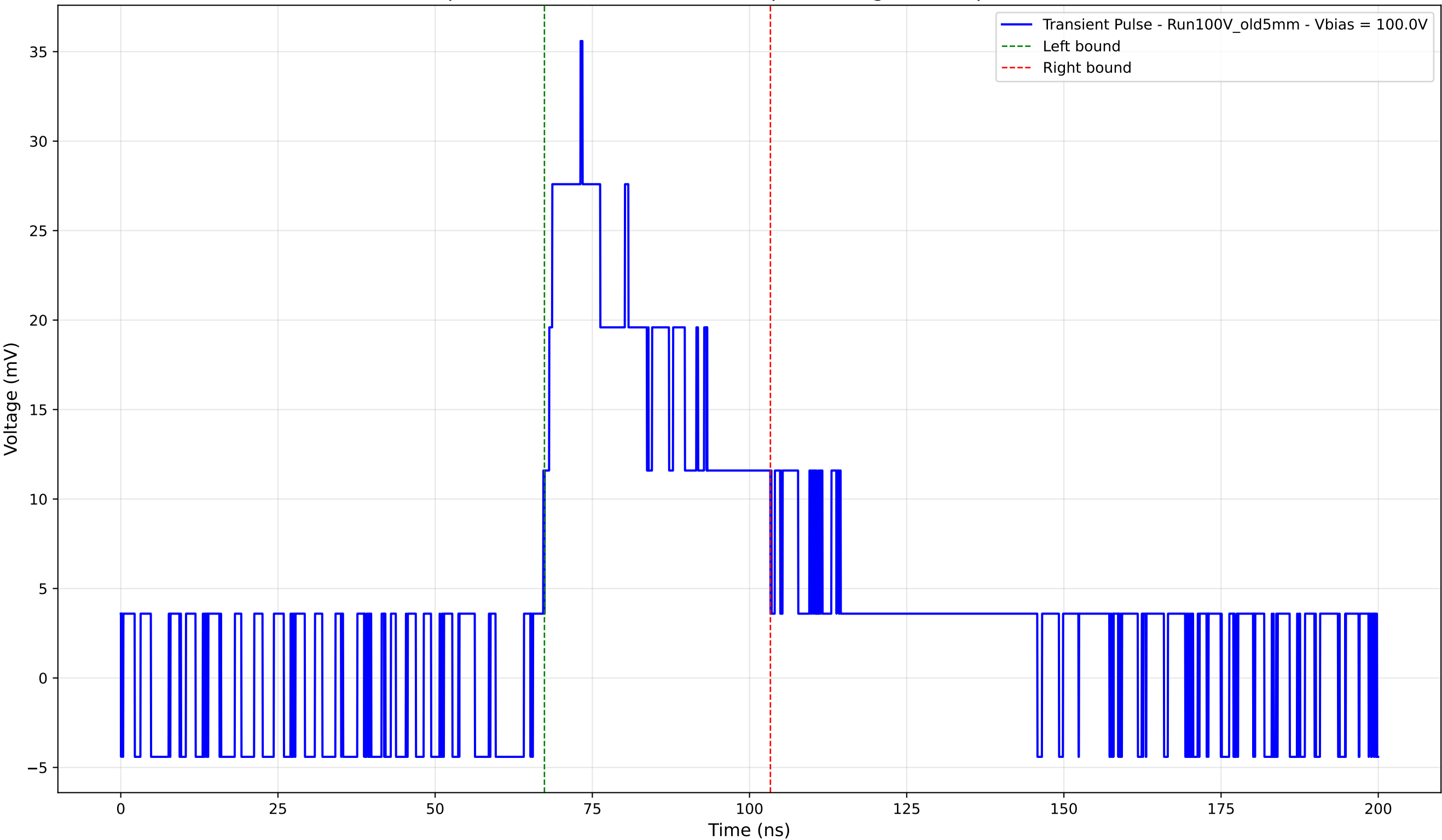
Transient Pulse - Sample: Old5mm - Position: 2420.0 \mu\text{m} - Charge: 13.04 pC - Rise Time: 0.00 ns (N/A)
