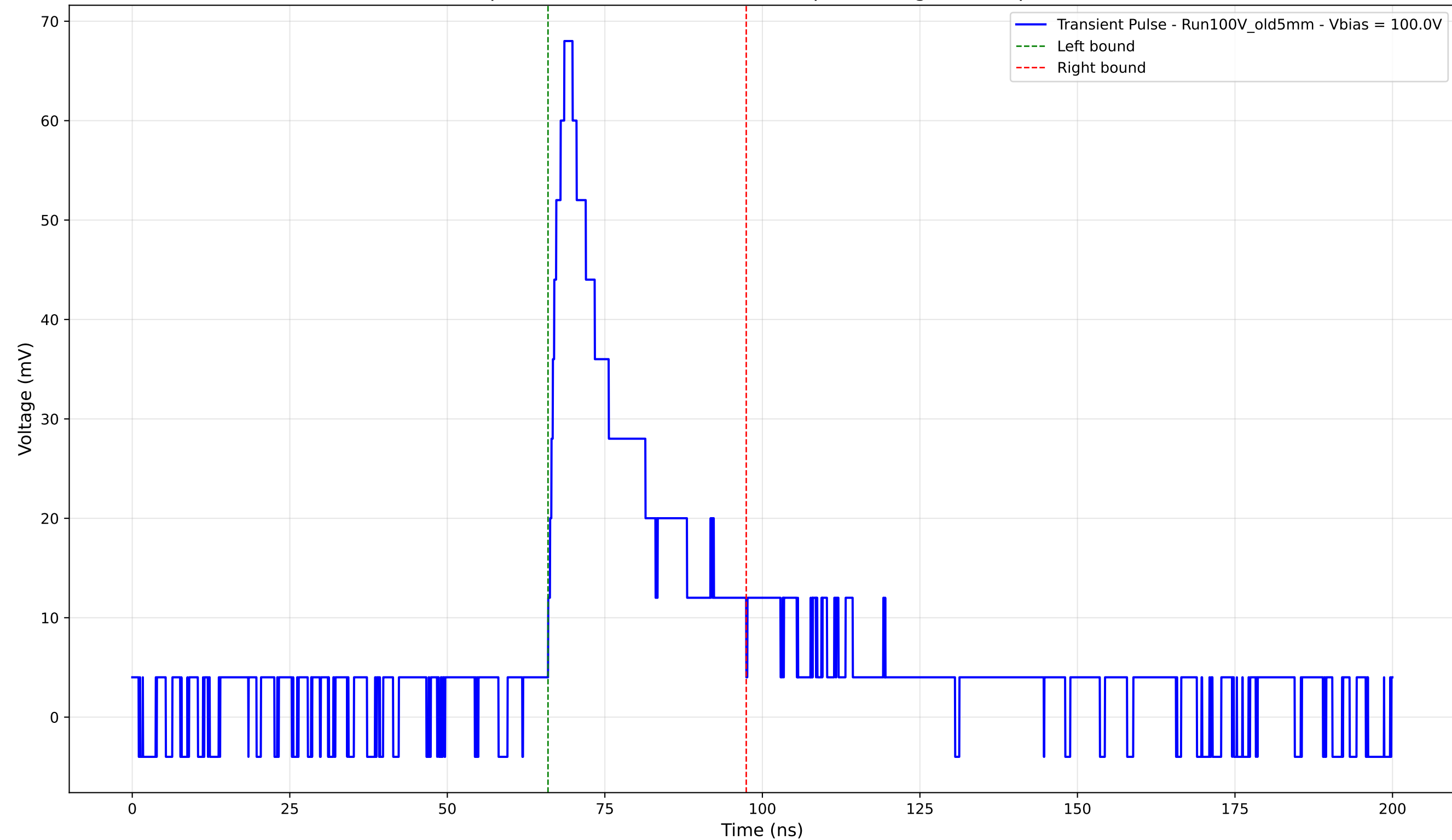
Transient Pulse - Sample: Old5mm - Position: 4485.0 \mu\text{m} - Charge: 17.26 pC - Rise Time: 2.57 ns
