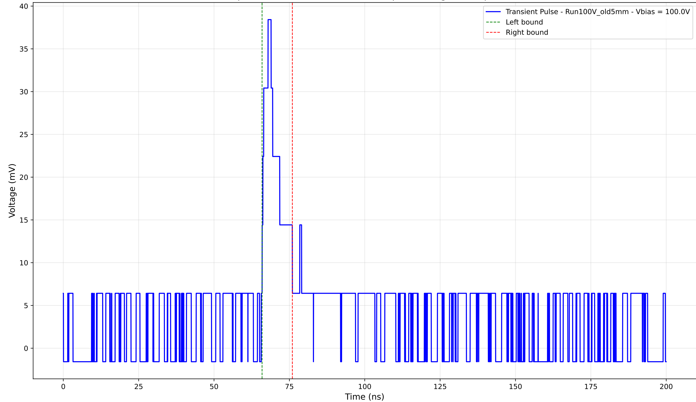
Transient Pulse - Sample: Old5mm - Position: 4060.0 \mu\text{m} - Charge: 4.43 pC - Rise Time: 2.27 ns
