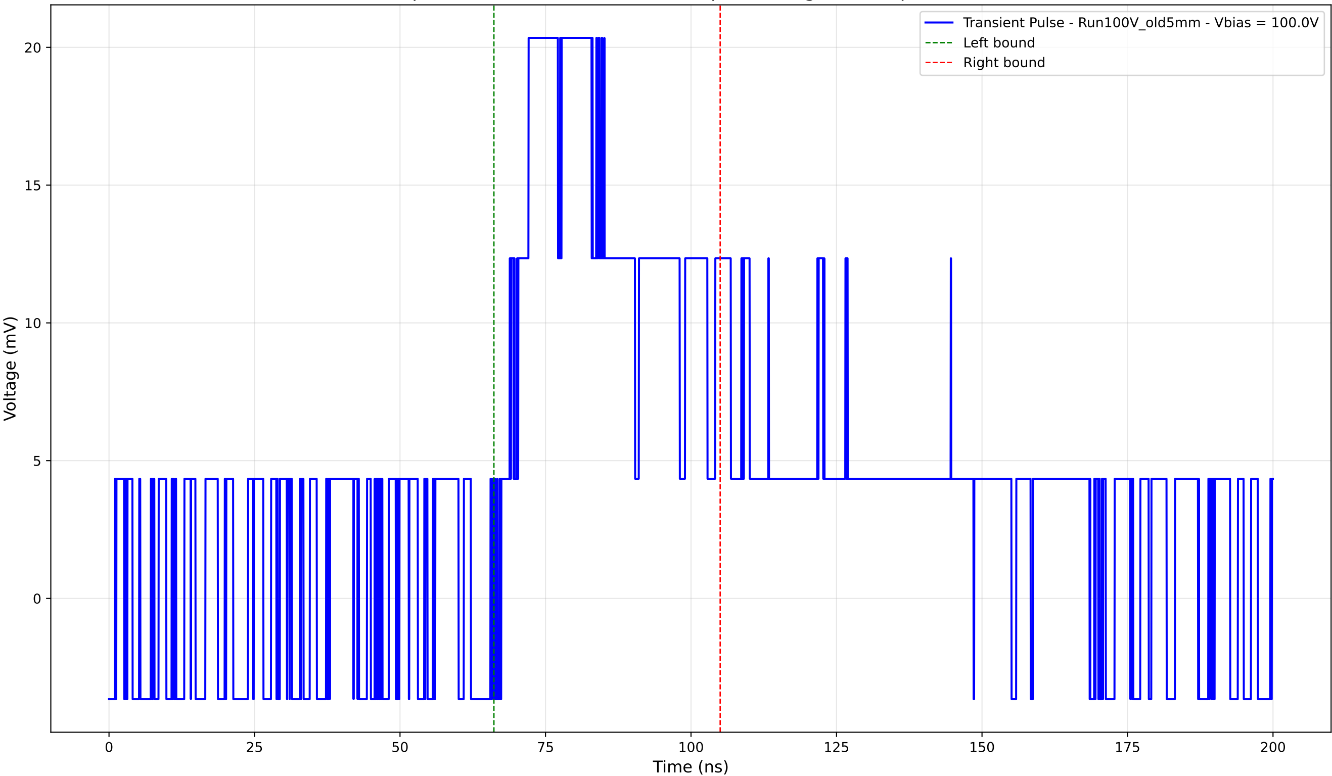
Transient Pulse - Sample: Old5mm - Position: 1805.0 \mu\text{m} - Charge: 10.18 pC - Rise Time: 0.00 ns (N/A)
