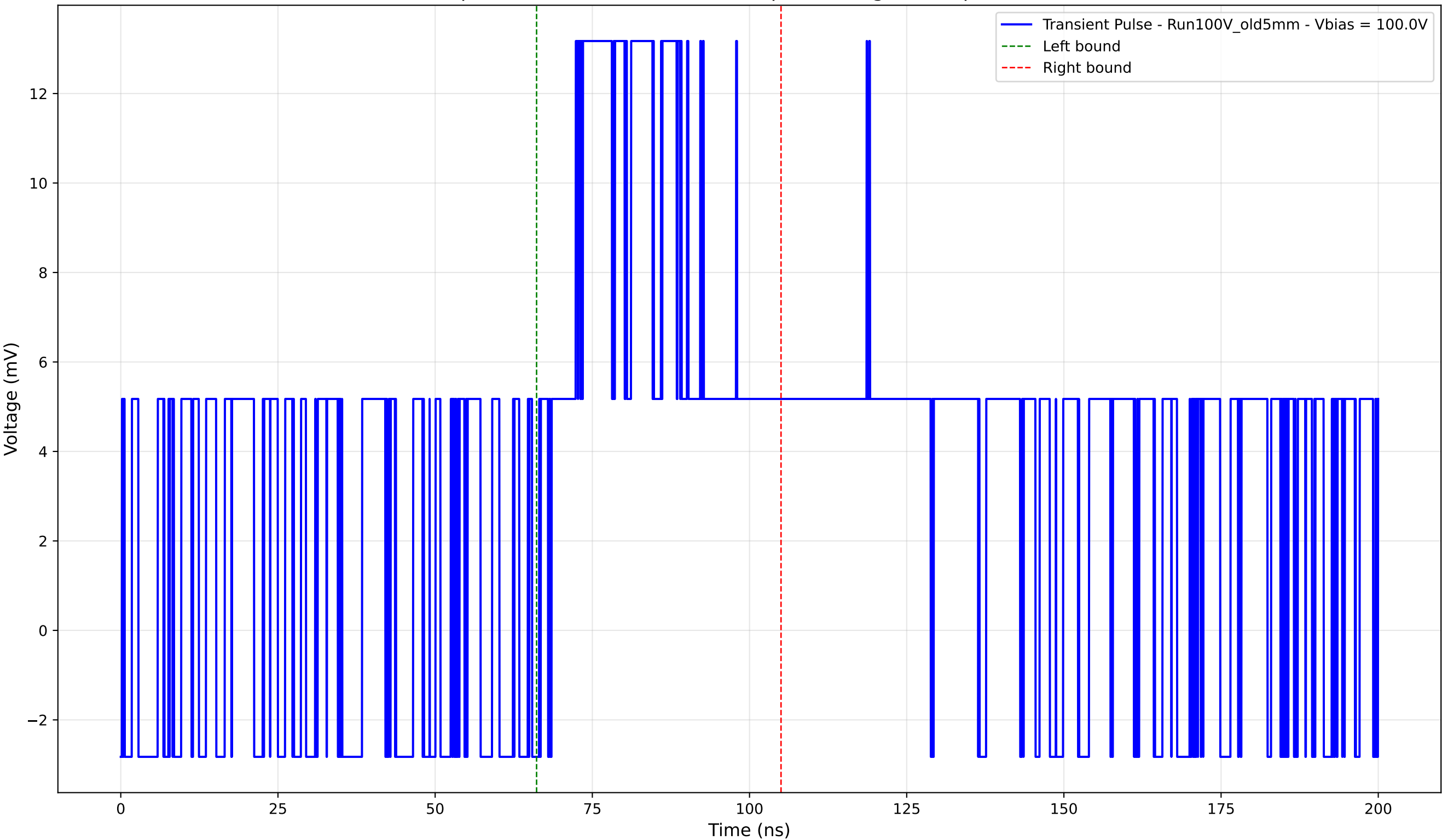
Transient Pulse - Sample: Old5mm - Position: 995.0 \mu\text{m} - Charge: 6.19 pC - Rise Time: 0.00 ns (N/A)
