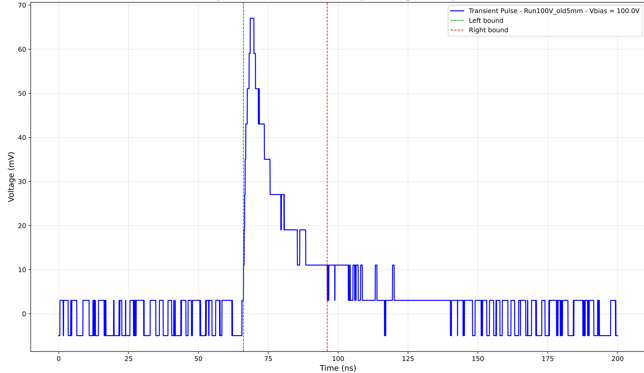
Transient Pulse - Sample: Old5mm - Position: 2950.0 \mu\text{m} - Charge: 15.99 pC - Rise Time: 2.43 ns
