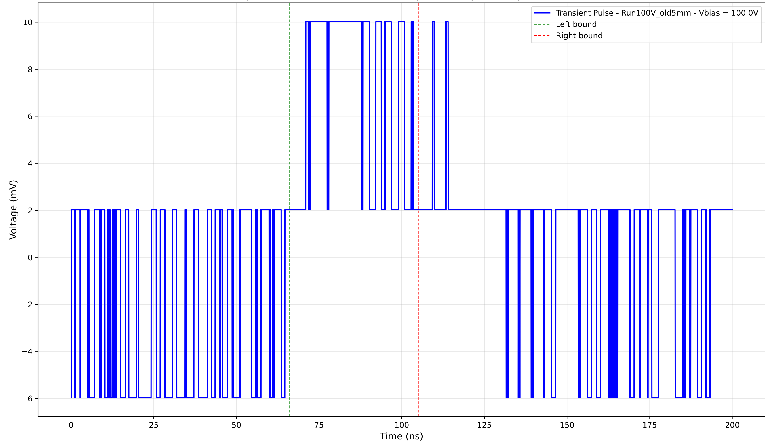
Transient Pulse - Sample: Old5mm - Position: 1080.0 \mu\text{m} - Charge: 5.44 pC - Rise Time: 0.00 ns (N/A)
