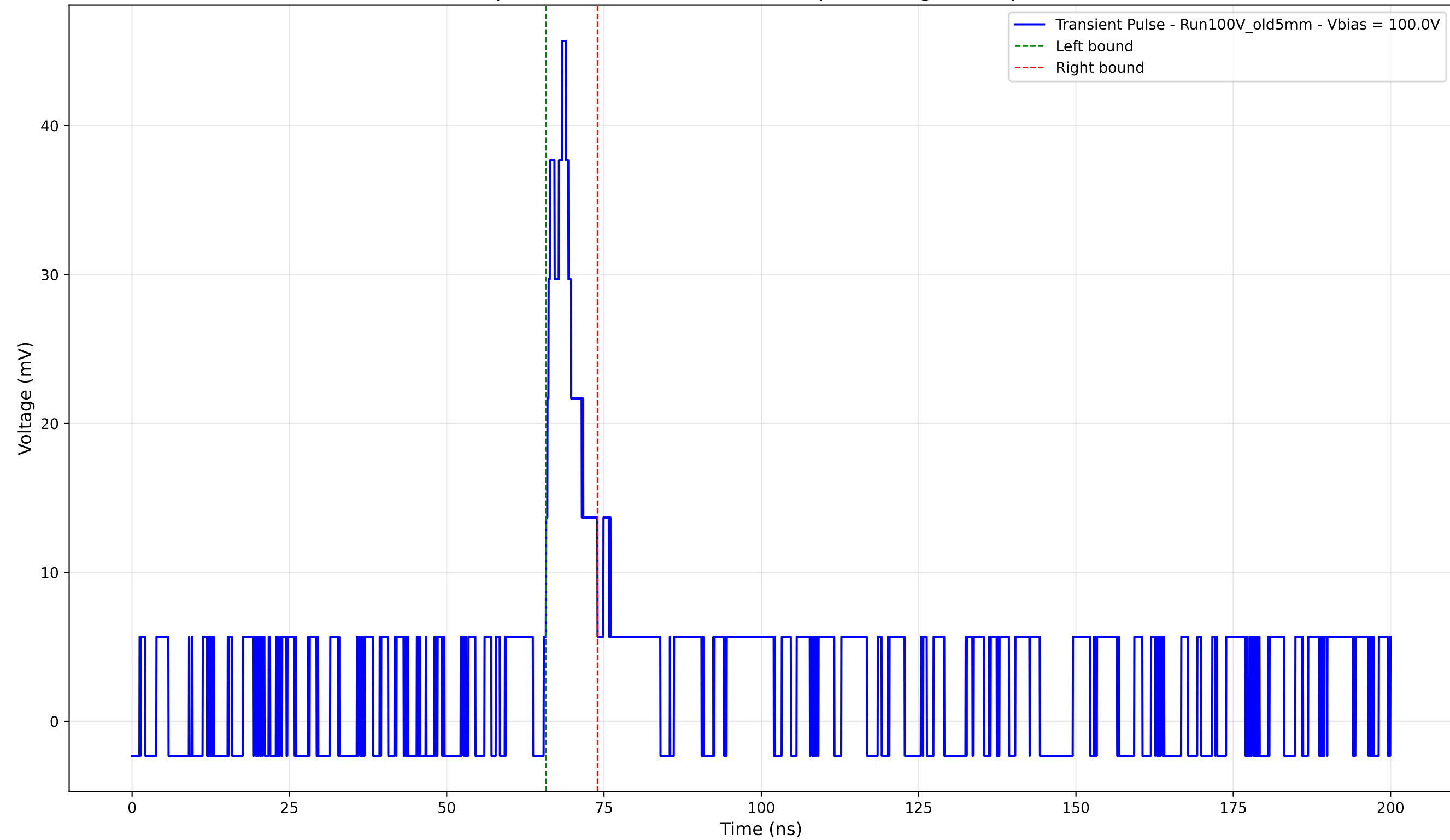
Transient Pulse - Sample: Old5mm - Position: 3455.0 \mu\text{m} - Charge: 4.15 pC - Rise Time: 2.95 ns
