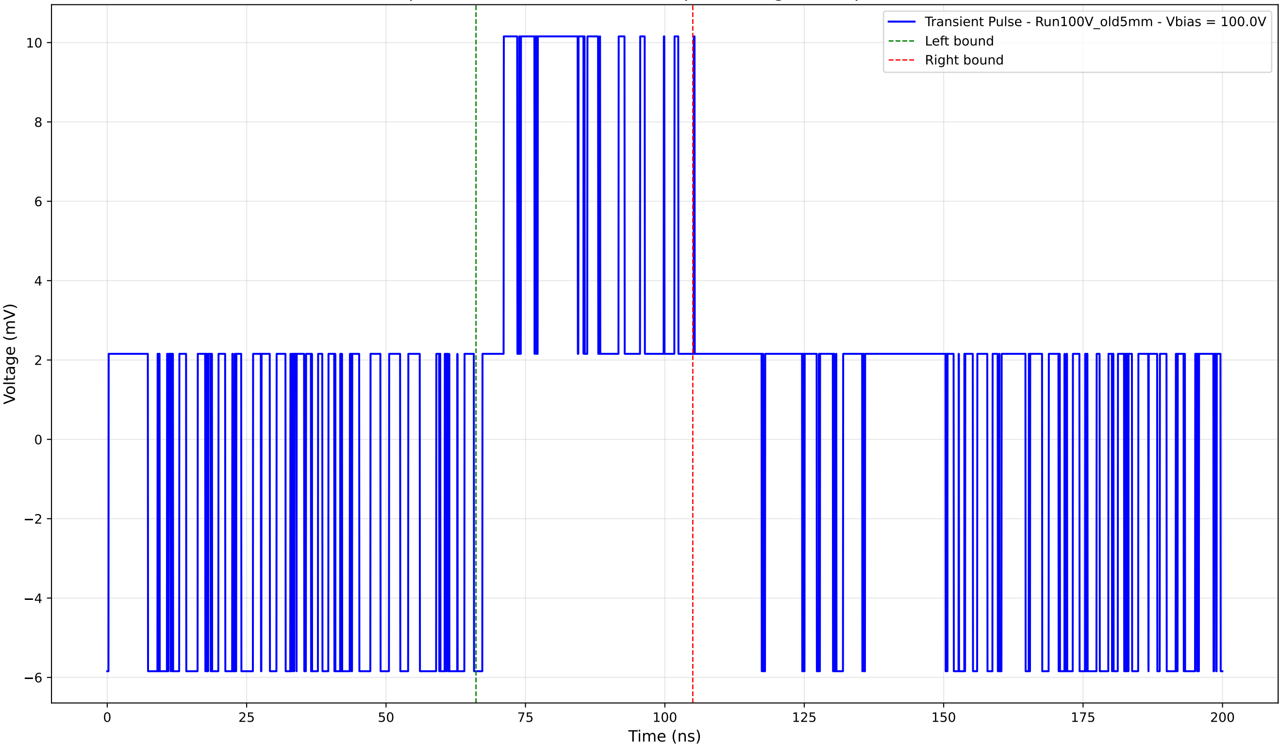
Transient Pulse - Sample: Old5mm - Position: 980.0 \mu\text{m} - Charge: 4.44 pC - Rise Time: 0.00 ns (N/A)
