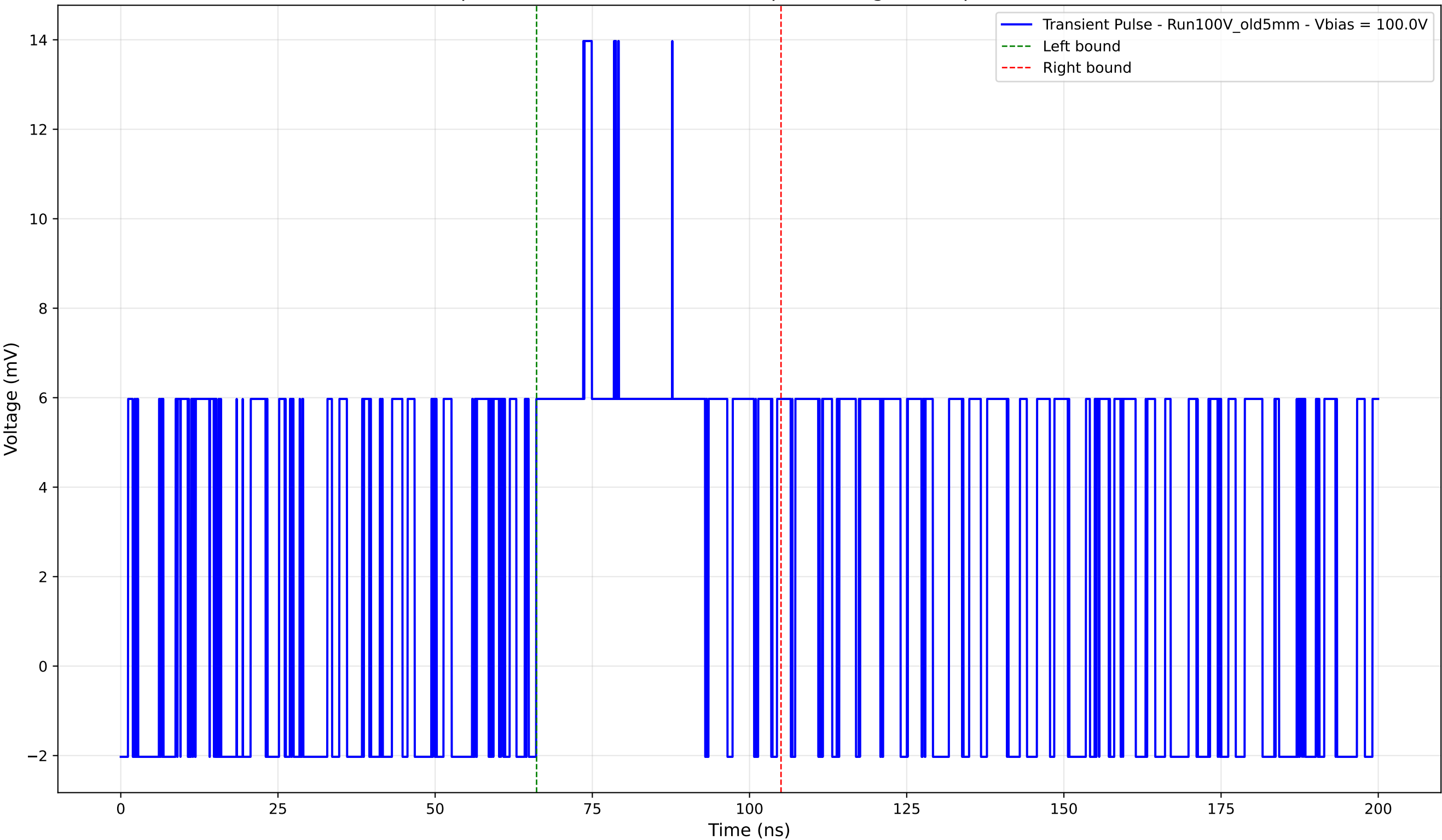
Transient Pulse - Sample: Old5mm - Position: 510.0 \mu\text{m} - Charge: 4.46 pC - Rise Time: 0.00 ns (N/A)
