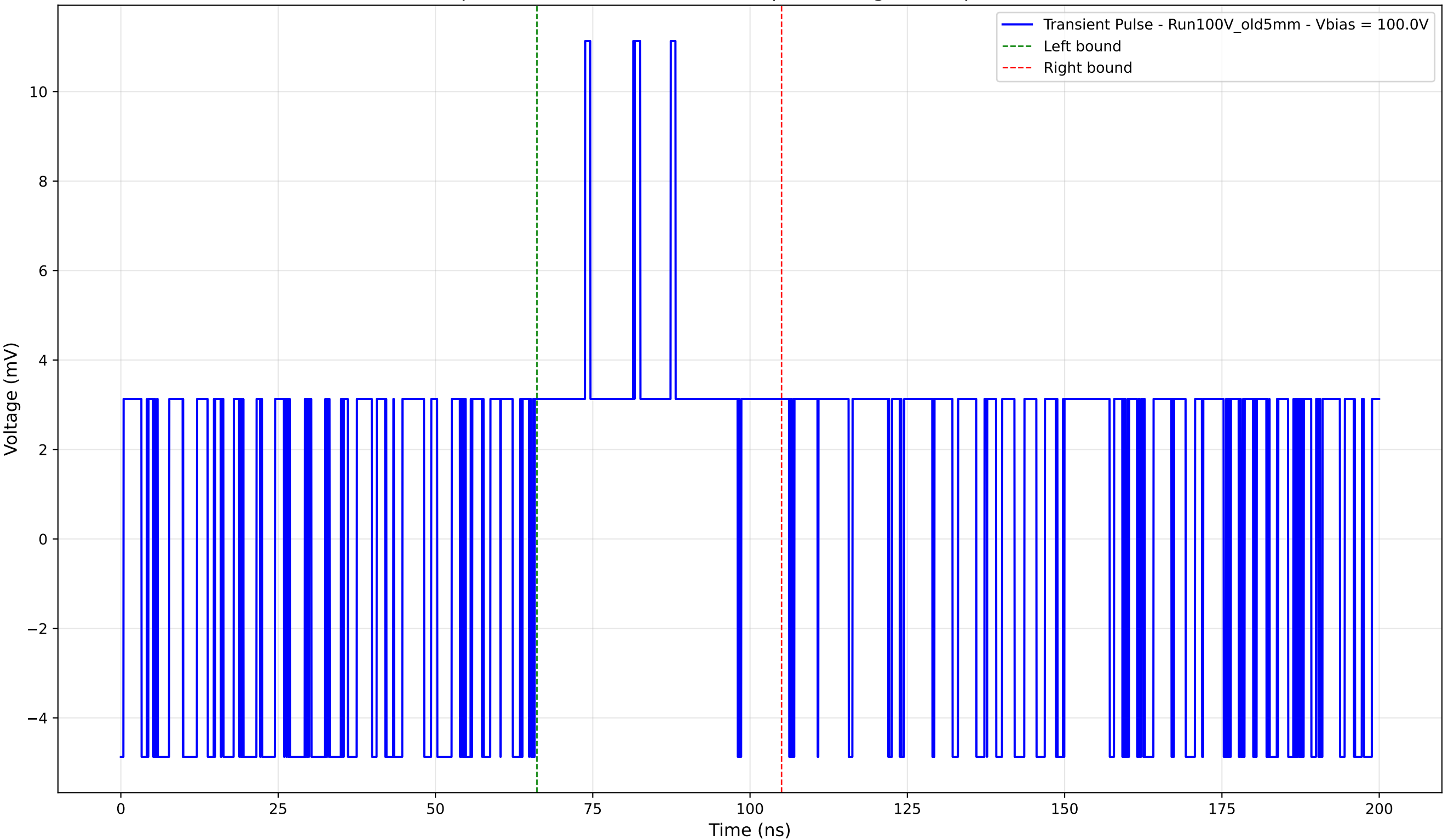
Transient Pulse - Sample: Old5mm - Position: 720.0 \mu\text{m} - Charge: 2.80 pC - Rise Time: 0.00 ns (N/A)
