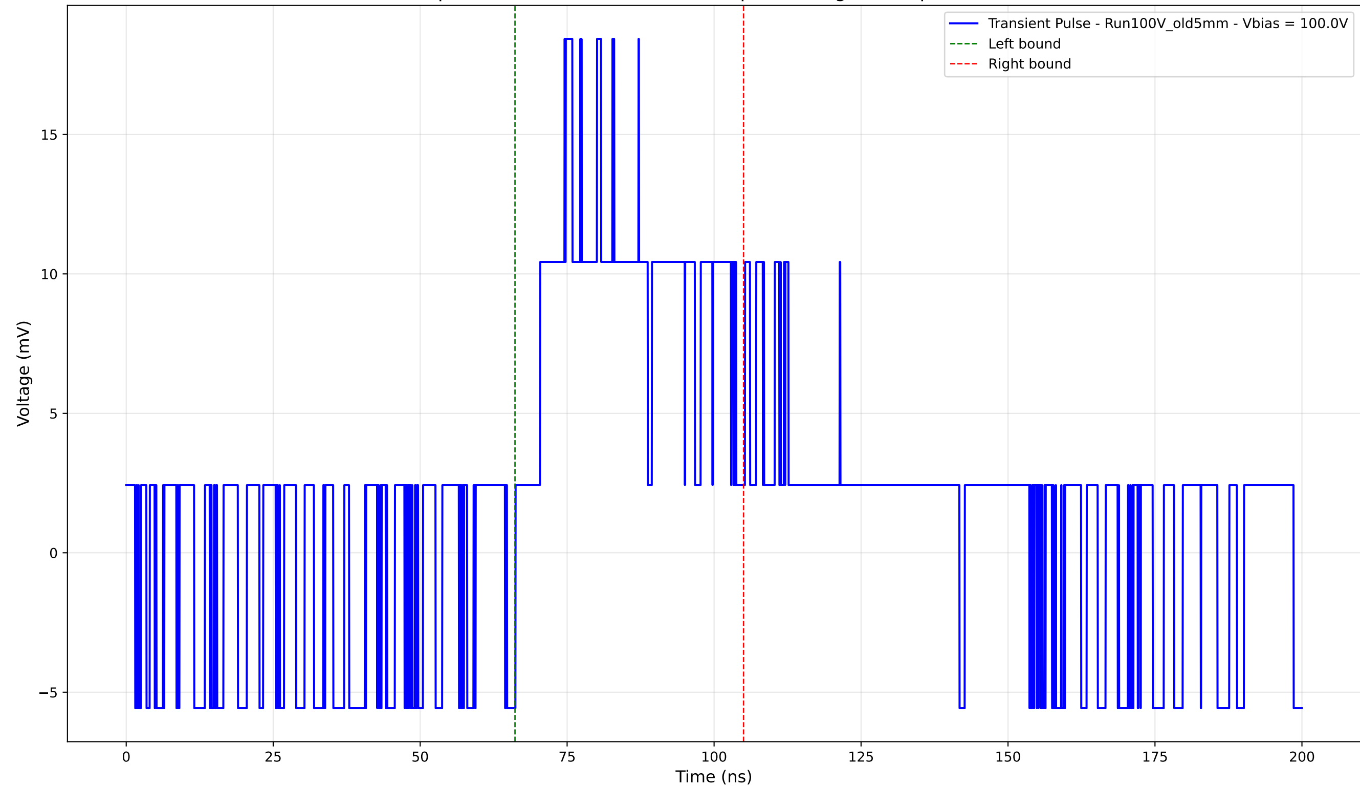
Transient Pulse - Sample: Old5mm - Position: 1180.0 \mu\text{m} - Charge: 7.24 pC - Rise Time: 0.00 ns (N/A)
