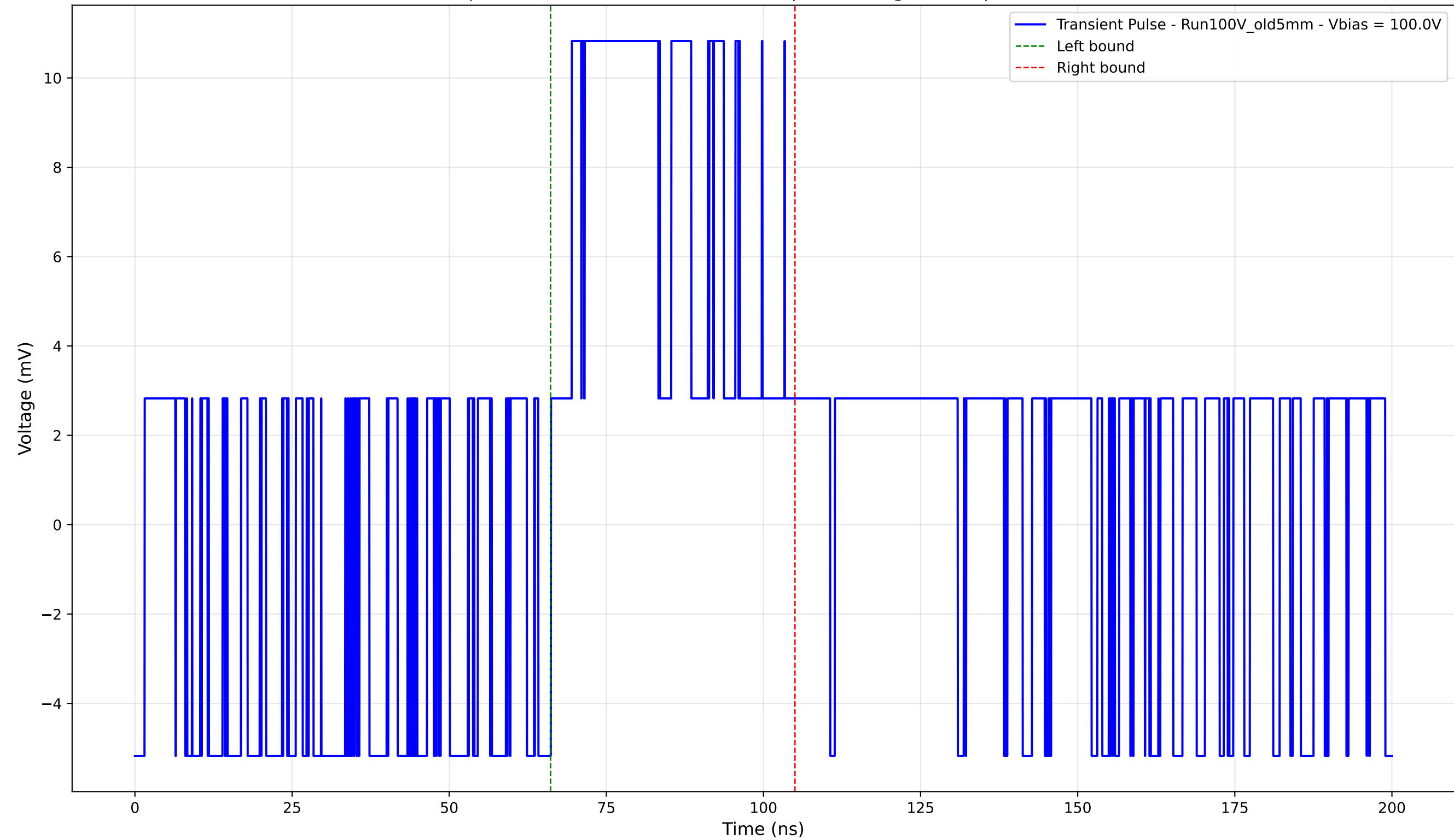
Transient Pulse - Sample: Old5mm - Position: 2160.0 \mu\text{m} - Charge: 5.40 pC - Rise Time: 0.00 ns (N/A)
