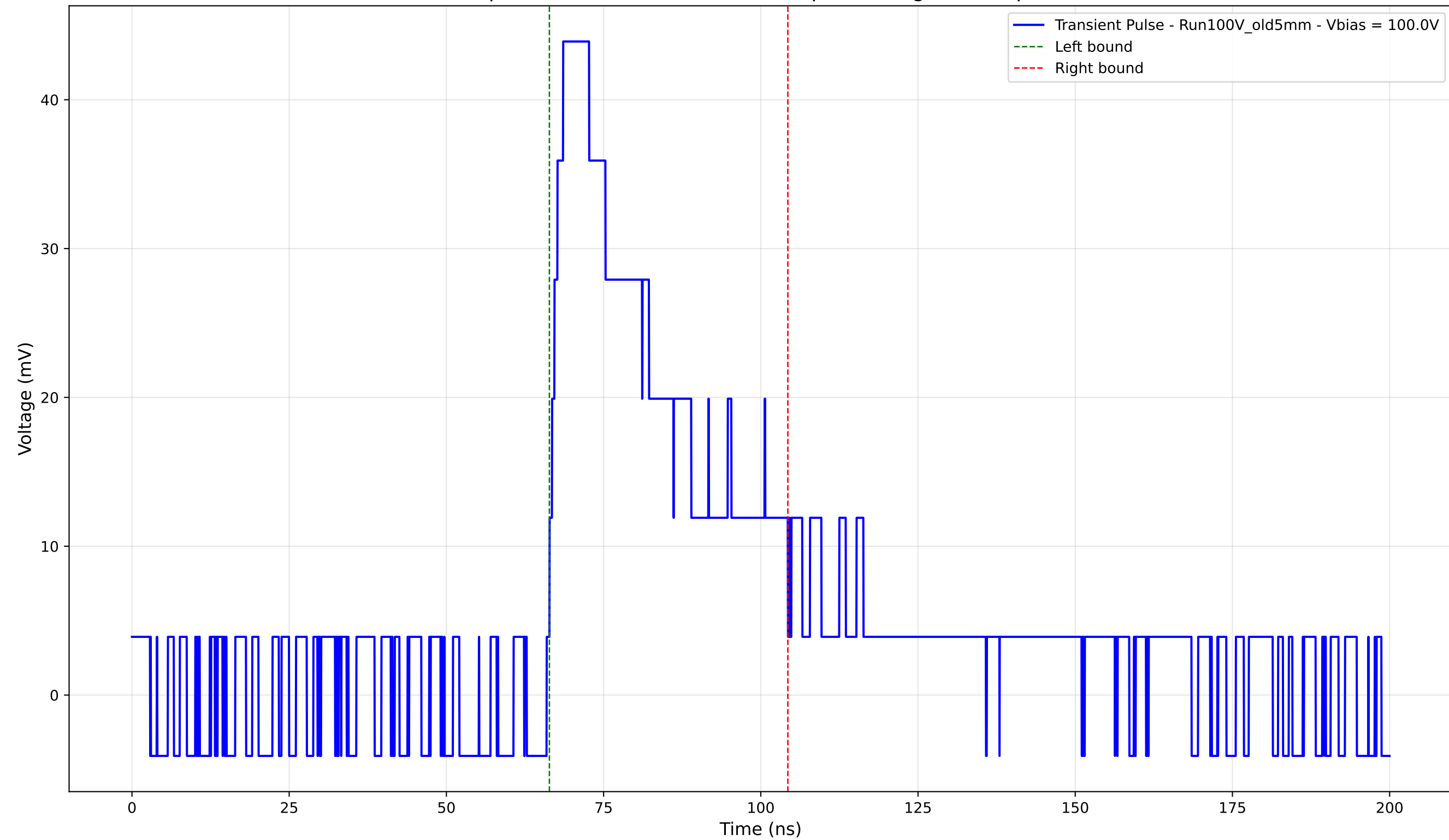
Transient Pulse - Sample: Old5mm - Position: 4785.0 \mu\text{m} - Charge: 16.97 pC - Rise Time: 2.18 ns
