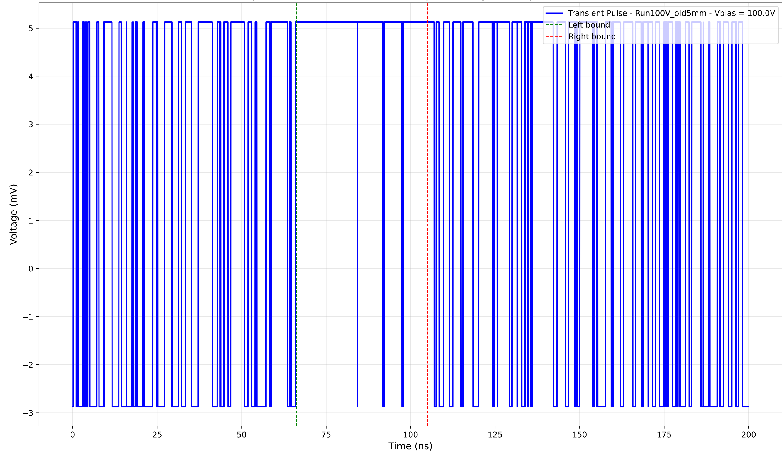
Transient Pulse - Sample: Old5mm - Position: 1935.0 \mu\text{m} - Charge: 3.89 pC - Rise Time: 0.00 ns (N/A)
