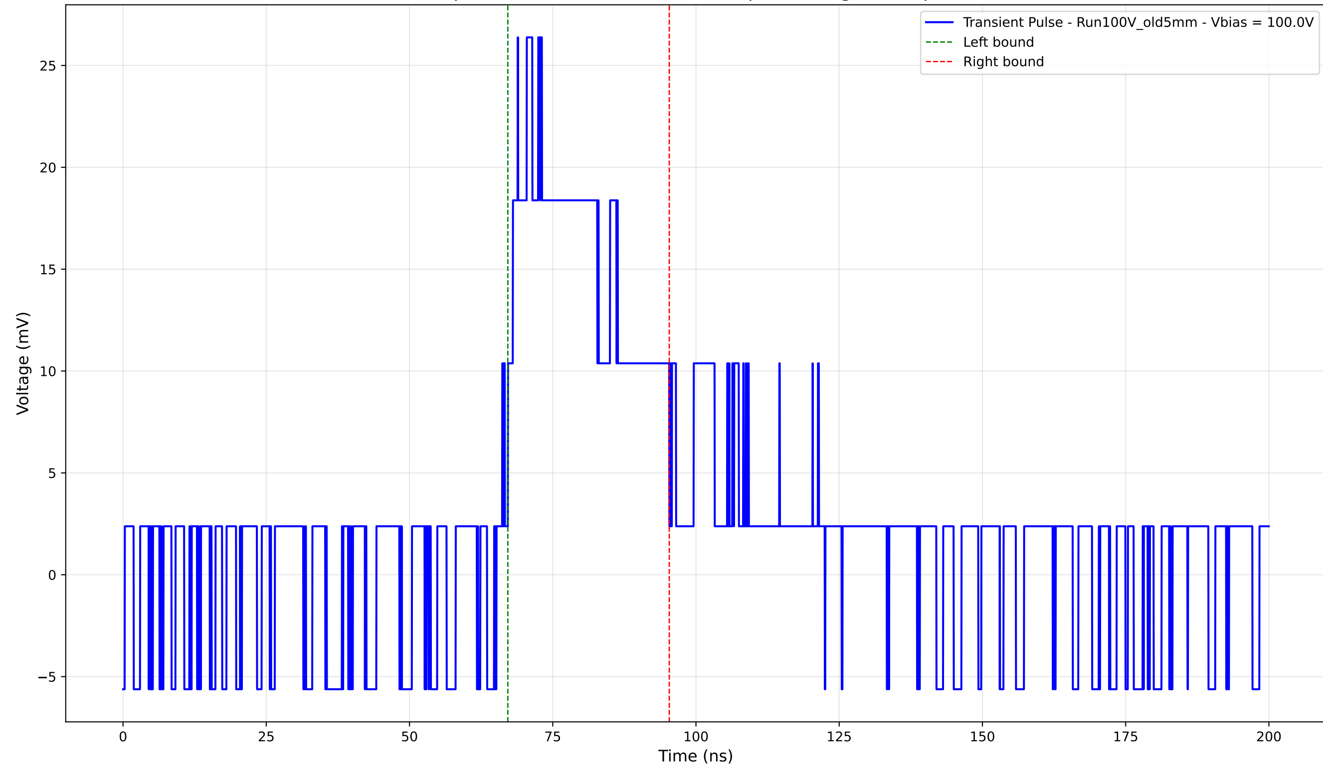
Transient Pulse - Sample: Old5mm - Position: 4990.0 \mu\text{m} - Charge: 8.69 pC - Rise Time: 1.72 ns
