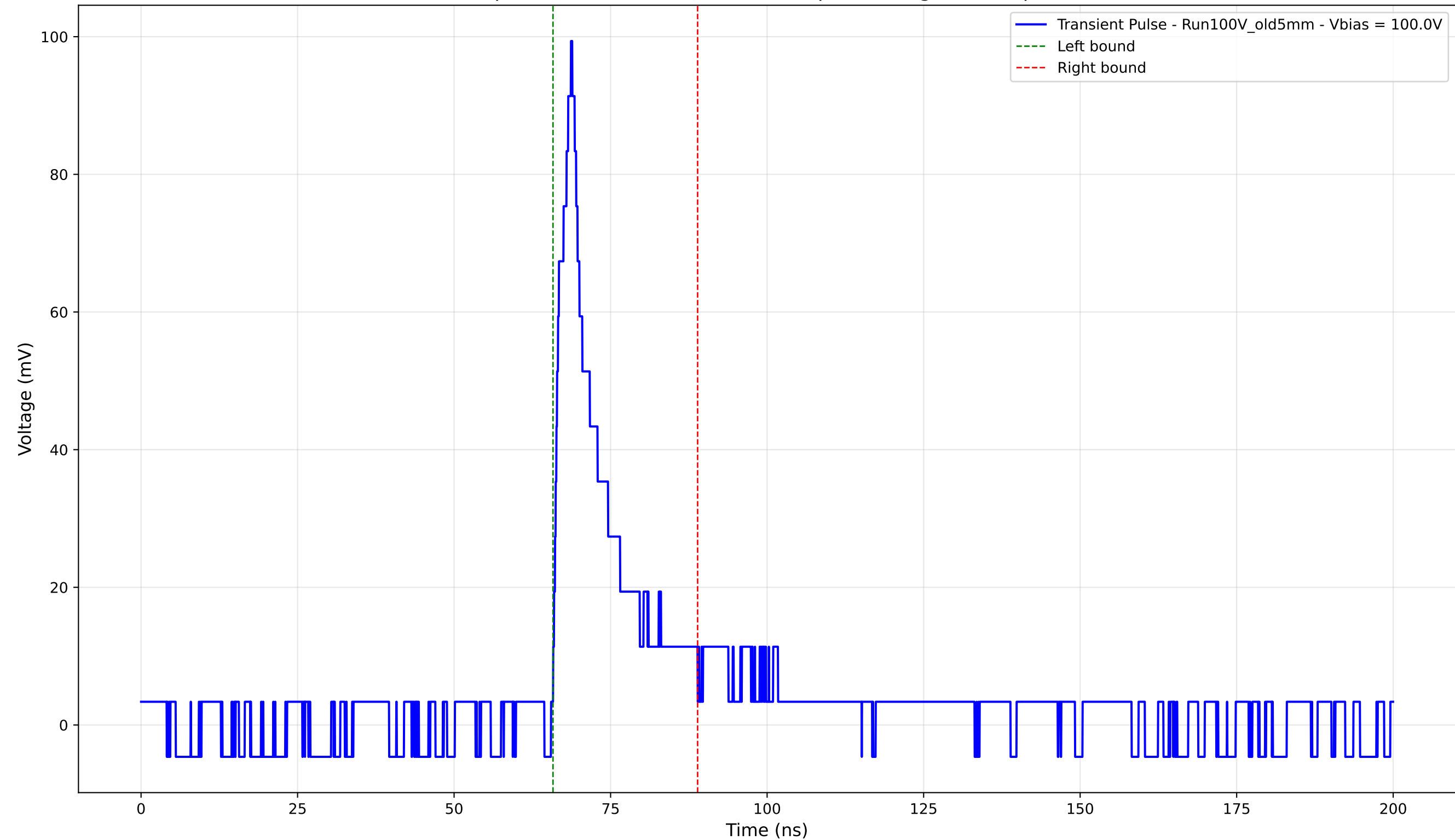
Transient Pulse - Sample: Old5mm - Position: 4200.0 \mu\text{m} - Charge: 14.45 pC - Rise Time: 2.40 ns
