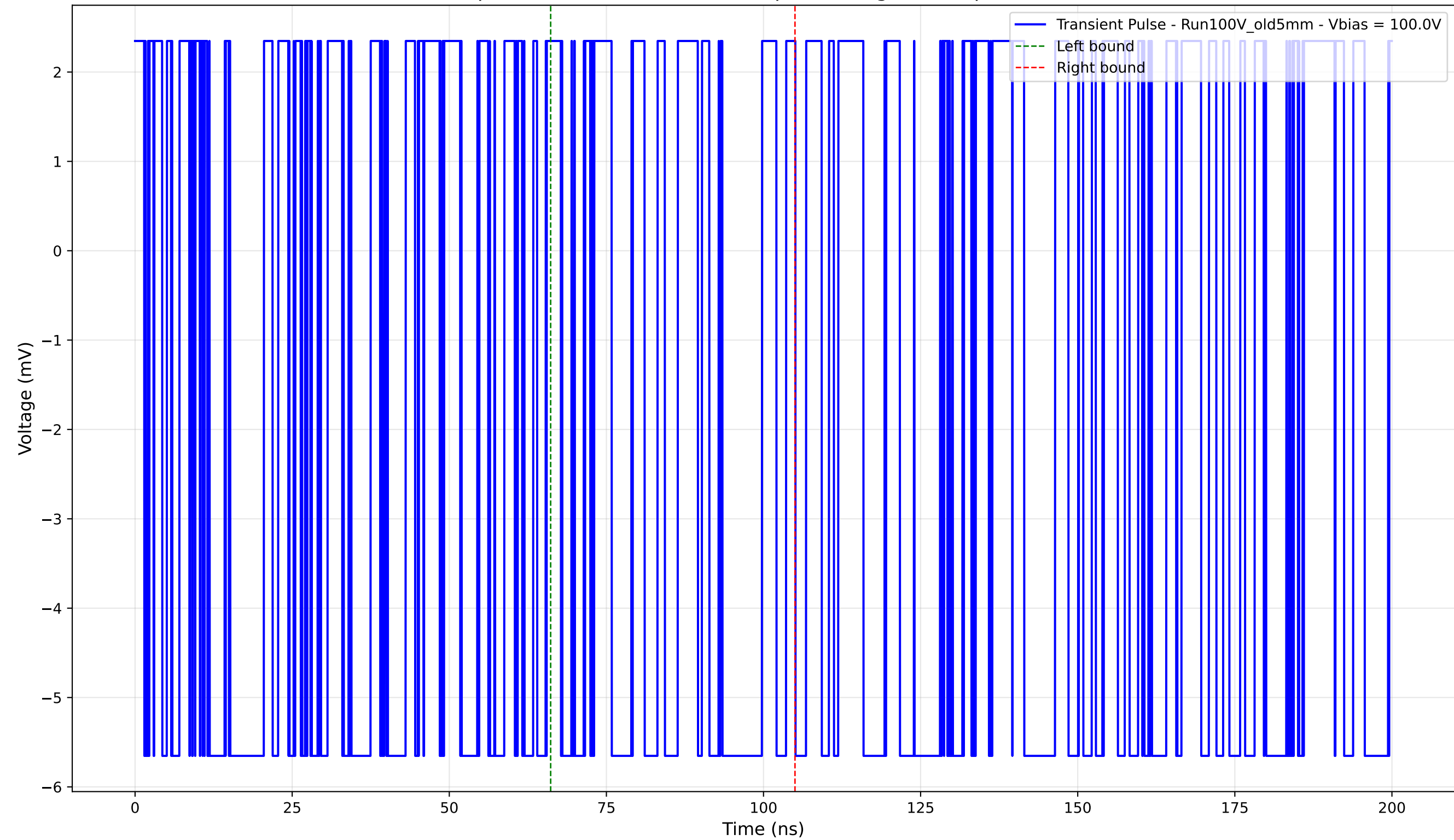
Transient Pulse - Sample: Old5mm - Position: 95.0 \mu\text{m} - Charge: -1.60 pC - Rise Time: 0.00 ns (N/A)
