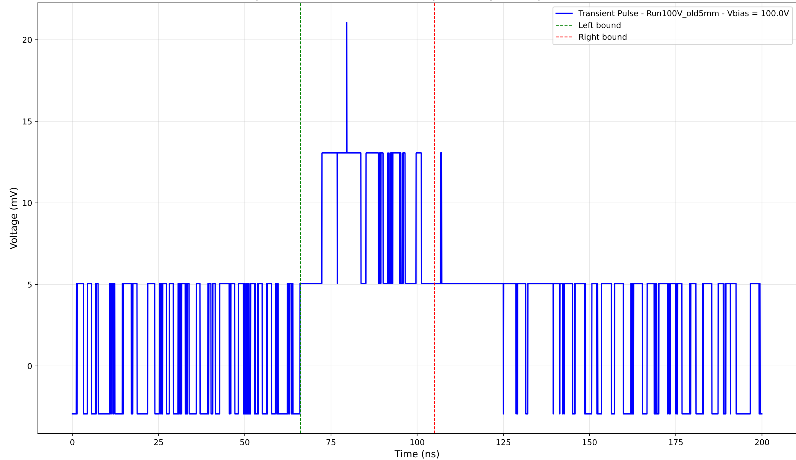
Transient Pulse - Sample: Old5mm - Position: 1170.0 \mu\text{m} - Charge: 7.23 pC - Rise Time: 0.00 ns (N/A)
