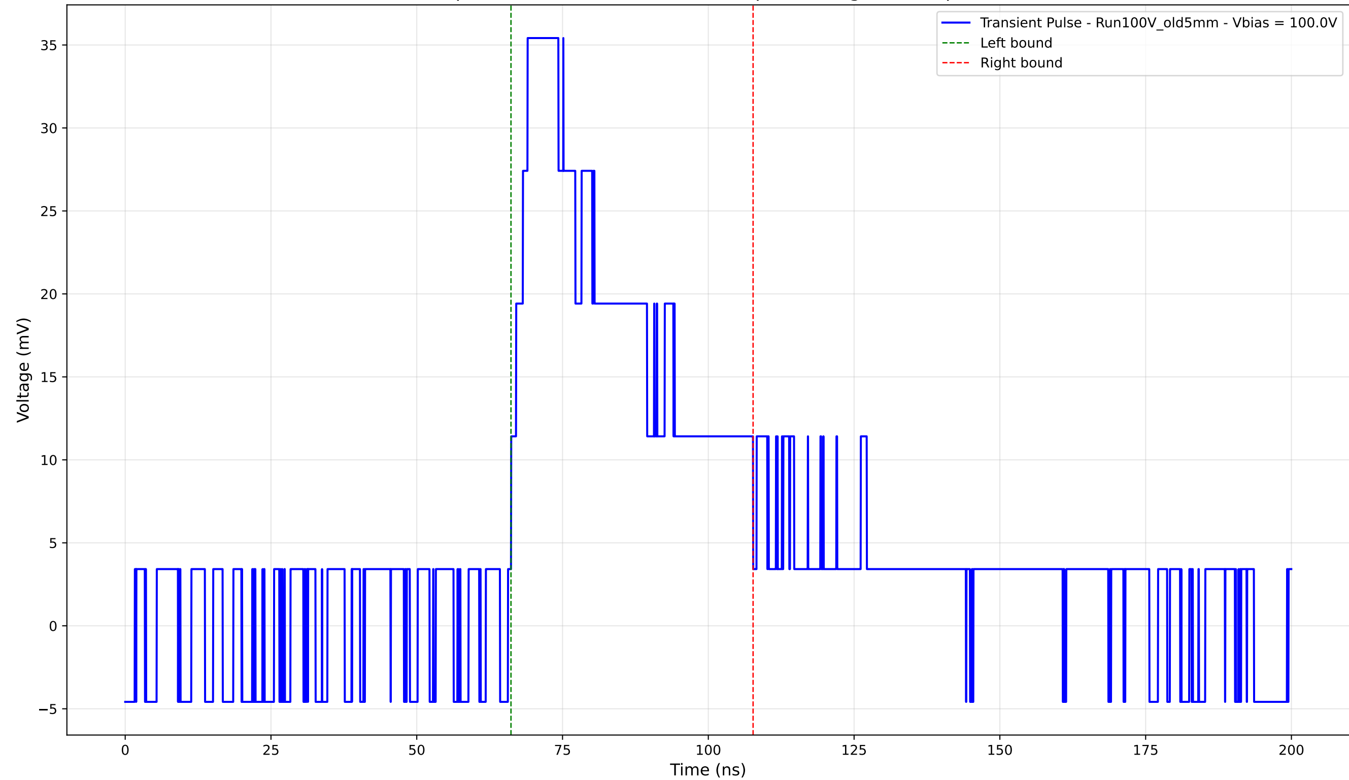
Transient Pulse - Sample: Old5mm - Position: 4955.0 \mu\text{m} - Charge: 15.98 pC - Rise Time: 2.84 ns
