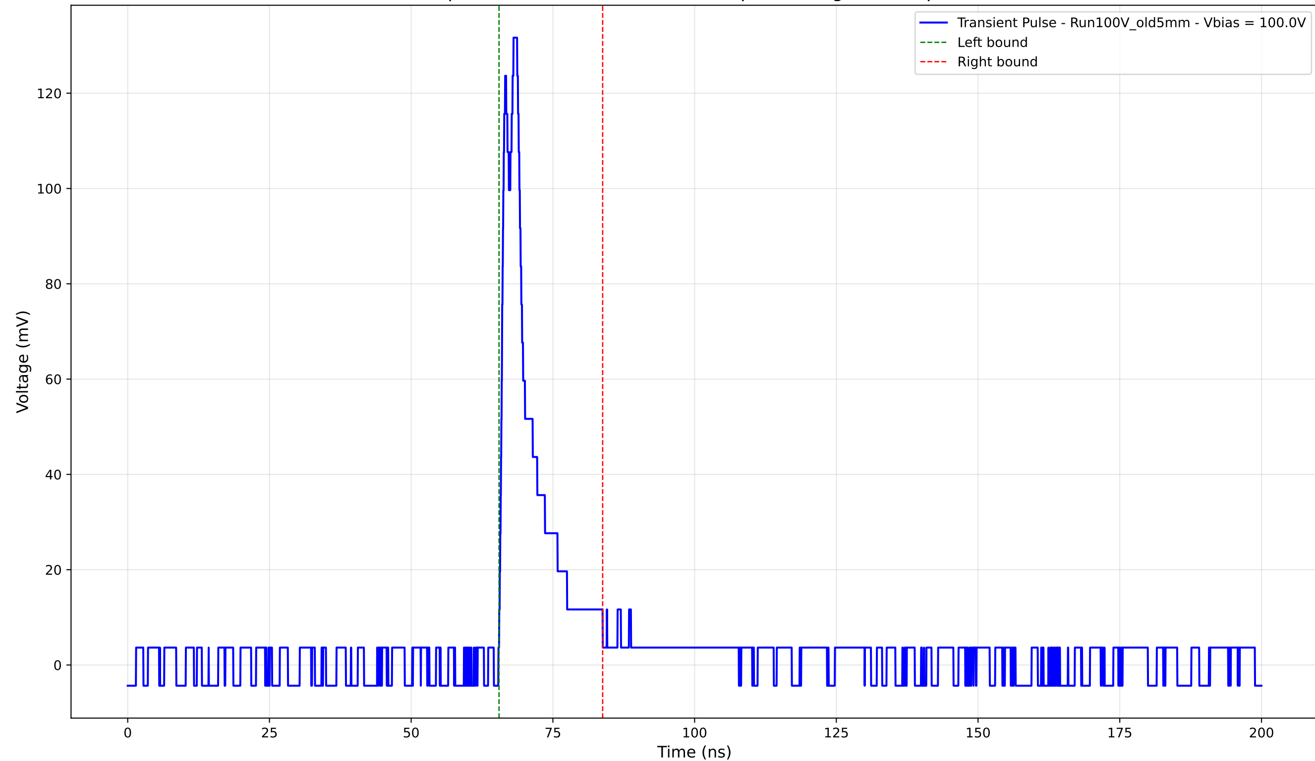
Transient Pulse - Sample: Old5mm - Position: 3920.0 \mu\text{m} - Charge: 15.23 pC - Rise Time: 0.96 ns
