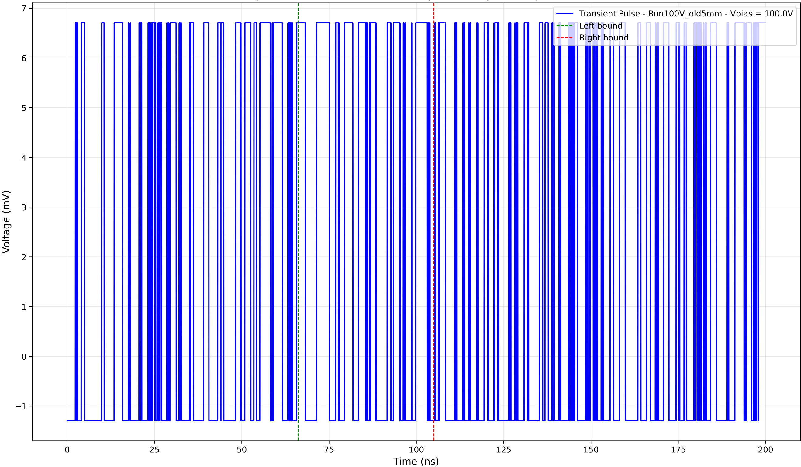
Transient Pulse - Sample: Old5mm - Position: 105.0 \mu\text{m} - Charge: 2.16 pC - Rise Time: 0.00 ns (N/A)
