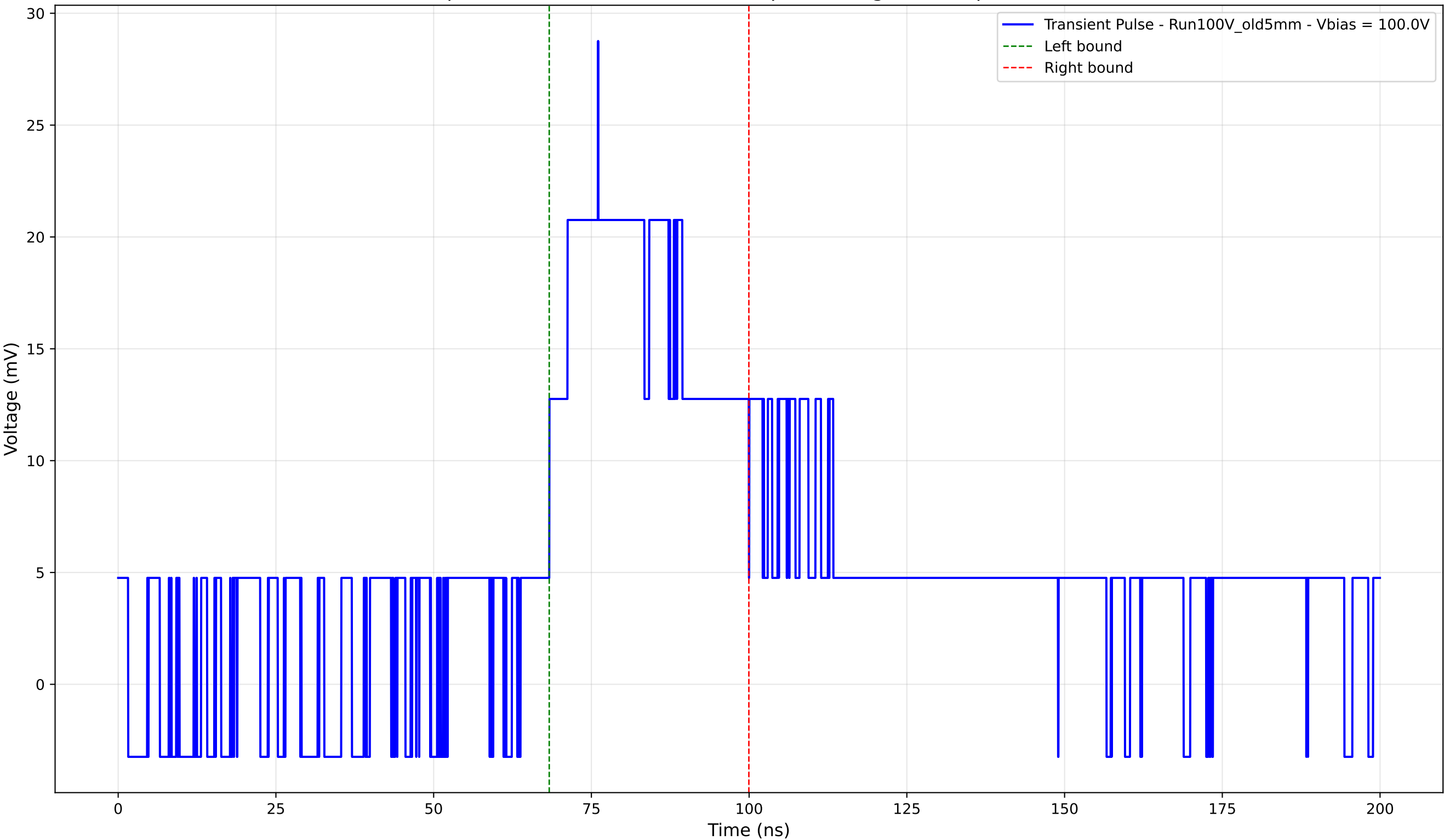
Transient Pulse - Sample: Old5mm - Position: 2010.0 \mu\text{m} - Charge: 10.73 pC - Rise Time: 0.00 ns (N/A)
