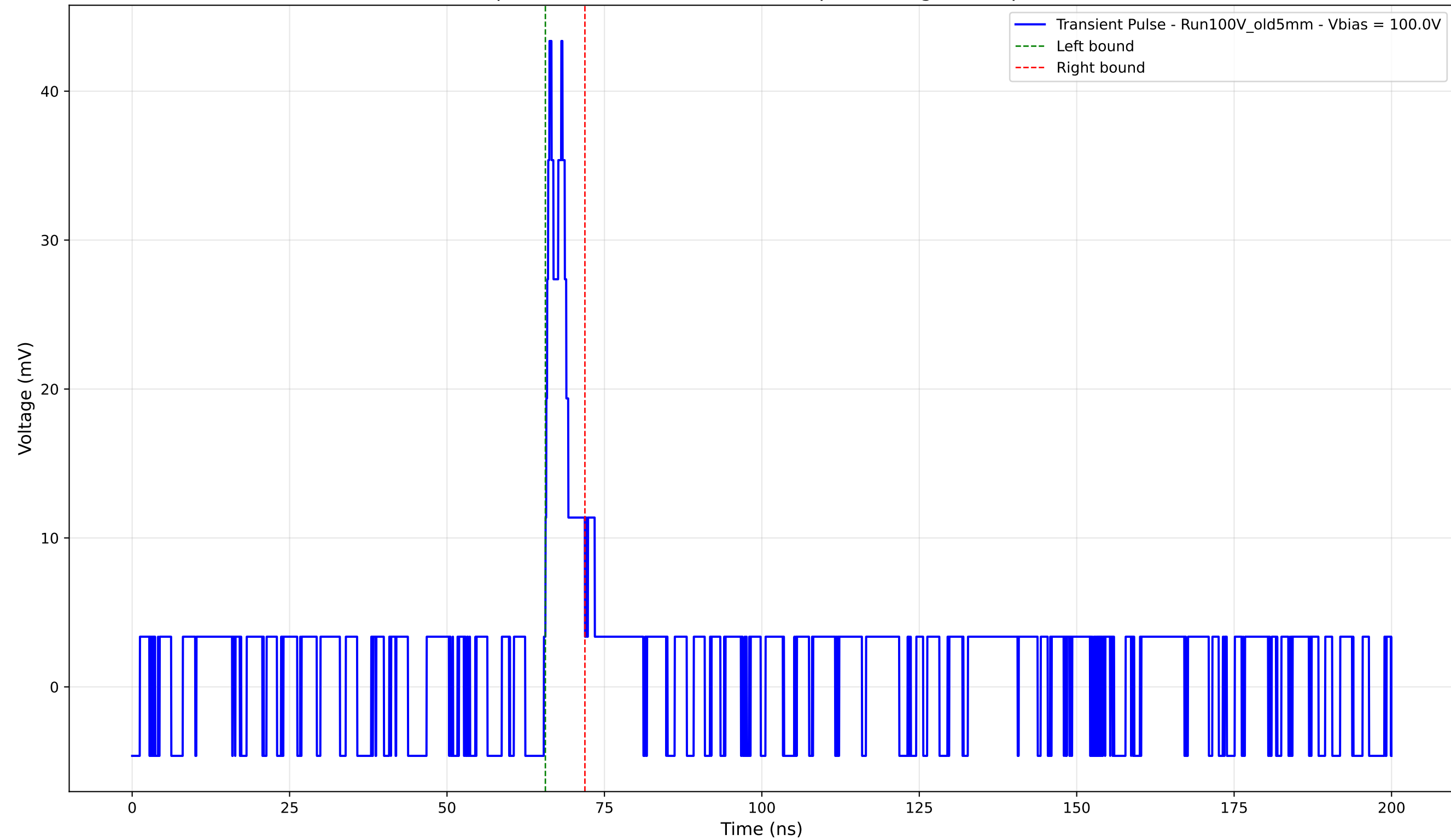
Transient Pulse - Sample: Old5mm - Position: 3665.0 \mu\text{m} - Charge: 2.86 pC - Rise Time: 0.64 ns
