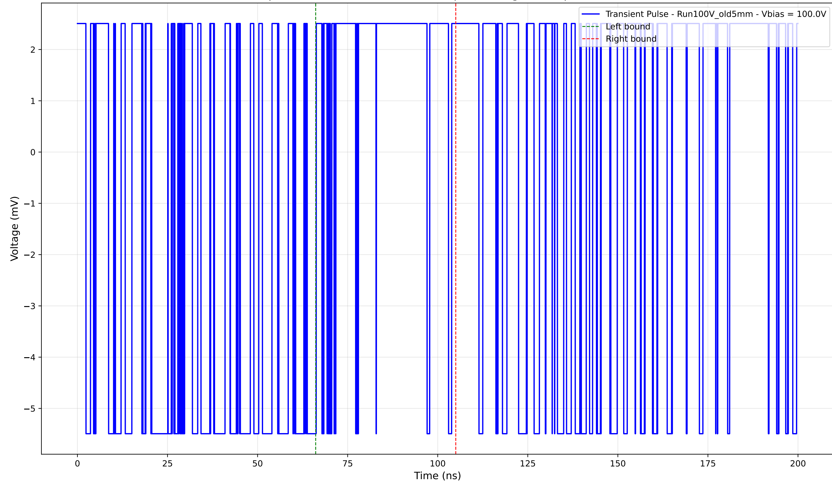
Transient Pulse - Sample: Old5mm - Position: 1300.0 \mu\text{m} - Charge: 1.35 pC - Rise Time: 0.00 ns (N/A)
