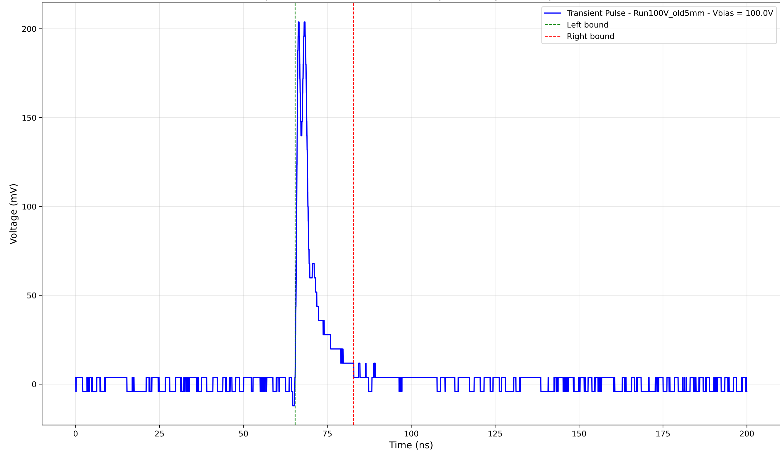
Transient Pulse - Sample: Old5mm - Position: 3595.0 \mu\text{m} - Charge: 19.95 pC - Rise Time: 0.72 ns
