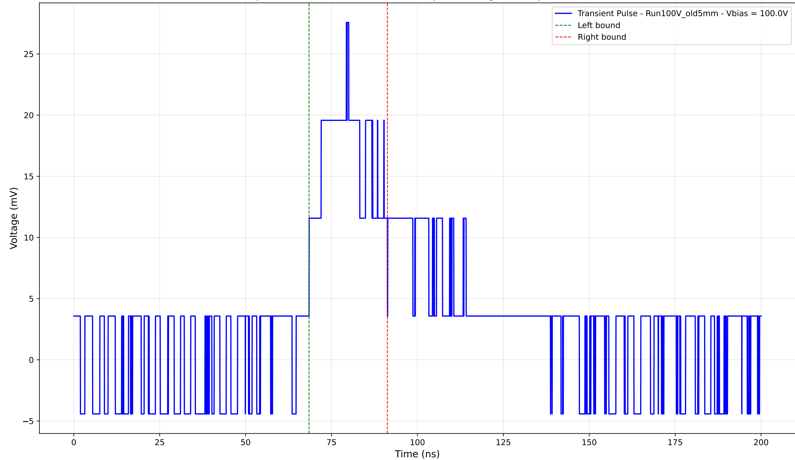
Transient Pulse - Sample: Old5mm - Position: 2025.0 \mu\text{m} - Charge: 7.52 pC - Rise Time: 0.00 ns (N/A)
