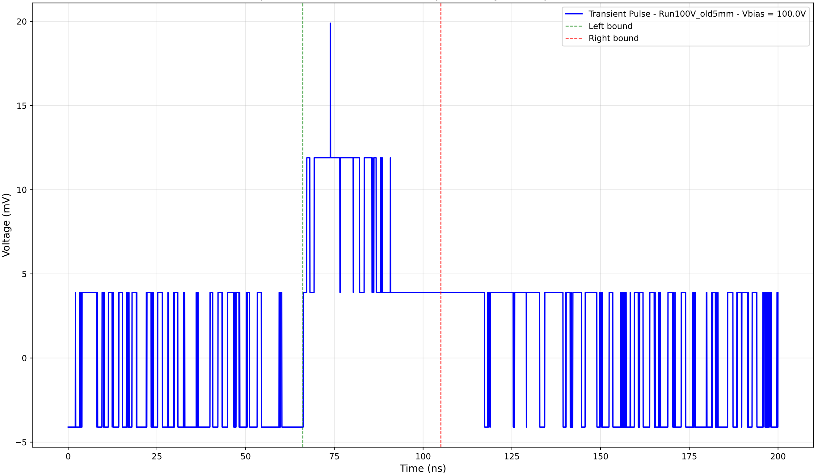
Transient Pulse - Sample: Old5mm - Position: 375.0 \mu\text{m} - Charge: 5.72 pC - Rise Time: 0.00 ns (N/A)
