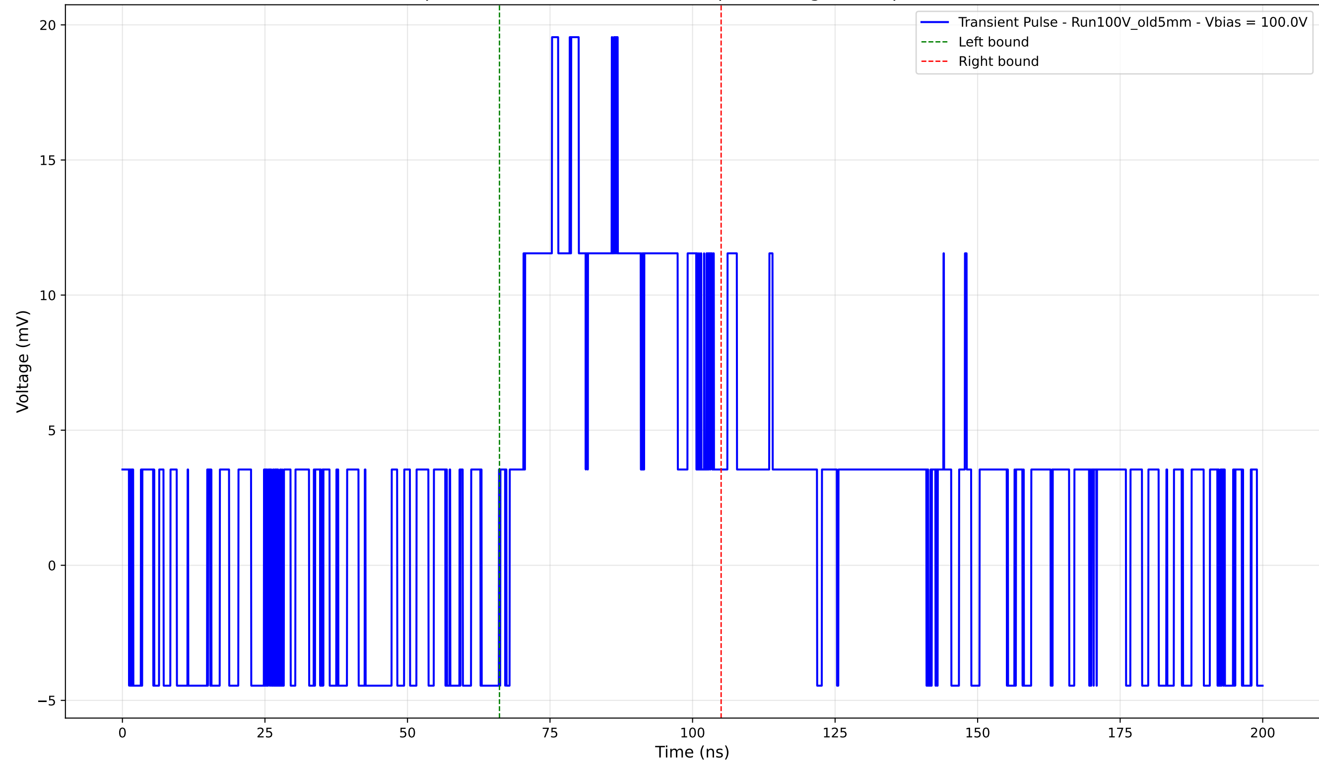
Transient Pulse - Sample: Old5mm - Position: 1640.0 \mu\text{m} - Charge: 7.82 pC - Rise Time: 0.00 ns (N/A)
