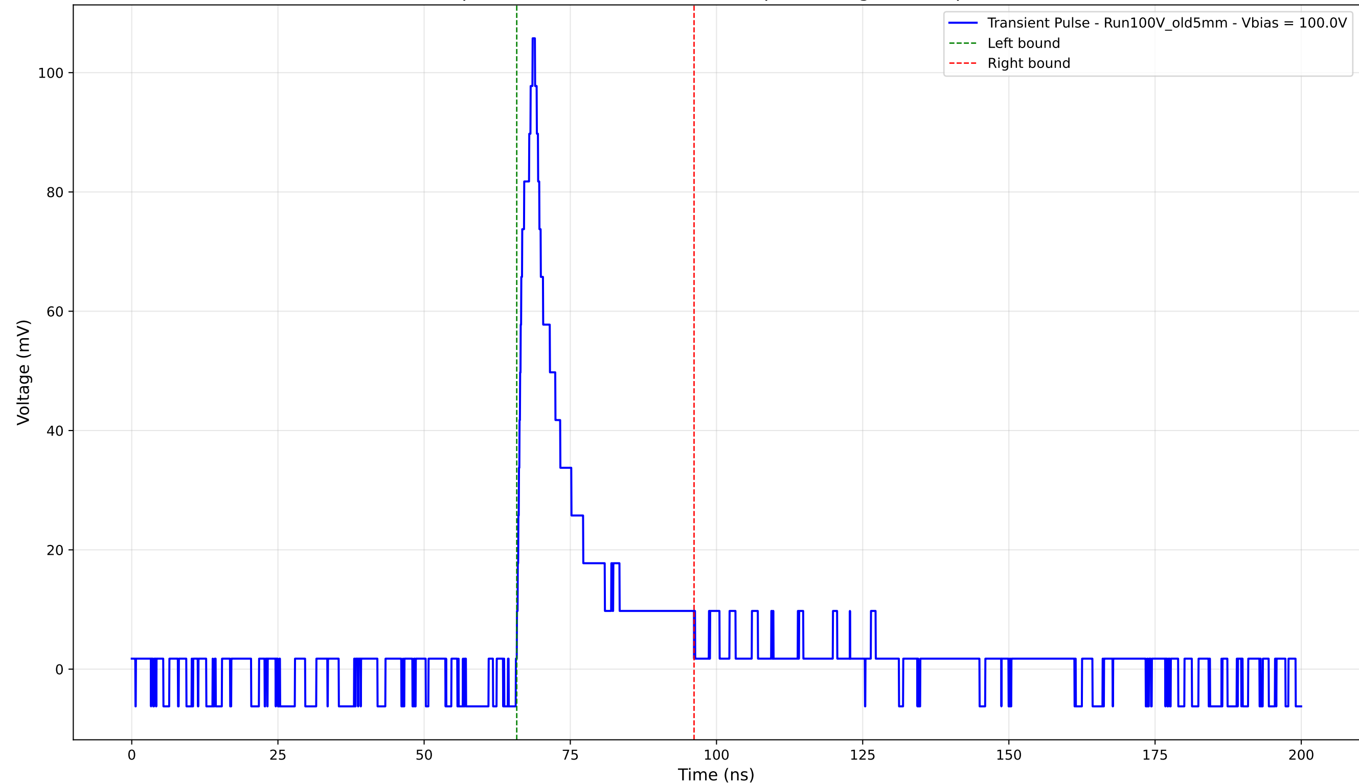
Transient Pulse - Sample: Old5mm - Position: 4190.0 \mu\text{m} - Charge: 16.60 pC - Rise Time: 2.22 ns
