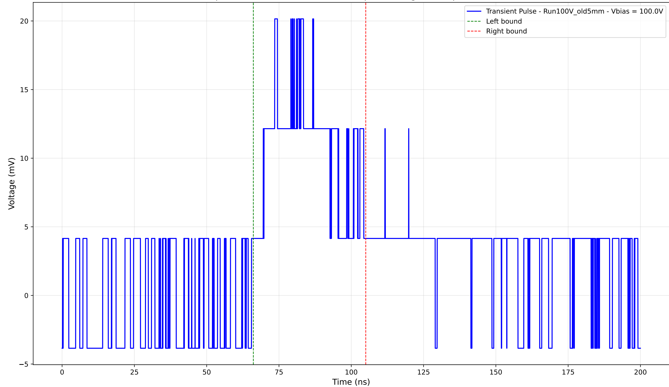
Transient Pulse - Sample: Old5mm - Position: 1635.0 \mu\text{m} - Charge: 8.31 pC - Rise Time: 0.00 ns (N/A)
