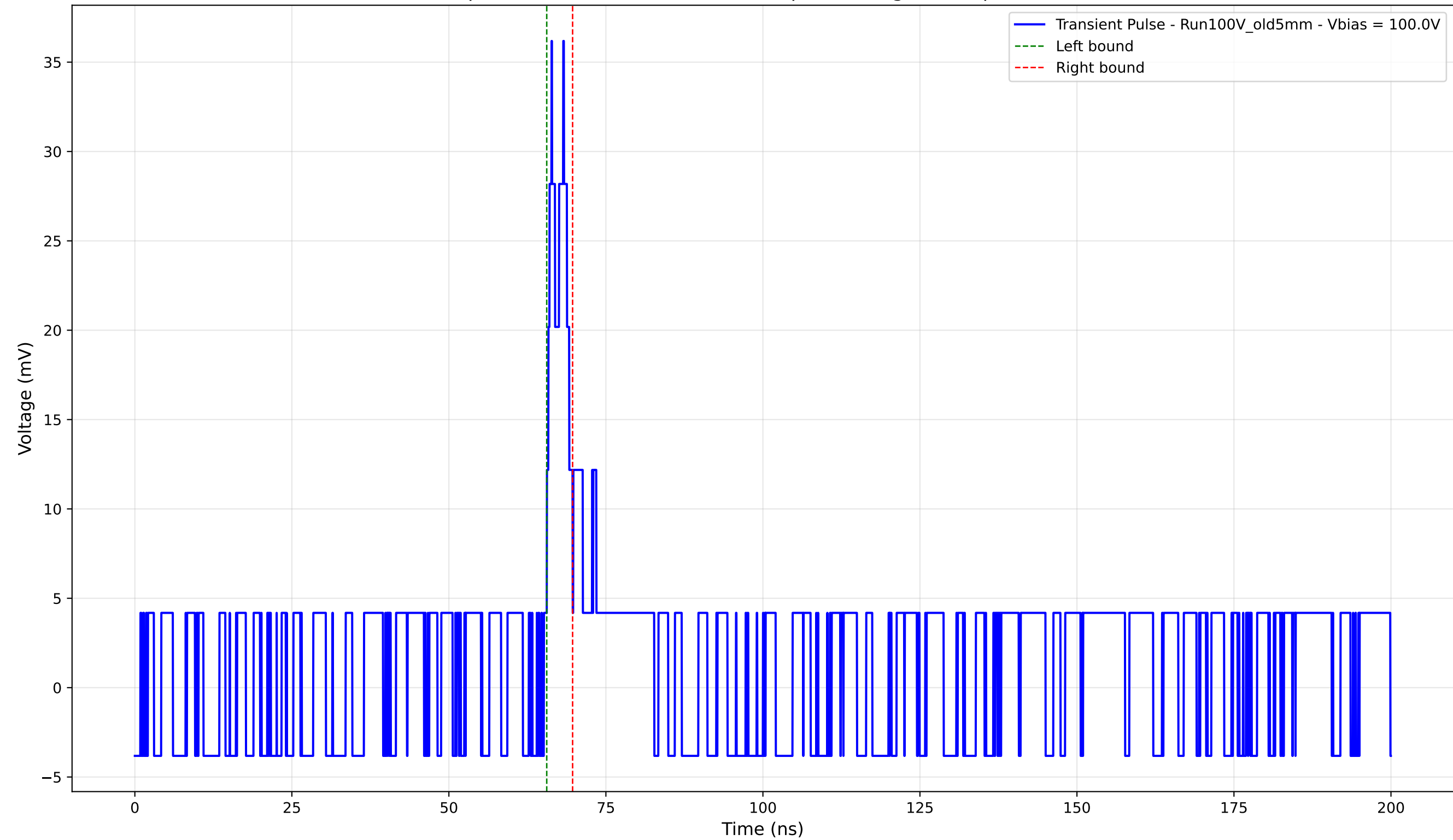
Transient Pulse - Sample: Old5mm - Position: 3670.0 \mu\text{m} - Charge: 1.91 pC - Rise Time: 0.00 ns (N/A)
