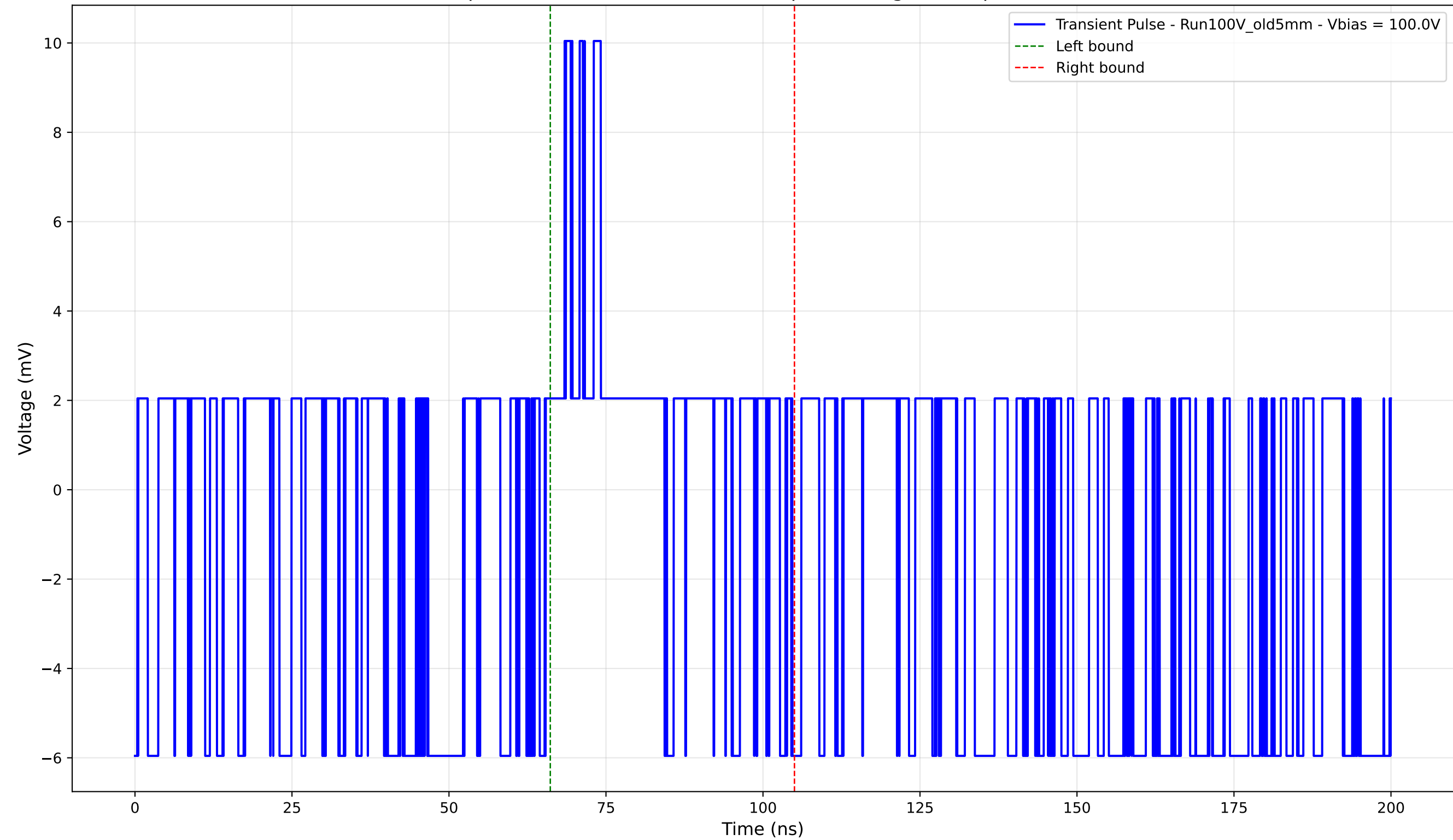
Transient Pulse - Sample: Old5mm - Position: 2840.0 \mu\text{m} - Charge: 1.27 pC - Rise Time: 0.00 ns (N/A)
