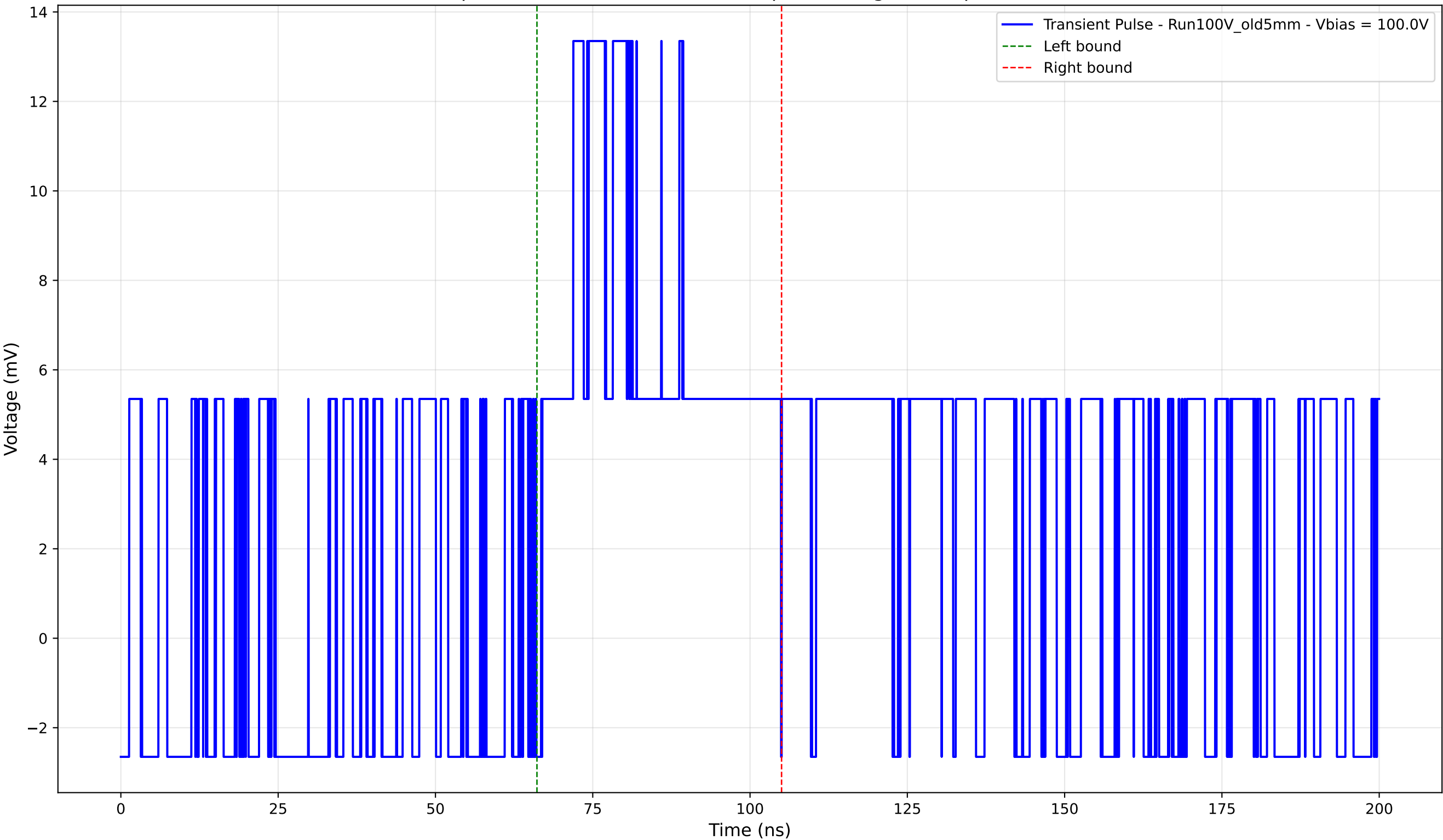
Transient Pulse - Sample: Old5mm - Position: 905.0 \mu\text{m} - Charge: 5.28 pC - Rise Time: 0.00 ns (N/A)
