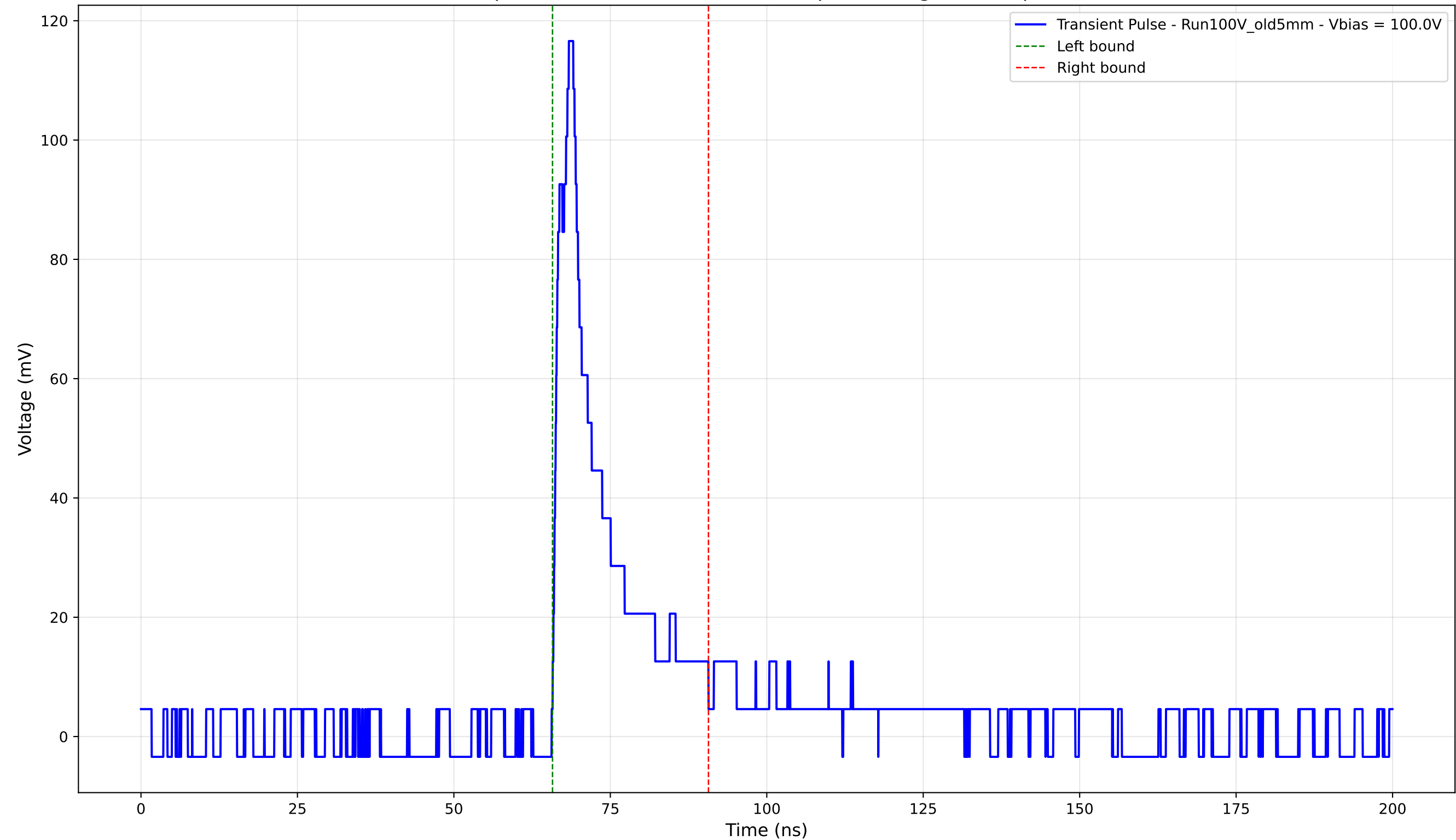
Transient Pulse - Sample: Old5mm - Position: 3250.0 \mu\text{m} - Charge: 17.86 pC - Rise Time: 2.36 ns
