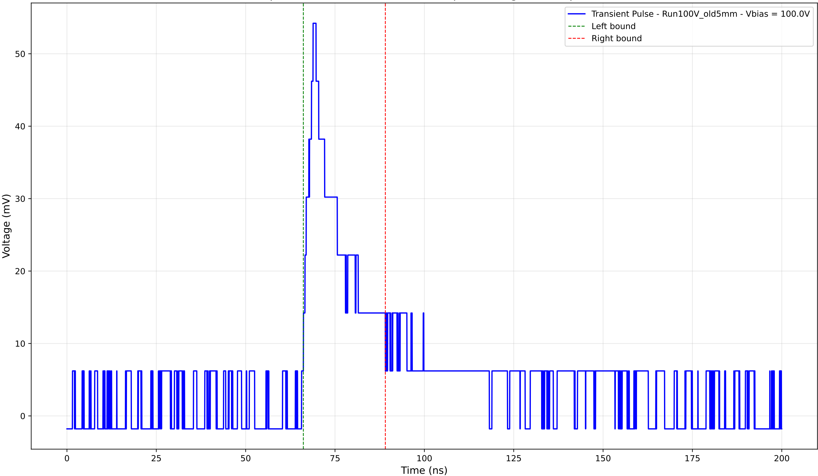
Transient Pulse - Sample: Old5mm - Position: 4525.0 \mu\text{m} - Charge: 11.33 pC - Rise Time: 3.22 ns
