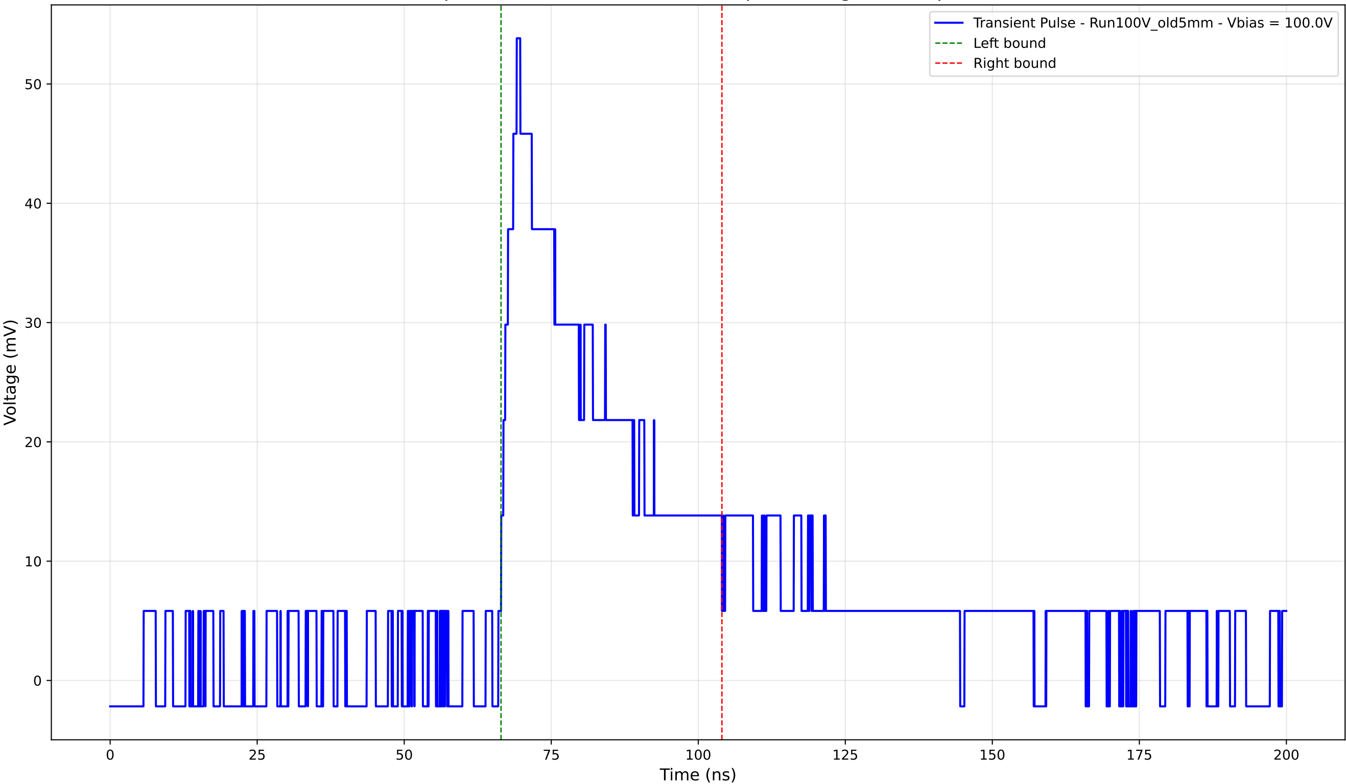
Transient Pulse - Sample: Old5mm - Position: 4805.0 \mu\text{m} - Charge: 18.22 pC - Rise Time: 3.12 ns
