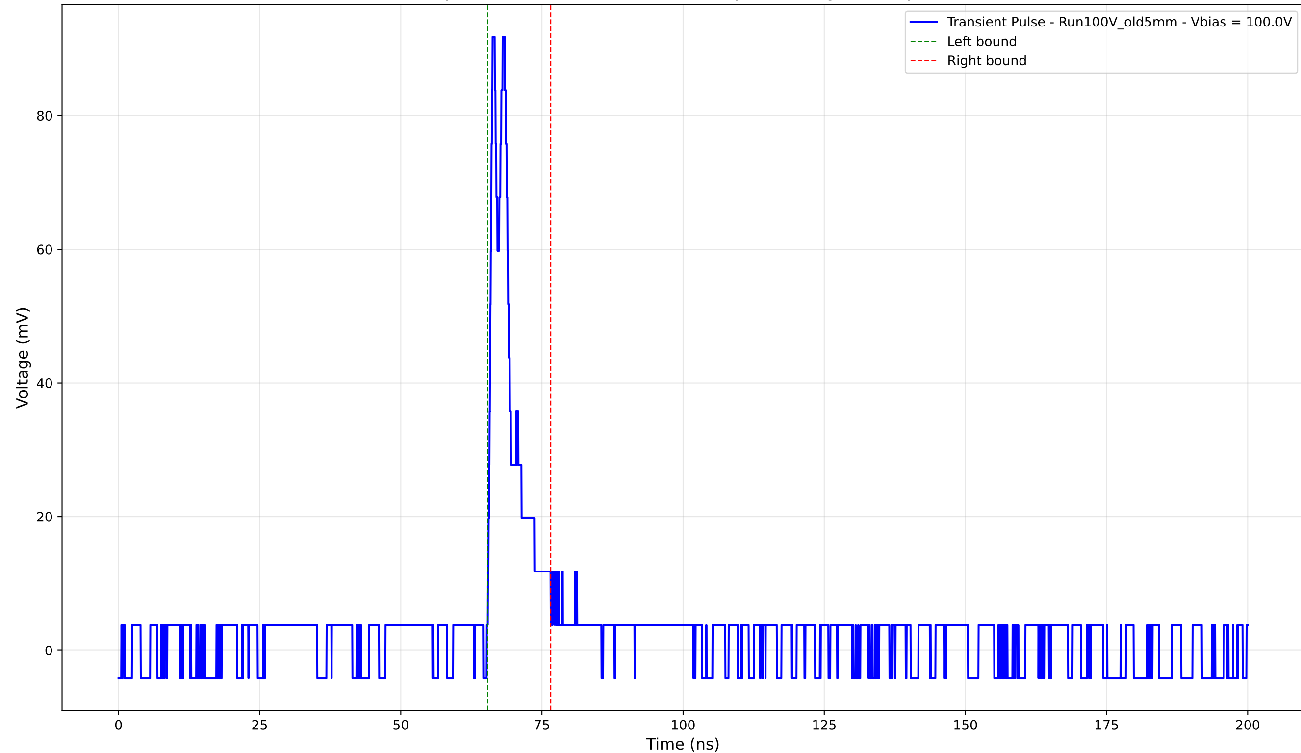
Transient Pulse - Sample: Old5mm - Position: 3770.0 \mu\text{m} - Charge: 8.15 pC - Rise Time: 0.73 ns
