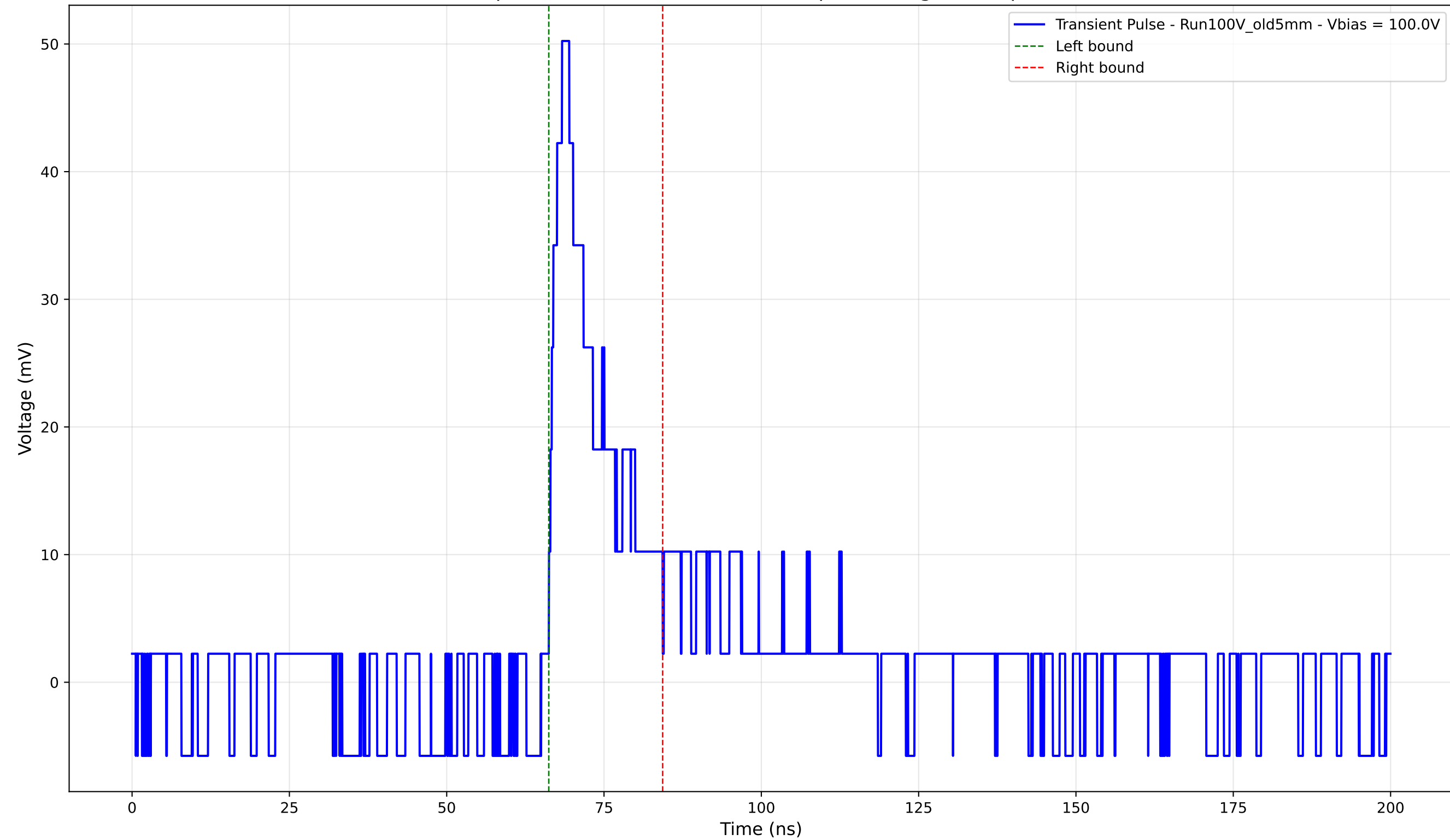
Transient Pulse - Sample: Old5mm - Position: 3020.0 \mu\text{m} - Charge: 8.14 pC - Rise Time: 2.09 ns
