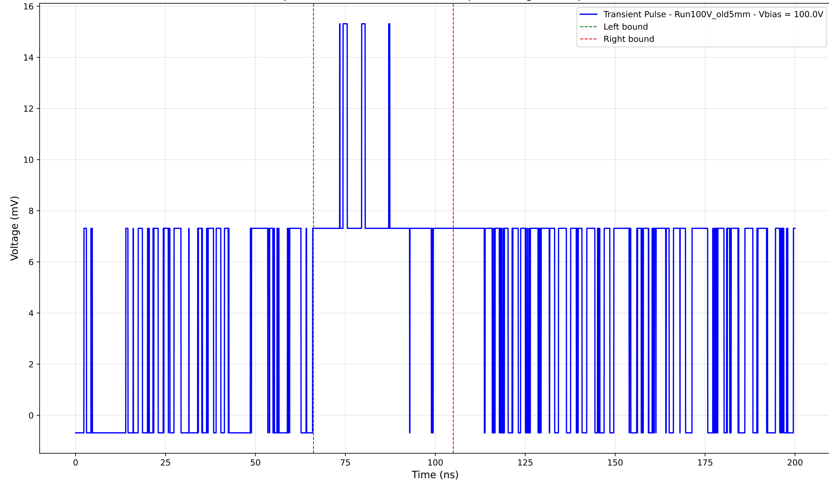
Transient Pulse - Sample: Old5mm - Position: 2140.0 \mu\text{m} - Charge: 5.97 pC - Rise Time: 7.54 ns
