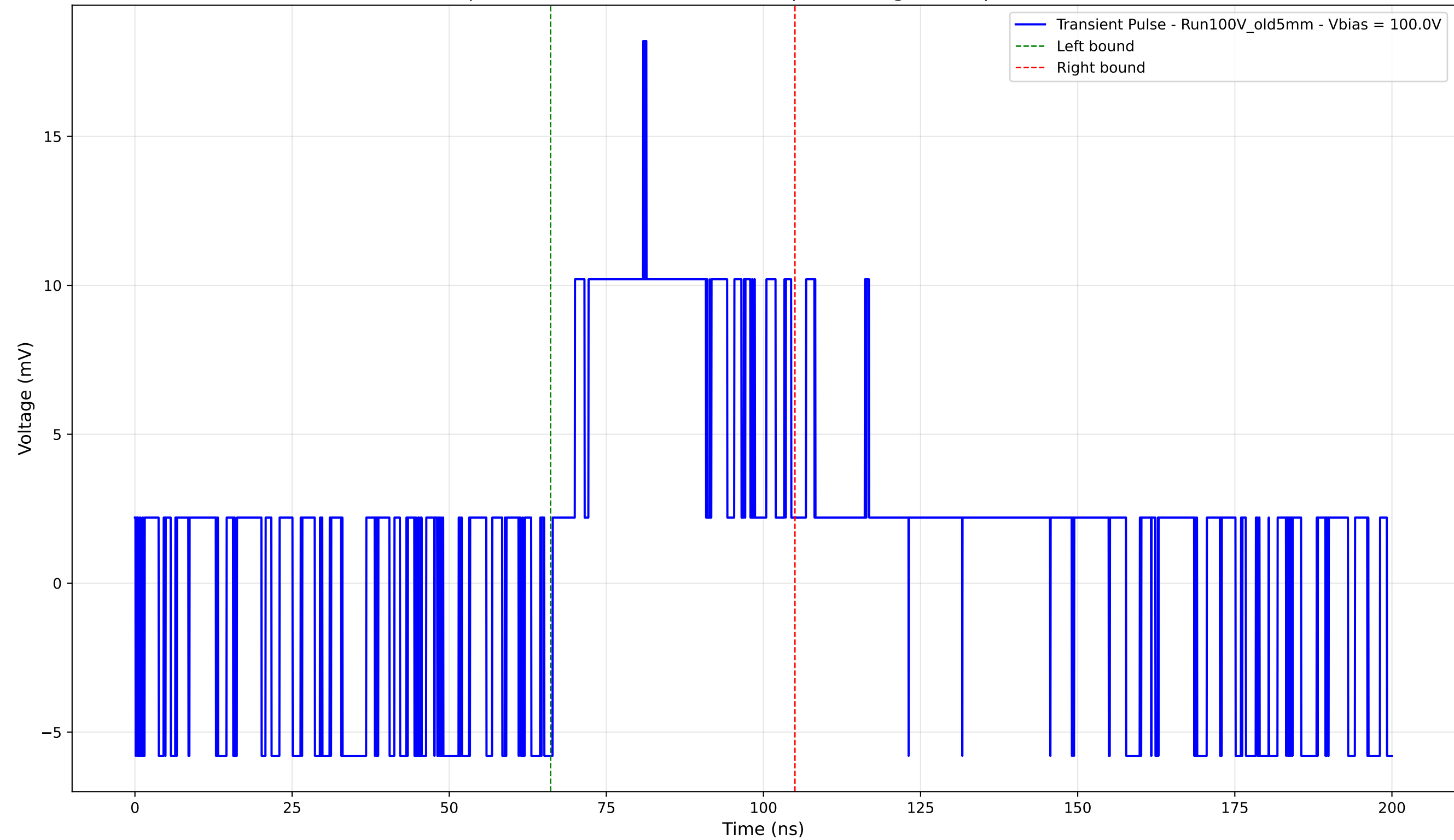
Transient Pulse - Sample: Old5mm - Position: 1770.0 \mu\text{m} - Charge: 6.14 pC - Rise Time: 0.00 ns (N/A)
