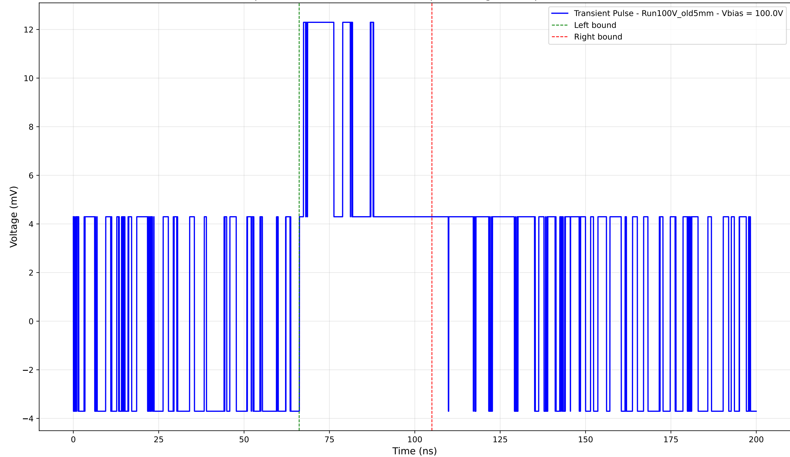
Transient Pulse - Sample: Old5mm - Position: 2555.0 \mu\text{m} - Charge: 5.29 pC - Rise Time: 0.00 ns (N/A)
