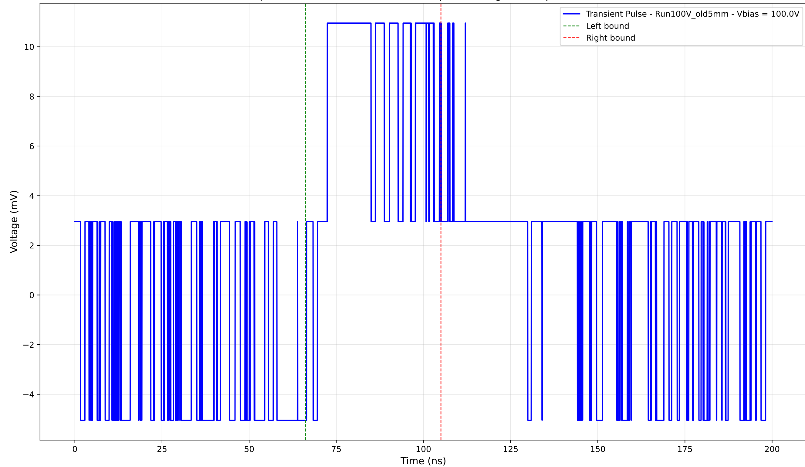
Transient Pulse - Sample: Old5mm - Position: 1235.0 \mu\text{m} - Charge: 6.08 pC - Rise Time: 0.00 ns (N/A)
