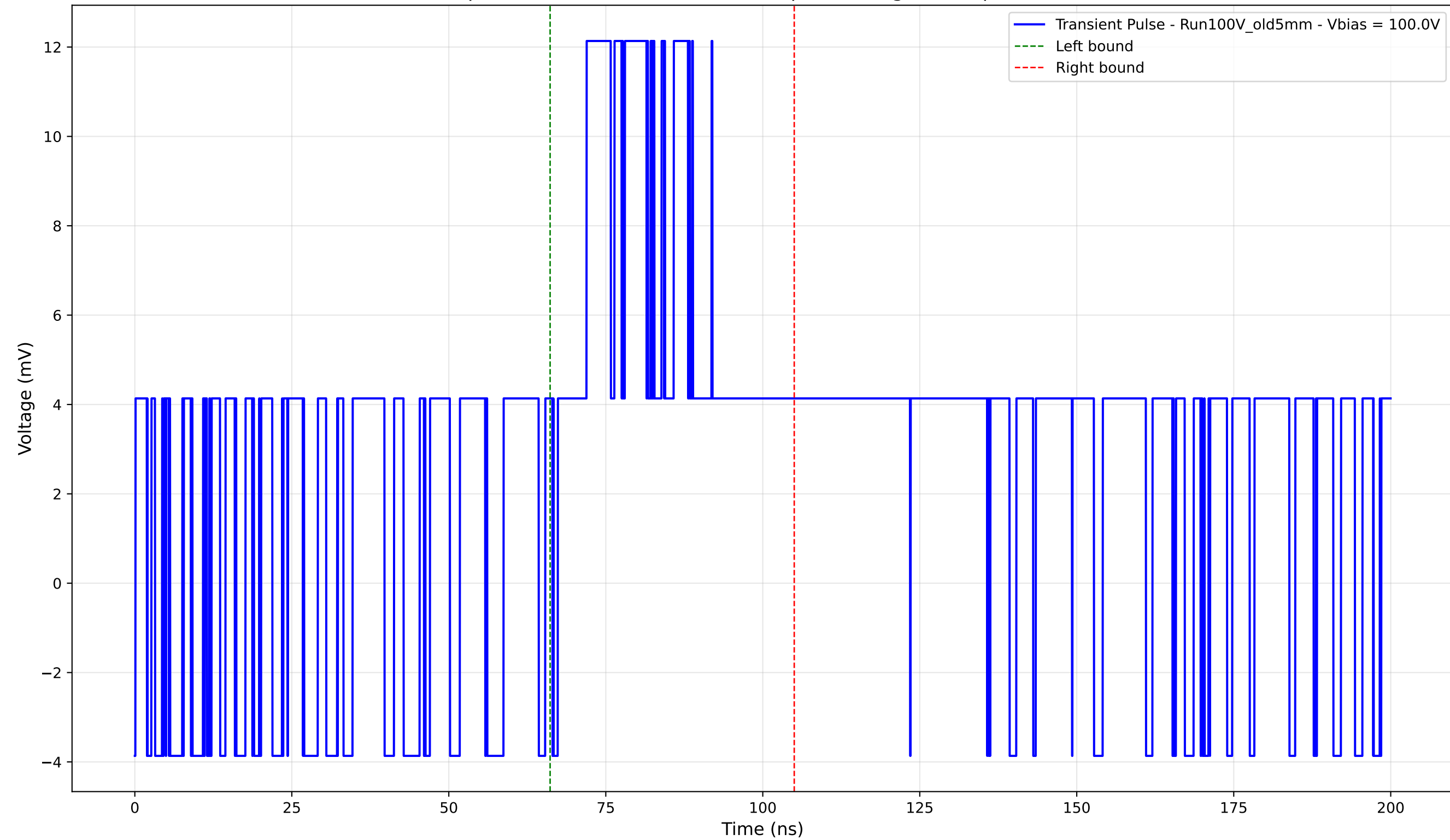
Transient Pulse - Sample: Old5mm - Position: 2080.0 \mu\text{m} - Charge: 5.06 pC - Rise Time: 0.00 ns (N/A)
