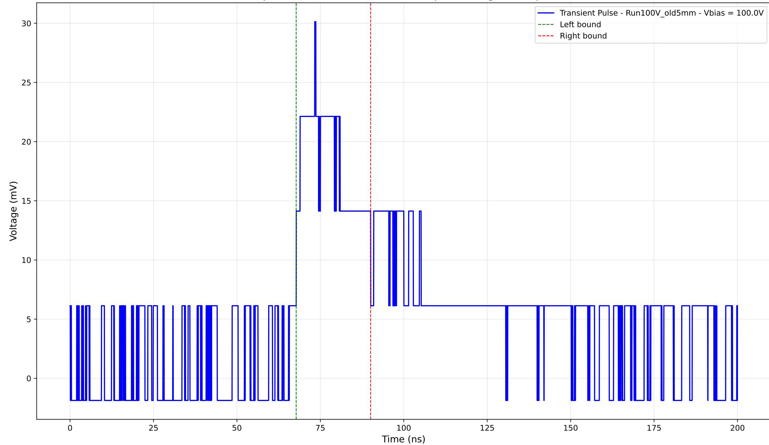
Transient Pulse - Sample: Old5mm - Position: 2460.0 \mu\text{m} - Charge: 8.14 pC - Rise Time: 7.63 ns
