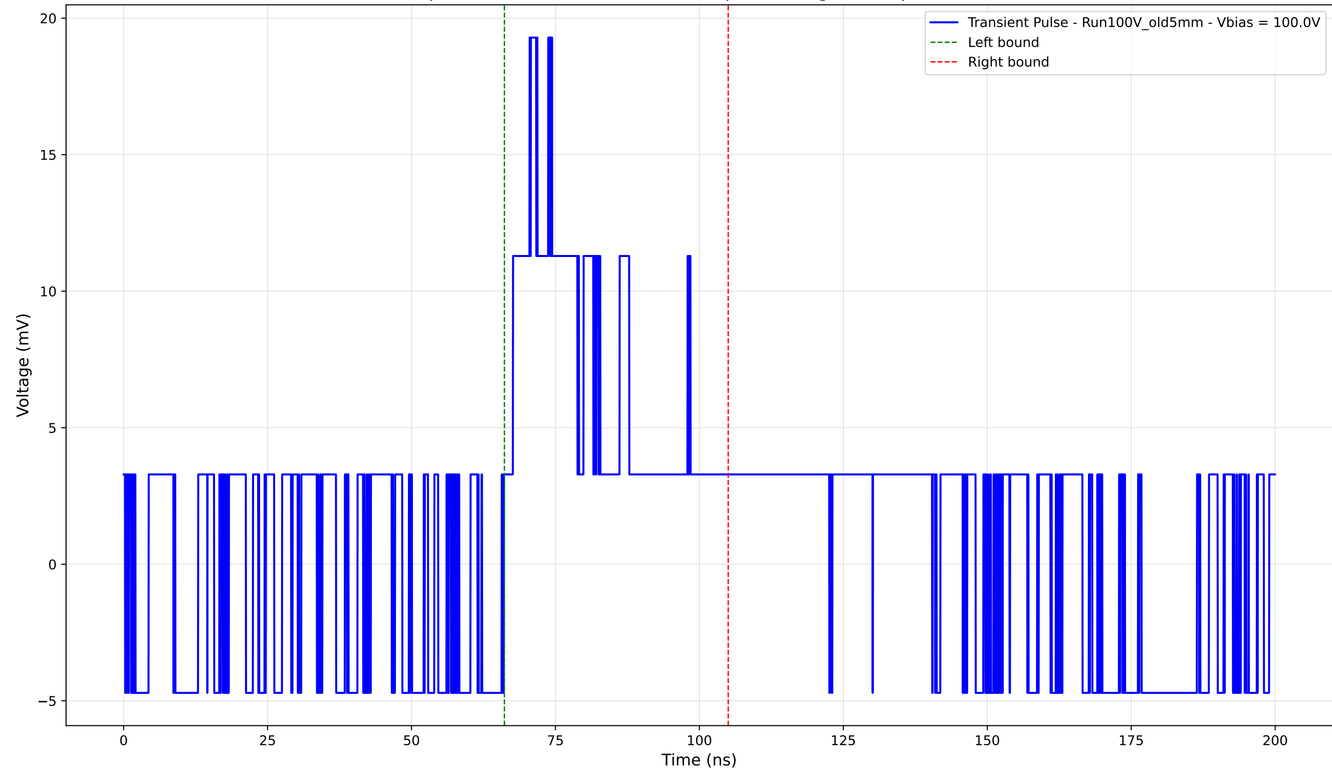
Transient Pulse - Sample: Old5mm - Position: 2560.0 \mu\text{m} - Charge: 5.37 pC - Rise Time: 0.00 ns (N/A)
