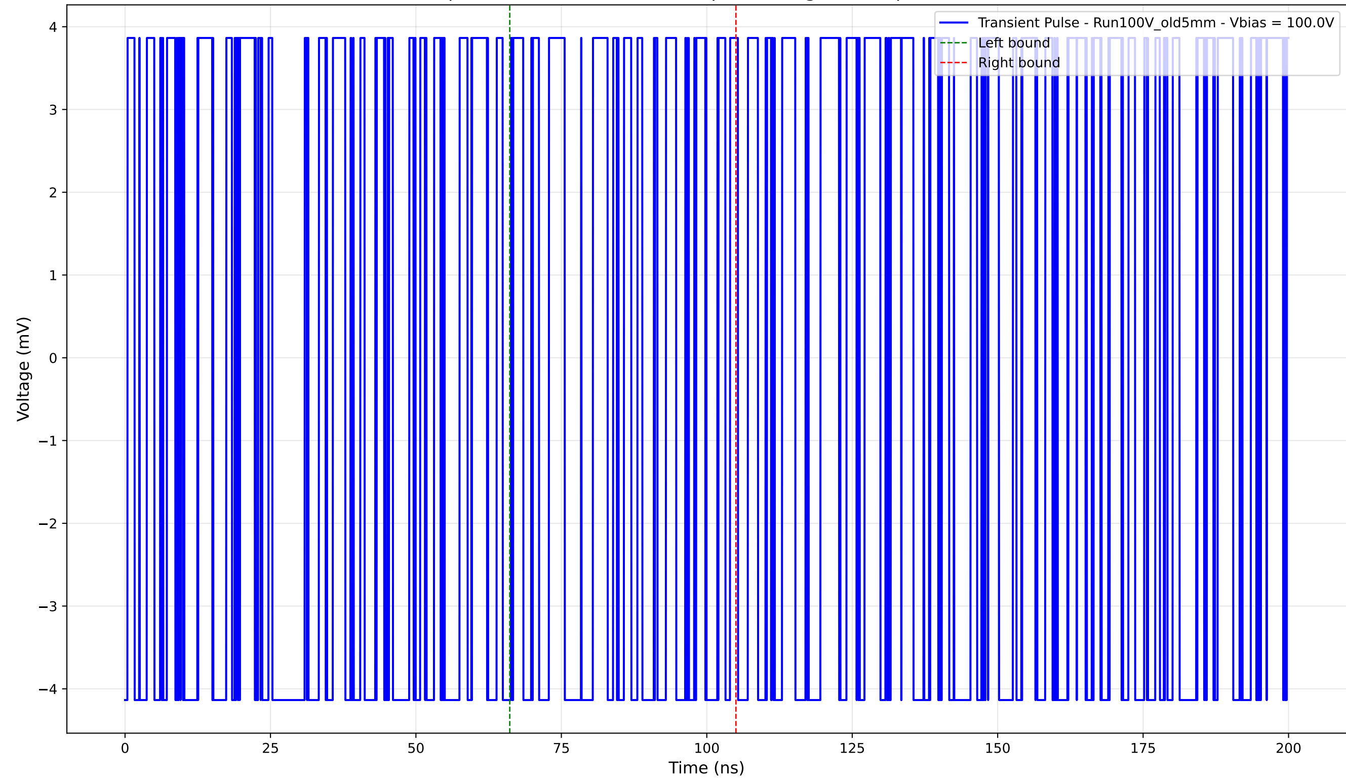
Transient Pulse - Sample: Old5mm - Position: 0.0 \mu\text{m} - Charge: -0.32 pC - Rise Time: 0.00 ns (N/A)
