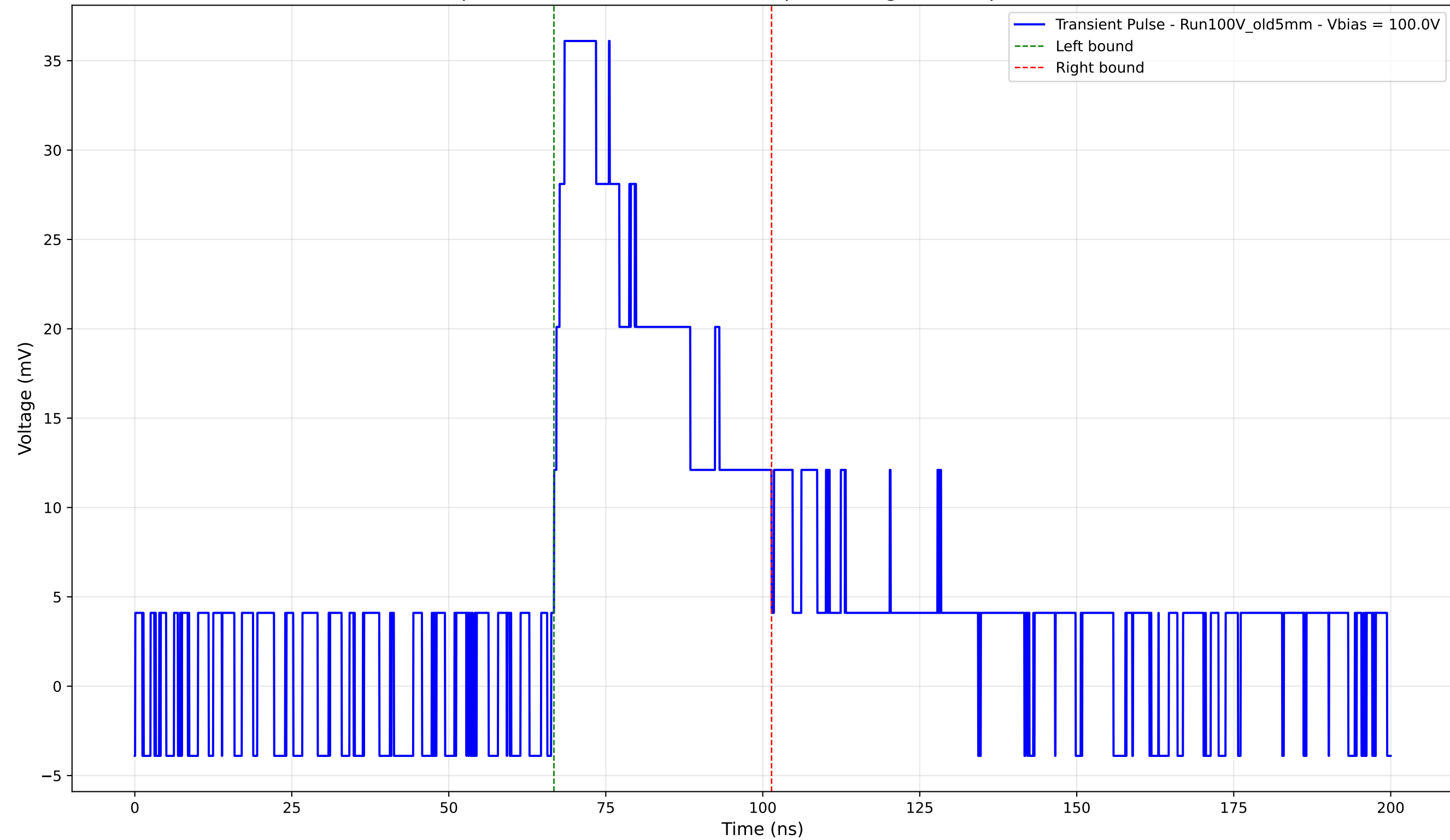
Transient Pulse - Sample: Old5mm - Position: 2630.0 \mu\text{m} - Charge: 14.42 pC - Rise Time: 0.00 ns (N/A)
