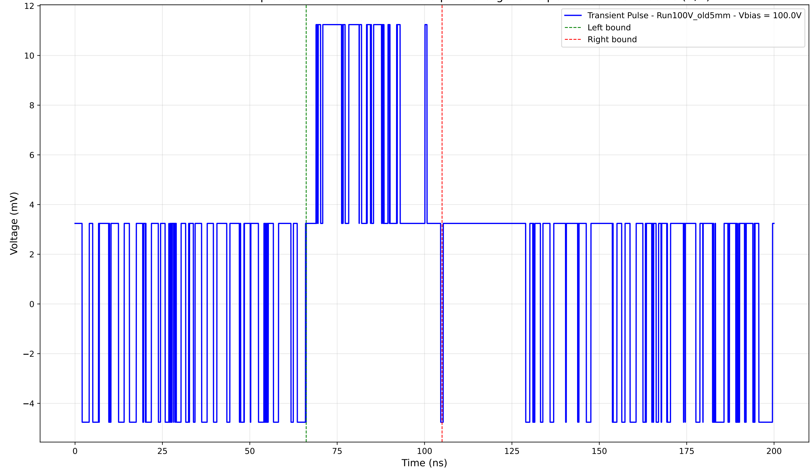
Transient Pulse - Sample: Old5mm - Position: 2155.0 \mu\text{m} - Charge: 5.16 pC - Rise Time: 0.00 ns (N/A)
