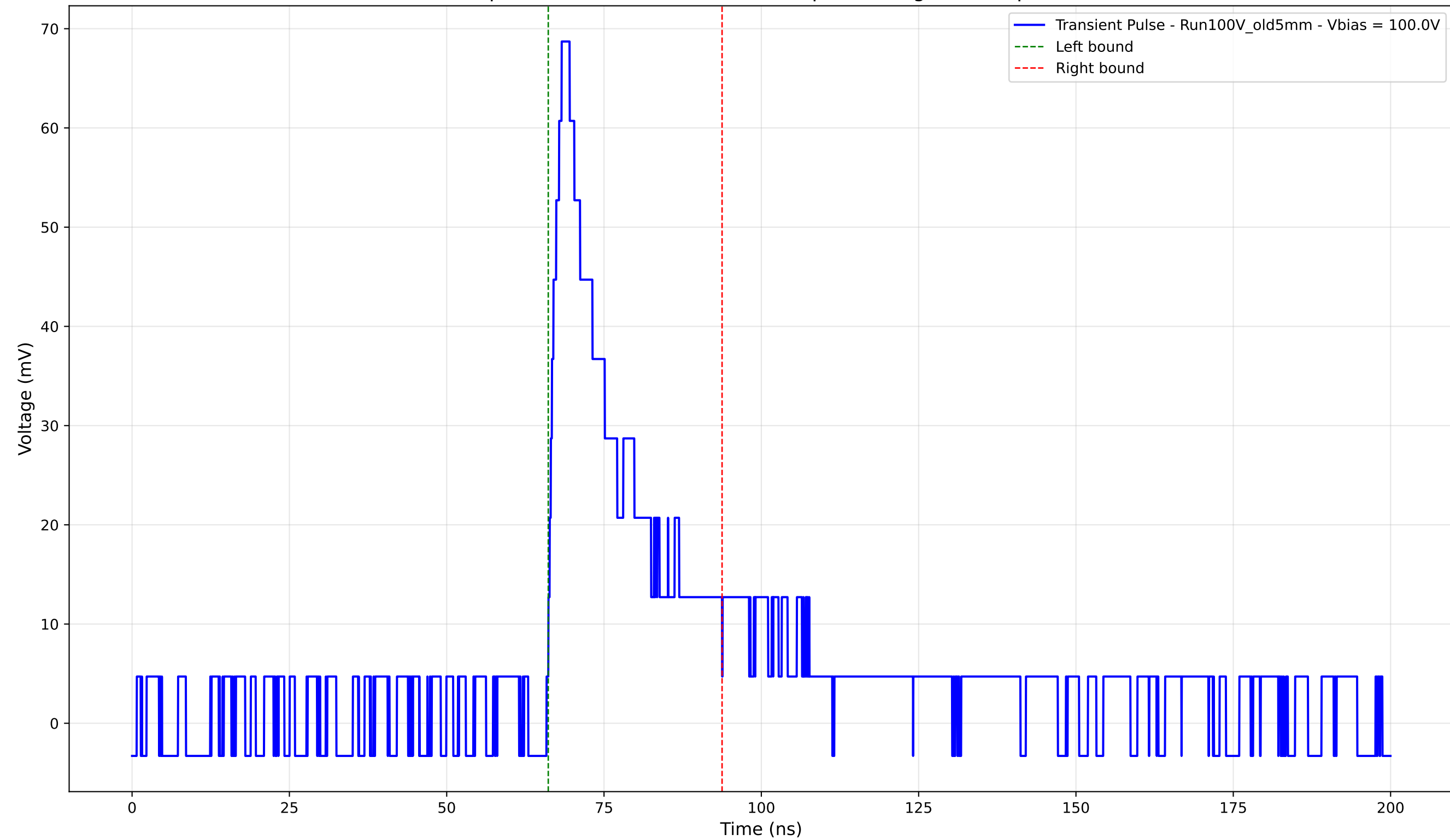
Transient Pulse - Sample: Old5mm - Position: 2970.0 \mu\text{m} - Charge: 15.33 pC - Rise Time: 2.11 ns
