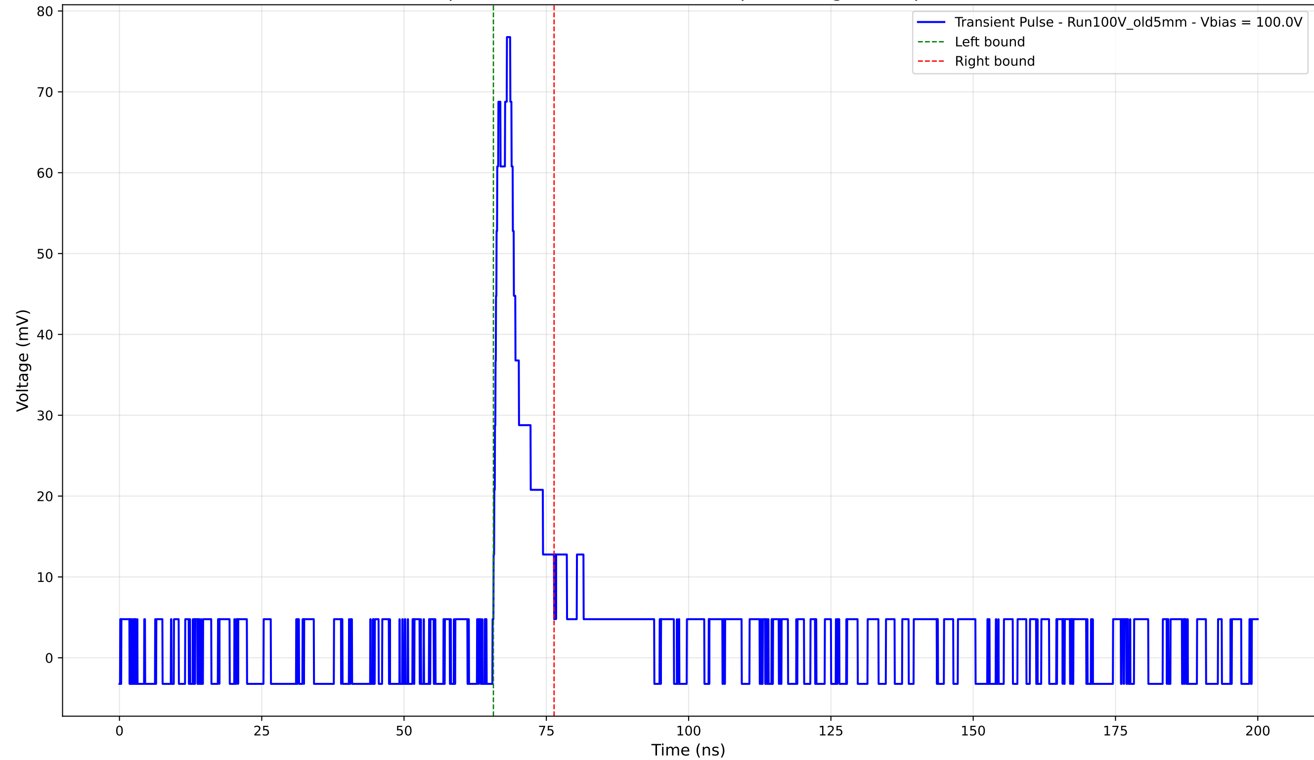
Transient Pulse - Sample: Old5mm - Position: 3945.0 \mu\text{m} - Charge: 7.57 pC - Rise Time: 2.35 ns
