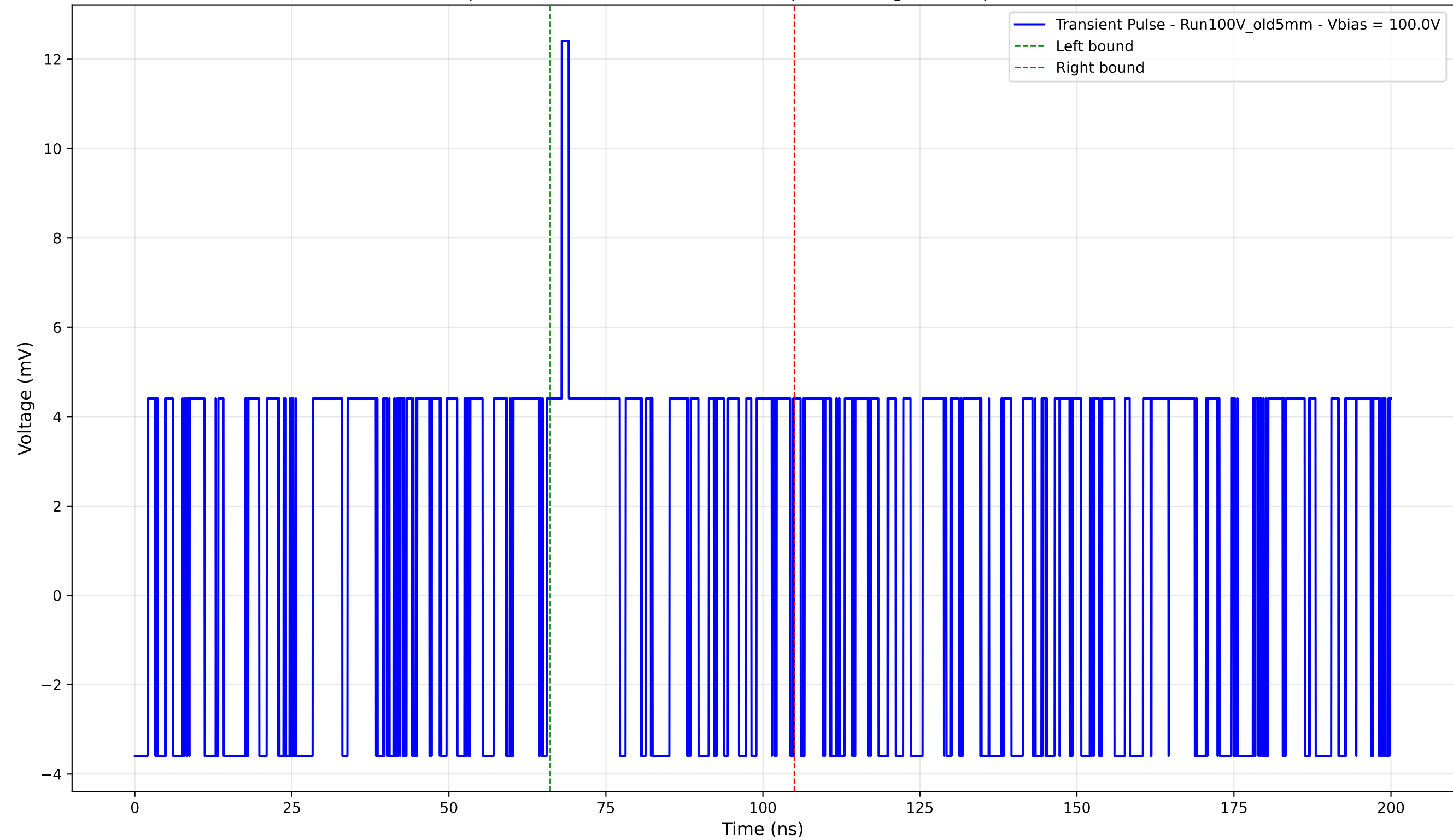
Transient Pulse - Sample: Old5mm - Position: 4005.0 \mu\text{m} - Charge: 2.00 pC - Rise Time: 0.00 ns (N/A)
