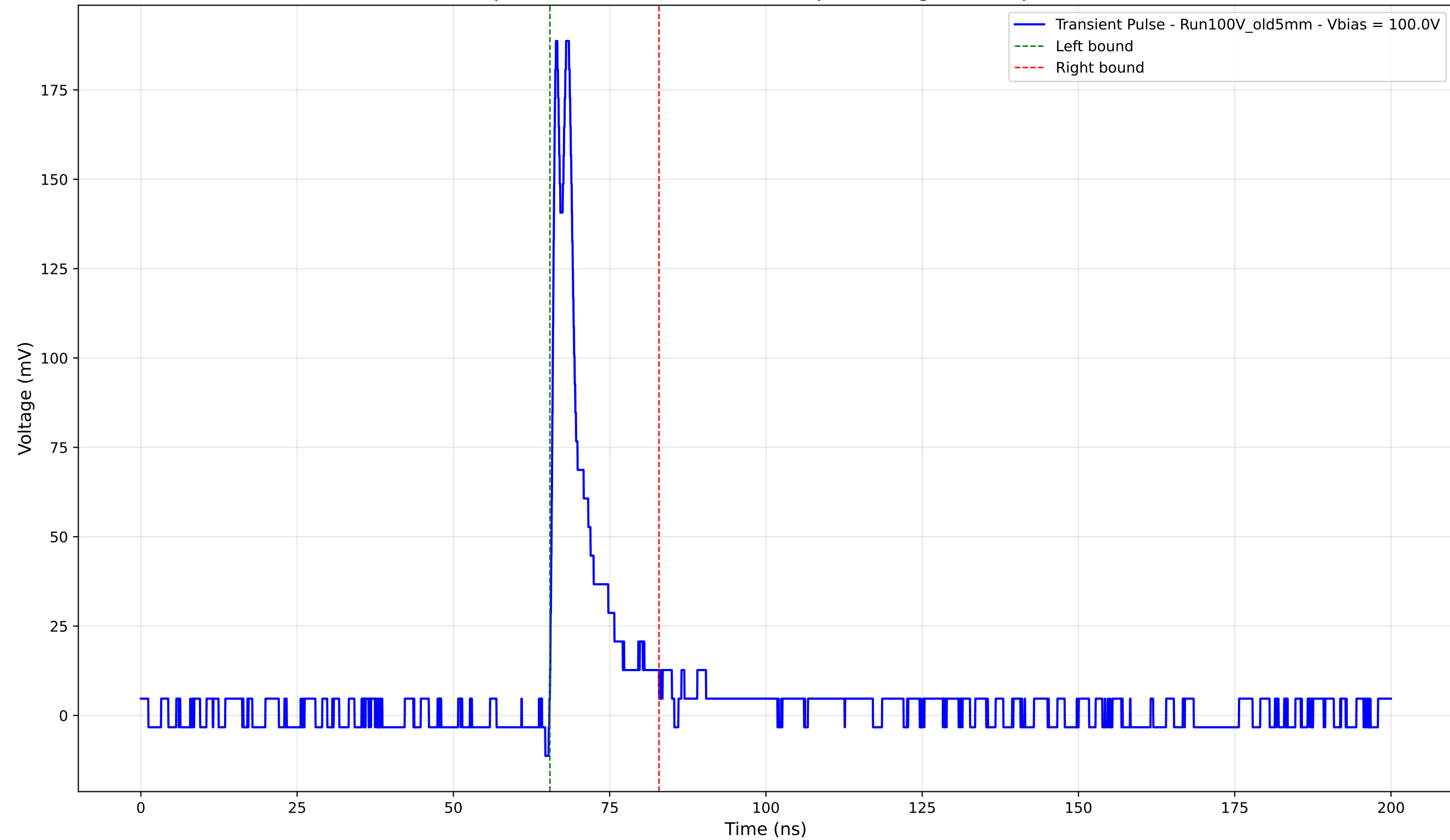
Transient Pulse - Sample: Old5mm - Position: 3850.0 \mu\text{m} - Charge: 19.78 pC - Rise Time: 0.72 ns
