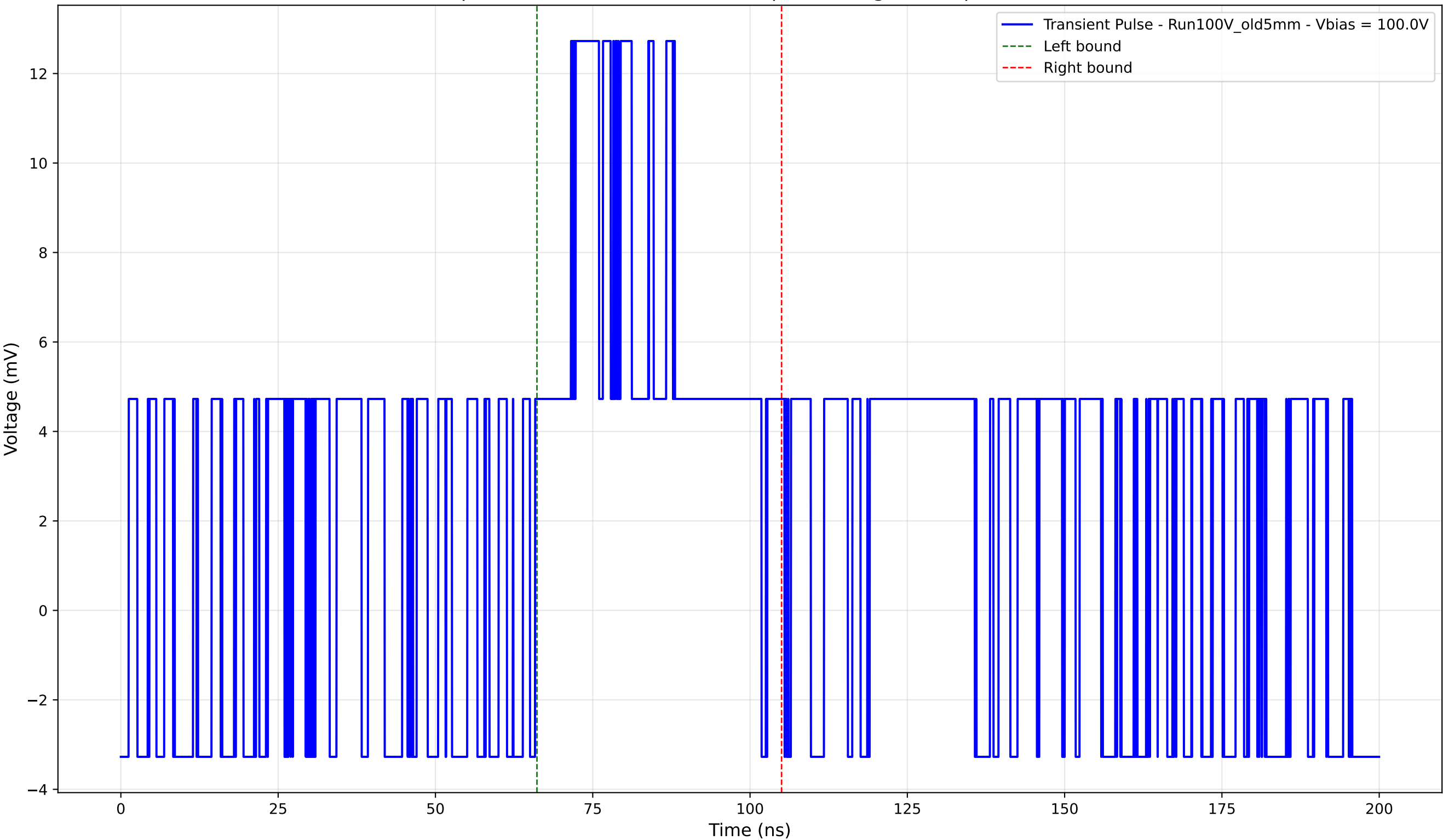
Transient Pulse - Sample: Old5mm - Position: 560.0 \mu\text{m} - Charge: 5.08 pC - Rise Time: 0.00 ns (N/A)
