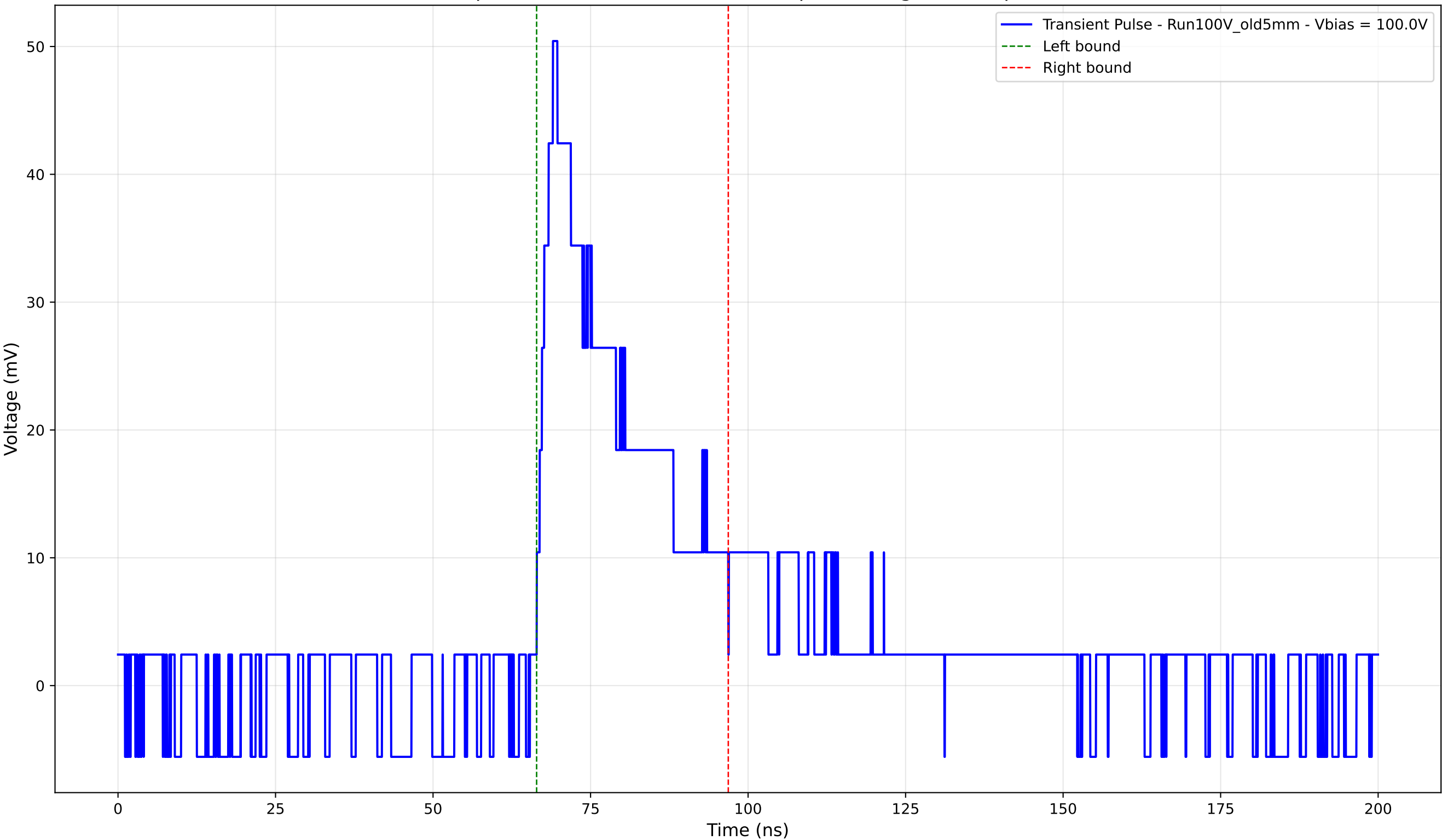
Transient Pulse - Sample: Old5mm - Position: 4755.0 \mu\text{m} - Charge: 13.57 pC - Rise Time: 2.57 ns
