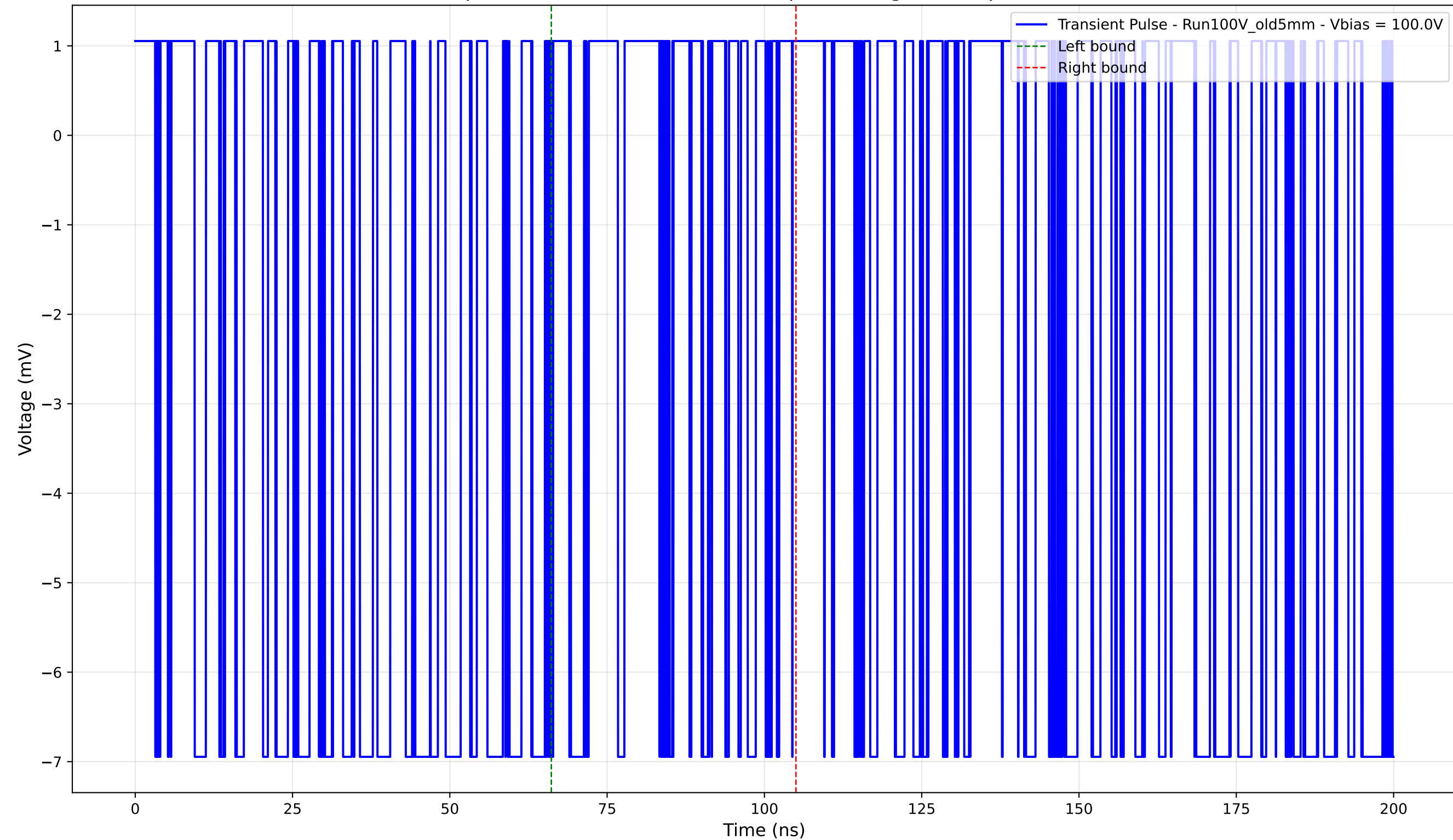
Transient Pulse - Sample: Old5mm - Position: 4630.0 \mu\text{m} - Charge: -0.74 pC - Rise Time: 0.00 ns (N/A)
