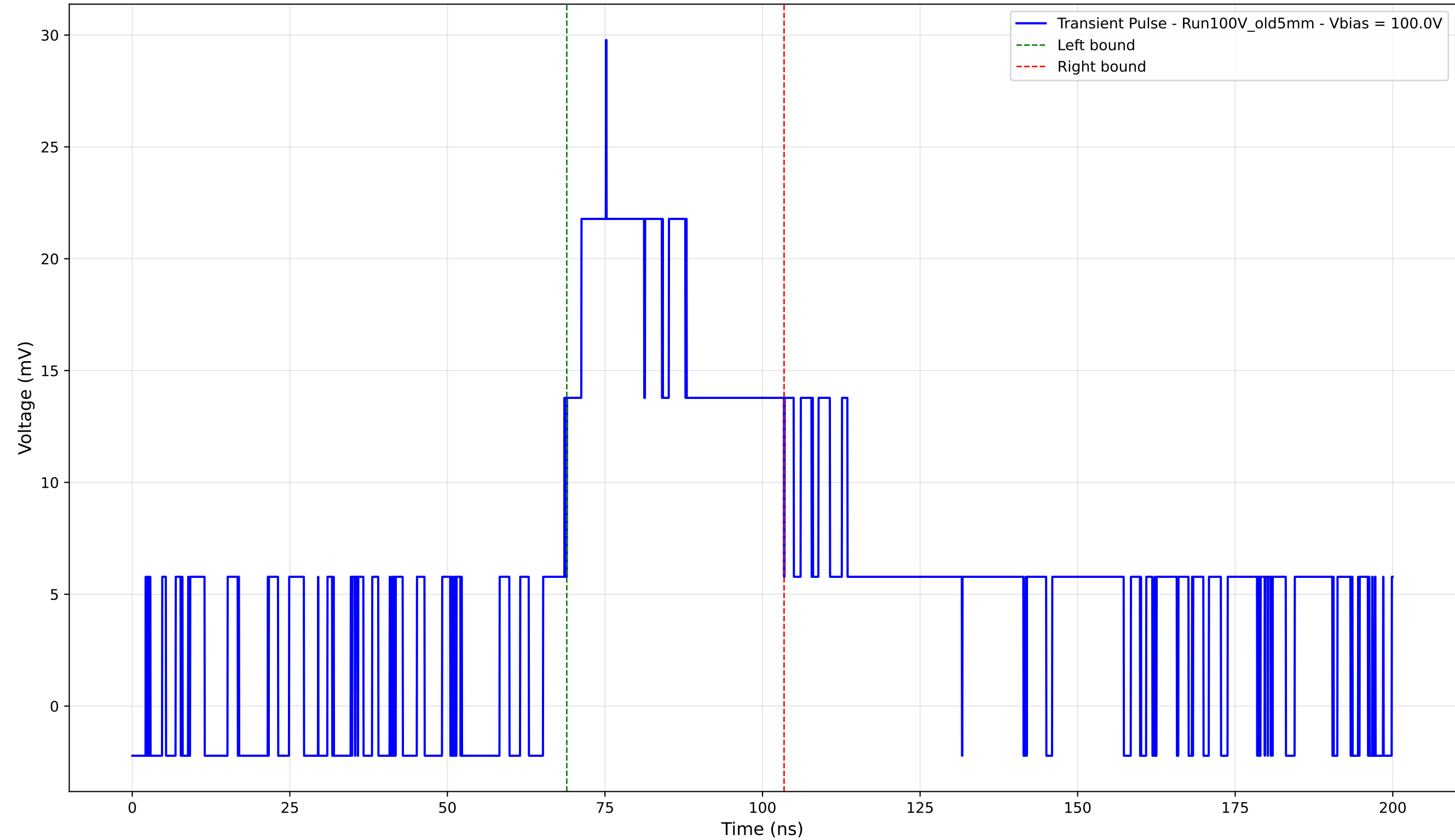
Transient Pulse - Sample: Old5mm - Position: 2030.0 \mu\text{m} - Charge: 11.97 pC - Rise Time: 10.00 ns
