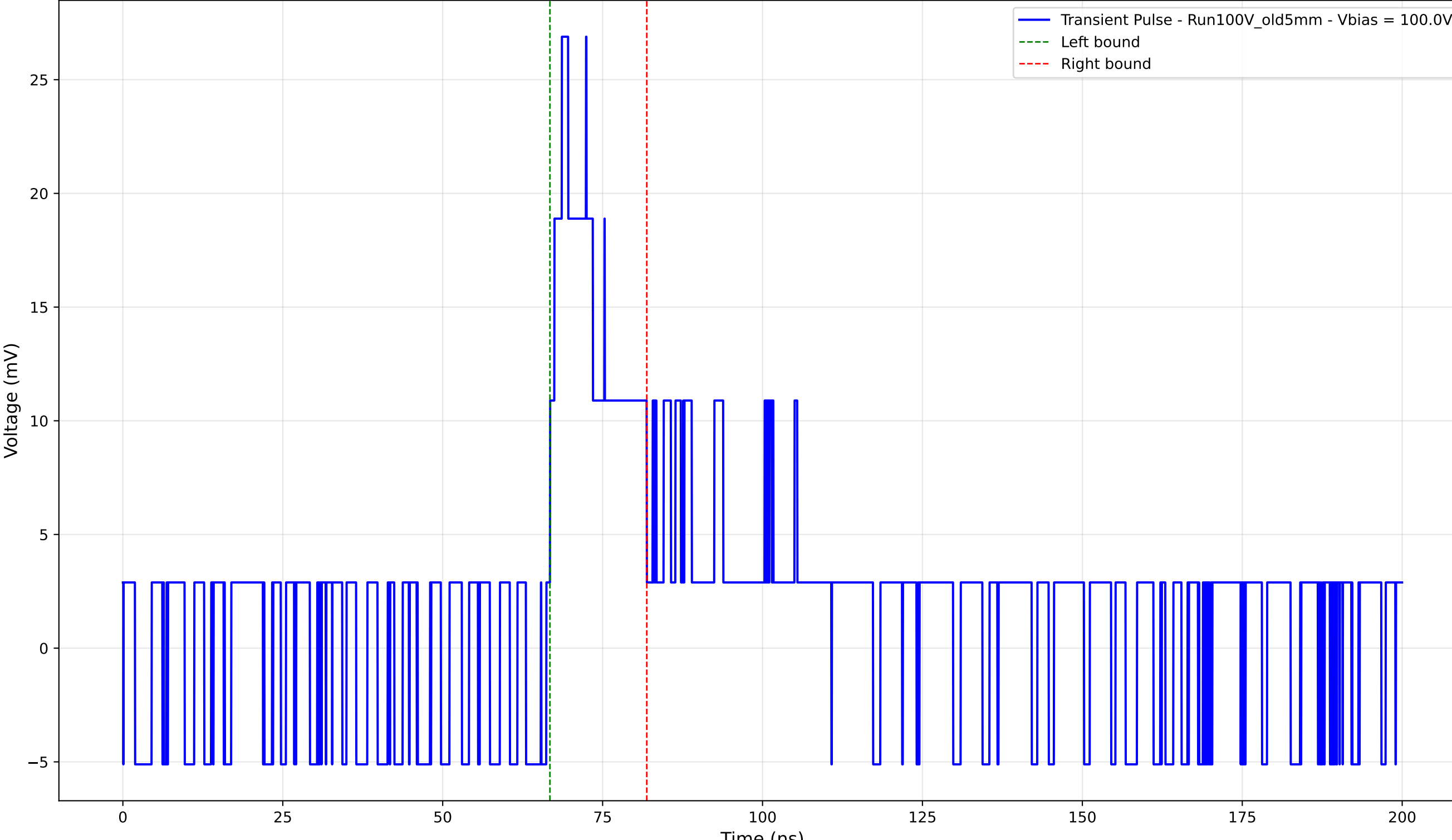
Transient Pulse - Sample: Old5mm - Position: 4685.0 \mu\text{m} - Charge: 4.44 pC - Rise Time: 0.00 ns (N/A)
