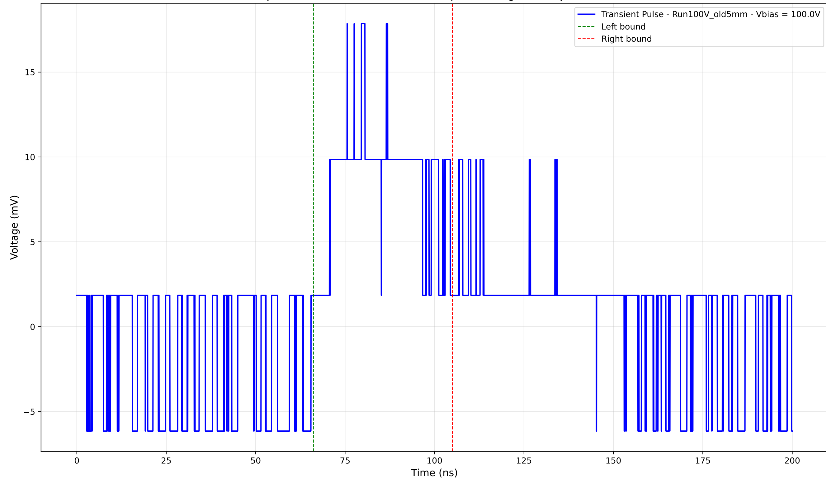
Transient Pulse - Sample: Old5mm - Position: 1645.0 \mu\text{m} - Charge: 6.54 pC - Rise Time: 0.00 ns (N/A)
