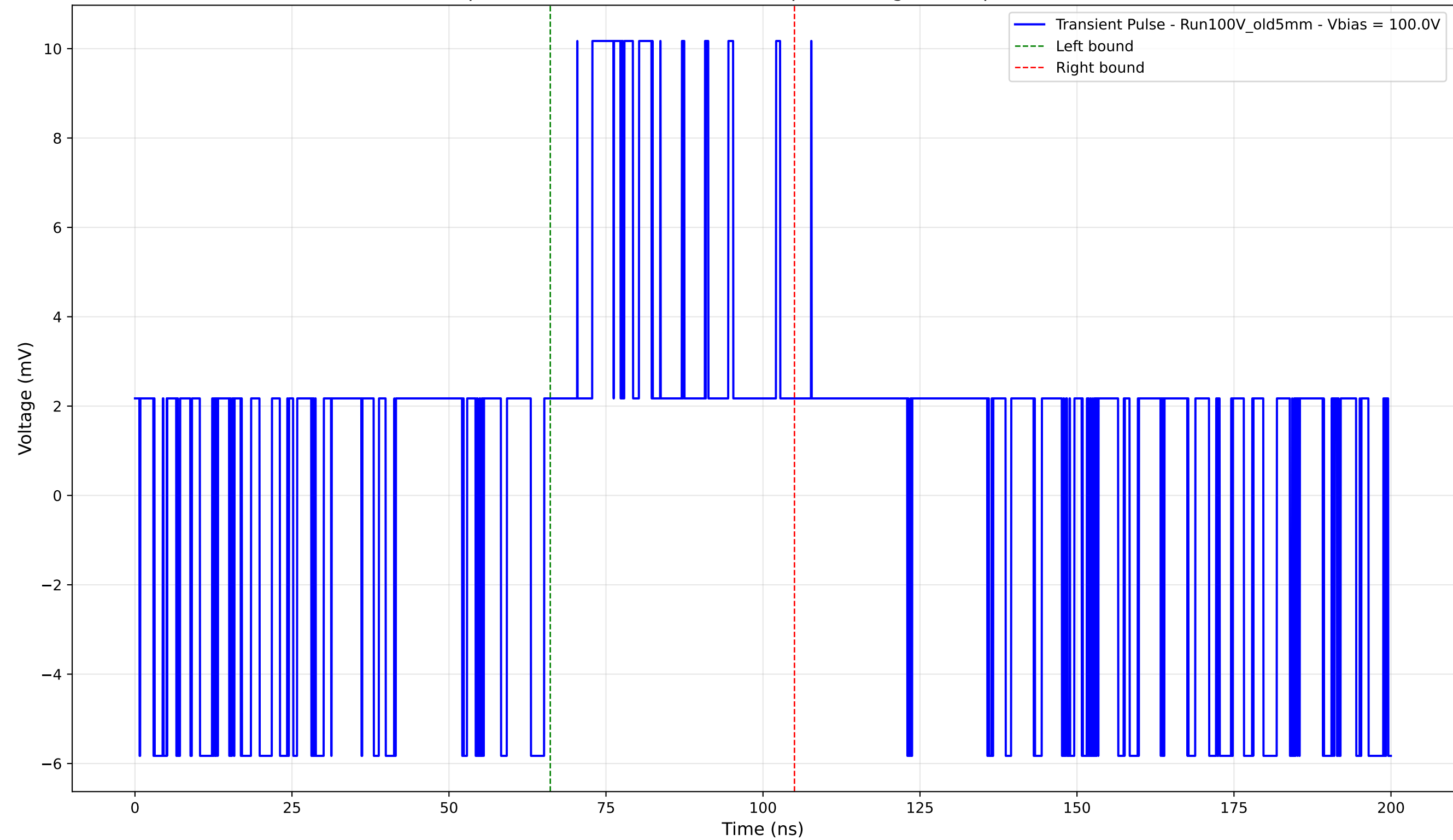
Transient Pulse - Sample: Old5mm - Position: 1000.0 \mu\text{m} - Charge: 3.33 pC - Rise Time: 0.00 ns (N/A)
