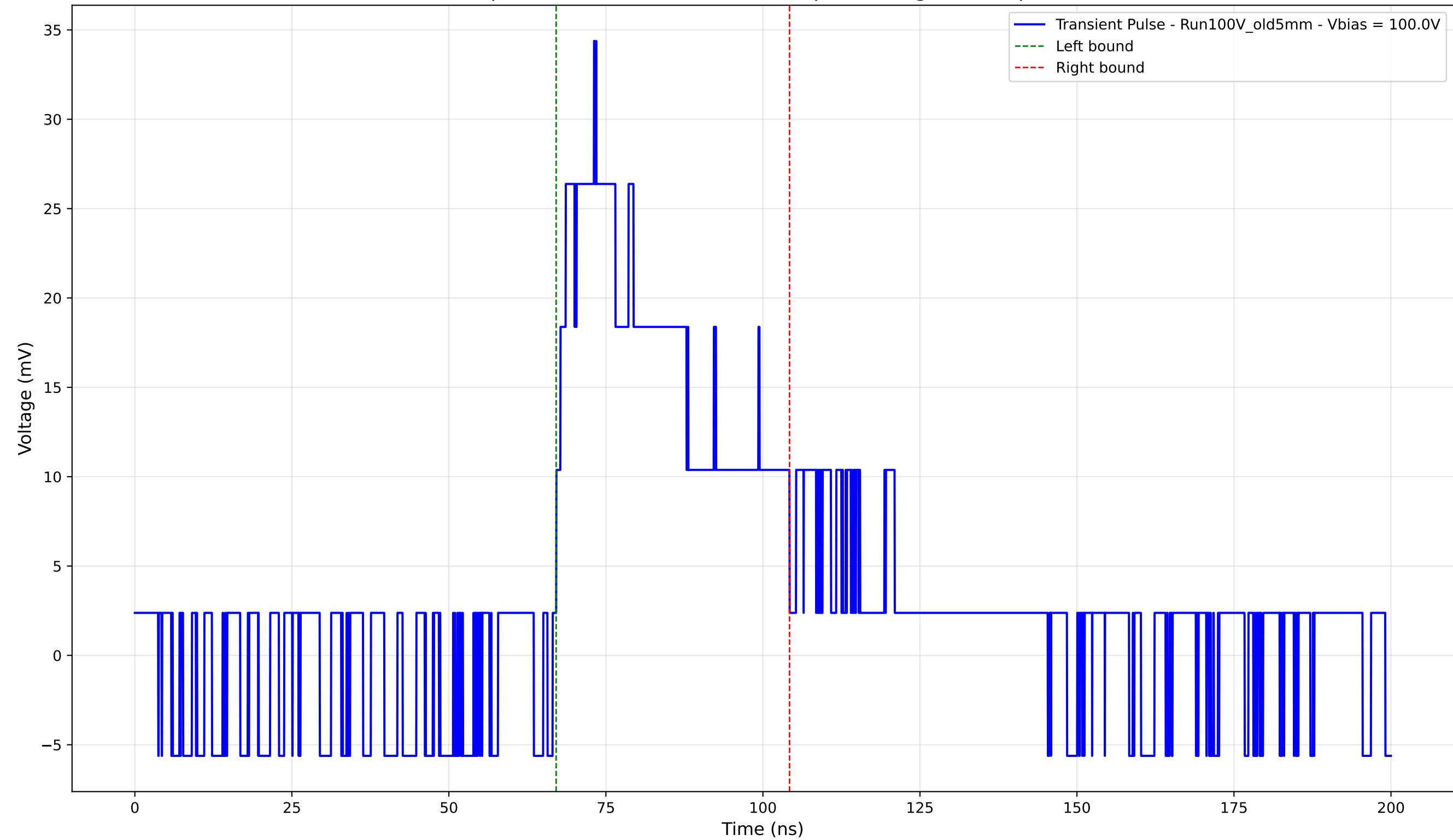
Transient Pulse - Sample: Old5mm - Position: 2425.0 \mu\text{m} - Charge: 12.42 pC - Rise Time: 6.02 ns
