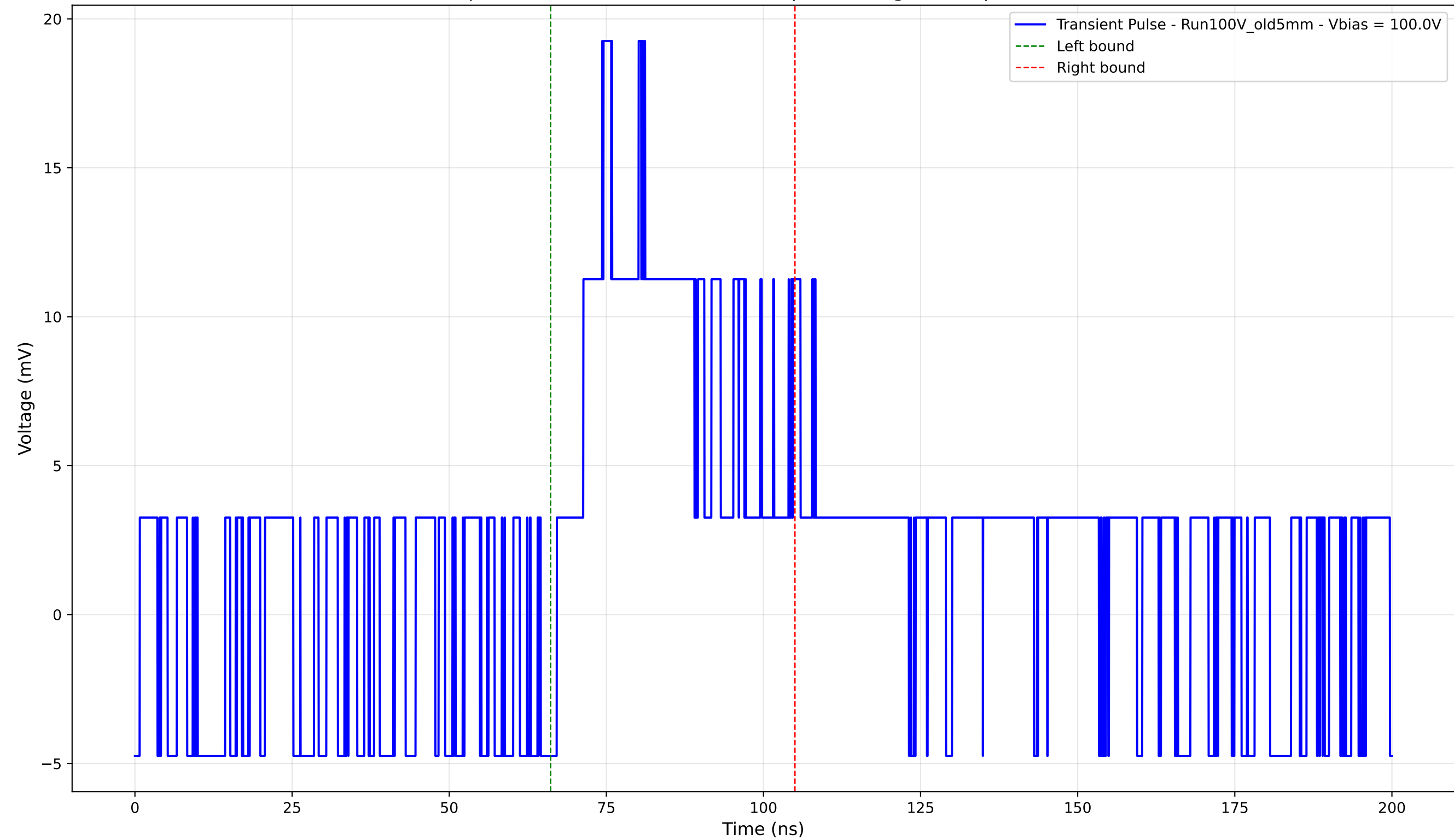
Transient Pulse - Sample: Old5mm - Position: 1445.0 \mu\text{m} - Charge: 6.42 pC - Rise Time: 0.00 ns (N/A)
