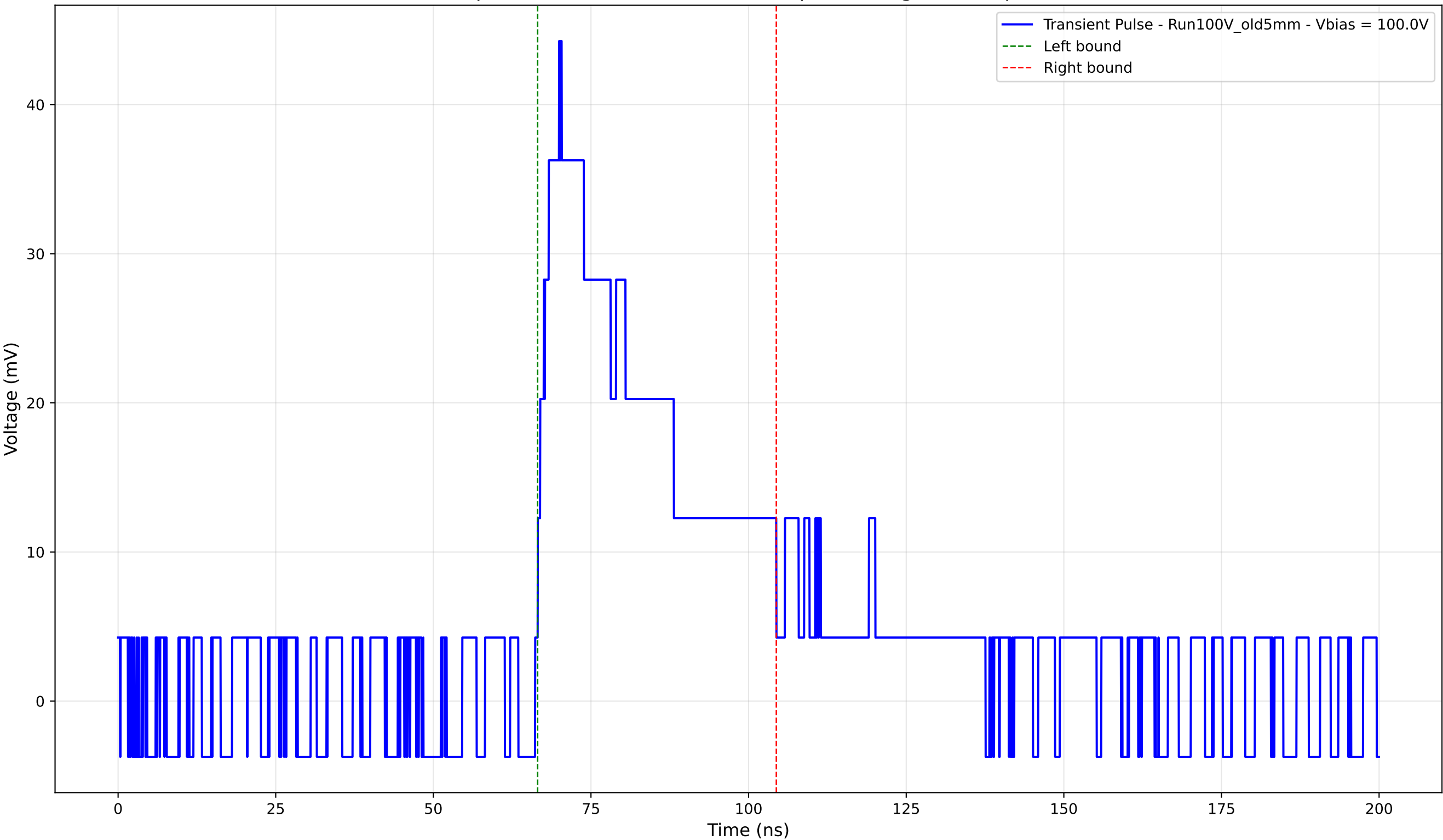
Transient Pulse - Sample: Old5mm - Position: 2660.0 \mu\text{m} - Charge: 15.54 pC - Rise Time: 3.40 ns
