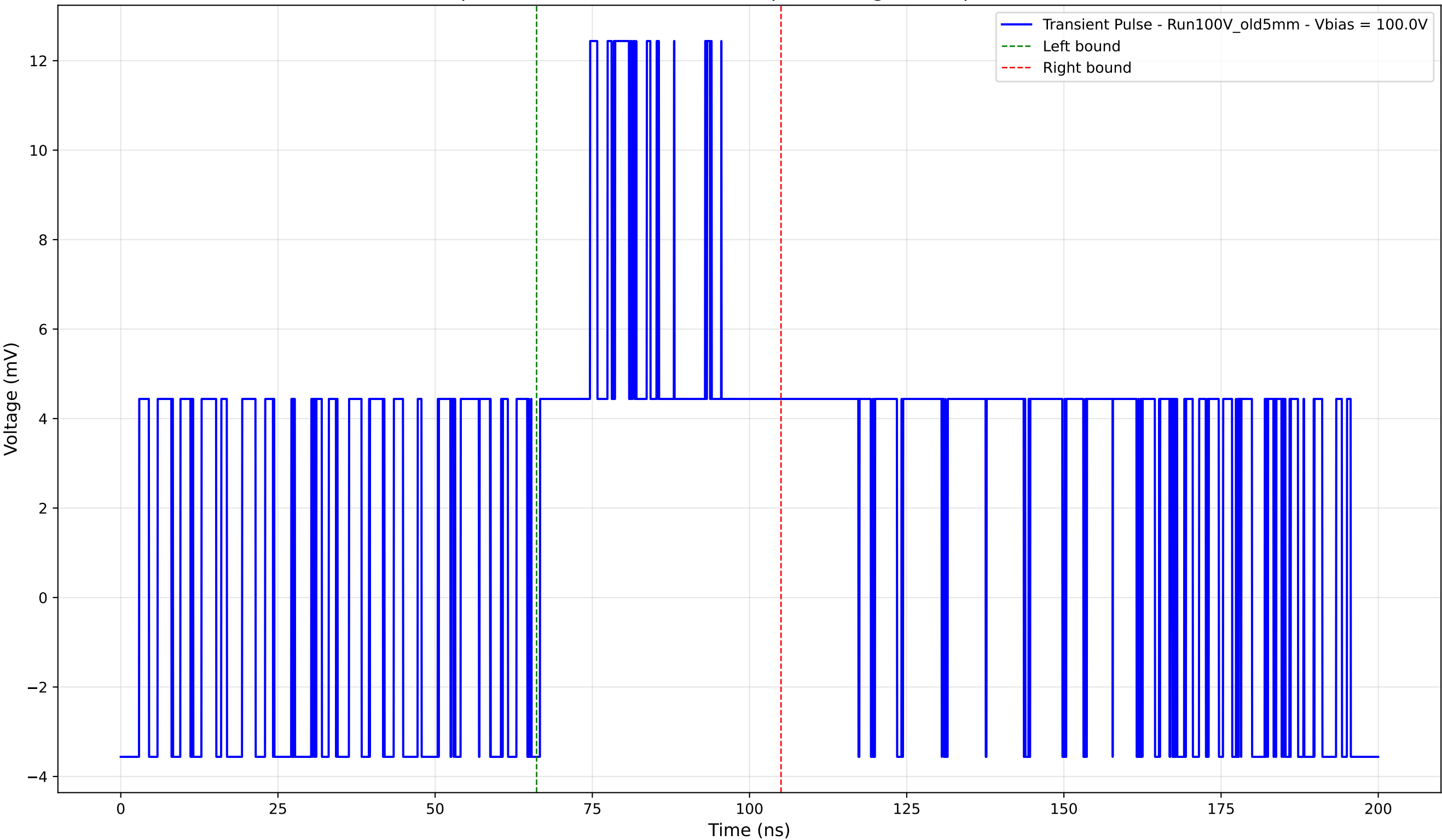
Transient Pulse - Sample: Old5mm - Position: 805.0 \mu\text{m} - Charge: 4.37 pC - Rise Time: 0.00 ns (N/A)
