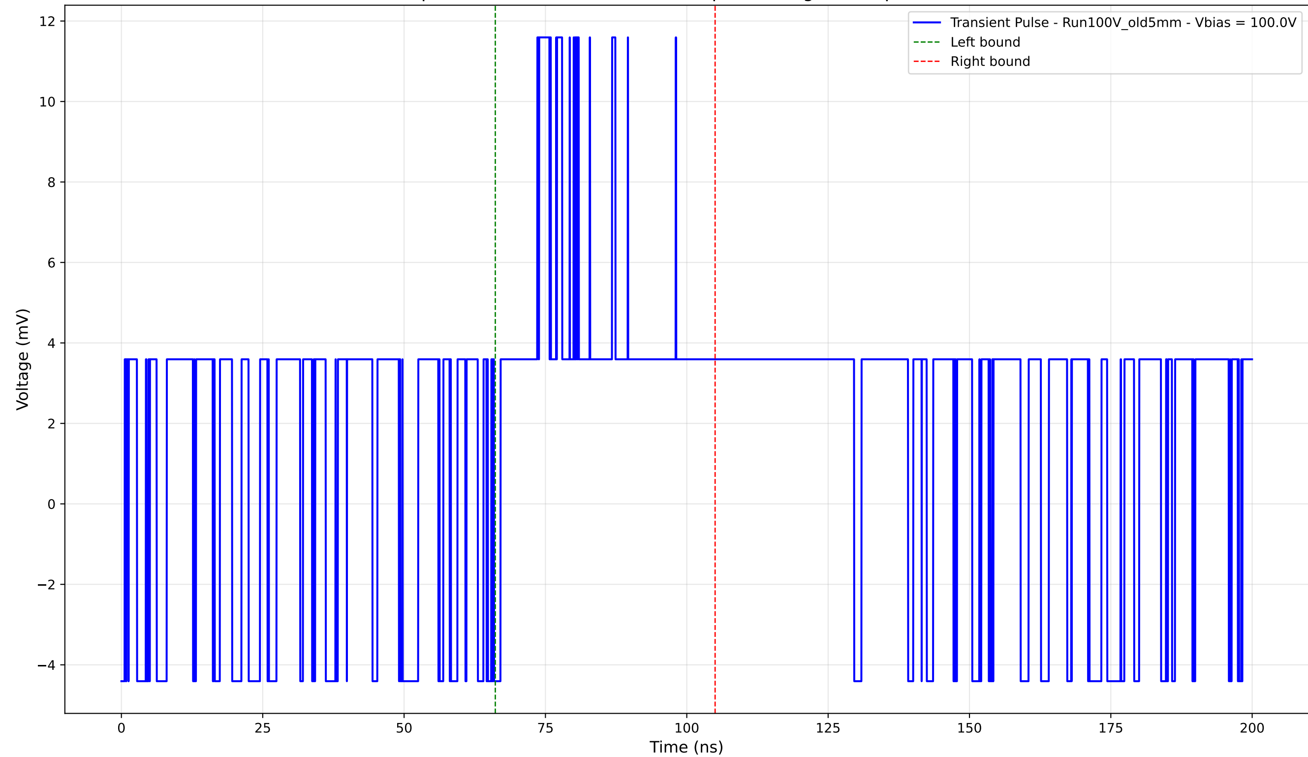
Transient Pulse - Sample: Old5mm - Position: 1475.0 \mu\text{m} - Charge: 3.37 pC - Rise Time: 0.00 ns (N/A)
