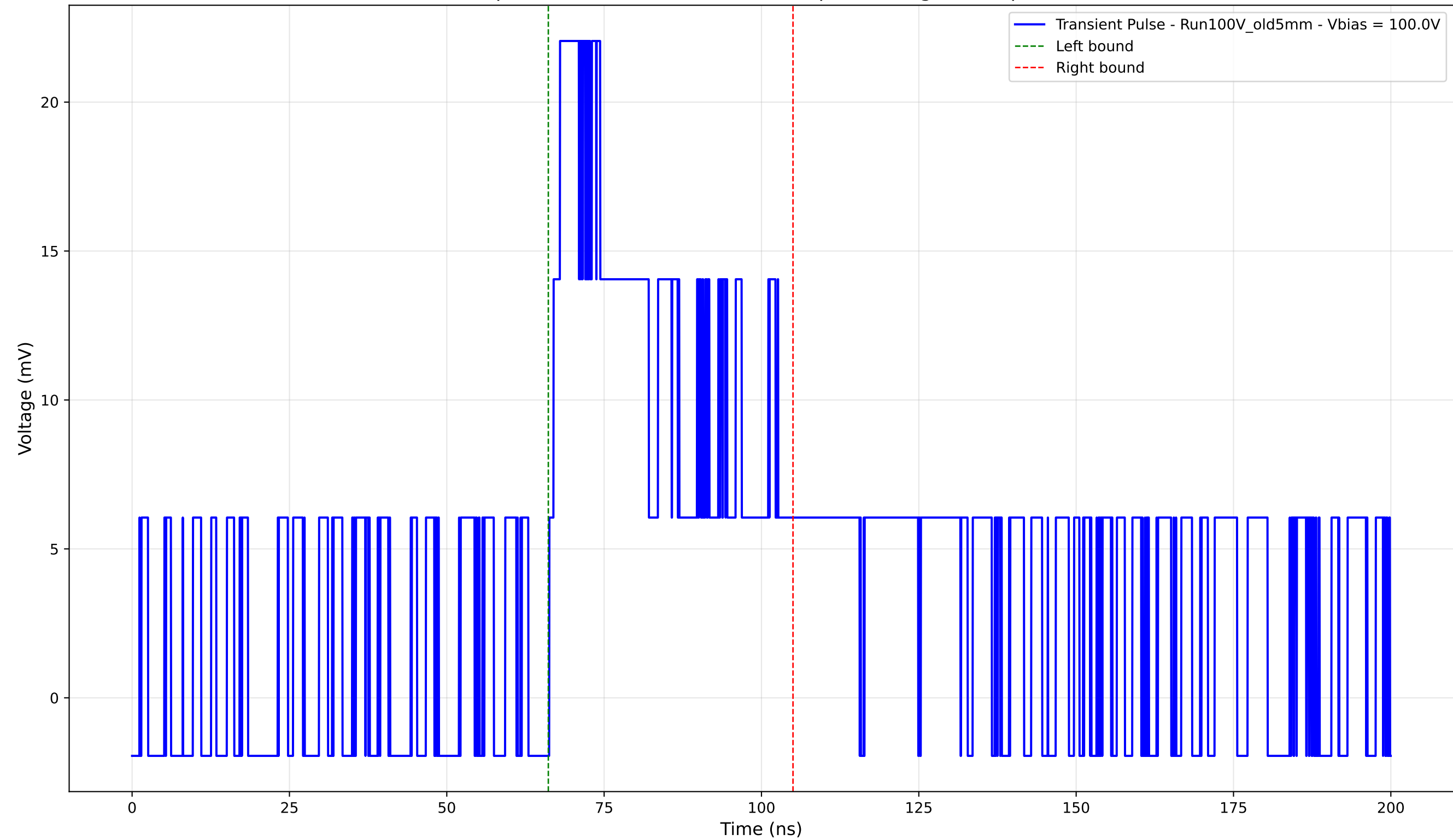
Transient Pulse - Sample: Old5mm - Position: 2730.0 \mu\text{m} - Charge: 9.20 pC - Rise Time: 1.72 ns
