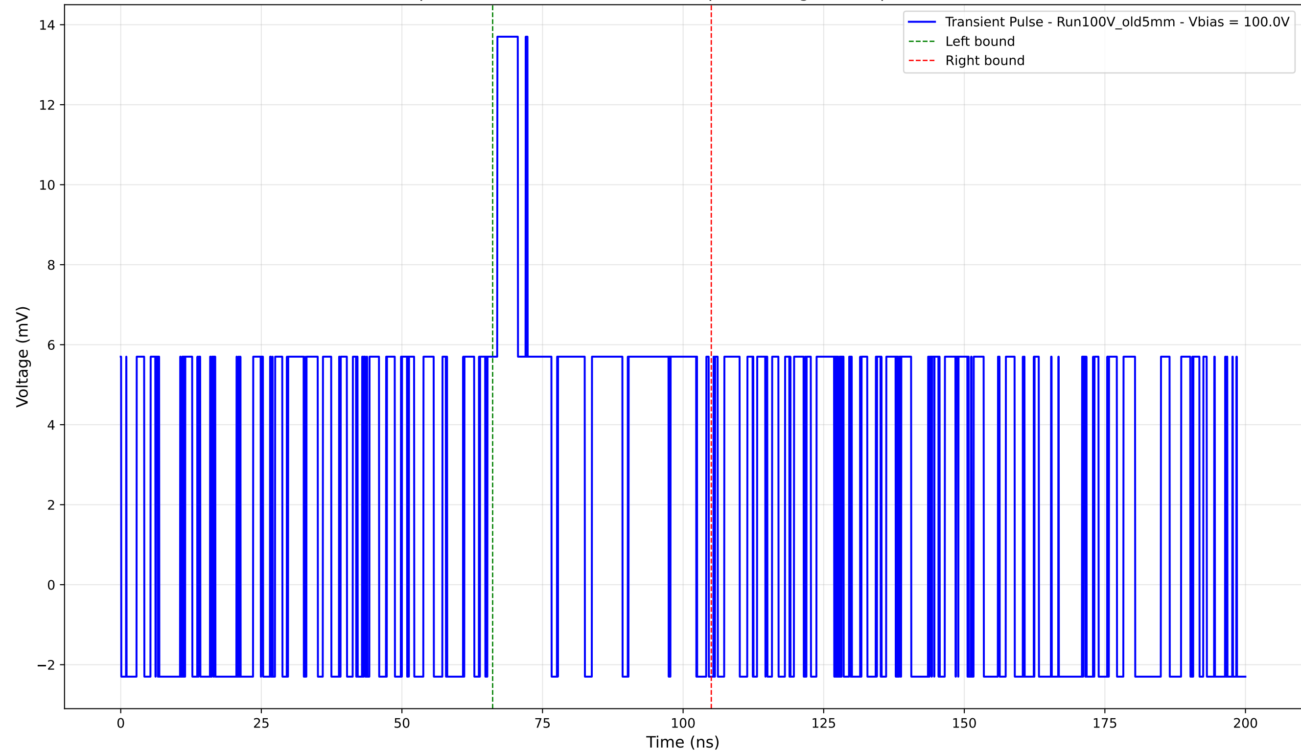
Transient Pulse - Sample: Old5mm - Position: 4270.0 \mu\text{m} - Charge: 4.14 pC - Rise Time: 0.00 ns (N/A)
