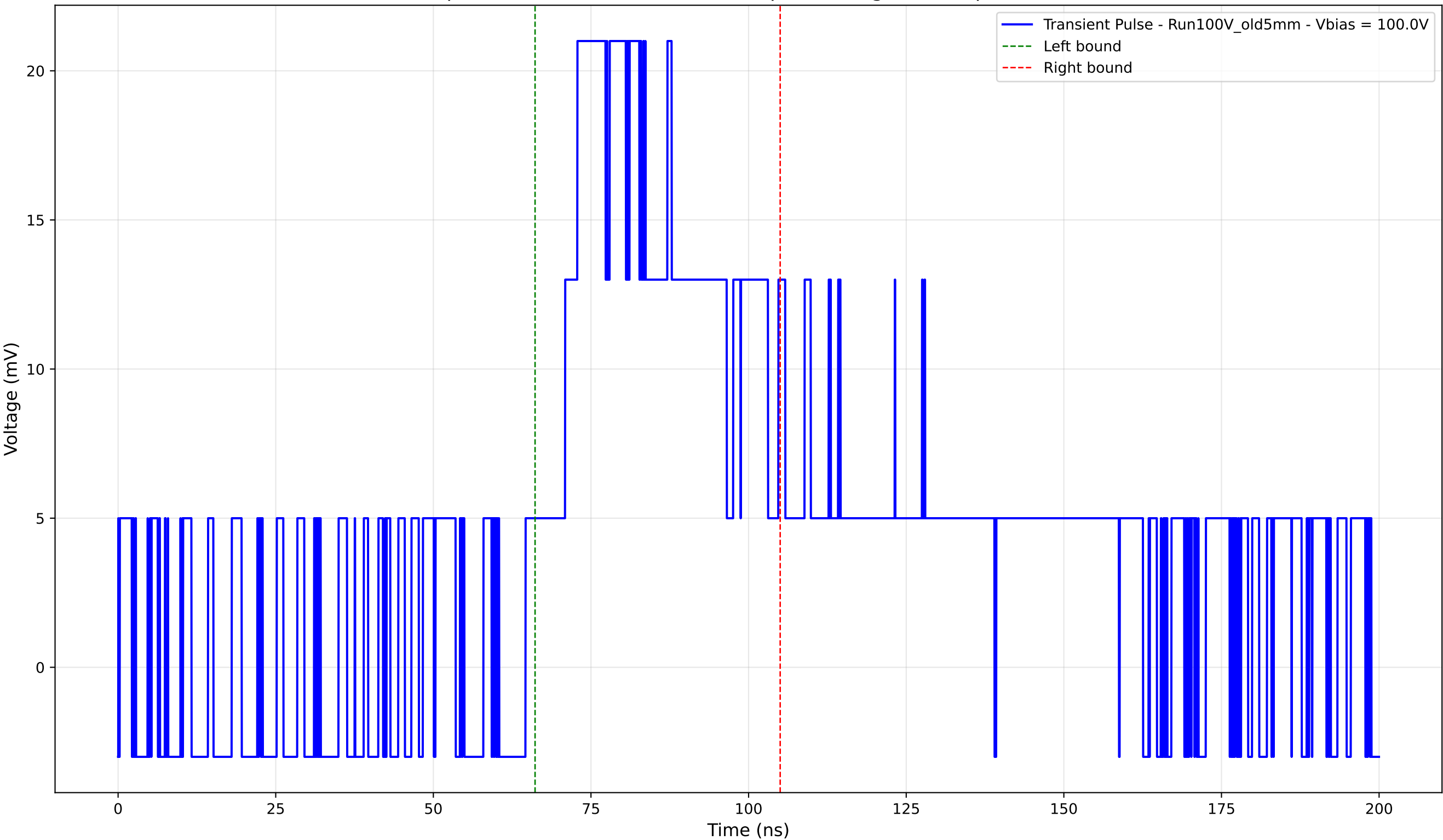
Transient Pulse - Sample: Old5mm - Position: 1610.0 \mu\text{m} - Charge: 10.48 pC - Rise Time: 0.00 ns (N/A)
