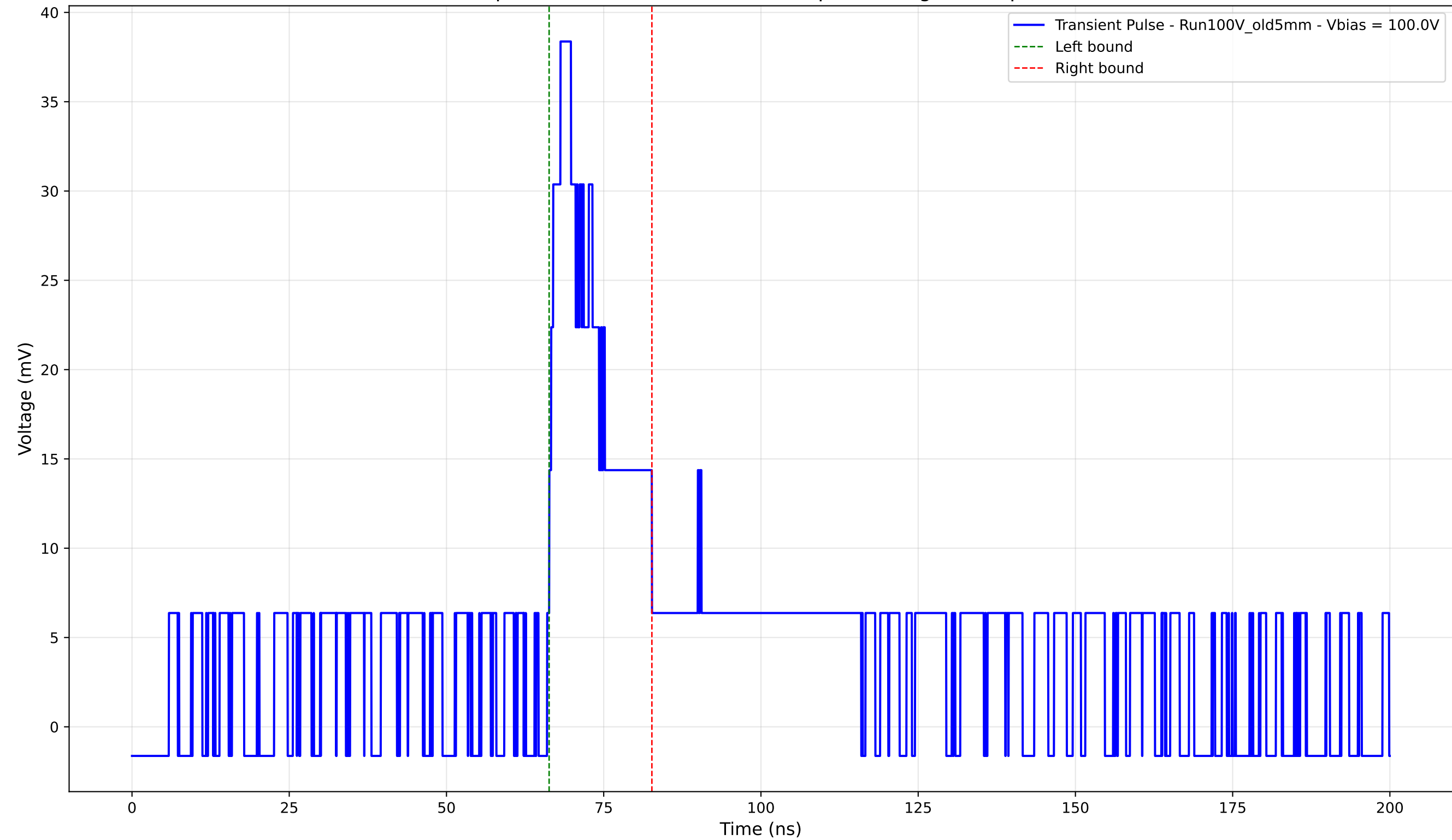
Transient Pulse - Sample: Old5mm - Position: 4380.0 \mu\text{m} - Charge: 7.03 pC - Rise Time: 2.13 ns
