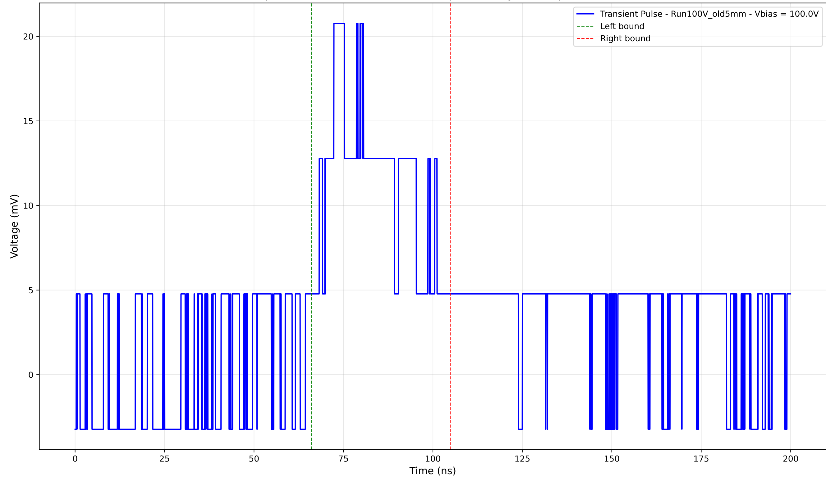
Transient Pulse - Sample: Old5mm - Position: 2060.0 \mu\text{m} - Charge: 8.61 pC - Rise Time: 0.00 ns (N/A)
