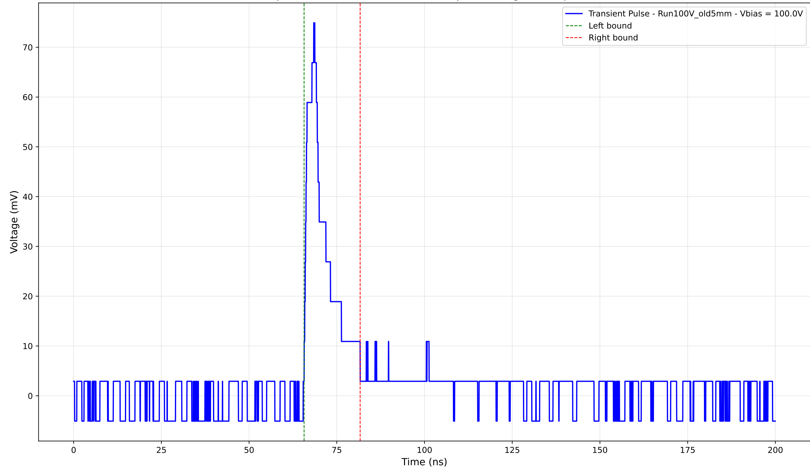
Transient Pulse - Sample: Old5mm - Position: 4085.0 \mu\text{m} - Charge: 9.08 pC - Rise Time: 2.73 ns
