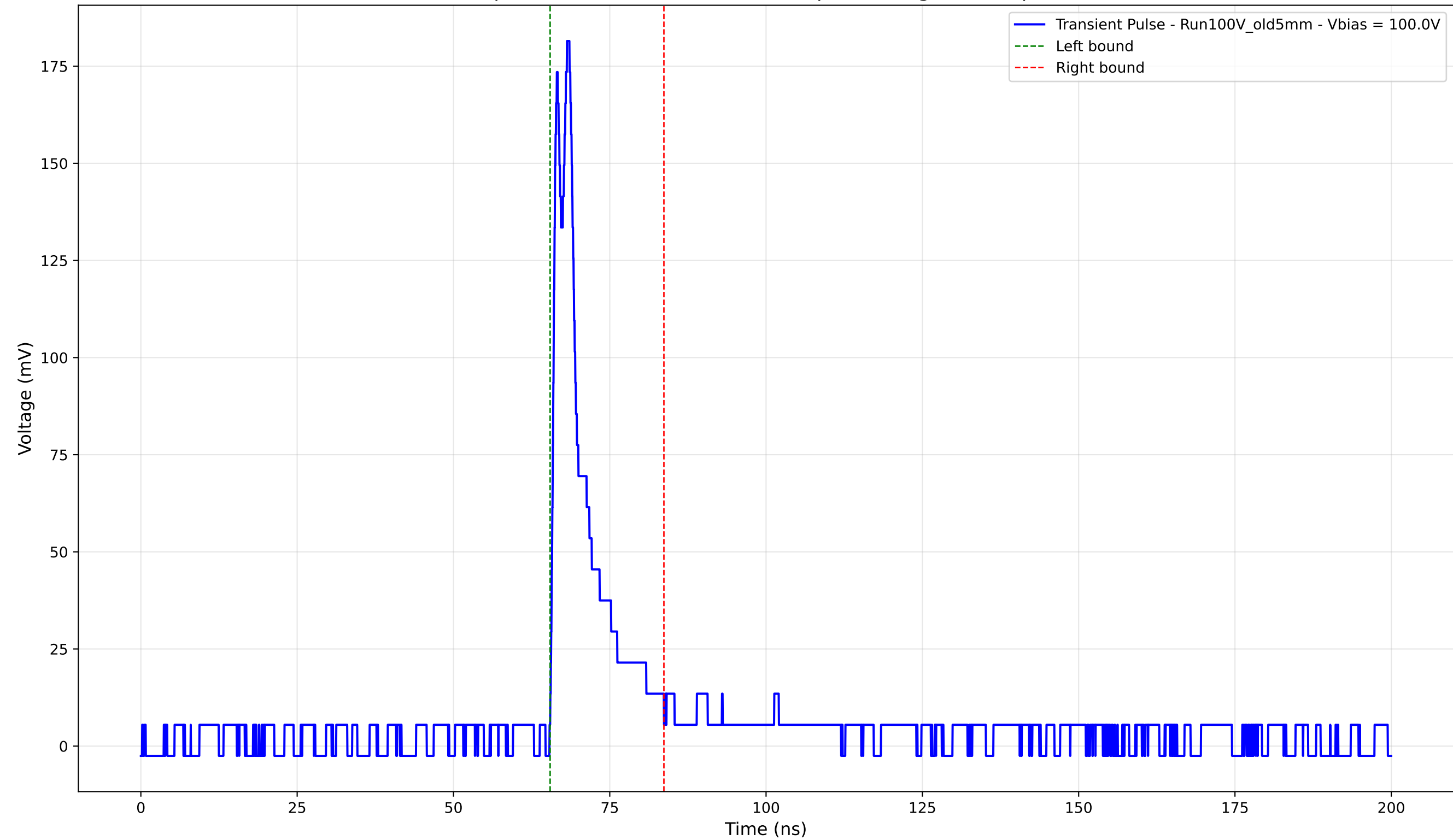
Transient Pulse - Sample: Old5mm - Position: 3535.0 \mu\text{m} - Charge: 20.47 pC - Rise Time: 0.85 ns
