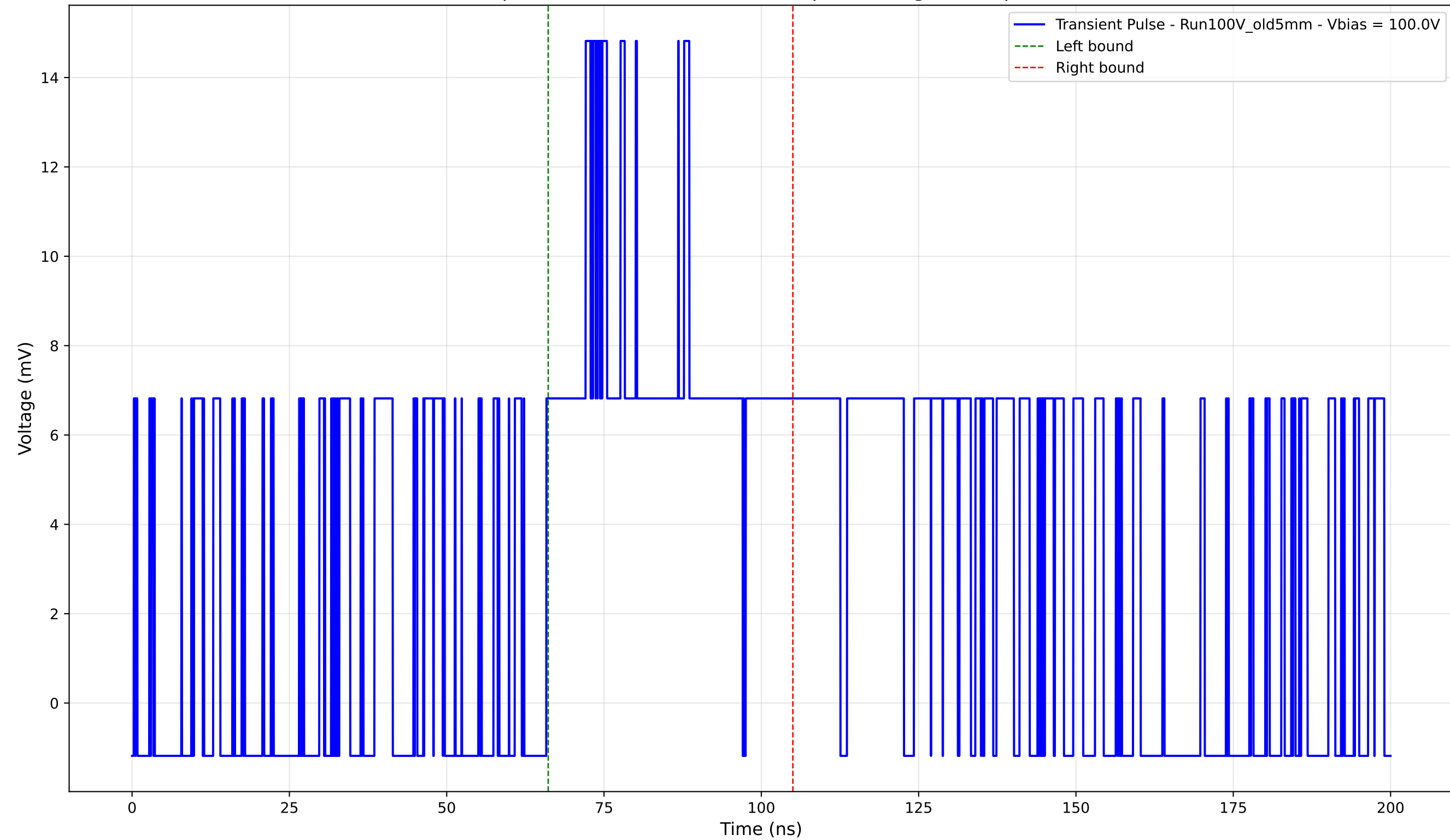
Transient Pulse - Sample: Old5mm - Position: 610.0 \mu\text{m} - Charge: 5.99 pC - Rise Time: 6.26 ns
