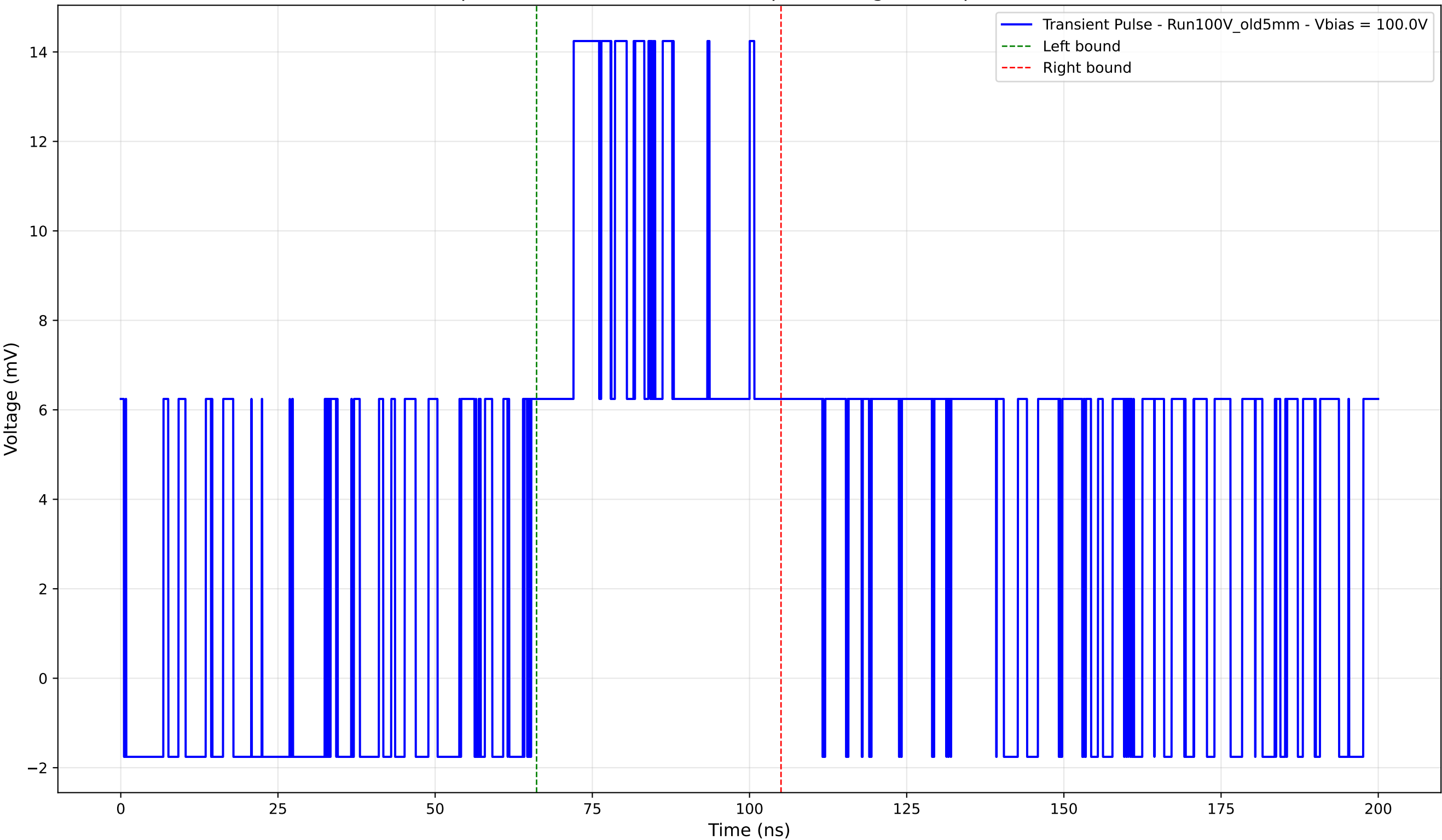
Transient Pulse - Sample: Old5mm - Position: 885.0 \mu\text{m} - Charge: 6.82 pC - Rise Time: 0.00 ns (N/A)
