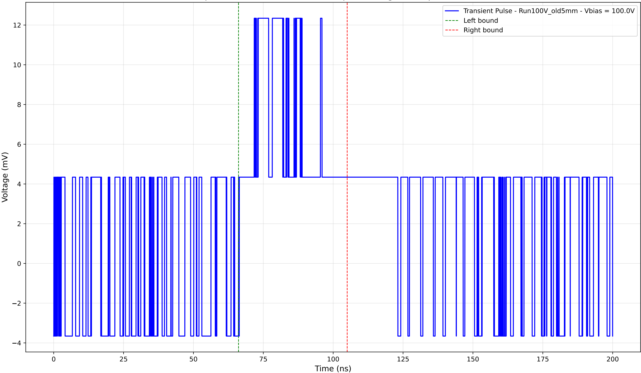
Transient Pulse - Sample: Old5mm - Position: 590.0 \mu\text{m} - Charge: 5.18 pC - Rise Time: 0.00 ns (N/A)
