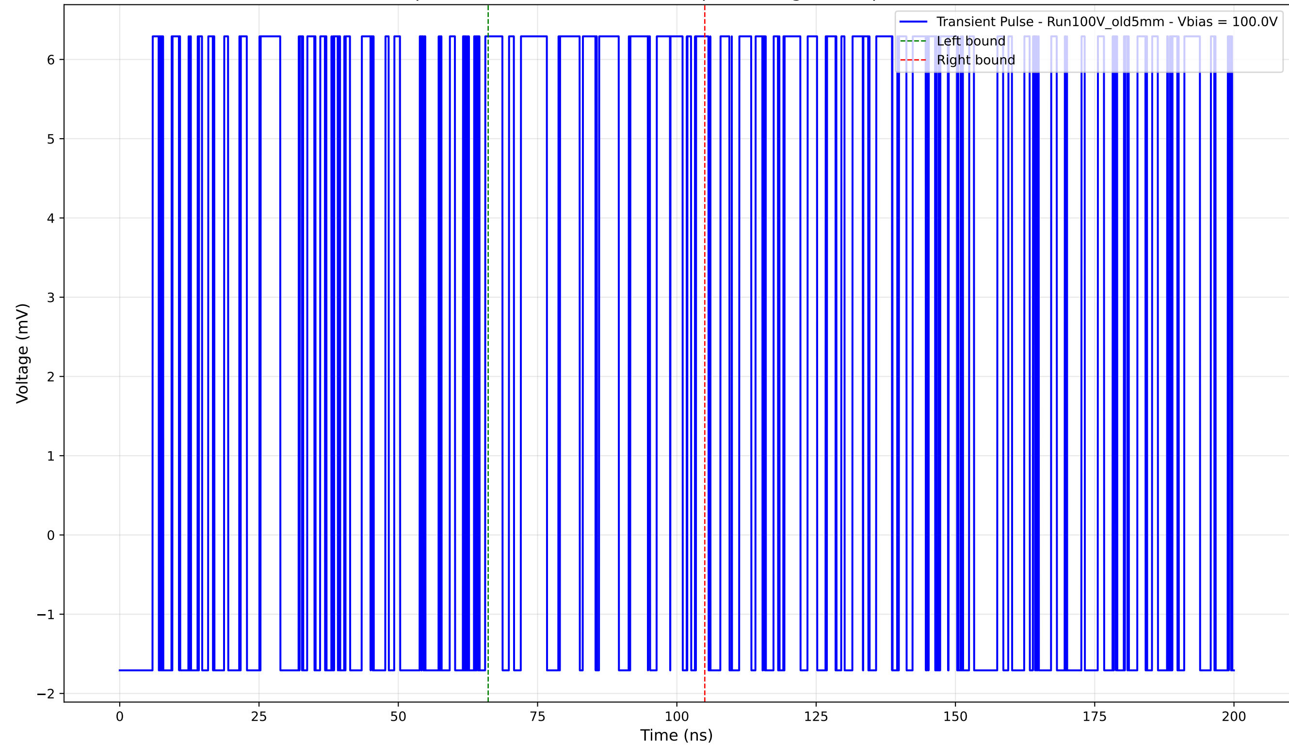
Transient Pulse - Sample: Old5mm - Position: 1315.0 \mu\text{m} - Charge: 3.22 pC - Rise Time: 0.00 ns (N/A)
