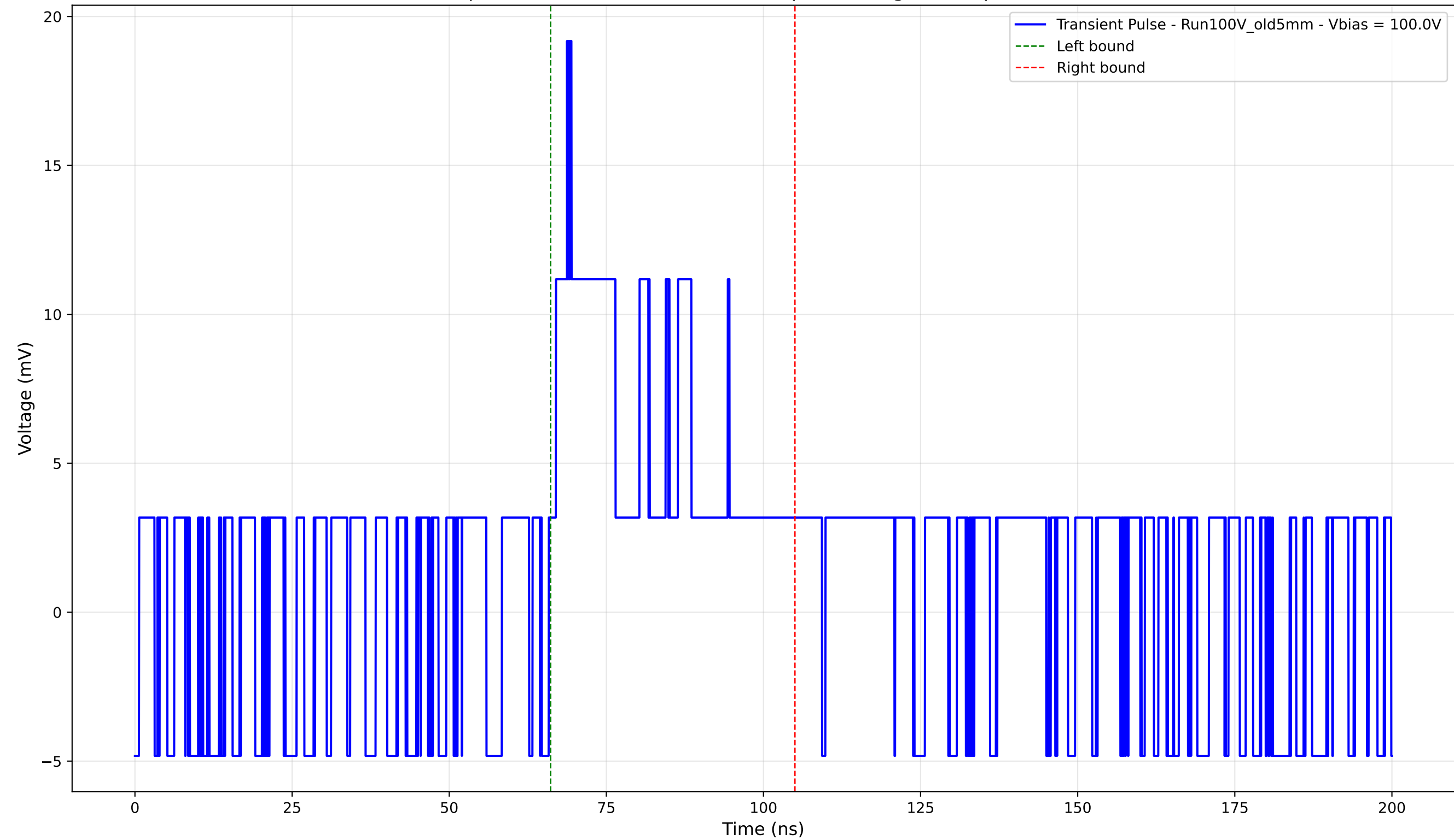
Transient Pulse - Sample: Old5mm - Position: 2740.0 \mu\text{m} - Charge: 4.78 pC - Rise Time: 0.00 ns (N/A)
