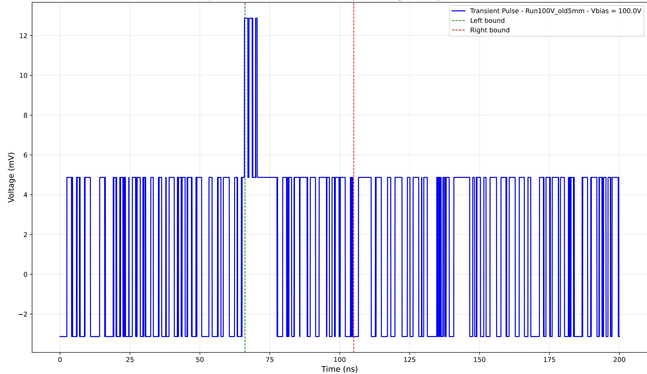
Transient Pulse - Sample: Old5mm - Position: 3700.0 \mu\text{m} - Charge: 2.66 pC - Rise Time: 0.00 ns (N/A)
