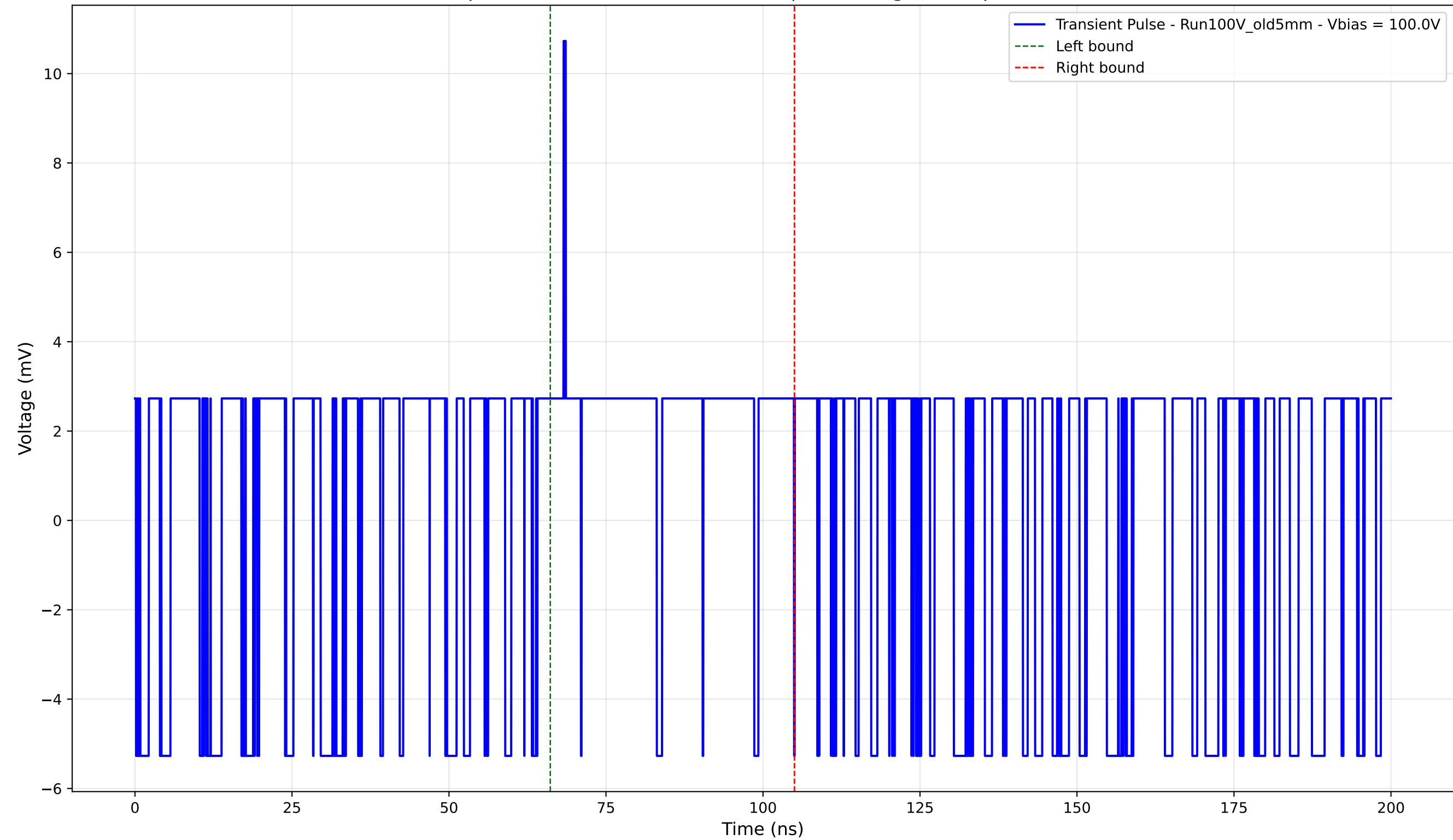
Transient Pulse - Sample: Old5mm - Position: 2515.0 \mu\text{m} - Charge: 1.88 pC - Rise Time: 0.00 ns (N/A)
