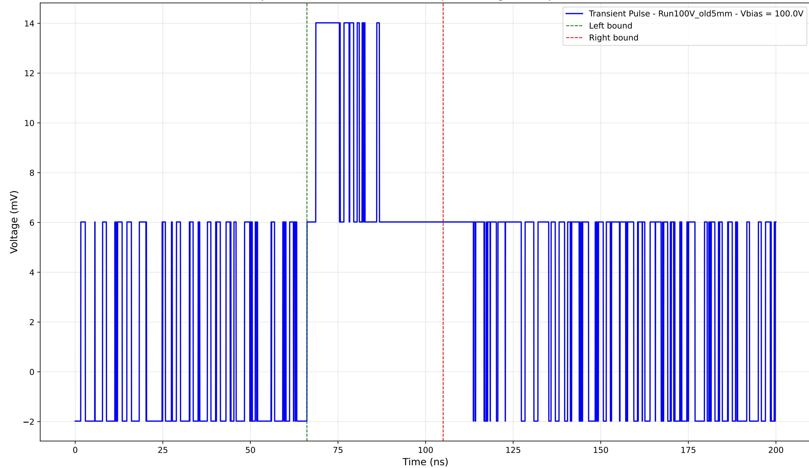
Transient Pulse - Sample: Old5mm - Position: 2355.0 \mu\text{m} - Charge: 6.50 pC - Rise Time: 0.00 ns (N/A)
