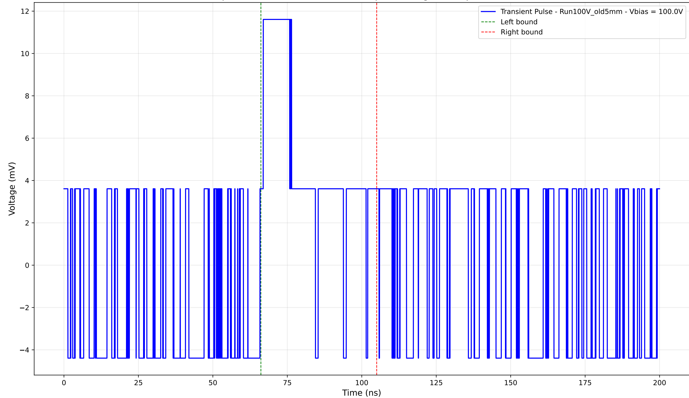
Transient Pulse - Sample: Old5mm - Position: 4670.0 \mu\text{m} - Charge: 3.91 pC - Rise Time: 0.00 ns (N/A)
