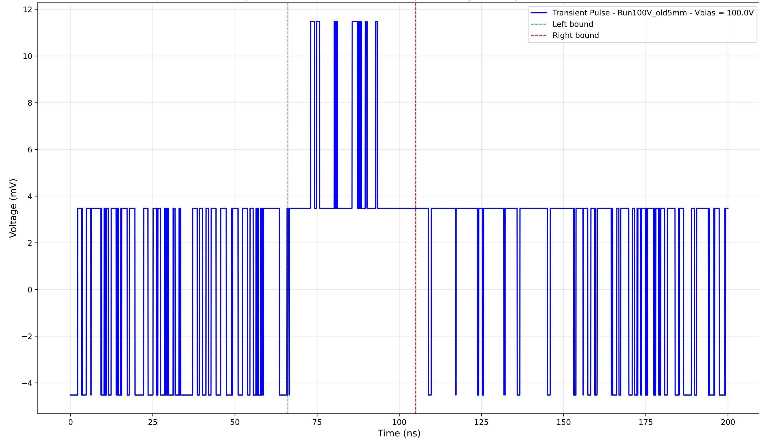
Transient Pulse - Sample: Old5mm - Position: 1675.0 \mu\text{m} - Charge: 3.60 pC - Rise Time: 0.00 ns (N/A)
