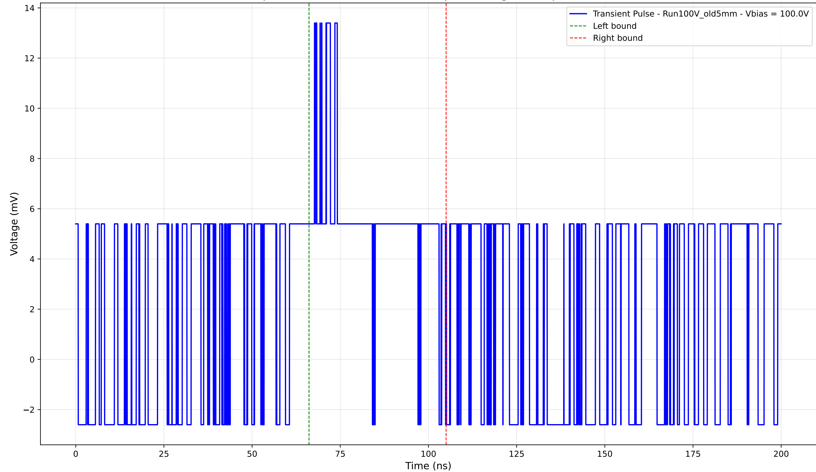
Transient Pulse - Sample: Old5mm - Position: 2835.0 \mu\text{m} - Charge: 4.35 pC - Rise Time: 0.00 ns (N/A)
