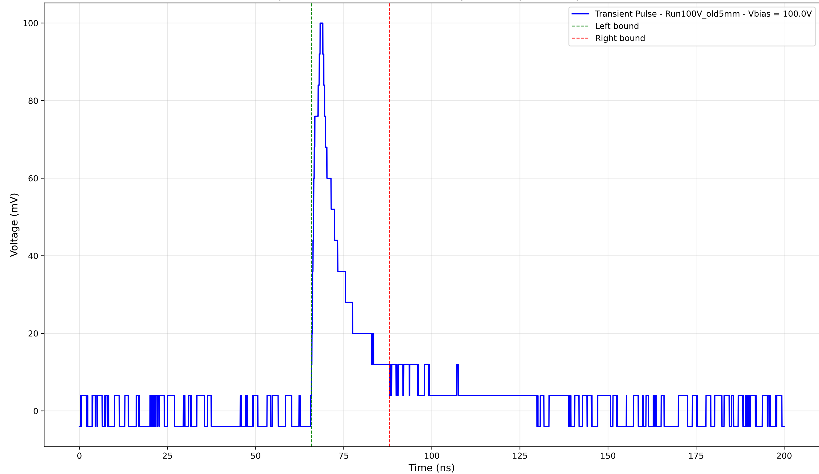
Transient Pulse - Sample: Old5mm - Position: 3220.0 \mu\text{m} - Charge: 15.96 pC - Rise Time: 2.20 ns
