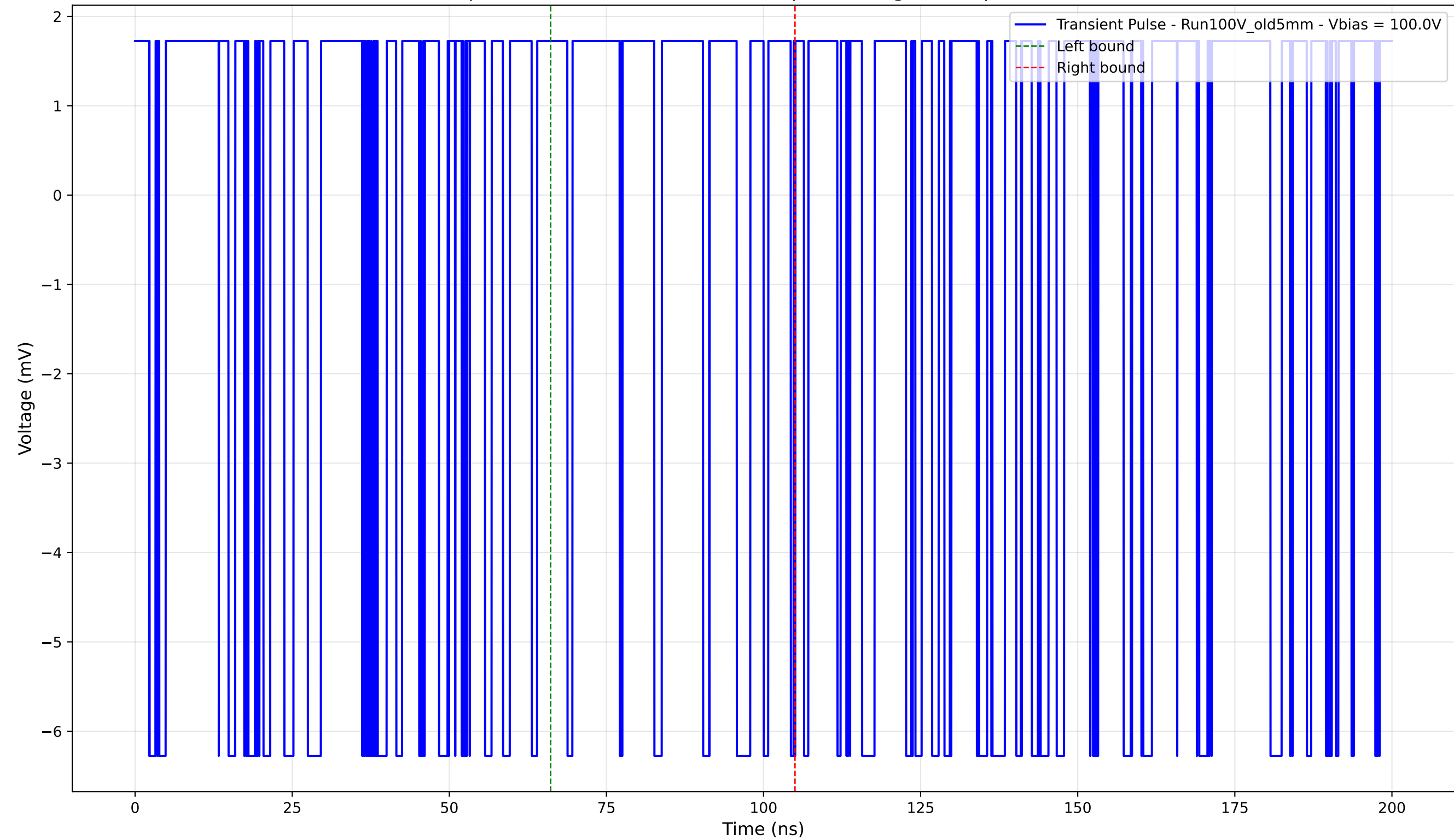
Transient Pulse - Sample: Old5mm - Position: 4300.0 \mu\text{m} - Charge: 0.24 pC - Rise Time: 0.00 ns (N/A)
