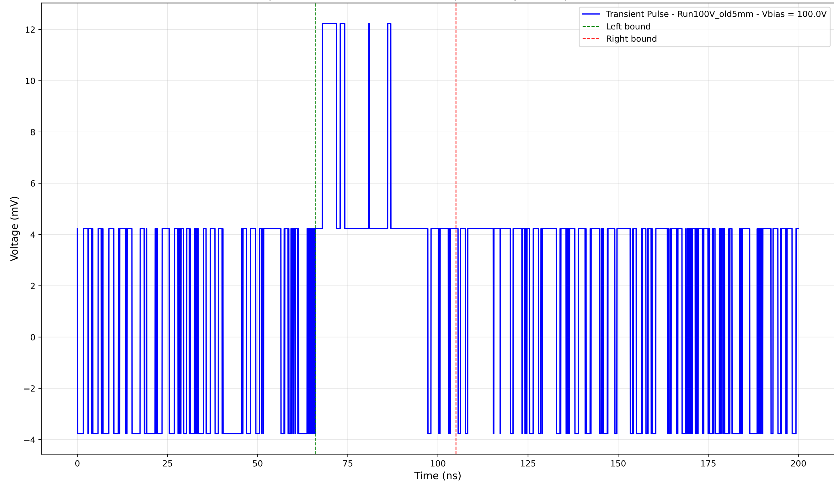
Transient Pulse - Sample: Old5mm - Position: 2755.0 \mu\text{m} - Charge: 4.05 pC - Rise Time: 0.00 ns (N/A)
