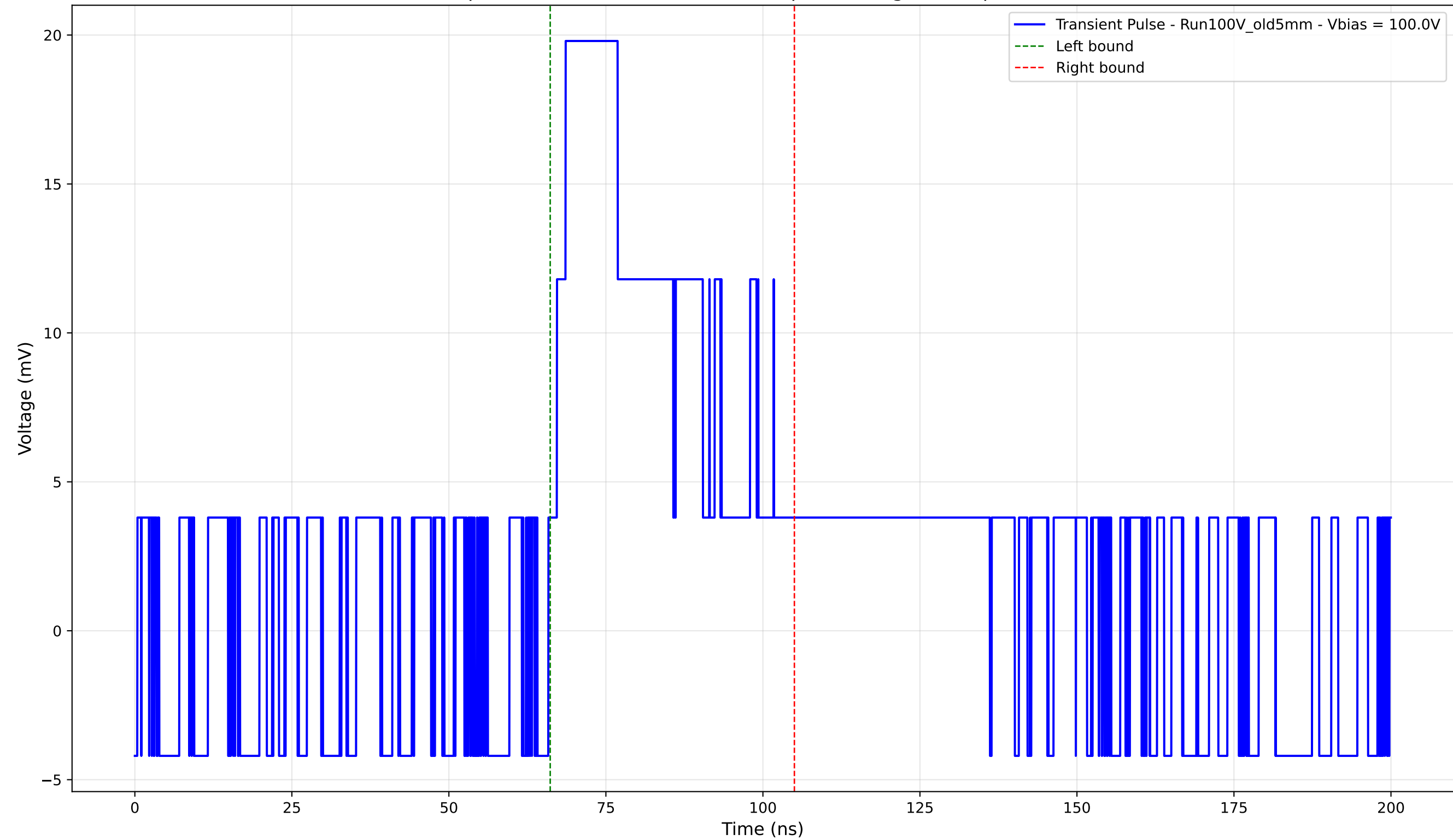
Transient Pulse - Sample: Old5mm - Position: 2575.0 \mu\text{m} - Charge: 8.32 pC - Rise Time: 0.00 ns (N/A)
