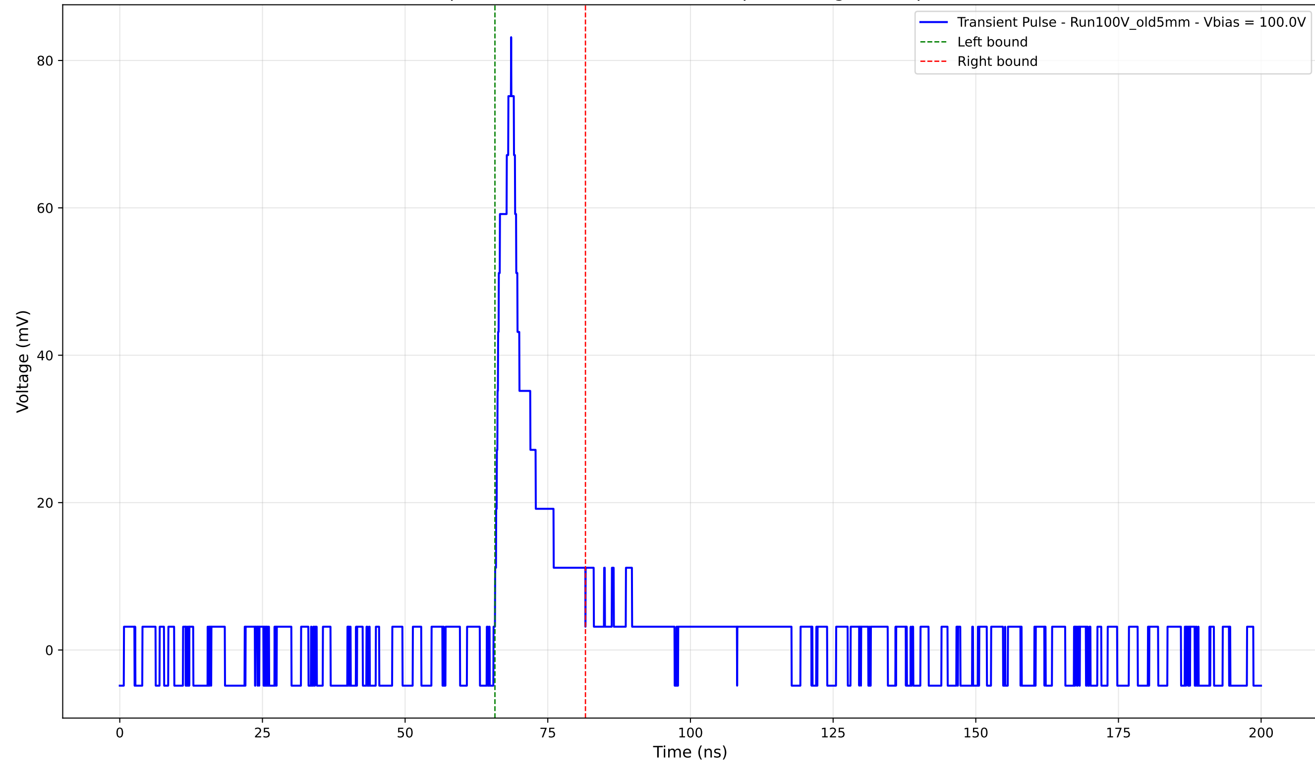
Transient Pulse - Sample: Old5mm - Position: 3330.0 \mu\text{m} - Charge: 9.14 pC - Rise Time: 2.33 ns
