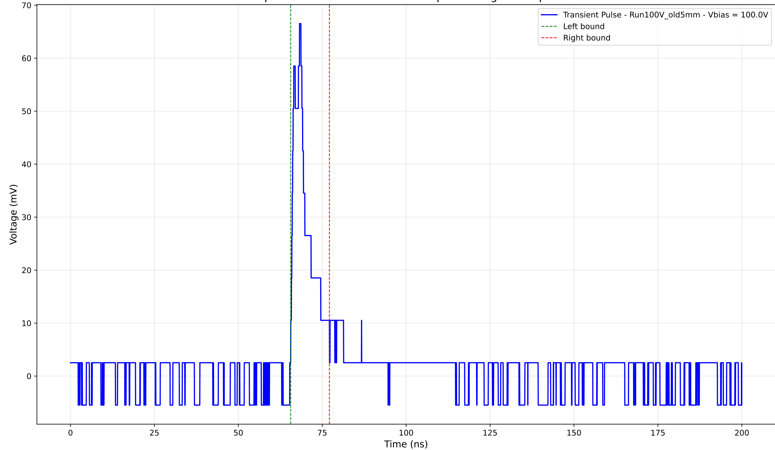
Transient Pulse - Sample: Old5mm - Position: 3950.0 \mu\text{m} - Charge: 6.62 pC - Rise Time: 2.61 ns
