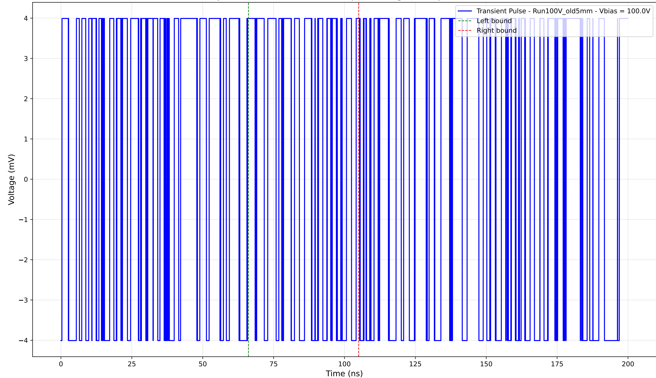
Transient Pulse - Sample: Old5mm - Position: 90.0 \mu\text{m} - Charge: 0.74 pC - Rise Time: 0.00 ns (N/A)
