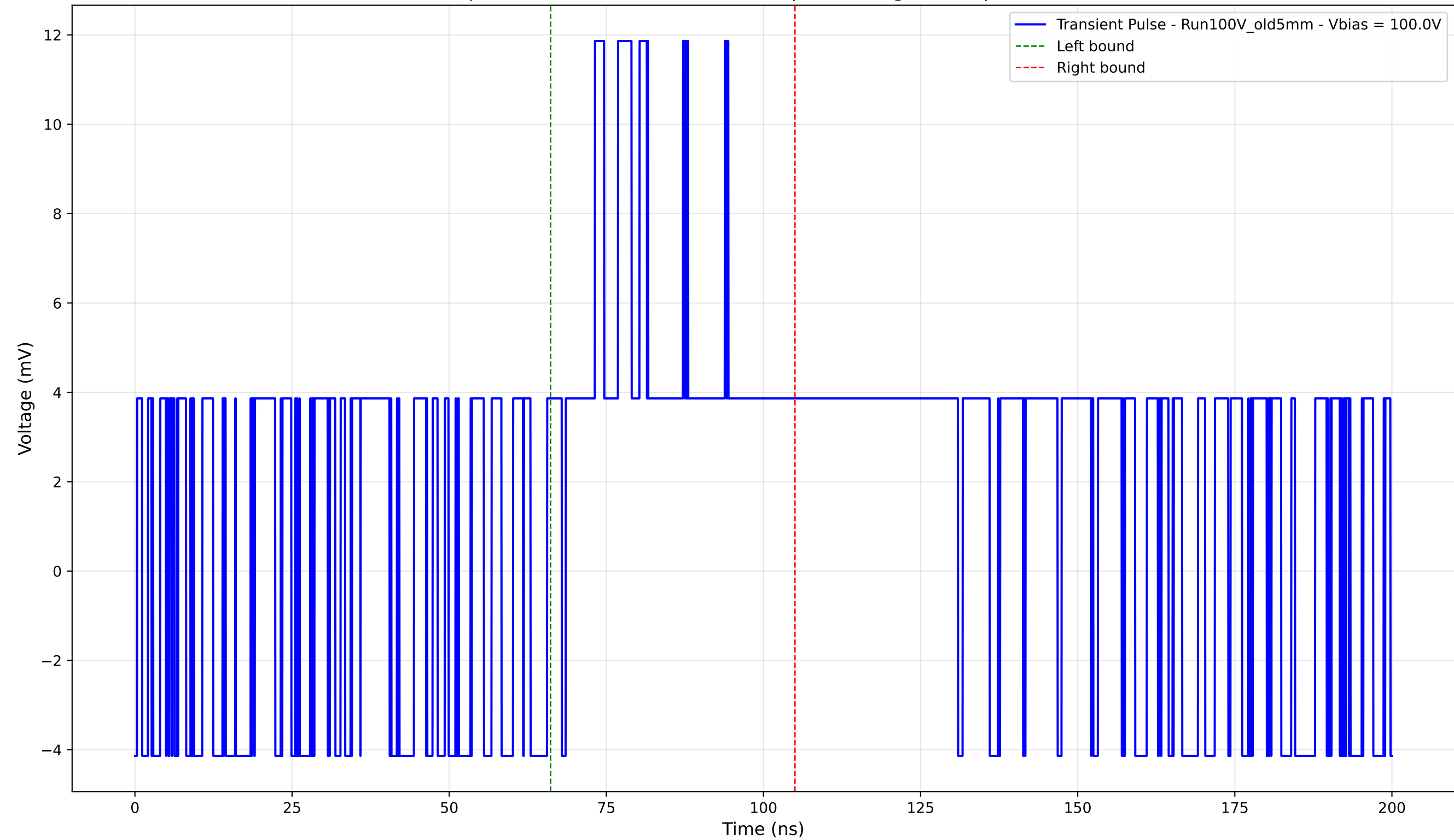
Transient Pulse - Sample: Old5mm - Position: 1265.0 \mu\text{m} - Charge: 3.86 pC - Rise Time: 0.00 ns (N/A)
