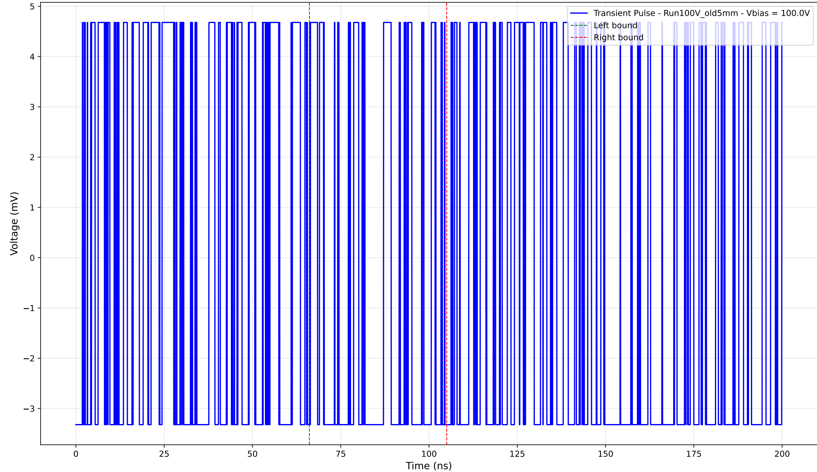
Transient Pulse - Sample: Old5mm - Position: 120.0 \mu\text{m} - Charge: -0.62 pC - Rise Time: 0.00 ns (N/A)
