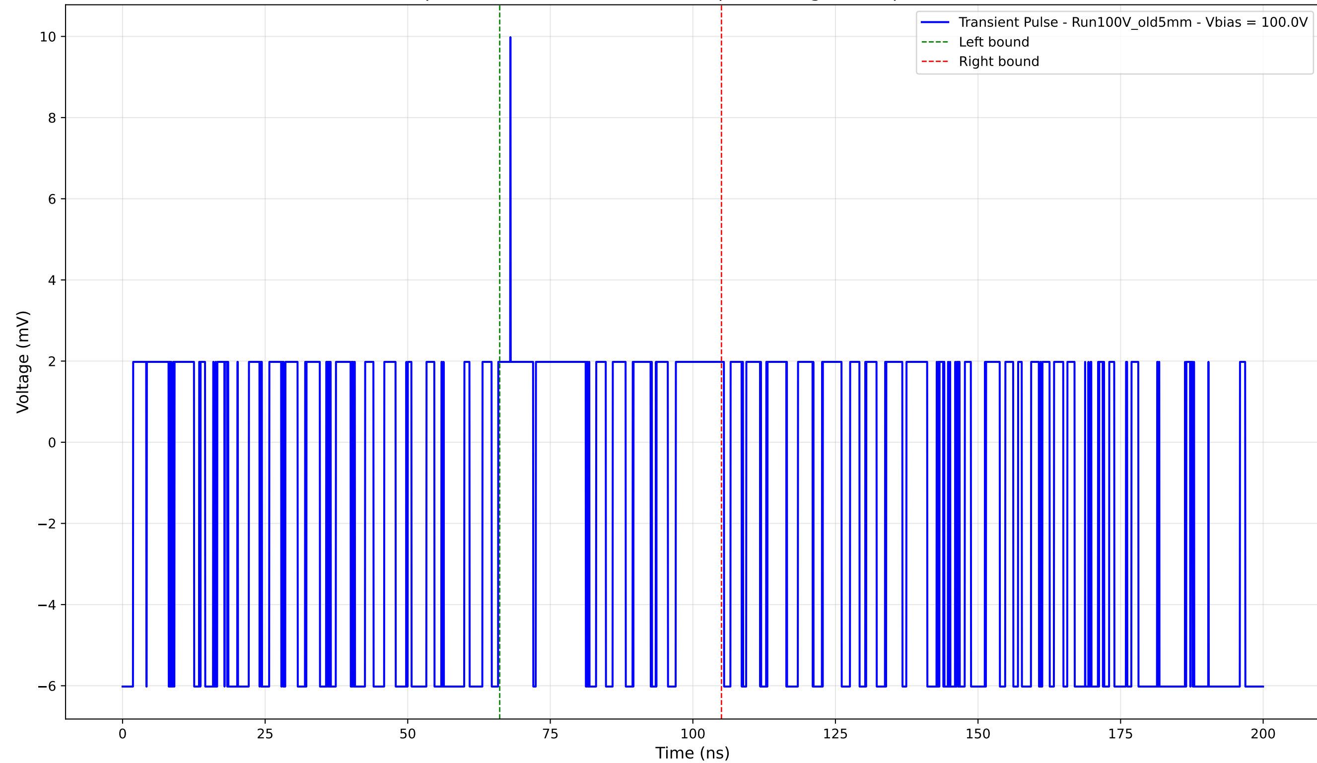
Transient Pulse - Sample: Old5mm - Position: 3075.0 \mu\text{m} - Charge: 0.48 pC - Rise Time: 0.00 ns (N/A)
