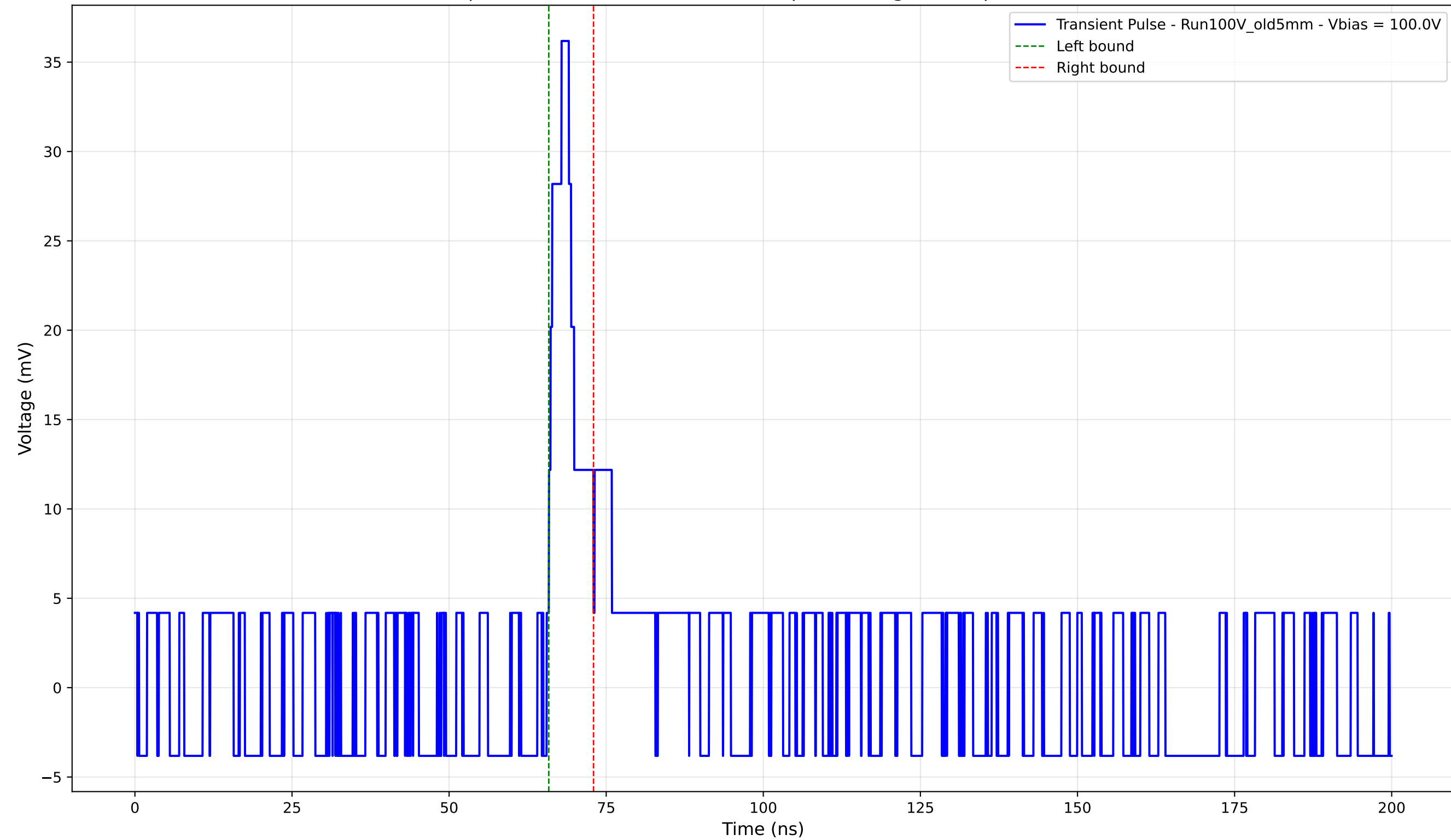
Transient Pulse - Sample: Old5mm - Position: 3355.0 \mu\text{m} - Charge: 3.01 pC - Rise Time: 0.00 ns (N/A)
