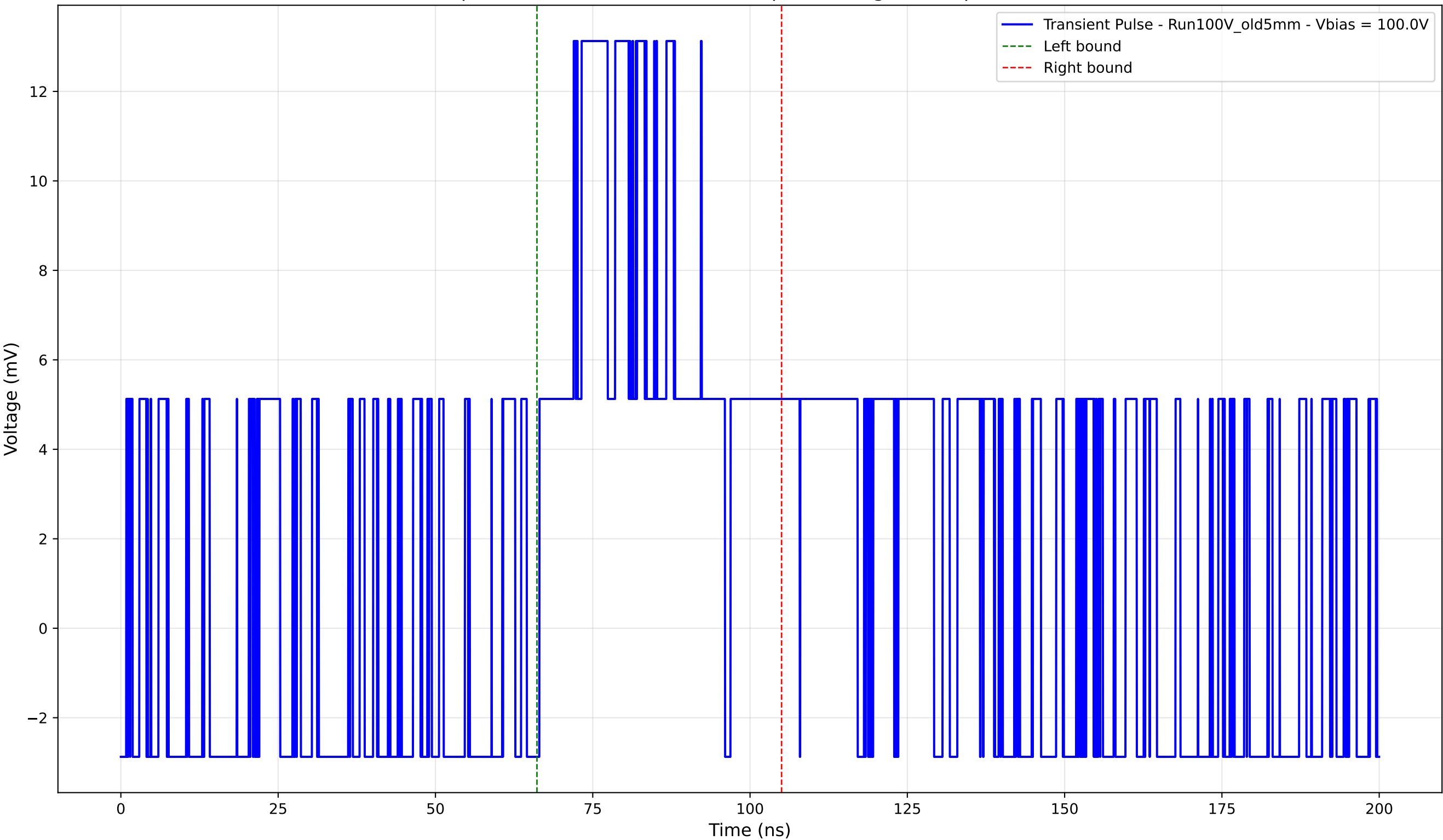
Transient Pulse - Sample: Old5mm - Position: 570.0 \mu\text{m} - Charge: 5.43 pC - Rise Time: 0.00 ns (N/A)
