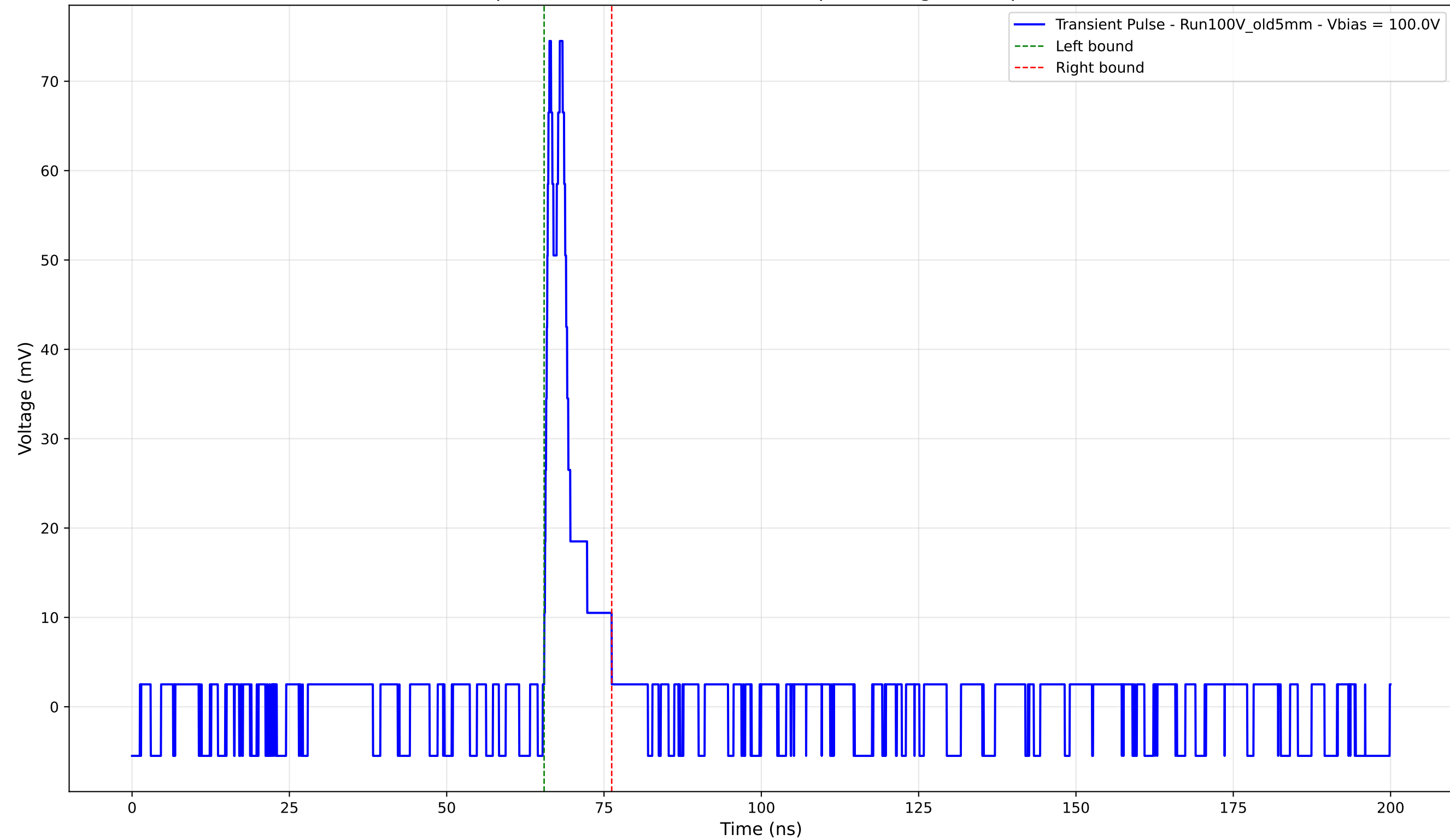
Transient Pulse - Sample: Old5mm - Position: 3650.0 \mu\text{m} - Charge: 6.24 pC - Rise Time: 0.83 ns
