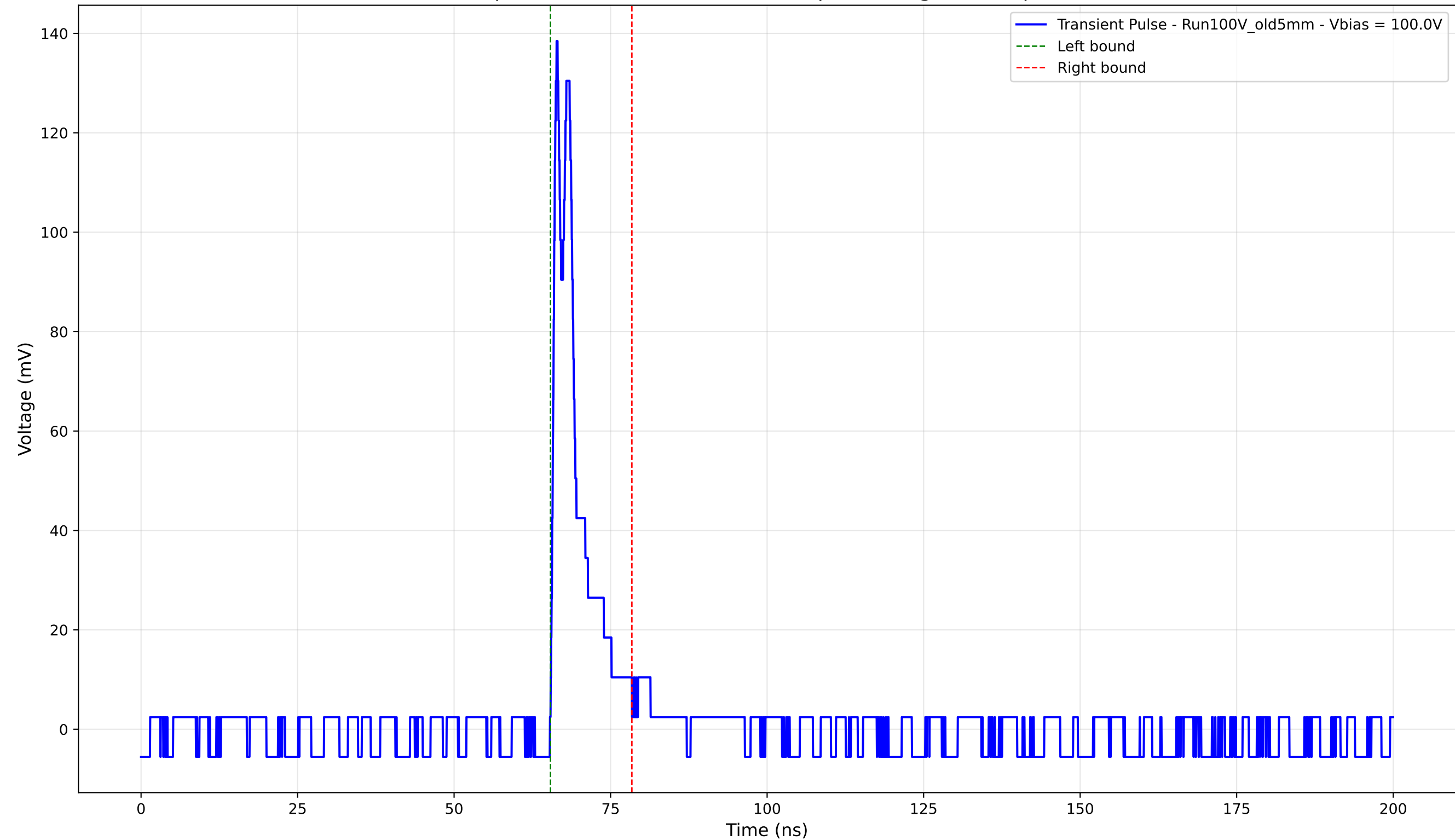
Transient Pulse - Sample: Old5mm - Position: 3630.0 \mu\text{m} - Charge: 12.02 pC - Rise Time: 0.75 ns
