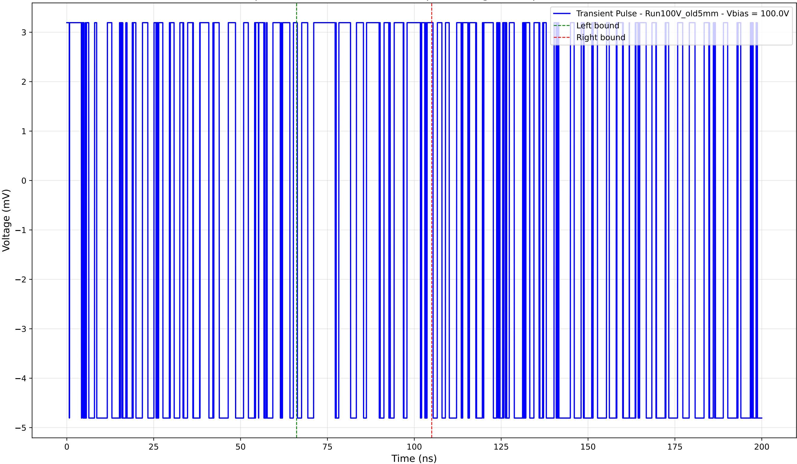
Transient Pulse - Sample: Old5mm - Position: 240.0 \mu\text{m} - Charge: 0.79 pC - Rise Time: 0.00 ns (N/A)
