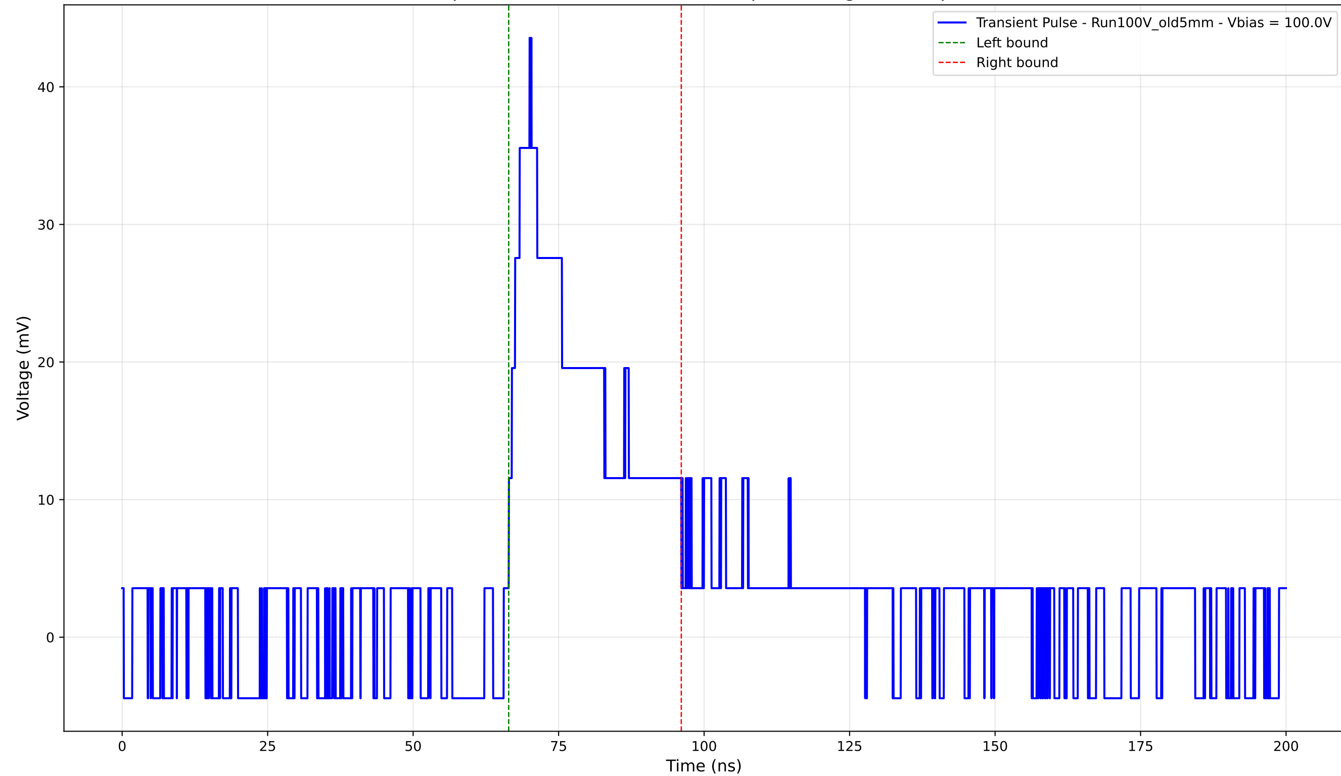
Transient Pulse - Sample: Old5mm - Position: 4710.0 \mu\text{m} - Charge: 11.33 pC - Rise Time: 3.58 ns
