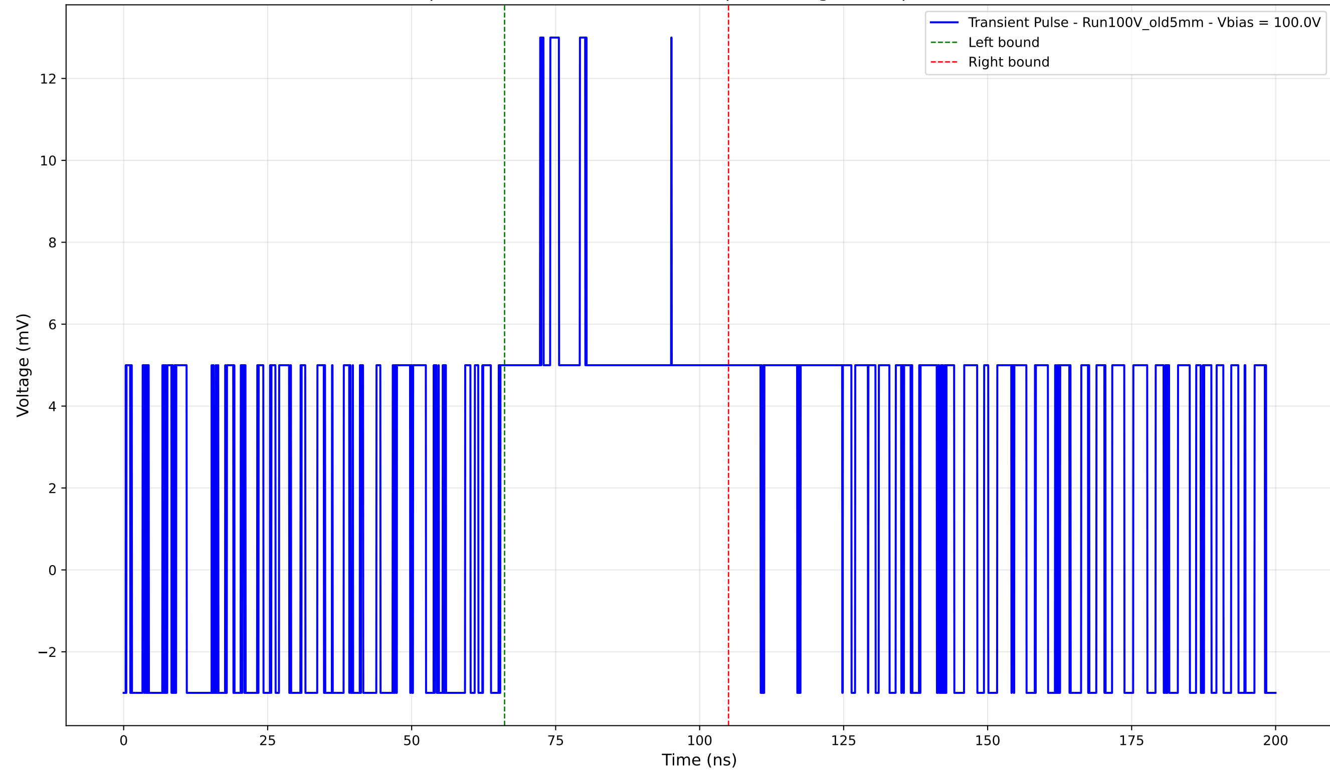
Transient Pulse - Sample: Old5mm - Position: 2085.0 \mu\text{m} - Charge: 4.38 pC - Rise Time: 0.00 ns (N/A)
