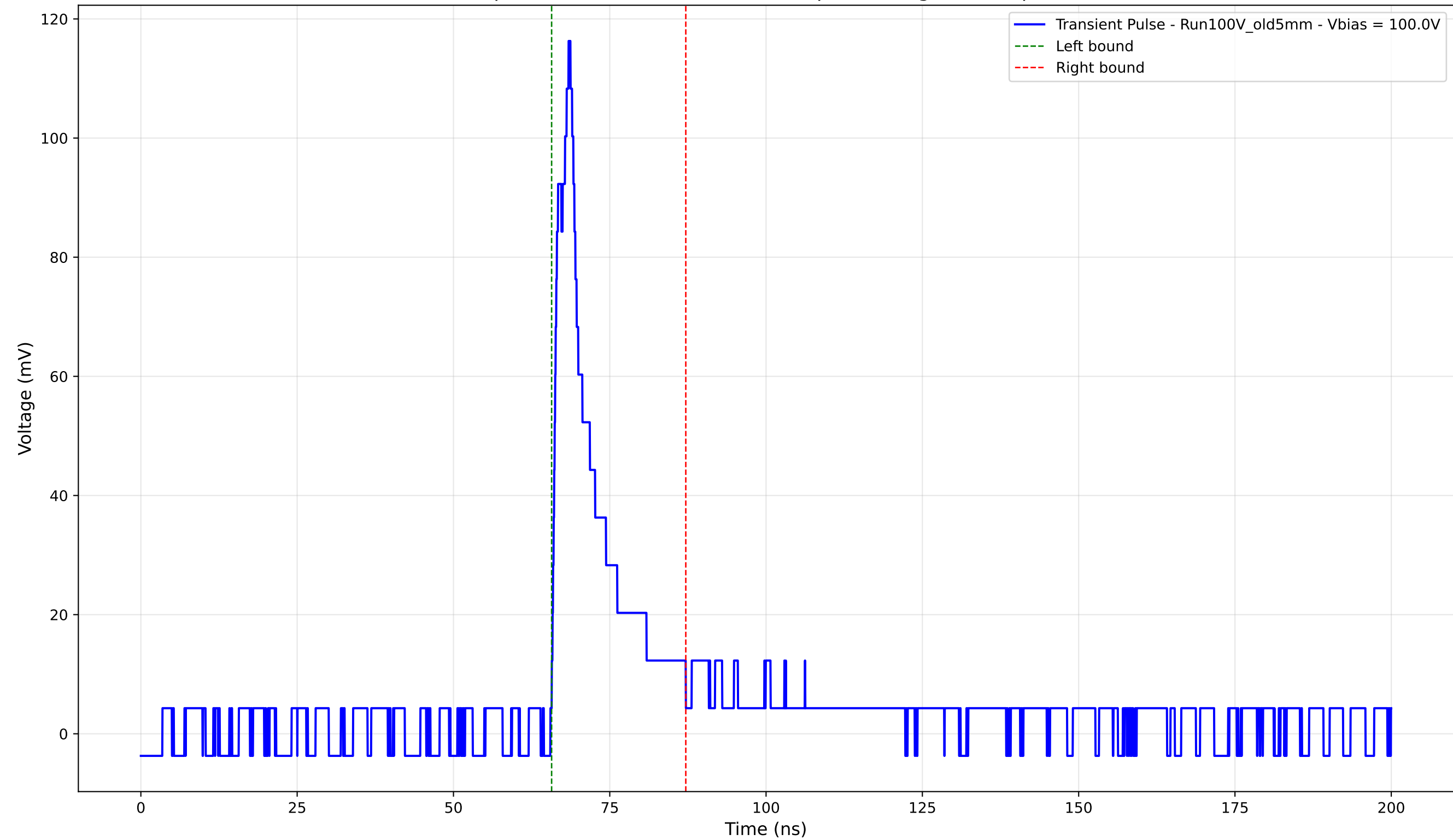
Transient Pulse - Sample: Old5mm - Position: 4115.0 \mu\text{m} - Charge: 15.68 pC - Rise Time: 2.38 ns
