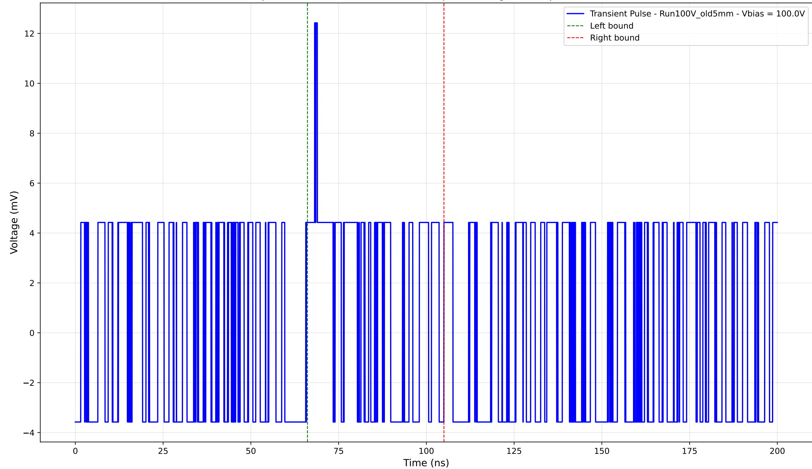
Transient Pulse - Sample: Old5mm - Position: 3410.0 \mu\text{m} - Charge: 1.32 pC - Rise Time: 0.00 ns (N/A)
