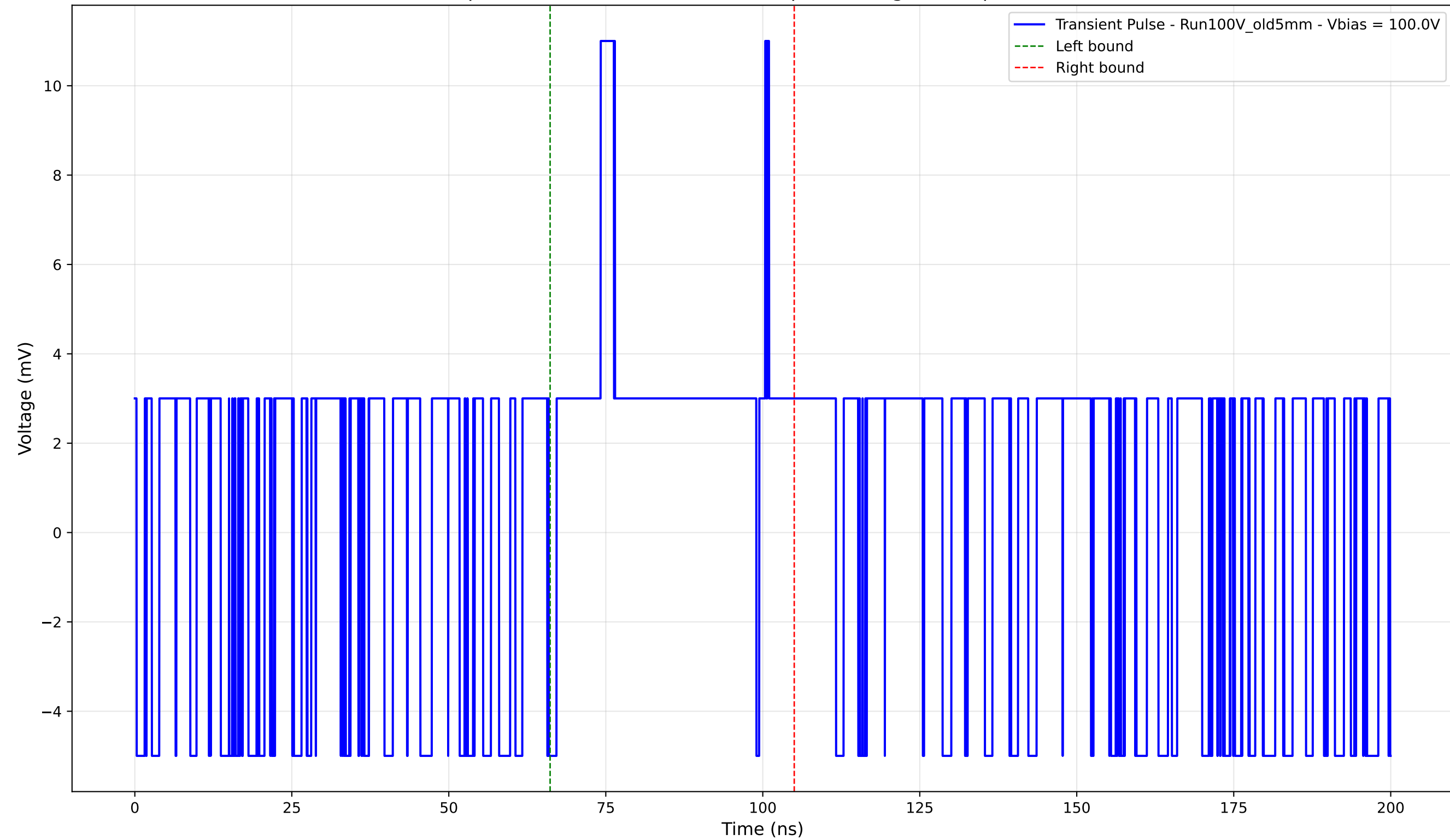
Transient Pulse - Sample: Old5mm - Position: 1940.0 \mu\text{m} - Charge: 2.52 pC - Rise Time: 0.00 ns (N/A)
