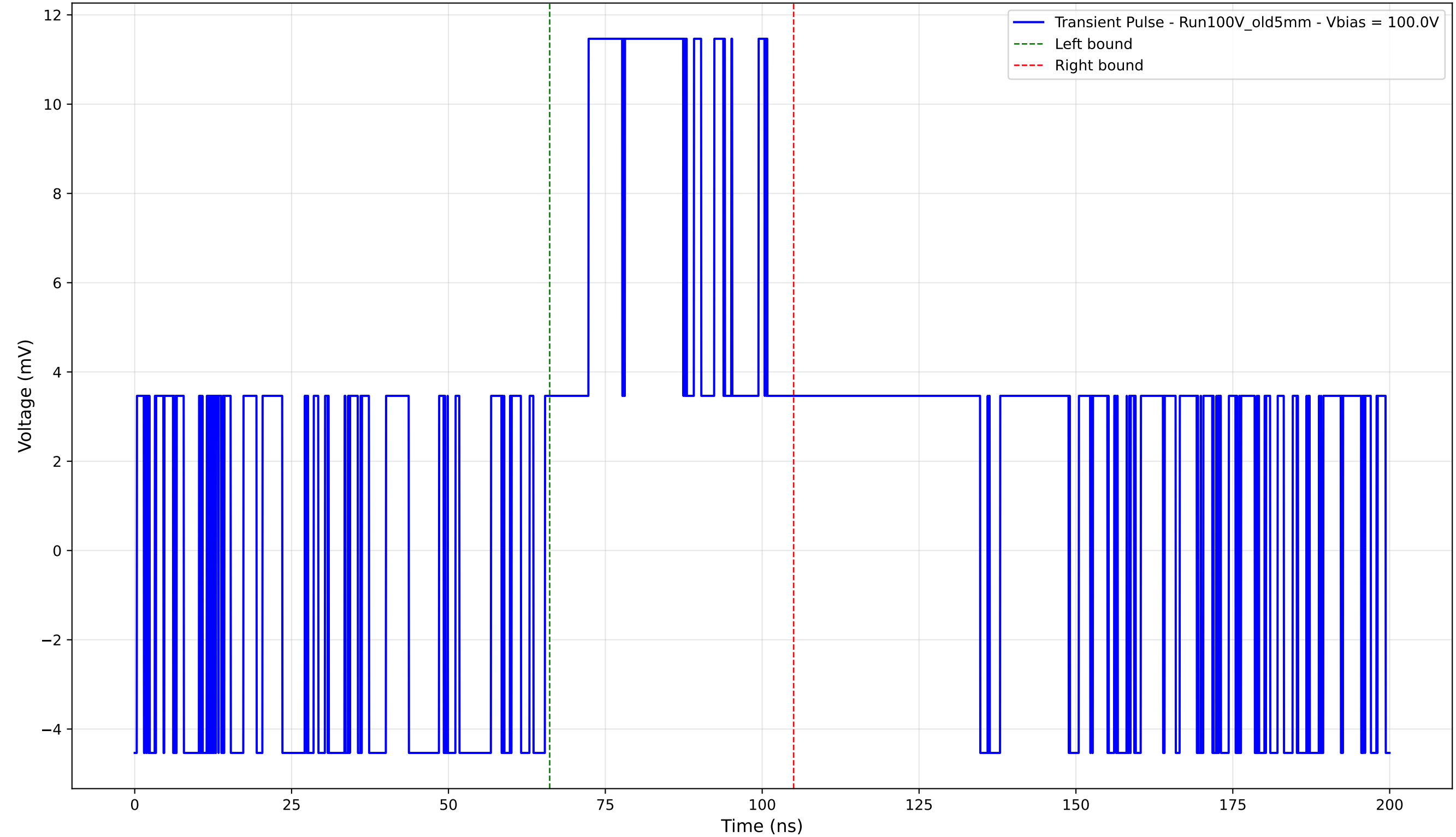
Transient Pulse - Sample: Old5mm - Position: 1660.0 \mu\text{m} - Charge: 5.79 pC - Rise Time: 0.00 ns (N/A)
