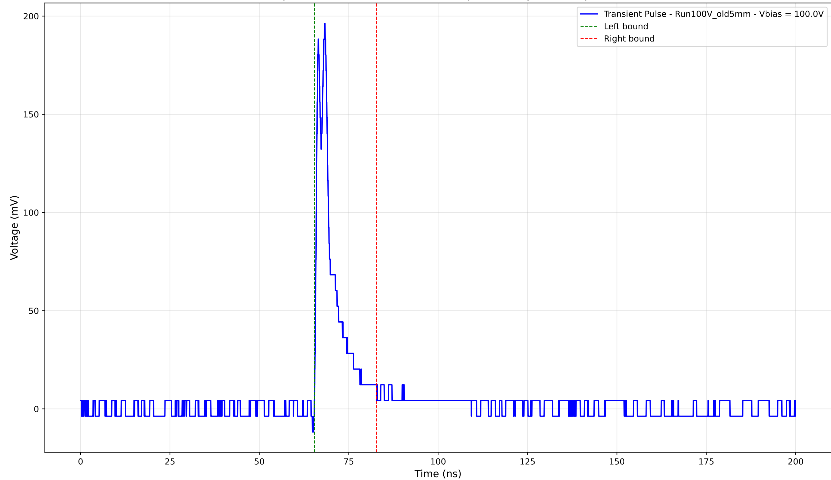
Transient Pulse - Sample: Old5mm - Position: 3855.0 \mu\text{m} - Charge: 19.89 pC - Rise Time: 0.84 ns
