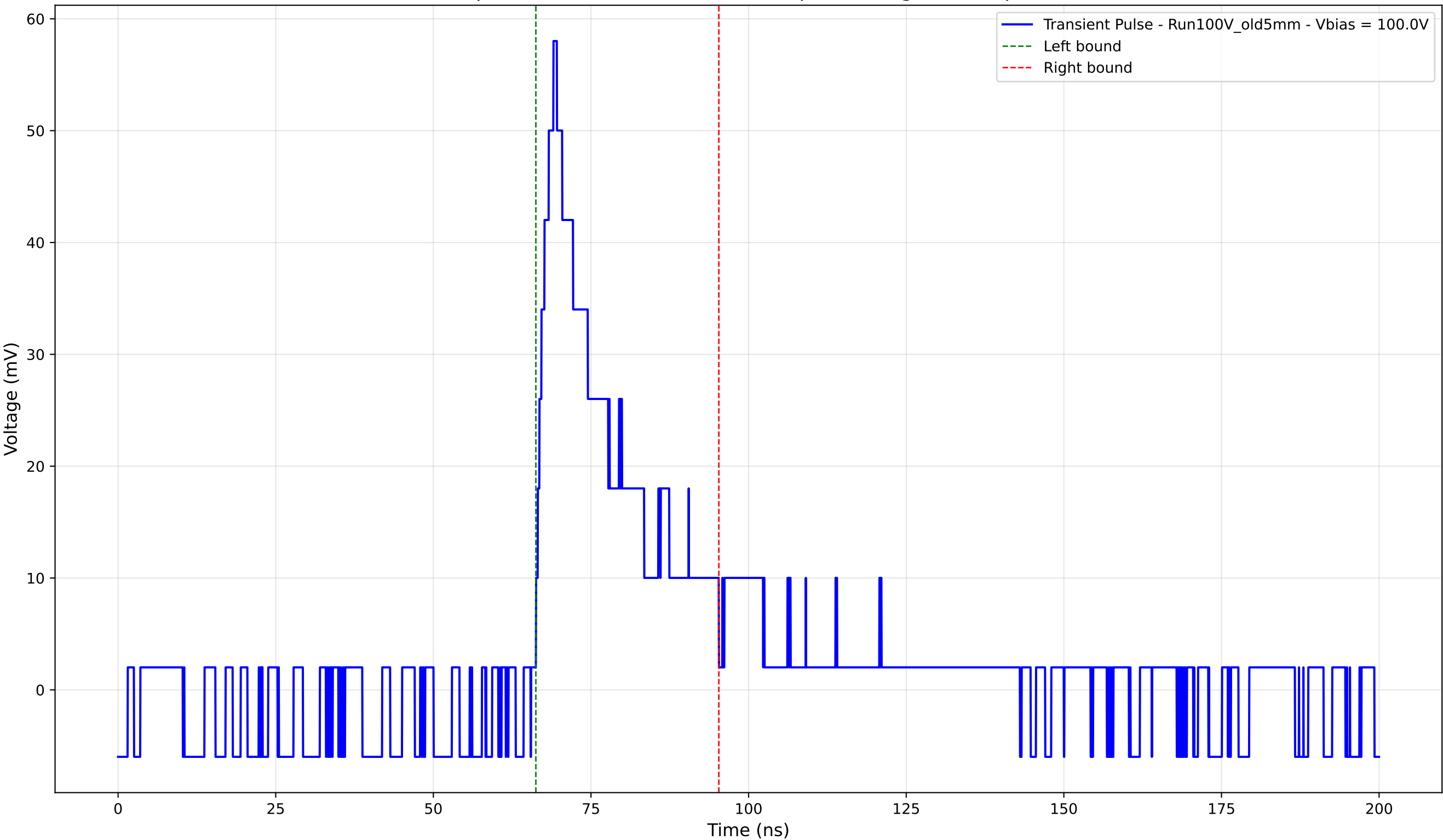
Transient Pulse - Sample: Old5mm - Position: 2905.0 \mu\text{m} - Charge: 12.93 pC - Rise Time: 2.77 ns
