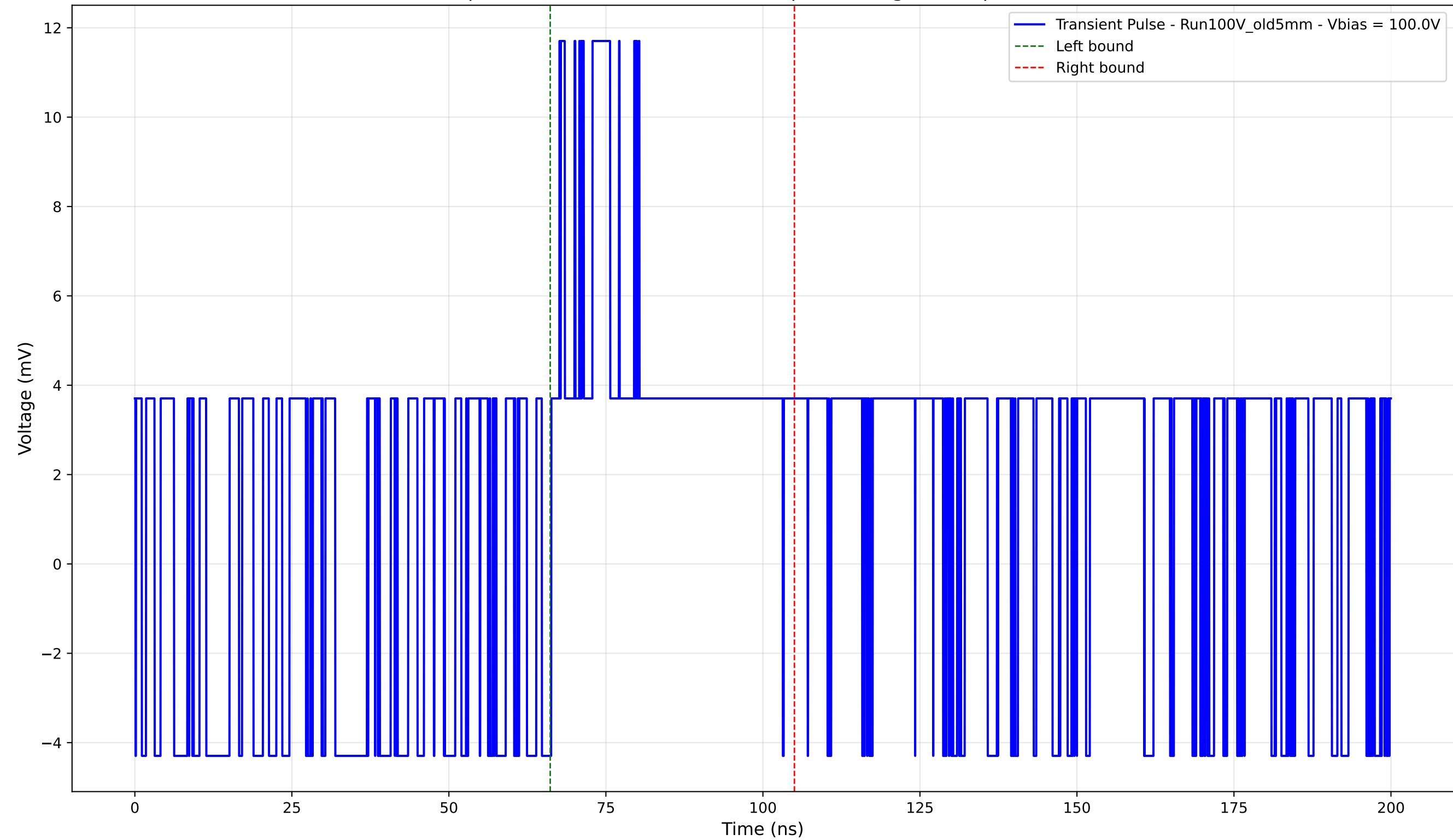
Transient Pulse - Sample: Old5mm - Position: 2545.0 \mu\text{m} - Charge: 3.59 pC - Rise Time: 0.00 ns (N/A)
