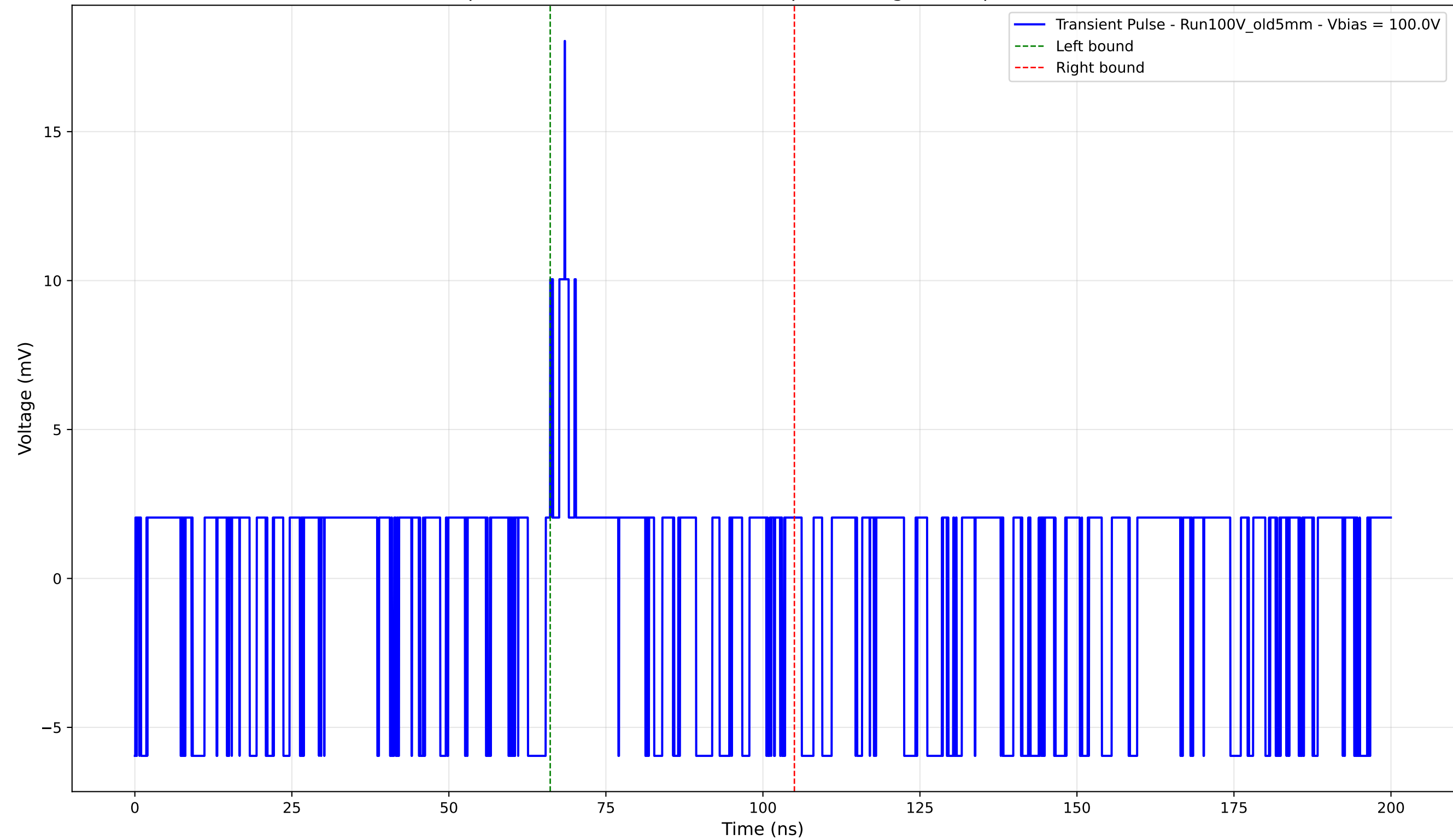
Transient Pulse - Sample: Old5mm - Position: 3720.0 \mu\text{m} - Charge: 0.50 pC - Rise Time: 0.00 ns (N/A)
