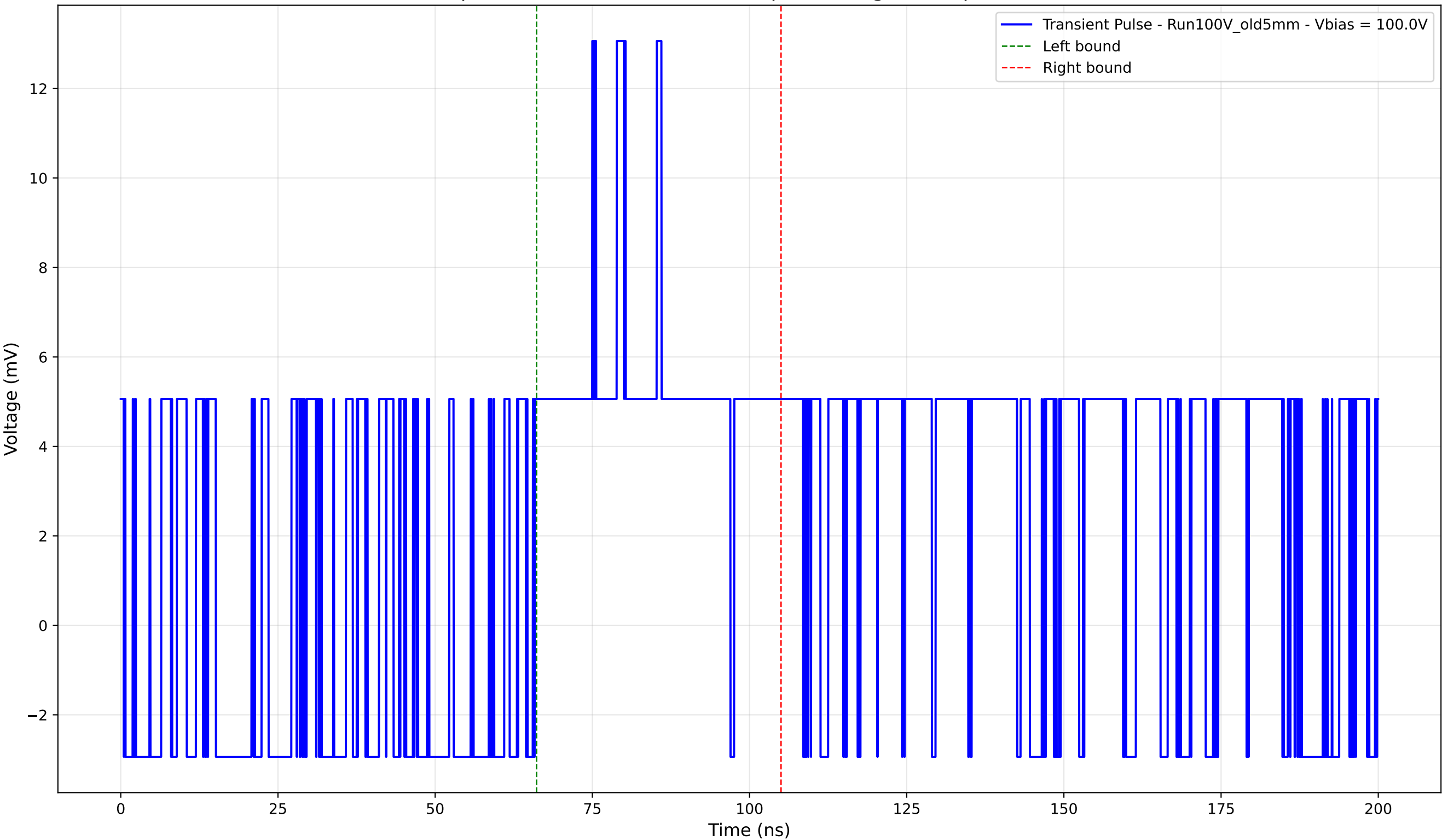
Transient Pulse - Sample: Old5mm - Position: 435.0 \mu\text{m} - Charge: 4.26 pC - Rise Time: 0.00 ns (N/A)
