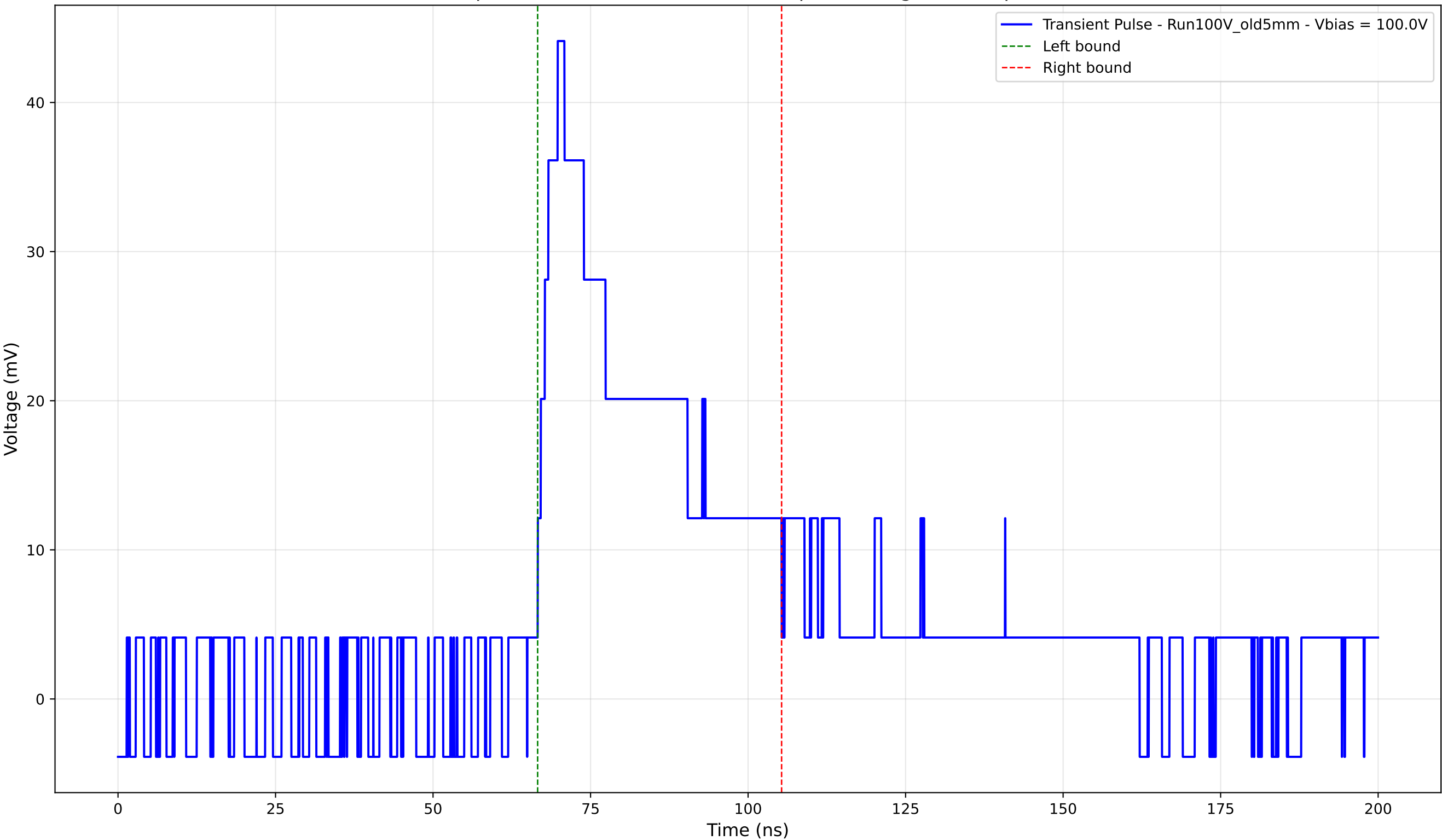
Transient Pulse - Sample: Old5mm - Position: 2635.0 \mu\text{m} - Charge: 15.80 pC - Rise Time: 3.18 ns
