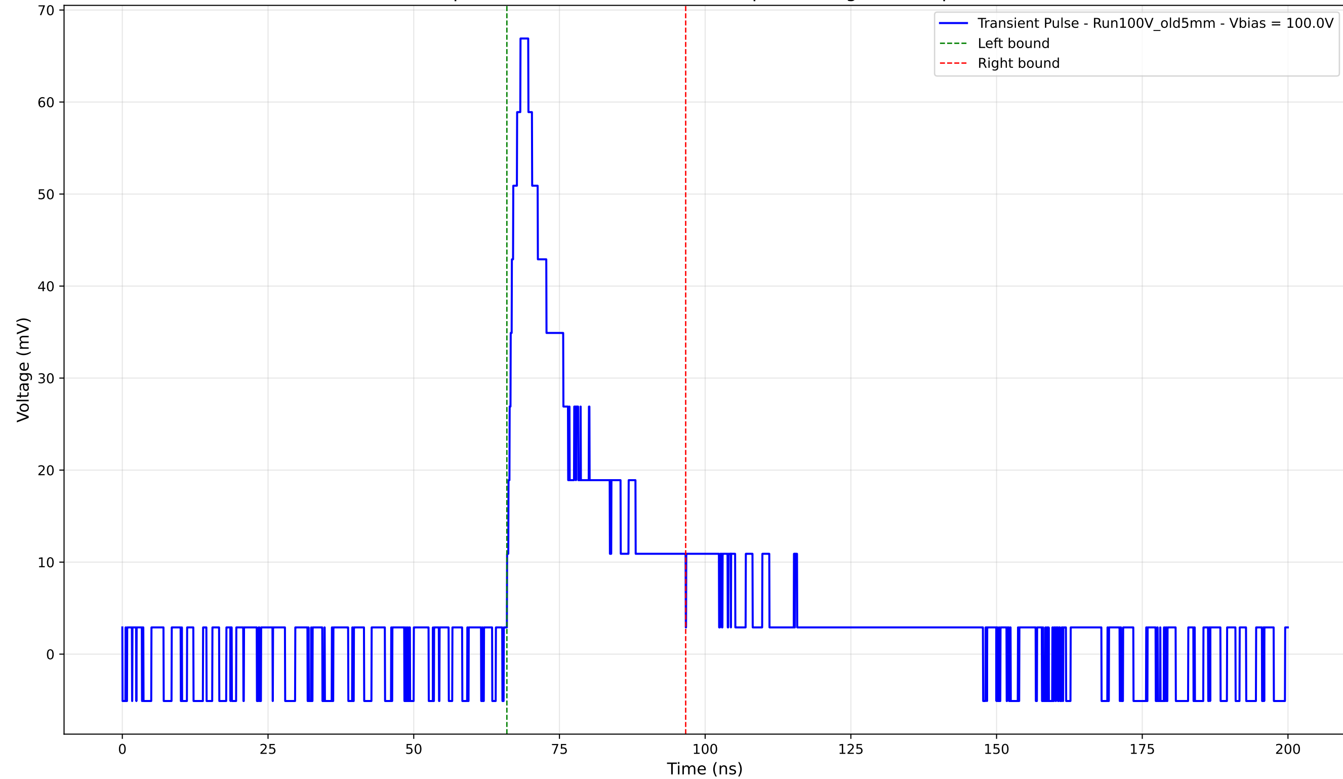
Transient Pulse - Sample: Old5mm - Position: 2980.0 \mu\text{m} - Charge: 15.37 pC - Rise Time: 2.31 ns
