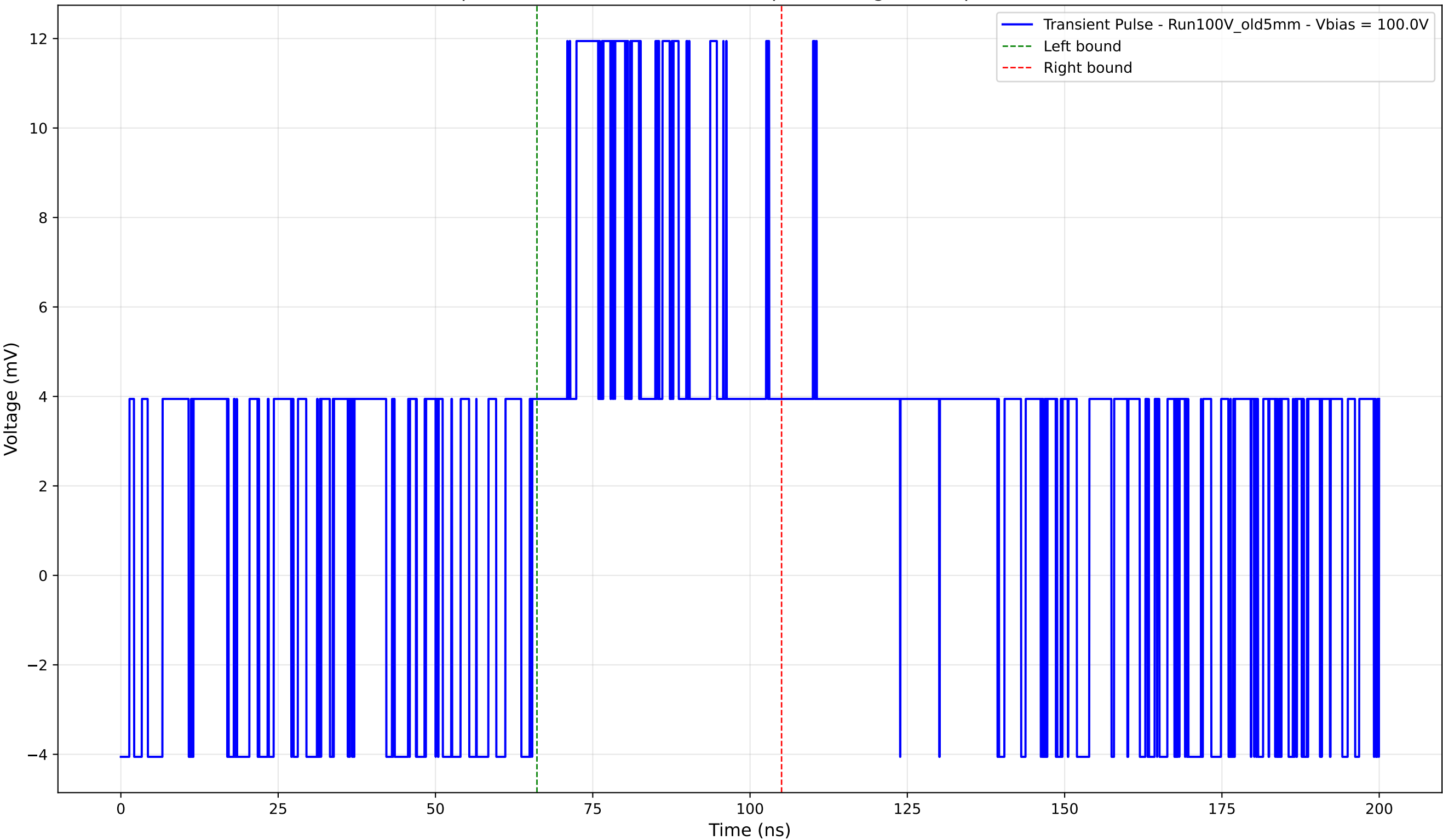
Transient Pulse - Sample: Old5mm - Position: 690.0 \mu\text{m} - Charge: 5.20 pC - Rise Time: 0.00 ns (N/A)
