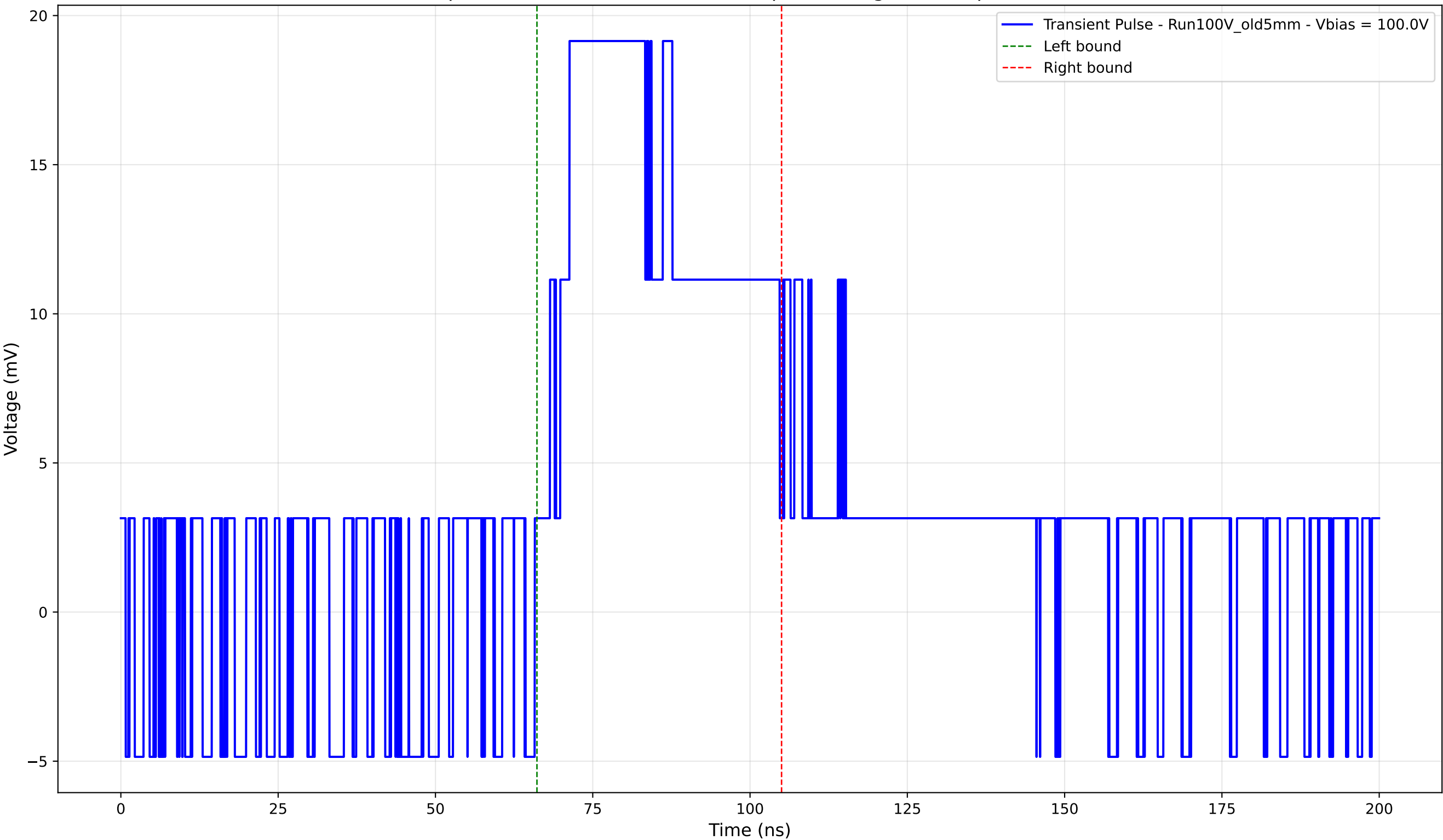
Transient Pulse - Sample: Old5mm - Position: 1995.0 \mu\text{m} - Charge: 10.38 pC - Rise Time: 0.00 ns (N/A)
