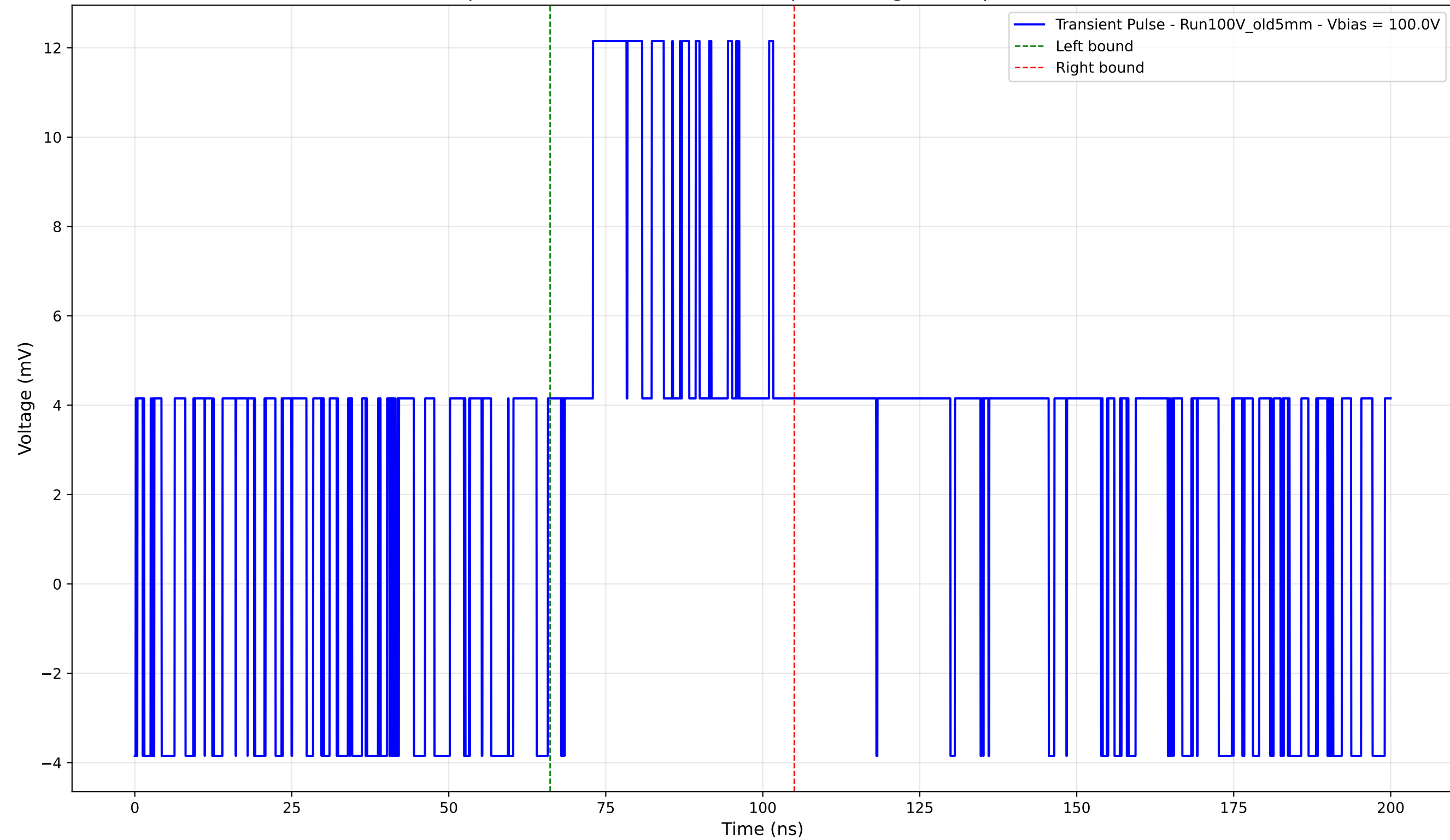
Transient Pulse - Sample: Old5mm - Position: 1255.0 \mu\text{m} - Charge: 5.34 pC - Rise Time: 0.00 ns (N/A)
