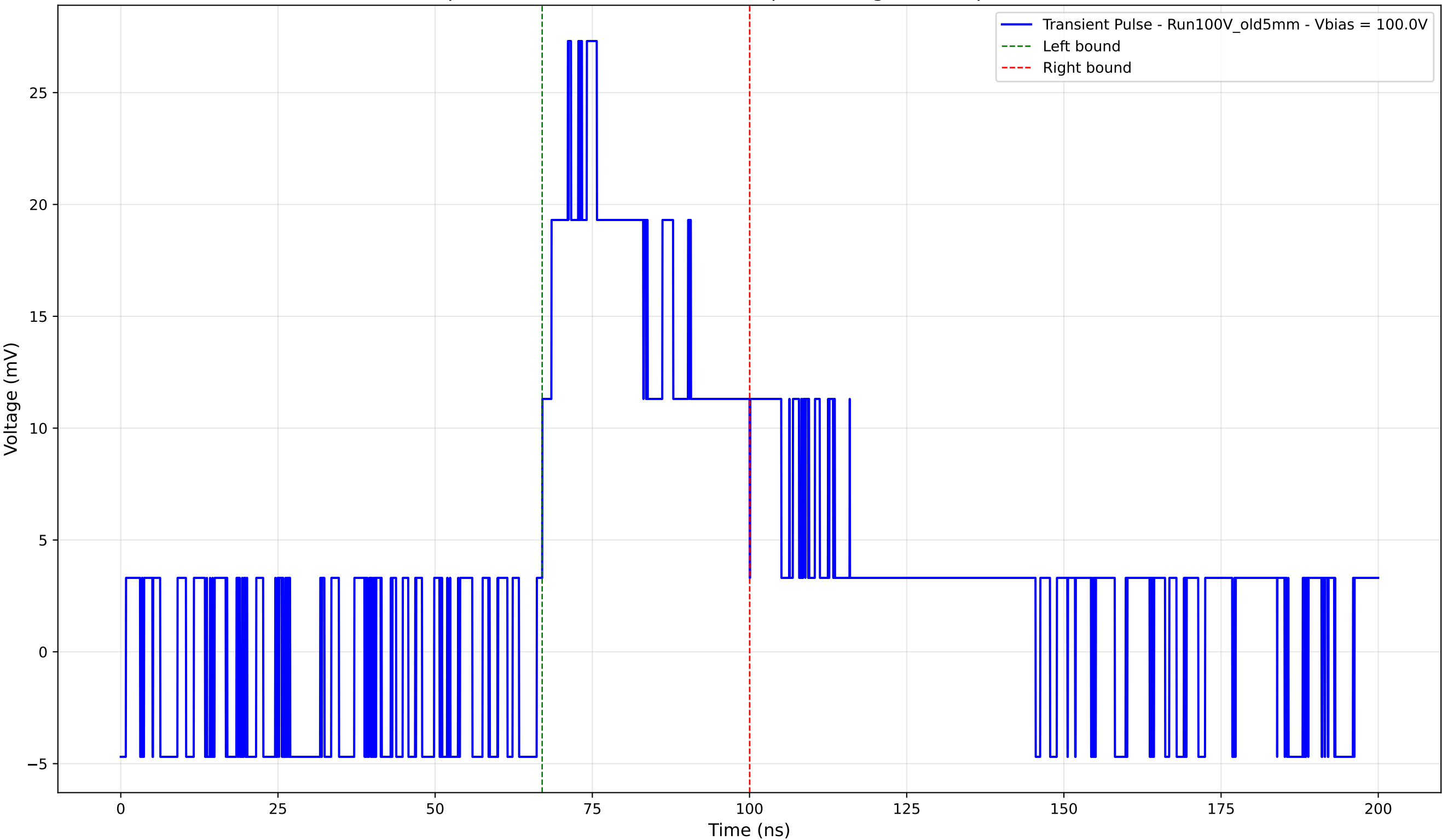
Transient Pulse - Sample: Old5mm - Position: 2390.0 \mu\text{m} - Charge: 10.62 pC - Rise Time: 0.00 ns (N/A)
