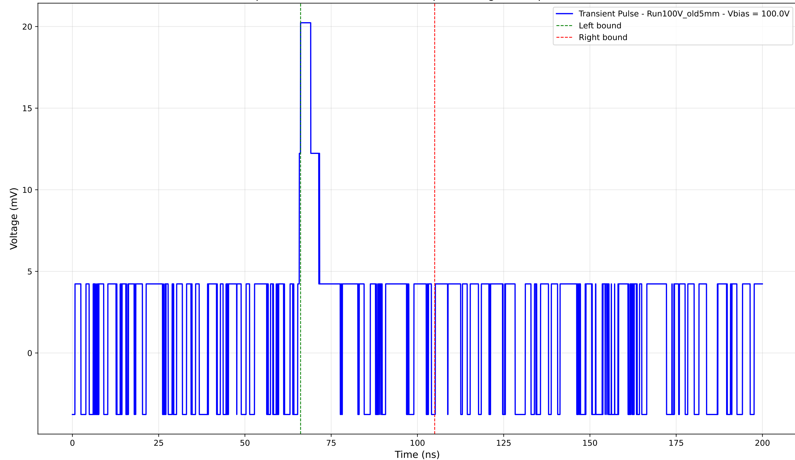
Transient Pulse - Sample: Old5mm - Position: 3740.0 \mu\text{m} - Charge: 3.38 pC - Rise Time: 0.00 ns (N/A)
