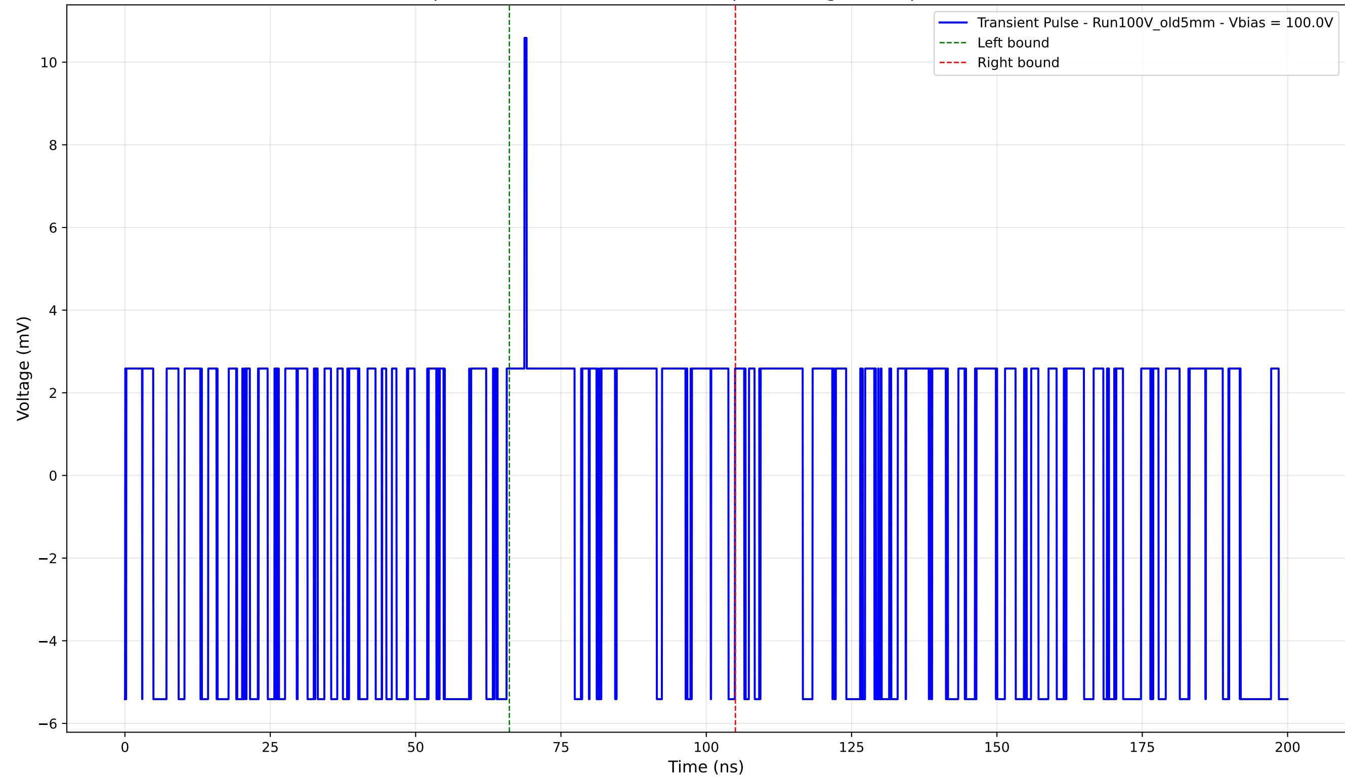
Transient Pulse - Sample: Old5mm - Position: 3400.0 \mu\text{m} - Charge: 1.31 pC - Rise Time: 0.00 ns (N/A)
