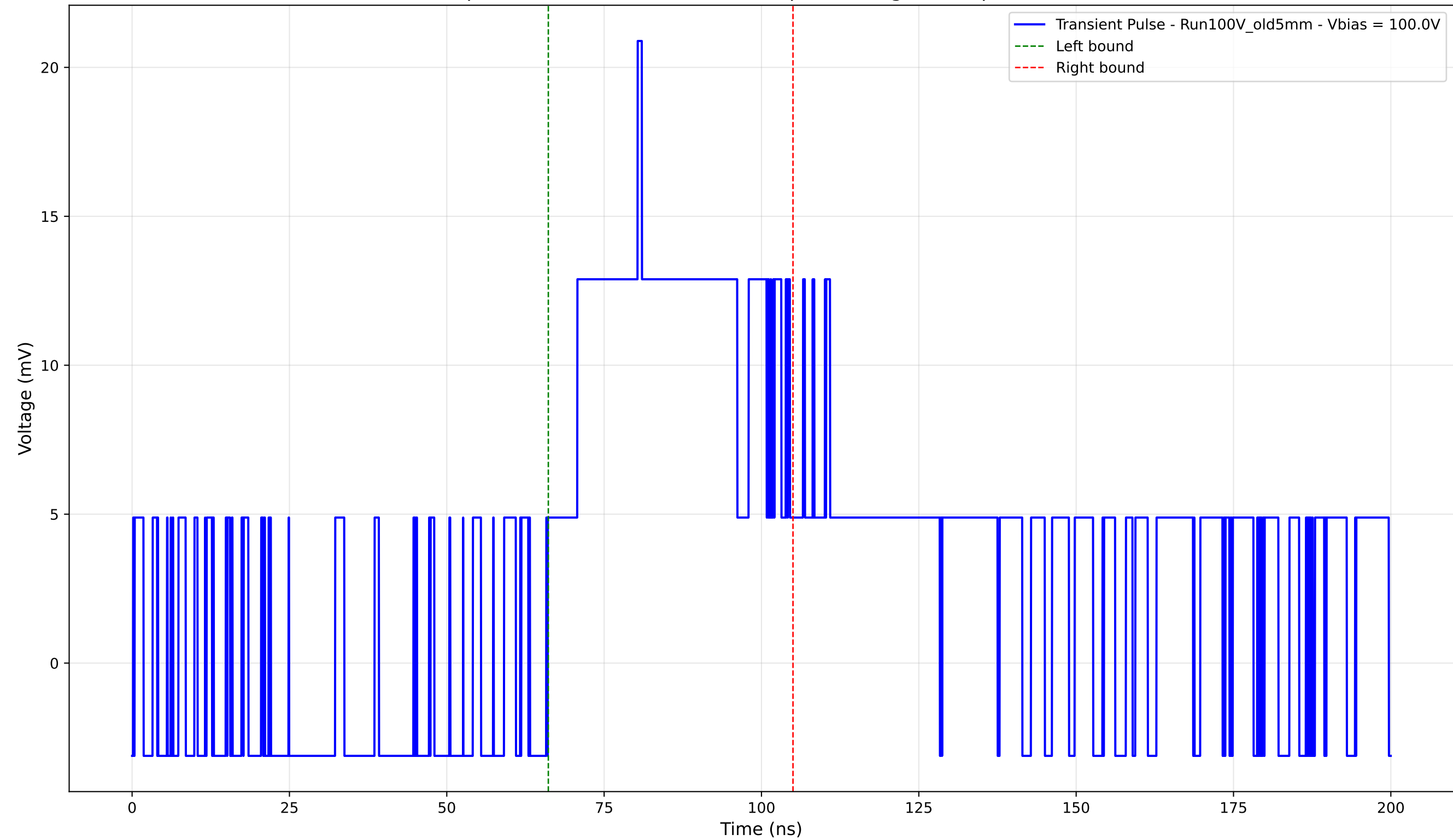
Transient Pulse - Sample: Old5mm - Position: 1440.0 \mu\text{m} - Charge: 8.78 pC - Rise Time: 0.00 ns (N/A)
