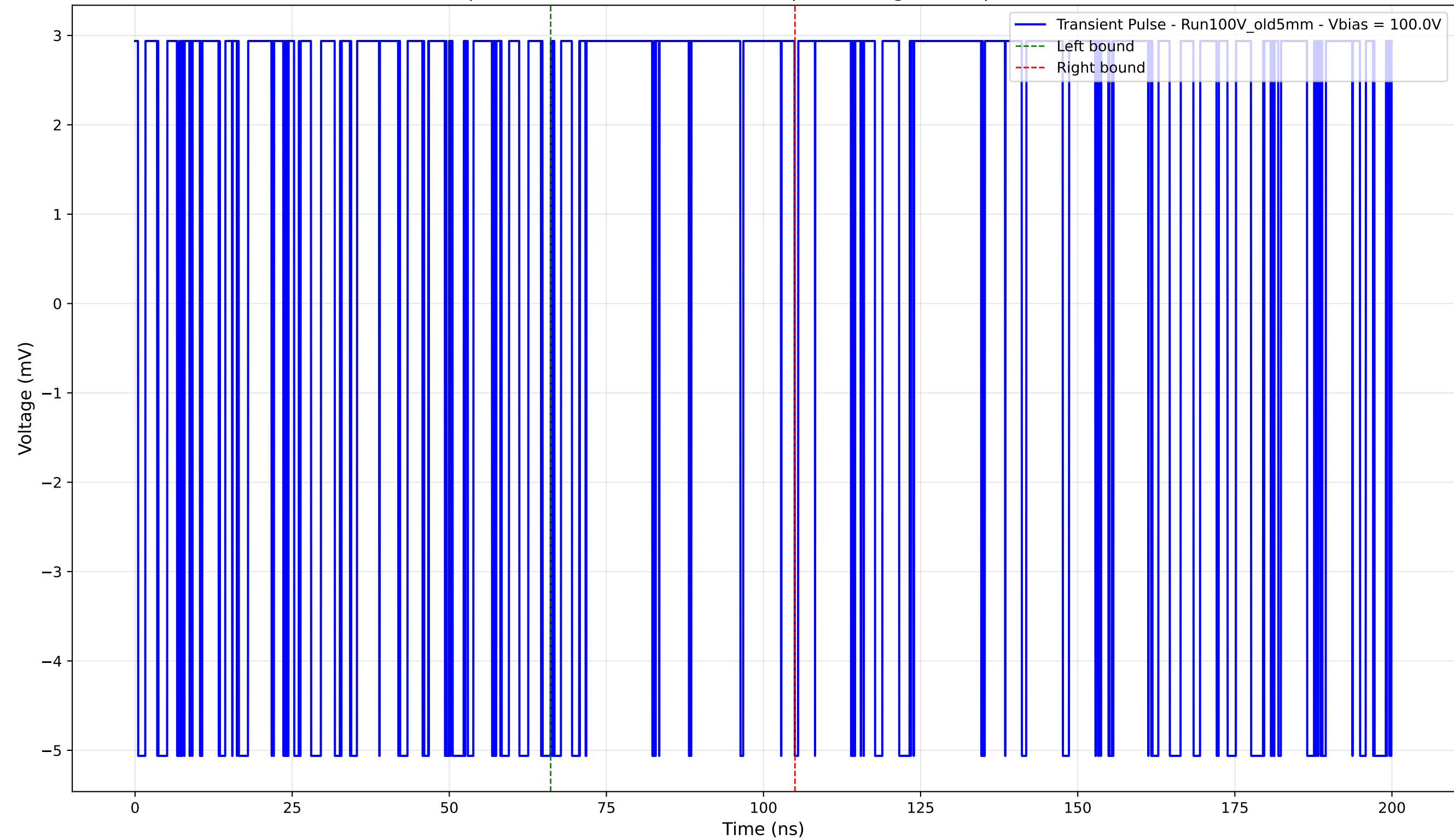
Transient Pulse - Sample: Old5mm - Position: 1295.0 \mu\text{m} - Charge: 1.67 pC - Rise Time: 0.00 ns (N/A)
