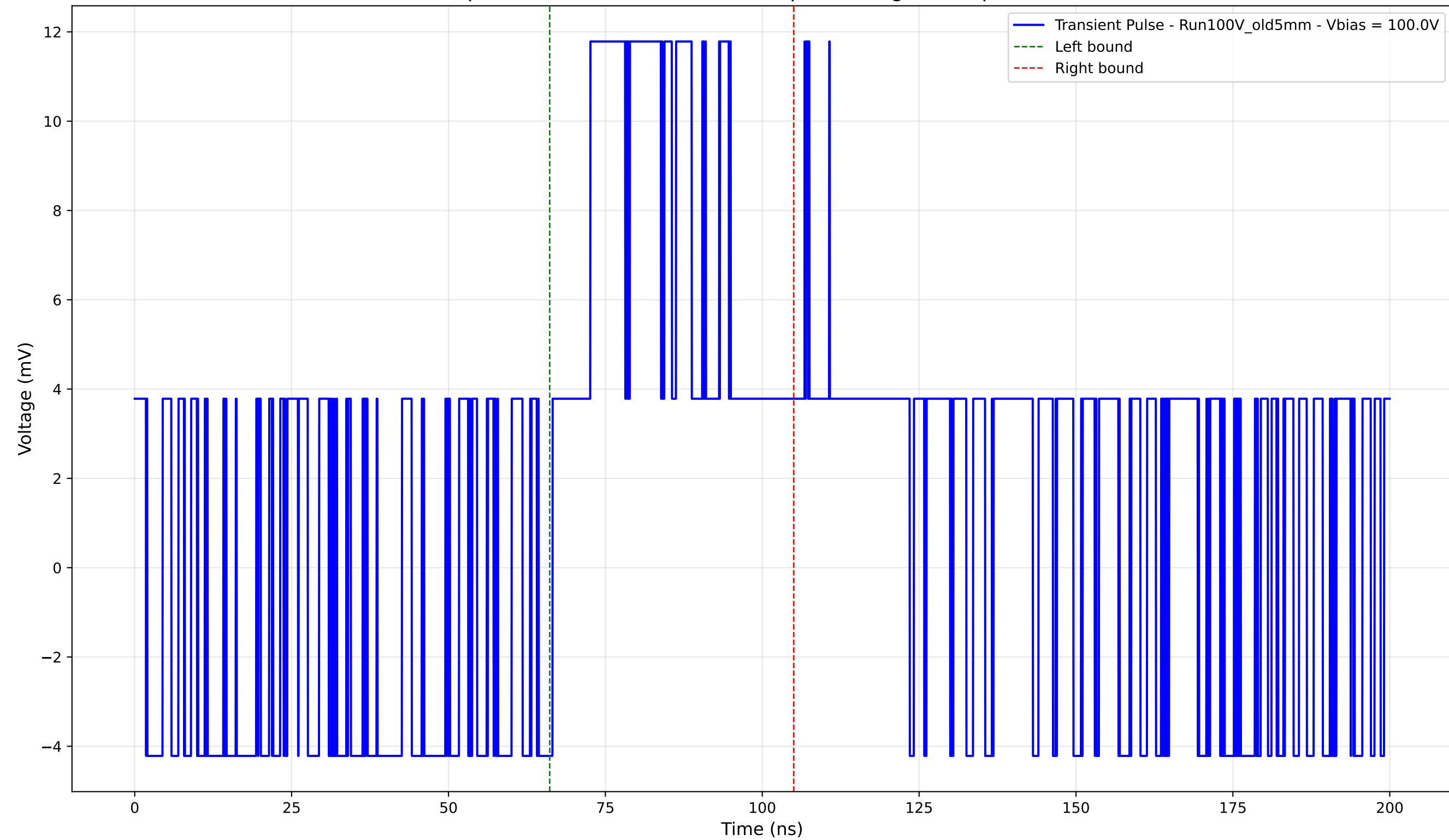
Transient Pulse - Sample: Old5mm - Position: 1065.0 \mu\text{m} - Charge: 5.53 pC - Rise Time: 0.00 ns (N/A)
