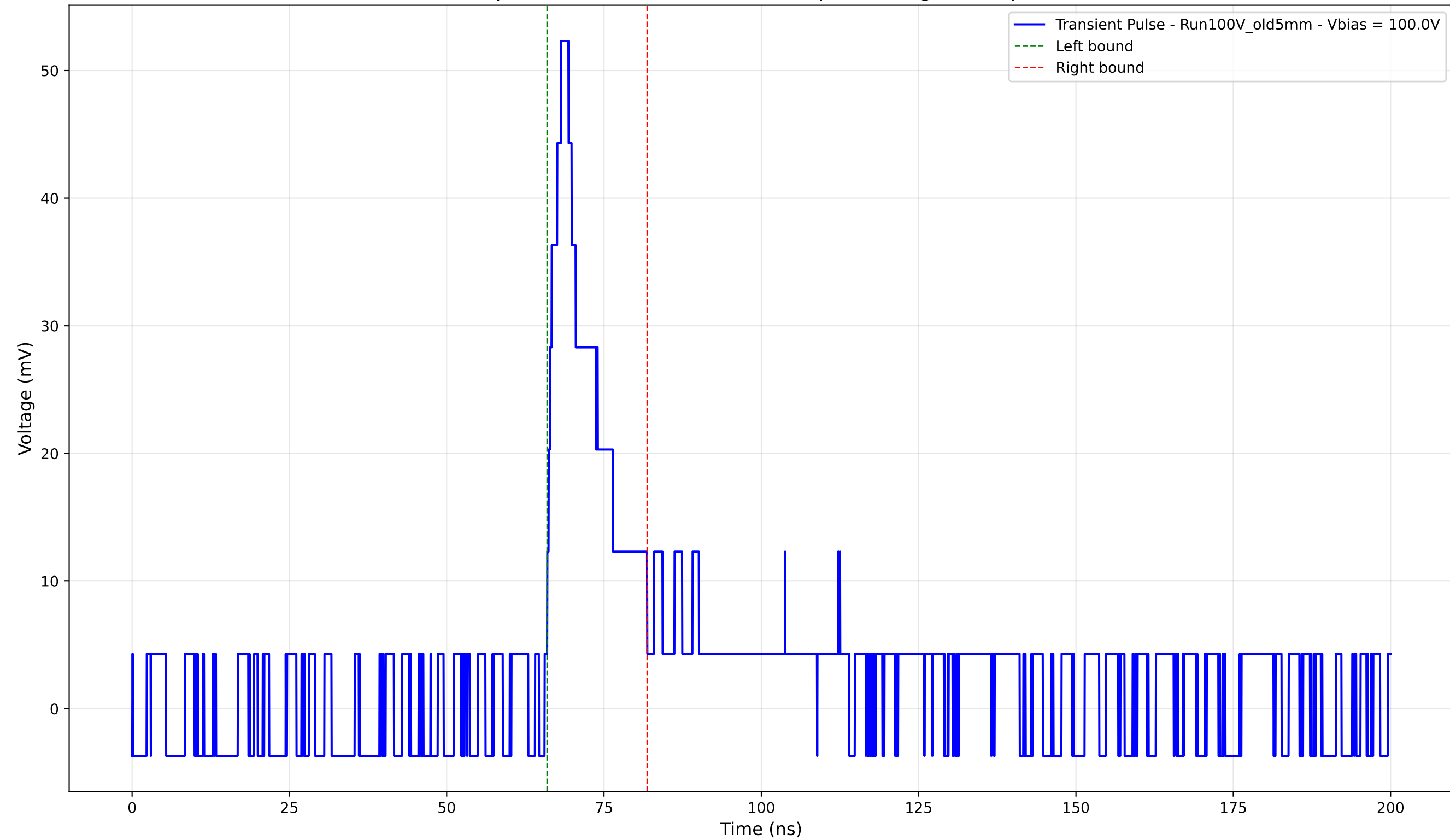
Transient Pulse - Sample: Old5mm - Position: 4235.0 \mu\text{m} - Charge: 7.90 pC - Rise Time: 2.20 ns
