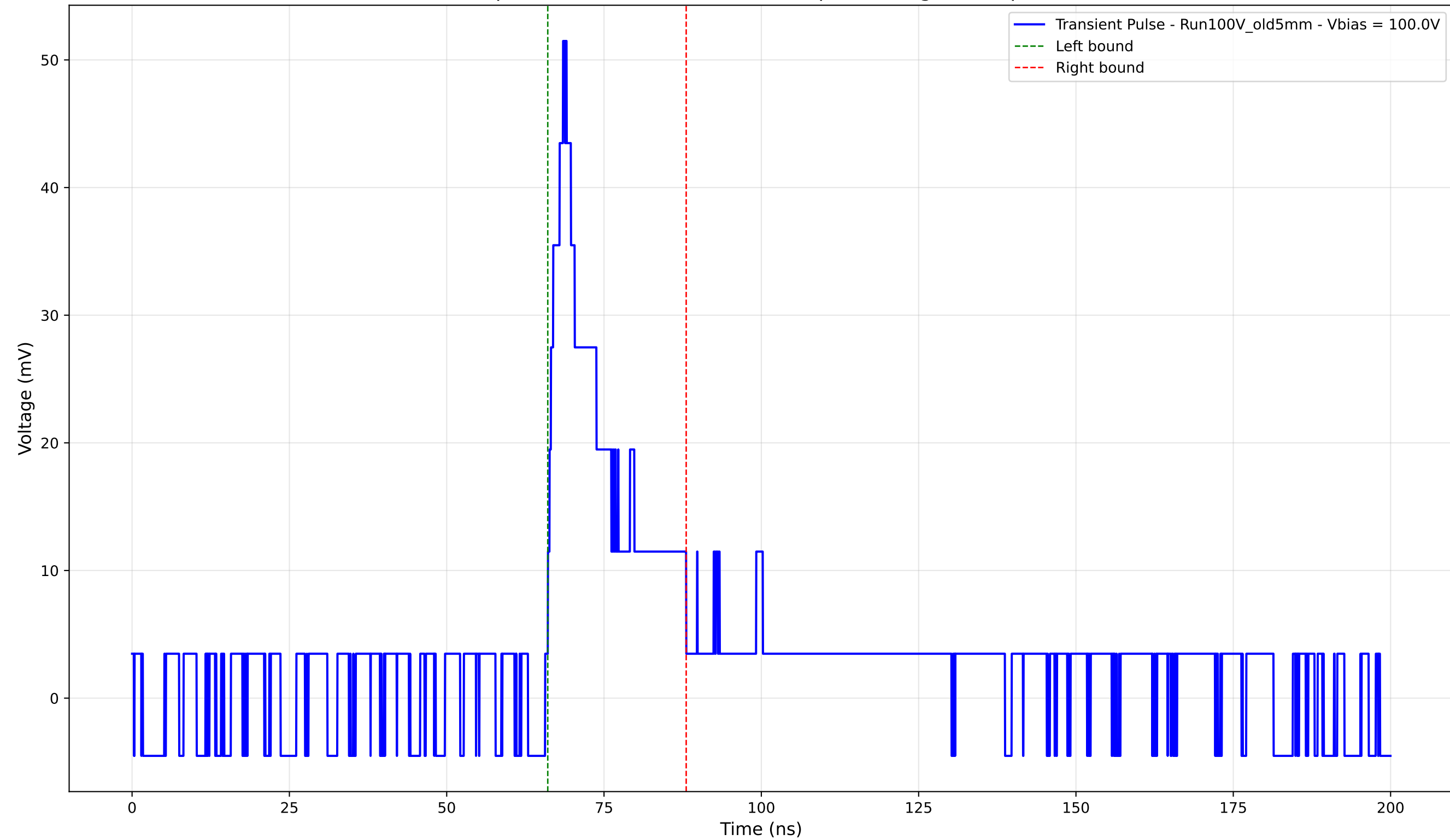
Transient Pulse - Sample: Old5mm - Position: 4390.0 \mu\text{m} - Charge: 8.85 pC - Rise Time: 2.42 ns
