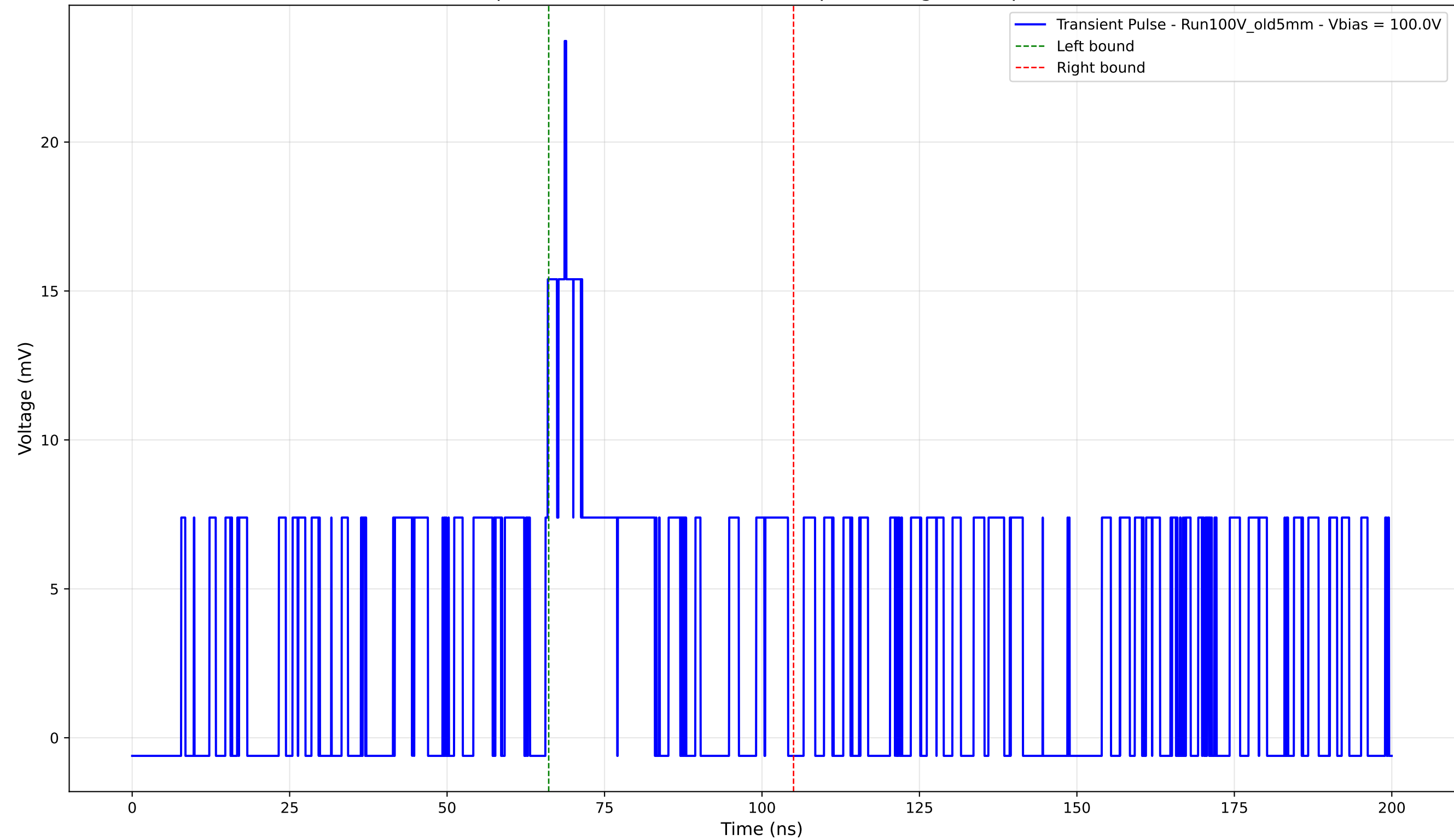
Transient Pulse - Sample: Old5mm - Position: 3435.0 \mu\text{m} - Charge: 4.61 pC - Rise Time: 3.05 ns
