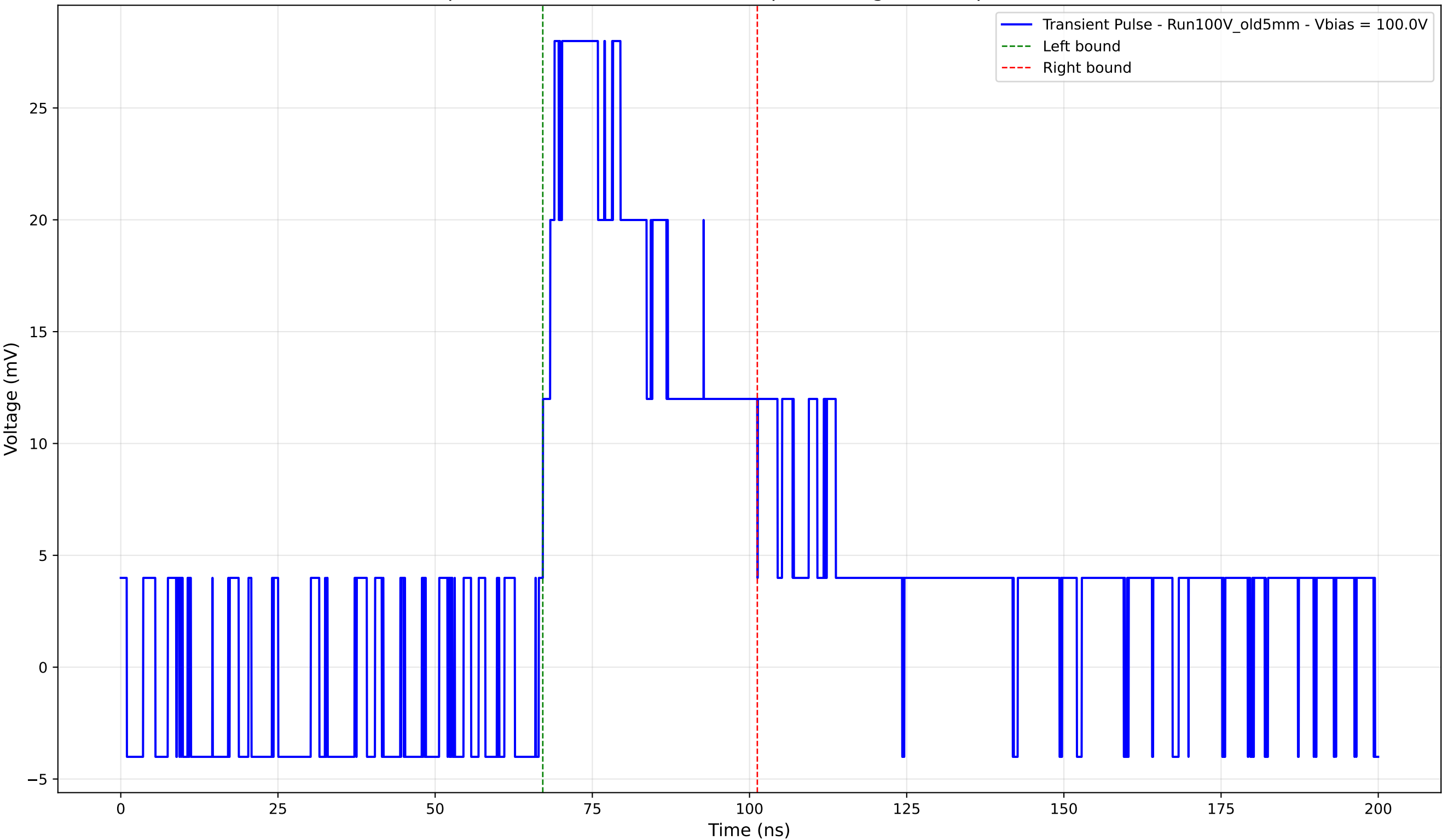
Transient Pulse - Sample: Old5mm - Position: 2430.0 \mu\text{m} - Charge: 12.30 pC - Rise Time: 0.00 ns (N/A)
