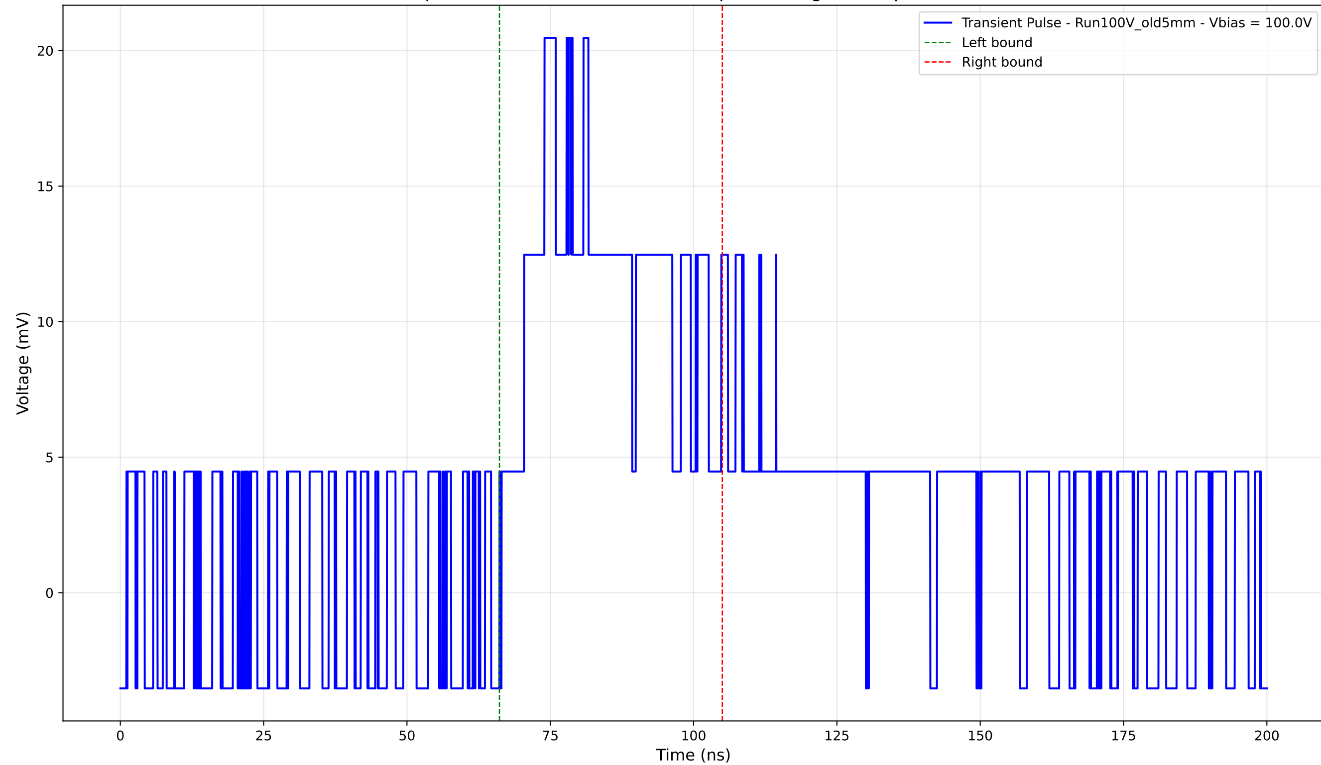
Transient Pulse - Sample: Old5mm - Position: 1220.0 \mu\text{m} - Charge: 8.72 pC - Rise Time: 0.00 ns (N/A)
