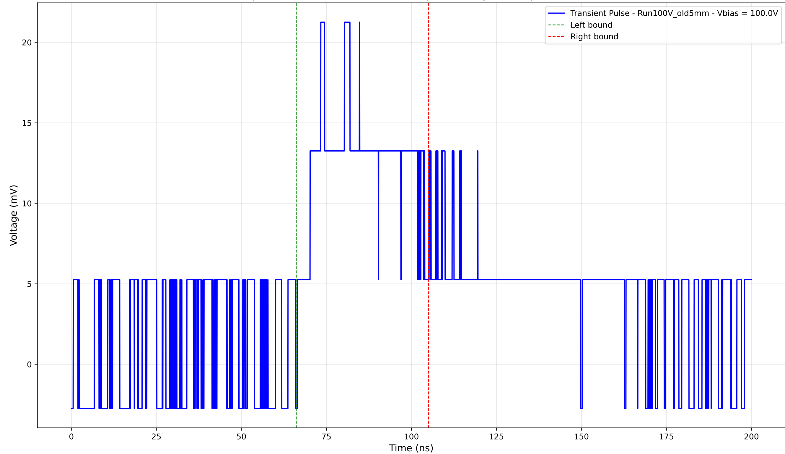
Transient Pulse - Sample: Old5mm - Position: 1395.0 \mu\text{m} - Charge: 9.80 pC - Rise Time: 0.00 ns (N/A)
