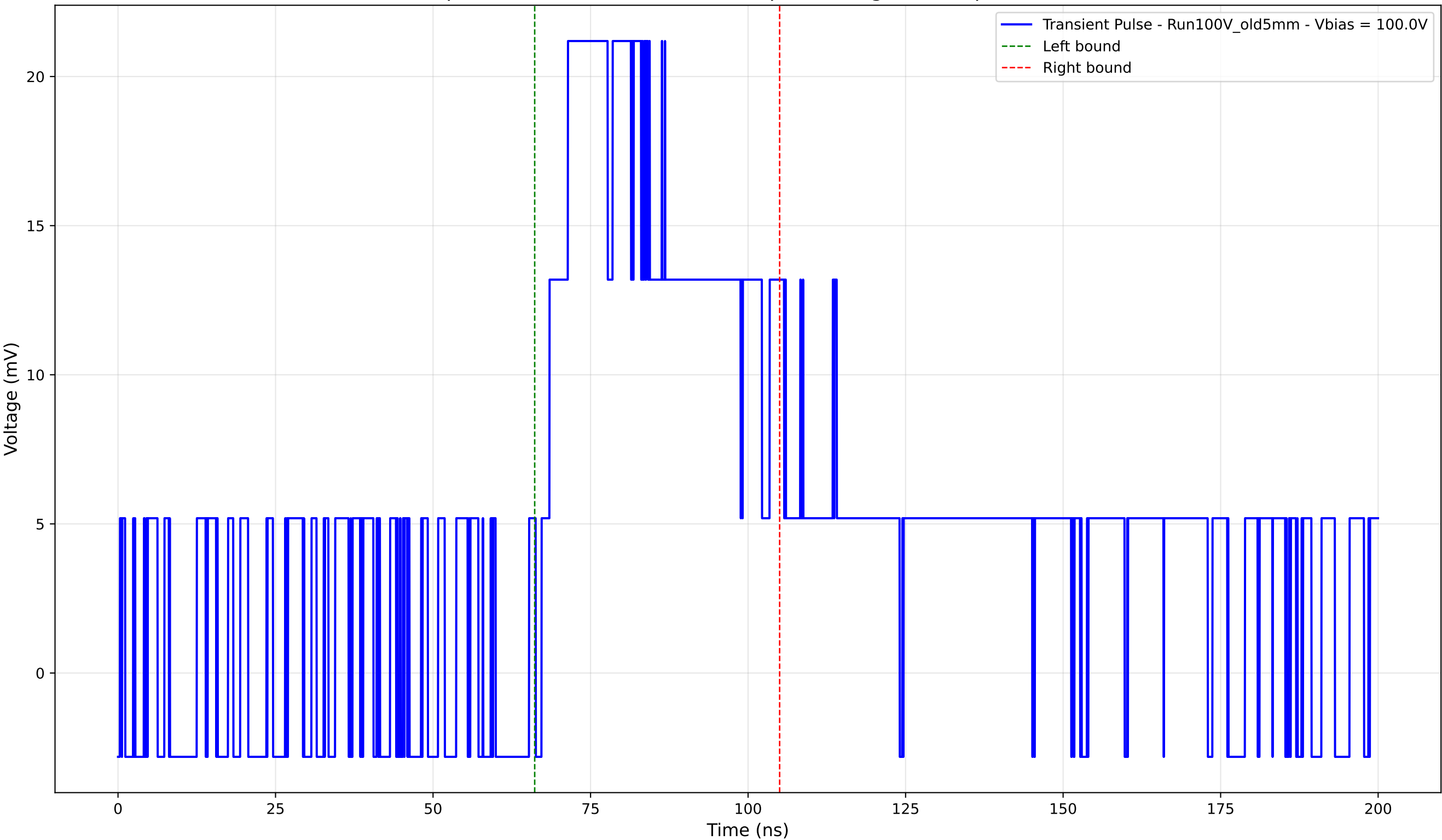
Transient Pulse - Sample: Old5mm - Position: 2040.0 \mu\text{m} - Charge: 11.33 pC - Rise Time: 0.00 ns (N/A)
