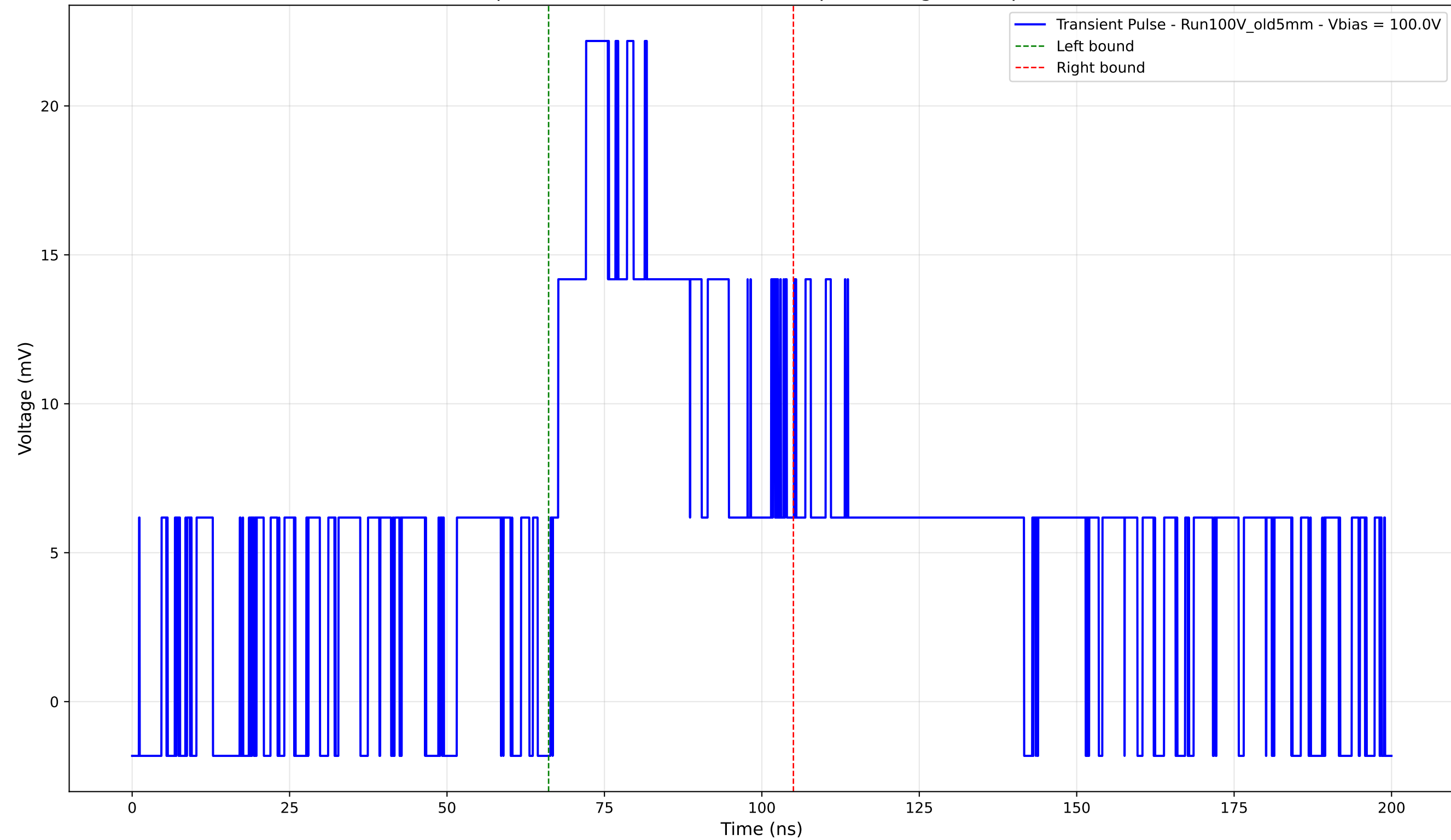
Transient Pulse - Sample: Old5mm - Position: 2175.0 \mu\text{m} - Charge: 9.95 pC - Rise Time: 5.30 ns
