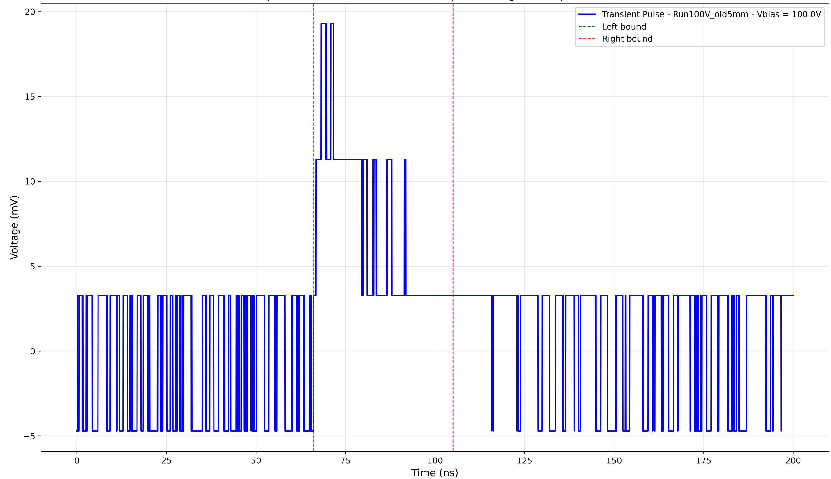
Transient Pulse - Sample: Old5mm - Position: 2855.0 \mu\text{m} - Charge: 5.55 pC - Rise Time: 0.00 ns (N/A)
