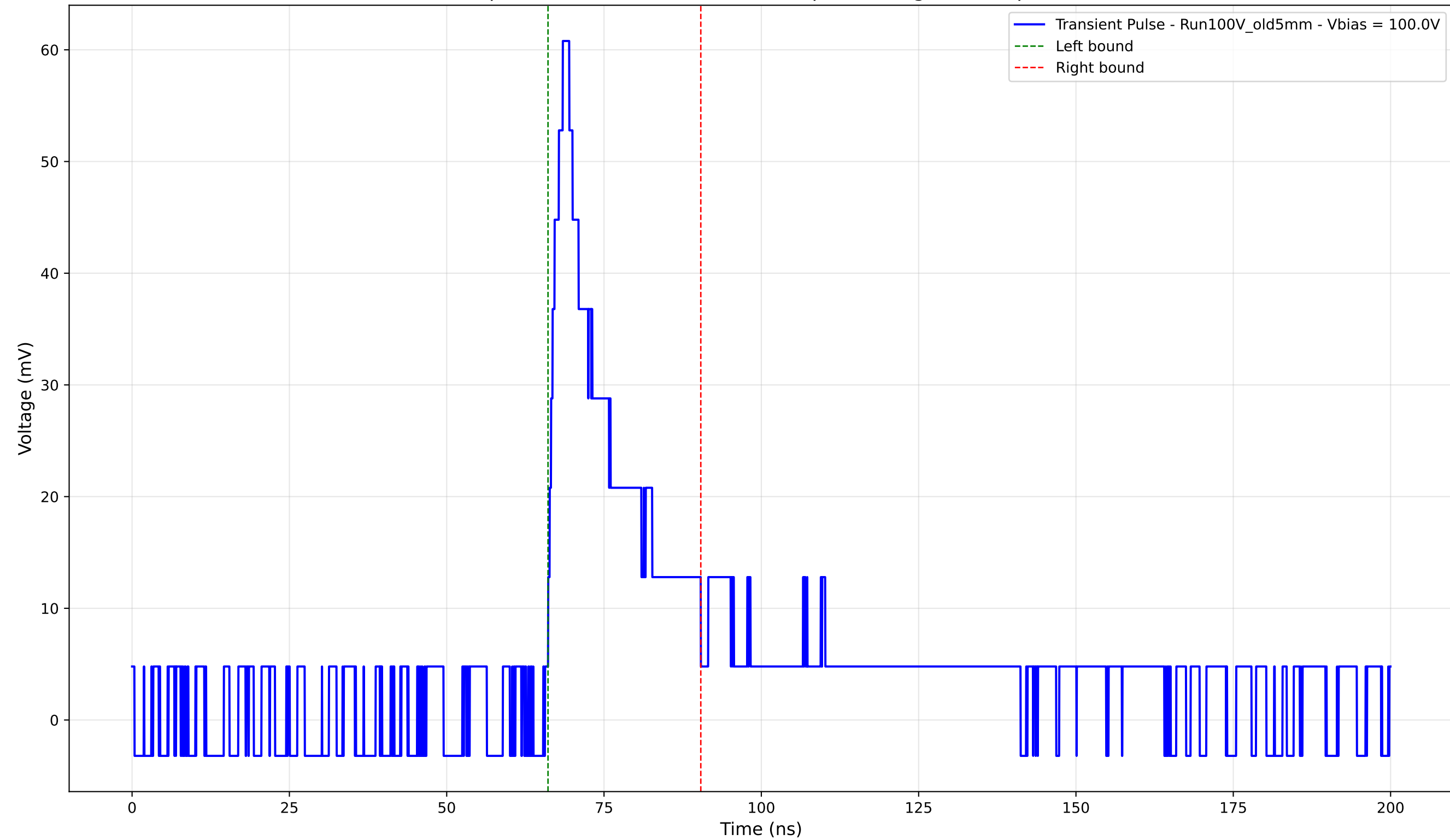
Transient Pulse - Sample: Old5mm - Position: 3010.0 \mu\text{m} - Charge: 12.35 pC - Rise Time: 2.34 ns
