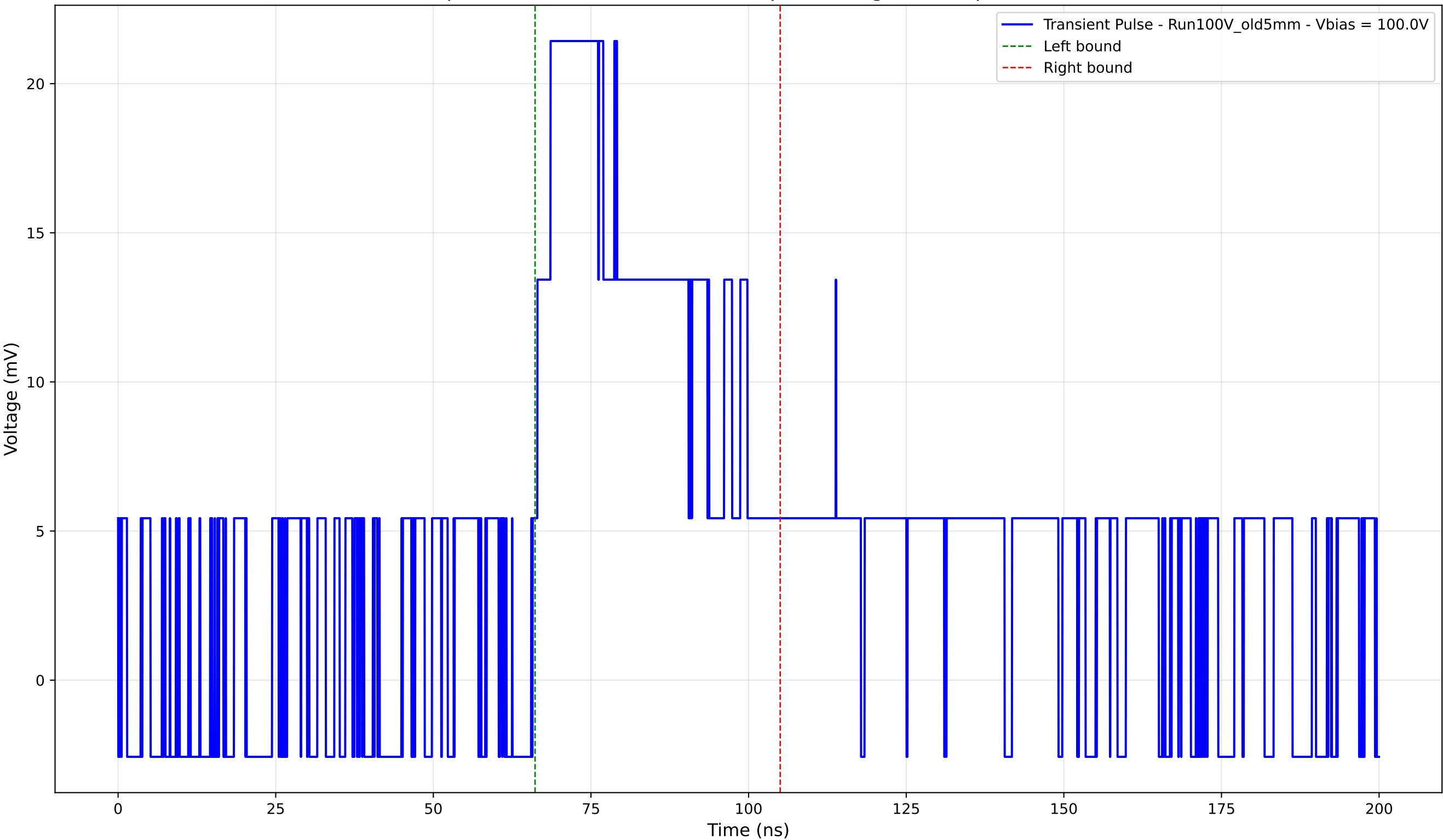
Transient Pulse - Sample: Old5mm - Position: 5000.0 \mu\text{m} - Charge: 10.27 pC - Rise Time: 0.00 ns (N/A)
