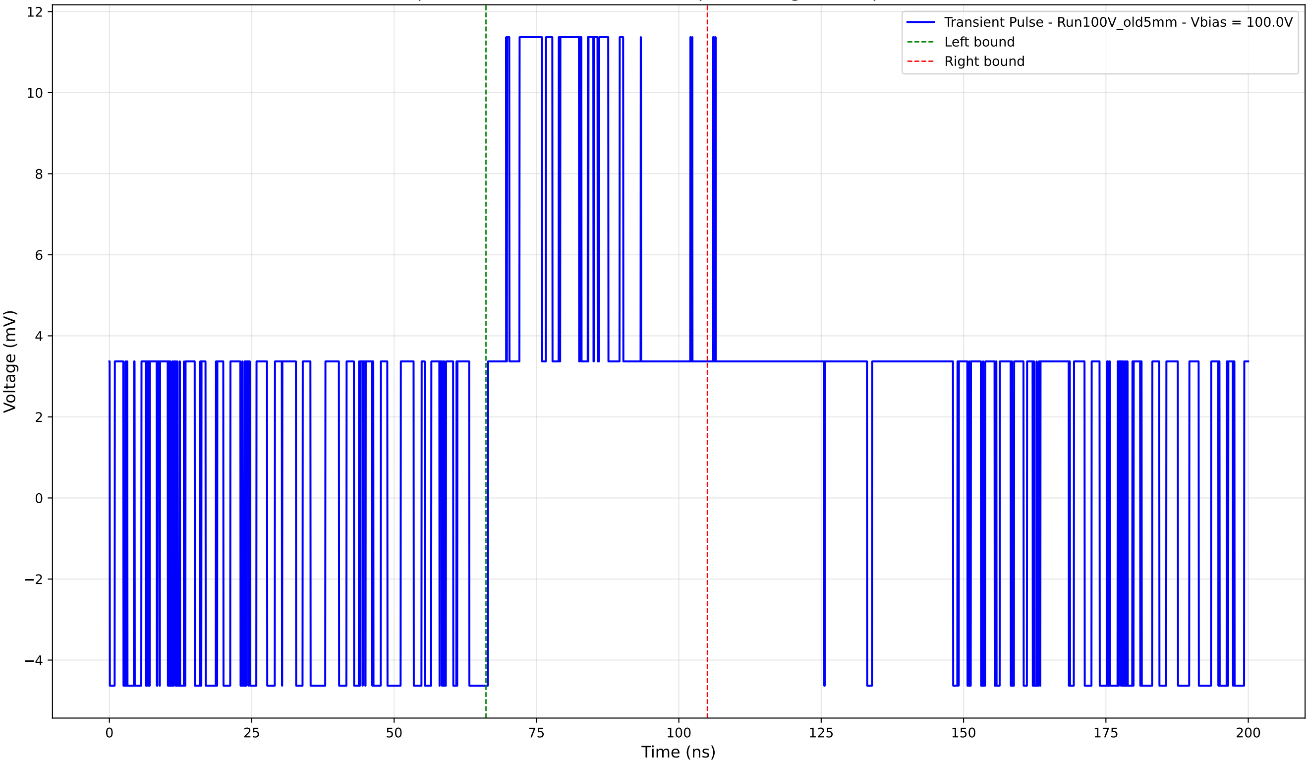
Transient Pulse - Sample: Old5mm - Position: 670.0 \mu\text{m} - Charge: 4.69 pC - Rise Time: 0.00 ns (N/A)
