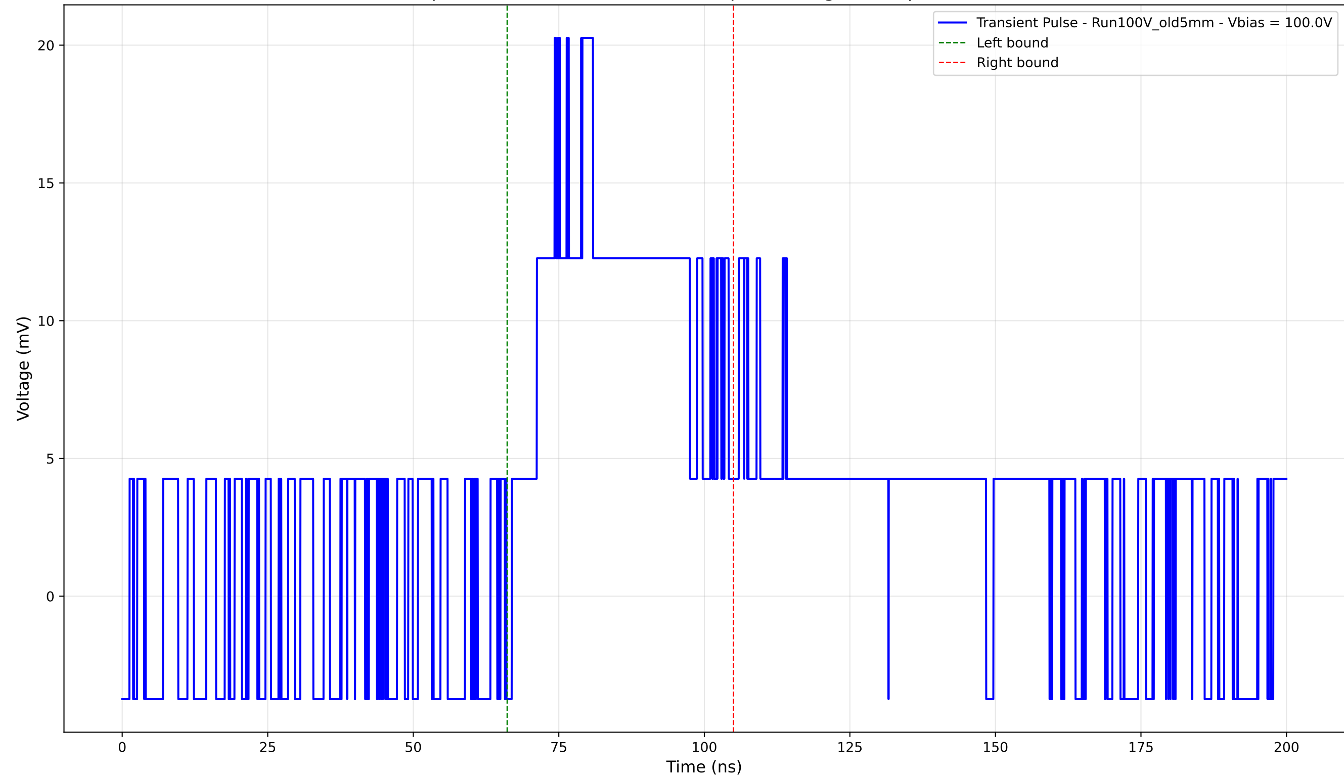
Transient Pulse - Sample: Old5mm - Position: 1205.0 \mu\text{m} - Charge: 8.31 pC - Rise Time: 0.00 ns (N/A)
