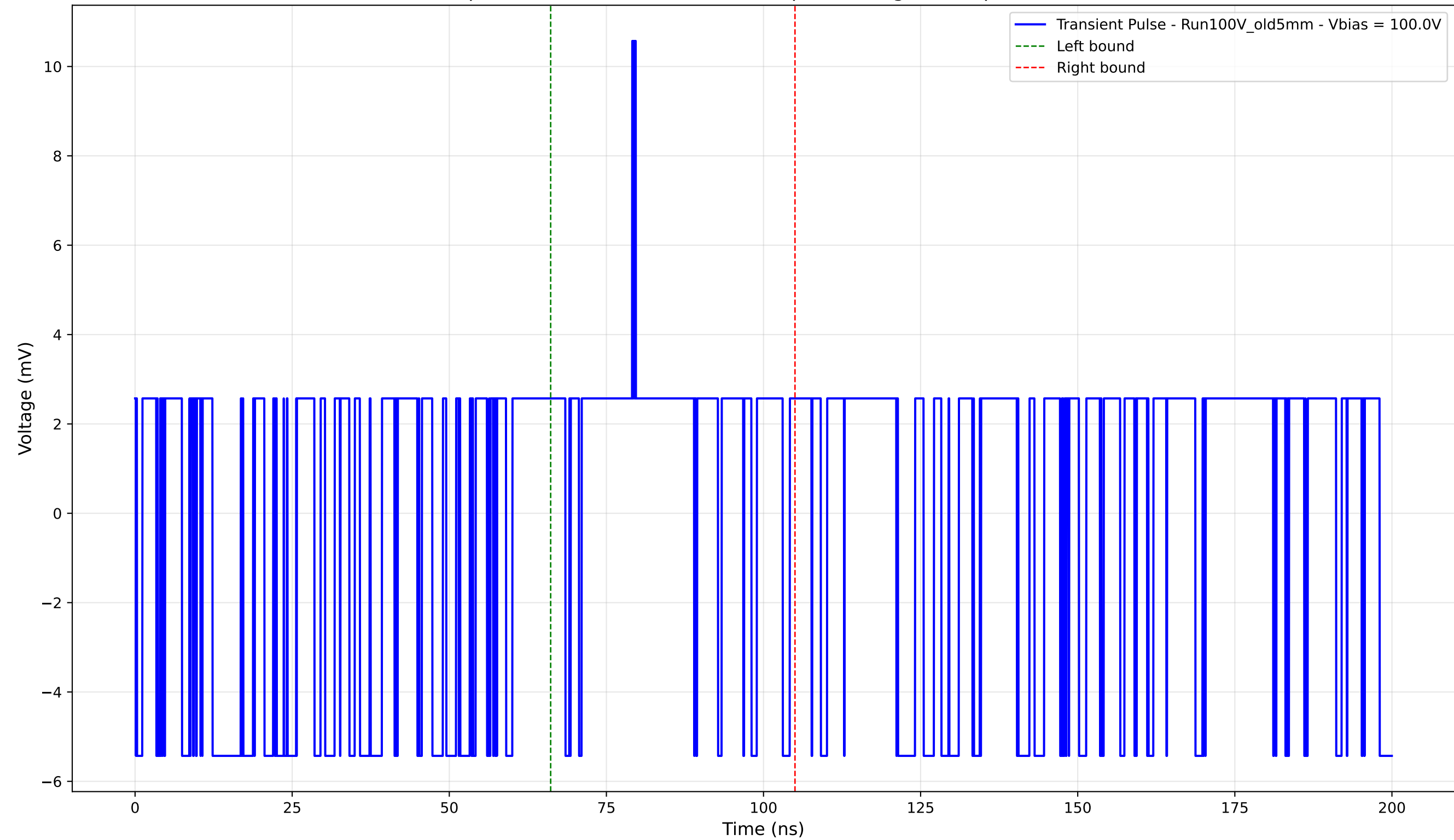
Transient Pulse - Sample: Old5mm - Position: 1925.0 \mu\text{m} - Charge: 1.41 pC - Rise Time: 0.00 ns (N/A)
