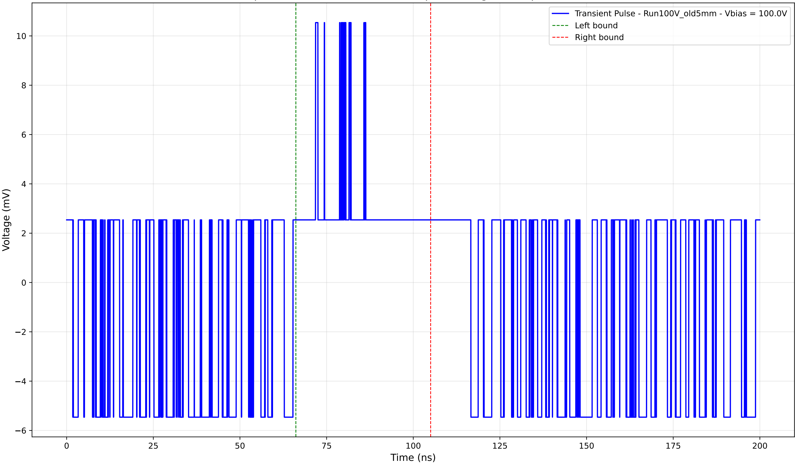
Transient Pulse - Sample: Old5mm - Position: 930.0 \mu\text{m} - Charge: 2.35 pC - Rise Time: 0.00 ns (N/A)
