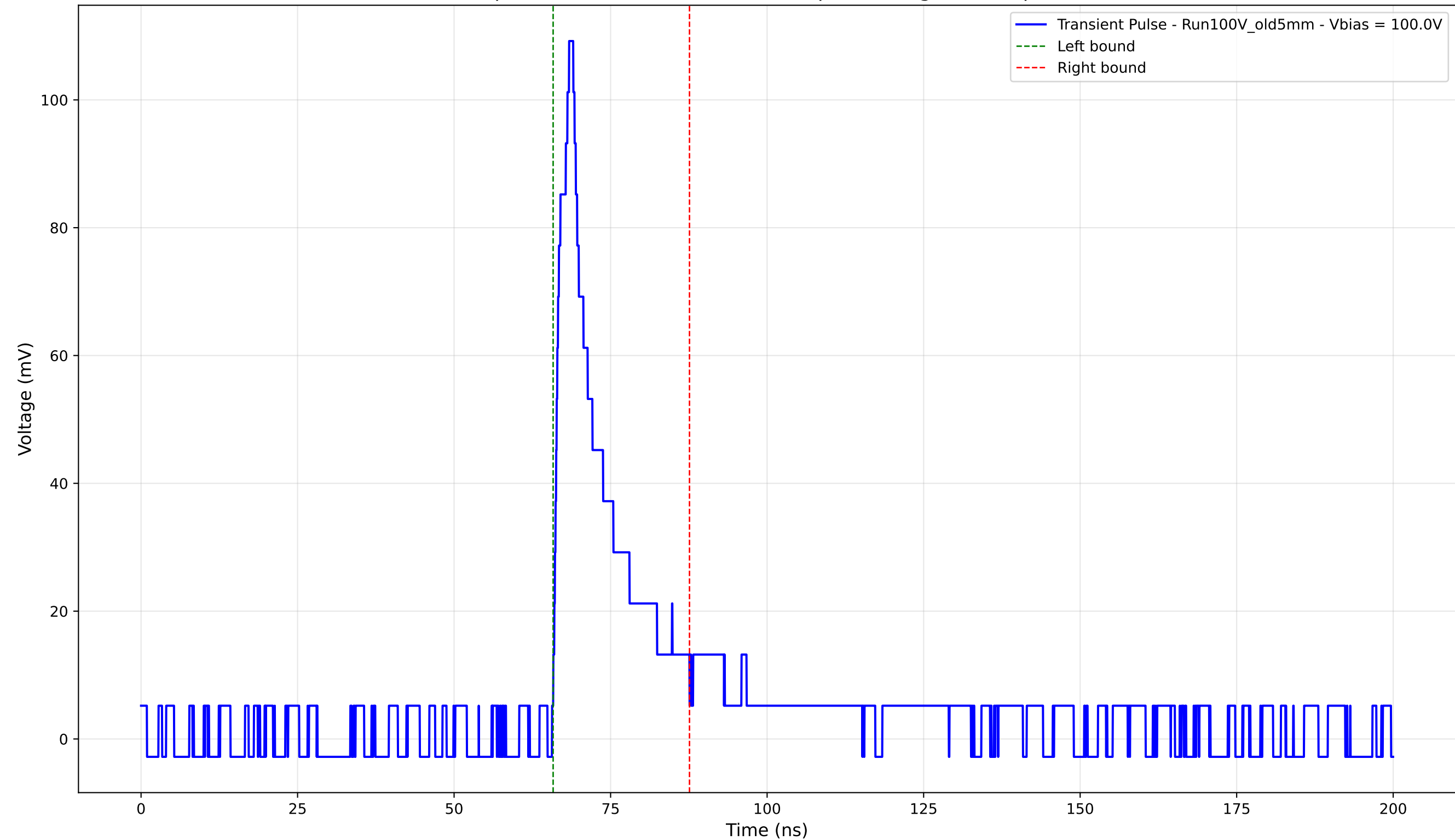
Transient Pulse - Sample: Old5mm - Position: 4185.0 \mu\text{m} - Charge: 16.80 pC - Rise Time: 2.27 ns
