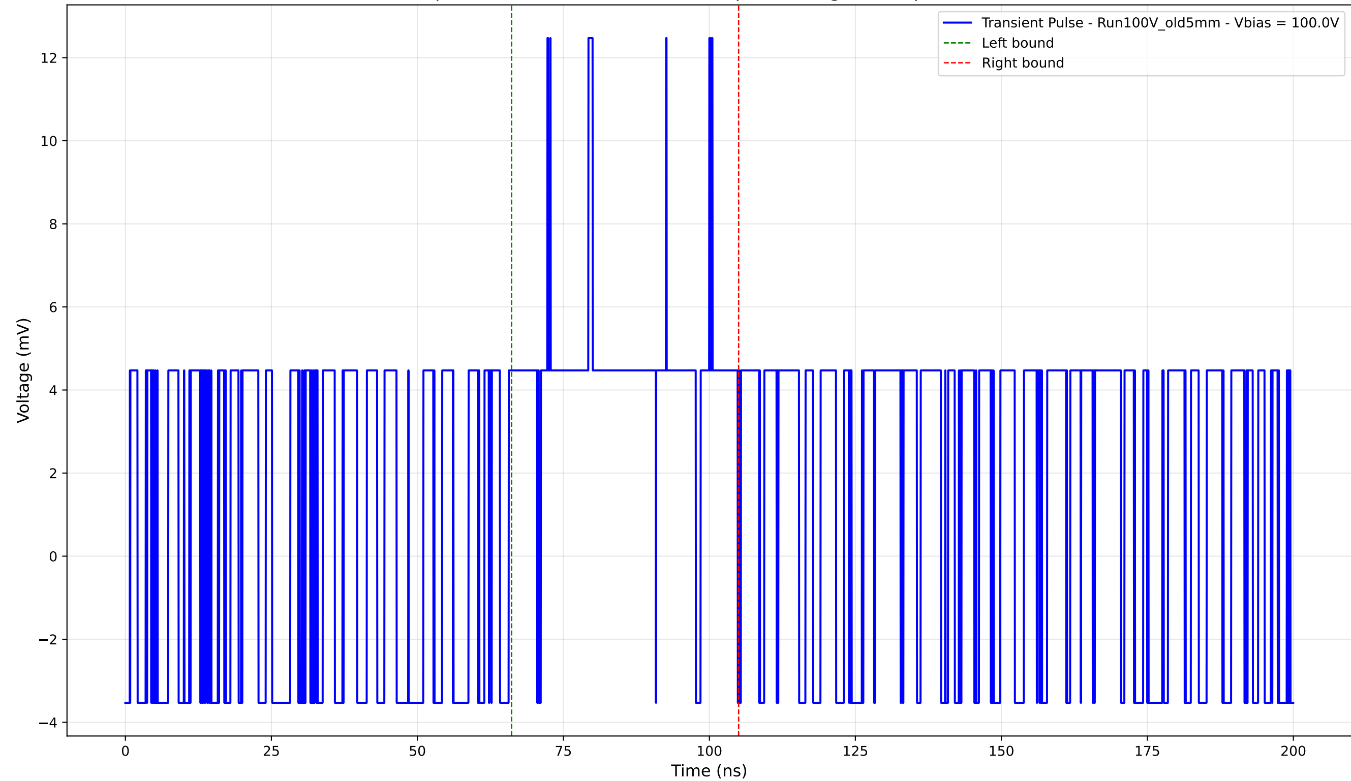
Transient Pulse - Sample: Old5mm - Position: 1685.0 \mu\text{m} - Charge: 3.47 pC - Rise Time: 0.00 ns (N/A)
