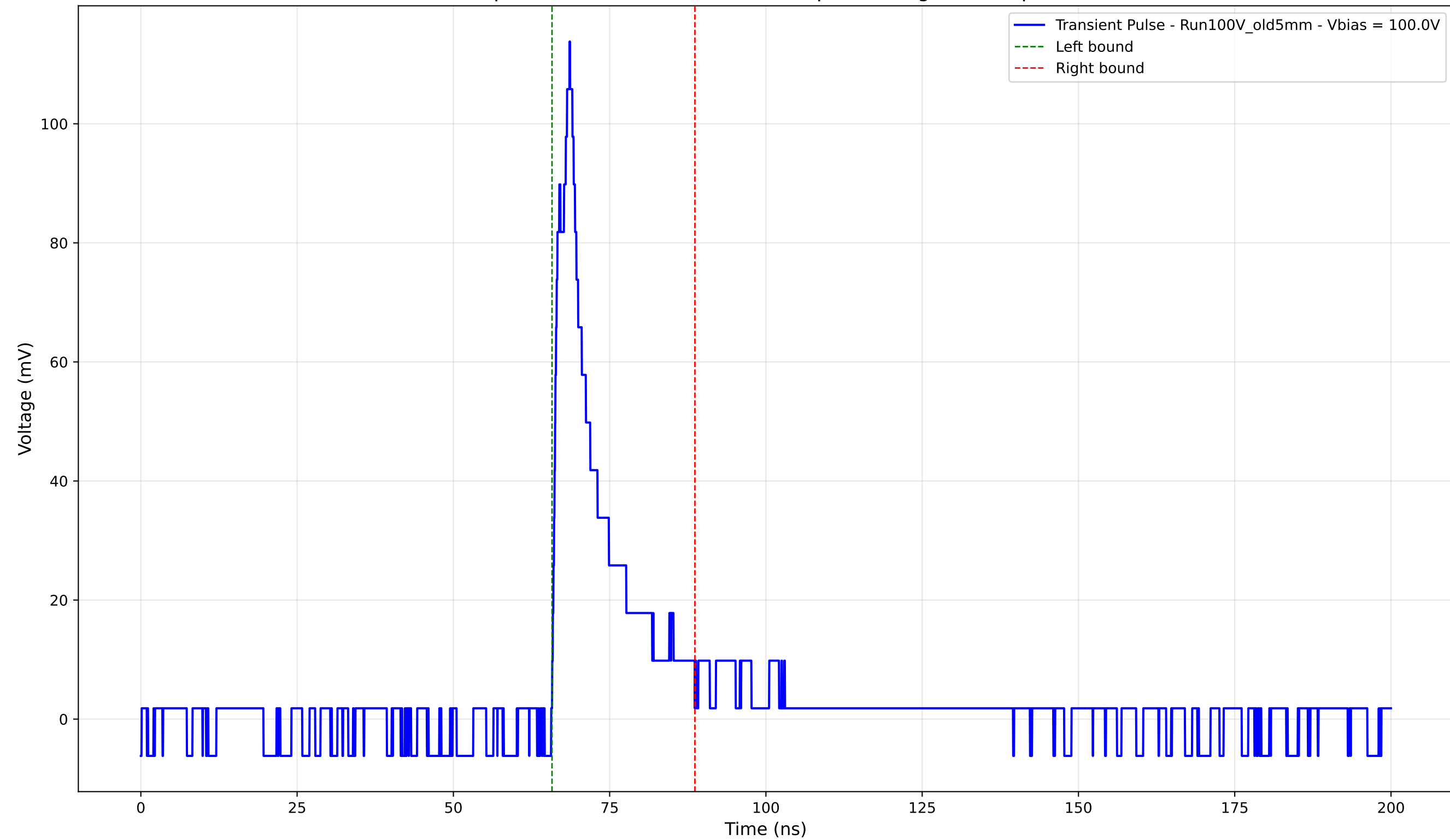
Transient Pulse - Sample: Old5mm - Position: 4160.0 \mu\text{m} - Charge: 15.55 pC - Rise Time: 2.30 ns
