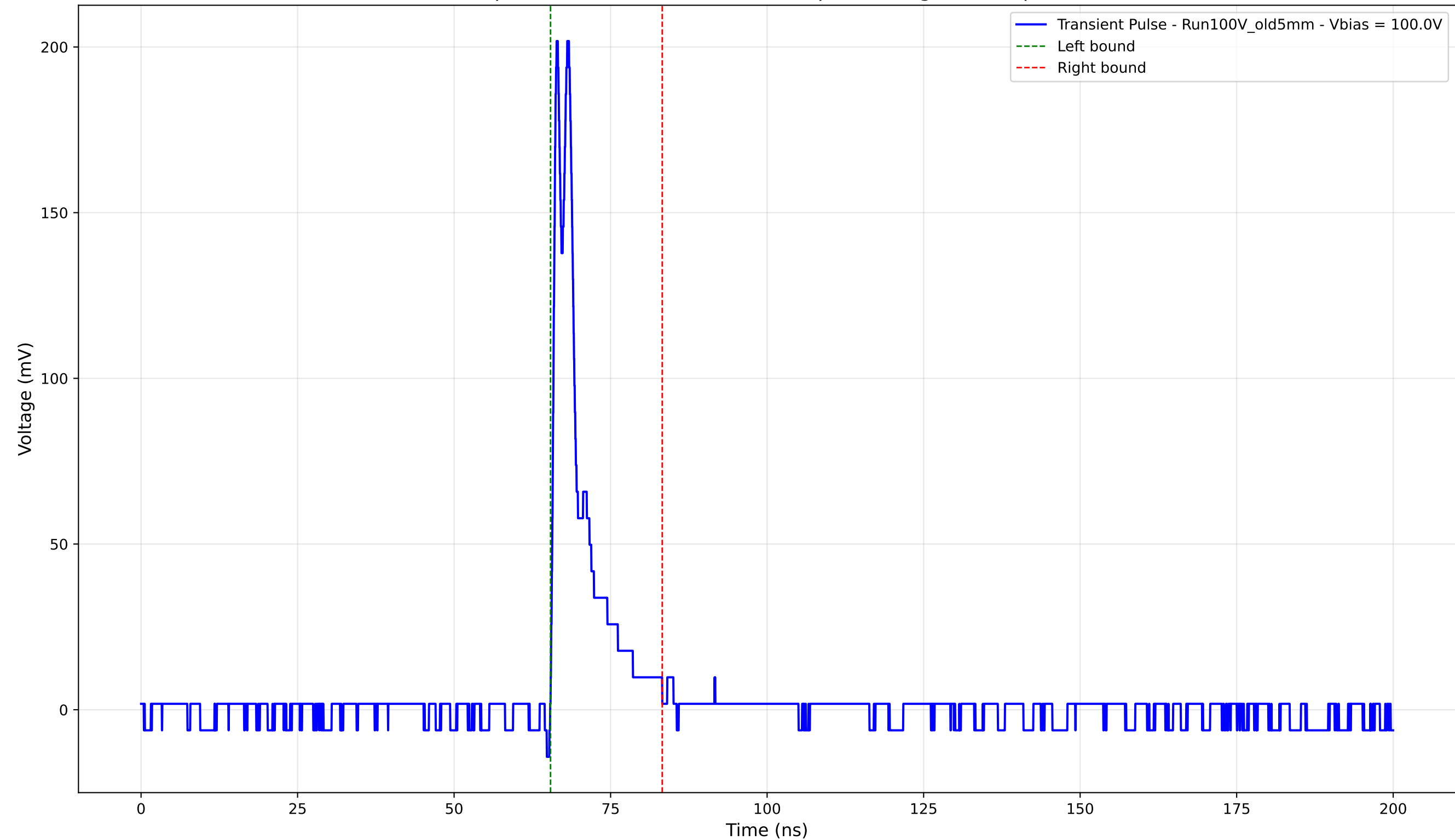
Transient Pulse - Sample: Old5mm - Position: 3600.0 \mu\text{m} - Charge: 19.37 pC - Rise Time: 0.71 ns
