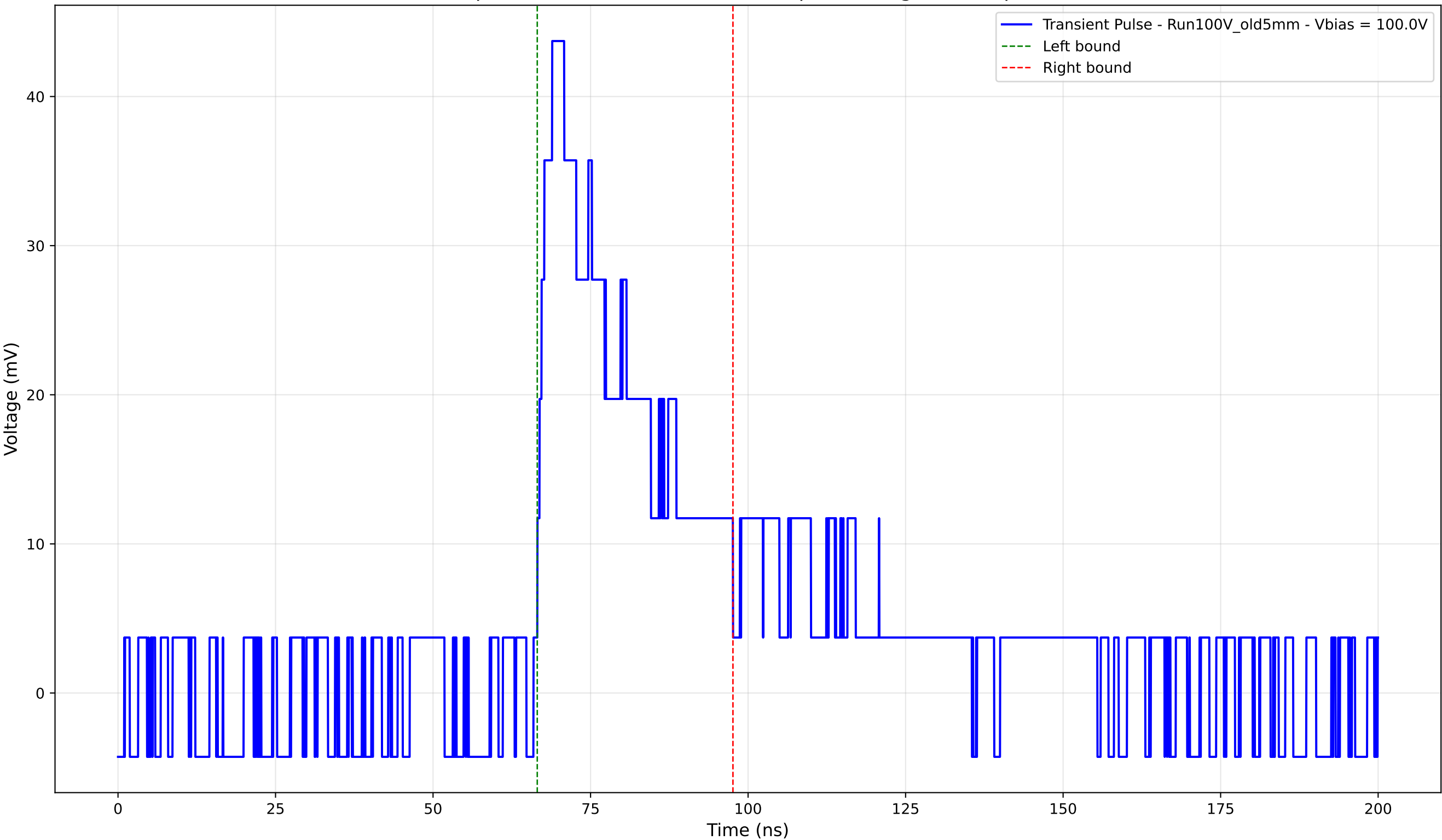
Transient Pulse - Sample: Old5mm - Position: 4725.0 \mu\text{m} - Charge: 13.37 pC - Rise Time: 2.36 ns
