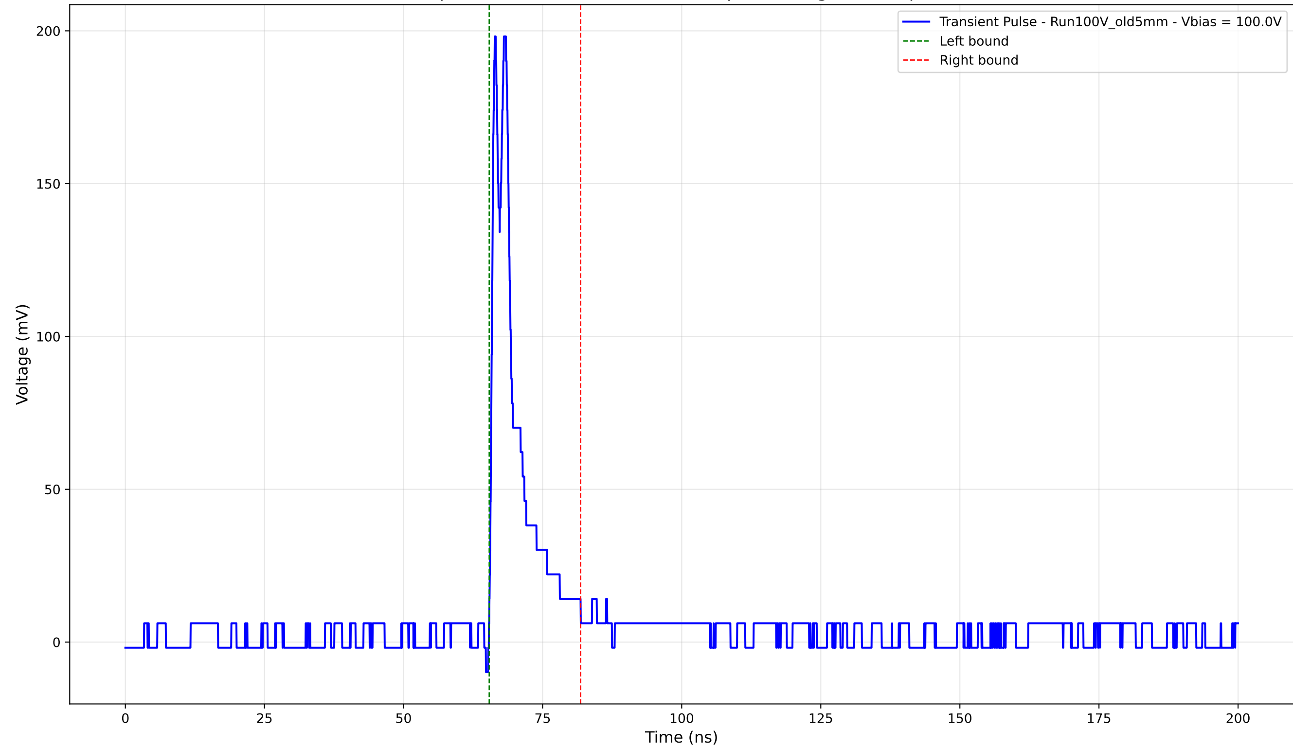
Transient Pulse - Sample: Old5mm - Position: 3825.0 \mu\text{m} - Charge: 19.91 pC - Rise Time: 0.77 ns
