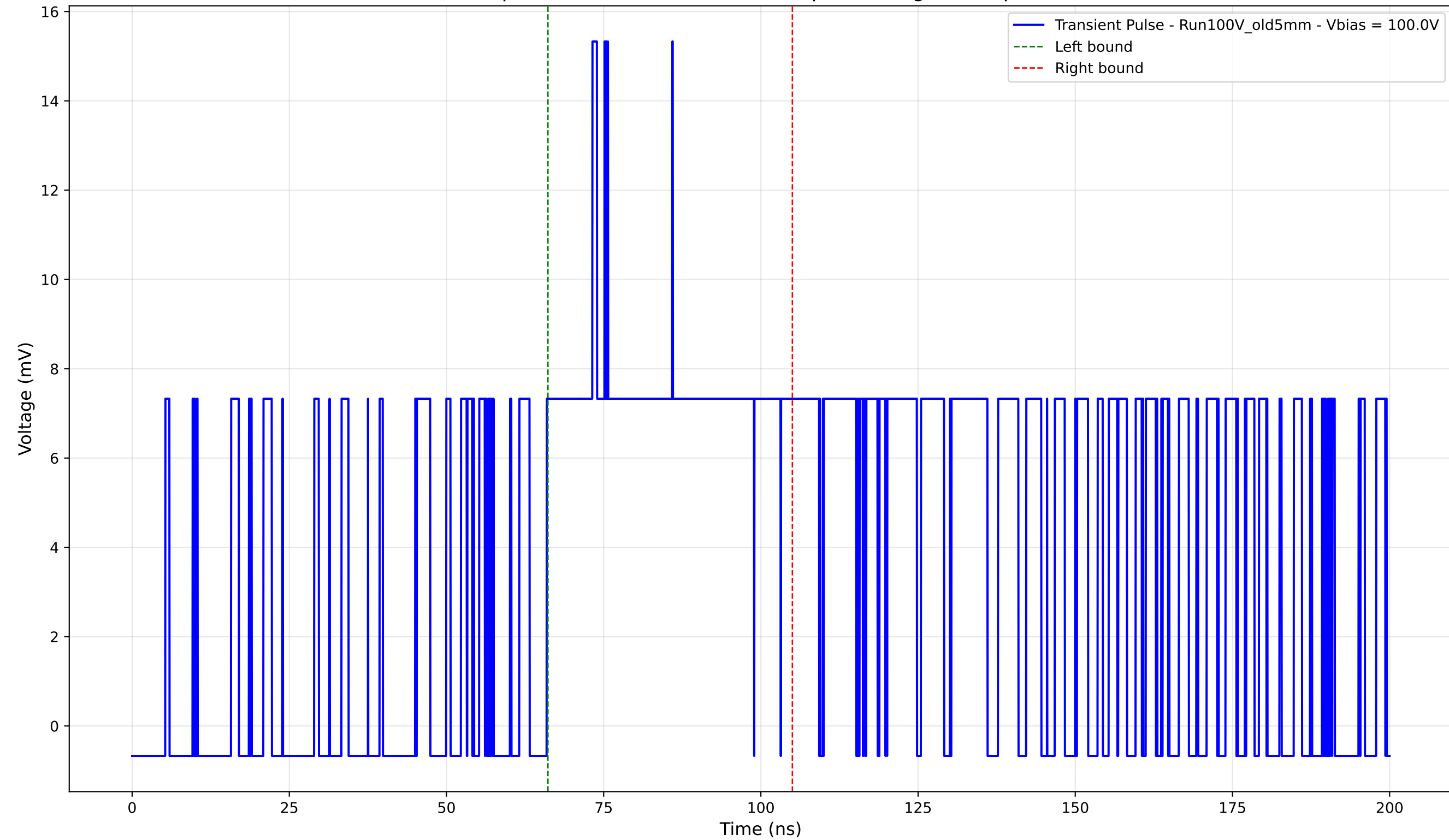
Transient Pulse - Sample: Old5mm - Position: 815.0 \mu\text{m} - Charge: 5.85 pC - Rise Time: 7.28 ns
