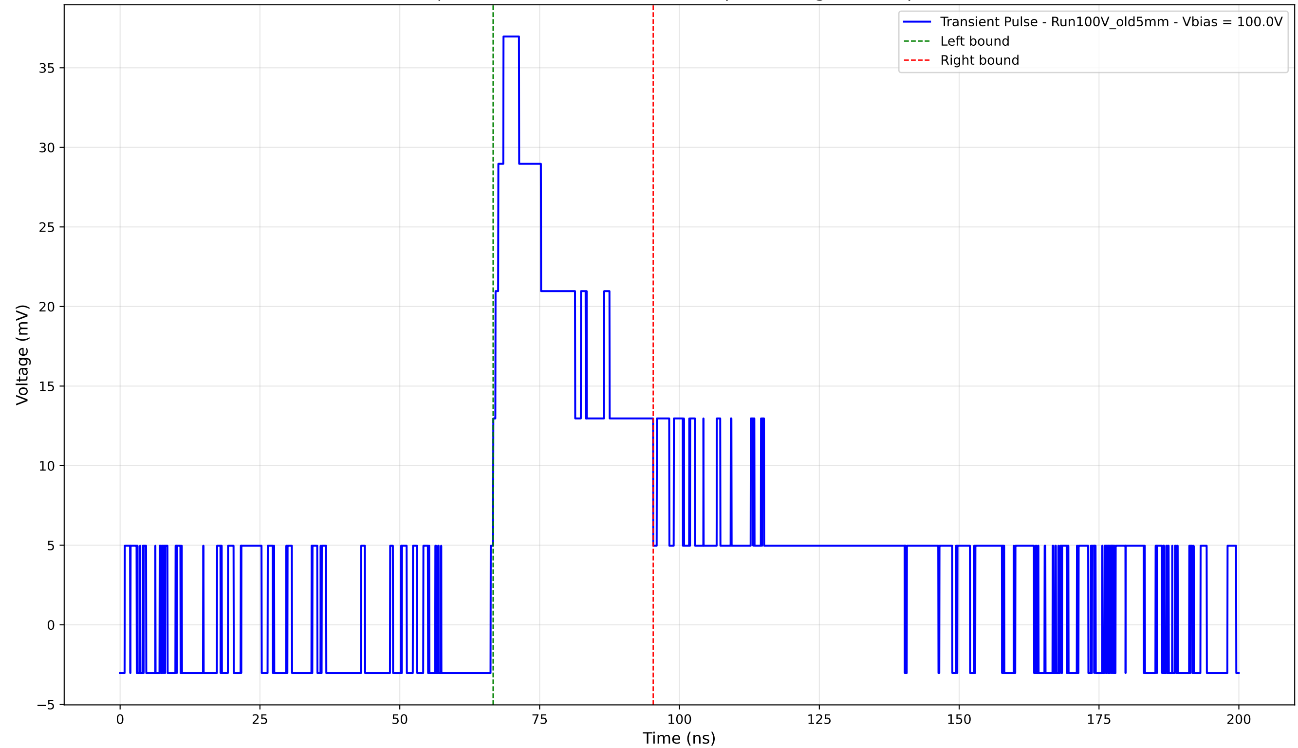
Transient Pulse - Sample: Old5mm - Position: 2690.0 \mu\text{m} - Charge: 11.67 pC - Rise Time: 2.29 ns
