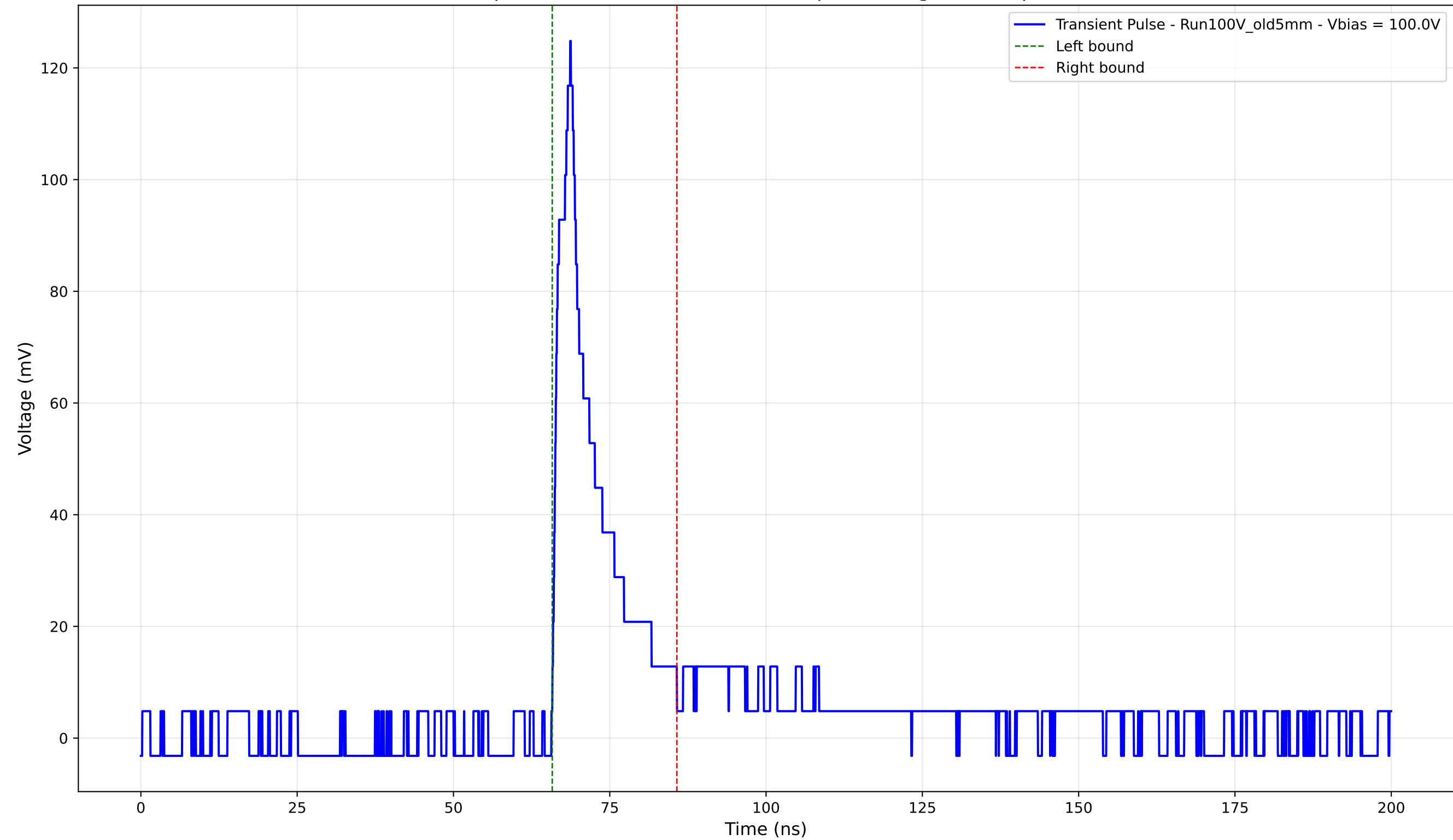
Transient Pulse - Sample: Old5mm - Position: 3245.0 \mu\text{m} - Charge: 16.84 pC - Rise Time: 2.46 ns
