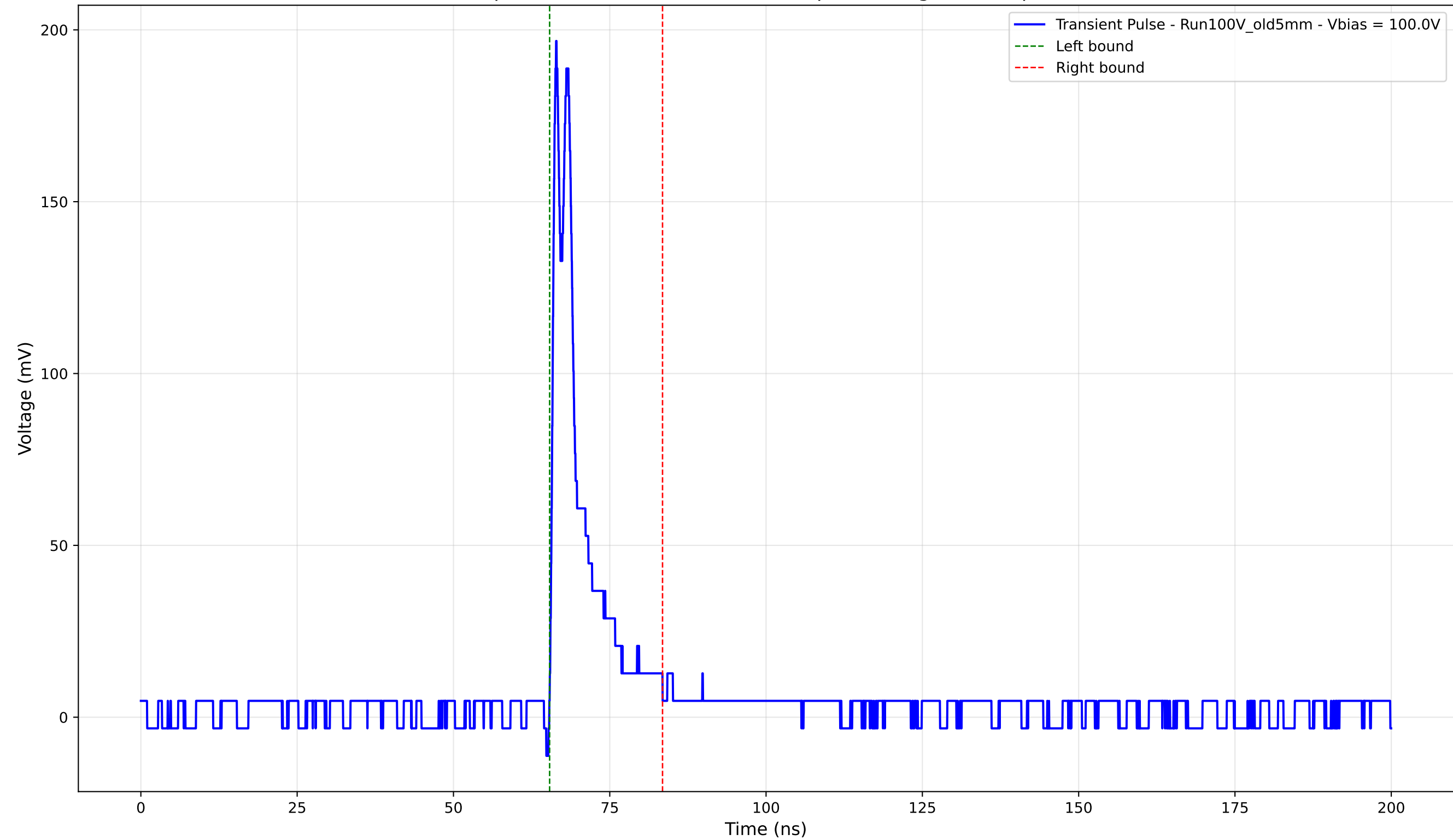
Transient Pulse - Sample: Old5mm - Position: 3815.0 \mu\text{m} - Charge: 19.12 pC - Rise Time: 0.76 ns
