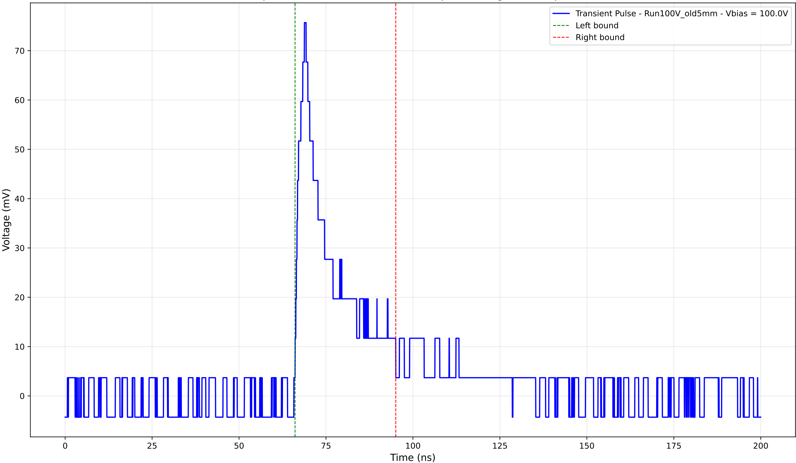
Transient Pulse - Sample: Old5mm - Position: 4440.0 \mu\text{m} - Charge: 15.22 pC - Rise Time: 2.67 ns
