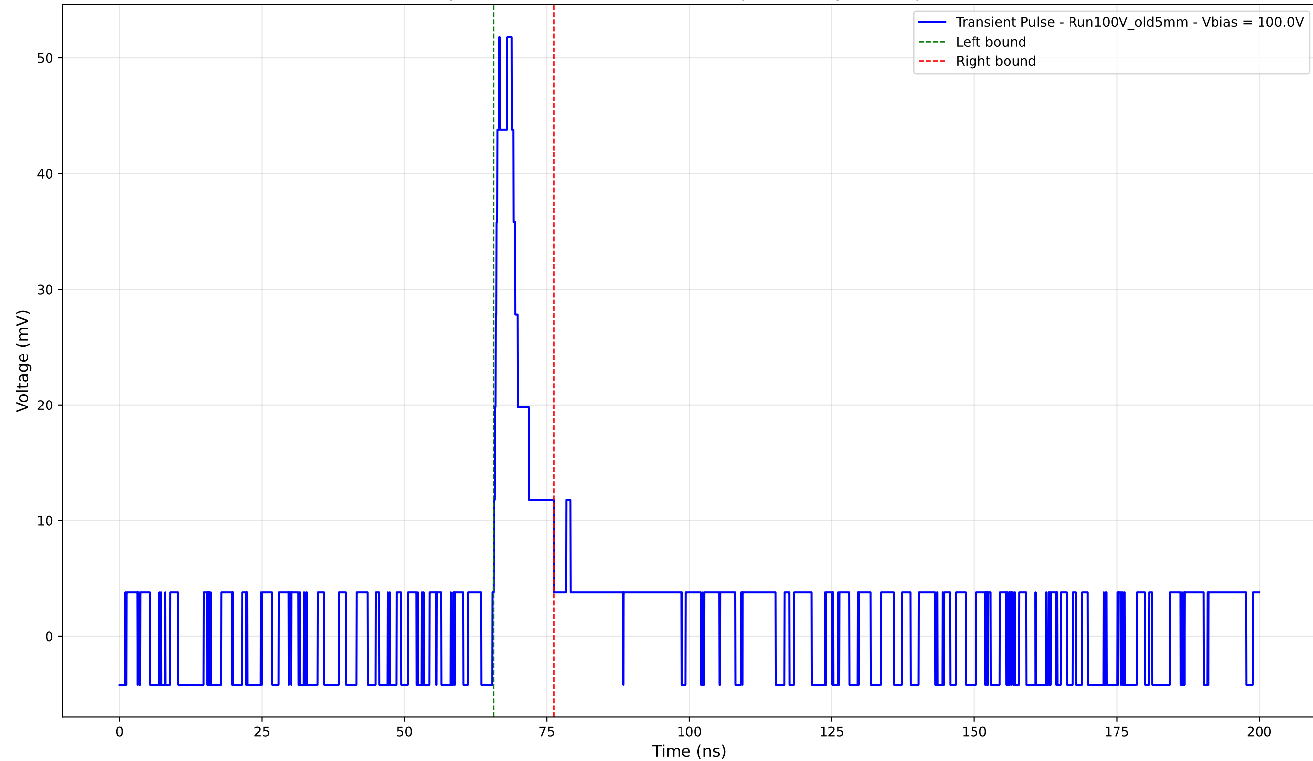
Transient Pulse - Sample: Old5mm - Position: 3955.0 \mu\text{m} - Charge: 5.17 pC - Rise Time: 0.94 ns
