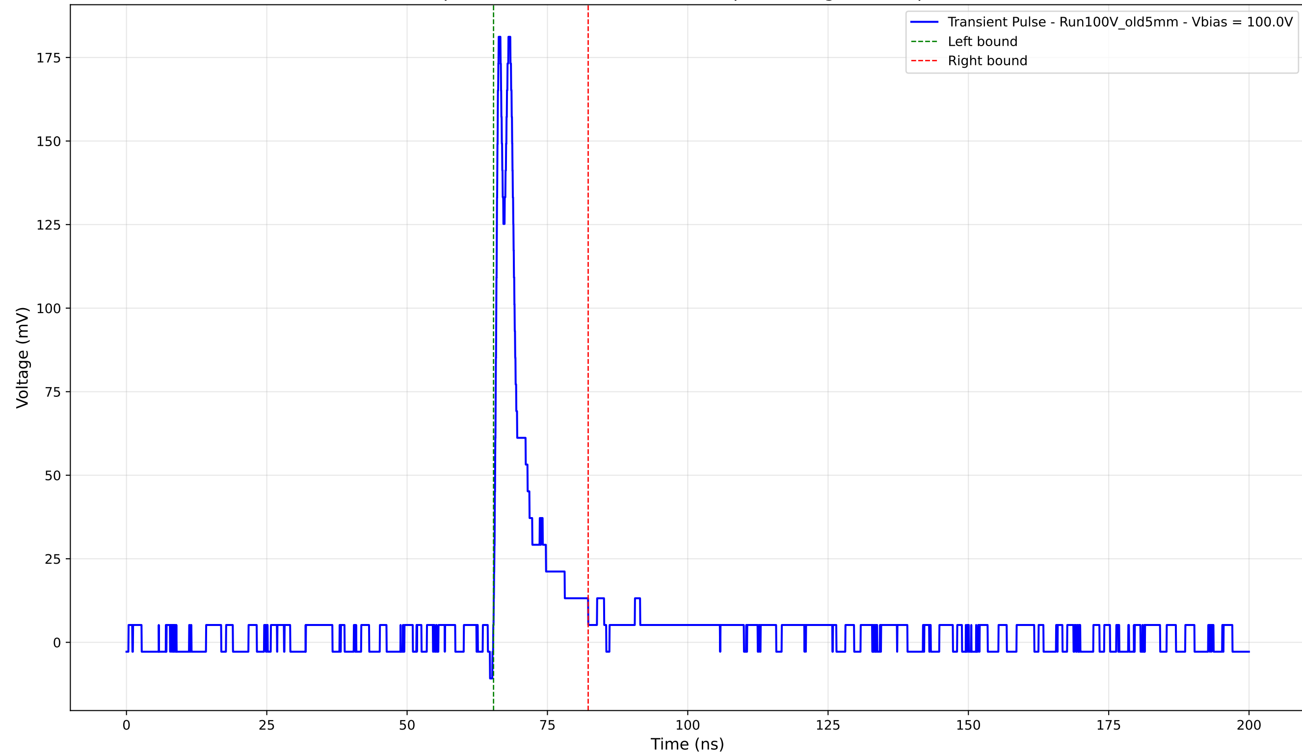
Transient Pulse - Sample: Old5mm - Position: 3810.0 \mu\text{m} - Charge: 18.04 pC - Rise Time: 0.71 ns
