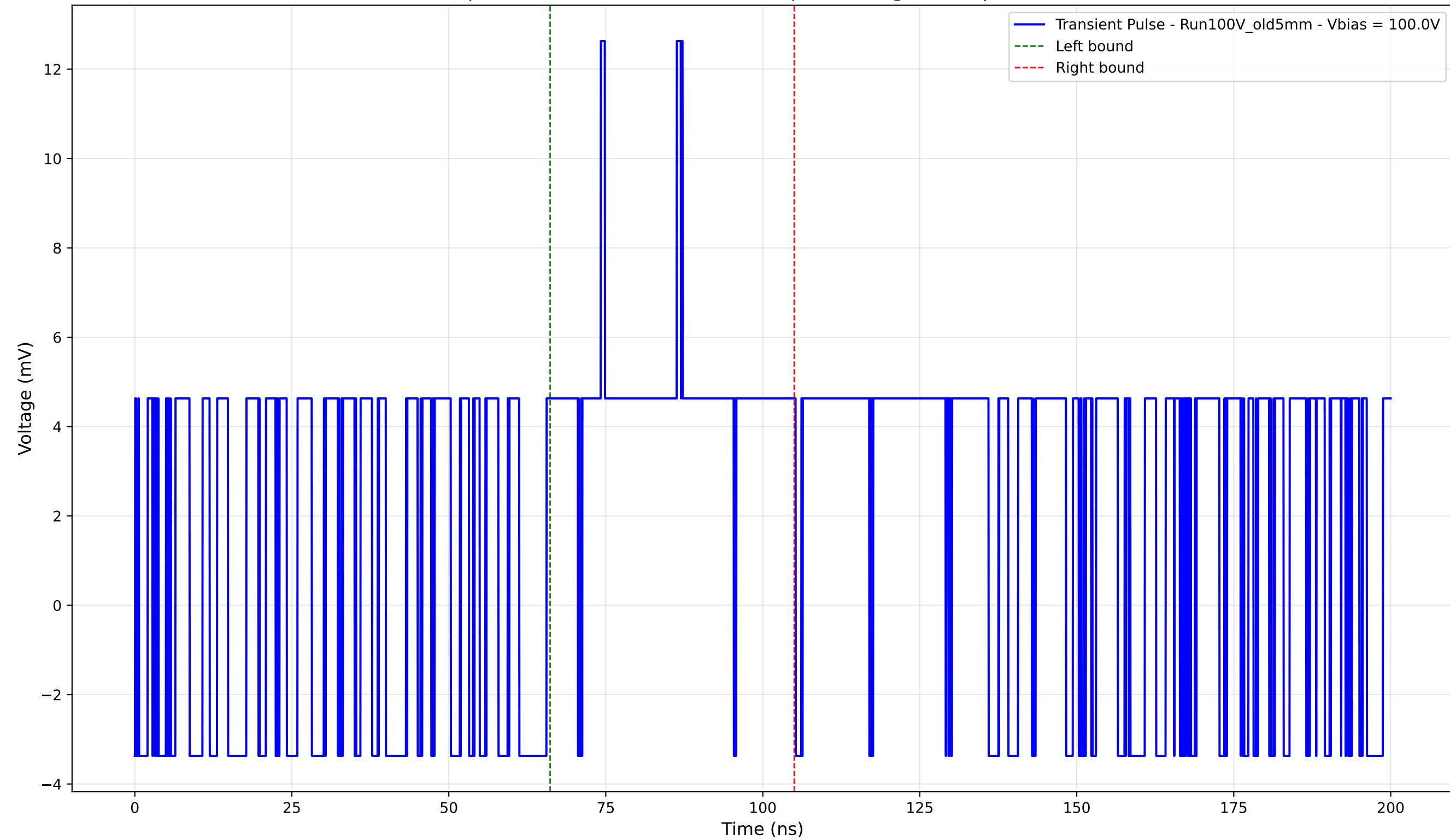
Transient Pulse - Sample: Old5mm - Position: 1340.0 \mu\text{m} - Charge: 3.73 pC - Rise Time: 0.00 ns (N/A)
