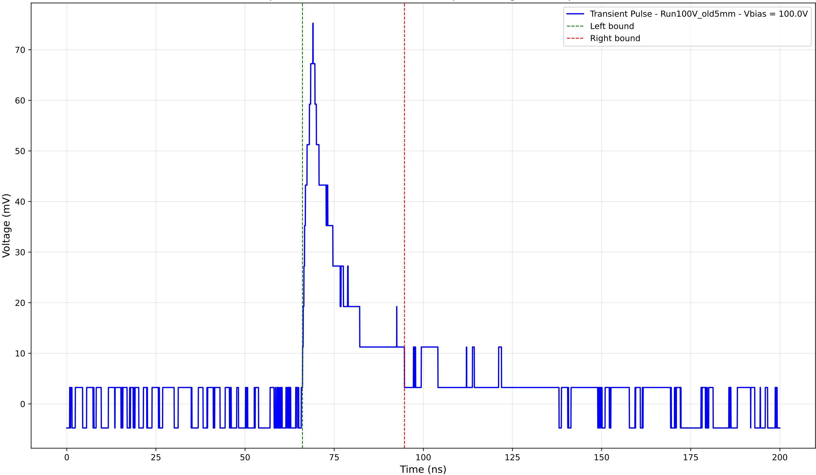
Transient Pulse - Sample: Old5mm - Position: 2985.0 \mu\text{m} - Charge: 14.03 pC - Rise Time: 2.91 ns
