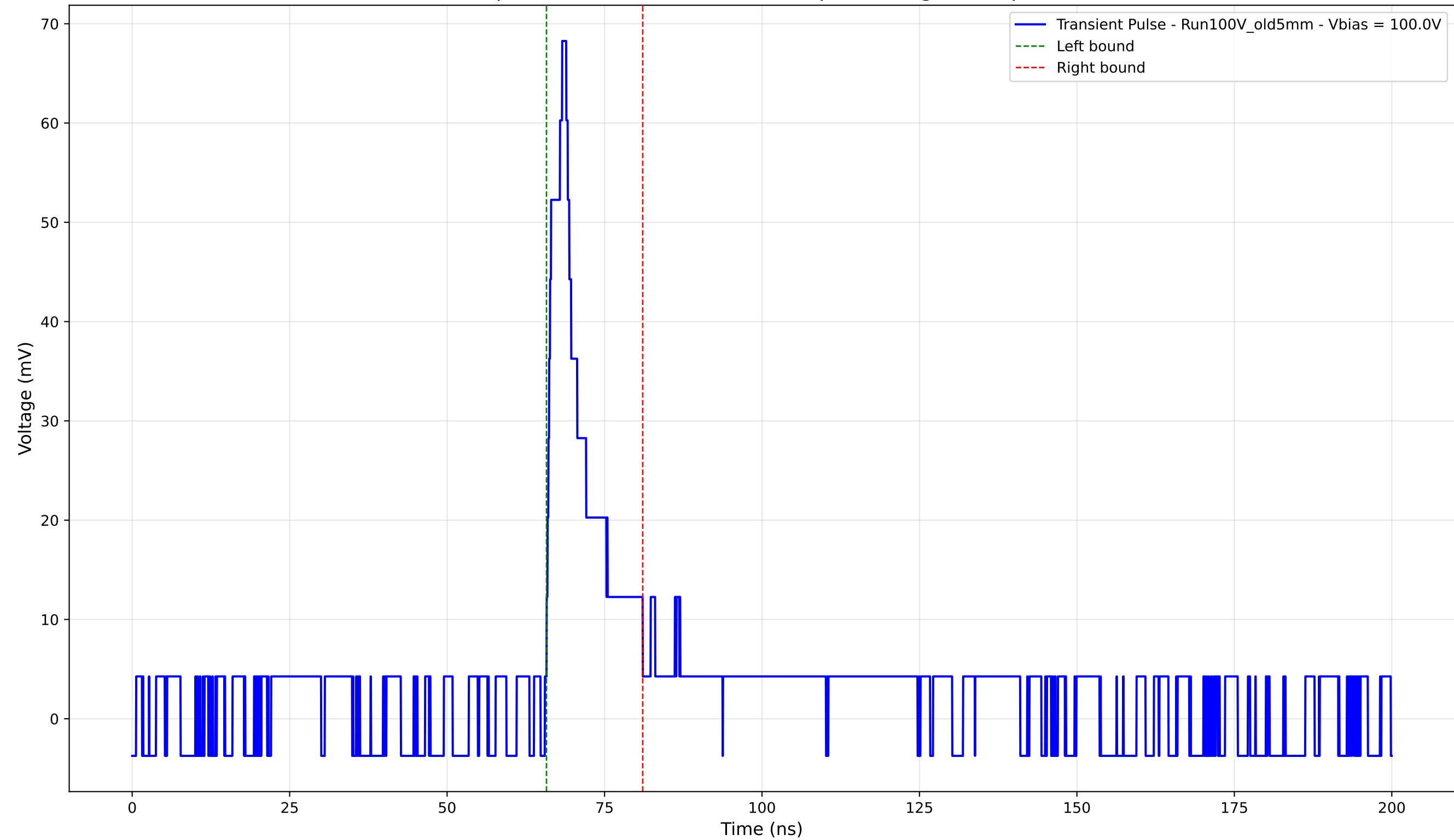
Transient Pulse - Sample: Old5mm - Position: 4080.0 \mu\text{m} - Charge: 8.24 pC - Rise Time: 2.47 ns
