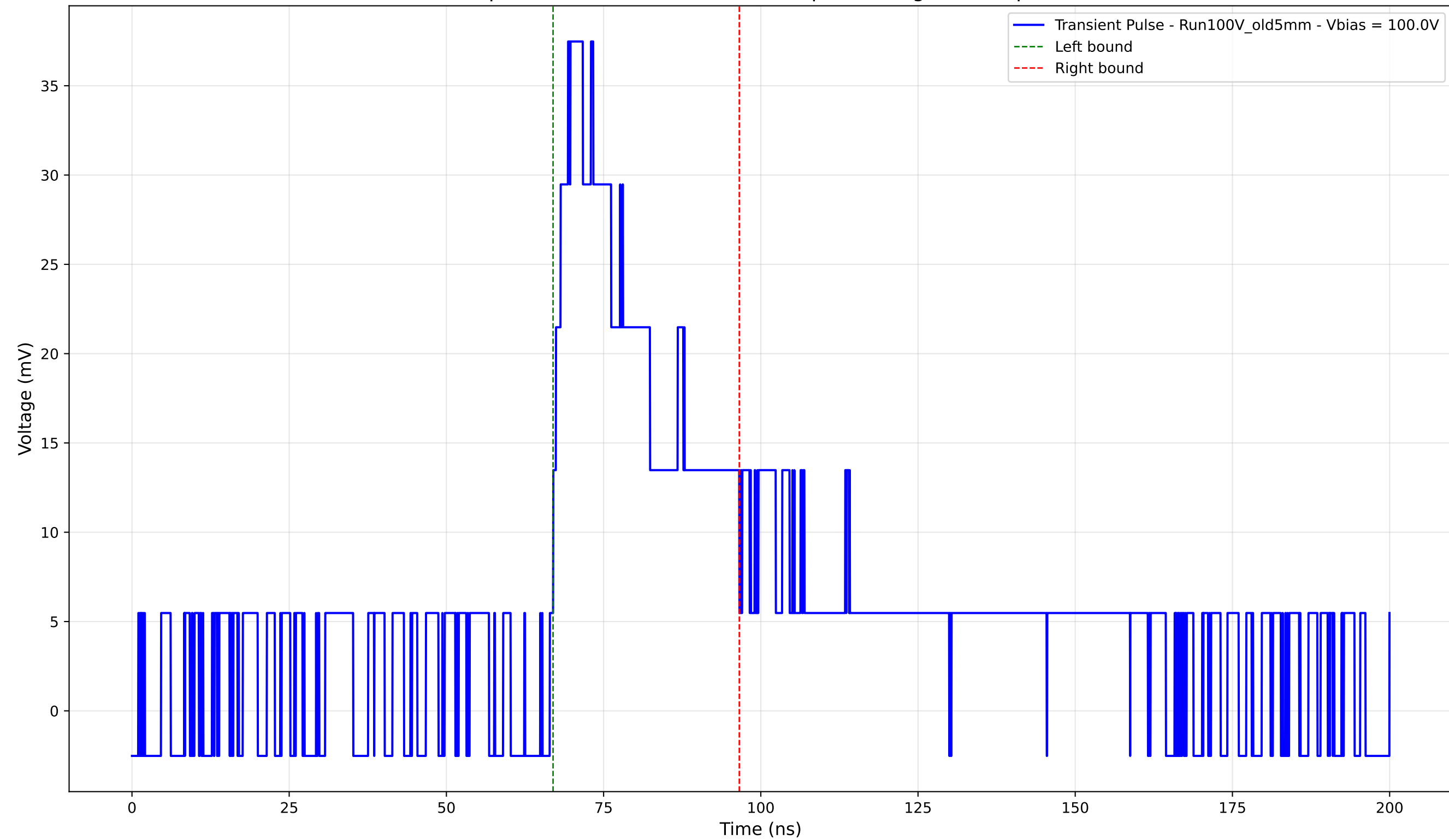
Transient Pulse - Sample: Old5mm - Position: 2605.0 \mu\text{m} - Charge: 12.25 pC - Rise Time: 2.91 ns
