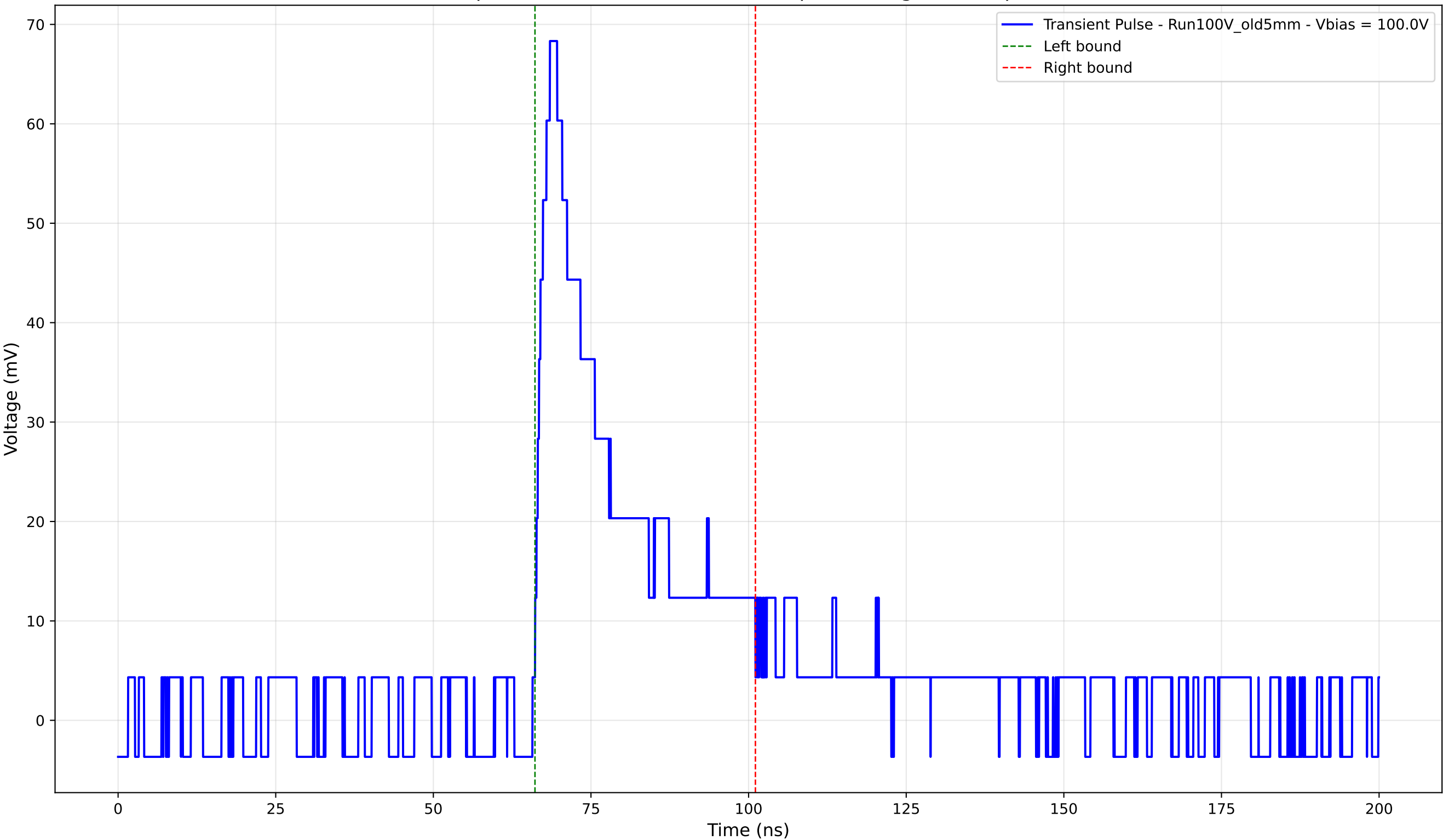
Transient Pulse - Sample: Old5mm - Position: 2955.0 \mu\text{m} - Charge: 17.34 pC - Rise Time: 2.35 ns
