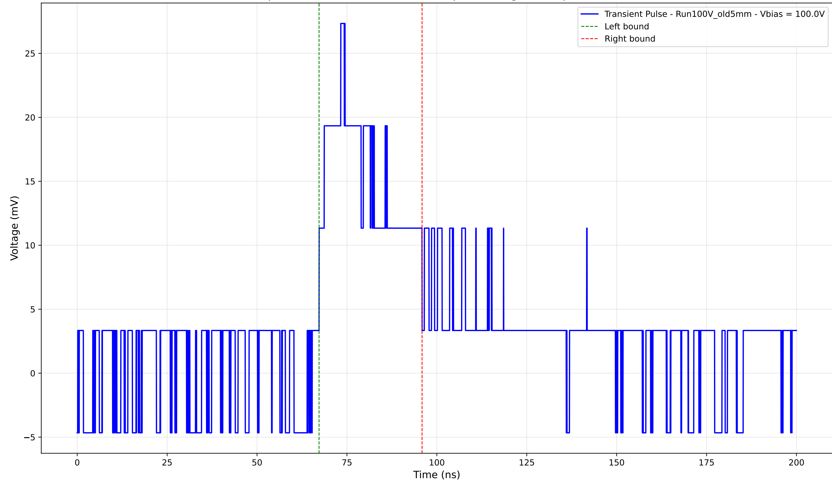
Transient Pulse - Sample: Old5mm - Position: 2385.0 \mu\text{m} - Charge: 8.81 pC - Rise Time: 0.00 ns (N/A)
