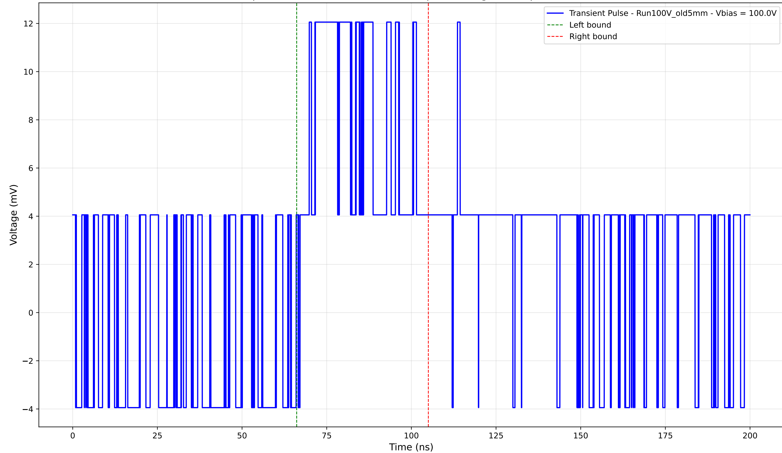
Transient Pulse - Sample: Old5mm - Position: 1870.0 \mu\text{m} - Charge: 6.03 pC - Rise Time: 0.00 ns (N/A)
