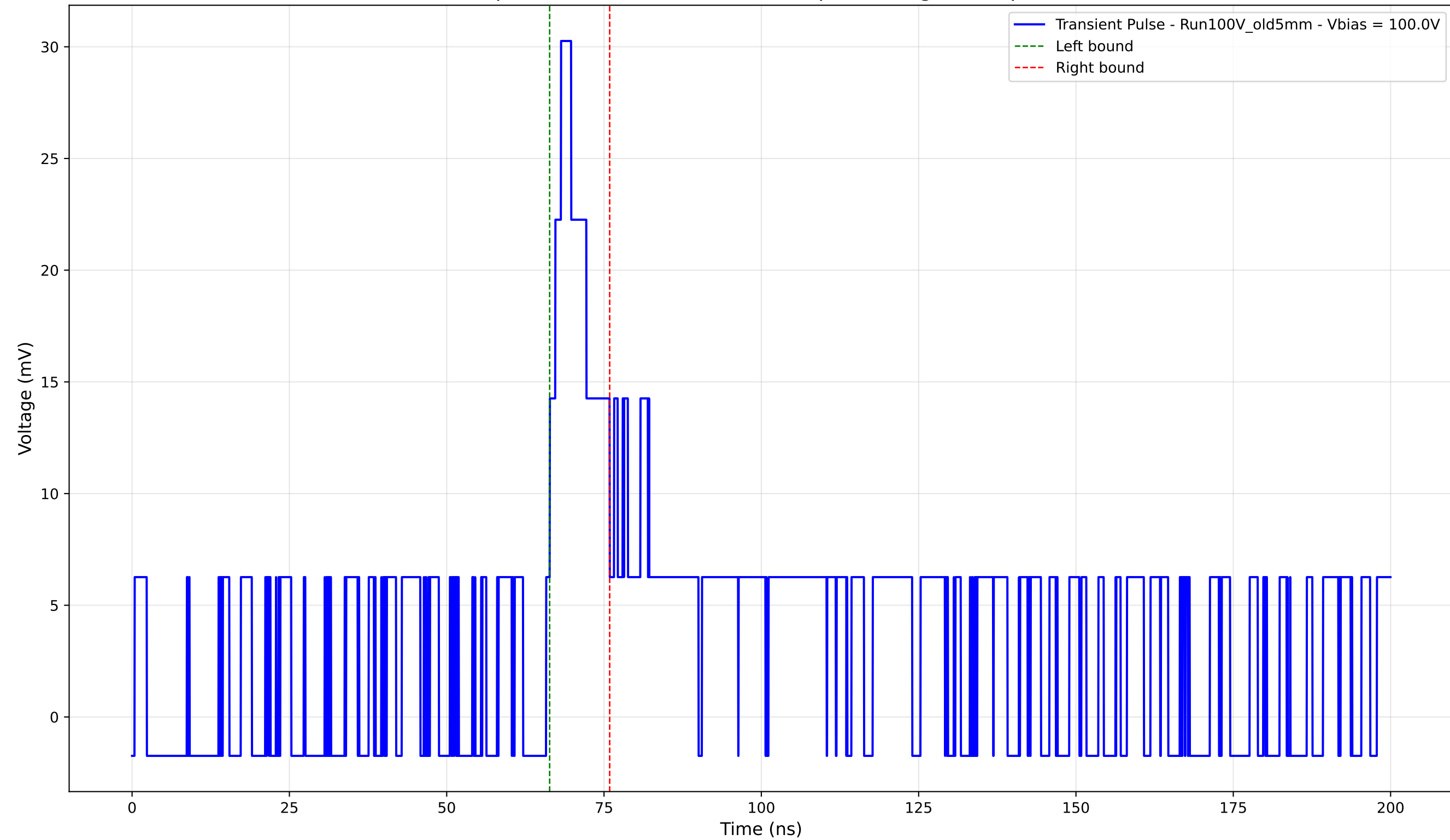
Transient Pulse - Sample: Old5mm - Position: 3045.0 \mu\text{m} - Charge: 3.77 pC - Rise Time: 2.37 ns
