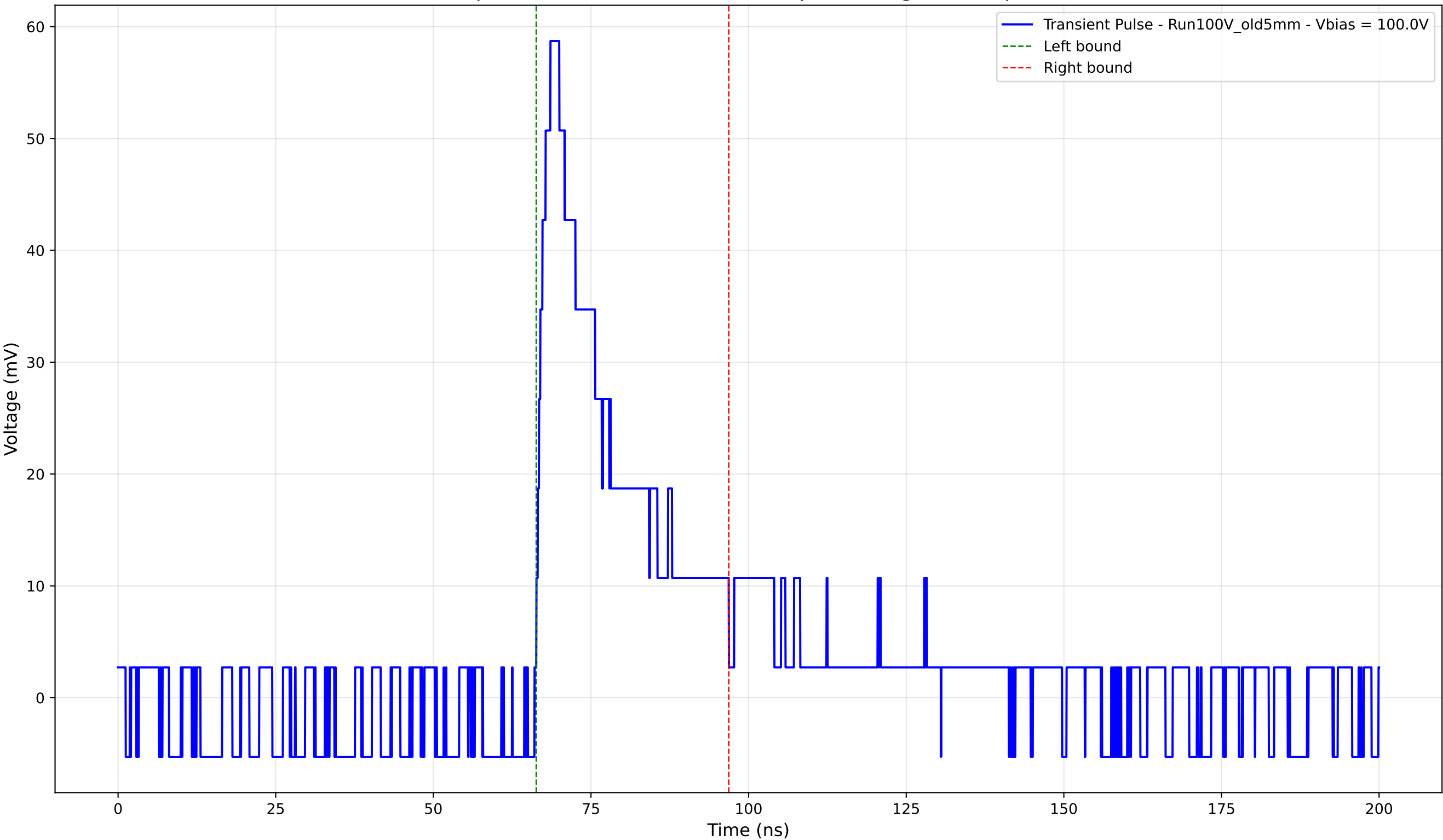
Transient Pulse - Sample: Old5mm - Position: 2920.0 \mu\text{m} - Charge: 14.38 pC - Rise Time: 2.23 ns
