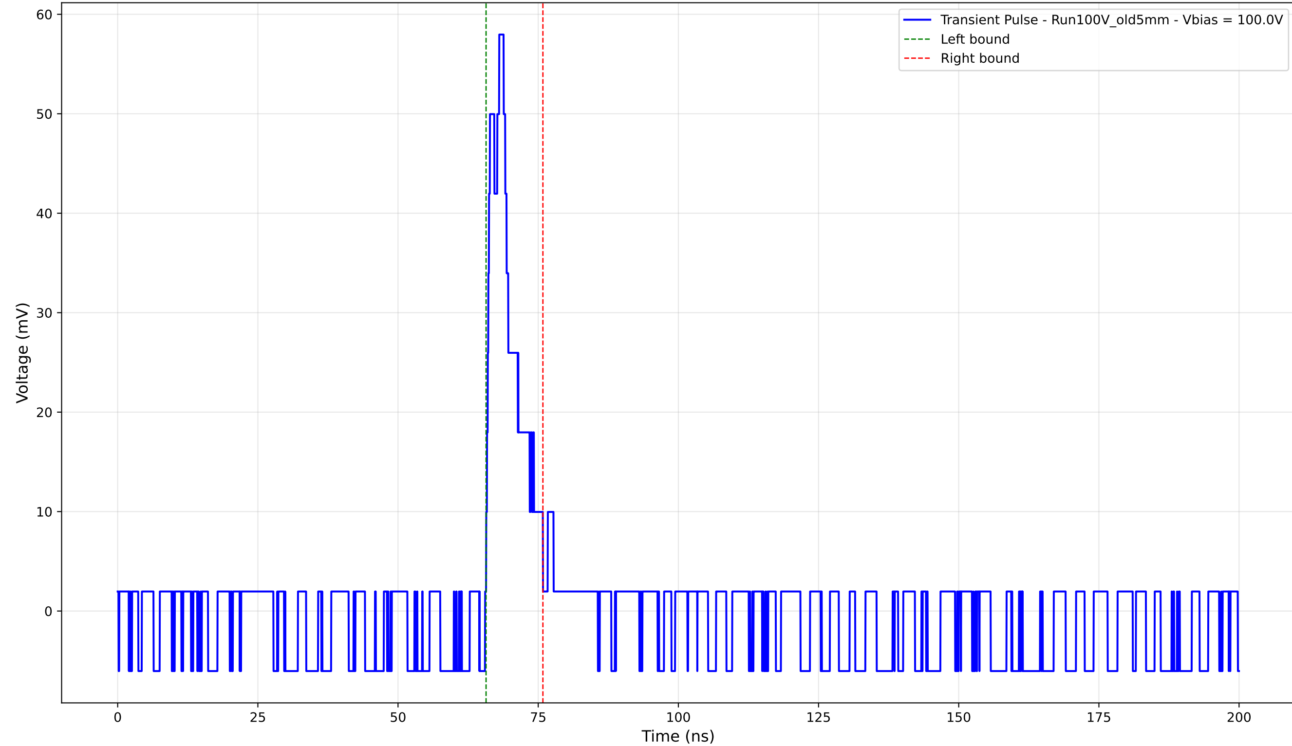
Transient Pulse - Sample: Old5mm - Position: 3465.0 \mu\text{m} - Charge: 5.72 pC - Rise Time: 2.33 ns
