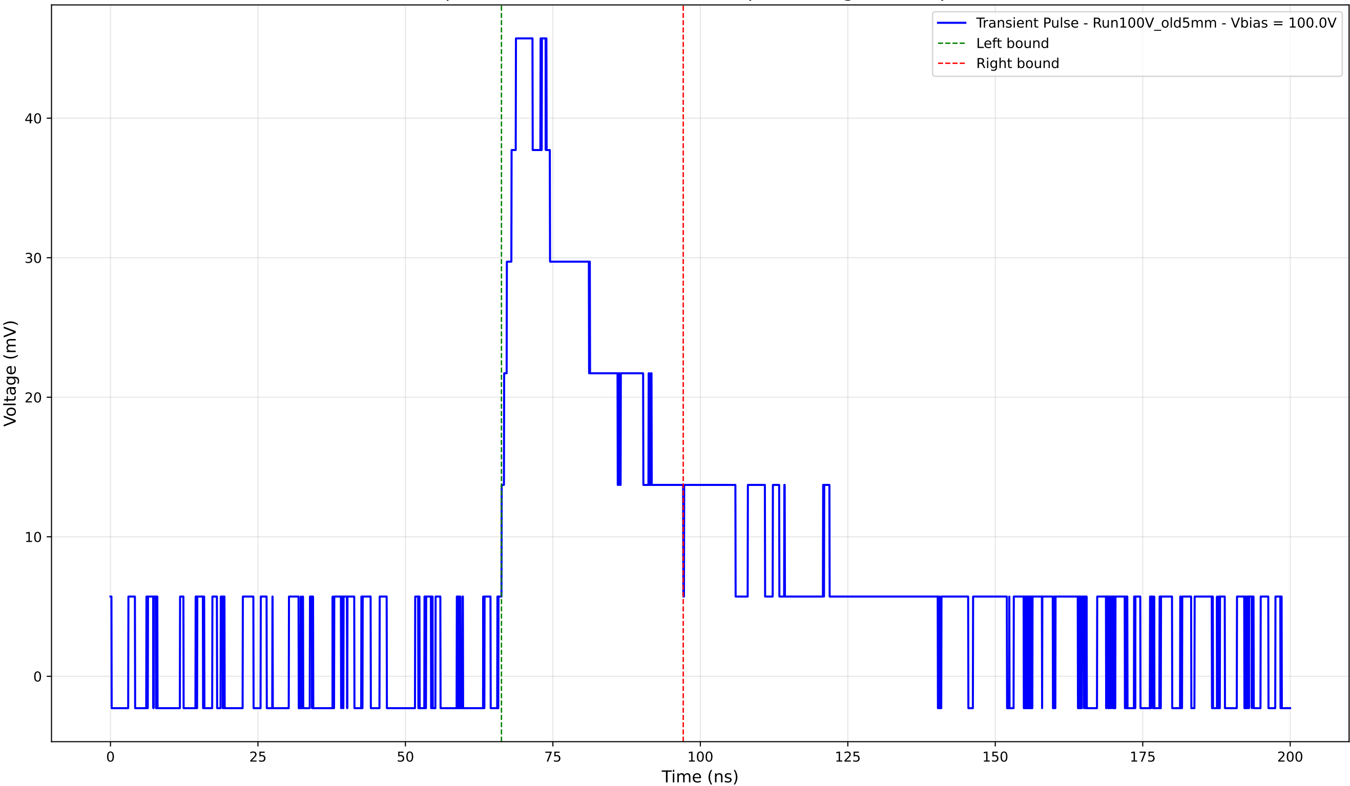
Transient Pulse - Sample: Old5mm - Position: 4790.0 \mu\text{m} - Charge: 16.11 pC - Rise Time: 2.97 ns
