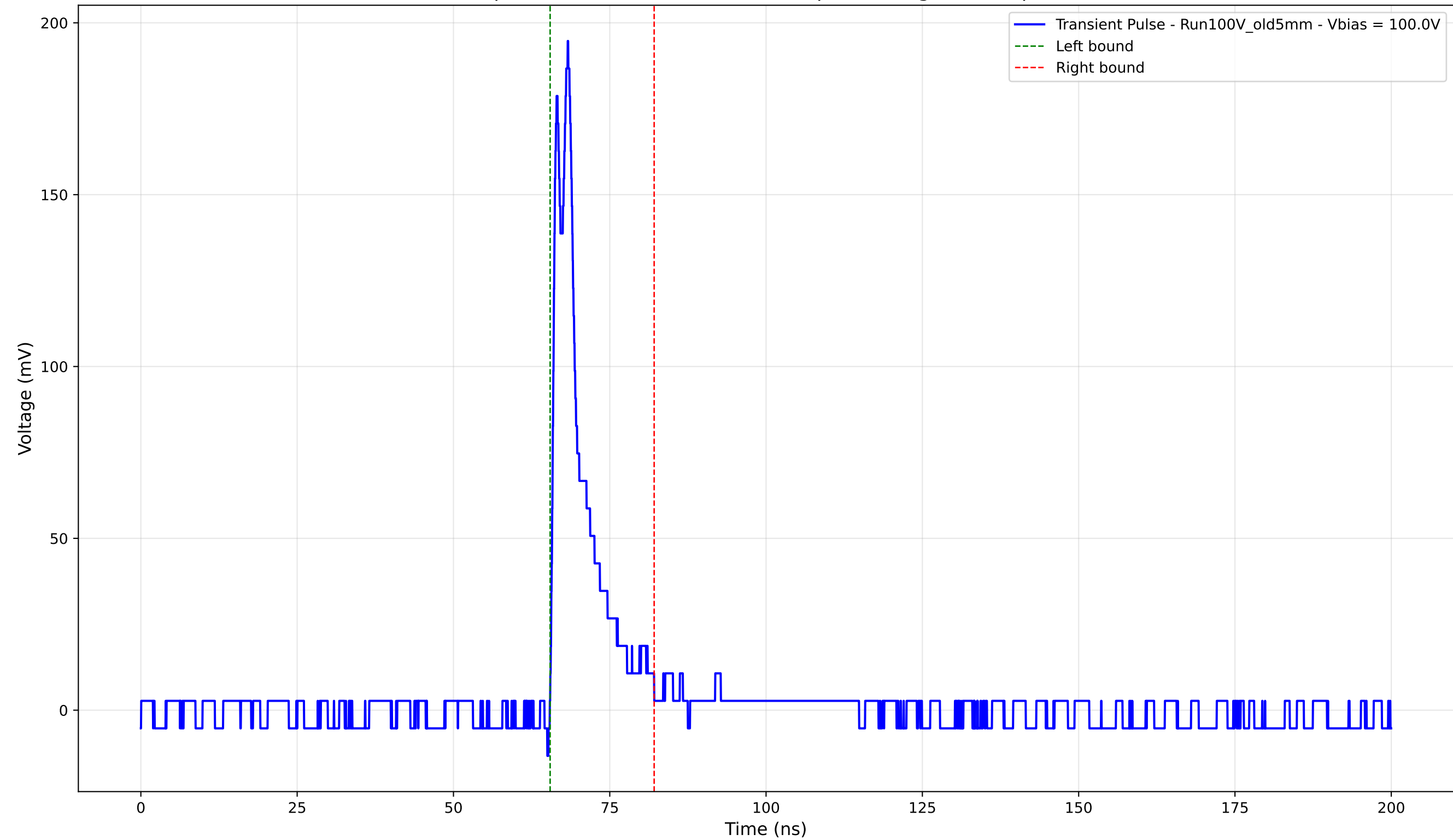
Transient Pulse - Sample: Old5mm - Position: 3870.0 \mu\text{m} - Charge: 19.37 pC - Rise Time: 0.88 ns
