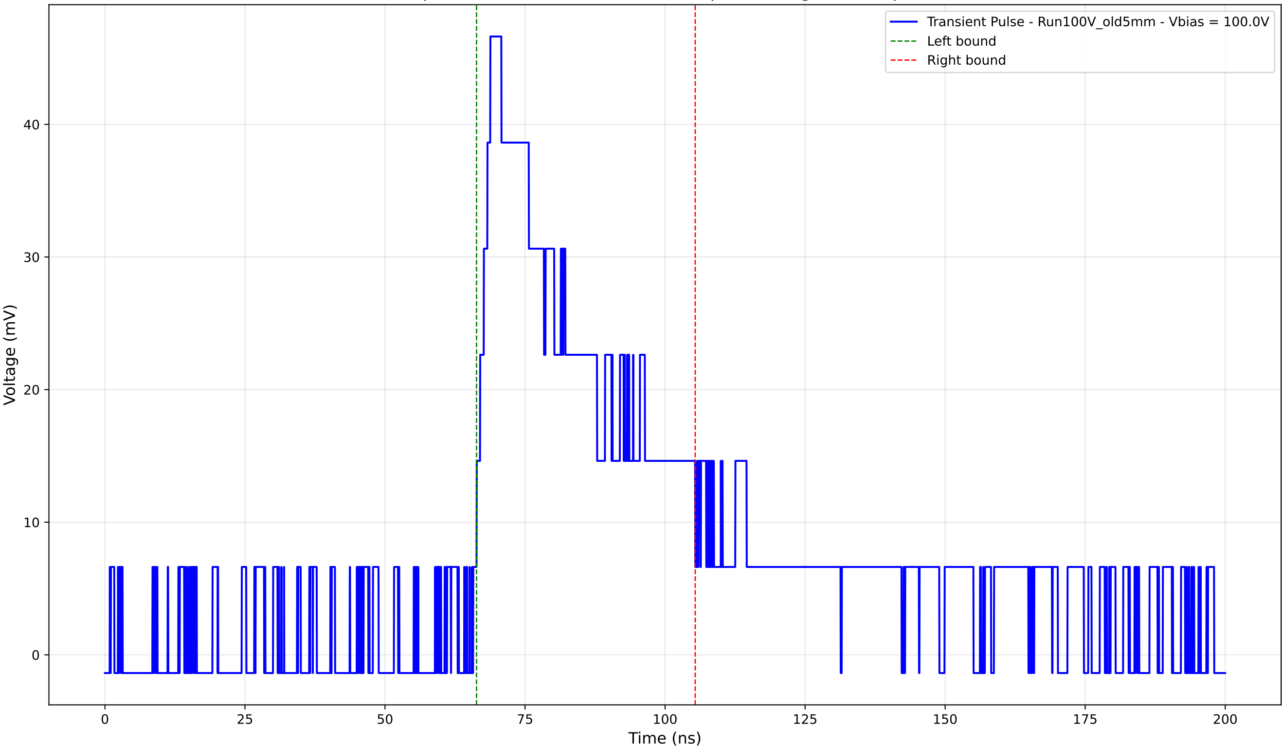
Transient Pulse - Sample: Old5mm - Position: 4820.0 \mu\text{m} - Charge: 18.85 pC - Rise Time: 3.07 ns
