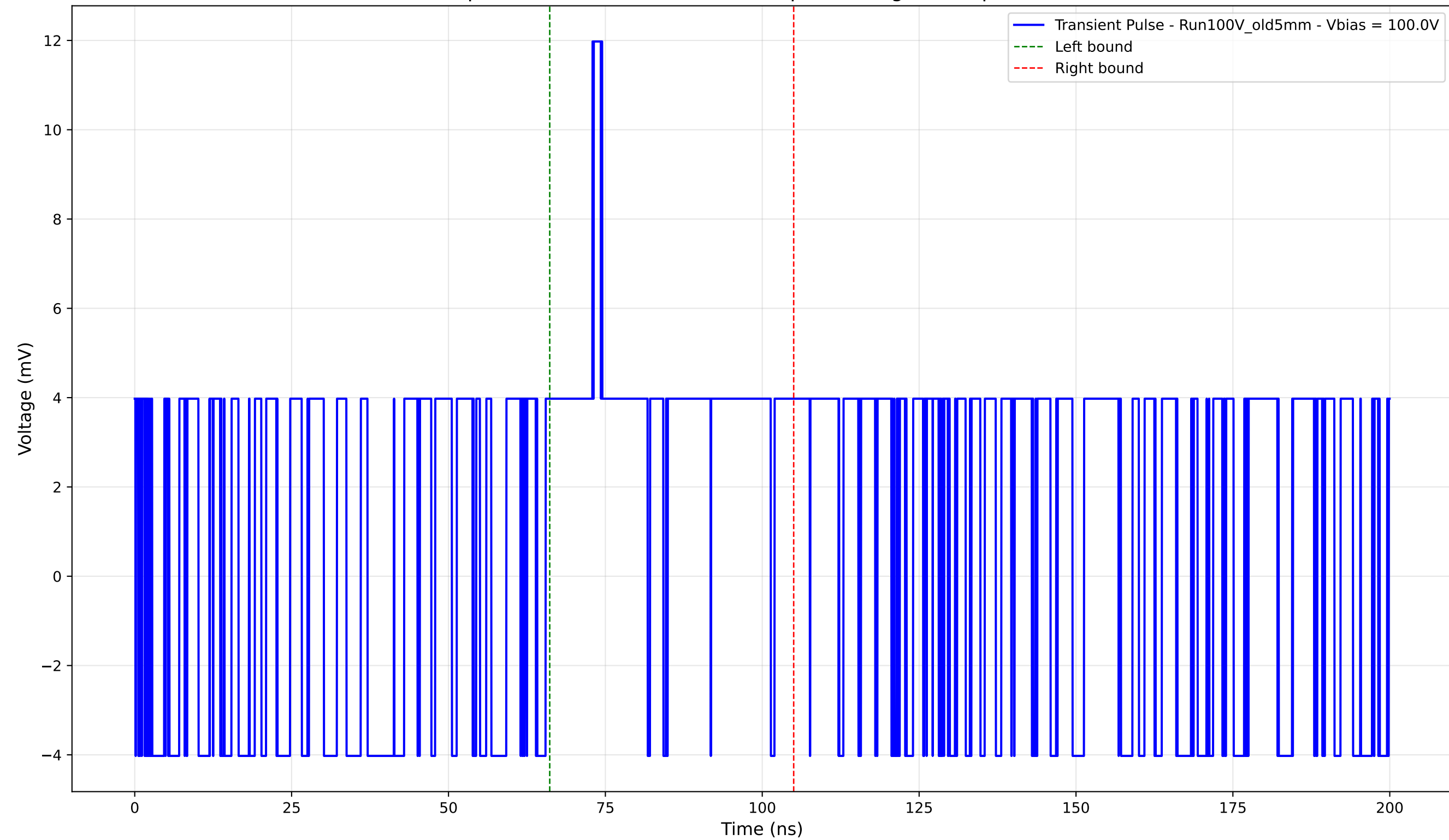
Transient Pulse - Sample: Old5mm - Position: 2135.0 \mu\text{m} - Charge: 3.07 pC - Rise Time: 0.00 ns (N/A)
