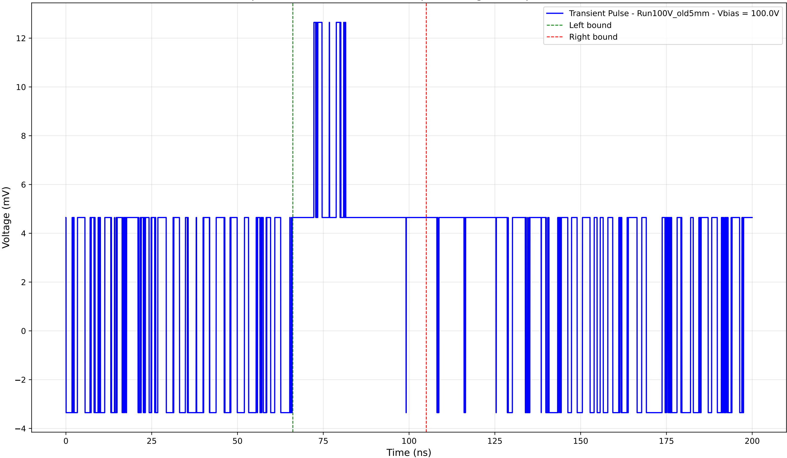
Transient Pulse - Sample: Old5mm - Position: 415.0 \mu\text{m} - Charge: 4.18 pC - Rise Time: 0.00 ns (N/A)
