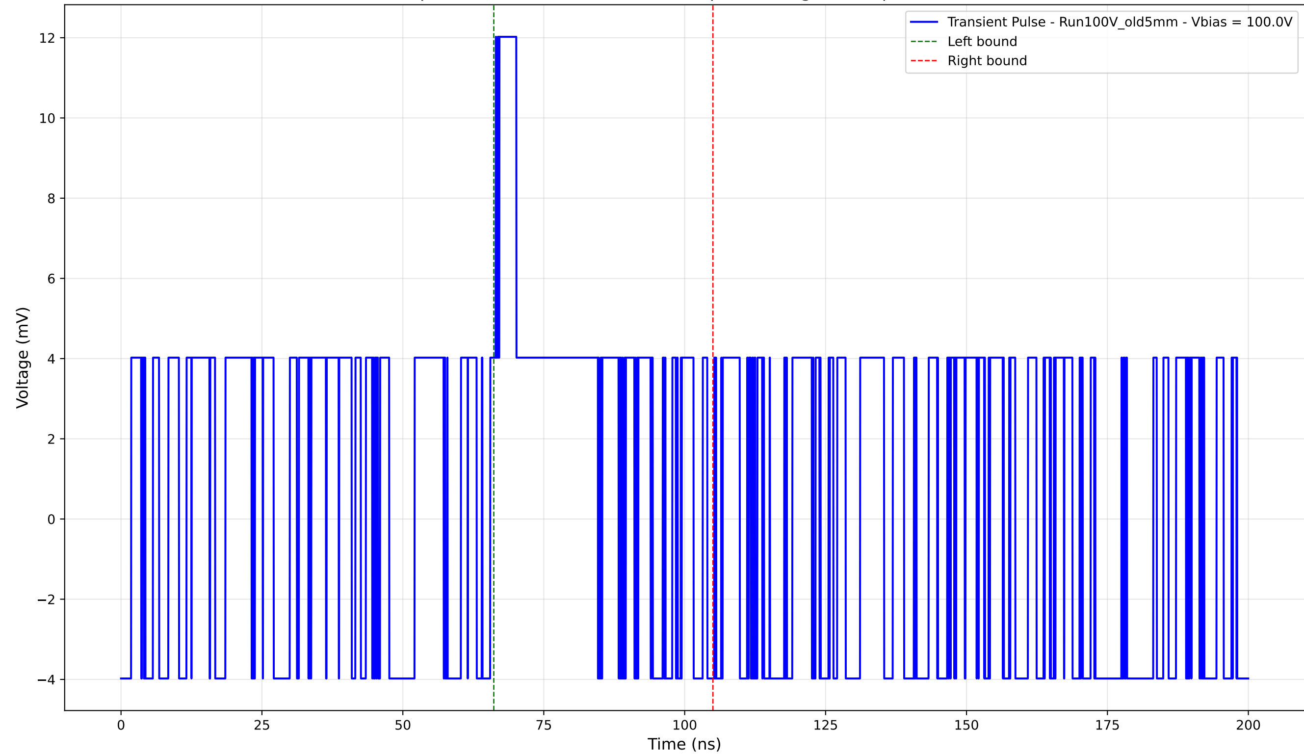
Transient Pulse - Sample: Old5mm - Position: 3135.0 \mu\text{m} - Charge: 2.29 pC - Rise Time: 0.00 ns (N/A)
