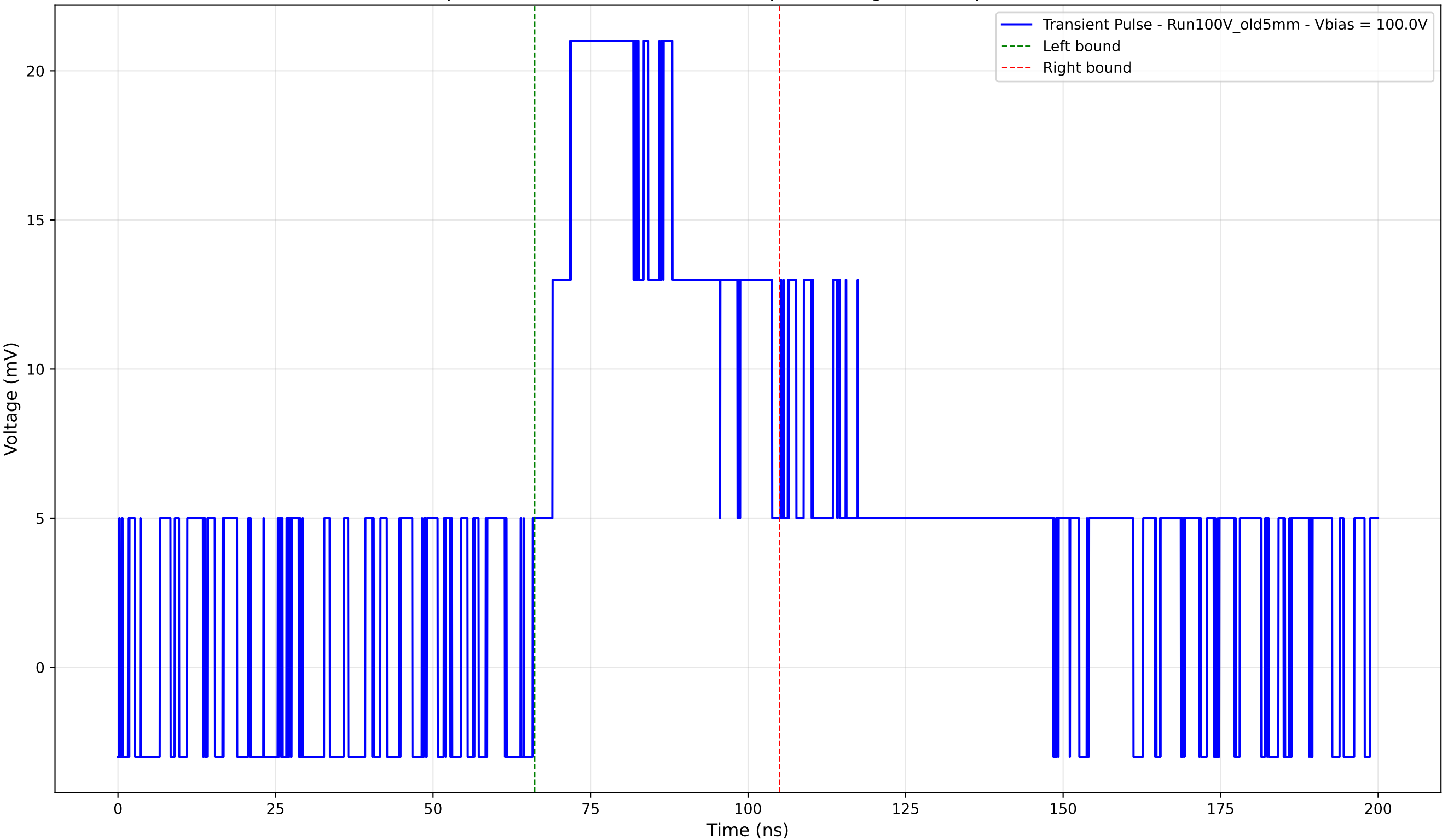
Transient Pulse - Sample: Old5mm - Position: 1815.0 \mu\text{m} - Charge: 11.47 pC - Rise Time: 0.00 ns (N/A)
