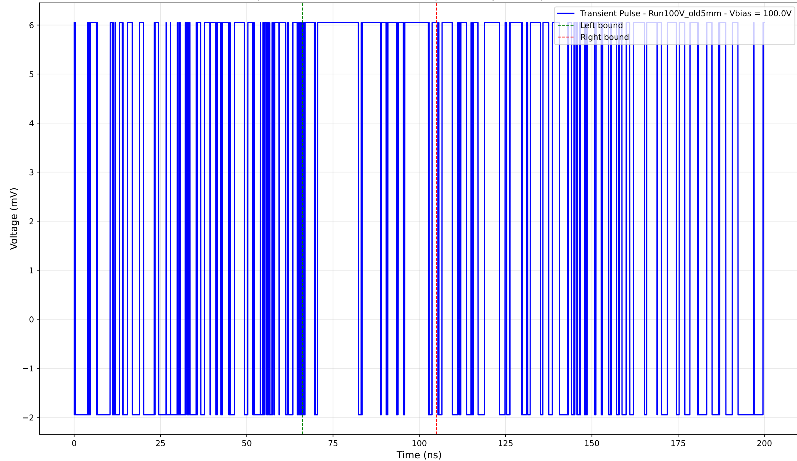
Transient Pulse - Sample: Old5mm - Position: 1695.0 \mu\text{m} - Charge: 3.99 pC - Rise Time: 0.00 ns (N/A)
