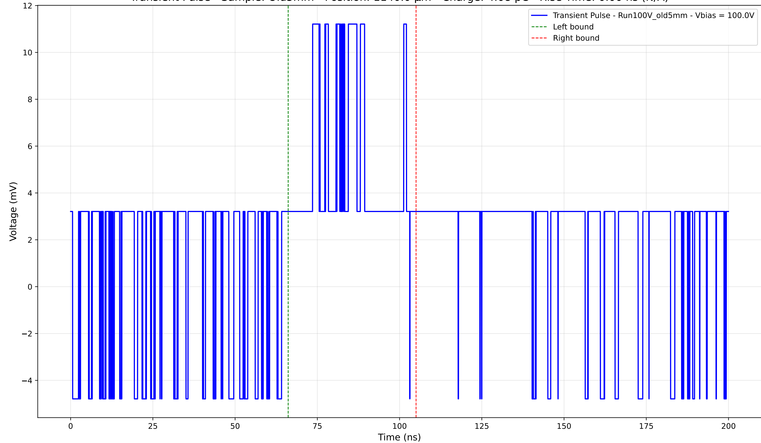
Transient Pulse - Sample: Old5mm - Position: 1140.0 \mu\text{m} - Charge: 4.08 pC - Rise Time: 0.00 ns (N/A)
