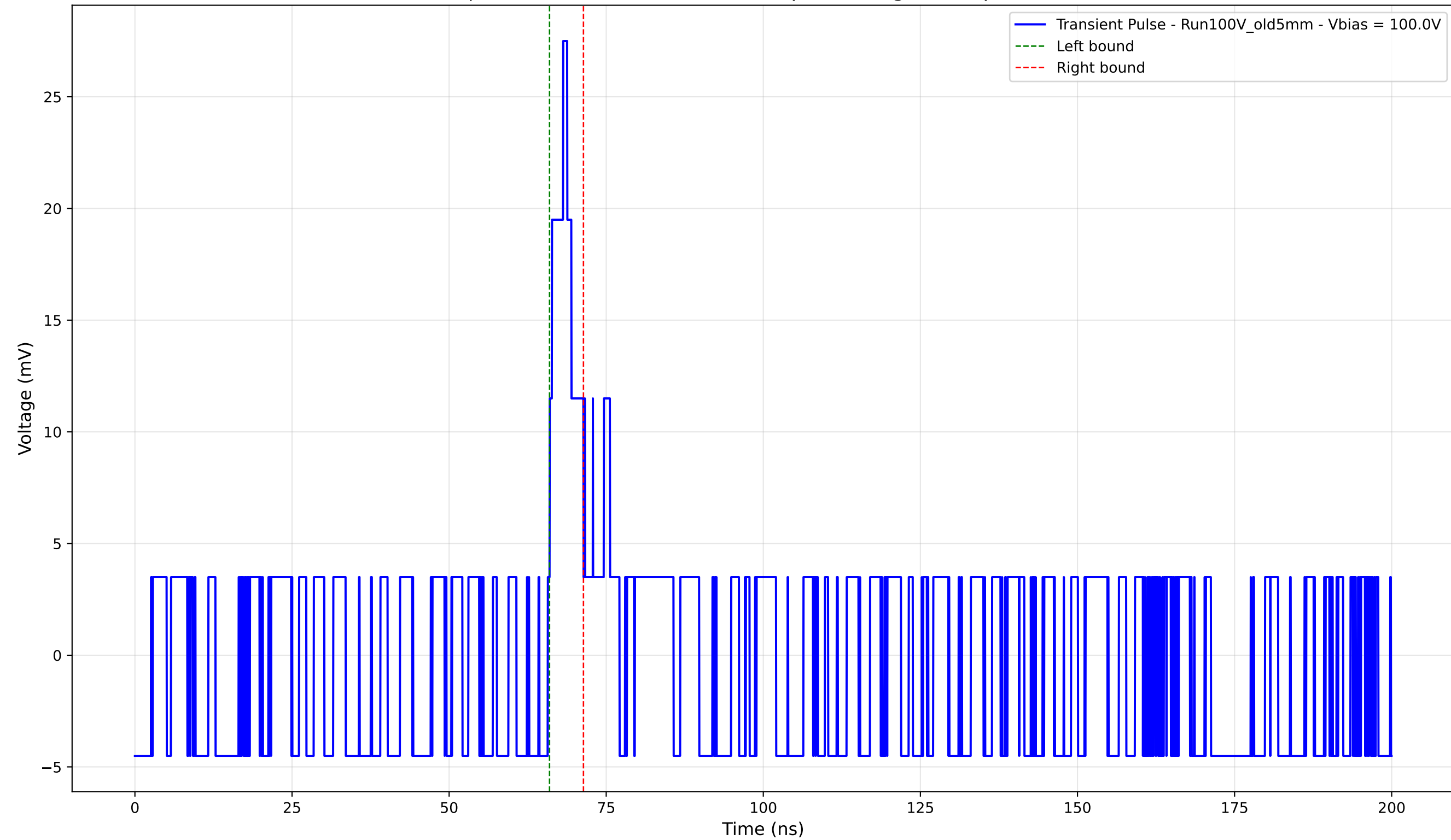
Transient Pulse - Sample: Old5mm - Position: 3445.0 \mu\text{m} - Charge: 1.84 pC - Rise Time: 0.00 ns (N/A)
