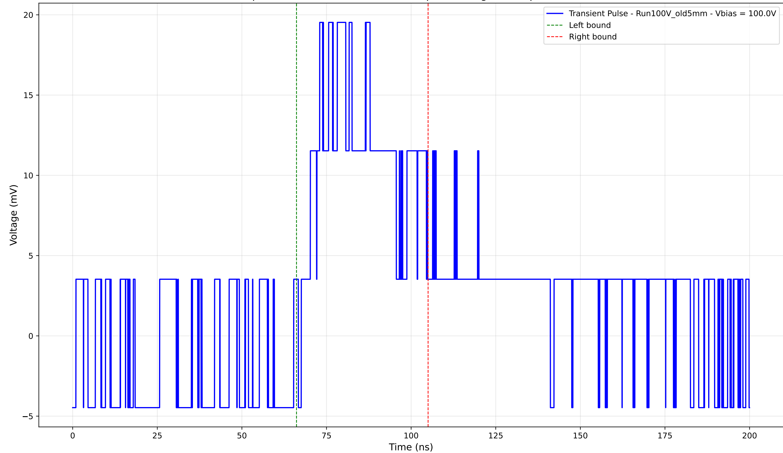
Transient Pulse - Sample: Old5mm - Position: 1420.0 \mu\text{m} - Charge: 8.74 pC - Rise Time: 0.00 ns (N/A)
