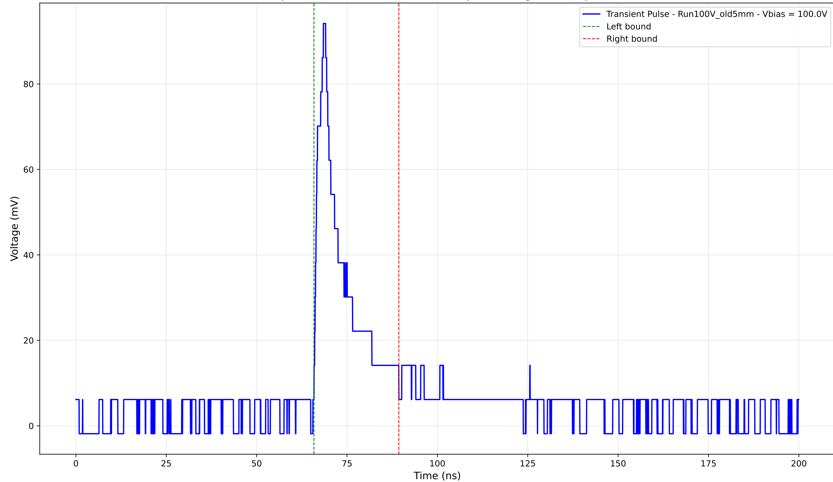
Transient Pulse - Sample: Old5mm - Position: 3200.0 \mu\text{m} - Charge: 15.65 pC - Rise Time: 2.27 ns
