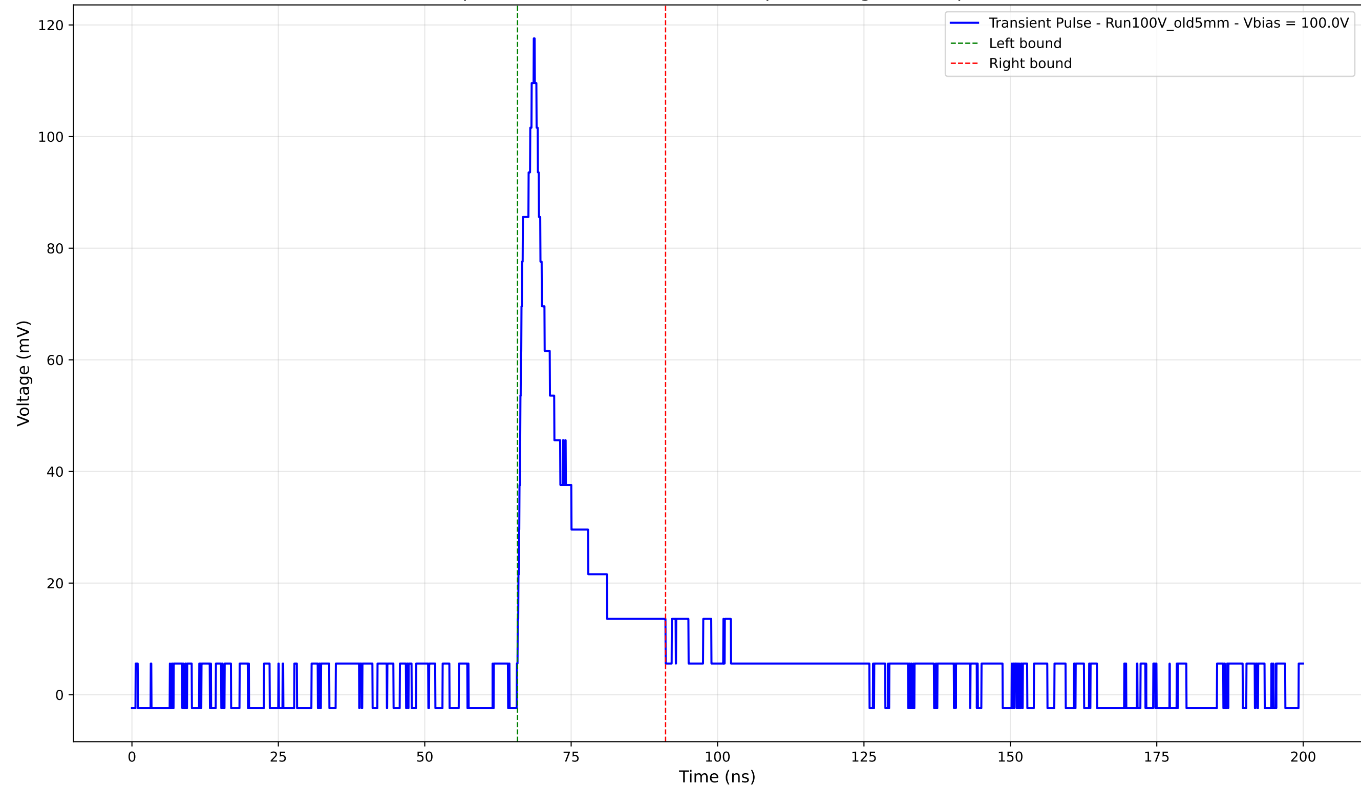
Transient Pulse - Sample: Old5mm - Position: 4175.0 \mu\text{m} - Charge: 17.77 pC - Rise Time: 2.38 ns
