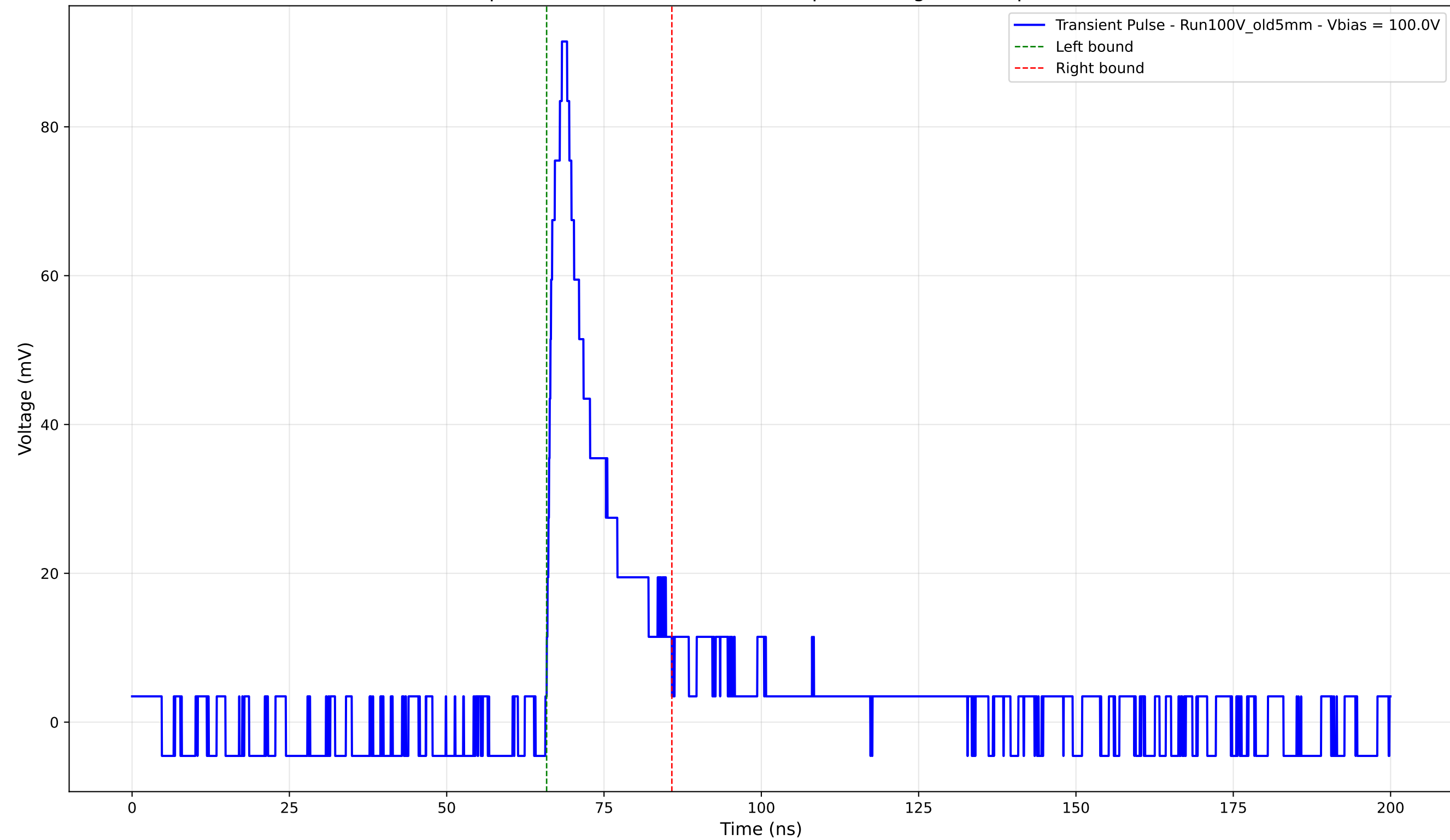
Transient Pulse - Sample: Old5mm - Position: 3205.0 \mu\text{m} - Charge: 14.40 pC - Rise Time: 2.09 ns
