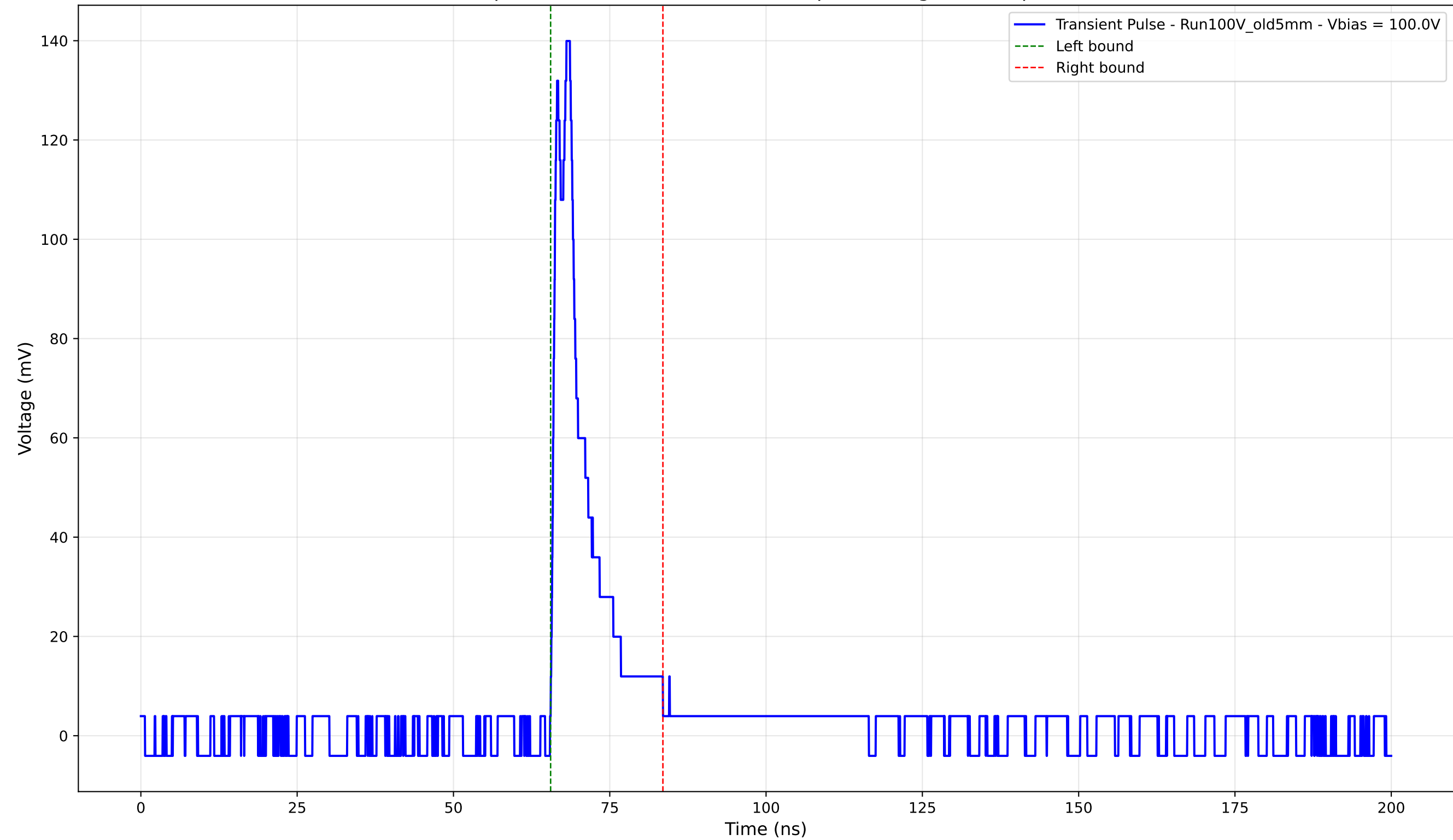
Transient Pulse - Sample: Old5mm - Position: 3915.0 \mu\text{m} - Charge: 15.68 pC - Rise Time: 0.93 ns
