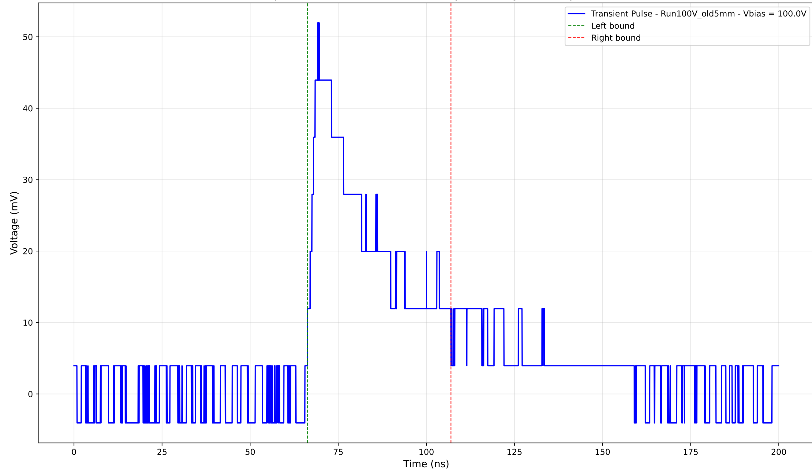
Transient Pulse - Sample: Old5mm - Position: 4825.0 \mu\text{m} - Charge: 18.39 pC - Rise Time: 2.88 ns
