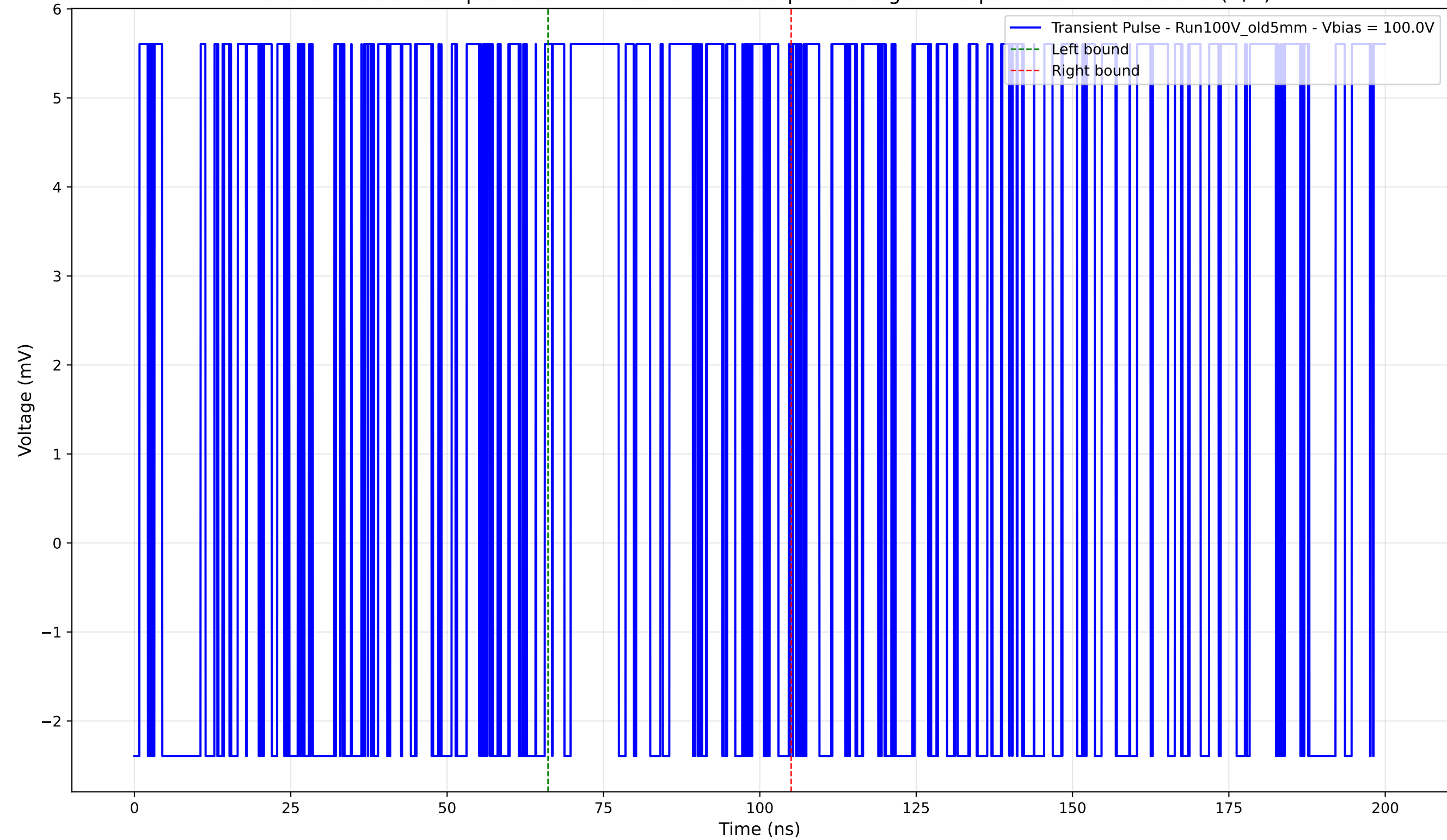
Transient Pulse - Sample: Old5mm - Position: 4605.0 \mu\text{m} - Charge: 2.49 pC - Rise Time: 0.00 ns (N/A)
