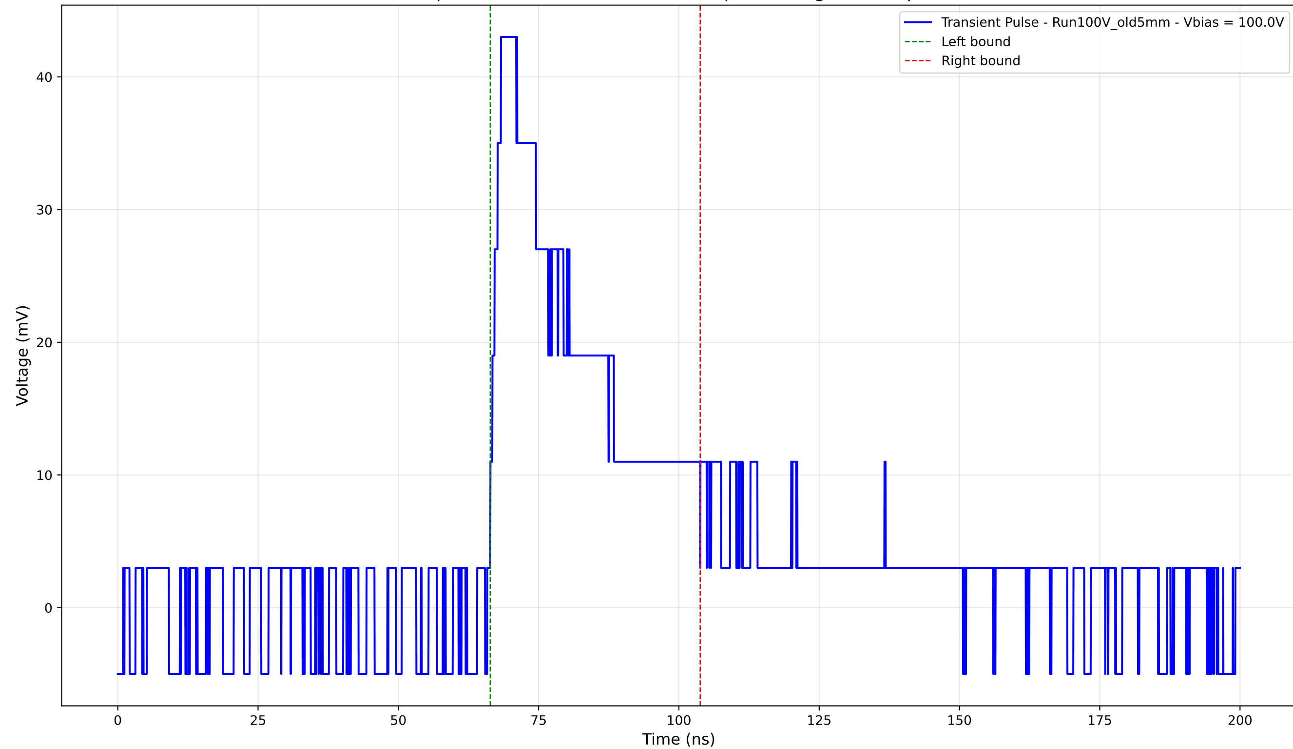
Transient Pulse - Sample: Old5mm - Position: 4750.0 \mu\text{m} - Charge: 15.13 pC - Rise Time: 1.90 ns
