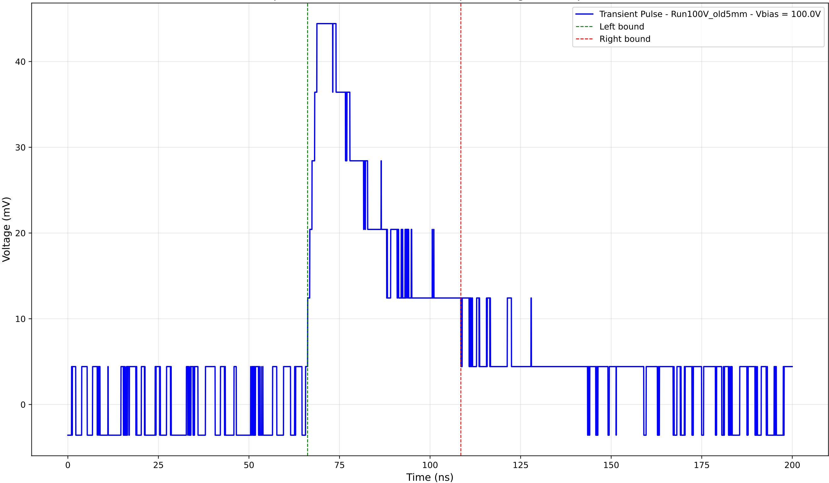
Transient Pulse - Sample: Old5mm - Position: 4855.0 \mu\text{m} - Charge: 19.23 pC - Rise Time: 2.56 ns
