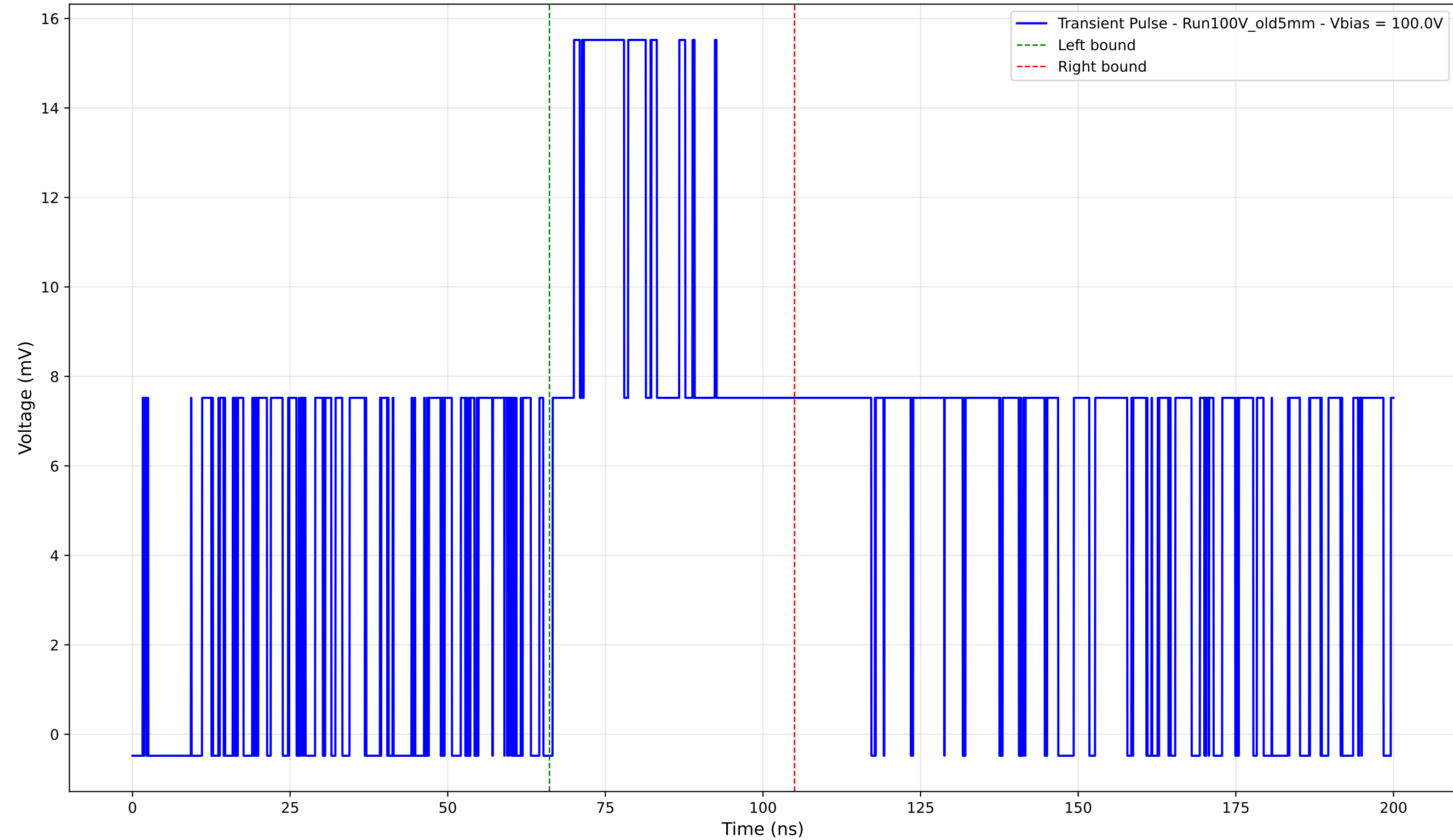
Transient Pulse - Sample: Old5mm - Position: 685.0 \mu\text{m} - Charge: 7.80 pC - Rise Time: 3.40 ns
