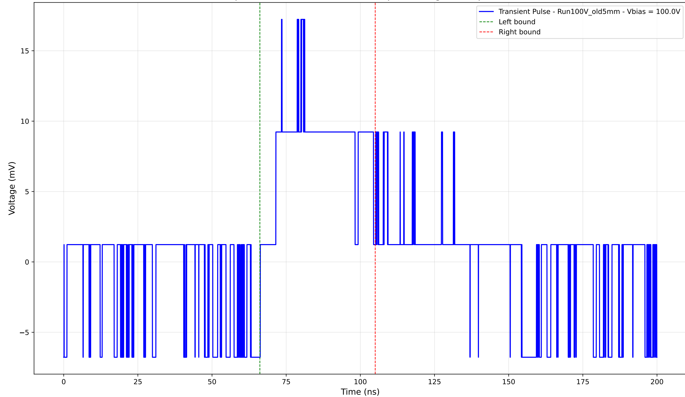
Transient Pulse - Sample: Old5mm - Position: 1390.0 \mu\text{m} - Charge: 6.28 pC - Rise Time: 1.92 ns
