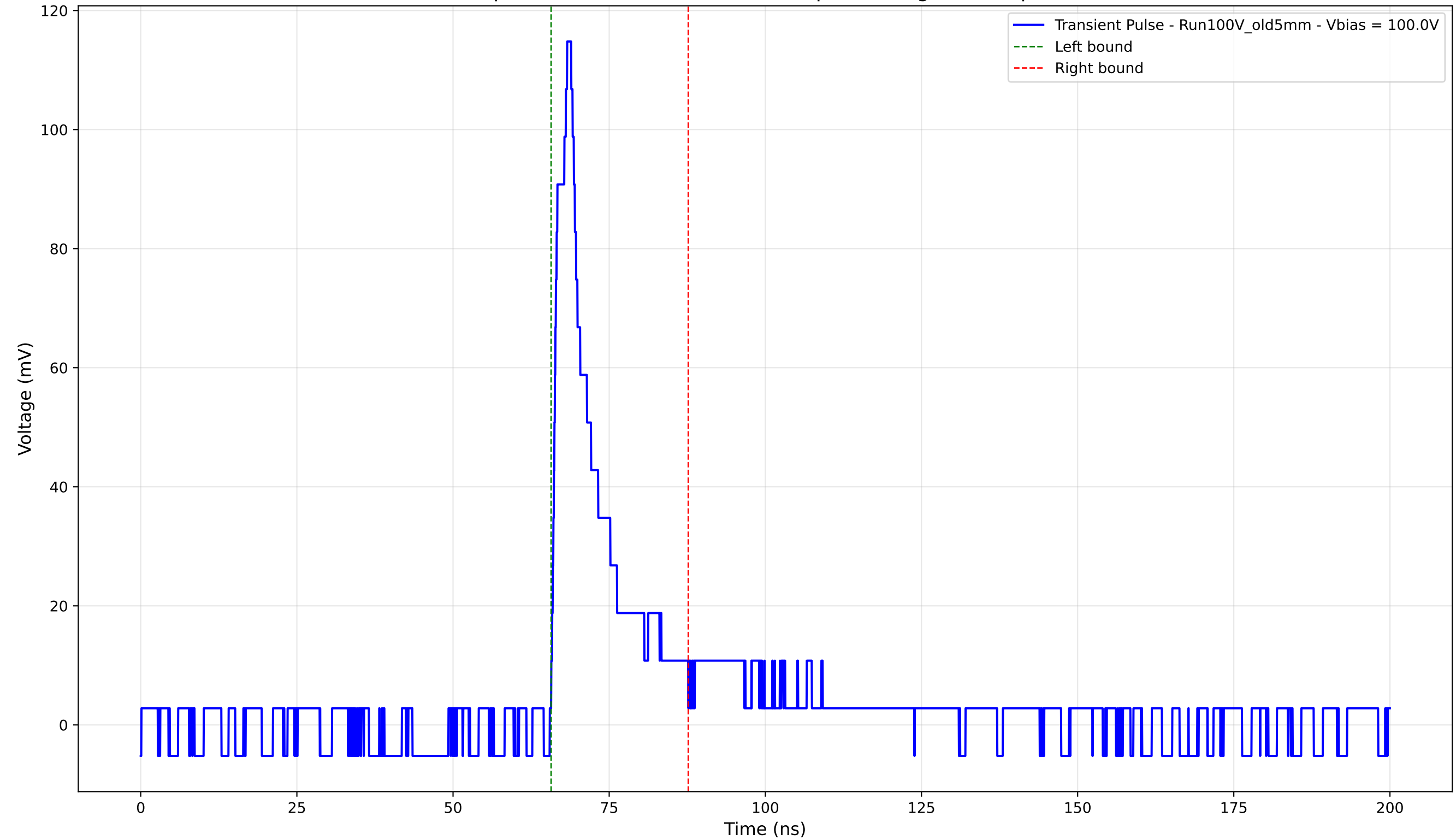
Transient Pulse - Sample: Old5mm - Position: 4140.0 \mu\text{m} - Charge: 16.09 pC - Rise Time: 2.22 ns
