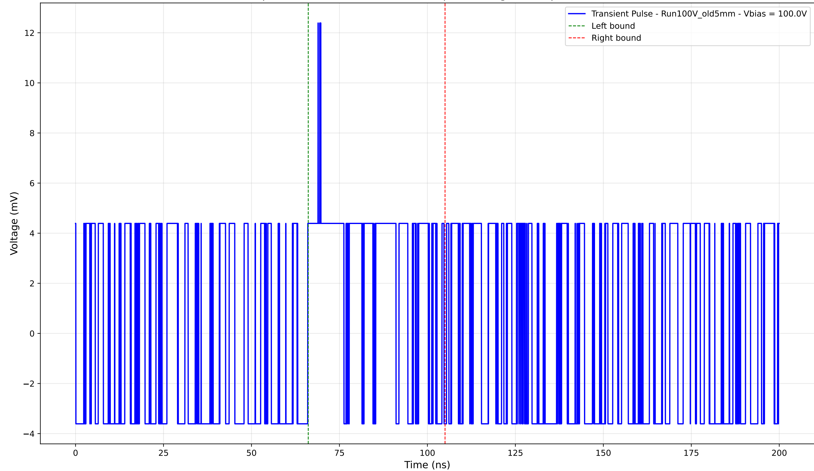
Transient Pulse - Sample: Old5mm - Position: 2760.0 \mu\text{m} - Charge: 2.21 pC - Rise Time: 0.00 ns (N/A)
