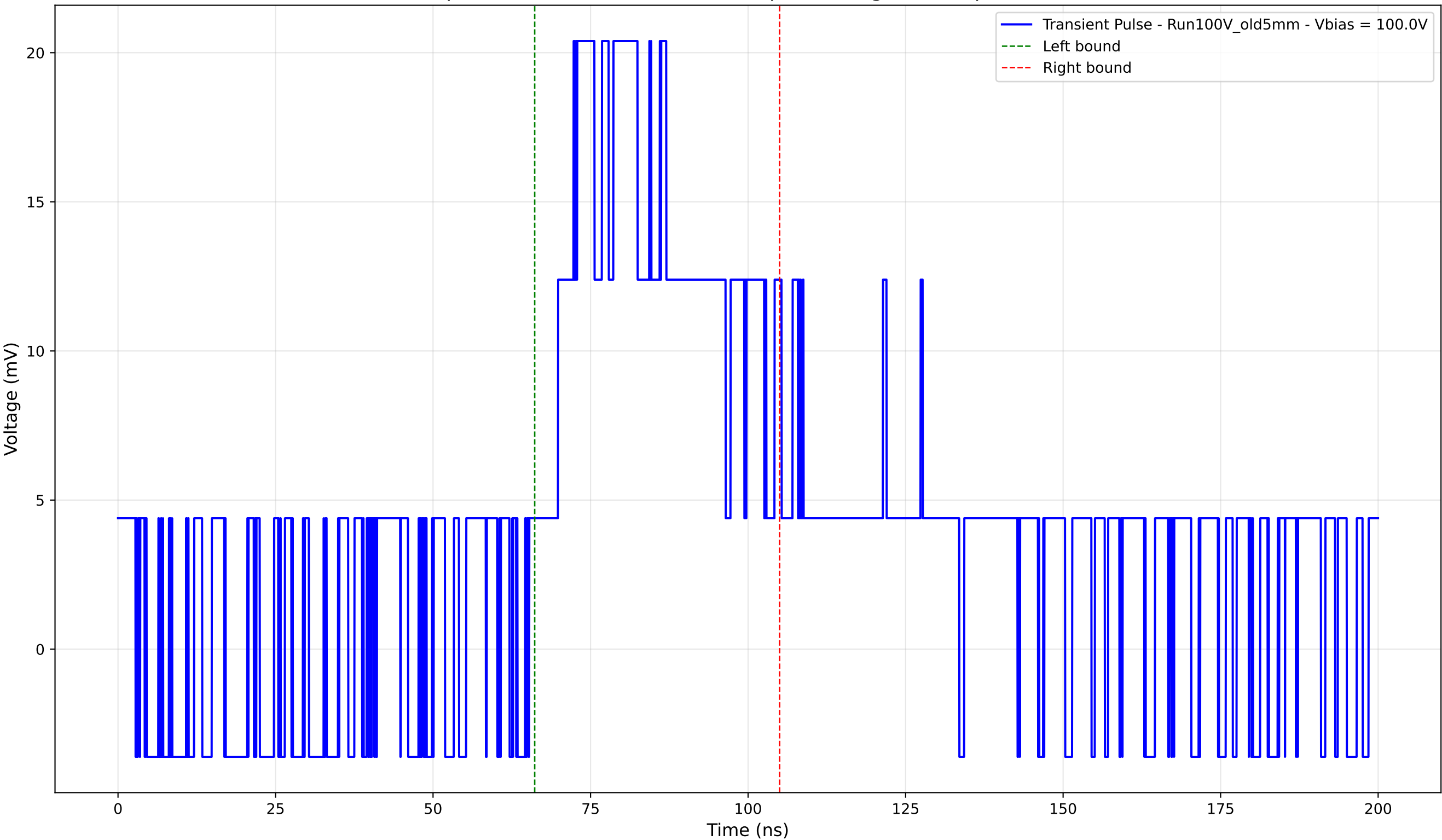
Transient Pulse - Sample: Old5mm - Position: 1835.0 \mu\text{m} - Charge: 10.08 pC - Rise Time: 0.00 ns (N/A)
