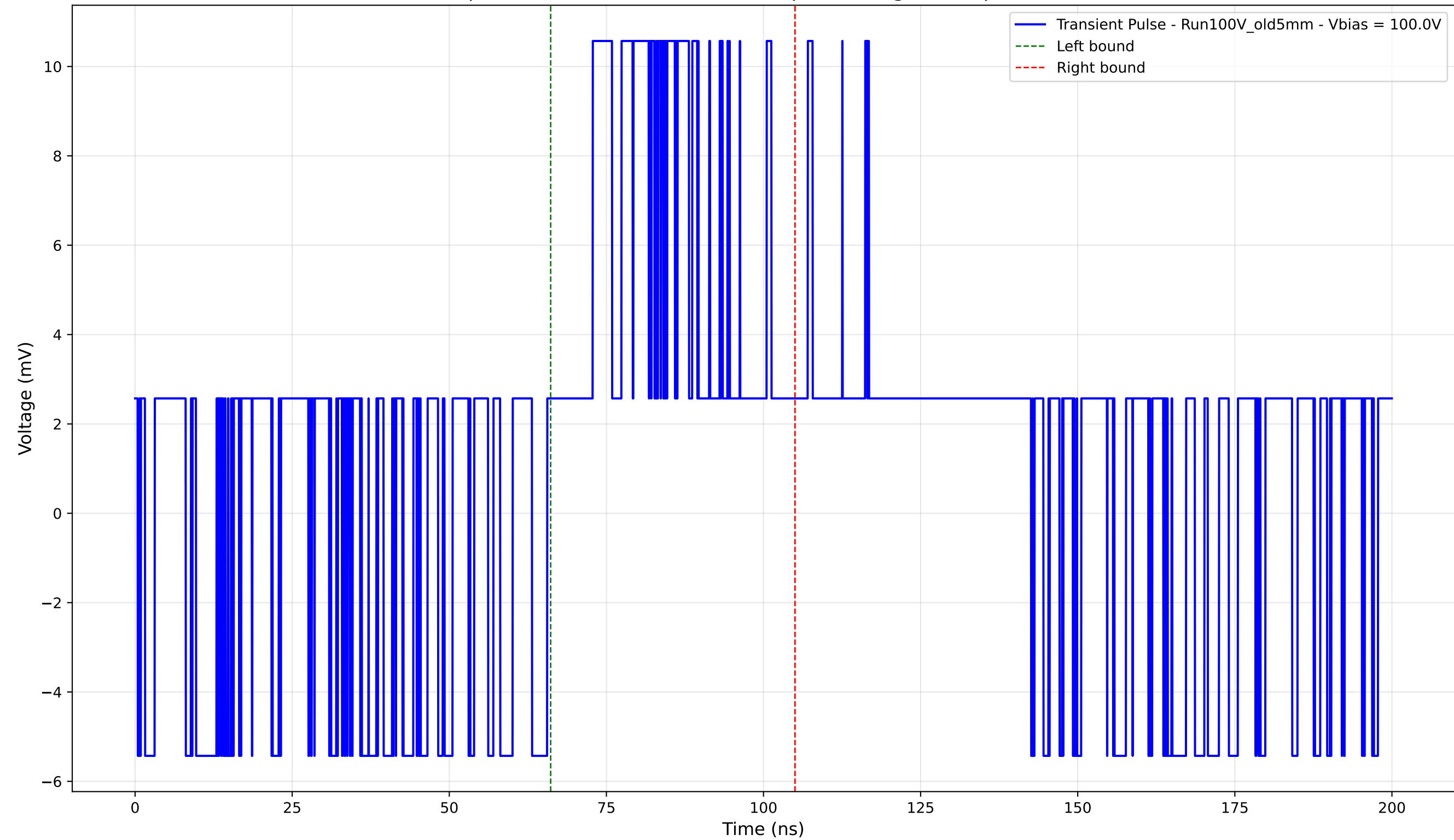
Transient Pulse - Sample: Old5mm - Position: 1105.0 \mu\text{m} - Charge: 4.35 pC - Rise Time: 0.00 ns (N/A)
