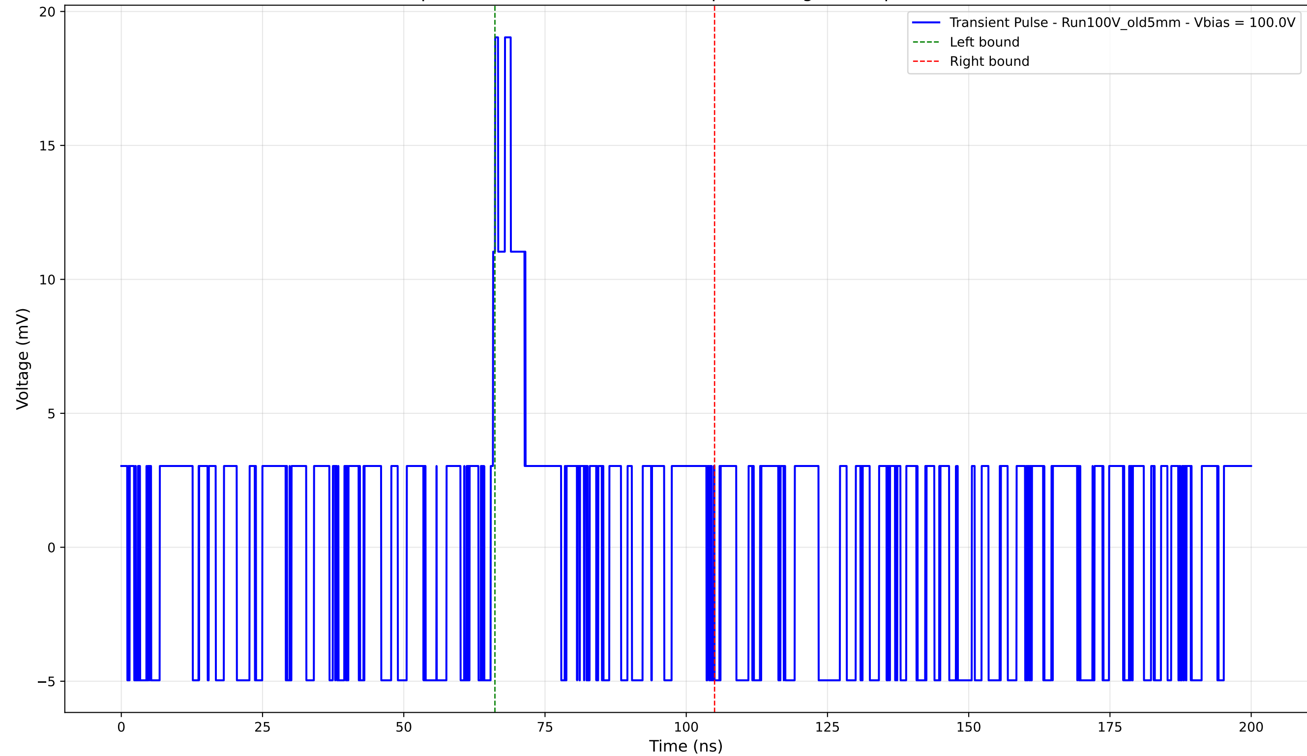
Transient Pulse - Sample: Old5mm - Position: 3735.0 \mu\text{m} - Charge: 2.16 pC - Rise Time: 0.00 ns (N/A)
