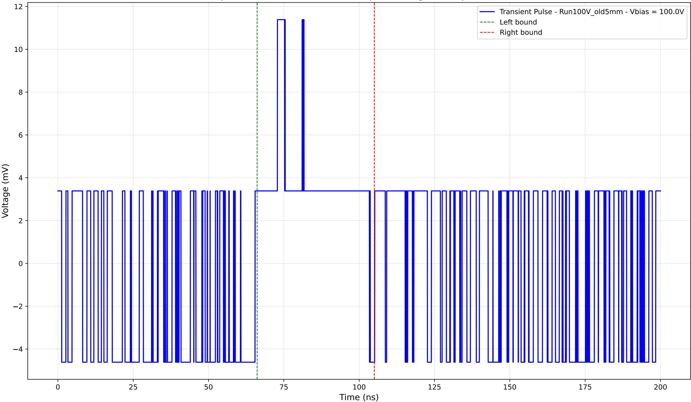
Transient Pulse - Sample: Old5mm - Position: 640.0 \mu\text{m} - Charge: 2.83 pC - Rise Time: 0.00 ns (N/A)
