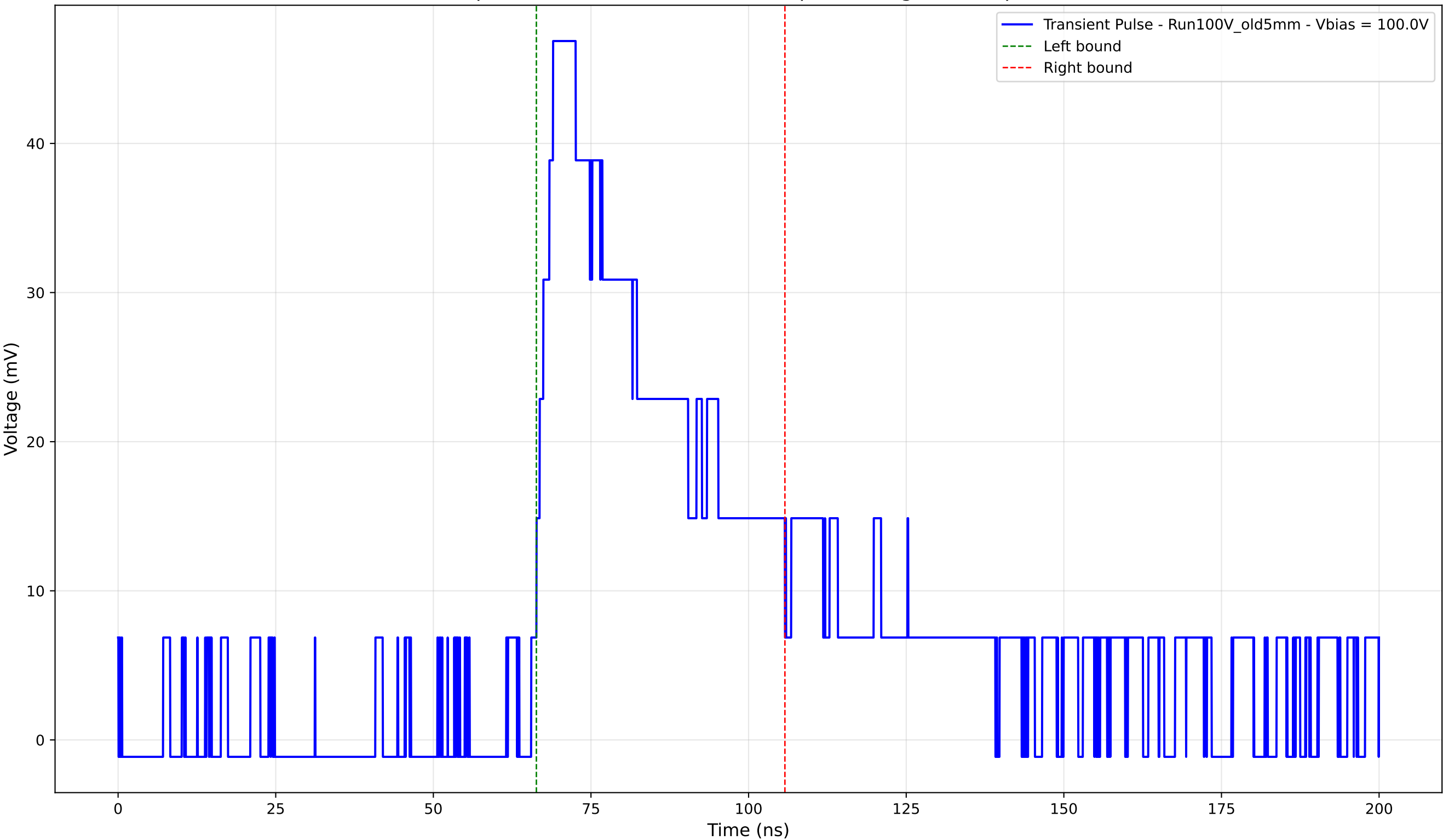
Transient Pulse - Sample: Old5mm - Position: 4860.0 \mu\text{m} - Charge: 20.15 pC - Rise Time: 3.47 ns
