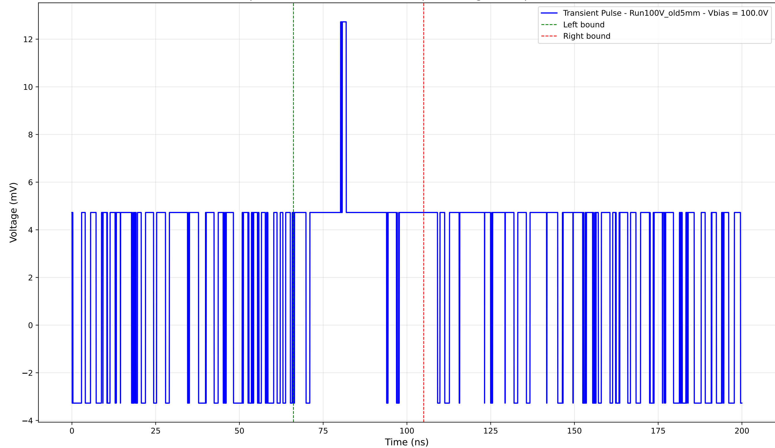
Transient Pulse - Sample: Old5mm - Position: 1690.0 \mu\text{m} - Charge: 3.55 pC - Rise Time: 0.00 ns (N/A)
