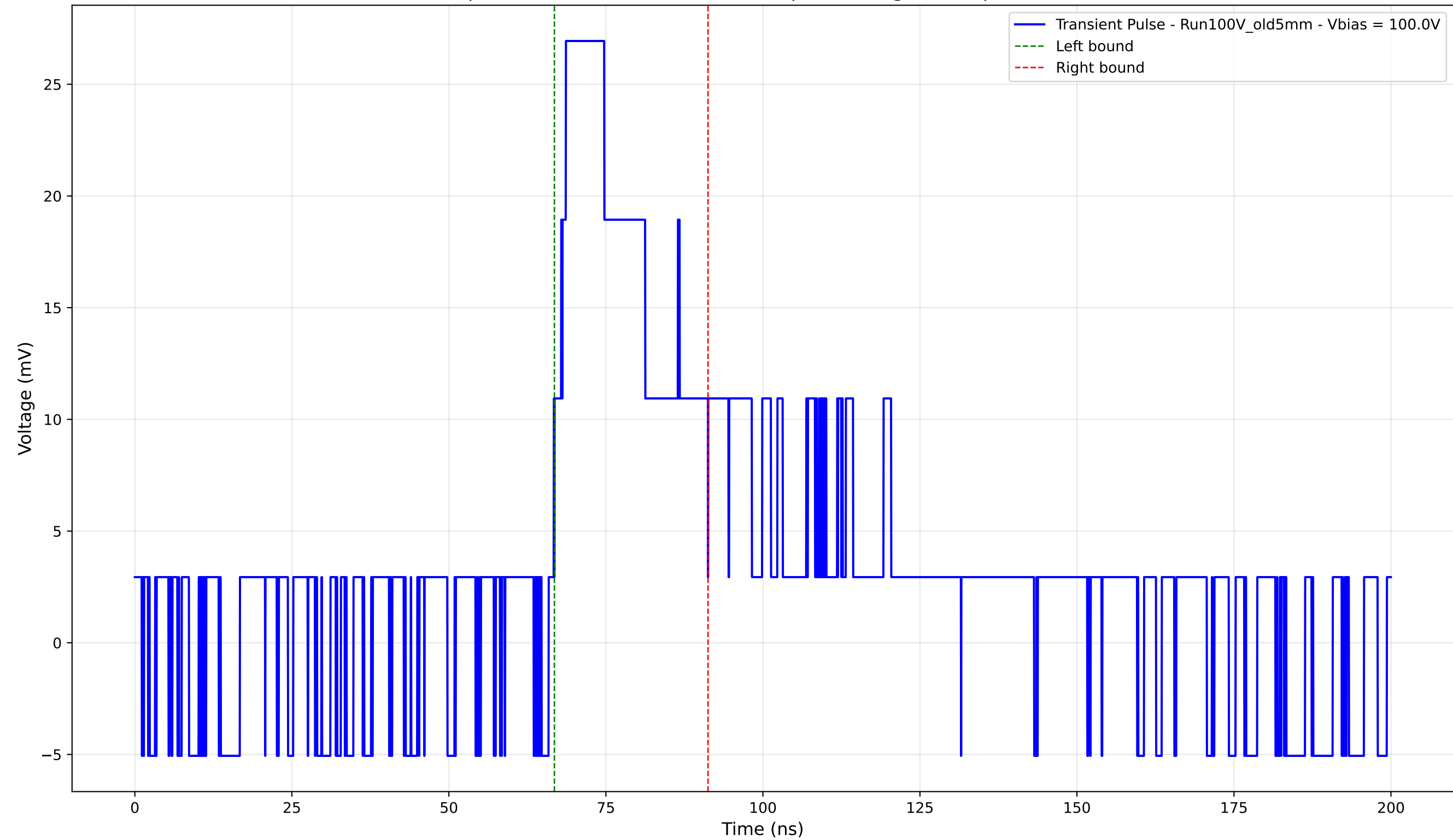
Transient Pulse - Sample: Old5mm - Position: 2585.0 \mu\text{m} - Charge: 8.49 pC - Rise Time: 0.00 ns (N/A)
