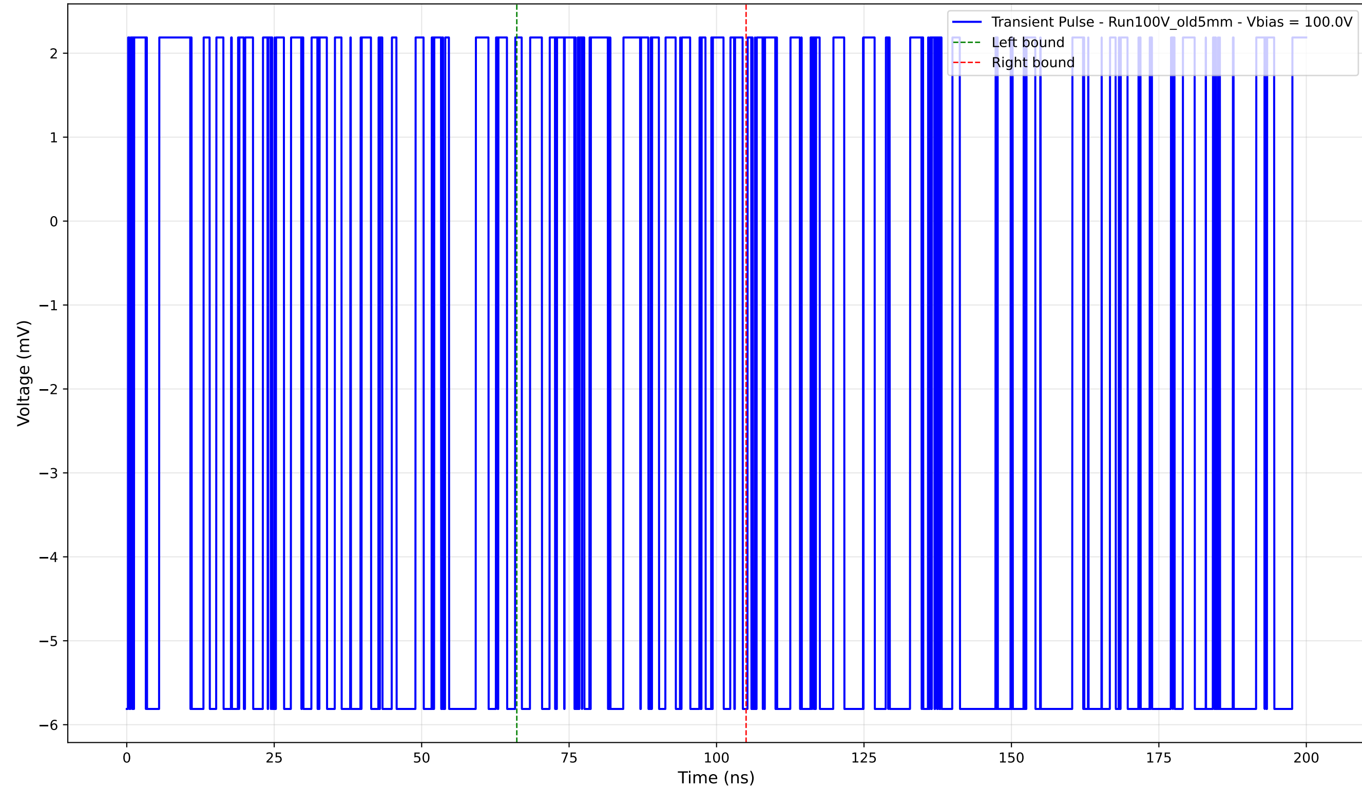
Transient Pulse - Sample: Old5mm - Position: 185.0 \mu\text{m} - Charge: -0.63 pC - Rise Time: 0.00 ns (N/A)
