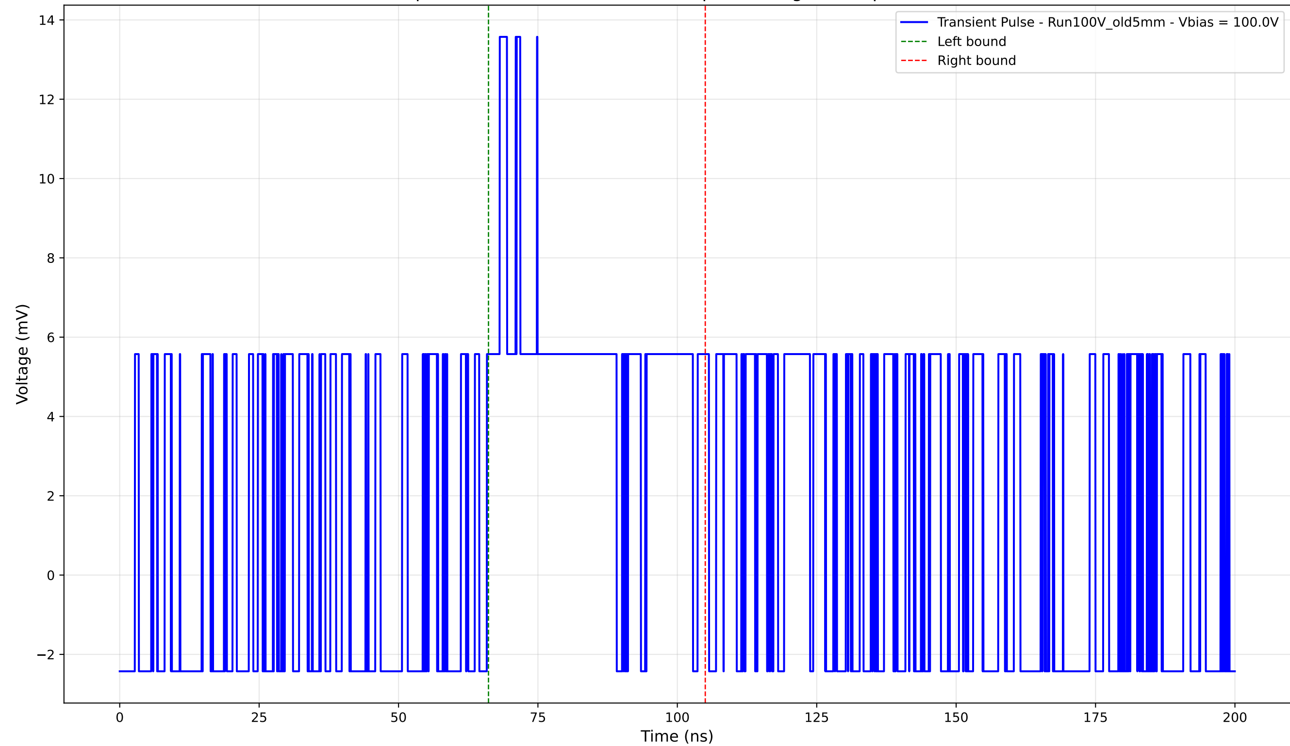
Transient Pulse - Sample: Old5mm - Position: 4660.0 \mu\text{m} - Charge: 4.19 pC - Rise Time: 0.00 ns (N/A)
