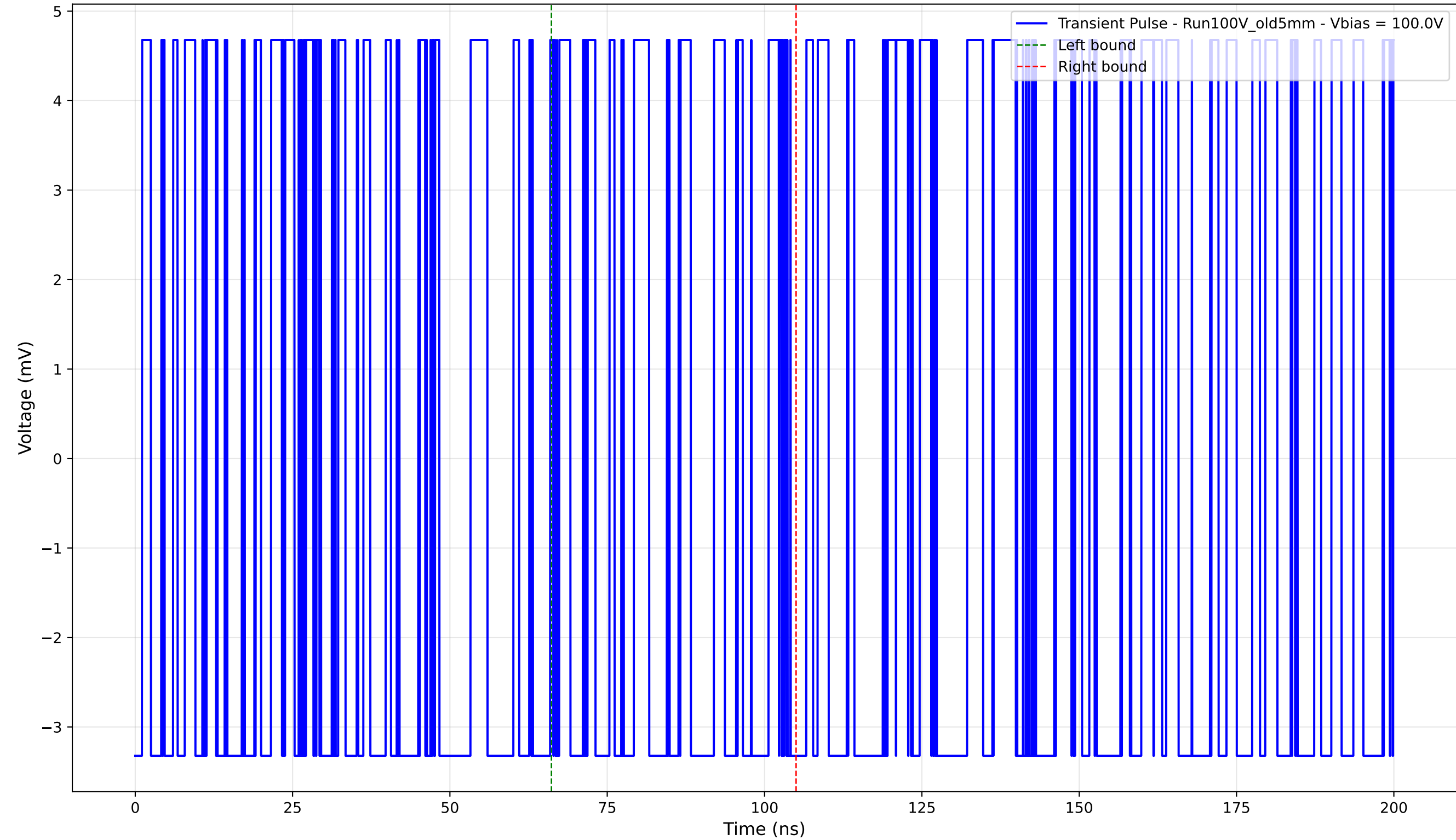
Transient Pulse - Sample: Old5mm - Position: 230.0 \mu\text{m} - Charge: -0.23 pC - Rise Time: 0.00 ns (N/A)
