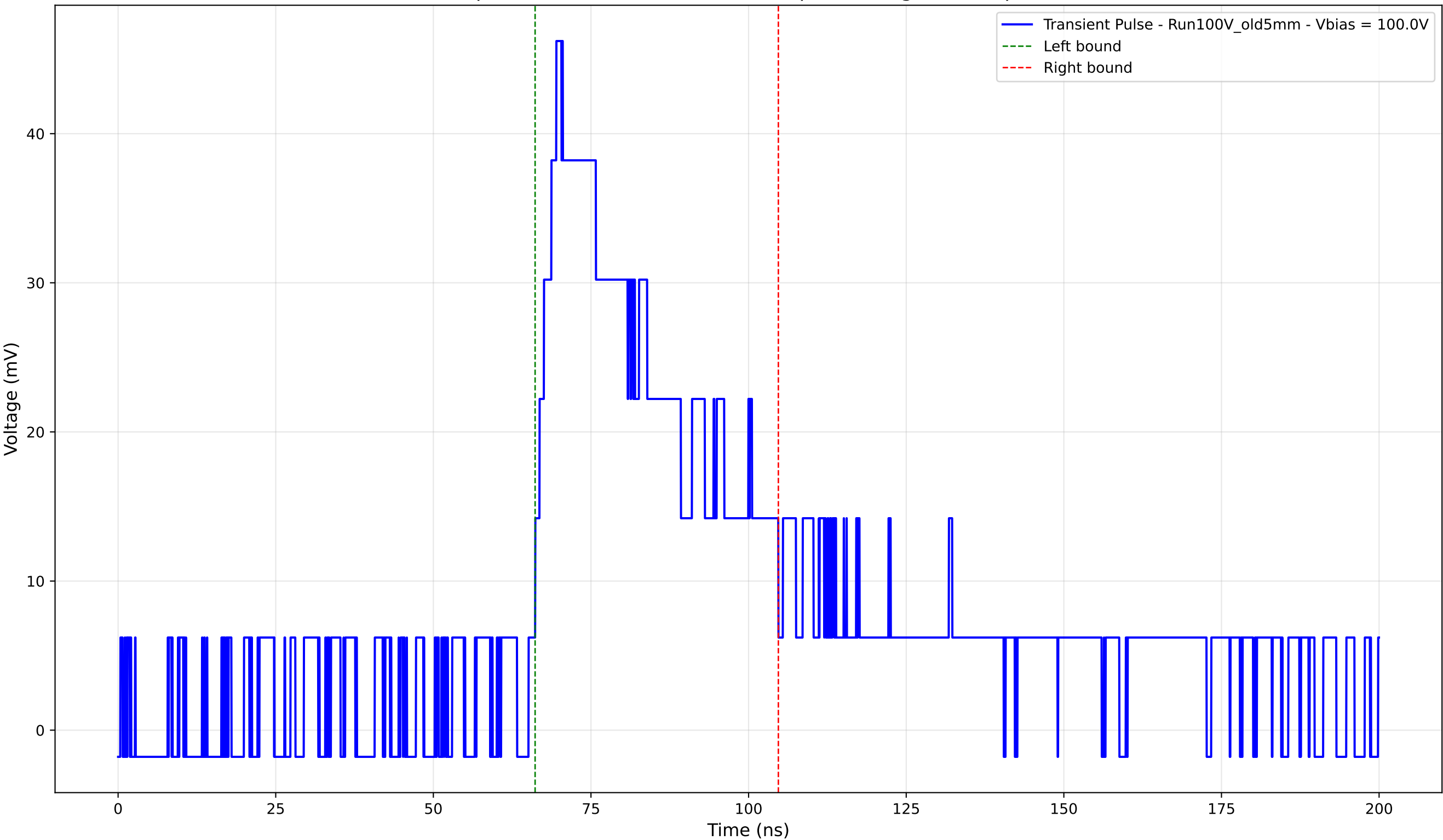
Transient Pulse - Sample: Old5mm - Position: 4915.0 \mu\text{m} - Charge: 18.92 pC - Rise Time: 4.41 ns
