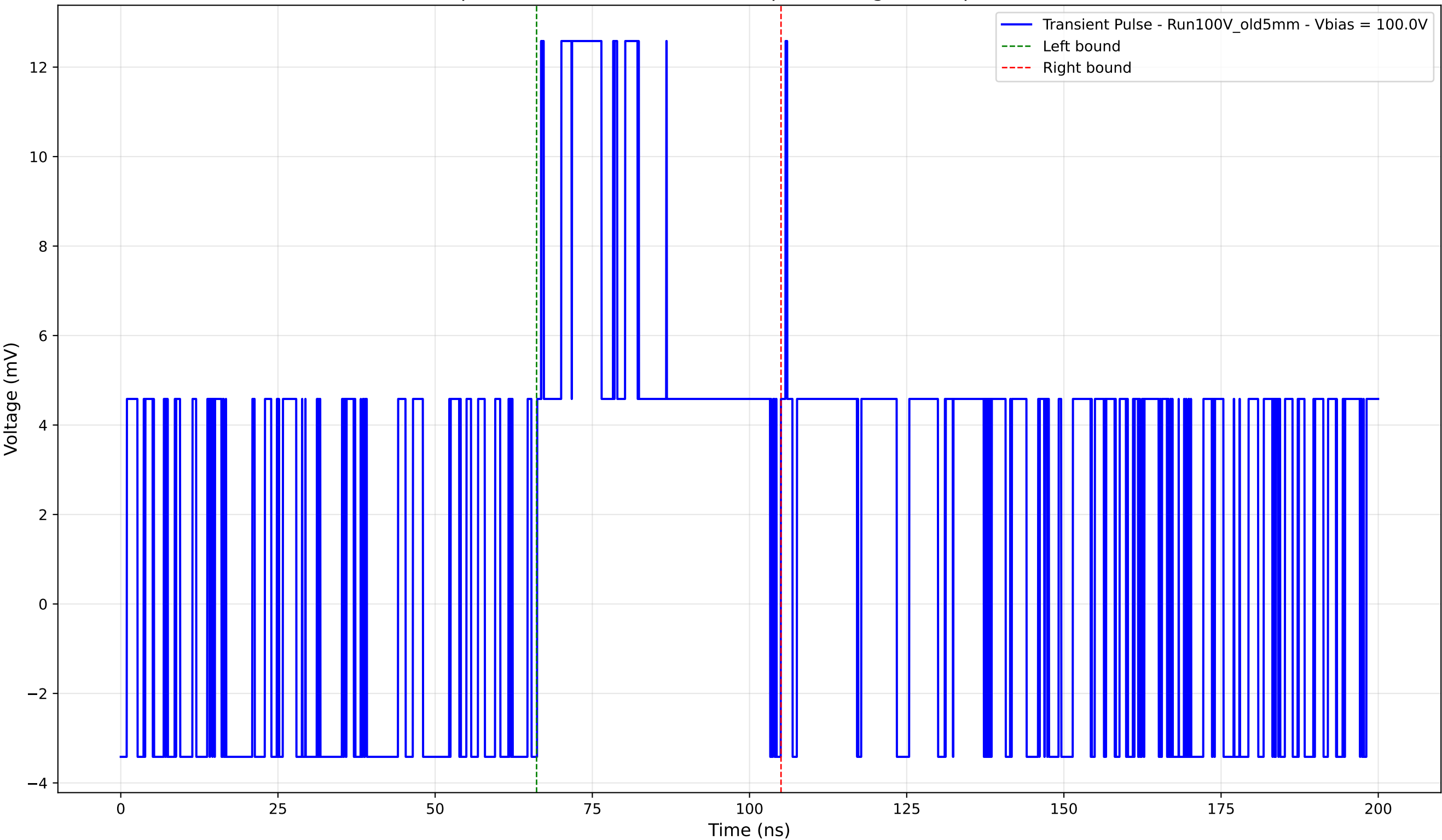
Transient Pulse - Sample: Old5mm - Position: 395.0 \mu\text{m} - Charge: 4.85 pC - Rise Time: 0.00 ns (N/A)
