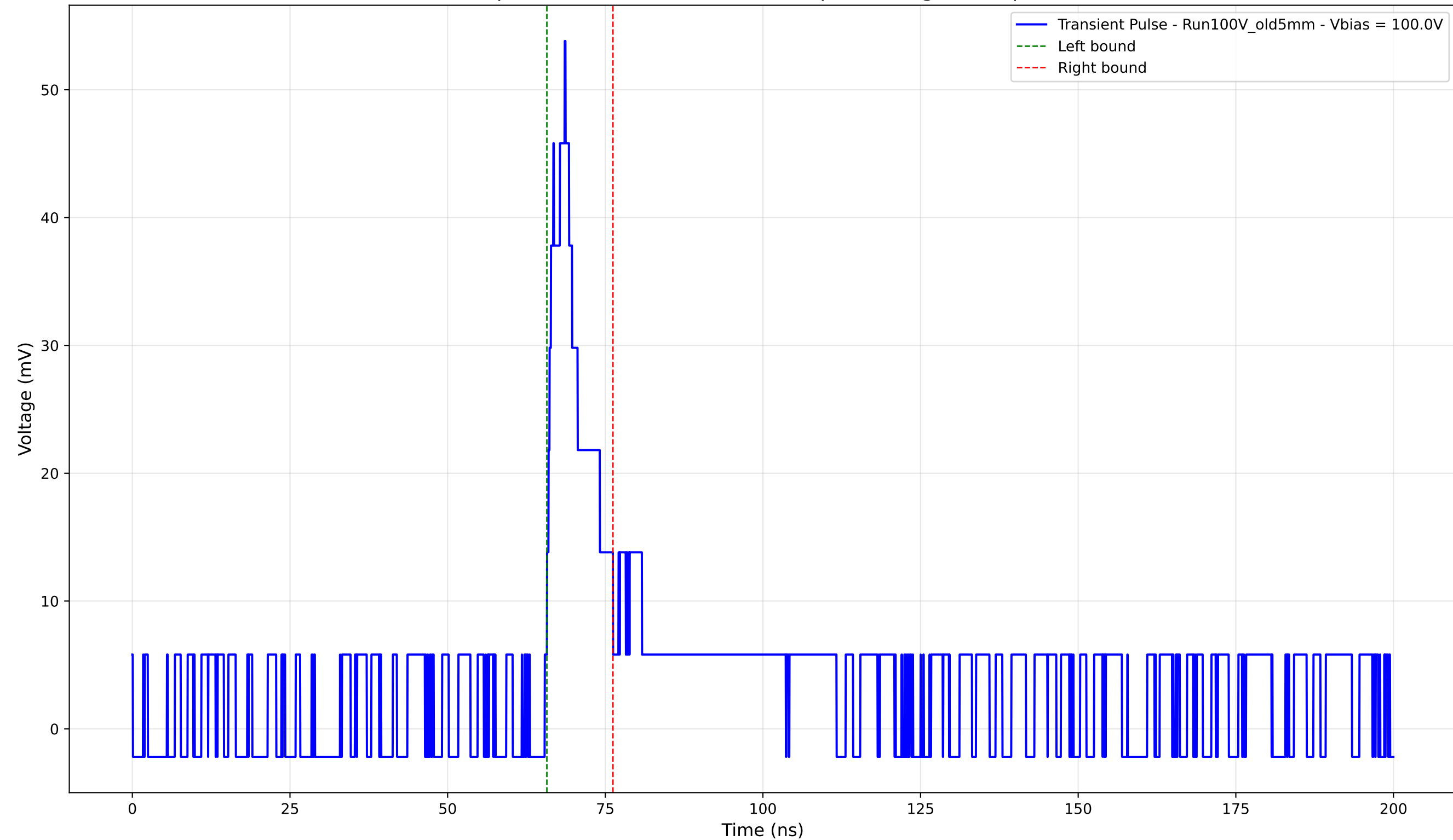
Transient Pulse - Sample: Old5mm - Position: 4070.0 \mu\text{m} - Charge: 5.72 pC - Rise Time: 3.16 ns
