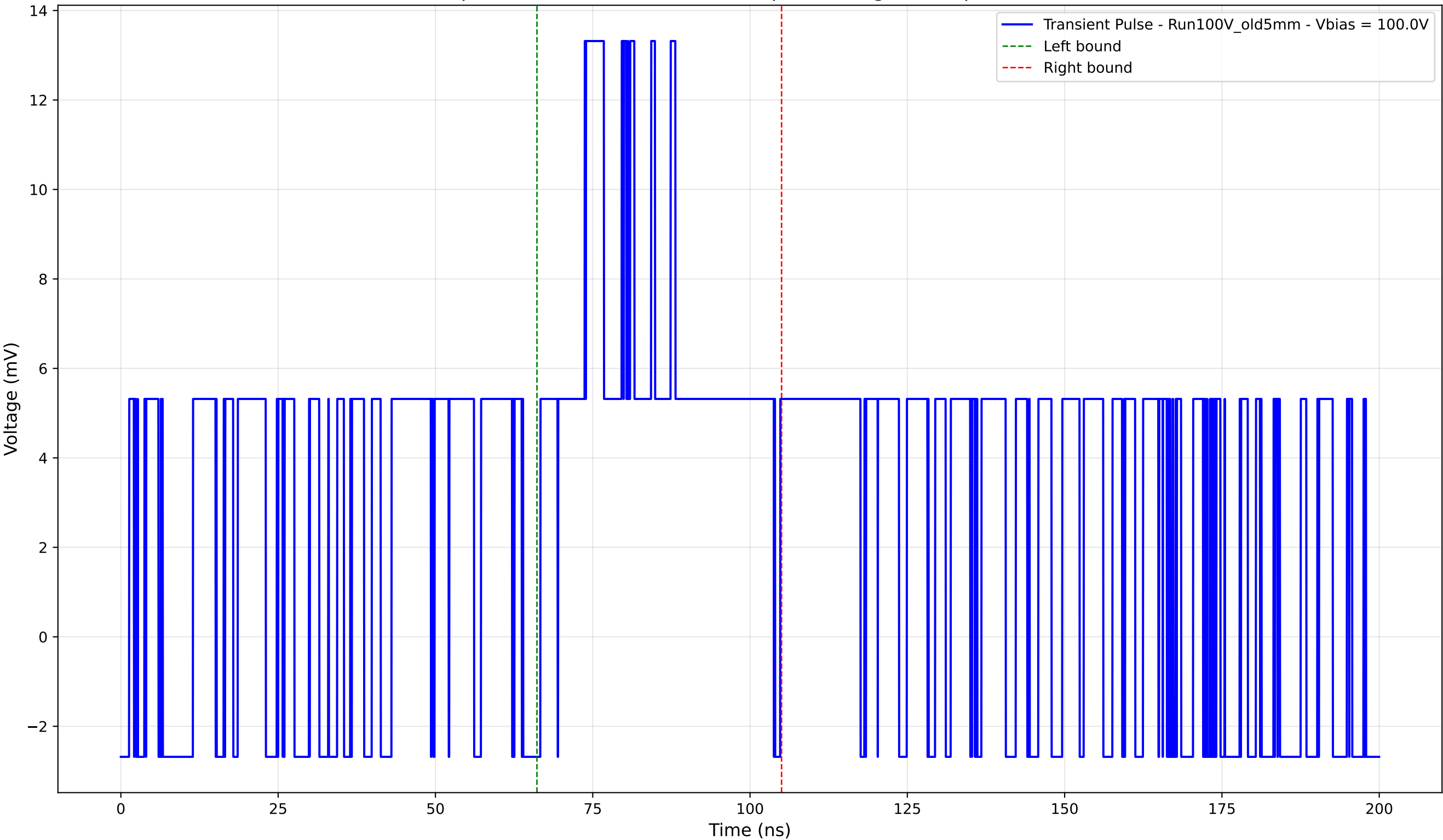
Transient Pulse - Sample: Old5mm - Position: 920.0 \mu\text{m} - Charge: 4.84 pC - Rise Time: 0.00 ns (N/A)
