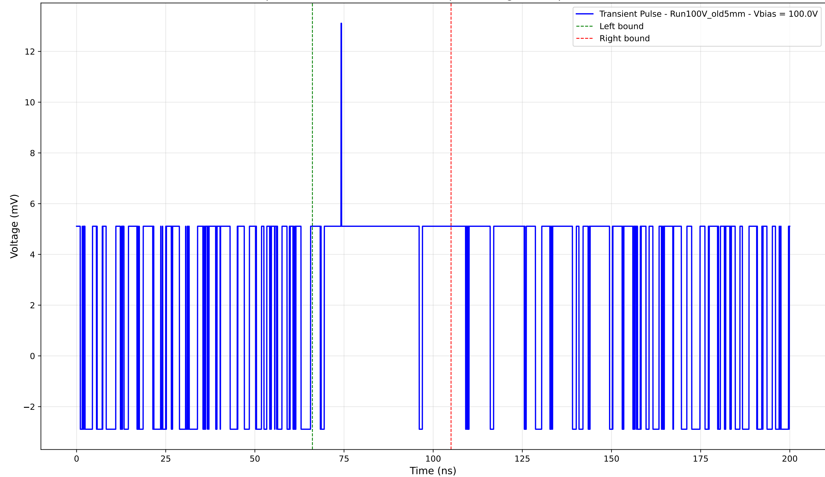
Transient Pulse - Sample: Old5mm - Position: 1275.0 \mu\text{m} - Charge: 3.68 pC - Rise Time: 0.00 ns (N/A)
