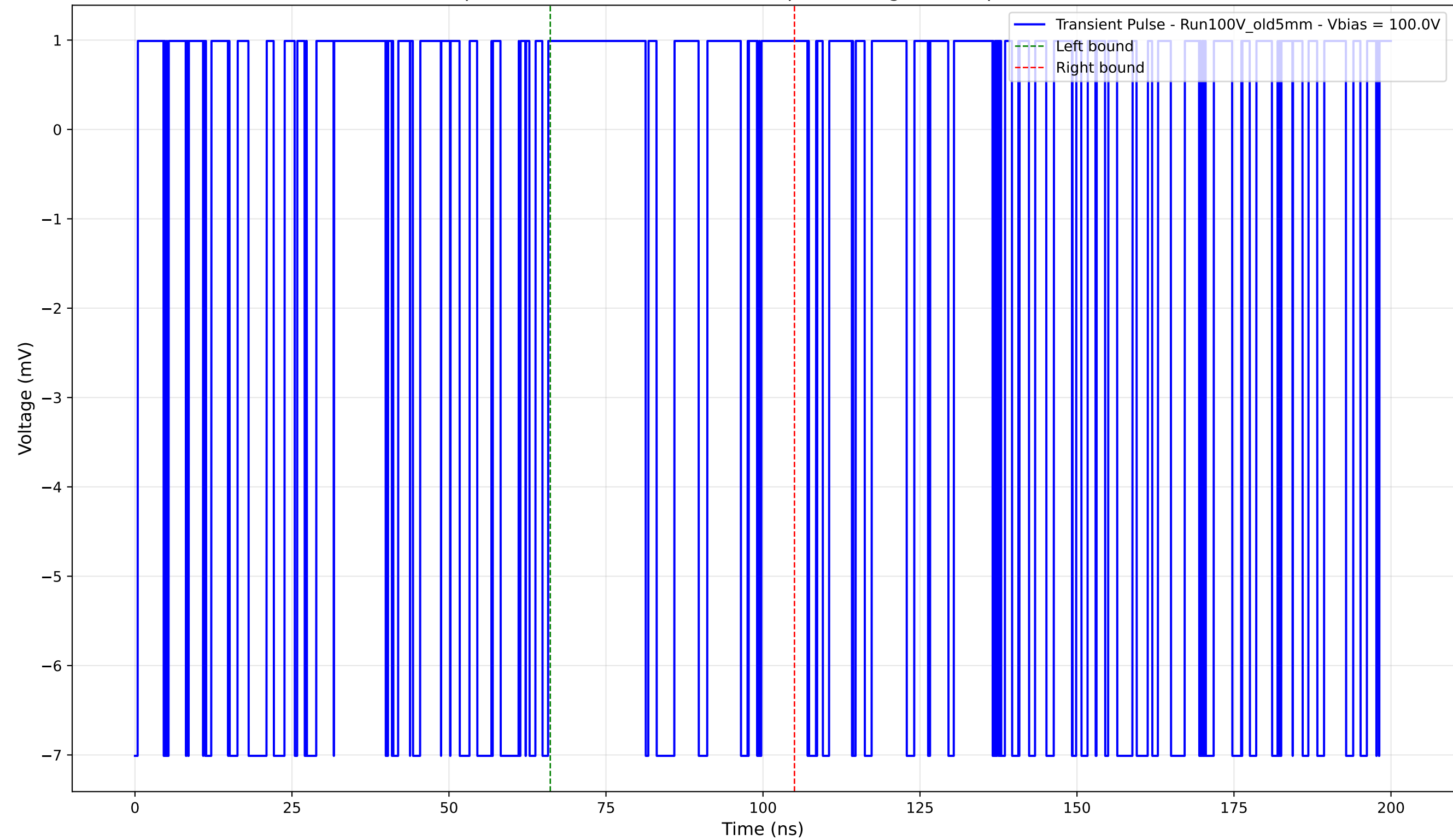
Transient Pulse - Sample: Old5mm - Position: 4010.0 \mu\text{m} - Charge: -0.25 pC - Rise Time: 0.00 ns (N/A)
