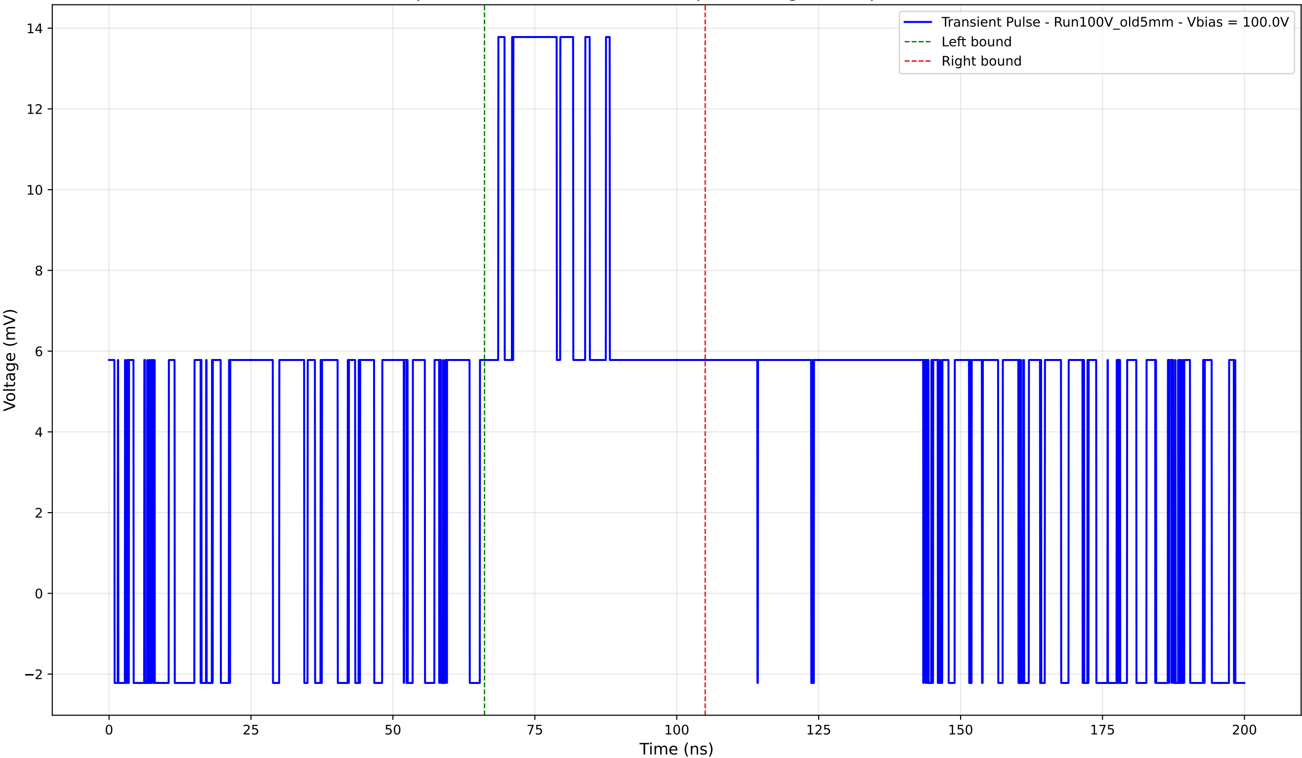
Transient Pulse - Sample: Old5mm - Position: 585.0 \mu\text{m} - Charge: 6.52 pC - Rise Time: 0.00 ns (N/A)
