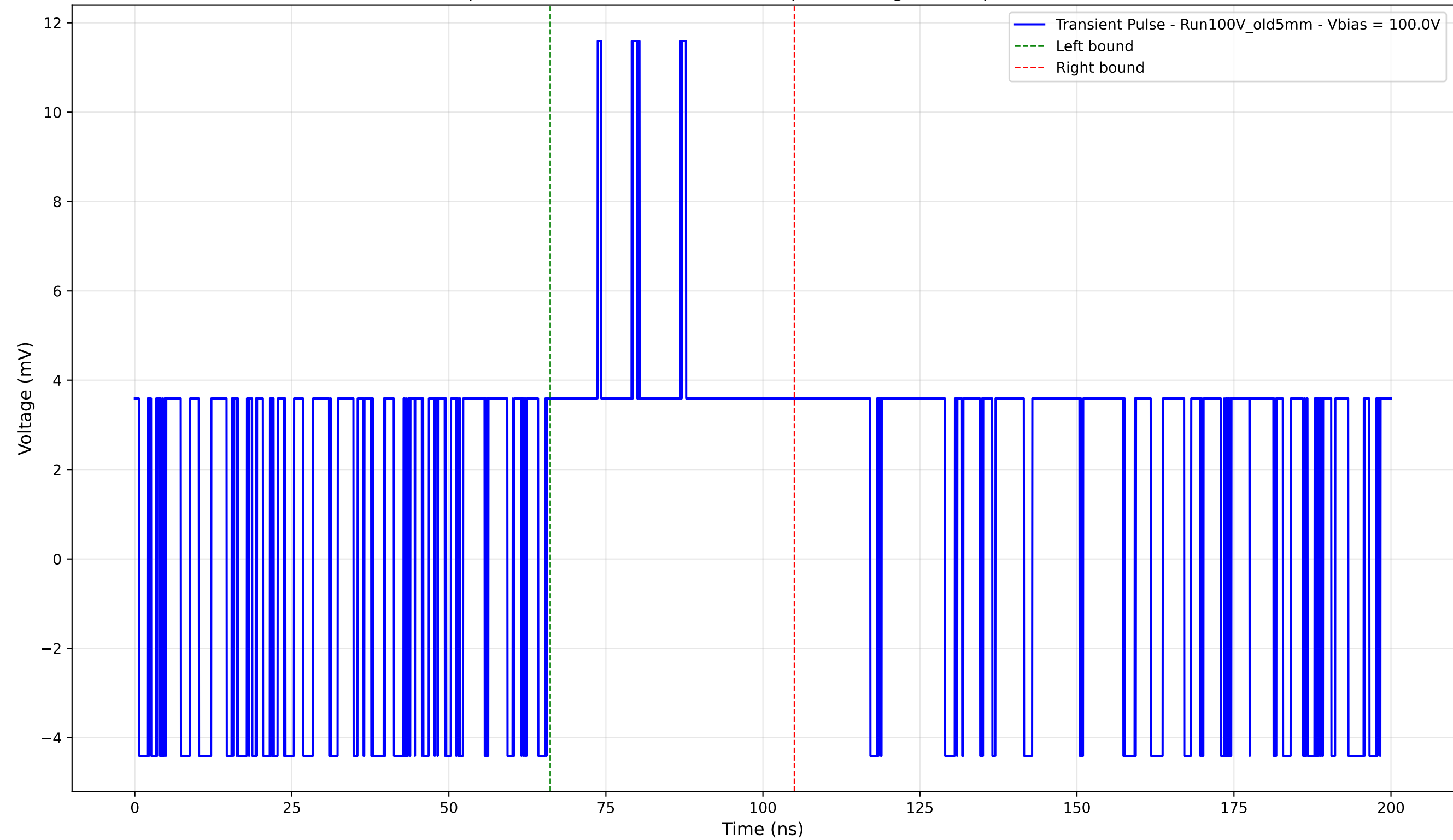
Transient Pulse - Sample: Old5mm - Position: 1740.0 \mu\text{m} - Charge: 3.16 pC - Rise Time: 0.00 ns (N/A)
