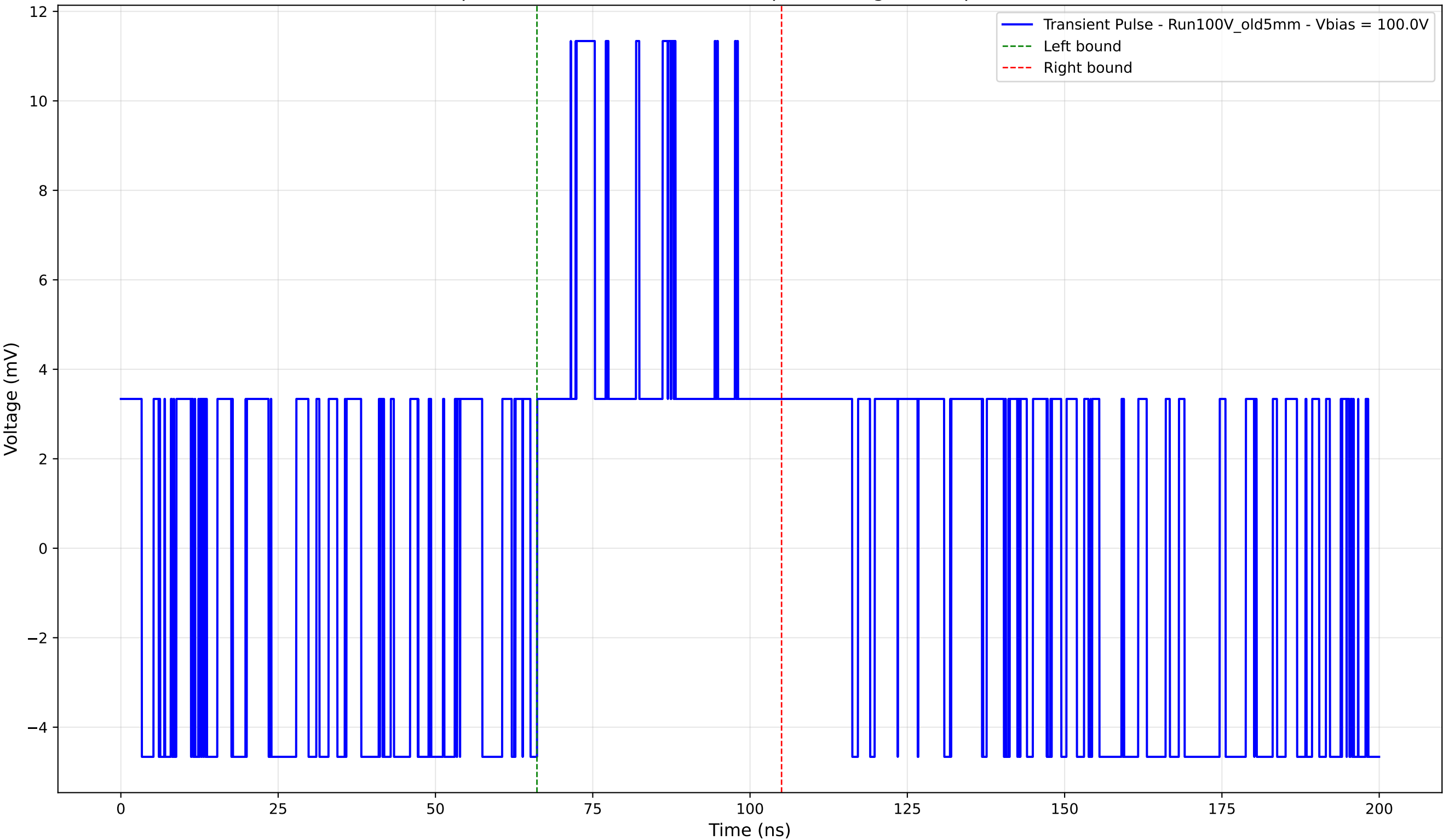
Transient Pulse - Sample: Old5mm - Position: 485.0 \mu\text{m} - Charge: 3.59 pC - Rise Time: 0.00 ns (N/A)
