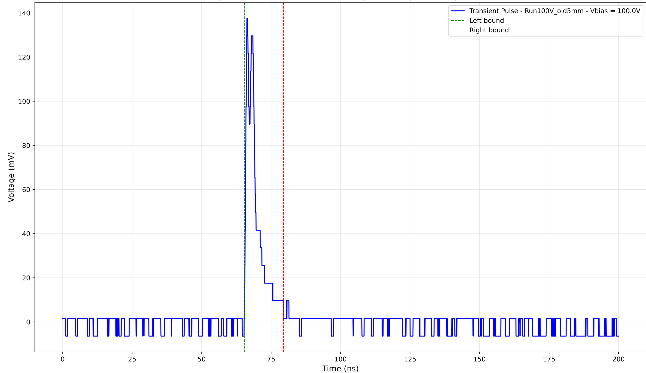
Transient Pulse - Sample: Old5mm - Position: 3785.0 \mu\text{m} - Charge: 11.99 pC - Rise Time: 0.73 ns
