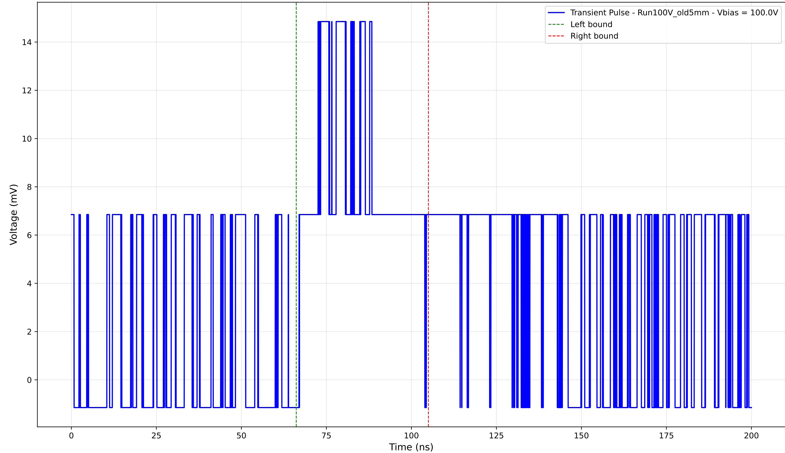
Transient Pulse - Sample: Old5mm - Position: 760.0 \mu\text{m} - Charge: 6.48 pC - Rise Time: 5.50 ns
