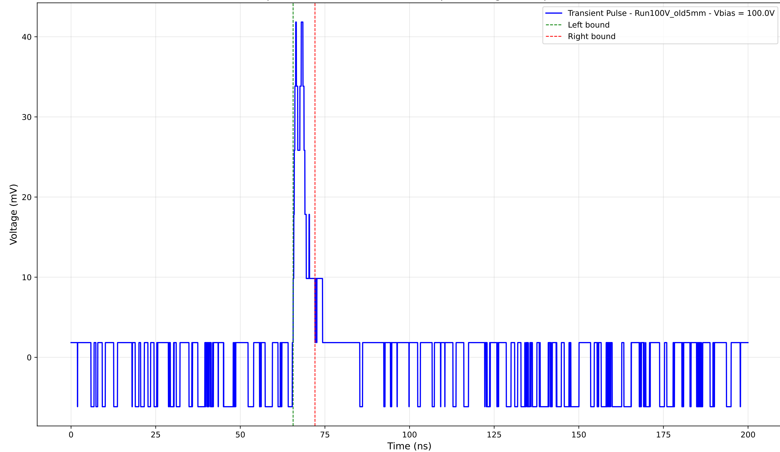
Transient Pulse - Sample: Old5mm - Position: 3750.0 \mu\text{m} - Charge: 2.82 pC - Rise Time: 0.75 ns
