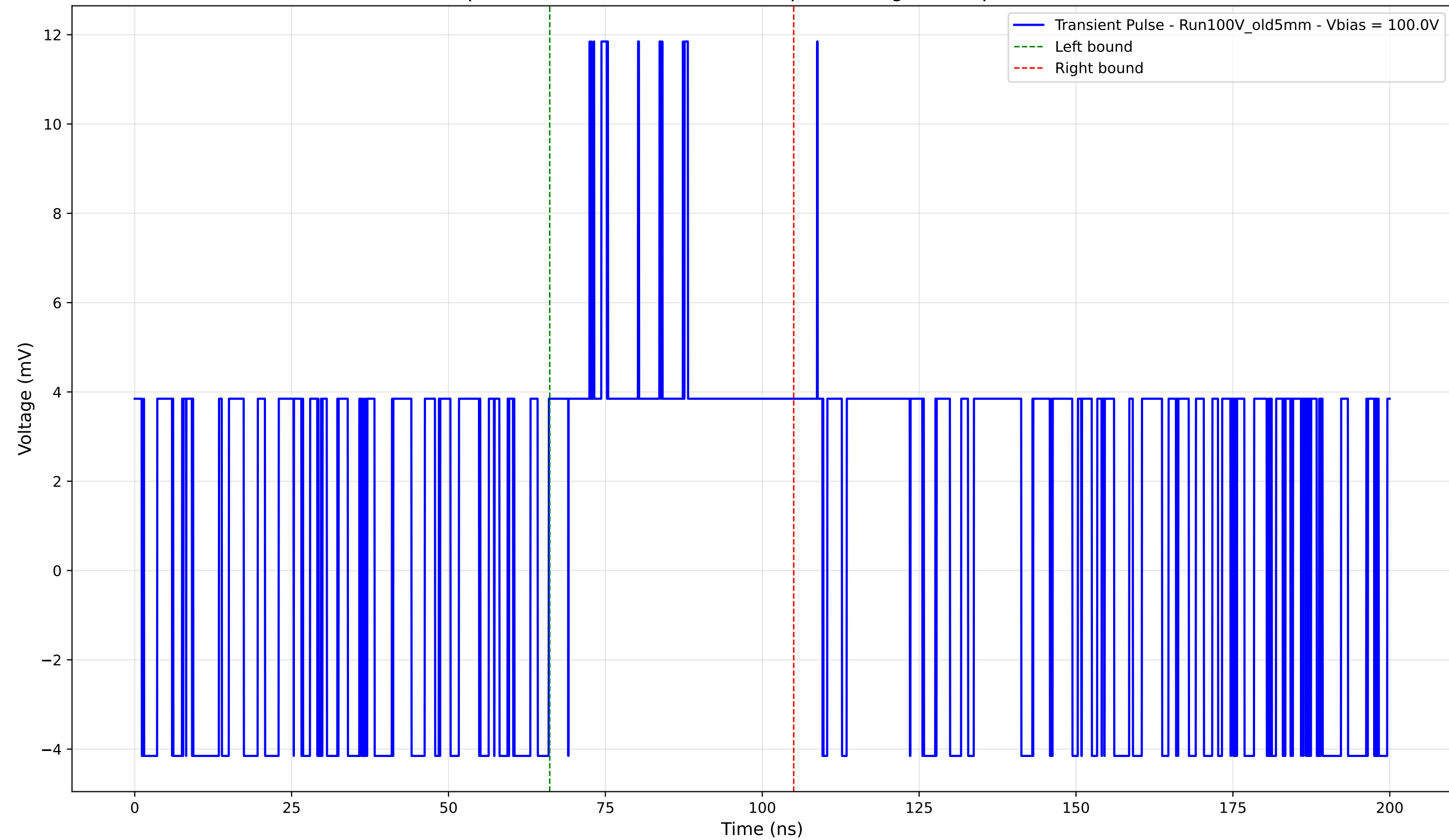
Transient Pulse - Sample: Old5mm - Position: 1040.0 \mu\text{m} - Charge: 3.33 pC - Rise Time: 0.00 ns (N/A)
