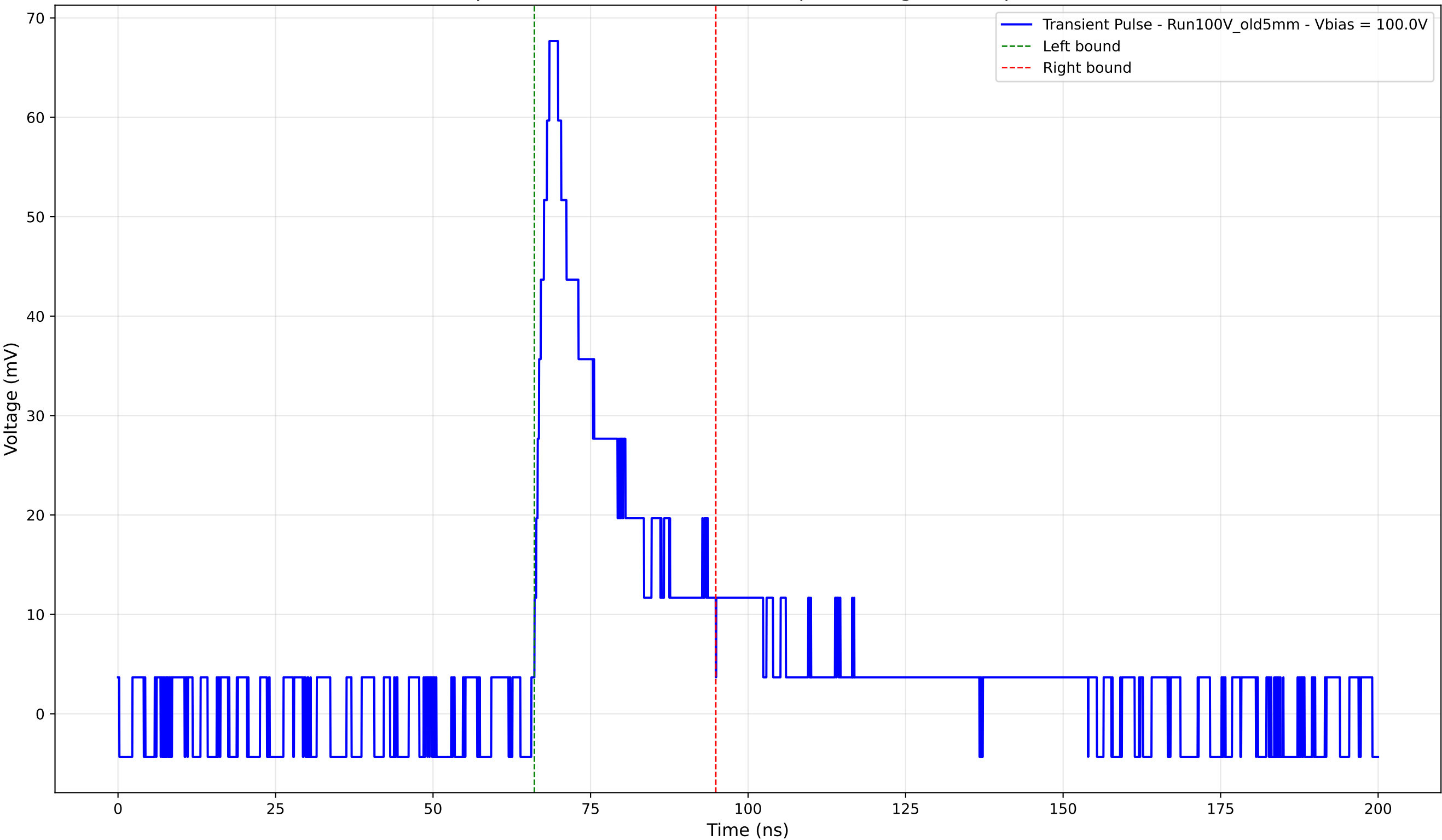
Transient Pulse - Sample: Old5mm - Position: 4475.0 \mu\text{m} - Charge: 15.62 pC - Rise Time: 2.37 ns
