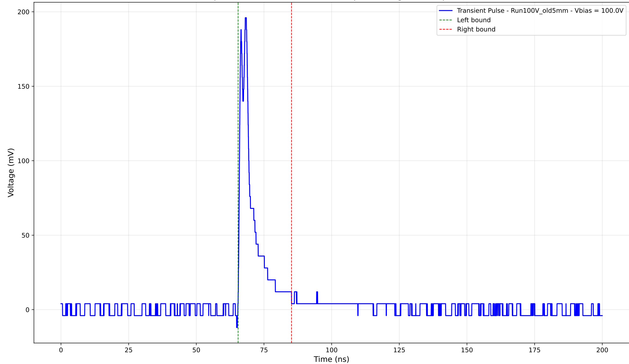
Transient Pulse - Sample: Old5mm - Position: 3555.0 \mu\text{m} - Charge: 20.81 pC - Rise Time: 0.84 ns
