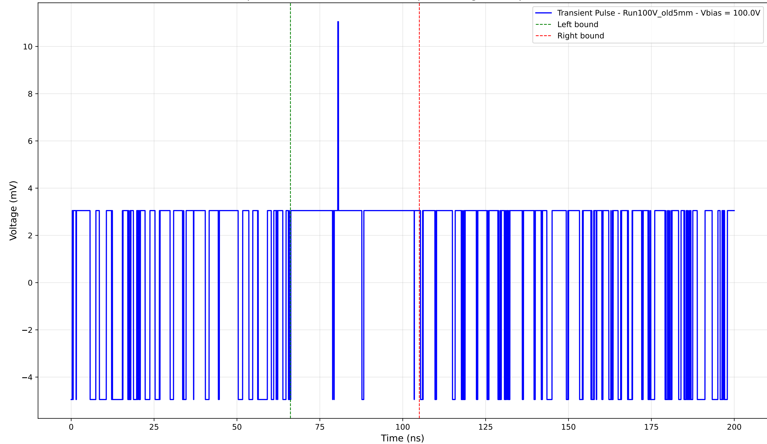
Transient Pulse - Sample: Old5mm - Position: 2520.0 \mu\text{m} - Charge: 2.27 pC - Rise Time: 0.00 ns (N/A)
