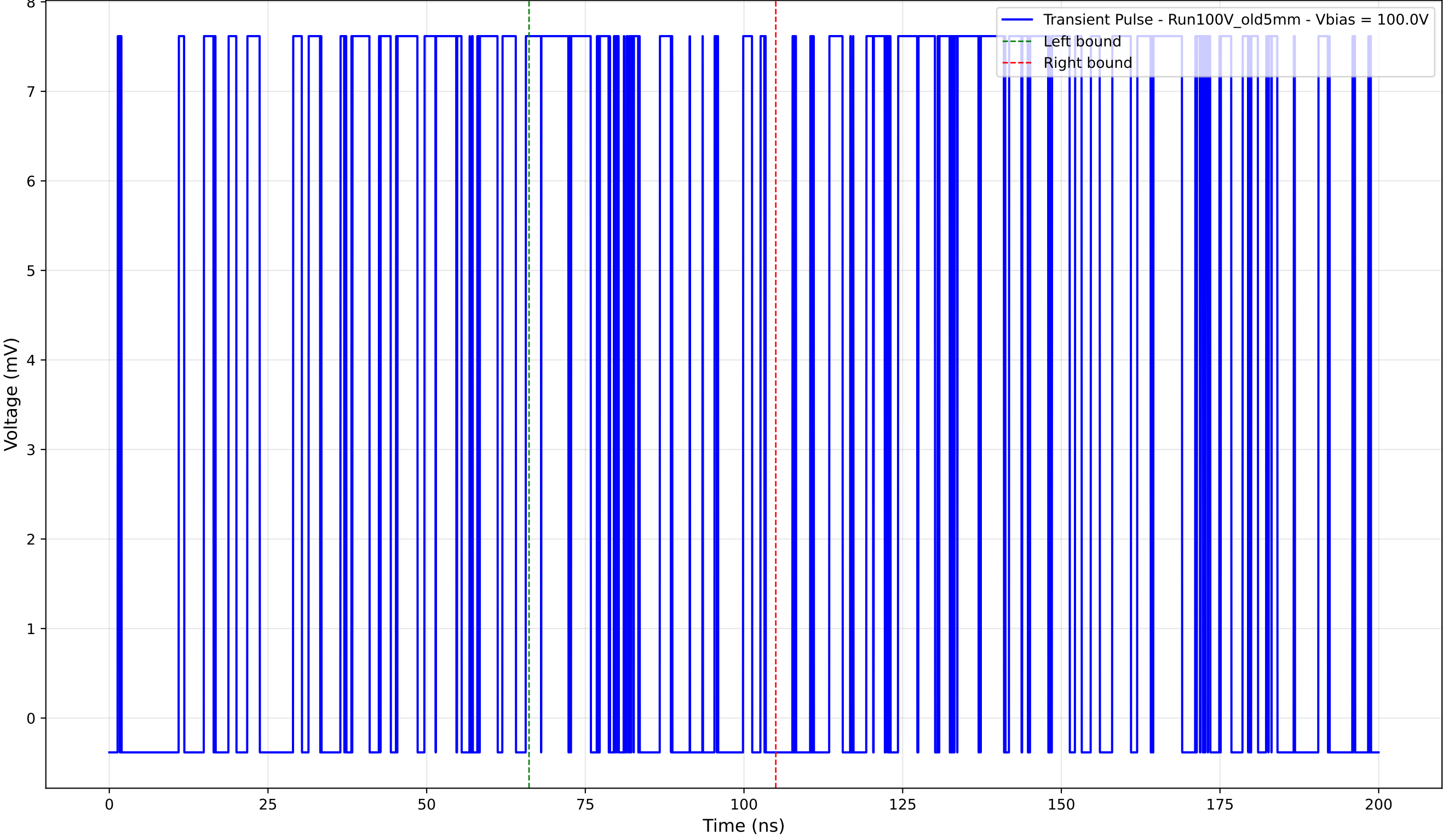
Transient Pulse - Sample: Old5mm - Position: 2775.0 \mu\text{m} - Charge: 2.59 pC - Rise Time: 0.02 ns
