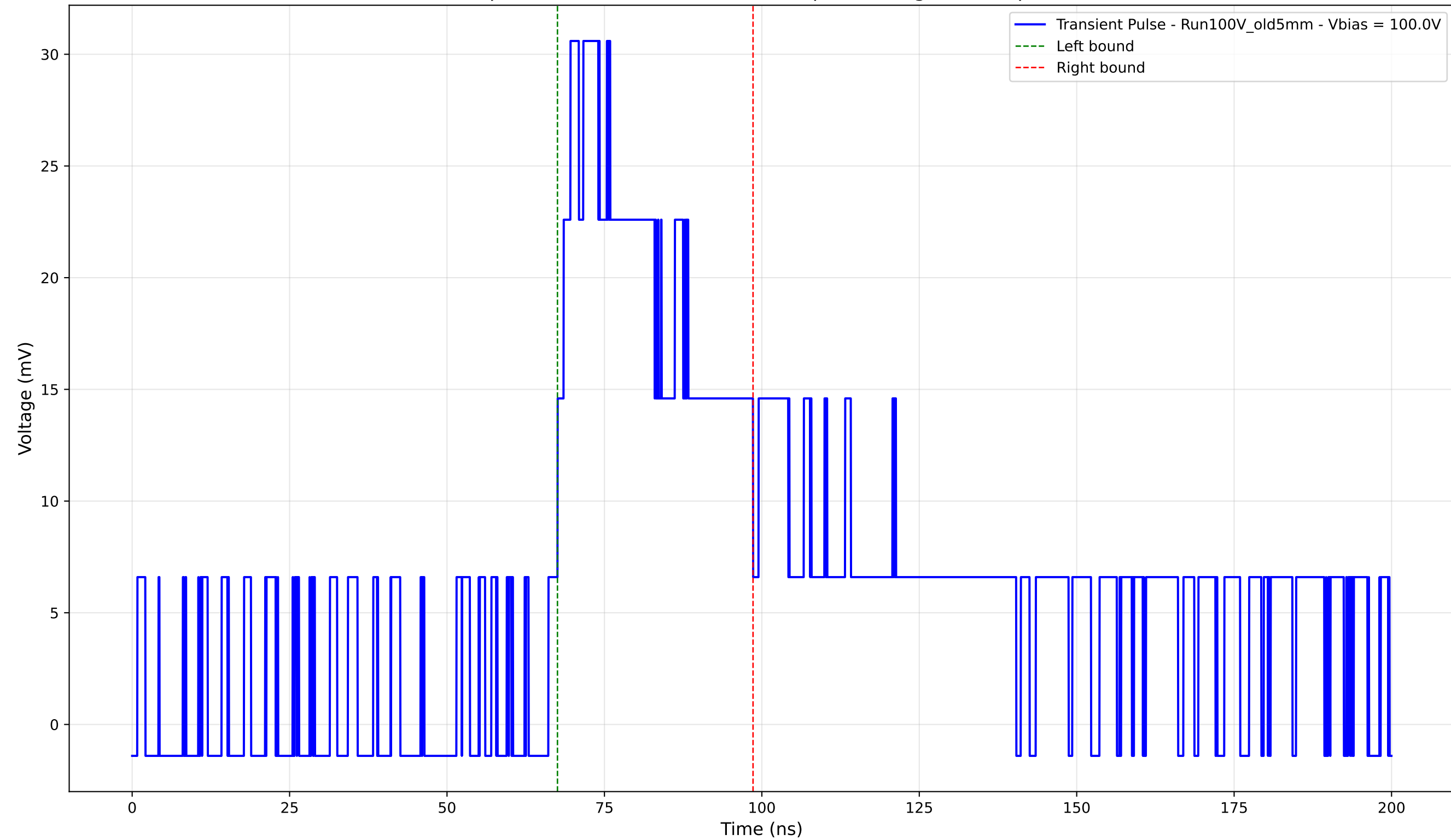
Transient Pulse - Sample: Old5mm - Position: 2400.0 \mu\text{m} - Charge: 12.38 pC - Rise Time: 3.51 ns
