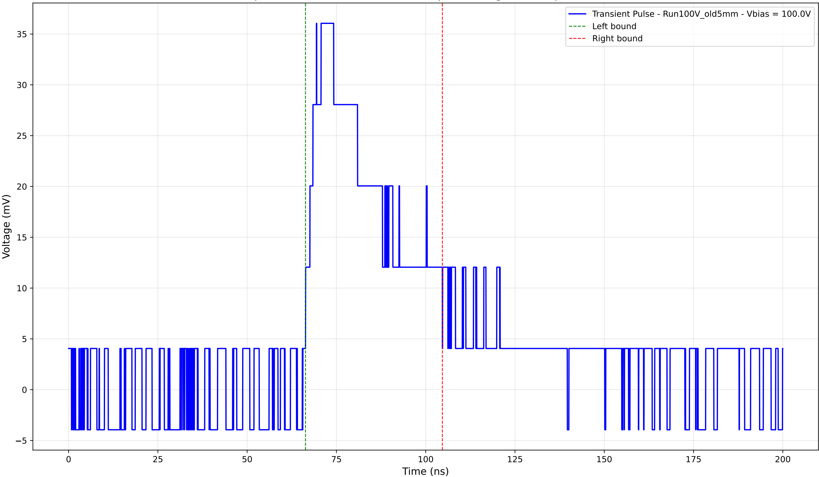
Transient Pulse - Sample: Old5mm - Position: 4960.0 \mu\text{m} - Charge: 15.36 pC - Rise Time: 0.00 ns (N/A)
