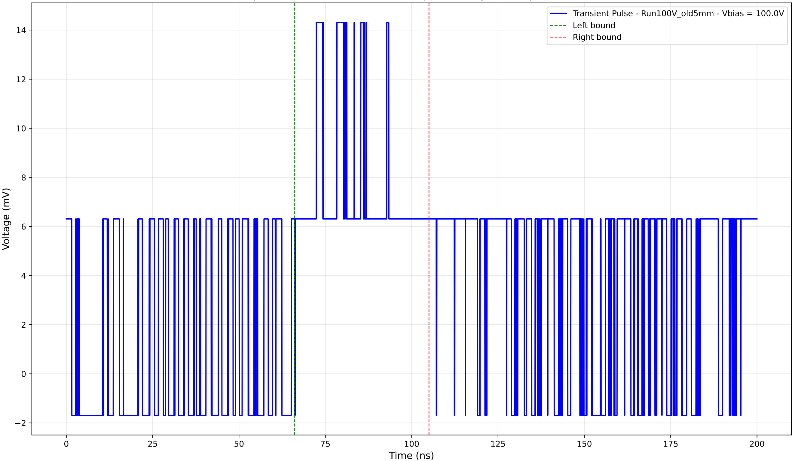
Transient Pulse - Sample: Old5mm - Position: 545.0 \mu\text{m} - Charge: 5.87 pC - Rise Time: 0.00 ns (N/A)
