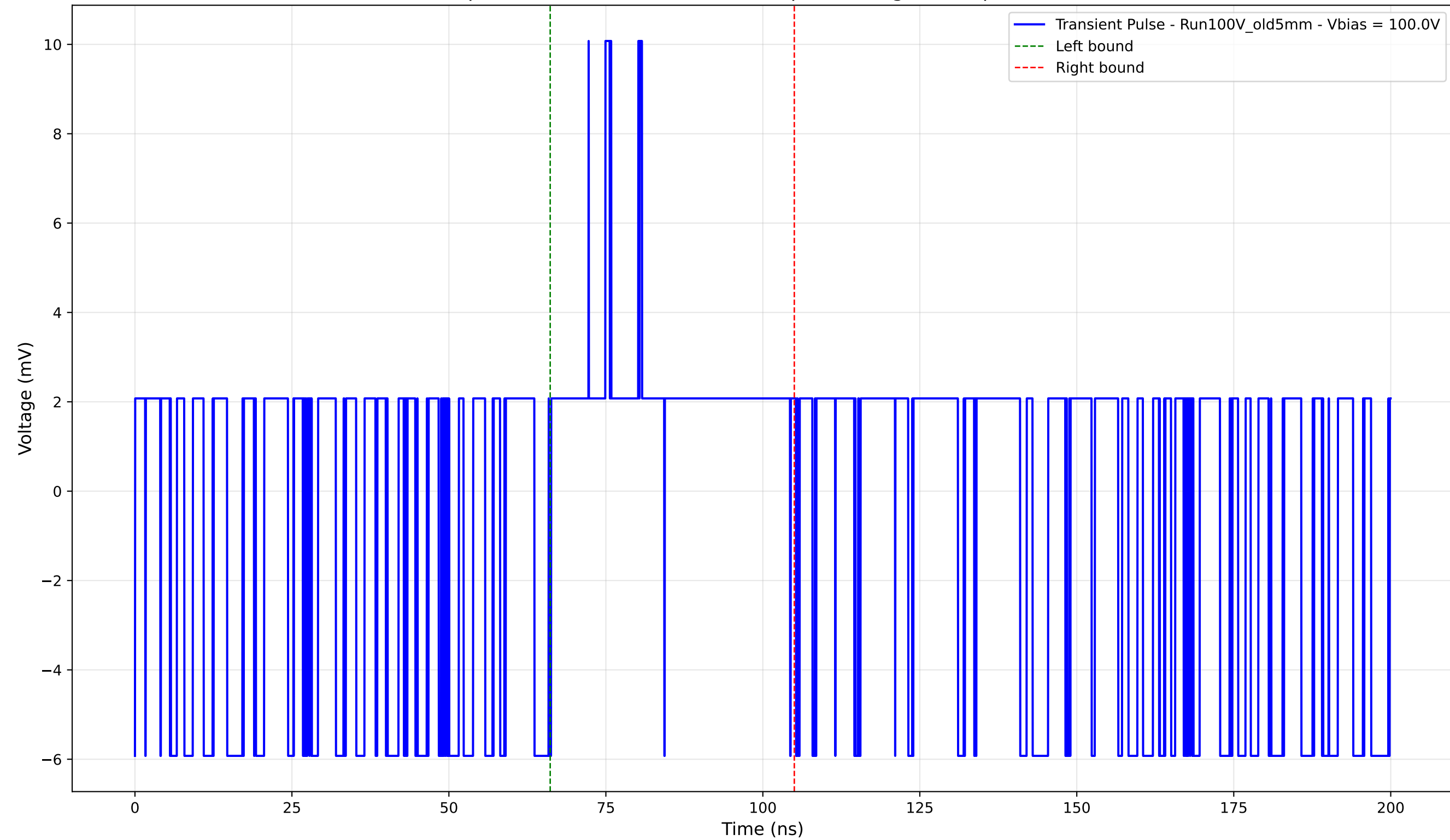
Transient Pulse - Sample: Old5mm - Position: 2540.0 \mu\text{m} - Charge: 1.79 pC - Rise Time: 0.00 ns (N/A)
