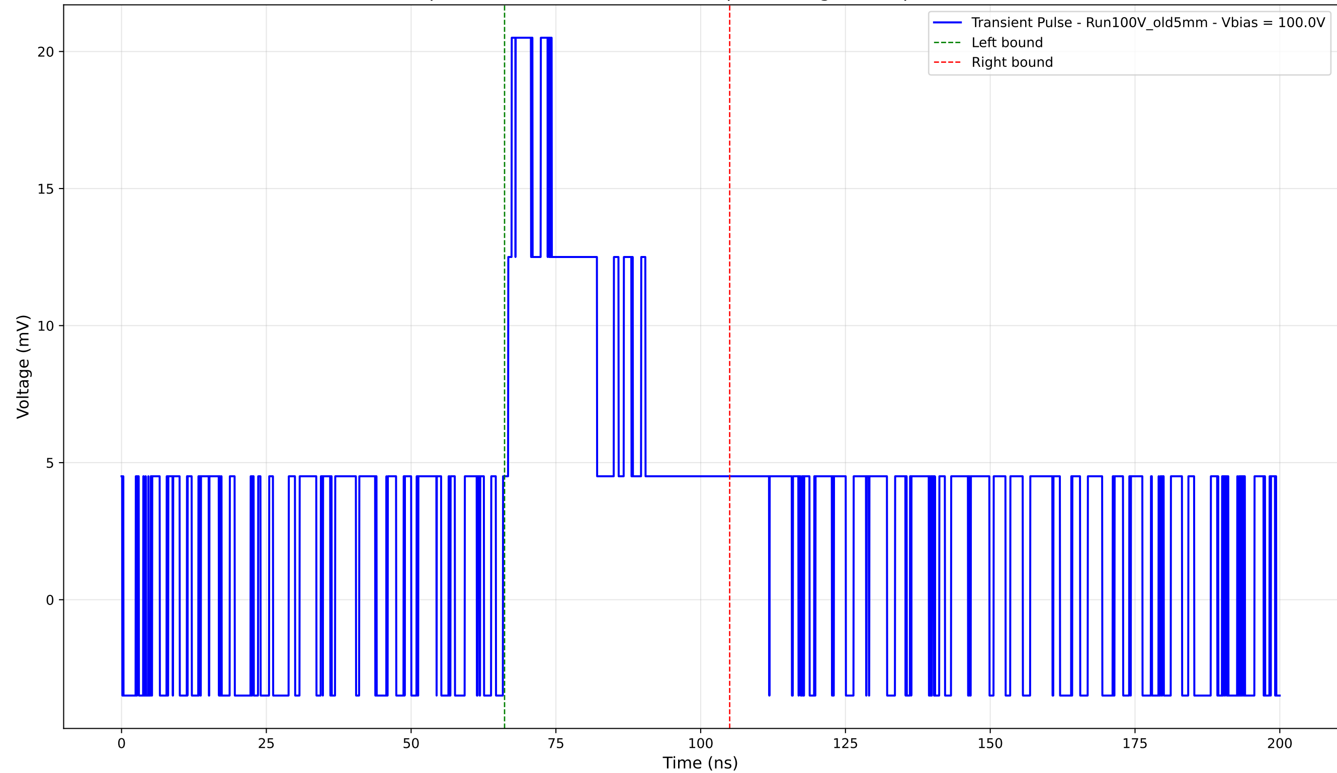
Transient Pulse - Sample: Old5mm - Position: 4680.0 \mu\text{m} - Charge: 7.26 pC - Rise Time: 0.00 ns (N/A)
