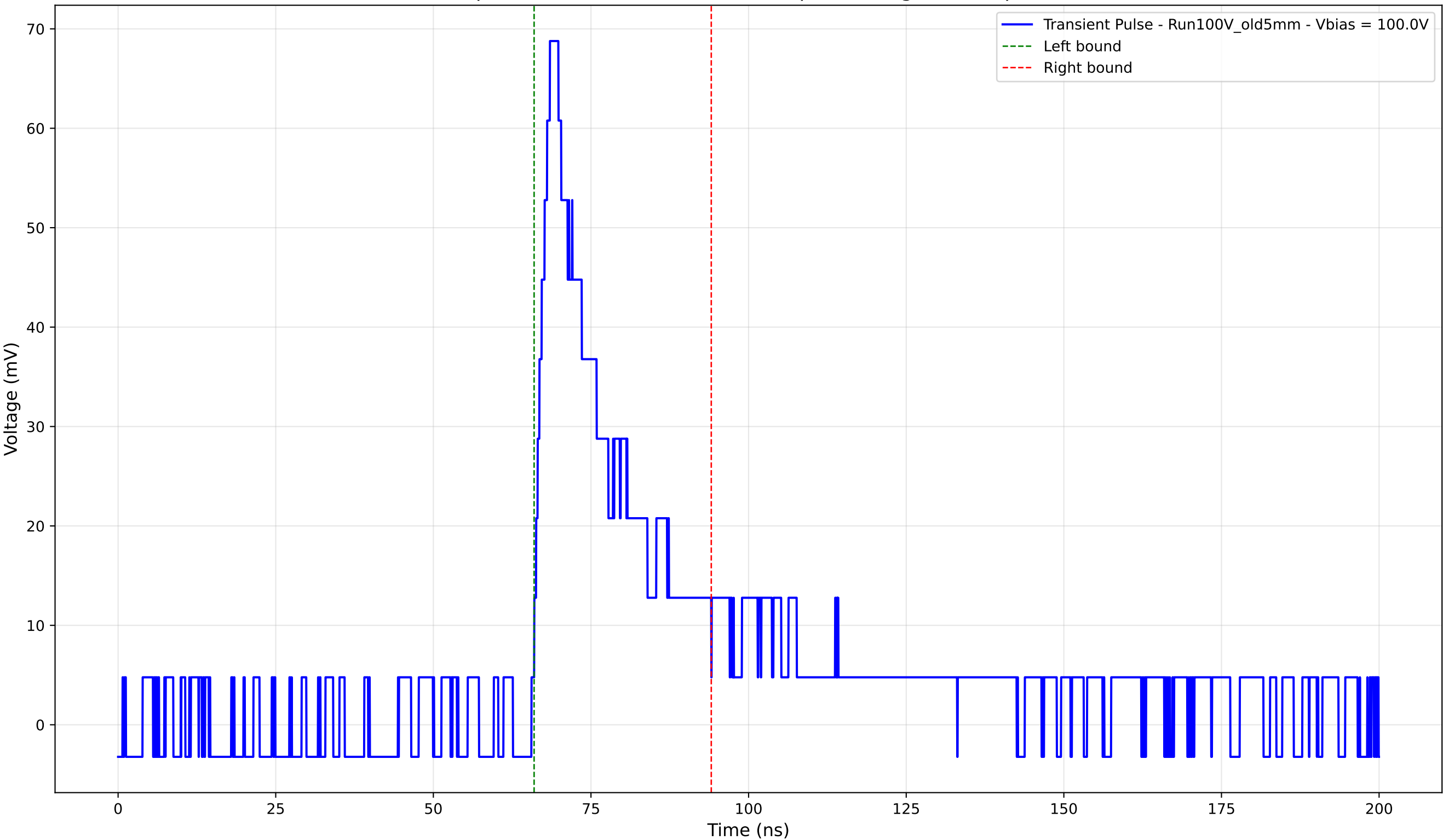
Transient Pulse - Sample: Old5mm - Position: 2945.0 \mu\text{m} - Charge: 16.05 pC - Rise Time: 2.49 ns
