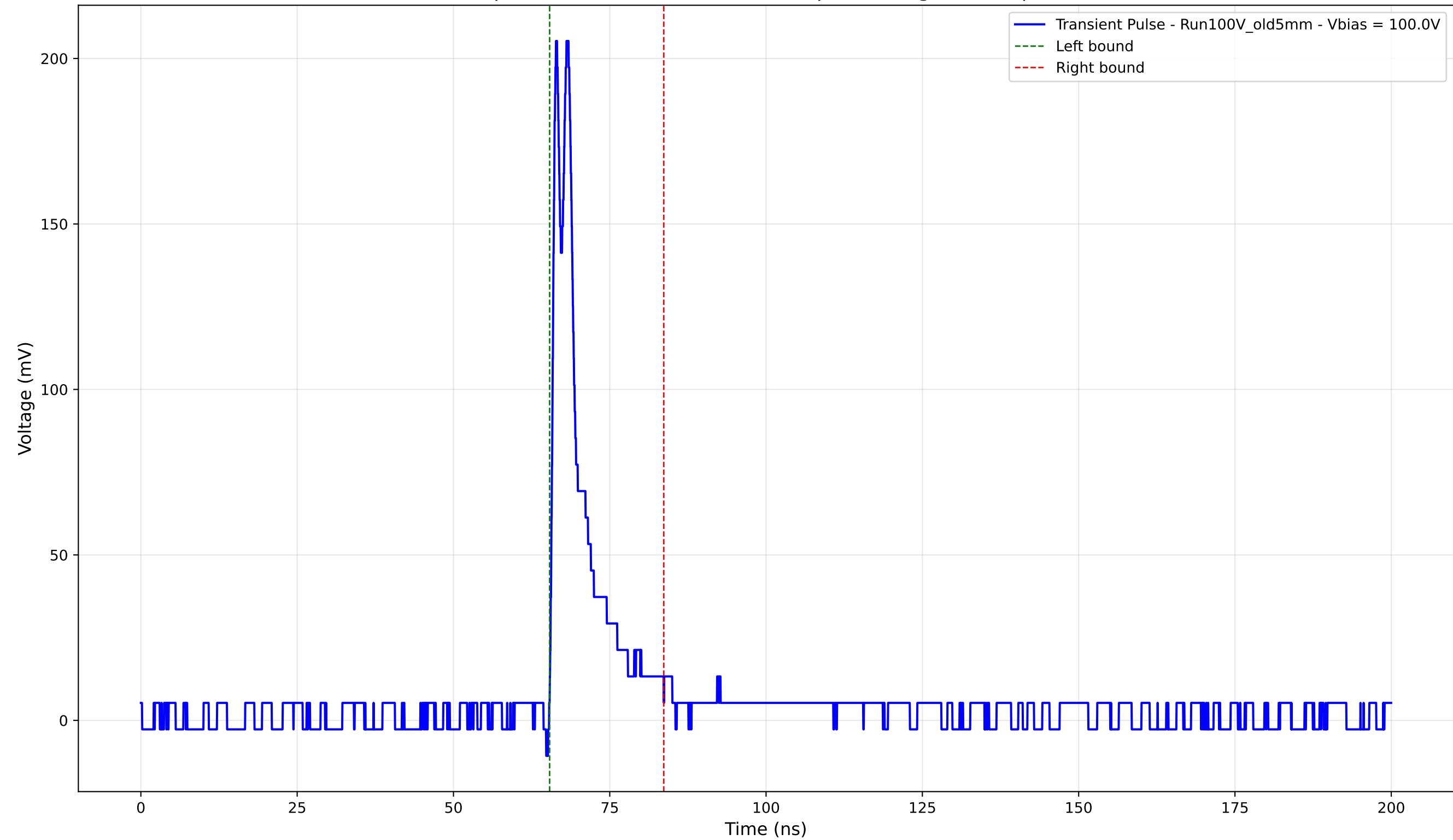
Transient Pulse - Sample: Old5mm - Position: 3585.0 \mu\text{m} - Charge: 21.16 pC - Rise Time: 0.78 ns
