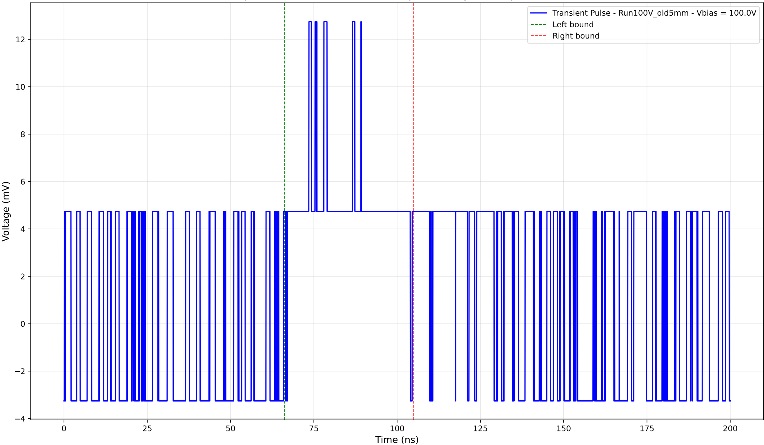
Transient Pulse - Sample: Old5mm - Position: 540.0 \mu\text{m} - Charge: 4.03 pC - Rise Time: 0.00 ns (N/A)
