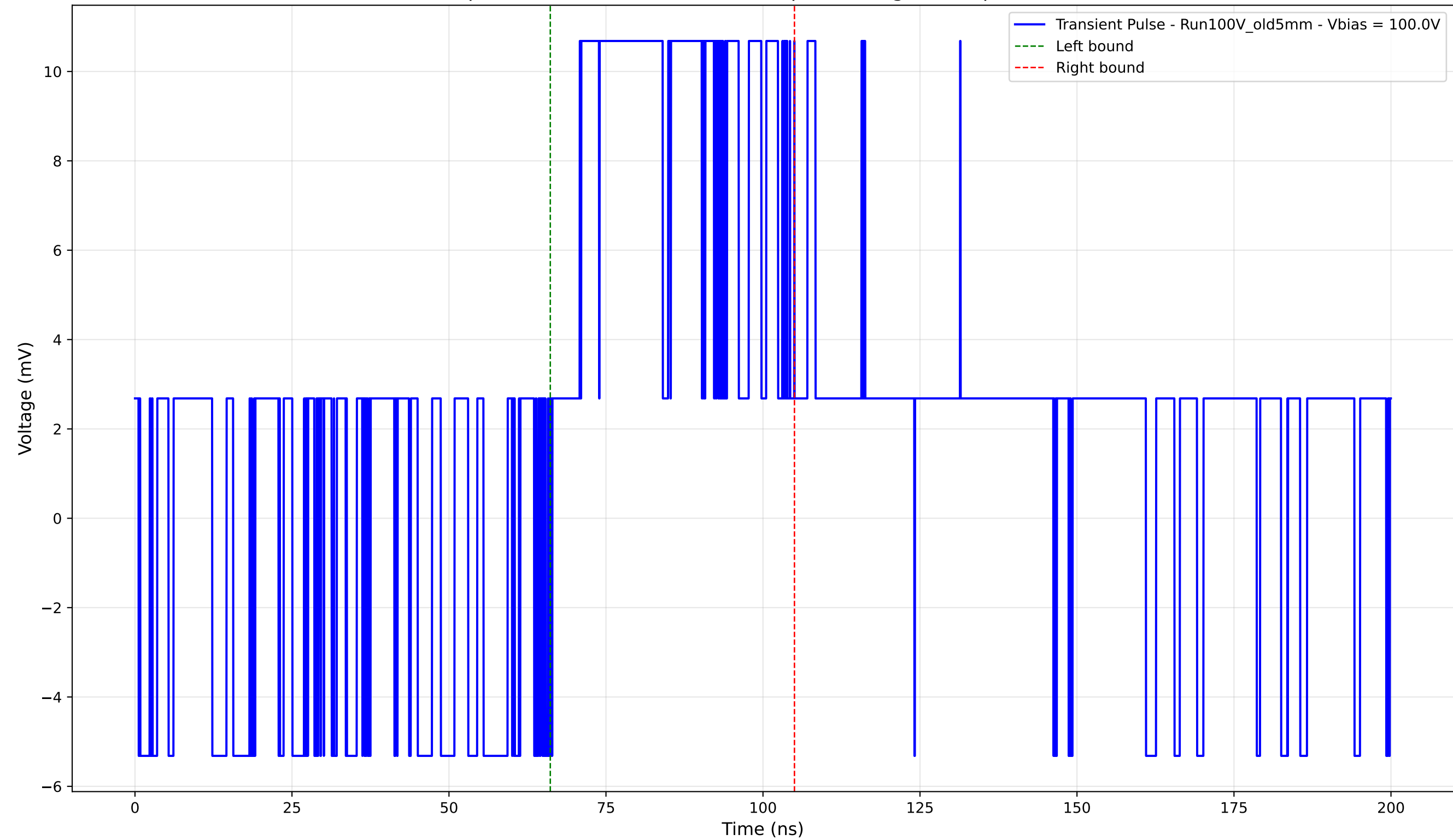
Transient Pulse - Sample: Old5mm - Position: 1655.0 \mu\text{m} - Charge: 6.40 pC - Rise Time: 0.00 ns (N/A)
