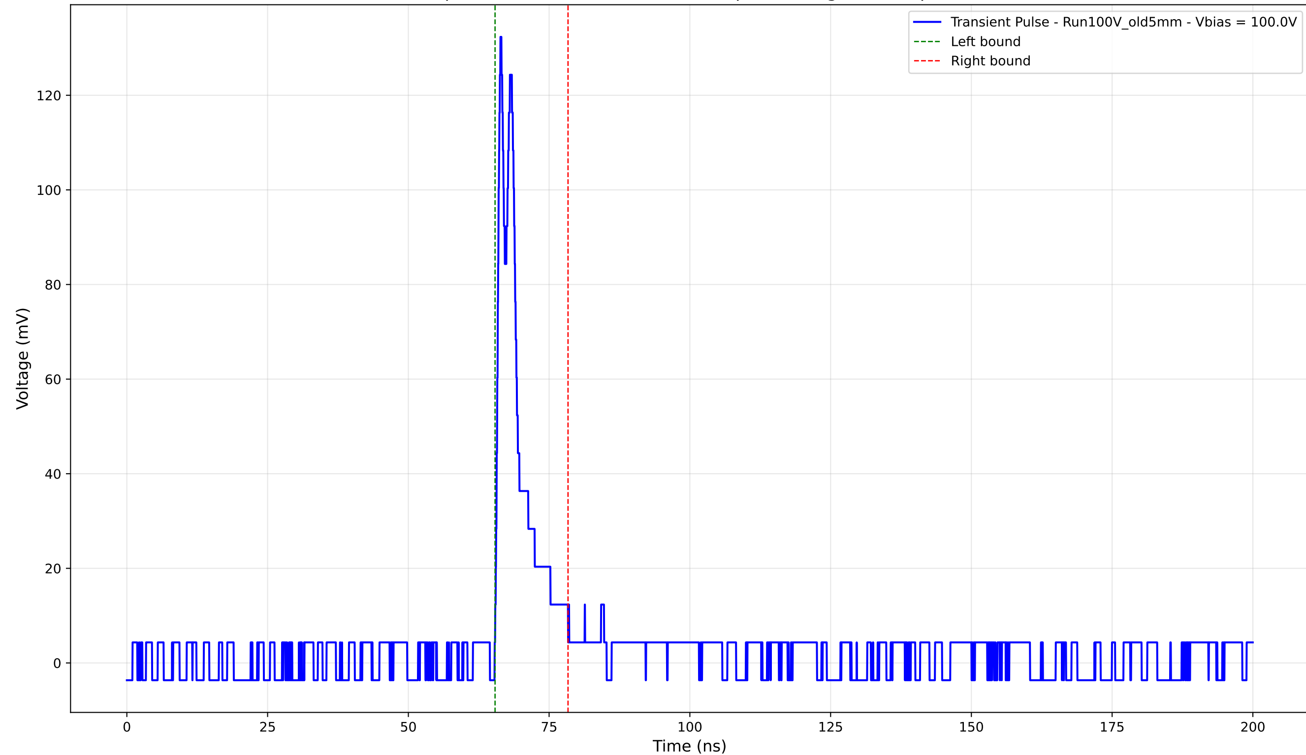
Transient Pulse - Sample: Old5mm - Position: 3635.0 \mu\text{m} - Charge: 11.46 pC - Rise Time: 0.74 ns
