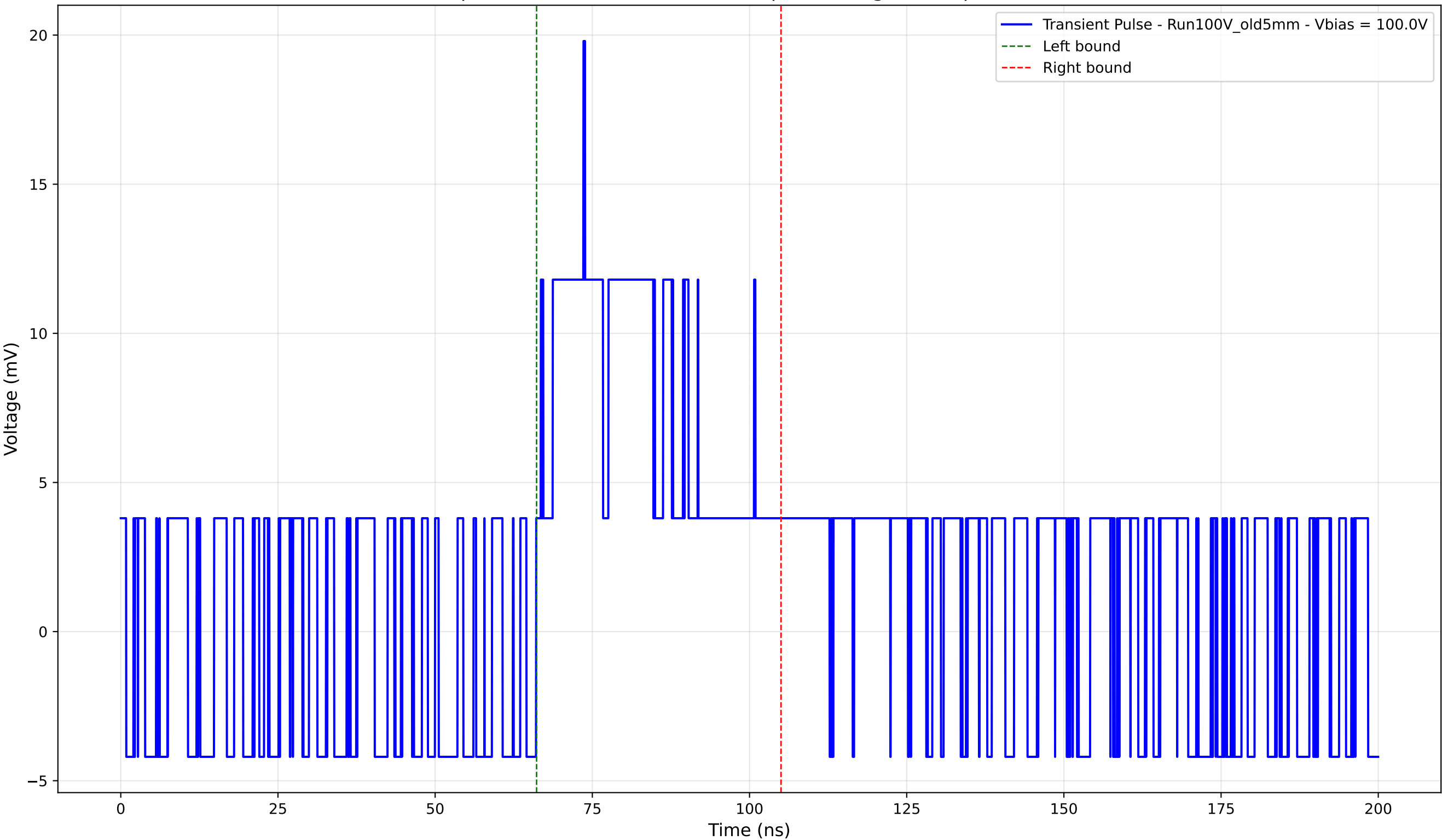
Transient Pulse - Sample: Old5mm - Position: 350.0 \mu\text{m} - Charge: 5.88 pC - Rise Time: 0.00 ns (N/A)
