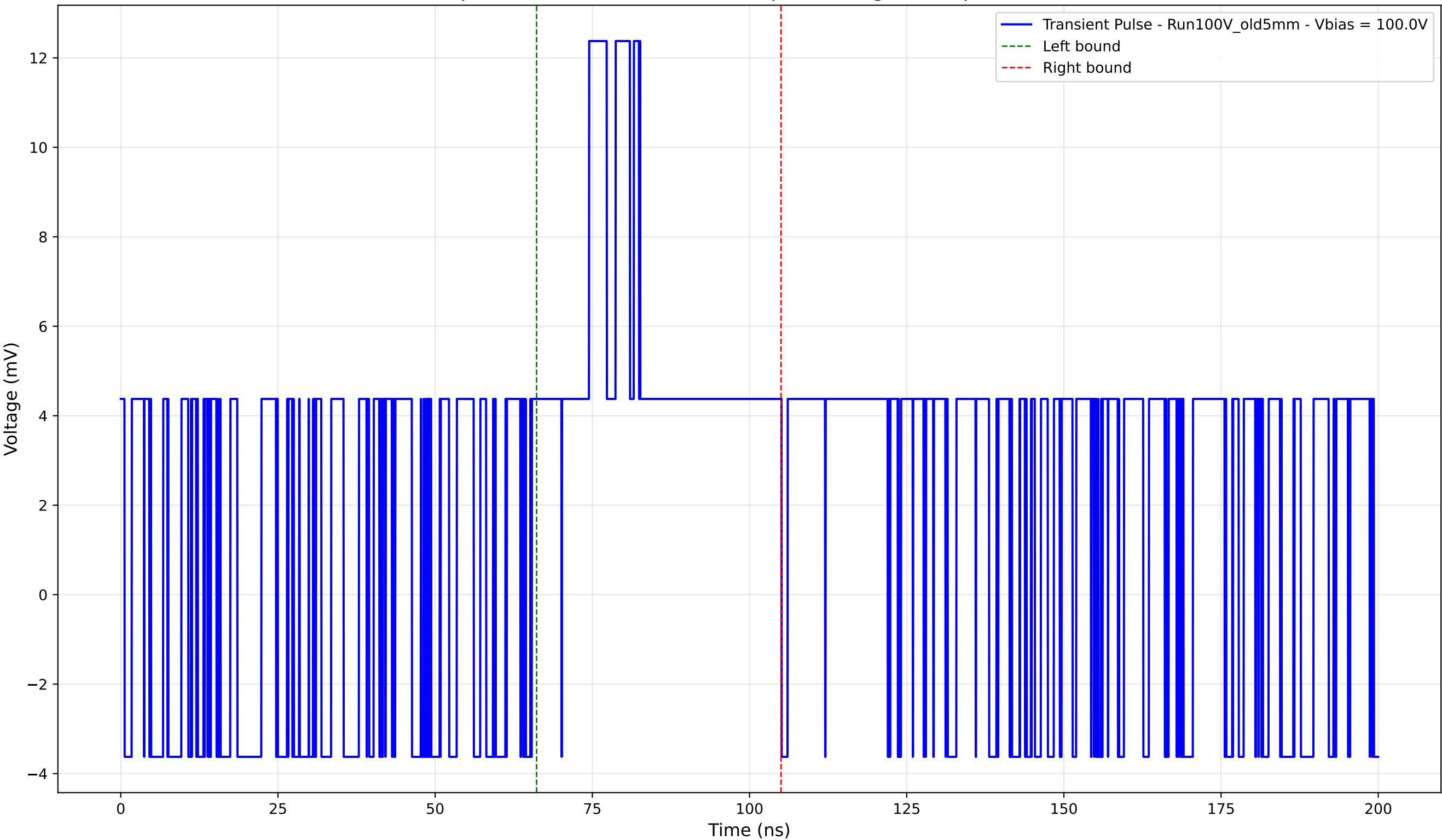
Transient Pulse - Sample: Old5mm - Position: 945.0 \mu\text{m} - Charge: 4.34 pC - Rise Time: 0.00 ns (N/A)
