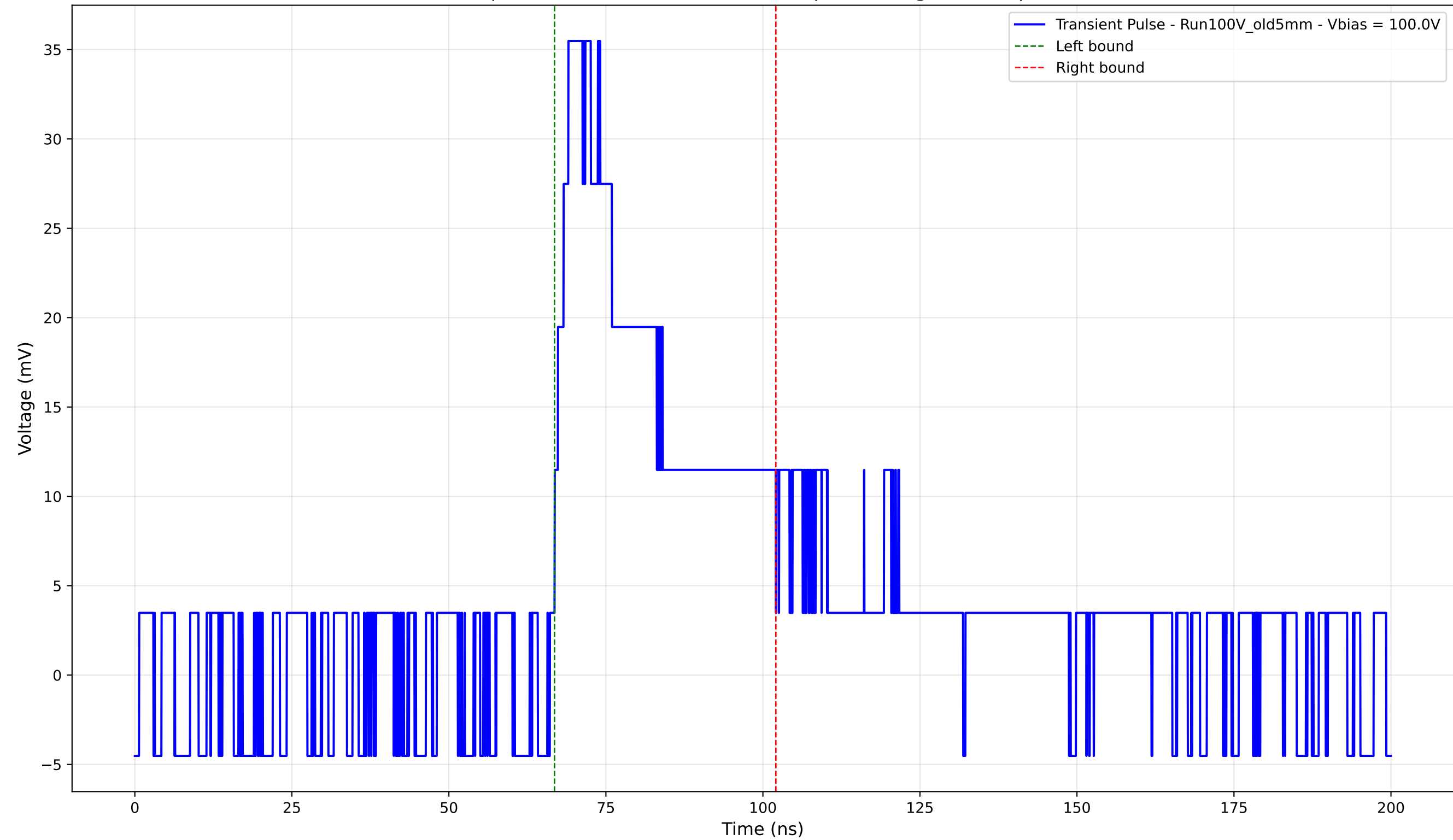
Transient Pulse - Sample: Old5mm - Position: 2600.0 \mu\text{m} - Charge: 12.45 pC - Rise Time: 2.20 ns
