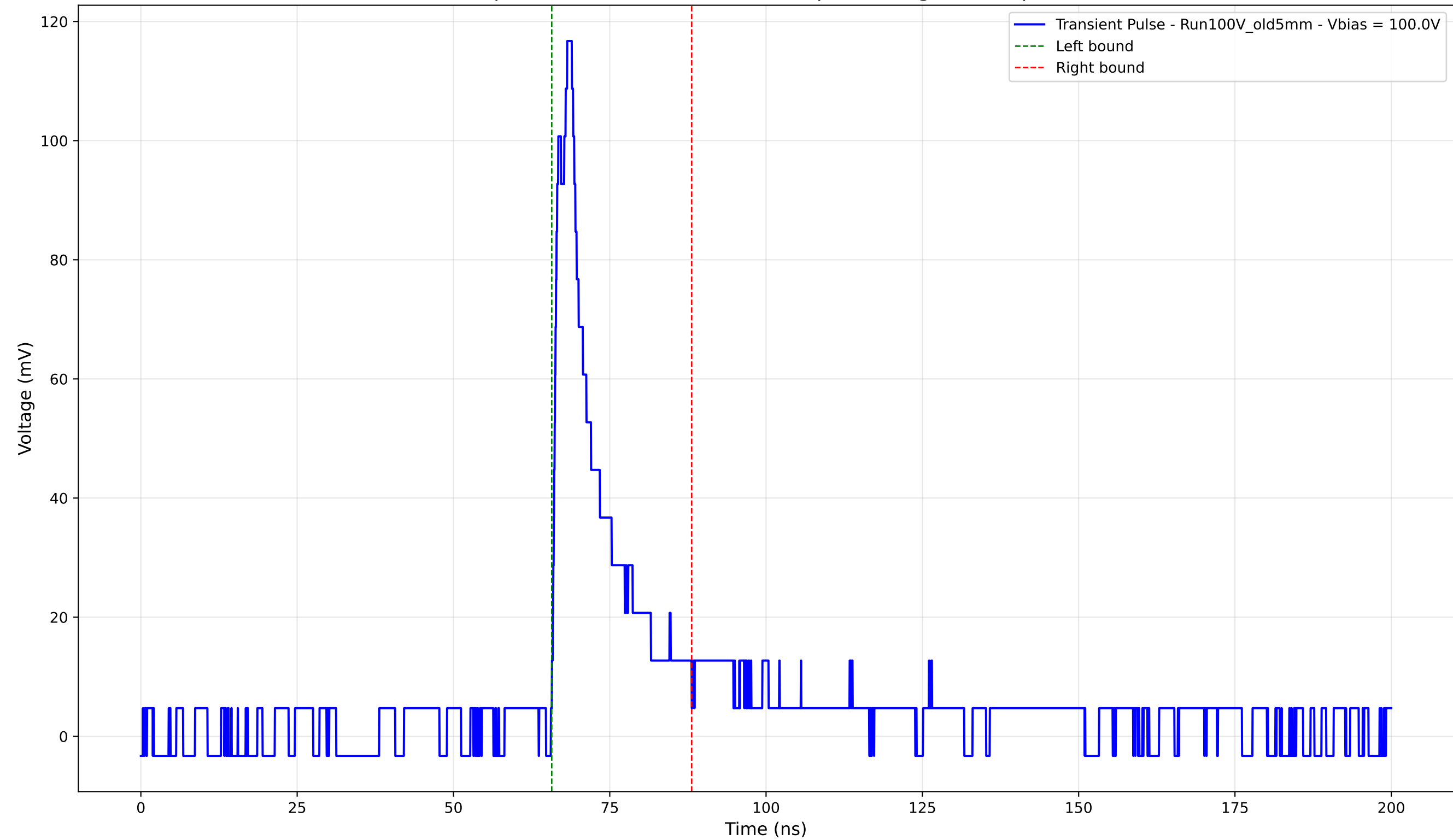
Transient Pulse - Sample: Old5mm - Position: 4130.0 \mu\text{m} - Charge: 17.49 pC - Rise Time: 2.20 ns
