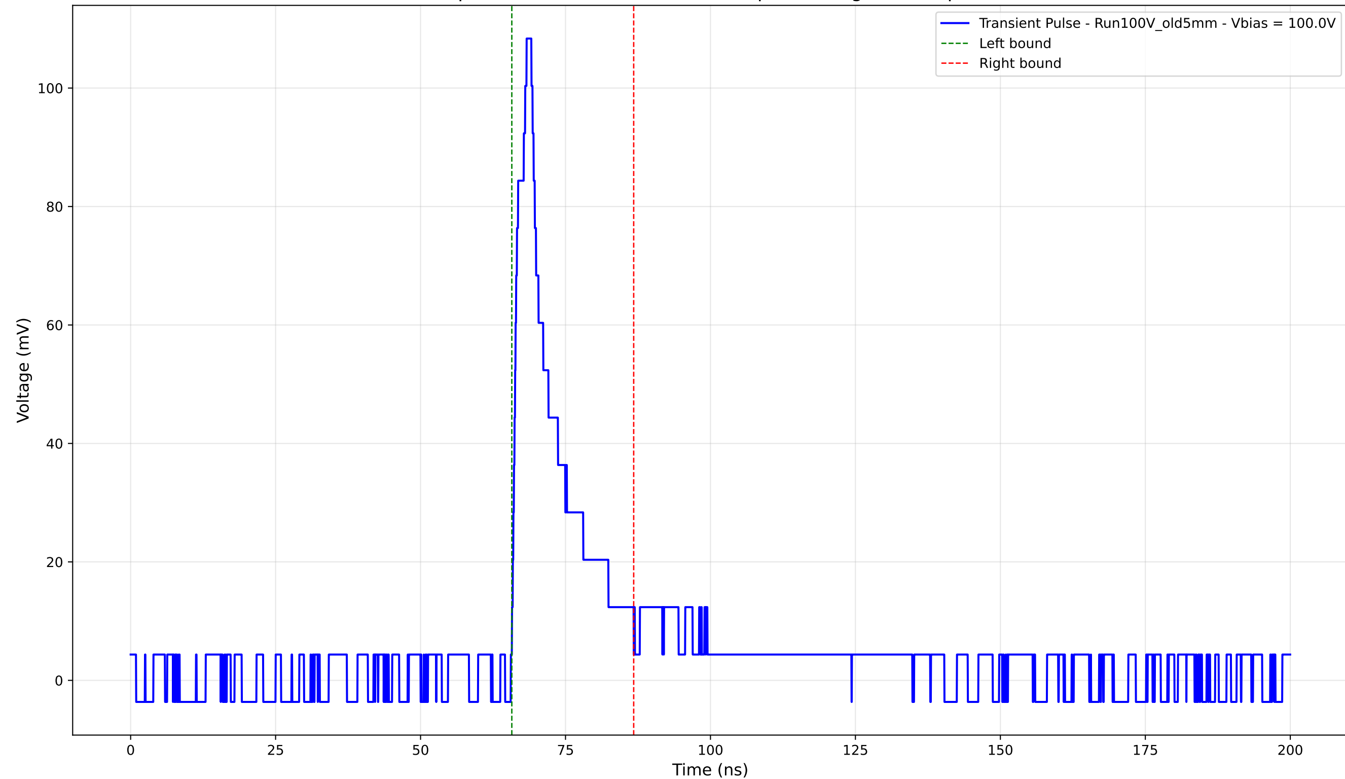
Transient Pulse - Sample: Old5mm - Position: 4170.0 \mu\text{m} - Charge: 16.30 pC - Rise Time: 2.28 ns
