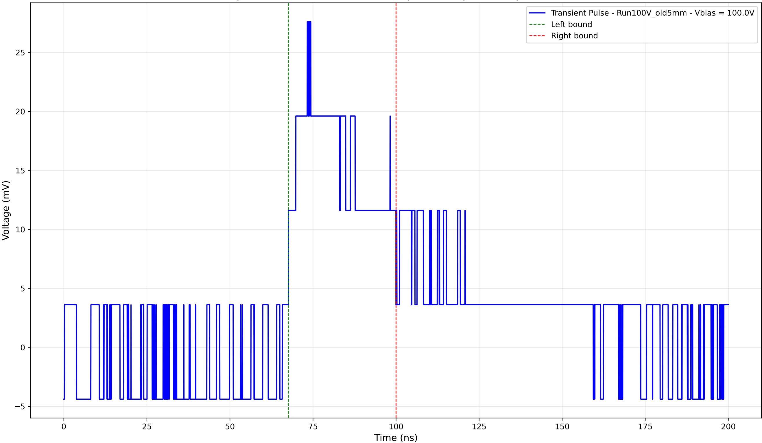
Transient Pulse - Sample: Old5mm - Position: 2225.0 \mu\text{m} - Charge: 10.26 pC - Rise Time: 0.00 ns (N/A)
