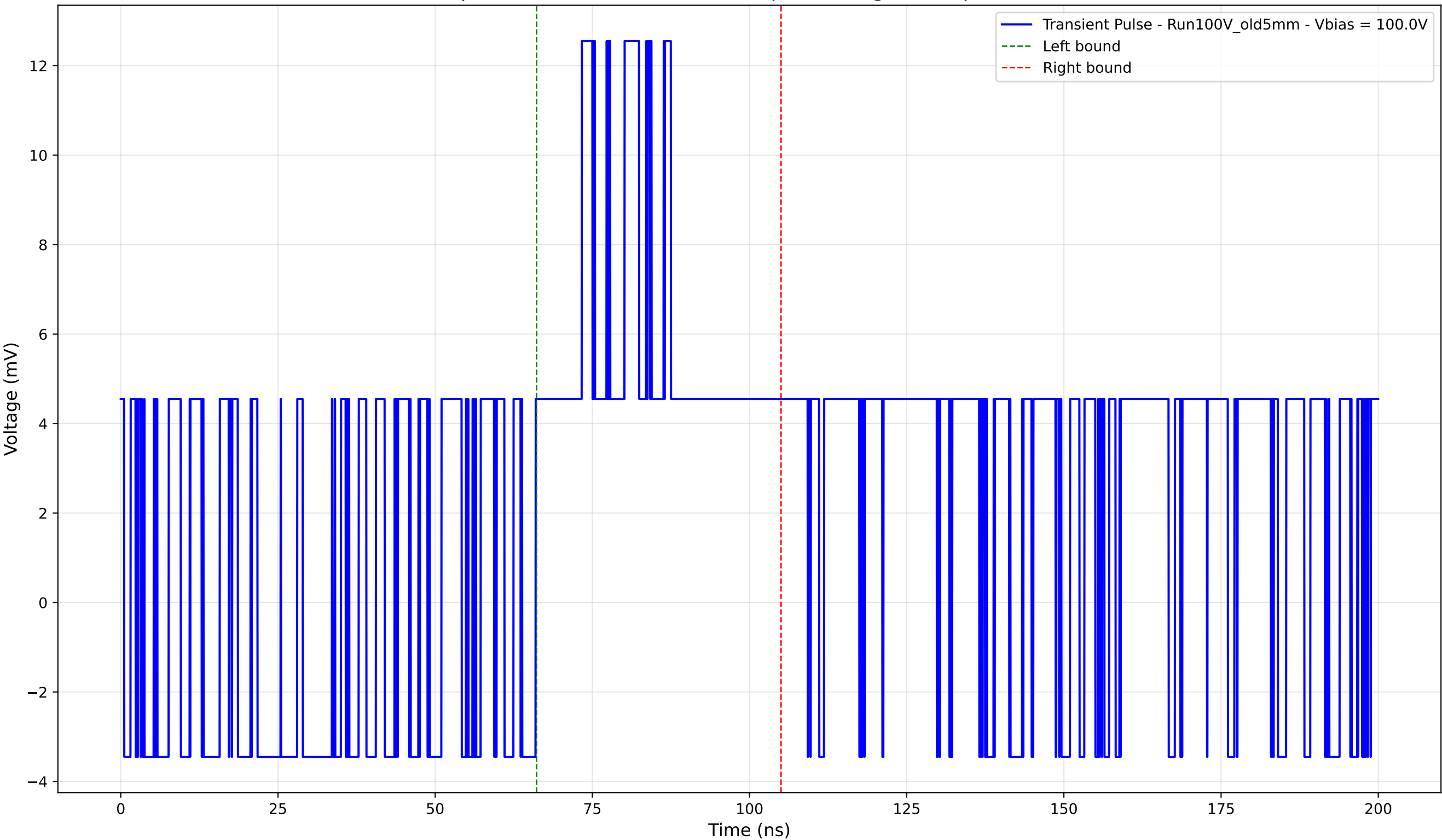
Transient Pulse - Sample: Old5mm - Position: 555.0 \mu\text{m} - Charge: 4.52 pC - Rise Time: 0.00 ns (N/A)
