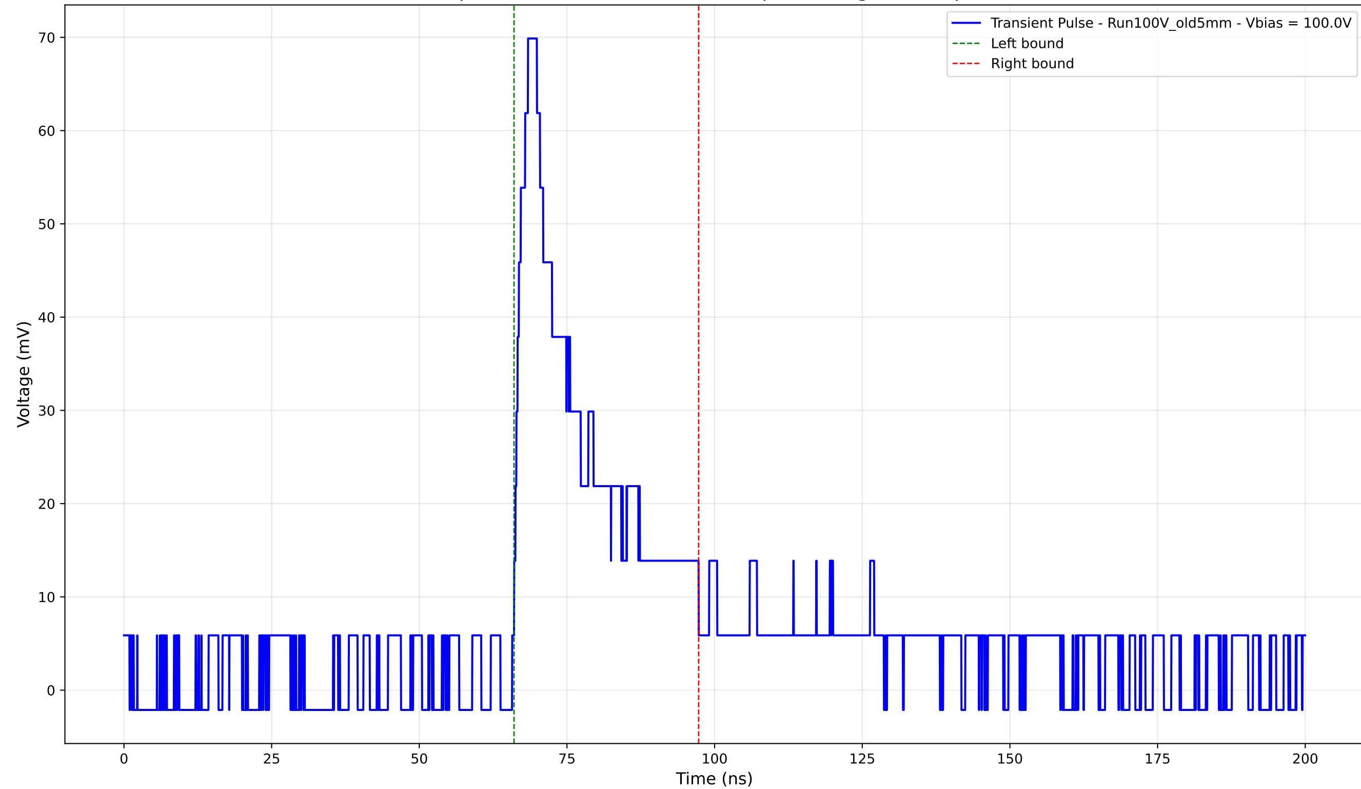
Transient Pulse - Sample: Old5mm - Position: 2975.0 \mu\text{m} - Charge: 17.34 pC - Rise Time: 2.36 ns
