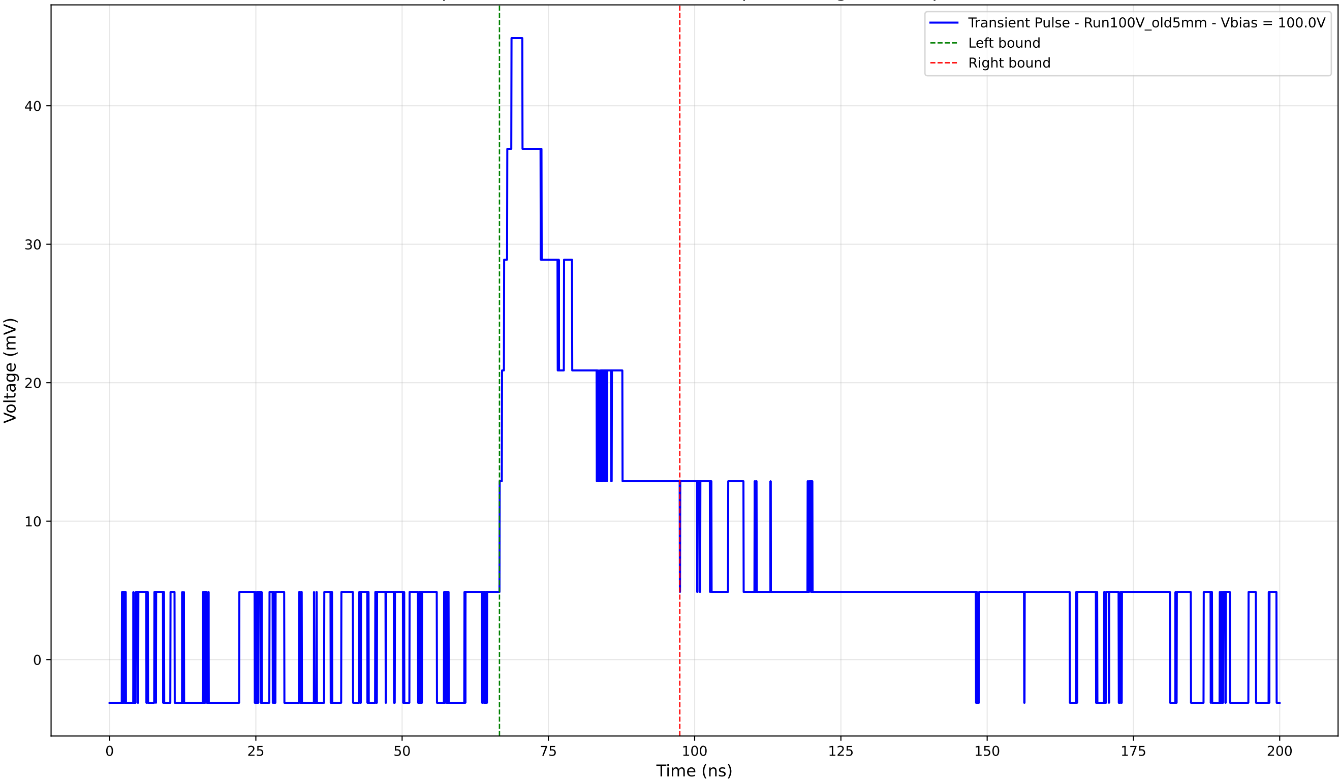
Transient Pulse - Sample: Old5mm - Position: 2675.0 \mu\text{m} - Charge: 14.03 pC - Rise Time: 4.16 ns
