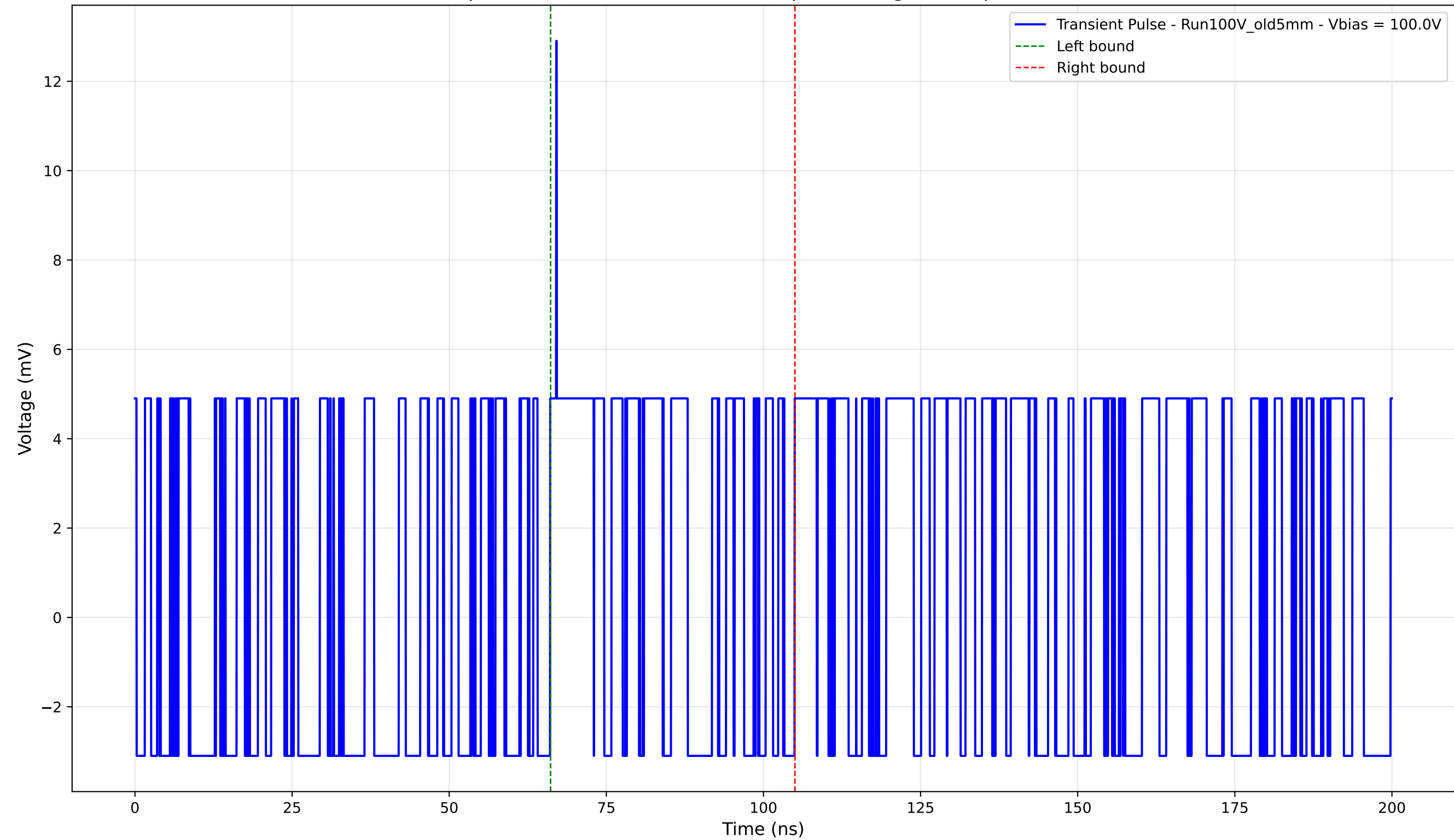
Transient Pulse - Sample: Old5mm - Position: 4285.0 \mu\text{m} - Charge: 1.54 pC - Rise Time: 0.00 ns (N/A)
