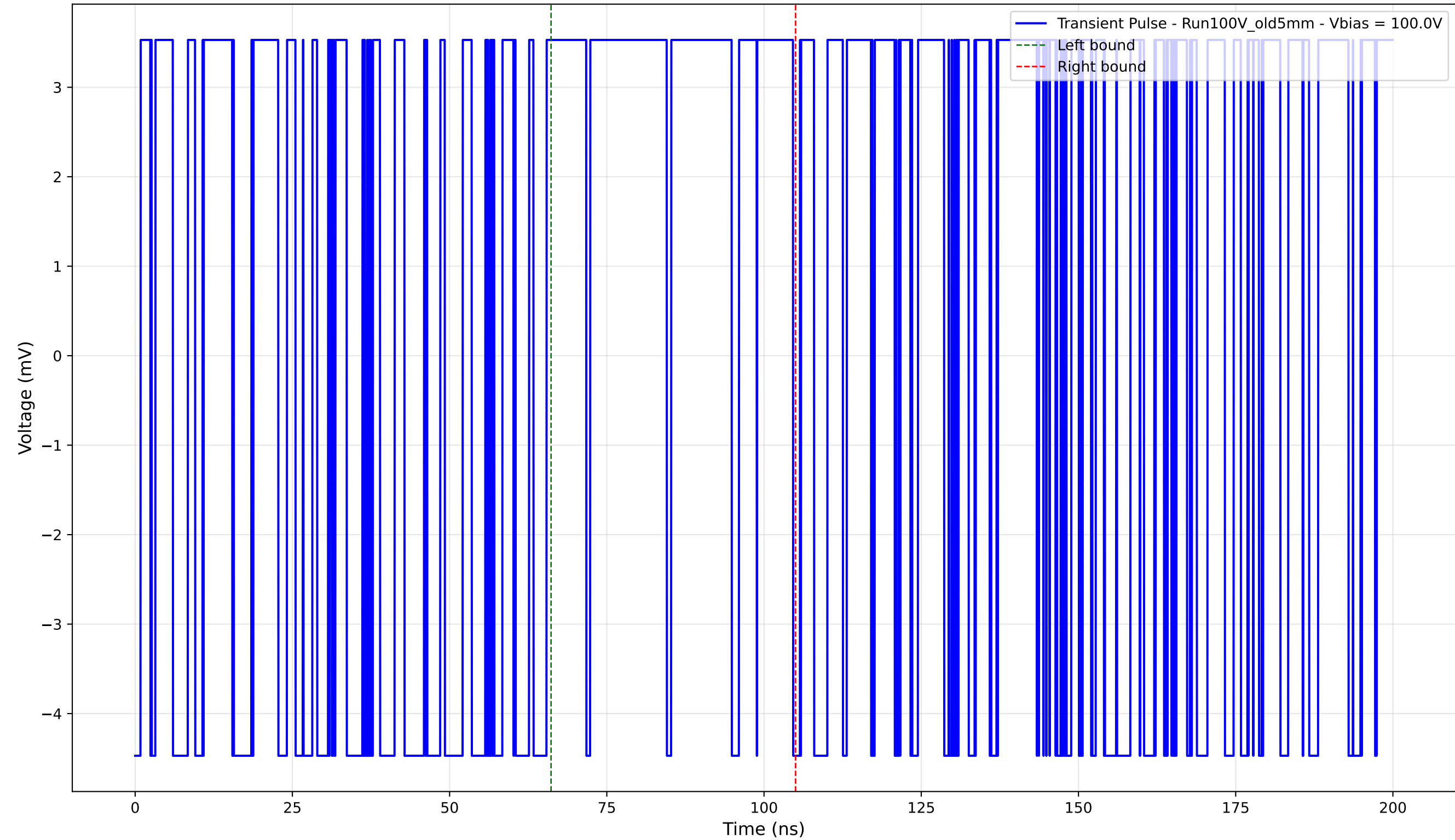
Transient Pulse - Sample: Old5mm - Position: 2105.0 \mu\text{m} - Charge: 2.27 pC - Rise Time: 0.00 ns (N/A)
