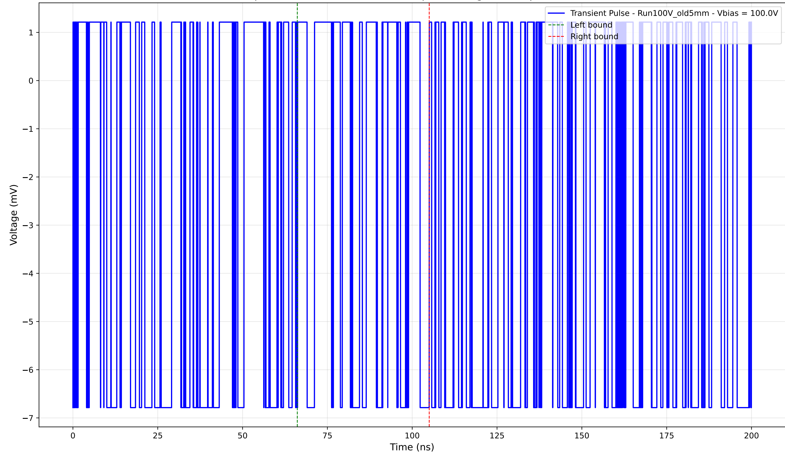
Transient Pulse - Sample: Old5mm - Position: 180.0 \mu\text{m} - Charge: -1.23 pC - Rise Time: 0.00 ns (N/A)
