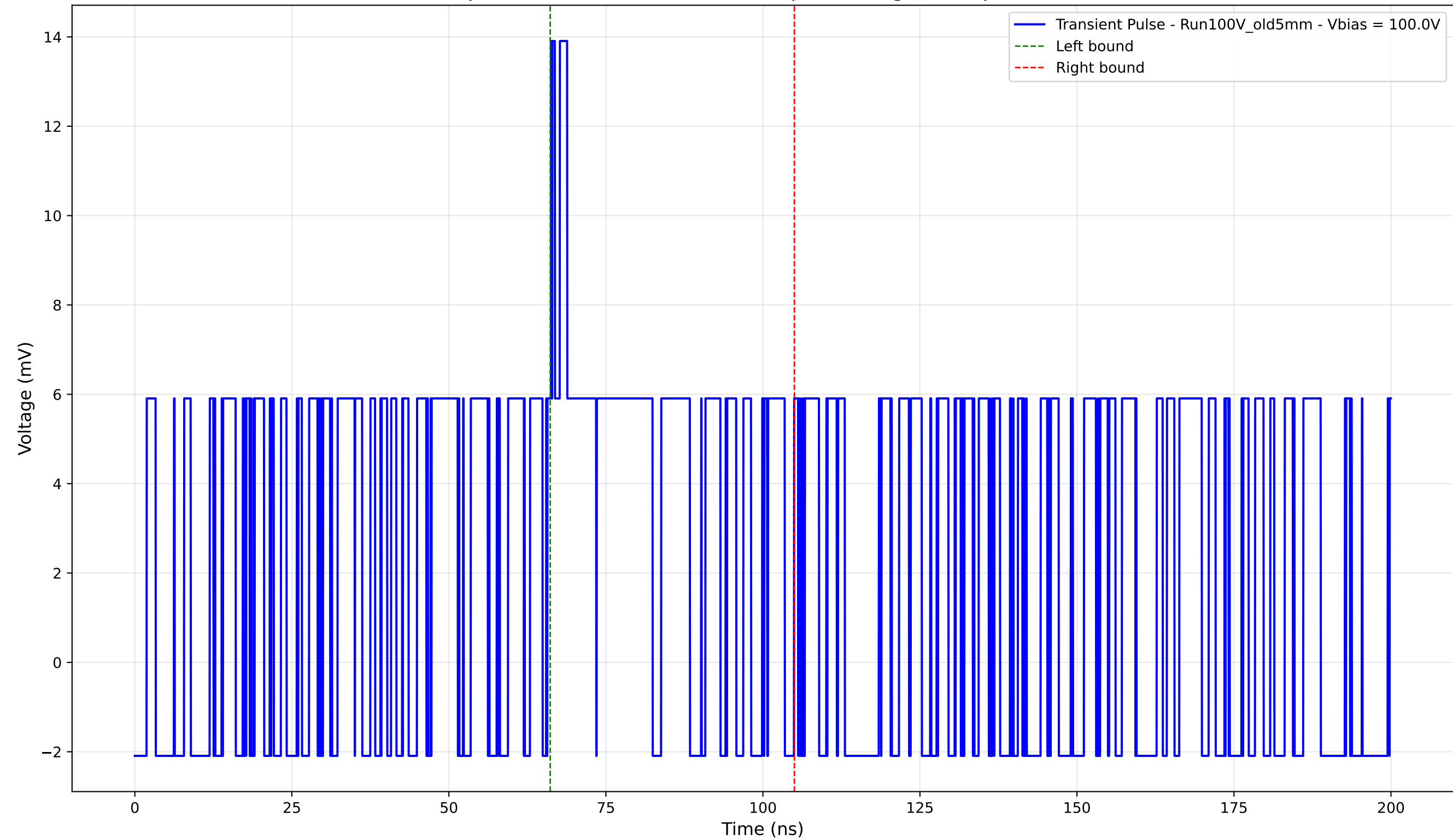
Transient Pulse - Sample: Old5mm - Position: 3995.0 \mu\text{m} - Charge: 3.37 pC - Rise Time: 0.00 ns (N/A)
