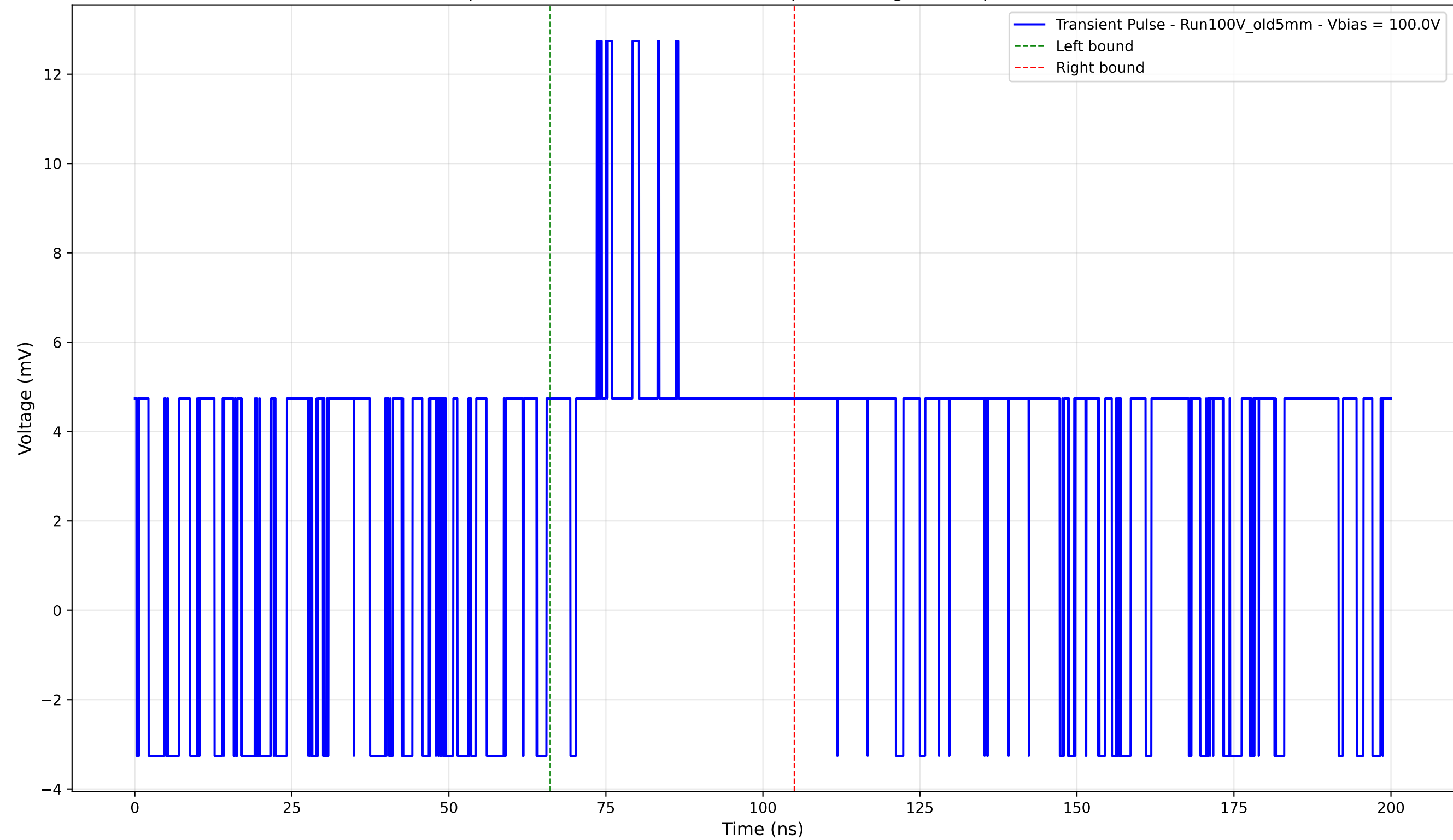
Transient Pulse - Sample: Old5mm - Position: 1030.0 \mu\text{m} - Charge: 4.03 pC - Rise Time: 0.00 ns (N/A)
