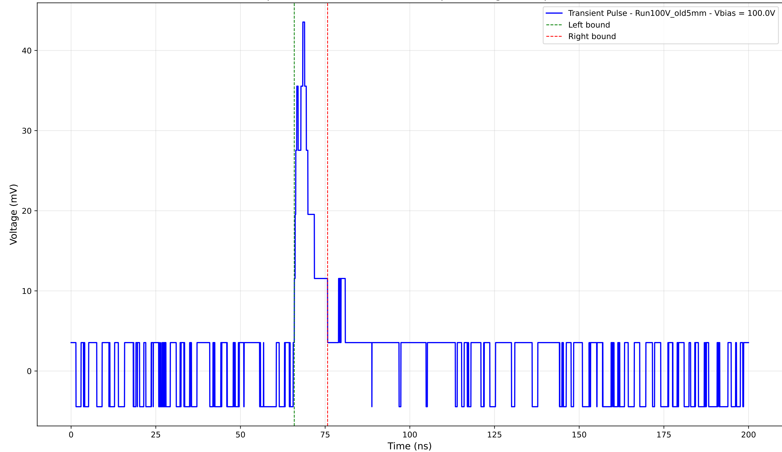
Transient Pulse - Sample: Old5mm - Position: 4065.0 \mu\text{m} - Charge: 4.16 pC - Rise Time: 2.52 ns
