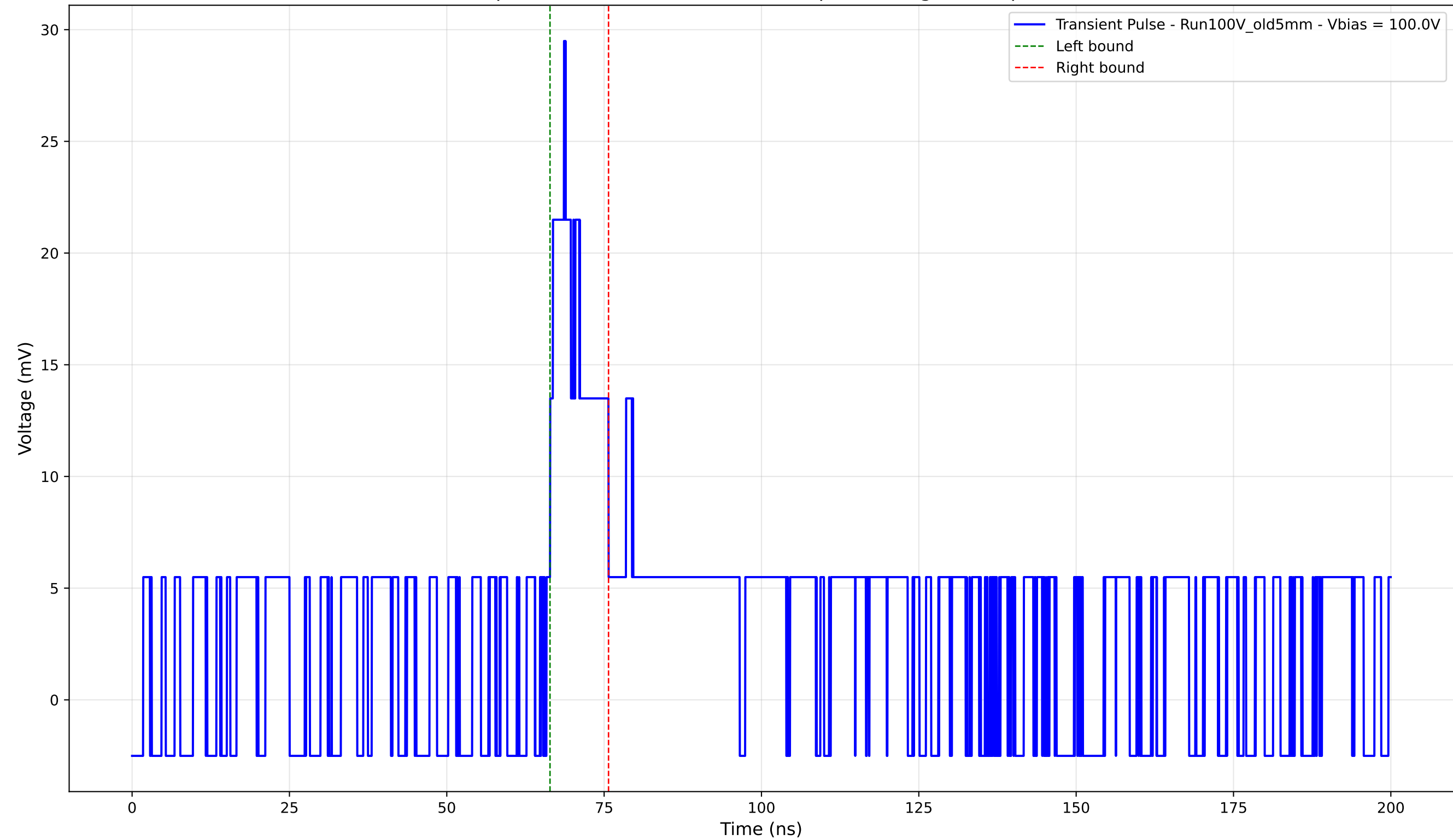
Transient Pulse - Sample: Old5mm - Position: 3150.0 \mu\text{m} - Charge: 3.10 pC - Rise Time: 2.80 ns
