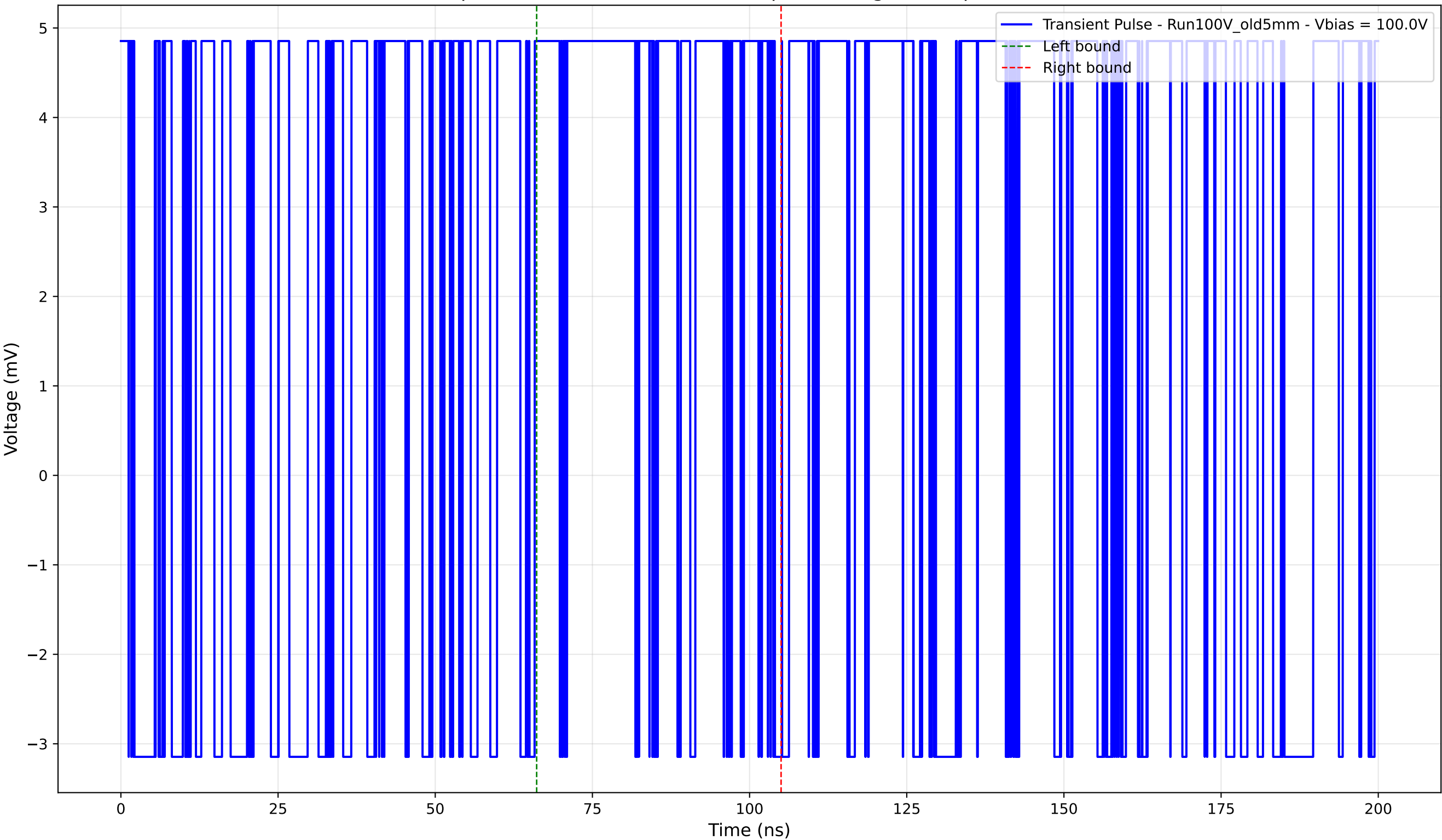
Transient Pulse - Sample: Old5mm - Position: 265.0 \mu\text{m} - Charge: 2.95 pC - Rise Time: 0.00 ns (N/A)
