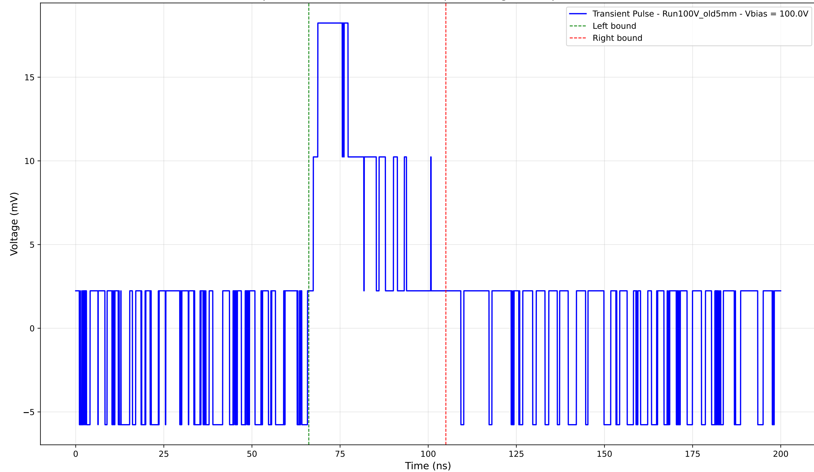
Transient Pulse - Sample: Old5mm - Position: 2570.0 \mu\text{m} - Charge: 6.51 pC - Rise Time: 0.00 ns (N/A)
