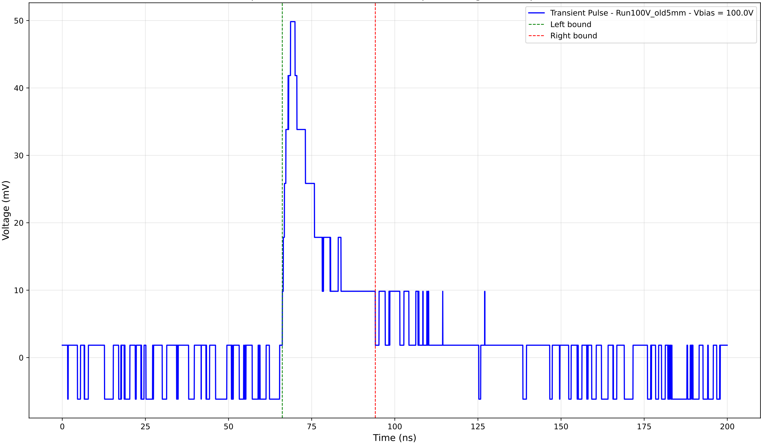
Transient Pulse - Sample: Old5mm - Position: 4520.0 \mu\text{m} - Charge: 10.86 pC - Rise Time: 2.47 ns
