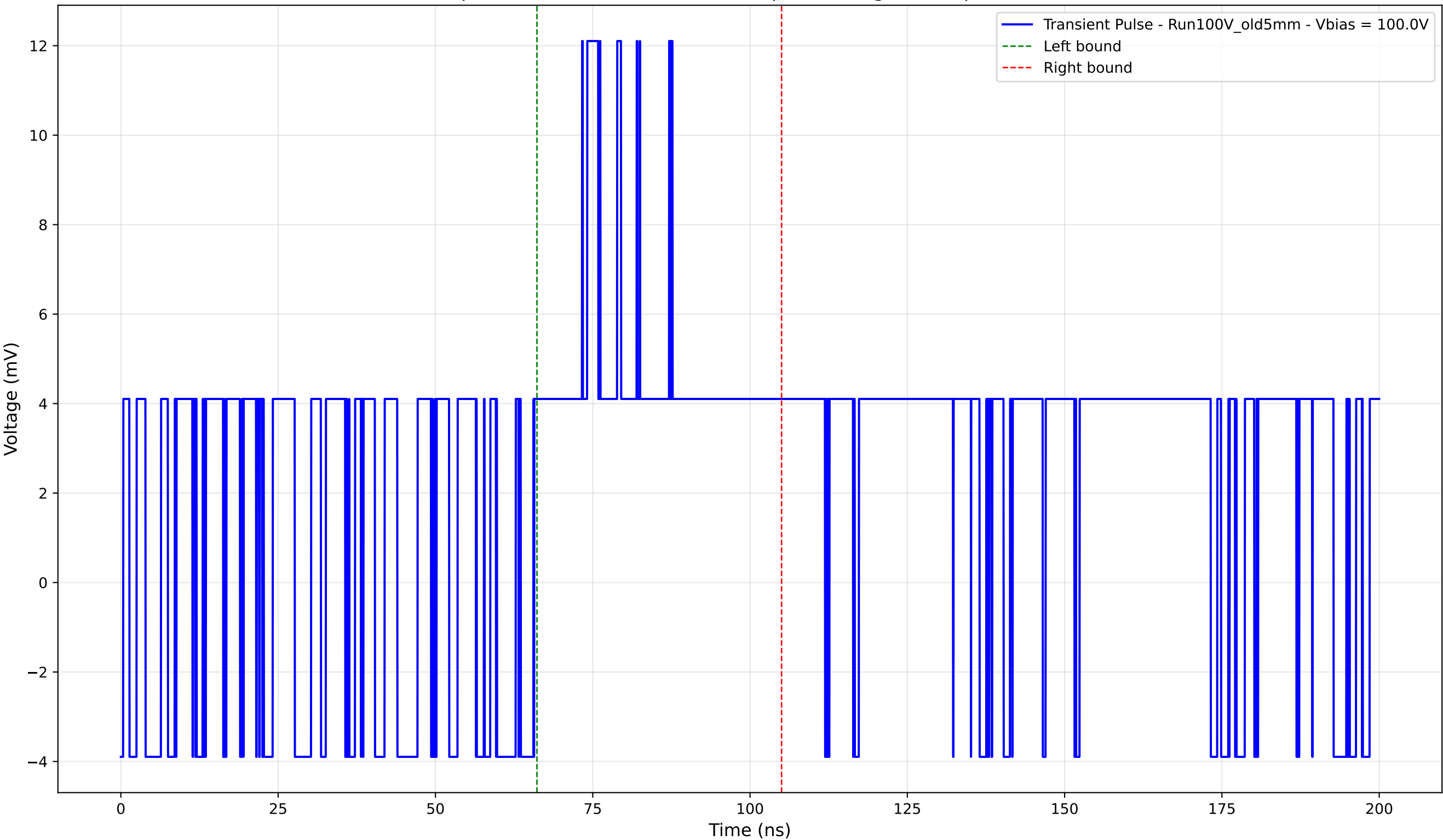
Transient Pulse - Sample: Old5mm - Position: 935.0 \mu\text{m} - Charge: 3.68 pC - Rise Time: 0.00 ns (N/A)
