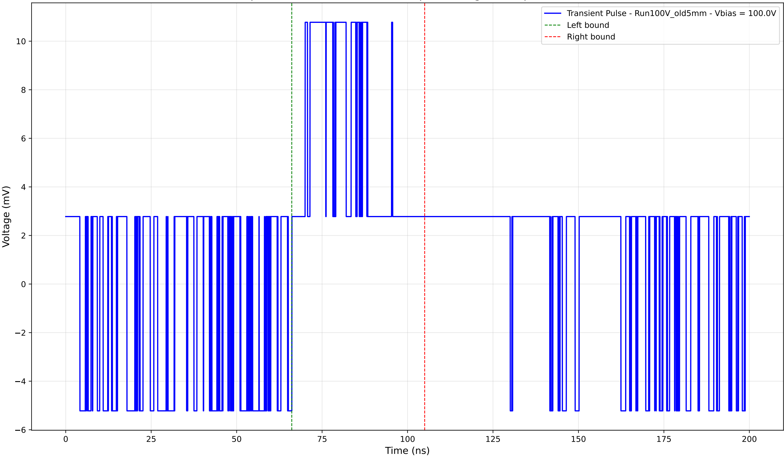
Transient Pulse - Sample: Old5mm - Position: 665.0 \mu\text{m} - Charge: 4.55 pC - Rise Time: 0.00 ns (N/A)
