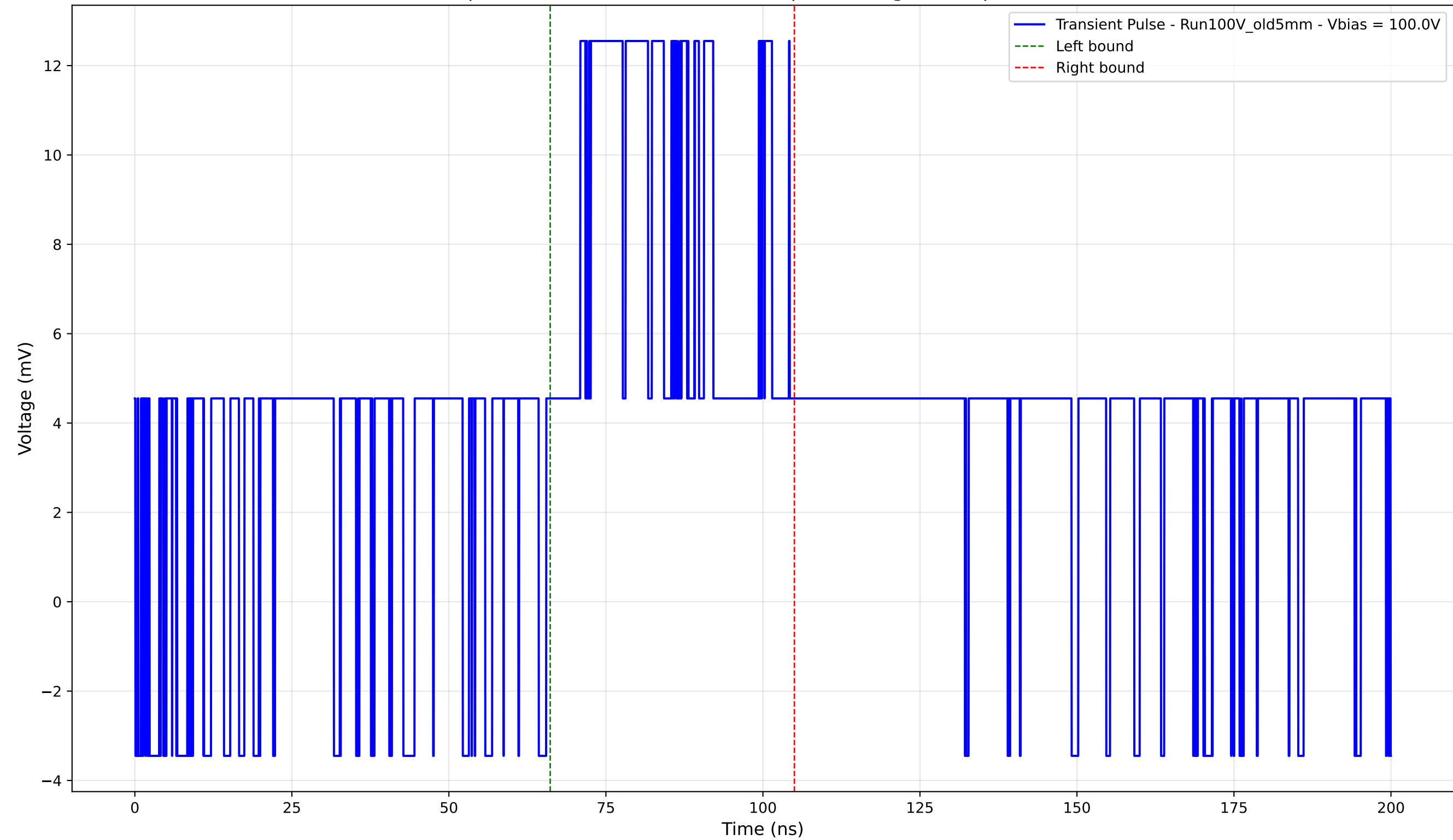
Transient Pulse - Sample: Old5mm - Position: 1560.0 \mu\text{m} - Charge: 6.35 pC - Rise Time: 0.00 ns (N/A)
