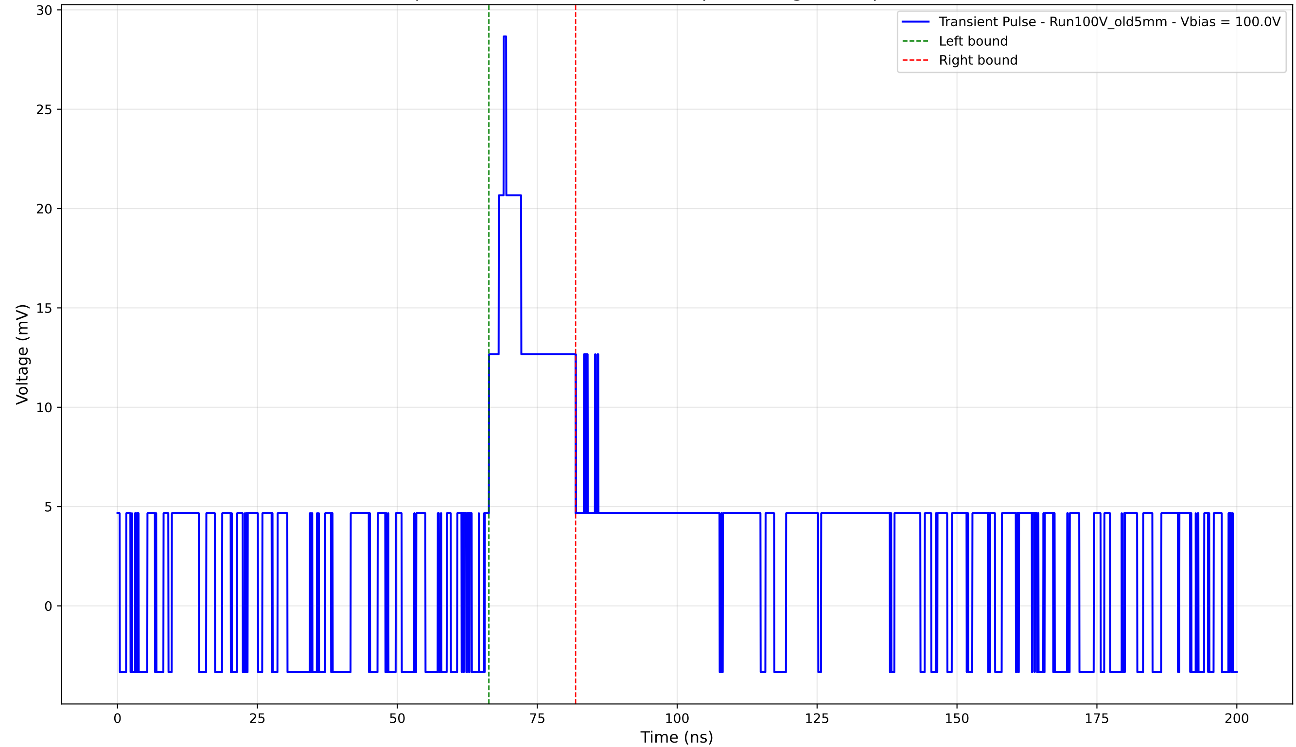
Transient Pulse - Sample: Old5mm - Position: 2860.0 \mu\text{m} - Charge: 4.64 pC - Rise Time: 0.00 ns (N/A)
