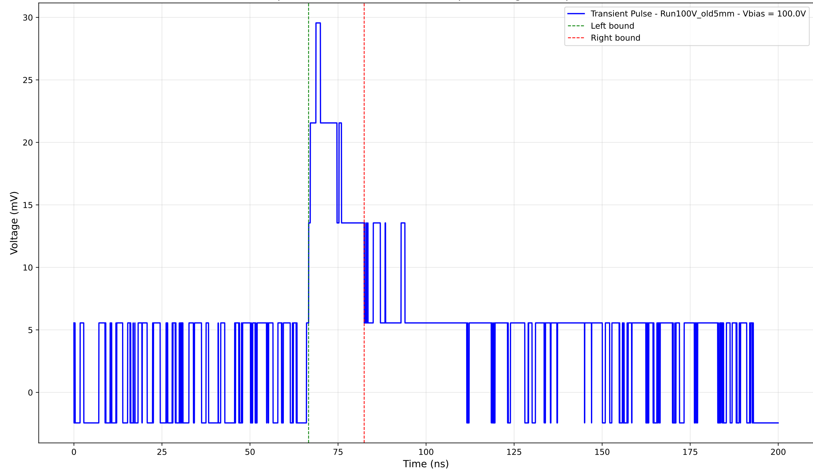
Transient Pulse - Sample: Old5mm - Position: 2865.0 \mu\text{m} - Charge: 5.80 pC - Rise Time: 2.70 ns
