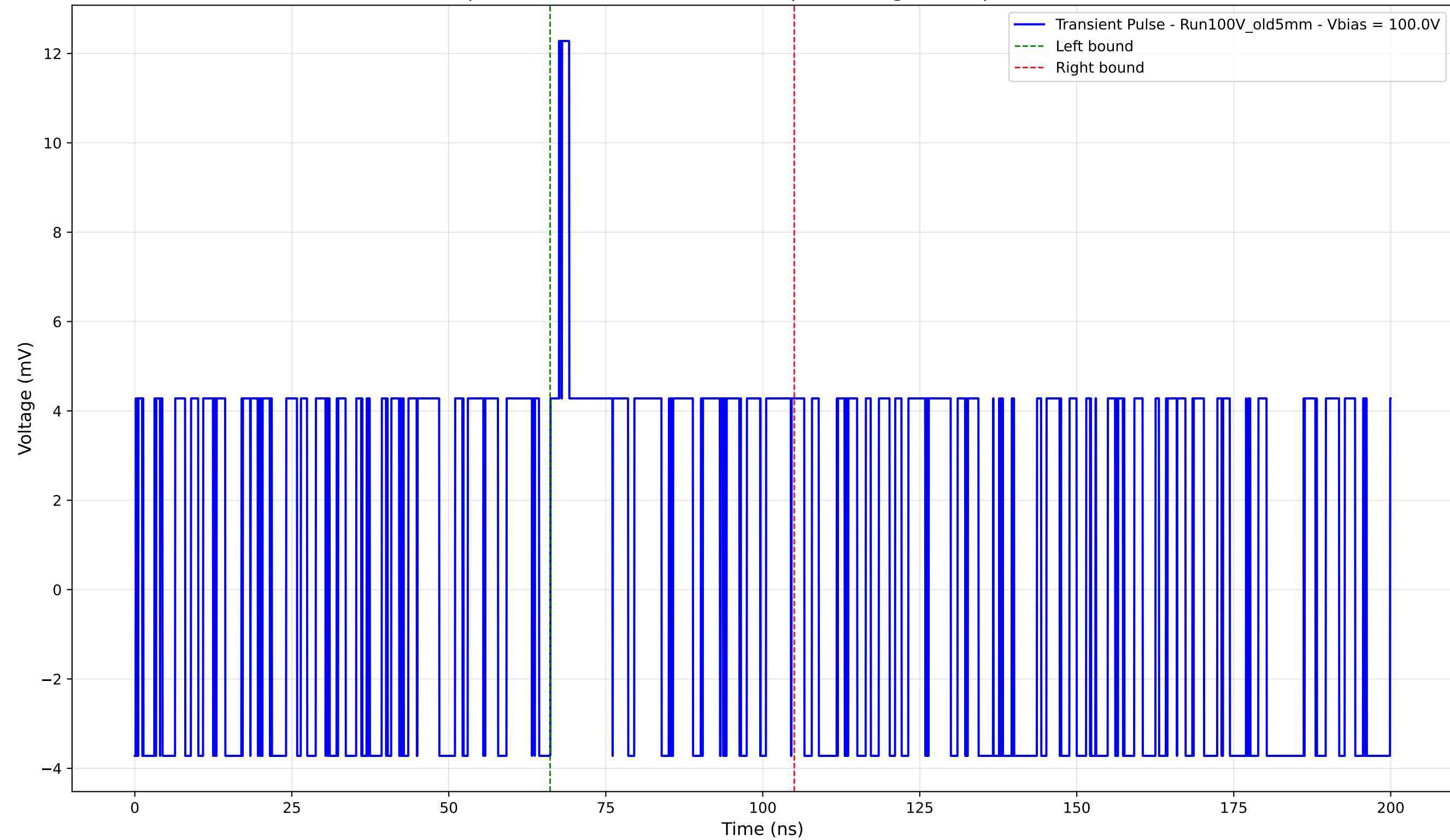
Transient Pulse - Sample: Old5mm - Position: 4000.0 \mu\text{m} - Charge: 2.51 pC - Rise Time: 0.00 ns (N/A)
