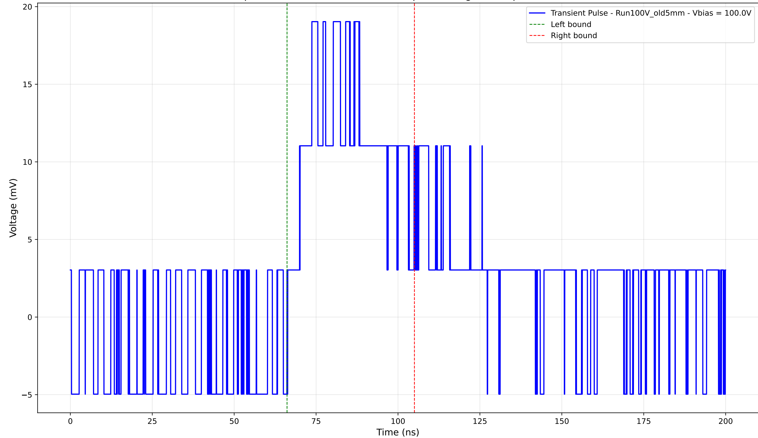
Transient Pulse - Sample: Old5mm - Position: 1595.0 \mu\text{m} - Charge: 8.85 pC - Rise Time: 0.00 ns (N/A)
