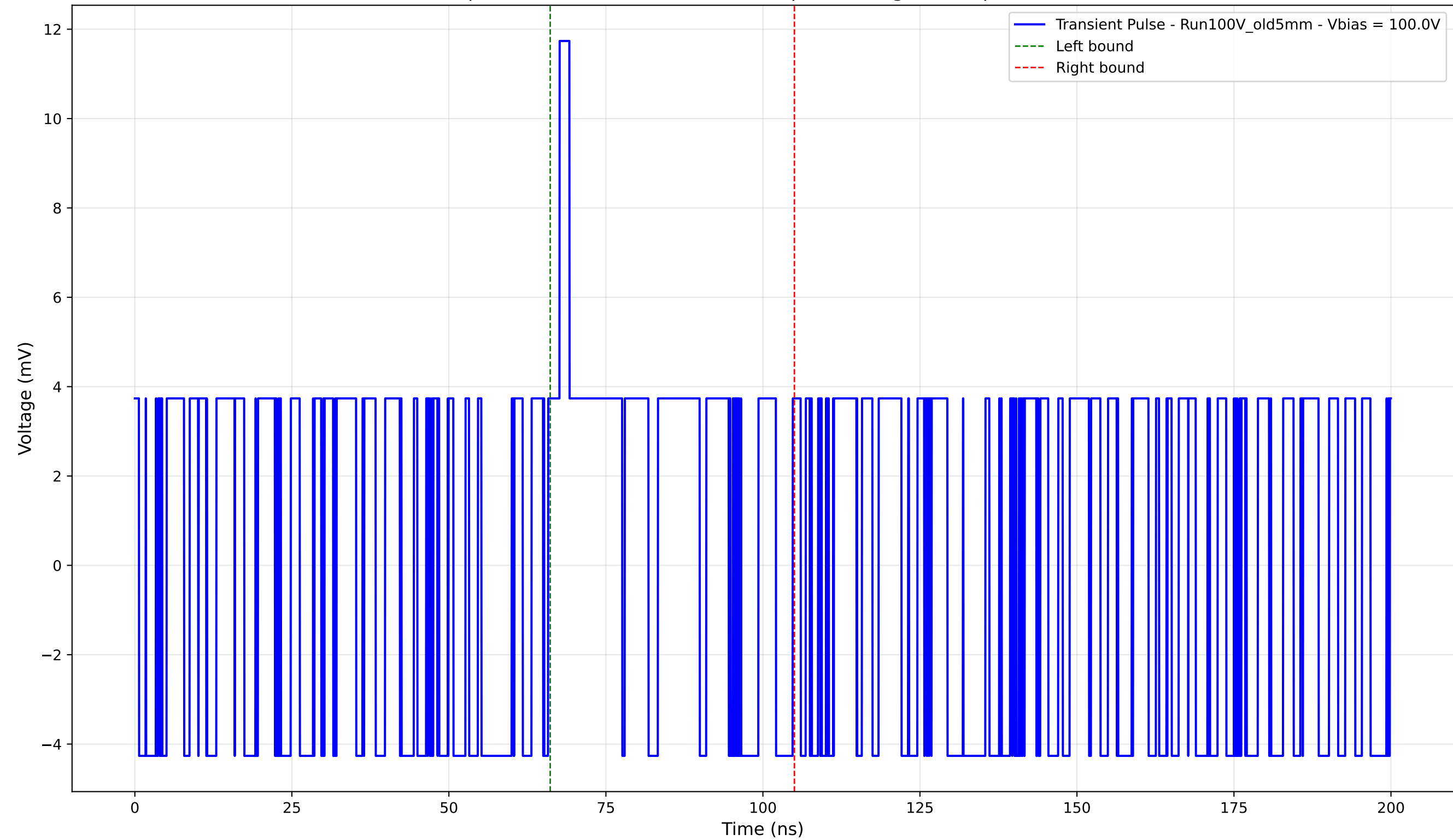
Transient Pulse - Sample: Old5mm - Position: 4280.0 \mu\text{m} - Charge: 1.63 pC - Rise Time: 0.00 ns (N/A)
