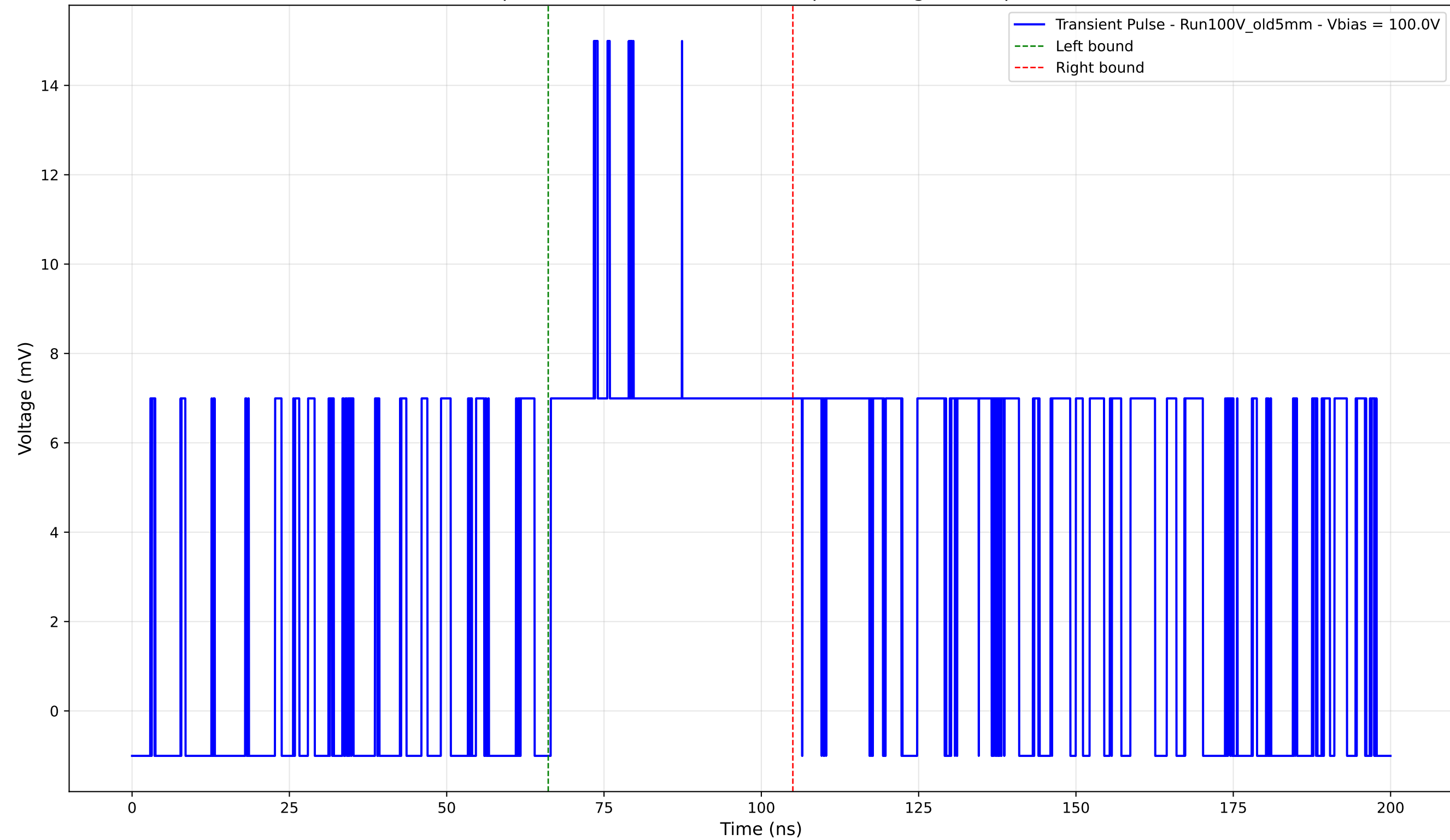
Transient Pulse - Sample: Old5mm - Position: 450.0 \mu\text{m} - Charge: 5.57 pC - Rise Time: 6.86 ns
