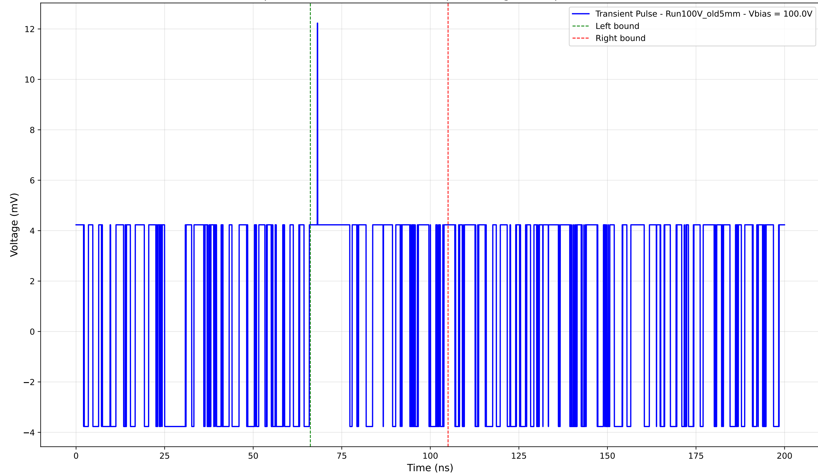
Transient Pulse - Sample: Old5mm - Position: 4015.0 \mu\text{m} - Charge: 1.86 pC - Rise Time: 0.00 ns (N/A)
