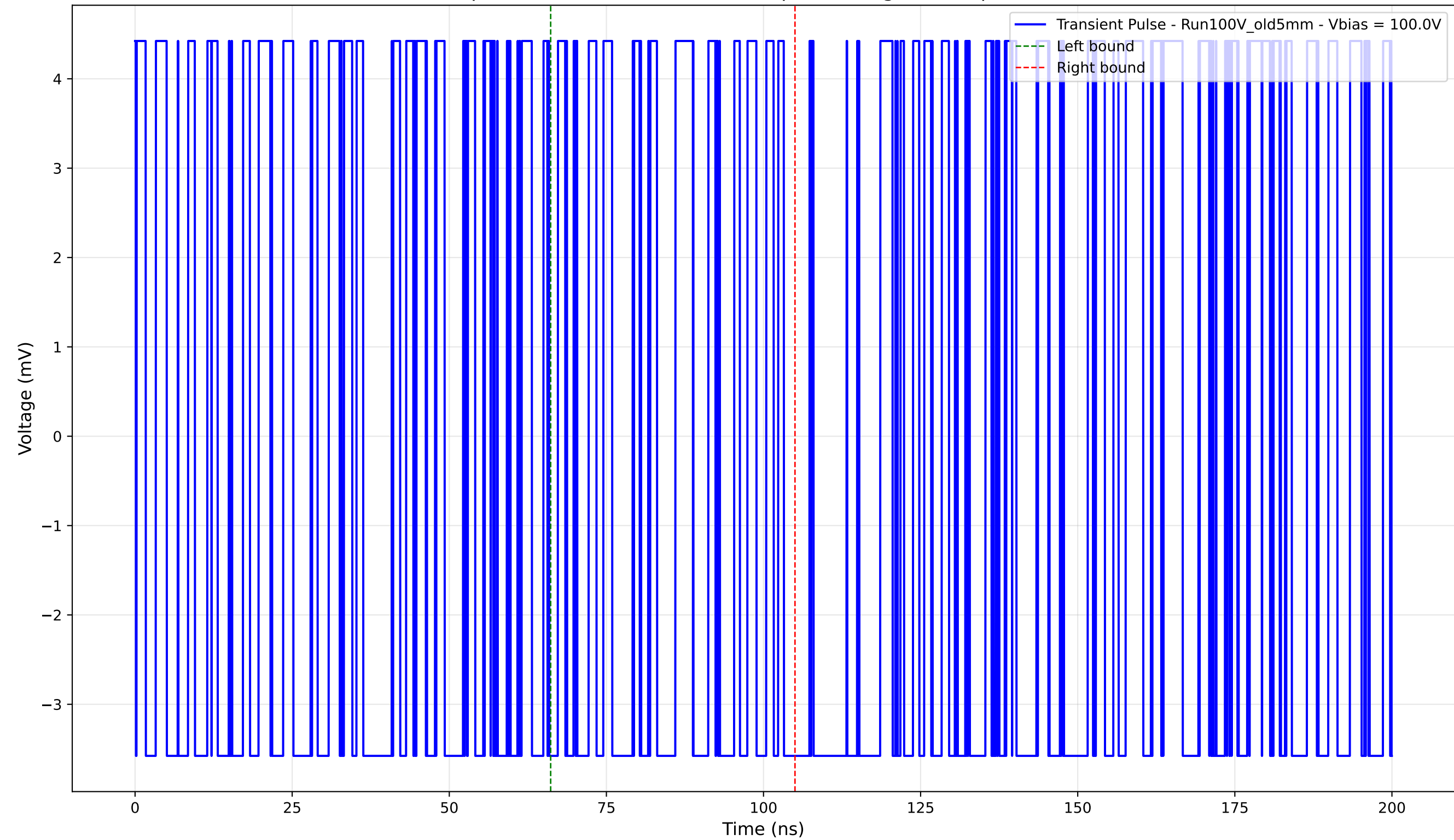
Transient Pulse - Sample: Old5mm - Position: 215.0 \mu\text{m} - Charge: -0.31 pC - Rise Time: 0.00 ns (N/A)
