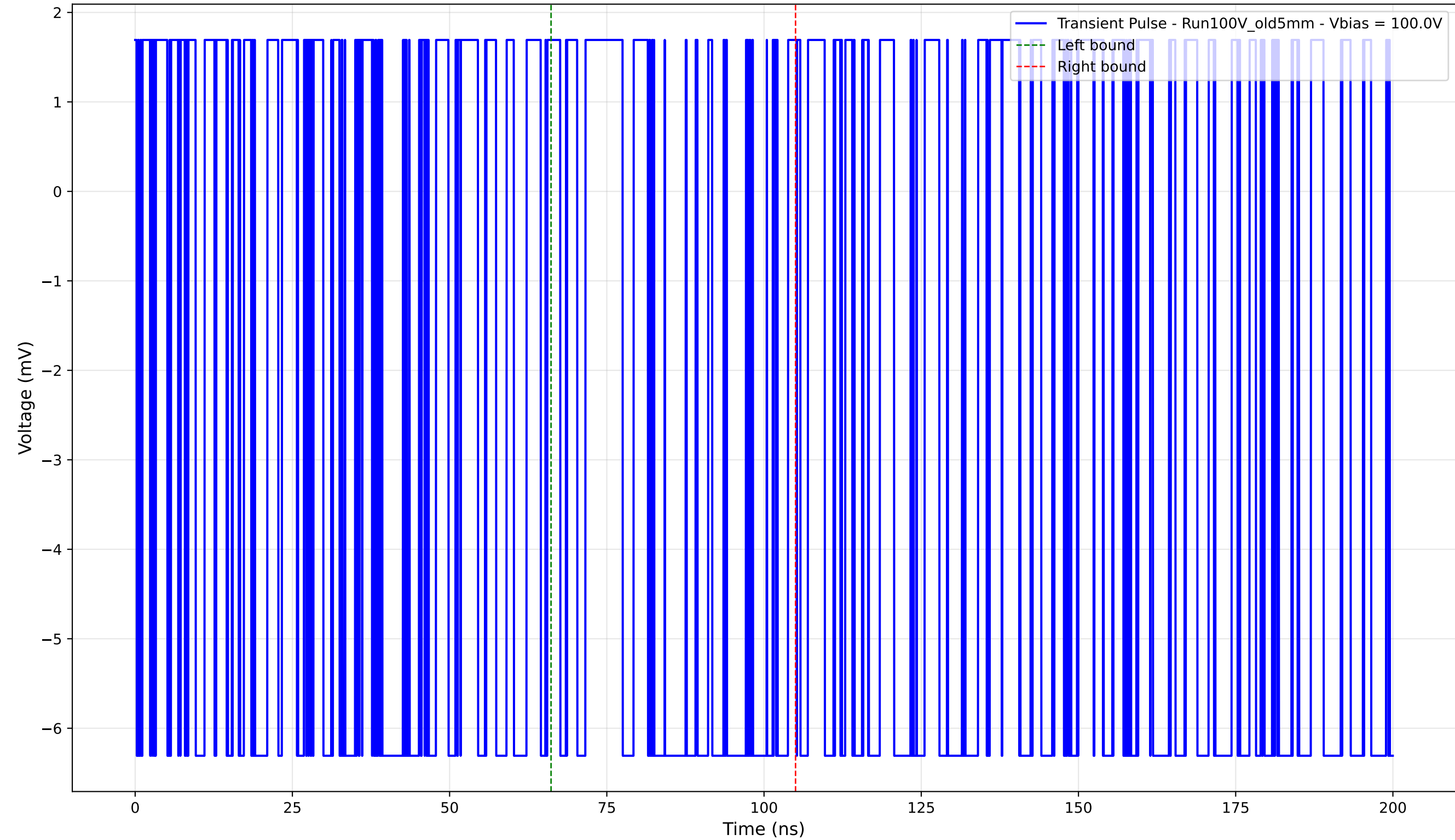
Transient Pulse - Sample: Old5mm - Position: 135.0 \mu\text{m} - Charge: -2.40 pC - Rise Time: 0.00 ns (N/A)
