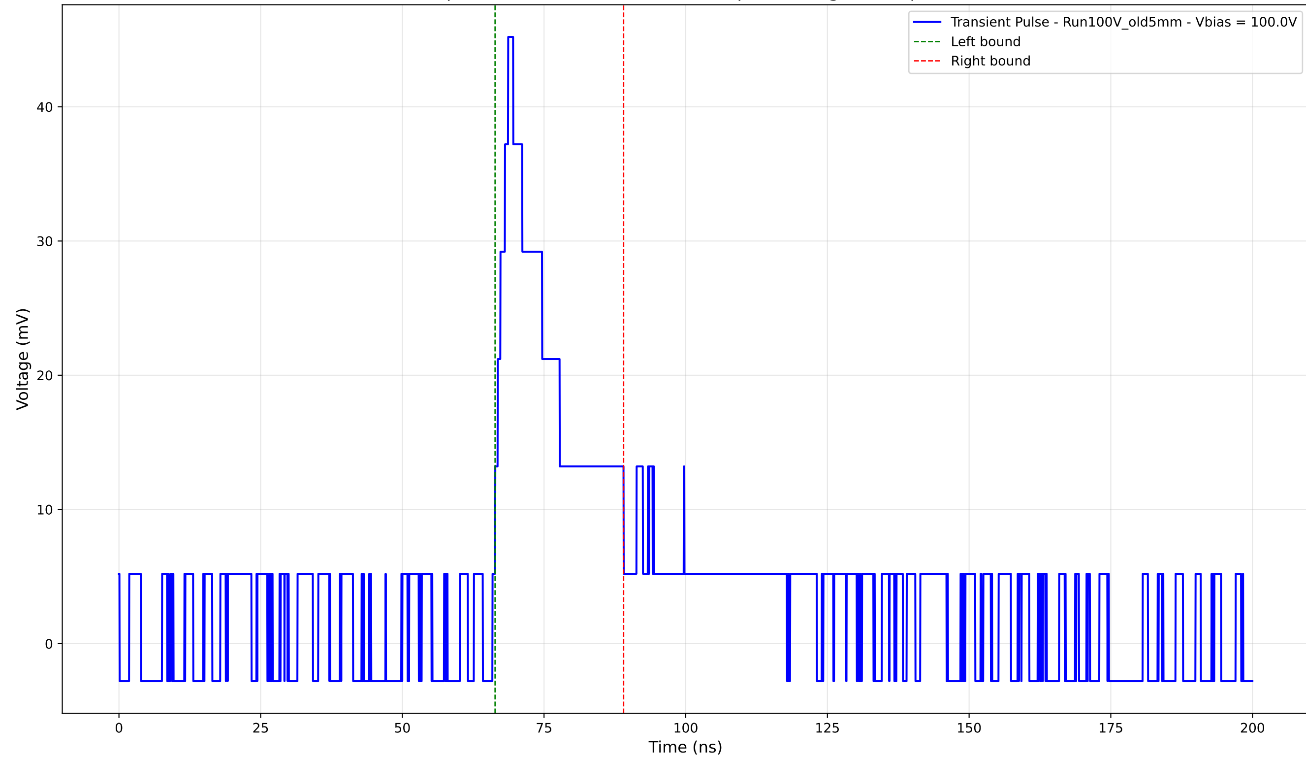
Transient Pulse - Sample: Old5mm - Position: 4535.0 \mu\text{m} - Charge: 9.55 pC - Rise Time: 2.77 ns
