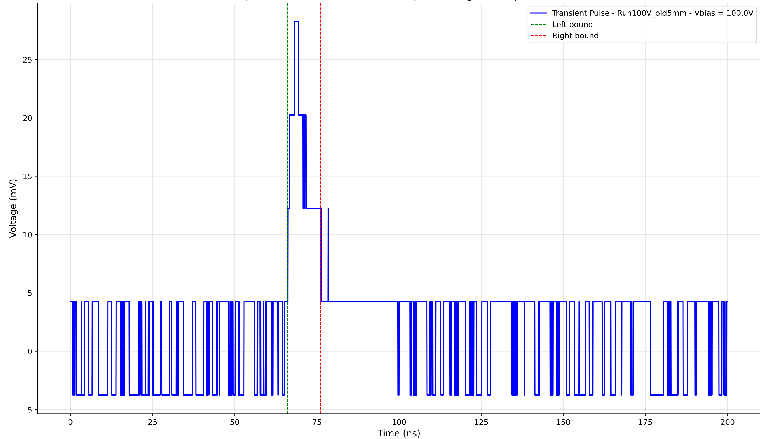
Transient Pulse - Sample: Old5mm - Position: 4255.0 \mu\text{m} - Charge: 3.39 pC - Rise Time: 0.00 ns (N/A)
