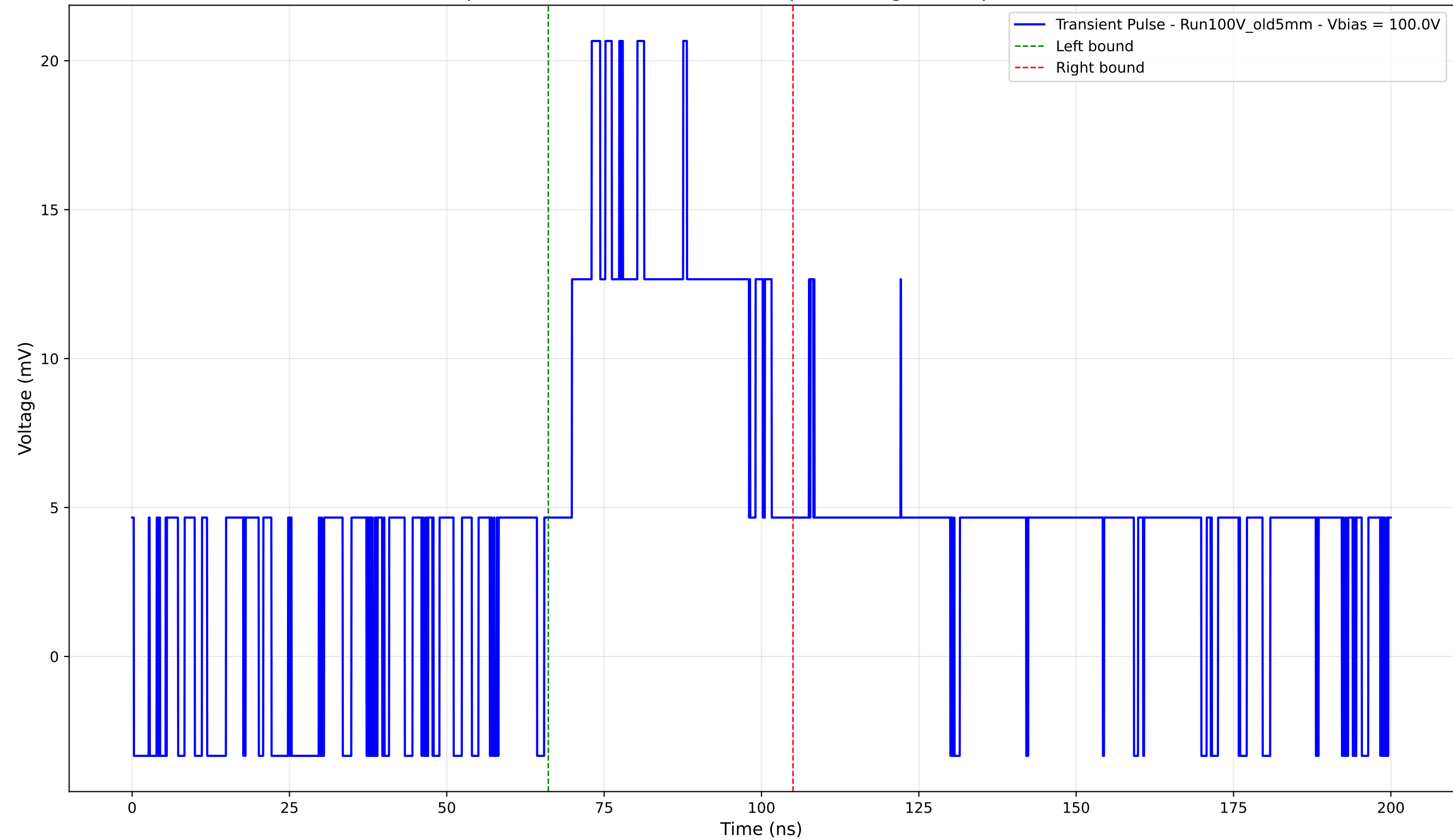
Transient Pulse - Sample: Old5mm - Position: 1435.0 \mu\text{m} - Charge: 9.24 pC - Rise Time: 0.00 ns (N/A)
