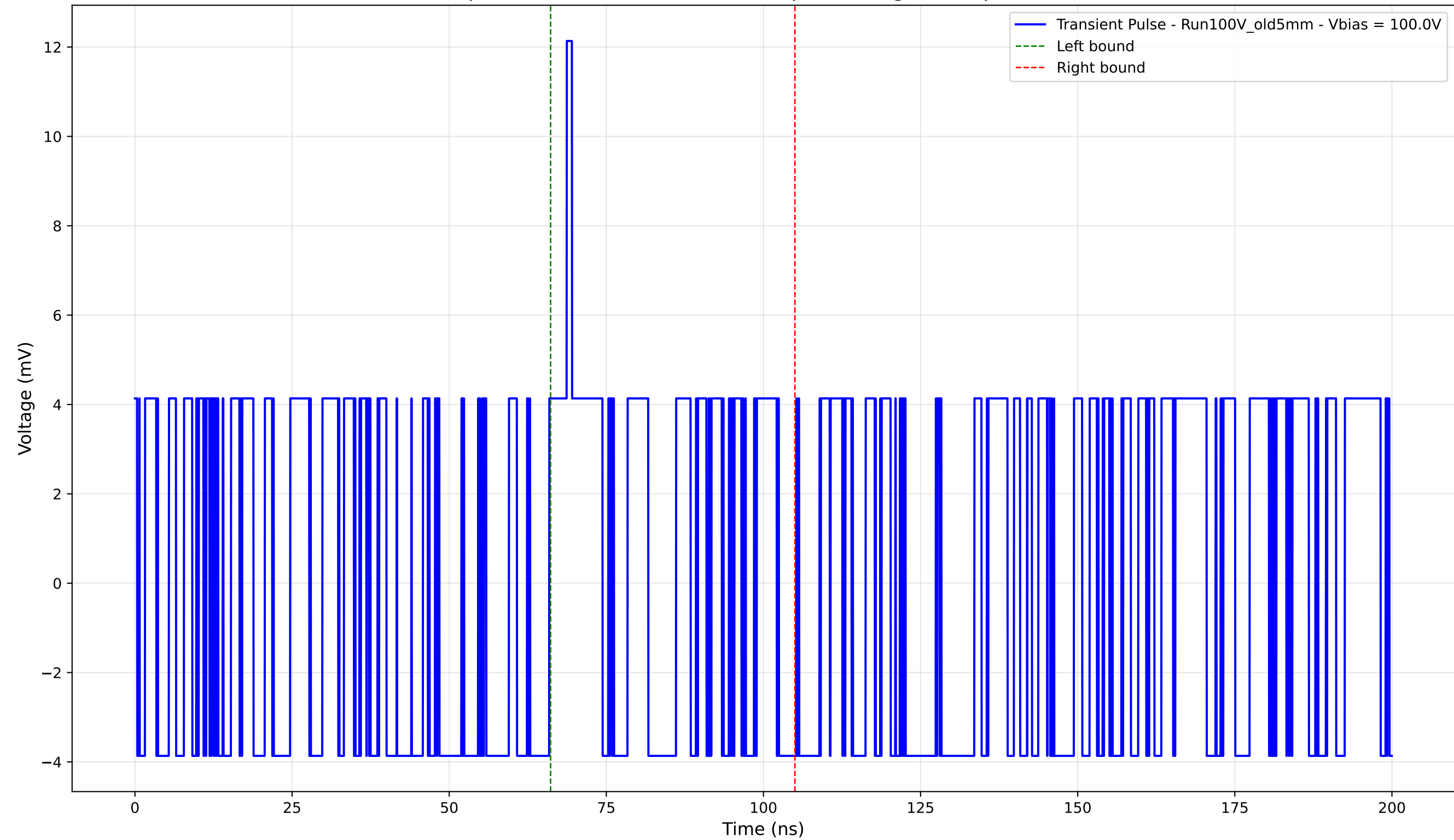
Transient Pulse - Sample: Old5mm - Position: 3415.0 \mu\text{m} - Charge: 0.92 pC - Rise Time: 0.00 ns (N/A)
