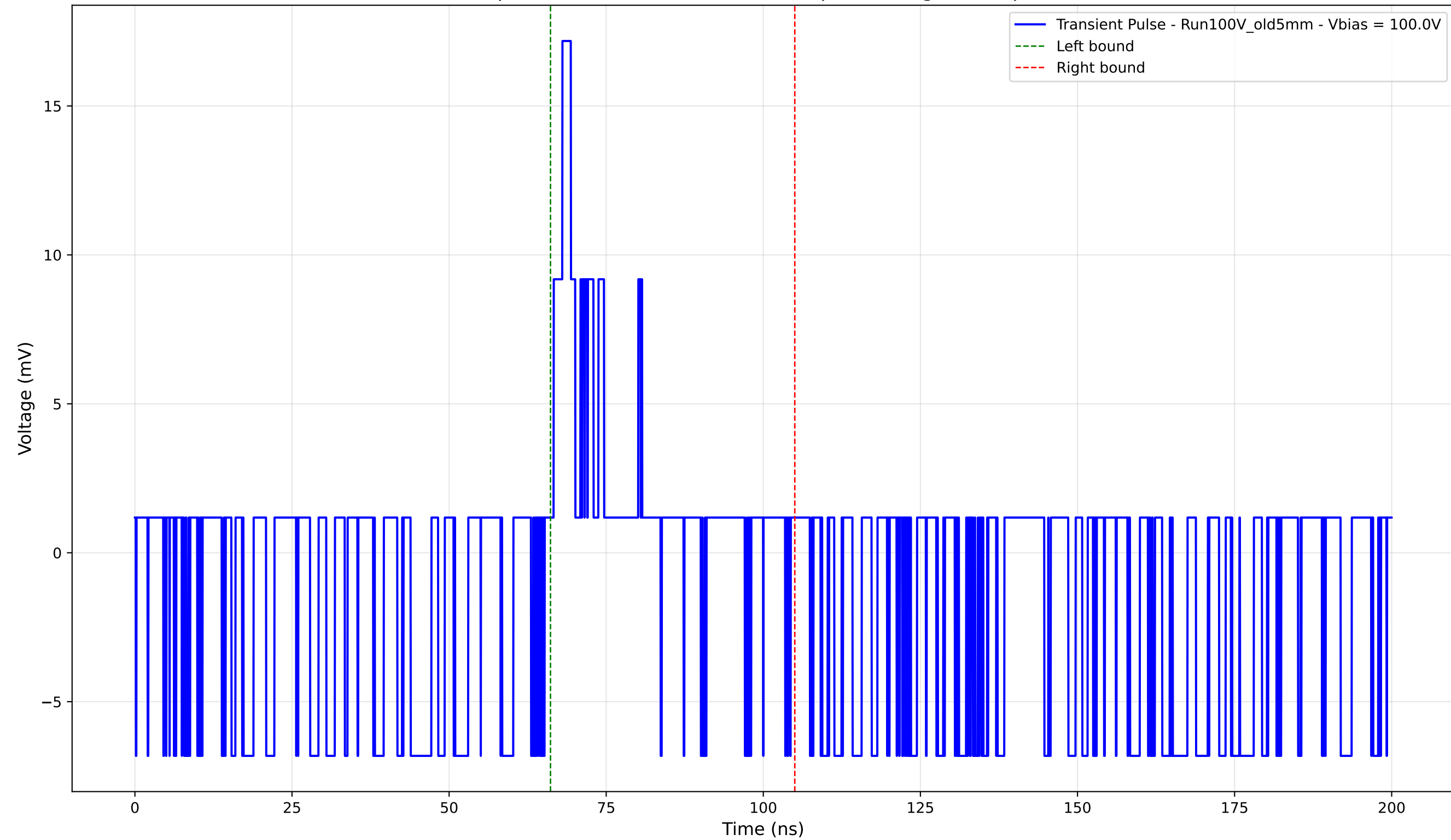
Transient Pulse - Sample: Old5mm - Position: 4265.0 \mu\text{m} - Charge: 1.83 pC - Rise Time: 1.40 ns
