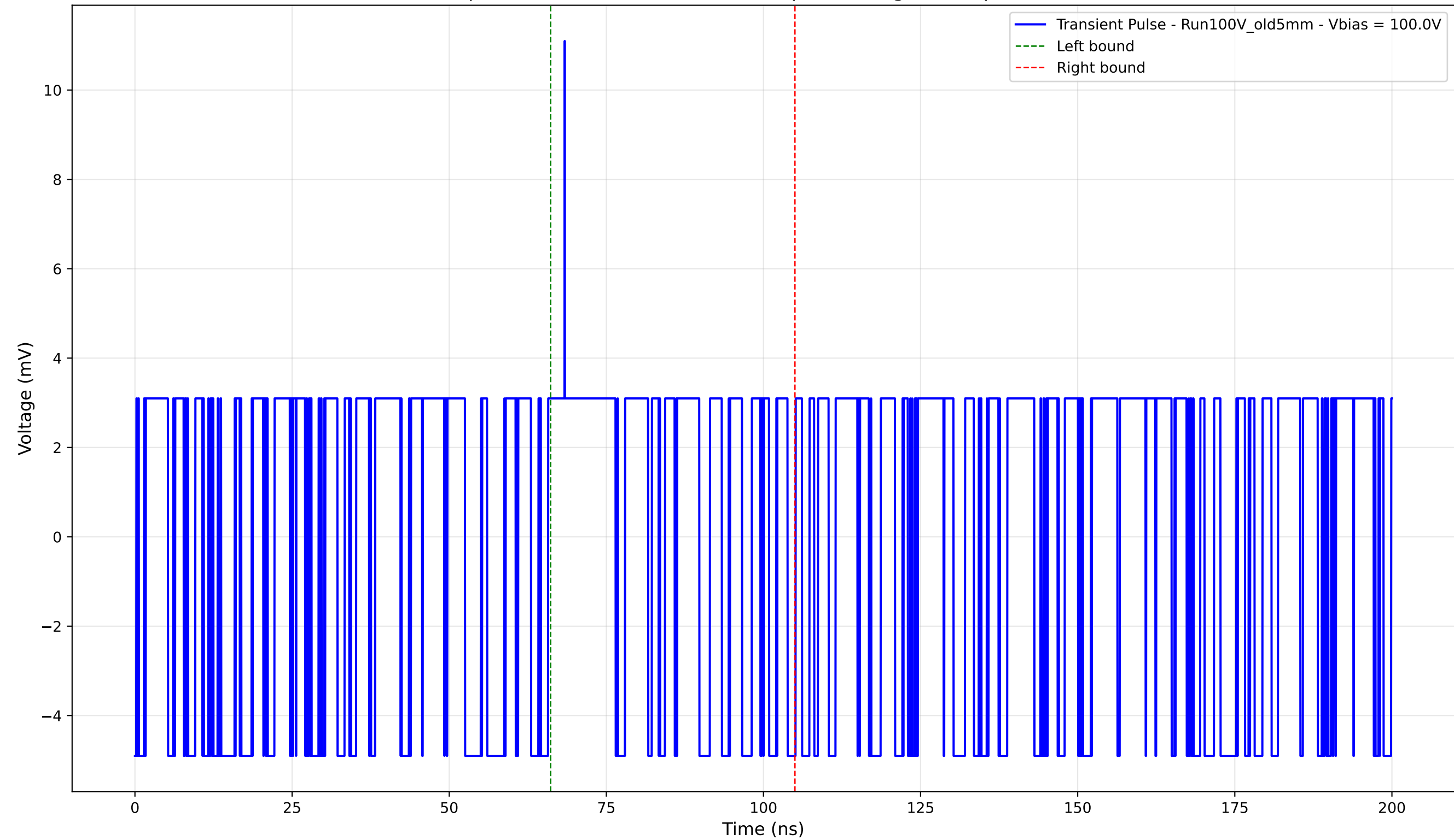
Transient Pulse - Sample: Old5mm - Position: 3085.0 \mu\text{m} - Charge: 0.79 pC - Rise Time: 0.00 ns (N/A)
