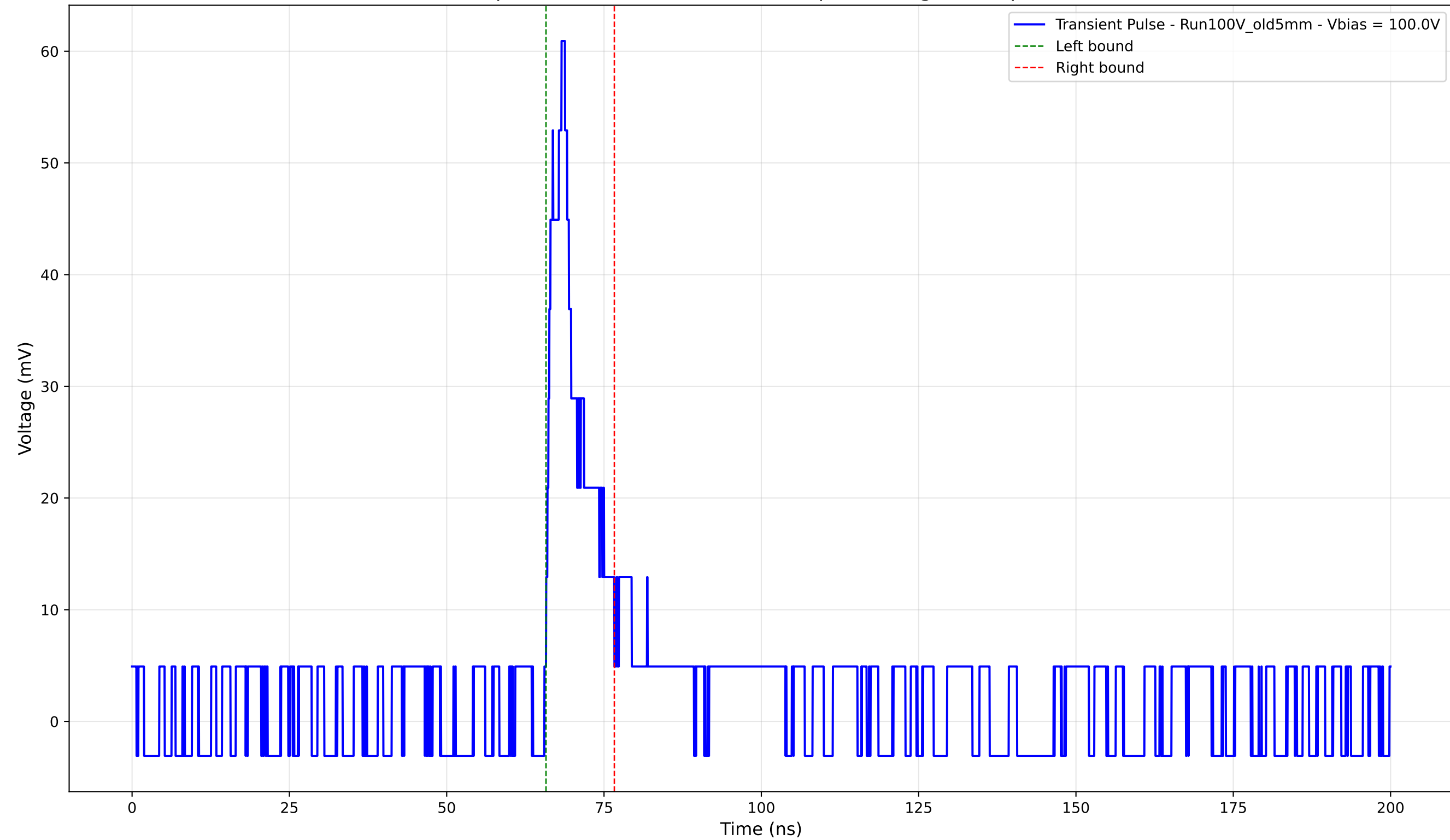
Transient Pulse - Sample: Old5mm - Position: 4075.0 \mu\text{m} - Charge: 6.39 pC - Rise Time: 2.46 ns
