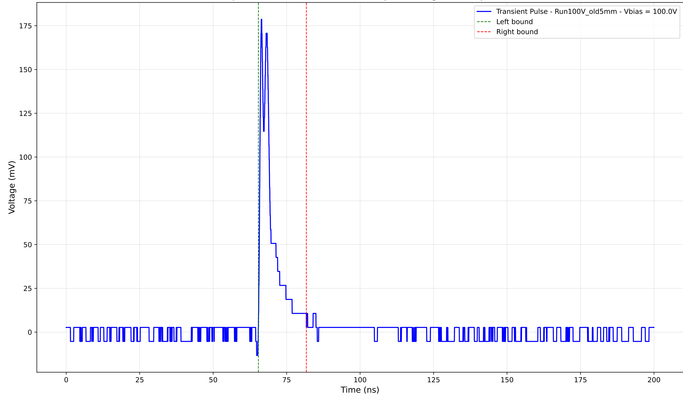
Transient Pulse - Sample: Old5mm - Position: 3615.0 \mu\text{m} - Charge: 16.17 pC - Rise Time: 0.70 ns
