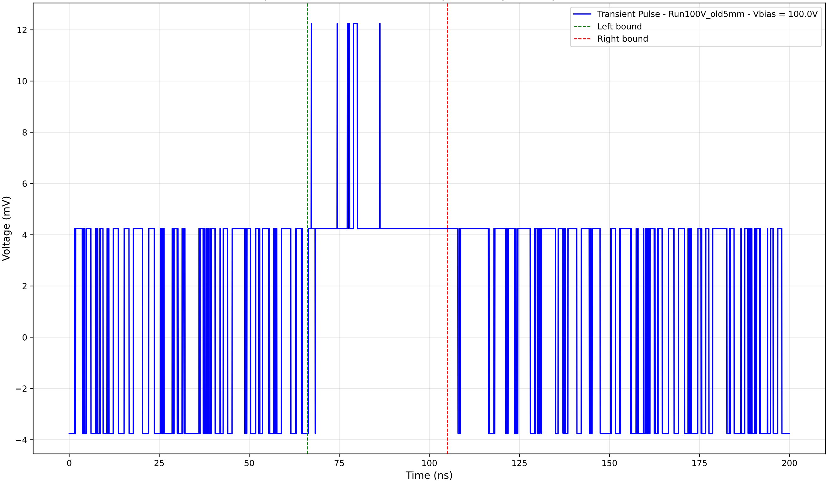
Transient Pulse - Sample: Old5mm - Position: 725.0 \mu\text{m} - Charge: 3.51 pC - Rise Time: 0.00 ns (N/A)
