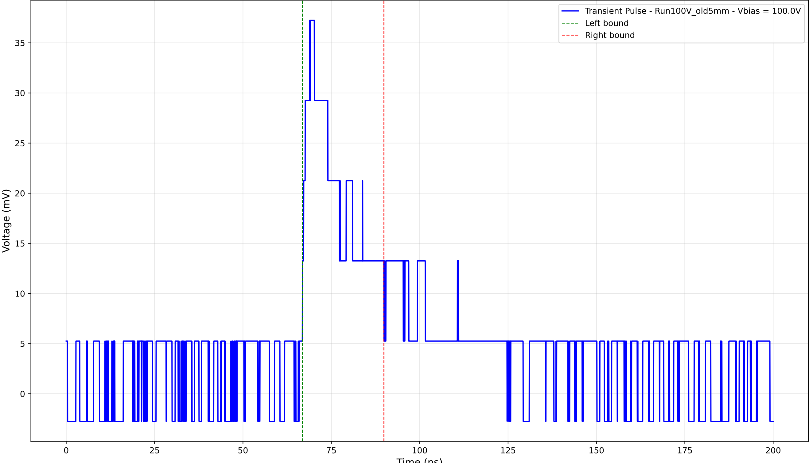
Transient Pulse - Sample: Old5mm - Position: 2710.0 \mu\text{m} - Charge: 9.26 pC - Rise Time: 3.05 ns
