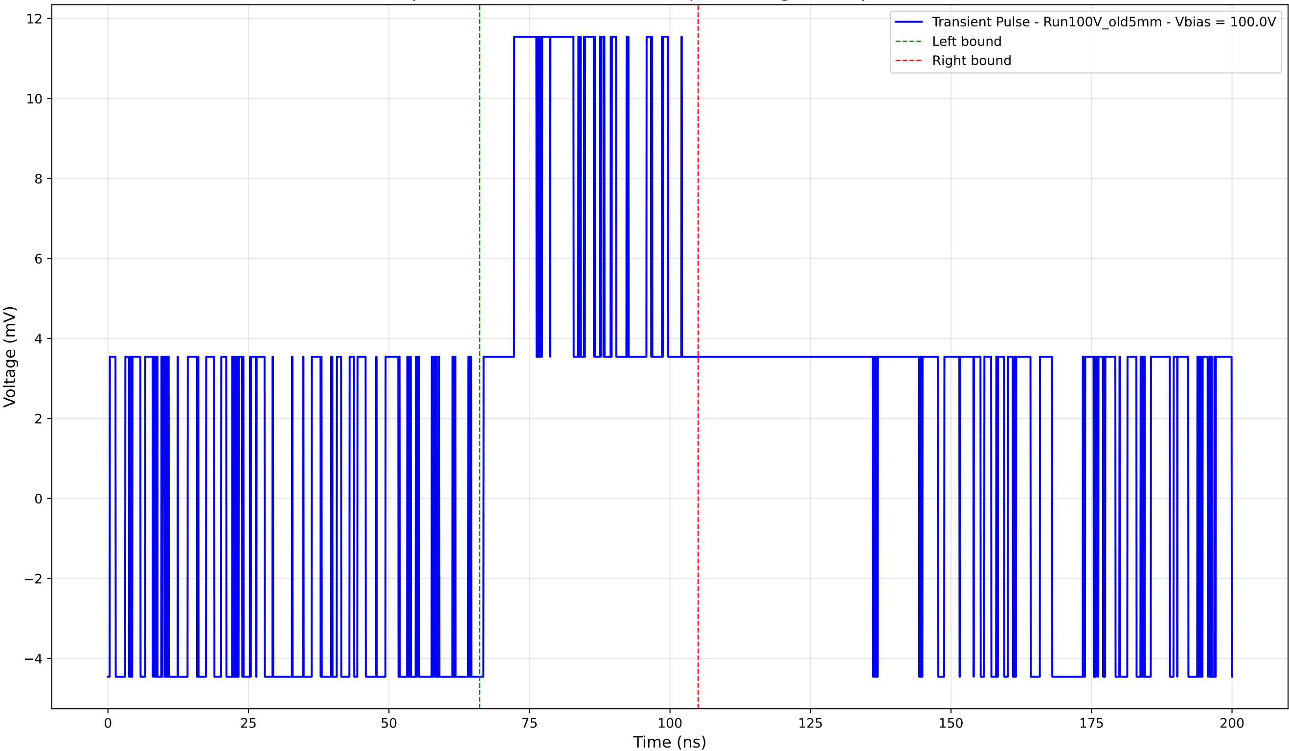
Transient Pulse - Sample: Old5mm - Position: 870.0 \mu\text{m} - Charge: 5.17 pC - Rise Time: 0.00 ns (N/A)
