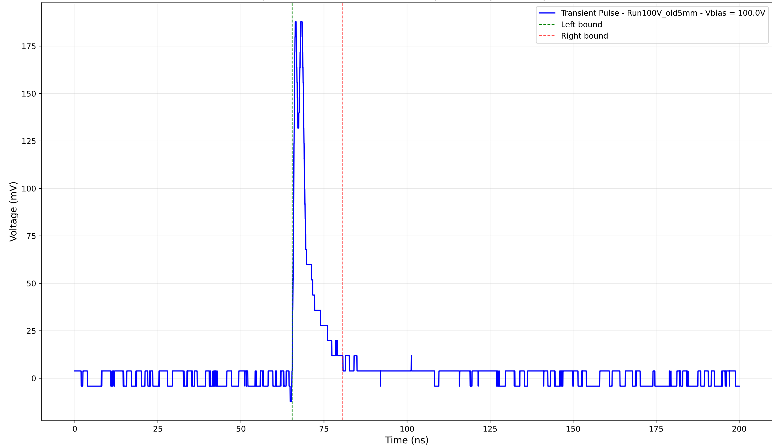
Transient Pulse - Sample: Old5mm - Position: 3820.0 \mu\text{m} - Charge: 18.17 pC - Rise Time: 0.70 ns
