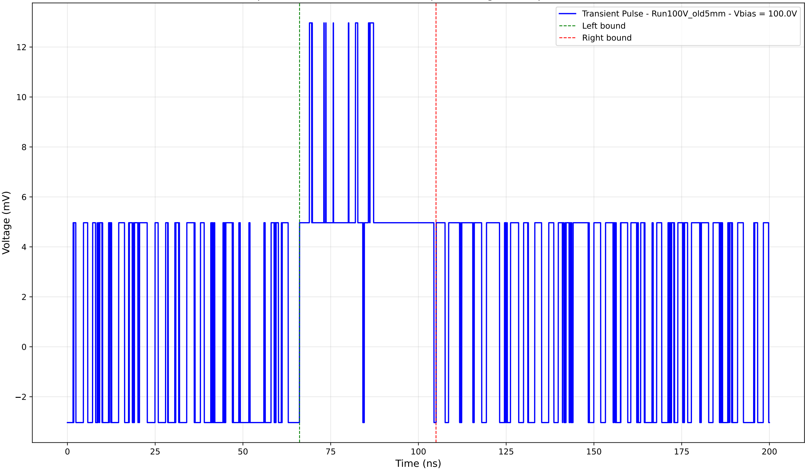
Transient Pulse - Sample: Old5mm - Position: 505.0 \mu\text{m} - Charge: 4.21 pC - Rise Time: 0.00 ns (N/A)
