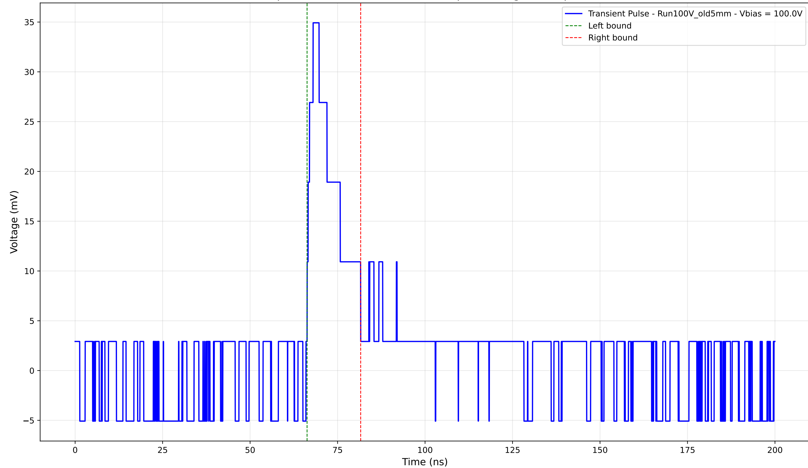
Transient Pulse - Sample: Old5mm - Position: 3035.0 \mu\text{m} - Charge: 5.89 pC - Rise Time: 1.72 ns
