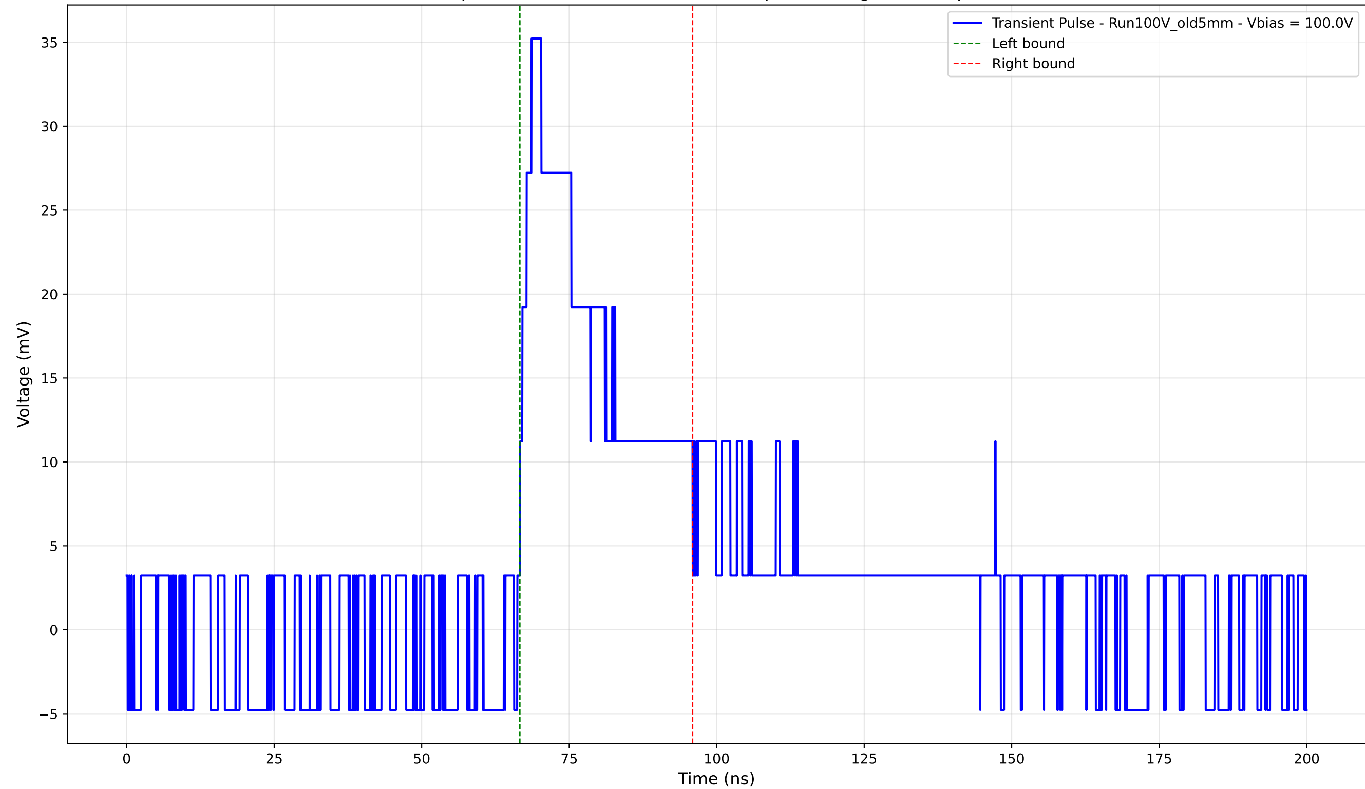
Transient Pulse - Sample: Old5mm - Position: 2705.0 \mu\text{m} - Charge: 10.36 pC - Rise Time: 1.96 ns
