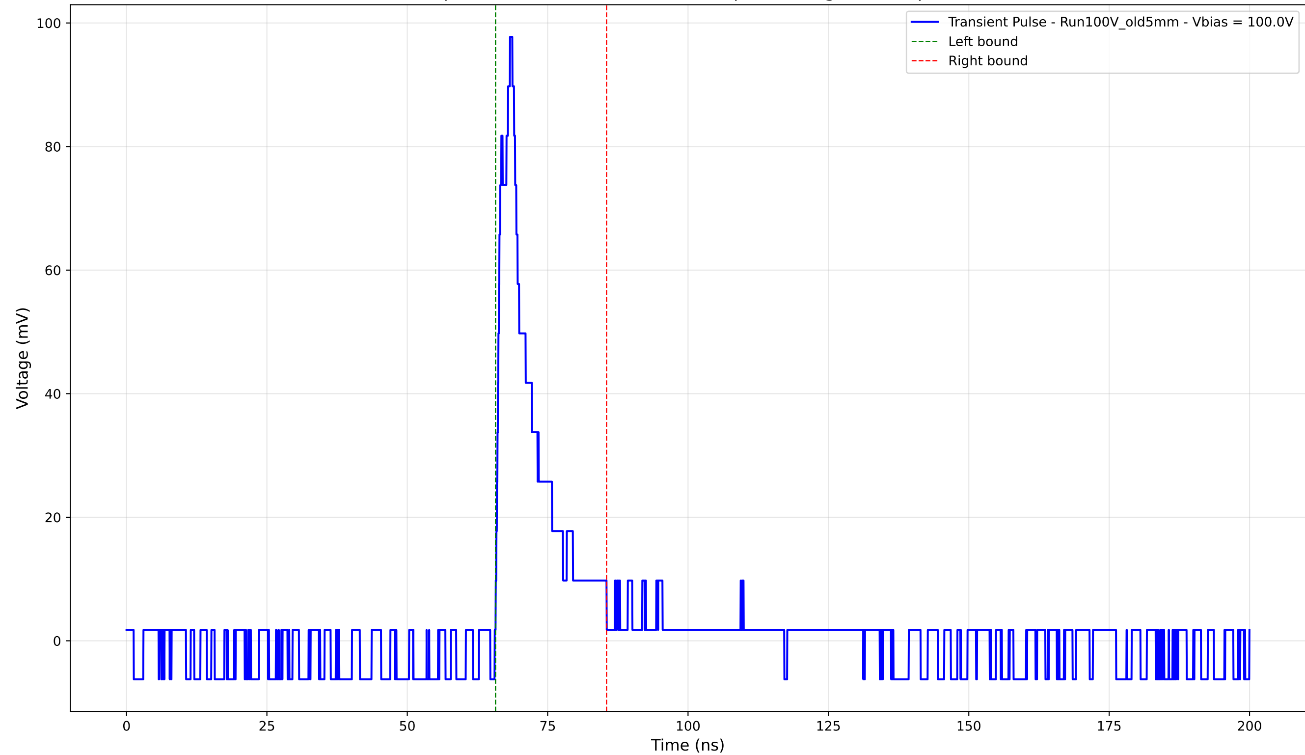
Transient Pulse - Sample: Old5mm - Position: 4100.0 \mu\text{m} - Charge: 12.50 pC - Rise Time: 2.10 ns
