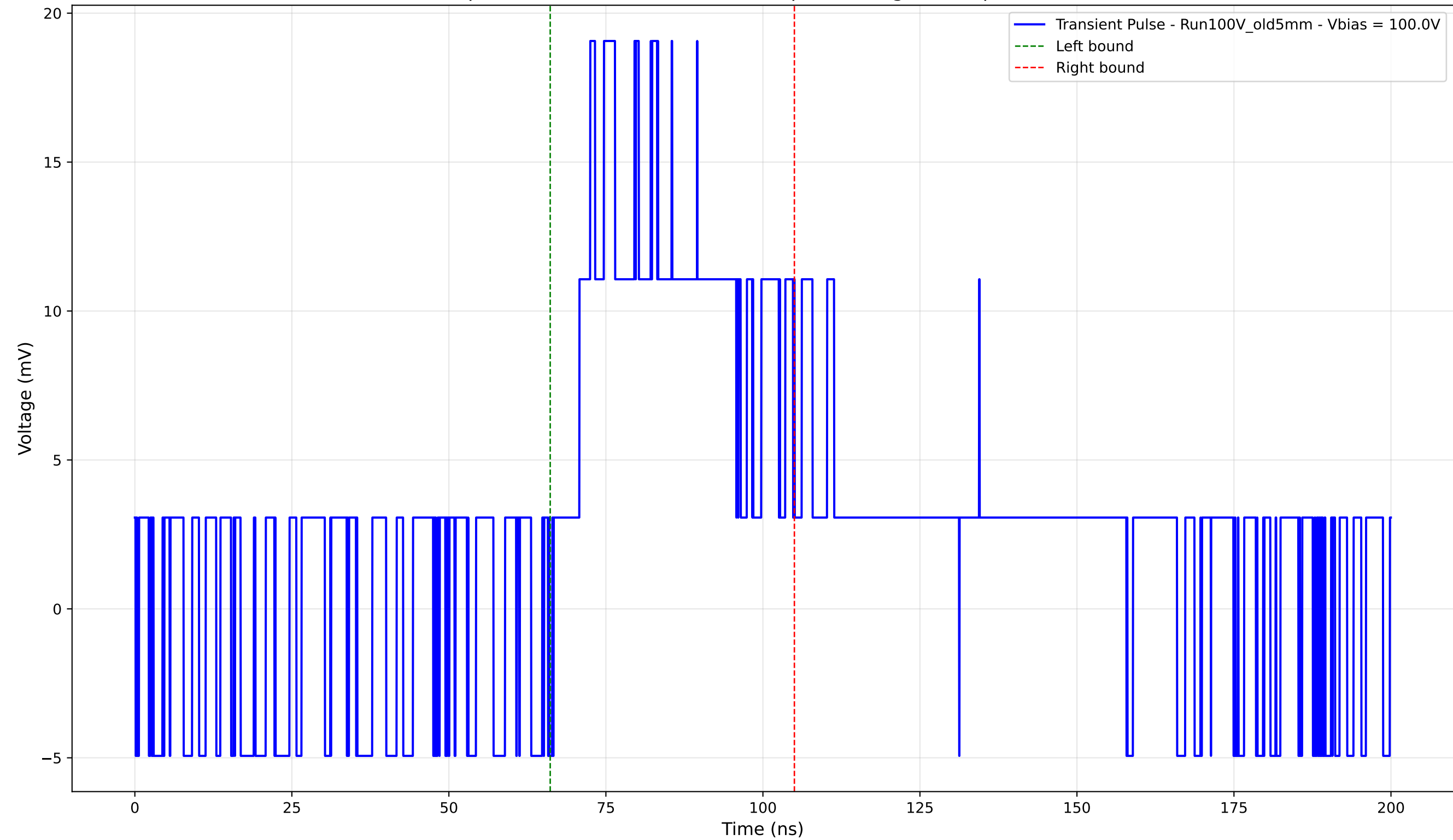
Transient Pulse - Sample: Old5mm - Position: 1200.0 \mu\text{m} - Charge: 7.91 pC - Rise Time: 0.00 ns (N/A)
