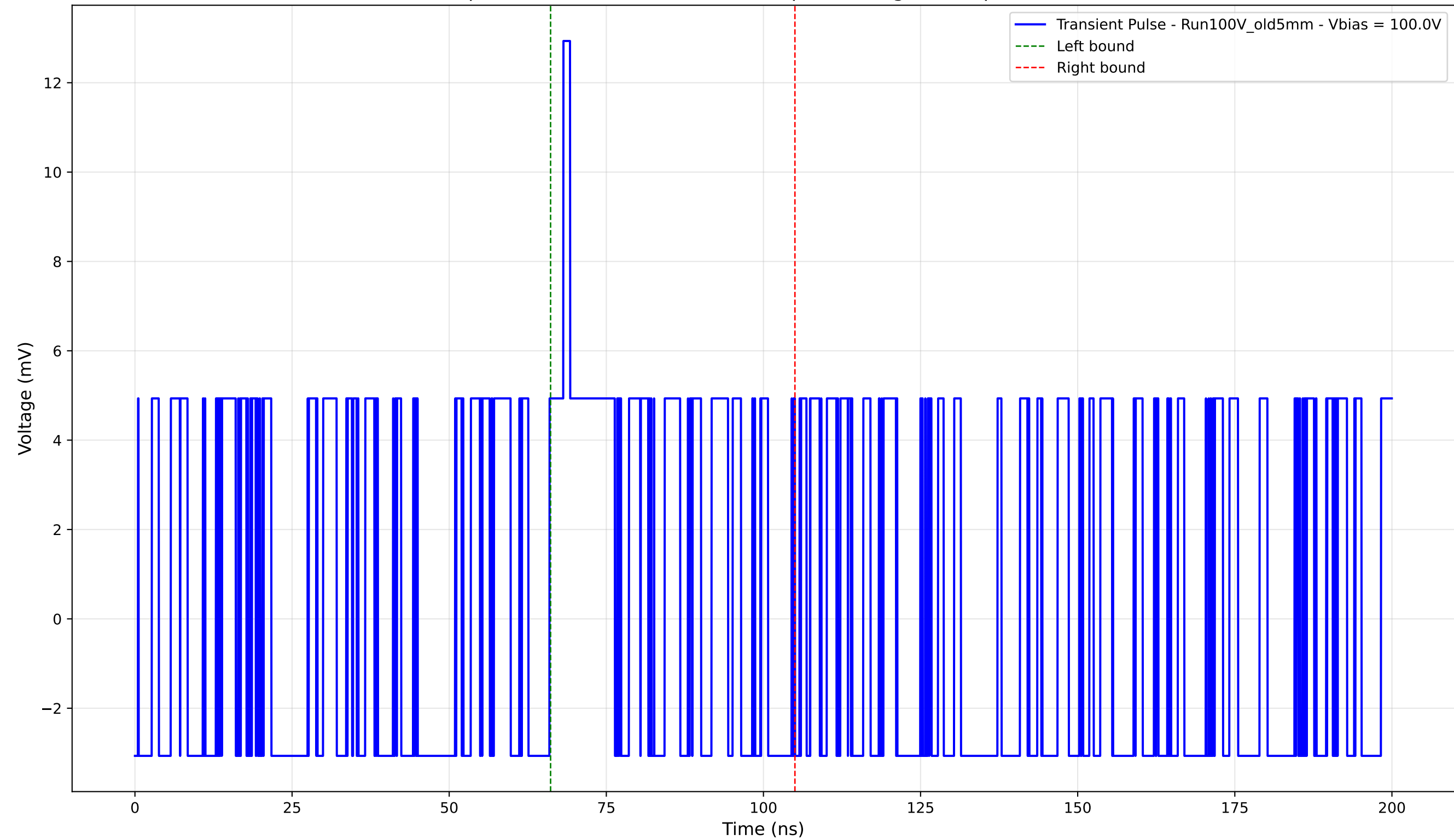
Transient Pulse - Sample: Old5mm - Position: 3425.0 \mu\text{m} - Charge: 1.58 pC - Rise Time: 0.00 ns (N/A)
