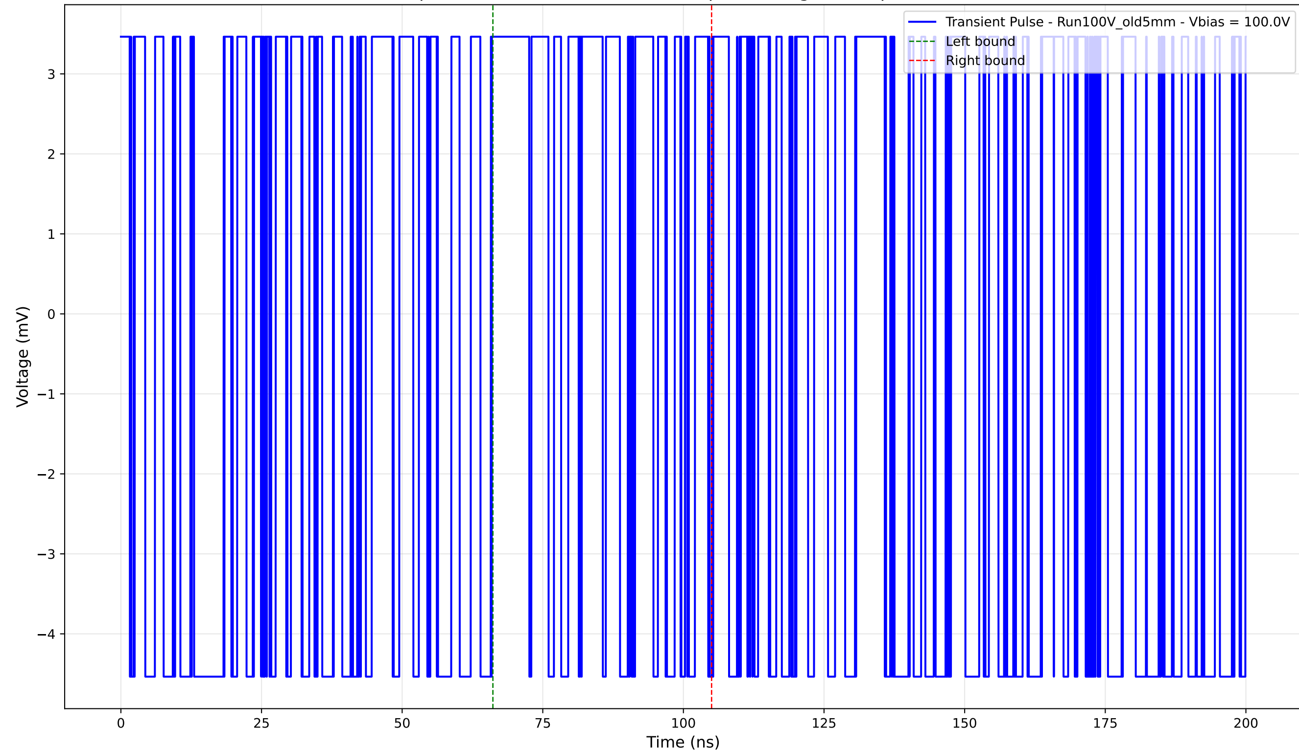
Transient Pulse - Sample: Old5mm - Position: 2790.0 \mu\text{m} - Charge: 1.06 pC - Rise Time: 0.00 ns (N/A)
