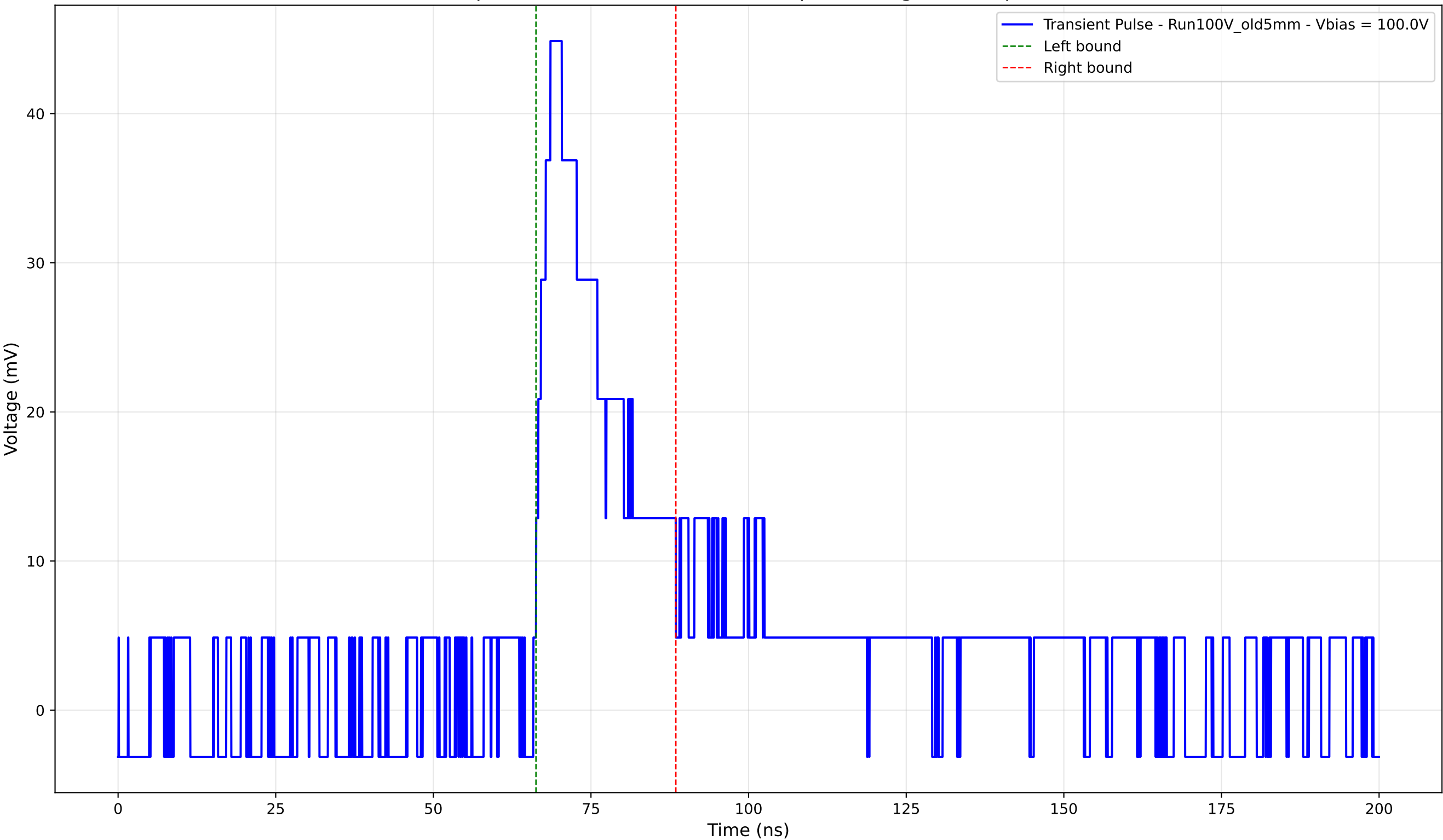
Transient Pulse - Sample: Old5mm - Position: 4530.0 \mu\text{m} - Charge: 10.44 pC - Rise Time: 2.70 ns
