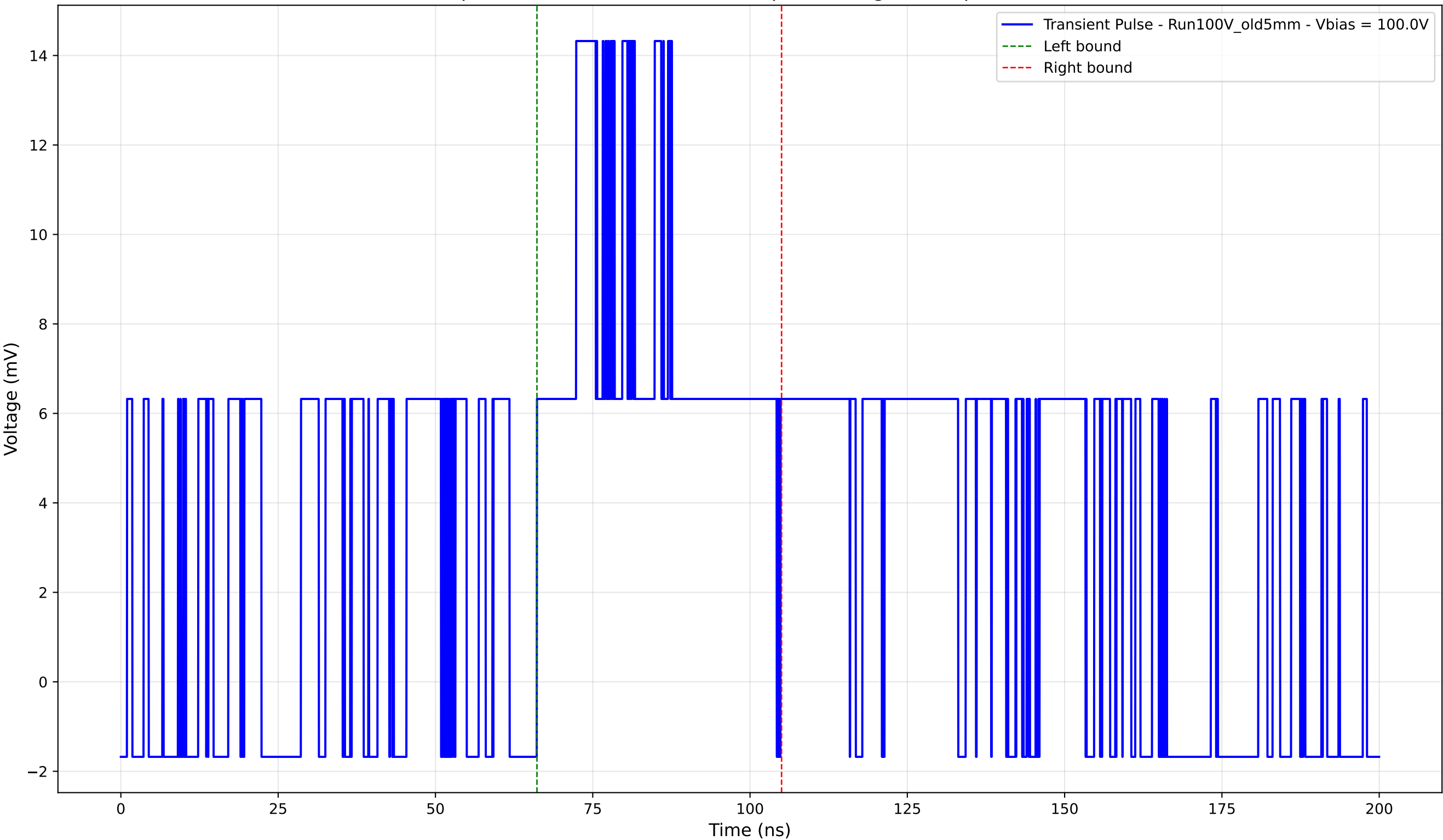
Transient Pulse - Sample: Old5mm - Position: 475.0 \mu\text{m} - Charge: 6.01 pC - Rise Time: 0.00 ns (N/A)
