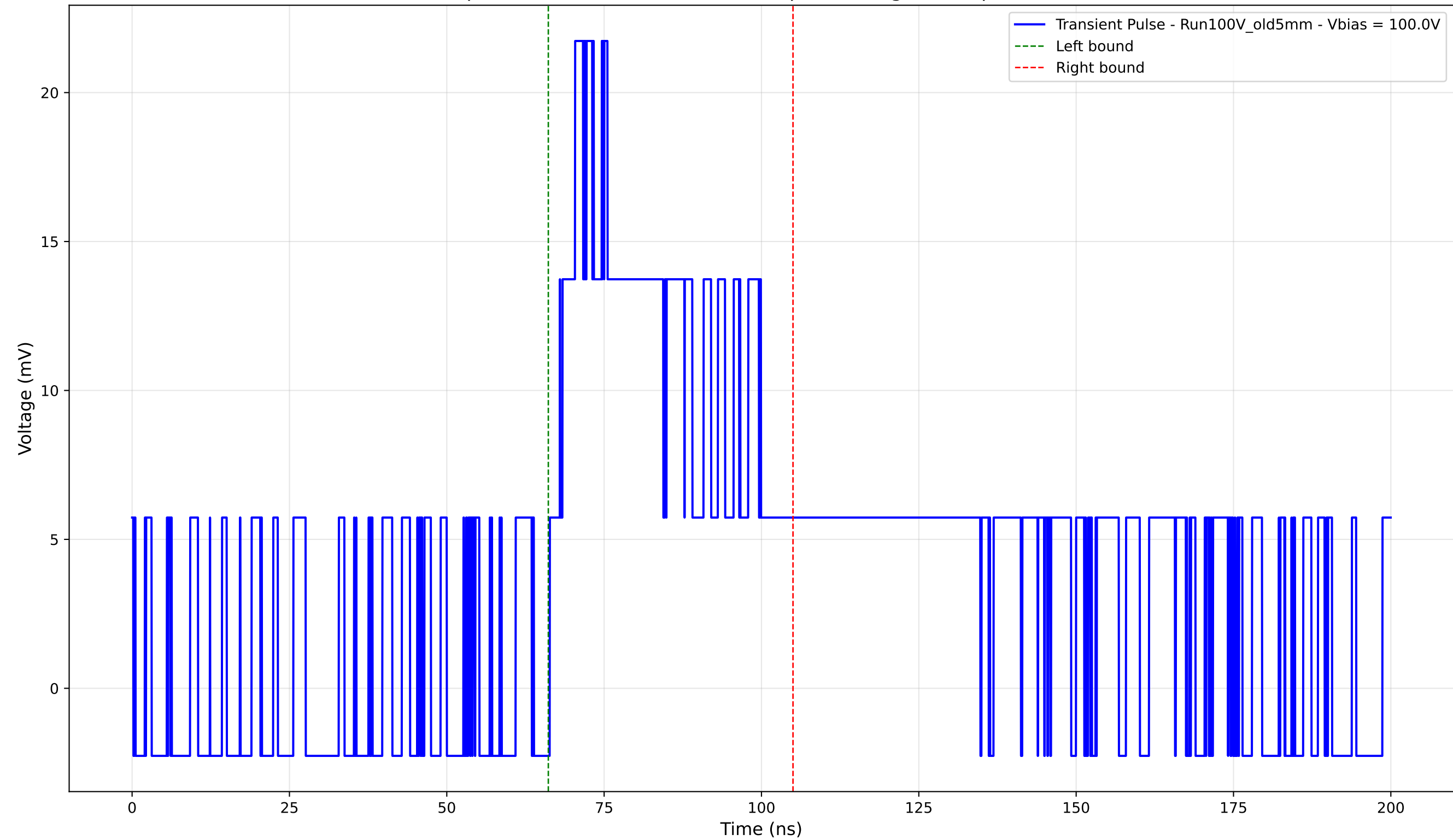
Transient Pulse - Sample: Old5mm - Position: 2370.0 \mu\text{m} - Charge: 9.05 pC - Rise Time: 0.00 ns (N/A)
