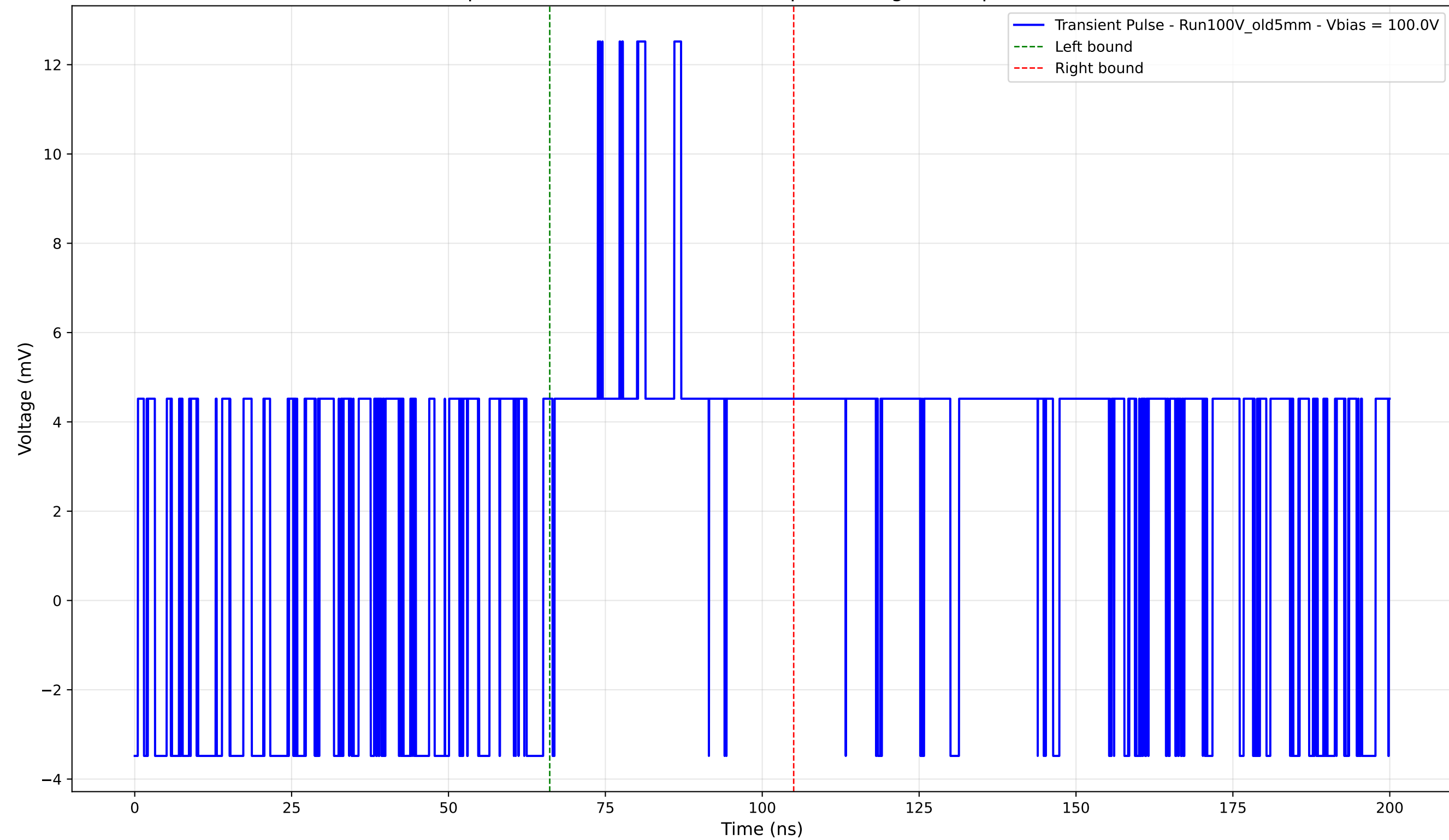
Transient Pulse - Sample: Old5mm - Position: 1945.0 \mu\text{m} - Charge: 3.89 pC - Rise Time: 0.00 ns (N/A)
