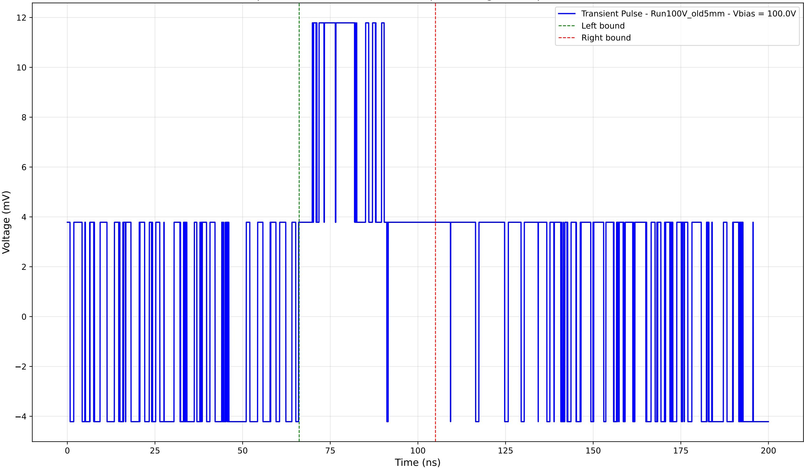
Transient Pulse - Sample: Old5mm - Position: 390.0 \mu\text{m} - Charge: 5.12 pC - Rise Time: 0.00 ns (N/A)
