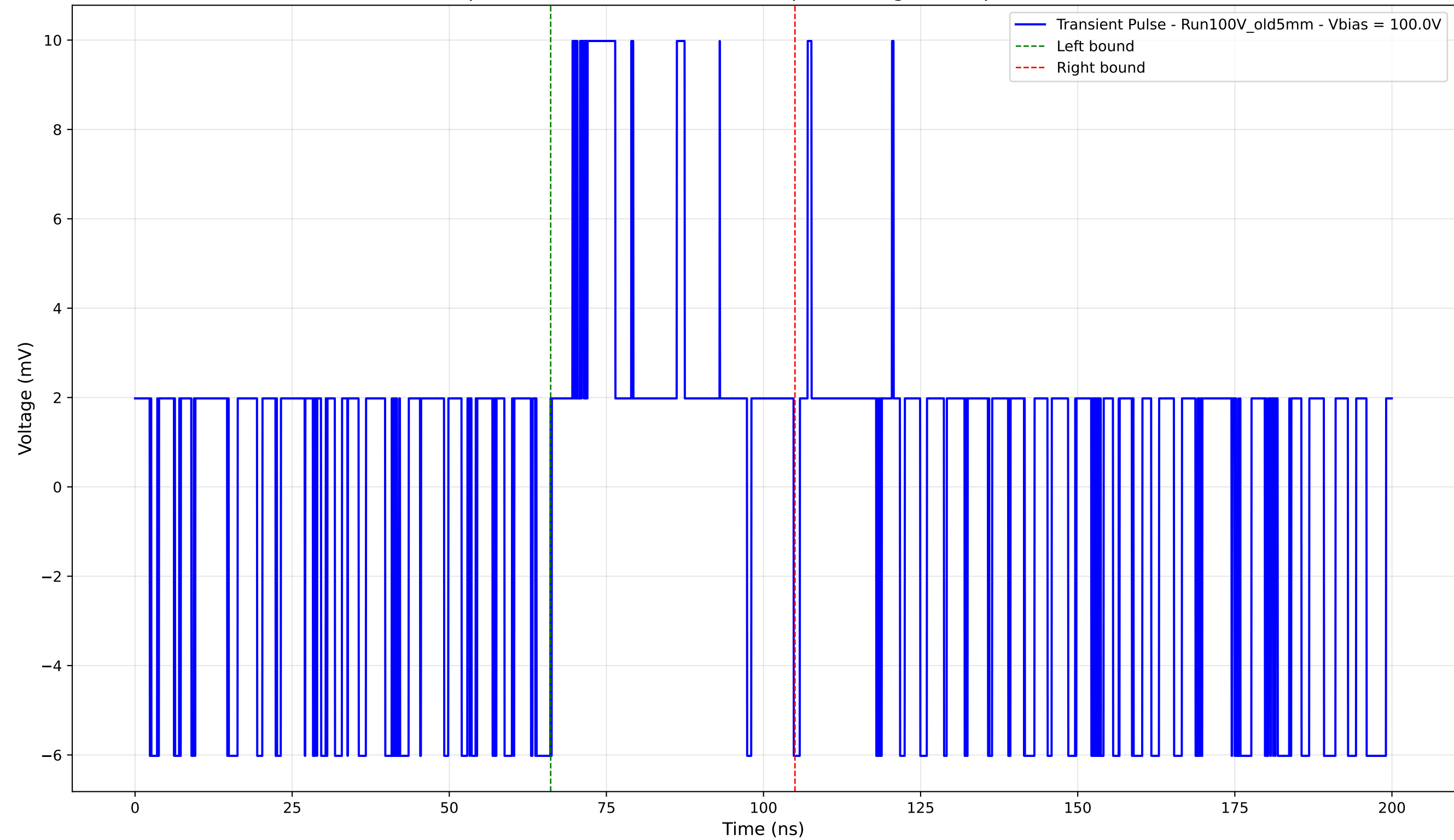
Transient Pulse - Sample: Old5mm - Position: 2145.0 \mu\text{m} - Charge: 2.50 pC - Rise Time: 0.00 ns (N/A)
