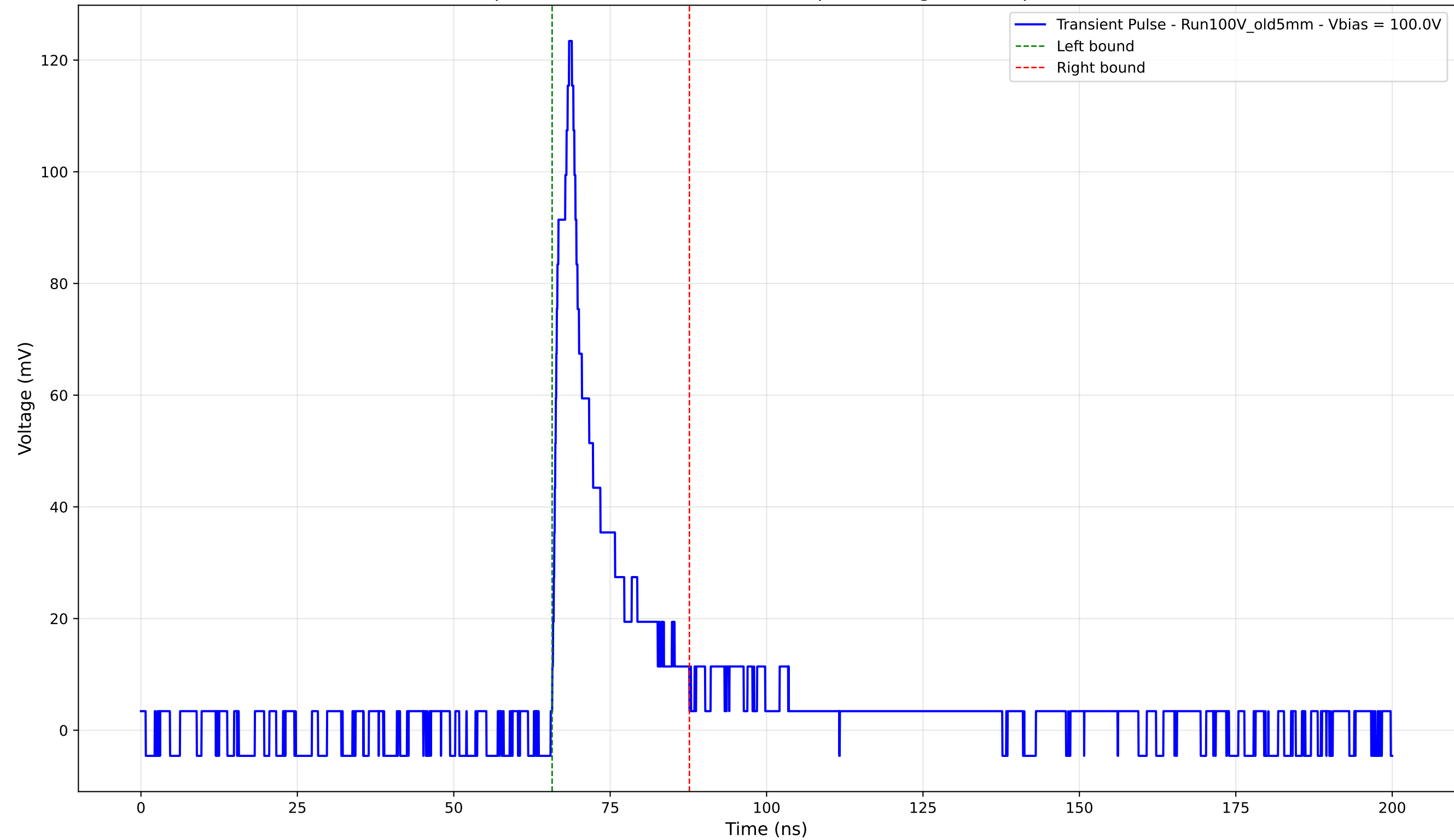
Transient Pulse - Sample: Old5mm - Position: 3255.0 \mu\text{m} - Charge: 17.18 pC - Rise Time: 2.36 ns
