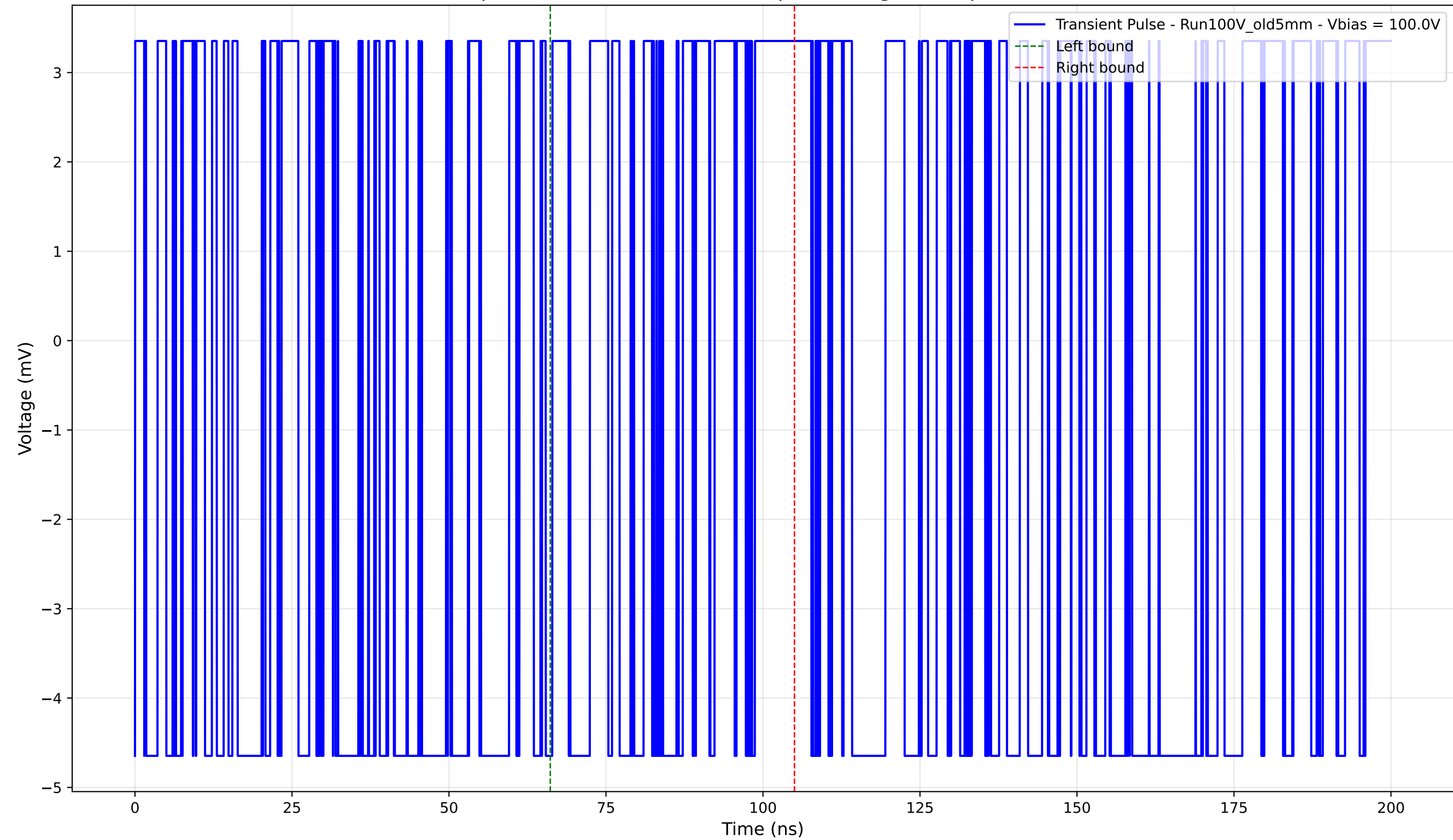
Transient Pulse - Sample: Old5mm - Position: 75.0 \mu\text{m} - Charge: 0.32 pC - Rise Time: 0.00 ns (N/A)
