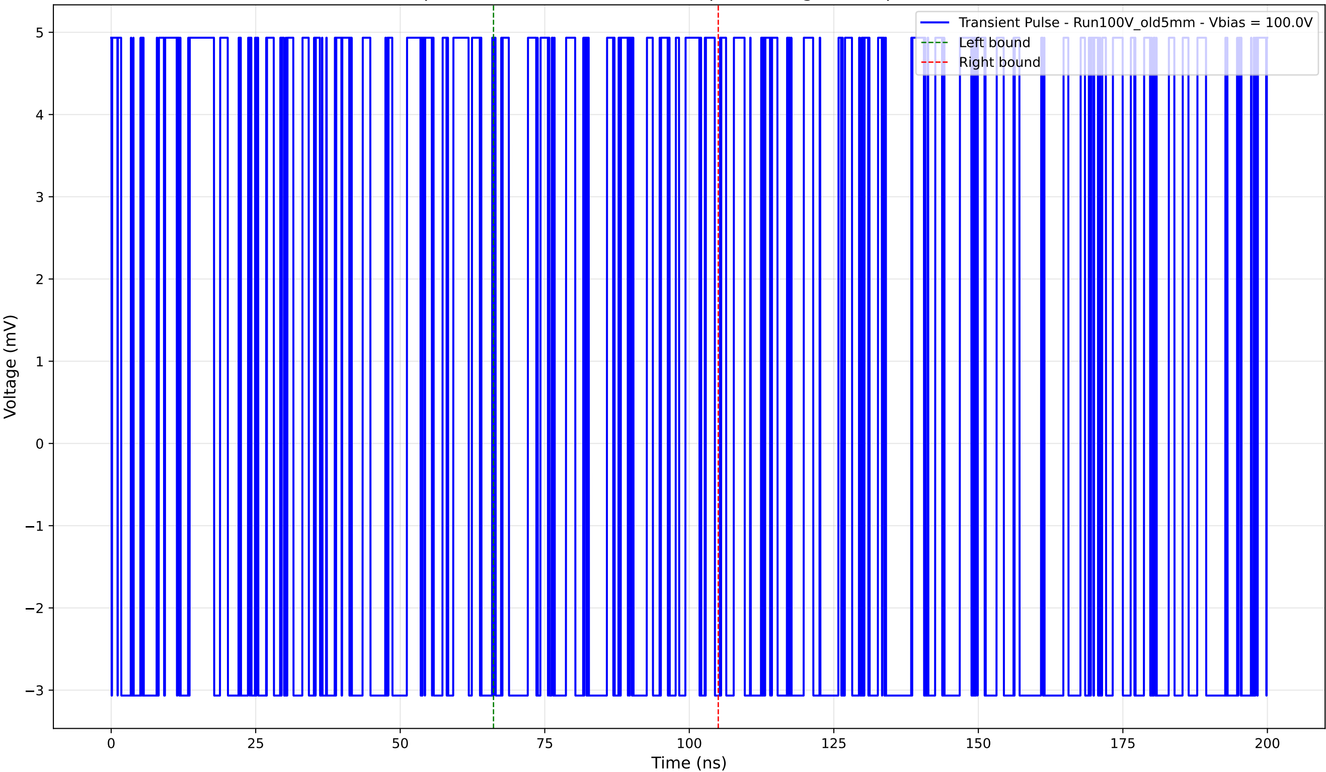
Transient Pulse - Sample: Old5mm - Position: 200.0 \mu\text{m} - Charge: 0.42 pC - Rise Time: 0.00 ns (N/A)
