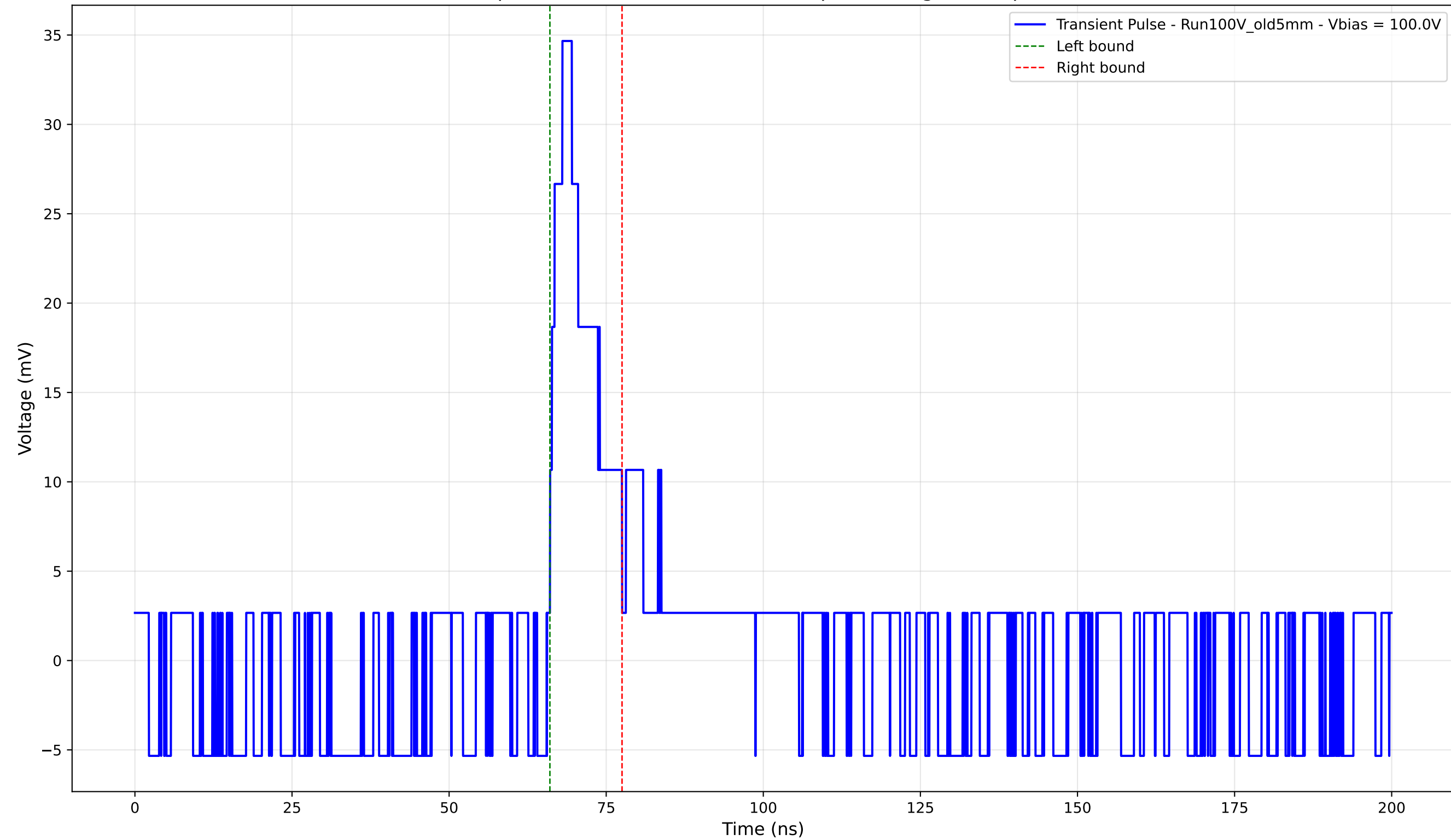
Transient Pulse - Sample: Old5mm - Position: 4245.0 \mu\text{m} - Charge: 4.48 pC - Rise Time: 1.98 ns
