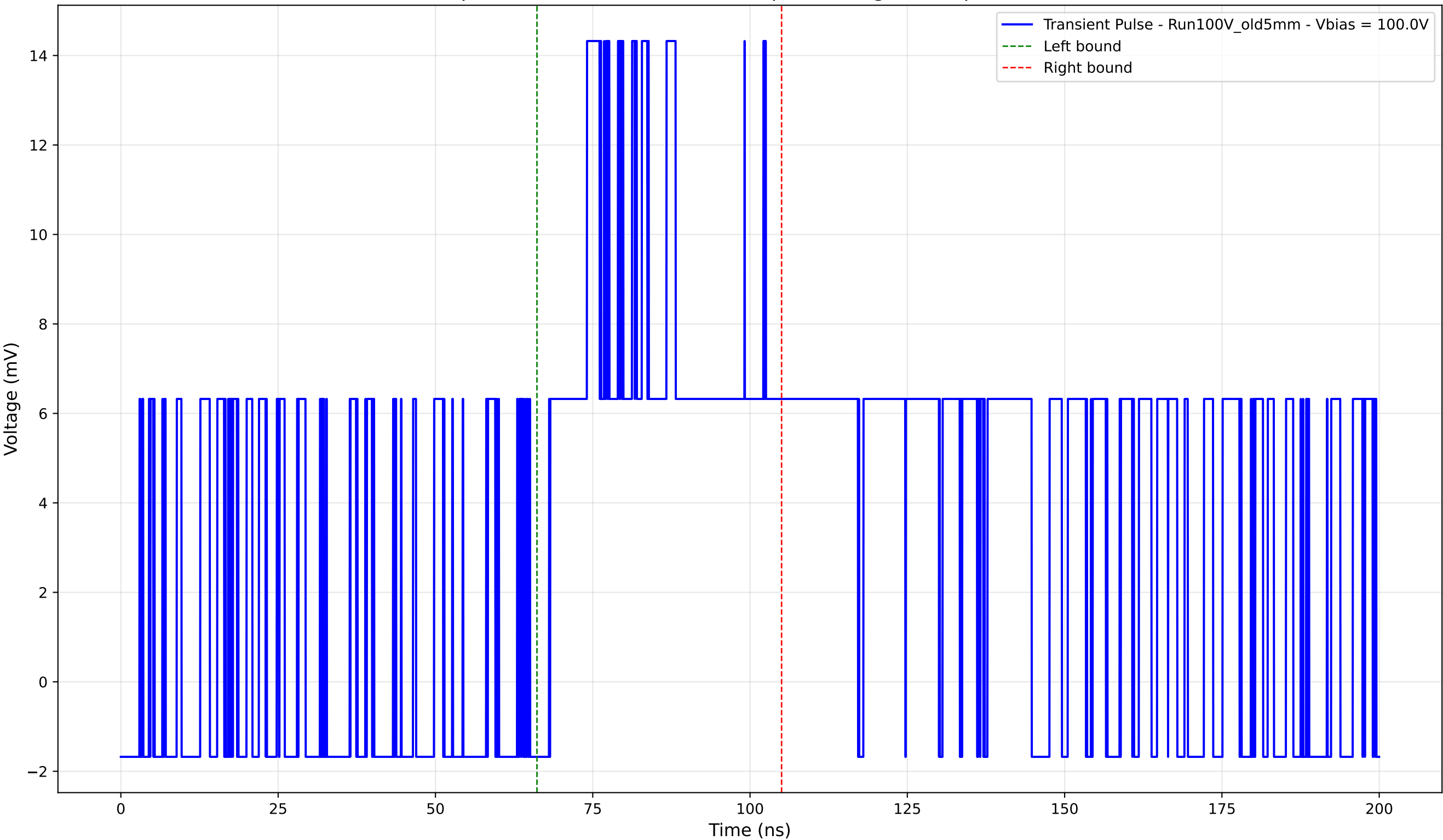
Transient Pulse - Sample: Old5mm - Position: 960.0 \mu\text{m} - Charge: 5.66 pC - Rise Time: 0.00 ns (N/A)
