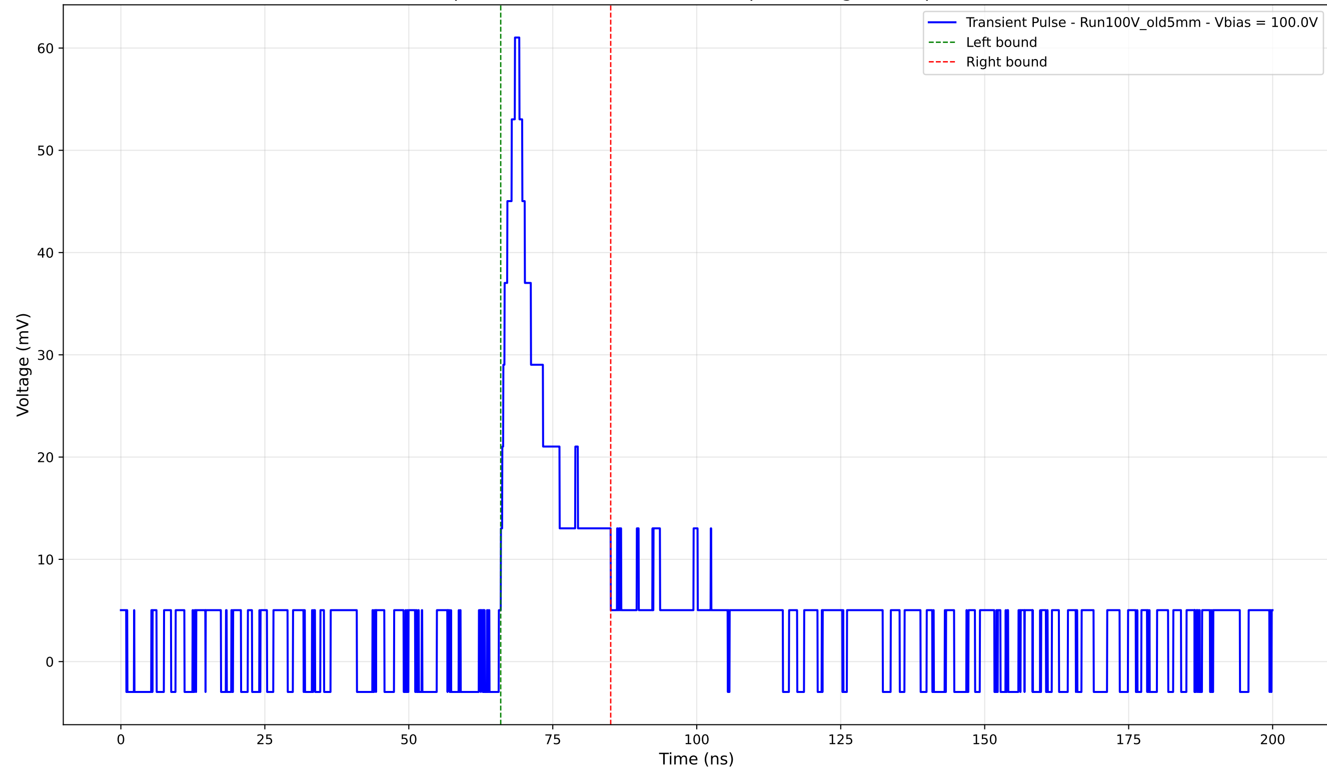
Transient Pulse - Sample: Old5mm - Position: 3175.0 \mu\text{m} - Charge: 9.38 pC - Rise Time: 2.46 ns
