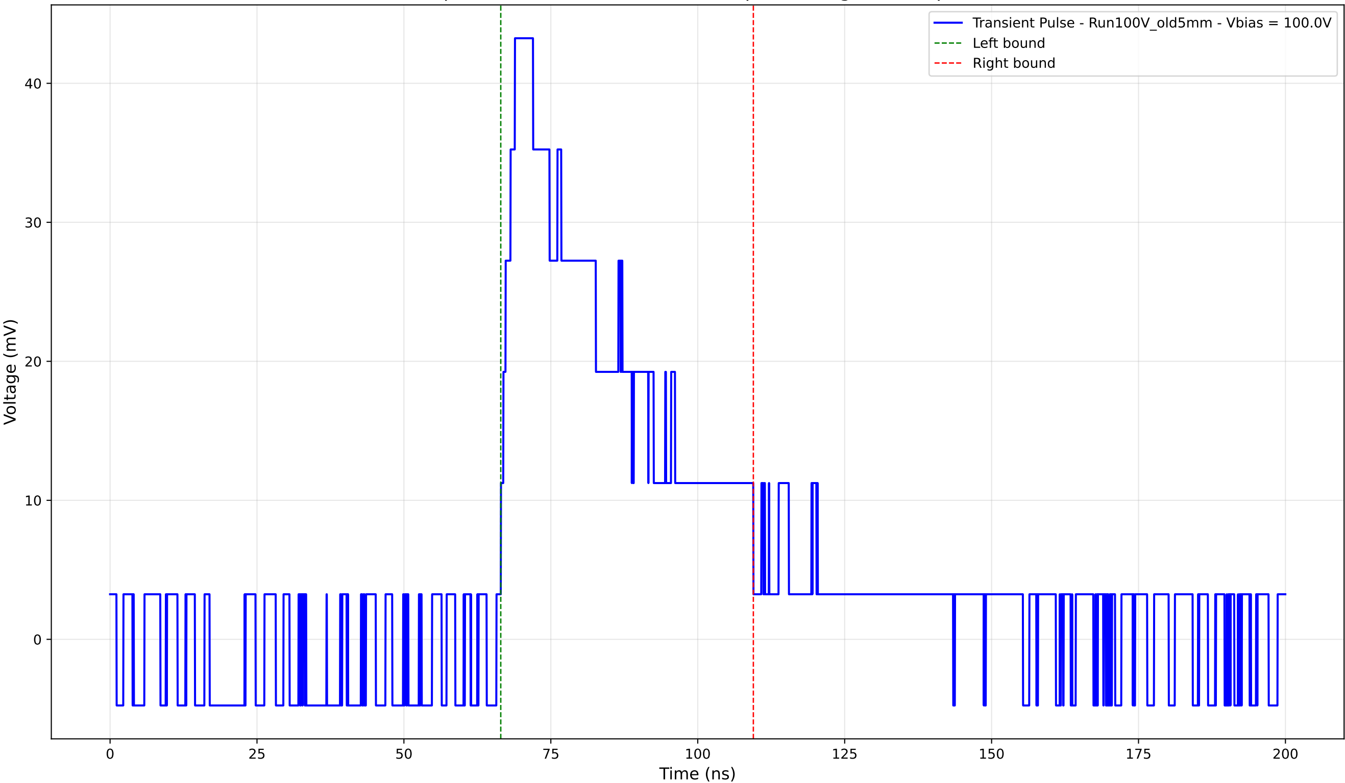
Transient Pulse - Sample: Old5mm - Position: 4850.0 \mu\text{m} - Charge: 18.06 pC - Rise Time: 2.40 ns
