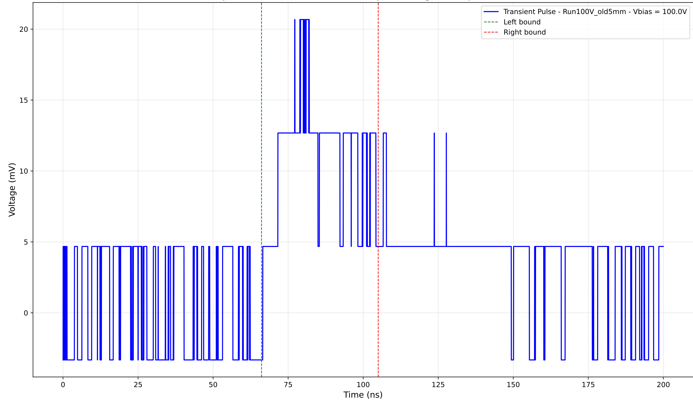
Transient Pulse - Sample: Old5mm - Position: 1425.0 \mu\text{m} - Charge: 8.54 pC - Rise Time: 0.00 ns (N/A)
