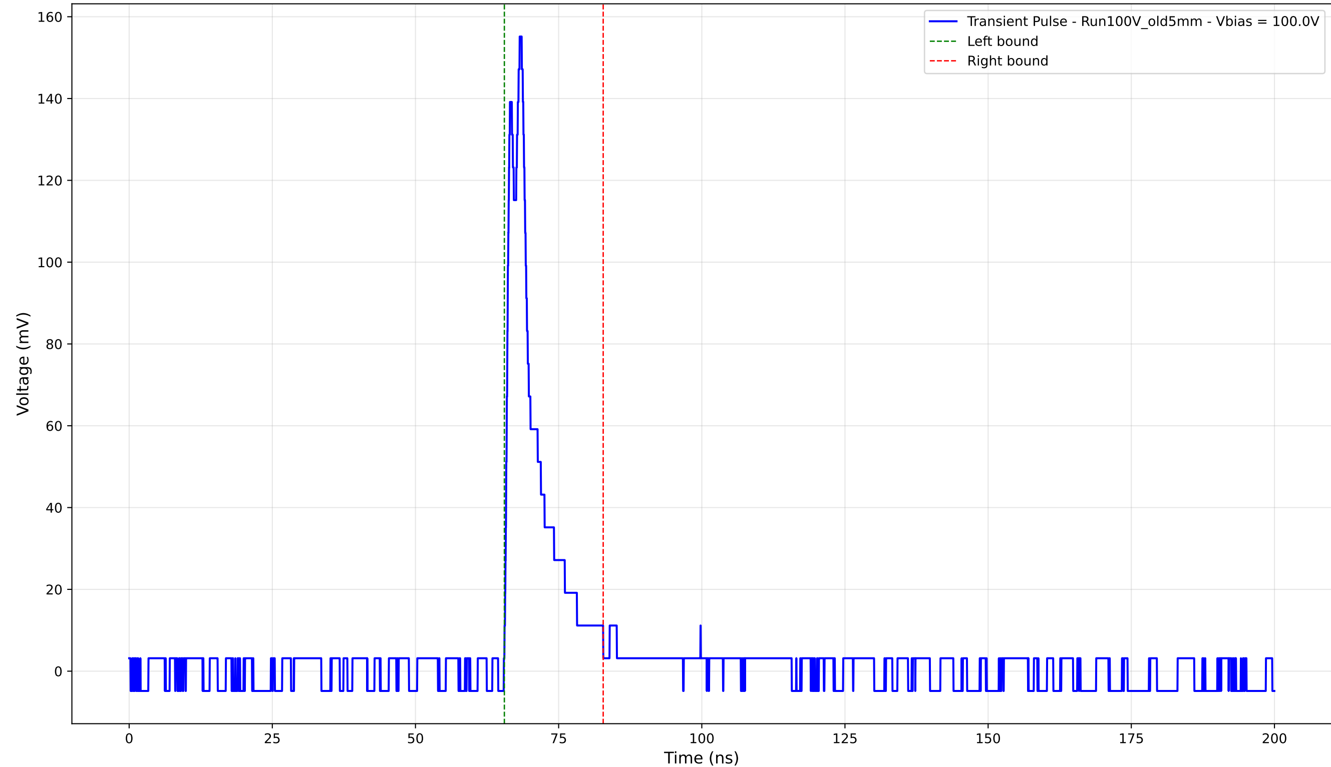
Transient Pulse - Sample: Old5mm - Position: 3910.0 \mu\text{m} - Charge: 16.66 pC - Rise Time: 2.37 ns
