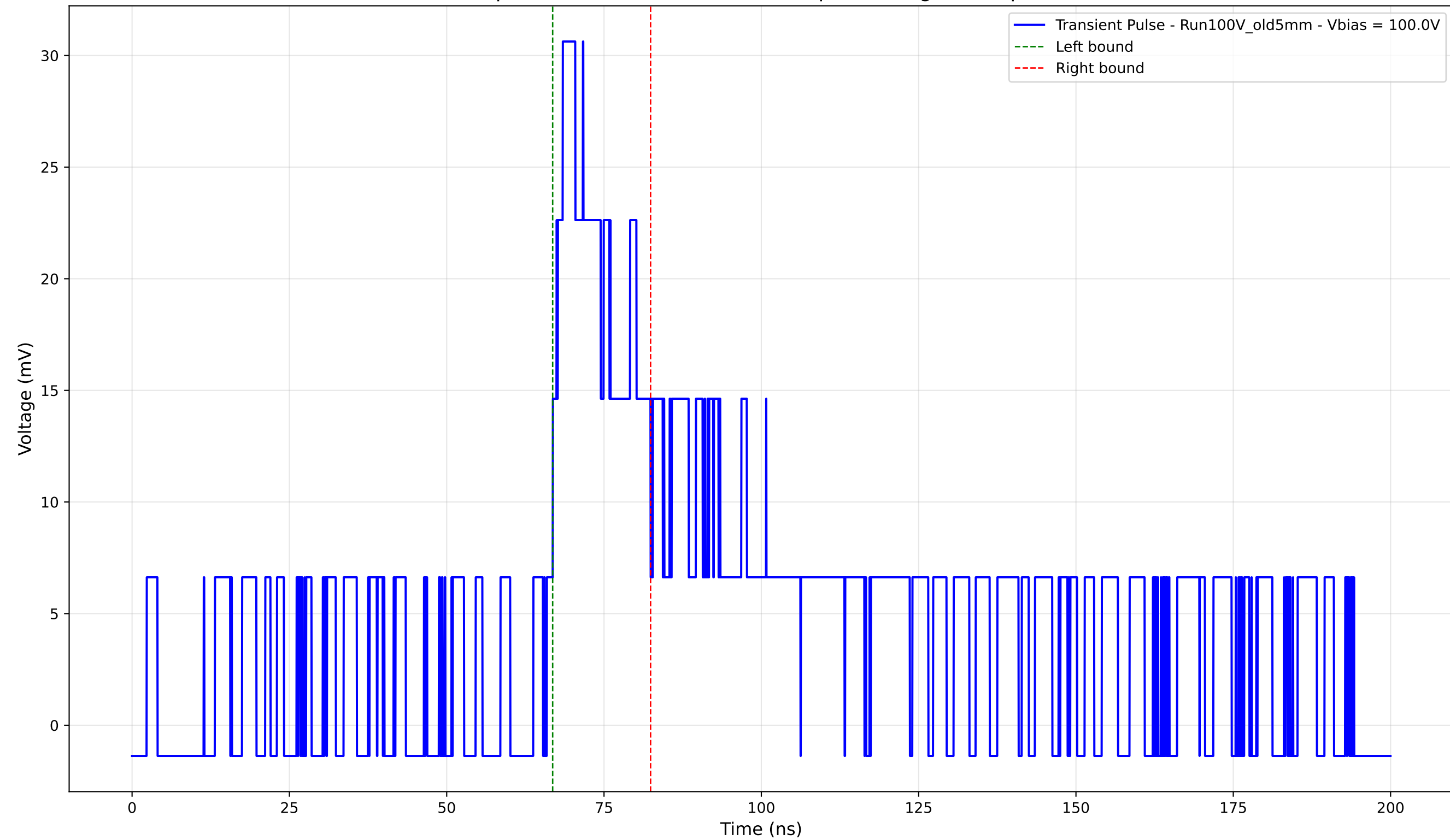
Transient Pulse - Sample: Old5mm - Position: 4690.0 \mu\text{m} - Charge: 6.30 pC - Rise Time: 2.55 ns
