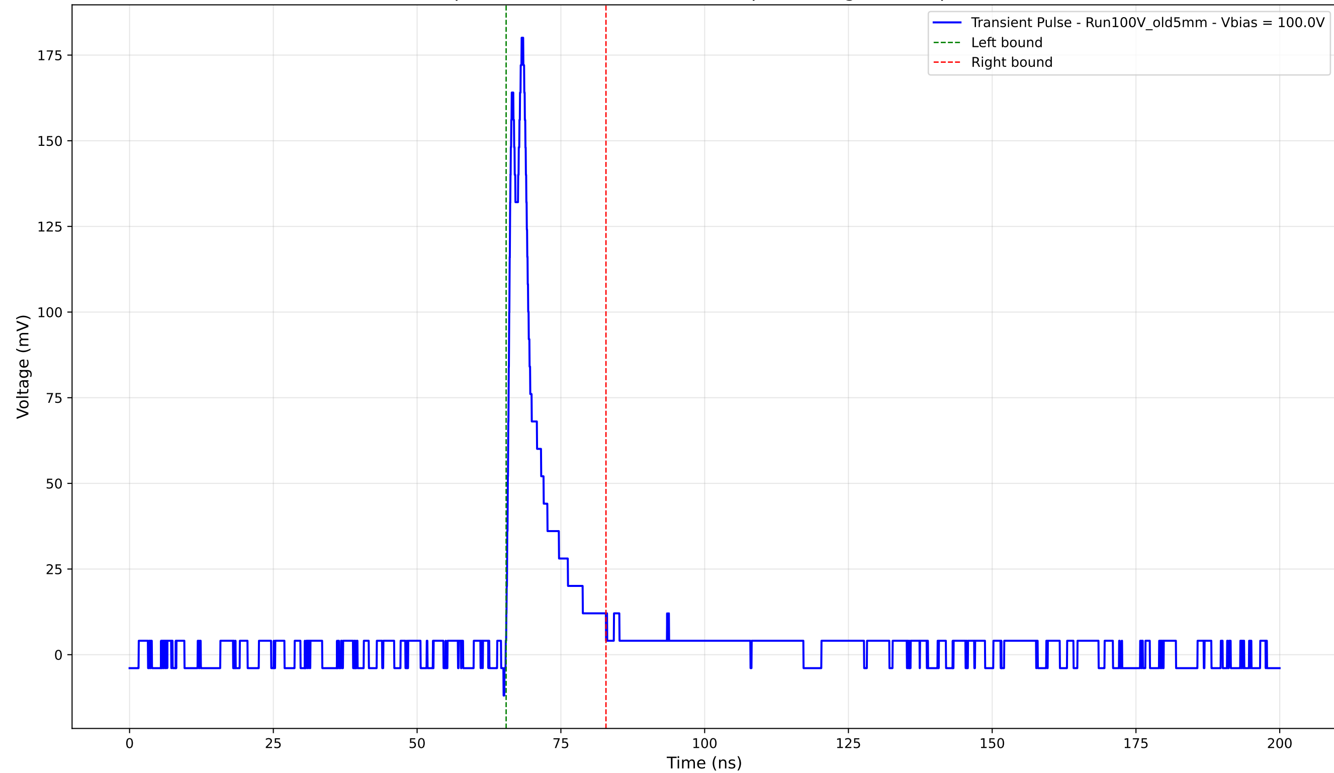
Transient Pulse - Sample: Old5mm - Position: 3880.0 \mu\text{m} - Charge: 18.81 pC - Rise Time: 0.89 ns
