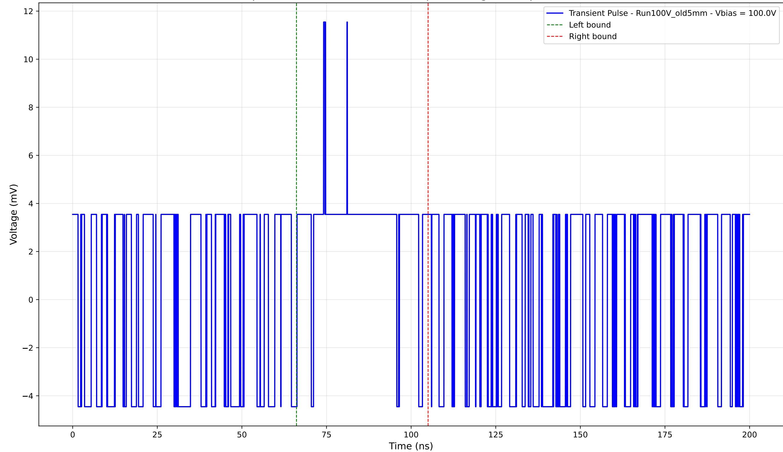
Transient Pulse - Sample: Old5mm - Position: 1730.0 \mu\text{m} - Charge: 2.44 pC - Rise Time: 0.00 ns (N/A)
