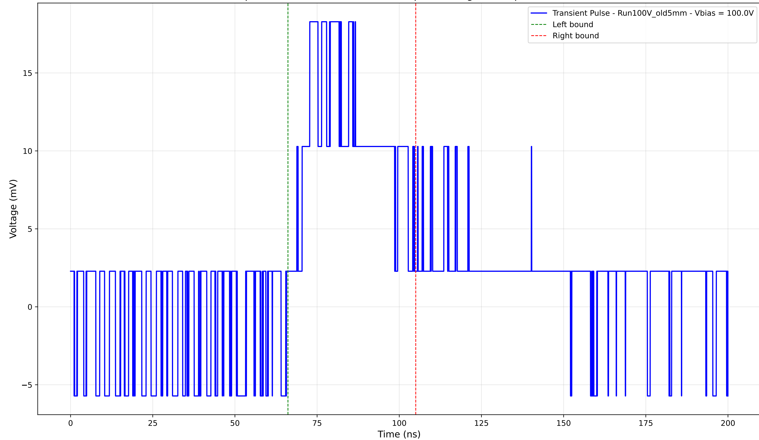
Transient Pulse - Sample: Old5mm - Position: 1630.0 \mu\text{m} - Charge: 8.30 pC - Rise Time: 0.00 ns (N/A)
