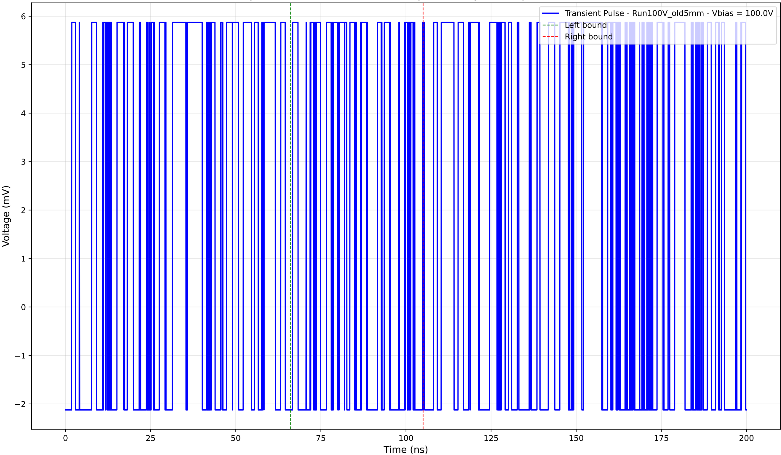
Transient Pulse - Sample: Old5mm - Position: 245.0 \mu\text{m} - Charge: 1.29 pC - Rise Time: 0.00 ns (N/A)
