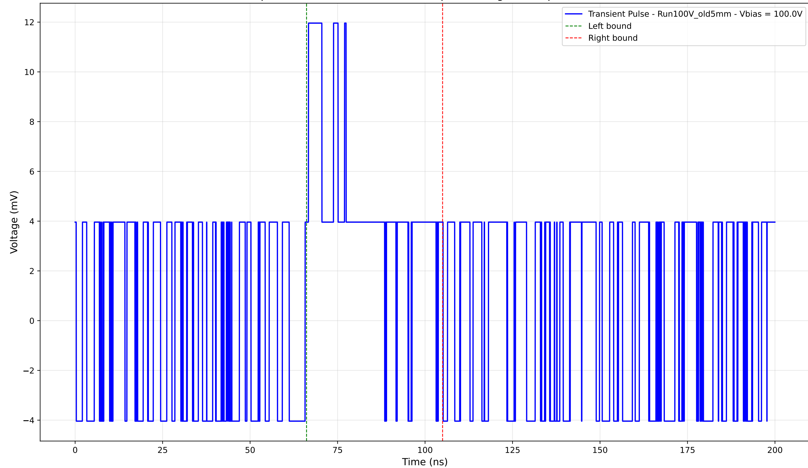
Transient Pulse - Sample: Old5mm - Position: 3060.0 \mu\text{m} - Charge: 3.69 pC - Rise Time: 0.00 ns (N/A)
