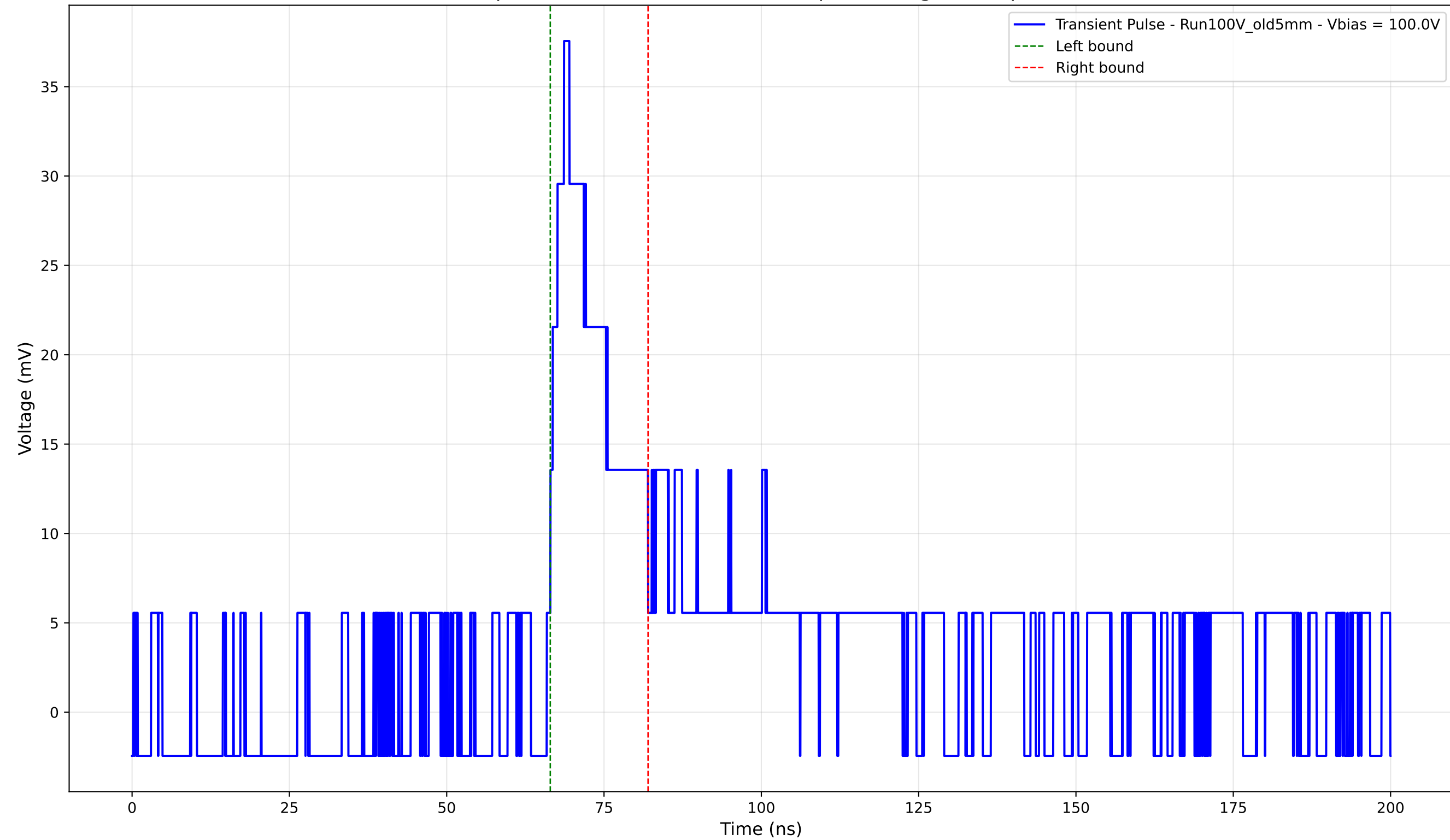
Transient Pulse - Sample: Old5mm - Position: 4545.0 \mu\text{m} - Charge: 6.40 pC - Rise Time: 2.75 ns
