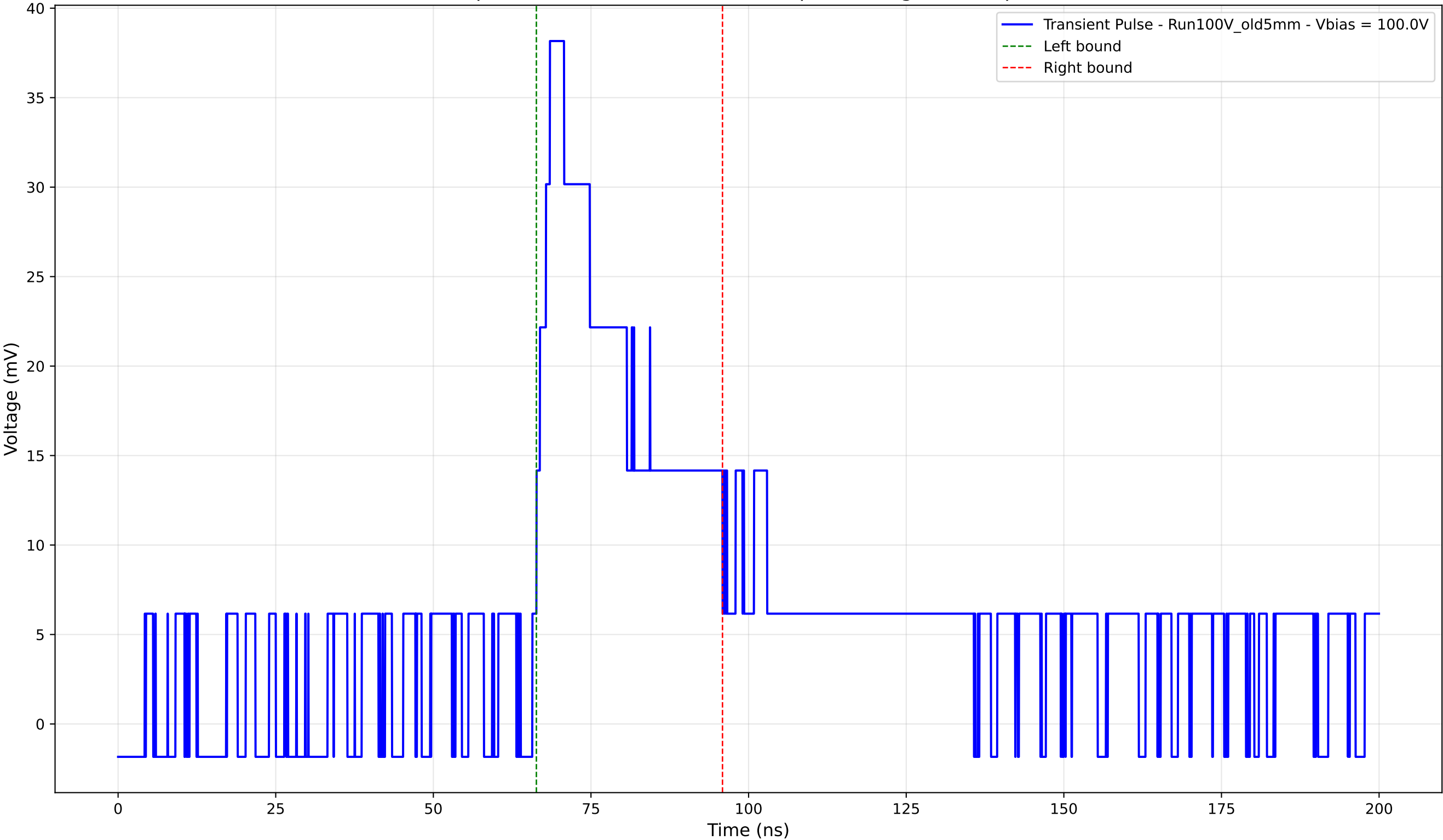
Transient Pulse - Sample: Old5mm - Position: 4705.0 \mu\text{m} - Charge: 12.08 pC - Rise Time: 2.79 ns
