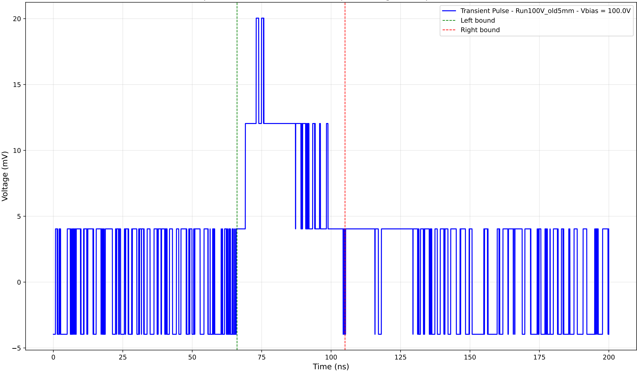
Transient Pulse - Sample: Old5mm - Position: 355.0 \mu\text{m} - Charge: 7.17 pC - Rise Time: 0.00 ns (N/A)
