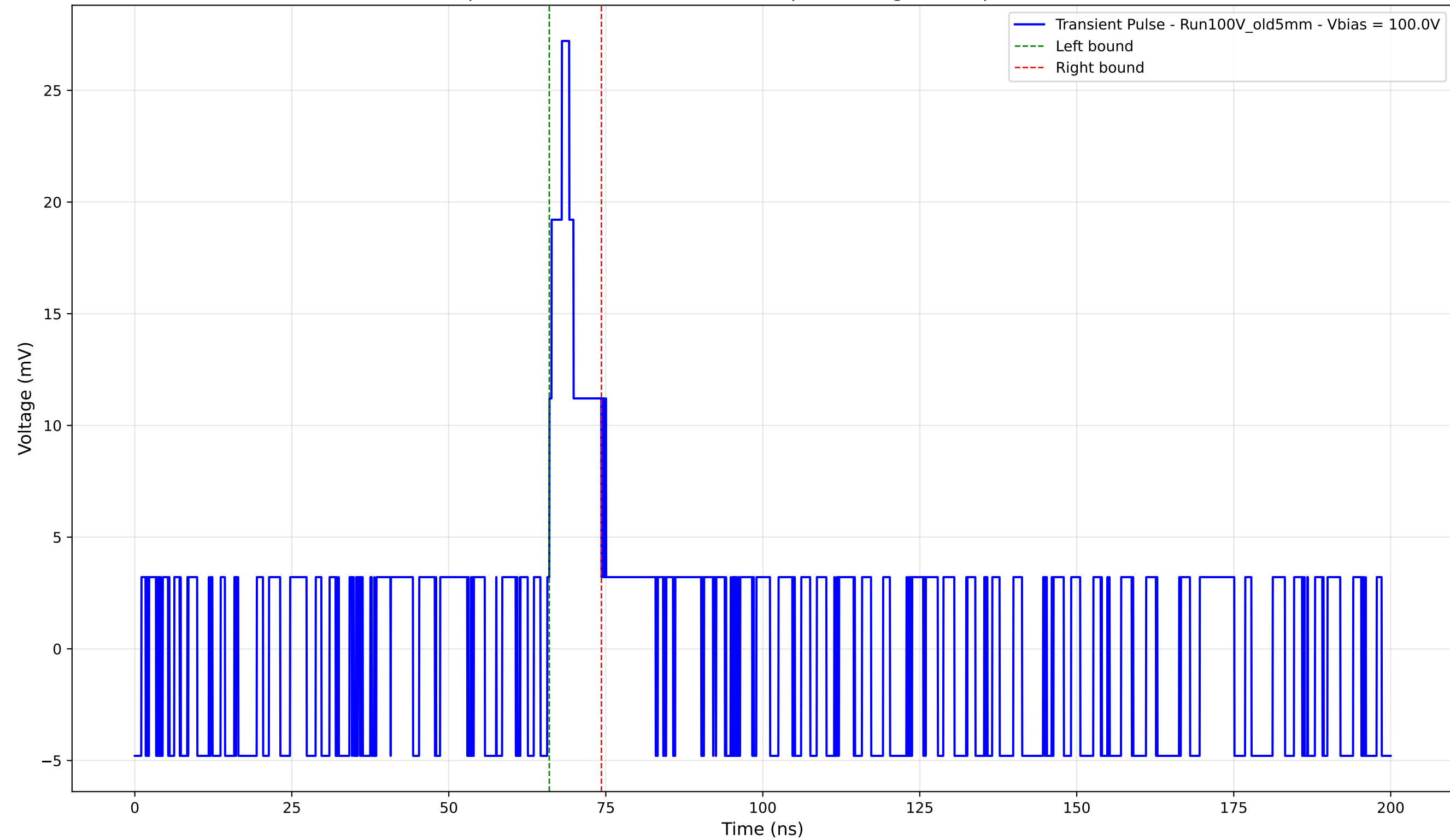
Transient Pulse - Sample: Old5mm - Position: 4055.0 \mu\text{m} - Charge: 2.61 pC - Rise Time: 0.00 ns (N/A)
