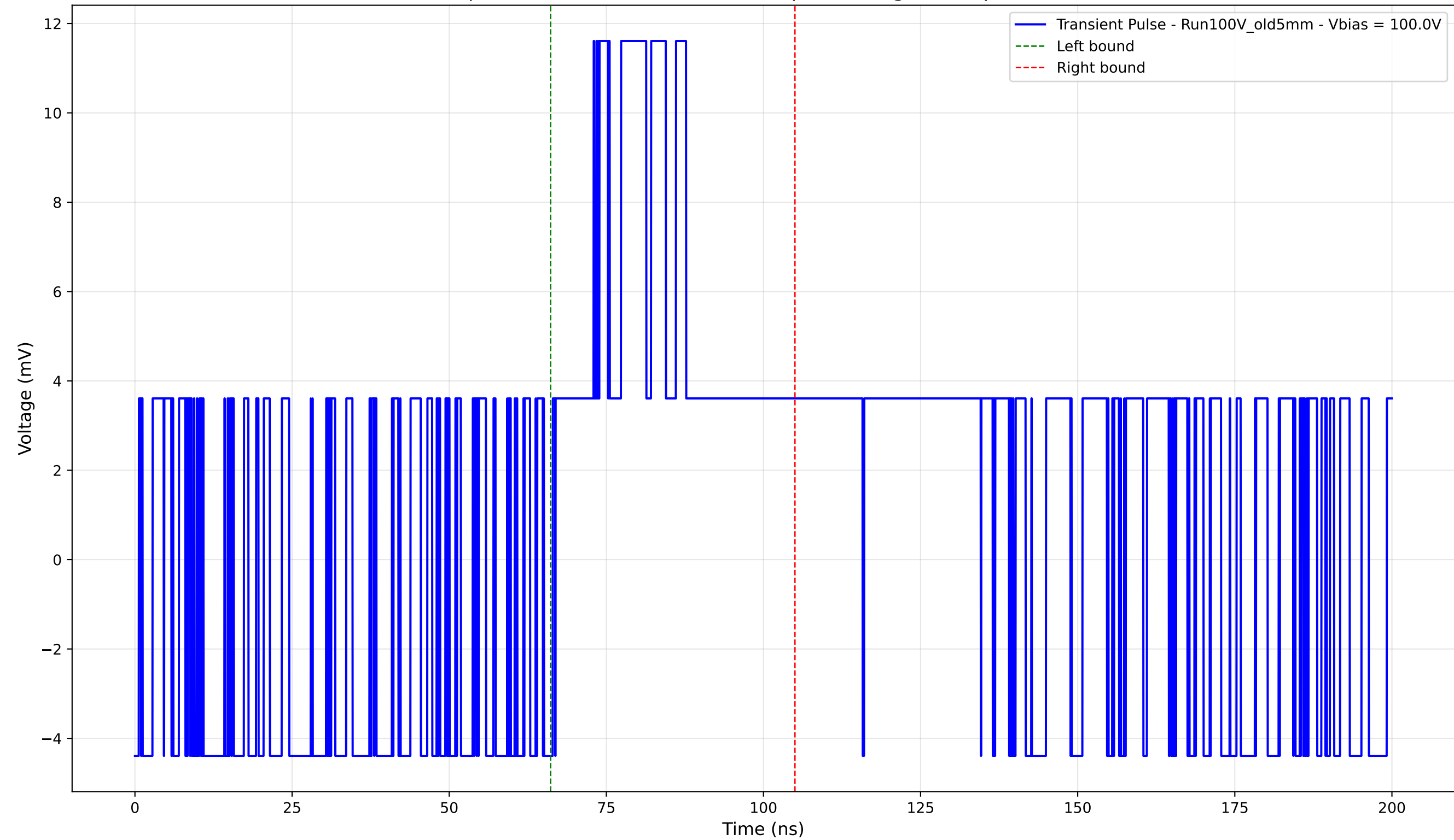
Transient Pulse - Sample: Old5mm - Position: 1755.0 \mu\text{m} - Charge: 4.33 pC - Rise Time: 0.00 ns (N/A)
