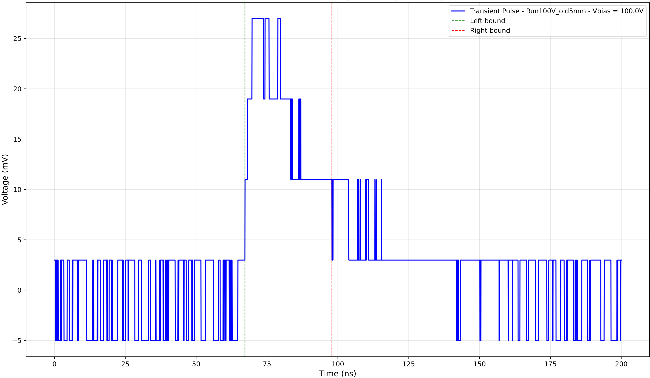
Transient Pulse - Sample: Old5mm - Position: 2405.0 \mu\text{m} - Charge: 10.33 pC - Rise Time: 0.00 ns (N/A)
