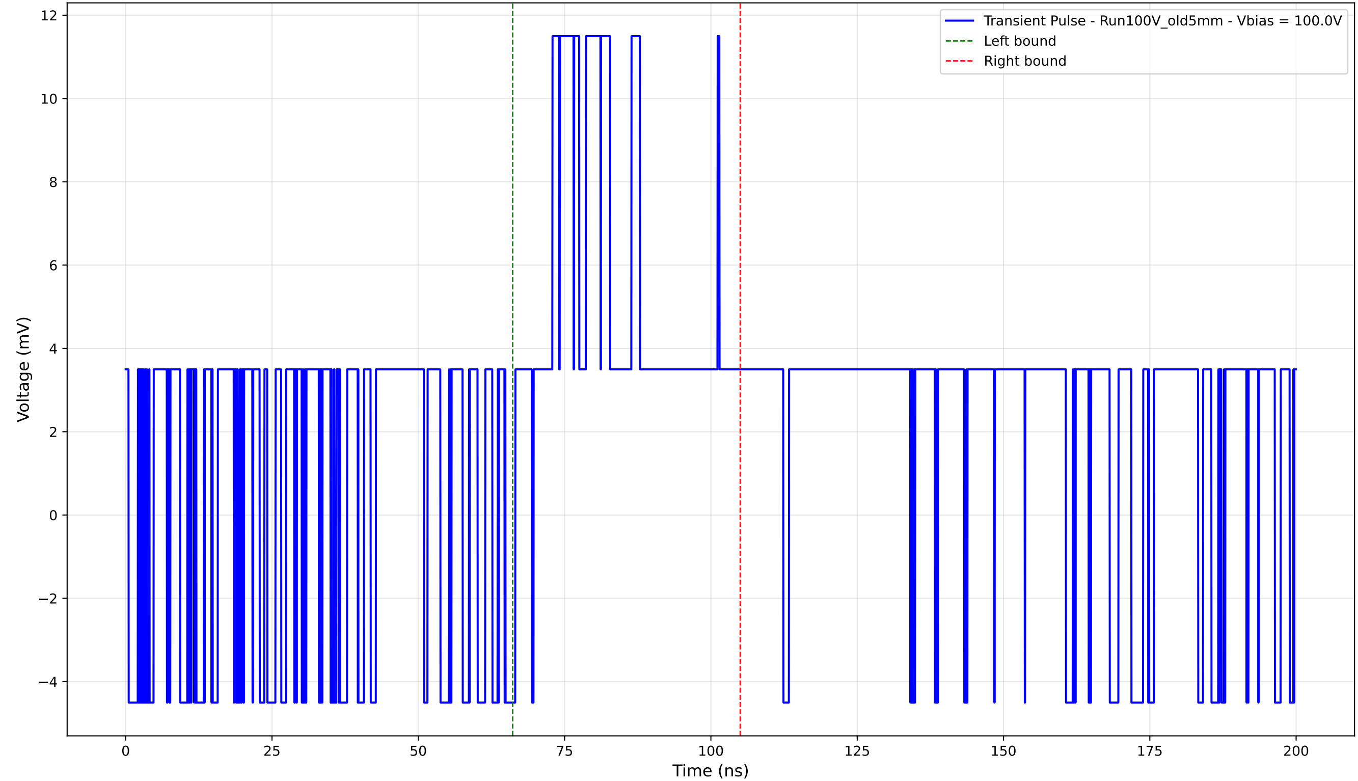
Transient Pulse - Sample: Old5mm - Position: 1550.0 \mu\text{m} - Charge: 4.24 pC - Rise Time: 0.00 ns (N/A)
