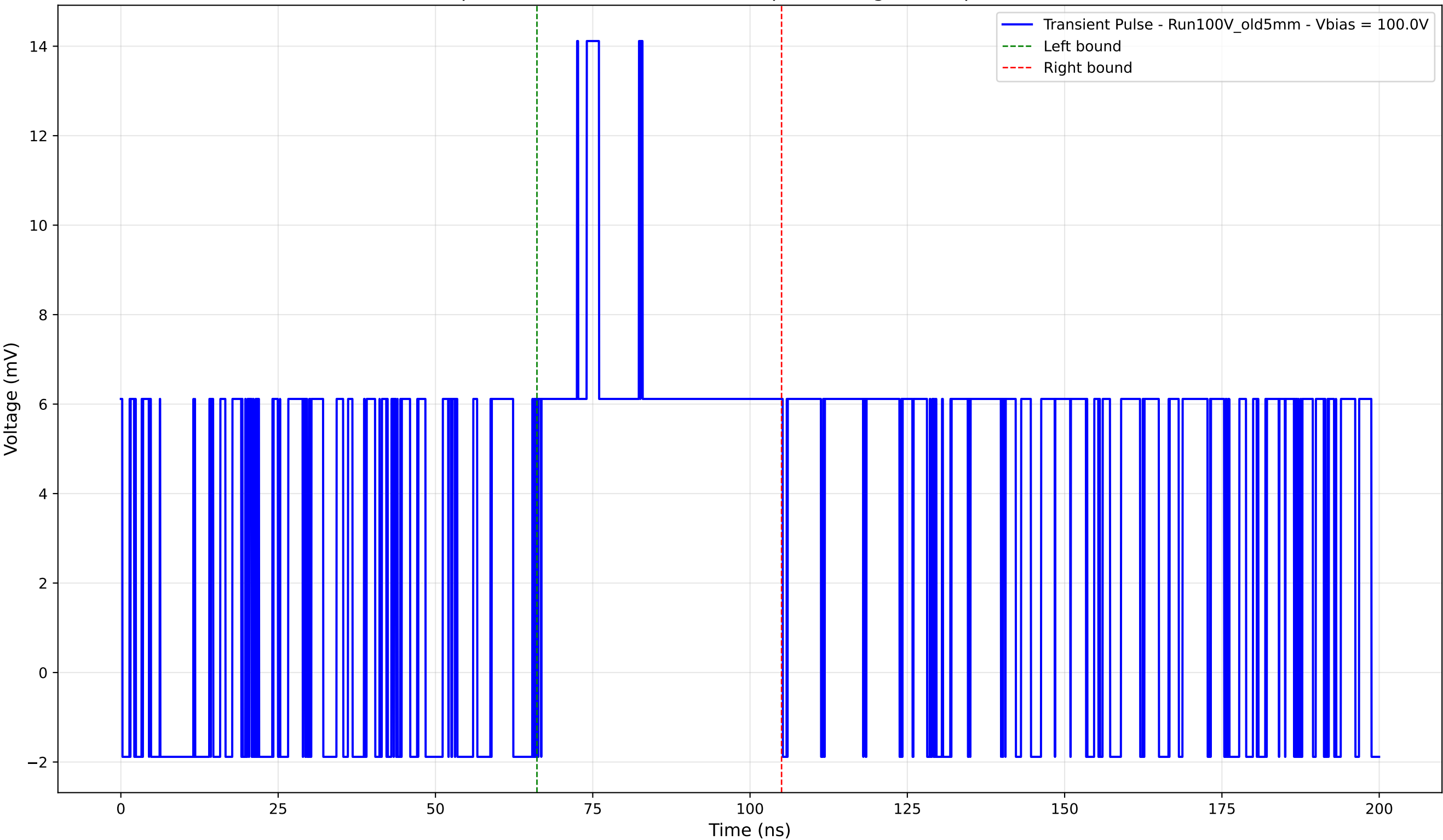
Transient Pulse - Sample: Old5mm - Position: 410.0 \mu\text{m} - Charge: 5.16 pC - Rise Time: 0.00 ns (N/A)
