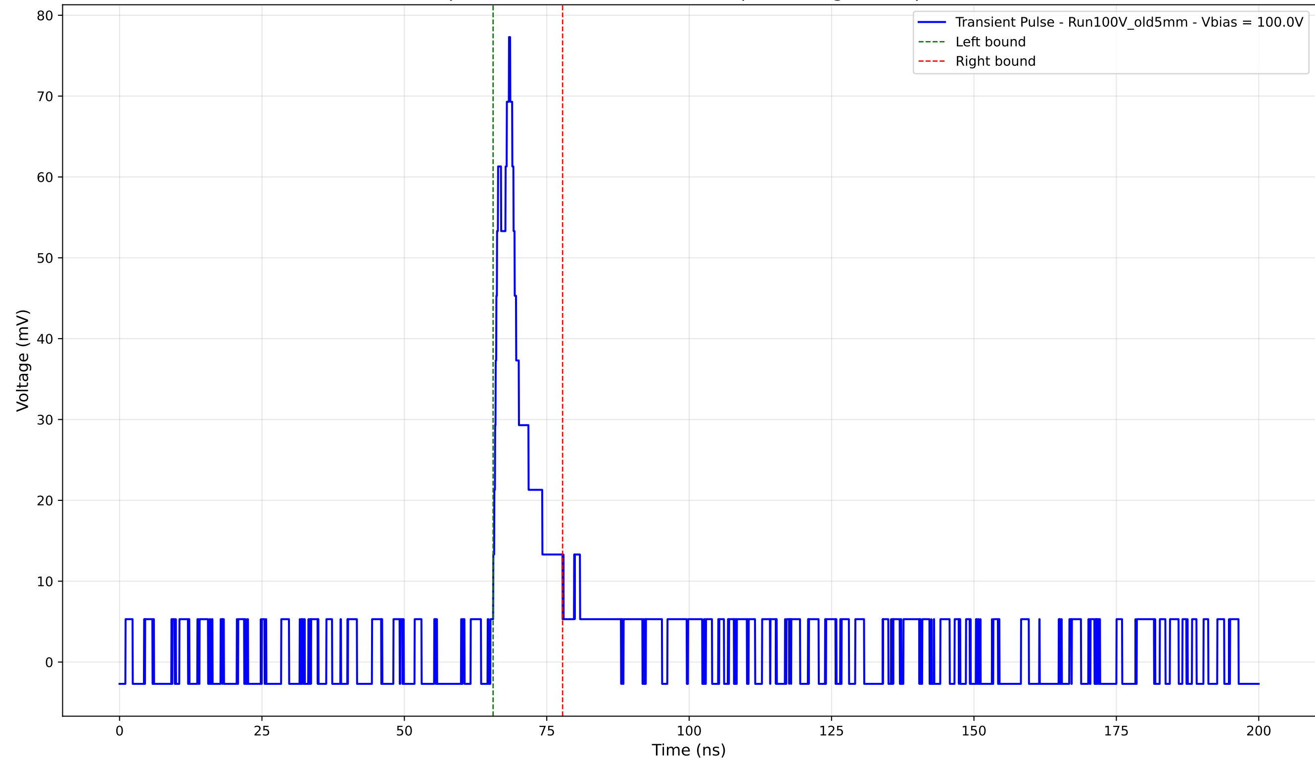
Transient Pulse - Sample: Old5mm - Position: 3470.0 \mu\text{m} - Charge: 7.74 pC - Rise Time: 2.77 ns
