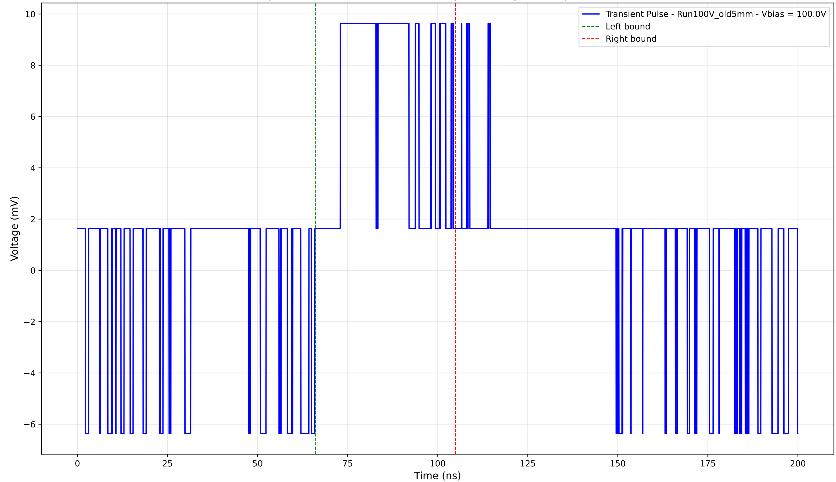
Transient Pulse - Sample: Old5mm - Position: 1455.0 \mu\text{m} - Charge: 4.99 pC - Rise Time: 0.00 ns (N/A)
