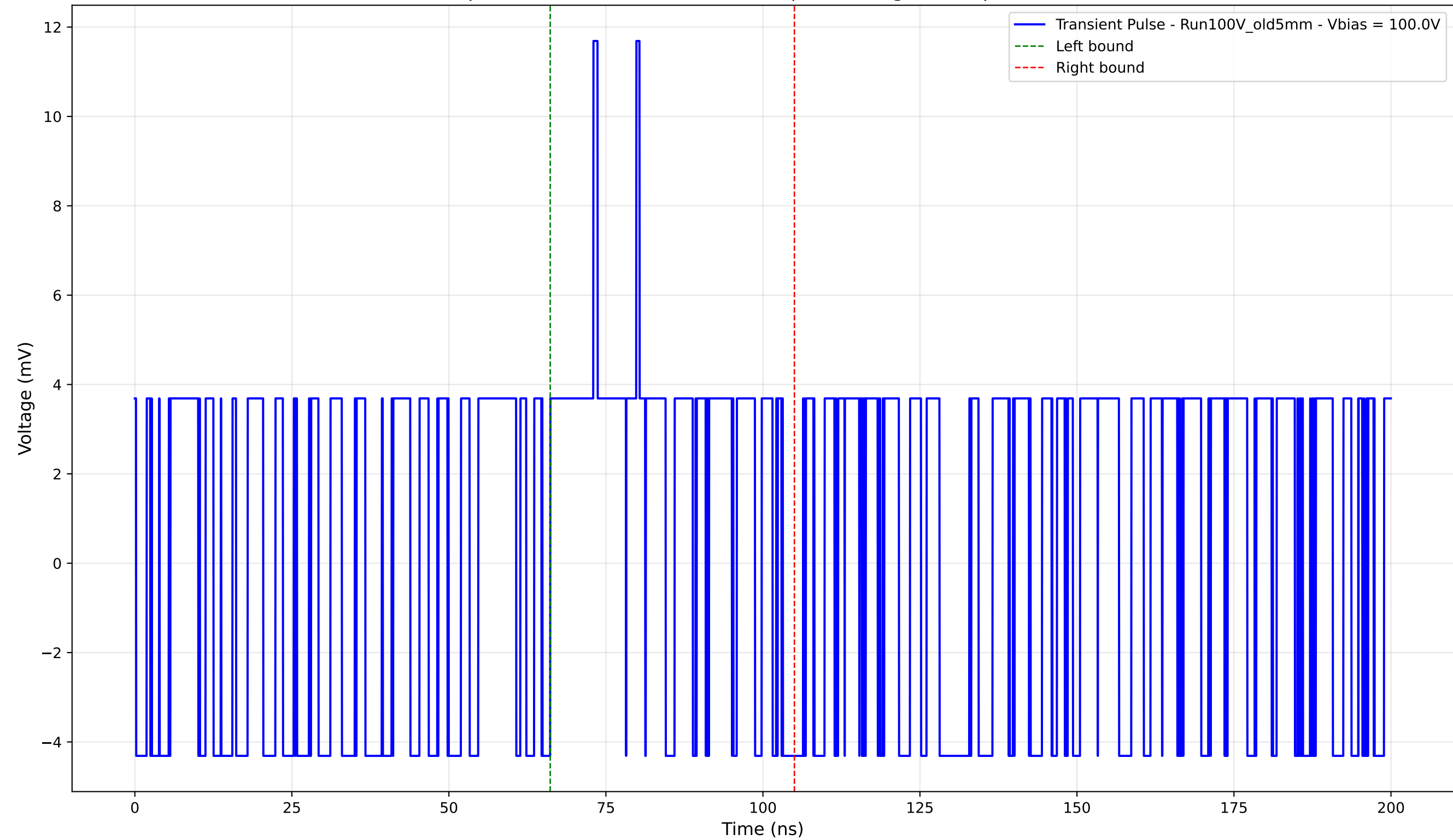
Transient Pulse - Sample: Old5mm - Position: 2815.0 \mu\text{m} - Charge: 2.01 pC - Rise Time: 0.00 ns (N/A)
