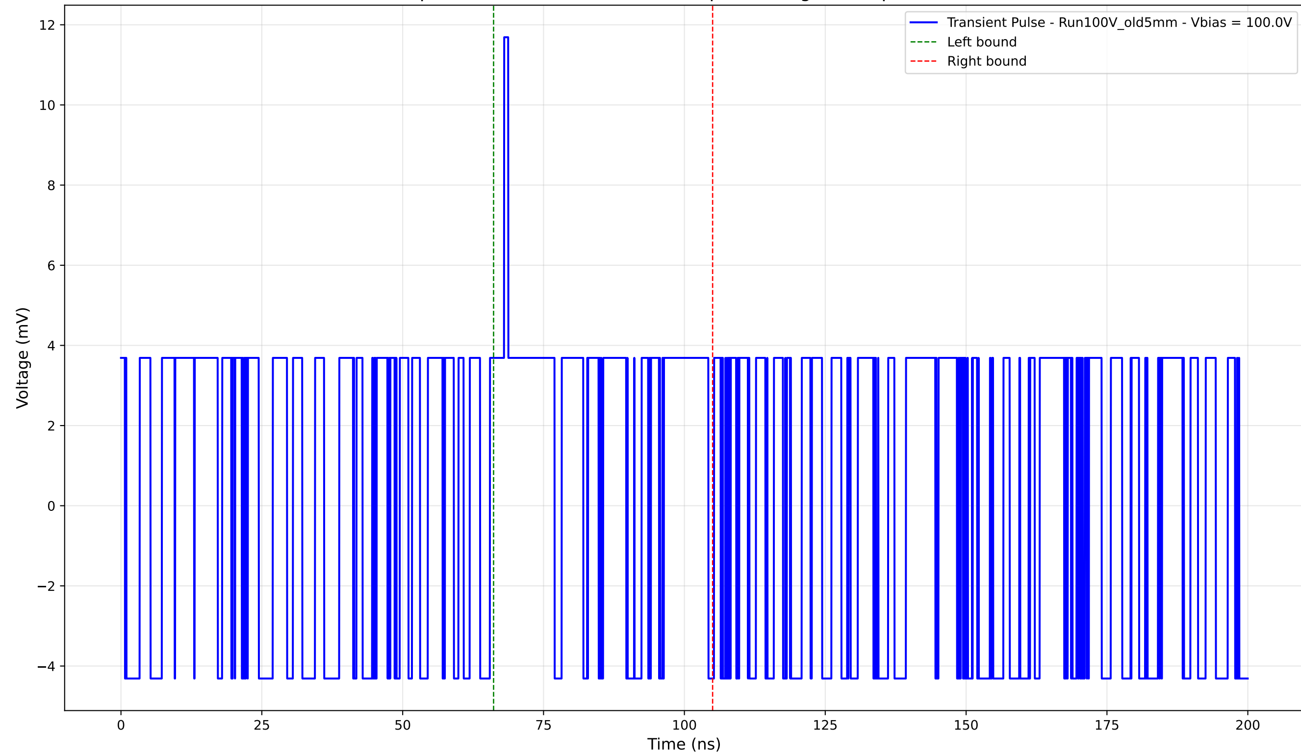
Transient Pulse - Sample: Old5mm - Position: 3420.0 \mu\text{m} - Charge: 1.88 pC - Rise Time: 0.00 ns (N/A)
