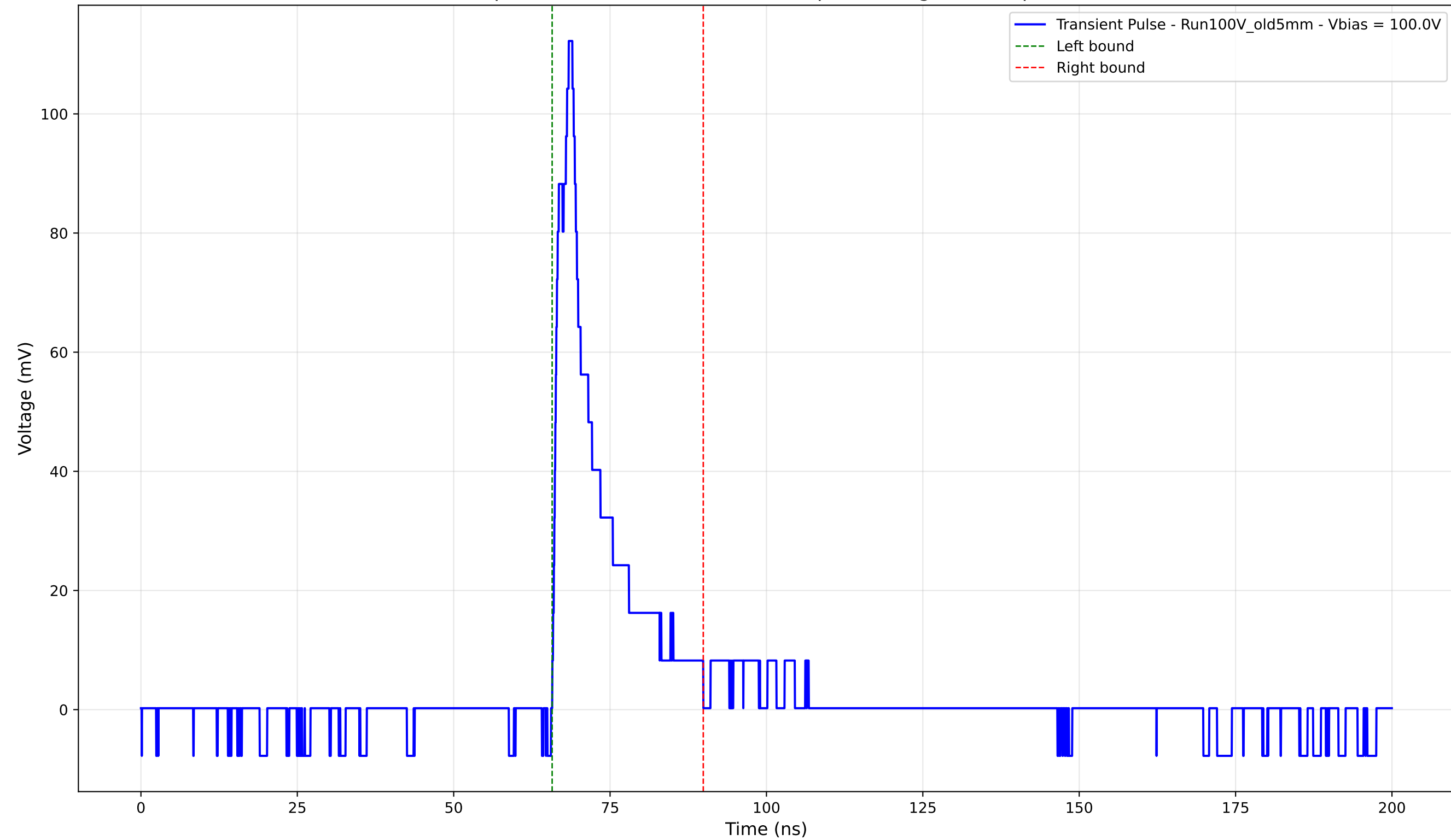
Transient Pulse - Sample: Old5mm - Position: 4155.0 \mu\text{m} - Charge: 15.72 pC - Rise Time: 2.25 ns
