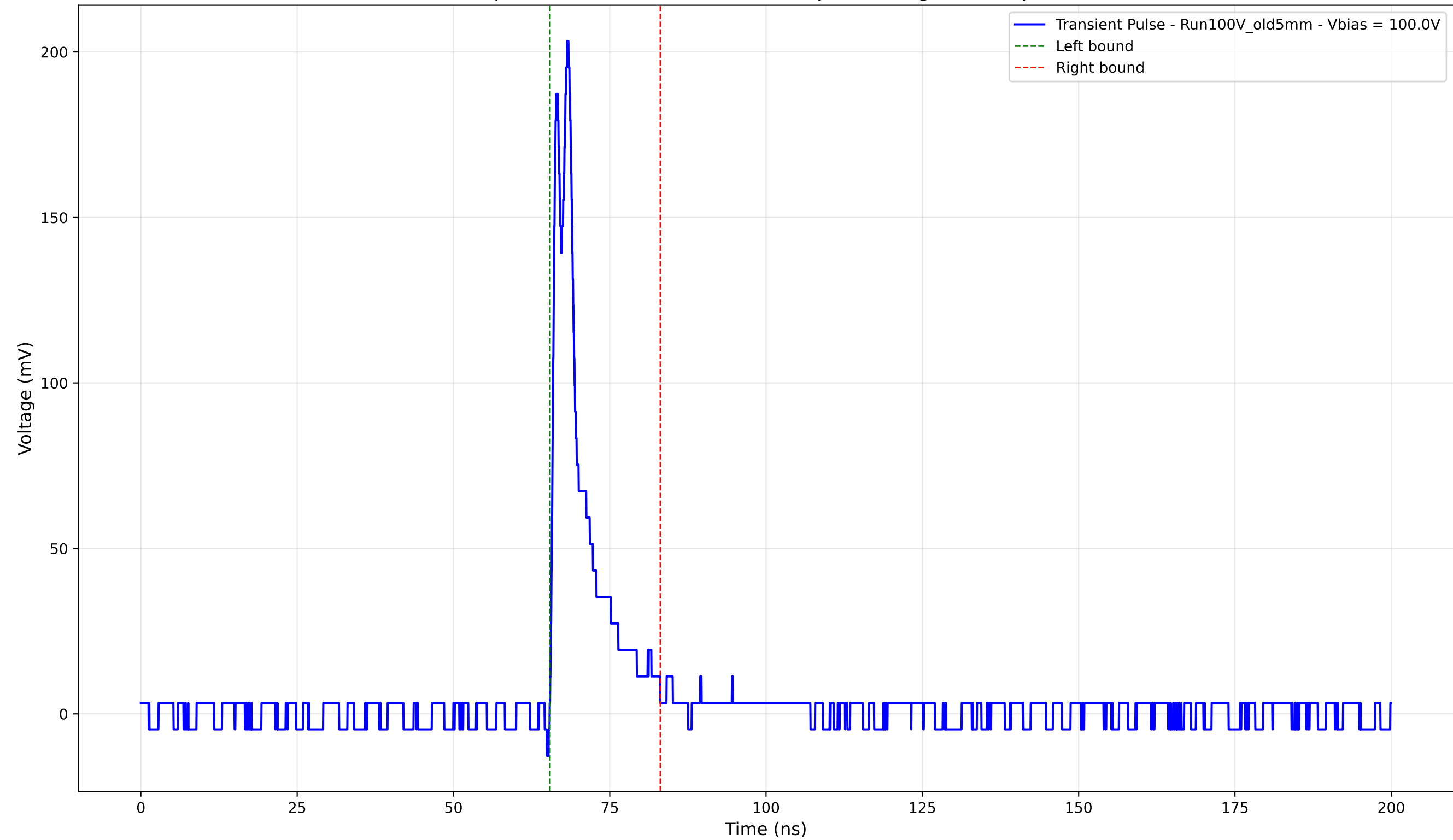
Transient Pulse - Sample: Old5mm - Position: 3560.0 \mu\text{m} - Charge: 20.45 pC - Rise Time: 0.84 ns
