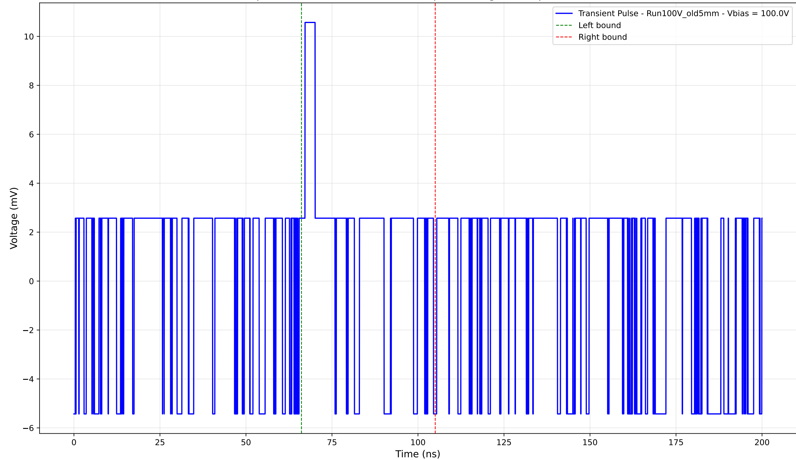
Transient Pulse - Sample: Old5mm - Position: 4275.0 \mu\text{m} - Charge: 1.45 pC - Rise Time: 0.00 ns (N/A)
