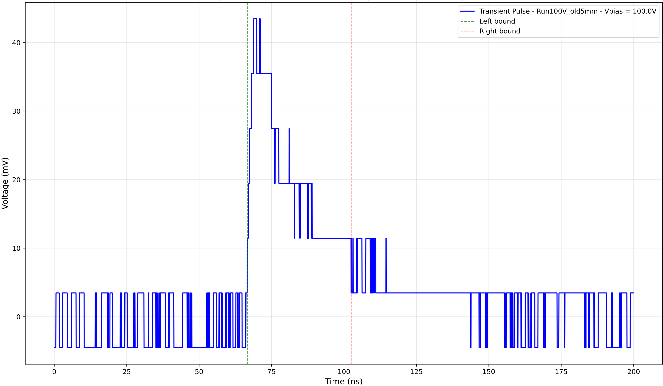
Transient Pulse - Sample: Old5mm - Position: 2670.0 \mu\text{m} - Charge: 14.58 pC - Rise Time: 2.22 ns
