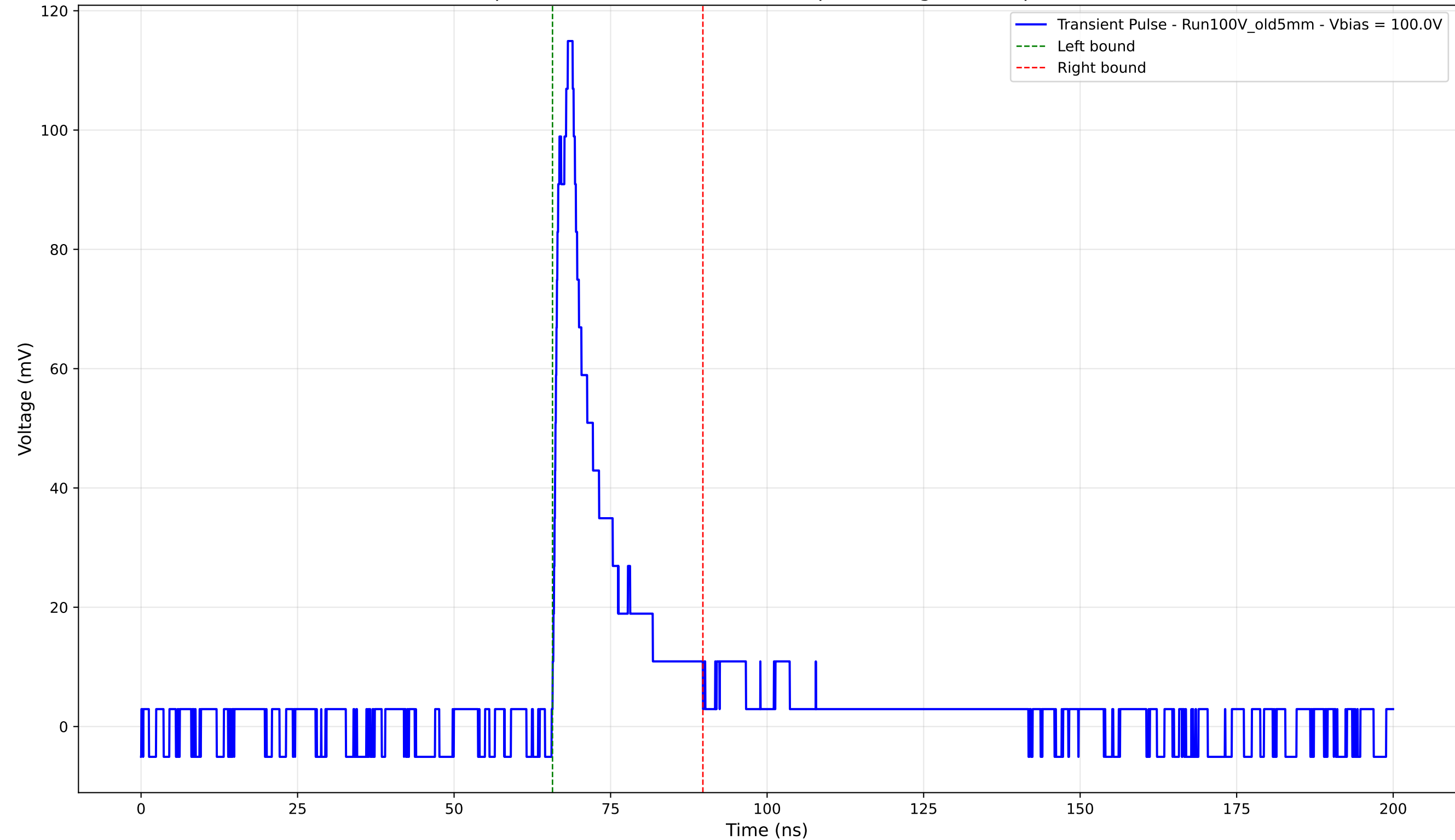
Transient Pulse - Sample: Old5mm - Position: 3290.0 \mu\text{m} - Charge: 16.66 pC - Rise Time: 2.06 ns
