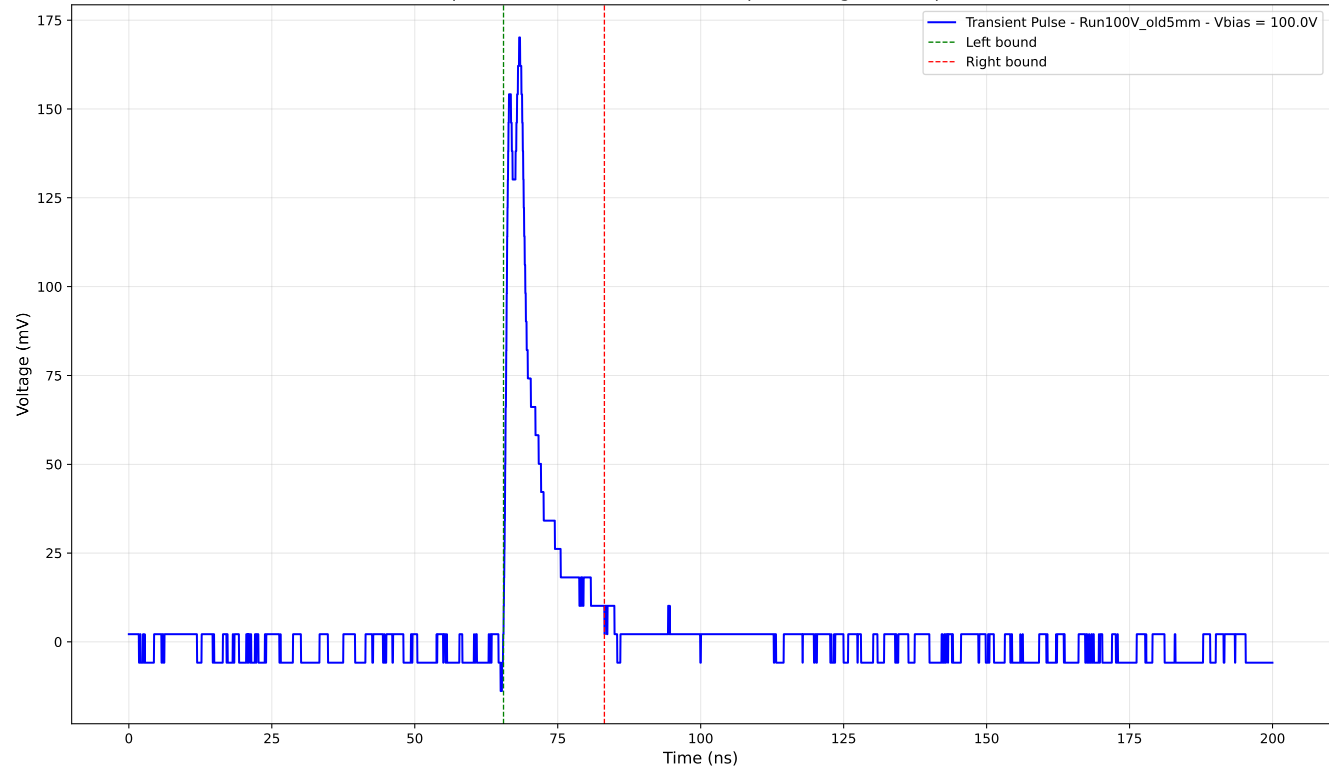
Transient Pulse - Sample: Old5mm - Position: 3520.0 \mu\text{m} - Charge: 18.01 pC - Rise Time: 0.86 ns
