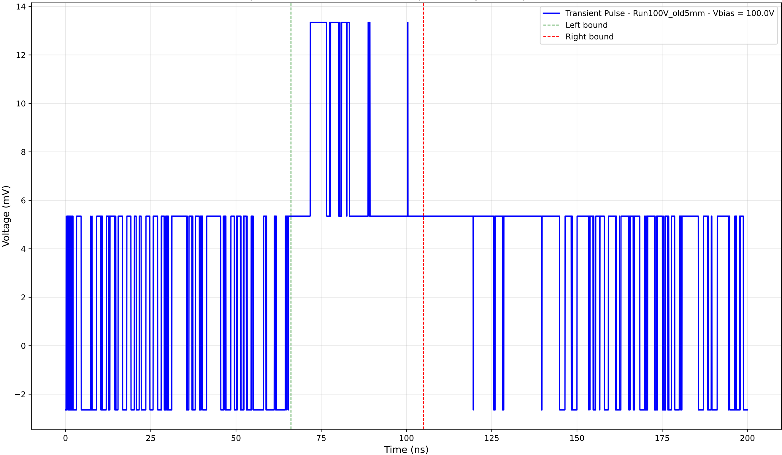
Transient Pulse - Sample: Old5mm - Position: 575.0 \mu\text{m} - Charge: 5.74 pC - Rise Time: 0.00 ns (N/A)
