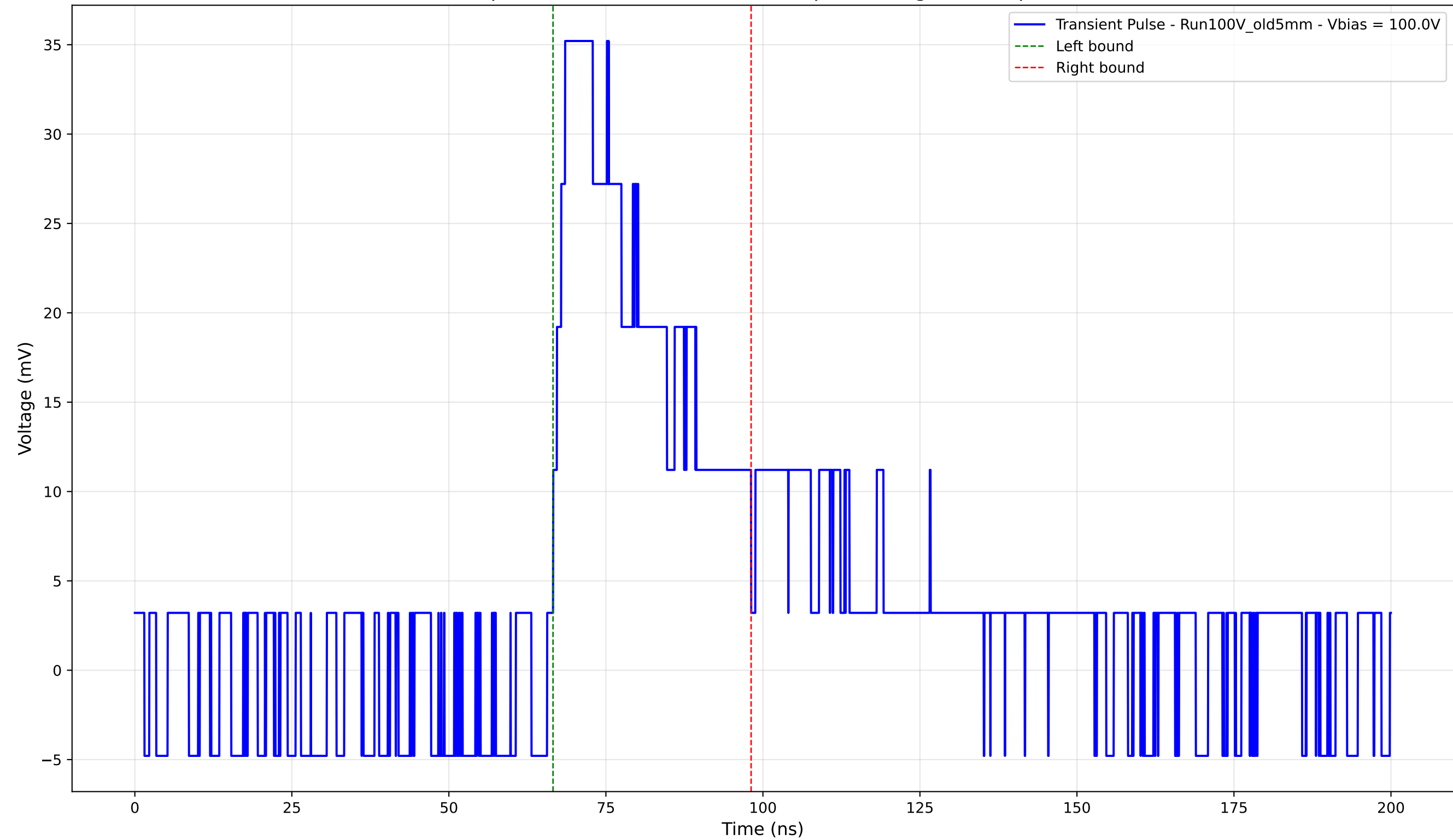
Transient Pulse - Sample: Old5mm - Position: 2615.0 \mu\text{m} - Charge: 12.74 pC - Rise Time: 1.92 ns
