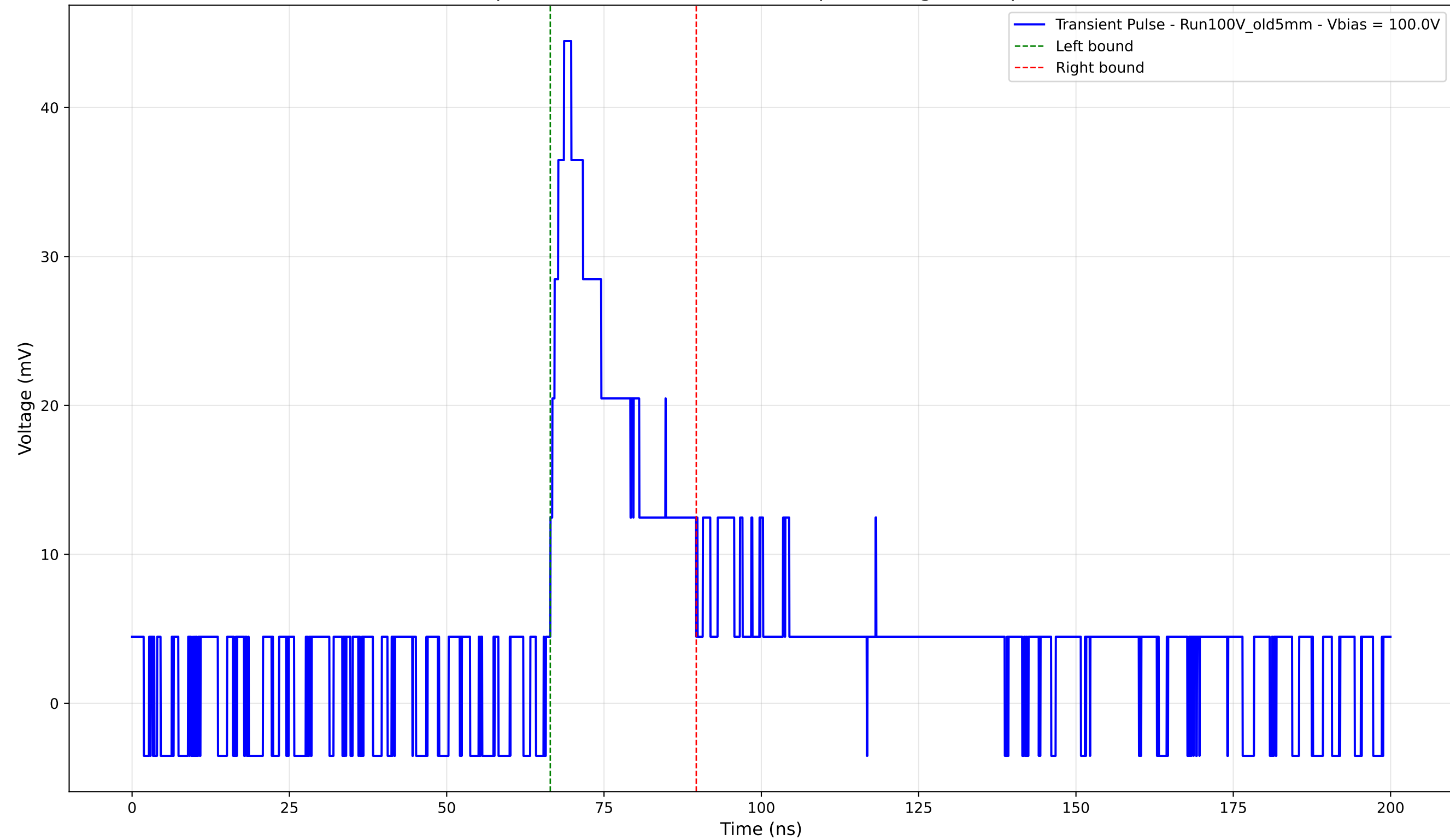
Transient Pulse - Sample: Old5mm - Position: 2885.0 \mu\text{m} - Charge: 9.98 pC - Rise Time: 2.88 ns
