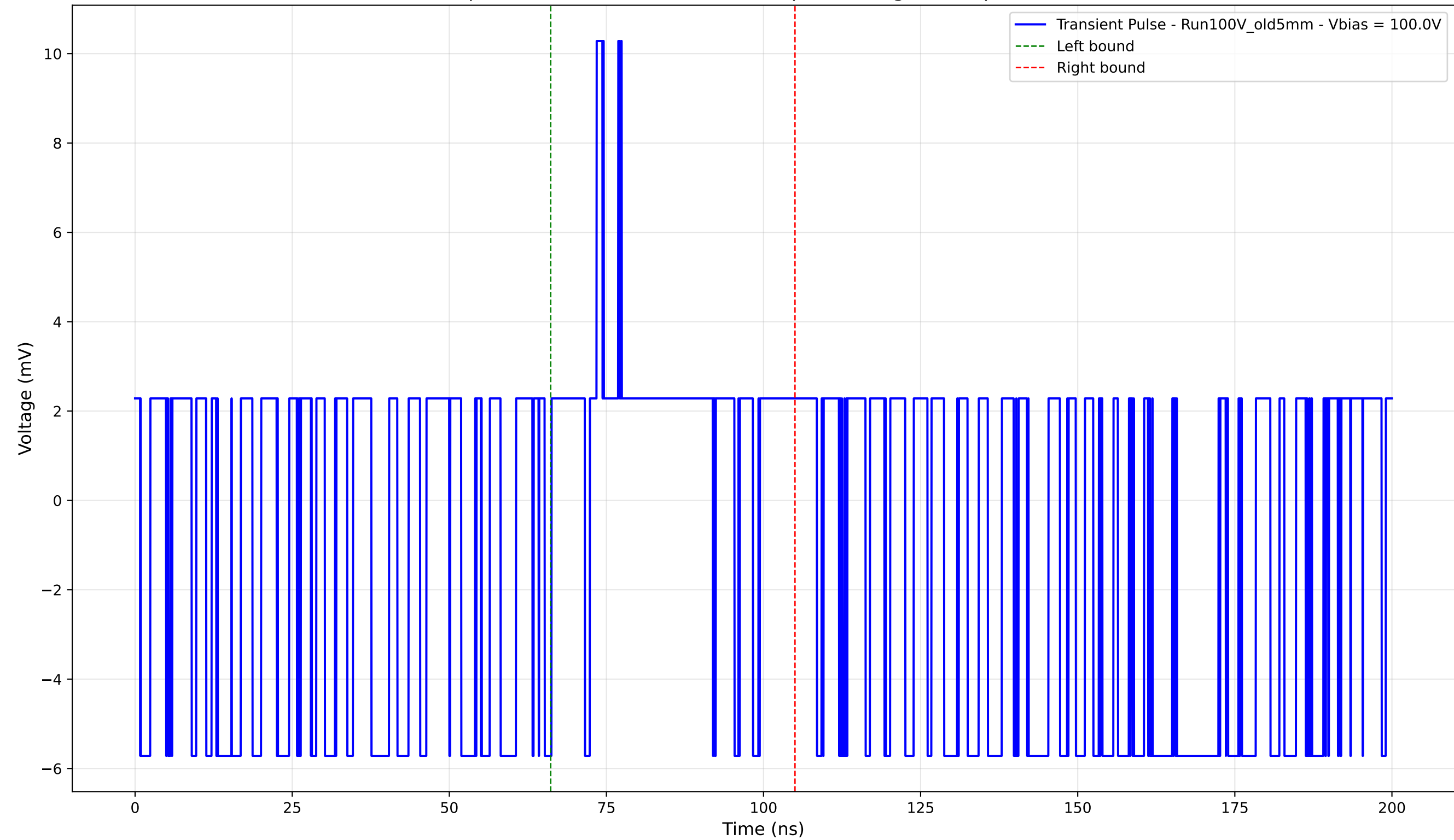
Transient Pulse - Sample: Old5mm - Position: 2310.0 \mu\text{m} - Charge: 1.52 pC - Rise Time: 0.00 ns (N/A)
