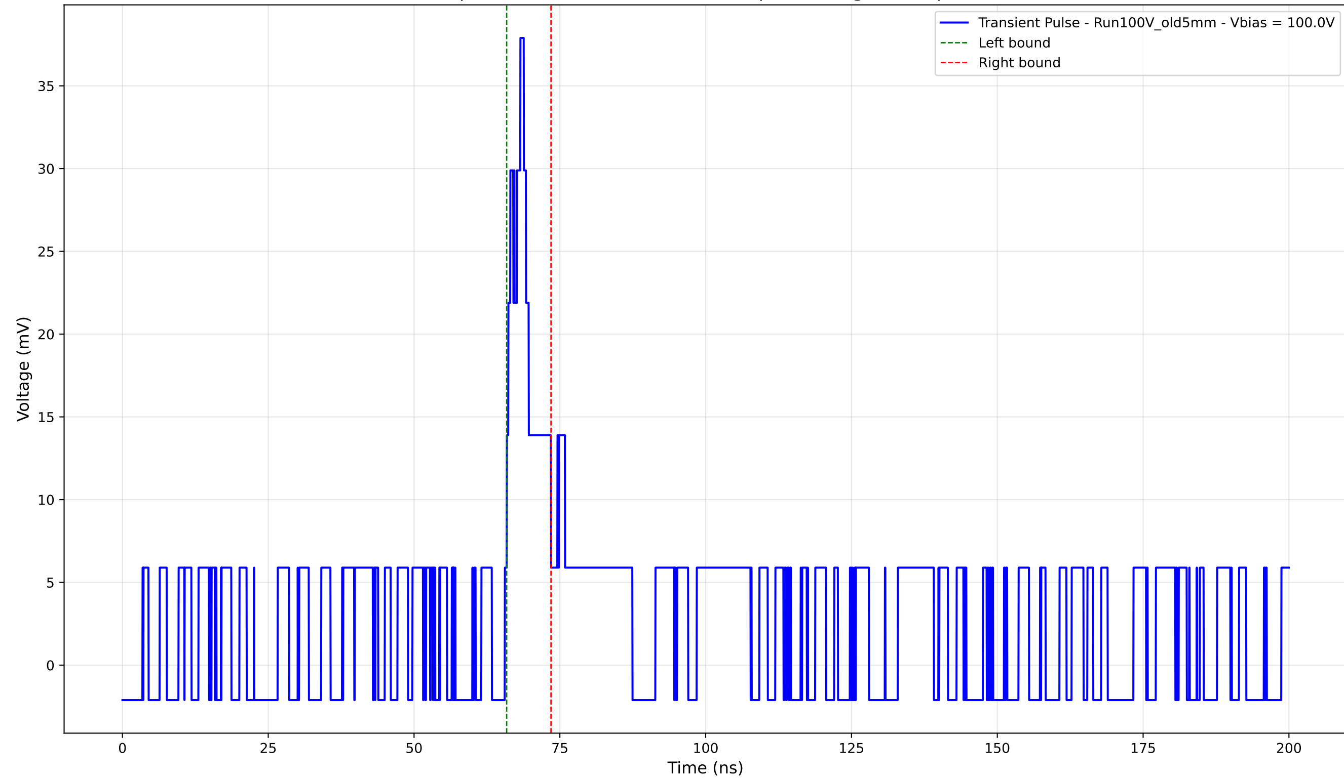
Transient Pulse - Sample: Old5mm - Position: 3450.0 \mu\text{m} - Charge: 3.11 pC - Rise Time: 2.67 ns
