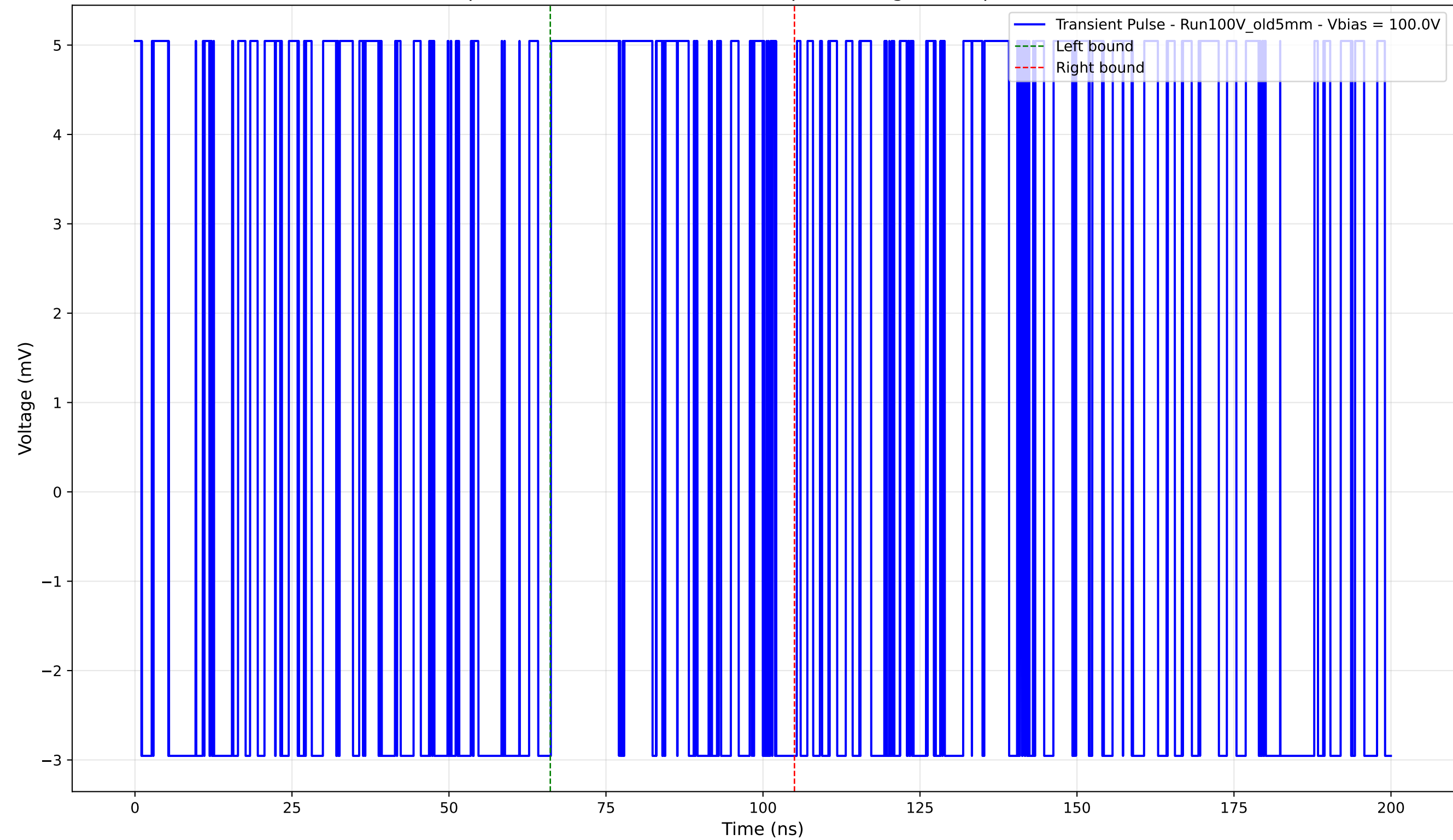
Transient Pulse - Sample: Old5mm - Position: 4585.0 \mu\text{m} - Charge: 1.78 pC - Rise Time: 0.00 ns (N/A)
