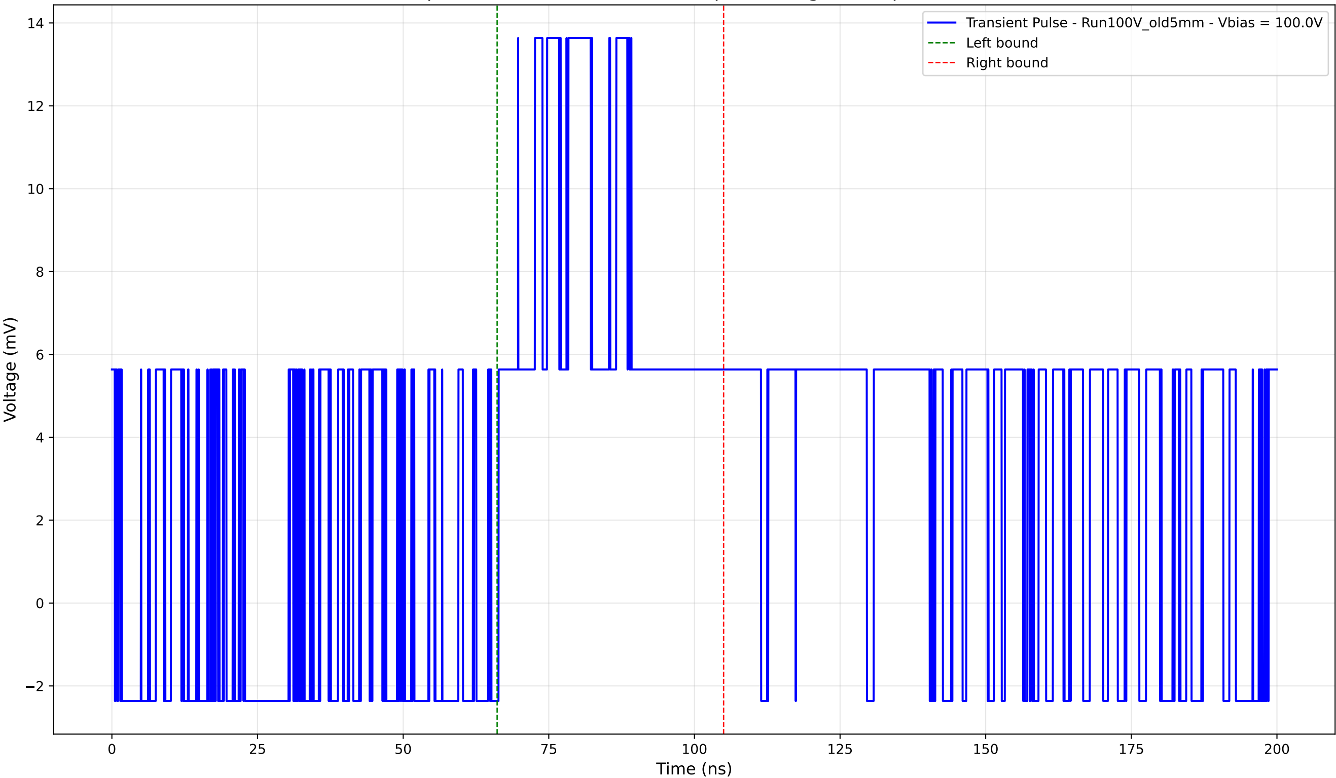
Transient Pulse - Sample: Old5mm - Position: 800.0 \mu\text{m} - Charge: 5.93 pC - Rise Time: 0.00 ns (N/A)
