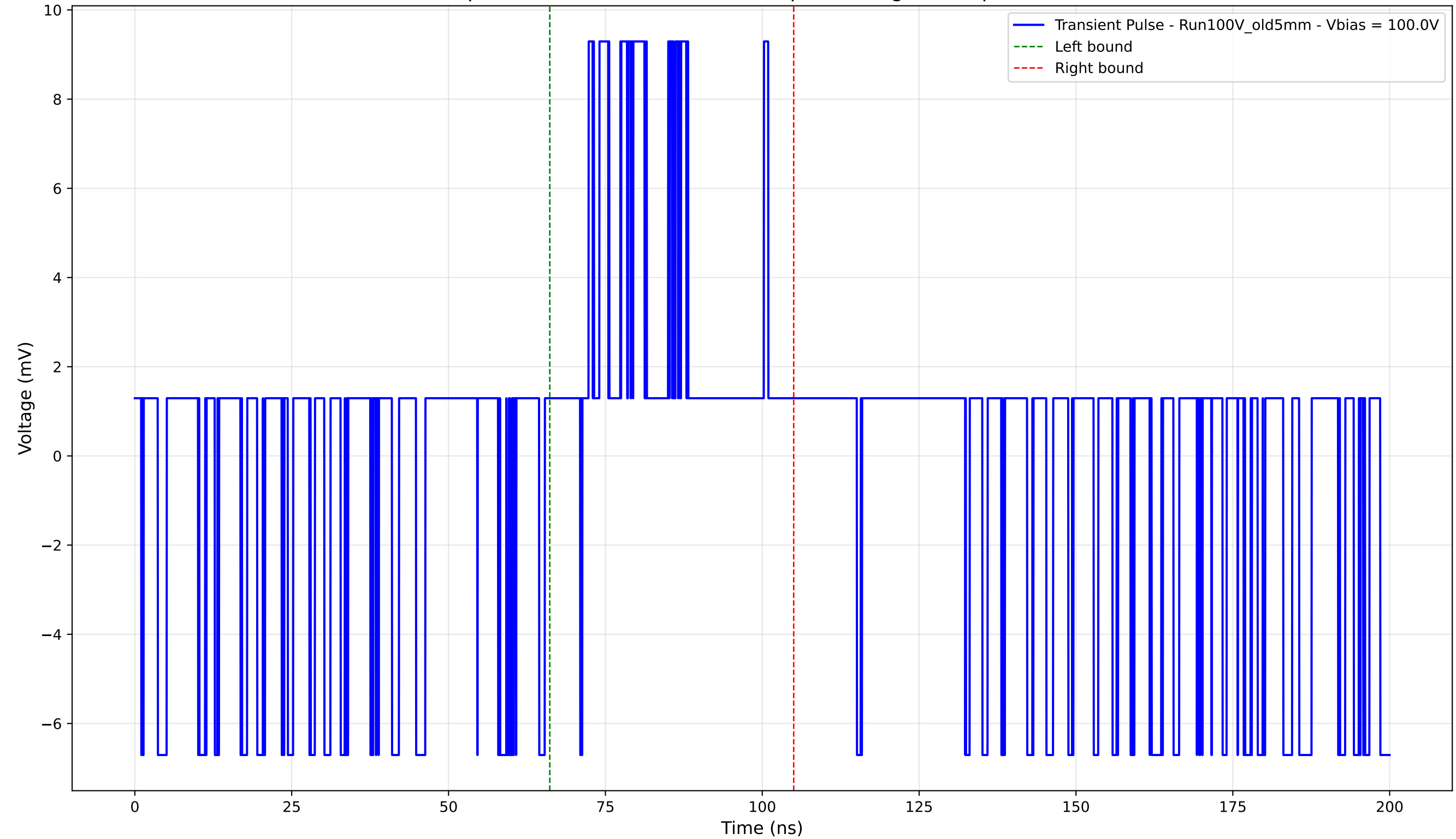
Transient Pulse - Sample: Old5mm - Position: 1110.0 \mu\text{m} - Charge: 2.42 pC - Rise Time: 0.00 ns (N/A)
