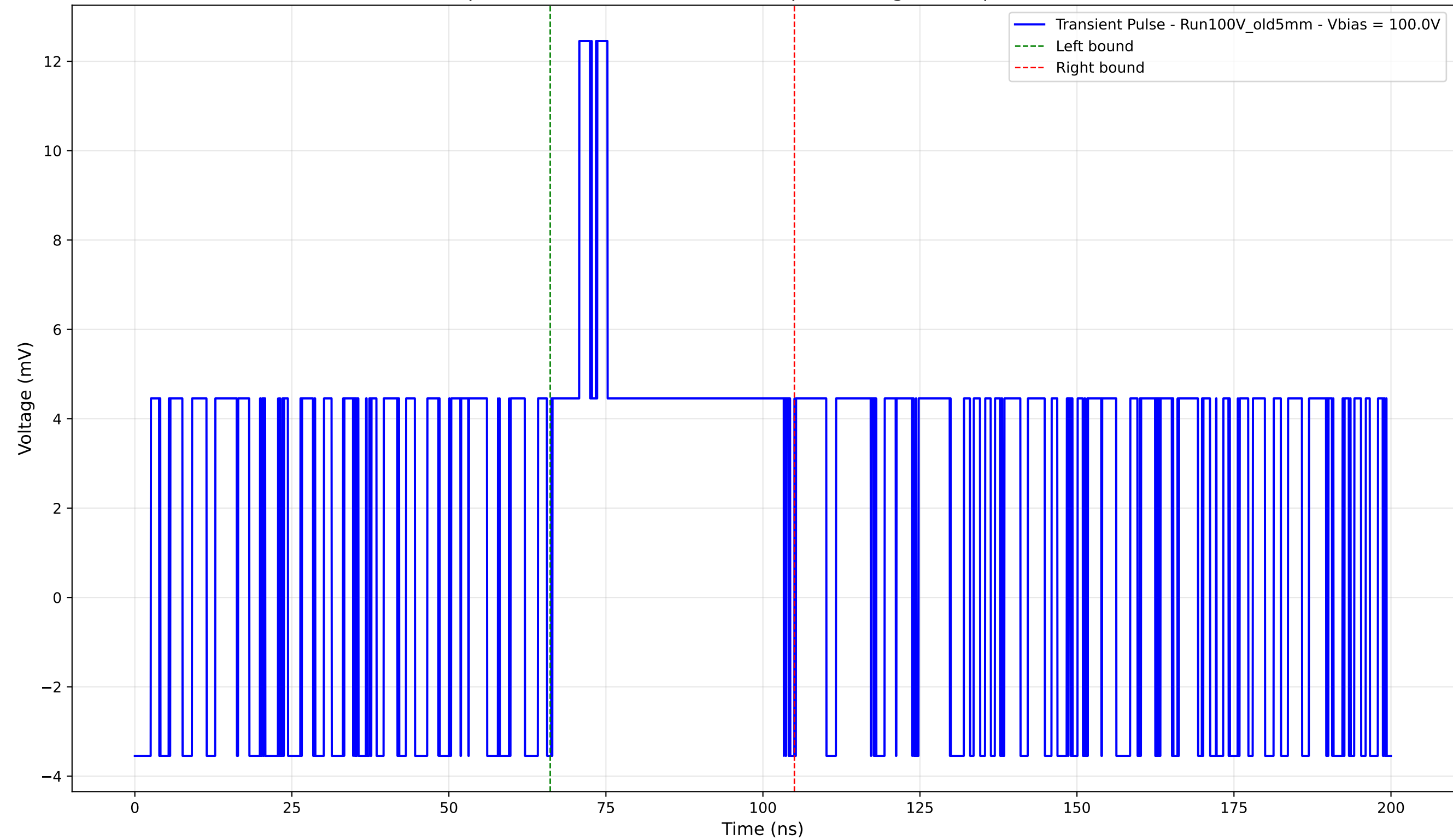
Transient Pulse - Sample: Old5mm - Position: 2505.0 \mu\text{m} - Charge: 3.85 pC - Rise Time: 0.00 ns (N/A)
