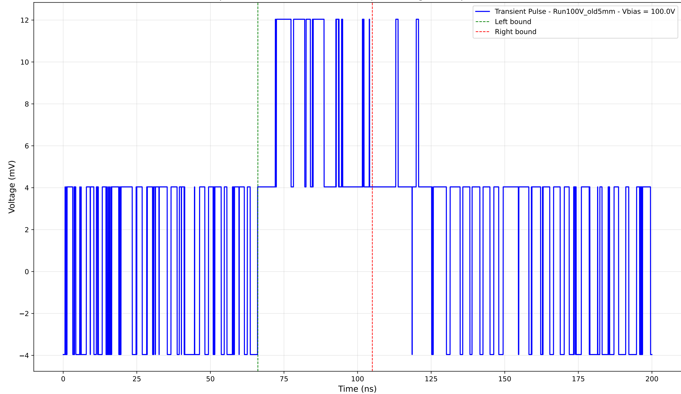
Transient Pulse - Sample: Old5mm - Position: 1075.0 \mu\text{m} - Charge: 5.69 pC - Rise Time: 0.00 ns (N/A)
