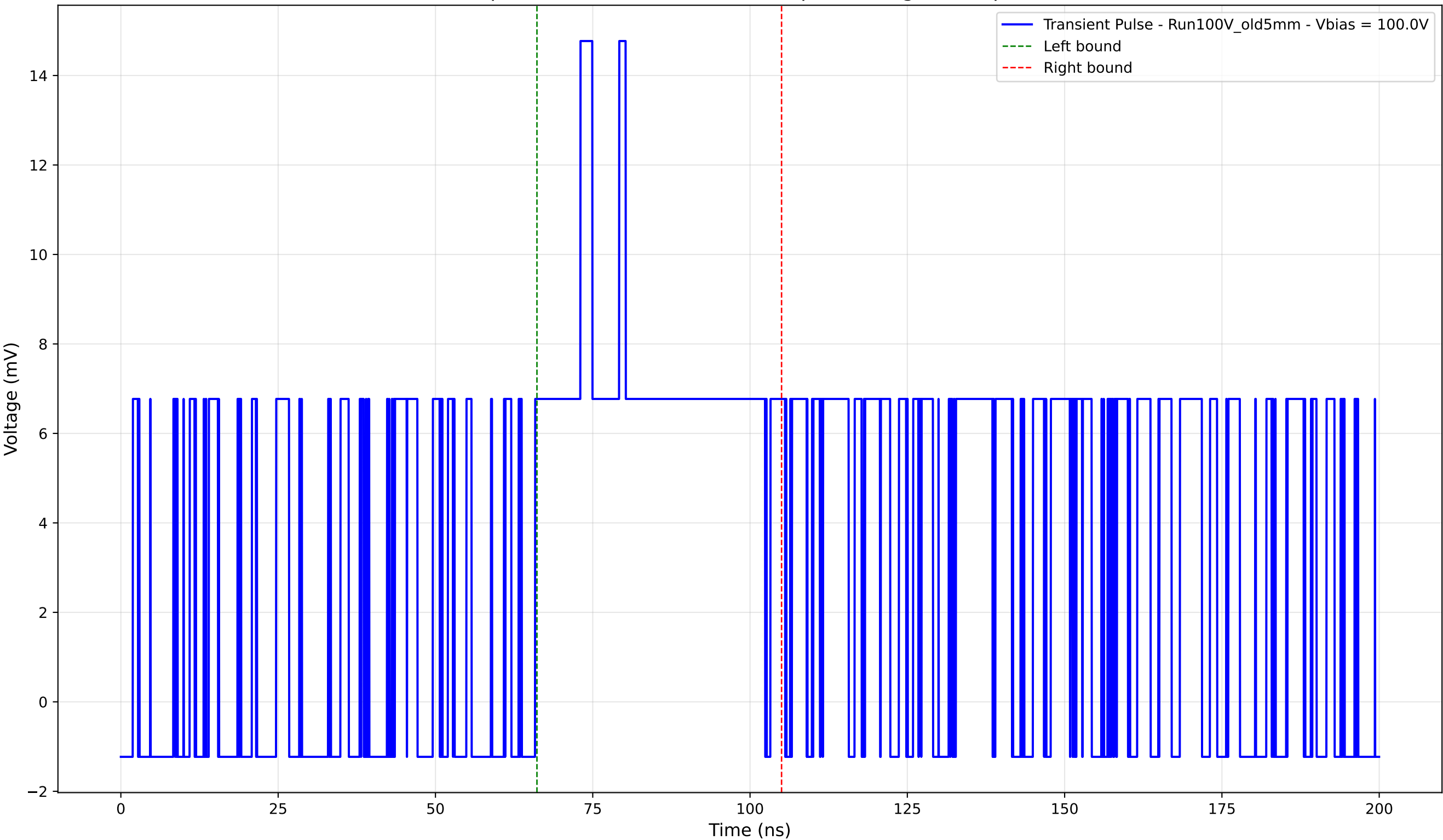
Transient Pulse - Sample: Old5mm - Position: 440.0 \mu\text{m} - Charge: 5.62 pC - Rise Time: 7.22 ns
