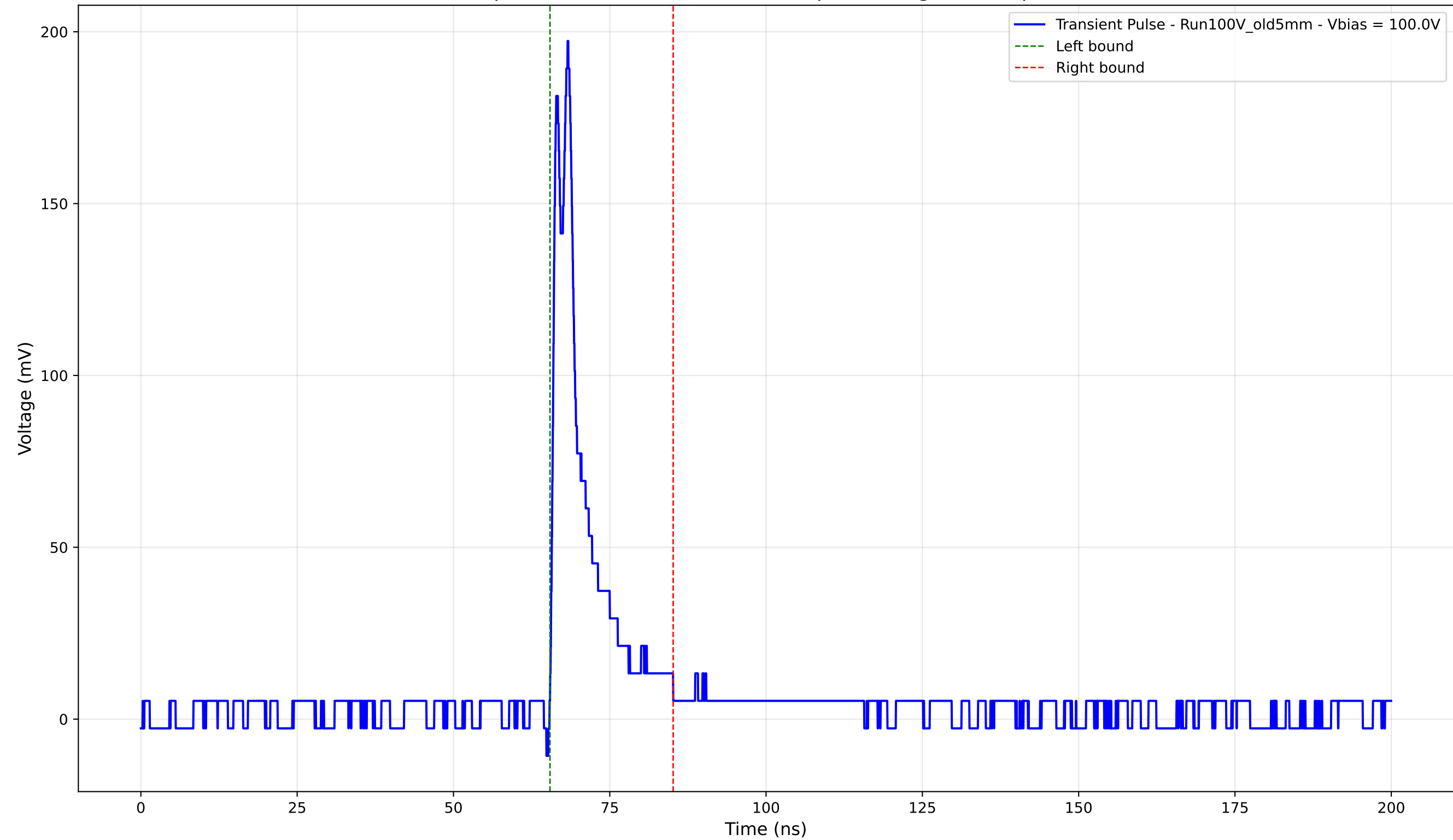
Transient Pulse - Sample: Old5mm - Position: 3550.0 \mu\text{m} - Charge: 21.07 pC - Rise Time: 0.88 ns
