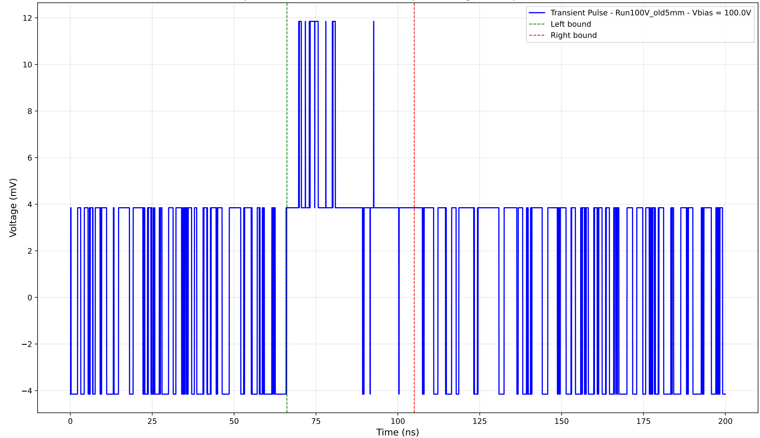
Transient Pulse - Sample: Old5mm - Position: 2495.0 \mu\text{m} - Charge: 3.59 pC - Rise Time: 0.00 ns (N/A)
