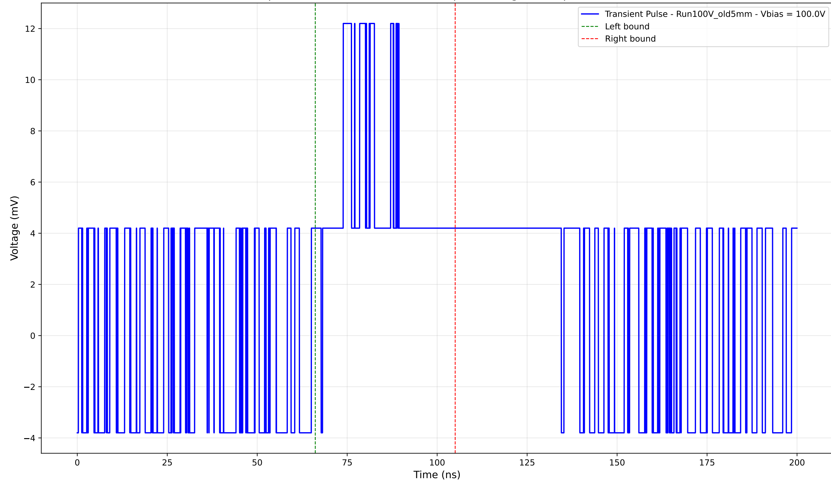
Transient Pulse - Sample: Old5mm - Position: 1055.0 \mu\text{m} - Charge: 4.28 pC - Rise Time: 0.00 ns (N/A)
