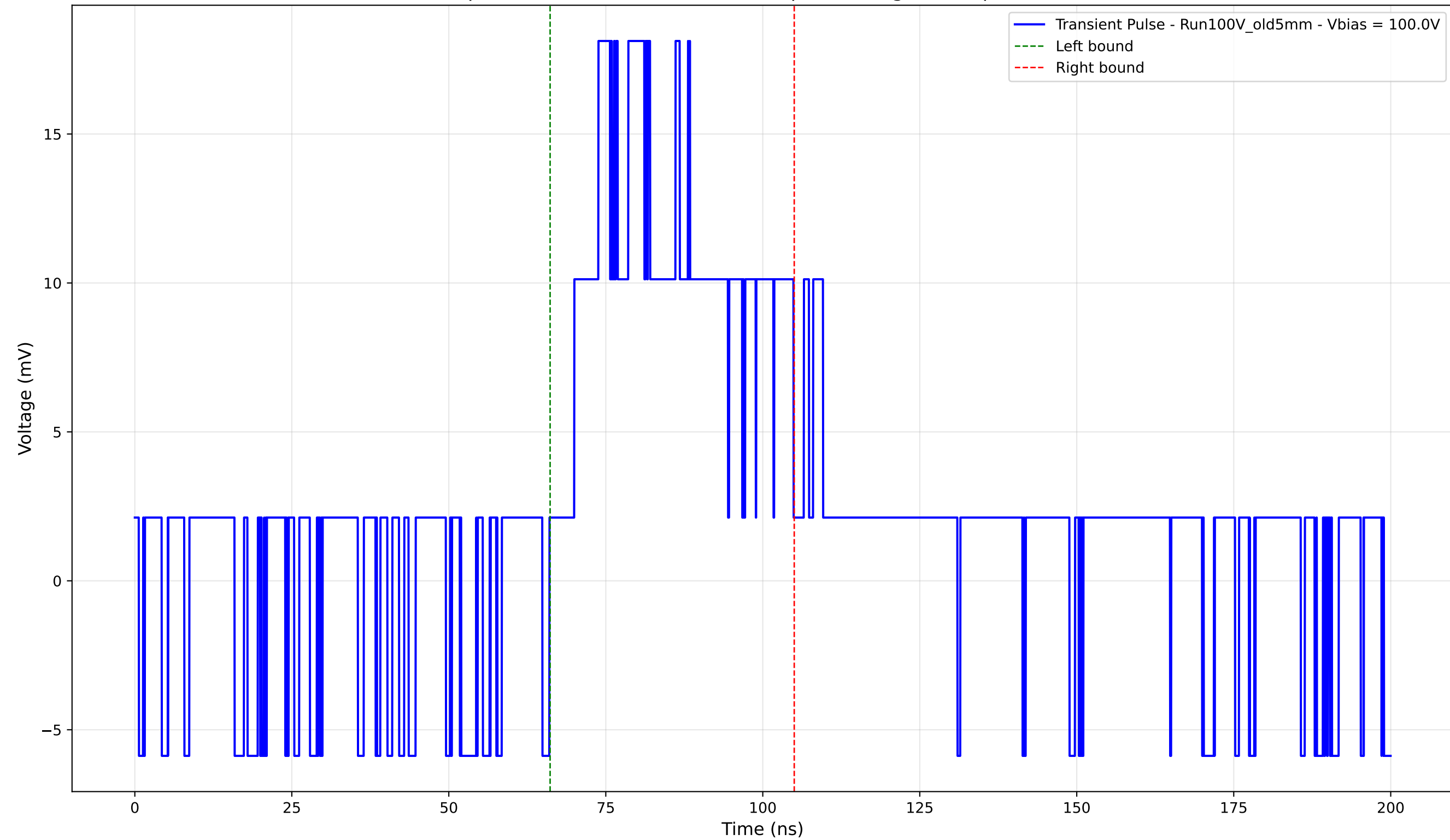
Transient Pulse - Sample: Old5mm - Position: 1590.0 \mu\text{m} - Charge: 8.14 pC - Rise Time: 0.00 ns (N/A)
