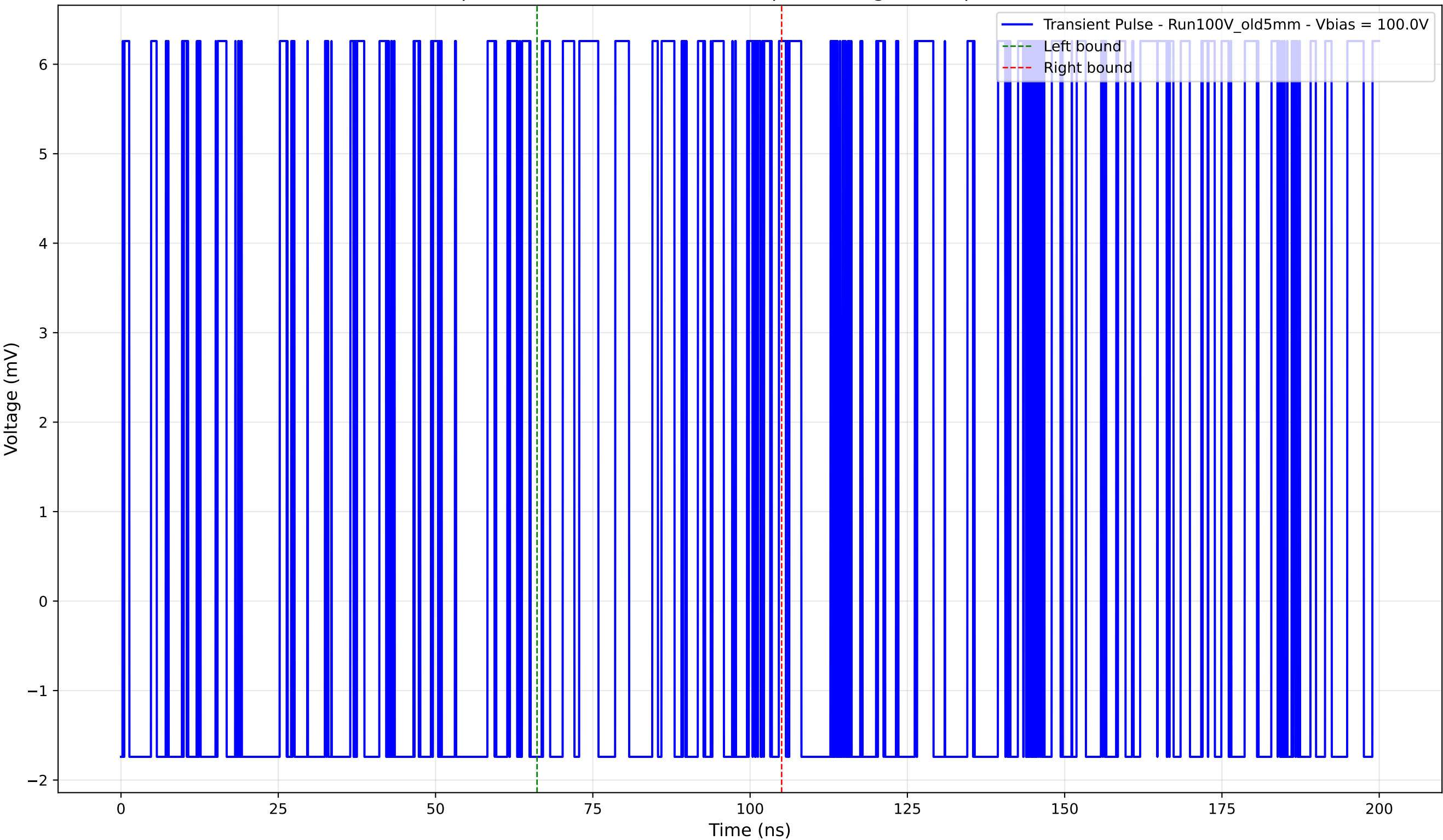
Transient Pulse - Sample: Old5mm - Position: 160.0 \mu\text{m} - Charge: 1.62 pC - Rise Time: 0.00 ns (N/A)
