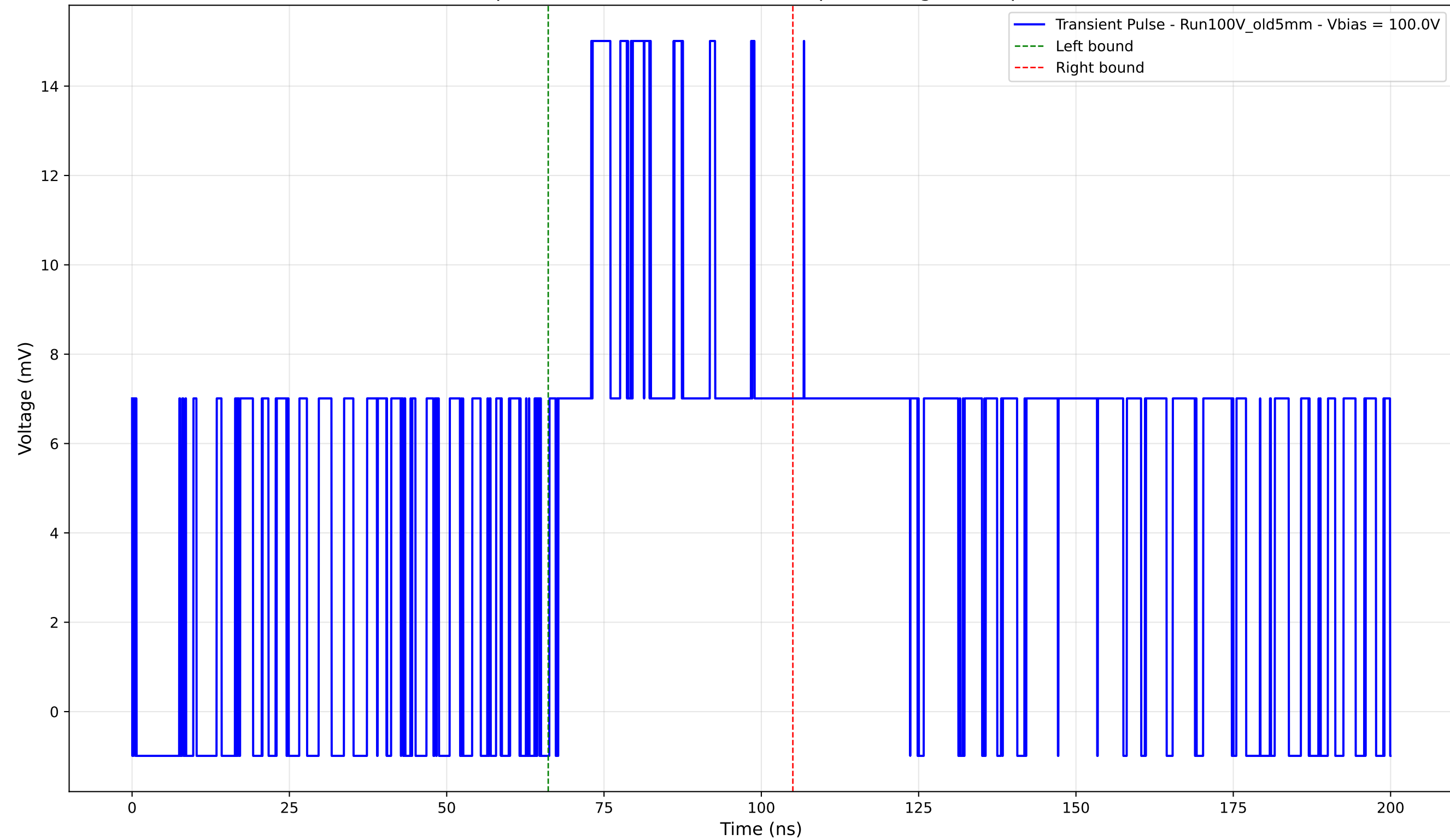
Transient Pulse - Sample: Old5mm - Position: 1260.0 \mu\text{m} - Charge: 6.93 pC - Rise Time: 5.24 ns
