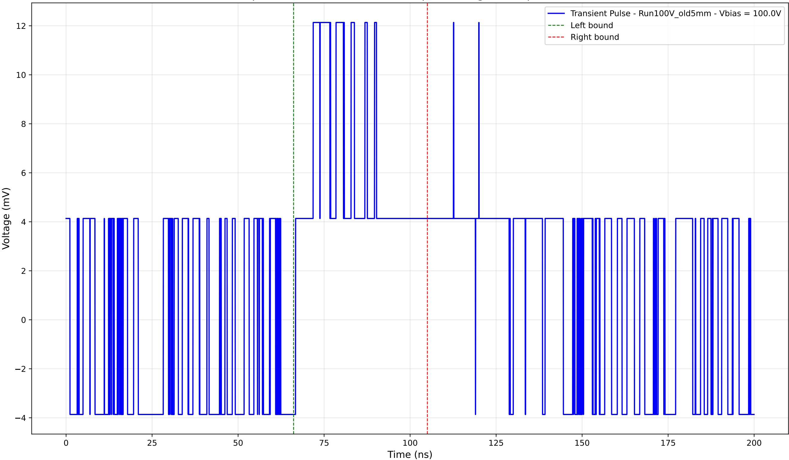
Transient Pulse - Sample: Old5mm - Position: 565.0 \mu\text{m} - Charge: 4.64 pC - Rise Time: 0.00 ns (N/A)
