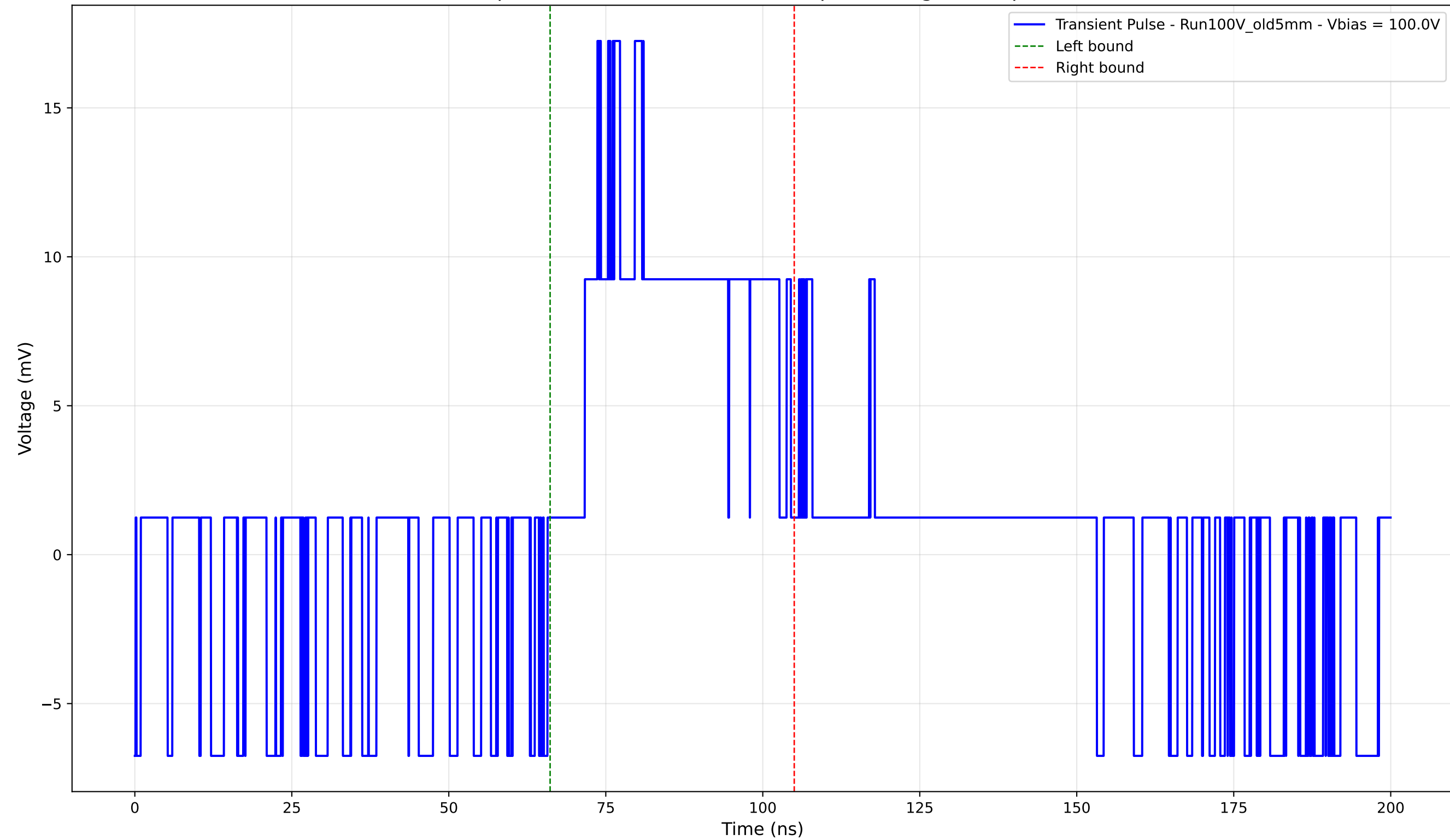
Transient Pulse - Sample: Old5mm - Position: 1195.0 \mu\text{m} - Charge: 6.46 pC - Rise Time: 2.02 ns
