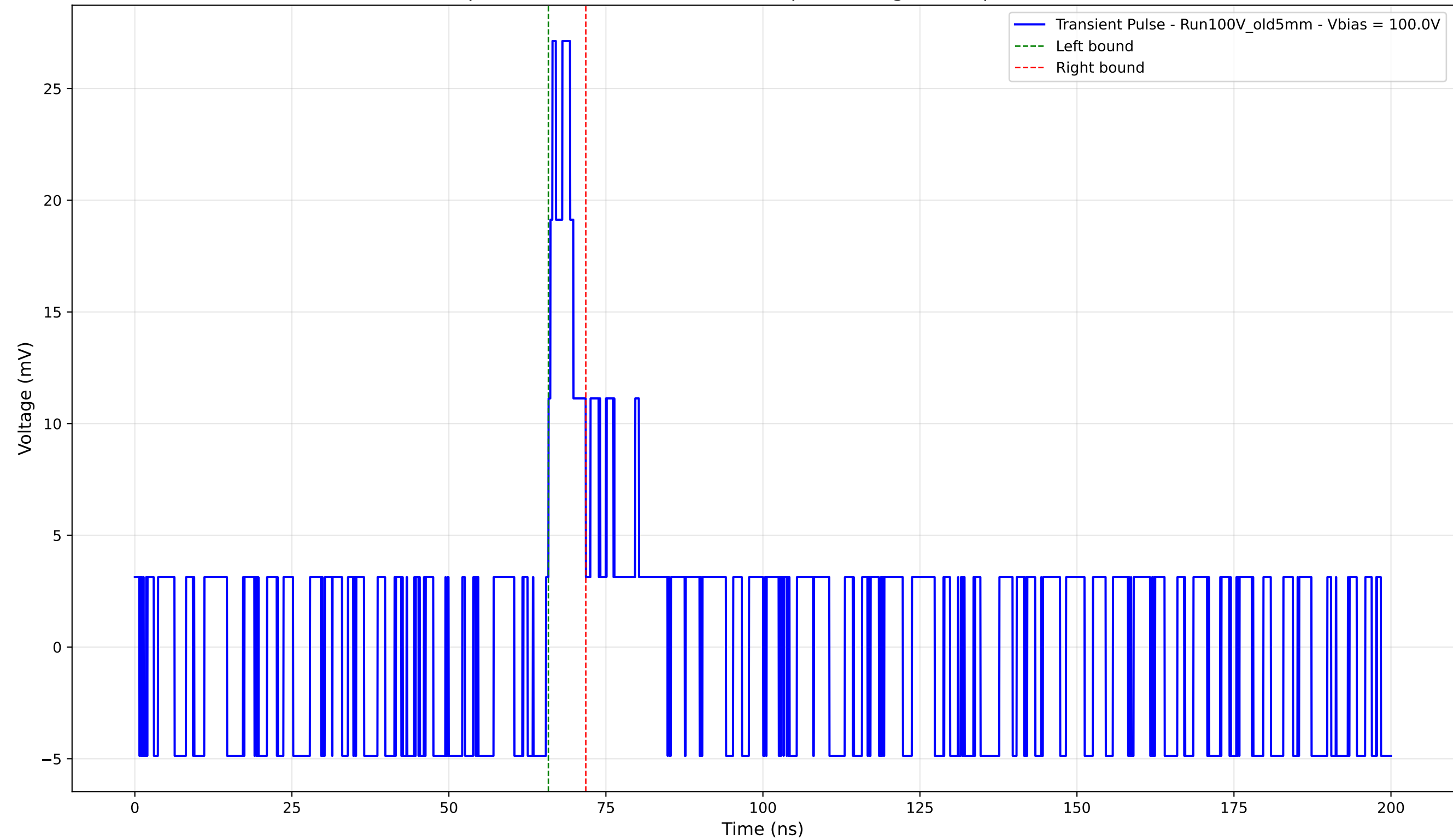
Transient Pulse - Sample: Old5mm - Position: 3360.0 \mu\text{m} - Charge: 2.20 pC - Rise Time: 0.00 ns (N/A)
