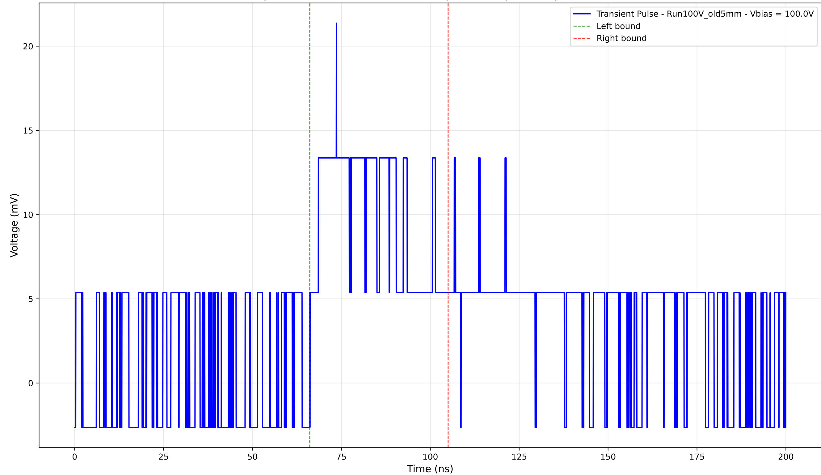
Transient Pulse - Sample: Old5mm - Position: 2270.0 \mu\text{m} - Charge: 7.75 pC - Rise Time: 0.00 ns (N/A)
