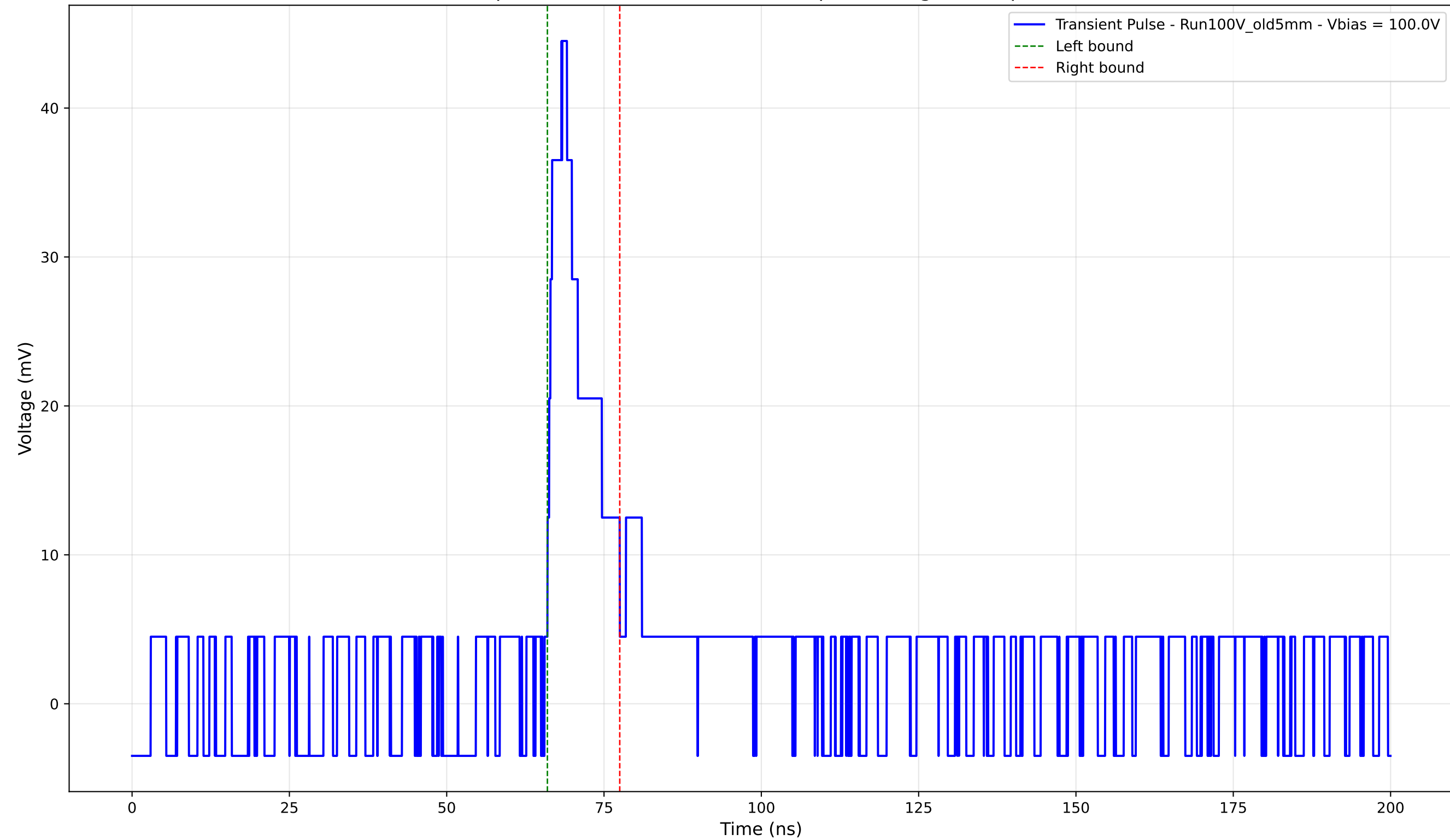
Transient Pulse - Sample: Old5mm - Position: 4240.0 \mu\text{m} - Charge: 5.54 pC - Rise Time: 2.70 ns
