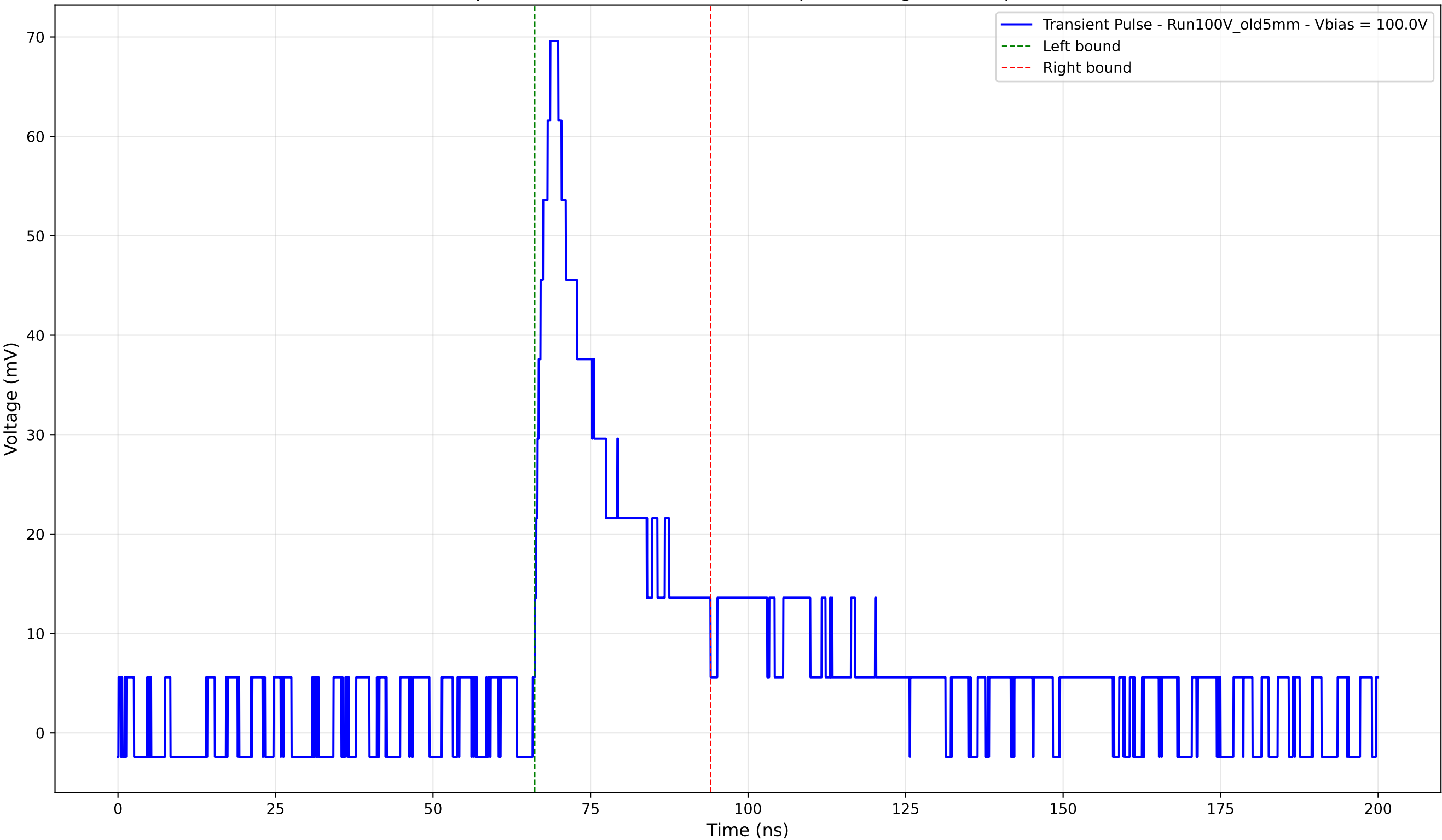
Transient Pulse - Sample: Old5mm - Position: 4480.0 \mu\text{m} - Charge: 15.88 pC - Rise Time: 2.46 ns
