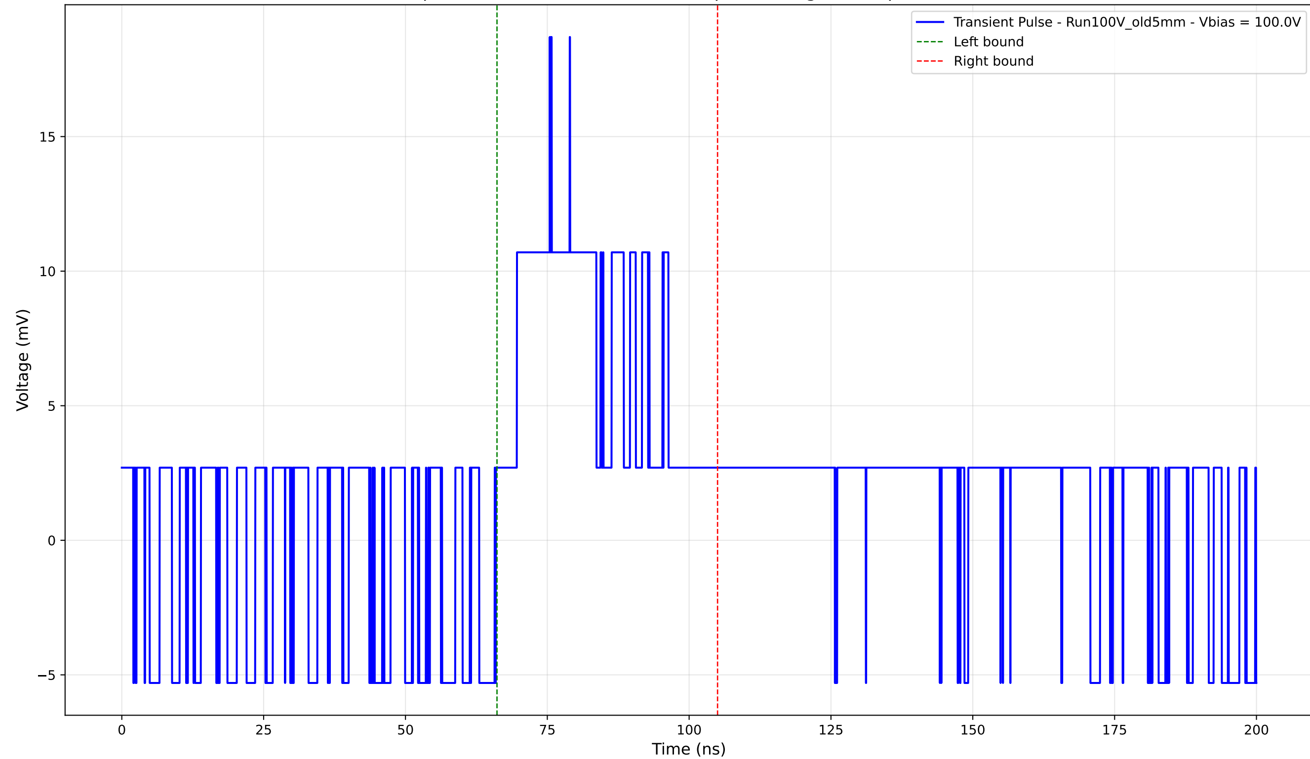
Transient Pulse - Sample: Old5mm - Position: 1965.0 \mu\text{m} - Charge: 5.27 pC - Rise Time: 0.00 ns (N/A)
