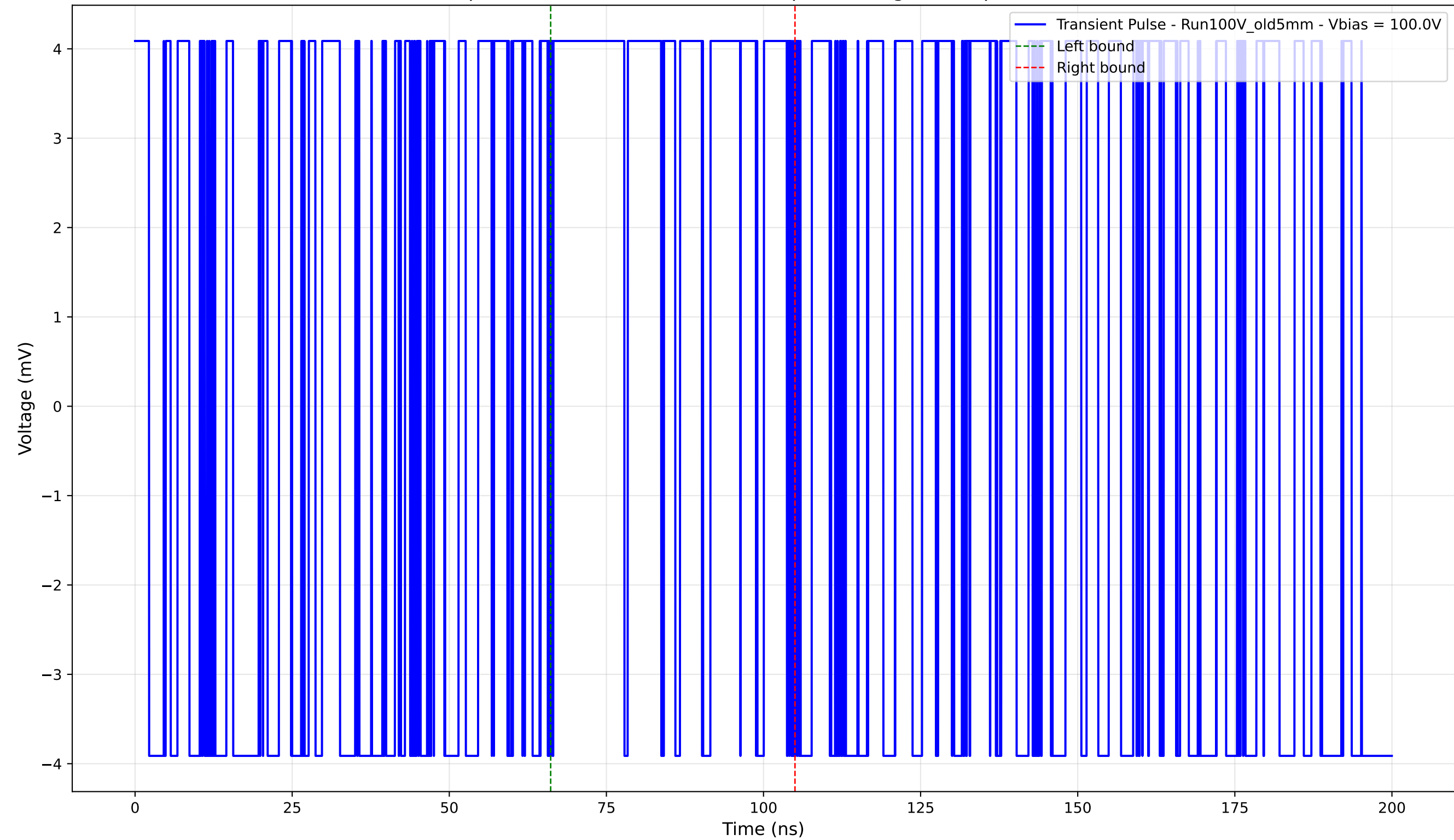
Transient Pulse - Sample: Old5mm - Position: 4650.0 \mu\text{m} - Charge: 2.39 pC - Rise Time: 0.00 ns (N/A)
