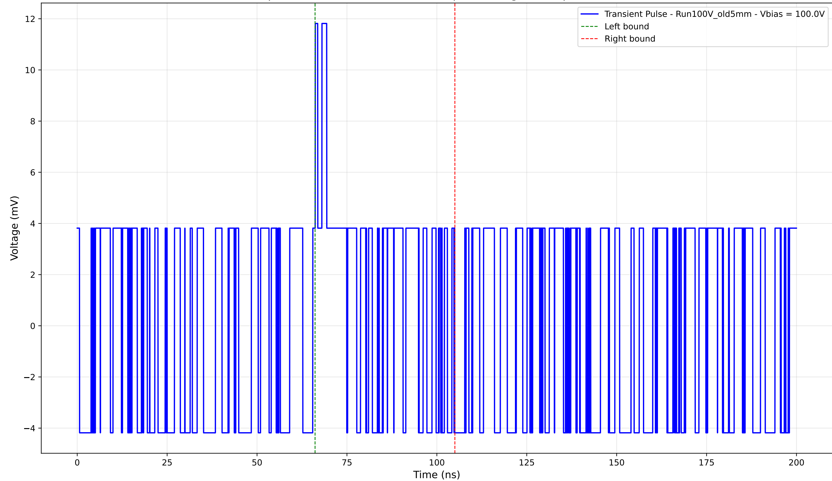
Transient Pulse - Sample: Old5mm - Position: 3715.0 \mu\text{m} - Charge: 1.48 pC - Rise Time: 0.00 ns (N/A)
