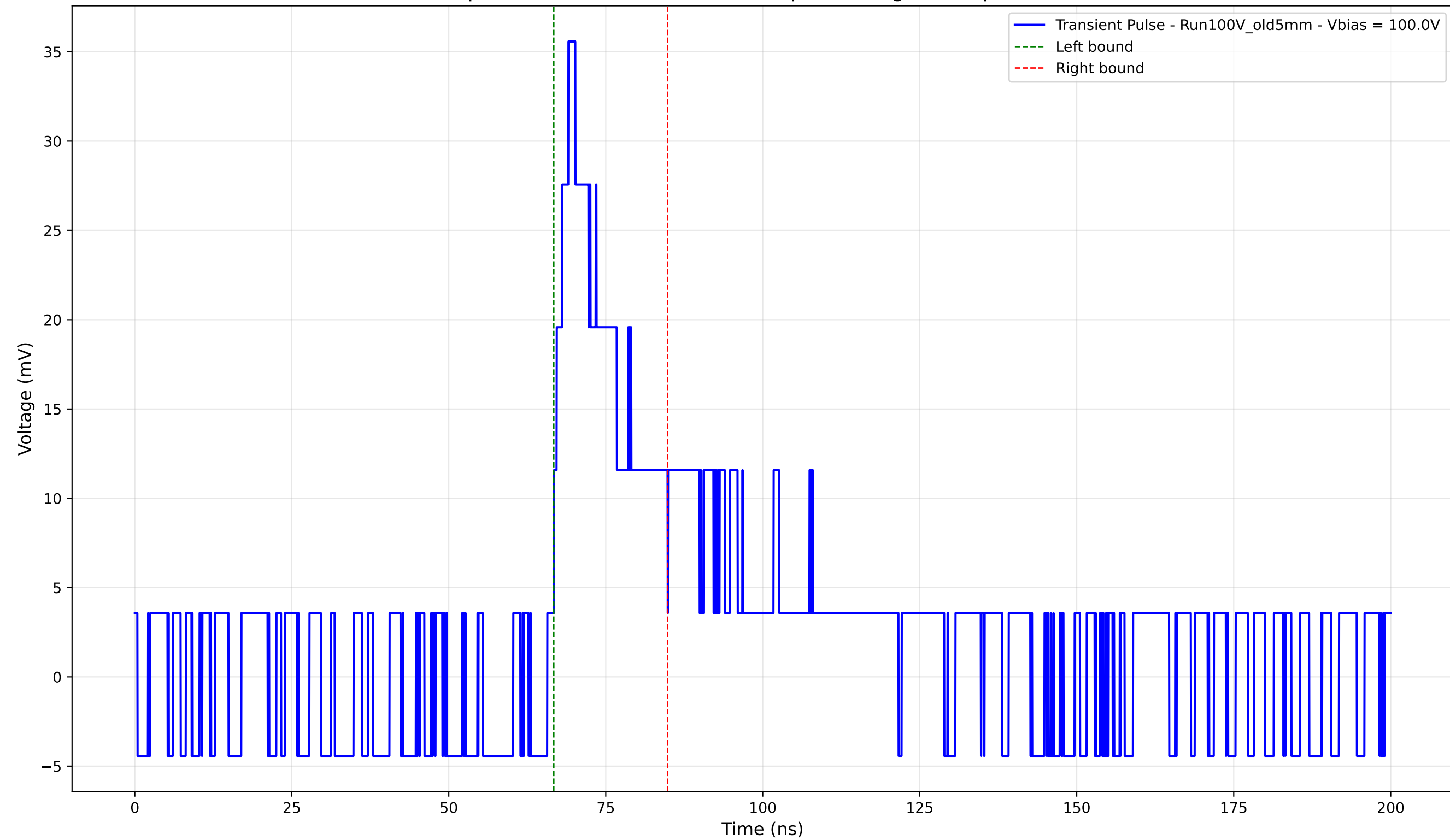
Transient Pulse - Sample: Old5mm - Position: 4695.0 \mu\text{m} - Charge: 6.70 pC - Rise Time: 0.00 ns (N/A)
