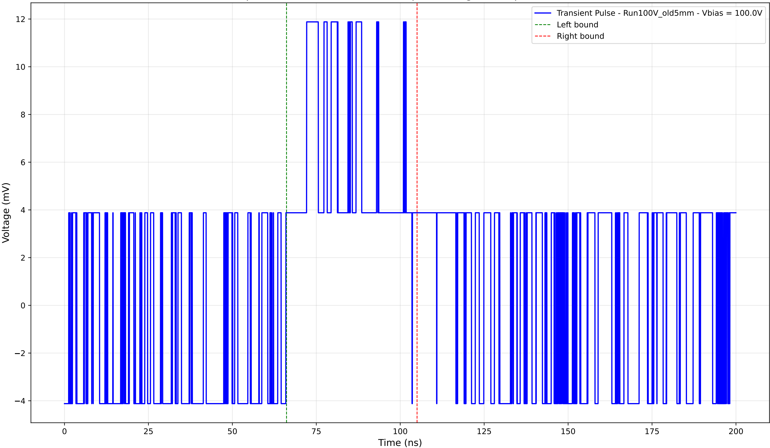
Transient Pulse - Sample: Old5mm - Position: 400.0 \mu\text{m} - Charge: 4.55 pC - Rise Time: 0.00 ns (N/A)
