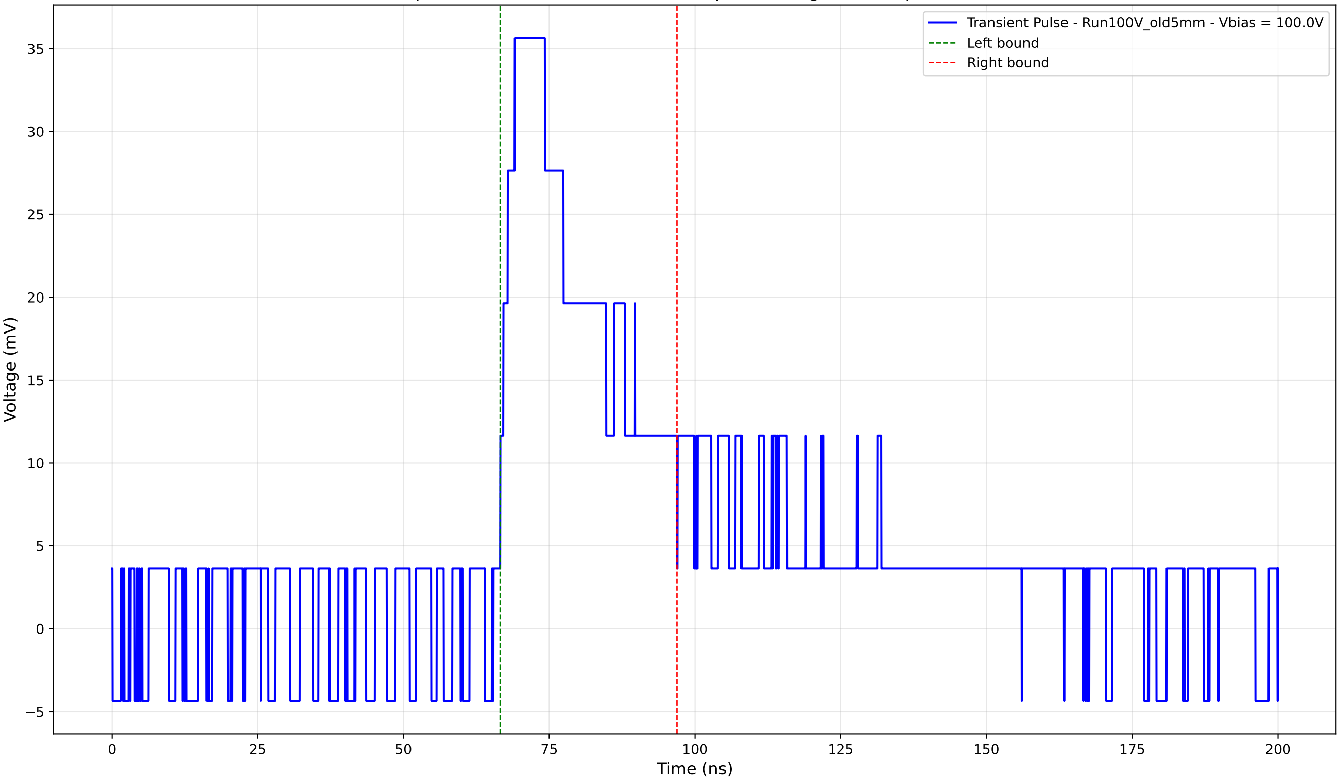
Transient Pulse - Sample: Old5mm - Position: 2610.0 \mu\text{m} - Charge: 12.53 pC - Rise Time: 0.00 ns (N/A)
