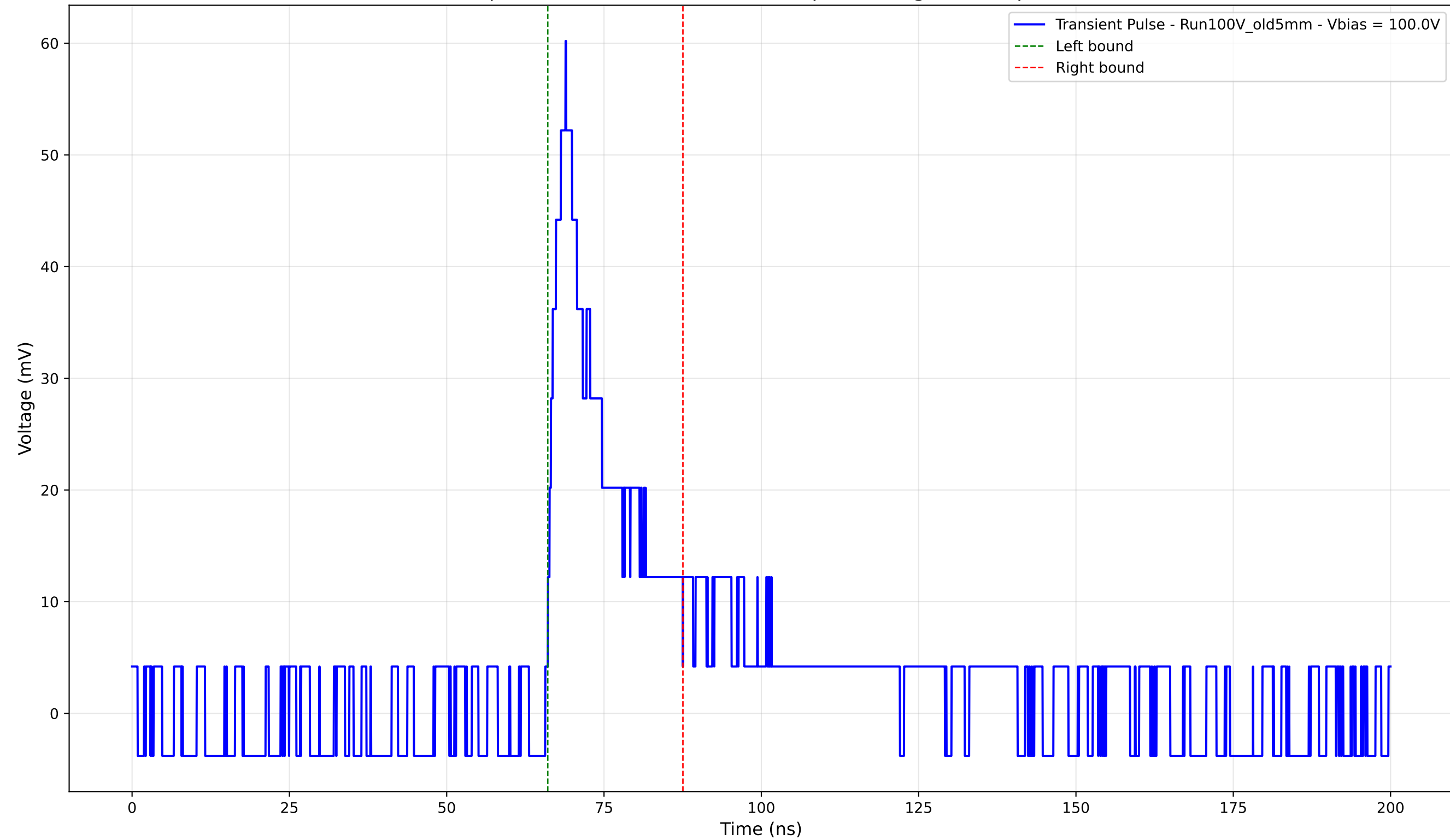
Transient Pulse - Sample: Old5mm - Position: 3015.0 \mu\text{m} - Charge: 10.53 pC - Rise Time: 2.82 ns
