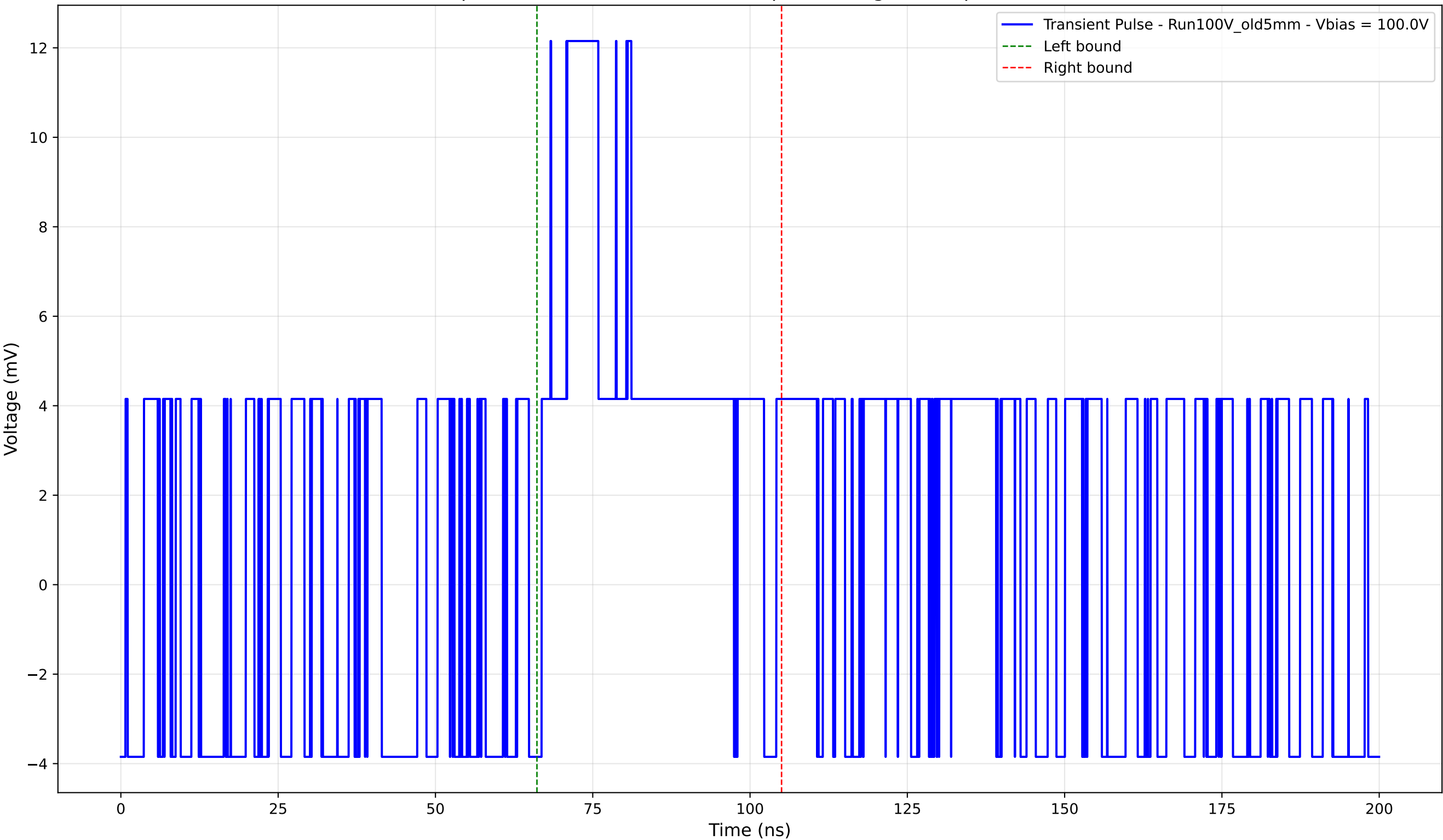
Transient Pulse - Sample: Old5mm - Position: 445.0 \mu\text{m} - Charge: 3.67 pC - Rise Time: 0.00 ns (N/A)
