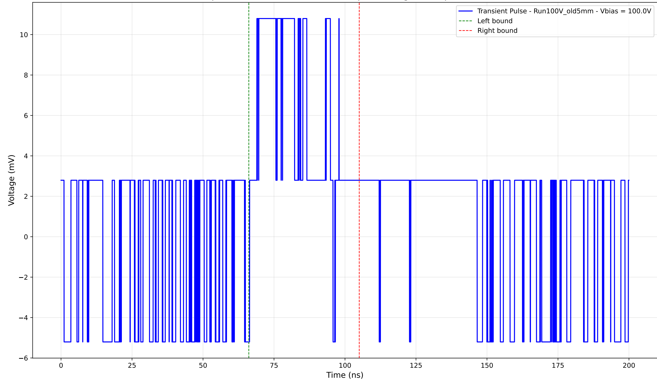
Transient Pulse - Sample: Old5mm - Position: 2485.0 \mu\text{m} - Charge: 4.62 pC - Rise Time: 0.00 ns (N/A)
