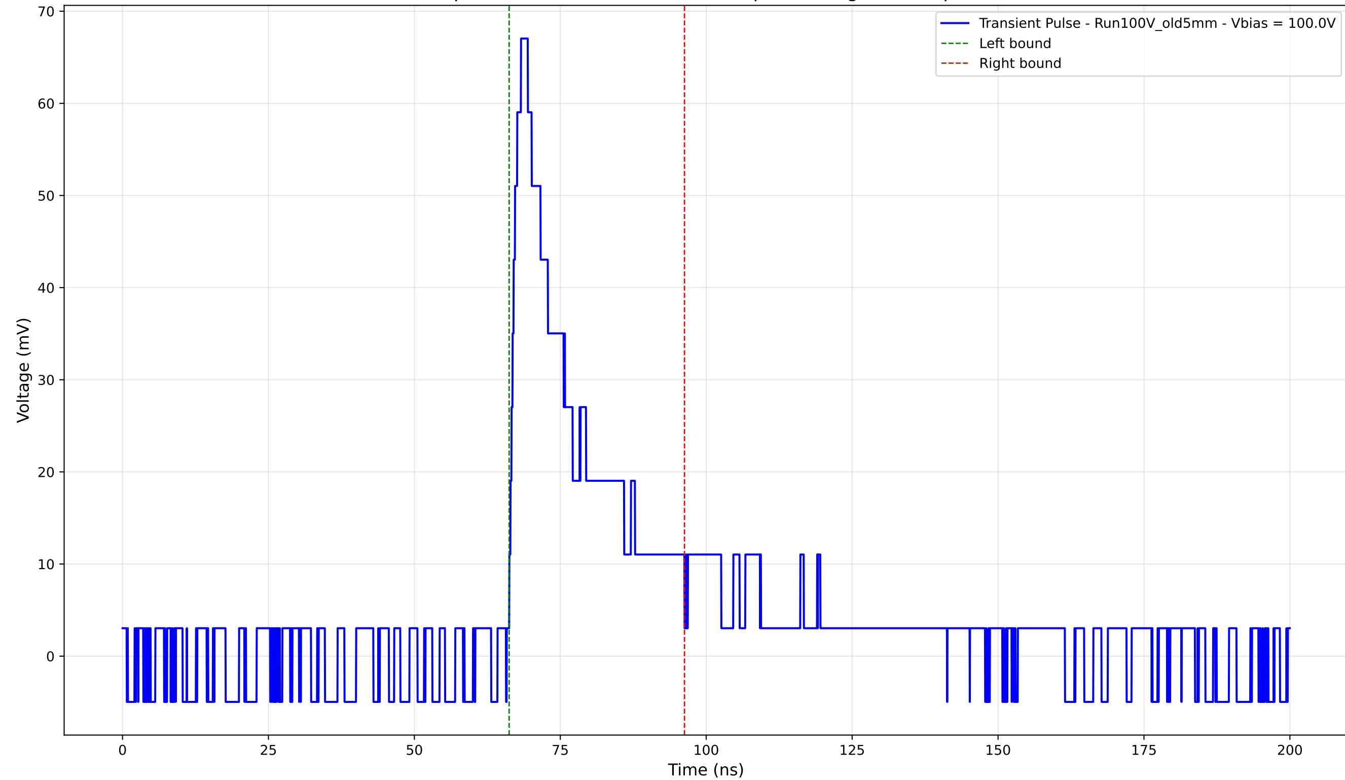
Transient Pulse - Sample: Old5mm - Position: 2965.0 \mu\text{m} - Charge: 15.33 pC - Rise Time: 2.01 ns
