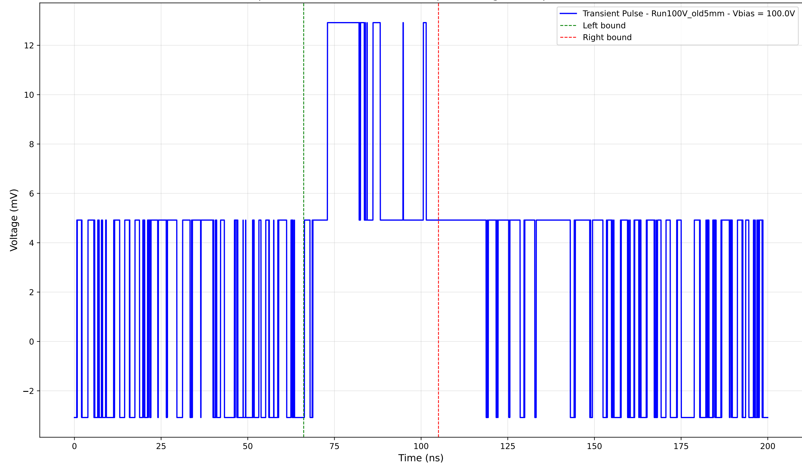
Transient Pulse - Sample: Old5mm - Position: 1160.0 \mu\text{m} - Charge: 5.83 pC - Rise Time: 0.00 ns (N/A)
