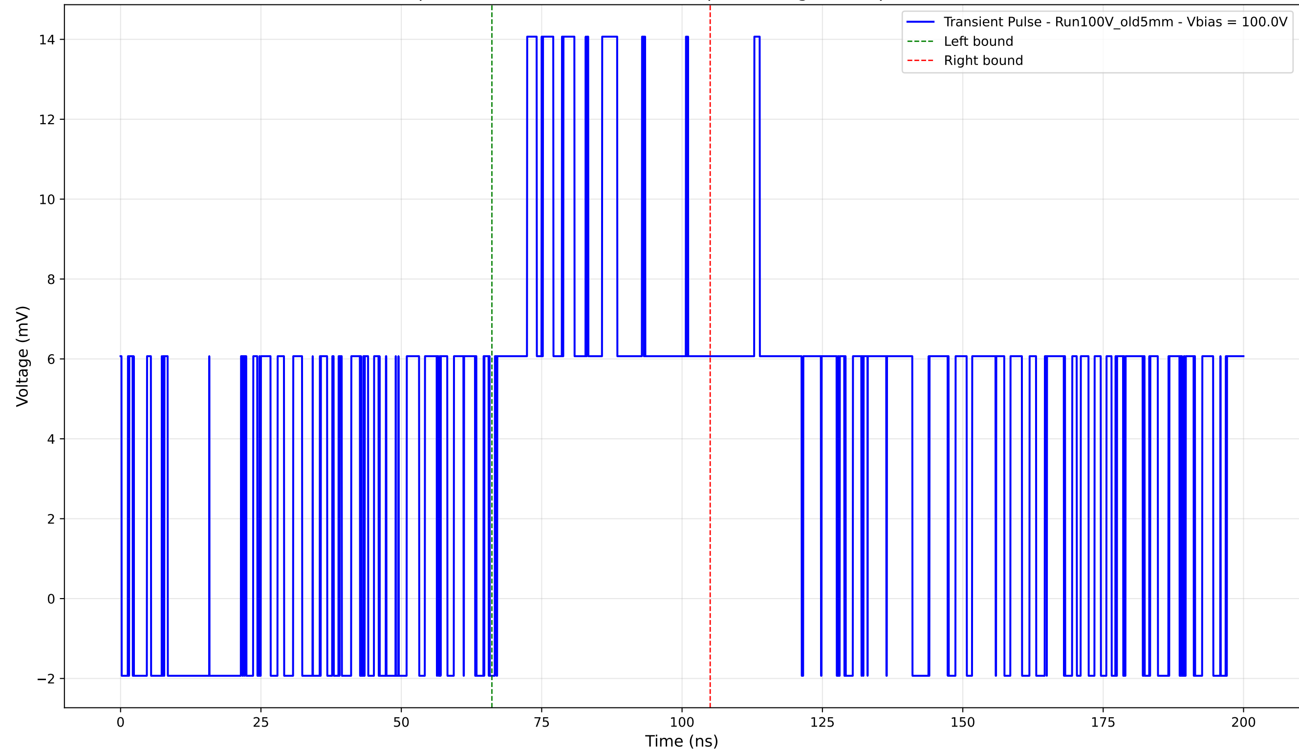
Transient Pulse - Sample: Old5mm - Position: 1750.0 \mu\text{m} - Charge: 6.12 pC - Rise Time: 0.00 ns (N/A)
