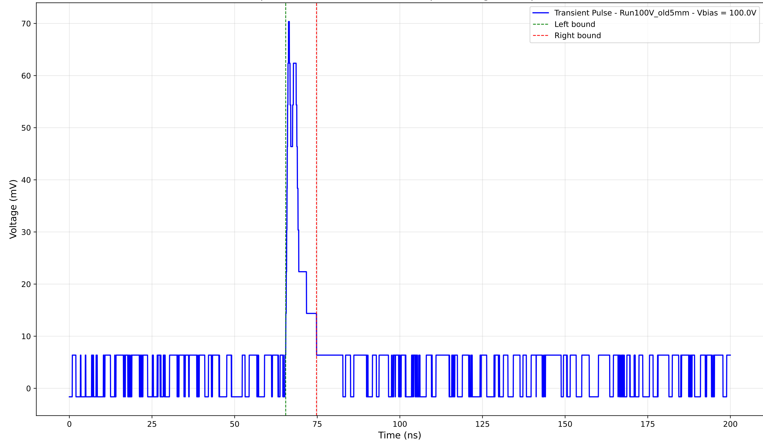
Transient Pulse - Sample: Old5mm - Position: 3655.0 \mu\text{m} - Charge: 5.90 pC - Rise Time: 0.84 ns
