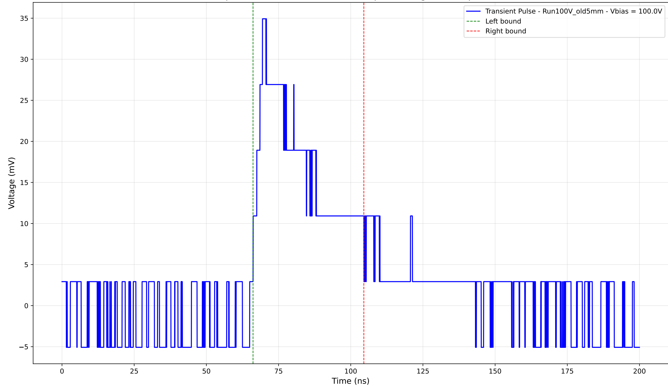
Transient Pulse - Sample: Old5mm - Position: 4970.0 \mu\text{m} - Charge: 13.16 pC - Rise Time: 3.26 ns
