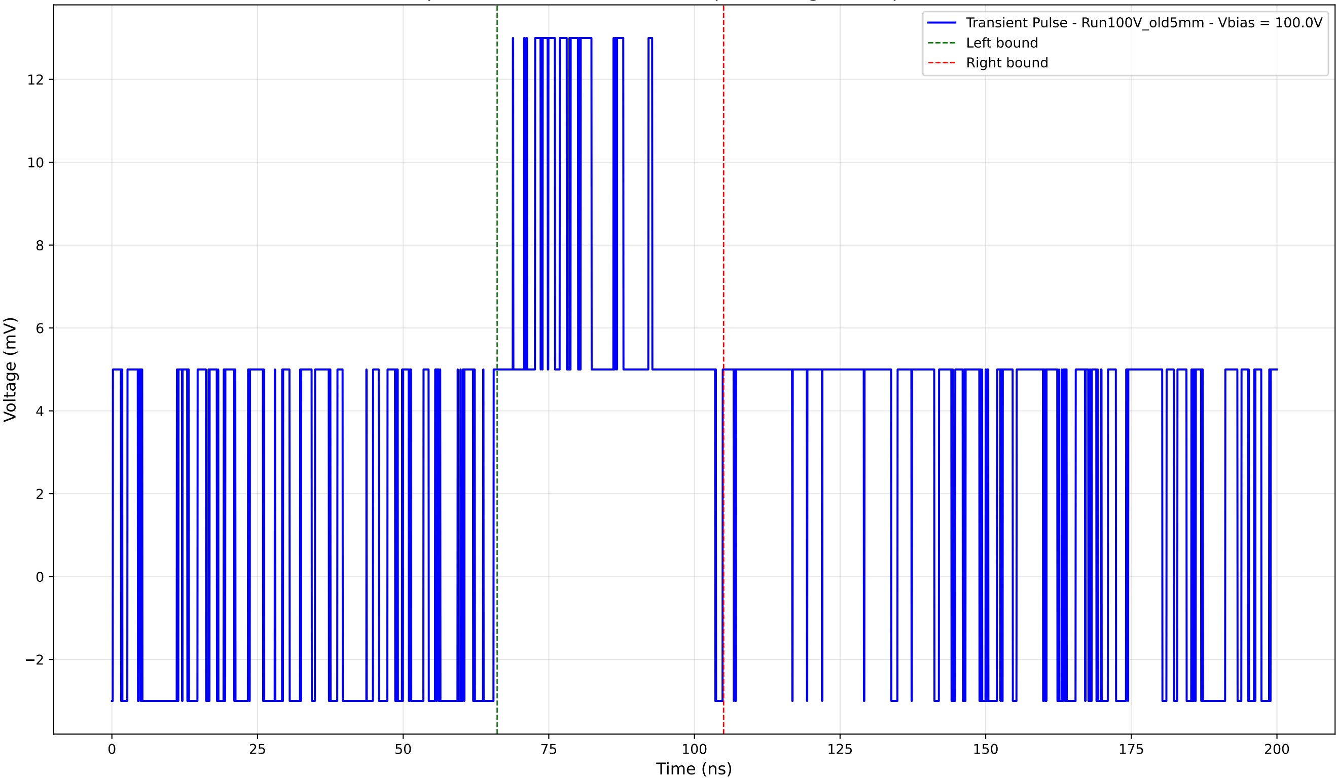
Transient Pulse - Sample: Old5mm - Position: 500.0 \mu\text{m} - Charge: 5.35 pC - Rise Time: 0.00 ns (N/A)
