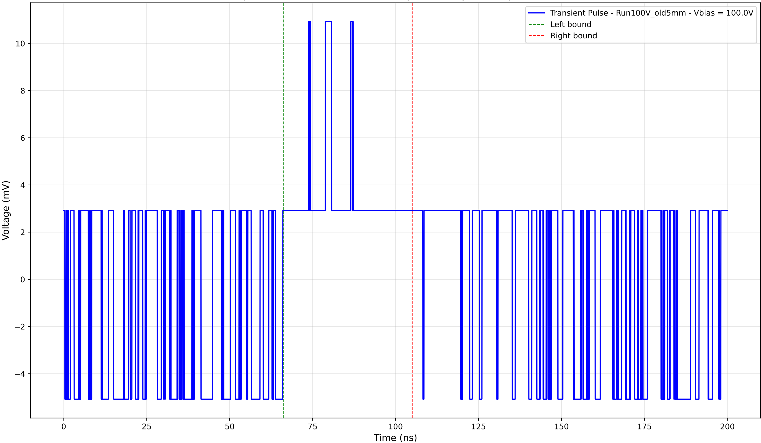
Transient Pulse - Sample: Old5mm - Position: 305.0 \mu\text{m} - Charge: 2.75 pC - Rise Time: 0.00 ns (N/A)
