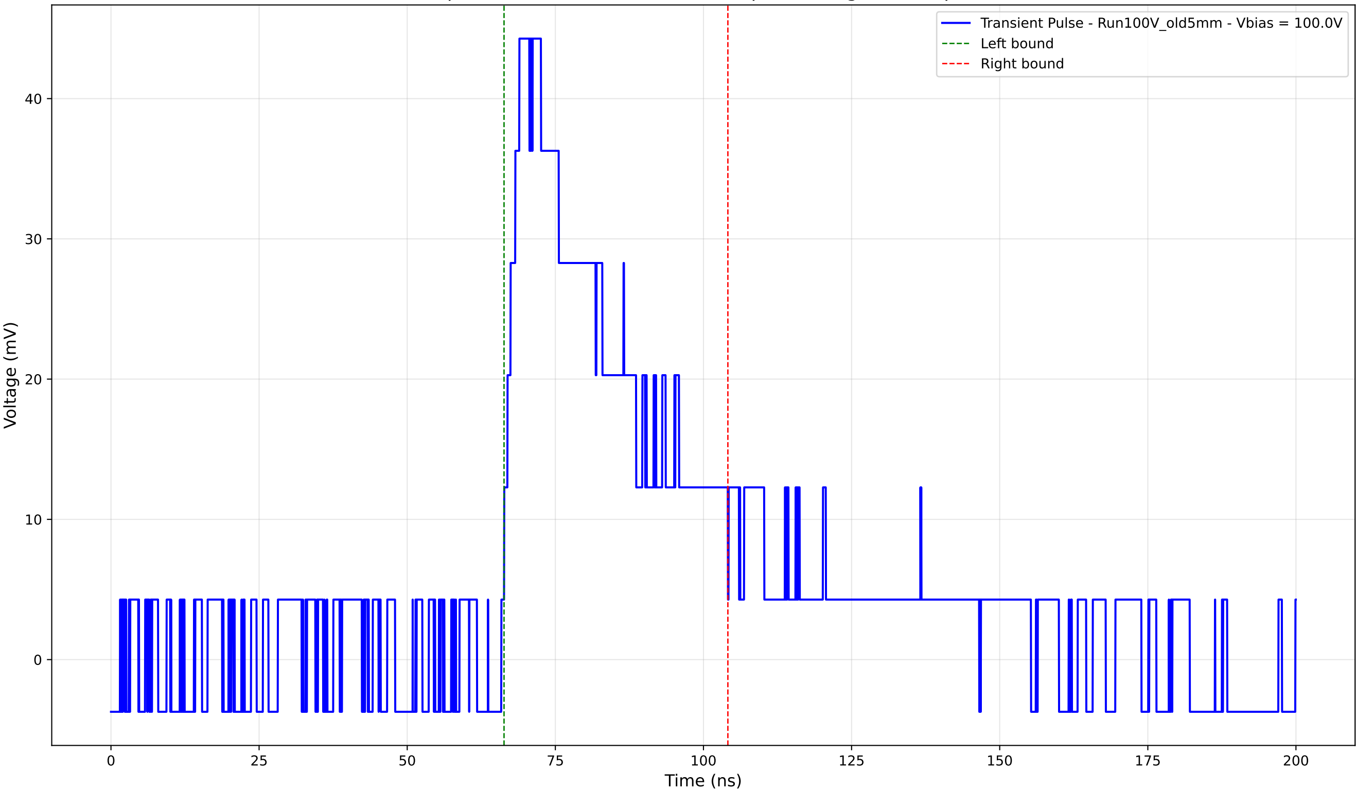
Transient Pulse - Sample: Old5mm - Position: 4875.0 \mu\text{m} - Charge: 17.30 pC - Rise Time: 2.58 ns
