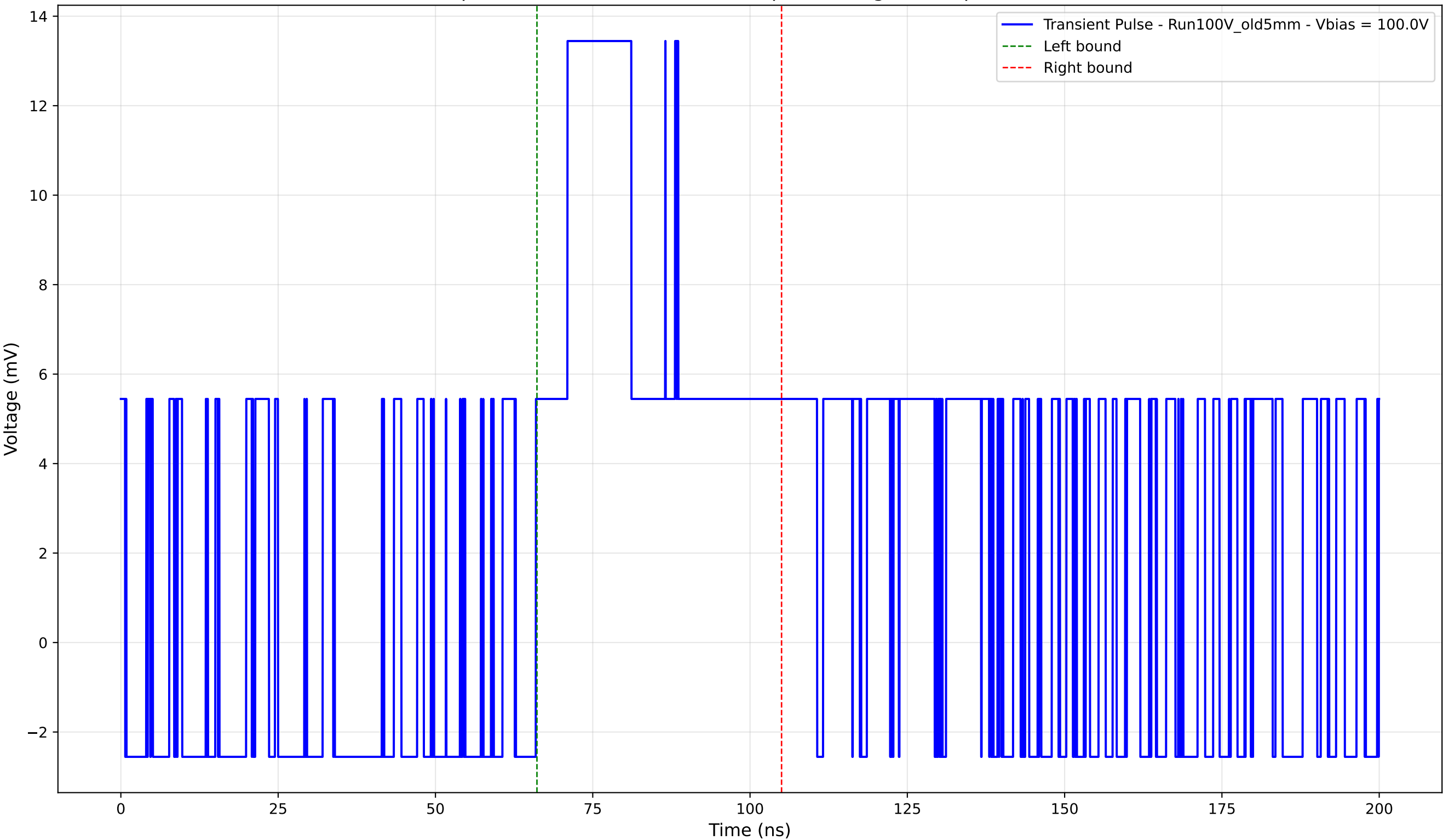
Transient Pulse - Sample: Old5mm - Position: 480.0 \mu\text{m} - Charge: 5.93 pC - Rise Time: 0.00 ns (N/A)
