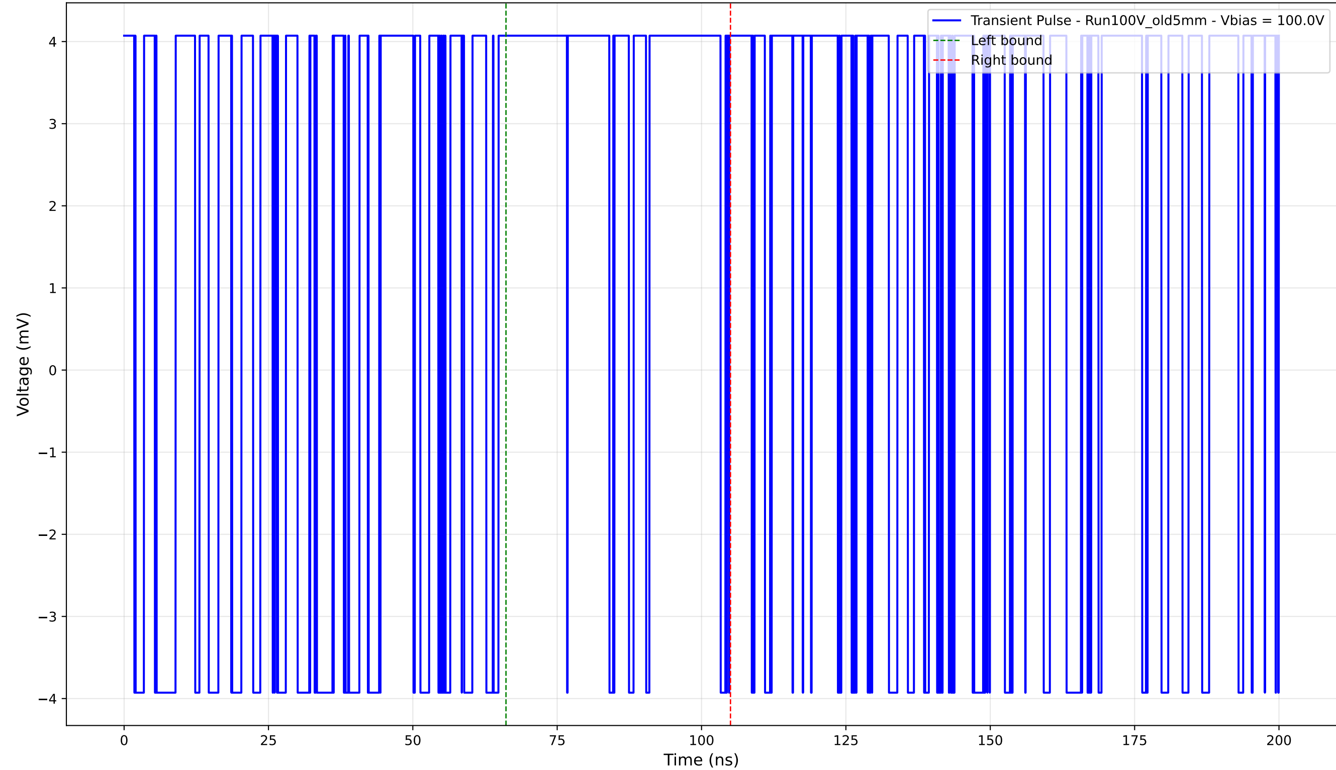
Transient Pulse - Sample: Old5mm - Position: 4310.0 \mu\text{m} - Charge: 2.63 pC - Rise Time: 0.00 ns (N/A)
