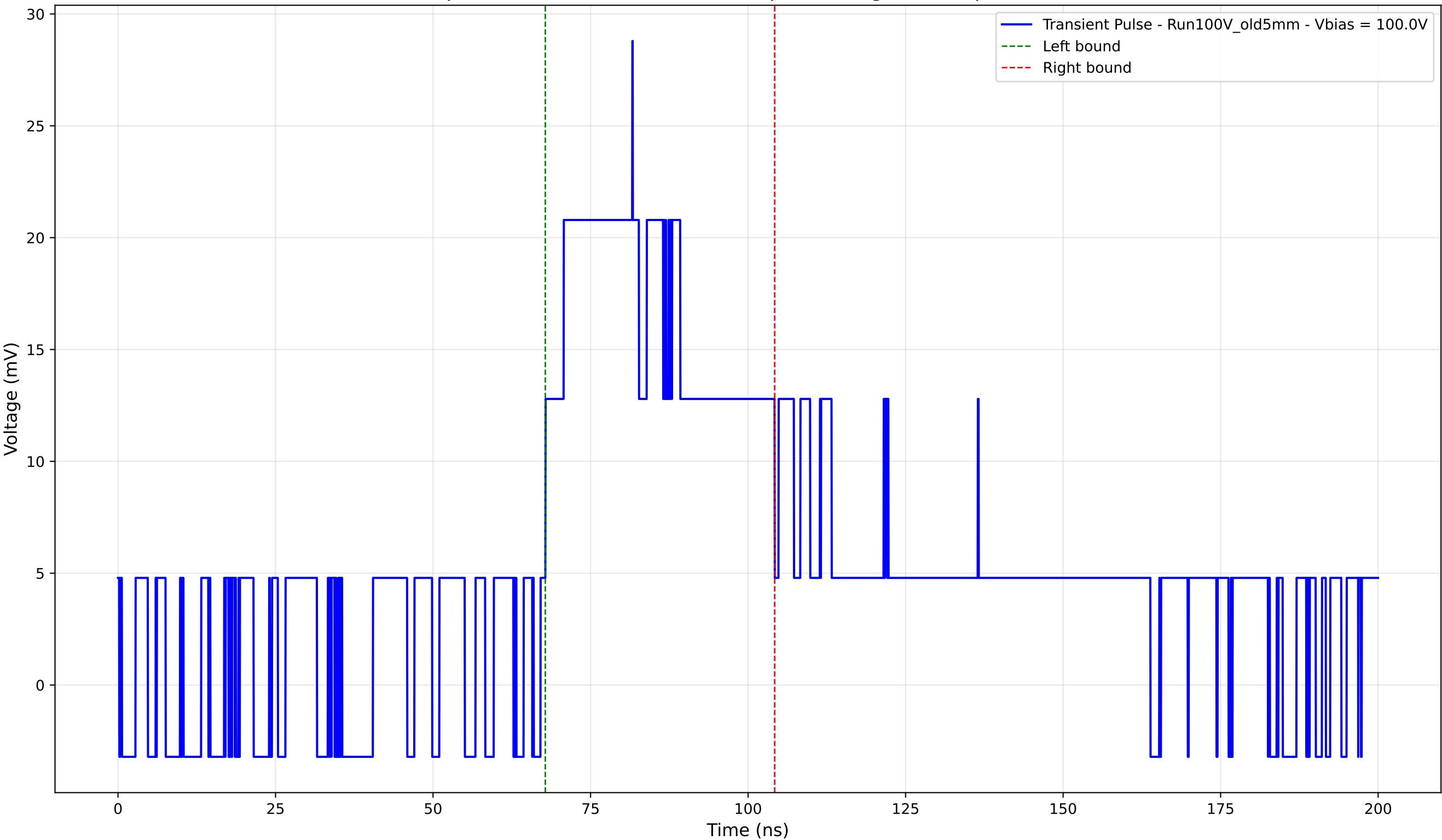
Transient Pulse - Sample: Old5mm - Position: 2020.0 \mu\text{m} - Charge: 11.94 pC - Rise Time: 0.00 ns (N/A)
