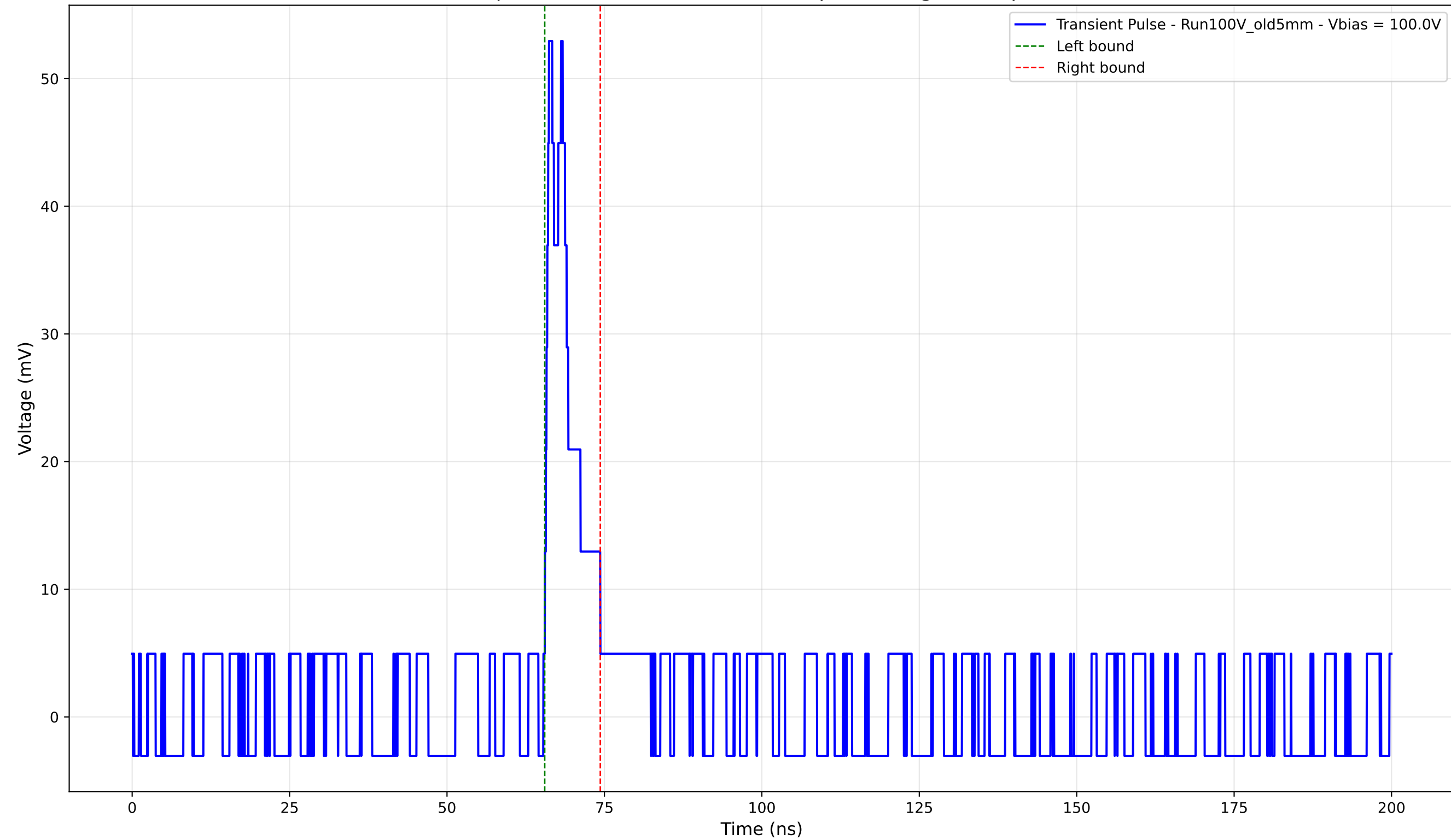
Transient Pulse - Sample: Old5mm - Position: 3755.0 \mu\text{m} - Charge: 4.66 pC - Rise Time: 0.66 ns
