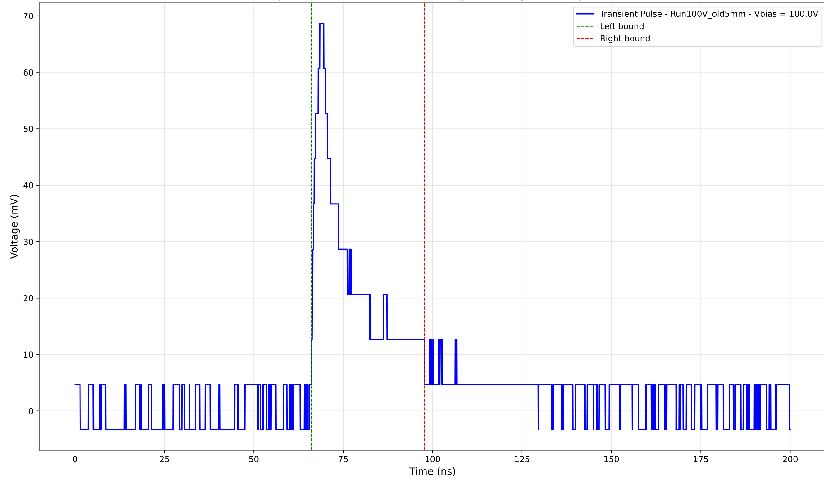
Transient Pulse - Sample: Old5mm - Position: 4415.0 \mu\text{m} - Charge: 15.23 pC - Rise Time: 2.37 ns
