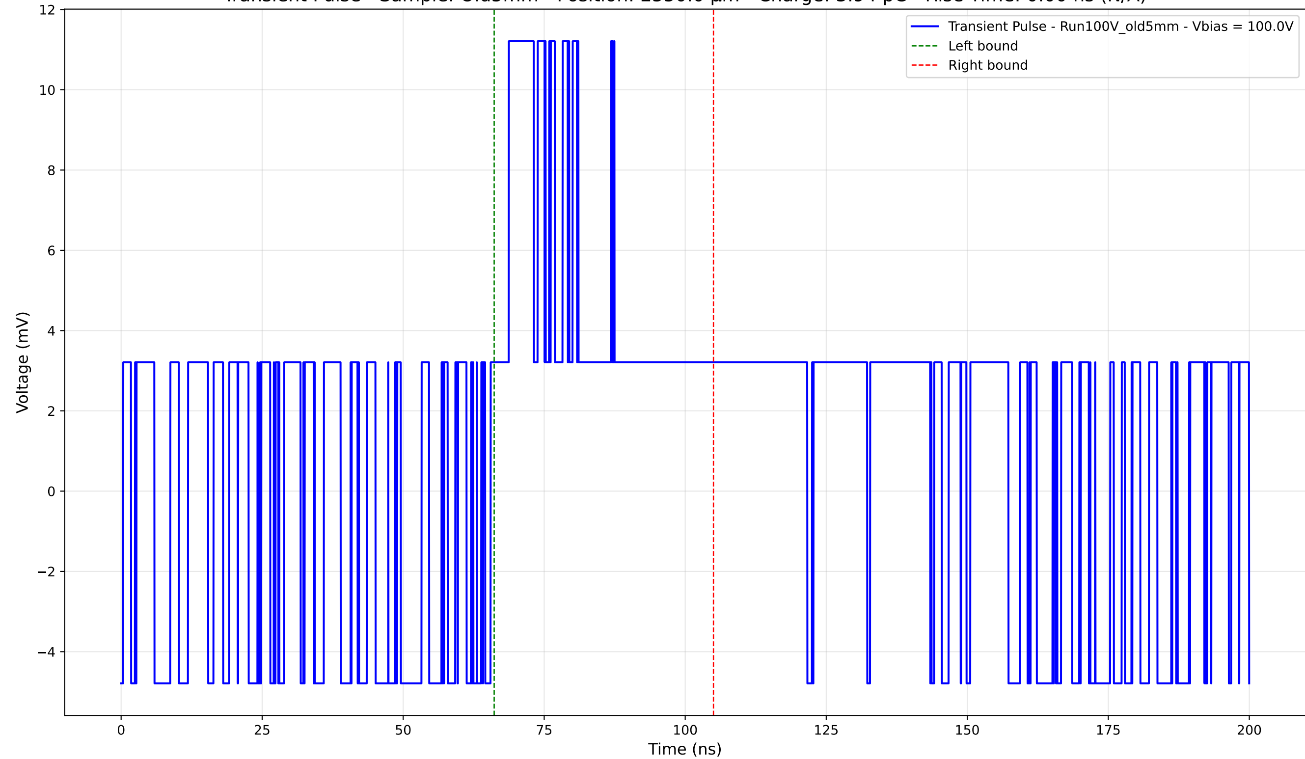
Transient Pulse - Sample: Old5mm - Position: 2550.0 \mu\text{m} - Charge: 3.94 pC - Rise Time: 0.00 ns (N/A)
