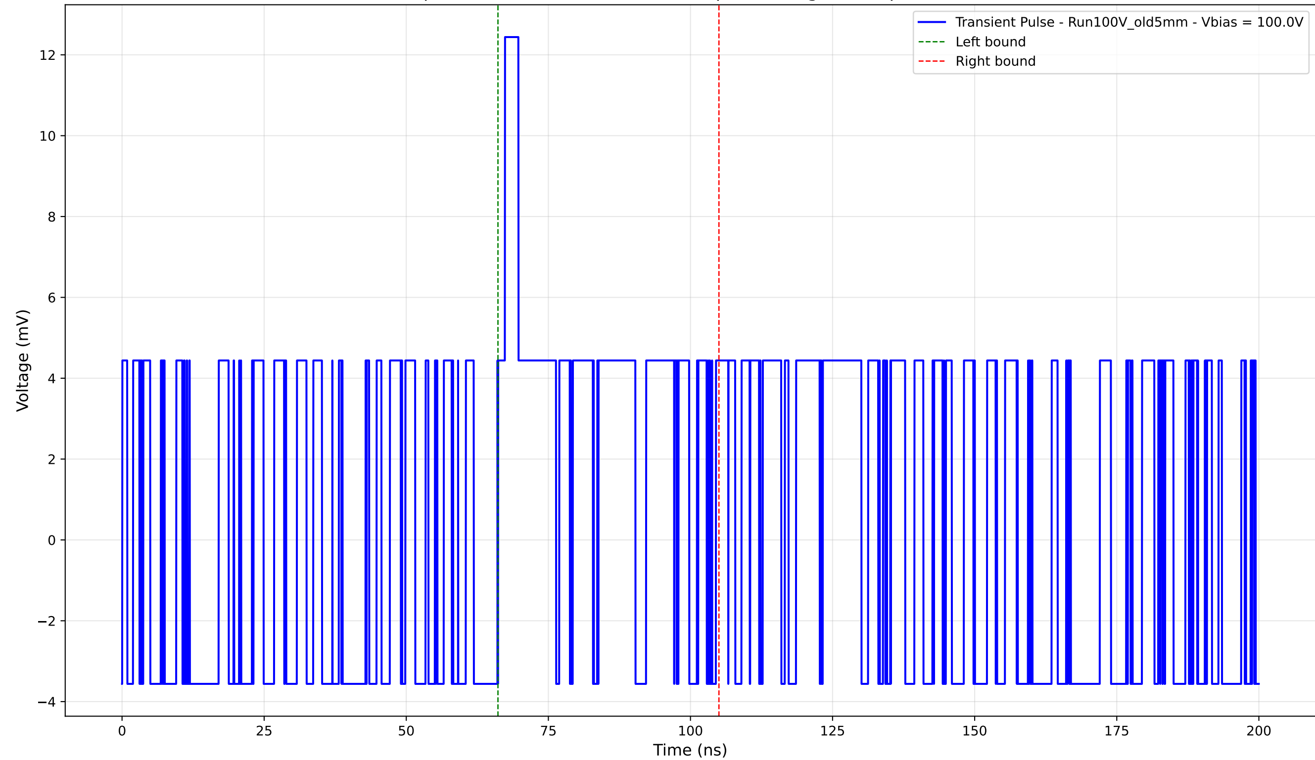
Transient Pulse - Sample: Old5mm - Position: 3065.0 \mu\text{m} - Charge: 2.77 pC - Rise Time: 0.00 ns (N/A)
