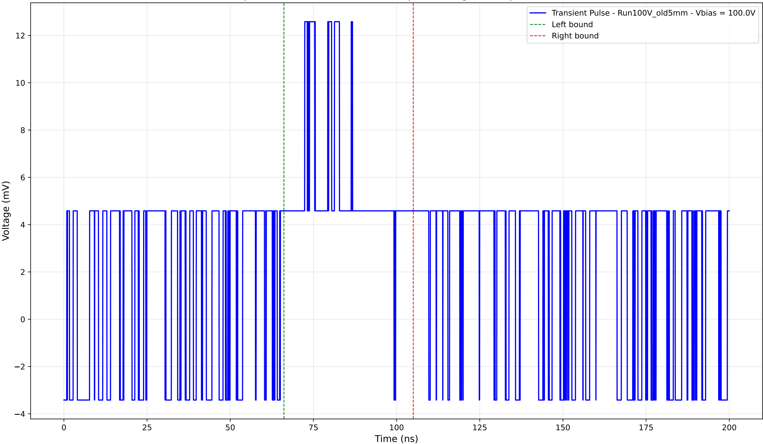
Transient Pulse - Sample: Old5mm - Position: 845.0 \mu\text{m} - Charge: 4.39 pC - Rise Time: 0.00 ns (N/A)
