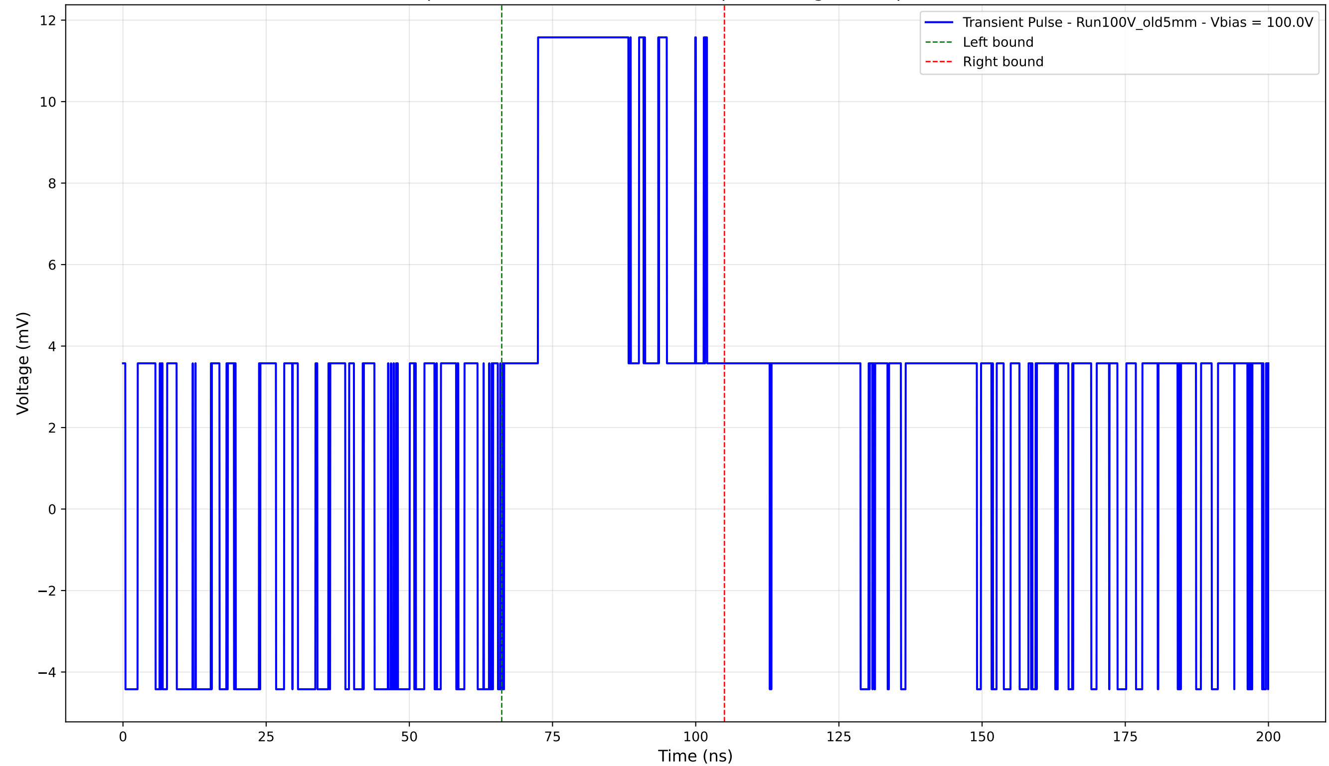
Transient Pulse - Sample: Old5mm - Position: 1245.0 \mu\text{m} - Charge: 5.75 pC - Rise Time: 0.00 ns (N/A)
