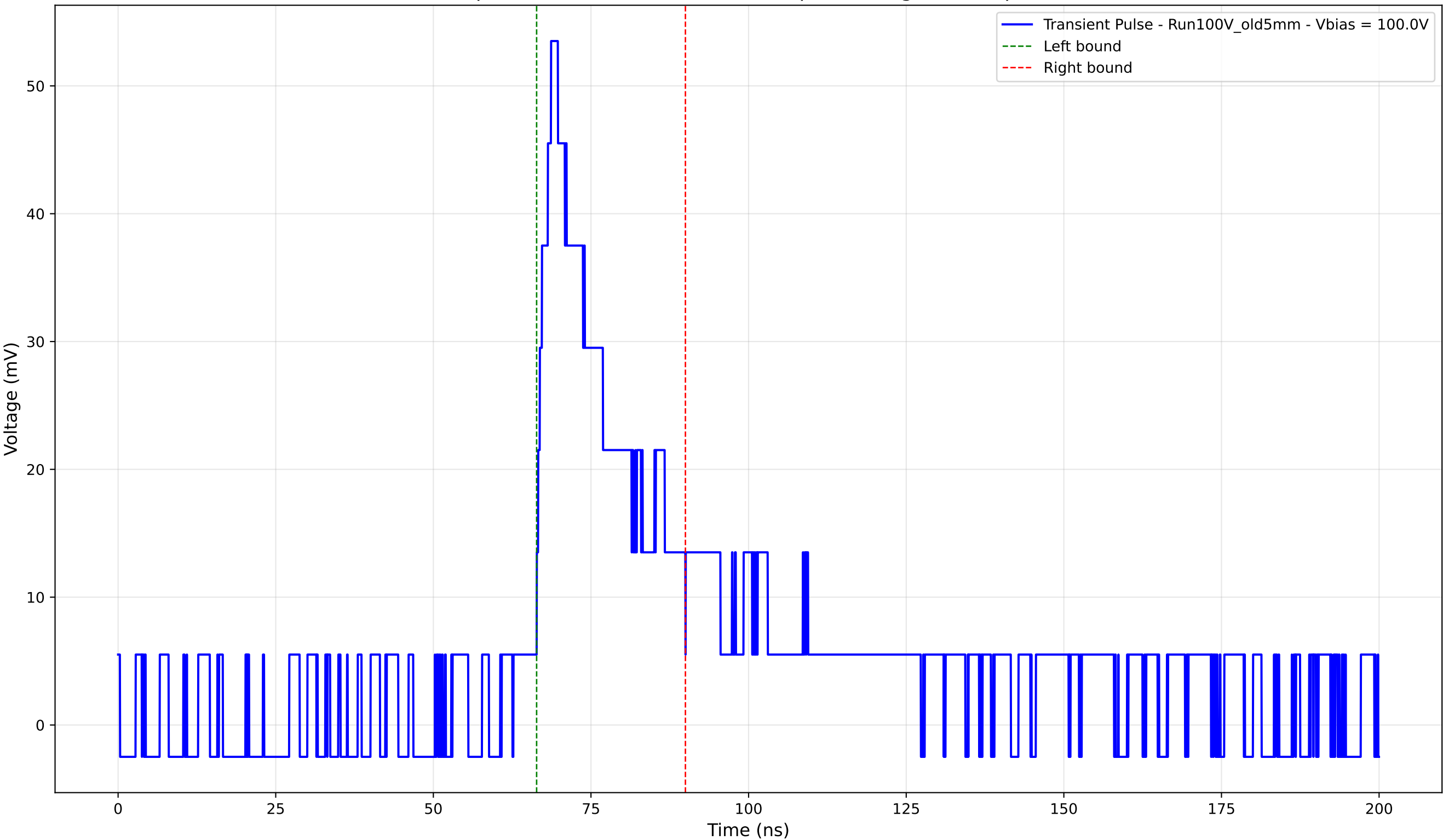
Transient Pulse - Sample: Old5mm - Position: 2900.0 \mu\text{m} - Charge: 12.44 pC - Rise Time: 5.96 ns
