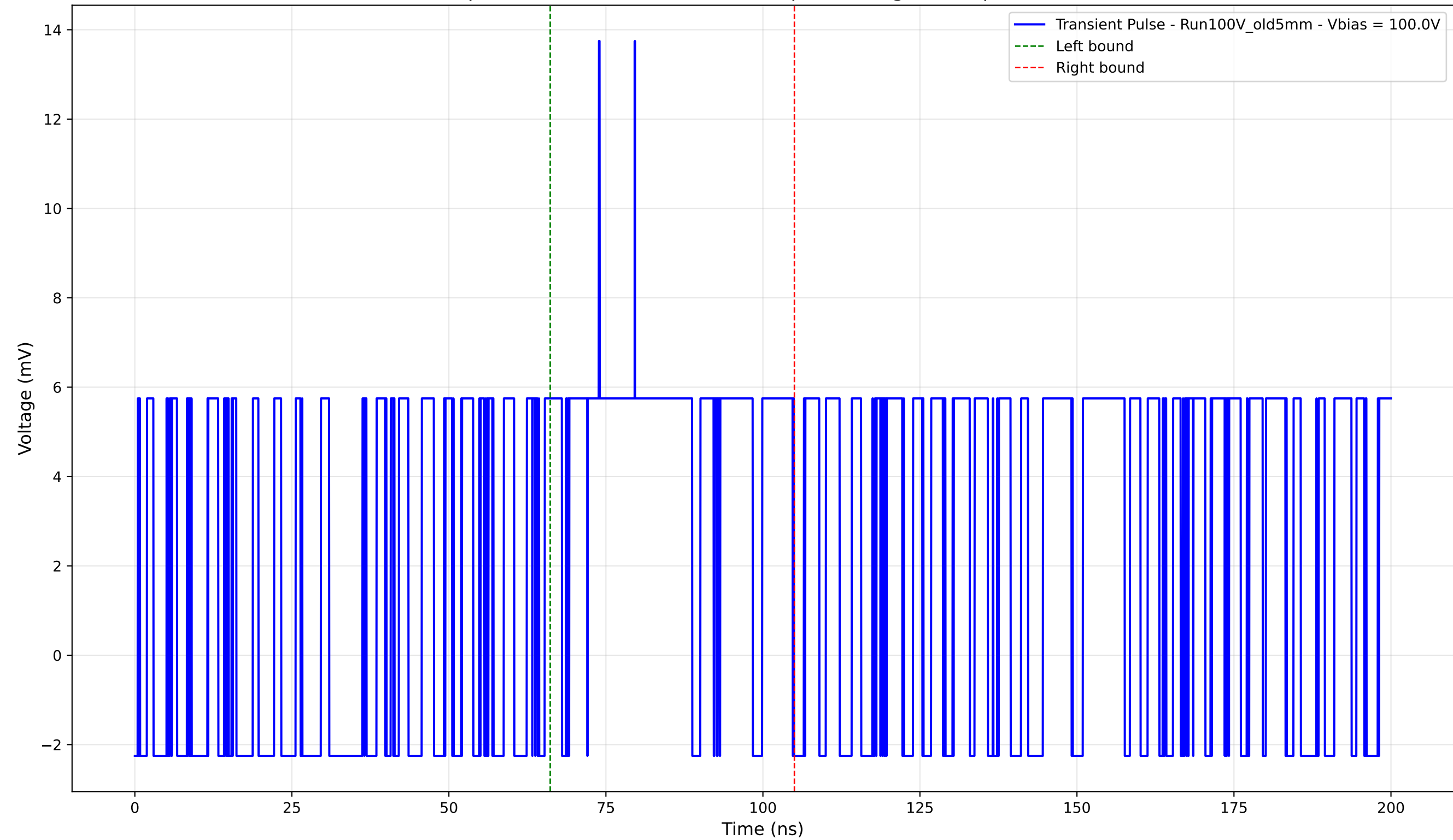
Transient Pulse - Sample: Old5mm - Position: 2120.0 \mu\text{m} - Charge: 3.81 pC - Rise Time: 0.00 ns (N/A)
