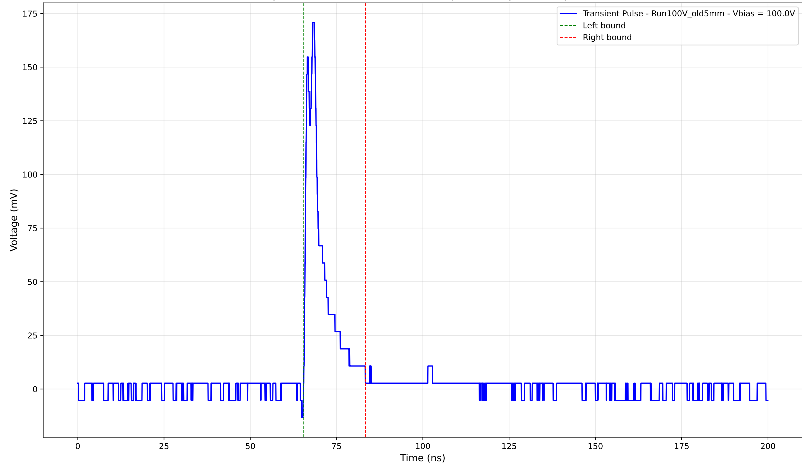
Transient Pulse - Sample: Old5mm - Position: 3895.0 \mu\text{m} - Charge: 17.96 pC - Rise Time: 0.90 ns
