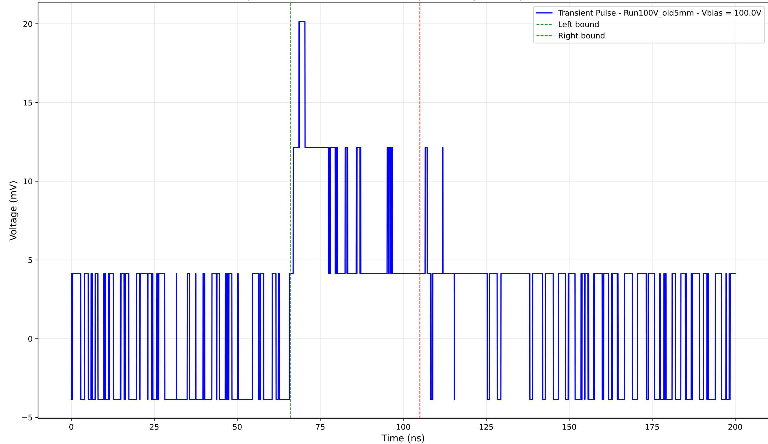
Transient Pulse - Sample: Old5mm - Position: 4675.0 \mu\text{m} - Charge: 6.06 pC - Rise Time: 0.00 ns (N/A)
