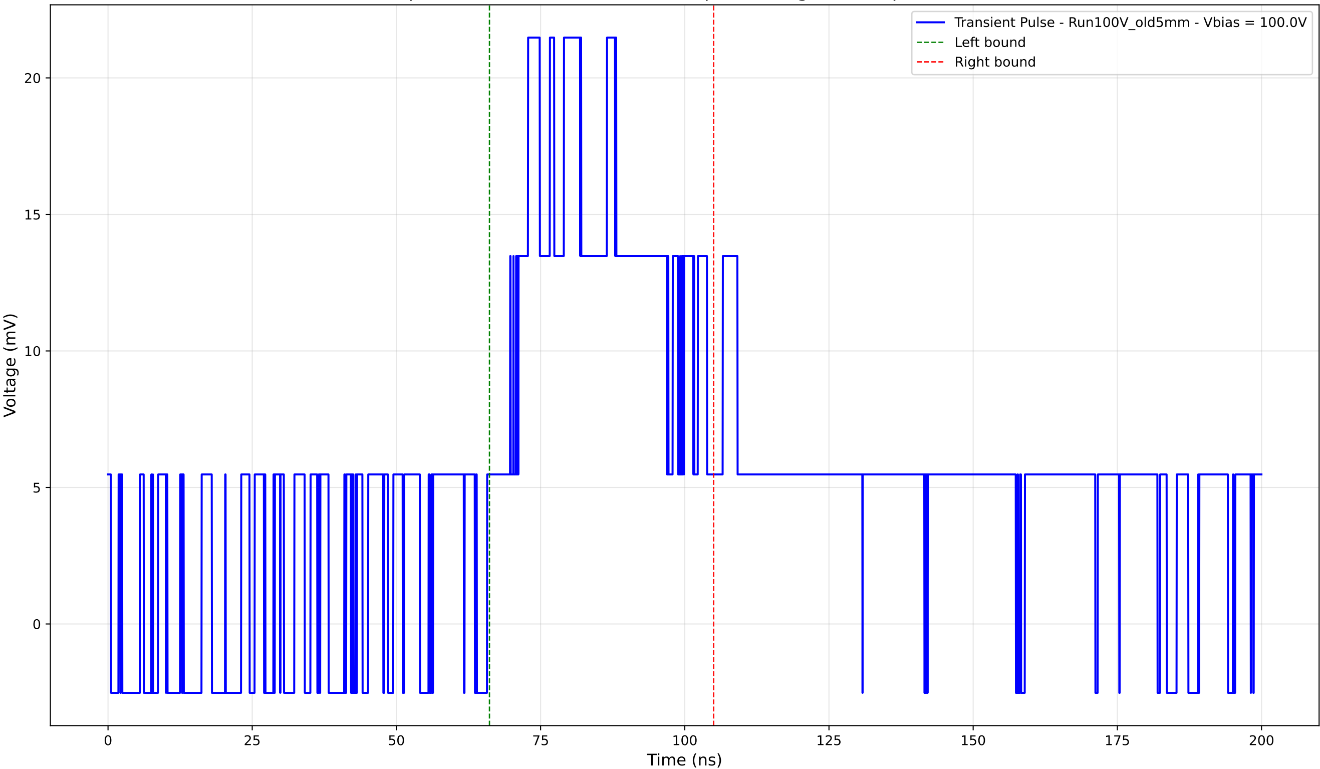
Transient Pulse - Sample: Old5mm - Position: 1410.0 \mu\text{m} - Charge: 10.33 pC - Rise Time: 0.00 ns (N/A)
