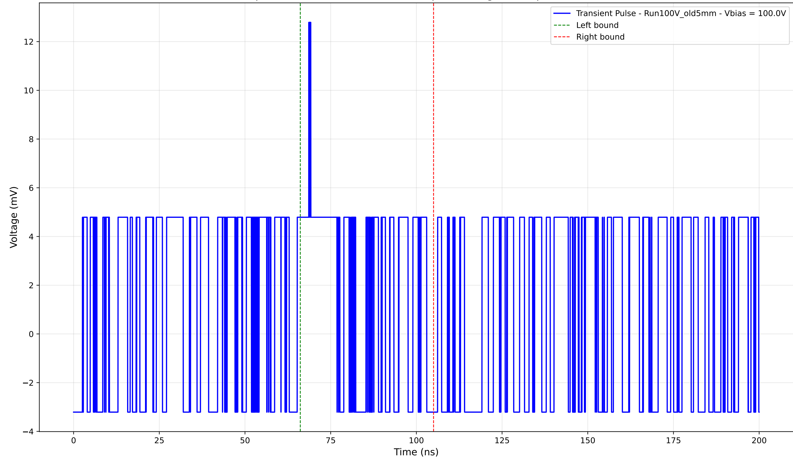
Transient Pulse - Sample: Old5mm - Position: 4025.0 \mu\text{m} - Charge: 1.61 pC - Rise Time: 0.00 ns (N/A)
