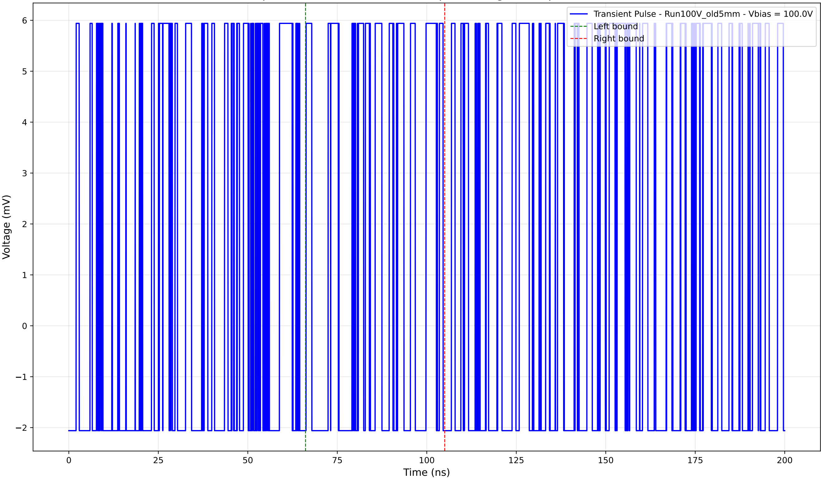
Transient Pulse - Sample: Old5mm - Position: 155.0 \mu\text{m} - Charge: 1.34 pC - Rise Time: 0.00 ns (N/A)
