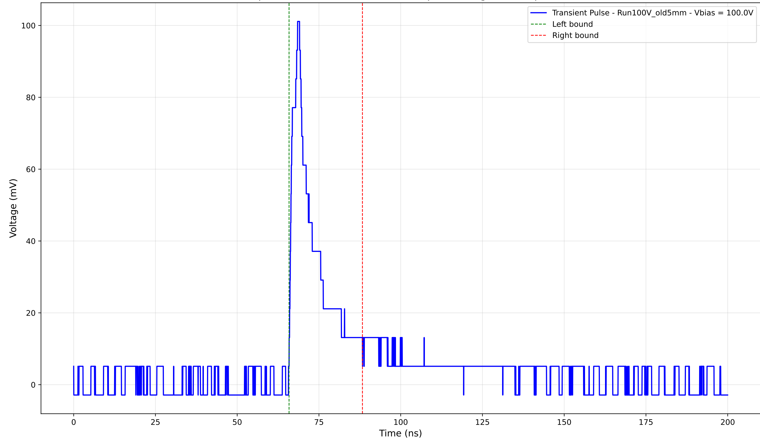
Transient Pulse - Sample: Old5mm - Position: 3210.0 \mu\text{m} - Charge: 15.74 pC - Rise Time: 2.31 ns
