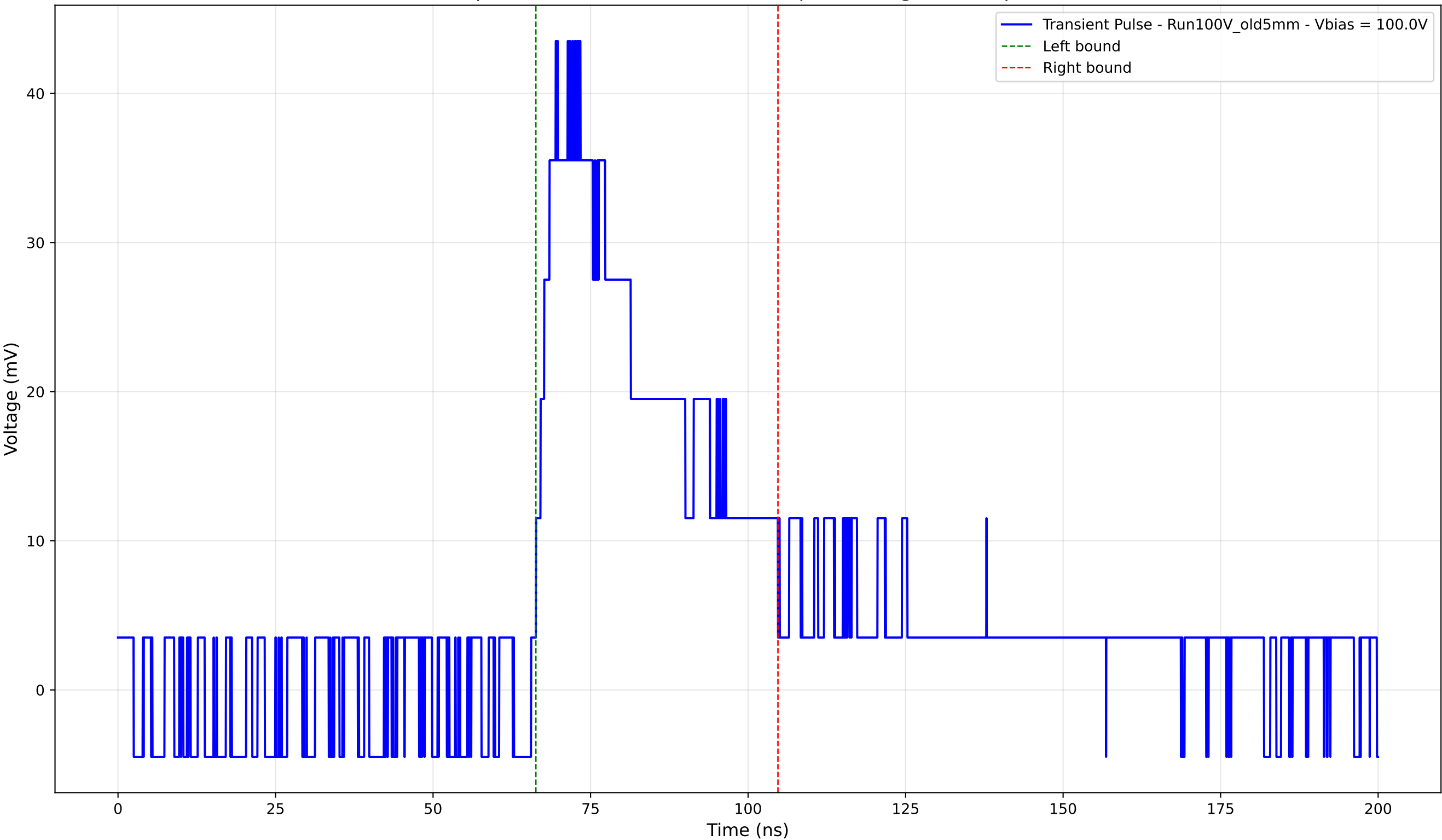
Transient Pulse - Sample: Old5mm - Position: 4900.0 \mu\text{m} - Charge: 16.69 pC - Rise Time: 3.14 ns
