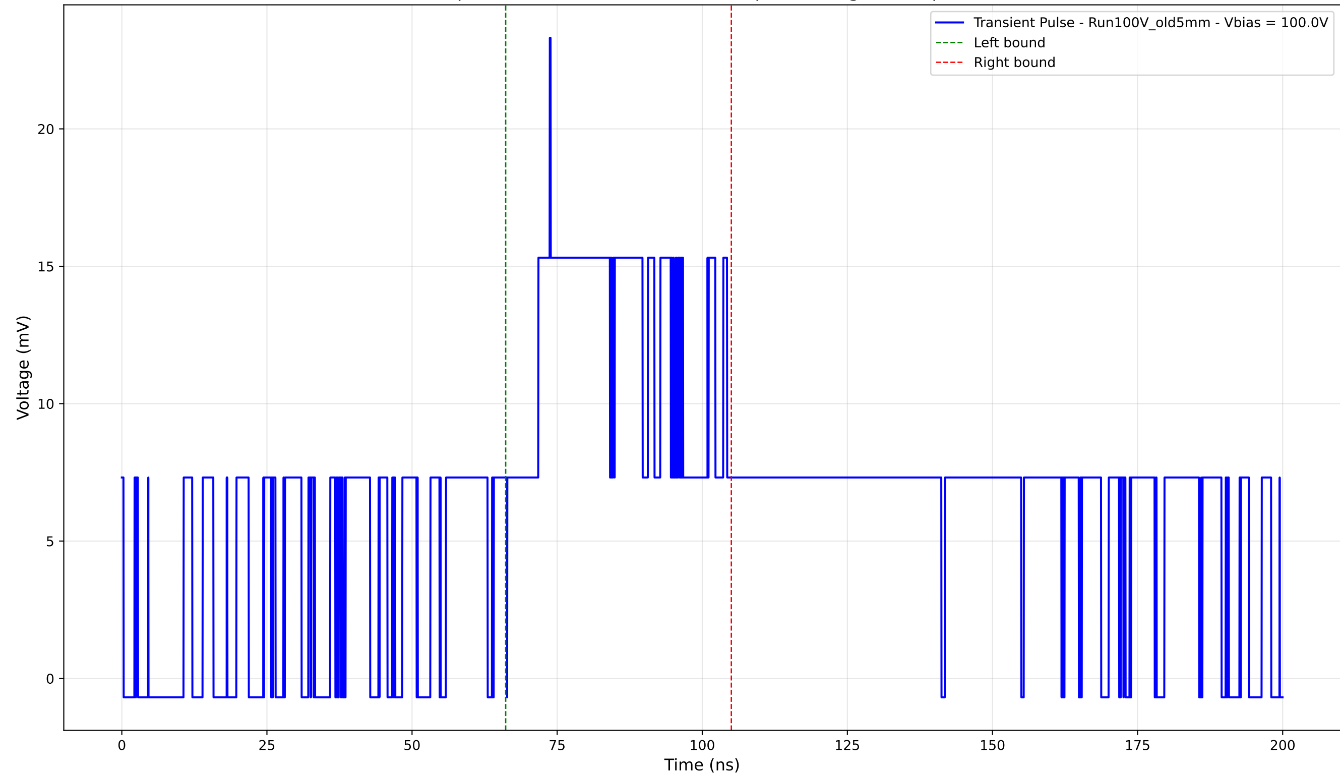
Transient Pulse - Sample: Old5mm - Position: 1370.0 \mu\text{m} - Charge: 9.39 pC - Rise Time: 7.34 ns
