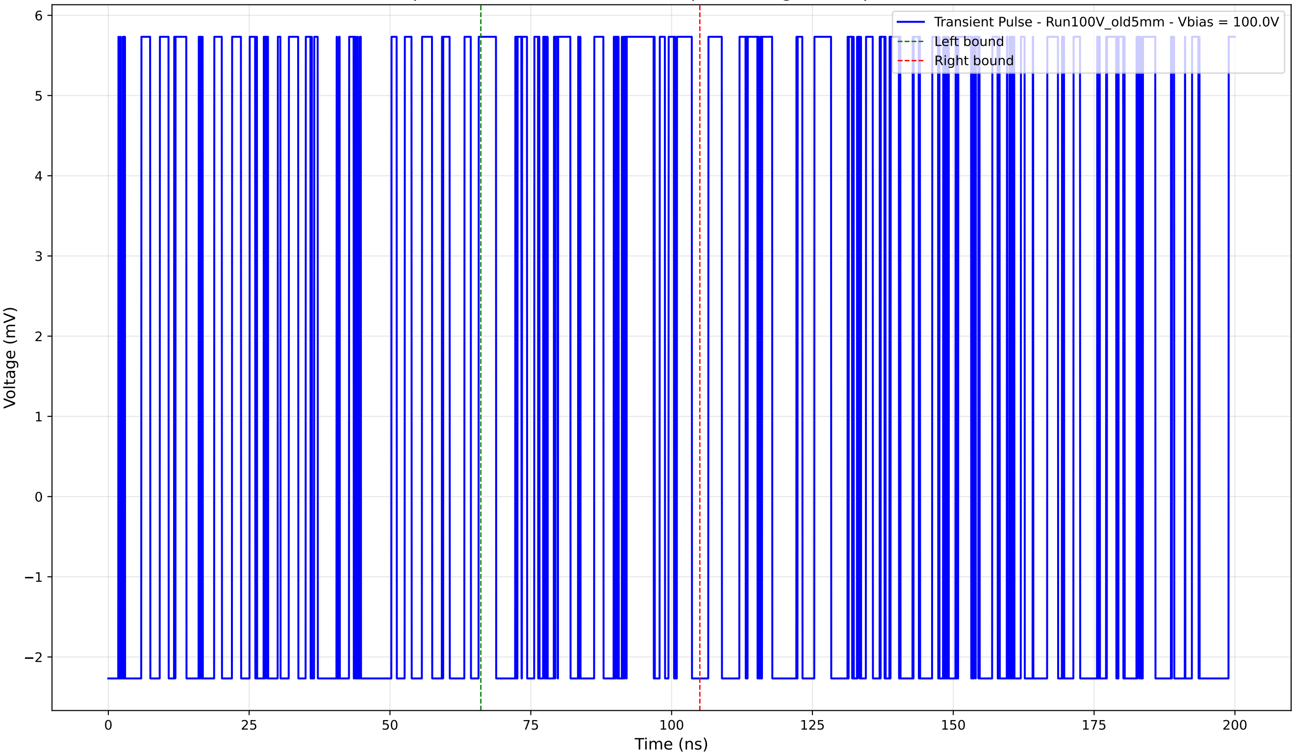
Transient Pulse - Sample: Old5mm - Position: 115.0 \mu\text{m} - Charge: 1.57 pC - Rise Time: 0.00 ns (N/A)
