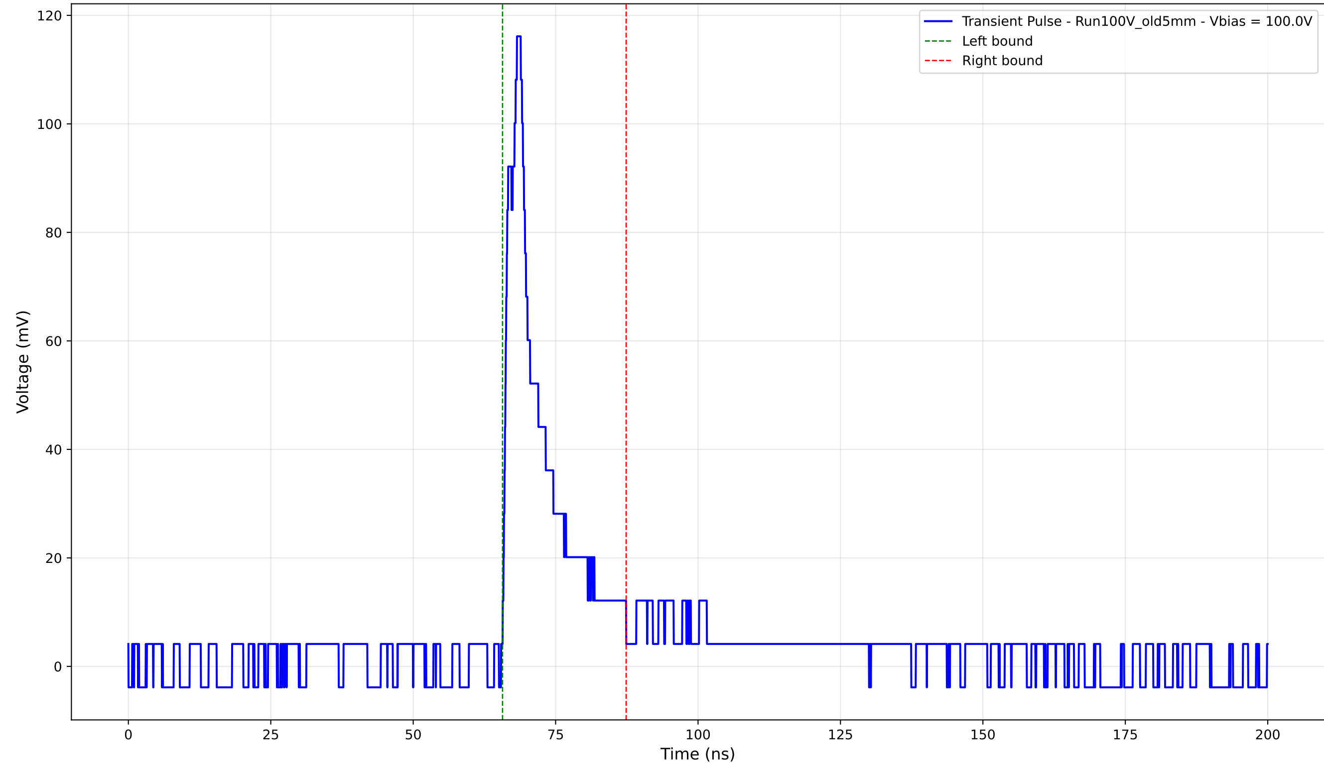
Transient Pulse - Sample: Old5mm - Position: 3295.0 \mu\text{m} - Charge: 16.17 pC - Rise Time: 2.28 ns
