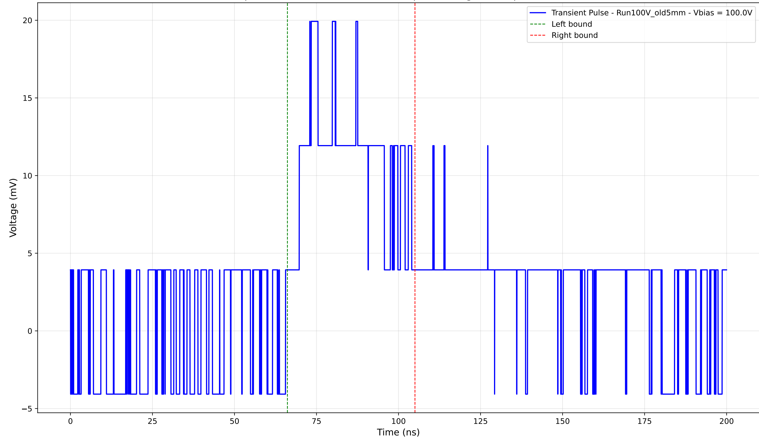
Transient Pulse - Sample: Old5mm - Position: 1980.0 \mu\text{m} - Charge: 8.45 pC - Rise Time: 0.00 ns (N/A)
