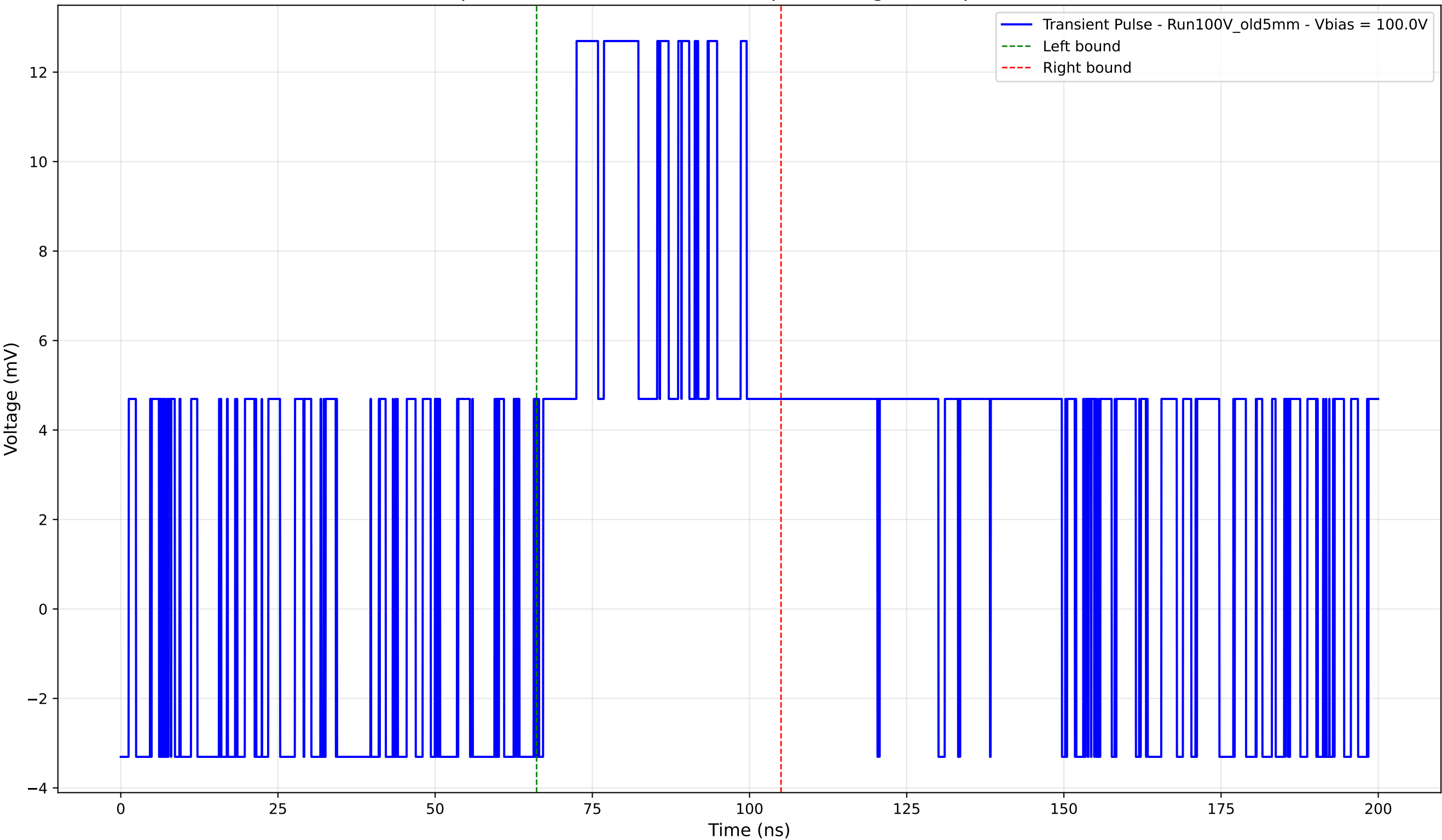
Transient Pulse - Sample: Old5mm - Position: 880.0 \mu\text{m} - Charge: 5.95 pC - Rise Time: 0.00 ns (N/A)
