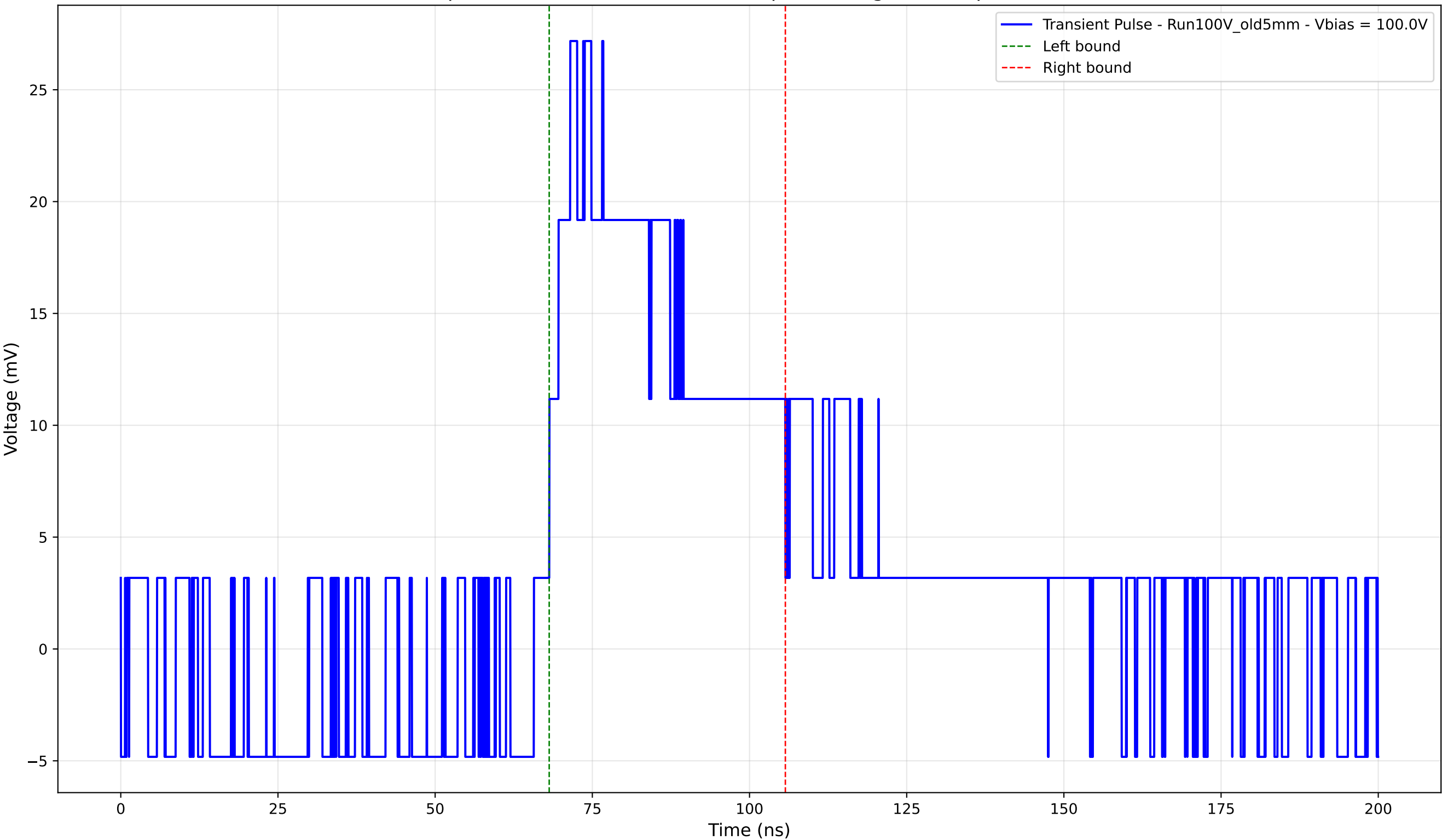
Transient Pulse - Sample: Old5mm - Position: 2235.0 \mu\text{m} - Charge: 11.67 pC - Rise Time: 0.00 ns (N/A)
