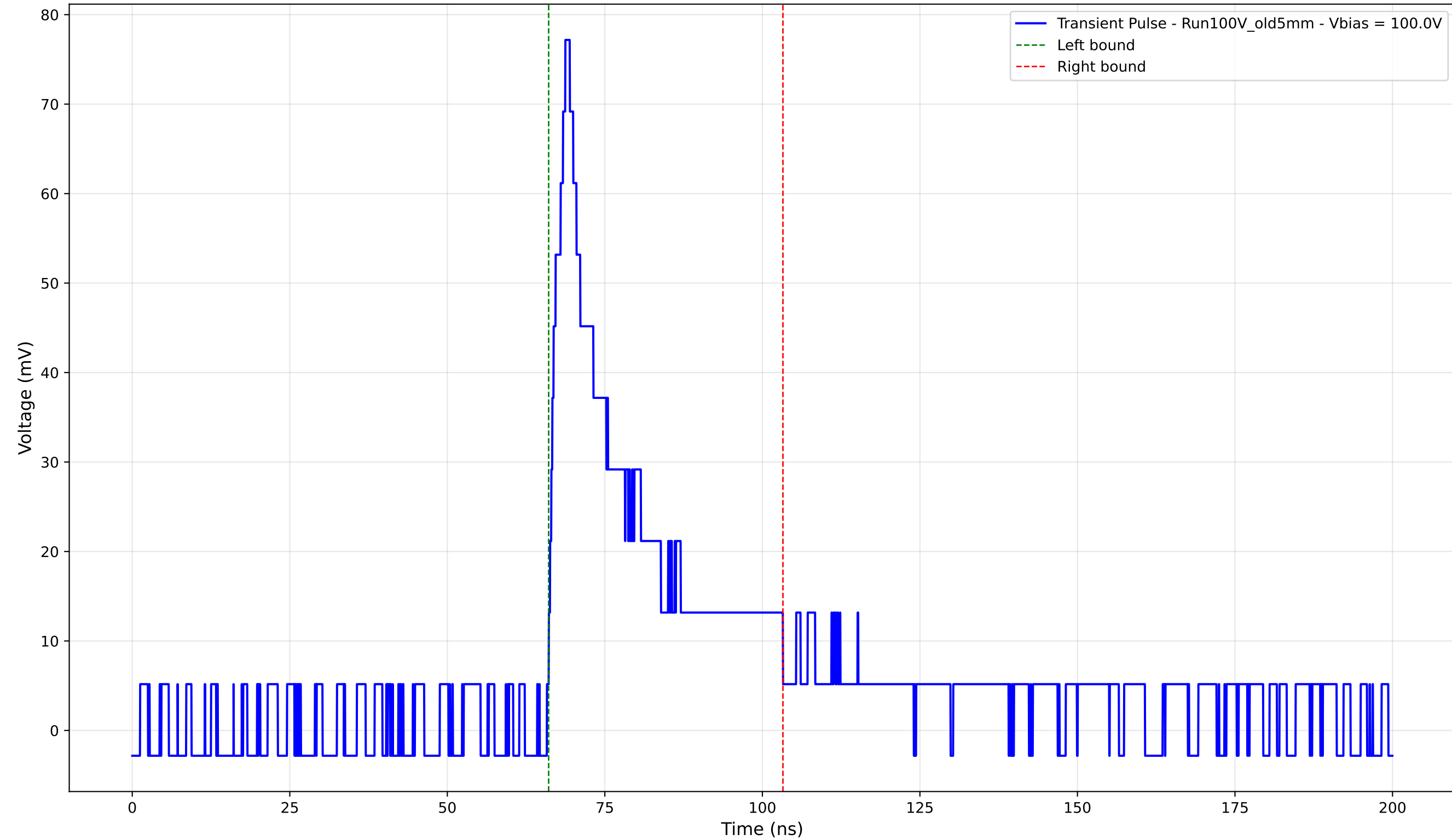
Transient Pulse - Sample: Old5mm - Position: 4455.0 \mu\text{m} - Charge: 18.79 pC - Rise Time: 2.63 ns
