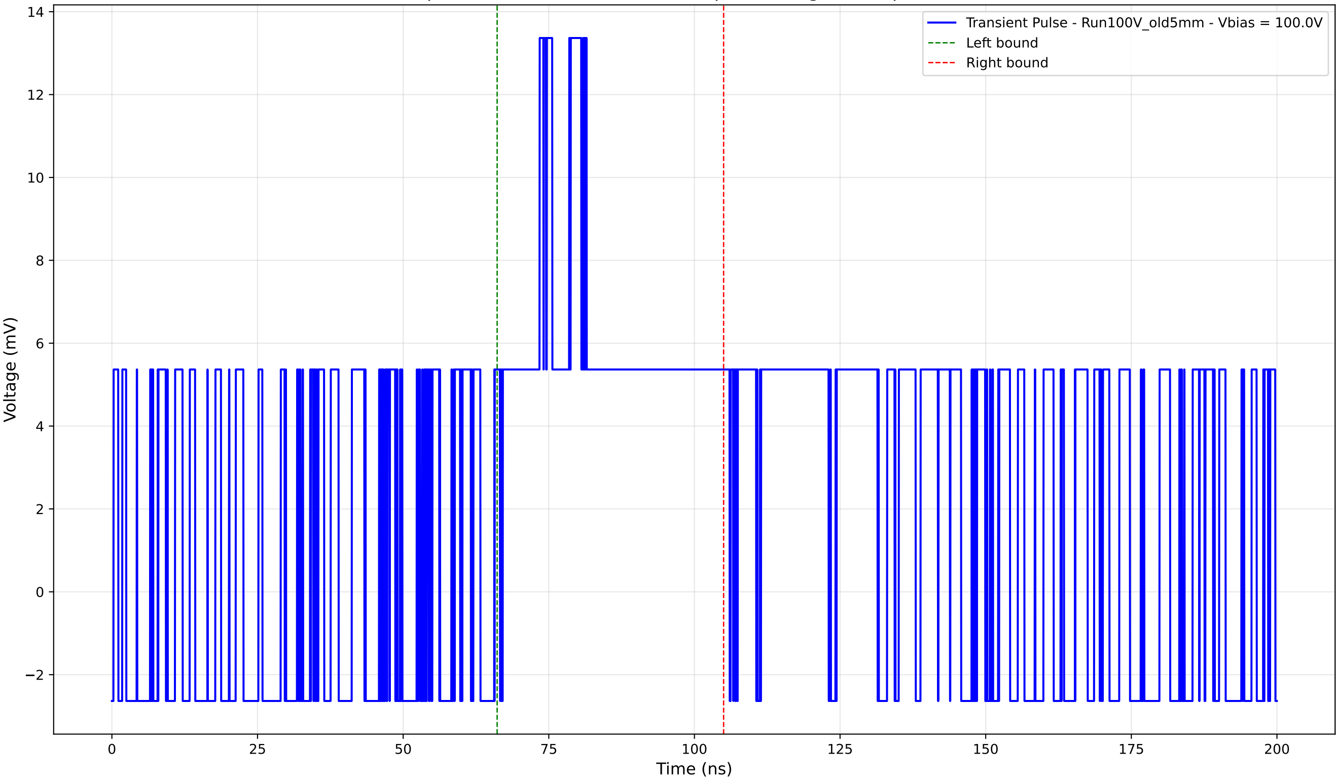
Transient Pulse - Sample: Old5mm - Position: 605.0 \mu\text{m} - Charge: 4.81 pC - Rise Time: 0.00 ns (N/A)
