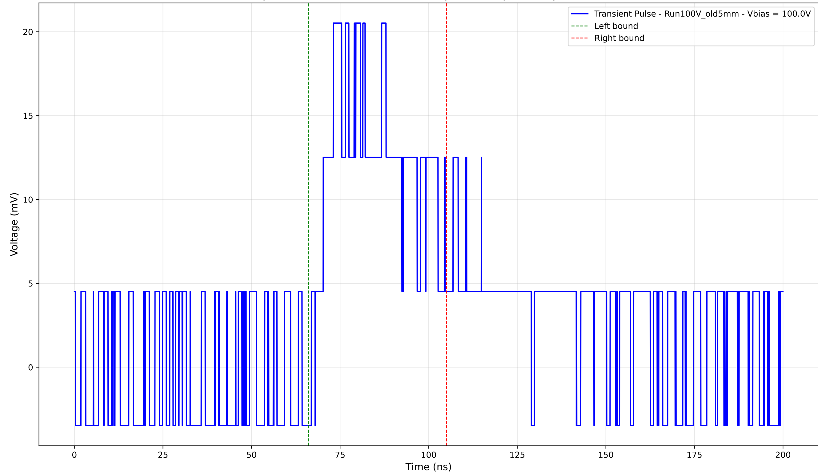
Transient Pulse - Sample: Old5mm - Position: 1625.0 \mu\text{m} - Charge: 9.48 pC - Rise Time: 0.00 ns (N/A)
