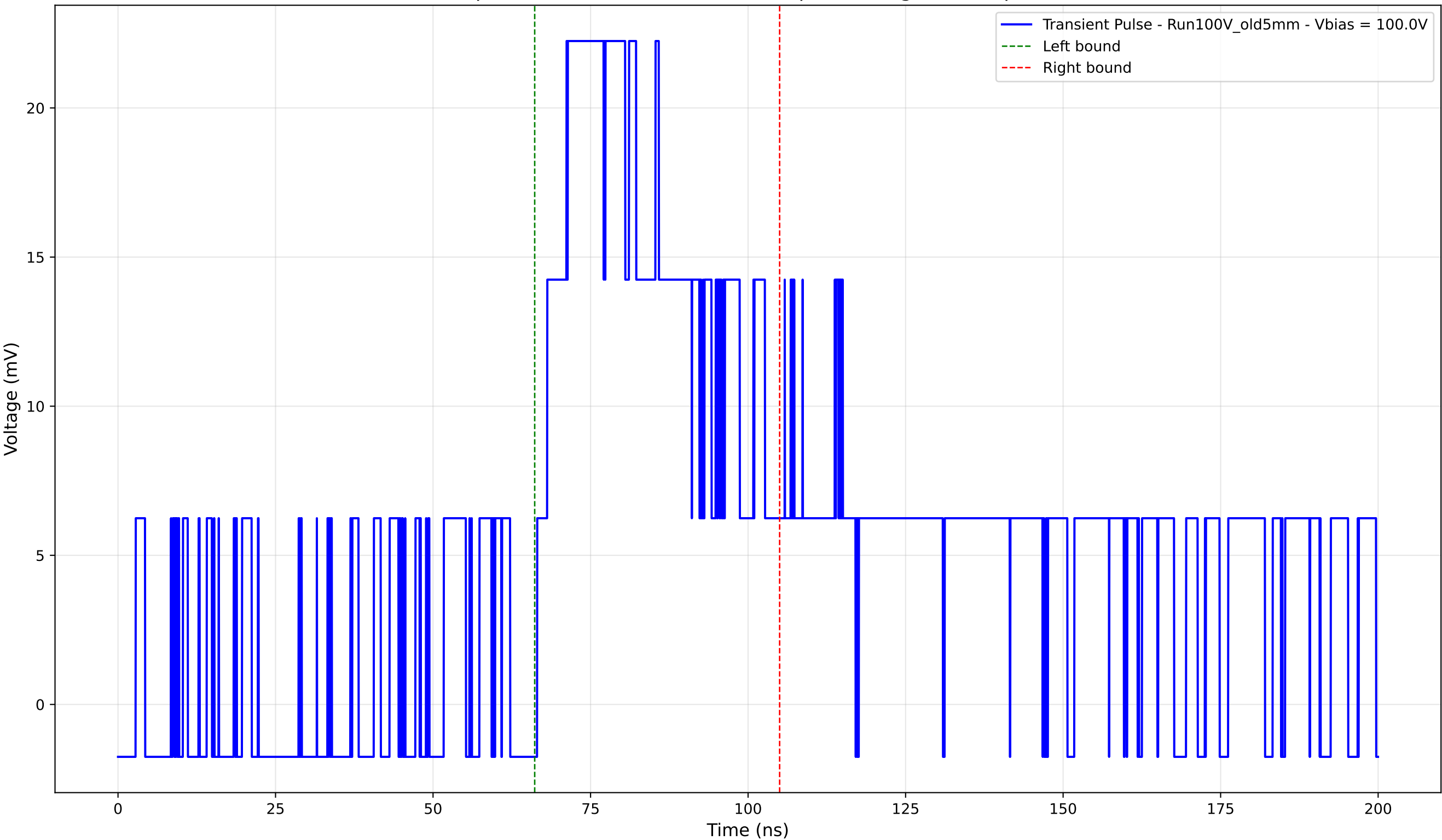
Transient Pulse - Sample: Old5mm - Position: 2255.0 \mu\text{m} - Charge: 11.39 pC - Rise Time: 4.68 ns
