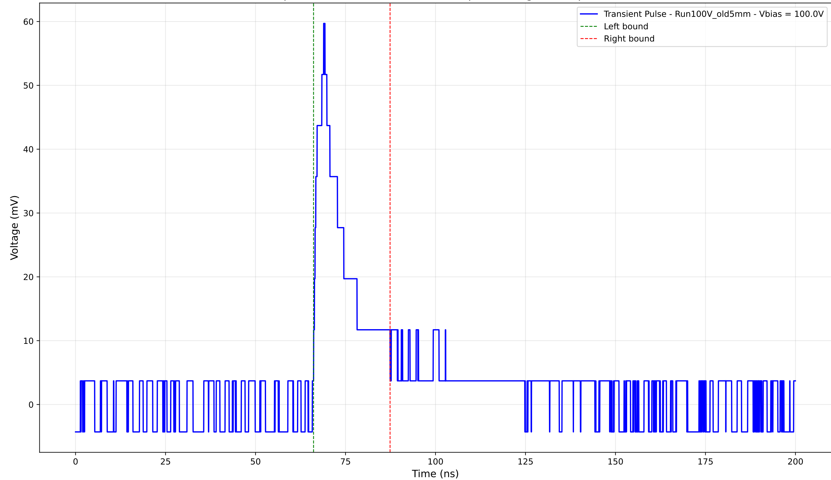
Transient Pulse - Sample: Old5mm - Position: 4400.0 \mu\text{m} - Charge: 9.95 pC - Rise Time: 2.79 ns
