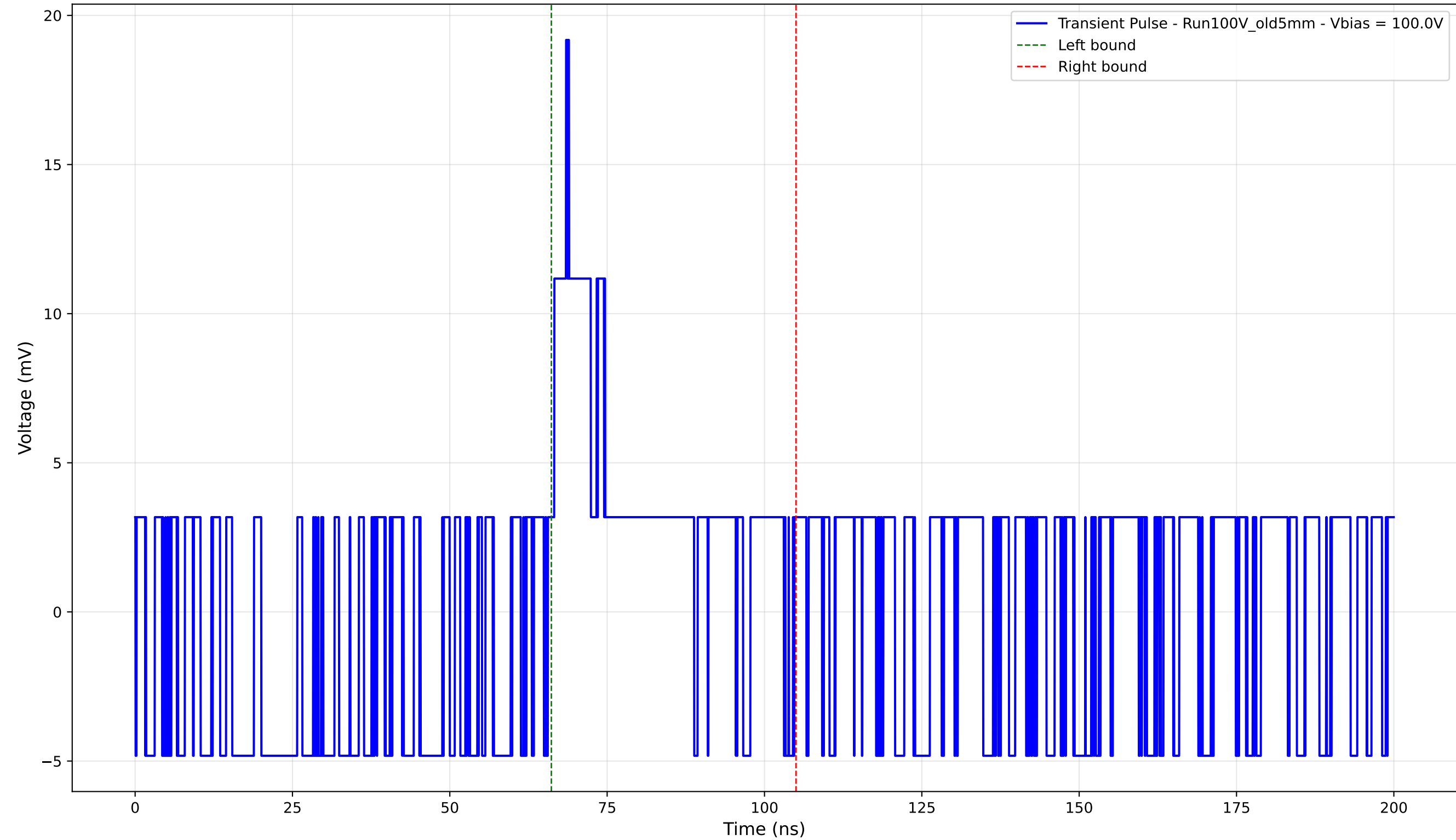
Transient Pulse - Sample: Old5mm - Position: 3140.0 \mu\text{m} - Charge: 3.11 pC - Rise Time: 0.00 ns (N/A)
