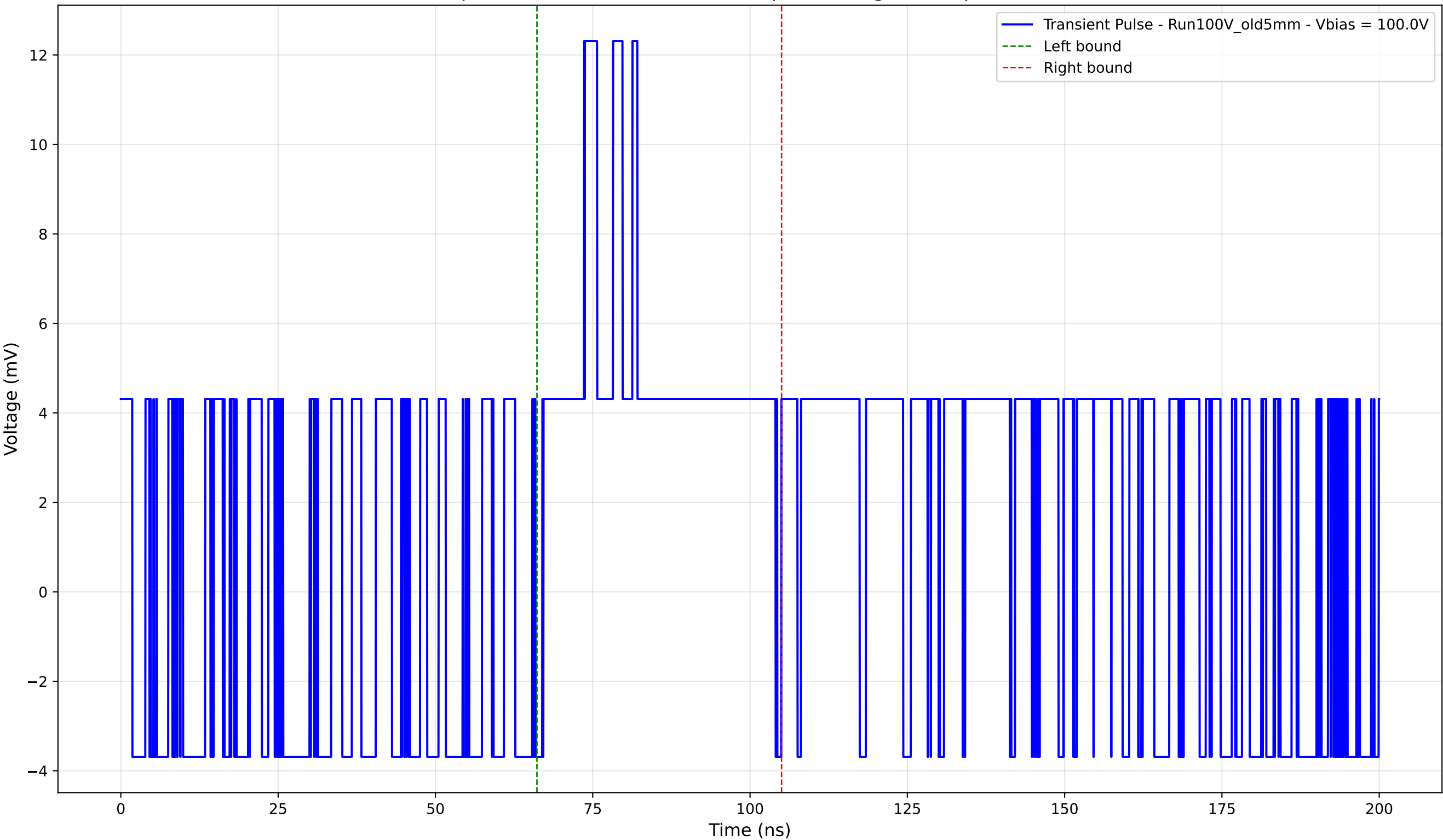
Transient Pulse - Sample: Old5mm - Position: 550.0 \mu\text{m} - Charge: 3.77 pC - Rise Time: 0.00 ns (N/A)
