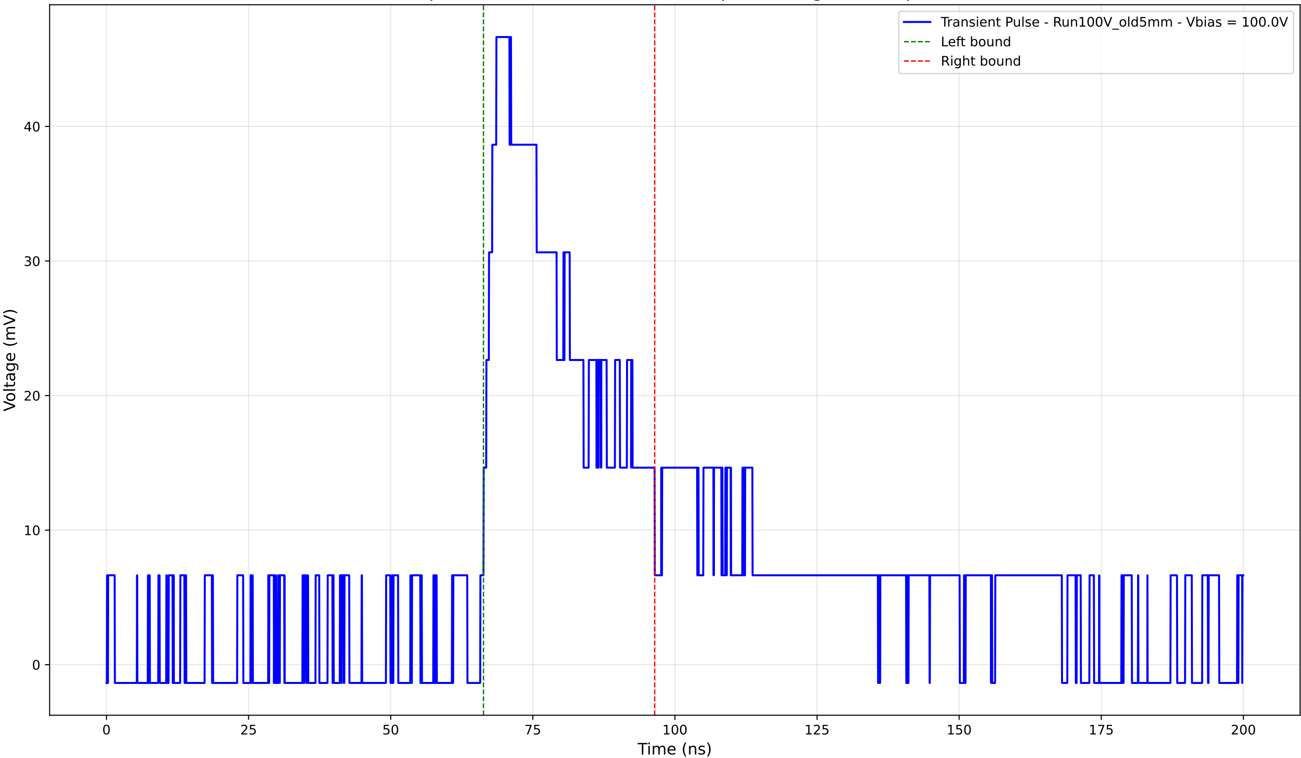
Transient Pulse - Sample: Old5mm - Position: 4765.0 \mu\text{m} - Charge: 16.02 pC - Rise Time: 2.83 ns
