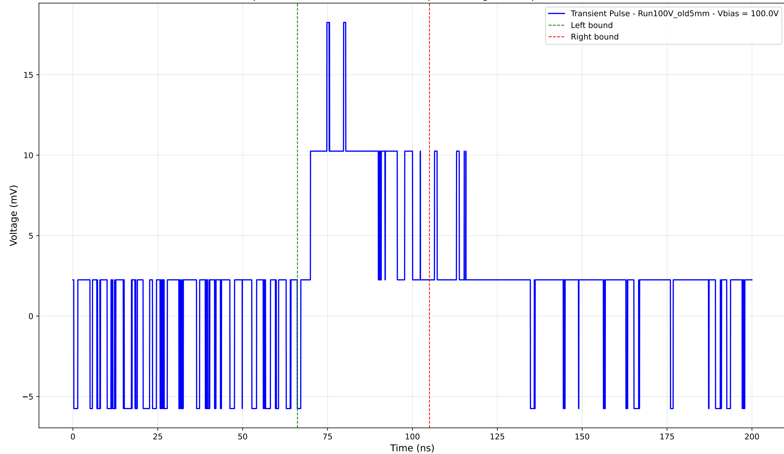
Transient Pulse - Sample: Old5mm - Position: 1375.0 \mu\text{m} - Charge: 6.17 pC - Rise Time: 0.00 ns (N/A)
