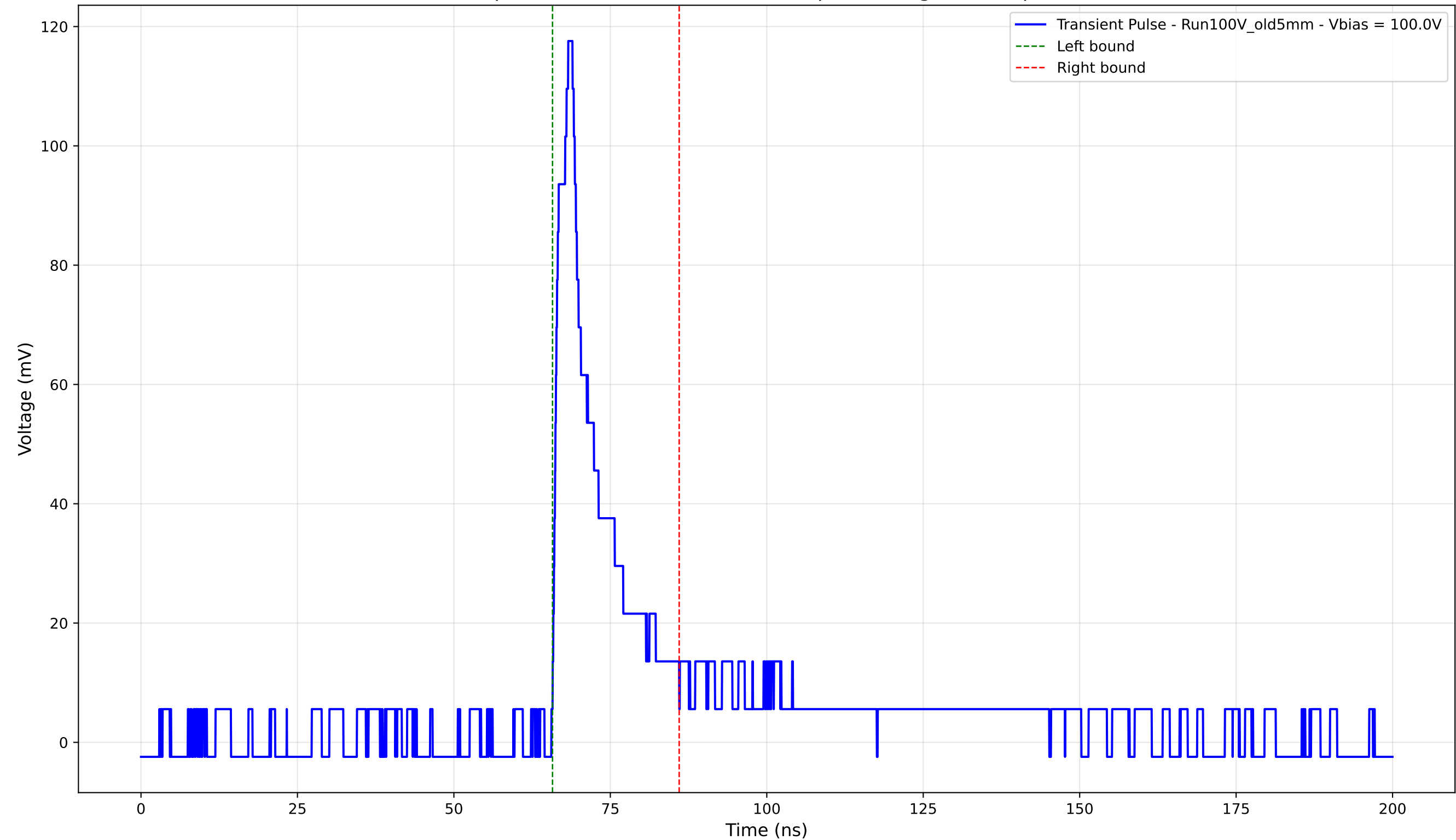
Transient Pulse - Sample: Old5mm - Position: 3260.0 \mu\text{m} - Charge: 16.92 pC - Rise Time: 2.22 ns
