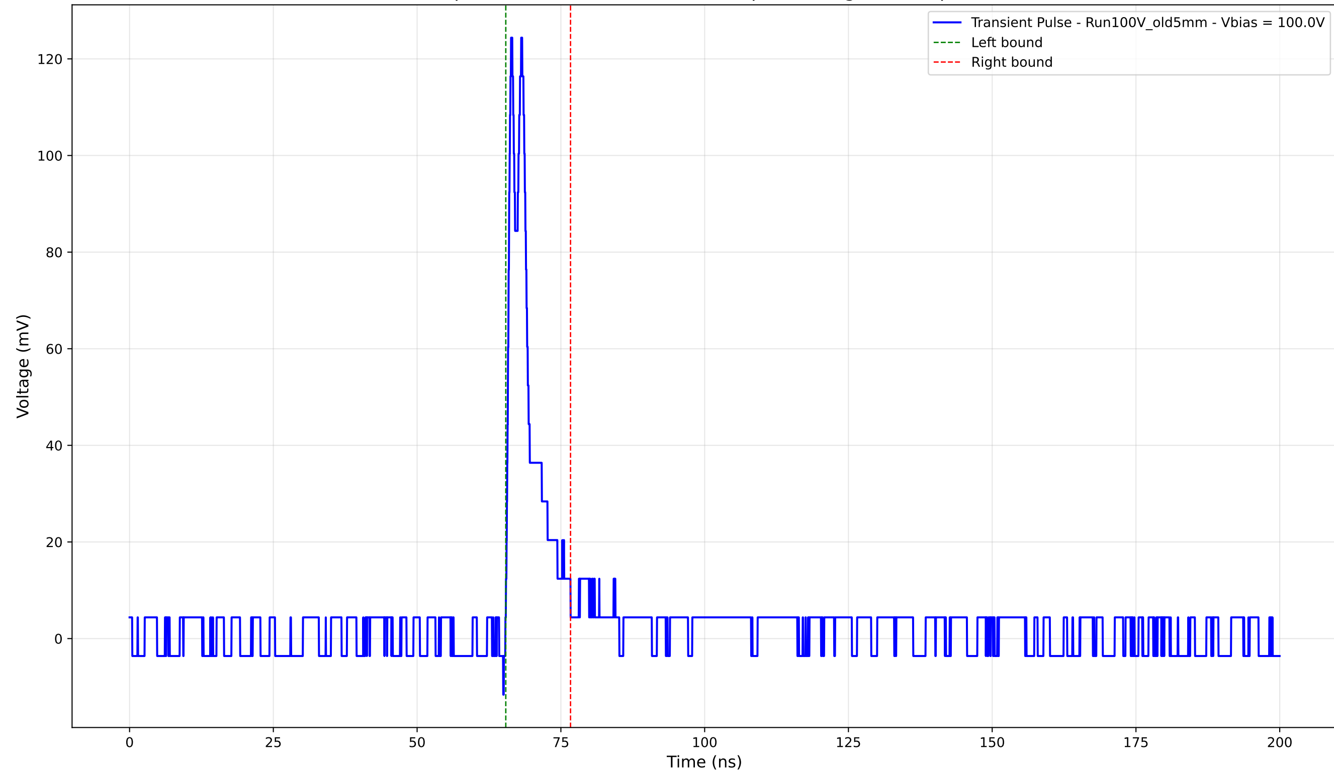
Transient Pulse - Sample: Old5mm - Position: 3780.0 \mu\text{m} - Charge: 10.72 pC - Rise Time: 0.70 ns
