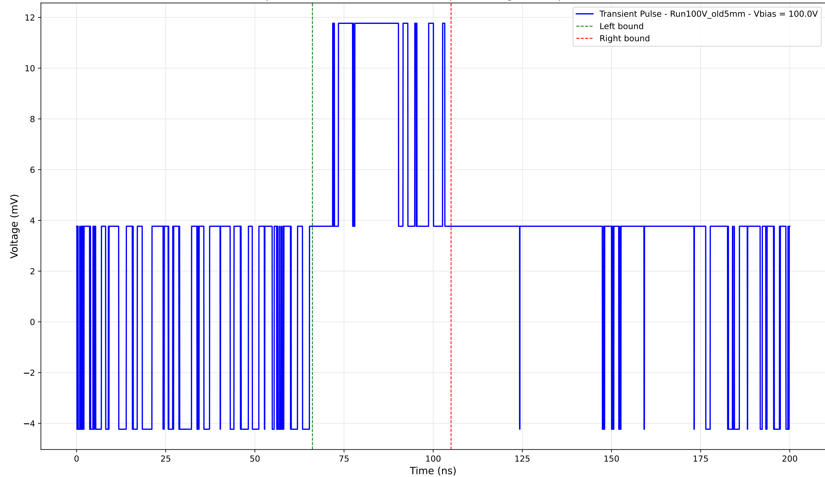
Transient Pulse - Sample: Old5mm - Position: 1090.0 \mu\text{m} - Charge: 6.22 pC - Rise Time: 0.00 ns (N/A)
