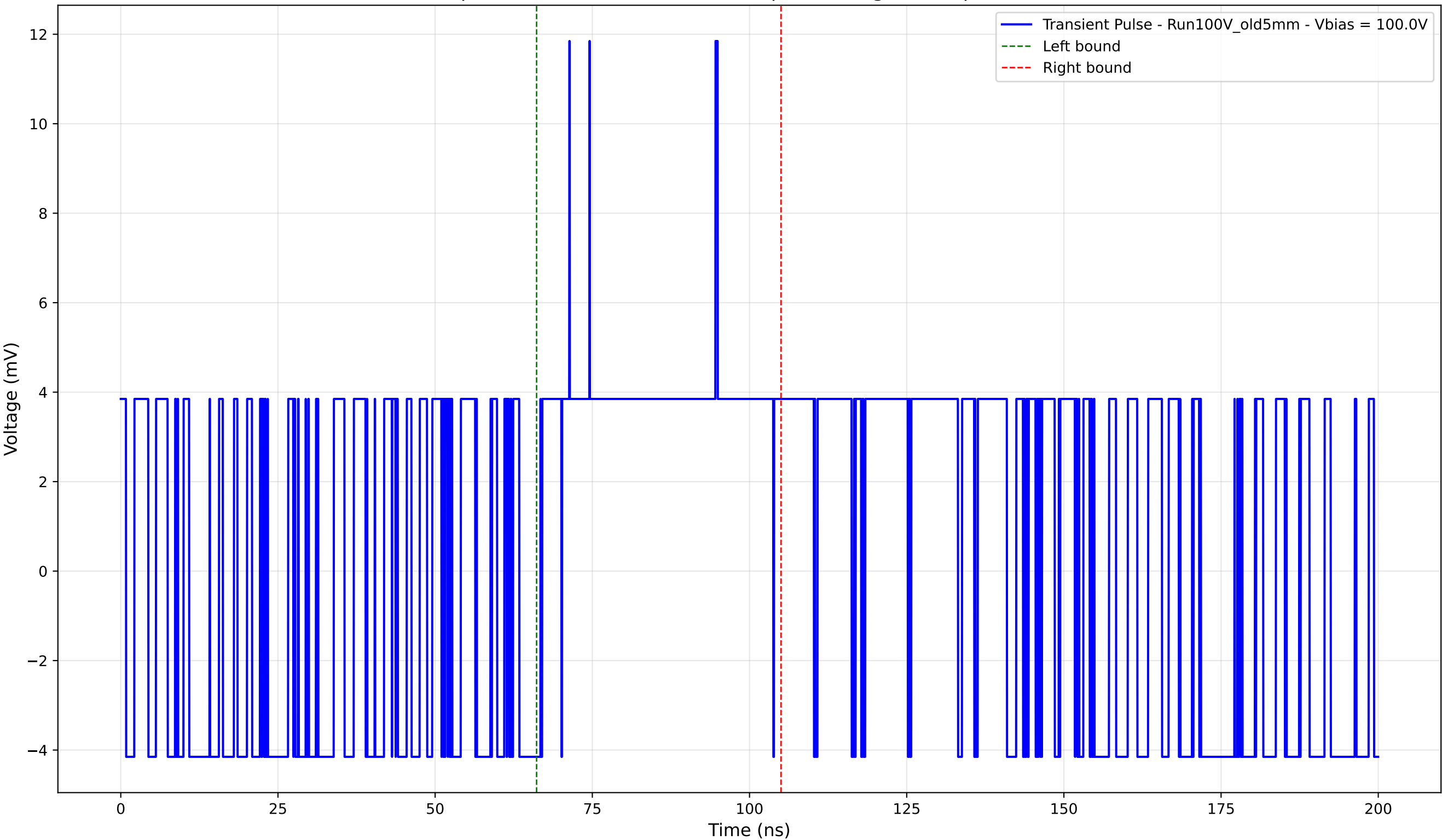
Transient Pulse - Sample: Old5mm - Position: 735.0 \mu\text{m} - Charge: 2.90 pC - Rise Time: 0.00 ns (N/A)
