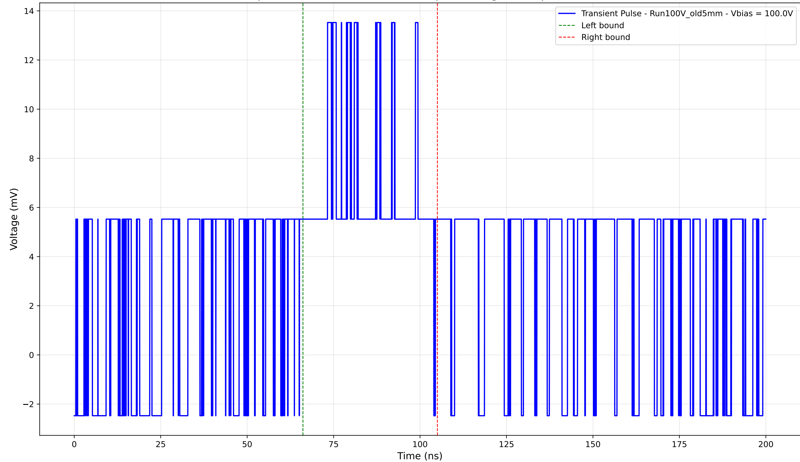
Transient Pulse - Sample: Old5mm - Position: 1130.0 \mu\text{m} - Charge: 5.39 pC - Rise Time: 0.00 ns (N/A)
