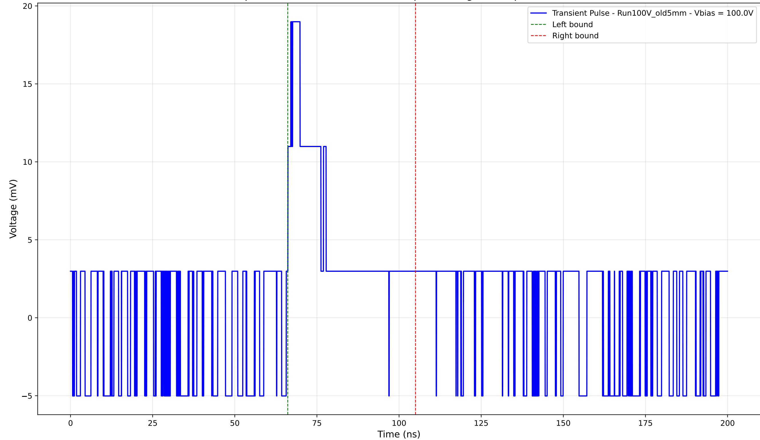
Transient Pulse - Sample: Old5mm - Position: 3050.0 \mu\text{m} - Charge: 4.44 pC - Rise Time: 0.00 ns (N/A)
