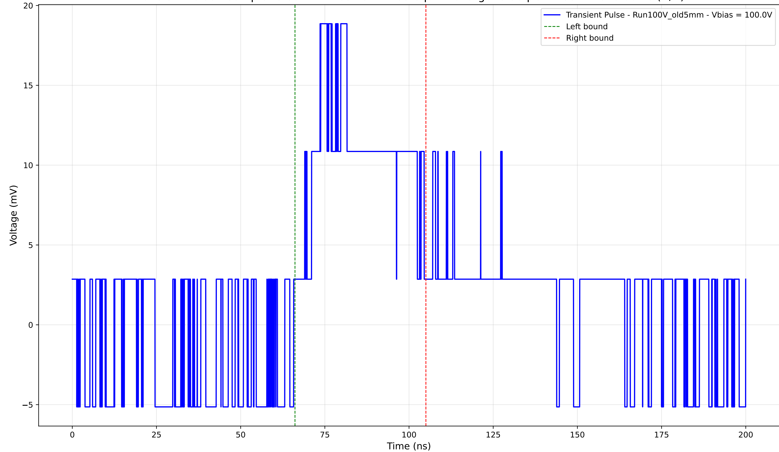
Transient Pulse - Sample: Old5mm - Position: 1405.0 \mu\text{m} - Charge: 8.36 pC - Rise Time: 0.00 ns (N/A)
