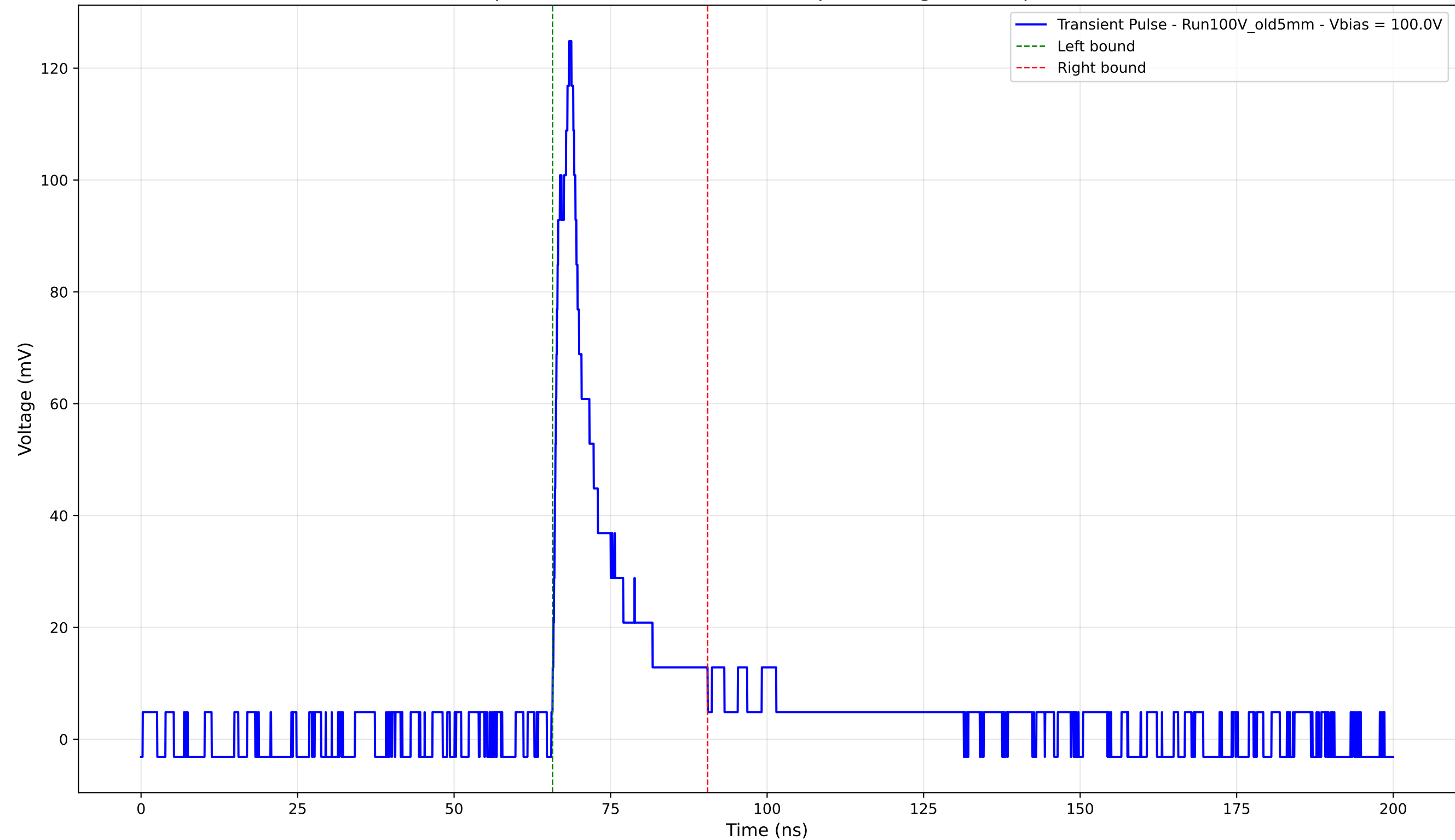
Transient Pulse - Sample: Old5mm - Position: 3275.0 \mu\text{m} - Charge: 18.03 pC - Rise Time: 2.36 ns
