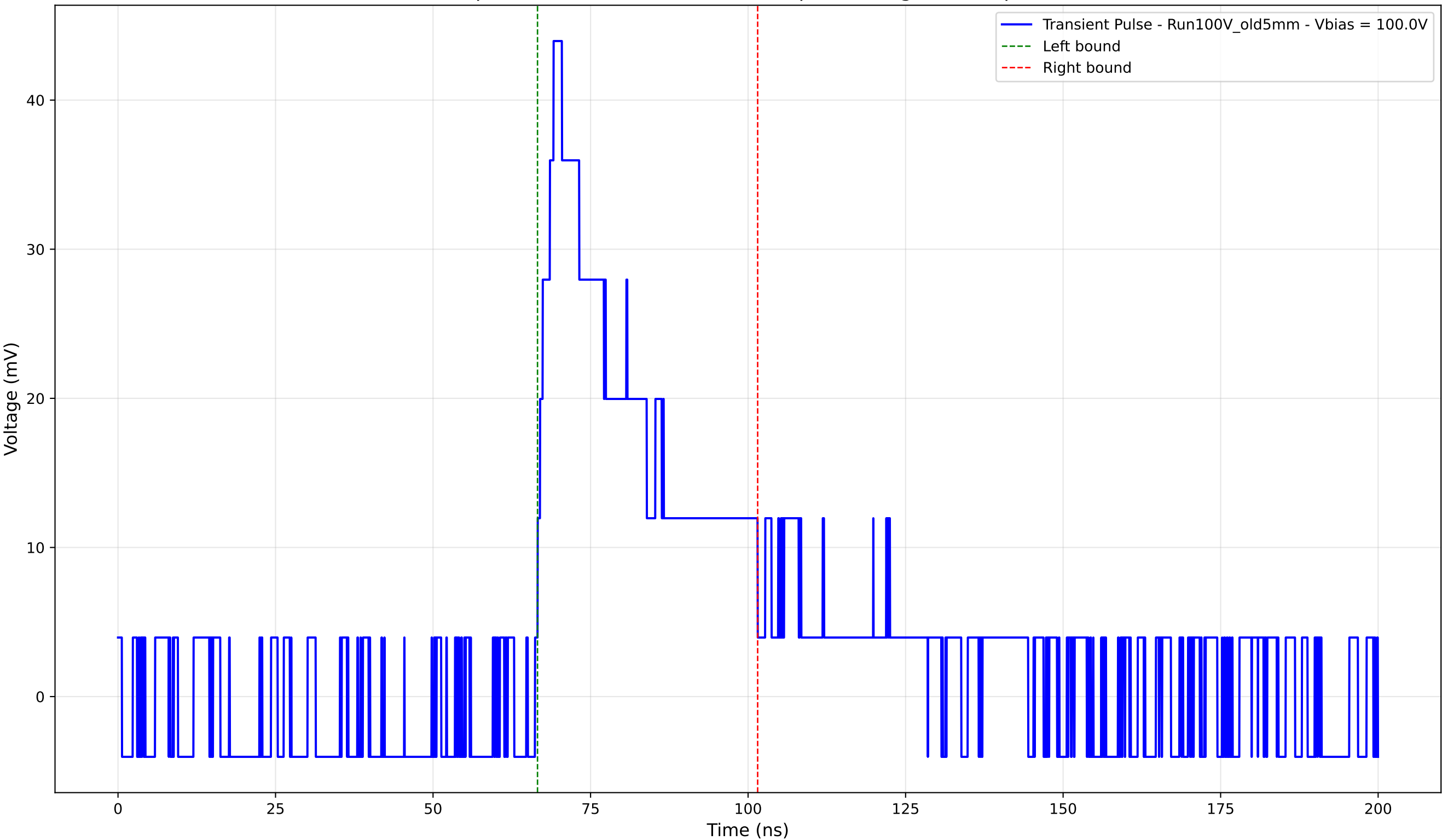
Transient Pulse - Sample: Old5mm - Position: 2680.0 \mu\text{m} - Charge: 13.82 pC - Rise Time: 2.54 ns
