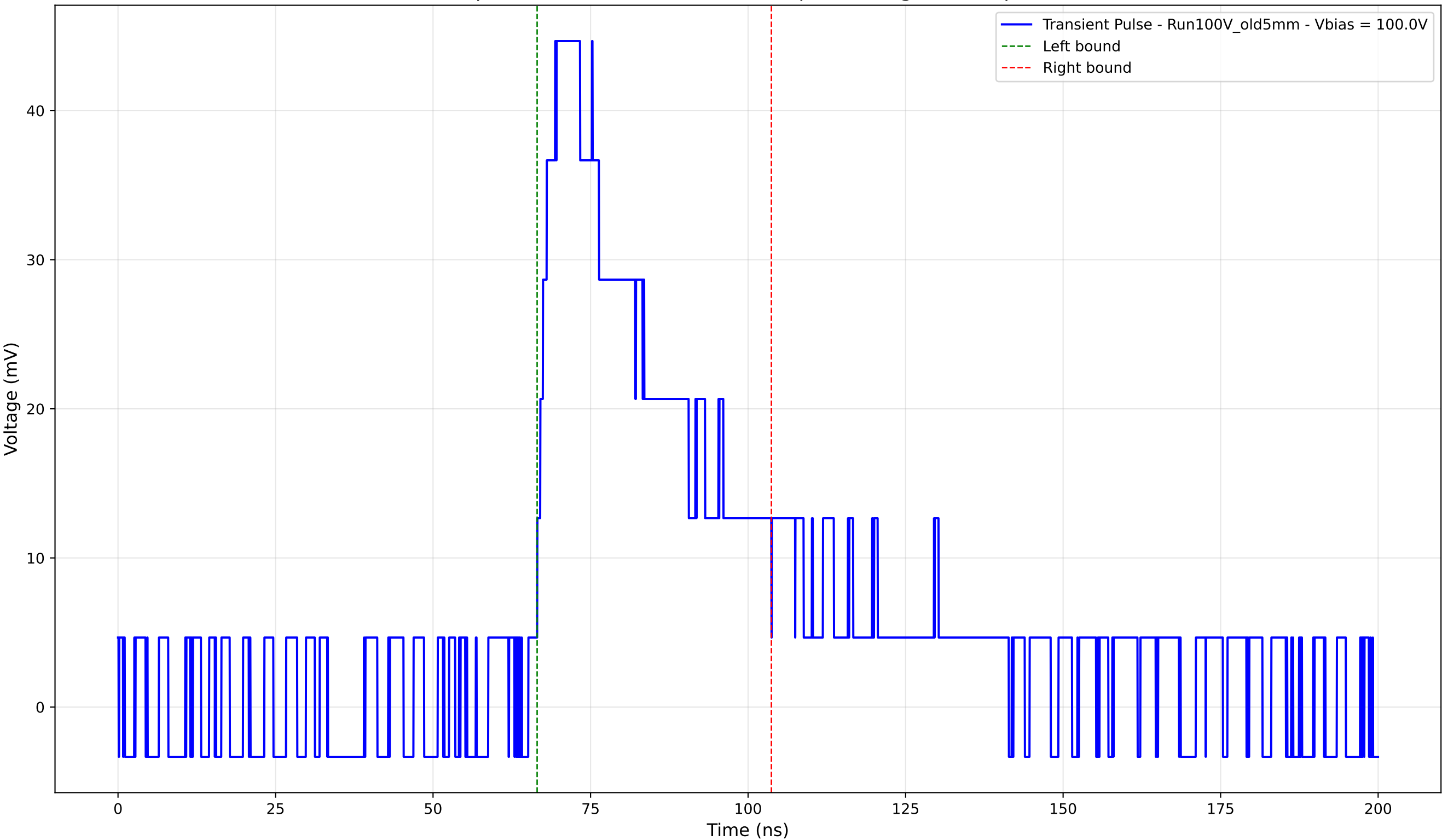
Transient Pulse - Sample: Old5mm - Position: 4880.0 \mu\text{m} - Charge: 18.04 pC - Rise Time: 4.26 ns
