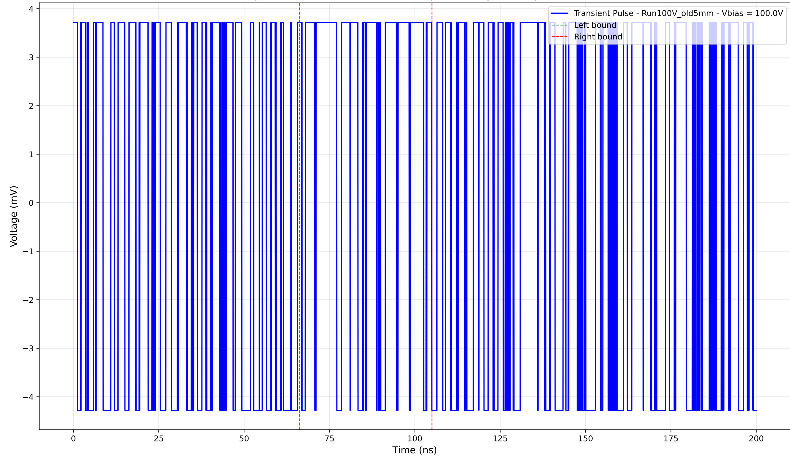
Transient Pulse - Sample: Old5mm - Position: 4610.0 \mu\text{m} - Charge: 1.71 pC - Rise Time: 0.00 ns (N/A)
