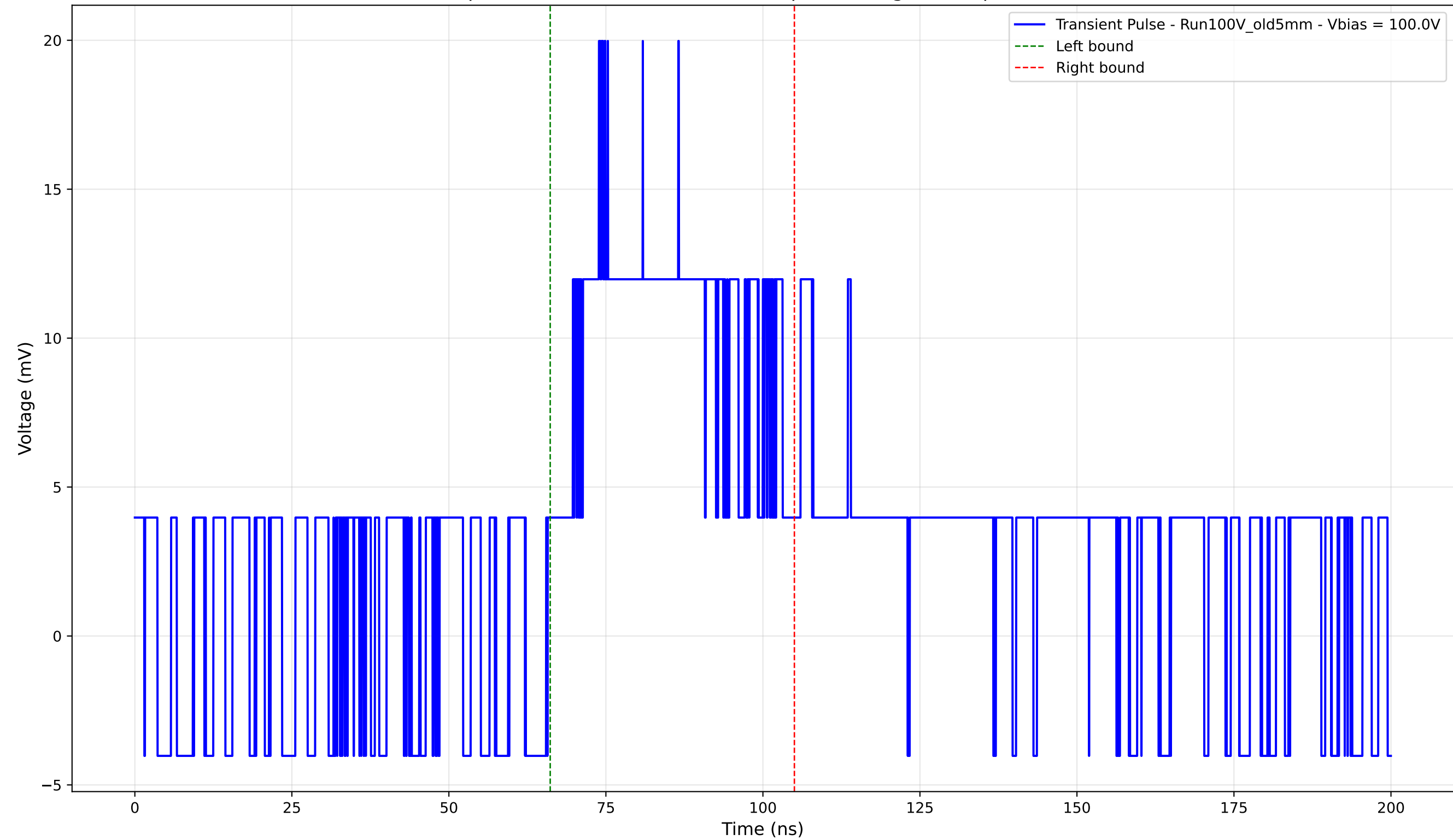
Transient Pulse - Sample: Old5mm - Position: 1850.0 \mu\text{m} - Charge: 7.85 pC - Rise Time: 0.00 ns (N/A)
