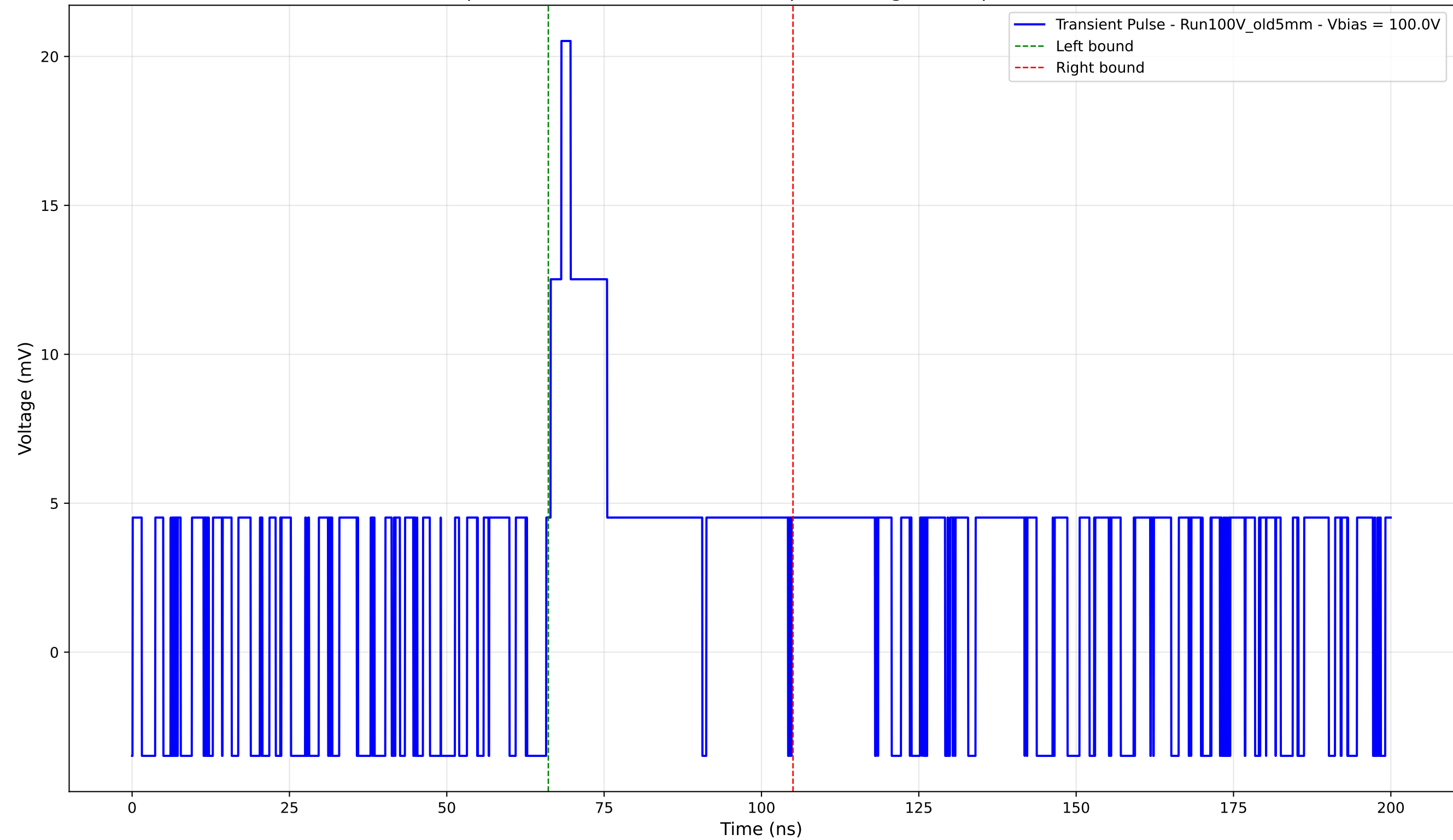
Transient Pulse - Sample: Old5mm - Position: 3055.0 \mu\text{m} - Charge: 5.05 pC - Rise Time: 0.00 ns (N/A)
