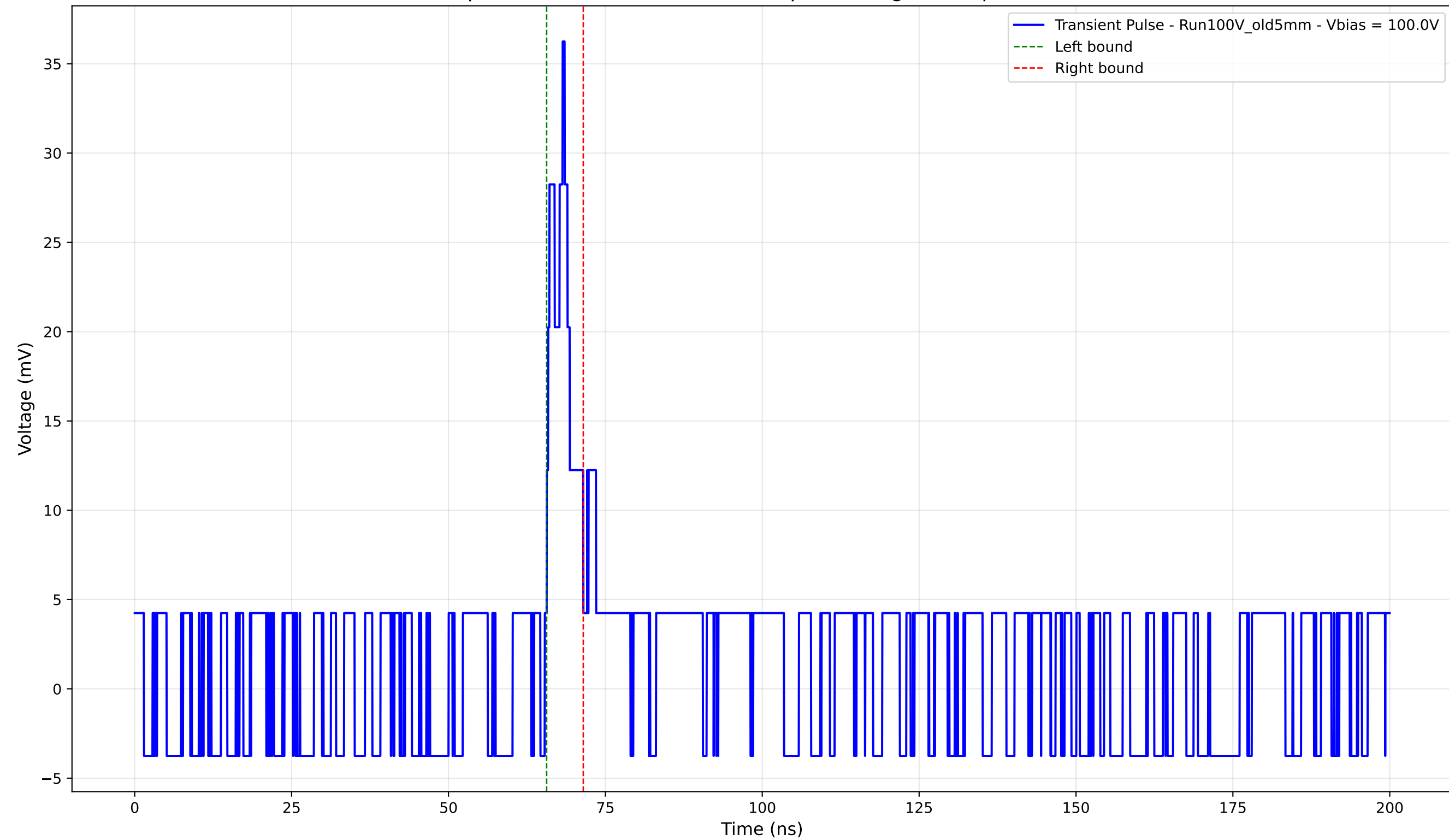
Transient Pulse - Sample: Old5mm - Position: 3745.0 \mu\text{m} - Charge: 2.37 pC - Rise Time: 0.00 ns (N/A)
