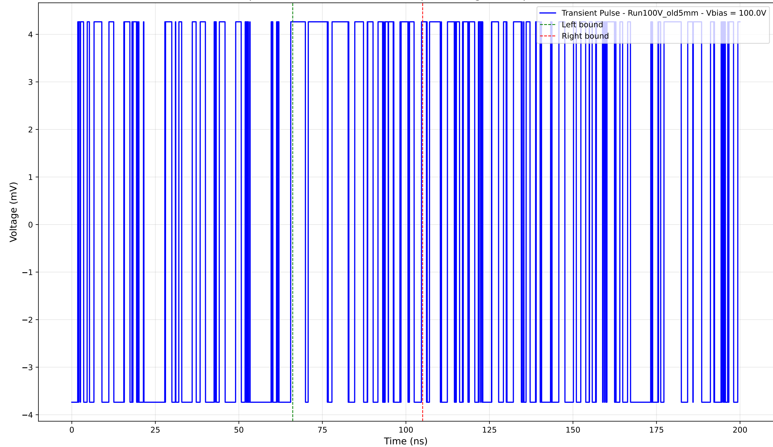
Transient Pulse - Sample: Old5mm - Position: 4290.0 \mu\text{m} - Charge: 1.43 pC - Rise Time: 0.00 ns (N/A)
