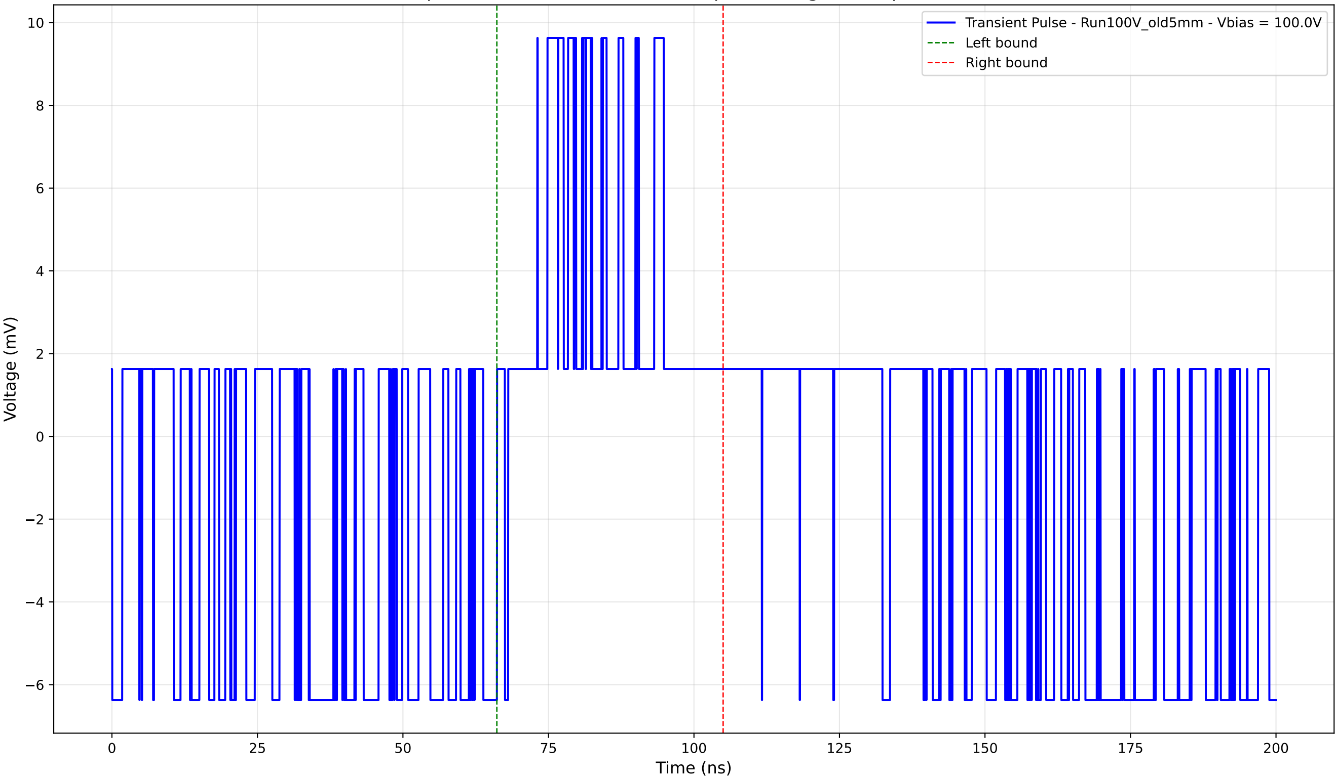
Transient Pulse - Sample: Old5mm - Position: 940.0 \mu\text{m} - Charge: 2.67 pC - Rise Time: 0.00 ns (N/A)
