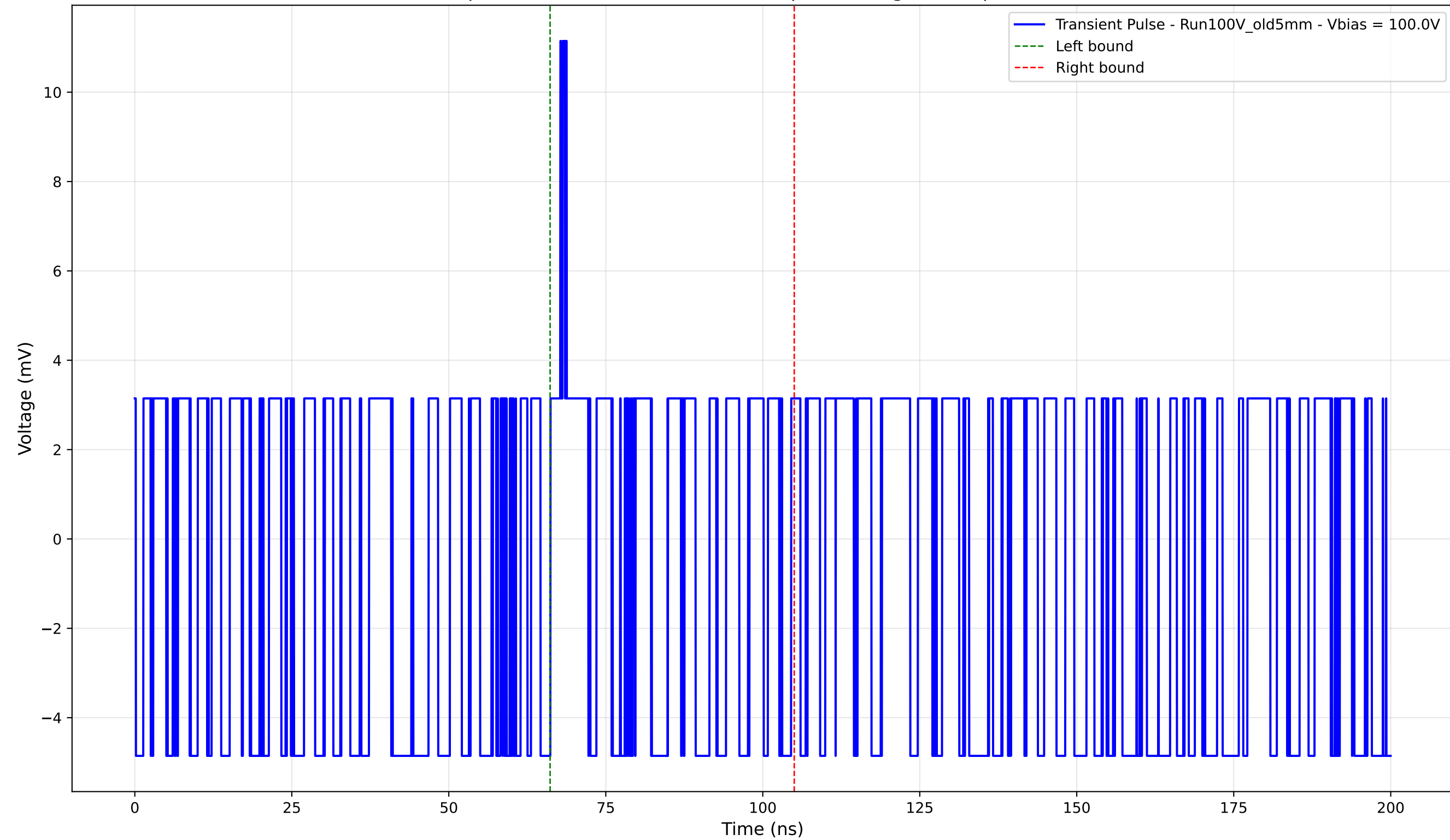
Transient Pulse - Sample: Old5mm - Position: 3395.0 \mu\text{m} - Charge: 0.25 pC - Rise Time: 0.00 ns (N/A)
