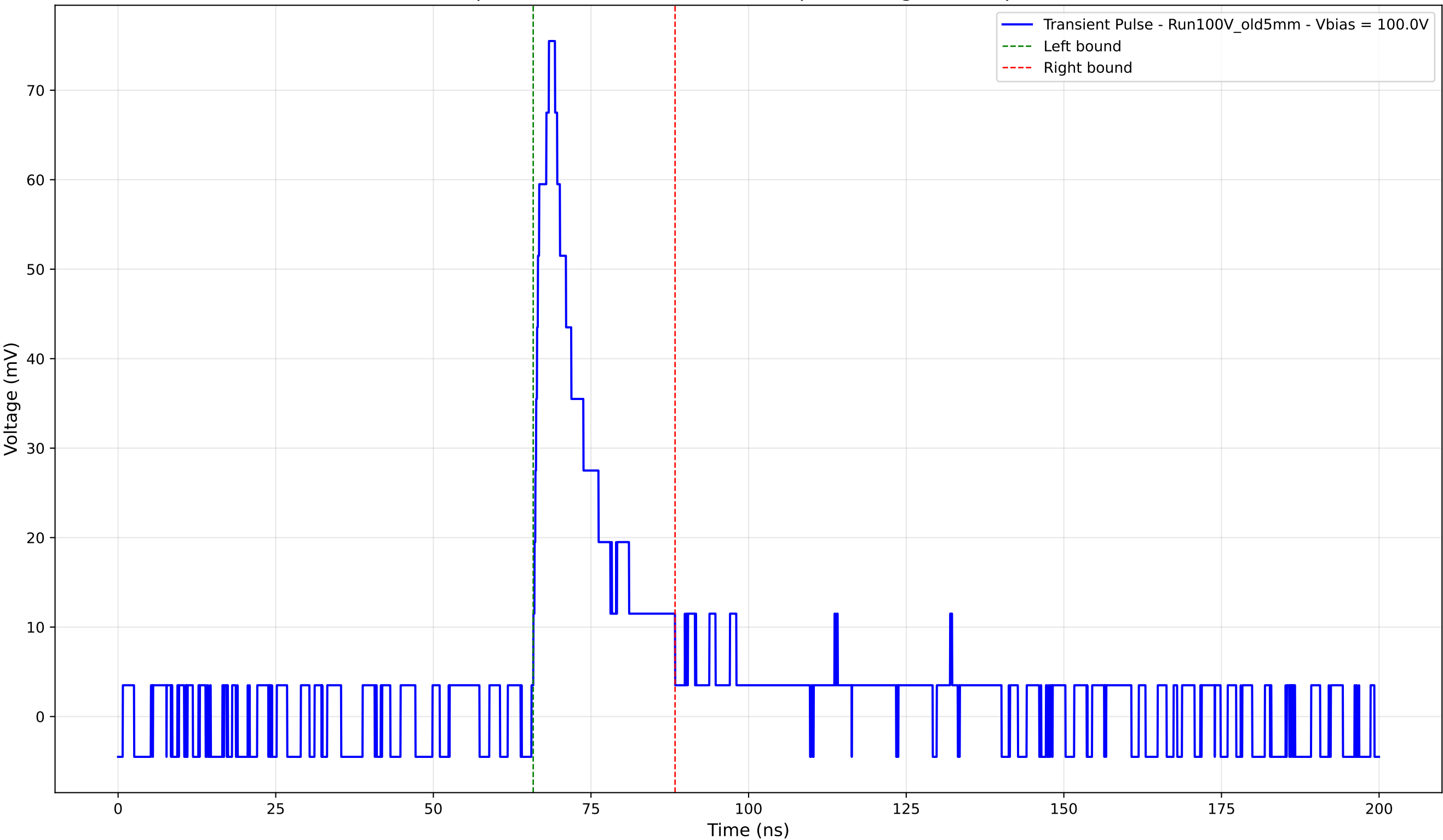
Transient Pulse - Sample: Old5mm - Position: 3190.0 \mu\text{m} - Charge: 12.76 pC - Rise Time: 2.47 ns
