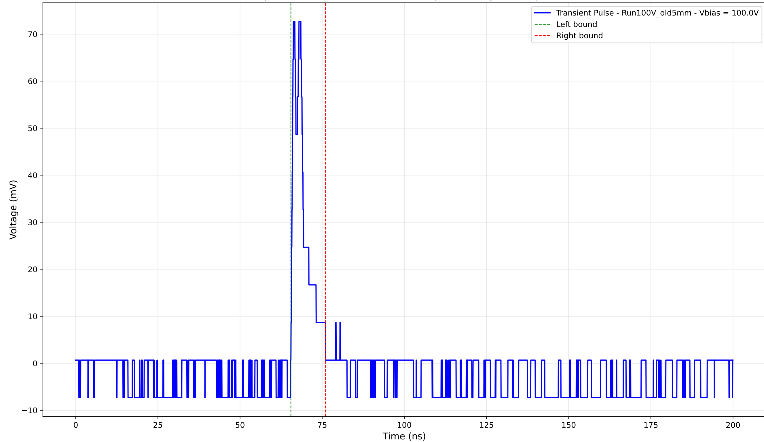
Transient Pulse - Sample: Old5mm - Position: 3765.0 \mu\text{m} - Charge: 6.28 pC - Rise Time: 0.70 ns
