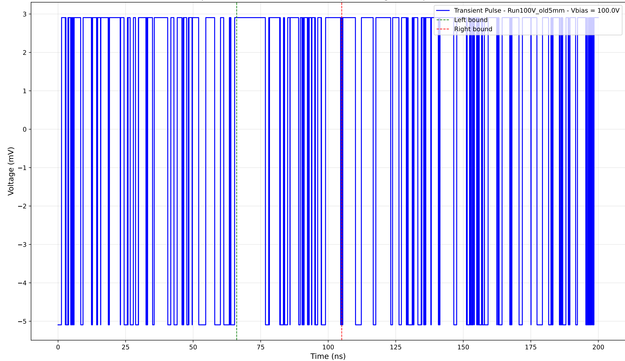
Transient Pulse - Sample: Old5mm - Position: 4305.0 \mu\text{m} - Charge: 0.90 pC - Rise Time: 0.00 ns (N/A)
