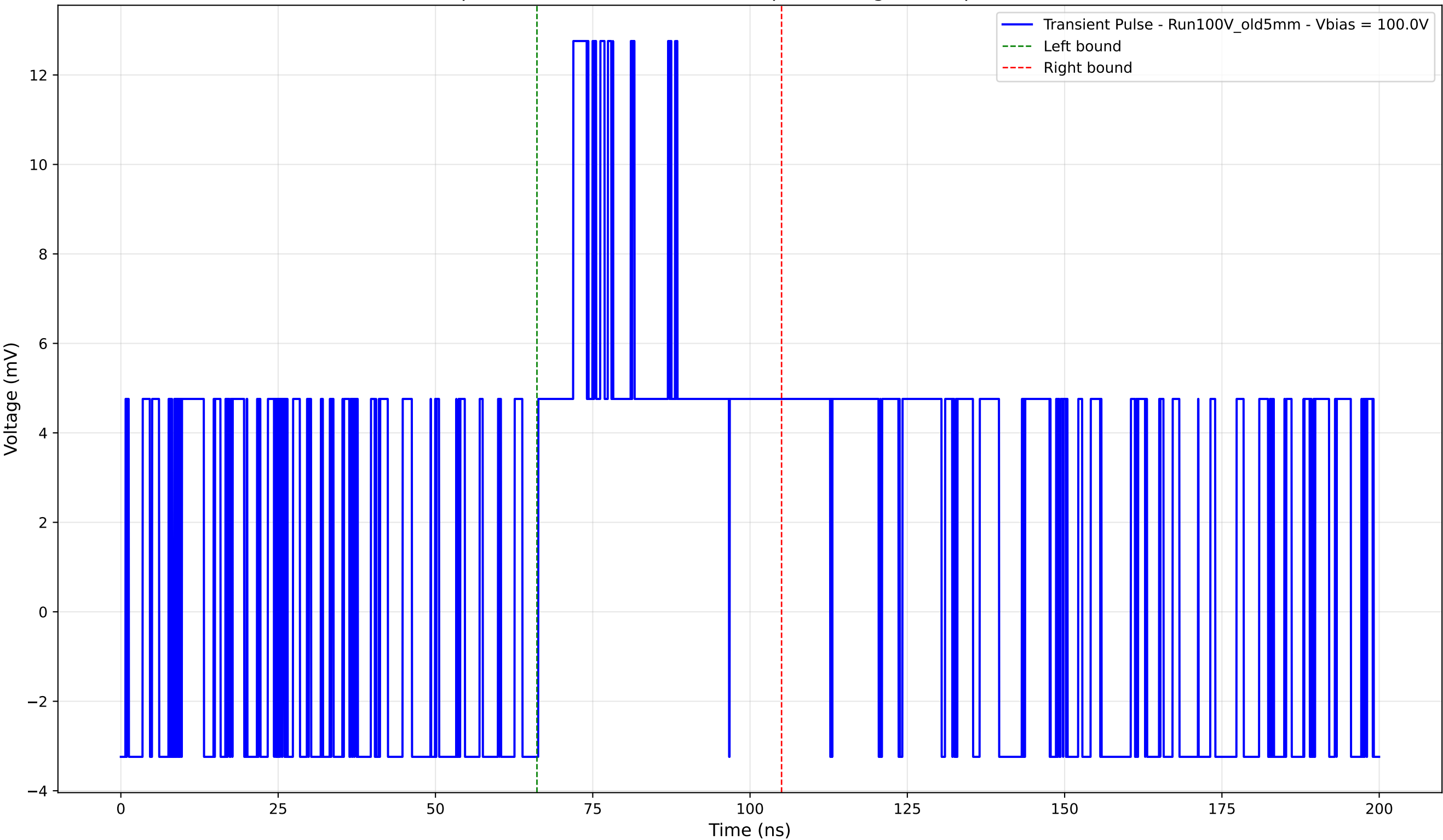
Transient Pulse - Sample: Old5mm - Position: 490.0 \mu\text{m} - Charge: 4.46 pC - Rise Time: 0.00 ns (N/A)
