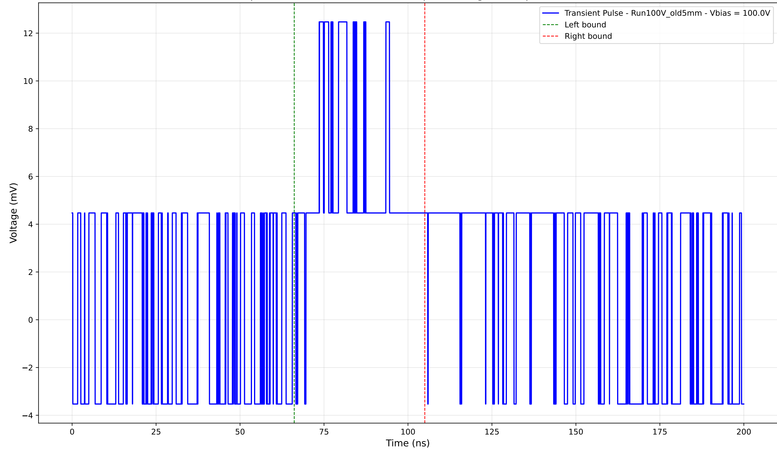
Transient Pulse - Sample: Old5mm - Position: 1135.0 \mu\text{m} - Charge: 4.57 pC - Rise Time: 0.00 ns (N/A)
