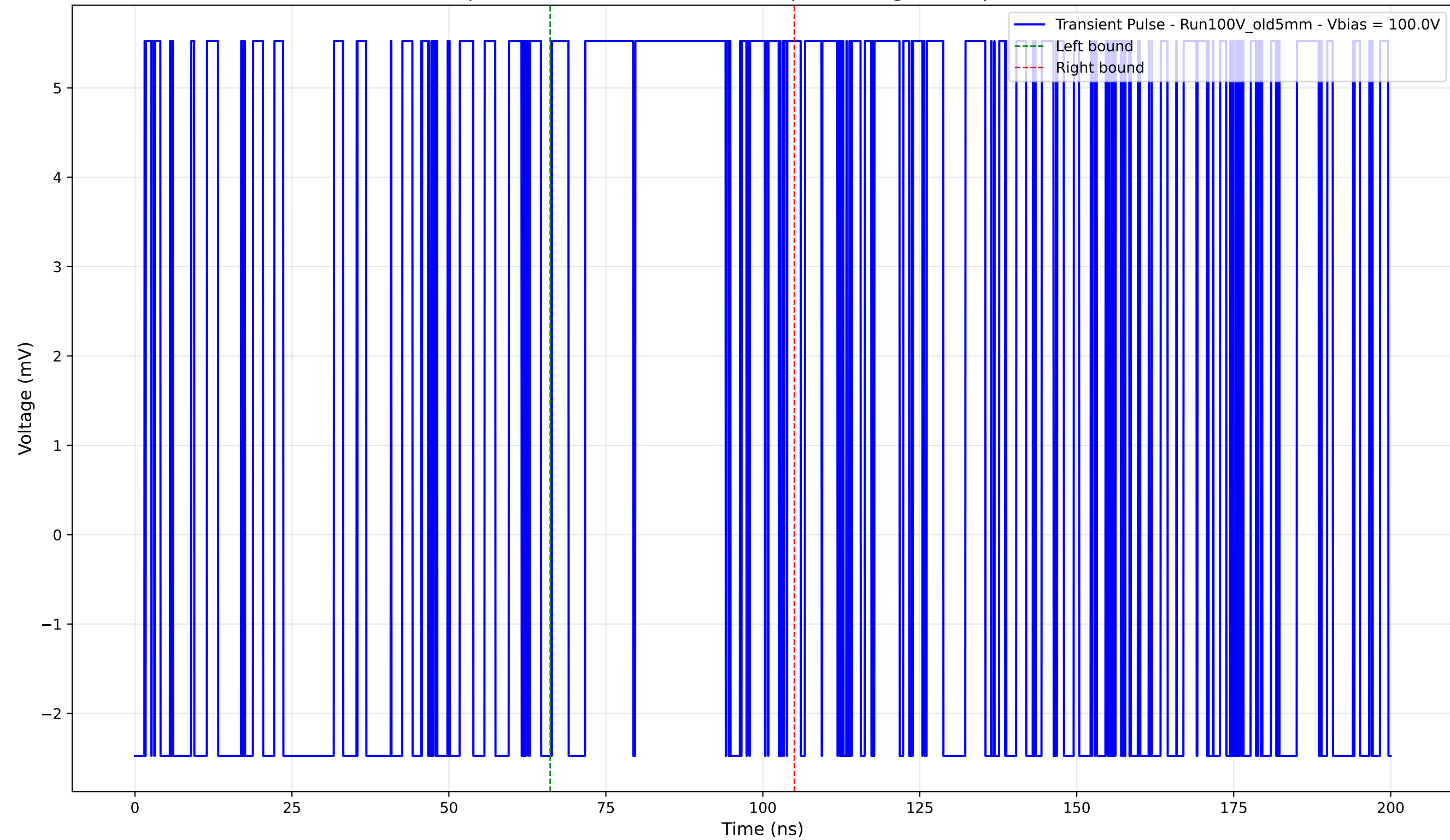
Transient Pulse - Sample: Old5mm - Position: 1495.0 \mu\text{m} - Charge: 3.34 pC - Rise Time: 0.00 ns (N/A)
