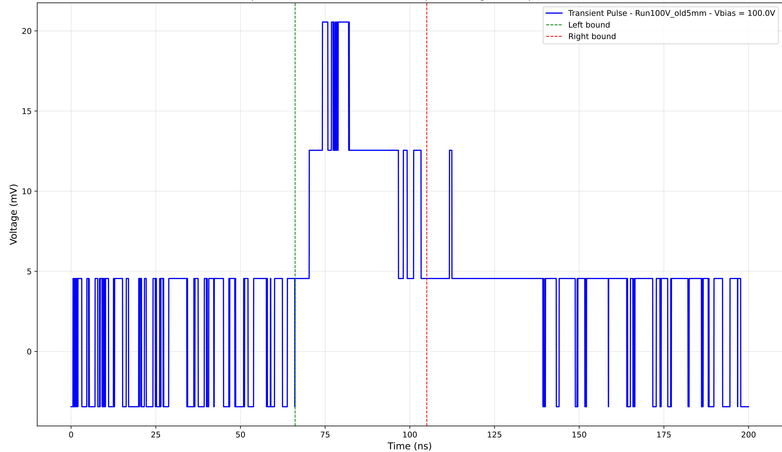
Transient Pulse - Sample: Old5mm - Position: 1190.0 \mu\text{m} - Charge: 9.24 pC - Rise Time: 0.00 ns (N/A)
