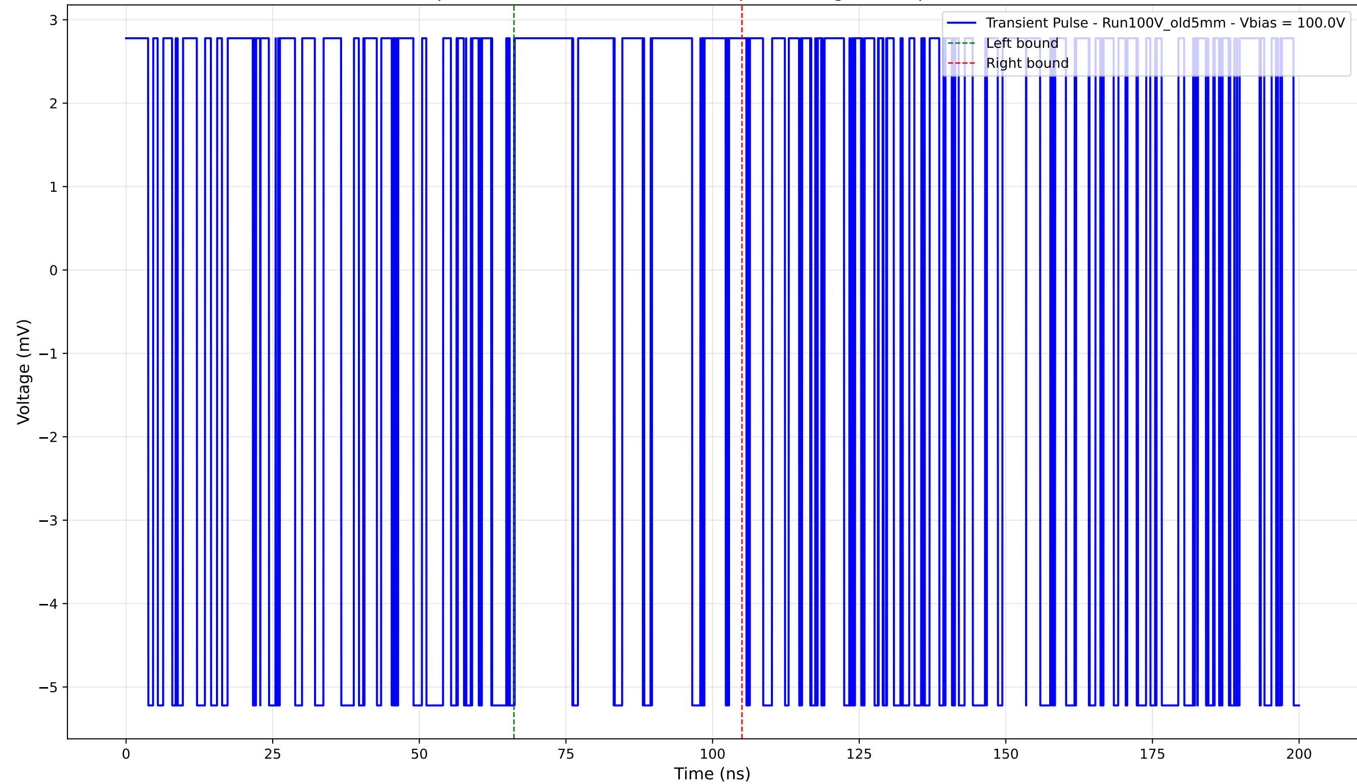
Transient Pulse - Sample: Old5mm - Position: 3120.0 \mu\text{m} - Charge: 1.24 pC - Rise Time: 0.00 ns (N/A)
