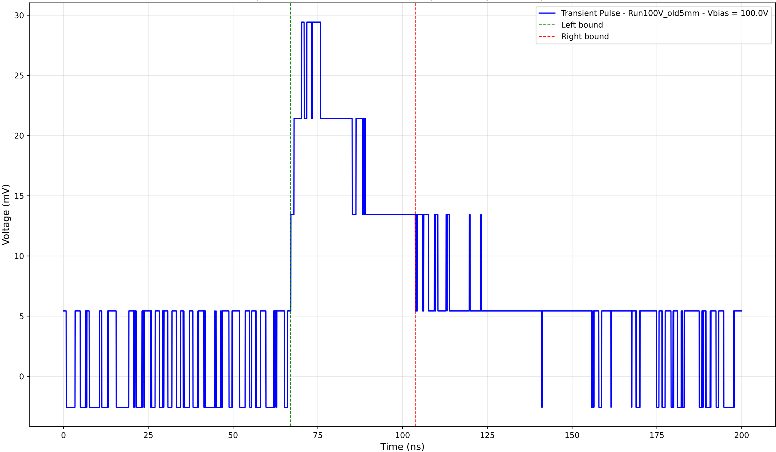
Transient Pulse - Sample: Old5mm - Position: 2440.0 \mu\text{m} - Charge: 13.73 pC - Rise Time: 4.18 ns
