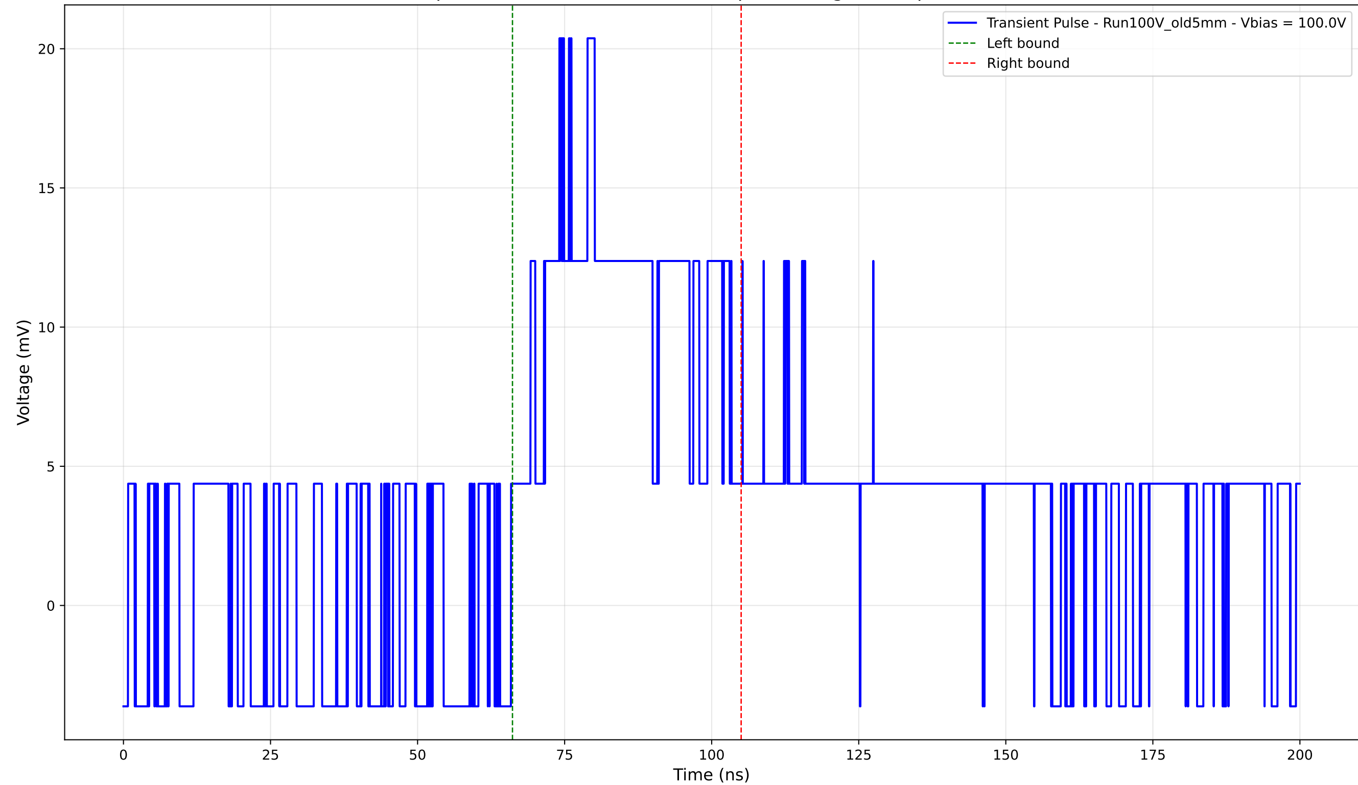
Transient Pulse - Sample: Old5mm - Position: 1575.0 \mu\text{m} - Charge: 8.41 pC - Rise Time: 0.00 ns (N/A)
