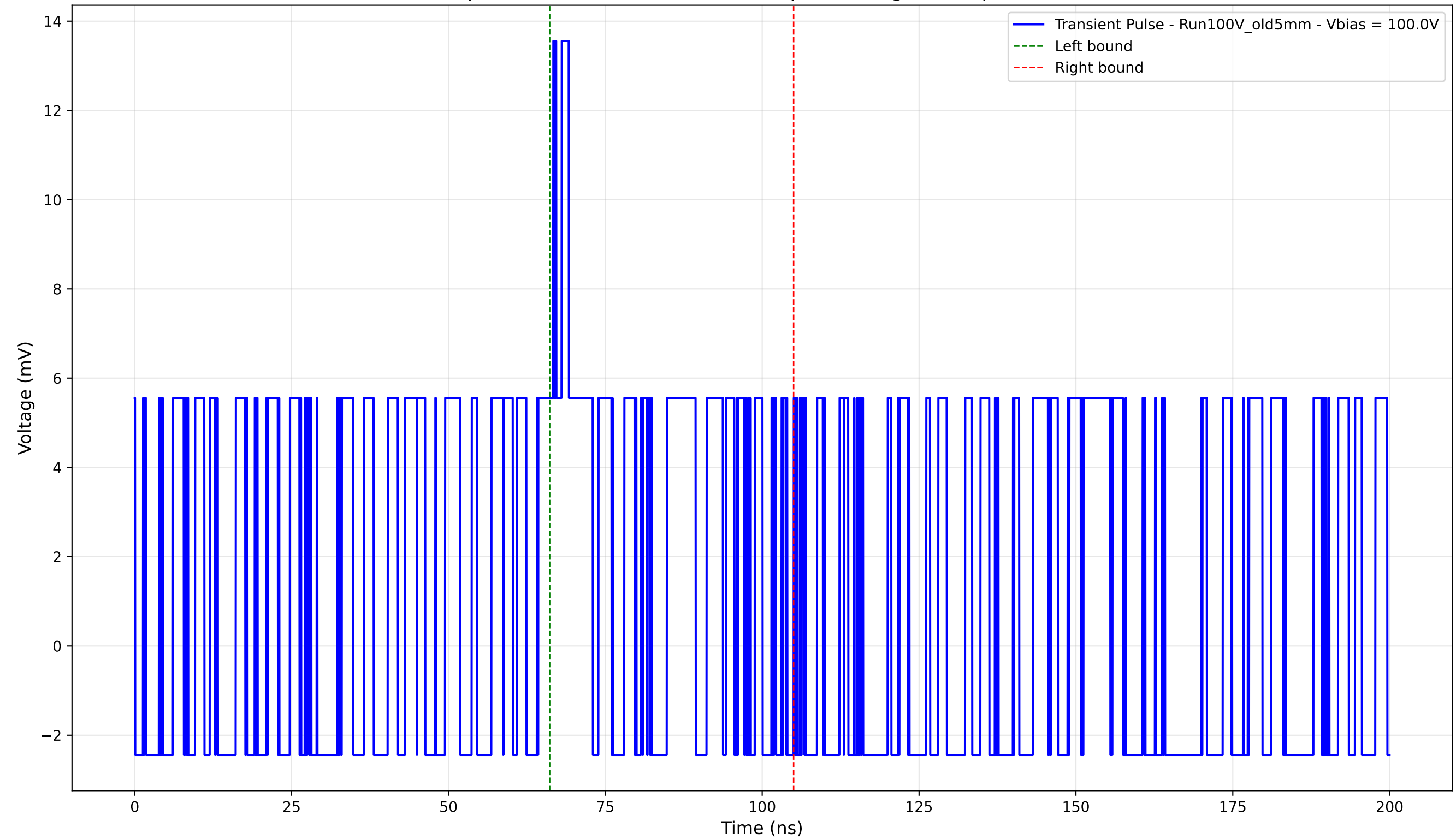
Transient Pulse - Sample: Old5mm - Position: 3710.0 \mu\text{m} - Charge: 2.27 pC - Rise Time: 0.00 ns (N/A)
