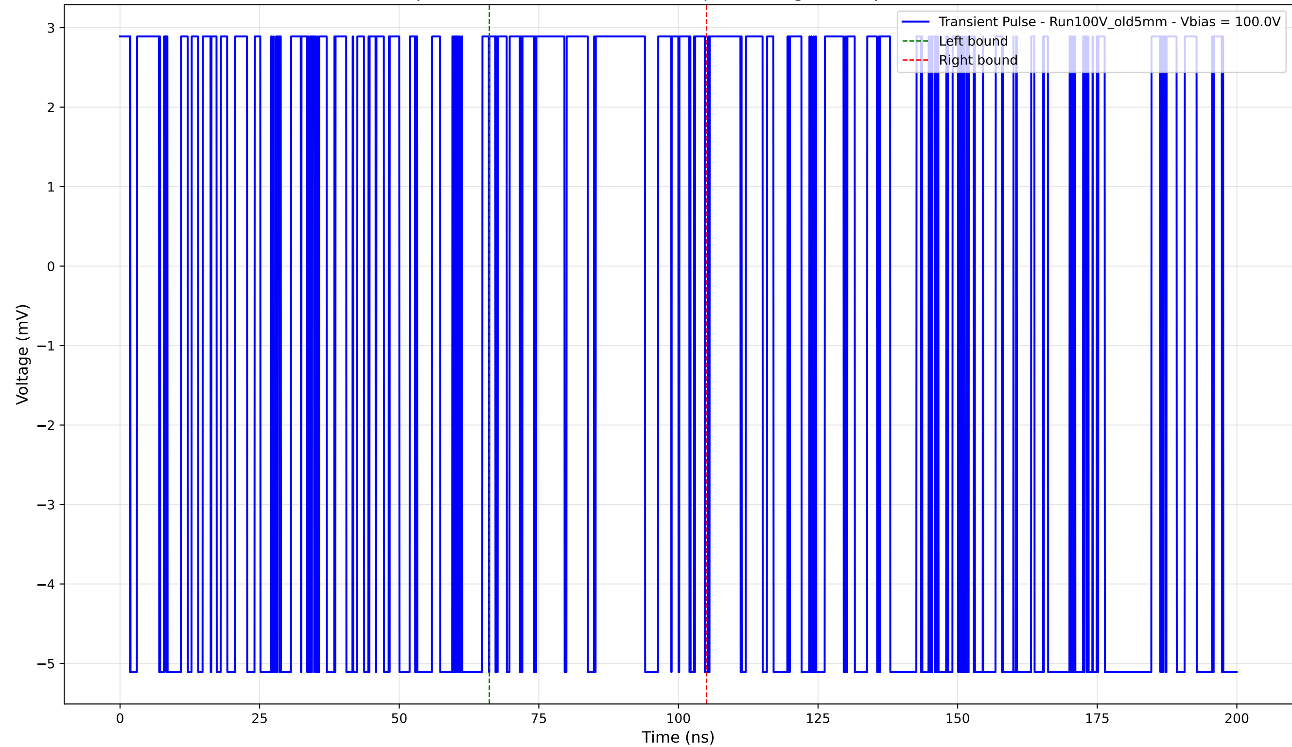
Transient Pulse - Sample: Old5mm - Position: 2800.0 \mu\text{m} - Charge: 1.22 pC - Rise Time: 0.00 ns (N/A)
