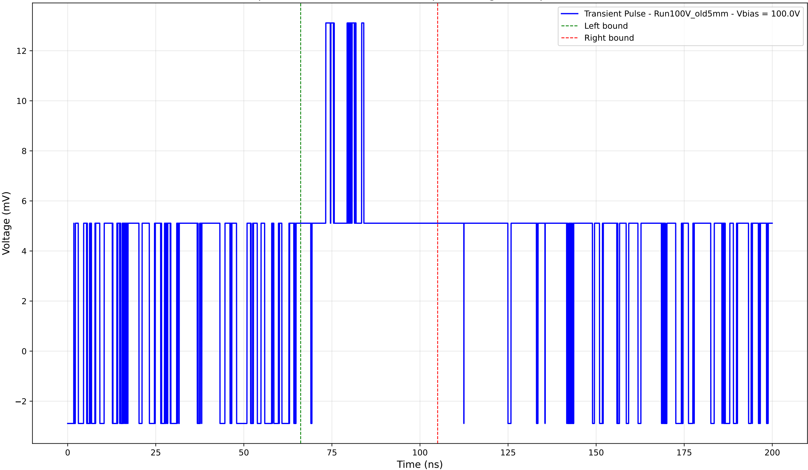
Transient Pulse - Sample: Old5mm - Position: 515.0 \mu\text{m} - Charge: 4.67 pC - Rise Time: 0.00 ns (N/A)
