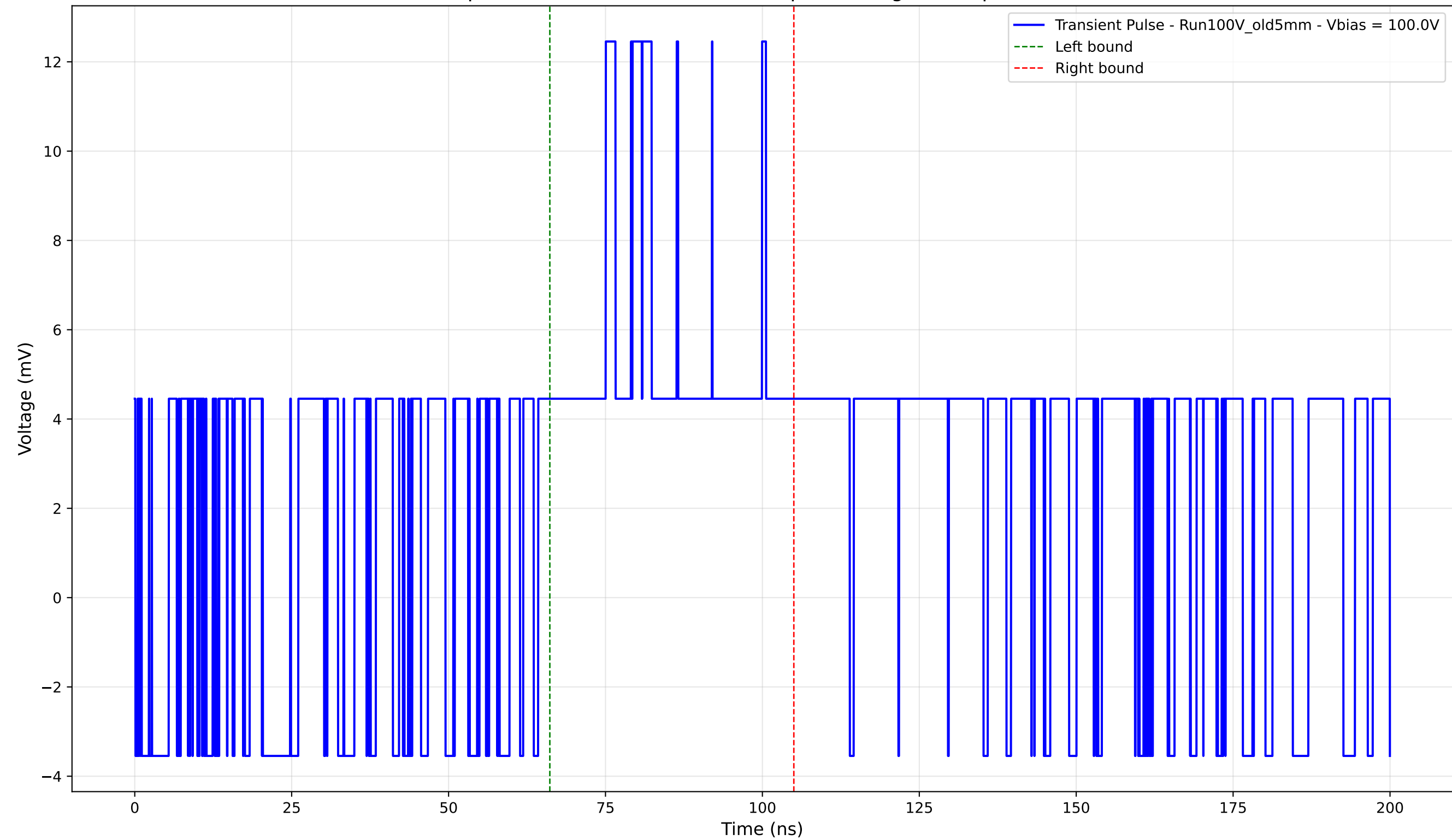
Transient Pulse - Sample: Old5mm - Position: 1350.0 \mu\text{m} - Charge: 4.36 pC - Rise Time: 0.00 ns (N/A)
