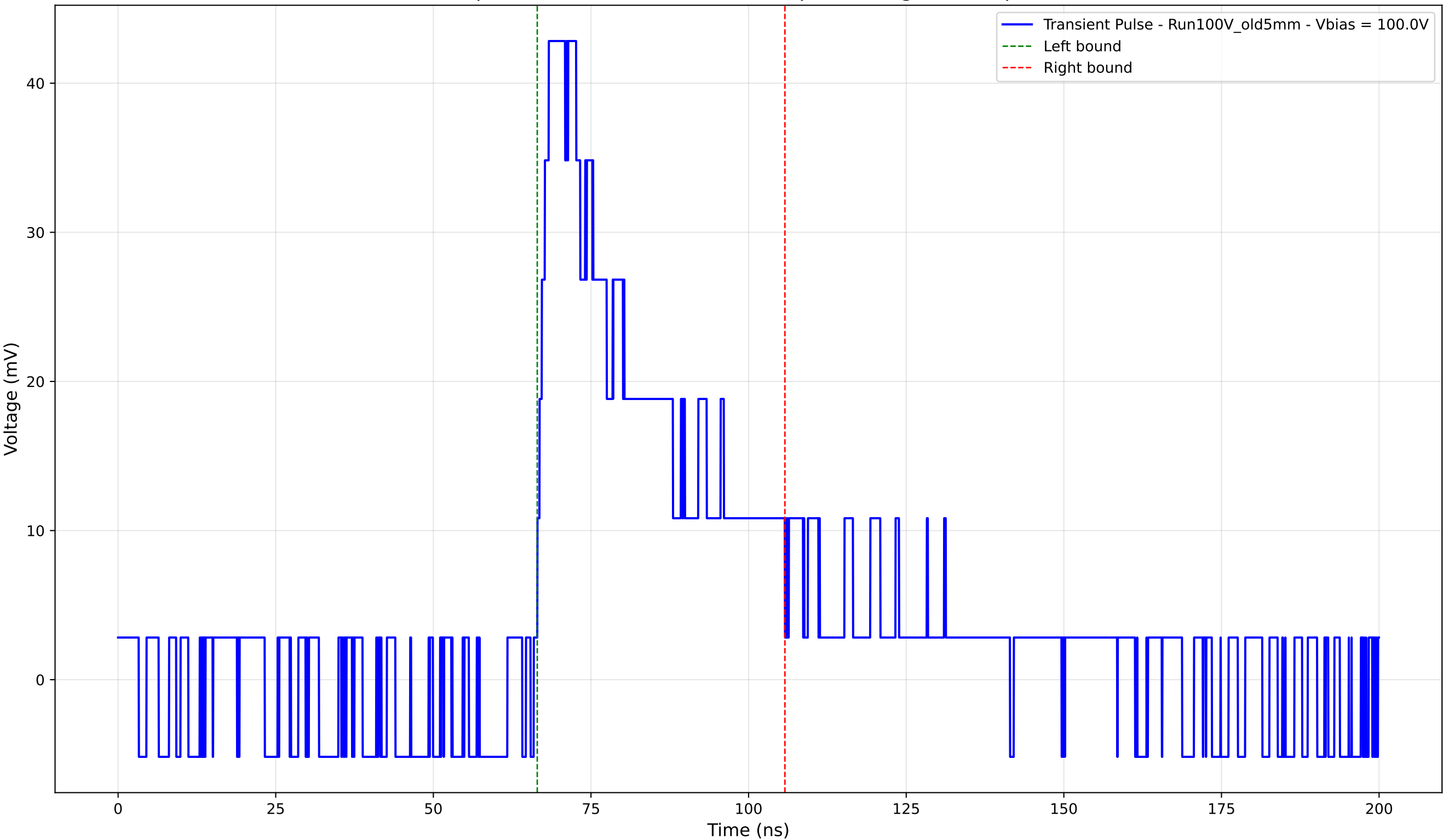
Transient Pulse - Sample: Old5mm - Position: 4745.0 \mu\text{m} - Charge: 15.90 pC - Rise Time: 1.82 ns
