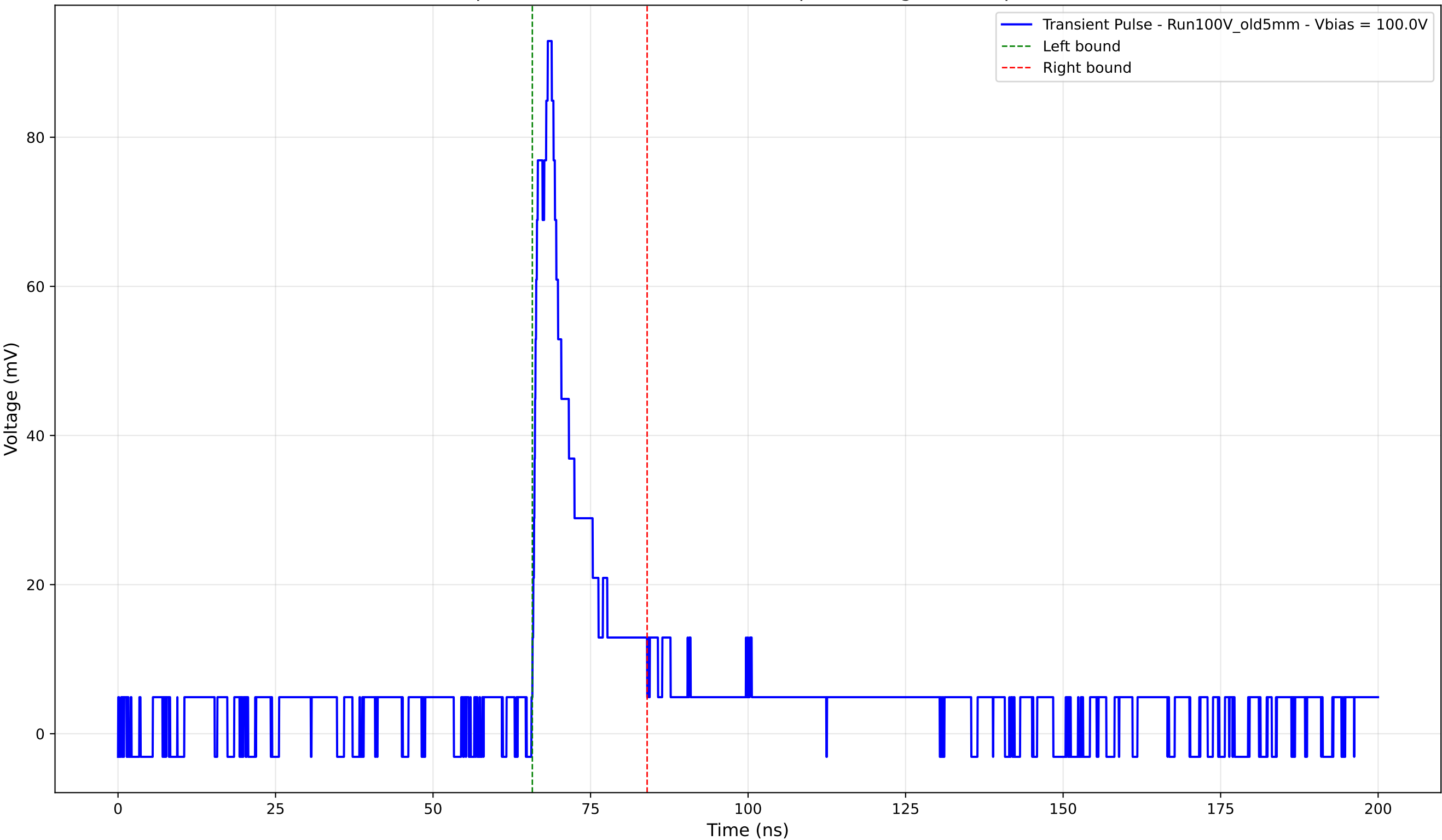
Transient Pulse - Sample: Old5mm - Position: 4095.0 \mu\text{m} - Charge: 12.22 pC - Rise Time: 2.19 ns
