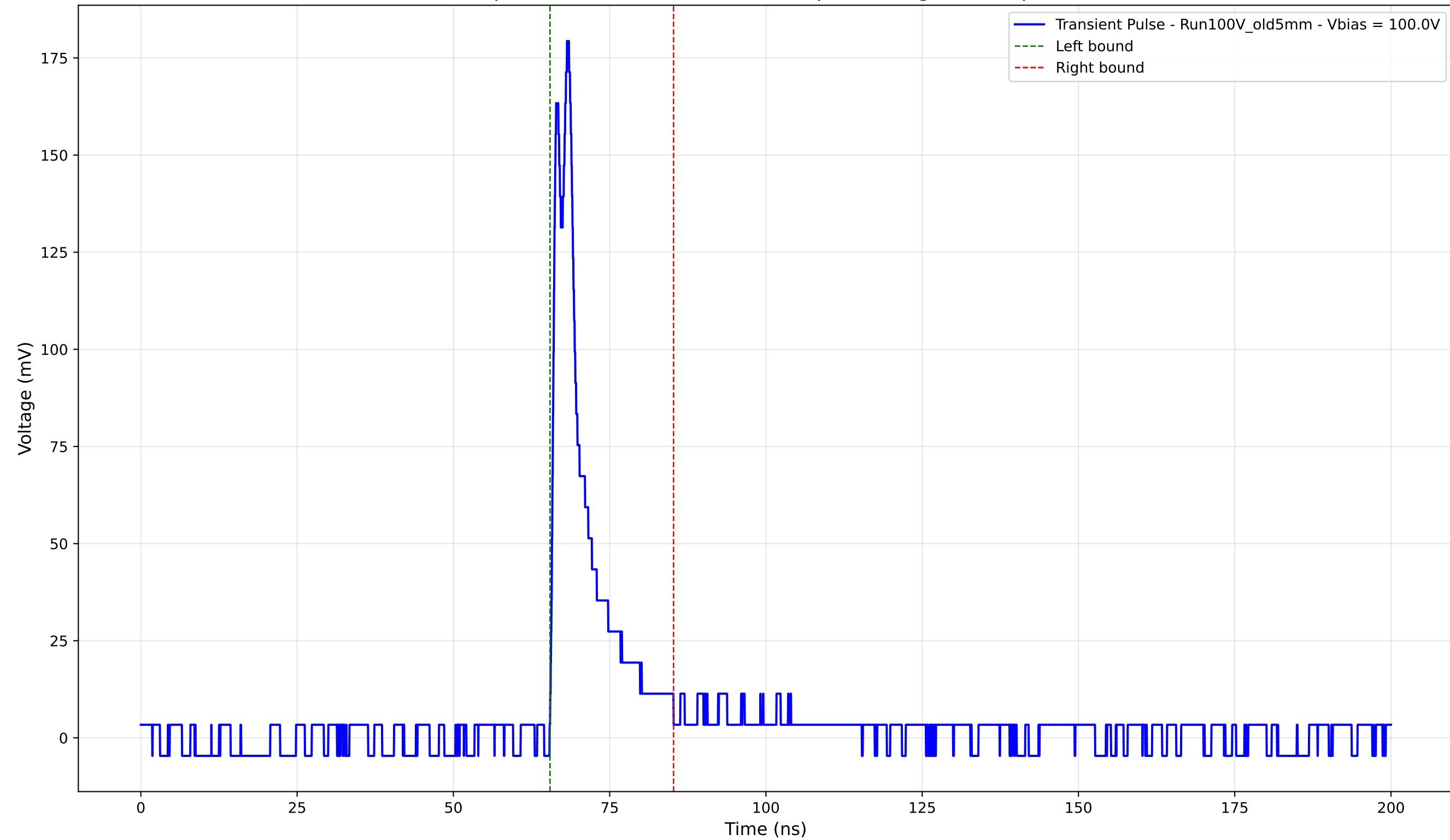
Transient Pulse - Sample: Old5mm - Position: 3885.0 \mu\text{m} - Charge: 19.80 pC - Rise Time: 0.86 ns
