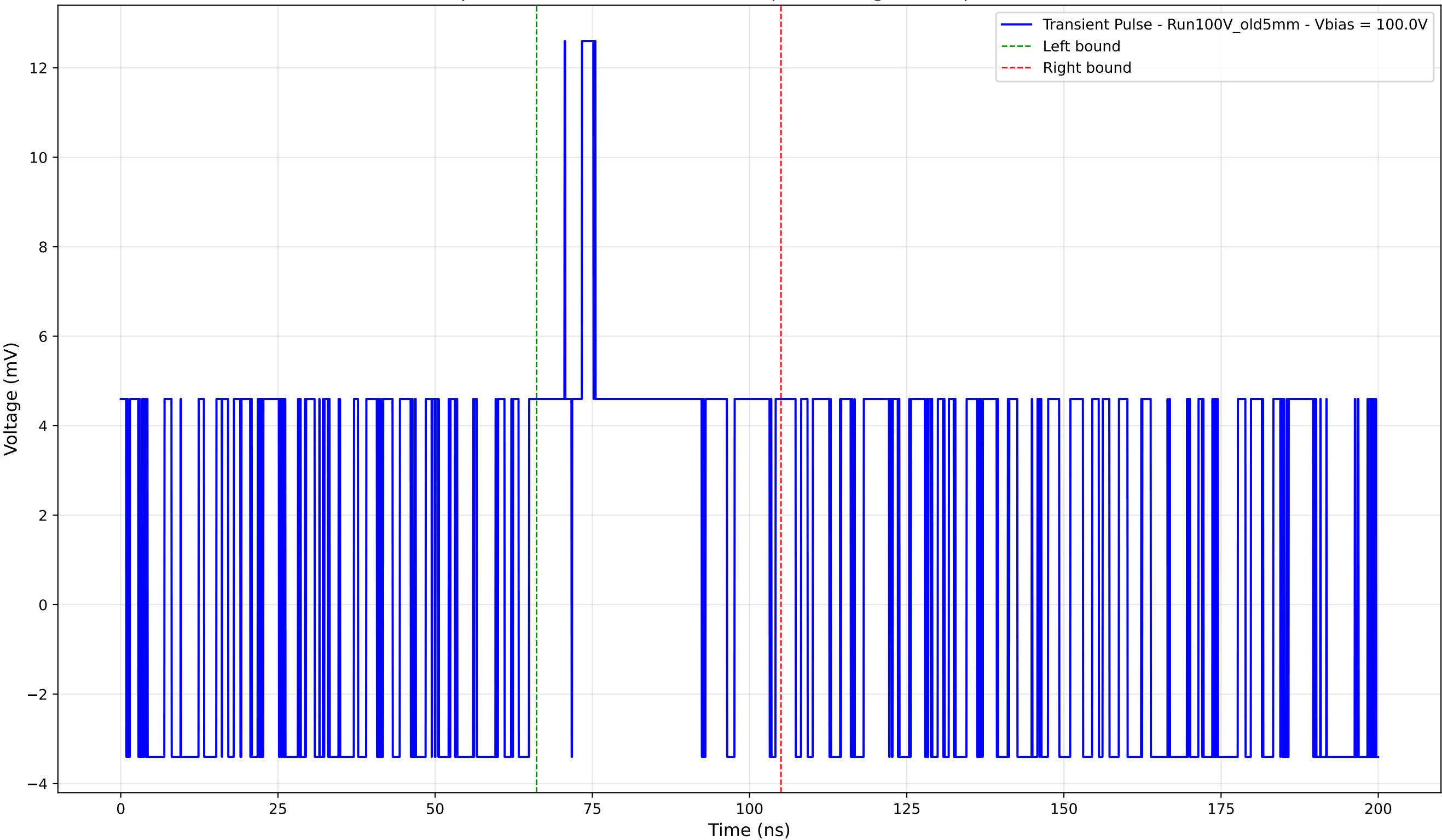
Transient Pulse - Sample: Old5mm - Position: 430.0 \mu\text{m} - Charge: 3.50 pC - Rise Time: 0.00 ns (N/A)
