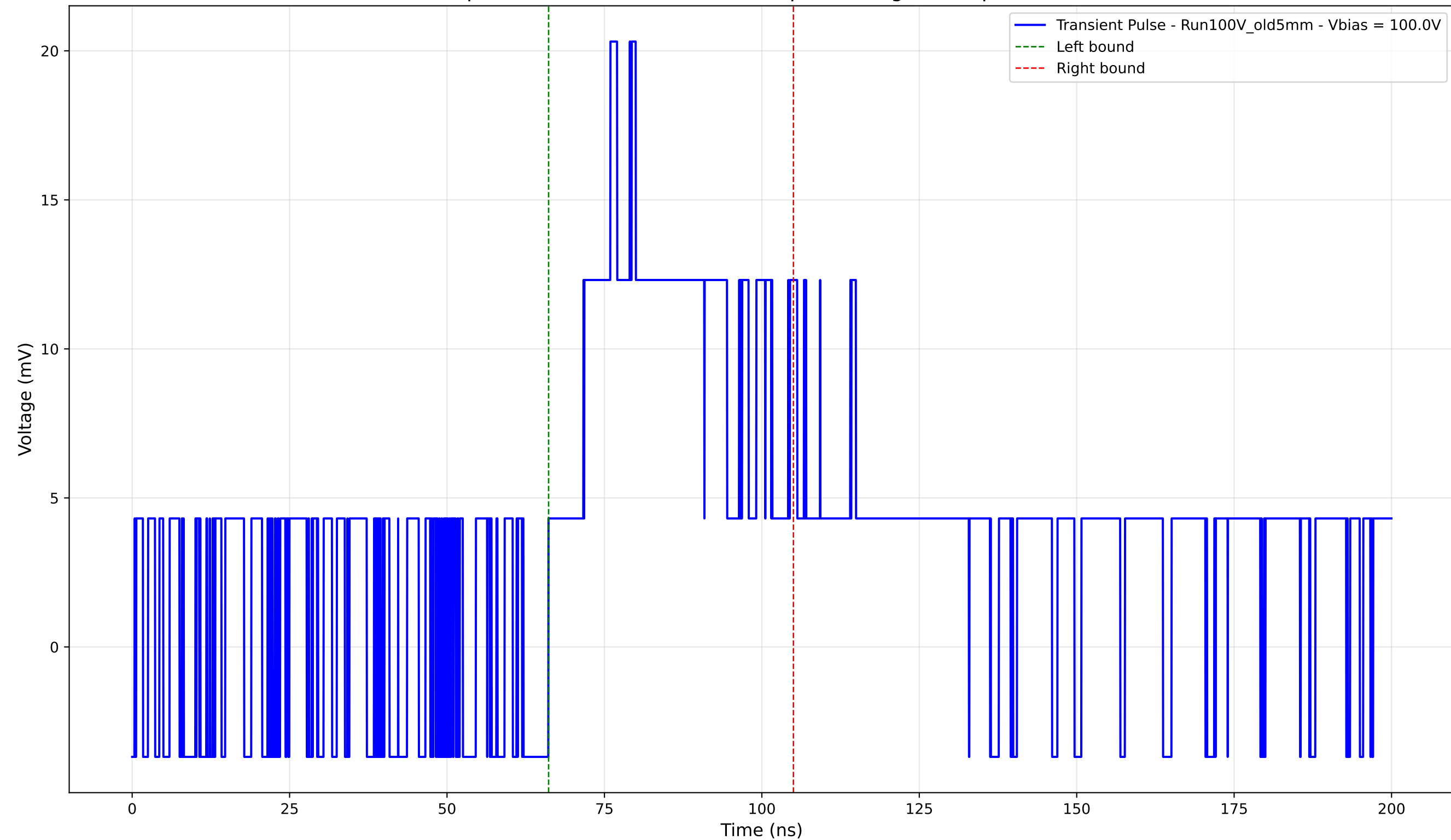
Transient Pulse - Sample: Old5mm - Position: 1380.0 \mu\text{m} - Charge: 7.96 pC - Rise Time: 0.00 ns (N/A)
