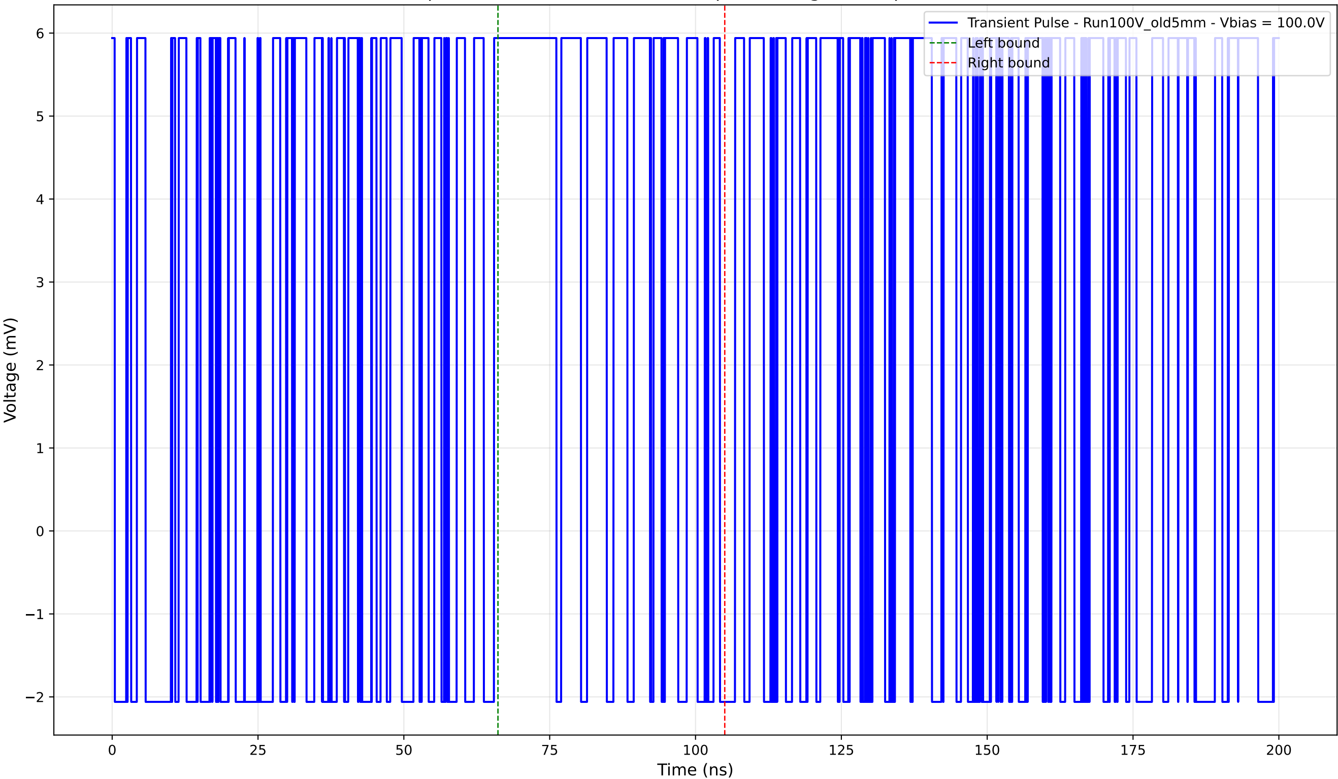
Transient Pulse - Sample: Old5mm - Position: 285.0 \mu\text{m} - Charge: 3.02 pC - Rise Time: 0.00 ns (N/A)
