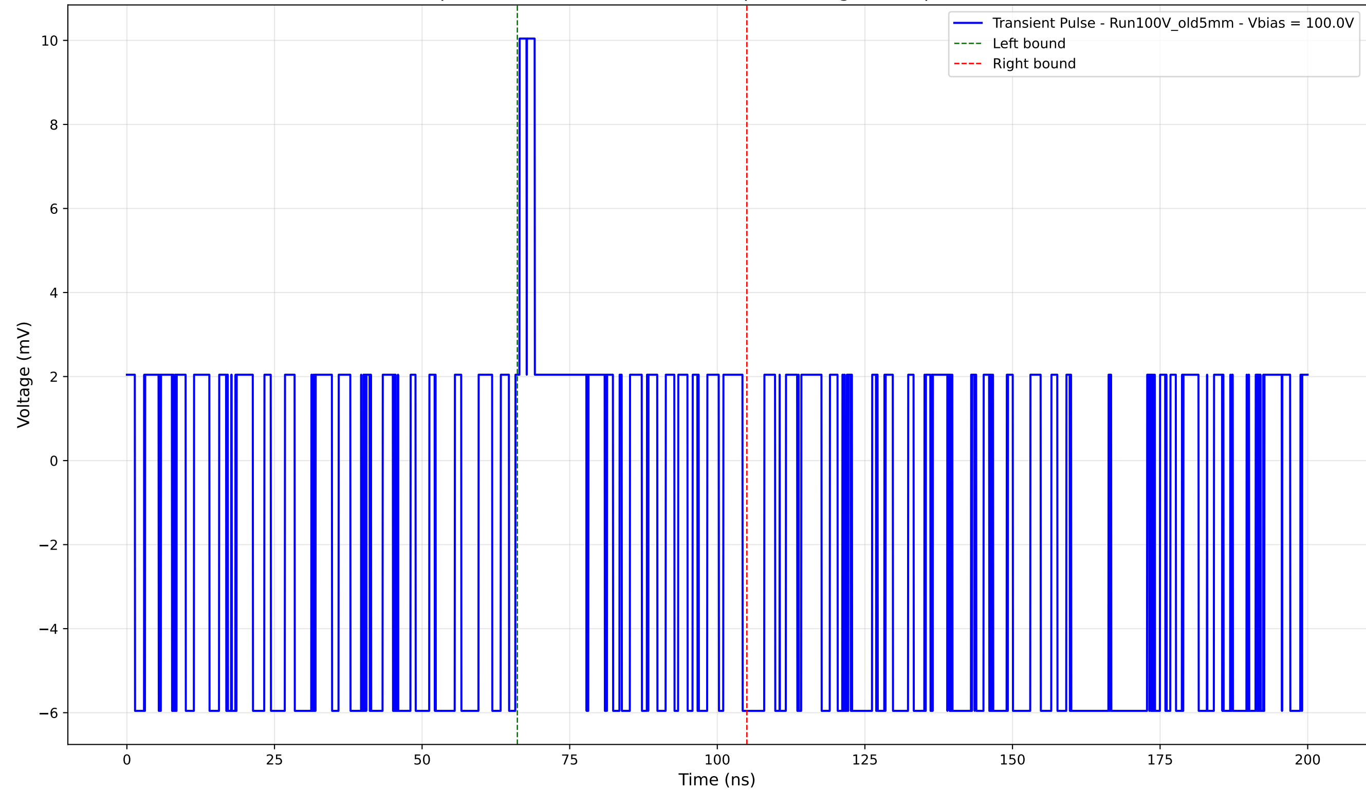
Transient Pulse - Sample: Old5mm - Position: 3990.0 \mu\text{m} - Charge: 0.44 pC - Rise Time: 0.00 ns (N/A)
