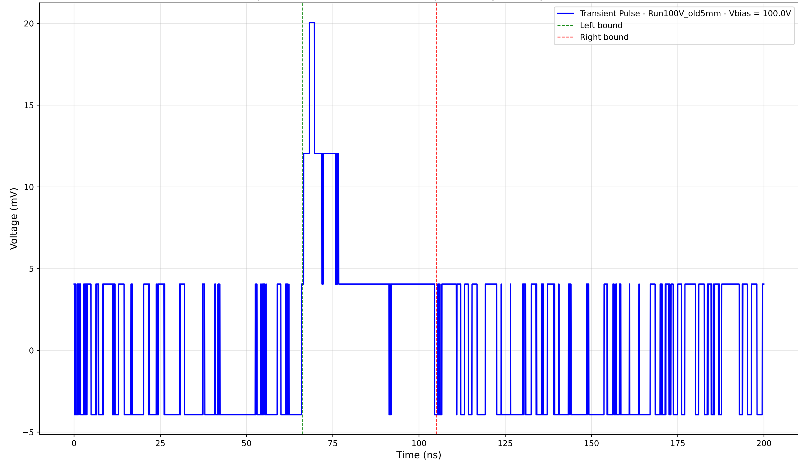
Transient Pulse - Sample: Old5mm - Position: 3145.0 \mu\text{m} - Charge: 4.77 pC - Rise Time: 0.00 ns (N/A)
