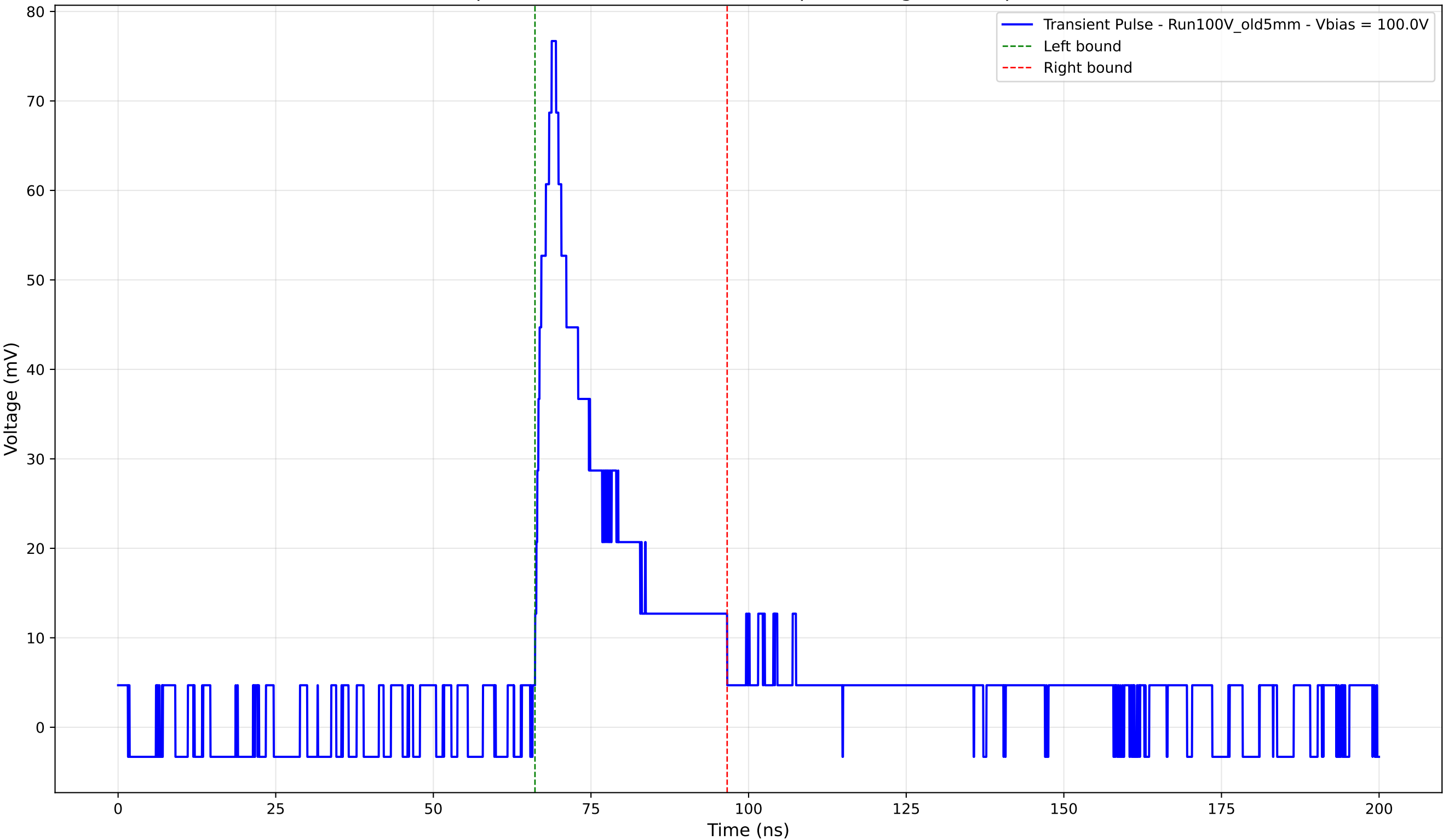
Transient Pulse - Sample: Old5mm - Position: 4435.0 \mu\text{m} - Charge: 15.98 pC - Rise Time: 2.63 ns
