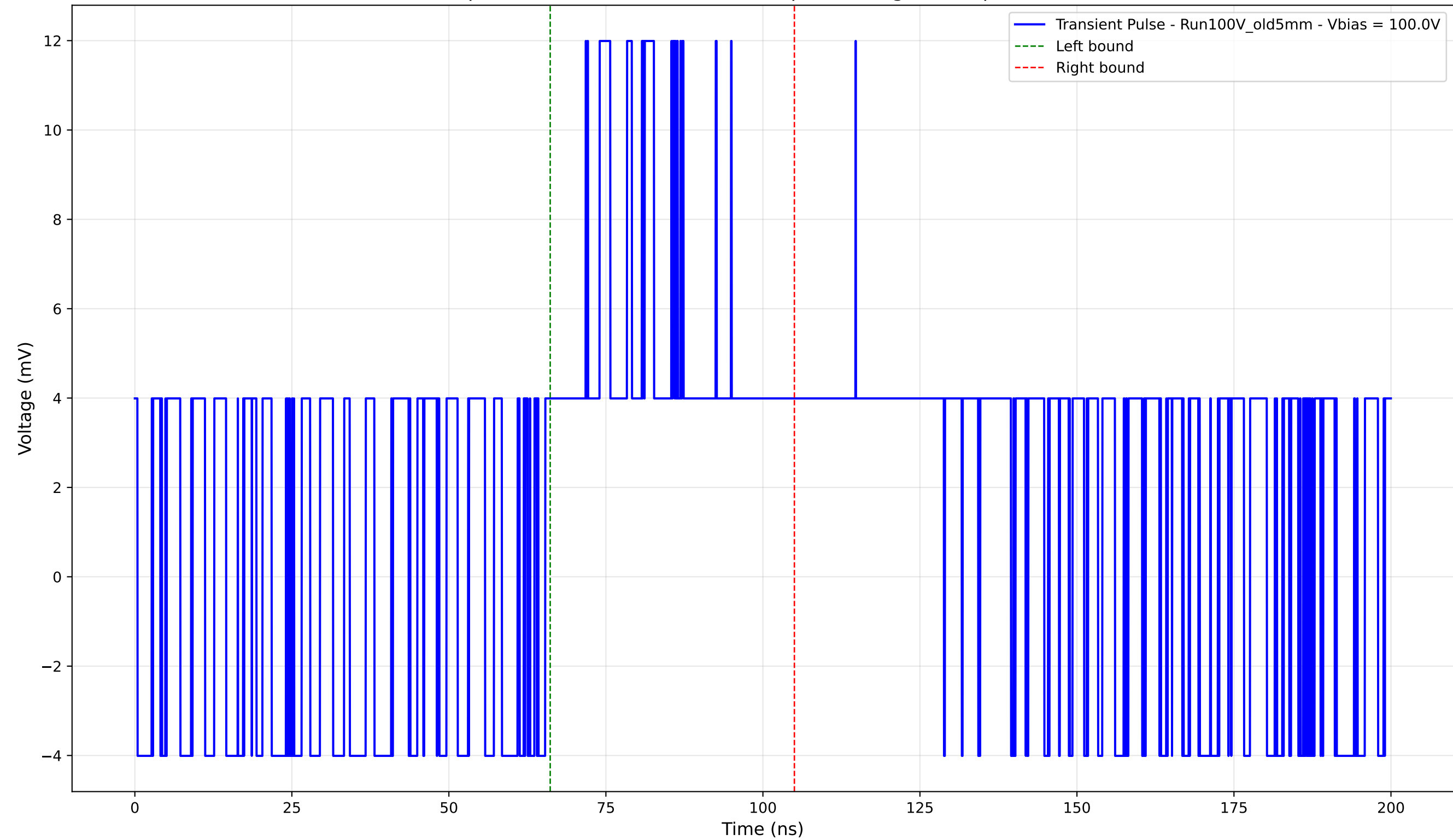
Transient Pulse - Sample: Old5mm - Position: 1120.0 \mu\text{m} - Charge: 4.00 pC - Rise Time: 0.00 ns (N/A)
