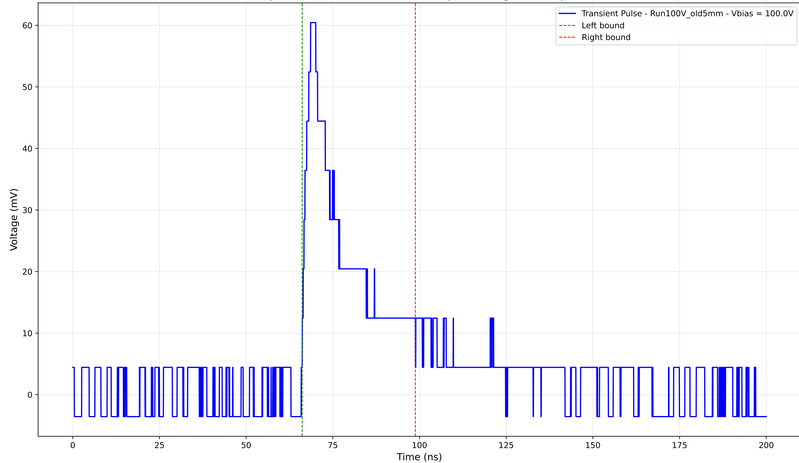
Transient Pulse - Sample: Old5mm - Position: 4505.0 \mu\text{m} - Charge: 15.34 pC - Rise Time: 2.42 ns
