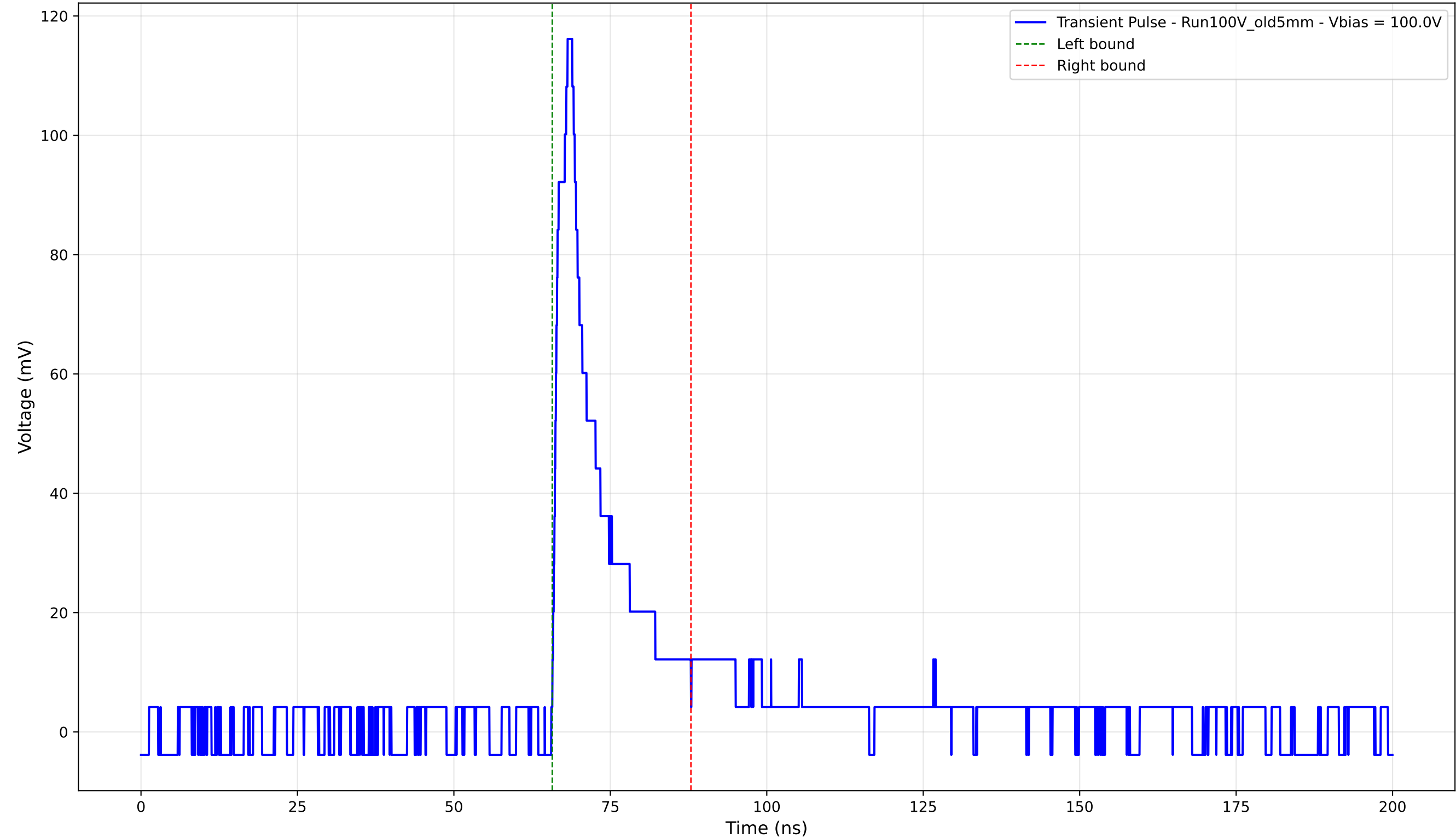
Transient Pulse - Sample: Old5mm - Position: 4145.0 \mu\text{m} - Charge: 17.13 pC - Rise Time: 2.22 ns
