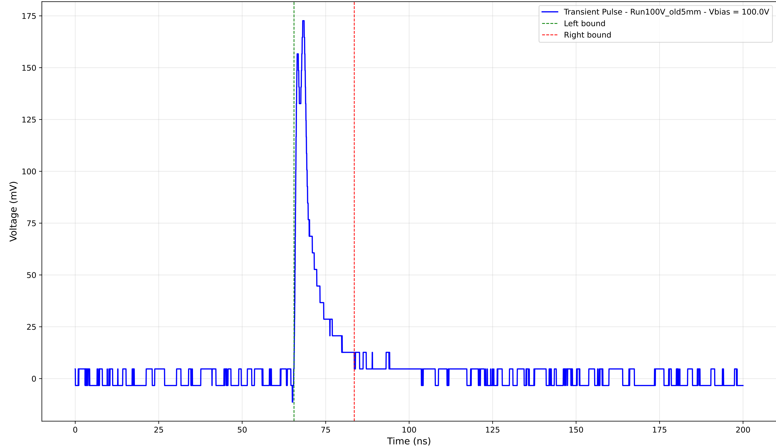
Transient Pulse - Sample: Old5mm - Position: 3900.0 \mu\text{m} - Charge: 19.38 pC - Rise Time: 0.85 ns
