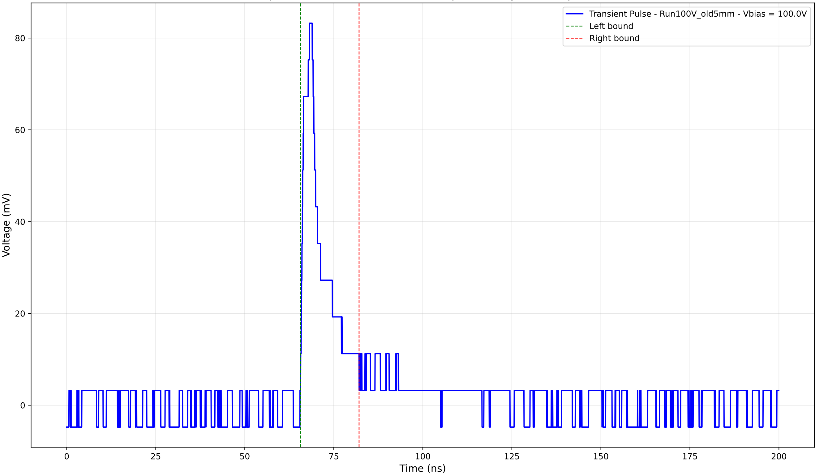
Transient Pulse - Sample: Old5mm - Position: 3325.0 \mu\text{m} - Charge: 10.32 pC - Rise Time: 2.13 ns
