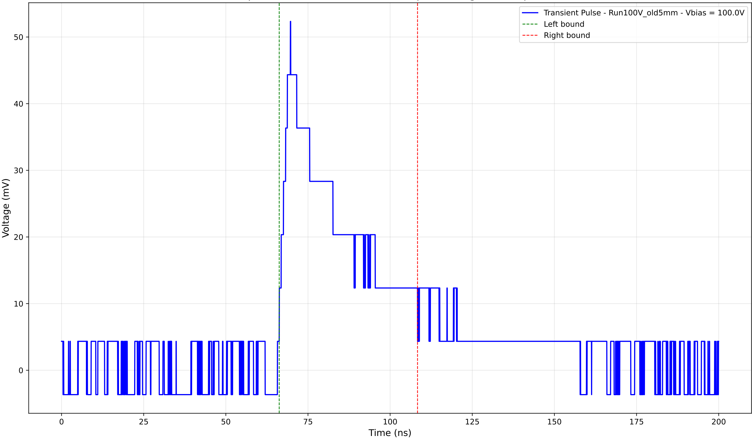
Transient Pulse - Sample: Old5mm - Position: 4840.0 \mu\text{m} - Charge: 18.84 pC - Rise Time: 3.40 ns
