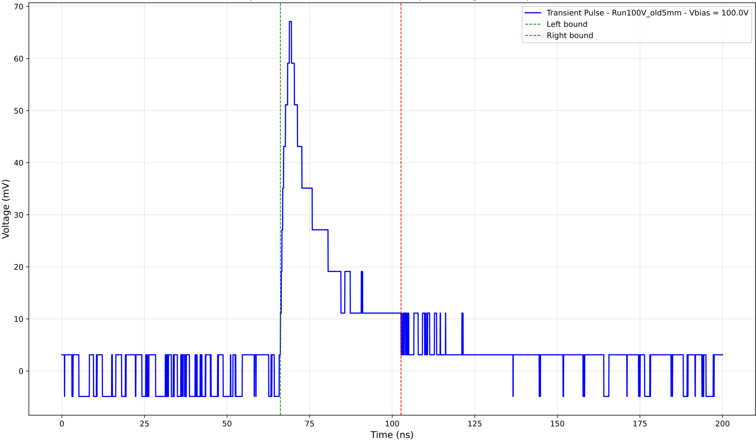
Transient Pulse - Sample: Old5mm - Position: 2930.0 \mu\text{m} - Charge: 16.87 pC - Rise Time: 2.71 ns
