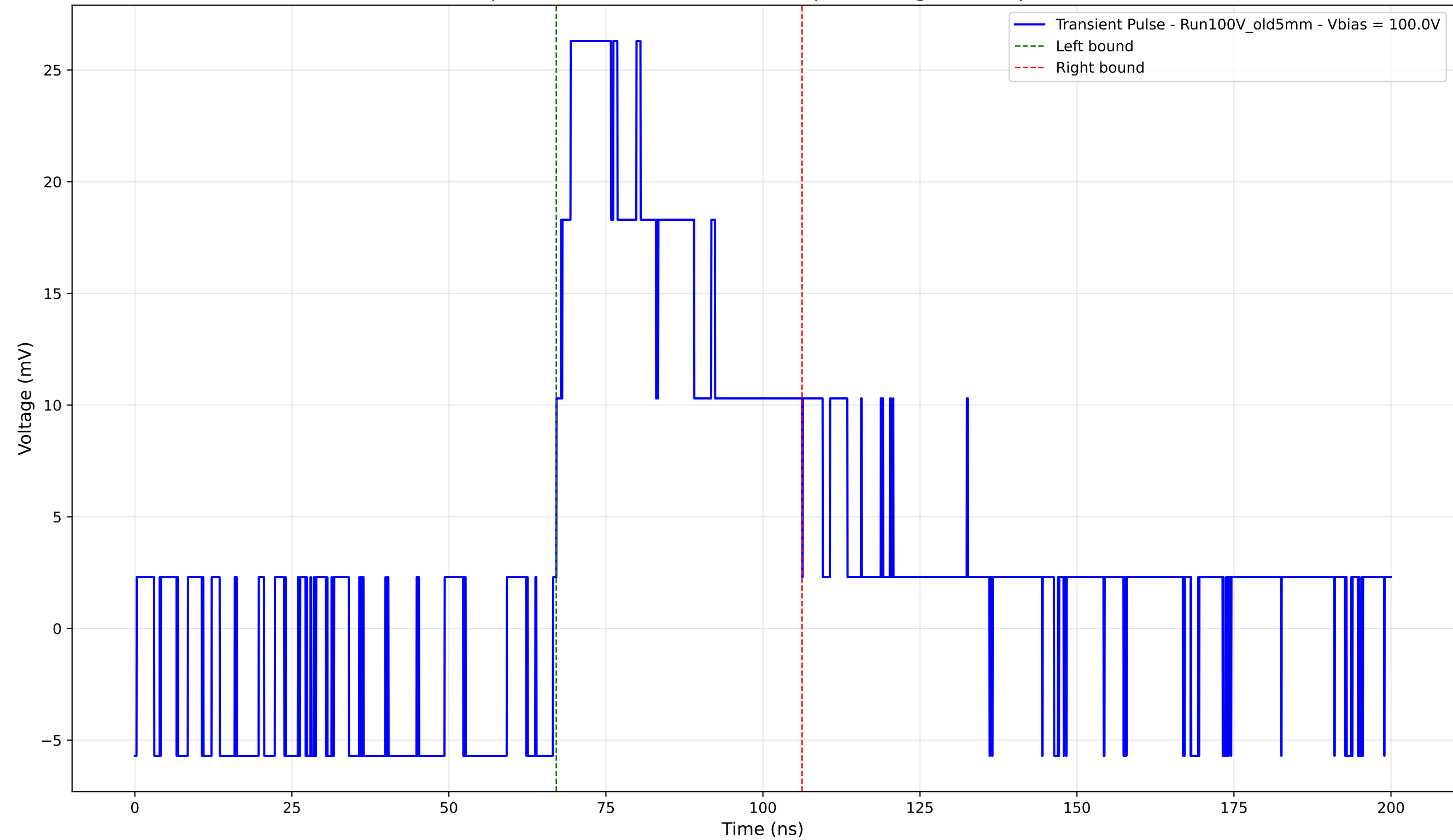
Transient Pulse - Sample: Old5mm - Position: 2435.0 \mu\text{m} - Charge: 12.75 pC - Rise Time: 2.28 ns
