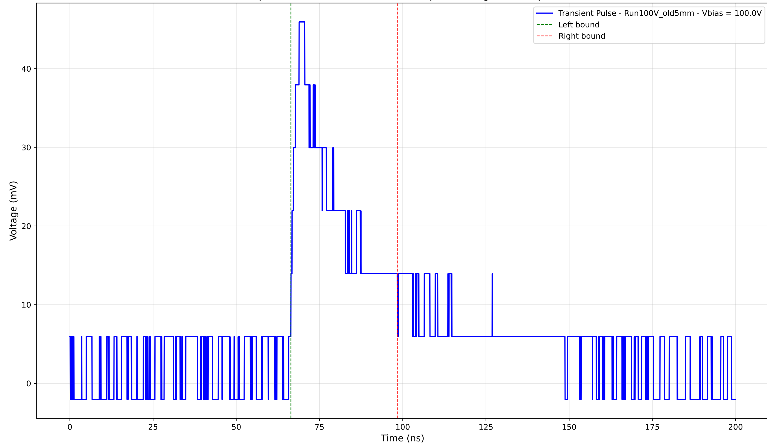
Transient Pulse - Sample: Old5mm - Position: 4715.0 \mu\text{m} - Charge: 14.40 pC - Rise Time: 3.13 ns
