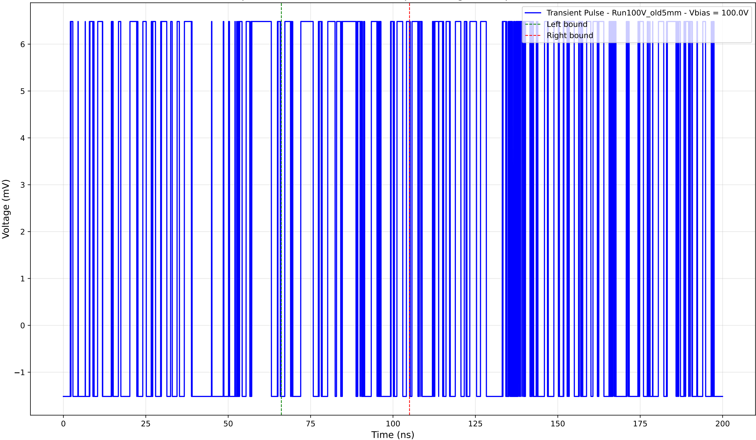
Transient Pulse - Sample: Old5mm - Position: 130.0 \mu\text{m} - Charge: 2.36 pC - Rise Time: 0.00 ns (N/A)
