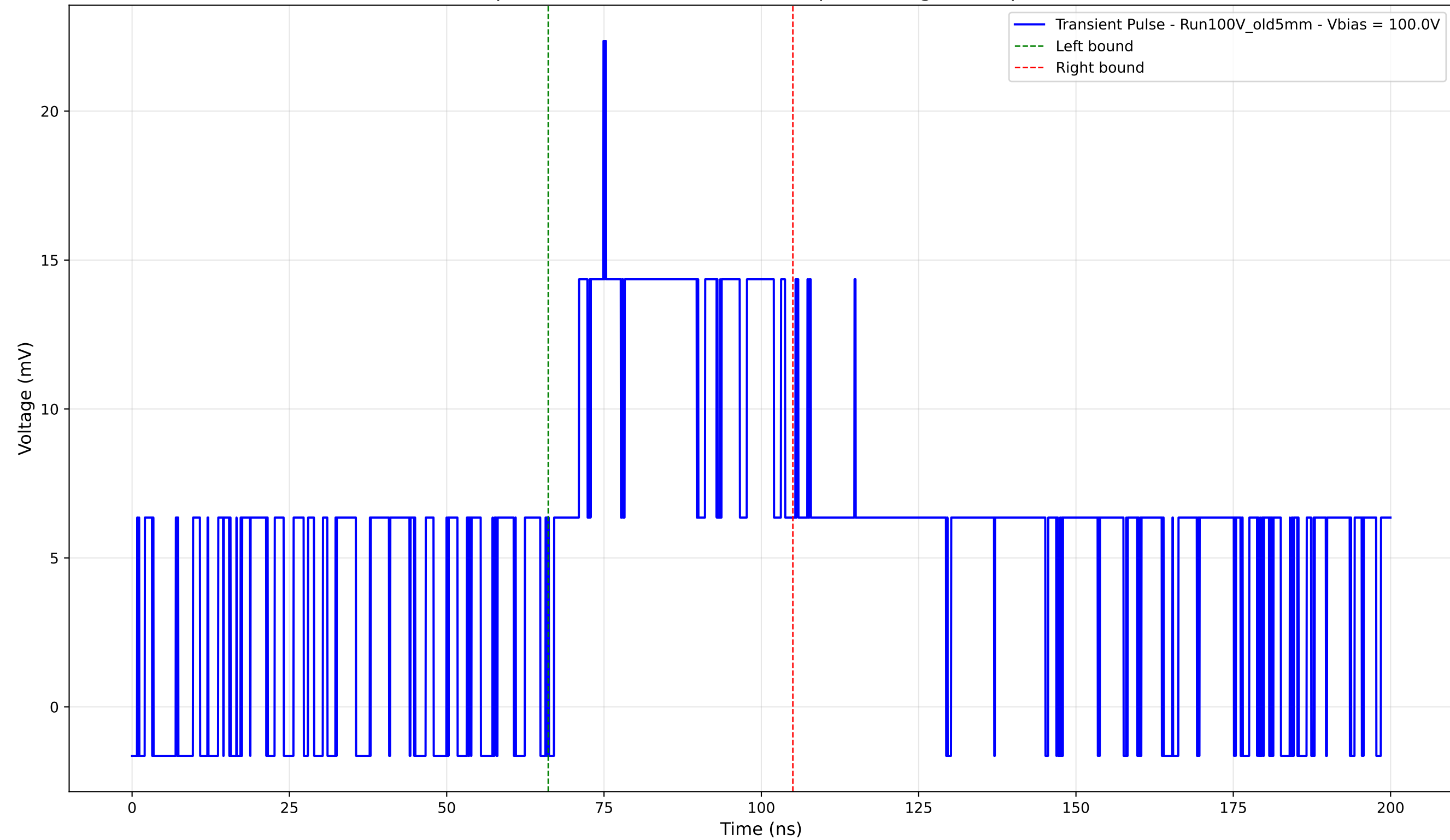
Transient Pulse - Sample: Old5mm - Position: 1570.0 \mu\text{m} - Charge: 9.34 pC - Rise Time: 7.86 ns
