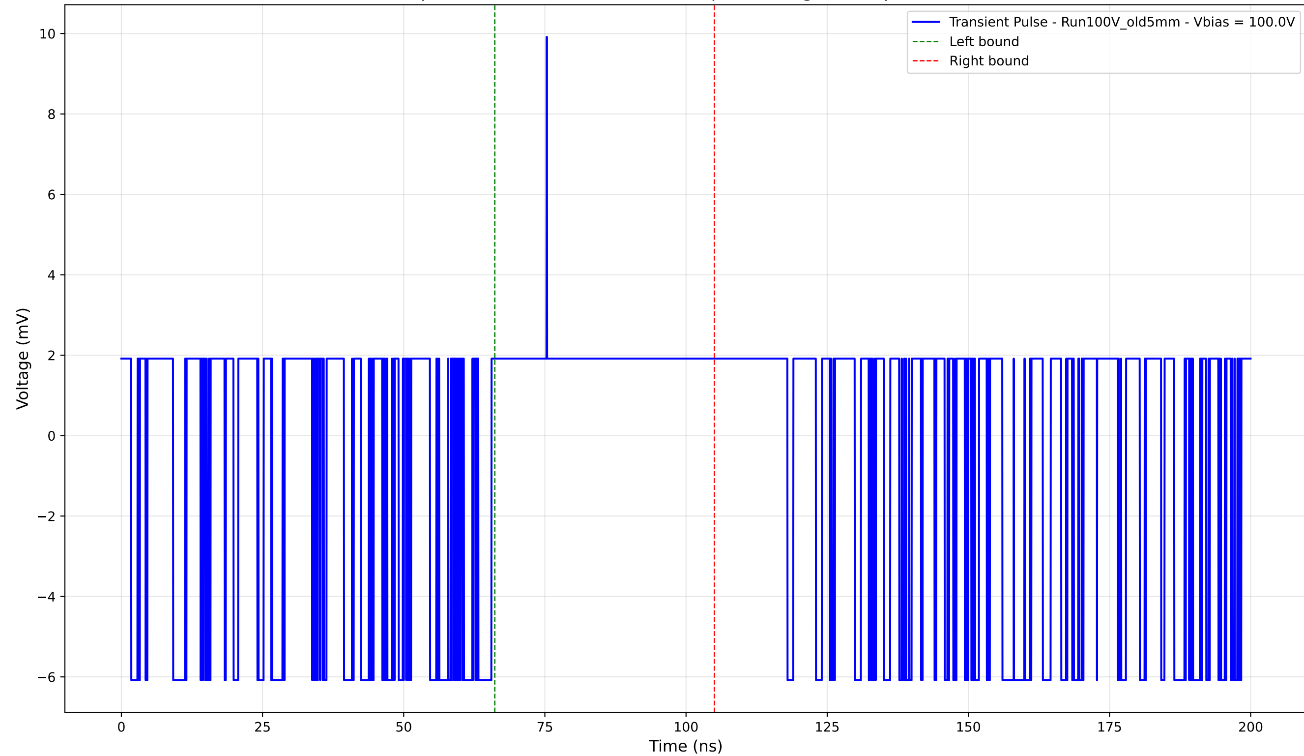
Transient Pulse - Sample: Old5mm - Position: 2340.0 \mu\text{m} - Charge: 1.50 pC - Rise Time: 0.00 ns (N/A)
