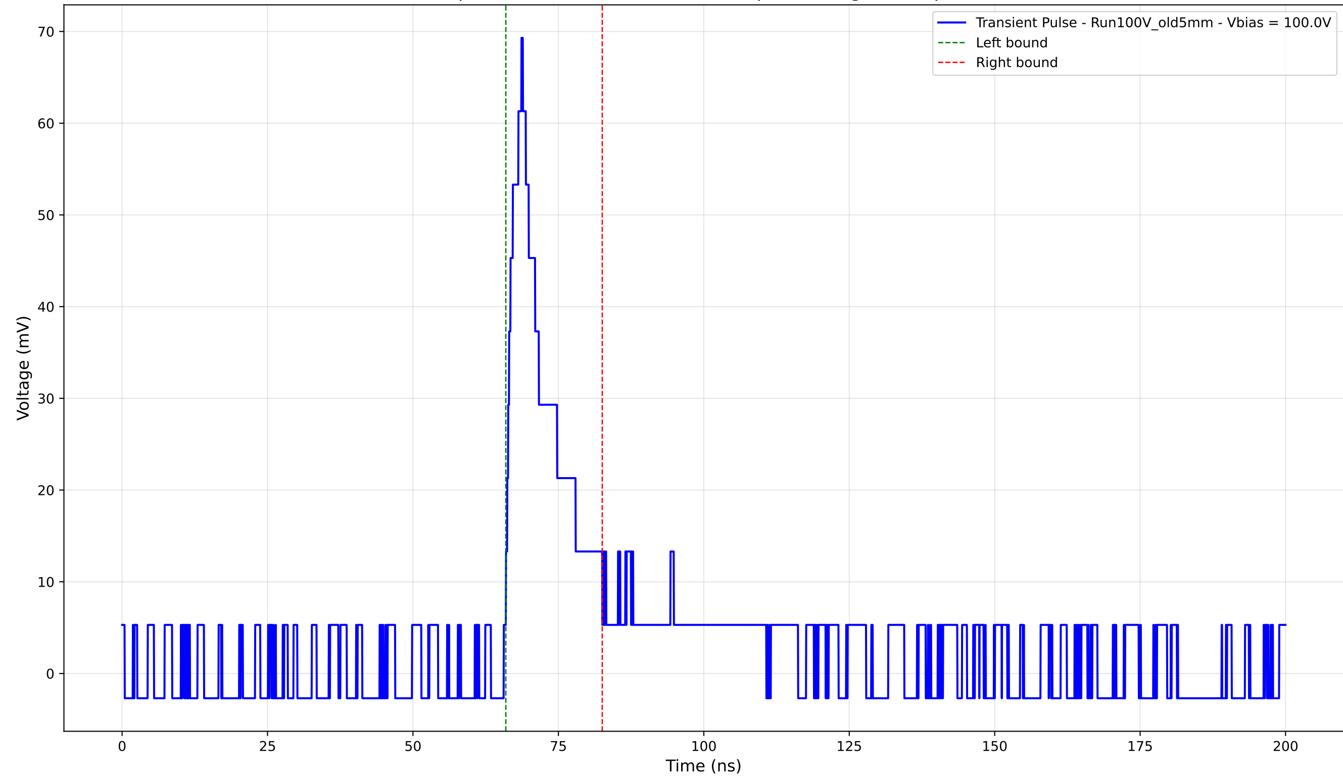
Transient Pulse - Sample: Old5mm - Position: 3180.0 \mu\text{m} - Charge: 9.82 pC - Rise Time: 2.68 ns
