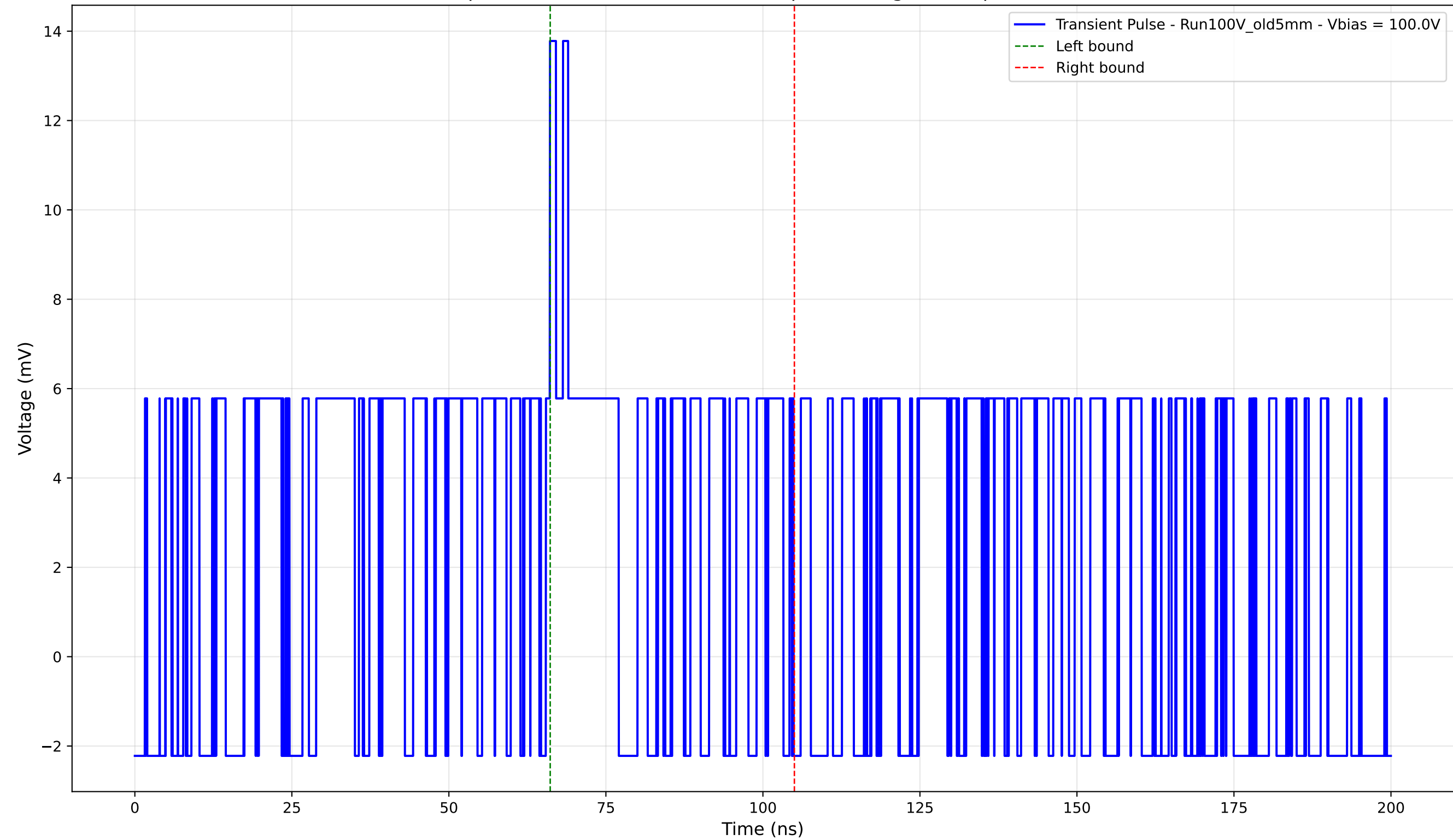
Transient Pulse - Sample: Old5mm - Position: 3695.0 \mu\text{m} - Charge: 2.73 pC - Rise Time: 0.00 ns (N/A)
