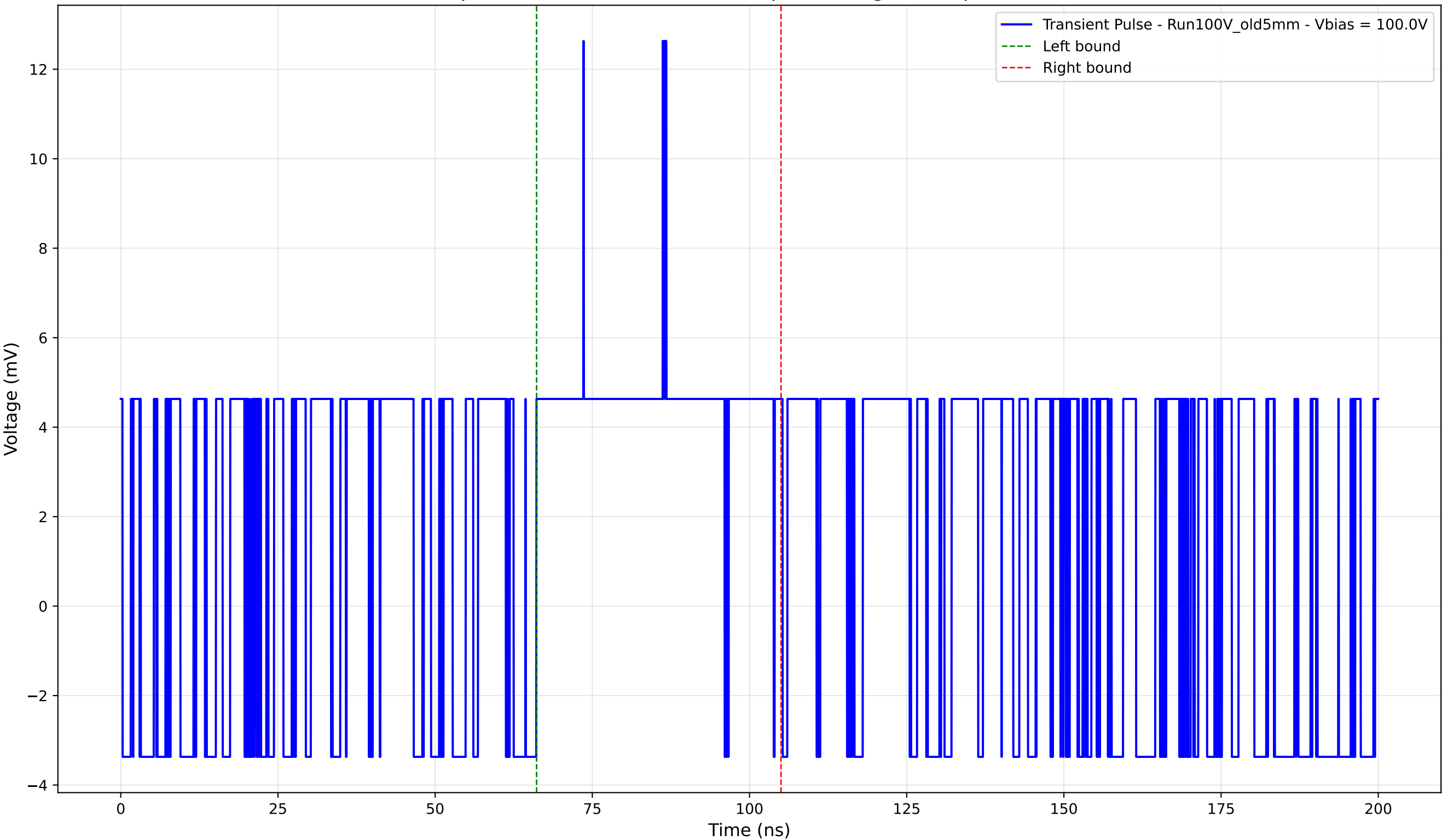
Transient Pulse - Sample: Old5mm - Position: 825.0 \mu\text{m} - Charge: 3.62 pC - Rise Time: 0.00 ns (N/A)
