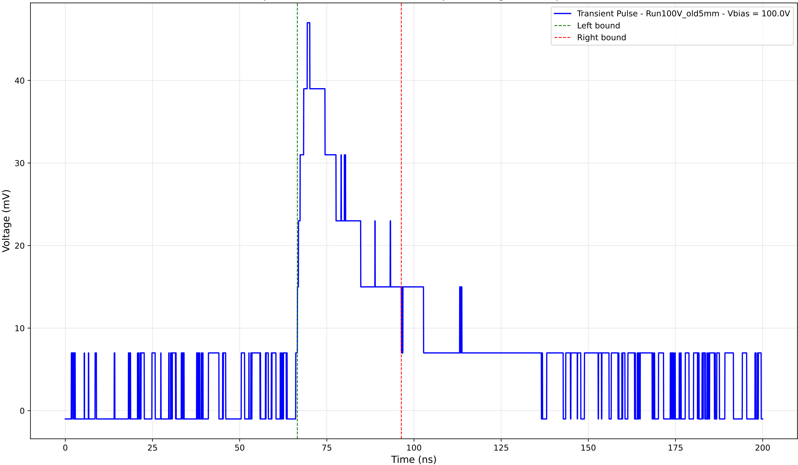
Transient Pulse - Sample: Old5mm - Position: 2665.0 \mu\text{m} - Charge: 14.60 pC - Rise Time: 3.31 ns
