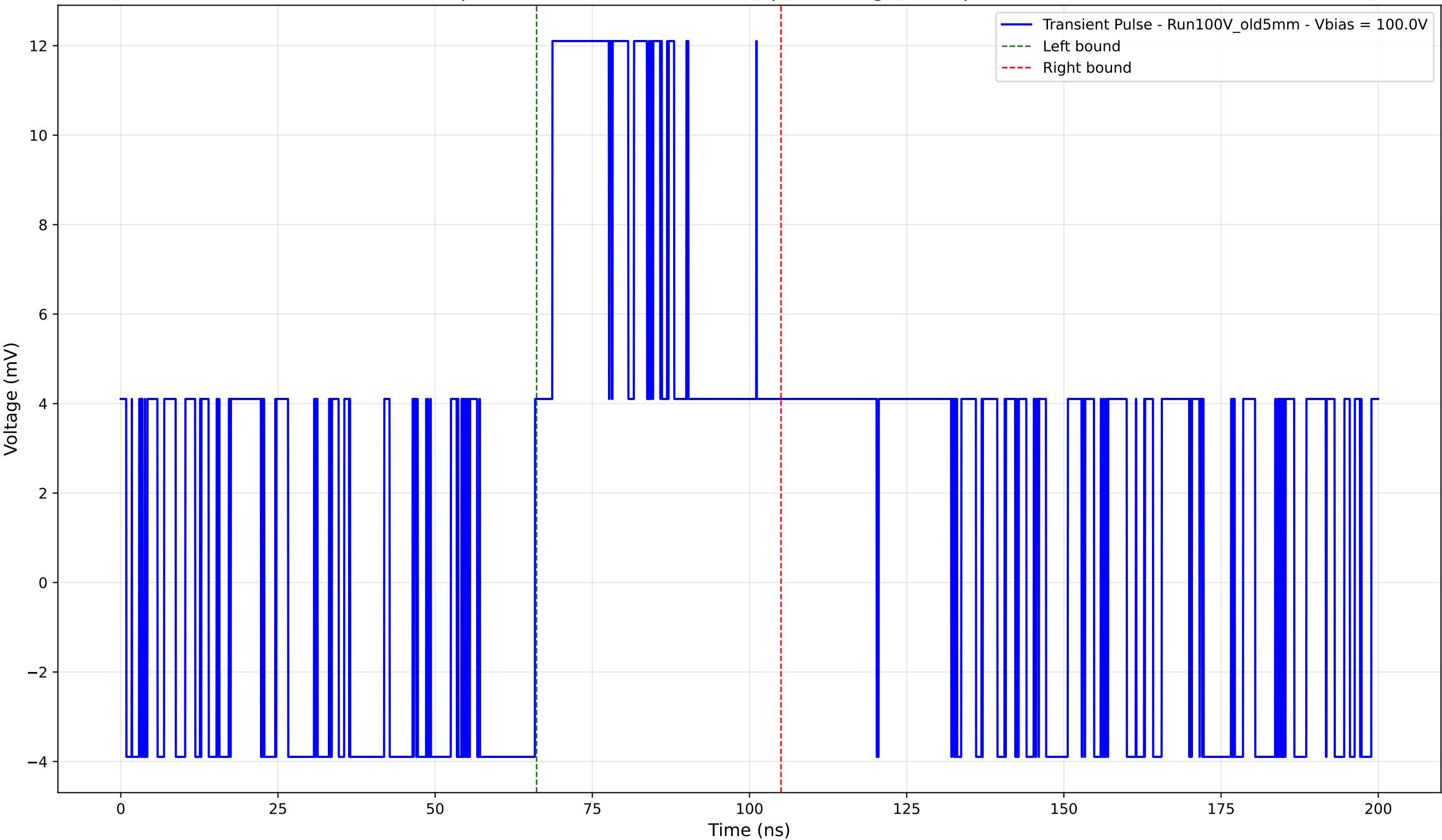
Transient Pulse - Sample: Old5mm - Position: 370.0 \mu\text{m} - Charge: 5.88 pC - Rise Time: 0.00 ns (N/A)
