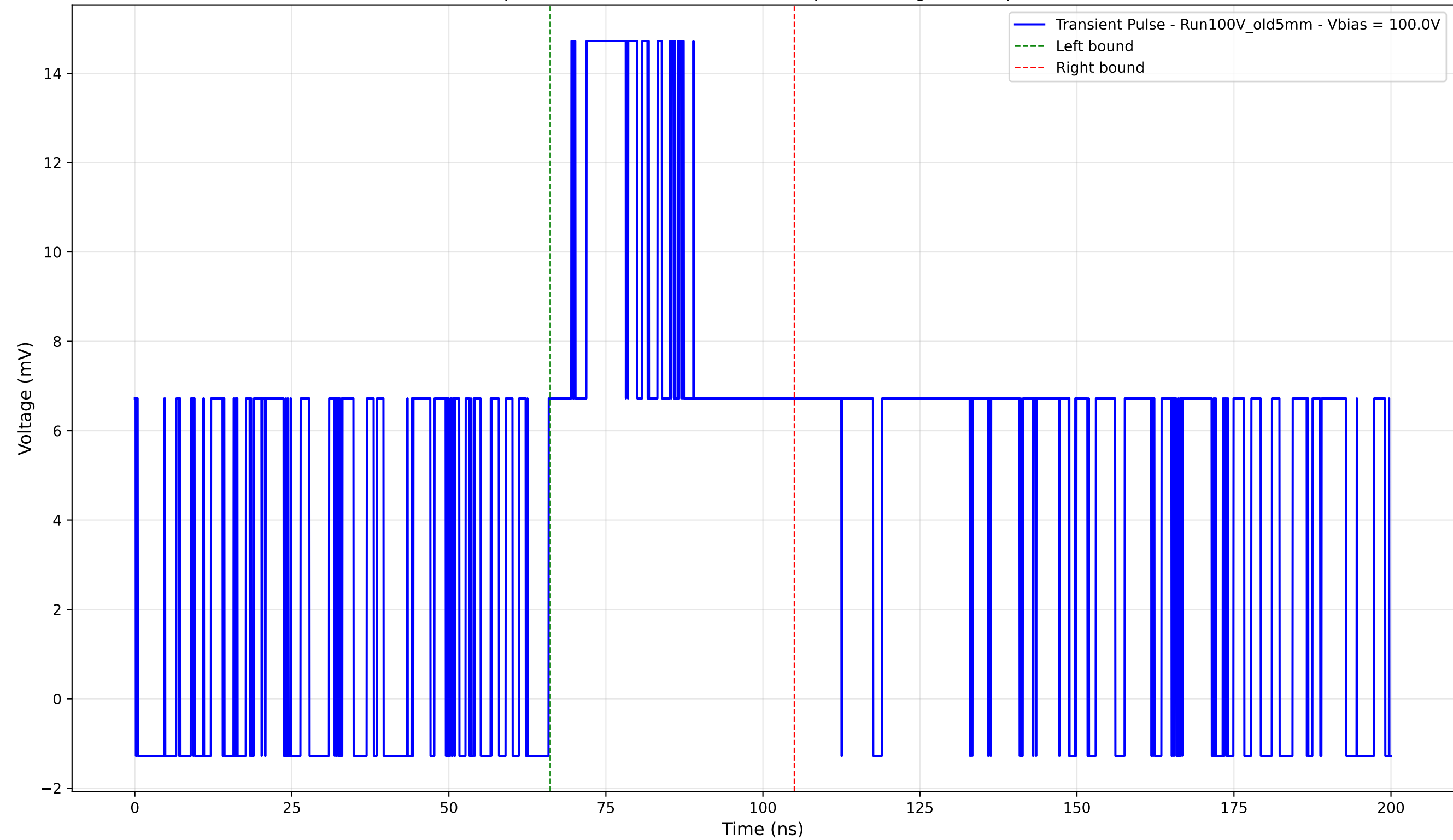
Transient Pulse - Sample: Old5mm - Position: 465.0 \mu\text{m} - Charge: 7.07 pC - Rise Time: 3.64 ns
