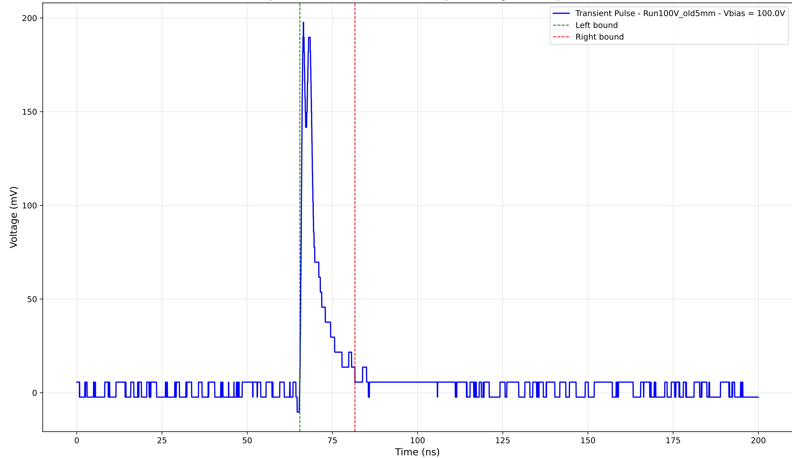
Transient Pulse - Sample: Old5mm - Position: 3845.0 \mu\text{m} - Charge: 19.92 pC - Rise Time: 0.74 ns
