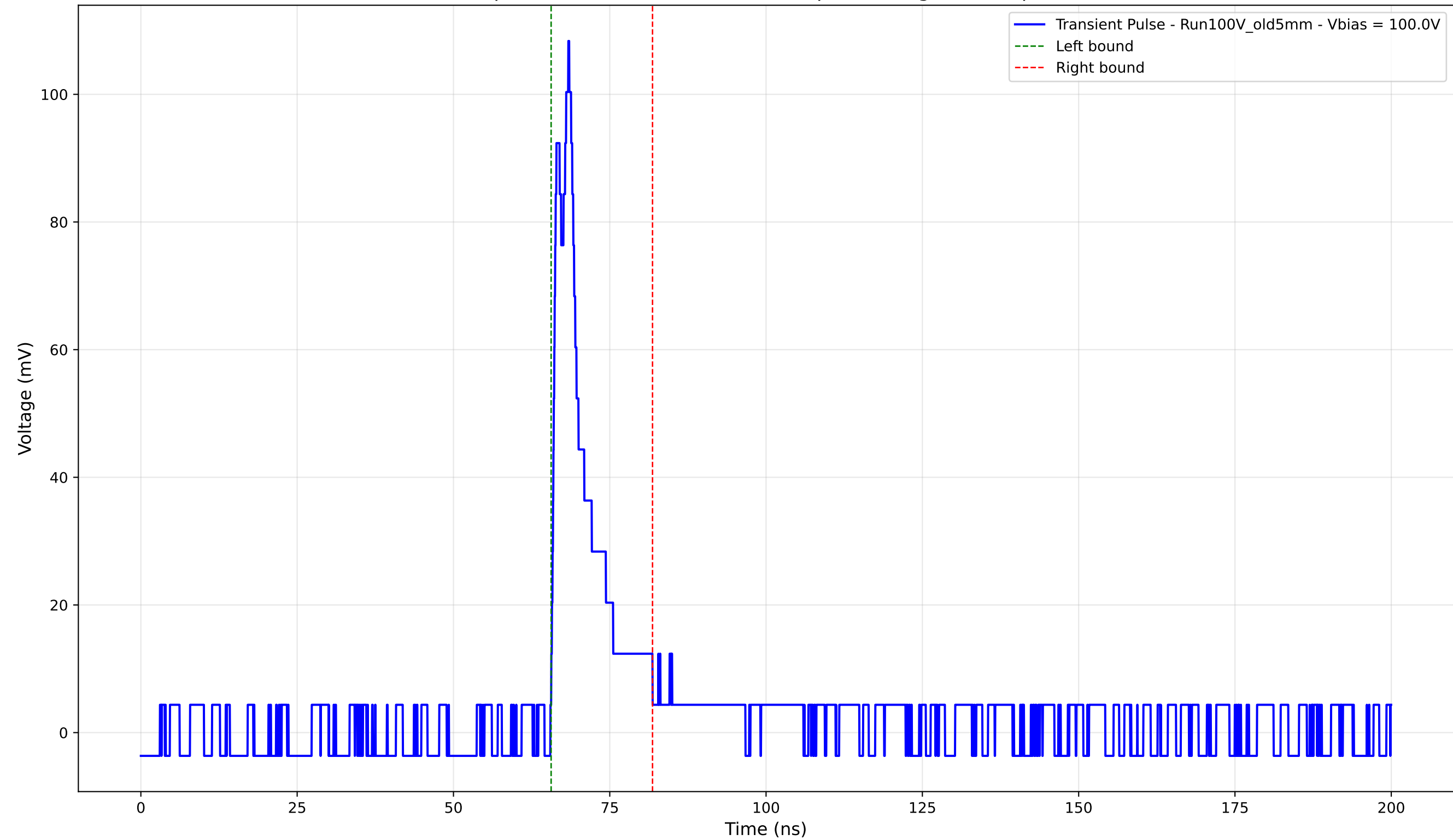
Transient Pulse - Sample: Old5mm - Position: 3485.0 \mu\text{m} - Charge: 11.75 pC - Rise Time: 2.38 ns
