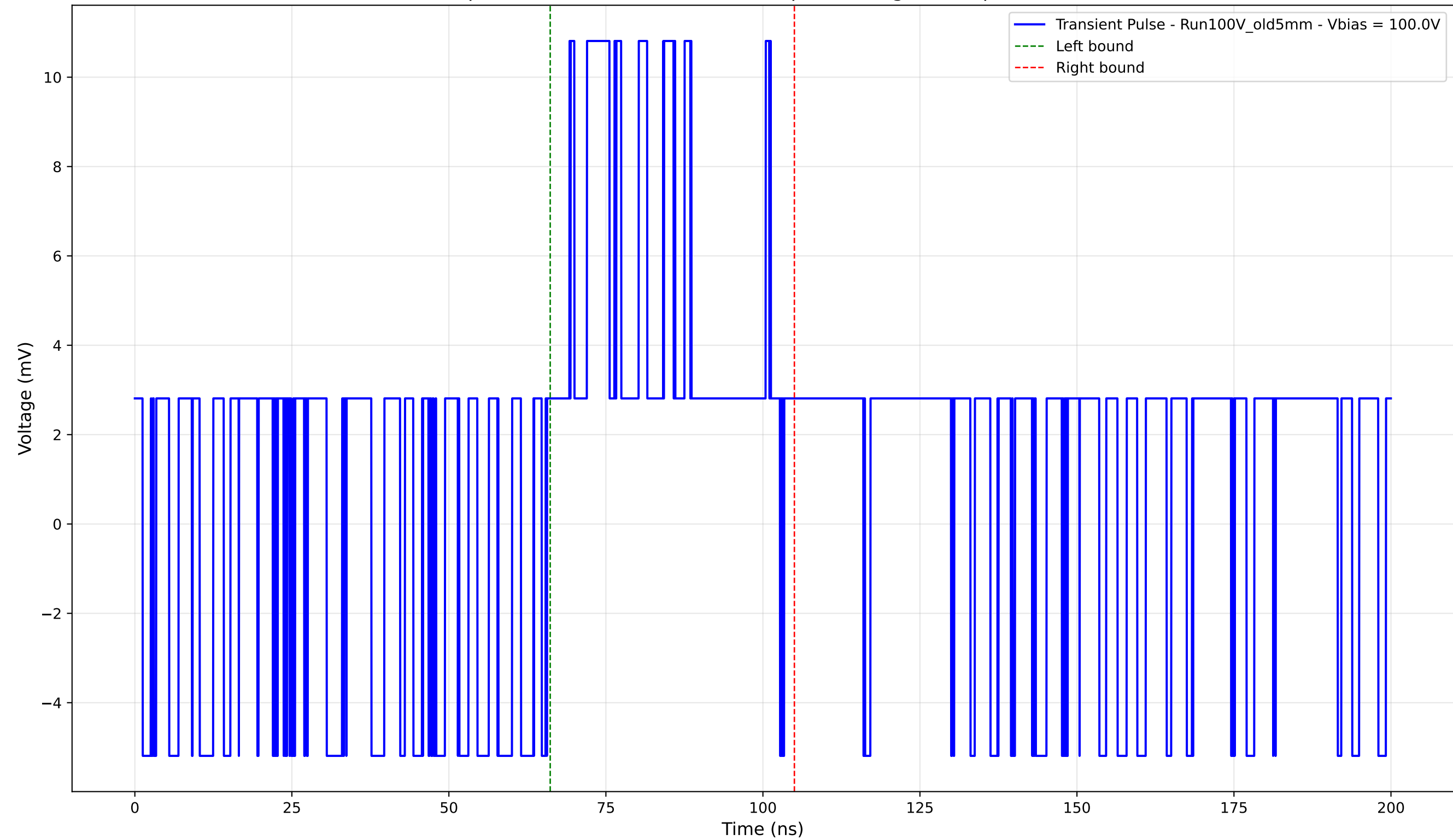
Transient Pulse - Sample: Old5mm - Position: 2285.0 \mu\text{m} - Charge: 3.70 pC - Rise Time: 0.00 ns (N/A)
