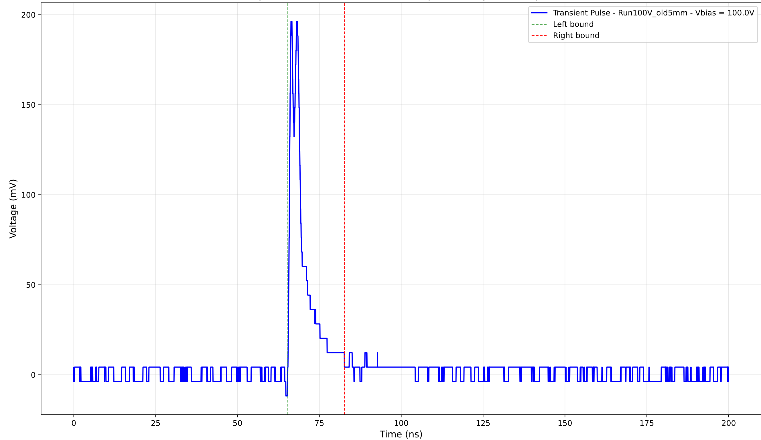
Transient Pulse - Sample: Old5mm - Position: 3605.0 \mu\text{m} - Charge: 18.91 pC - Rise Time: 0.72 ns
