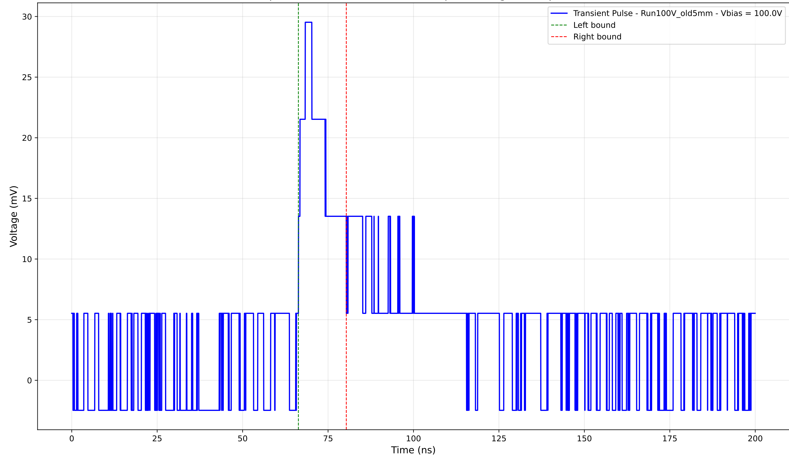
Transient Pulse - Sample: Old5mm - Position: 4550.0 \mu\text{m} - Charge: 5.29 pC - Rise Time: 2.60 ns
