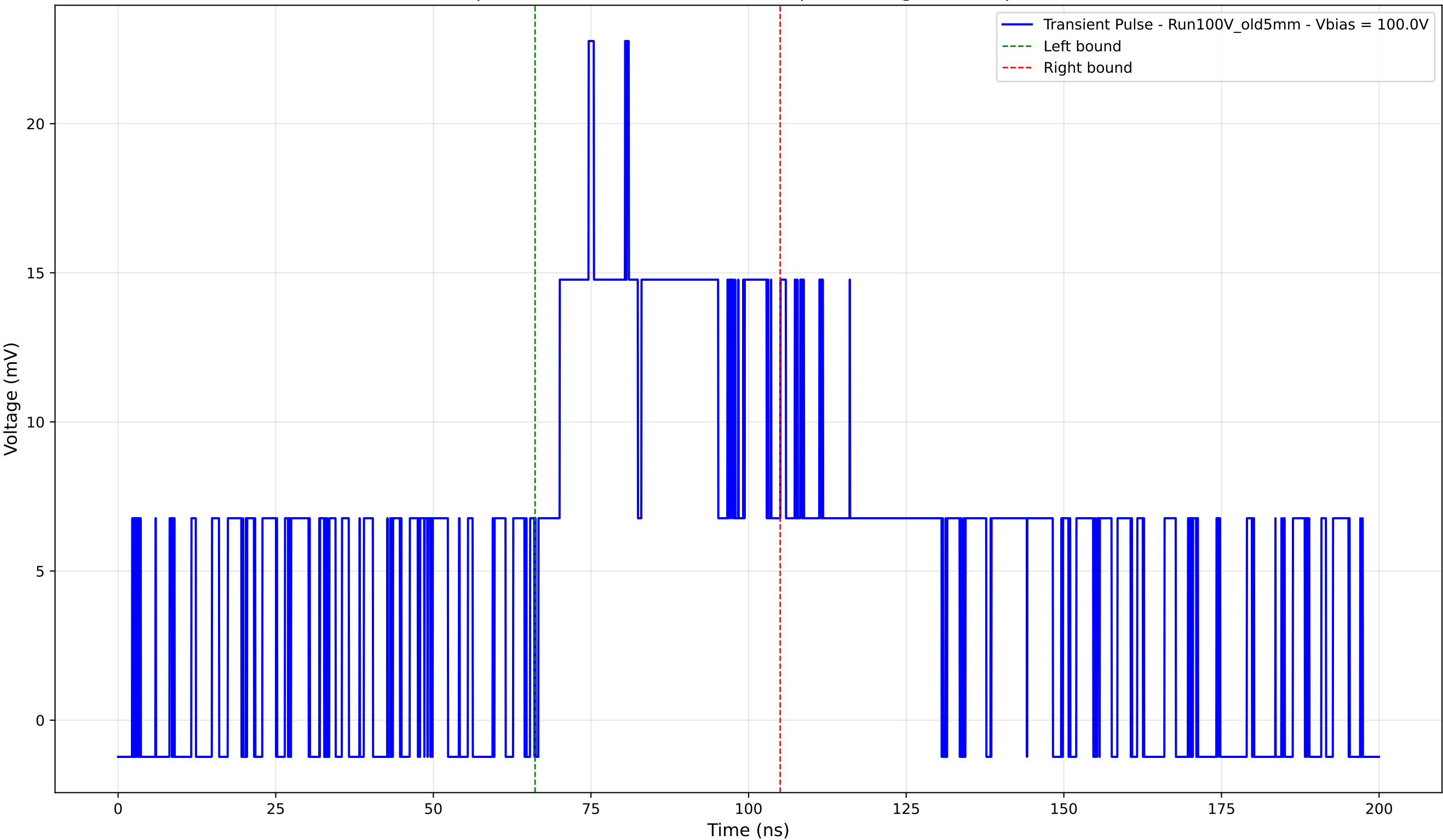
Transient Pulse - Sample: Old5mm - Position: 1230.0 \mu\text{m} - Charge: 10.04 pC - Rise Time: 7.98 ns
