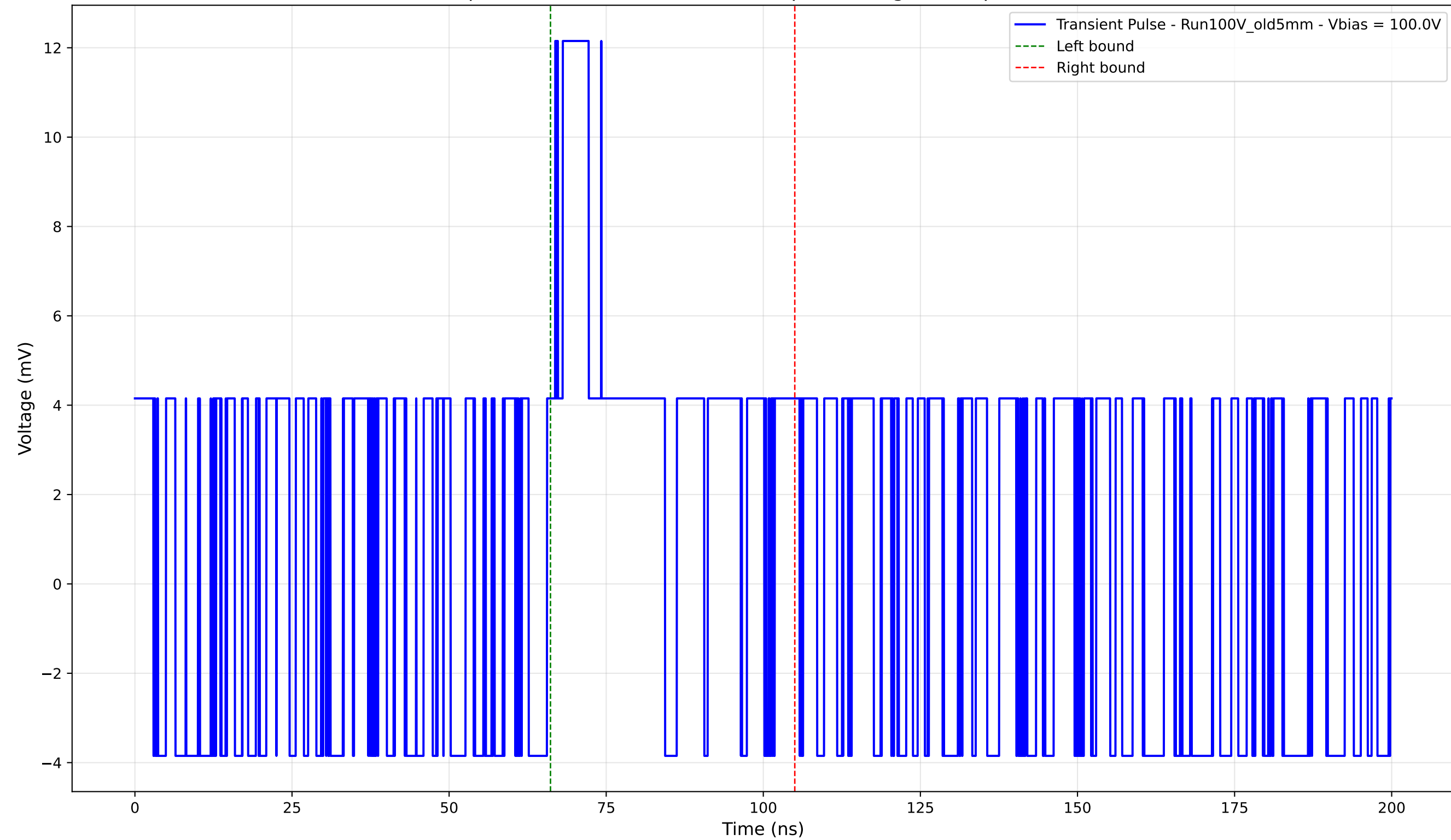
Transient Pulse - Sample: Old5mm - Position: 4350.0 \mu\text{m} - Charge: 3.26 pC - Rise Time: 0.00 ns (N/A)
