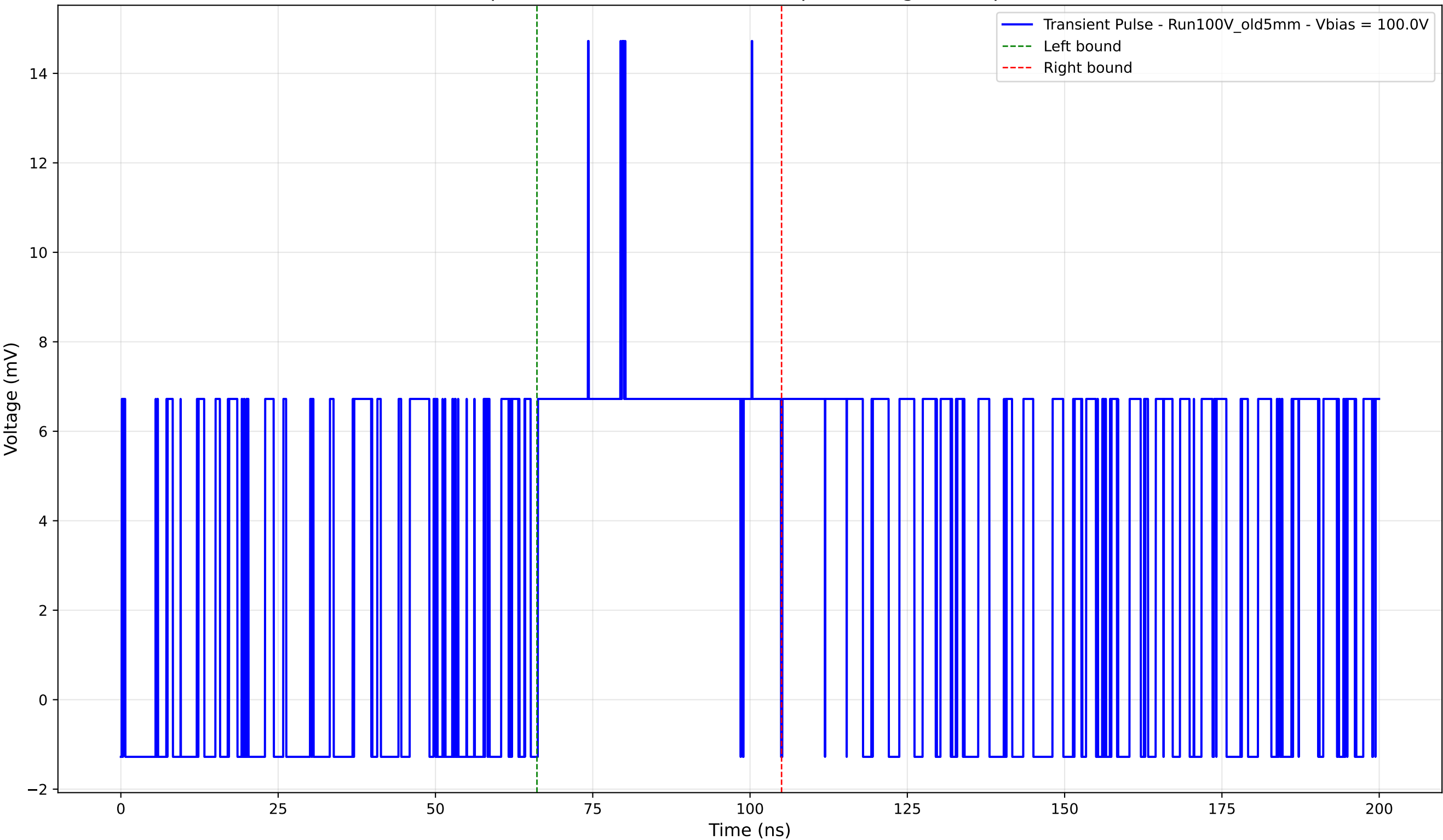
Transient Pulse - Sample: Old5mm - Position: 425.0 \mu\text{m} - Charge: 5.26 pC - Rise Time: 7.98 ns
