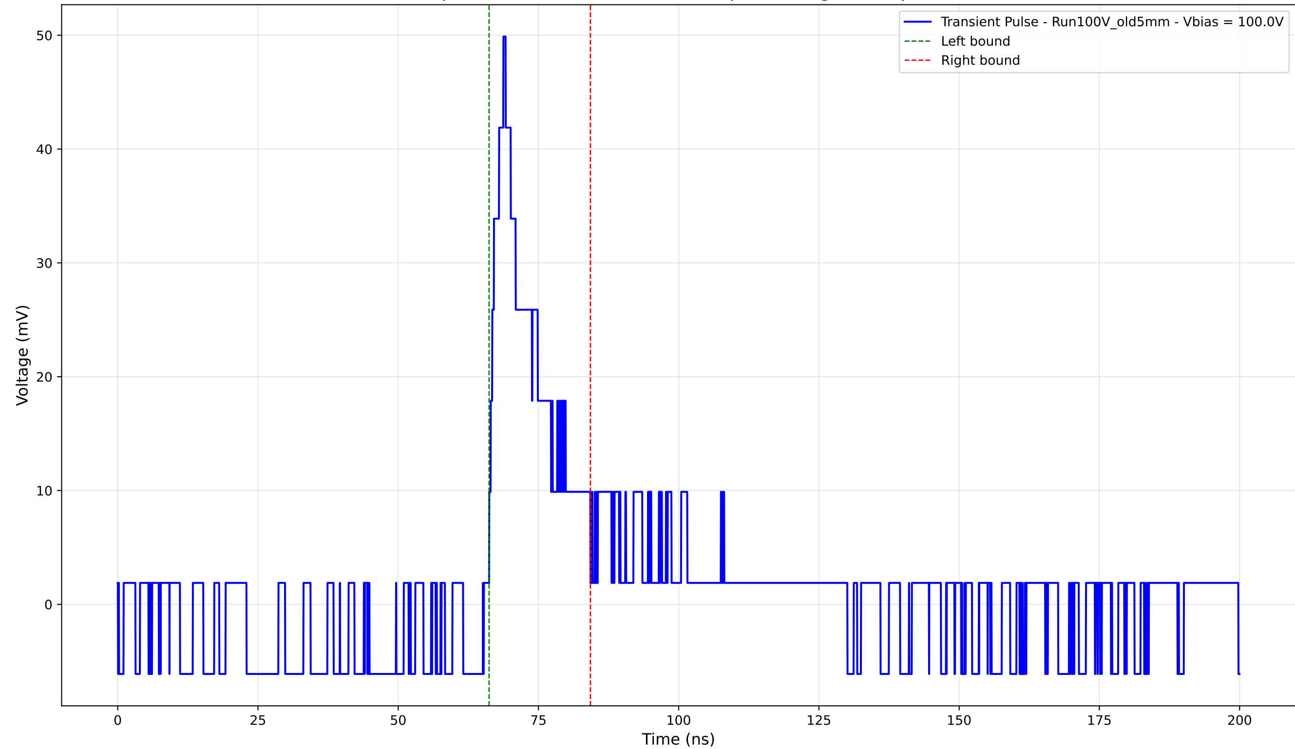
Transient Pulse - Sample: Old5mm - Position: 3025.0 \mu\text{m} - Charge: 7.76 pC - Rise Time: 2.53 ns
