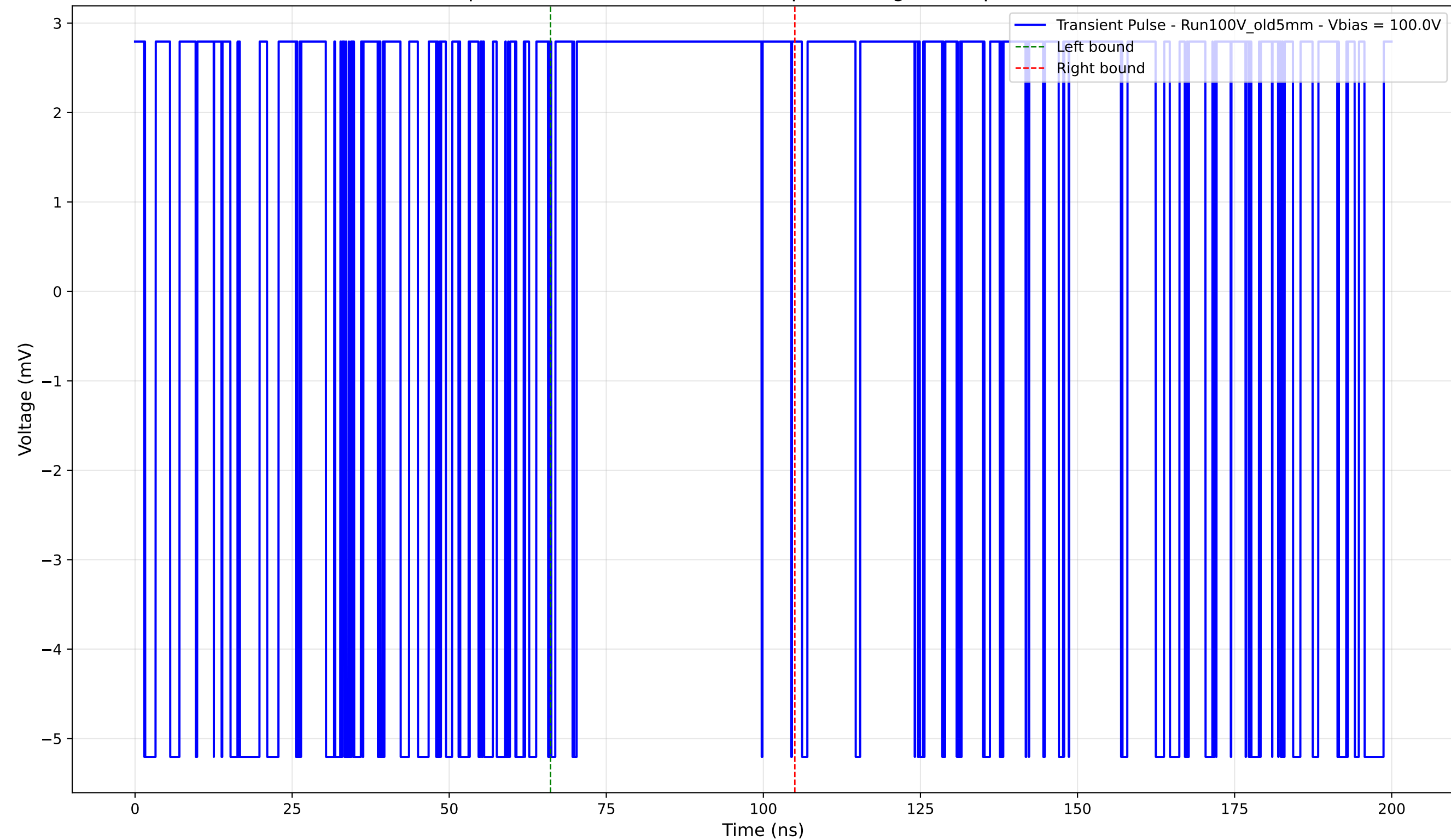
Transient Pulse - Sample: Old5mm - Position: 1335.0 \mu\text{m} - Charge: 1.94 pC - Rise Time: 0.00 ns (N/A)
