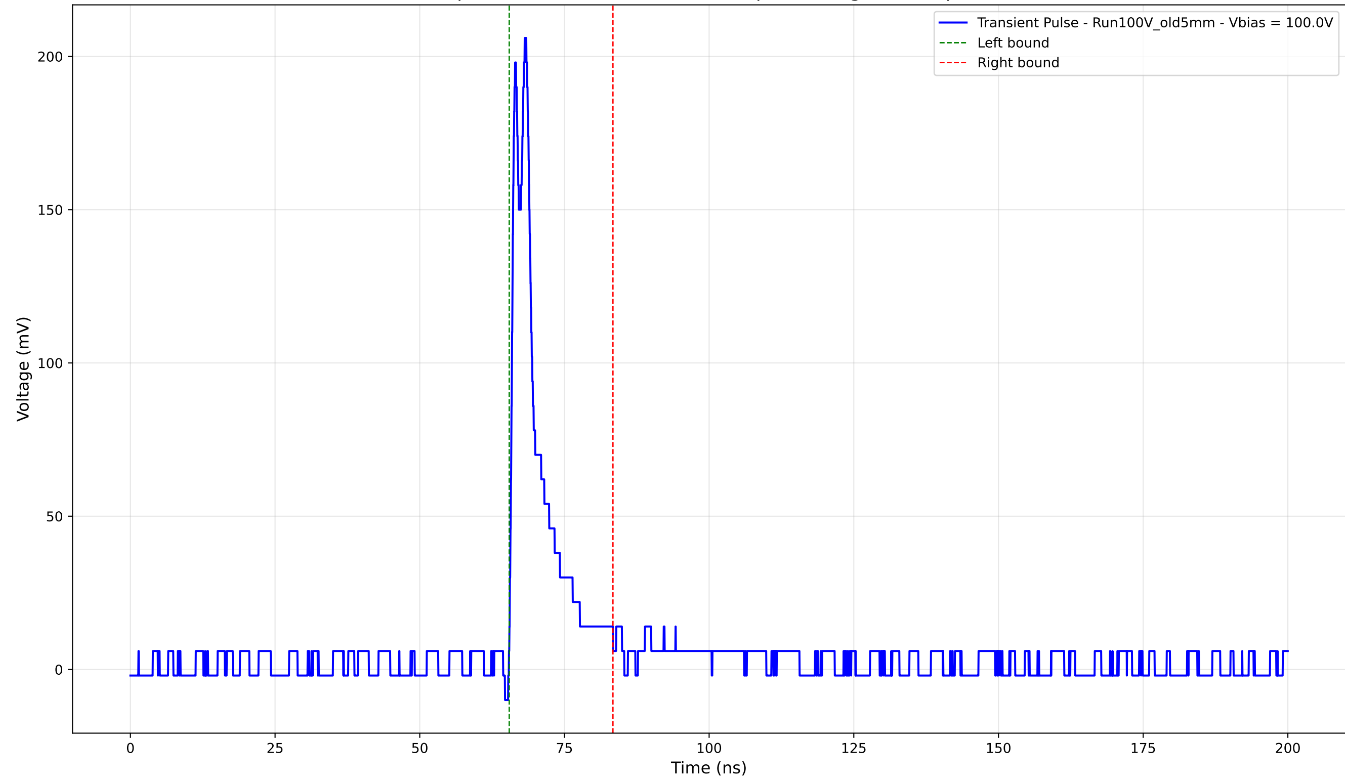
Transient Pulse - Sample: Old5mm - Position: 3565.0 \mu\text{m} - Charge: 21.08 pC - Rise Time: 0.82 ns
