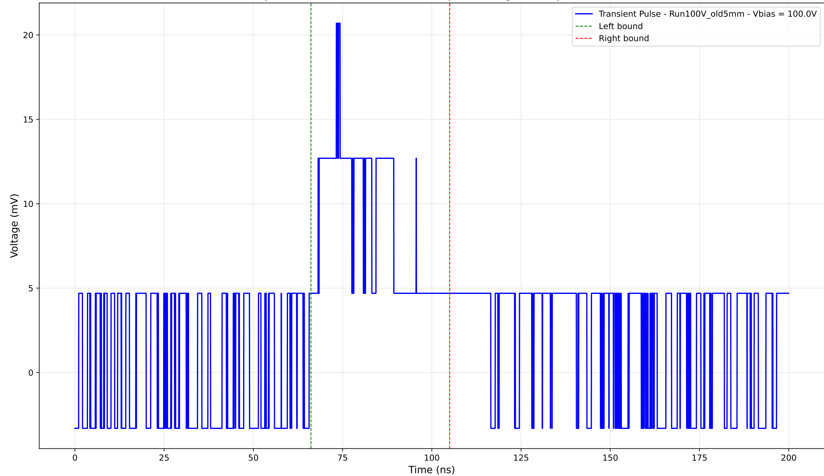
Transient Pulse - Sample: Old5mm - Position: 2480.0 \mu\text{m} - Charge: 6.83 pC - Rise Time: 0.00 ns (N/A)
