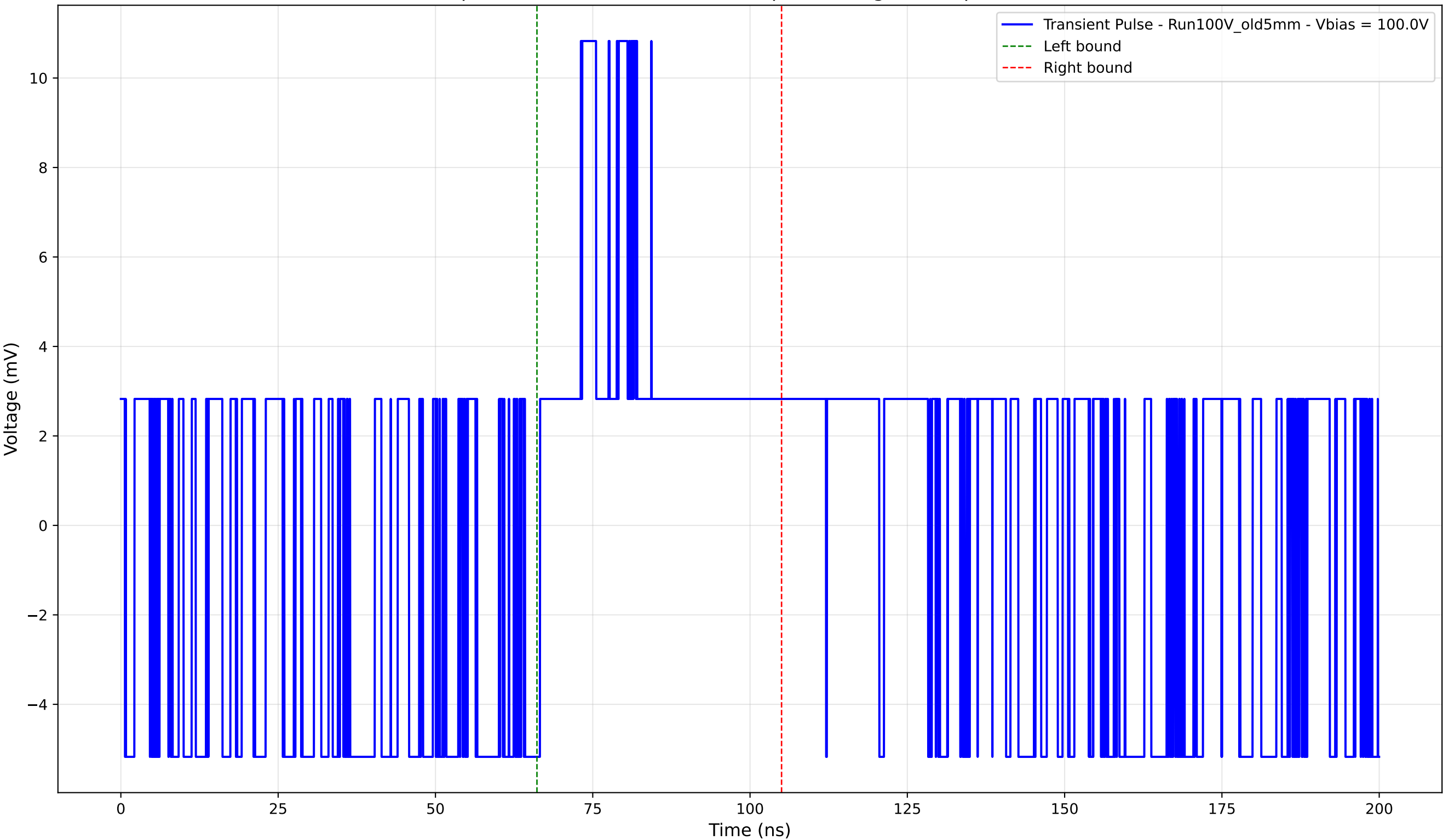
Transient Pulse - Sample: Old5mm - Position: 650.0 \mu\text{m} - Charge: 2.89 pC - Rise Time: 0.00 ns (N/A)
