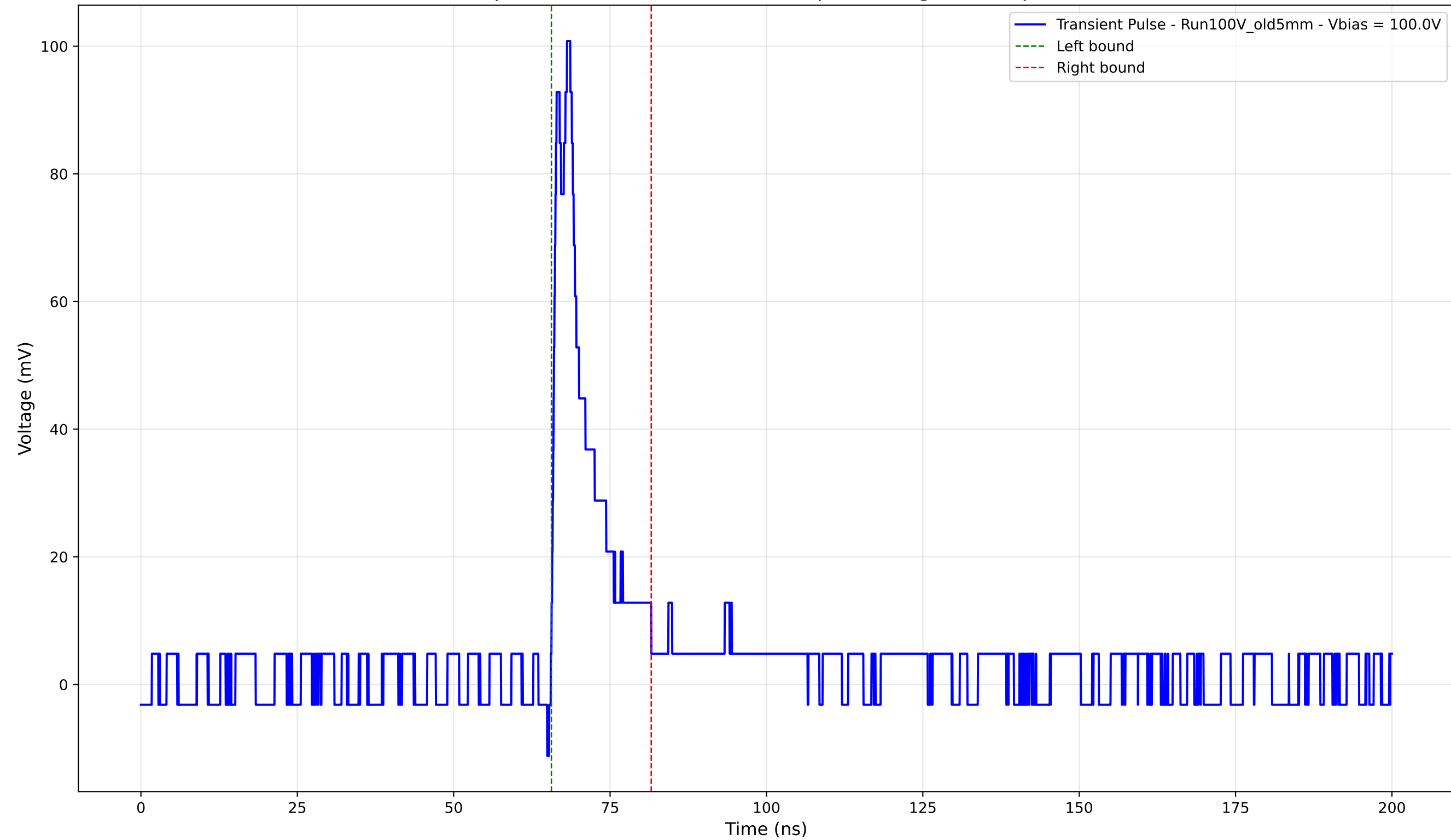
Transient Pulse - Sample: Old5mm - Position: 3935.0 \mu\text{m} - Charge: 11.84 pC - Rise Time: 0.81 ns
