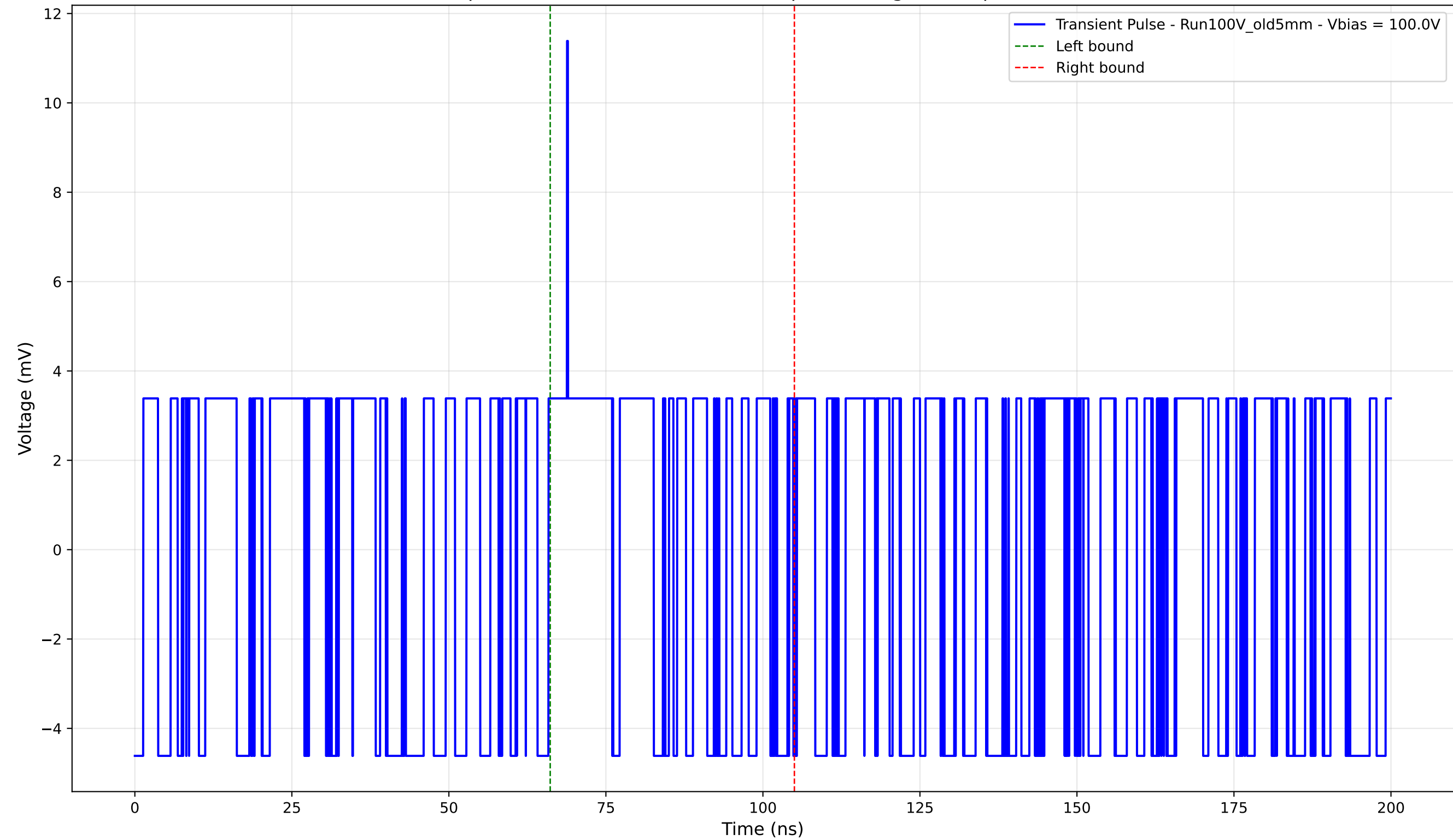
Transient Pulse - Sample: Old5mm - Position: 4340.0 \mu\text{m} - Charge: 0.59 pC - Rise Time: 0.00 ns (N/A)
