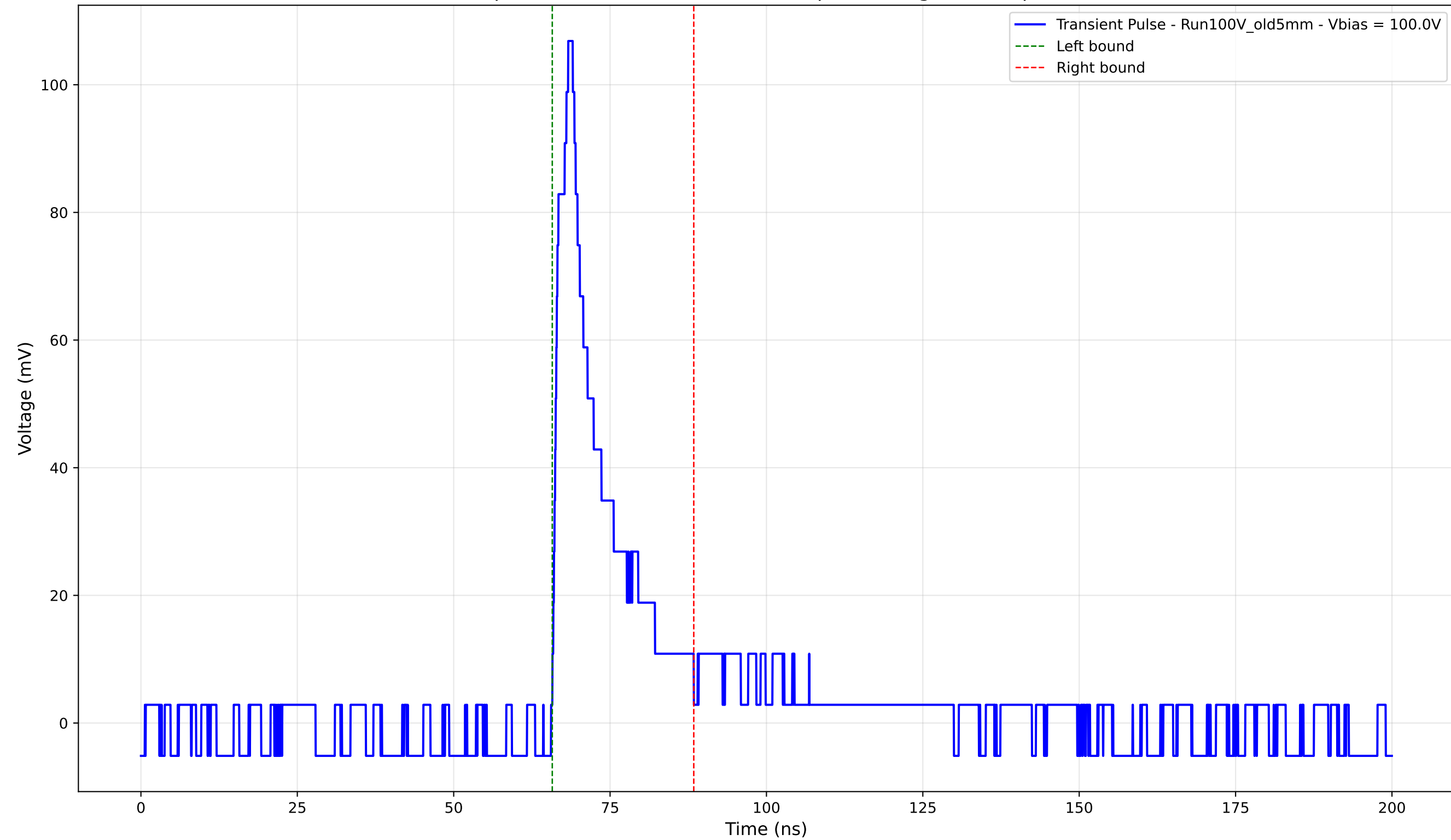
Transient Pulse - Sample: Old5mm - Position: 3235.0 \mu\text{m} - Charge: 16.39 pC - Rise Time: 2.24 ns
