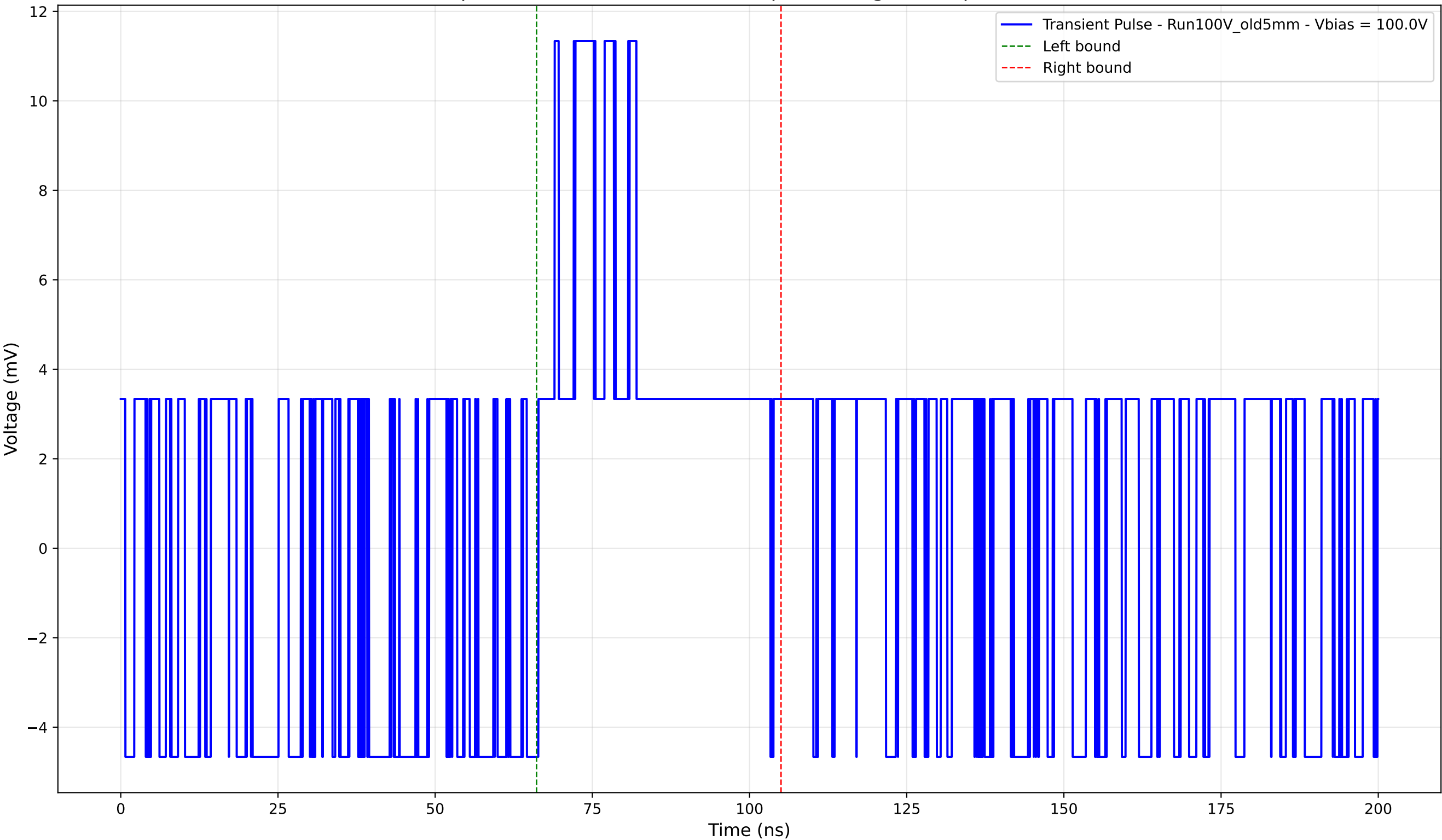
Transient Pulse - Sample: Old5mm - Position: 310.0 \mu\text{m} - Charge: 3.56 pC - Rise Time: 0.00 ns (N/A)
