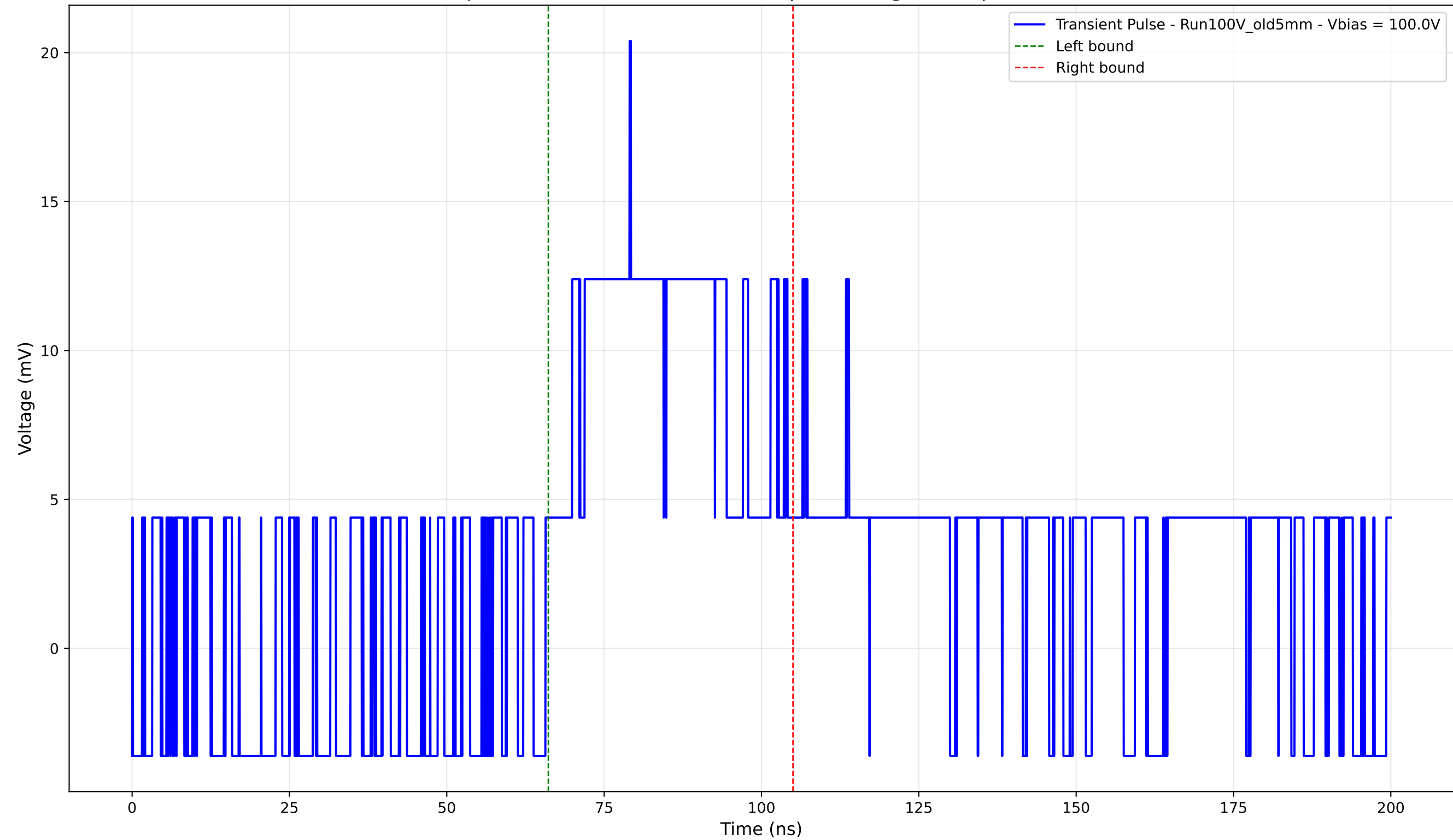
Transient Pulse - Sample: Old5mm - Position: 1240.0 \mu\text{m} - Charge: 7.62 pC - Rise Time: 0.00 ns (N/A)
