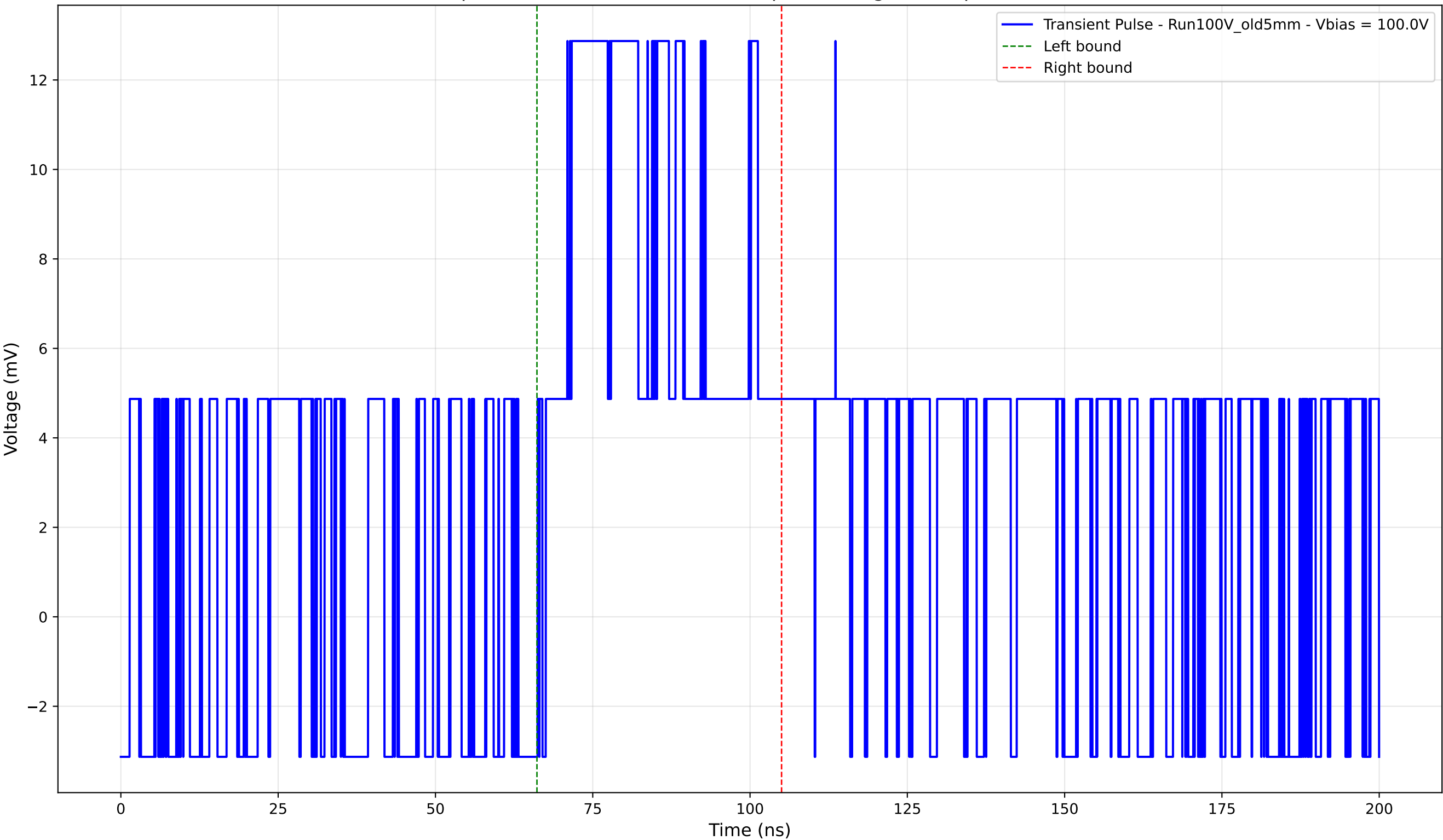
Transient Pulse - Sample: Old5mm - Position: 775.0 \mu\text{m} - Charge: 6.21 pC - Rise Time: 0.00 ns (N/A)
