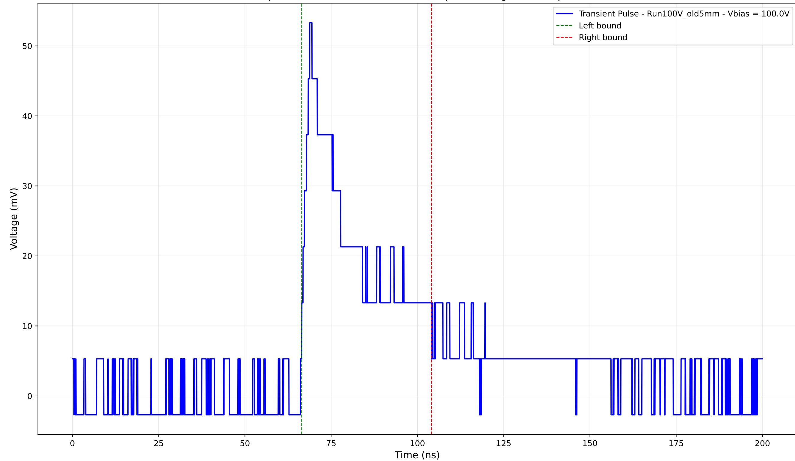
Transient Pulse - Sample: Old5mm - Position: 4735.0 \mu\text{m} - Charge: 16.56 pC - Rise Time: 2.32 ns
