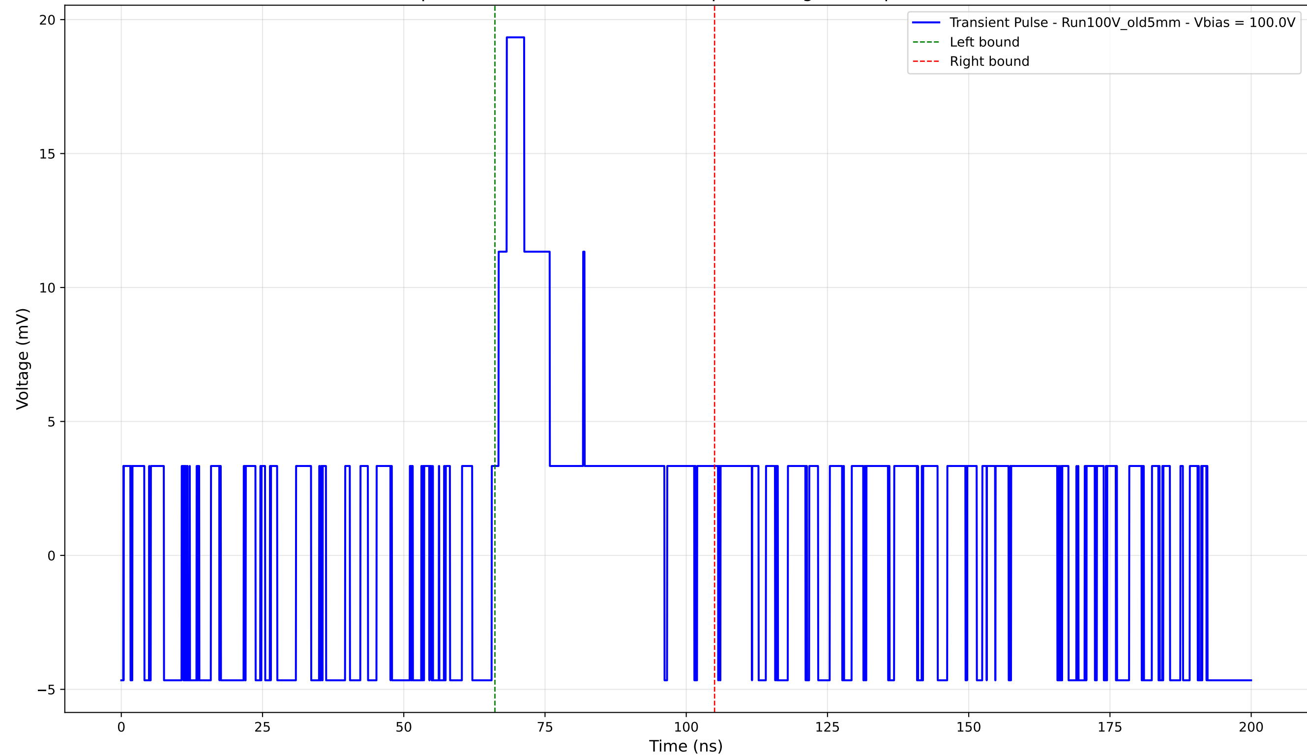
Transient Pulse - Sample: Old5mm - Position: 4560.0 \mu\text{m} - Charge: 4.45 pC - Rise Time: 0.00 ns (N/A)
