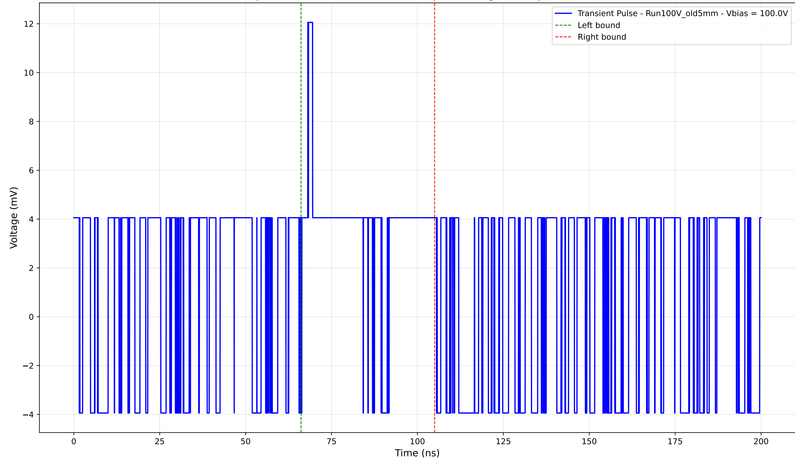
Transient Pulse - Sample: Old5mm - Position: 4335.0 \mu\text{m} - Charge: 2.97 pC - Rise Time: 0.00 ns (N/A)
