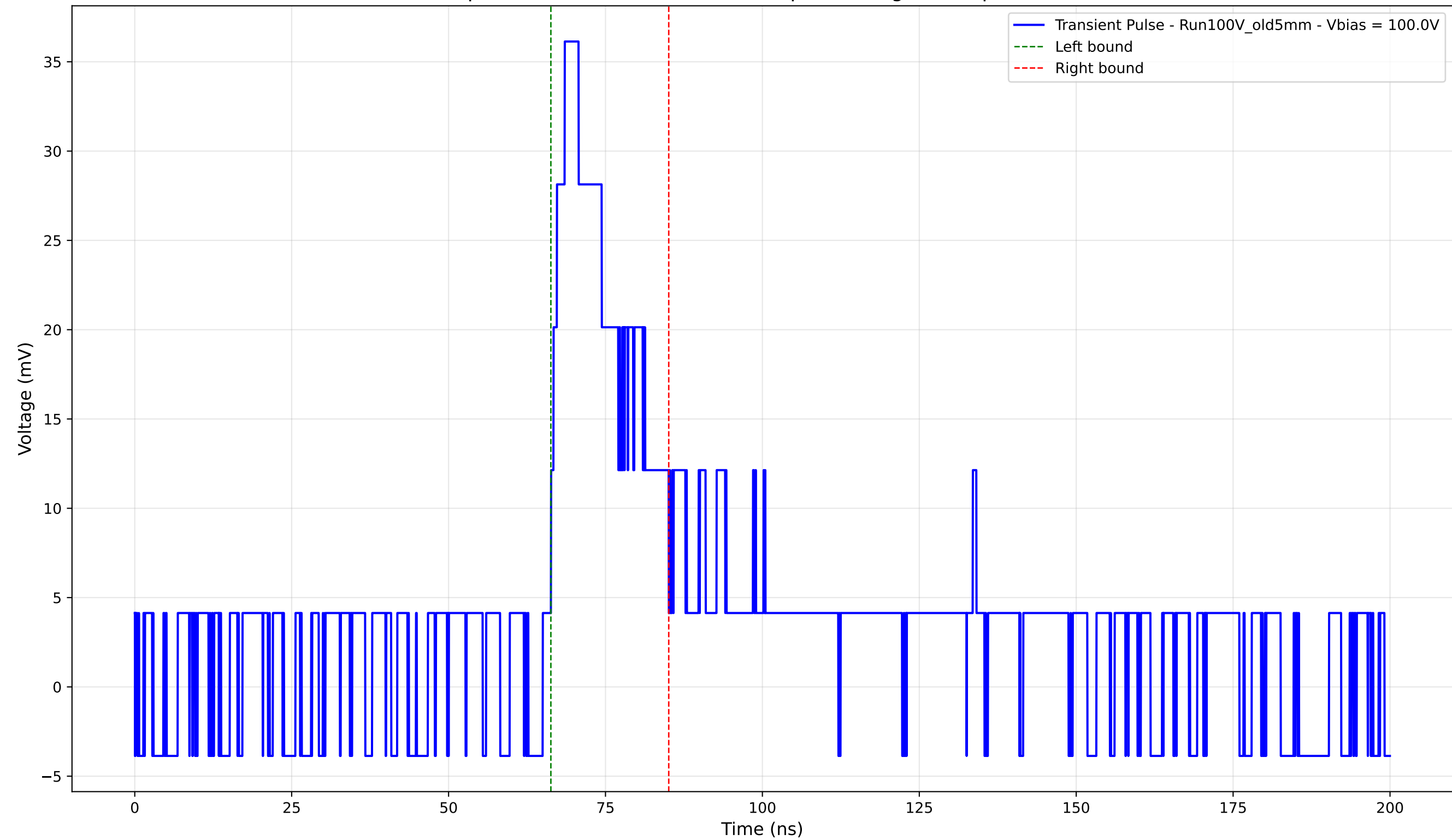
Transient Pulse - Sample: Old5mm - Position: 2880.0 \mu\text{m} - Charge: 8.23 pC - Rise Time: 0.00 ns (N/A)
