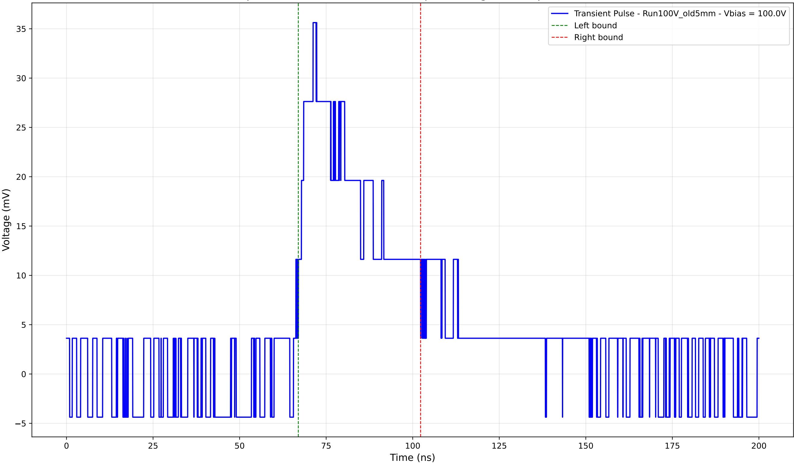
Transient Pulse - Sample: Old5mm - Position: 4975.0 \mu\text{m} - Charge: 13.17 pC - Rise Time: 0.00 ns (N/A)
