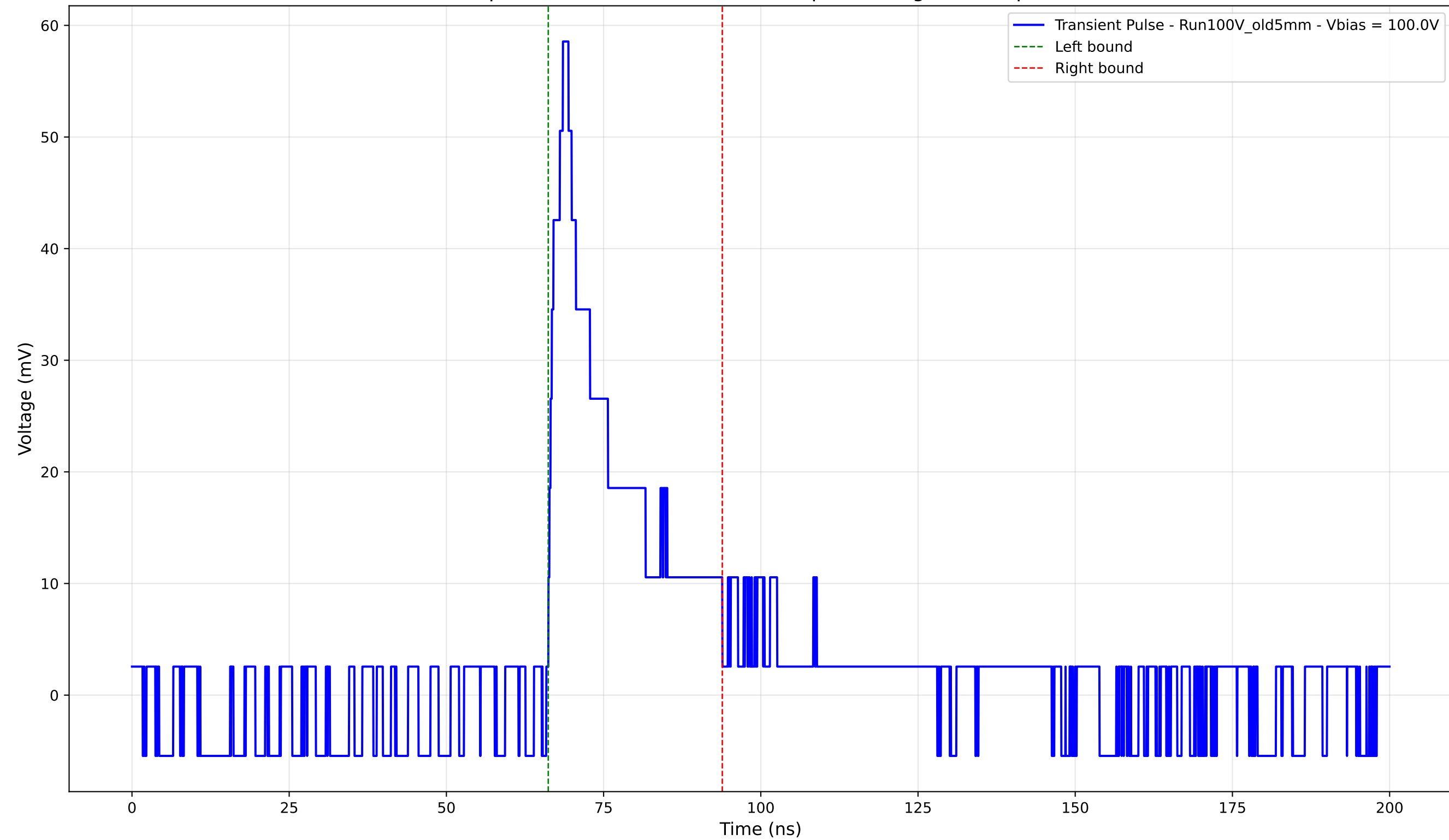
Transient Pulse - Sample: Old5mm - Position: 4405.0 \mu\text{m} - Charge: 11.88 pC - Rise Time: 2.31 ns
