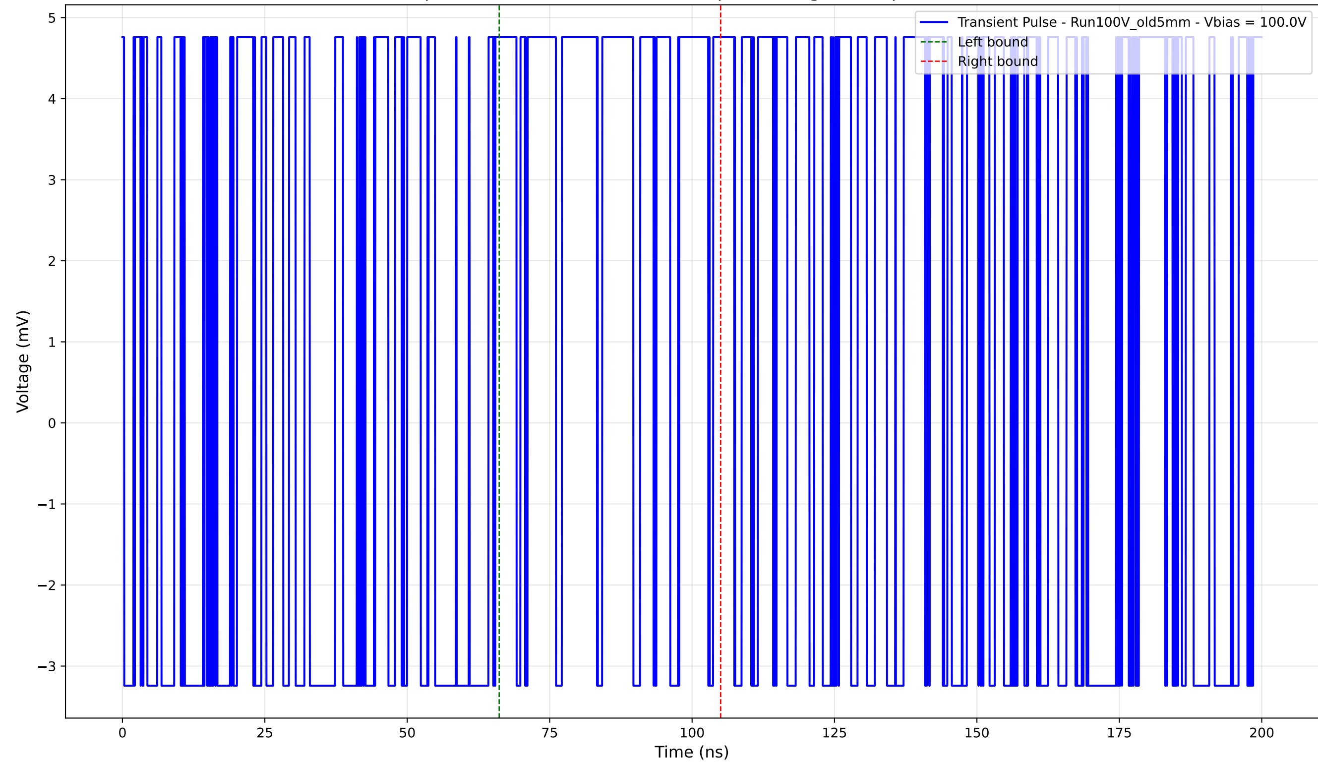
Transient Pulse - Sample: Old5mm - Position: 1325.0 \mu\text{m} - Charge: 2.66 pC - Rise Time: 0.00 ns (N/A)
