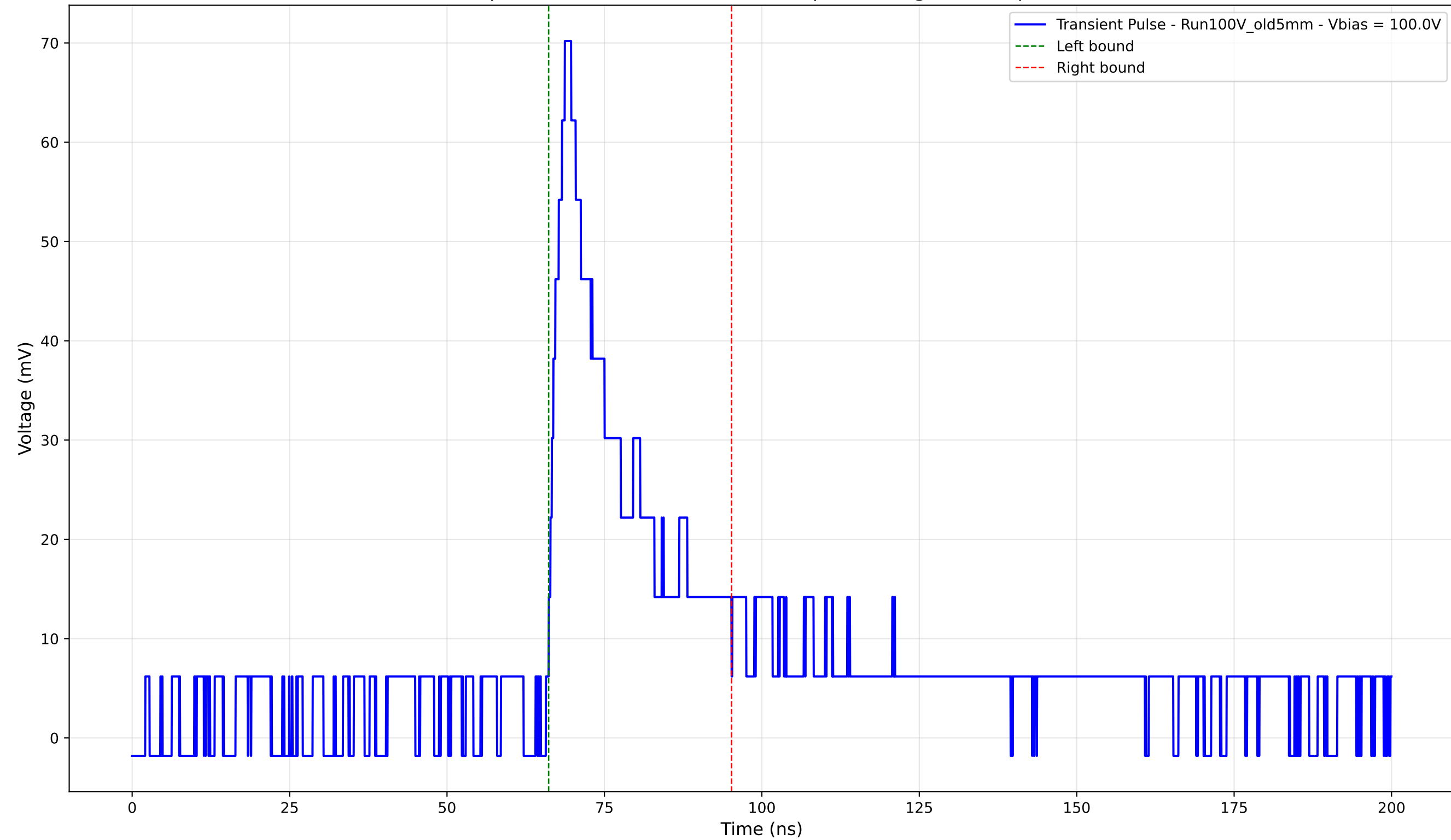
Transient Pulse - Sample: Old5mm - Position: 4490.0 \mu\text{m} - Charge: 16.34 pC - Rise Time: 2.56 ns
