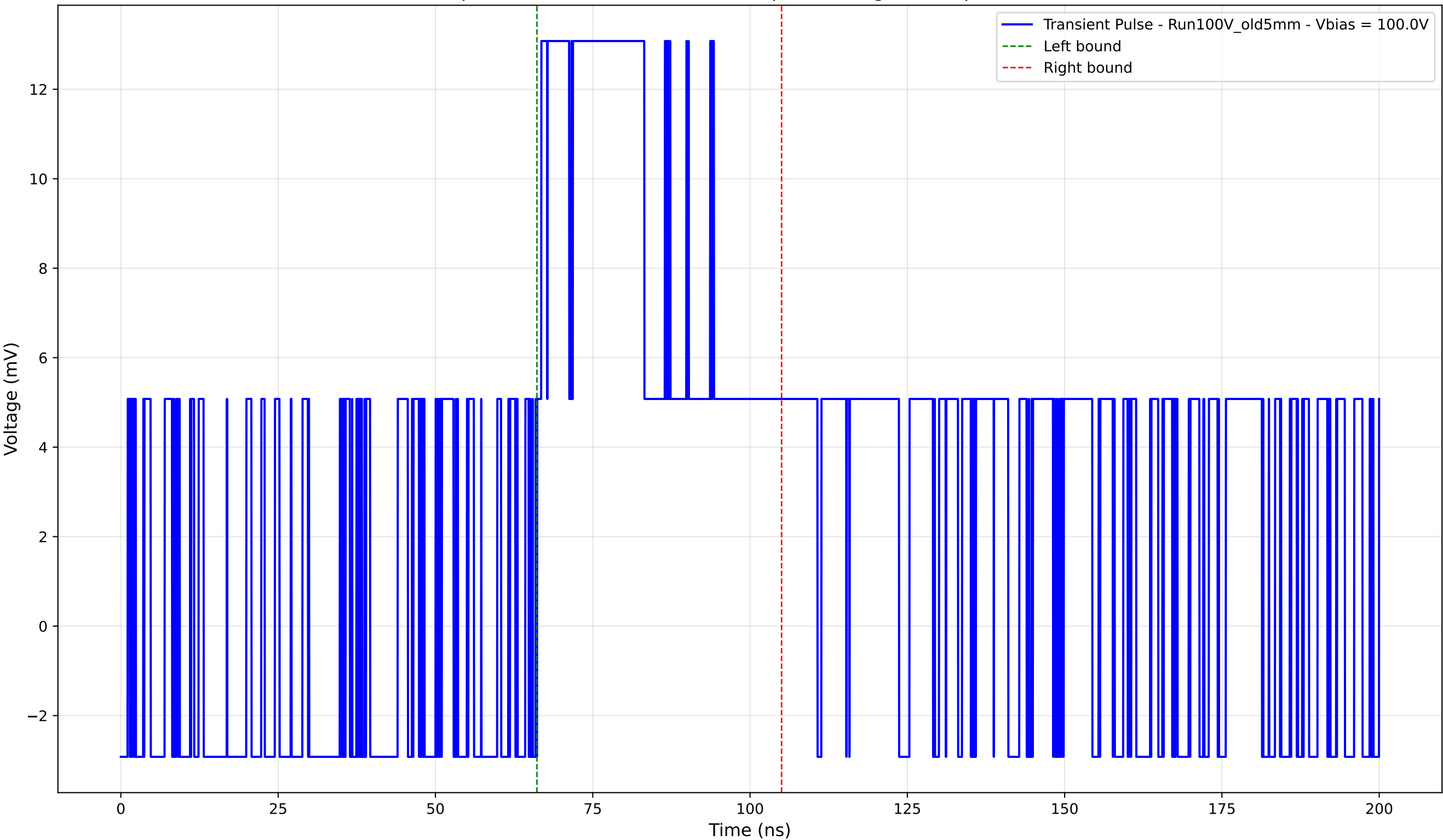
Transient Pulse - Sample: Old5mm - Position: 335.0 \mu\text{m} - Charge: 6.64 pC - Rise Time: 0.00 ns (N/A)
