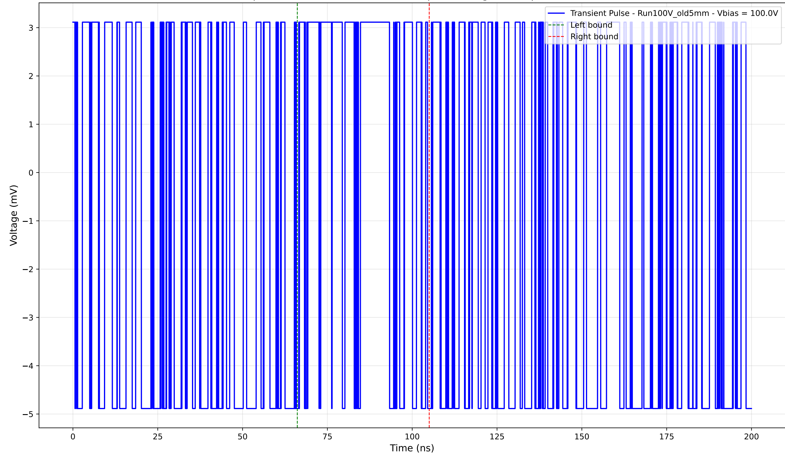
Transient Pulse - Sample: Old5mm - Position: 1310.0 \mu\text{m} - Charge: 0.87 pC - Rise Time: 0.00 ns (N/A)
