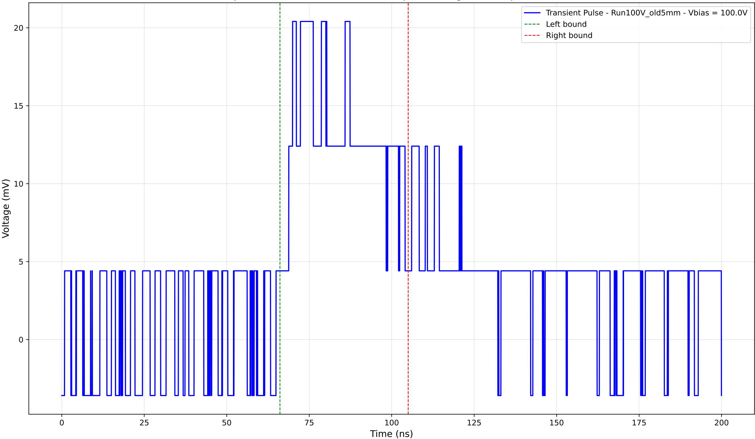
Transient Pulse - Sample: Old5mm - Position: 2180.0 \mu\text{m} - Charge: 10.28 pC - Rise Time: 0.00 ns (N/A)
