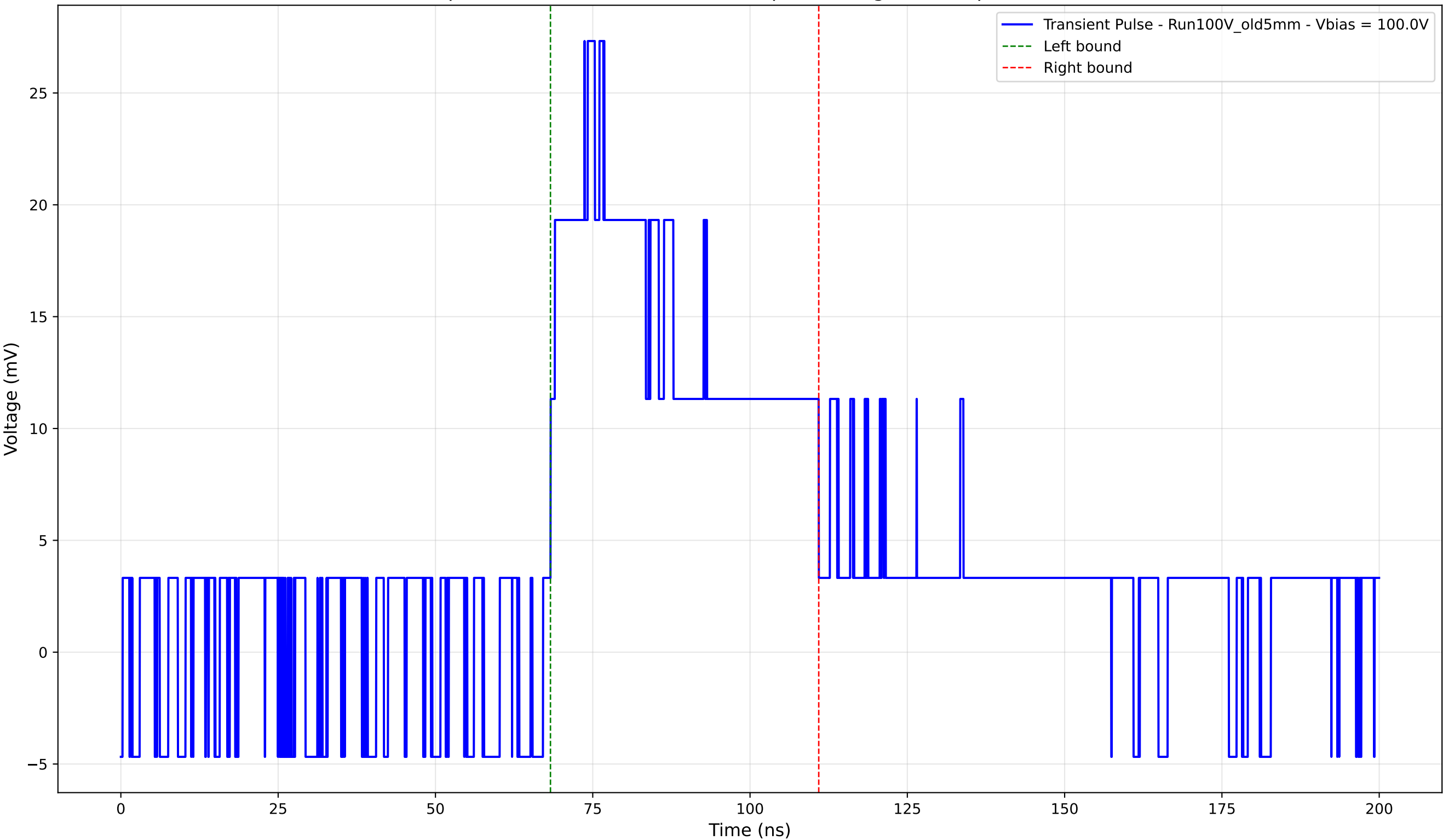
Transient Pulse - Sample: Old5mm - Position: 2220.0 \mu\text{m} - Charge: 12.81 pC - Rise Time: 0.00 ns (N/A)
