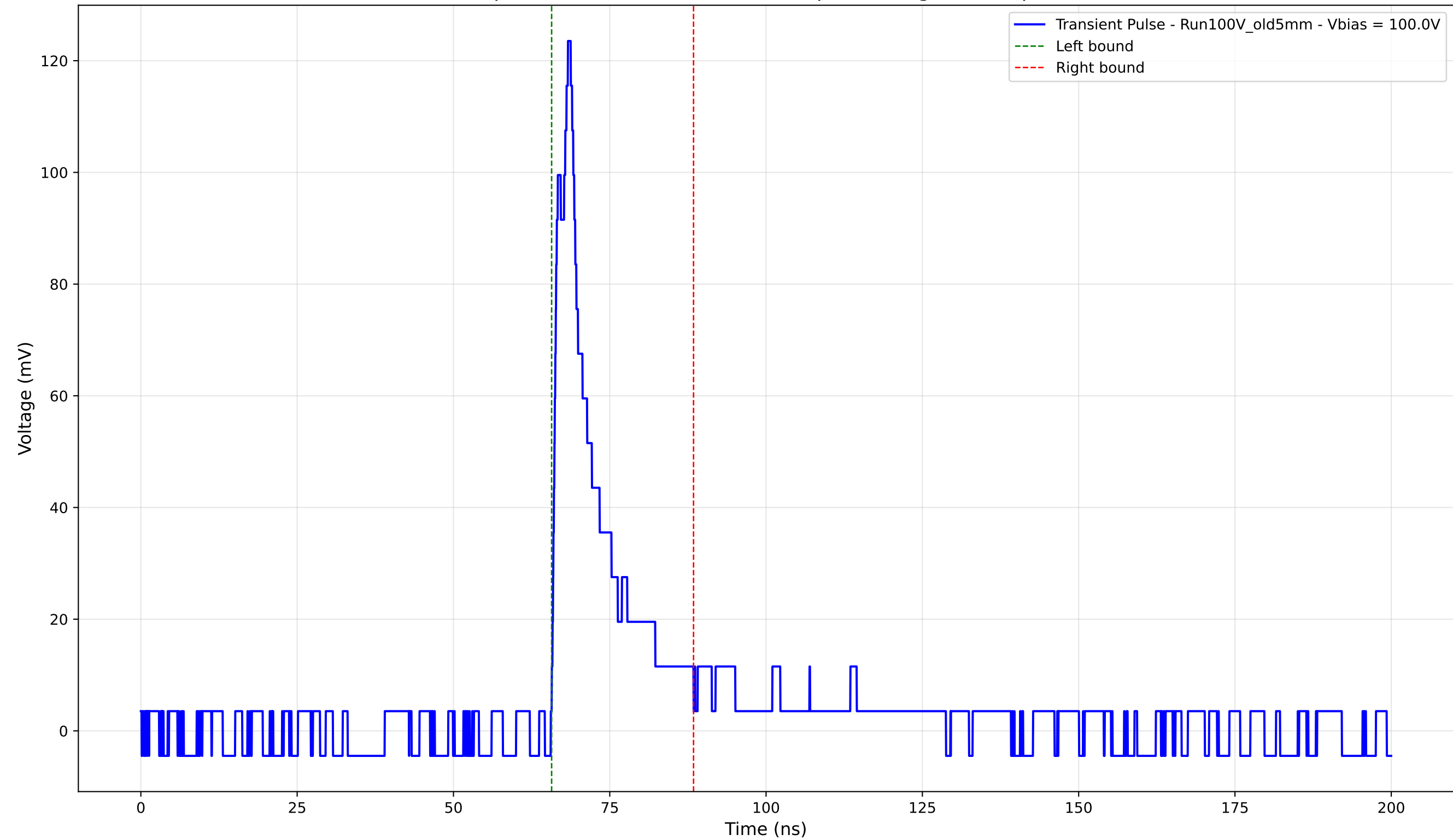
Transient Pulse - Sample: Old5mm - Position: 3285.0 \mu\text{m} - Charge: 17.12 pC - Rise Time: 2.26 ns
