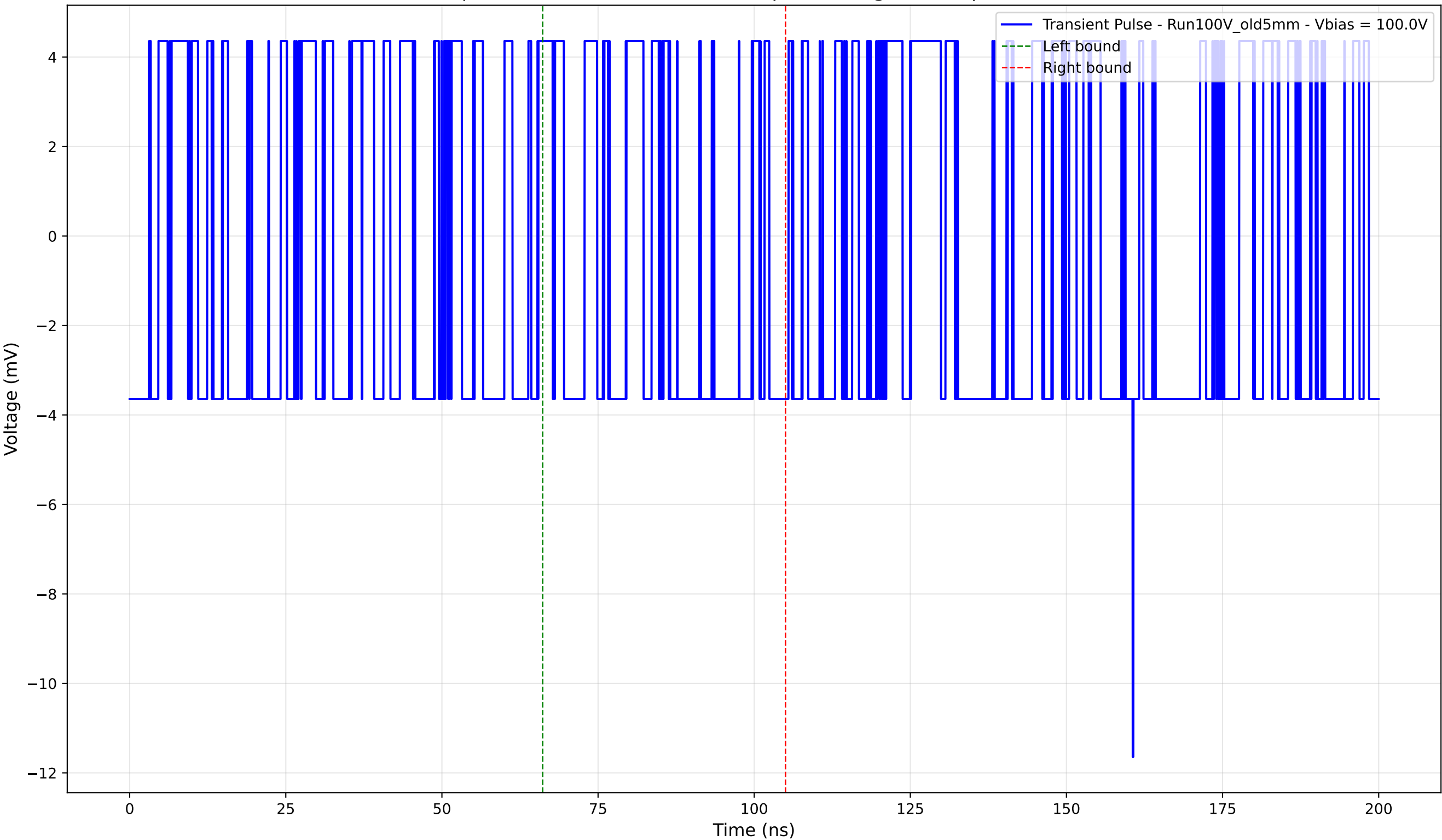
Transient Pulse - Sample: Old5mm - Position: 195.0 \mu\text{m} - Charge: -0.65 pC - Rise Time: 0.00 ns (N/A)
