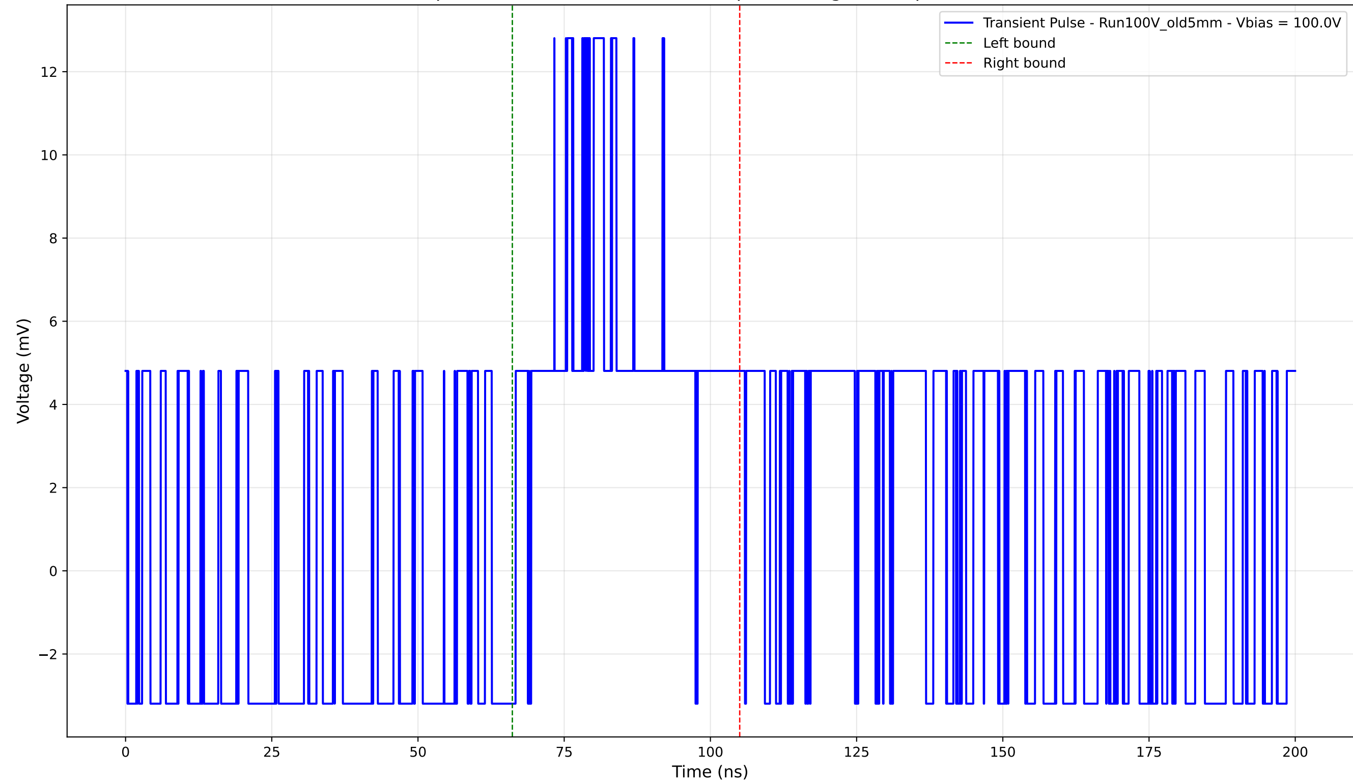
Transient Pulse - Sample: Old5mm - Position: 1010.0 \mu\text{m} - Charge: 4.31 pC - Rise Time: 0.00 ns (N/A)
