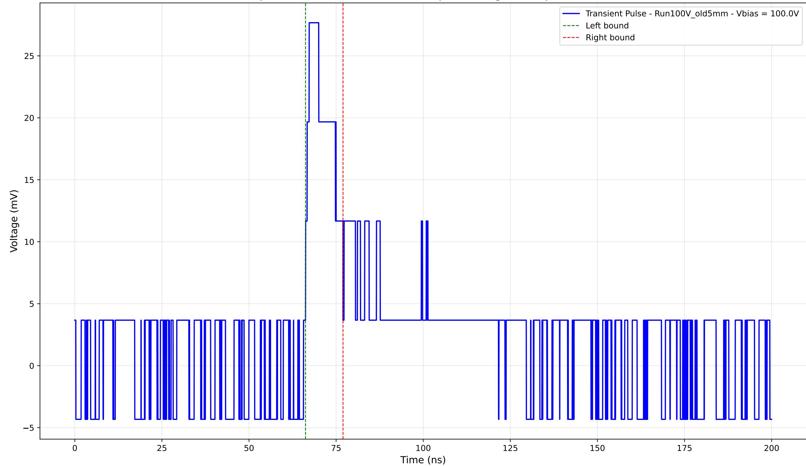
Transient Pulse - Sample: Old5mm - Position: 3040.0 \mu\text{m} - Charge: 4.26 pC - Rise Time: 0.00 ns (N/A)
