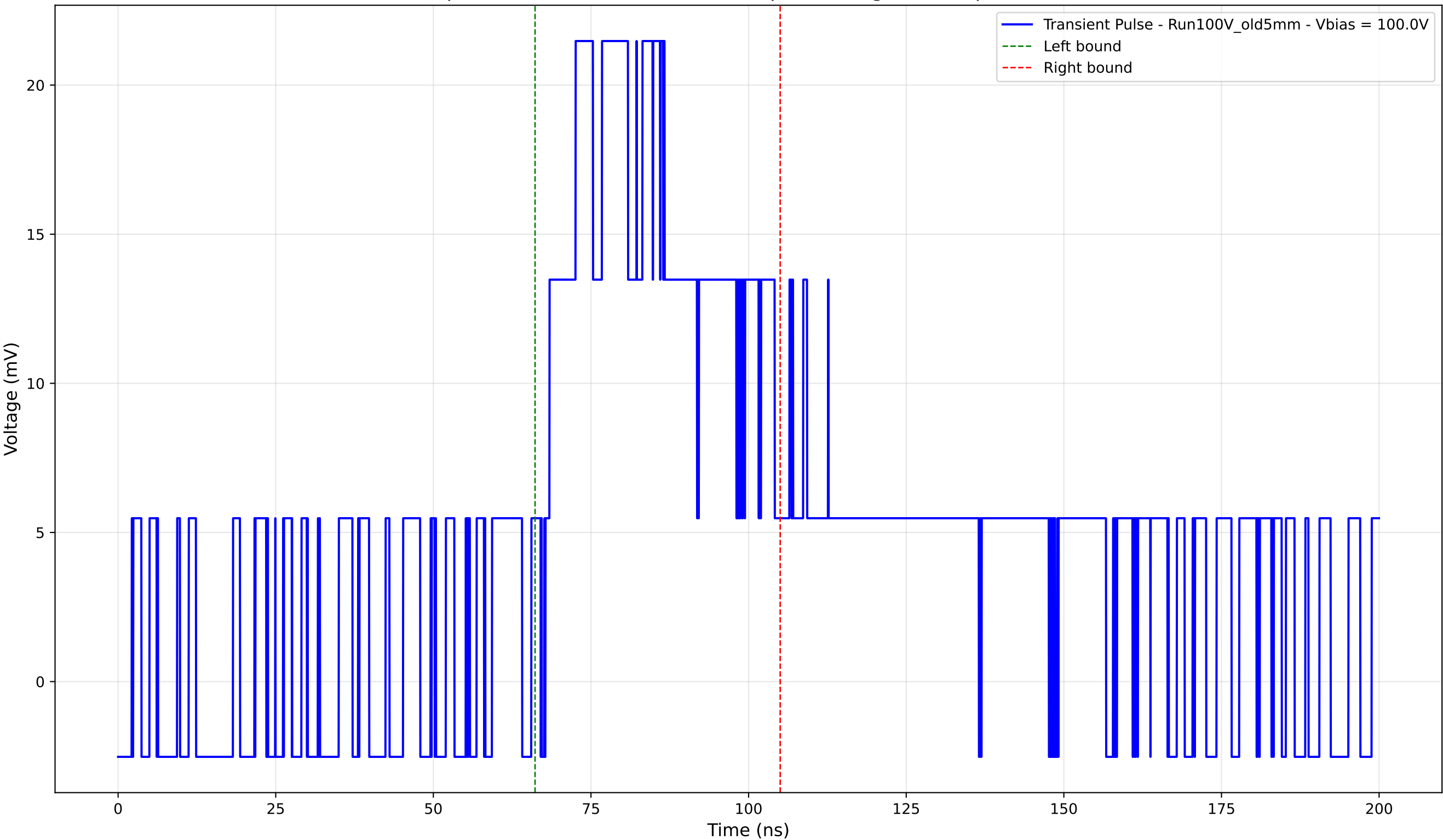
Transient Pulse - Sample: Old5mm - Position: 1795.0 \mu\text{m} - Charge: 11.34 pC - Rise Time: 0.00 ns (N/A)
