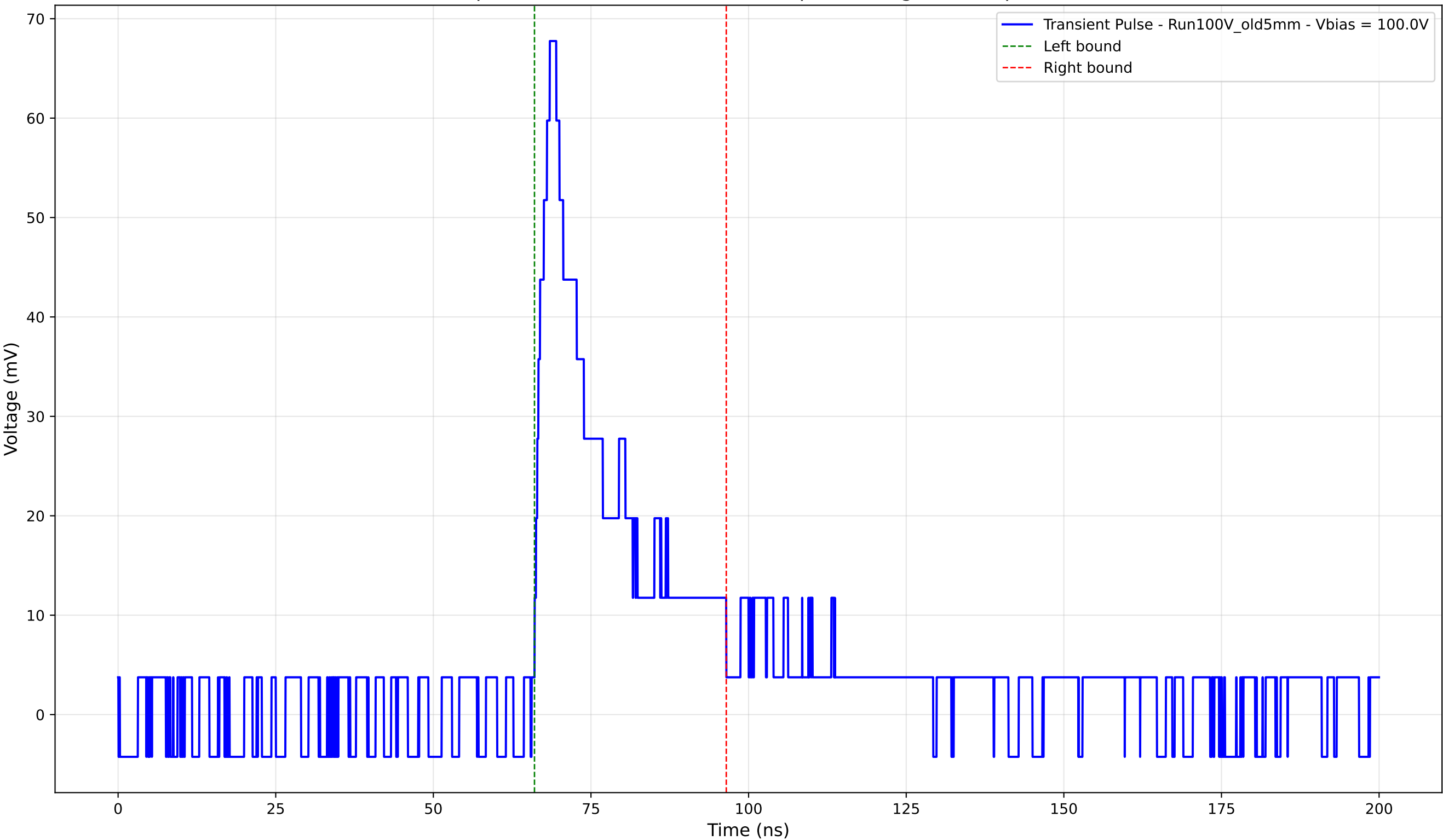
Transient Pulse - Sample: Old5mm - Position: 3000.0 \mu\text{m} - Charge: 14.79 pC - Rise Time: 2.41 ns
