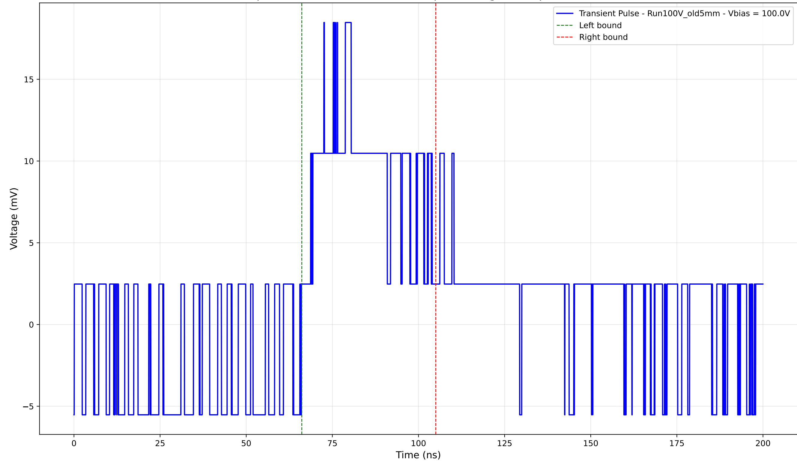
Transient Pulse - Sample: Old5mm - Position: 1975.0 \mu\text{m} - Charge: 7.12 pC - Rise Time: 0.00 ns (N/A)
