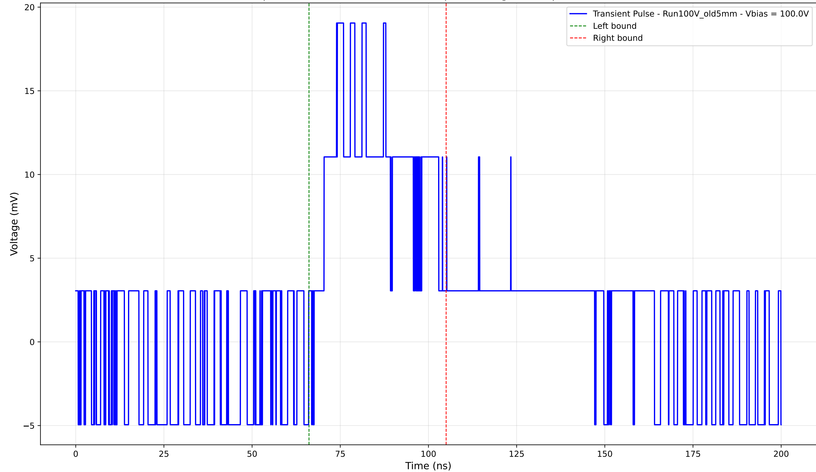
Transient Pulse - Sample: Old5mm - Position: 1415.0 \mu\text{m} - Charge: 8.07 pC - Rise Time: 0.00 ns (N/A)
