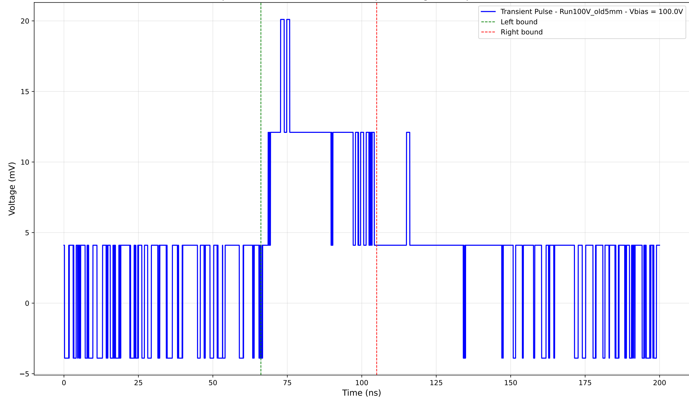
Transient Pulse - Sample: Old5mm - Position: 2170.0 \mu\text{m} - Charge: 8.53 pC - Rise Time: 0.00 ns (N/A)
