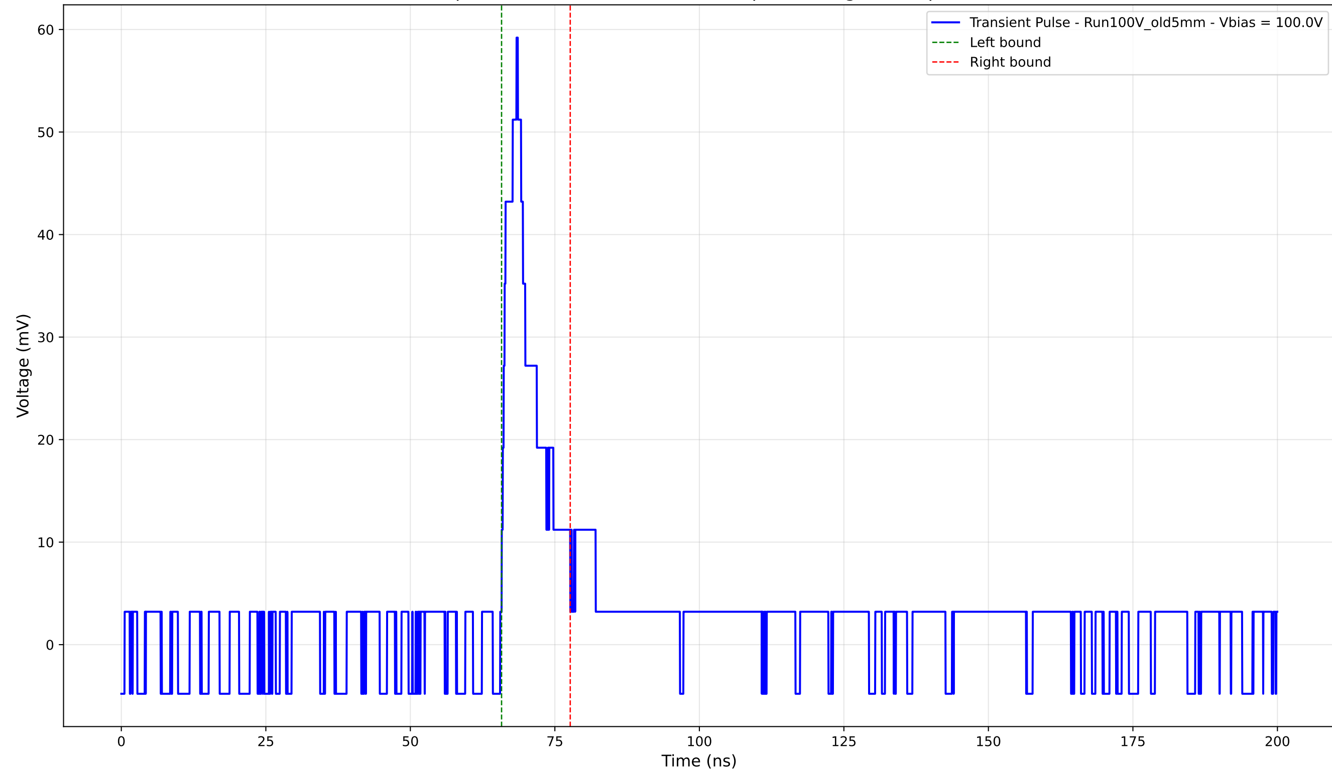
Transient Pulse - Sample: Old5mm - Position: 3340.0 \mu\text{m} - Charge: 6.25 pC - Rise Time: 2.57 ns
