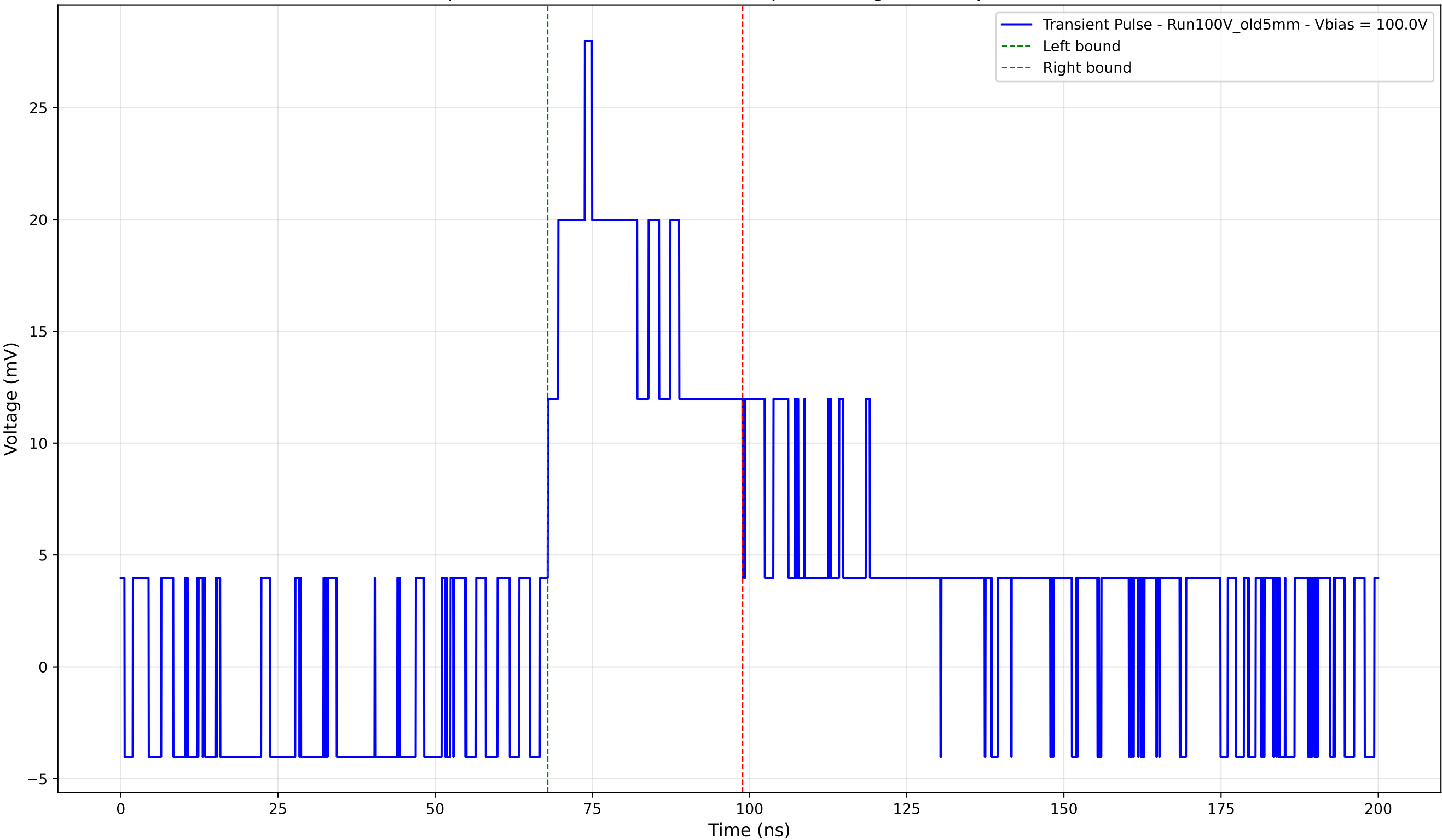
Transient Pulse - Sample: Old5mm - Position: 2200.0 \mu\text{m} - Charge: 10.11 pC - Rise Time: 0.00 ns (N/A)
