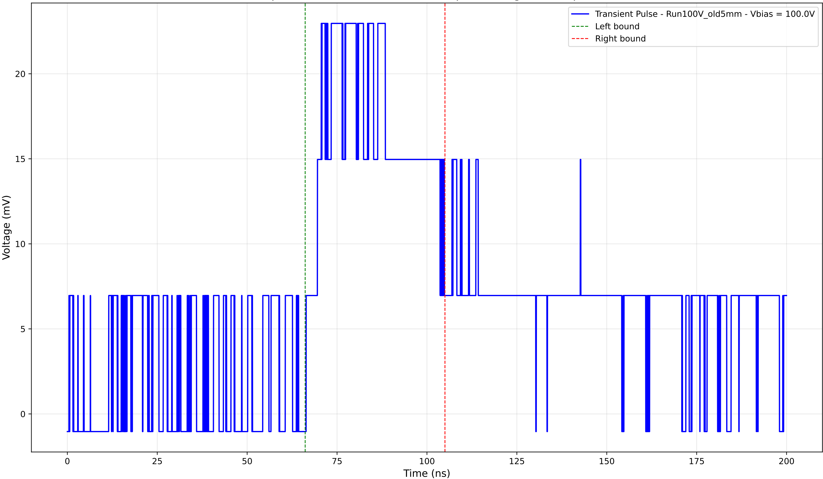
Transient Pulse - Sample: Old5mm - Position: 1810.0 \mu\text{m} - Charge: 12.95 pC - Rise Time: 4.22 ns
