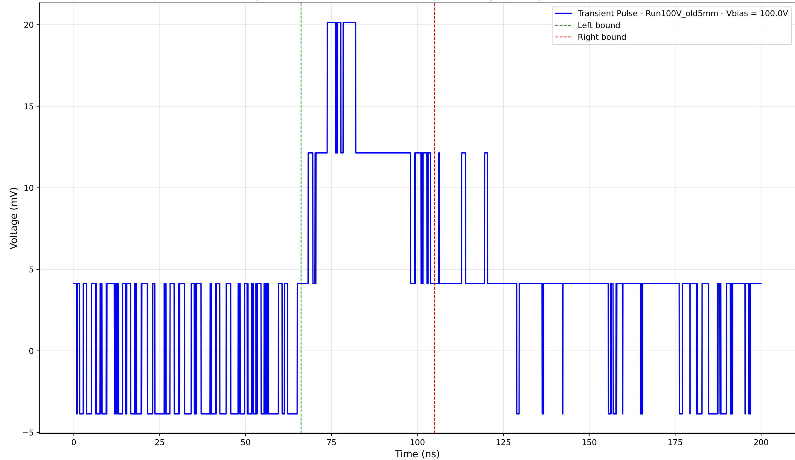
Transient Pulse - Sample: Old5mm - Position: 1790.0 \mu\text{m} - Charge: 9.61 pC - Rise Time: 0.00 ns (N/A)
