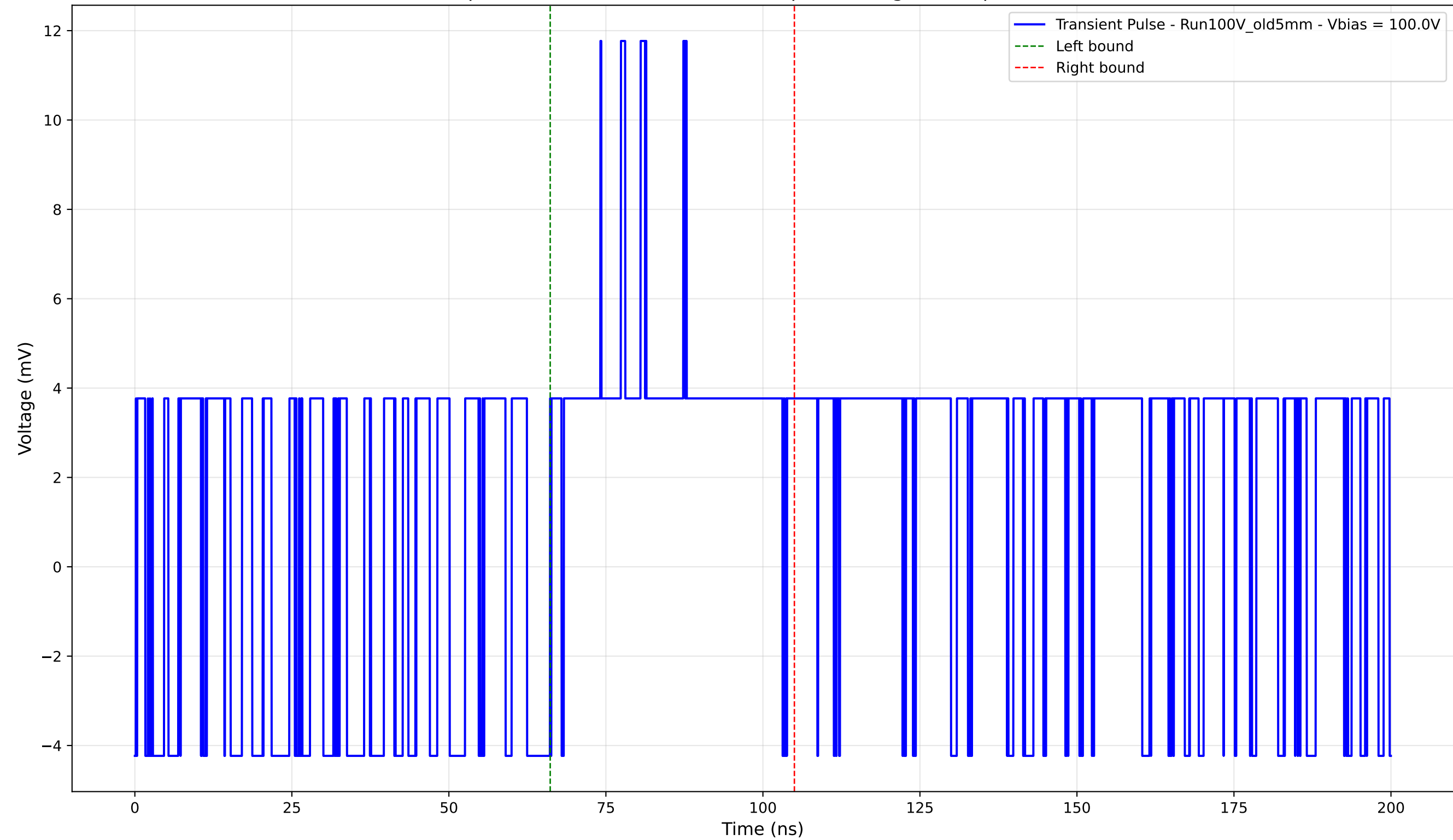
Transient Pulse - Sample: Old5mm - Position: 1540.0 \mu\text{m} - Charge: 3.12 pC - Rise Time: 0.00 ns (N/A)
