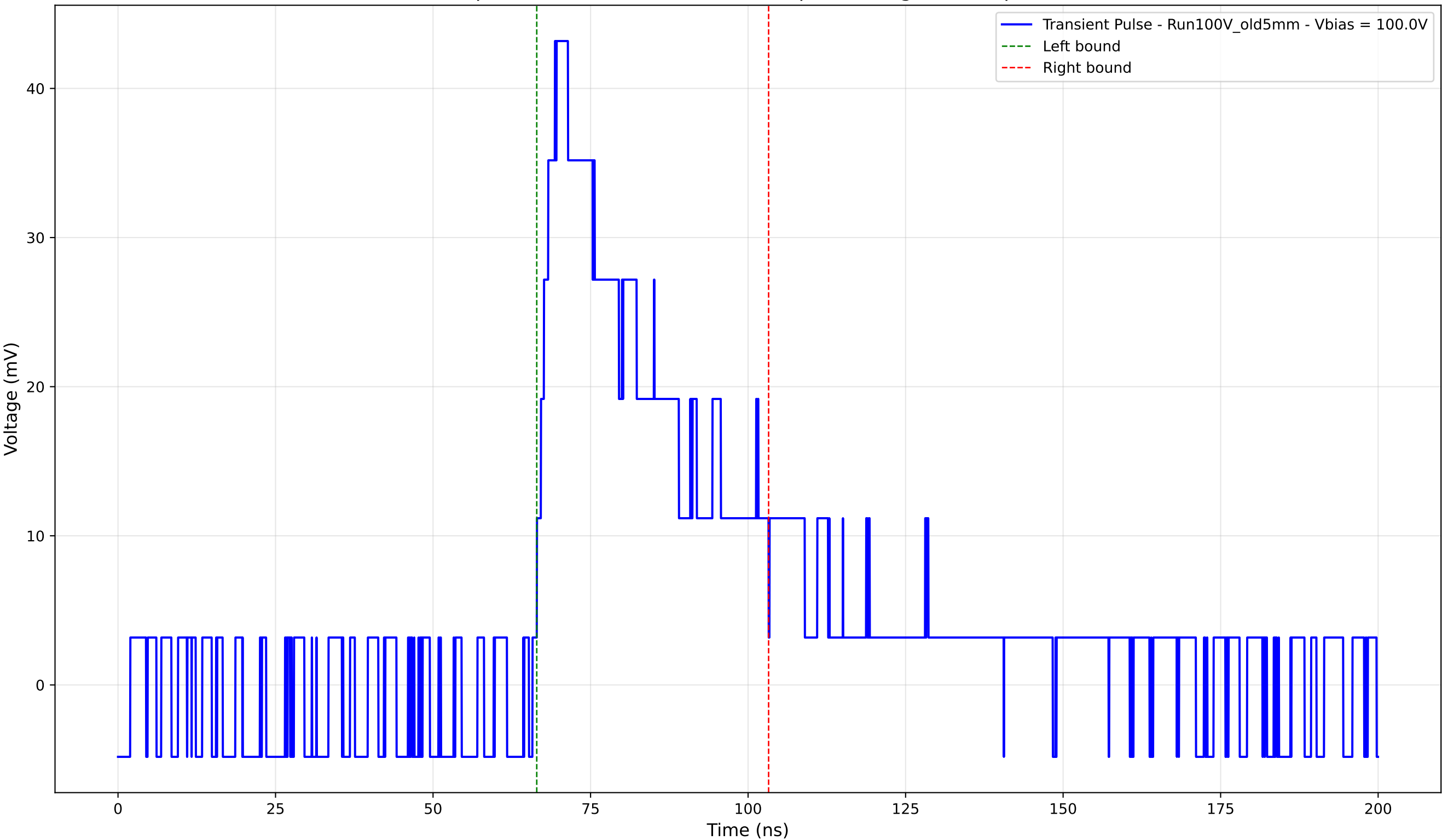
Transient Pulse - Sample: Old5mm - Position: 4895.0 \mu\text{m} - Charge: 15.85 pC - Rise Time: 2.88 ns
