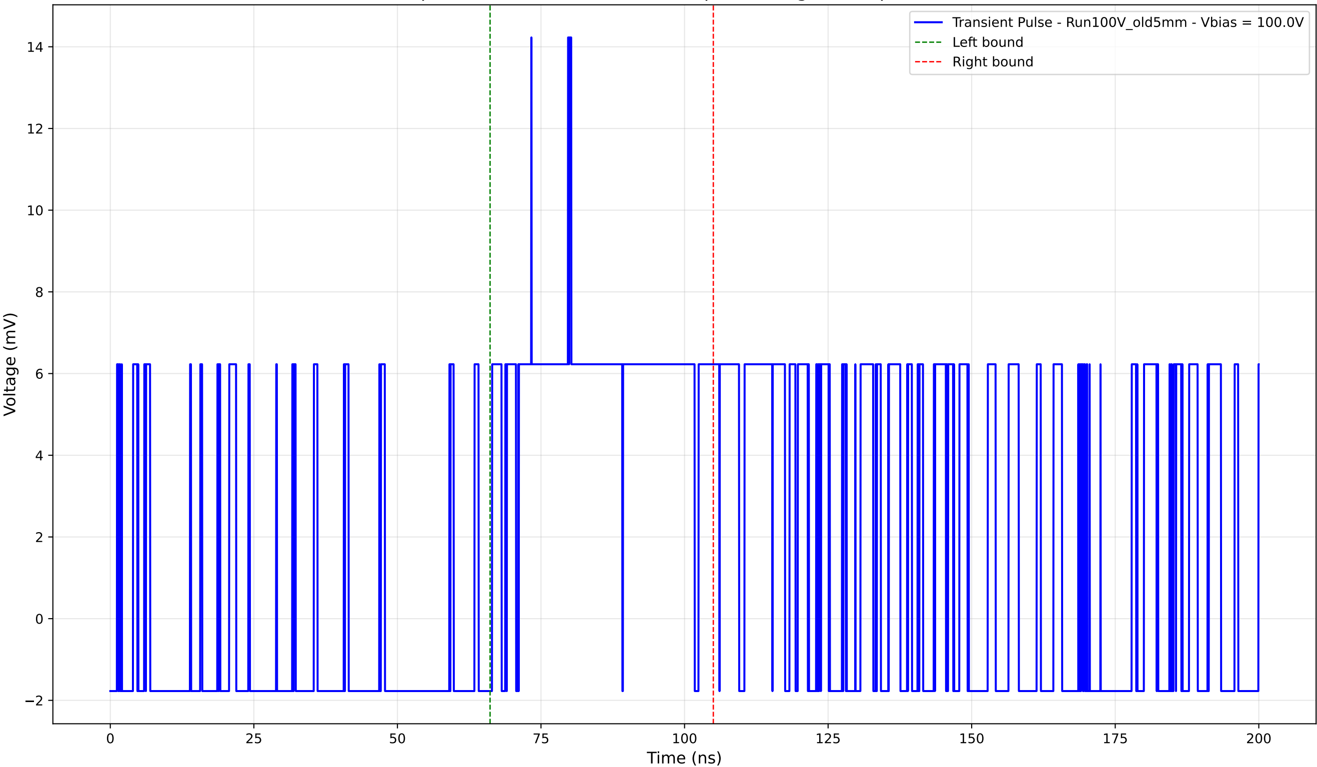
Transient Pulse - Sample: Old5mm - Position: 520.0 \mu\text{m} - Charge: 4.58 pC - Rise Time: 0.00 ns (N/A)
