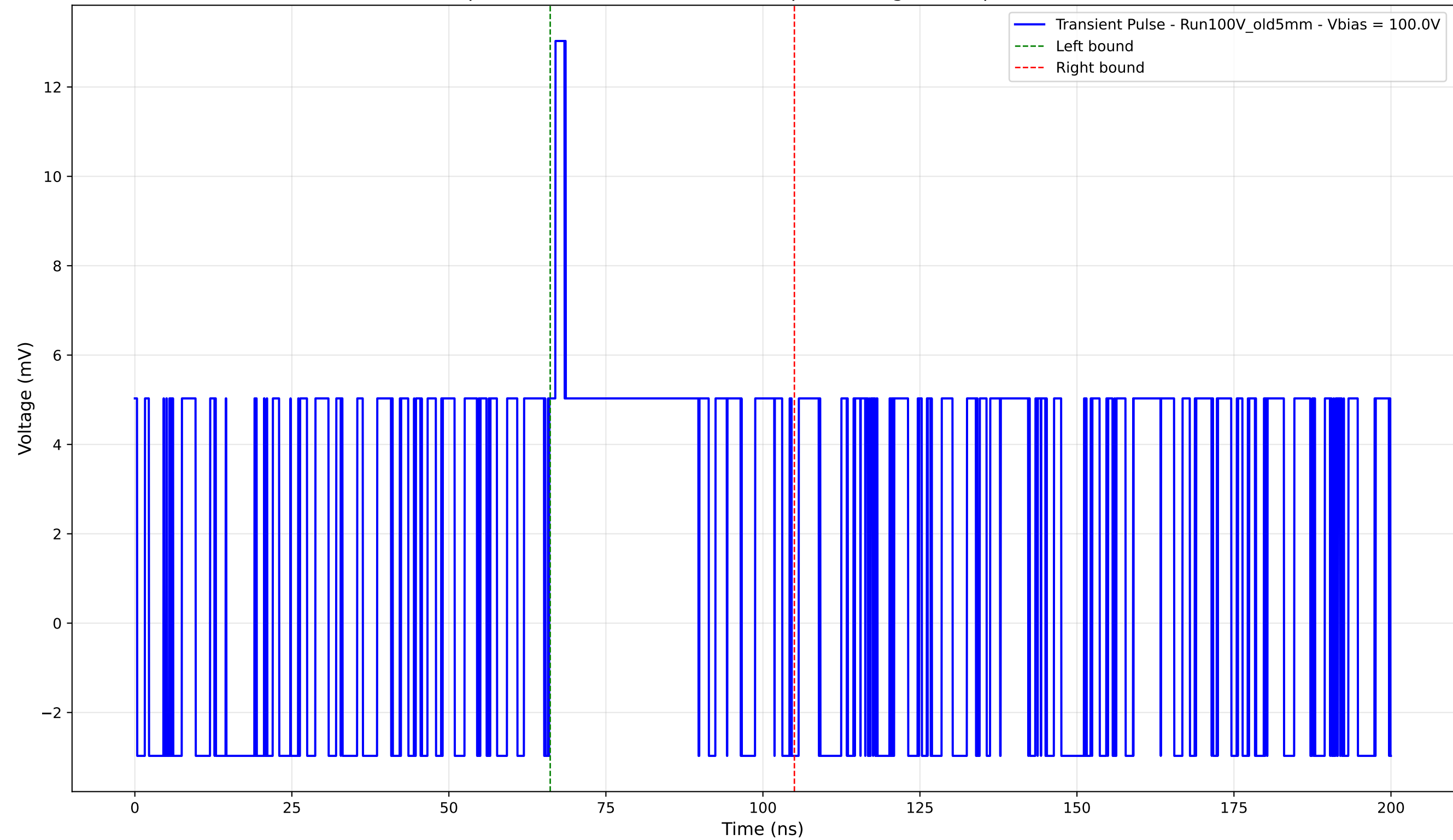
Transient Pulse - Sample: Old5mm - Position: 3070.0 \mu\text{m} - Charge: 3.33 pC - Rise Time: 0.00 ns (N/A)
