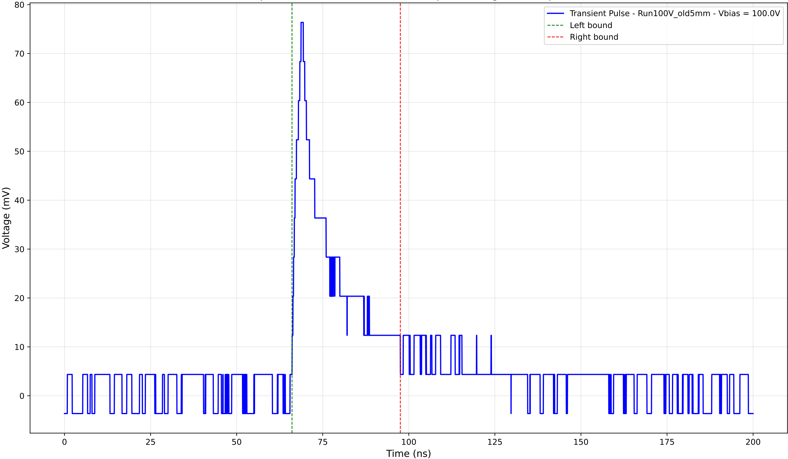
Transient Pulse - Sample: Old5mm - Position: 2960.0 \mu\text{m} - Charge: 16.91 pC - Rise Time: 2.61 ns
