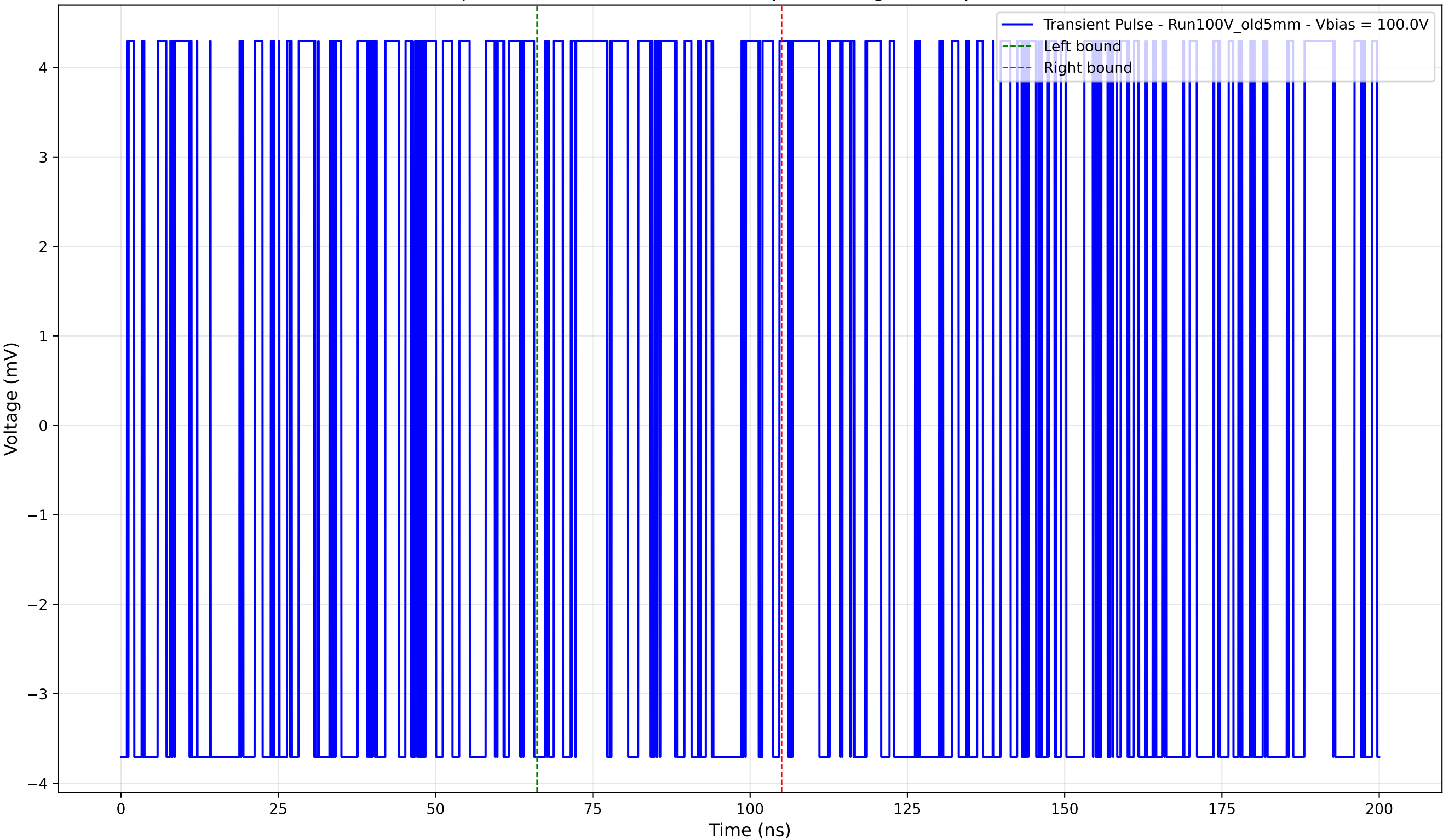
Transient Pulse - Sample: Old5mm - Position: 235.0 \mu\text{m} - Charge: 0.70 pC - Rise Time: 0.00 ns (N/A)
