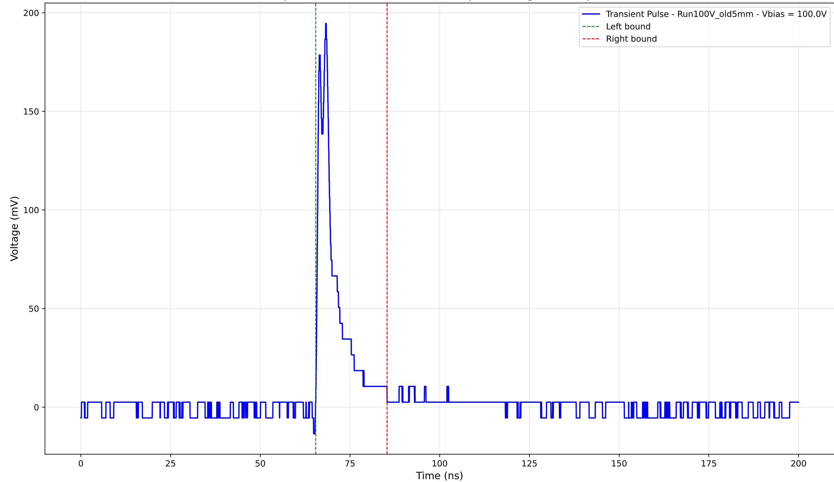
Transient Pulse - Sample: Old5mm - Position: 3865.0 \mu\text{m} - Charge: 20.01 pC - Rise Time: 0.84 ns
