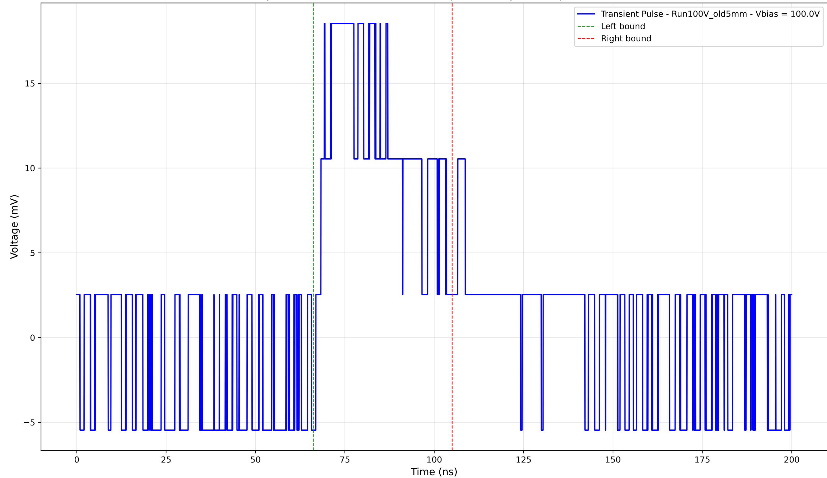
Transient Pulse - Sample: Old5mm - Position: 2250.0 \mu\text{m} - Charge: 8.80 pC - Rise Time: 0.00 ns (N/A)
