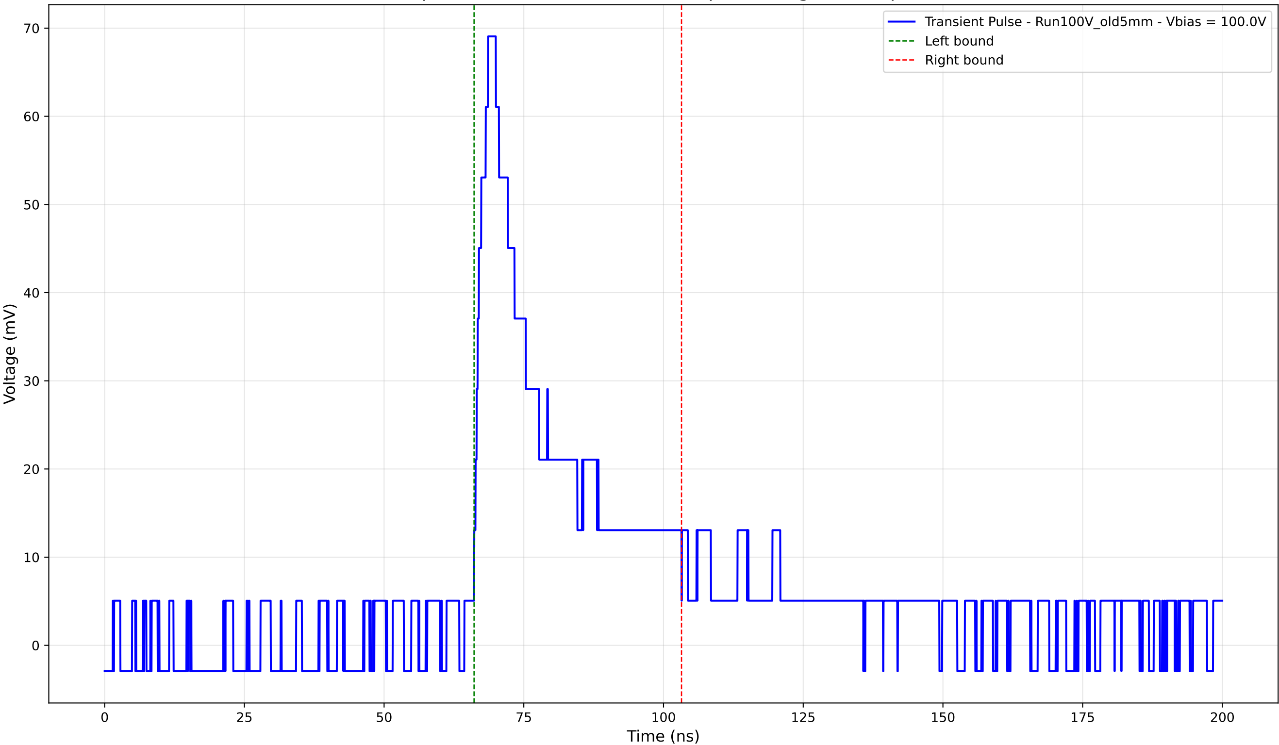
Transient Pulse - Sample: Old5mm - Position: 2940.0 \mu\text{m} - Charge: 18.64 pC - Rise Time: 2.50 ns
