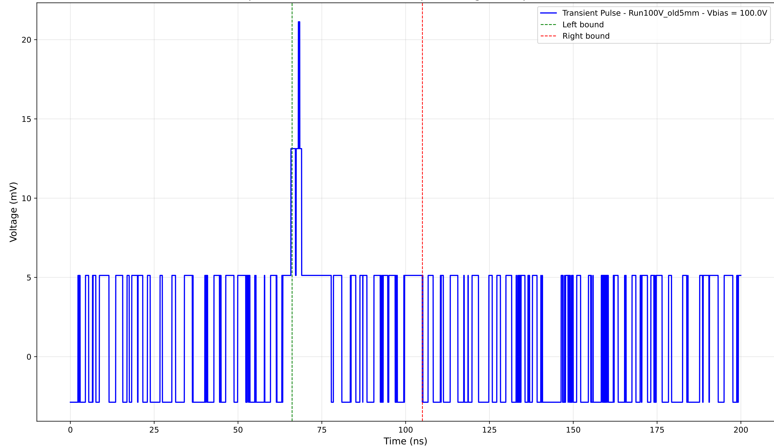
Transient Pulse - Sample: Old5mm - Position: 3685.0 \mu\text{m} - Charge: 2.90 pC - Rise Time: 0.00 ns (N/A)
