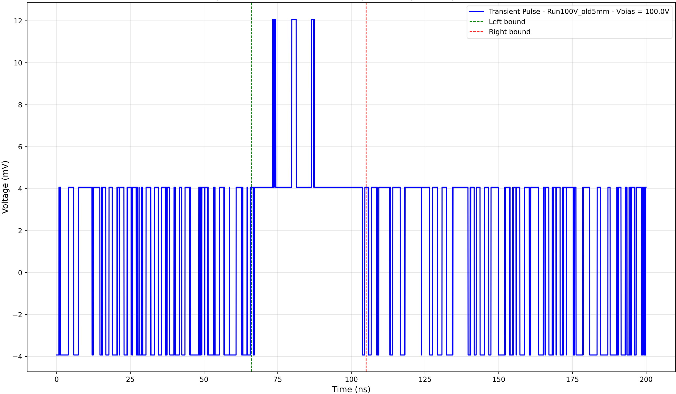
Transient Pulse - Sample: Old5mm - Position: 820.0 \mu\text{m} - Charge: 3.48 pC - Rise Time: 0.00 ns (N/A)
