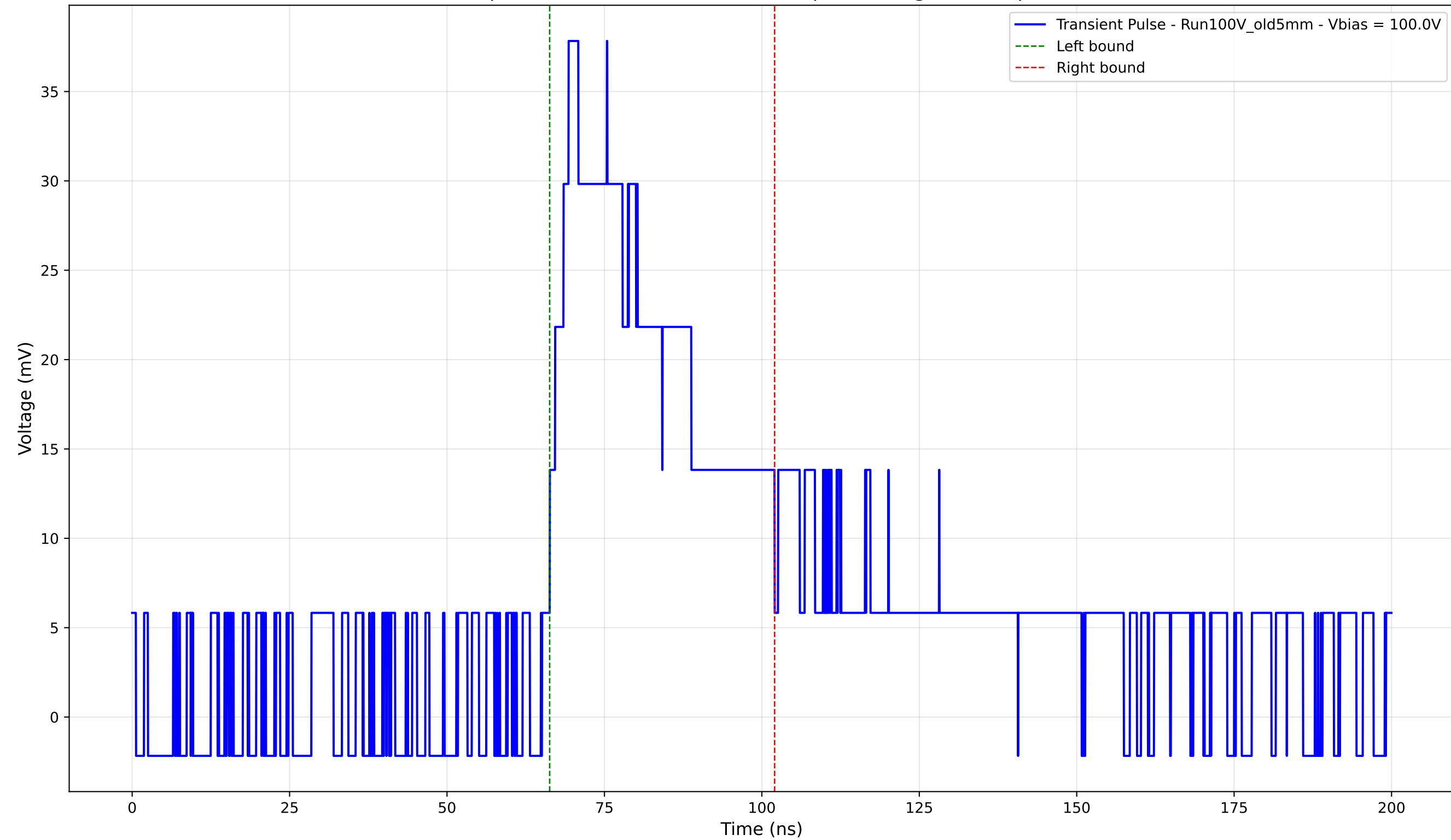
Transient Pulse - Sample: Old5mm - Position: 4965.0 \mu\text{m} - Charge: 15.32 pC - Rise Time: 4.23 ns
