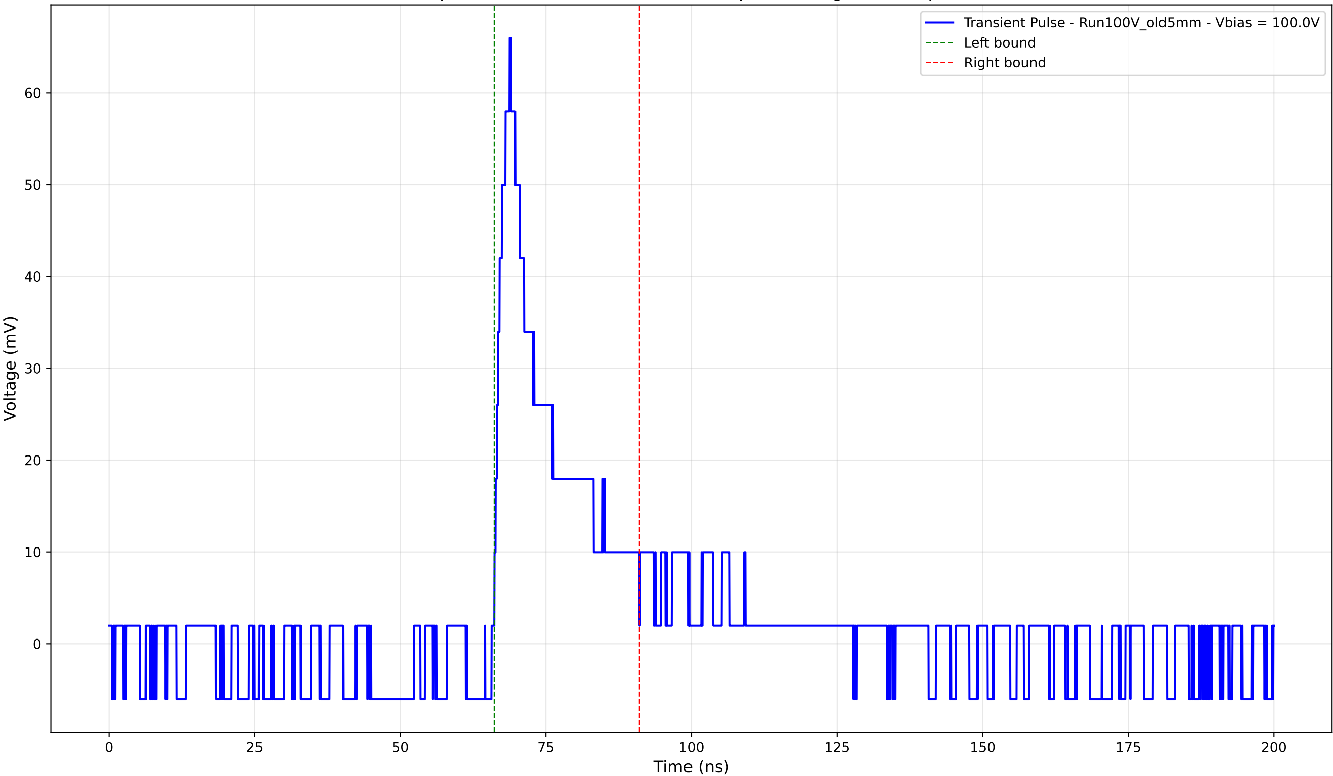
Transient Pulse - Sample: Old5mm - Position: 3005.0 \mu\text{m} - Charge: 11.70 pC - Rise Time: 2.61 ns
