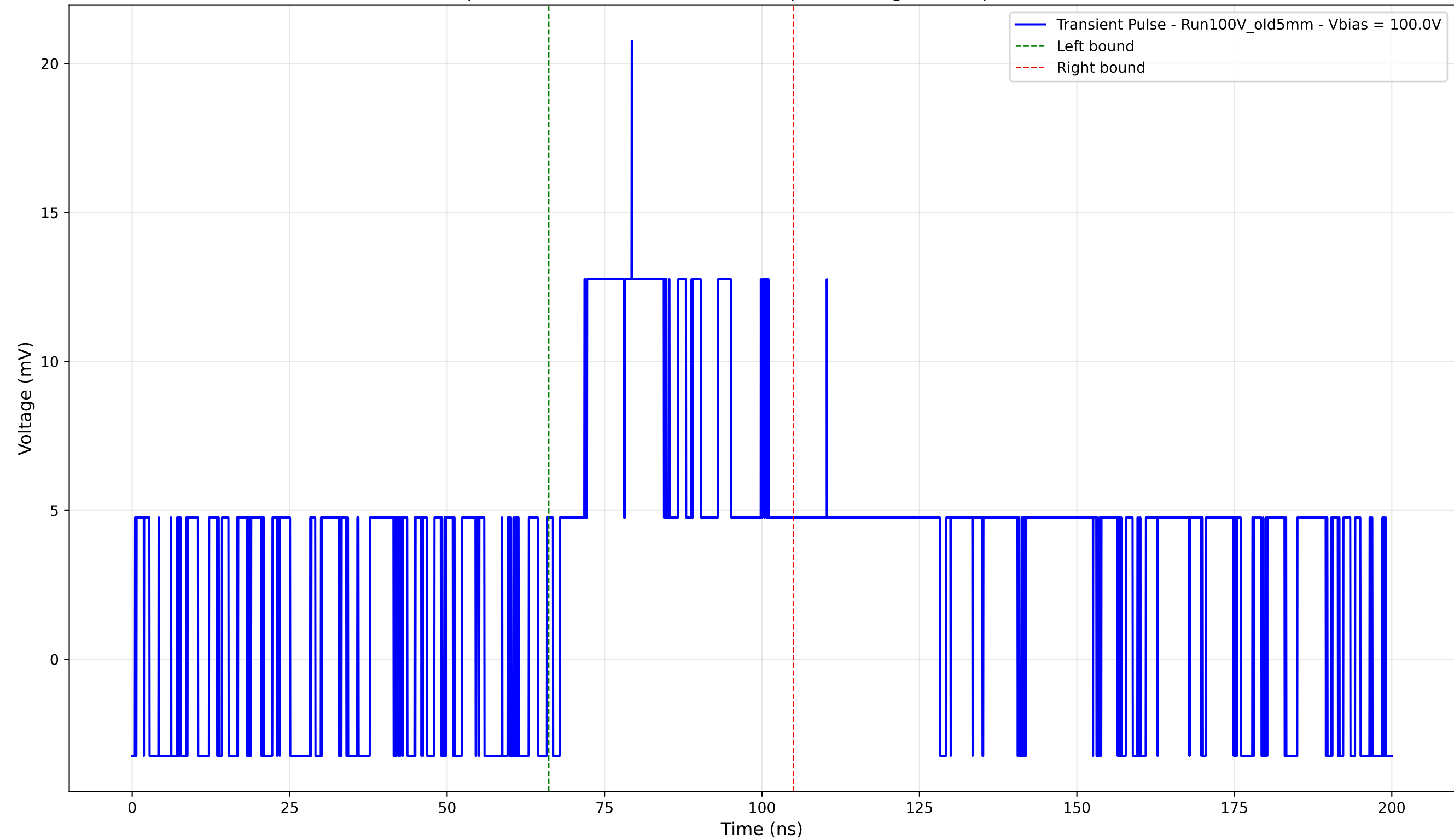
Transient Pulse - Sample: Old5mm - Position: 1865.0 \mu\text{m} - Charge: 6.41 pC - Rise Time: 0.00 ns (N/A)
