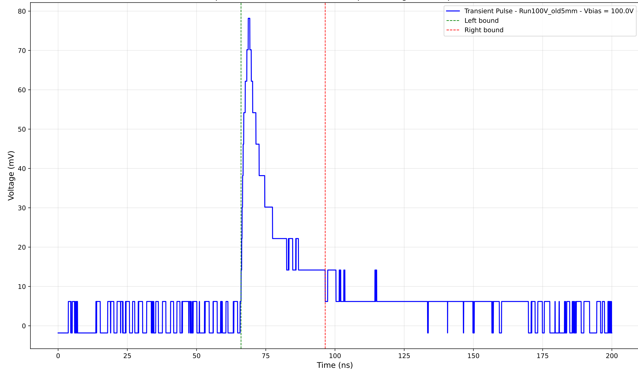
Transient Pulse - Sample: Old5mm - Position: 4430.0 \mu\text{m} - Charge: 17.03 pC - Rise Time: 2.60 ns
