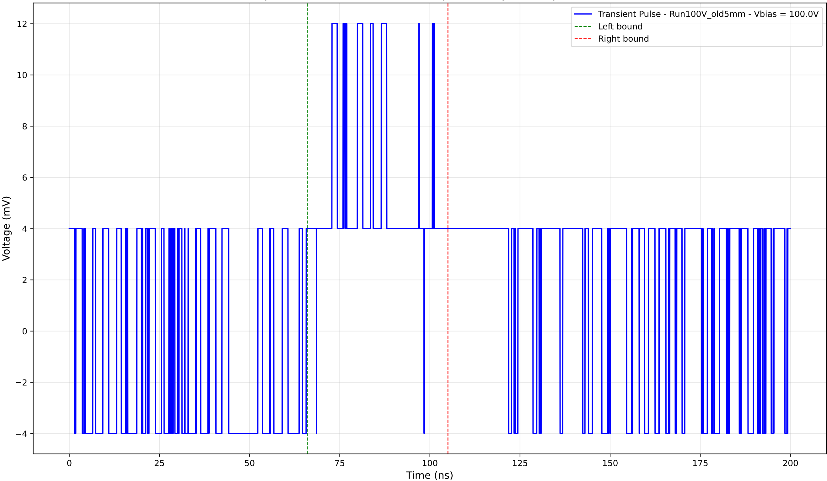
Transient Pulse - Sample: Old5mm - Position: 910.0 \mu\text{m} - Charge: 4.11 pC - Rise Time: 0.00 ns (N/A)
