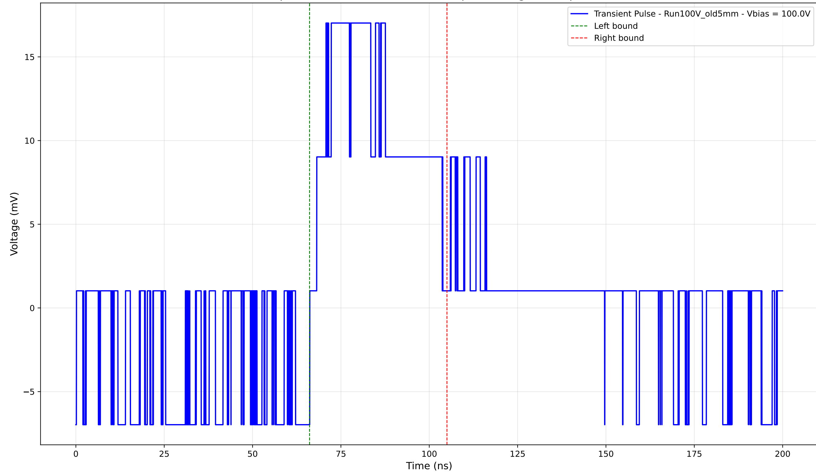
Transient Pulse - Sample: Old5mm - Position: 2035.0 \mu\text{m} - Charge: 8.66 pC - Rise Time: 2.64 ns
