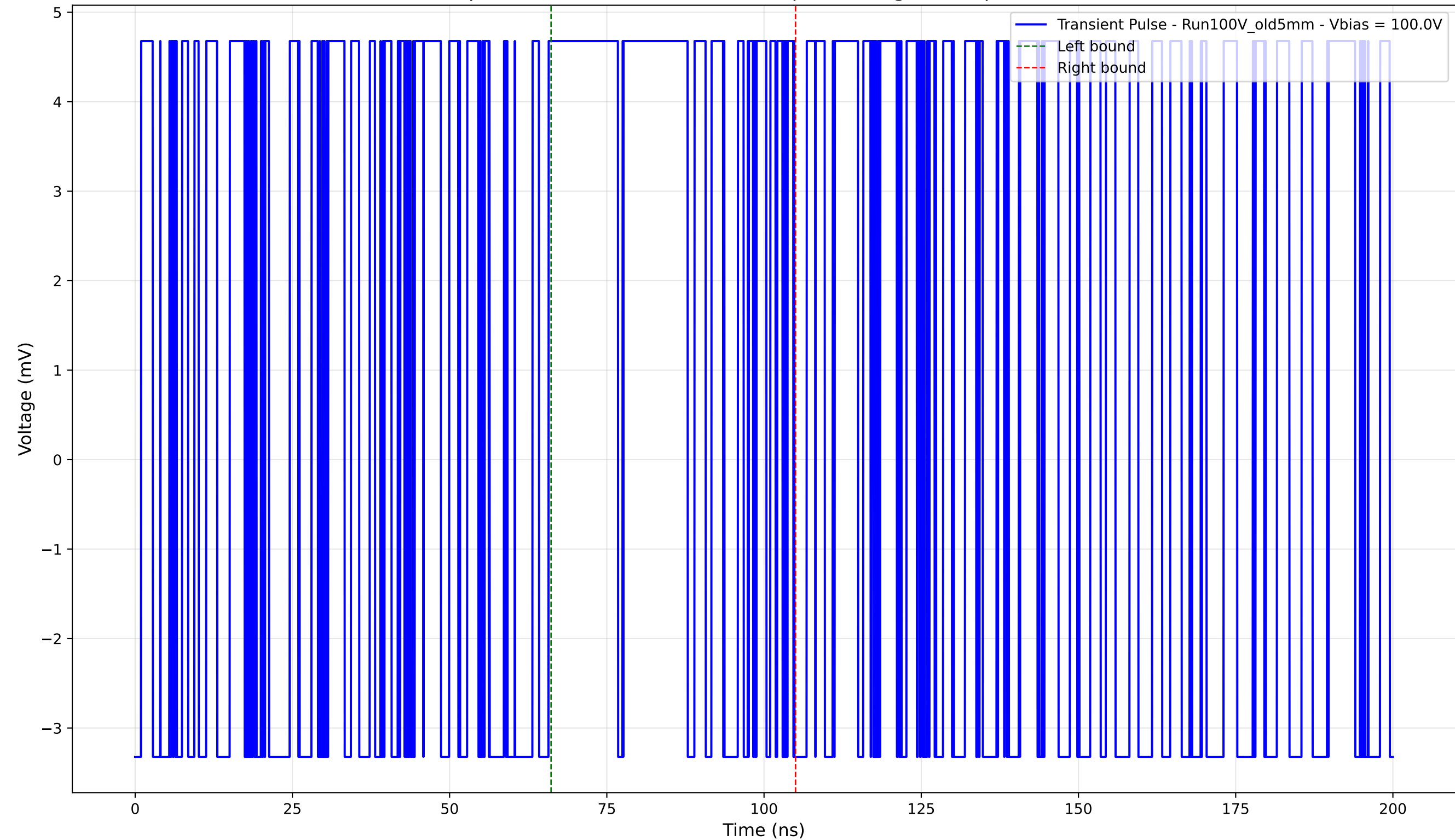
Transient Pulse - Sample: Old5mm - Position: 4635.0 \mu\text{m} - Charge: 2.42 pC - Rise Time: 0.00 ns (N/A)
