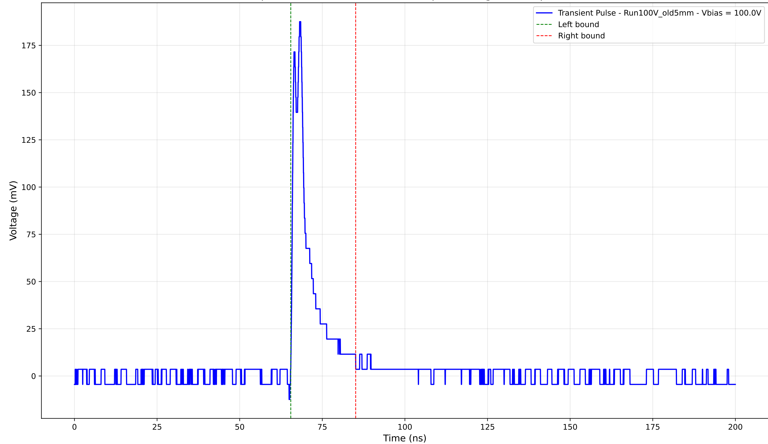
Transient Pulse - Sample: Old5mm - Position: 3875.0 \mu\text{m} - Charge: 20.20 pC - Rise Time: 0.88 ns
