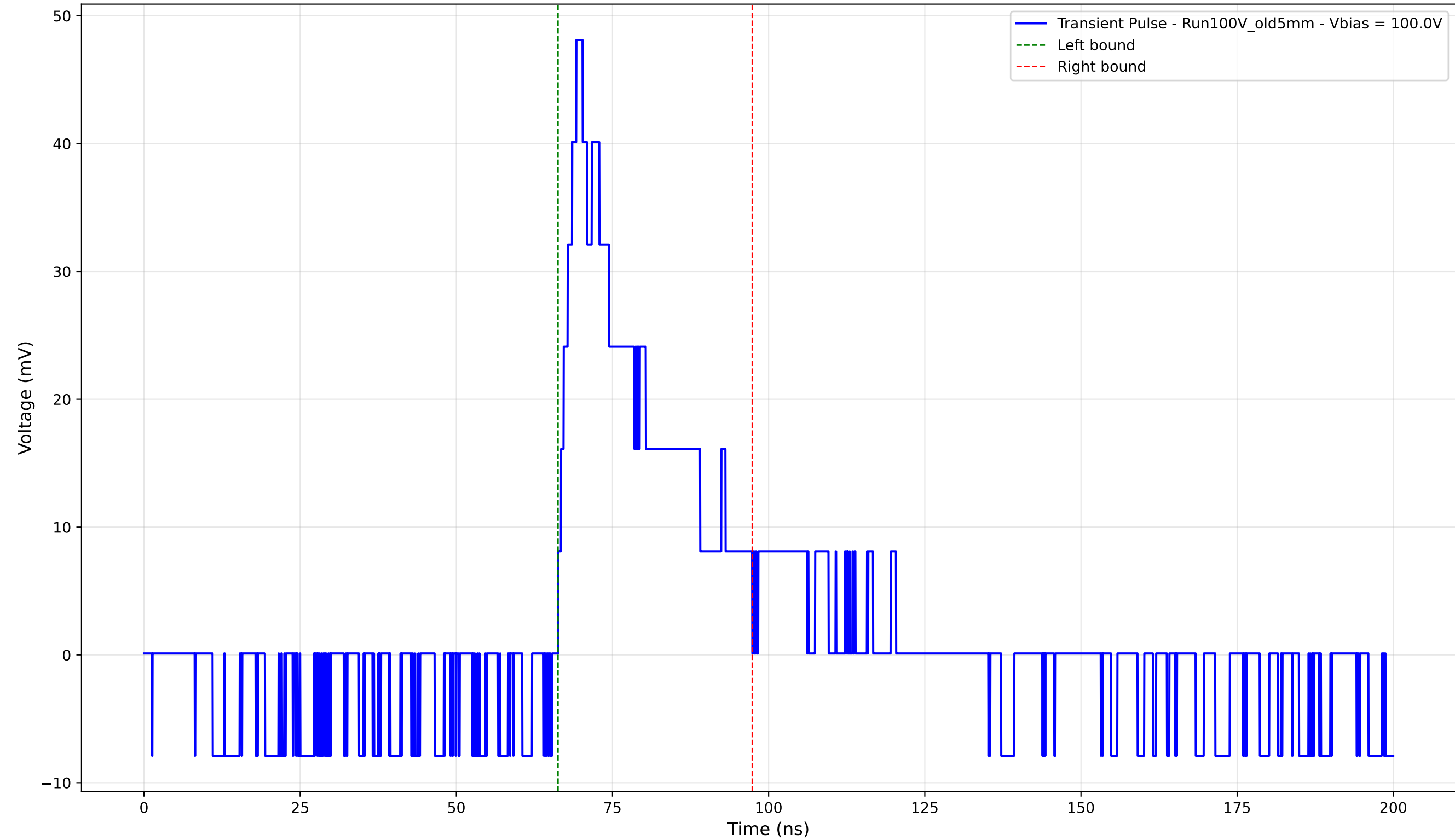
Transient Pulse - Sample: Old5mm - Position: 4780.0 \mu\text{m} - Charge: 12.55 pC - Rise Time: 2.91 ns
