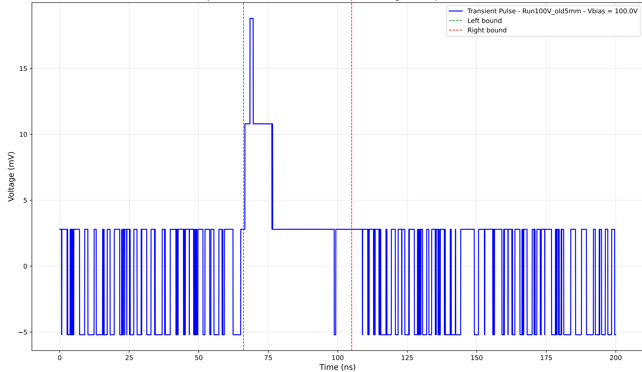
Transient Pulse - Sample: Old5mm - Position: 4360.0 \mu\text{m} - Charge: 3.84 pC - Rise Time: 0.00 ns (N/A)
