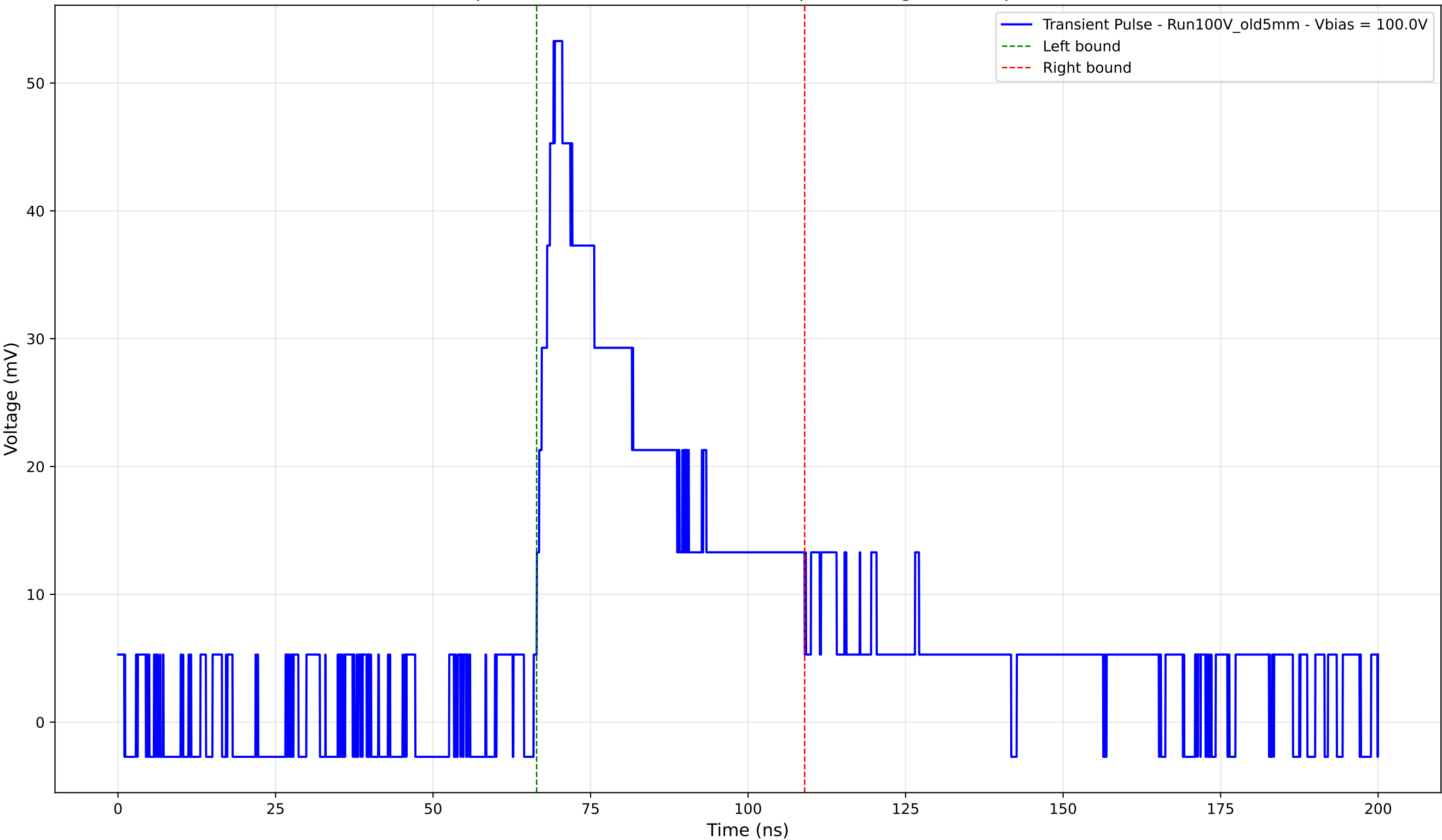
Transient Pulse - Sample: Old5mm - Position: 4775.0 \mu\text{m} - Charge: 19.30 pC - Rise Time: 2.68 ns
