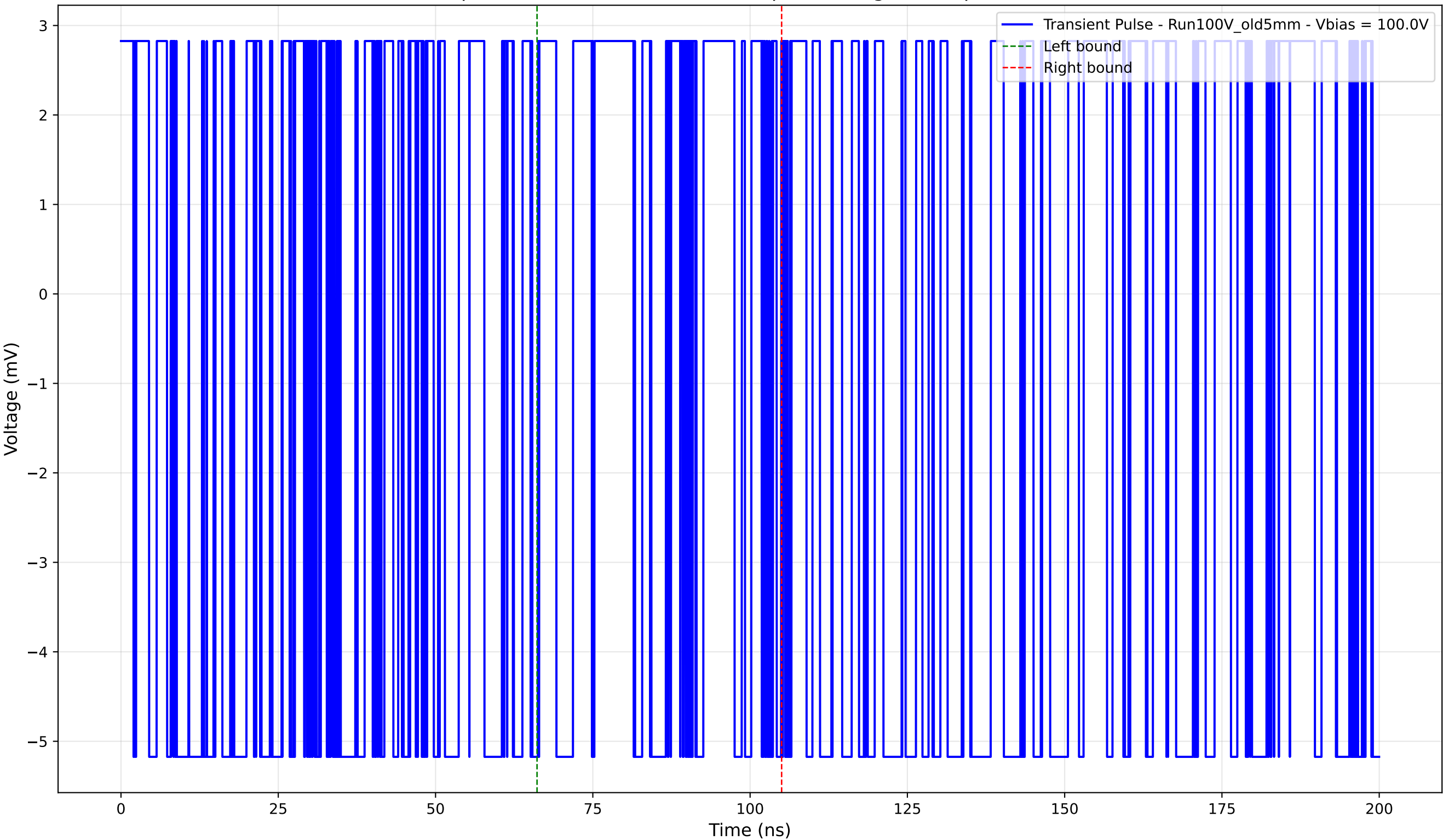
Transient Pulse - Sample: Old5mm - Position: 250.0 \mu\text{m} - Charge: 0.10 pC - Rise Time: 0.00 ns (N/A)
