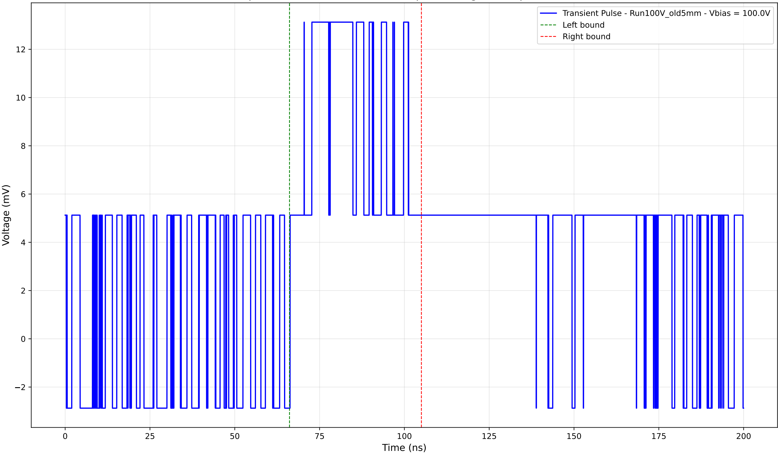
Transient Pulse - Sample: Old5mm - Position: 985.0 \mu\text{m} - Charge: 6.88 pC - Rise Time: 0.00 ns (N/A)
