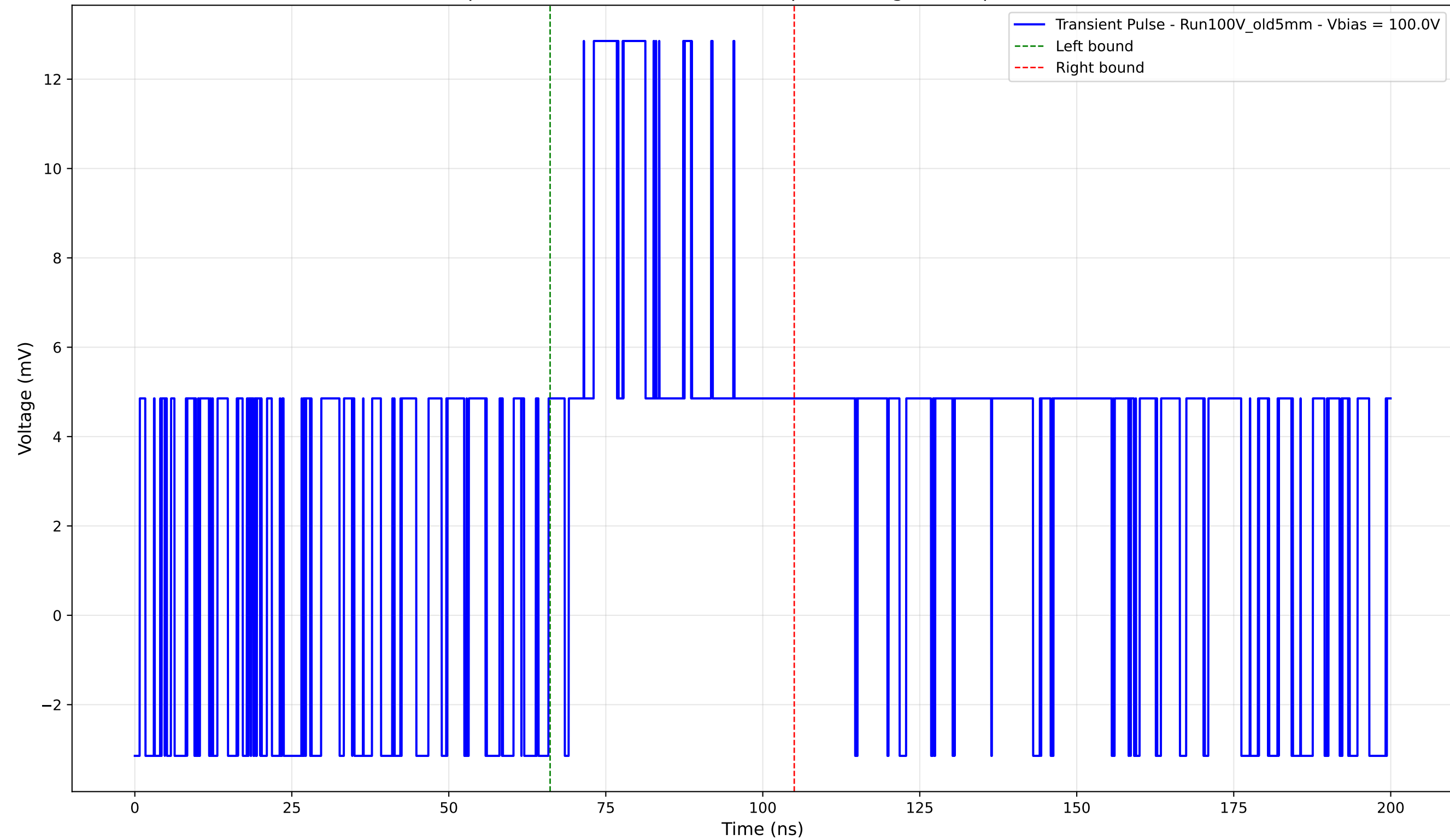
Transient Pulse - Sample: Old5mm - Position: 1050.0 \mu\text{m} - Charge: 5.16 pC - Rise Time: 0.00 ns (N/A)
