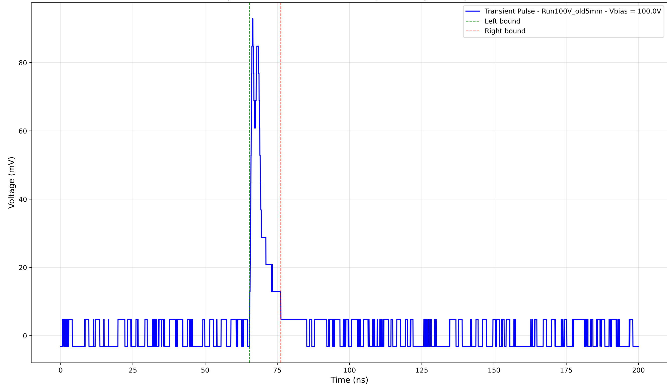
Transient Pulse - Sample: Old5mm - Position: 3645.0 \mu\text{m} - Charge: 7.88 pC - Rise Time: 0.73 ns
