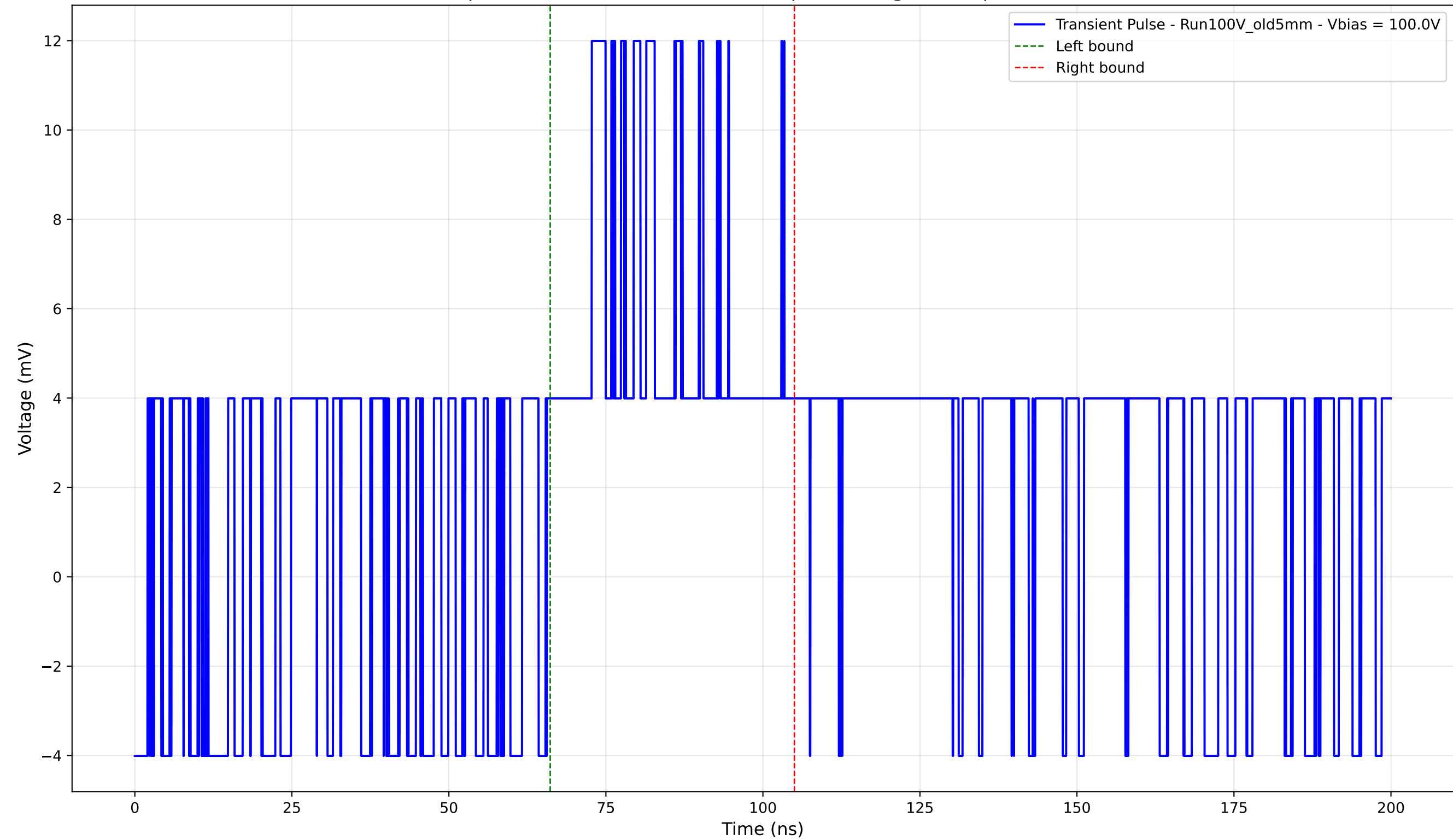
Transient Pulse - Sample: Old5mm - Position: 1880.0 \mu\text{m} - Charge: 4.39 pC - Rise Time: 0.00 ns (N/A)
