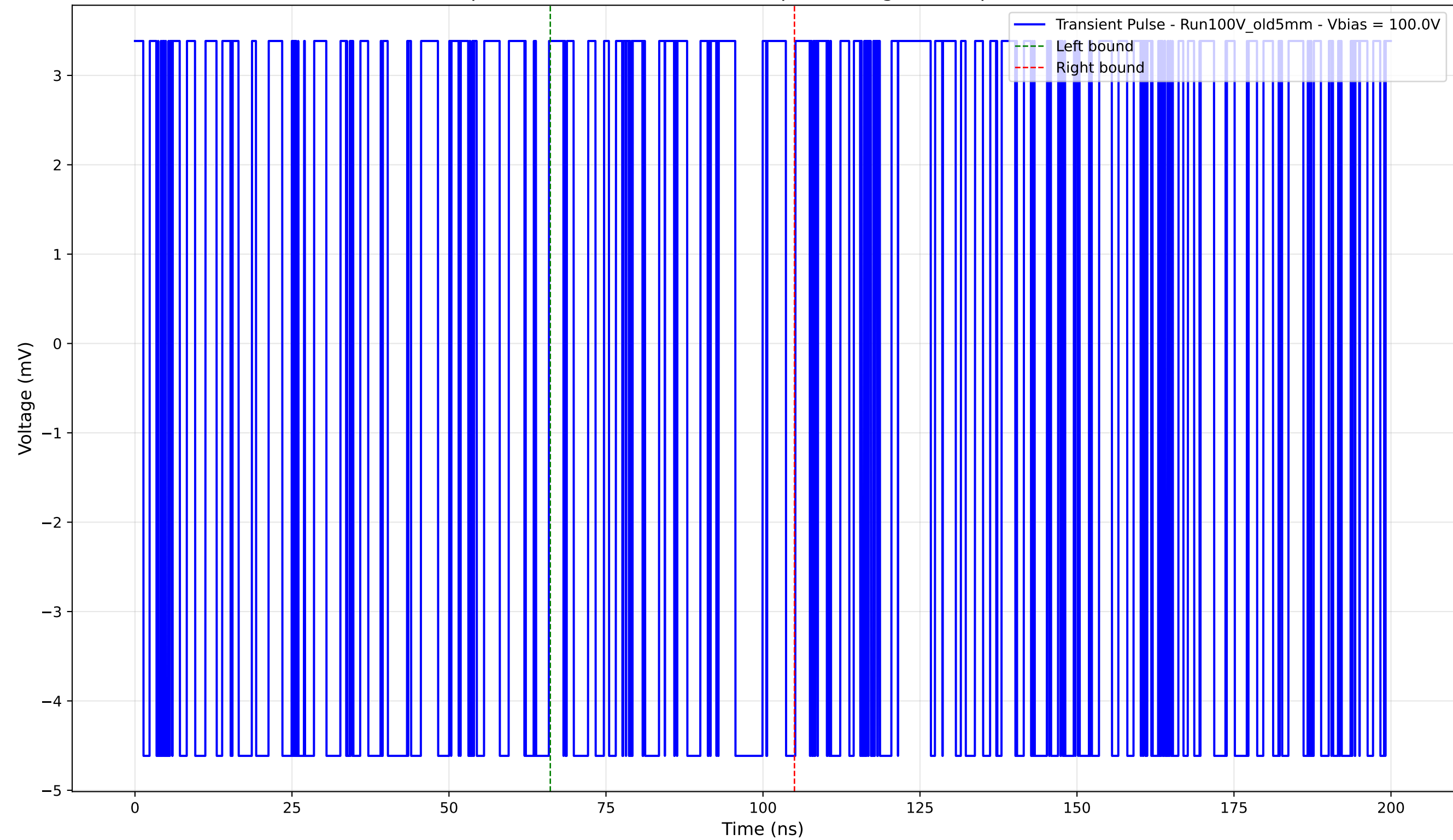
Transient Pulse - Sample: Old5mm - Position: 170.0 \mu\text{m} - Charge: -0.02 pC - Rise Time: 0.00 ns (N/A)
