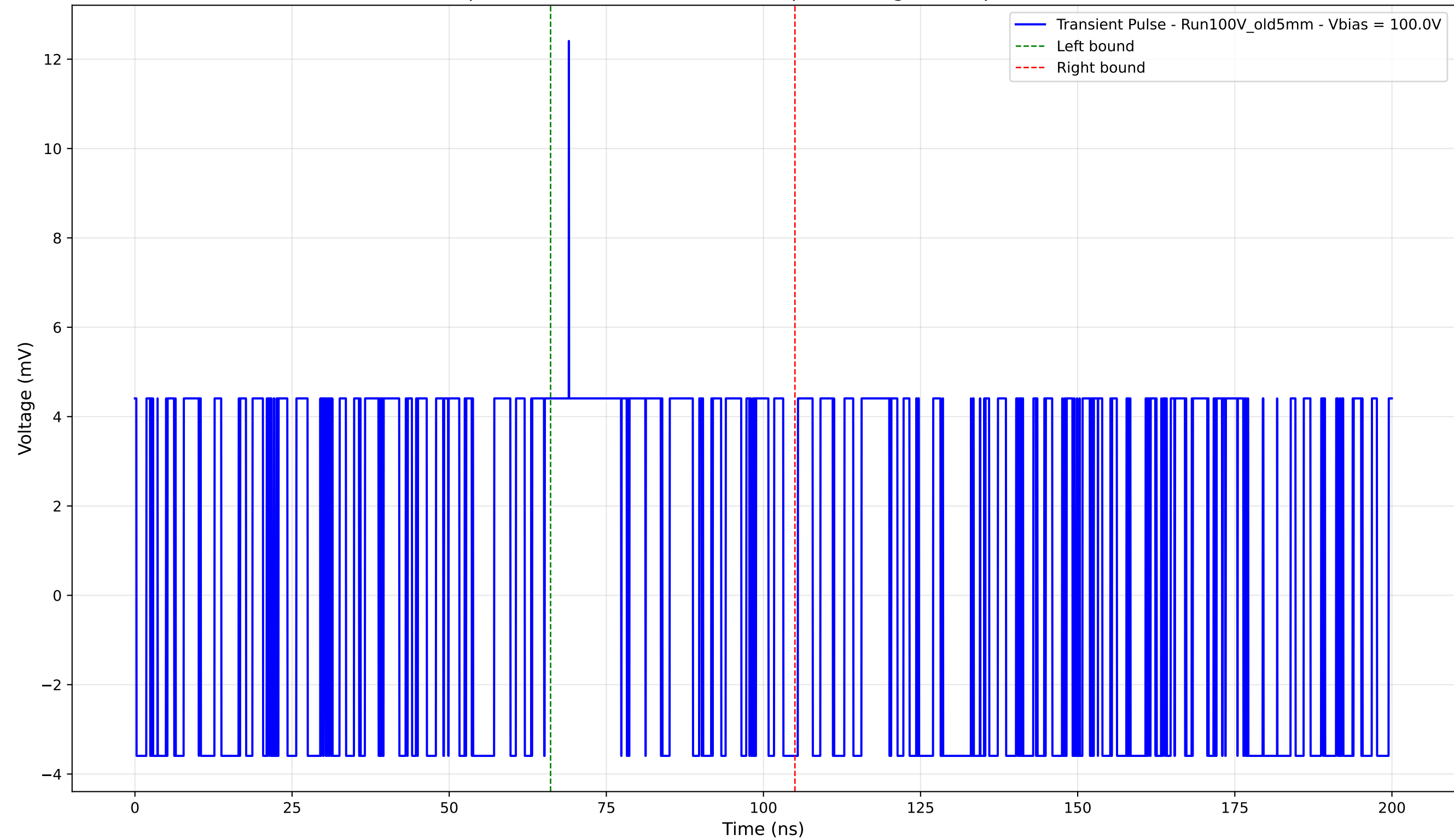
Transient Pulse - Sample: Old5mm - Position: 3115.0 \mu\text{m} - Charge: 2.00 pC - Rise Time: 0.00 ns (N/A)
