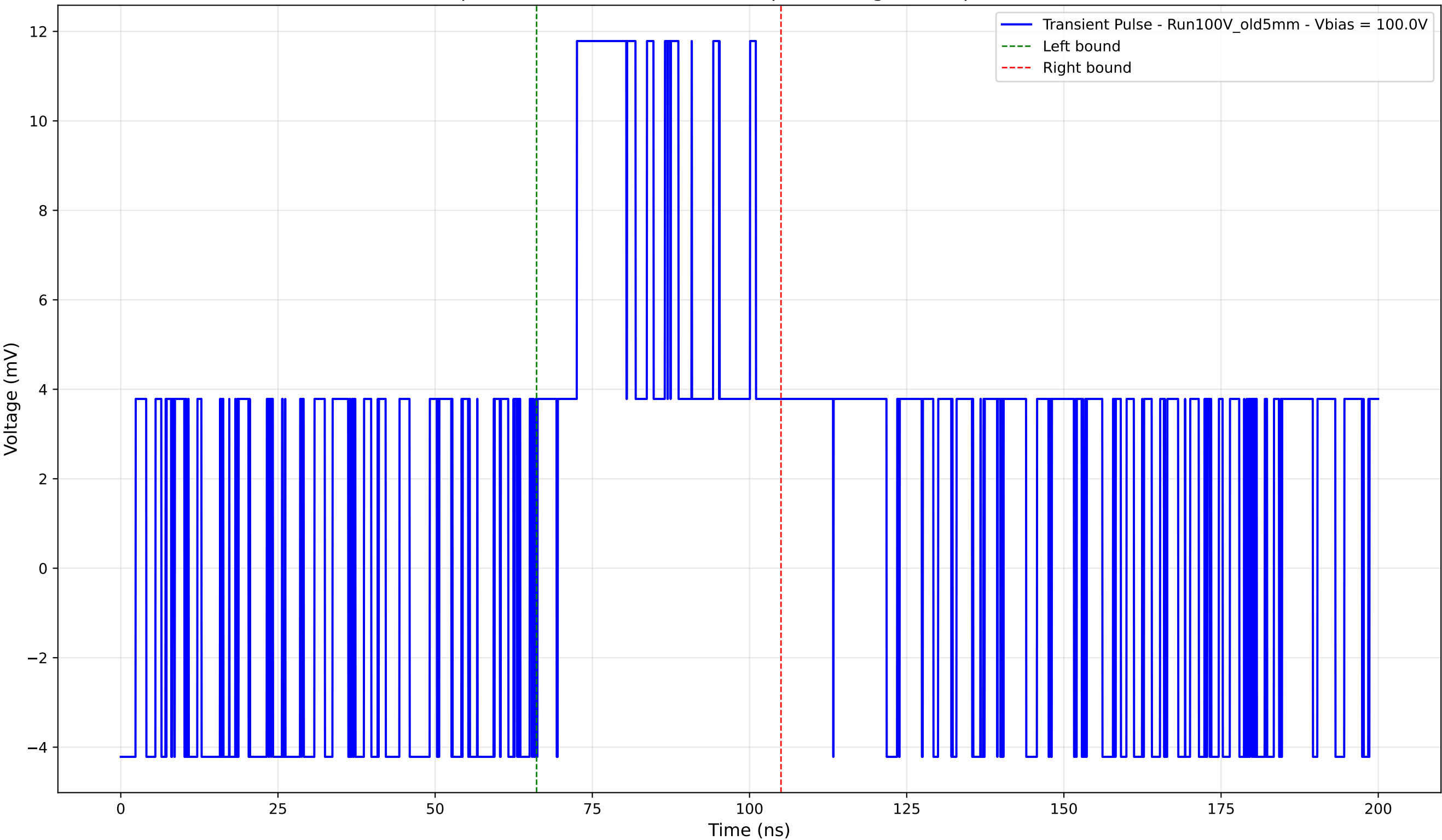
Transient Pulse - Sample: Old5mm - Position: 875.0 \mu\text{m} - Charge: 5.18 pC - Rise Time: 0.00 ns (N/A)
