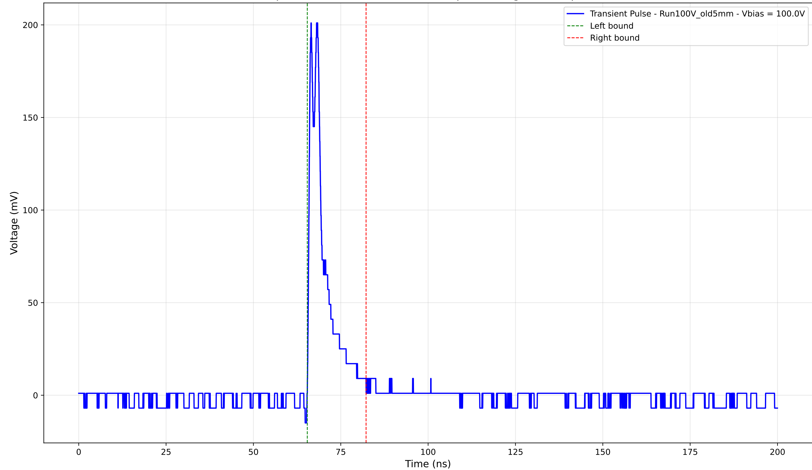
Transient Pulse - Sample: Old5mm - Position: 3580.0 \mu\text{m} - Charge: 19.72 pC - Rise Time: 0.71 ns
