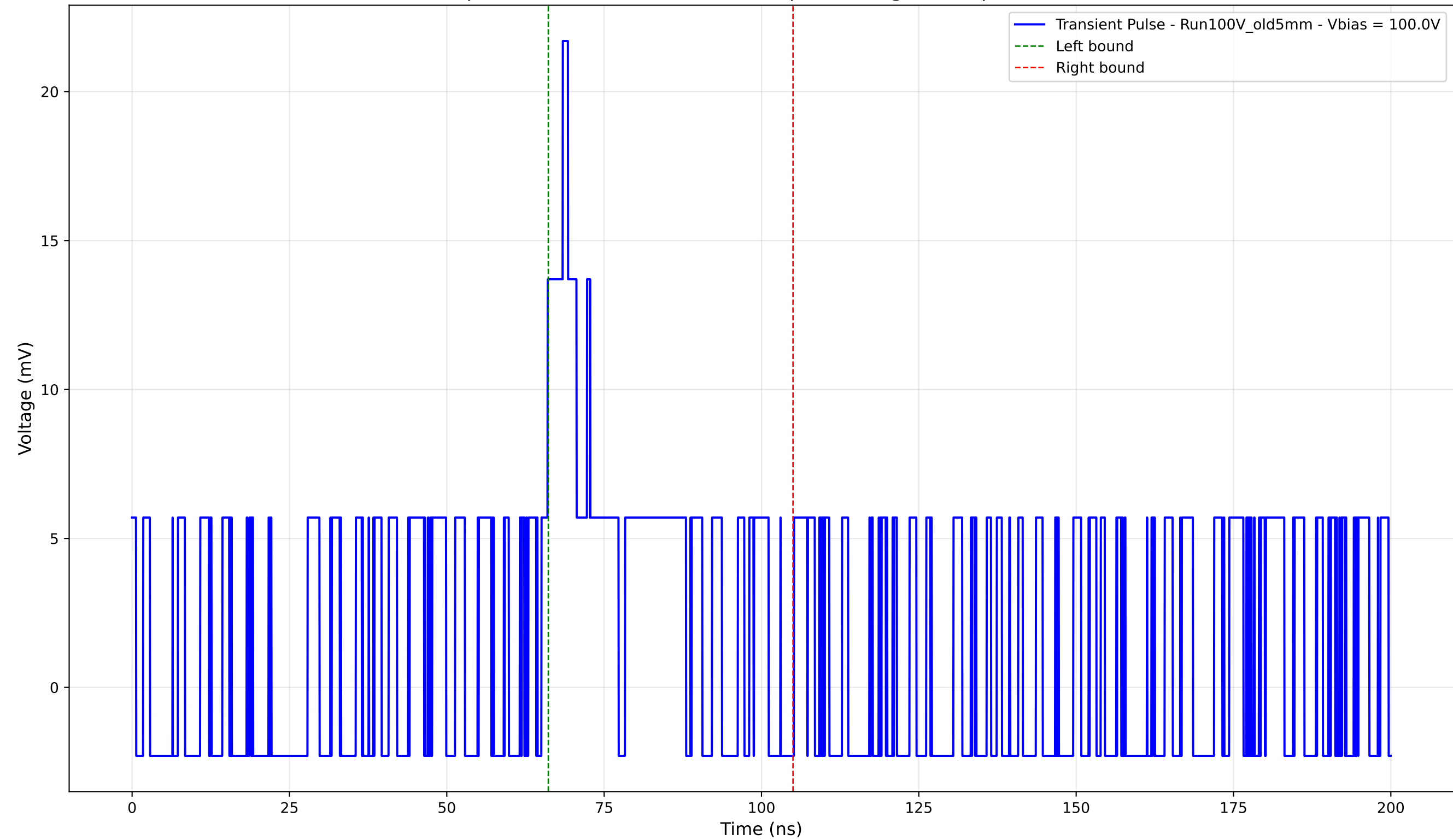
Transient Pulse - Sample: Old5mm - Position: 4045.0 \mu\text{m} - Charge: 3.66 pC - Rise Time: 0.00 ns (N/A)
