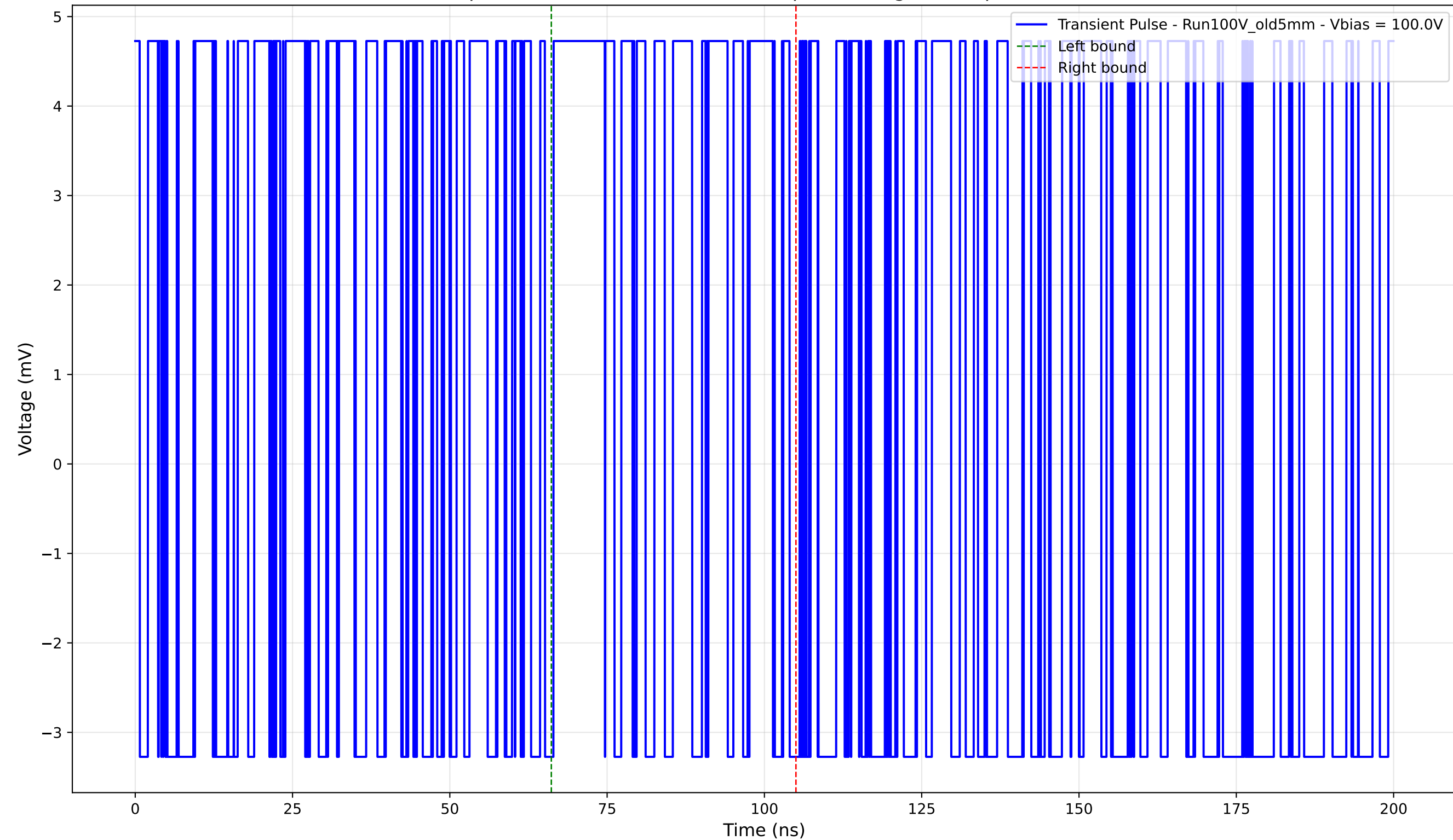
Transient Pulse - Sample: Old5mm - Position: 2780.0 \mu\text{m} - Charge: 1.90 pC - Rise Time: 0.00 ns (N/A)
