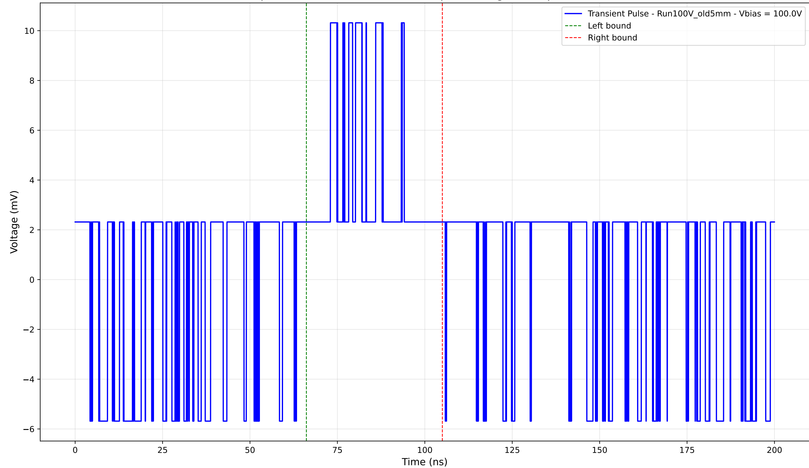
Transient Pulse - Sample: Old5mm - Position: 1875.0 \mu\text{m} - Charge: 3.11 pC - Rise Time: 0.00 ns (N/A)
