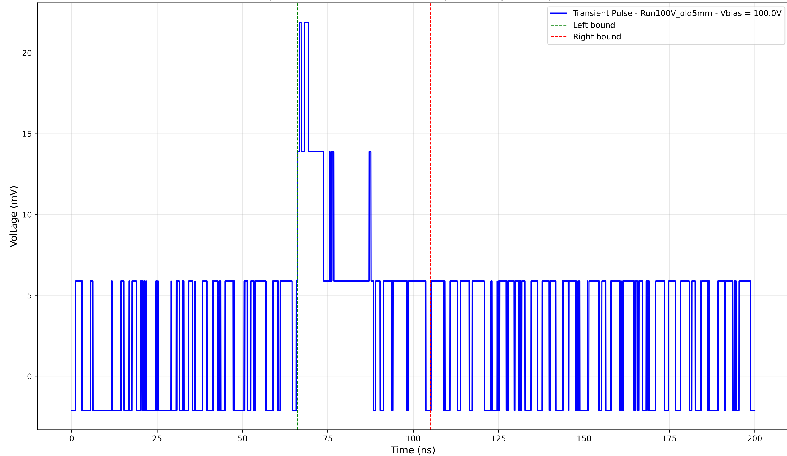
Transient Pulse - Sample: Old5mm - Position: 4260.0 \mu\text{m} - Charge: 5.70 pC - Rise Time: 0.96 ns
