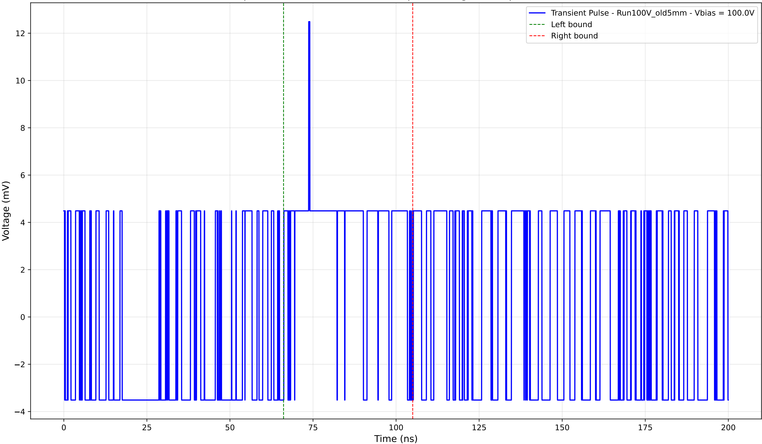
Transient Pulse - Sample: Old5mm - Position: 290.0 \mu\text{m} - Charge: 2.89 pC - Rise Time: 0.00 ns (N/A)
