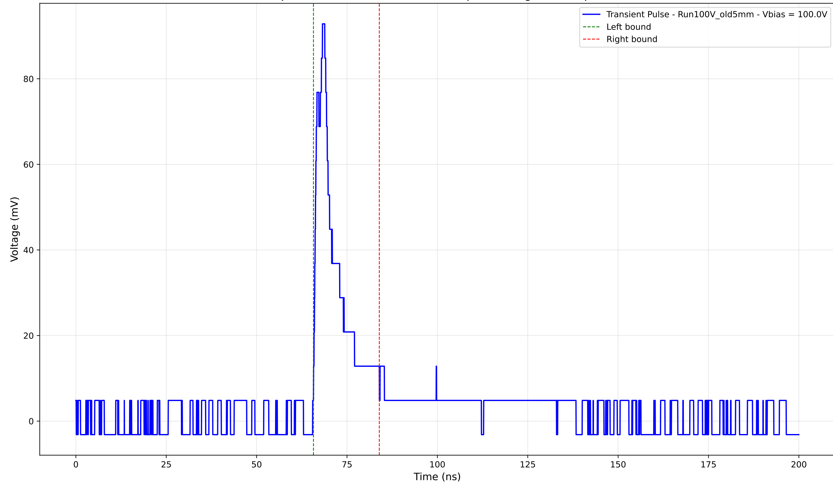
Transient Pulse - Sample: Old5mm - Position: 3320.0 \mu\text{m} - Charge: 11.94 pC - Rise Time: 2.19 ns
