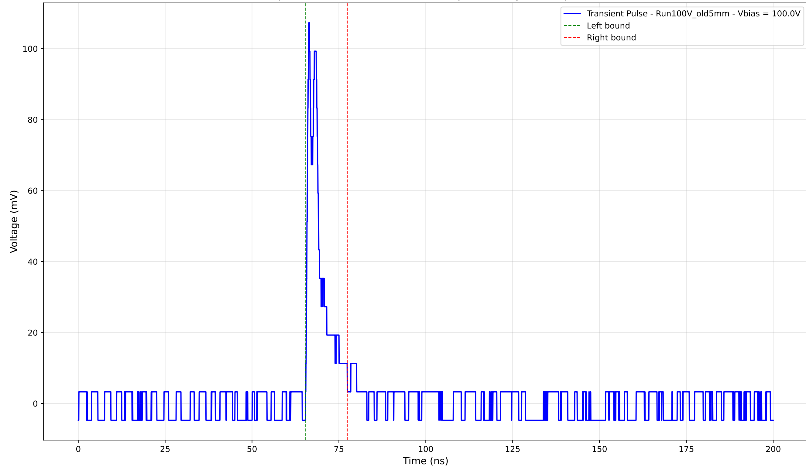
Transient Pulse - Sample: Old5mm - Position: 3775.0 \mu\text{m} - Charge: 9.16 pC - Rise Time: 0.72 ns
