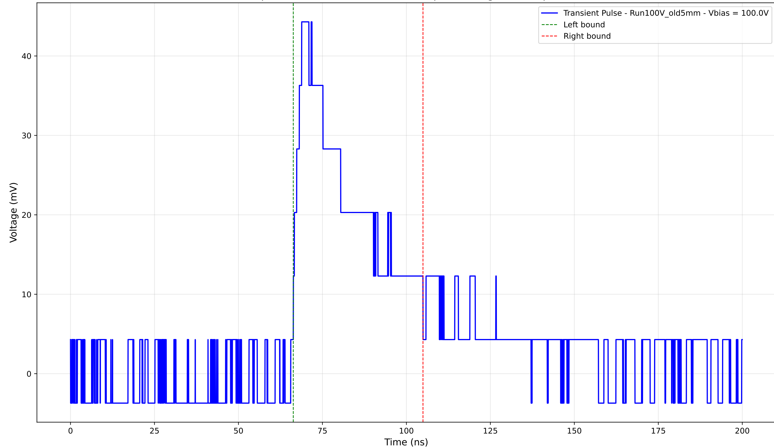
Transient Pulse - Sample: Old5mm - Position: 4815.0 \mu\text{m} - Charge: 17.15 pC - Rise Time: 2.50 ns
