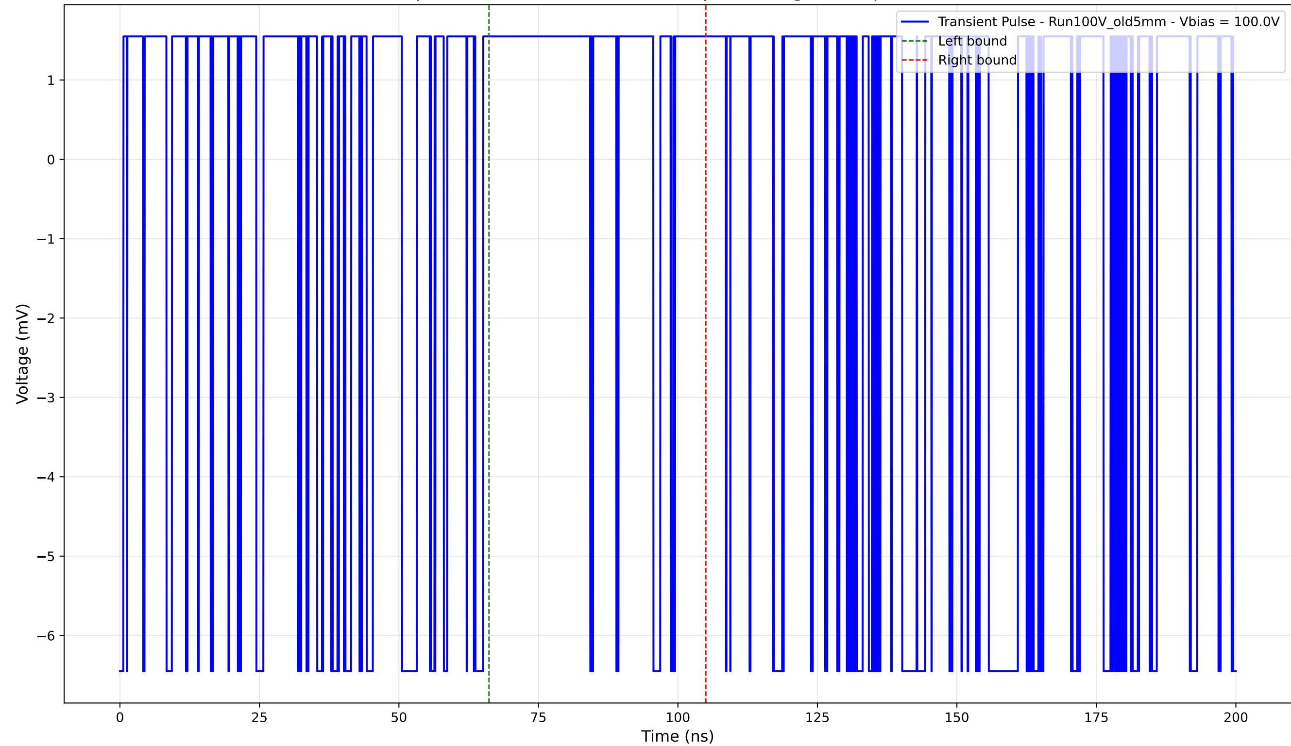
Transient Pulse - Sample: Old5mm - Position: 2530.0 \mu\text{m} - Charge: 0.82 pC - Rise Time: 0.00 ns (N/A)
