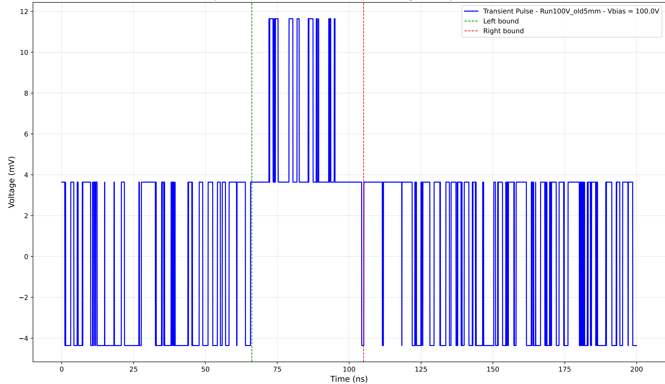
Transient Pulse - Sample: Old5mm - Position: 1950.0 \mu\text{m} - Charge: 3.84 pC - Rise Time: 0.00 ns (N/A)
