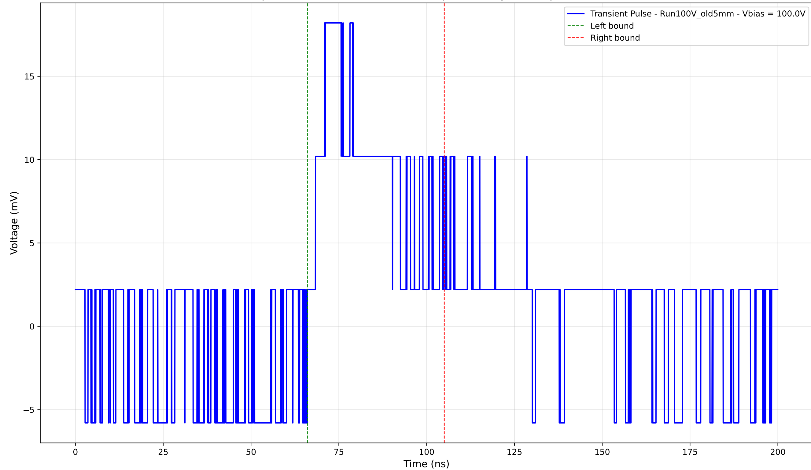
Transient Pulse - Sample: Old5mm - Position: 2375.0 \mu\text{m} - Charge: 7.20 pC - Rise Time: 0.00 ns (N/A)
