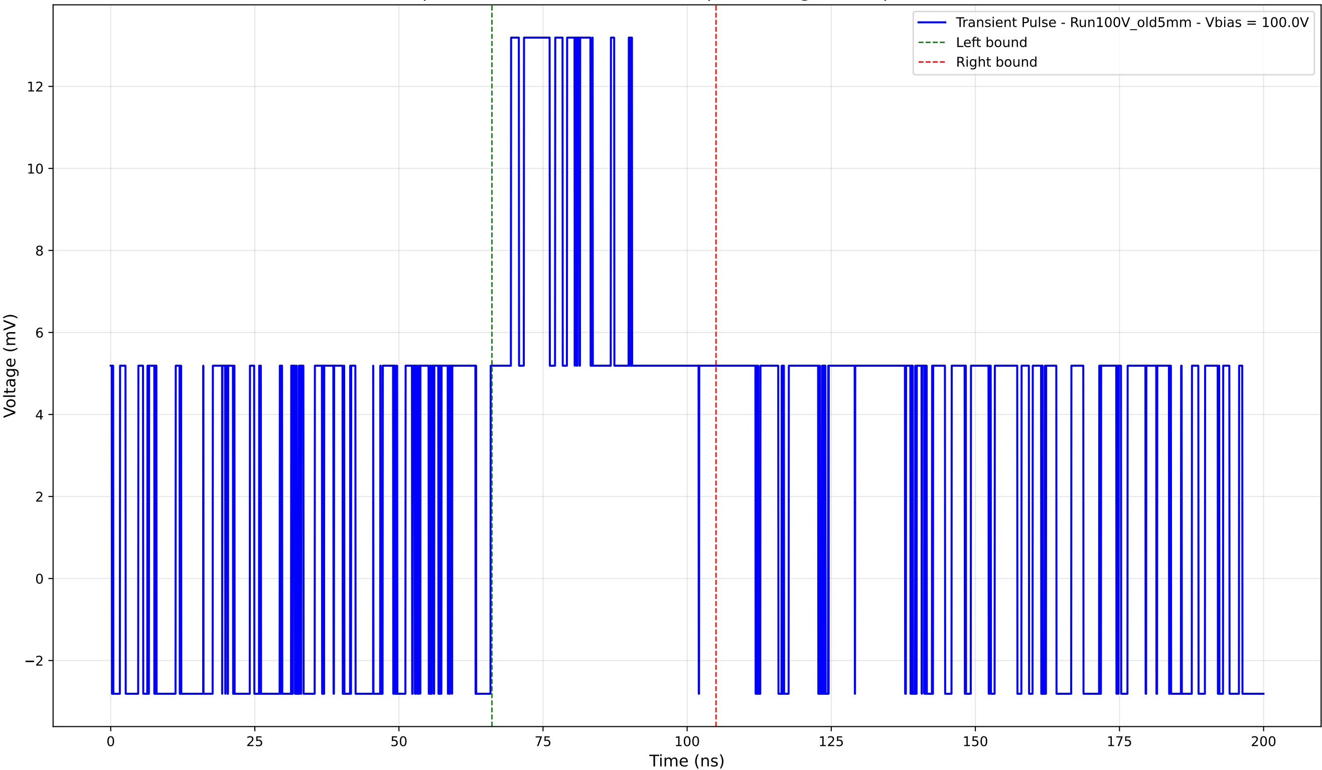
Transient Pulse - Sample: Old5mm - Position: 320.0 \mu\text{m} - Charge: 5.93 pC - Rise Time: 0.00 ns (N/A)
