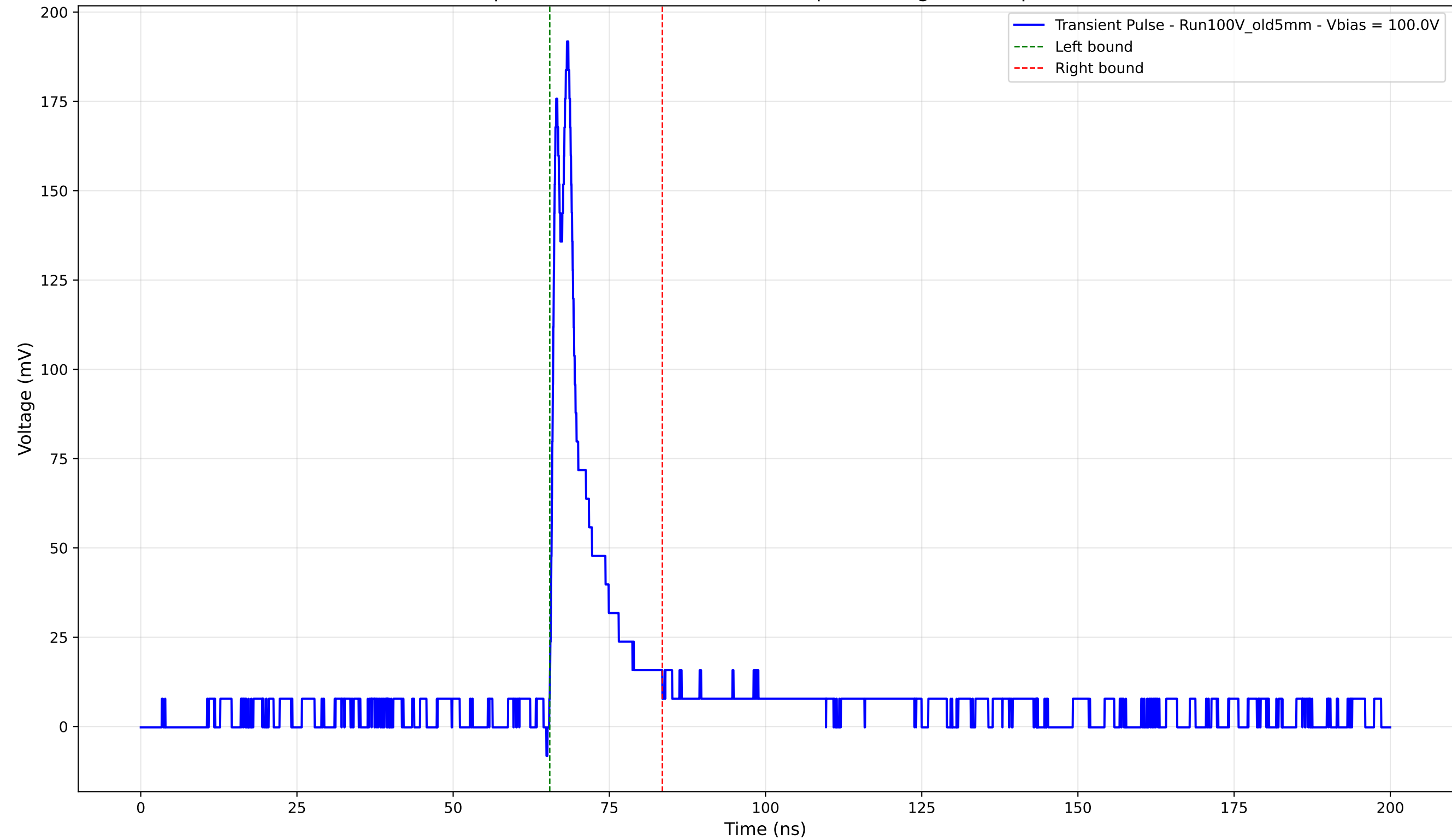
Transient Pulse - Sample: Old5mm - Position: 3540.0 \mu\text{m} - Charge: 21.24 pC - Rise Time: 0.95 ns
