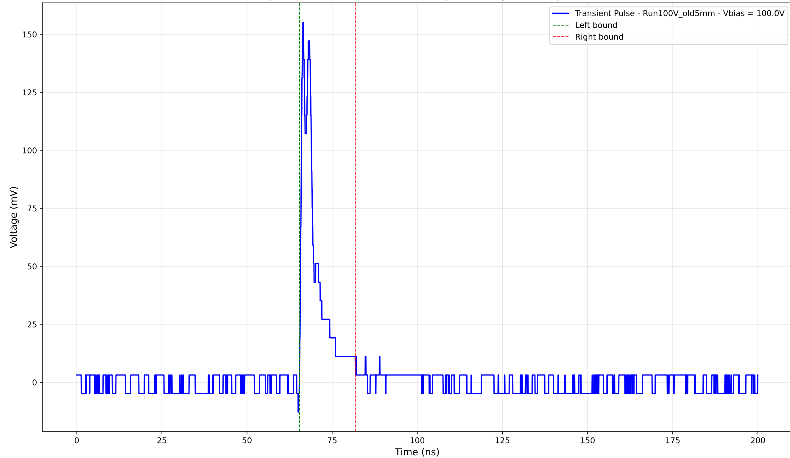
Transient Pulse - Sample: Old5mm - Position: 3790.0 \mu\text{m} - Charge: 14.39 pC - Rise Time: 0.79 ns
