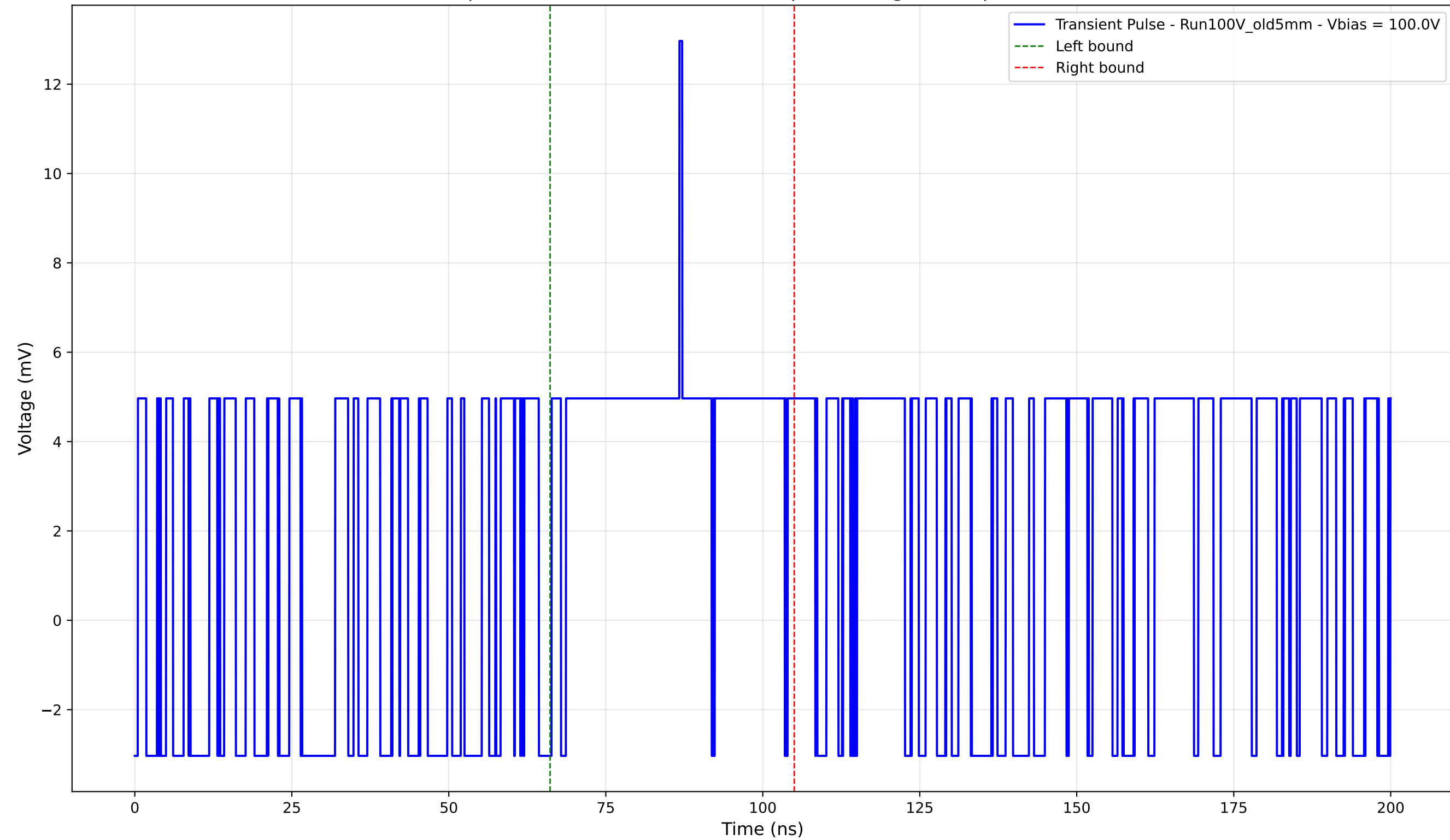
Transient Pulse - Sample: Old5mm - Position: 1520.0 \mu\text{m} - Charge: 3.66 pC - Rise Time: 0.00 ns (N/A)
