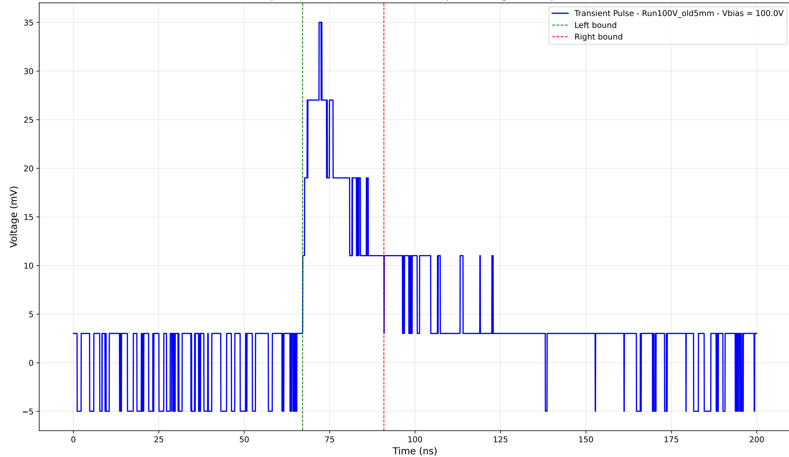
Transient Pulse - Sample: Old5mm - Position: 2590.0 \mu\text{m} - Charge: 8.96 pC - Rise Time: 4.80 ns
