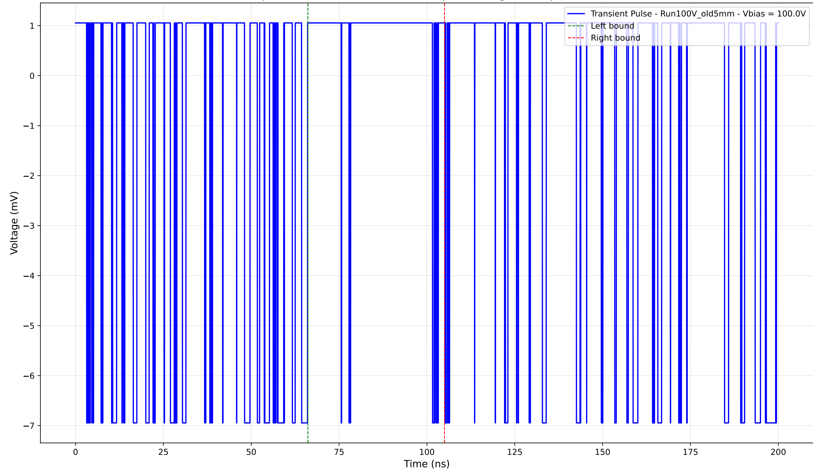
Transient Pulse - Sample: Old5mm - Position: 2110.0 \mu\text{m} - Charge: 0.60 pC - Rise Time: 0.00 ns (N/A)
