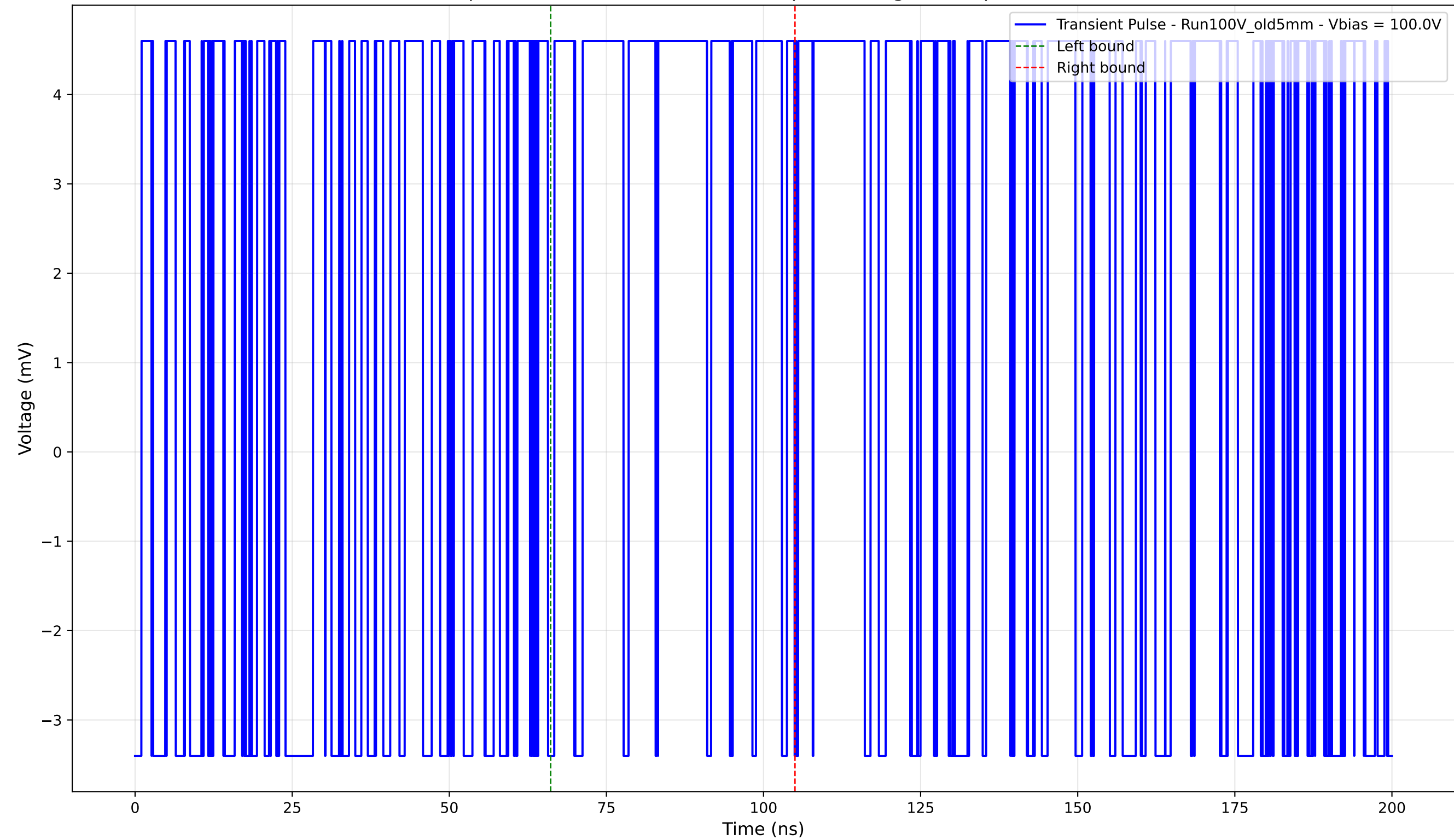
Transient Pulse - Sample: Old5mm - Position: 1515.0 \mu\text{m} - Charge: 2.72 pC - Rise Time: 0.00 ns (N/A)
