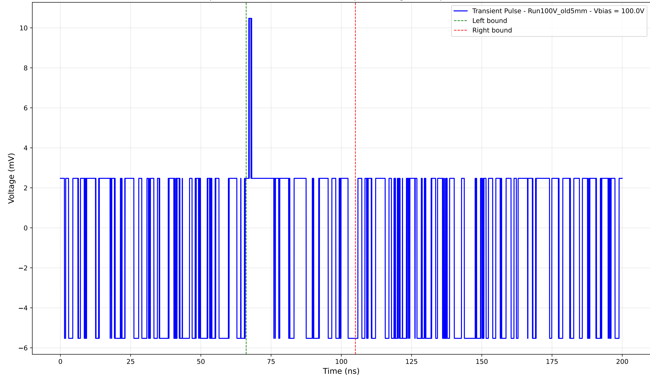
Transient Pulse - Sample: Old5mm - Position: 4020.0 \mu\text{m} - Charge: 0.17 pC - Rise Time: 0.00 ns (N/A)
