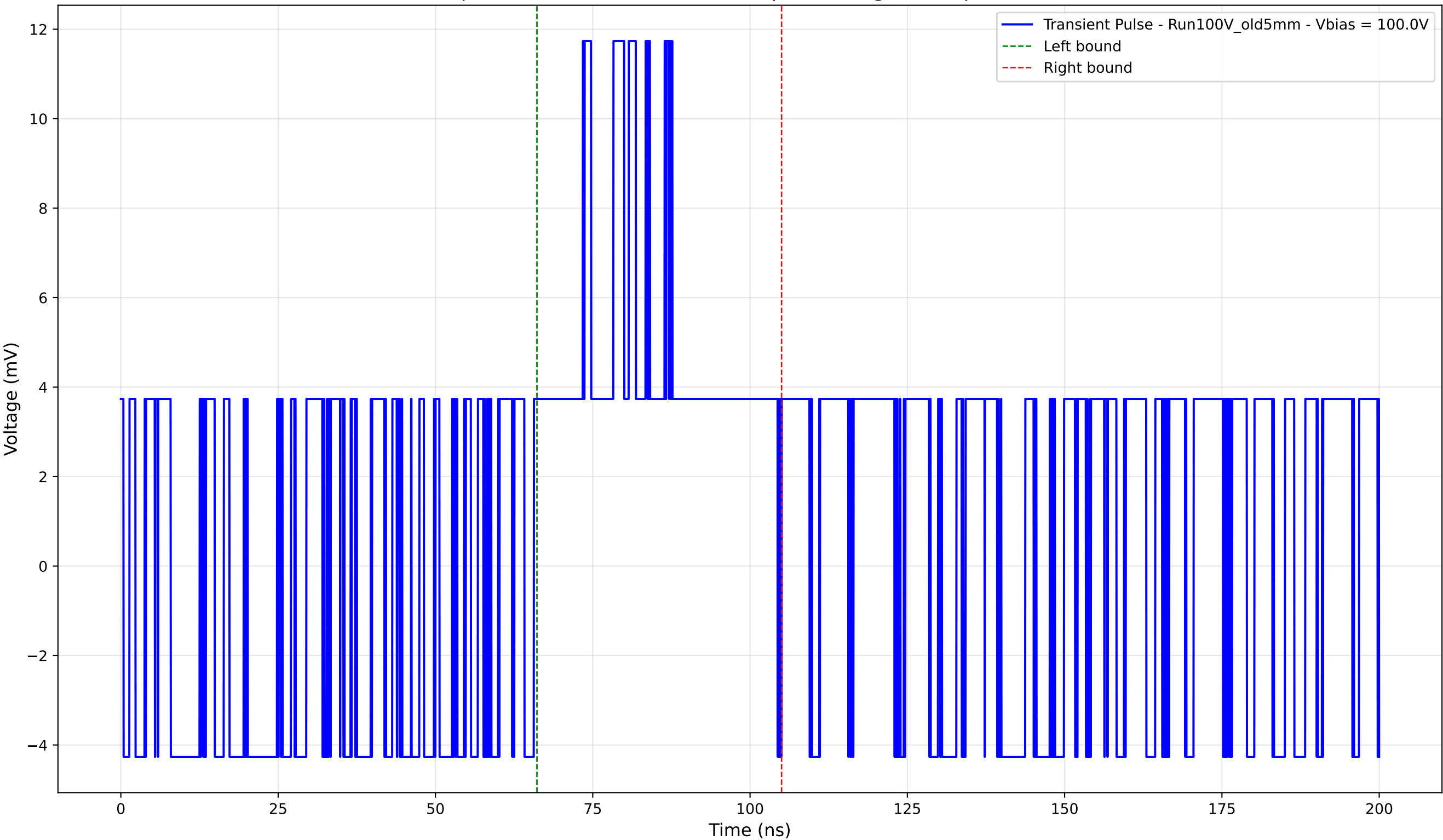
Transient Pulse - Sample: Old5mm - Position: 835.0 \mu\text{m} - Charge: 3.72 pC - Rise Time: 0.00 ns (N/A)
