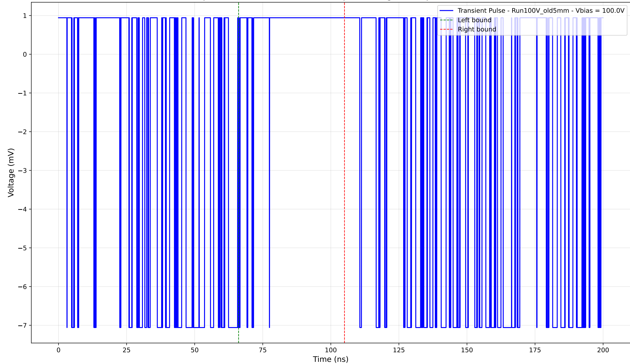
Transient Pulse - Sample: Old5mm - Position: 1725.0 \mu\text{m} - Charge: 0.53 pC - Rise Time: 0.00 ns (N/A)
