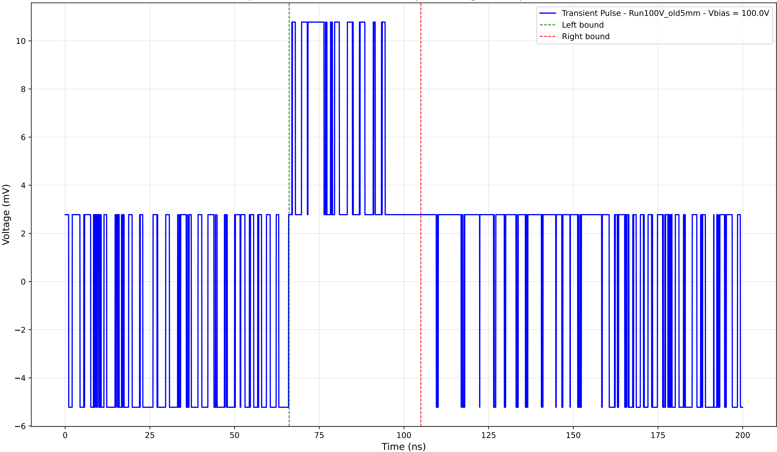
Transient Pulse - Sample: Old5mm - Position: 470.0 \mu\text{m} - Charge: 4.41 pC - Rise Time: 0.00 ns (N/A)
