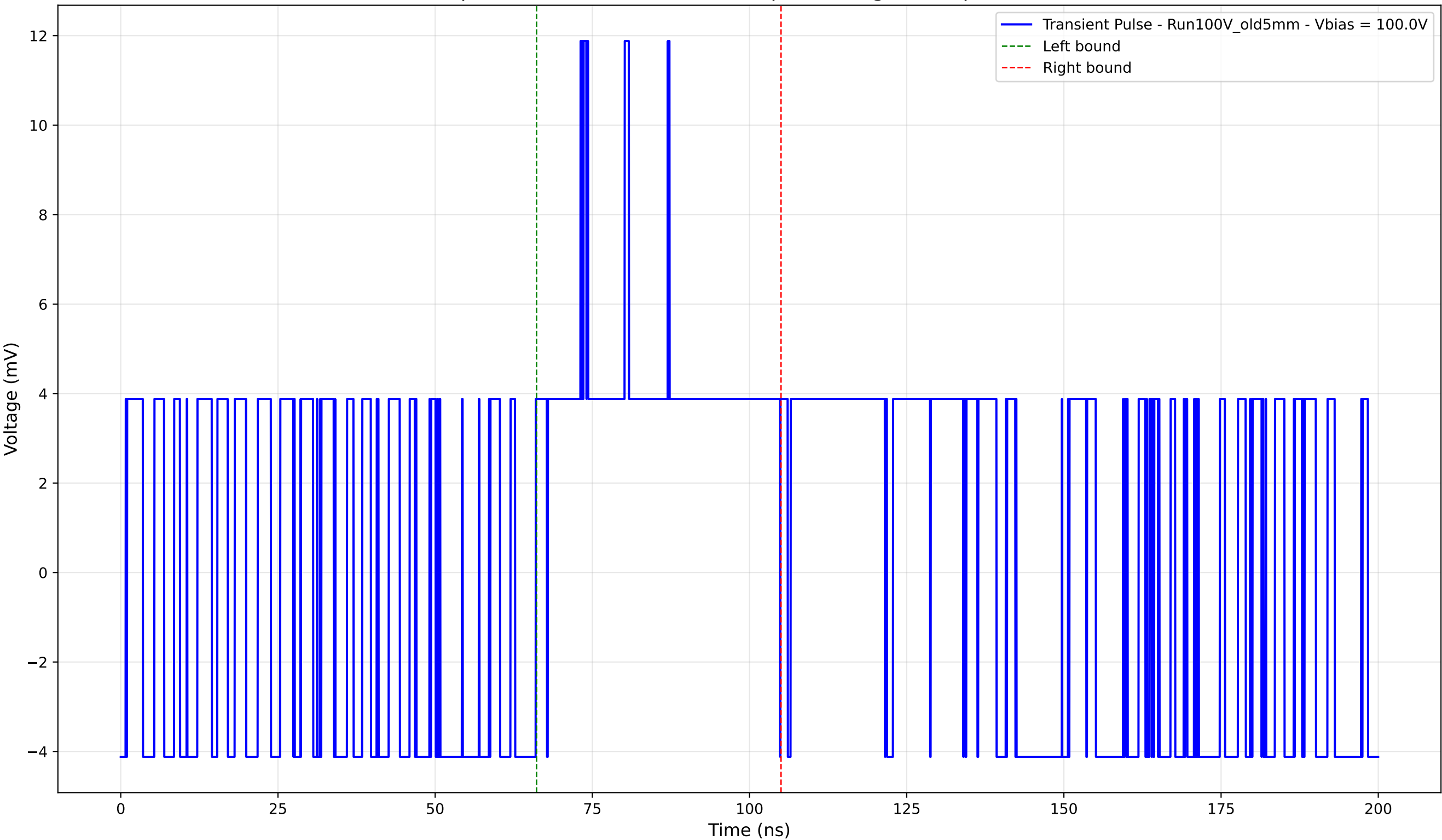
Transient Pulse - Sample: Old5mm - Position: 615.0 \mu\text{m} - Charge: 3.27 pC - Rise Time: 0.00 ns (N/A)
