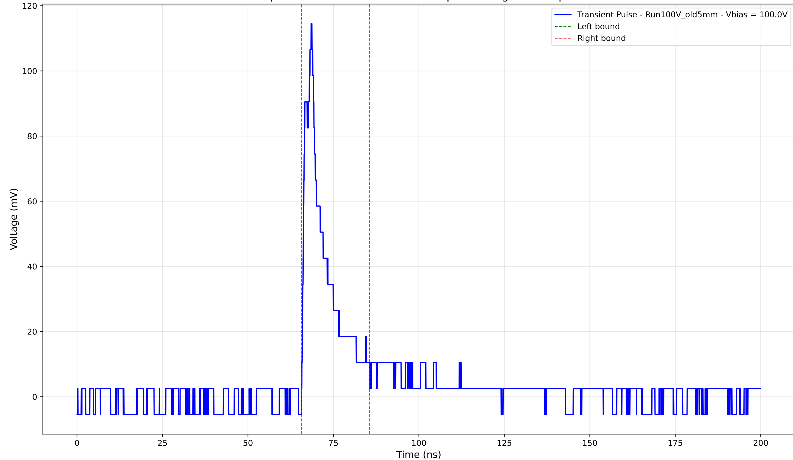
Transient Pulse - Sample: Old5mm - Position: 4120.0 \mu\text{m} - Charge: 15.00 pC - Rise Time: 2.30 ns
