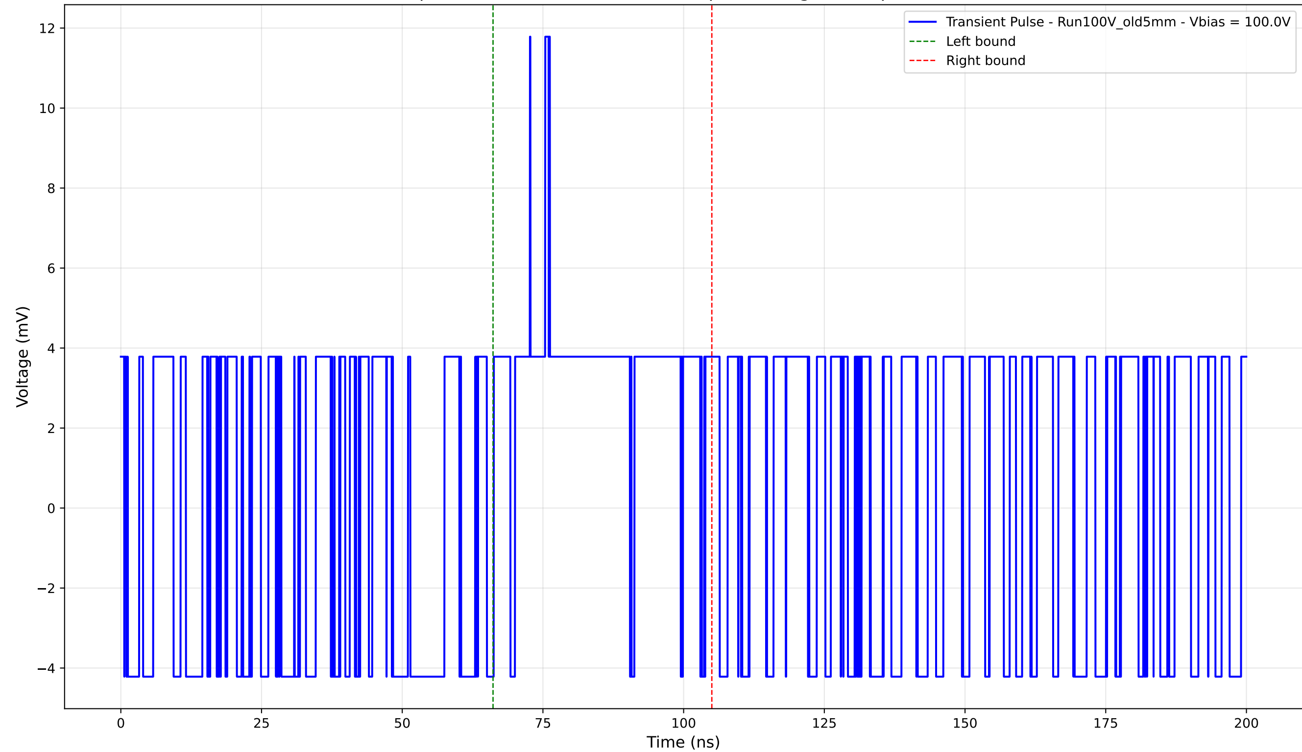
Transient Pulse - Sample: Old5mm - Position: 2095.0 \mu\text{m} - Charge: 2.65 pC - Rise Time: 0.00 ns (N/A)
