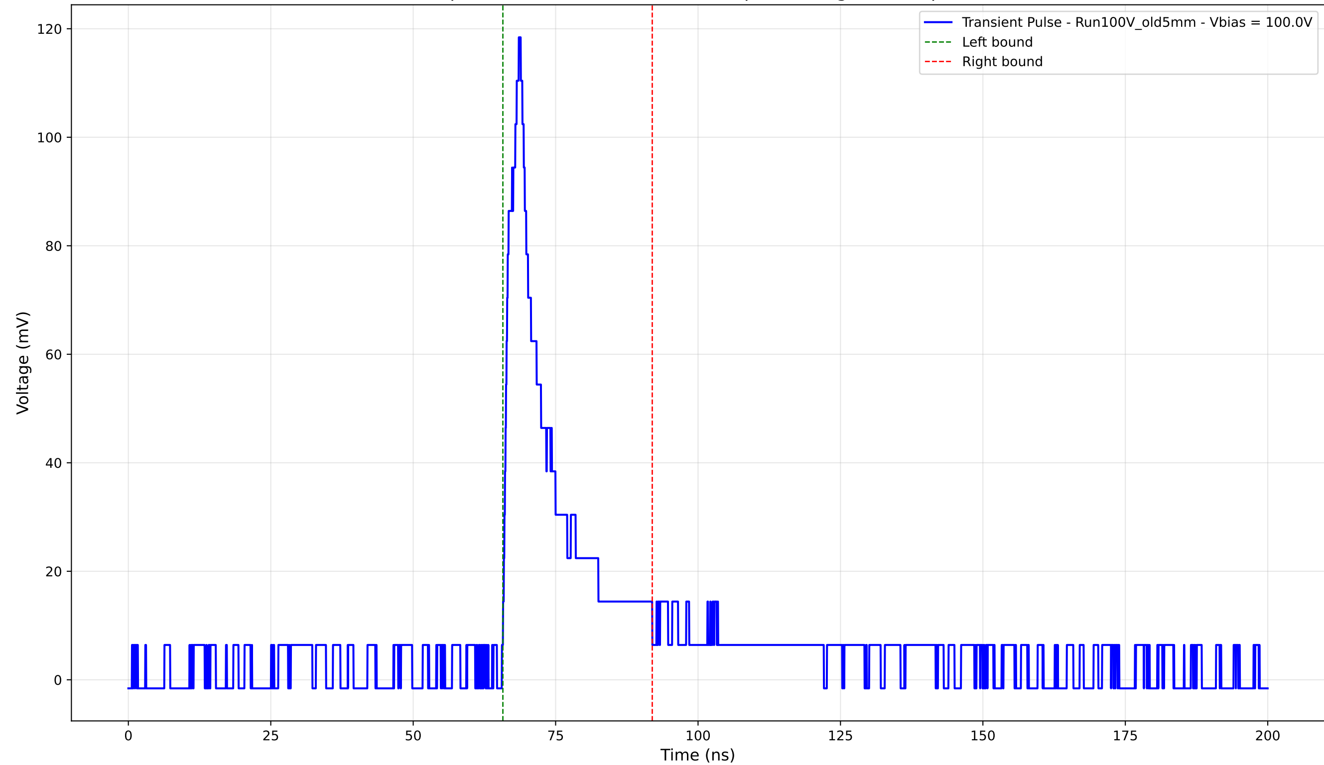
Transient Pulse - Sample: Old5mm - Position: 3240.0 \mu\text{m} - Charge: 19.16 pC - Rise Time: 2.41 ns
