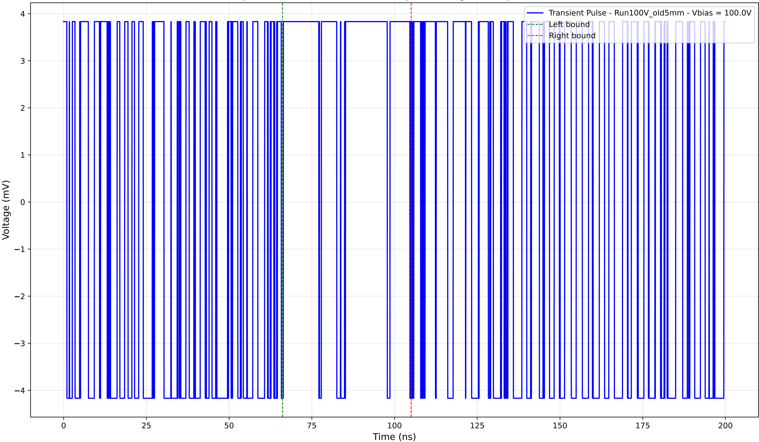
Transient Pulse - Sample: Old5mm - Position: 270.0 \mu\text{m} - Charge: 2.26 pC - Rise Time: 0.00 ns (N/A)
