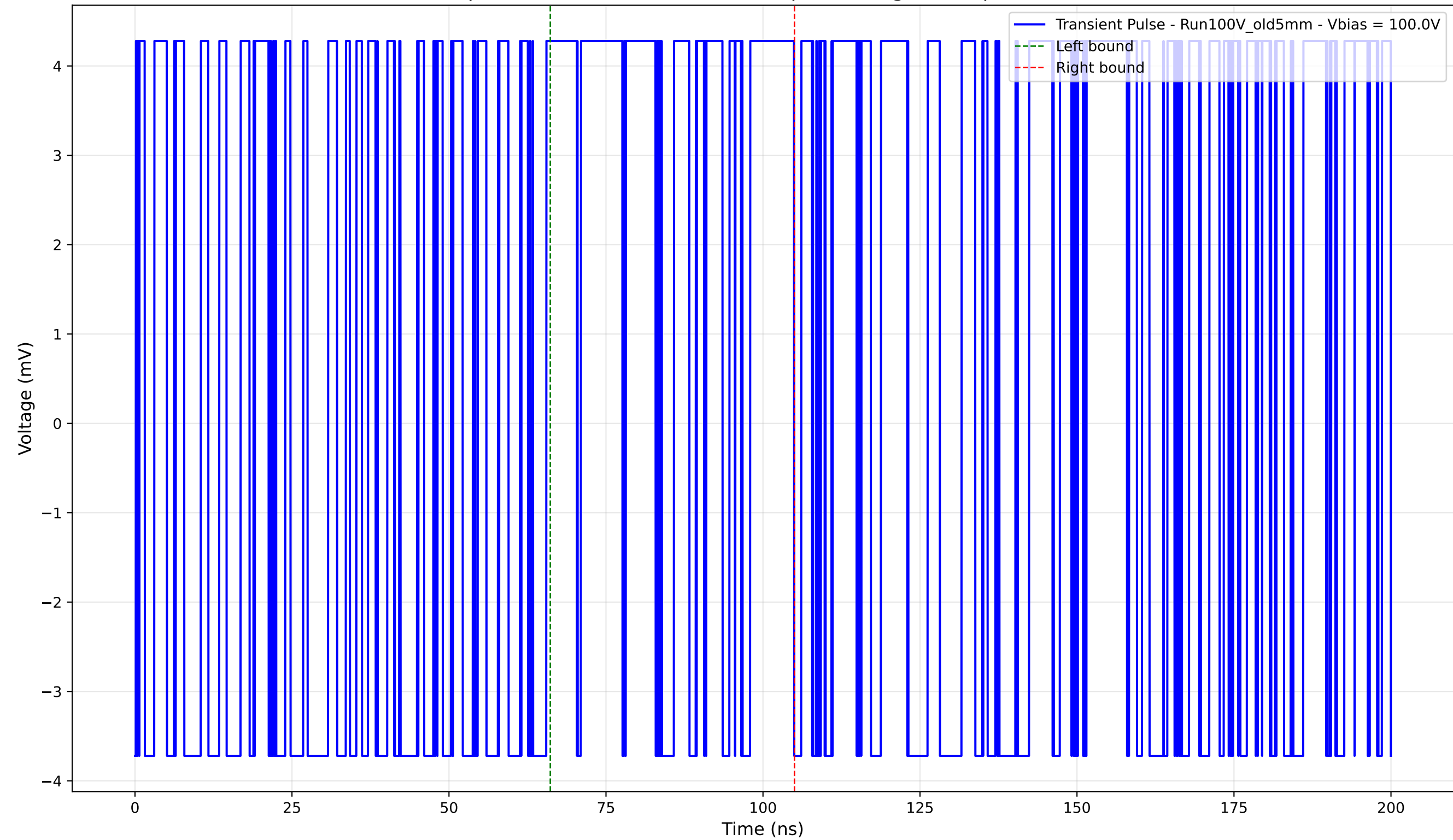
Transient Pulse - Sample: Old5mm - Position: 2770.0 \mu\text{m} - Charge: 2.19 pC - Rise Time: 0.00 ns (N/A)
