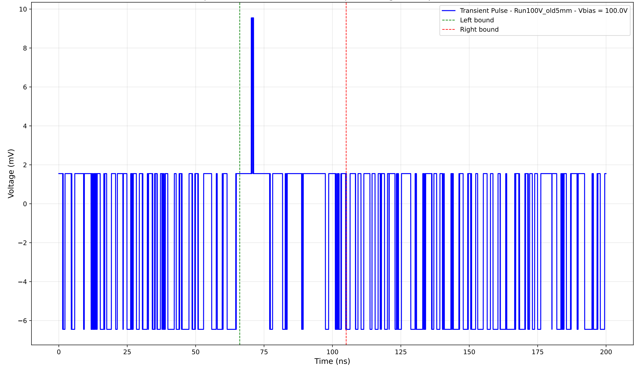
Transient Pulse - Sample: Old5mm - Position: 3125.0 \mu\text{m} - Charge: 0.39 pC - Rise Time: 0.00 ns (N/A)
