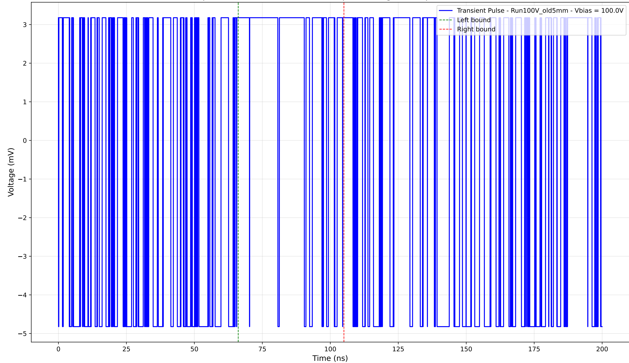
Transient Pulse - Sample: Old5mm - Position: 2510.0 \mu\text{m} - Charge: 1.79 pC - Rise Time: 0.00 ns (N/A)
