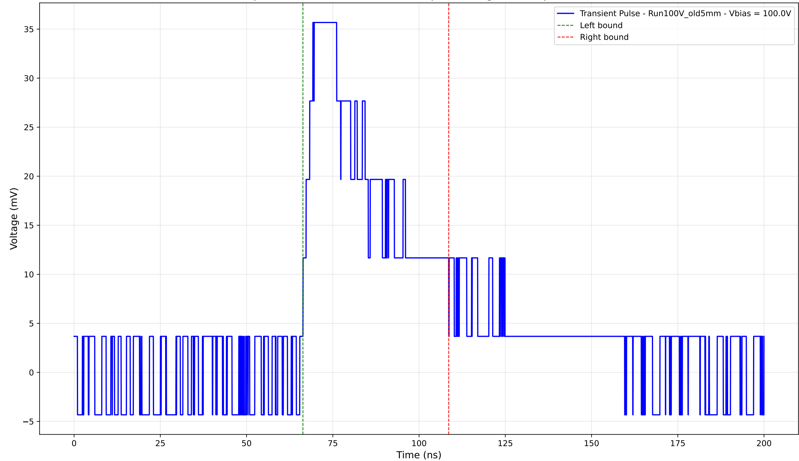
Transient Pulse - Sample: Old5mm - Position: 4950.0 \mu\text{m} - Charge: 17.00 pC - Rise Time: 0.00 ns (N/A)
