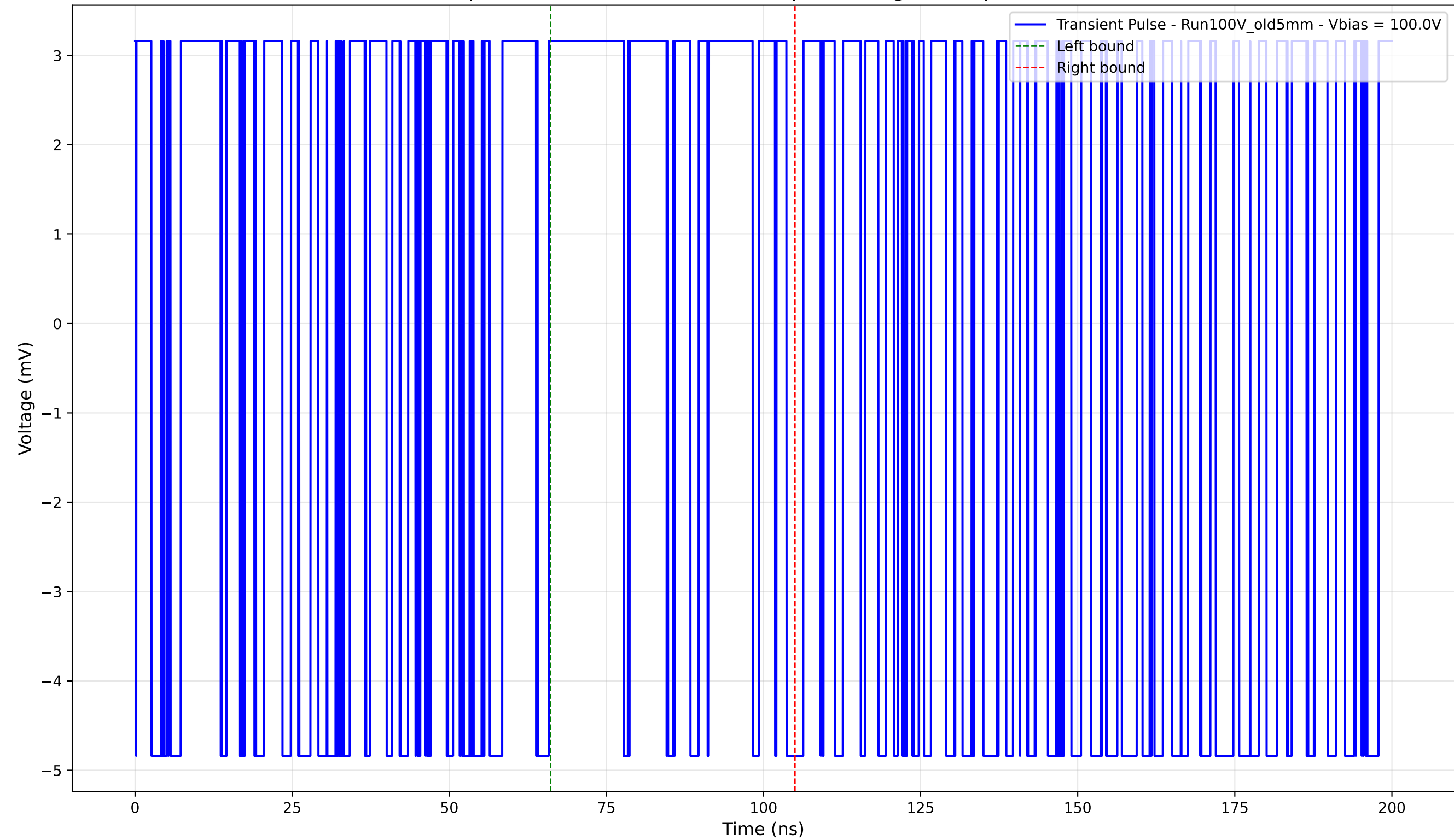
Transient Pulse - Sample: Old5mm - Position: 4315.0 \mu\text{m} - Charge: 1.52 pC - Rise Time: 0.00 ns (N/A)
