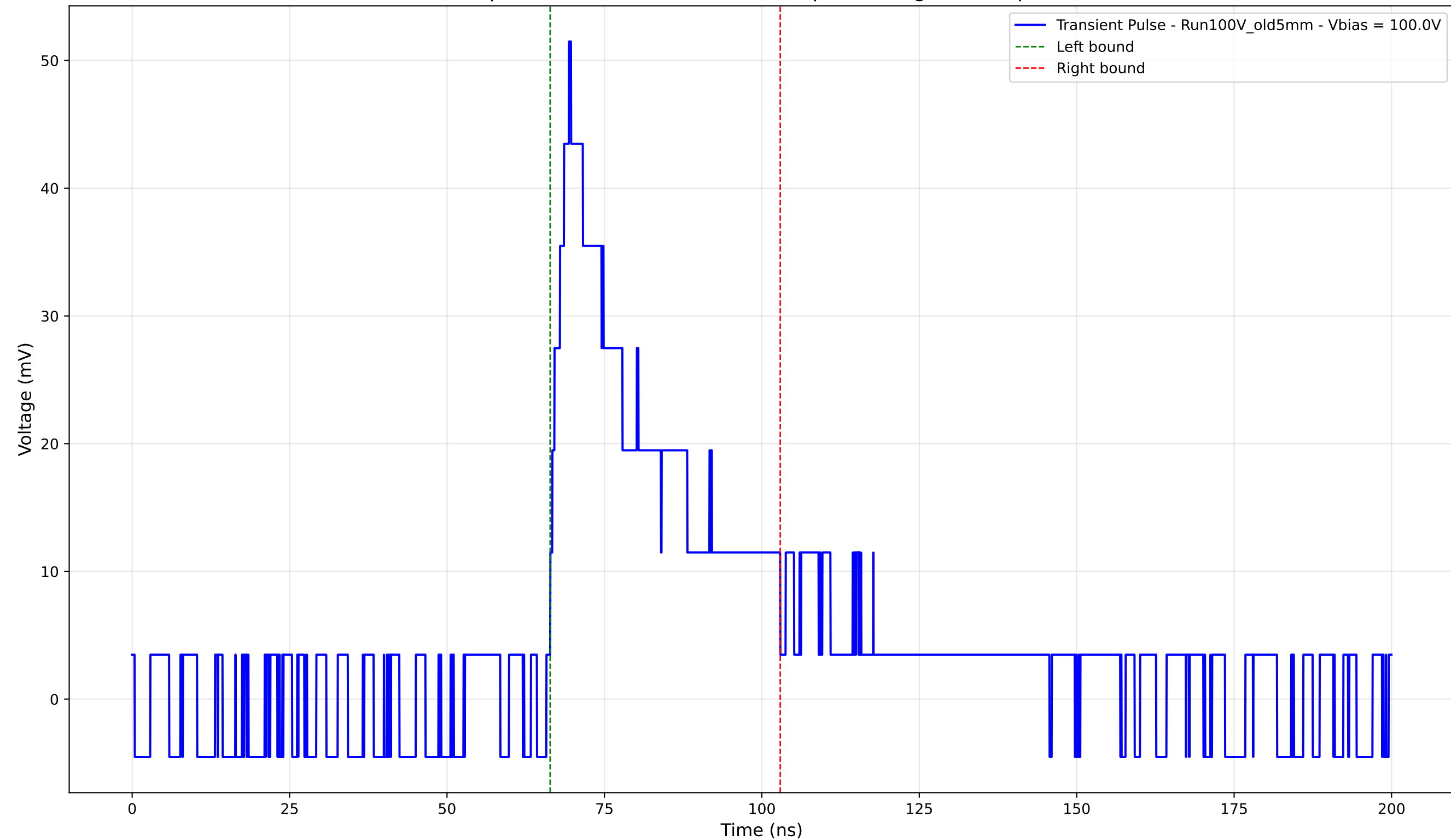
Transient Pulse - Sample: Old5mm - Position: 4740.0 \mu\text{m} - Charge: 15.24 pC - Rise Time: 2.98 ns
