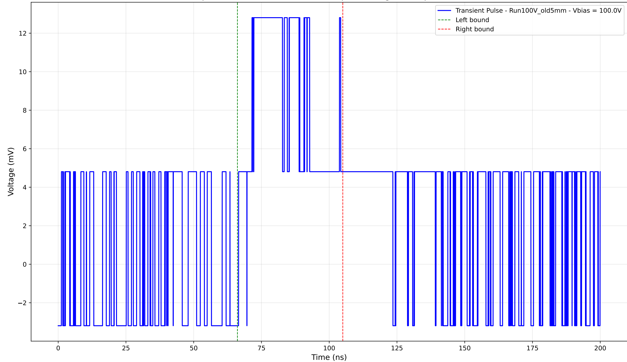
Transient Pulse - Sample: Old5mm - Position: 1070.0 \mu\text{m} - Charge: 6.57 pC - Rise Time: 0.00 ns (N/A)
