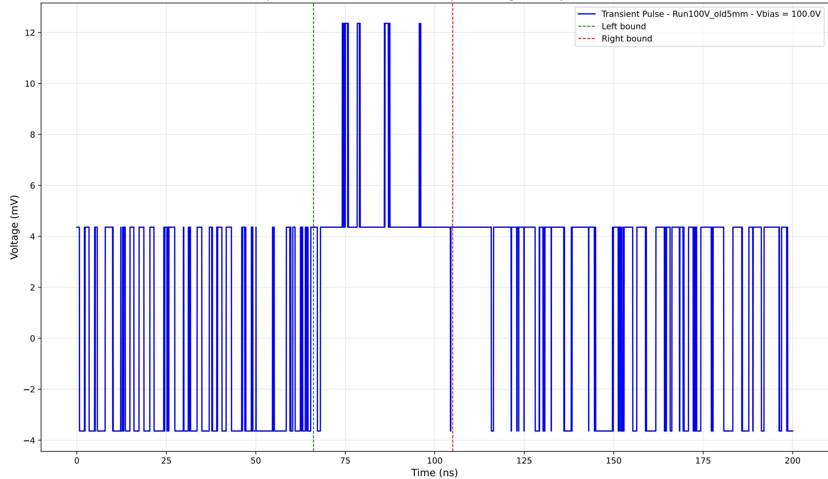
Transient Pulse - Sample: Old5mm - Position: 1480.0 \mu\text{m} - Charge: 3.73 pC - Rise Time: 0.00 ns (N/A)
