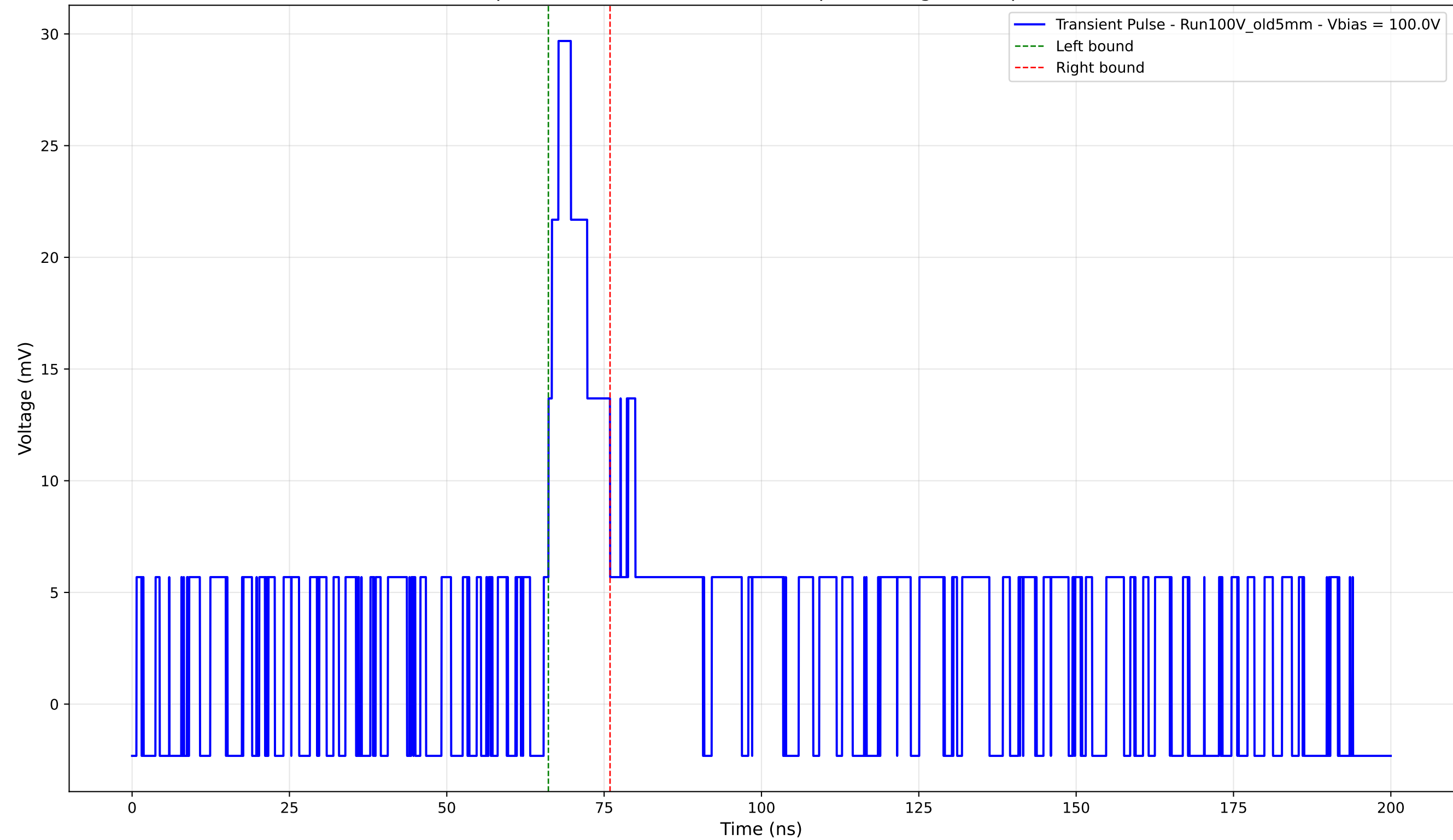
Transient Pulse - Sample: Old5mm - Position: 3155.0 \mu\text{m} - Charge: 3.89 pC - Rise Time: 2.36 ns
