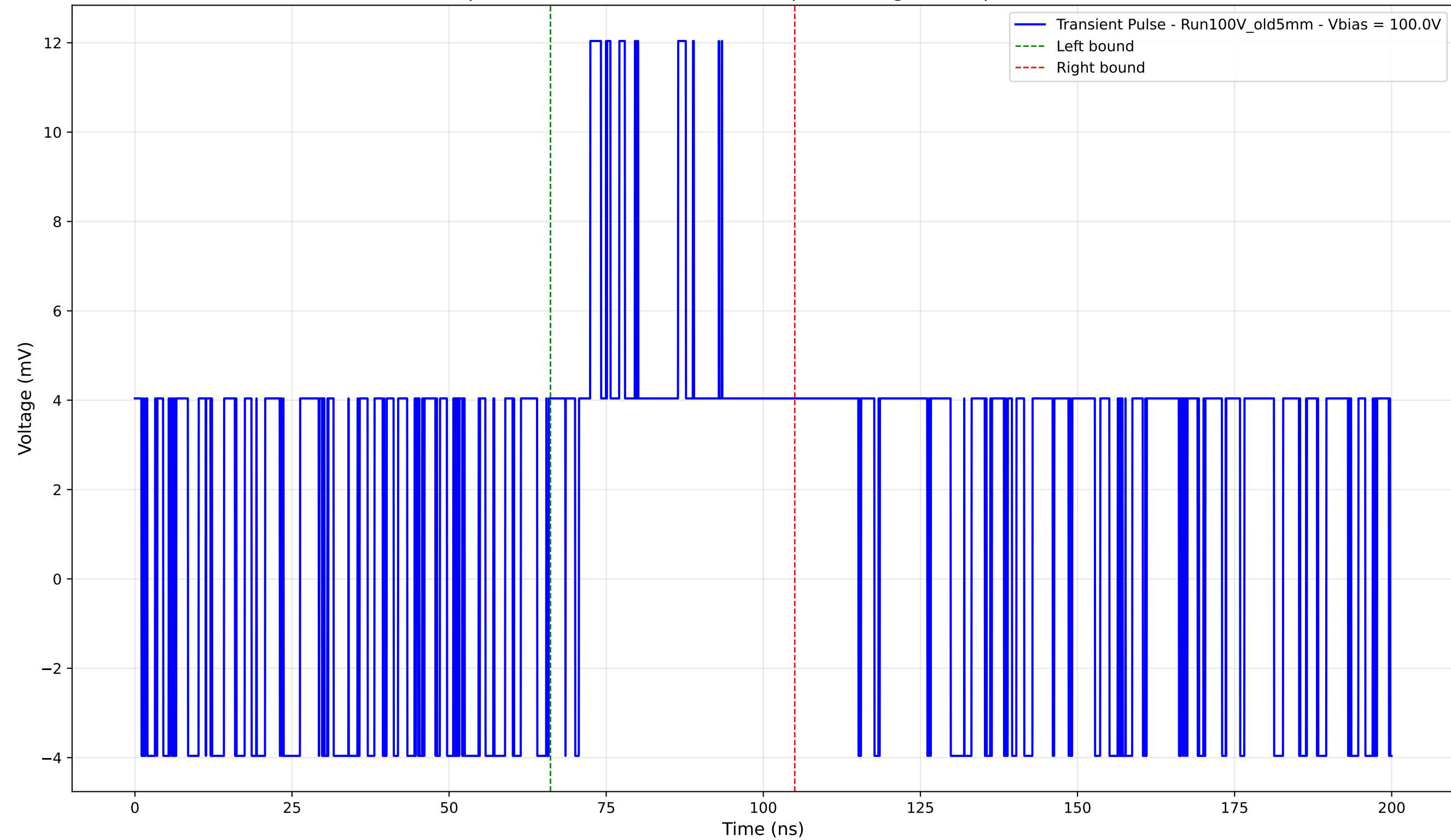
Transient Pulse - Sample: Old5mm - Position: 1470.0 \mu\text{m} - Charge: 3.83 pC - Rise Time: 0.00 ns (N/A)
