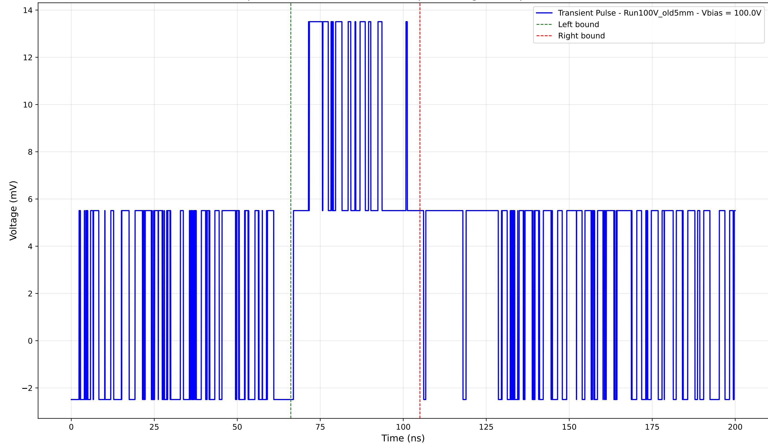
Transient Pulse - Sample: Old5mm - Position: 2280.0 \mu\text{m} - Charge: 6.24 pC - Rise Time: 0.00 ns (N/A)
