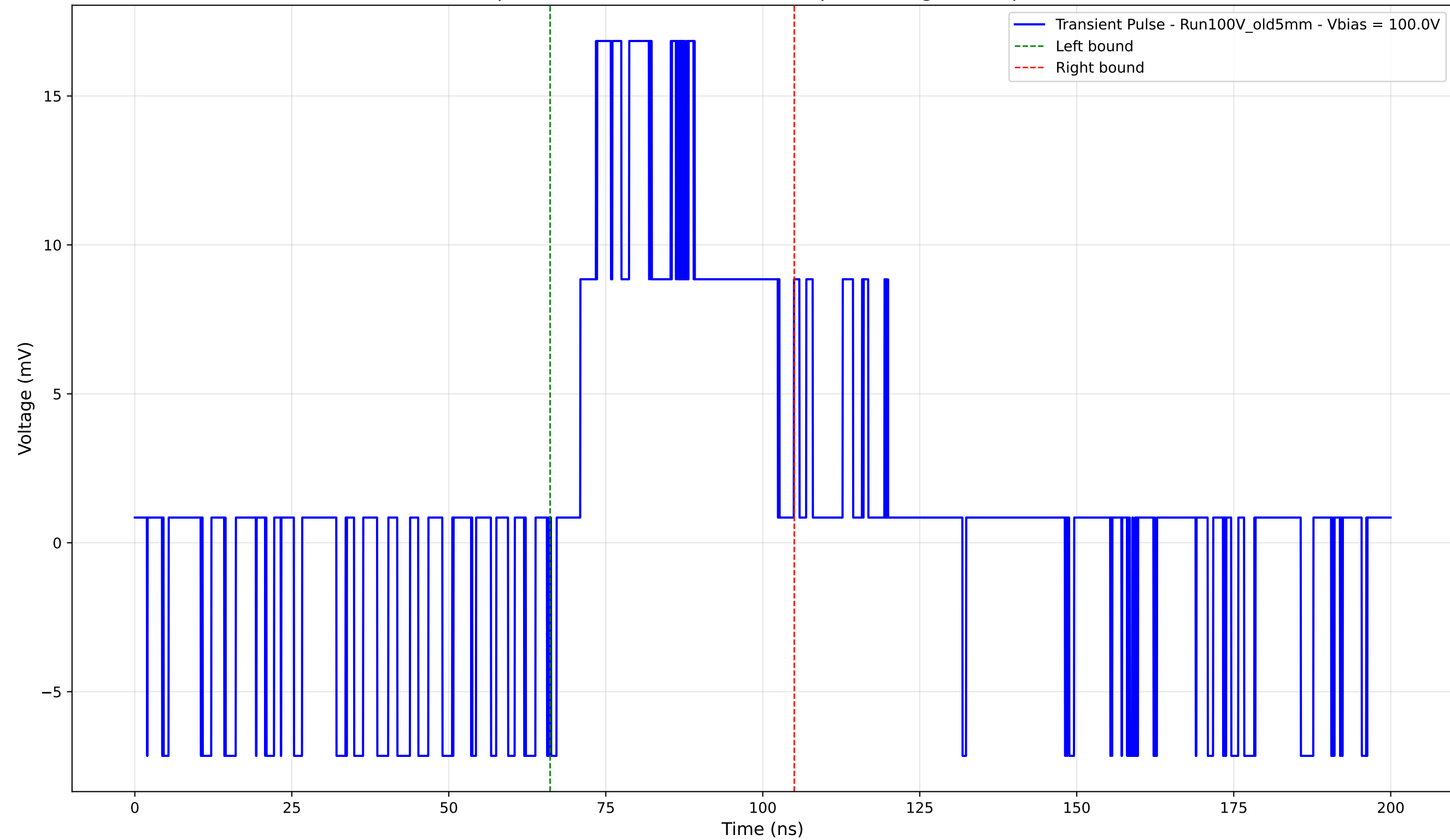
Transient Pulse - Sample: Old5mm - Position: 1600.0 \mu\text{m} - Charge: 7.13 pC - Rise Time: 2.52 ns
