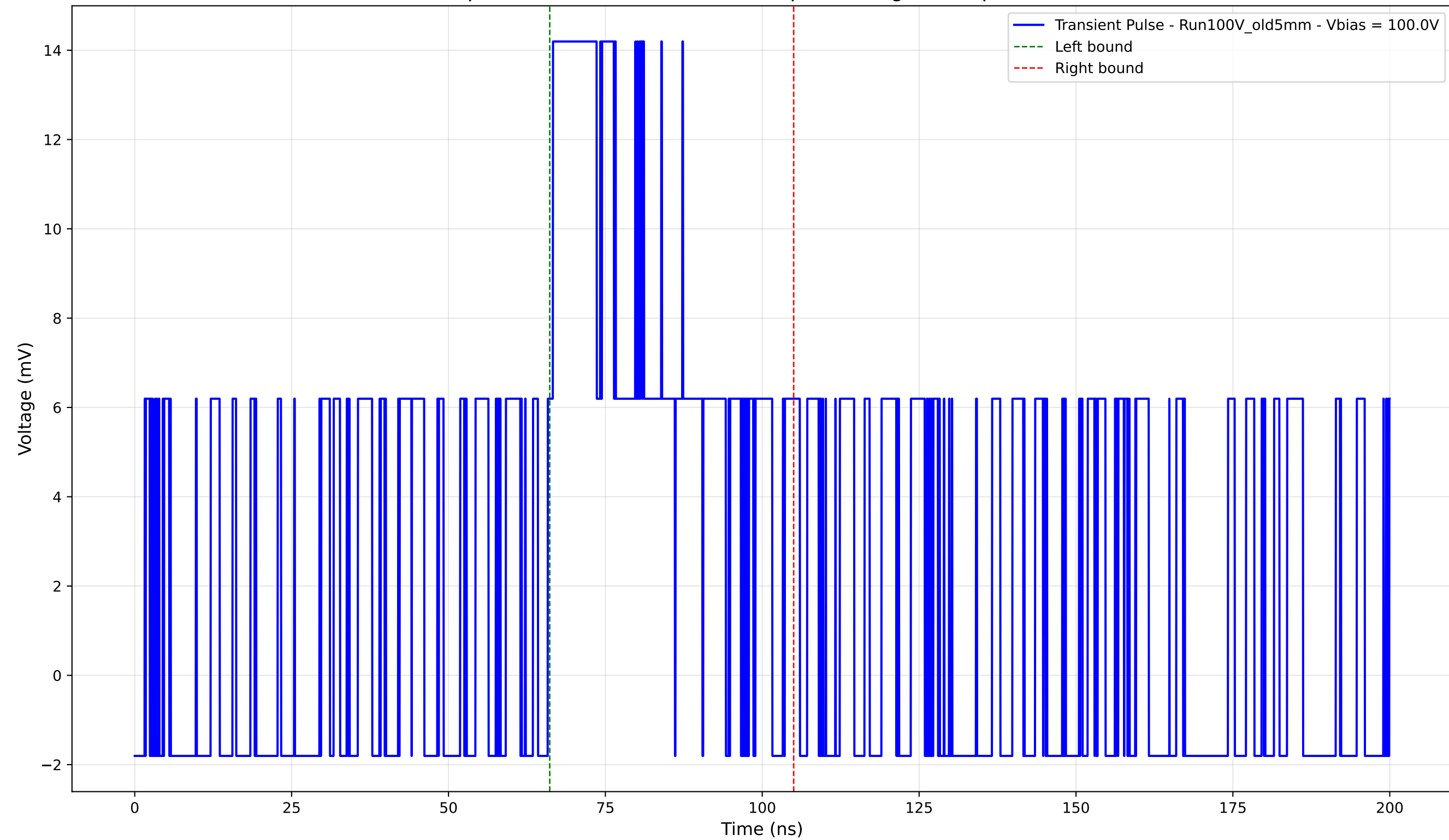
Transient Pulse - Sample: Old5mm - Position: 4565.0 \mu\text{m} - Charge: 5.88 pC - Rise Time: 0.00 ns (N/A)
