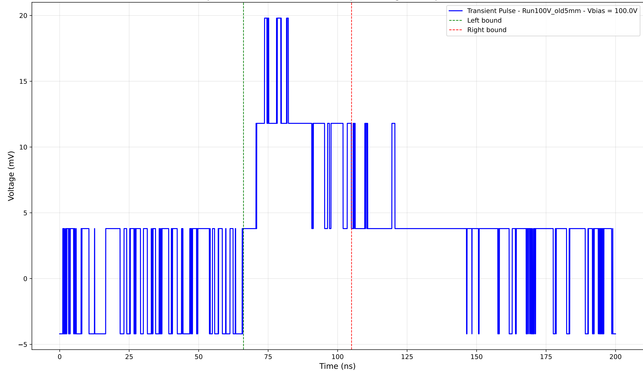
Transient Pulse - Sample: Old5mm - Position: 1780.0 \mu\text{m} - Charge: 8.35 pC - Rise Time: 0.00 ns (N/A)
