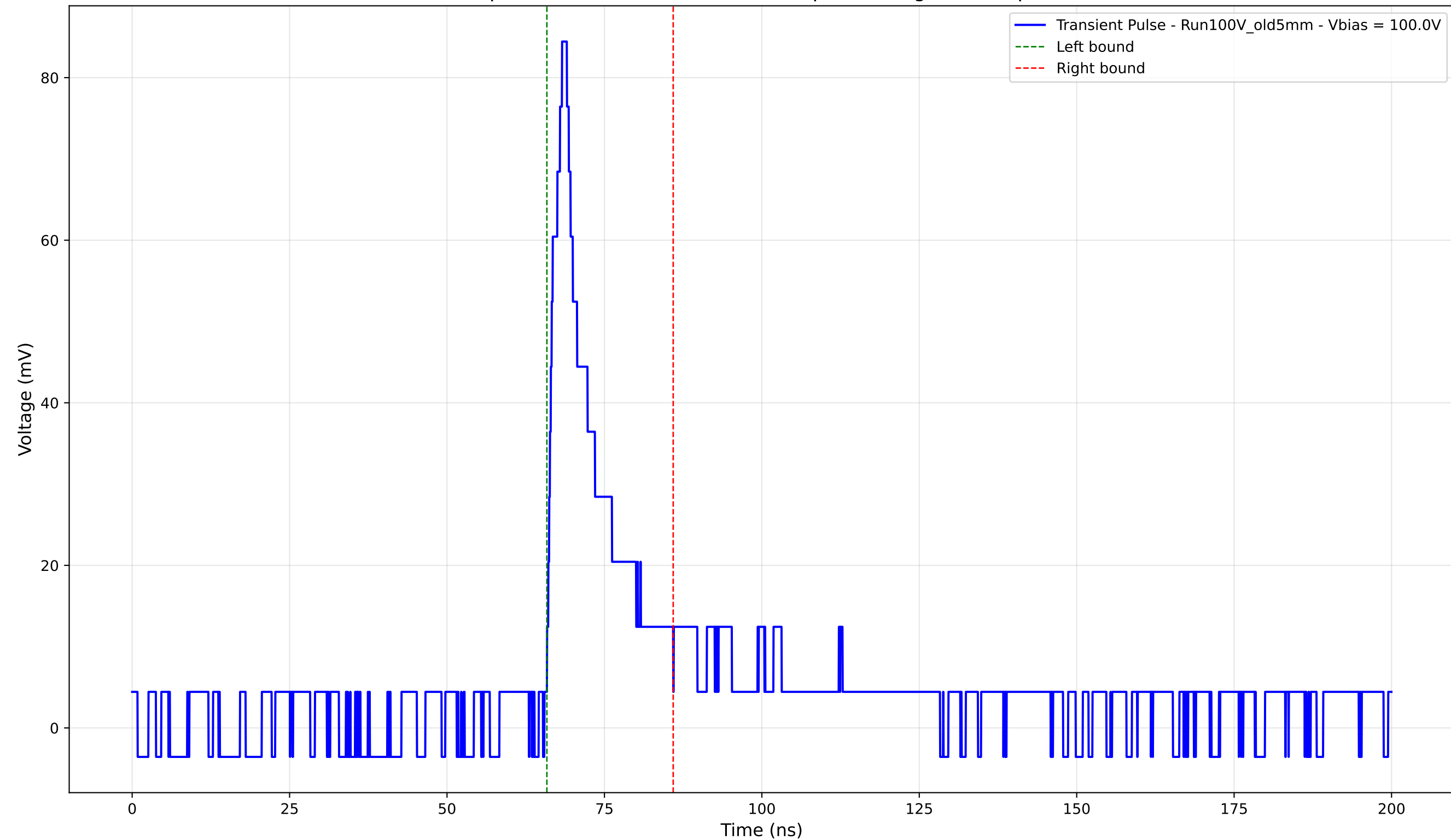
Transient Pulse - Sample: Old5mm - Position: 3195.0 \mu\text{m} - Charge: 12.76 pC - Rise Time: 2.07 ns
