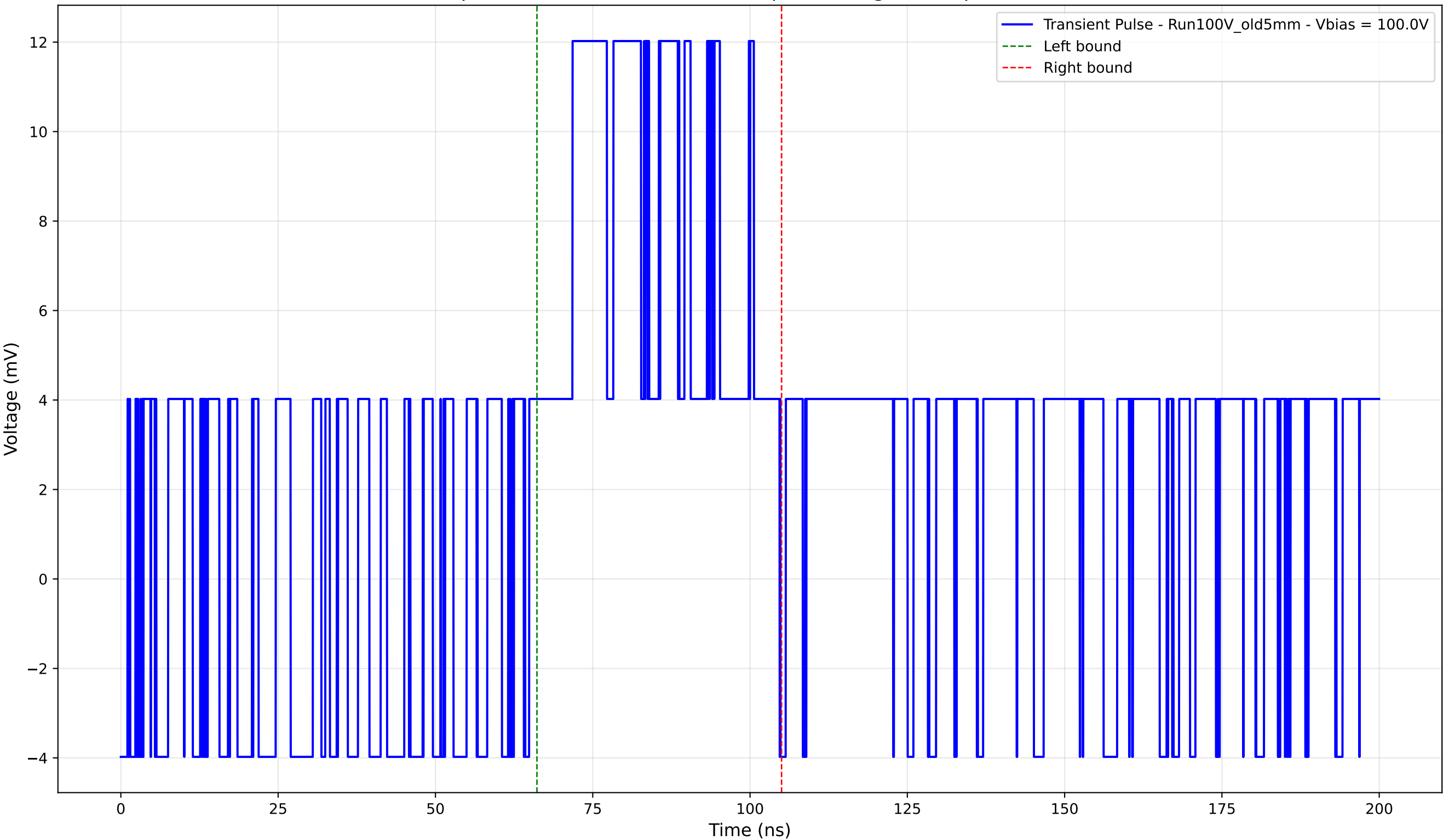
Transient Pulse - Sample: Old5mm - Position: 860.0 \mu\text{m} - Charge: 5.79 pC - Rise Time: 0.00 ns (N/A)
