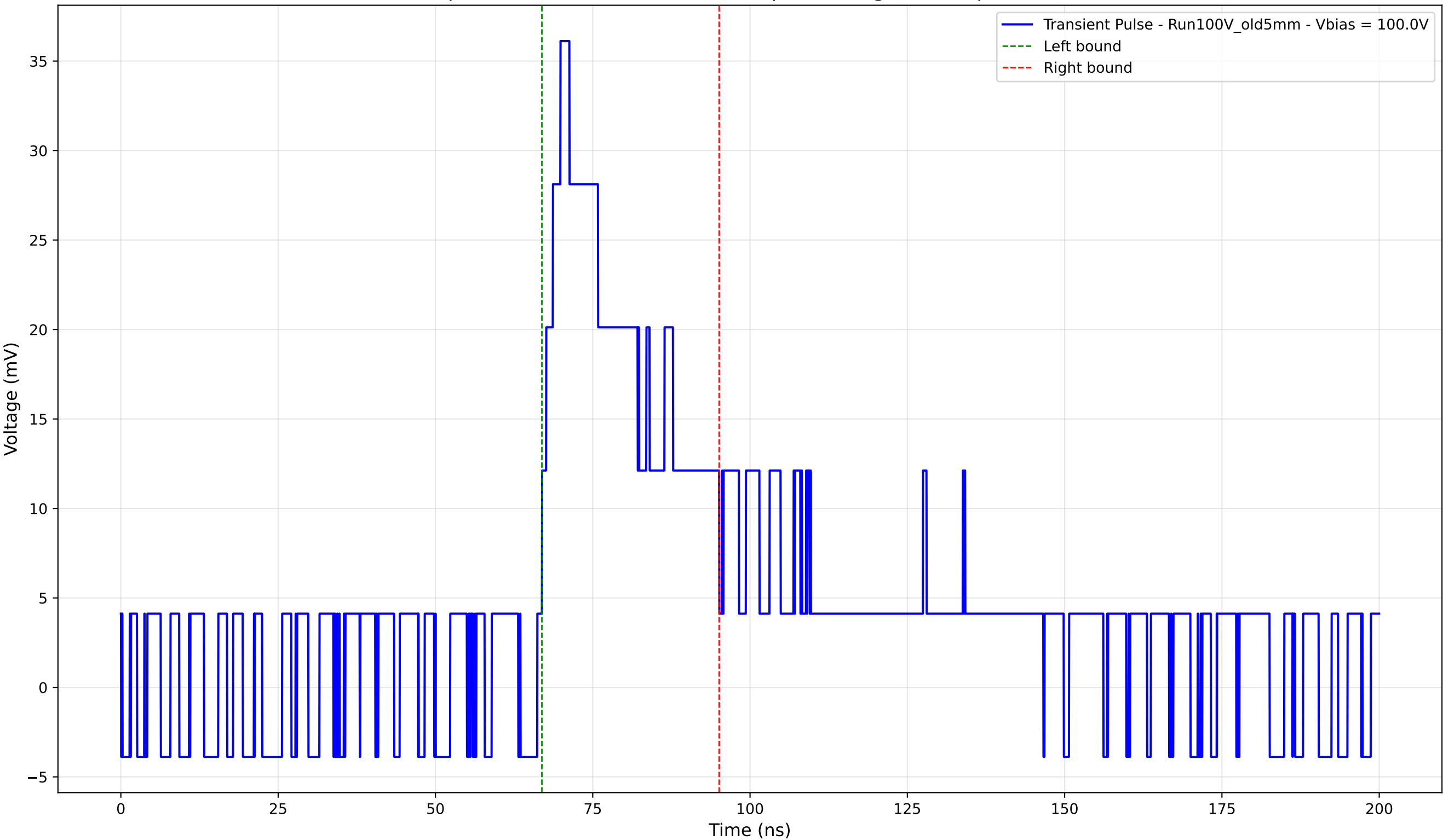
Transient Pulse - Sample: Old5mm - Position: 2595.0 \mu\text{m} - Charge: 10.86 pC - Rise Time: 0.00 ns (N/A)
