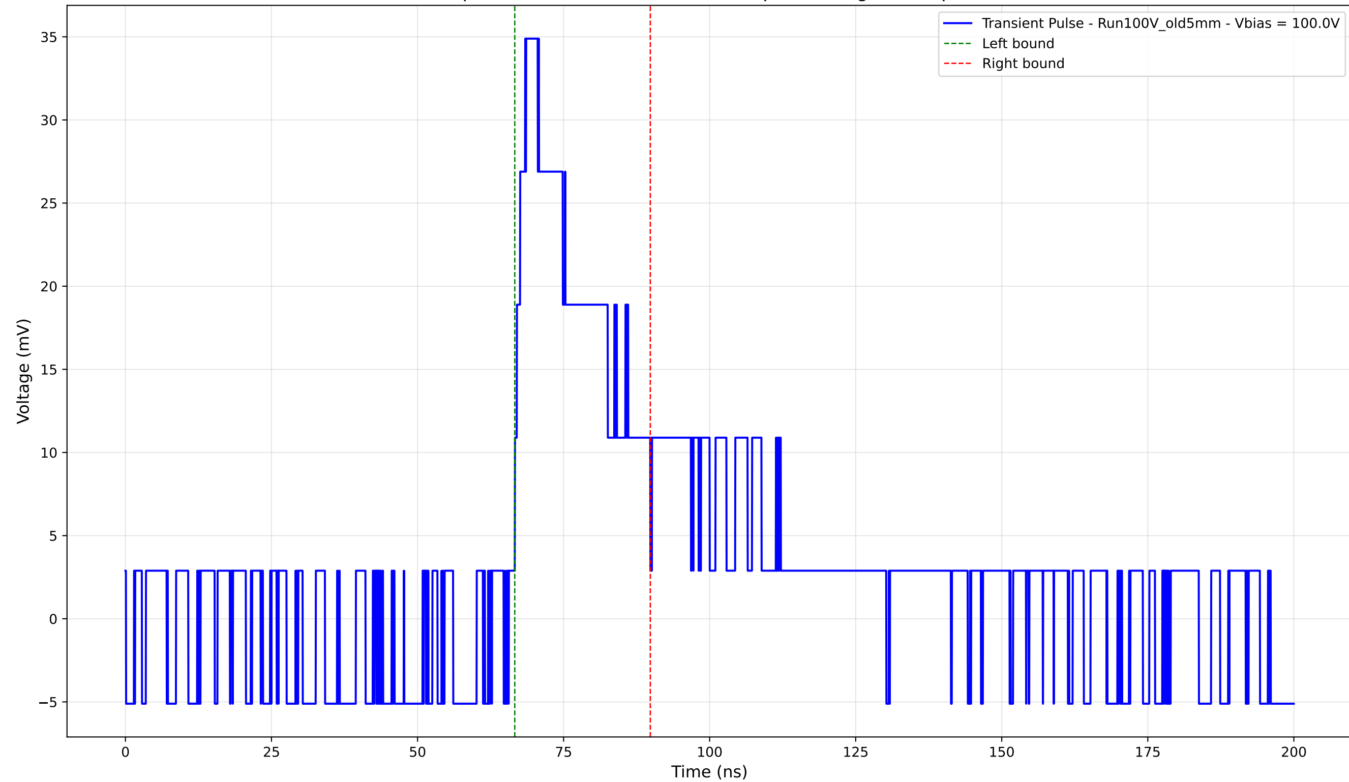
Transient Pulse - Sample: Old5mm - Position: 2700.0 \mu\text{m} - Charge: 9.16 pC - Rise Time: 1.78 ns
