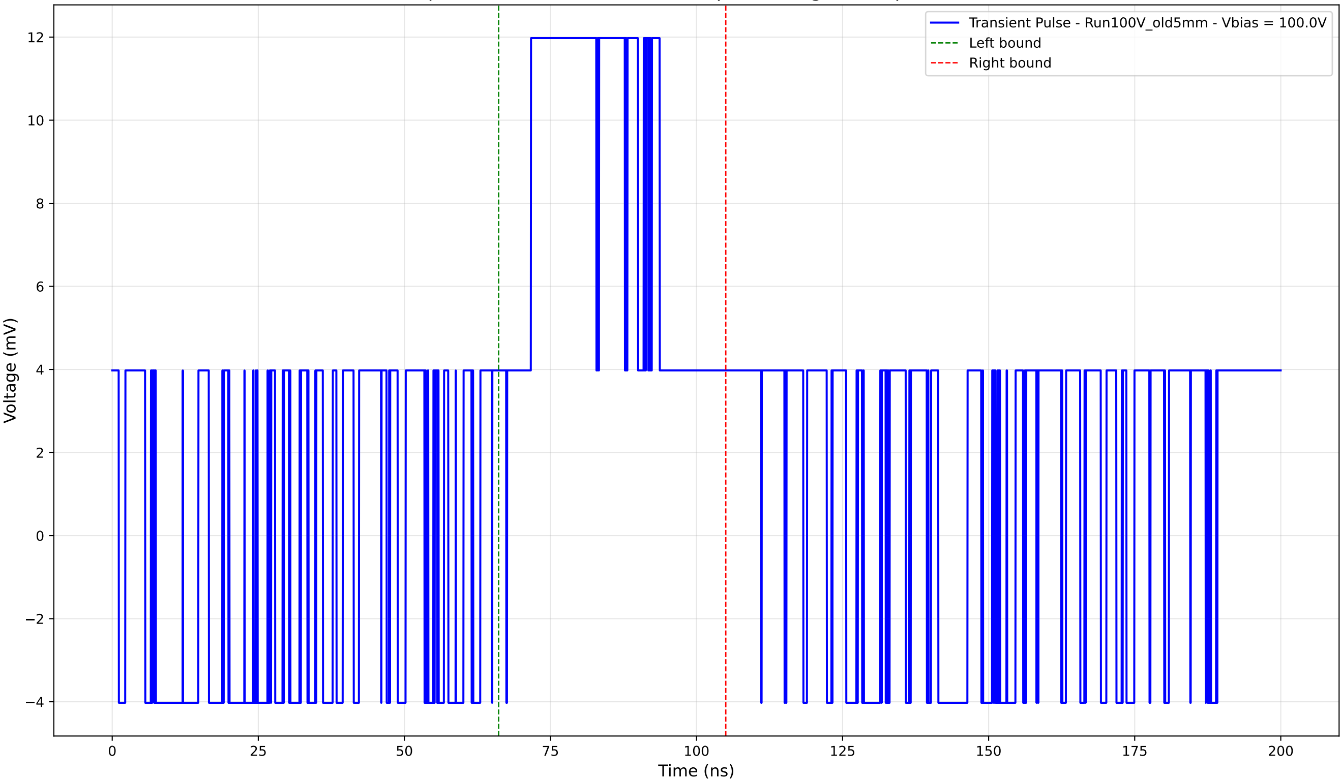
Transient Pulse - Sample: Old5mm - Position: 990.0 \mu\text{m} - Charge: 6.25 pC - Rise Time: 0.00 ns (N/A)
