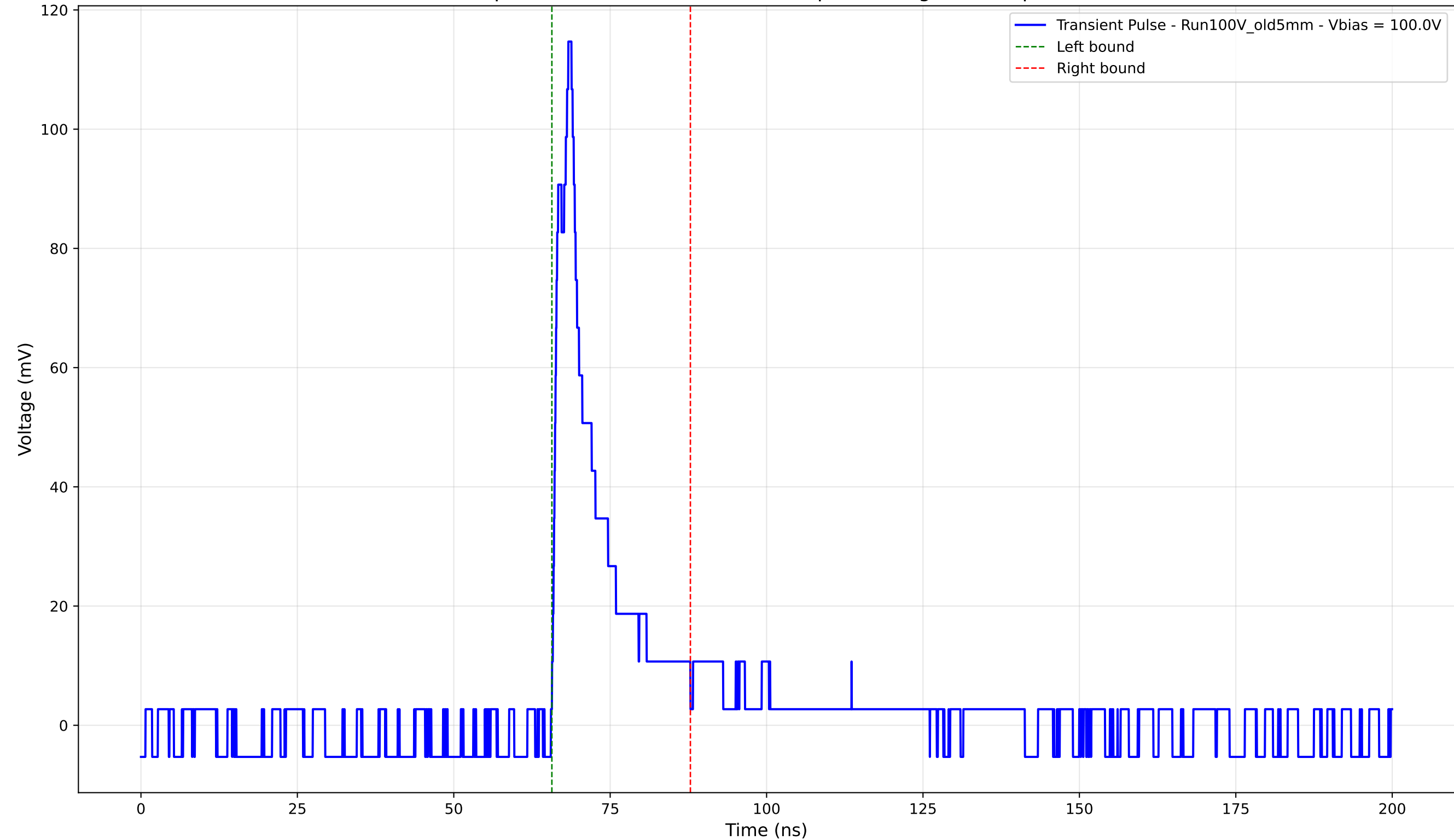
Transient Pulse - Sample: Old5mm - Position: 3300.0 \mu\text{m} - Charge: 15.14 pC - Rise Time: 2.28 ns
