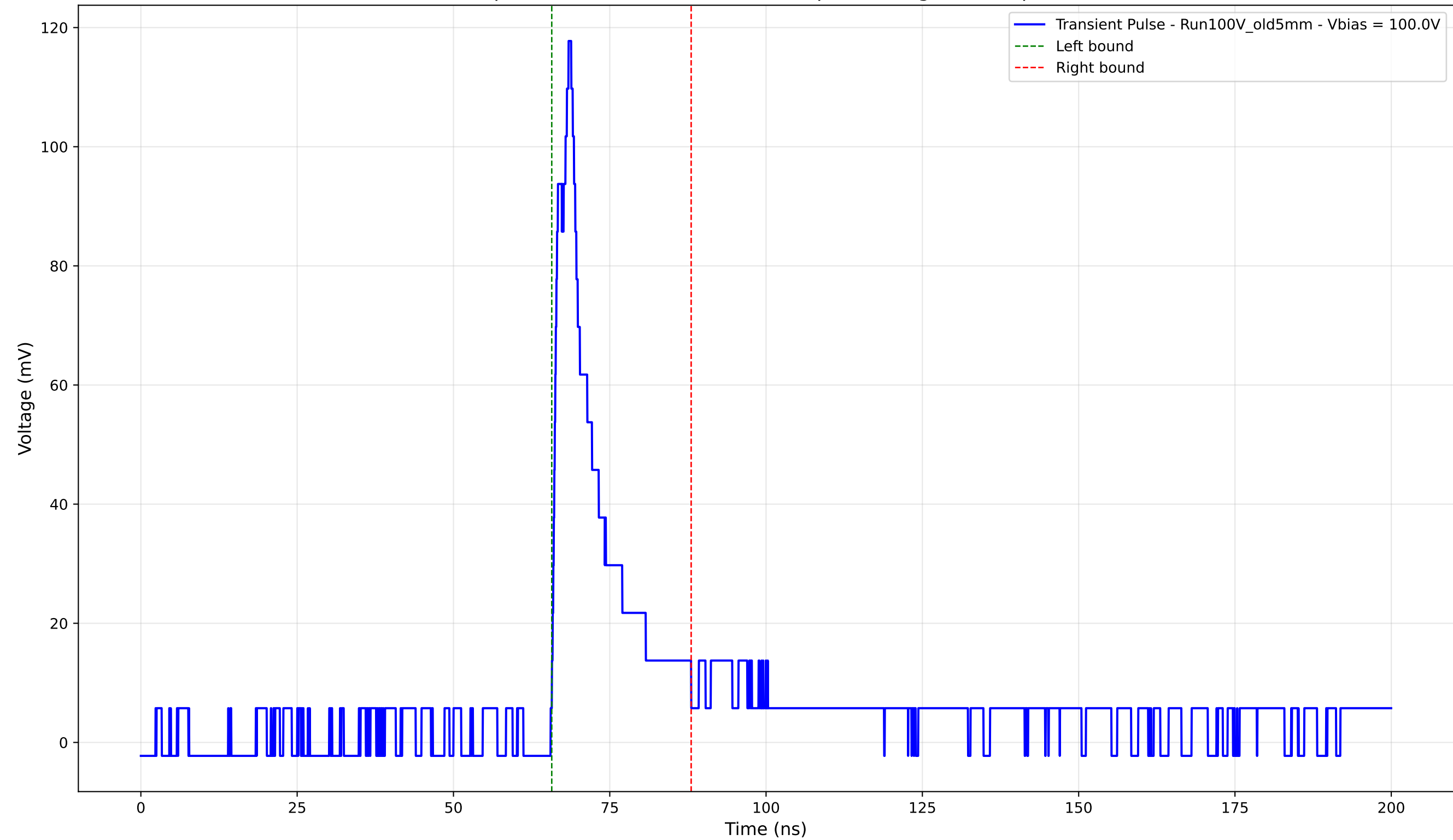
Transient Pulse - Sample: Old5mm - Position: 4135.0 \mu\text{m} - Charge: 17.03 pC - Rise Time: 2.40 ns
