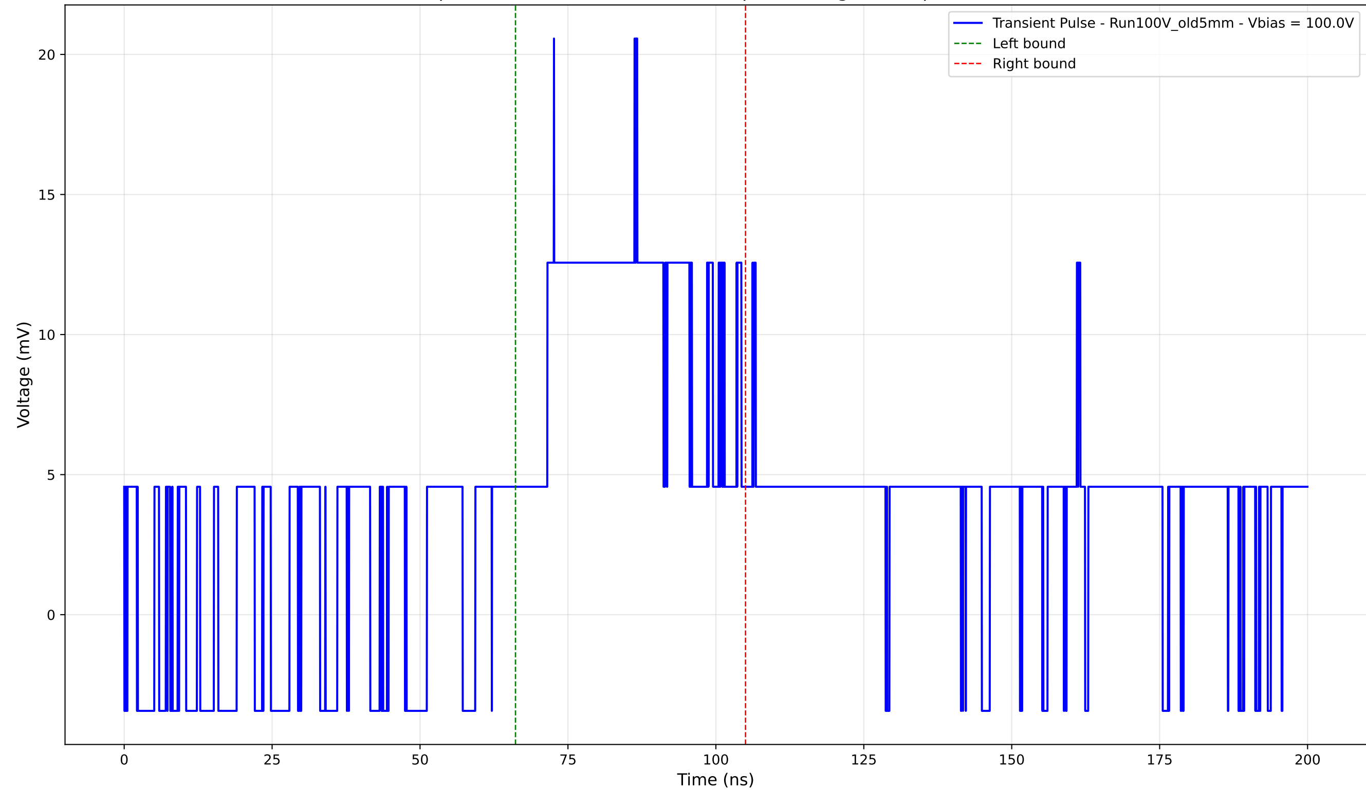
Transient Pulse - Sample: Old5mm - Position: 1650.0 \mu\text{m} - Charge: 7.78 pC - Rise Time: 0.00 ns (N/A)
