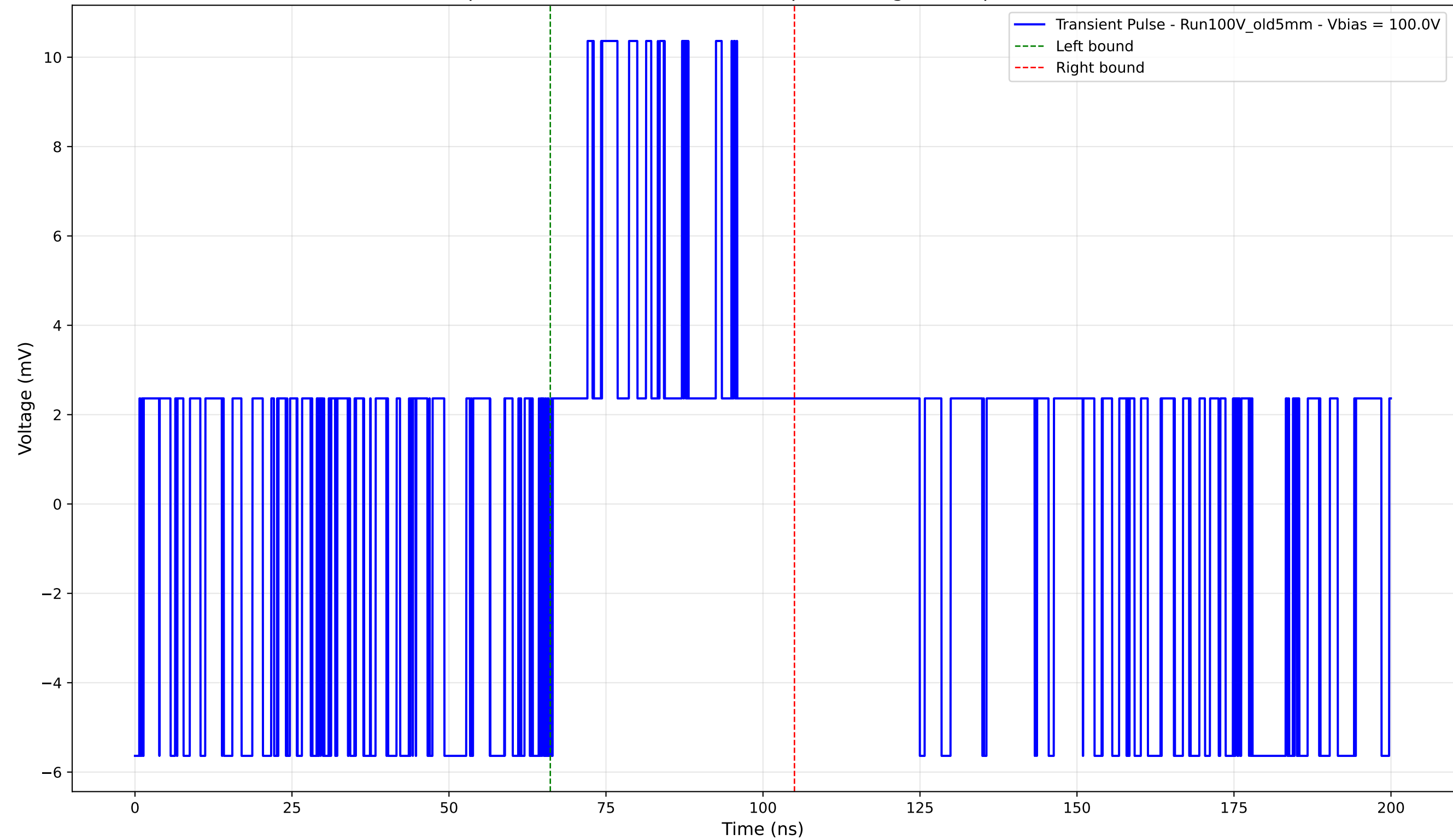
Transient Pulse - Sample: Old5mm - Position: 1355.0 \mu\text{m} - Charge: 3.14 pC - Rise Time: 0.00 ns (N/A)
