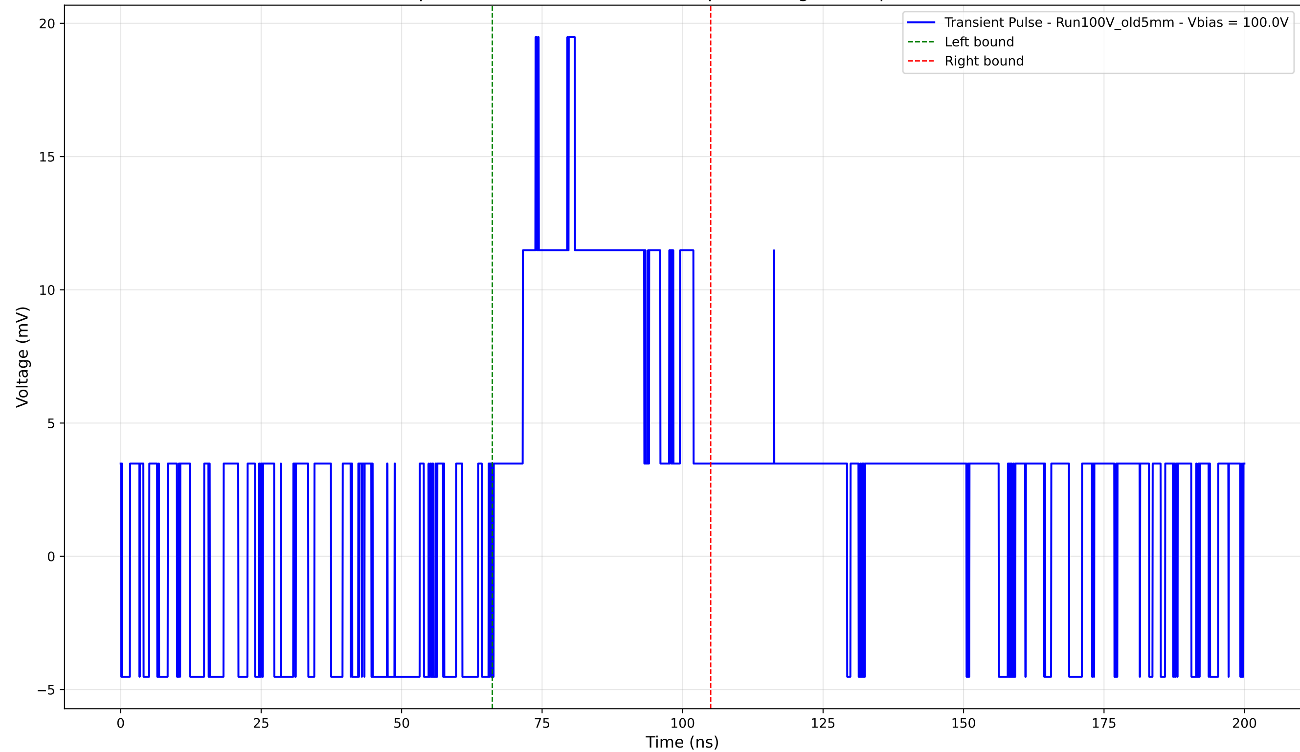
Transient Pulse - Sample: Old5mm - Position: 1385.0 \mu\text{m} - Charge: 7.21 pC - Rise Time: 0.00 ns (N/A)
