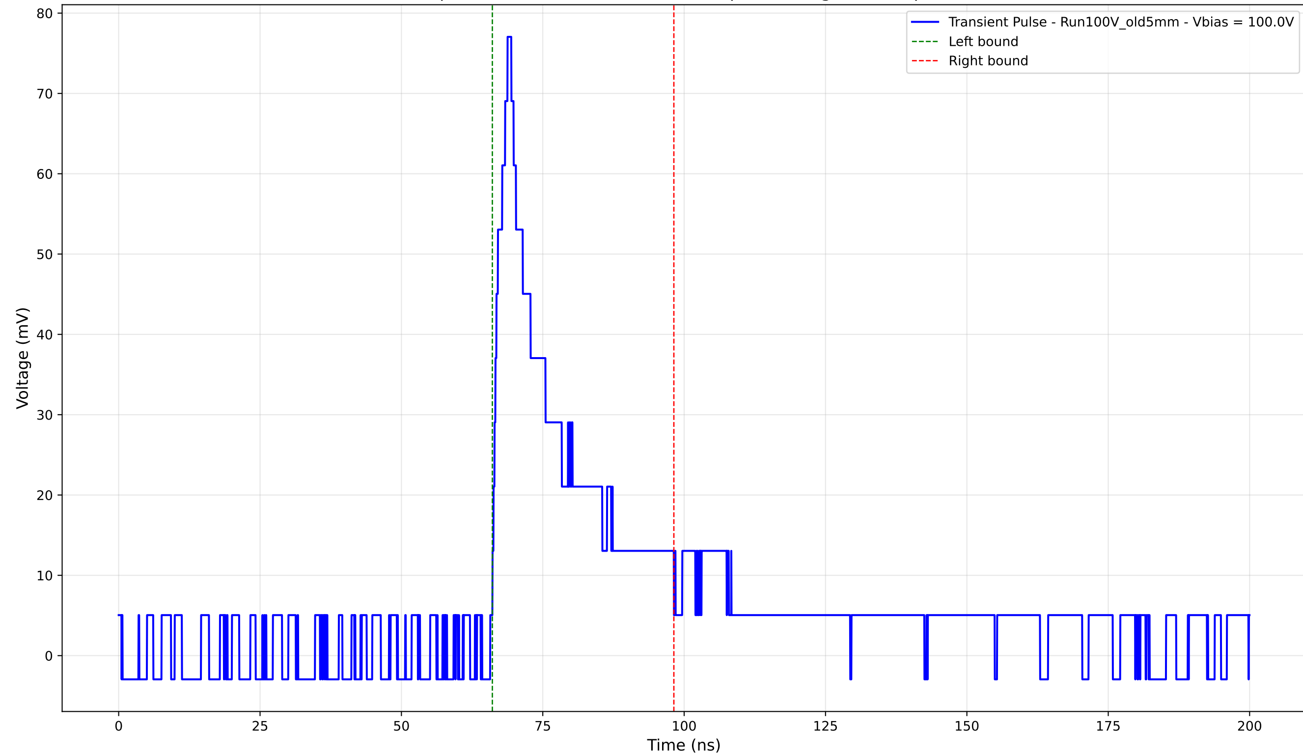
Transient Pulse - Sample: Old5mm - Position: 4445.0 \mu\text{m} - Charge: 17.36 pC - Rise Time: 2.67 ns
