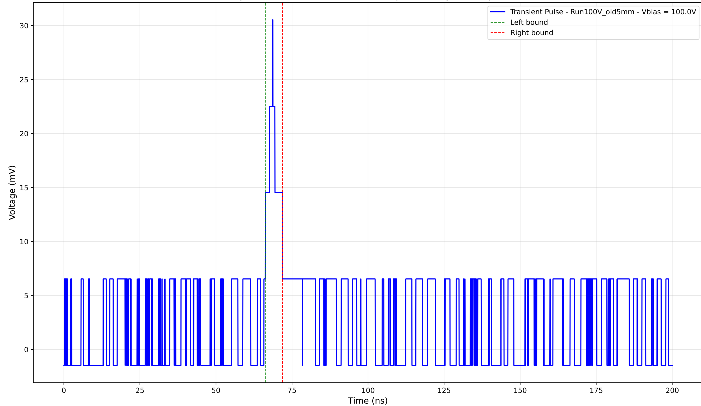
Transient Pulse - Sample: Old5mm - Position: 3440.0 \mu\text{m} - Charge: 1.94 pC - Rise Time: 2.85 ns
