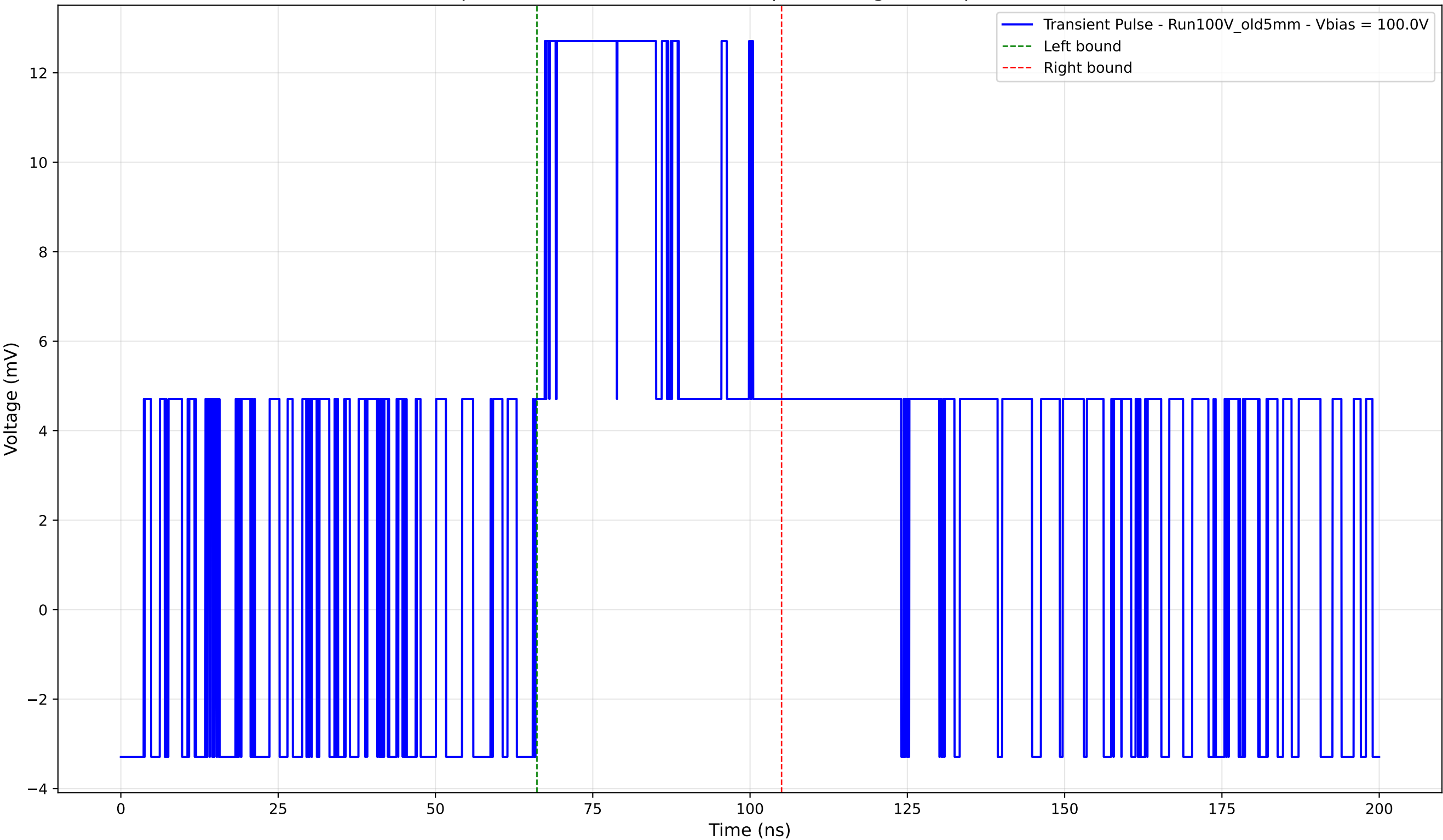
Transient Pulse - Sample: Old5mm - Position: 330.0 \mu\text{m} - Charge: 6.95 pC - Rise Time: 0.00 ns (N/A)
