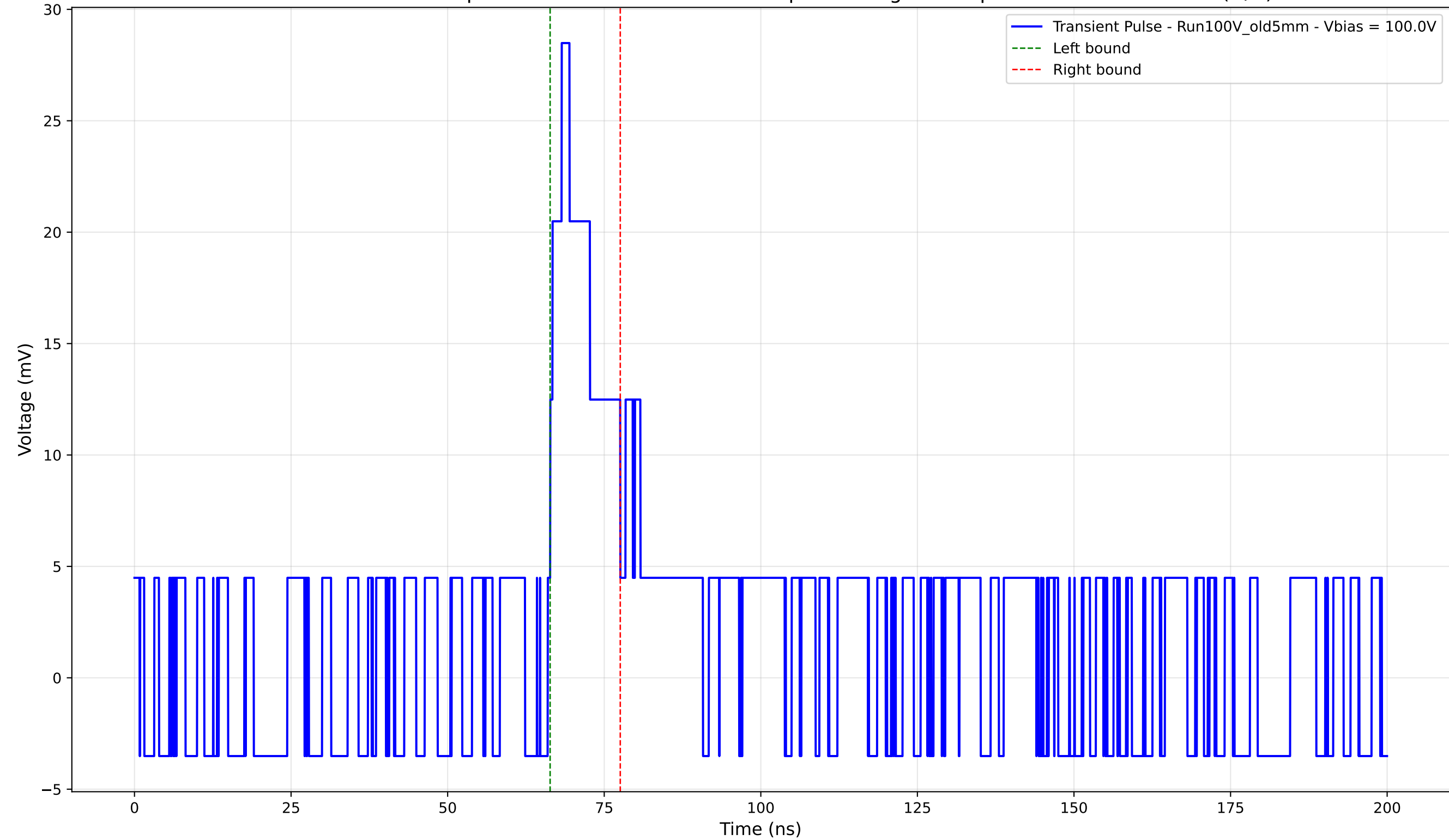
Transient Pulse - Sample: Old5mm - Position: 4370.0 \mu\text{m} - Charge: 3.95 pC - Rise Time: 0.00 ns (N/A)
