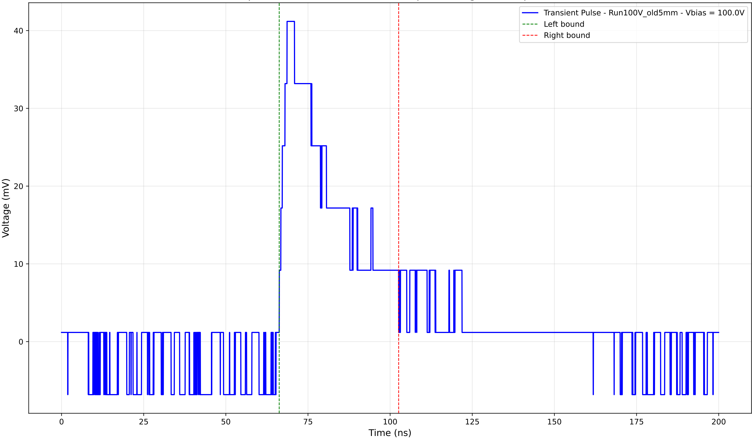
Transient Pulse - Sample: Old5mm - Position: 4800.0 \mu\text{m} - Charge: 14.12 pC - Rise Time: 2.37 ns
