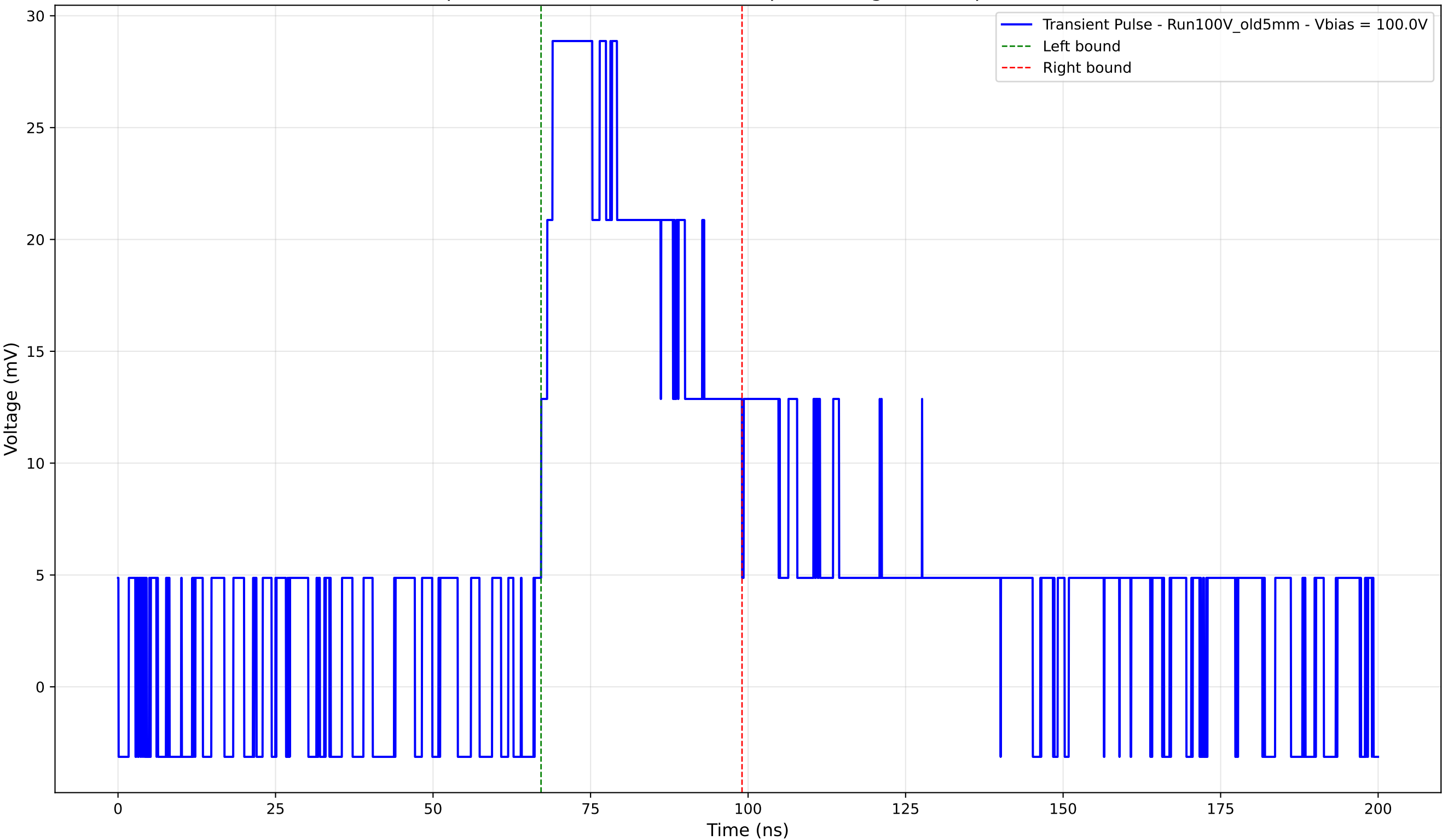
Transient Pulse - Sample: Old5mm - Position: 2415.0 \mu\text{m} - Charge: 12.96 pC - Rise Time: 0.00 ns (N/A)
