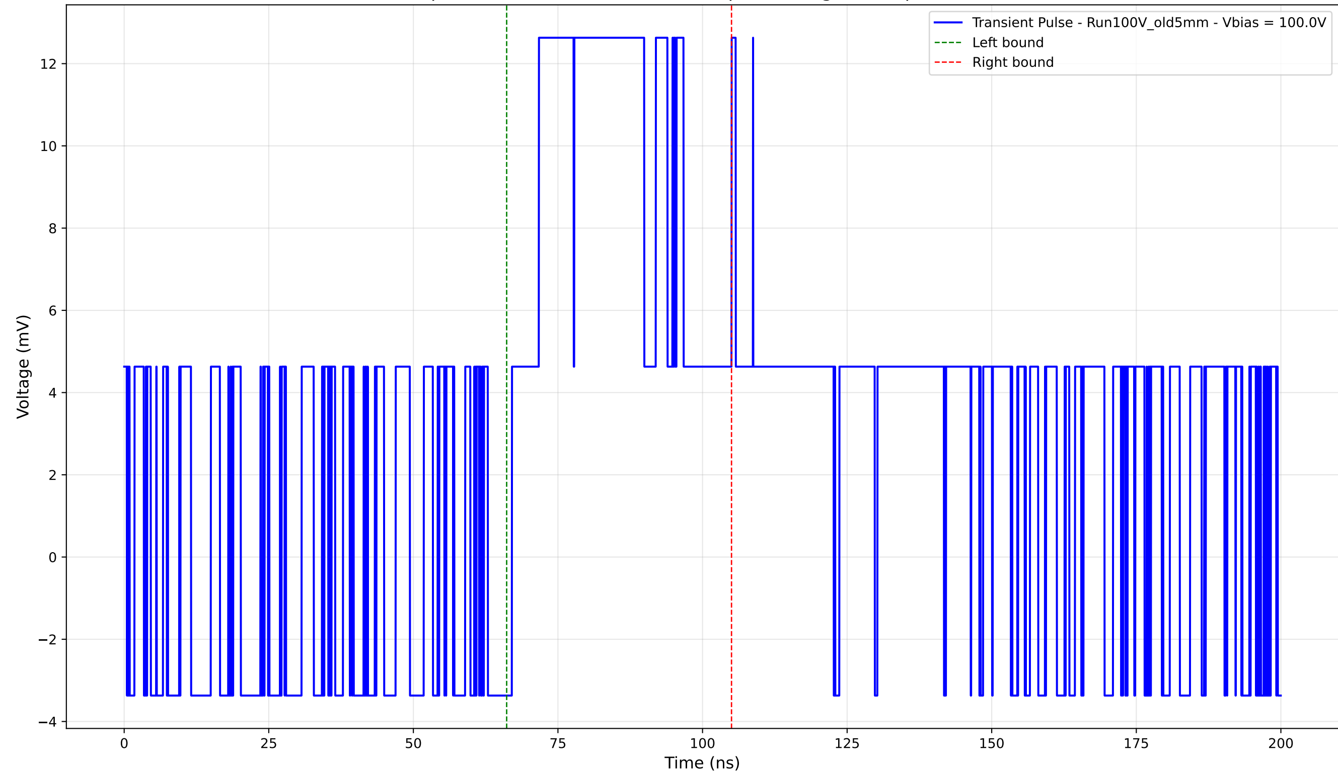
Transient Pulse - Sample: Old5mm - Position: 1565.0 \mu\text{m} - Charge: 6.92 pC - Rise Time: 0.00 ns (N/A)
