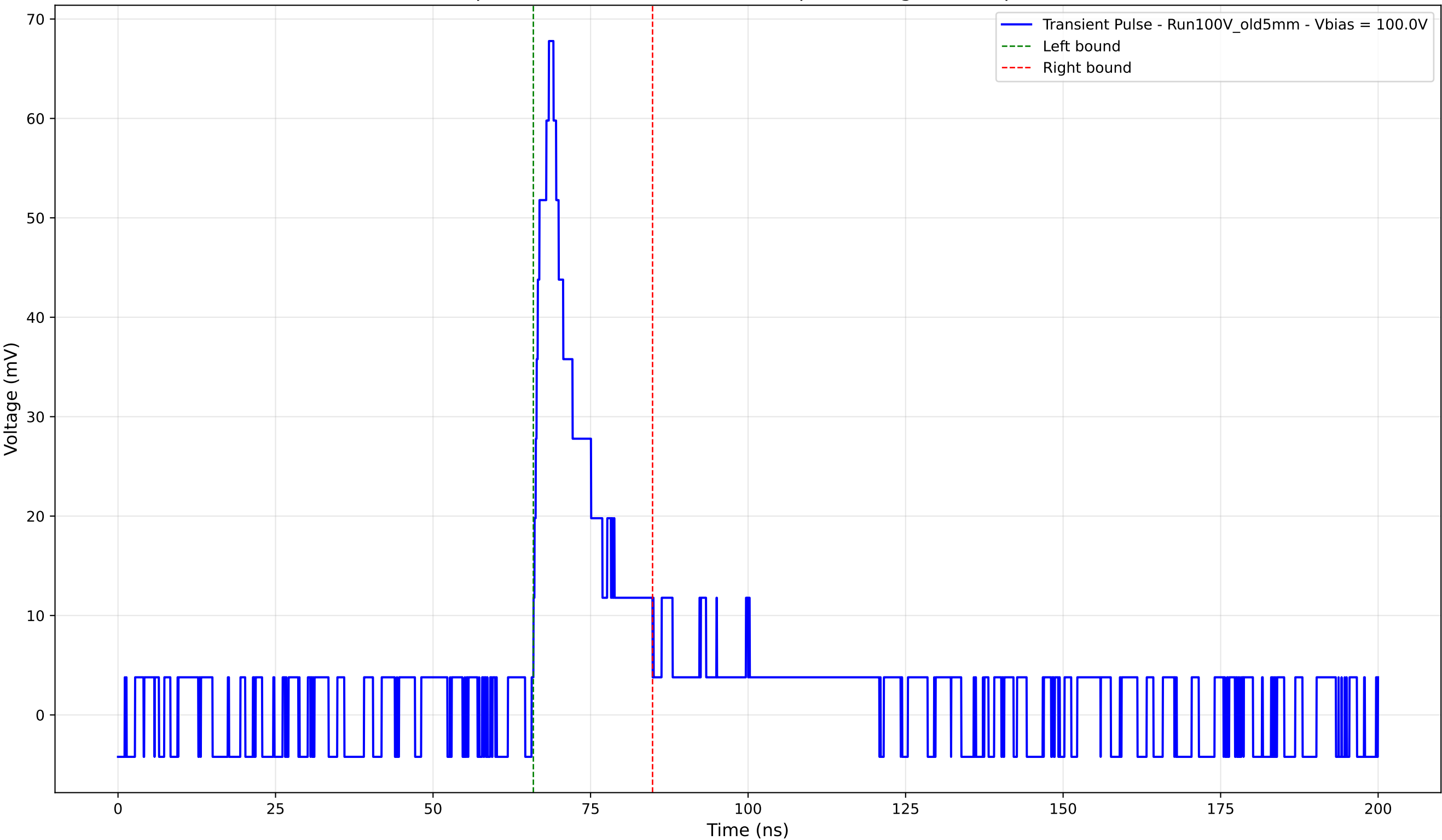
Transient Pulse - Sample: Old5mm - Position: 4225.0 \mu\text{m} - Charge: 10.15 pC - Rise Time: 2.45 ns
