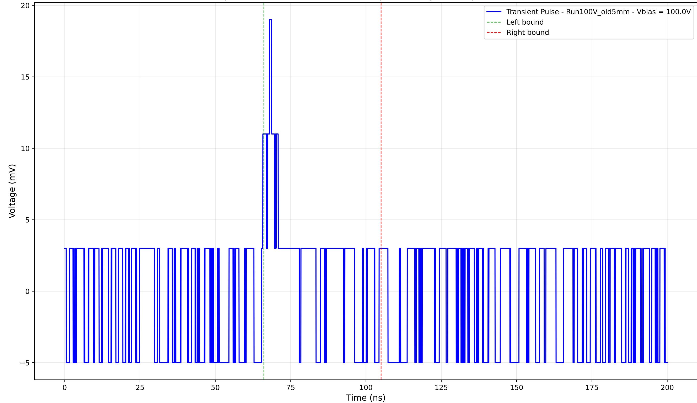
Transient Pulse - Sample: Old5mm - Position: 3730.0 \mu\text{m} - Charge: 1.85 pC - Rise Time: 0.00 ns (N/A)
