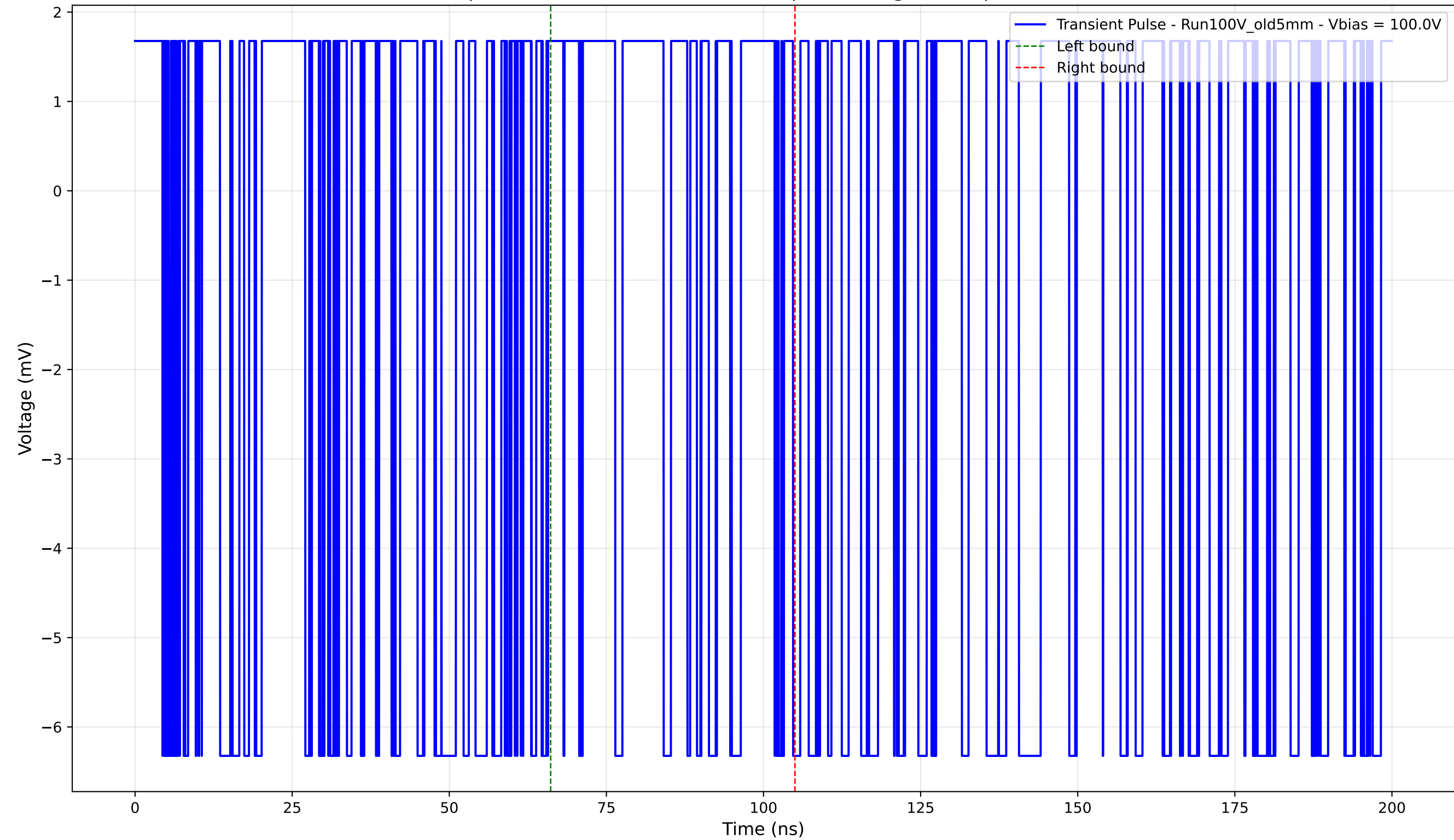
Transient Pulse - Sample: Old5mm - Position: 2805.0 \mu\text{m} - Charge: 0.03 pC - Rise Time: 0.00 ns (N/A)
