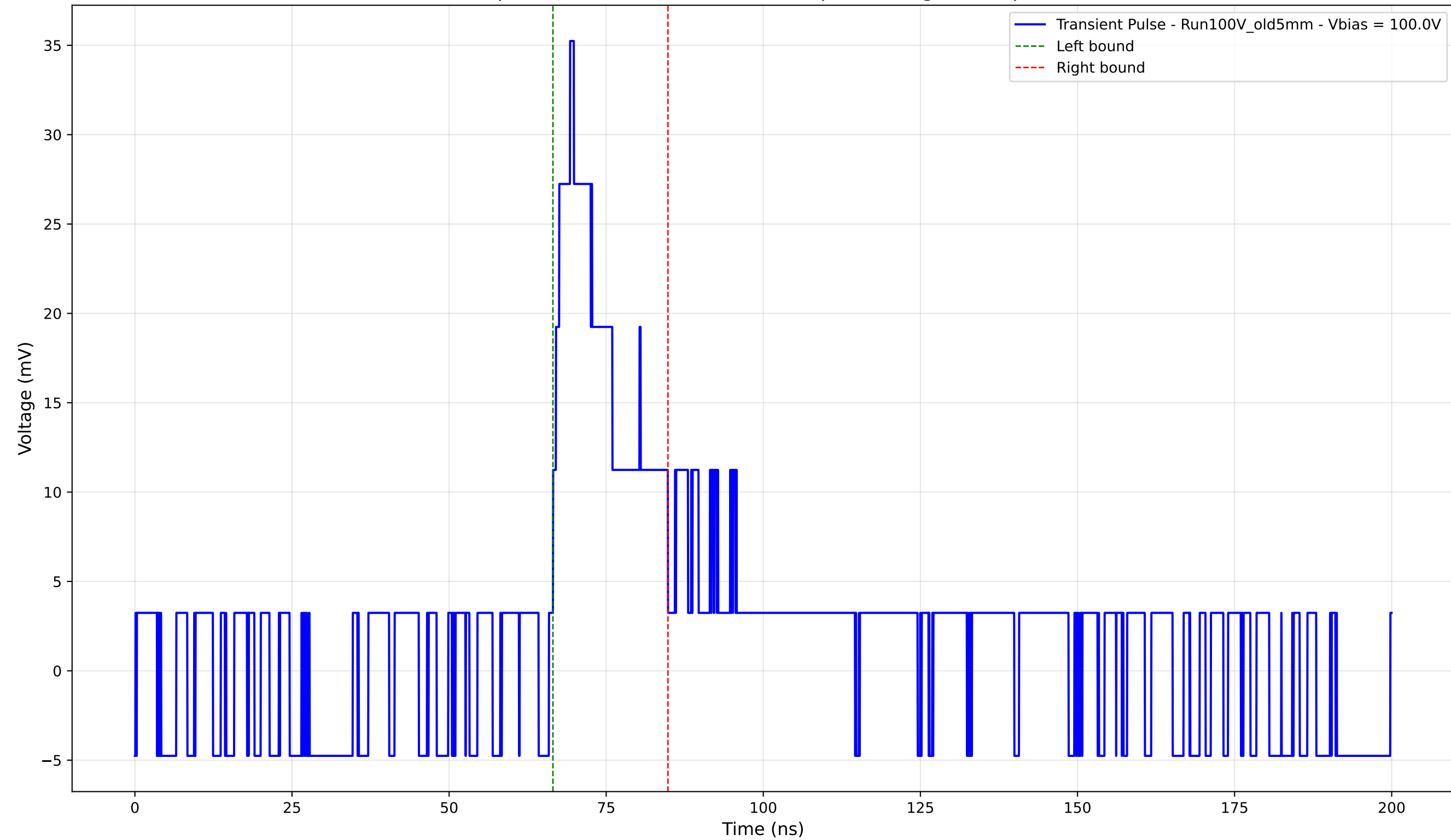
Transient Pulse - Sample: Old5mm - Position: 2875.0 \mu\text{m} - Charge: 6.50 pC - Rise Time: 2.72 ns
