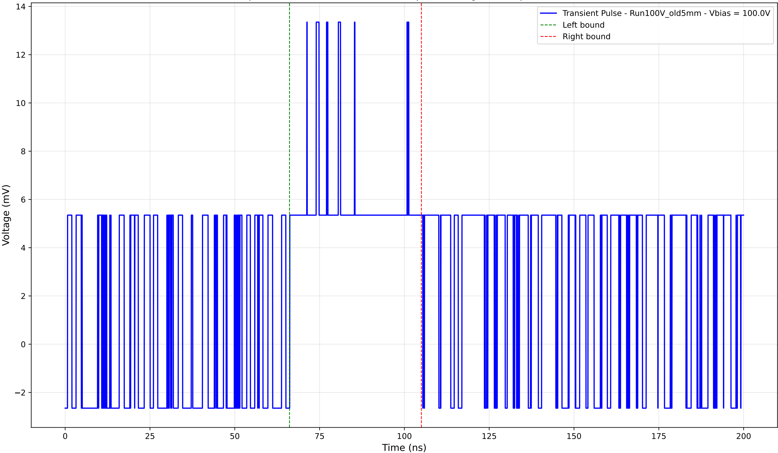
Transient Pulse - Sample: Old5mm - Position: 300.0 \mu\text{m} - Charge: 4.50 pC - Rise Time: 0.00 ns (N/A)
