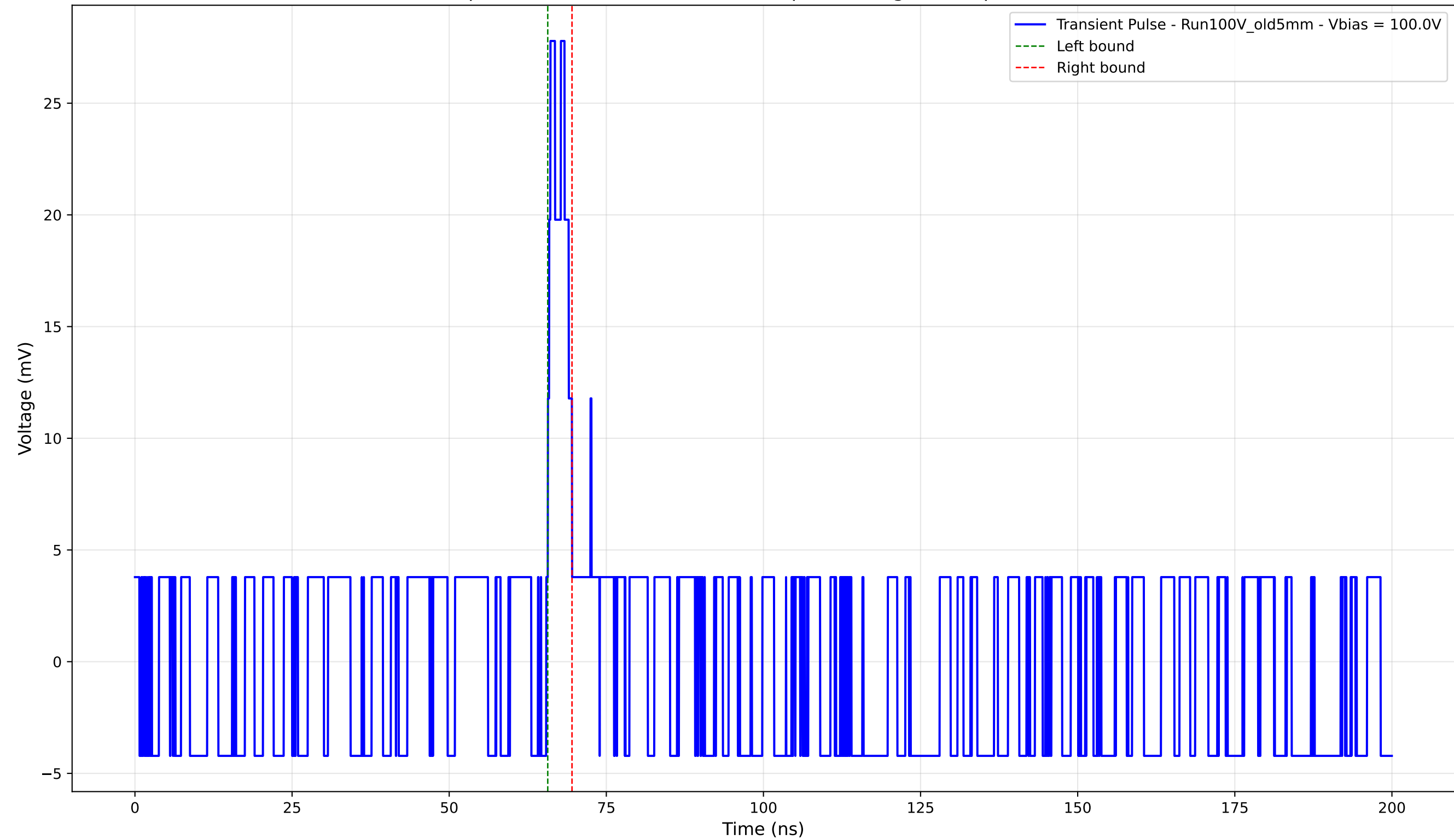
Transient Pulse - Sample: Old5mm - Position: 3675.0 \mu\text{m} - Charge: 1.62 pC - Rise Time: 0.00 ns (N/A)
