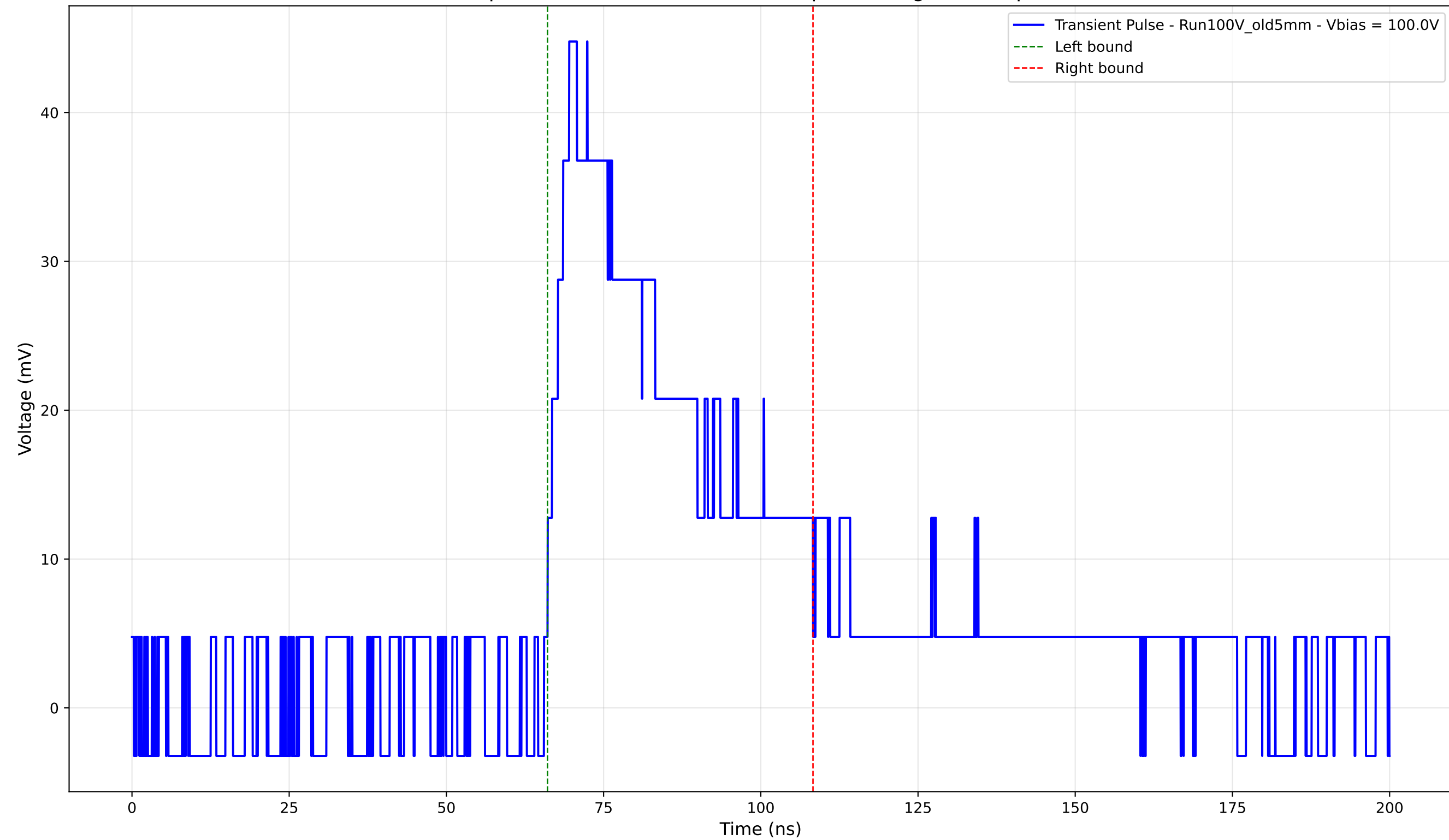
Transient Pulse - Sample: Old5mm - Position: 4930.0 \mu\text{m} - Charge: 18.75 pC - Rise Time: 4.00 ns
