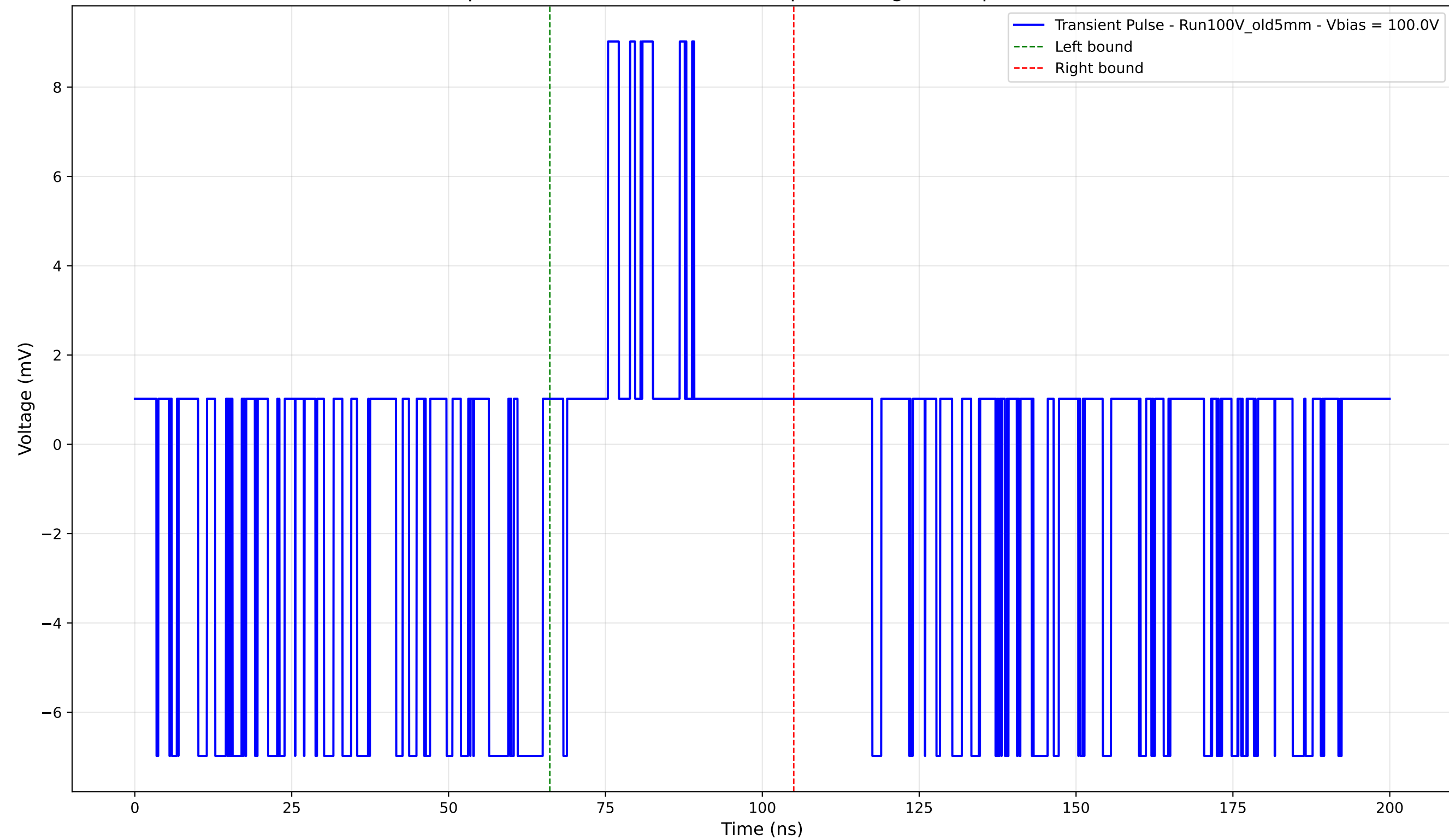
Transient Pulse - Sample: Old5mm - Position: 1680.0 \mu\text{m} - Charge: 1.57 pC - Rise Time: 0.00 ns (N/A)
