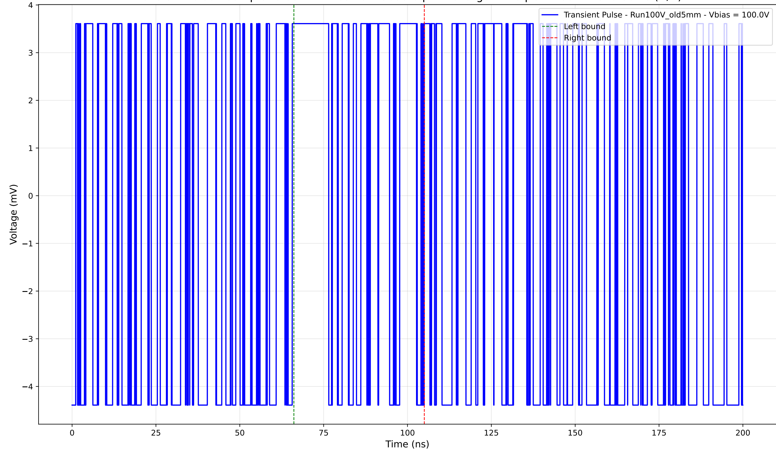
Transient Pulse - Sample: Old5mm - Position: 3095.0 \mu\text{m} - Charge: 1.20 pC - Rise Time: 0.00 ns (N/A)
