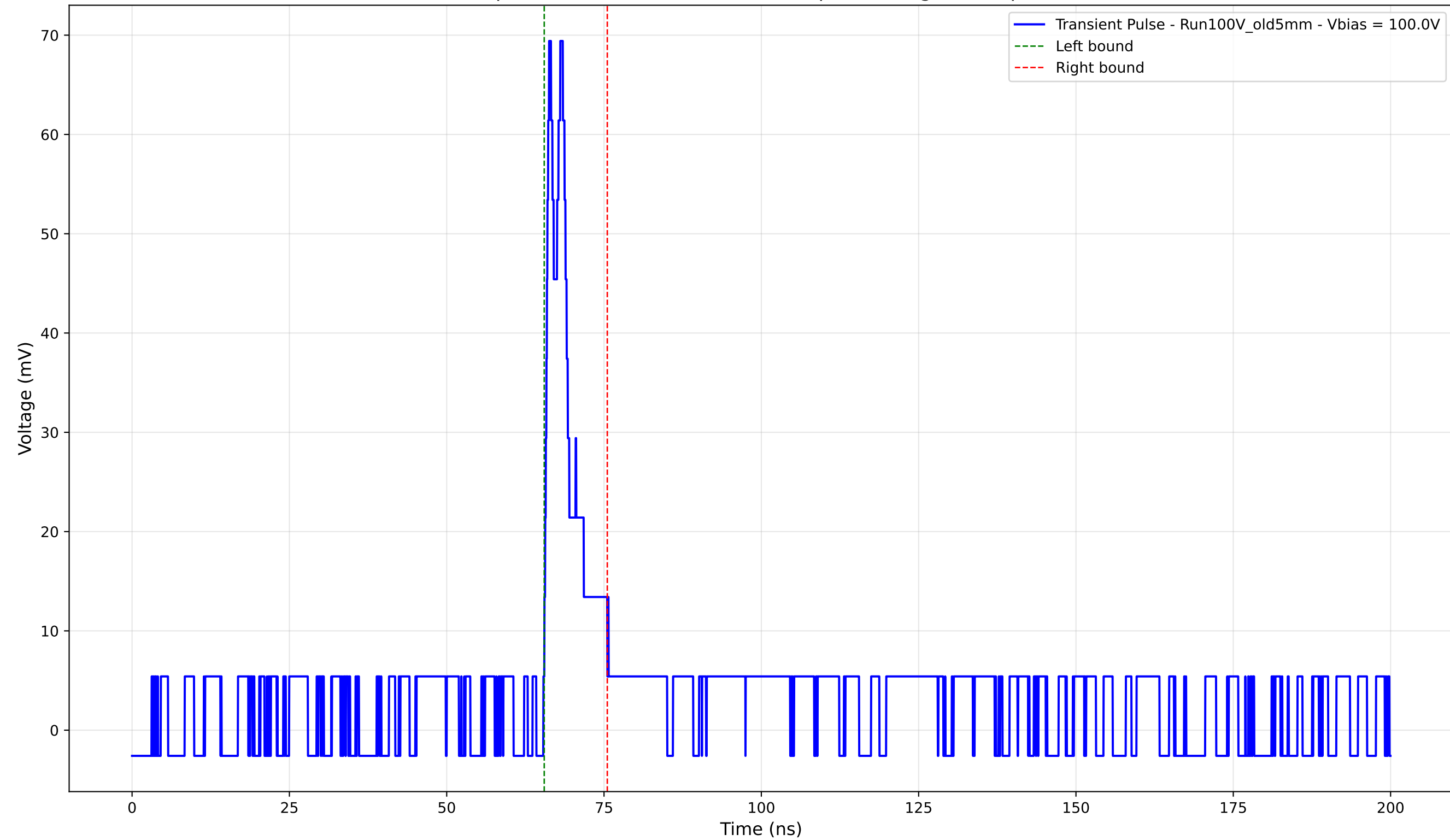
Transient Pulse - Sample: Old5mm - Position: 3760.0 \mu\text{m} - Charge: 6.08 pC - Rise Time: 0.76 ns
