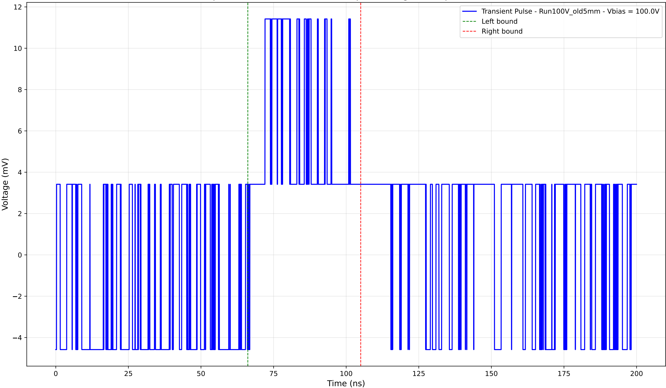
Transient Pulse - Sample: Old5mm - Position: 855.0 \mu\text{m} - Charge: 4.47 pC - Rise Time: 0.00 ns (N/A)
