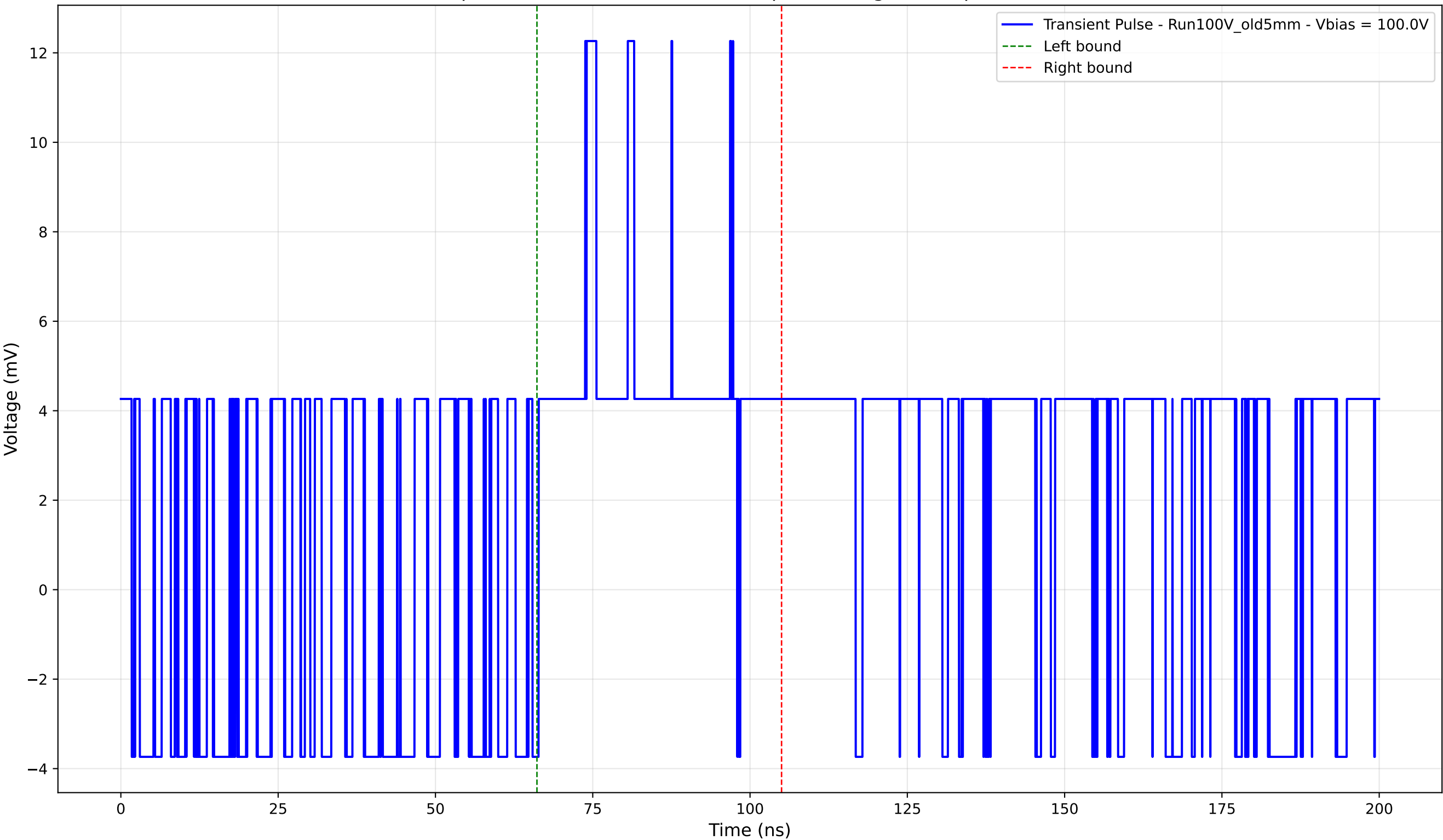
Transient Pulse - Sample: Old5mm - Position: 915.0 \mu\text{m} - Charge: 3.73 pC - Rise Time: 0.00 ns (N/A)
