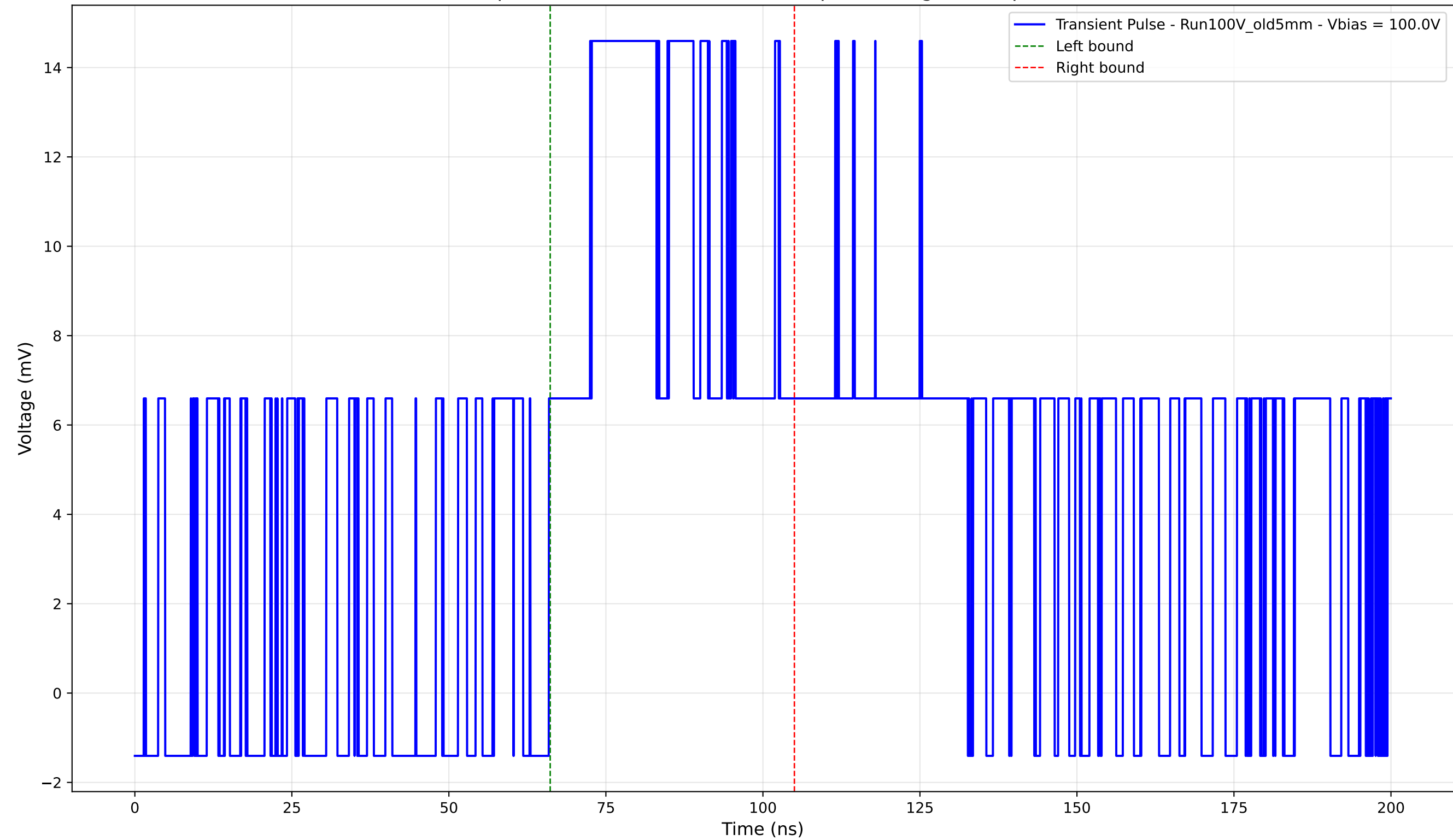
Transient Pulse - Sample: Old5mm - Position: 1450.0 \mu\text{m} - Charge: 8.04 pC - Rise Time: 6.58 ns
