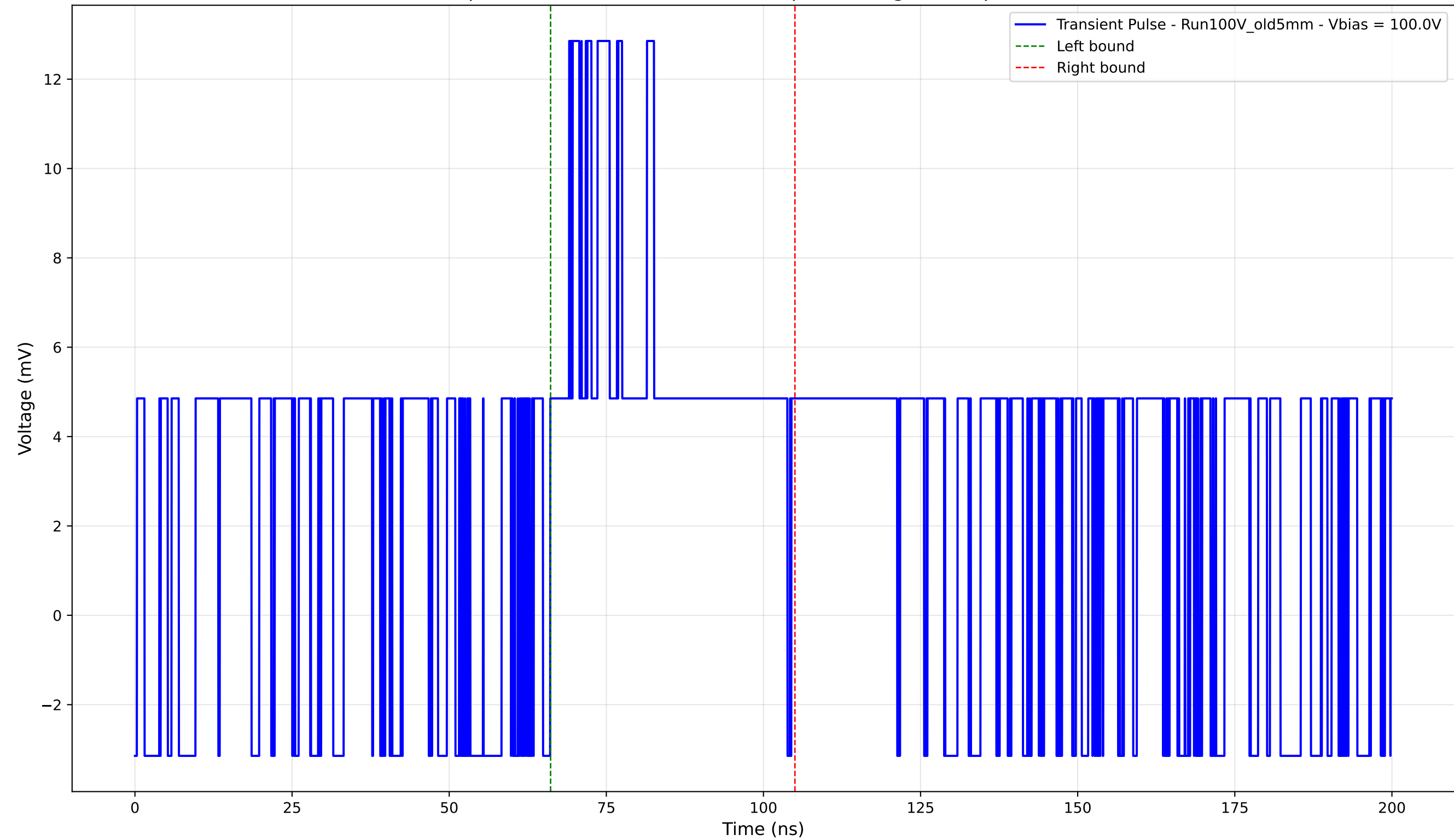
Transient Pulse - Sample: Old5mm - Position: 2350.0 \mu\text{m} - Charge: 4.65 pC - Rise Time: 0.00 ns (N/A)
