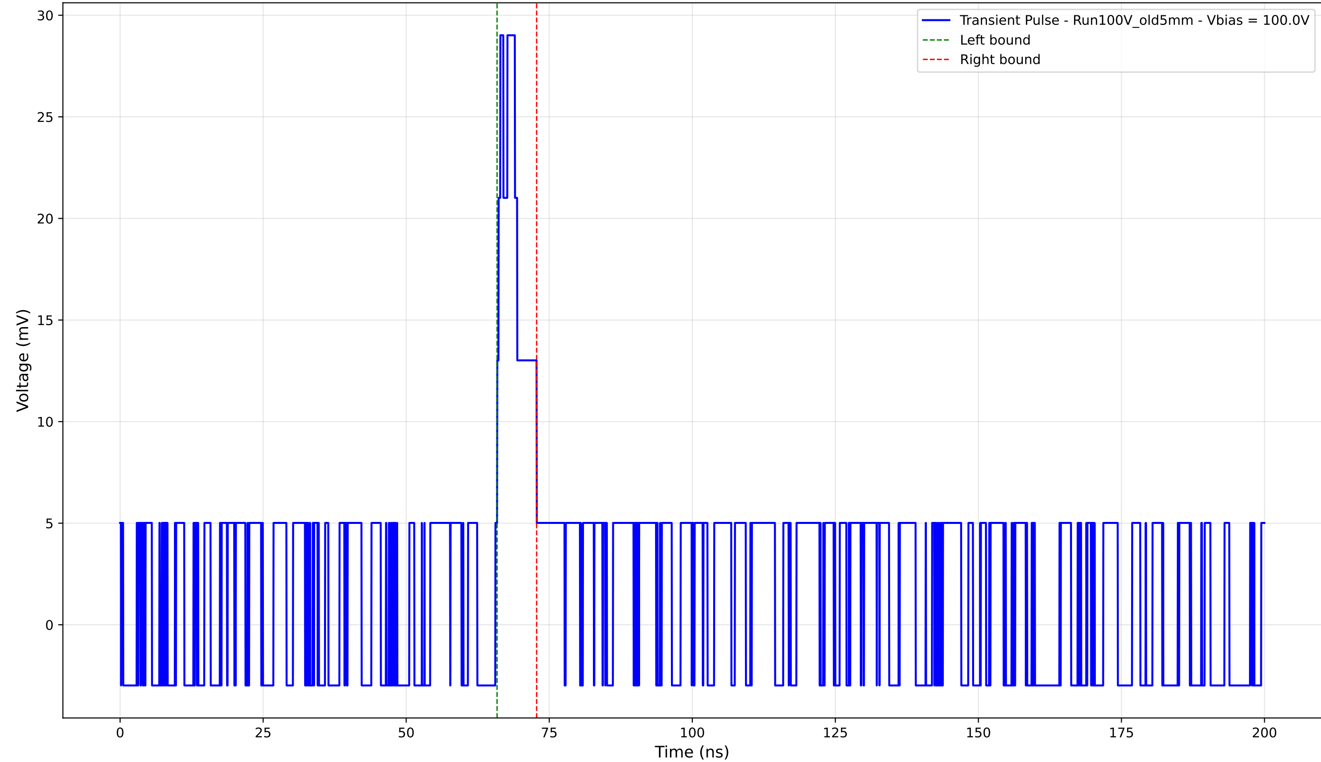
Transient Pulse - Sample: Old5mm - Position: 3970.0 \mu\text{m} - Charge: 2.62 pC - Rise Time: 0.00 ns (N/A)
