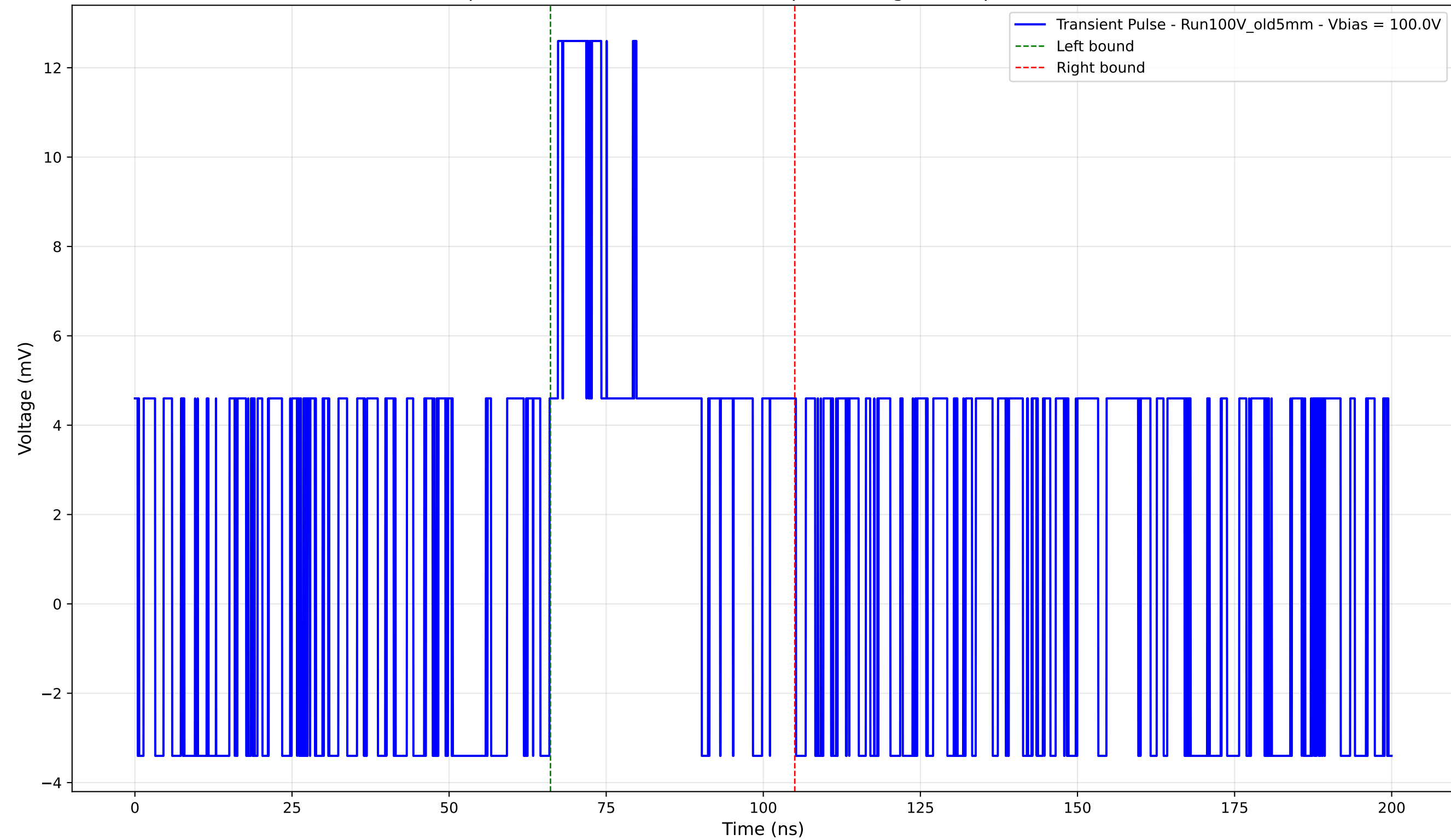
Transient Pulse - Sample: Old5mm - Position: 4665.0 \mu\text{m} - Charge: 4.22 pC - Rise Time: 0.00 ns (N/A)
