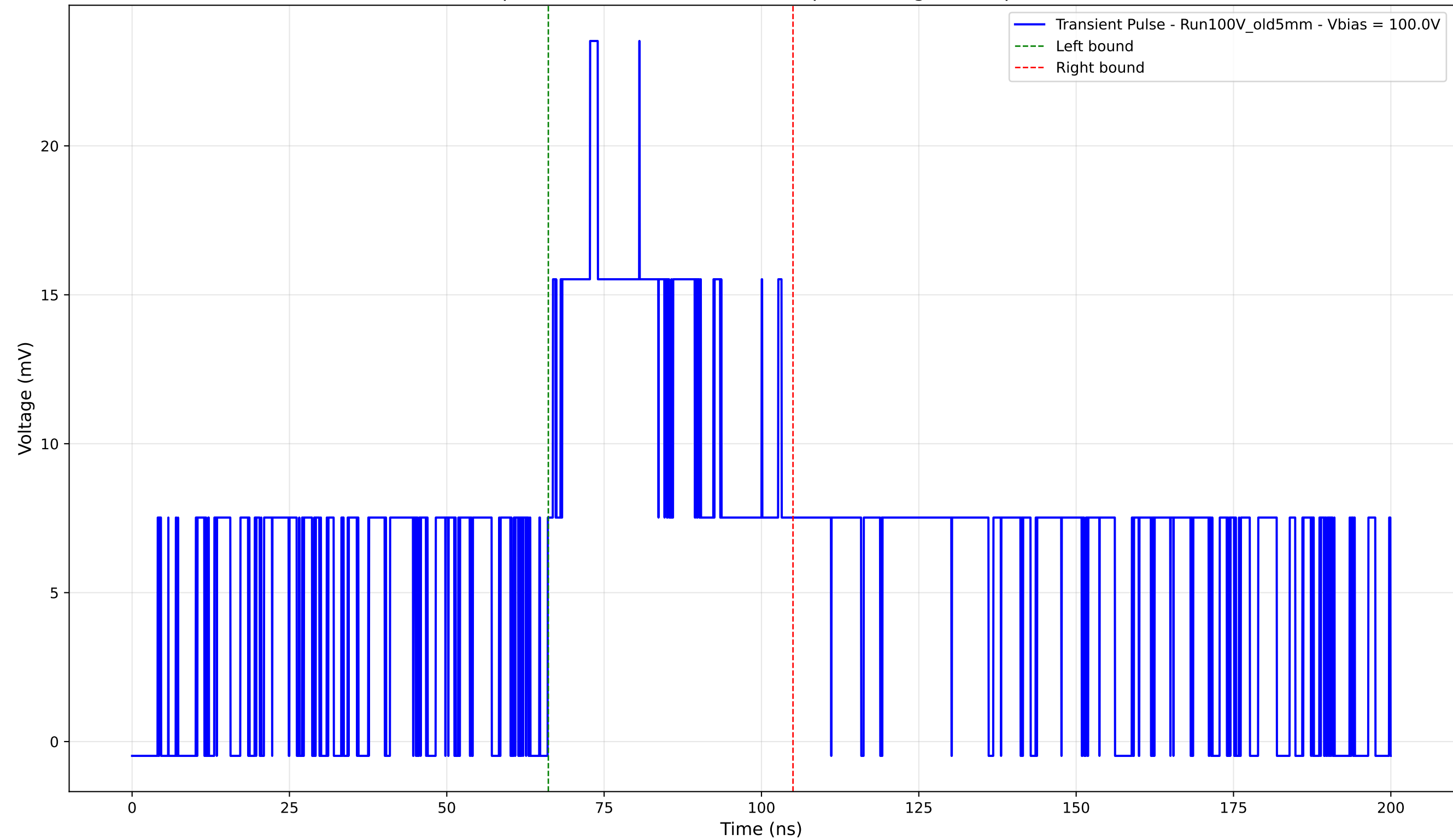
Transient Pulse - Sample: Old5mm - Position: 365.0 \mu\text{m} - Charge: 9.76 pC - Rise Time: 6.73 ns
