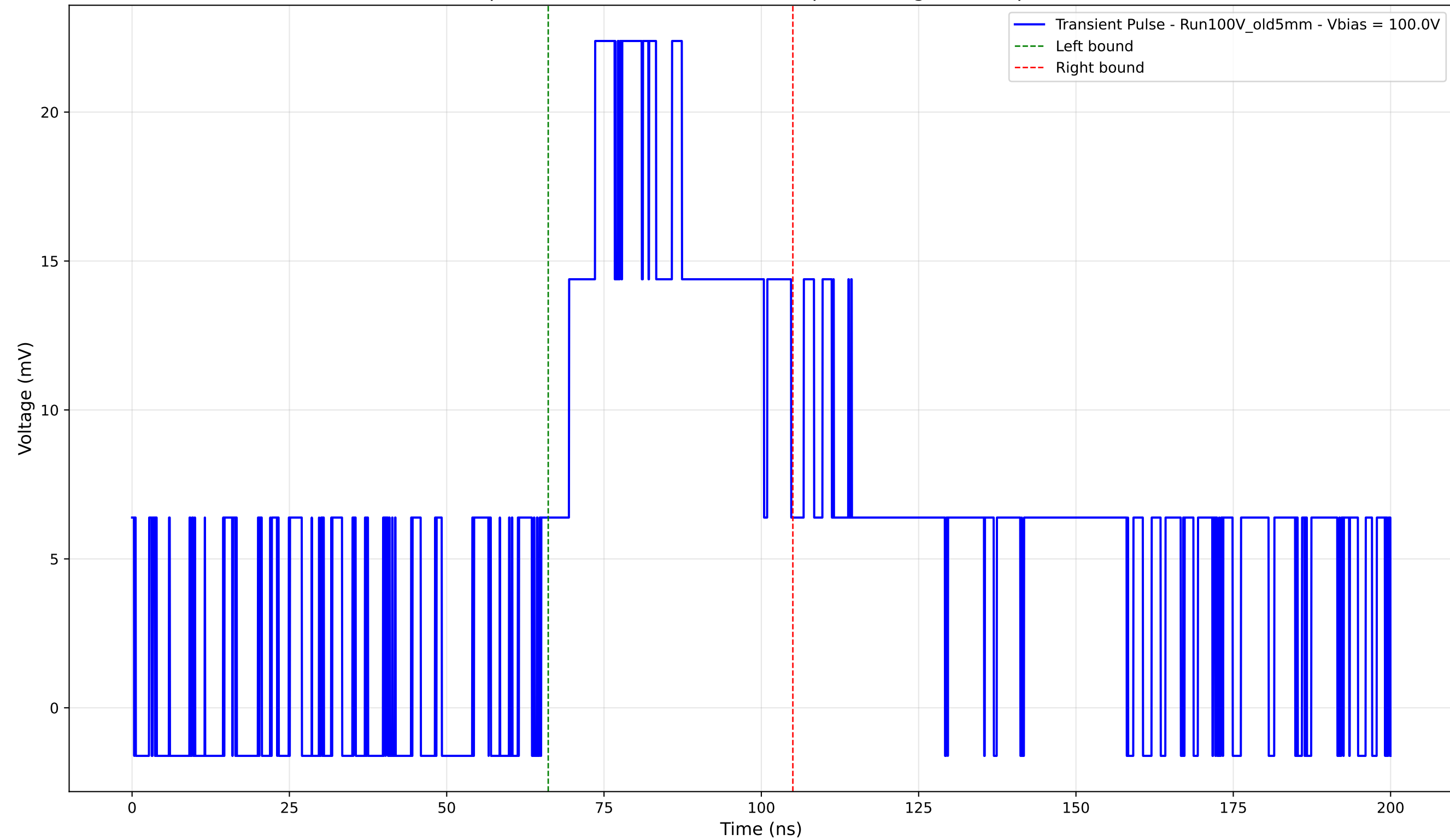
Transient Pulse - Sample: Old5mm - Position: 1605.0 \mu\text{m} - Charge: 12.17 pC - Rise Time: 8.58 ns
