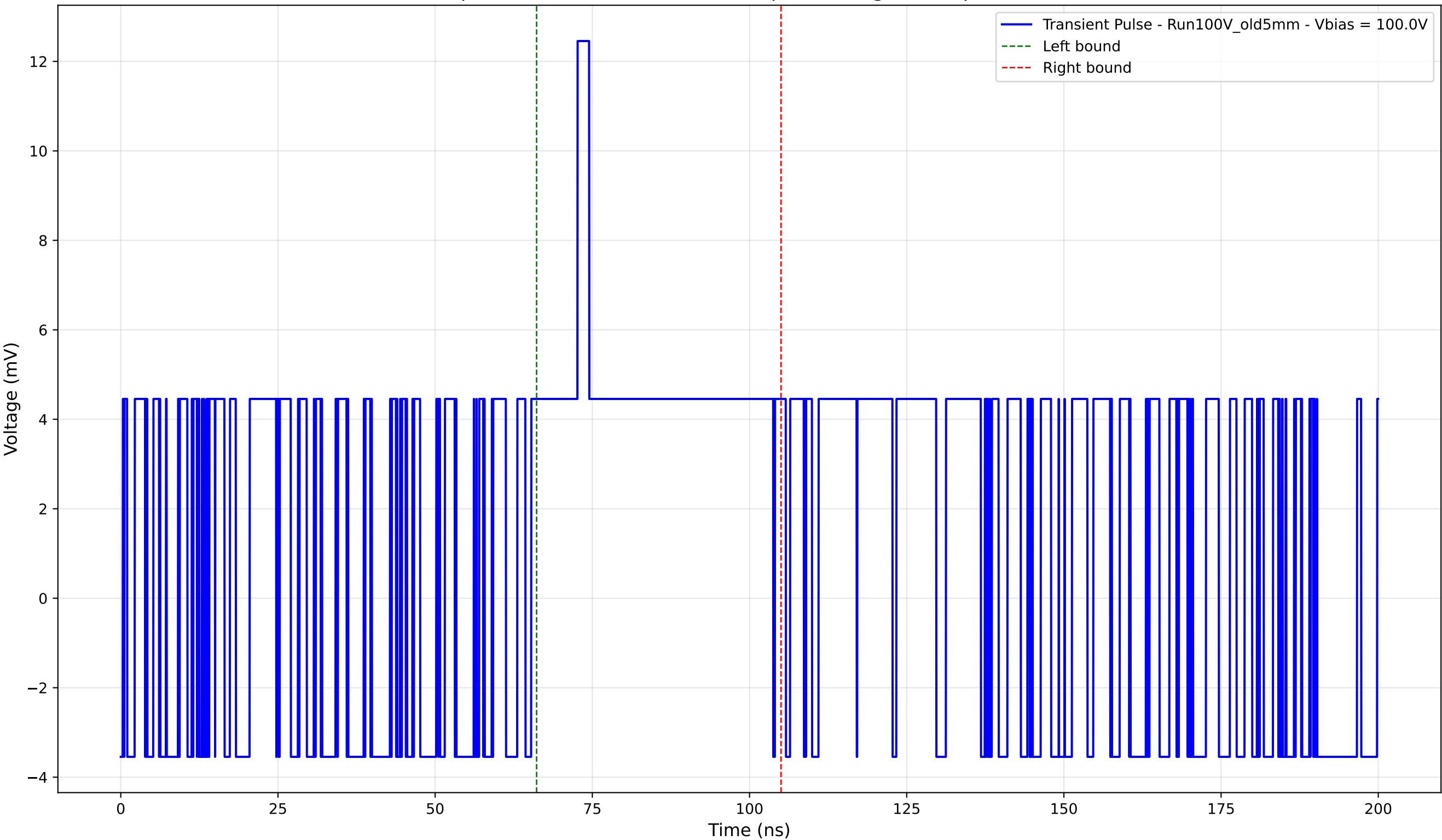
Transient Pulse - Sample: Old5mm - Position: 625.0 \mu\text{m} - Charge: 3.74 pC - Rise Time: 0.00 ns (N/A)
