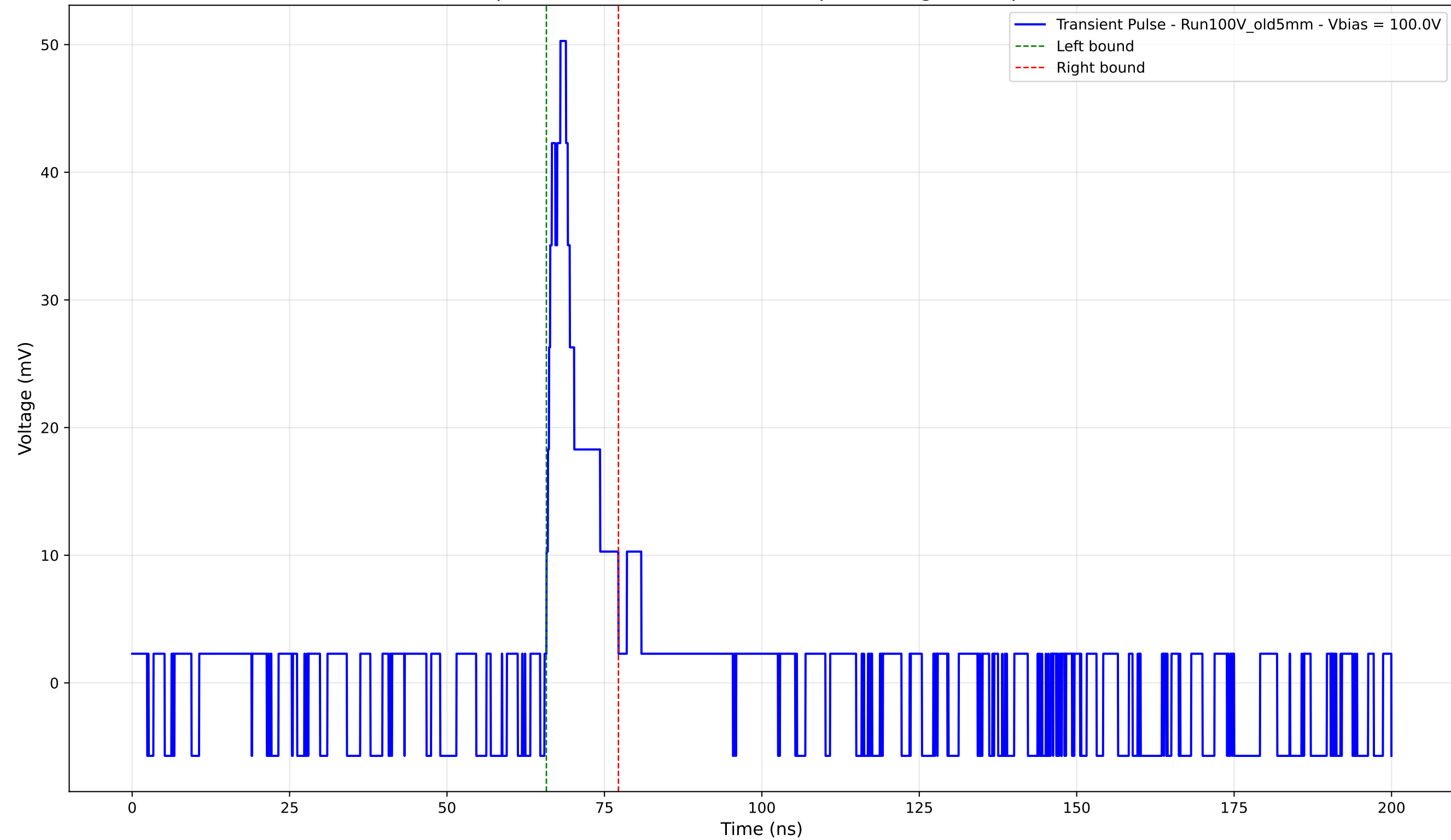
Transient Pulse - Sample: Old5mm - Position: 3345.0 \mu\text{m} - Charge: 5.32 pC - Rise Time: 2.21 ns
