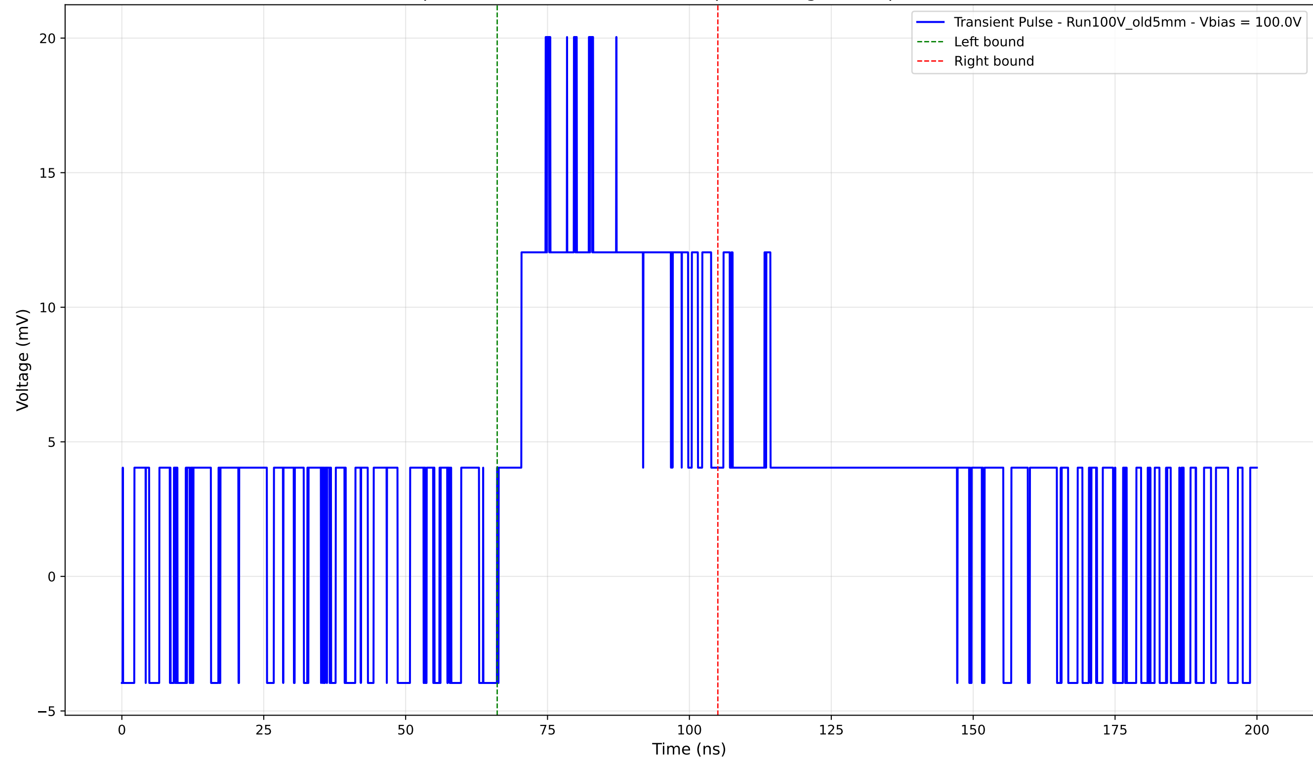
Transient Pulse - Sample: Old5mm - Position: 1775.0 \mu\text{m} - Charge: 8.47 pC - Rise Time: 0.00 ns (N/A)
