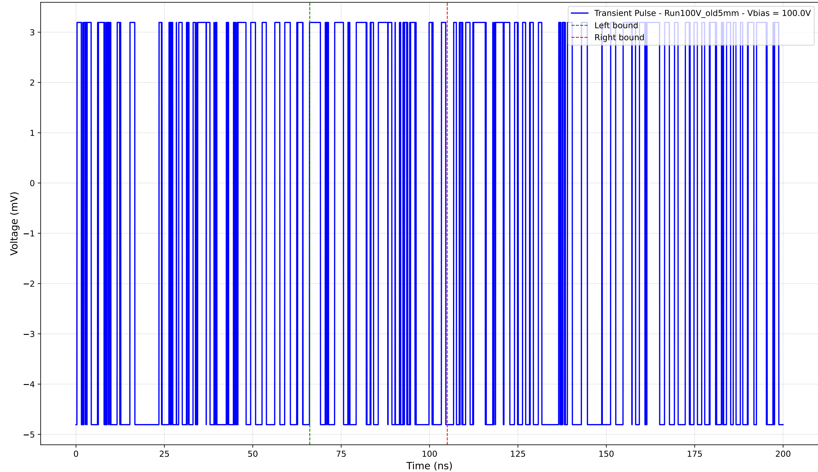
Transient Pulse - Sample: Old5mm - Position: 175.0 \mu\text{m} - Charge: -0.67 pC - Rise Time: 0.00 ns (N/A)
