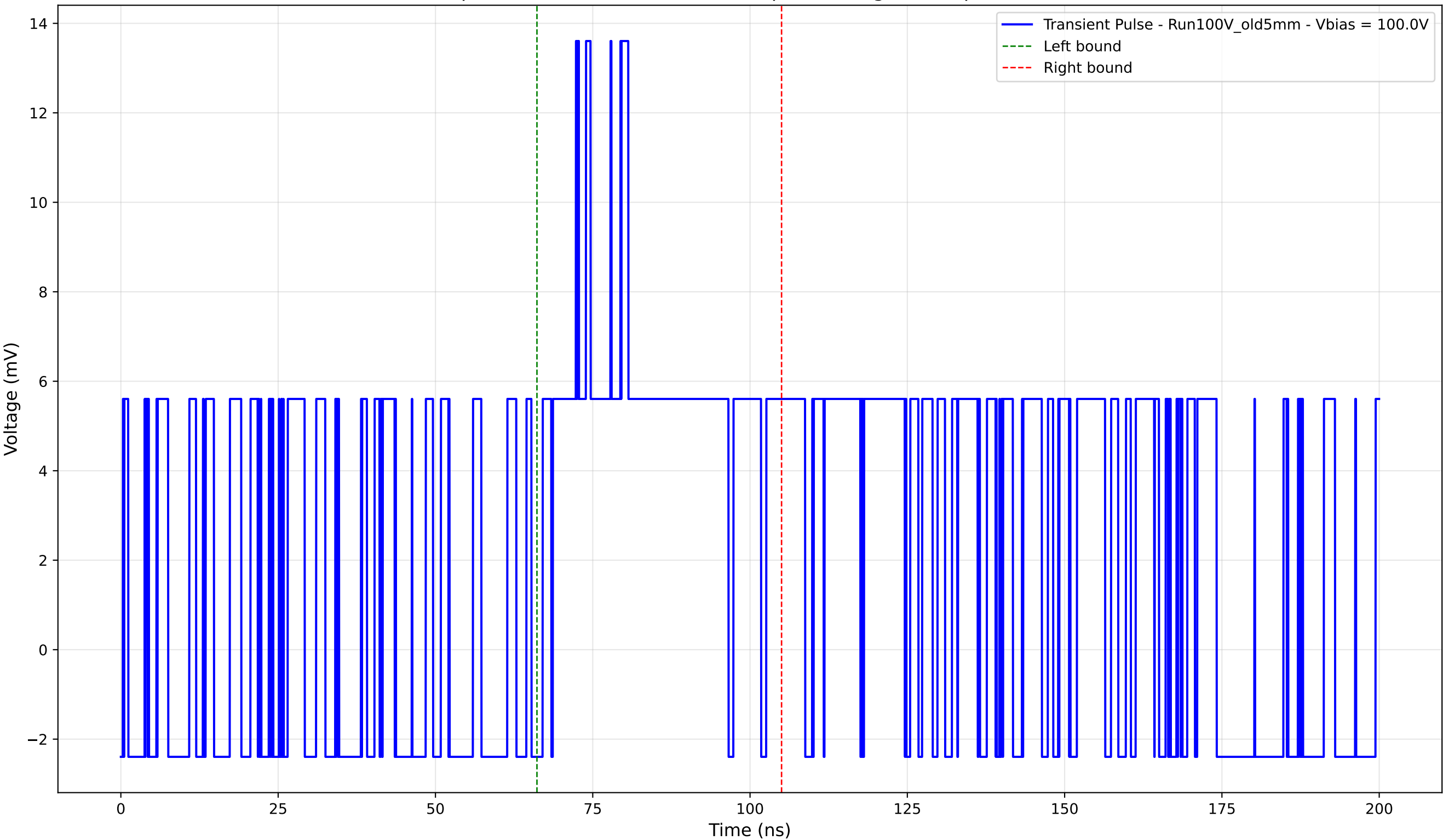
Transient Pulse - Sample: Old5mm - Position: 925.0 \mu\text{m} - Charge: 4.31 pC - Rise Time: 0.00 ns (N/A)
