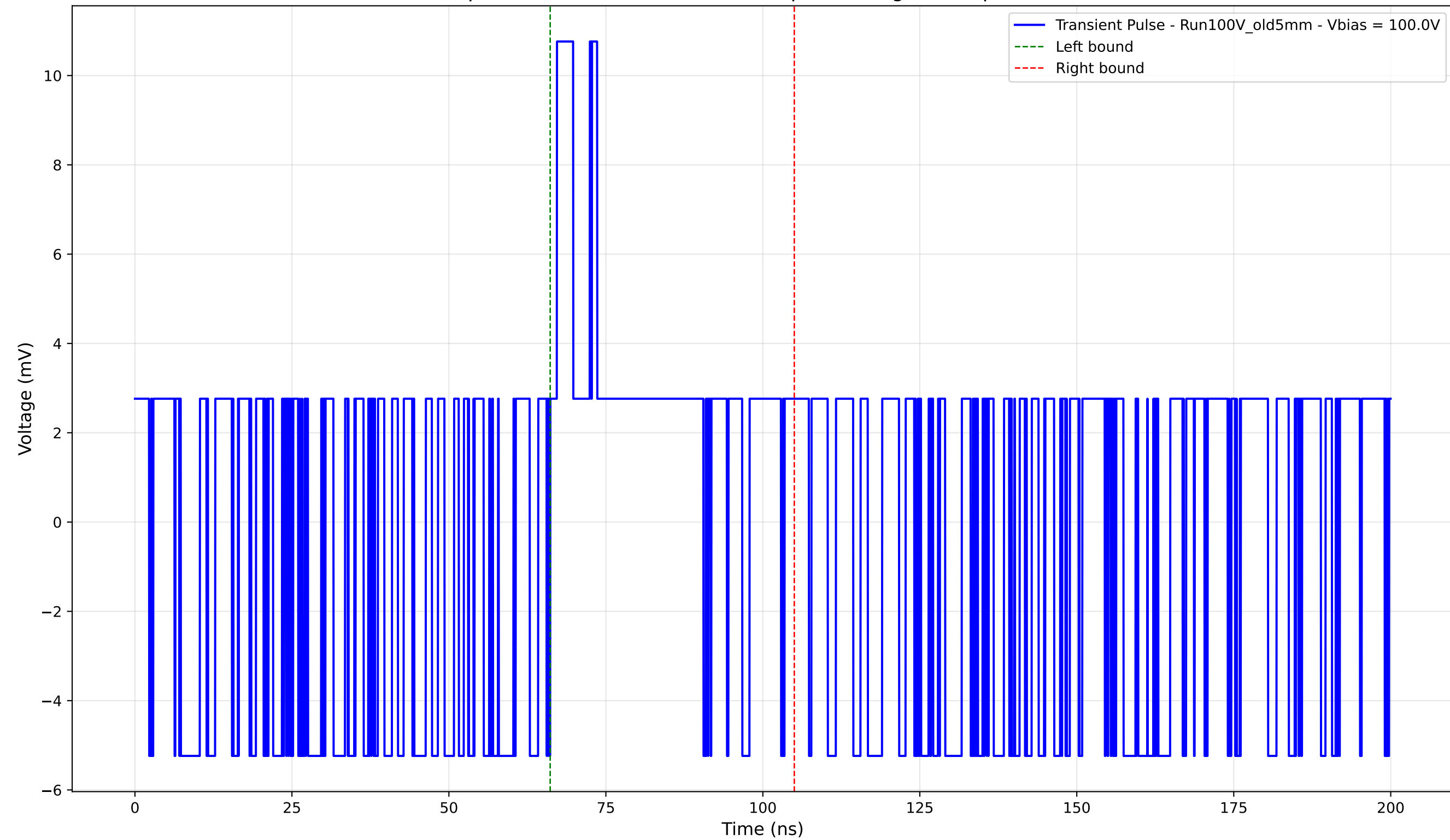
Transient Pulse - Sample: Old5mm - Position: 4580.0 \mu\text{m} - Charge: 2.34 pC - Rise Time: 0.00 ns (N/A)
