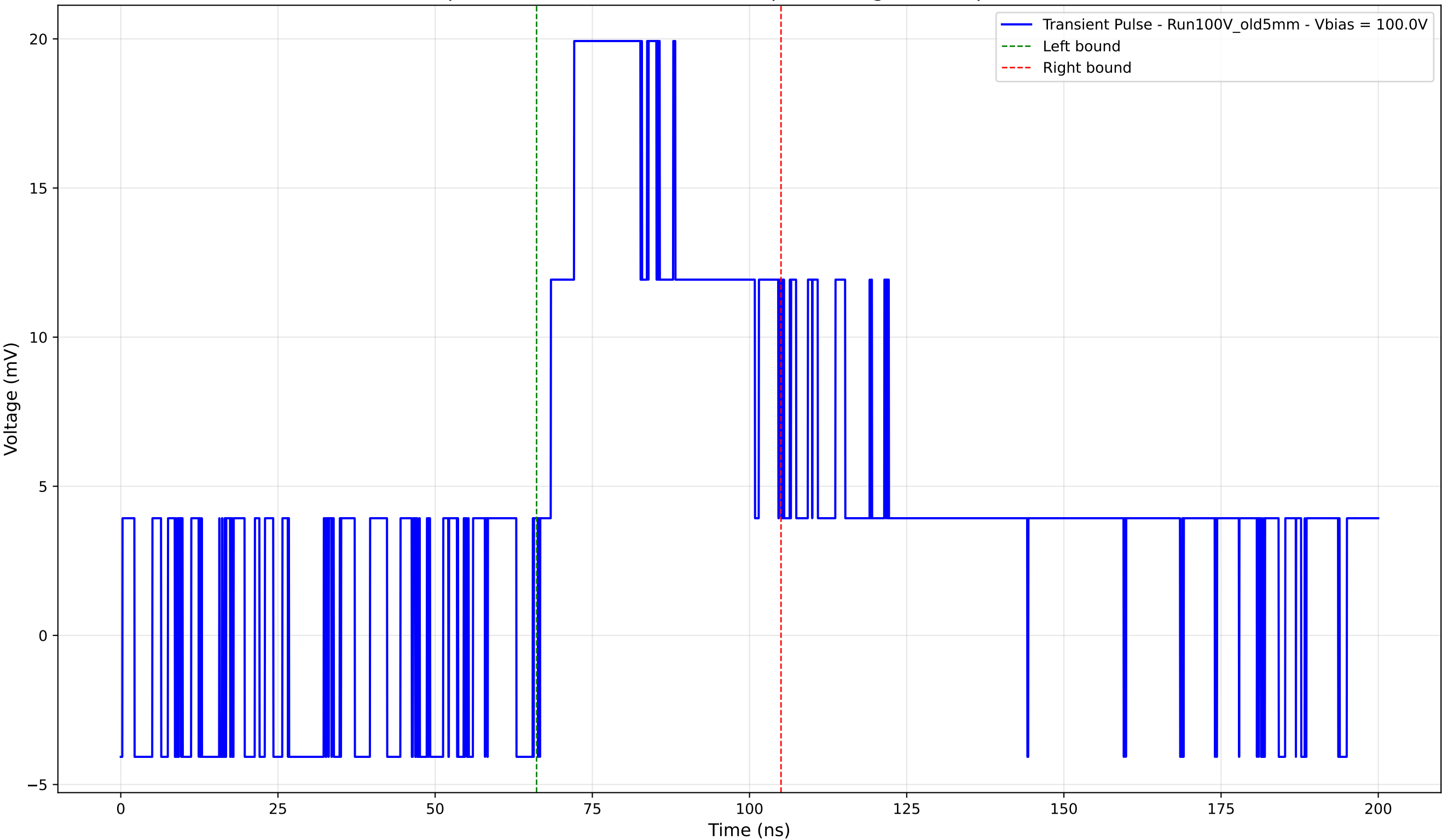
Transient Pulse - Sample: Old5mm - Position: 1800.0 \mu\text{m} - Charge: 10.80 pC - Rise Time: 0.00 ns (N/A)
