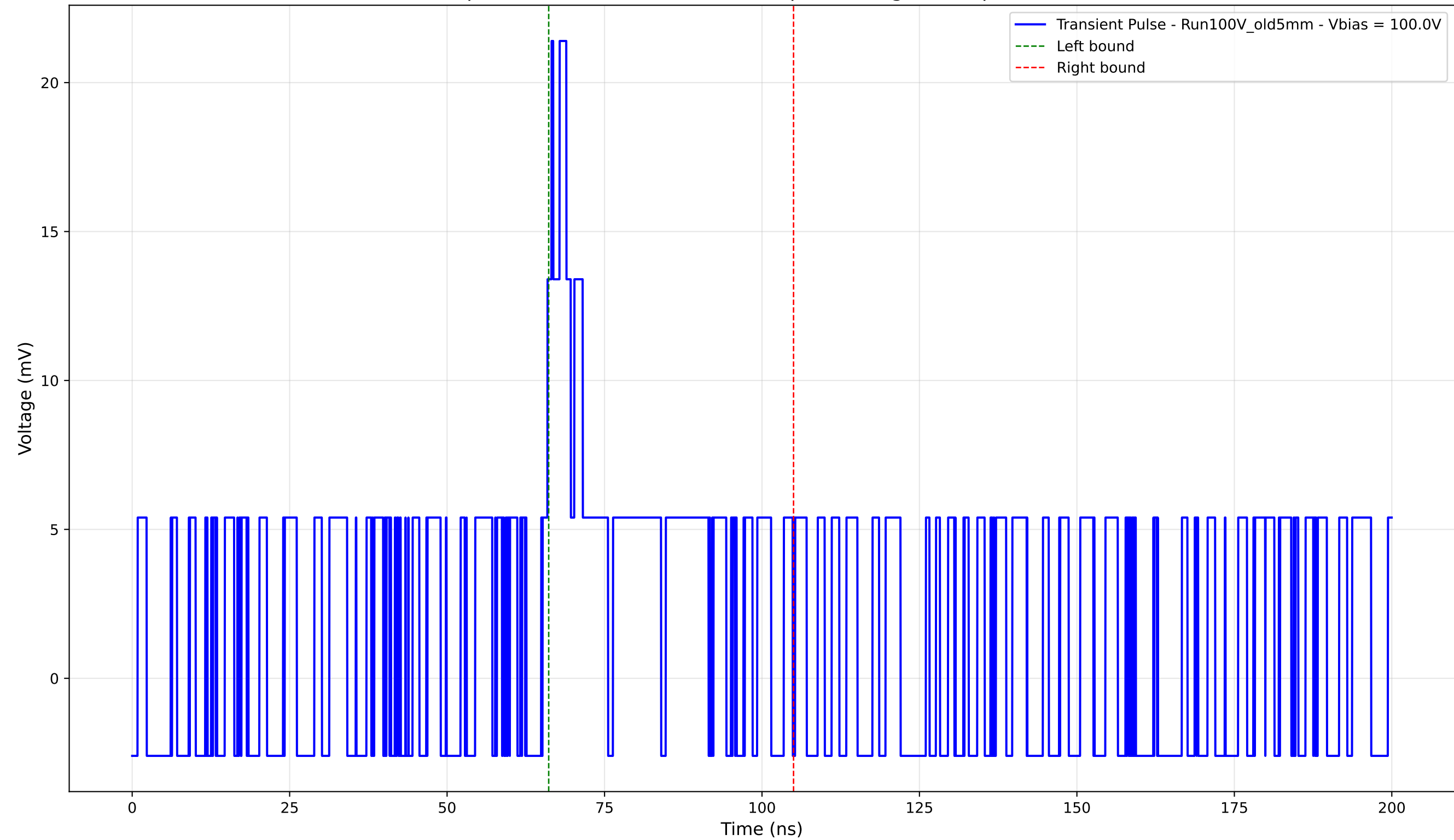
Transient Pulse - Sample: Old5mm - Position: 3370.0 \mu\text{m} - Charge: 4.07 pC - Rise Time: 0.00 ns (N/A)
