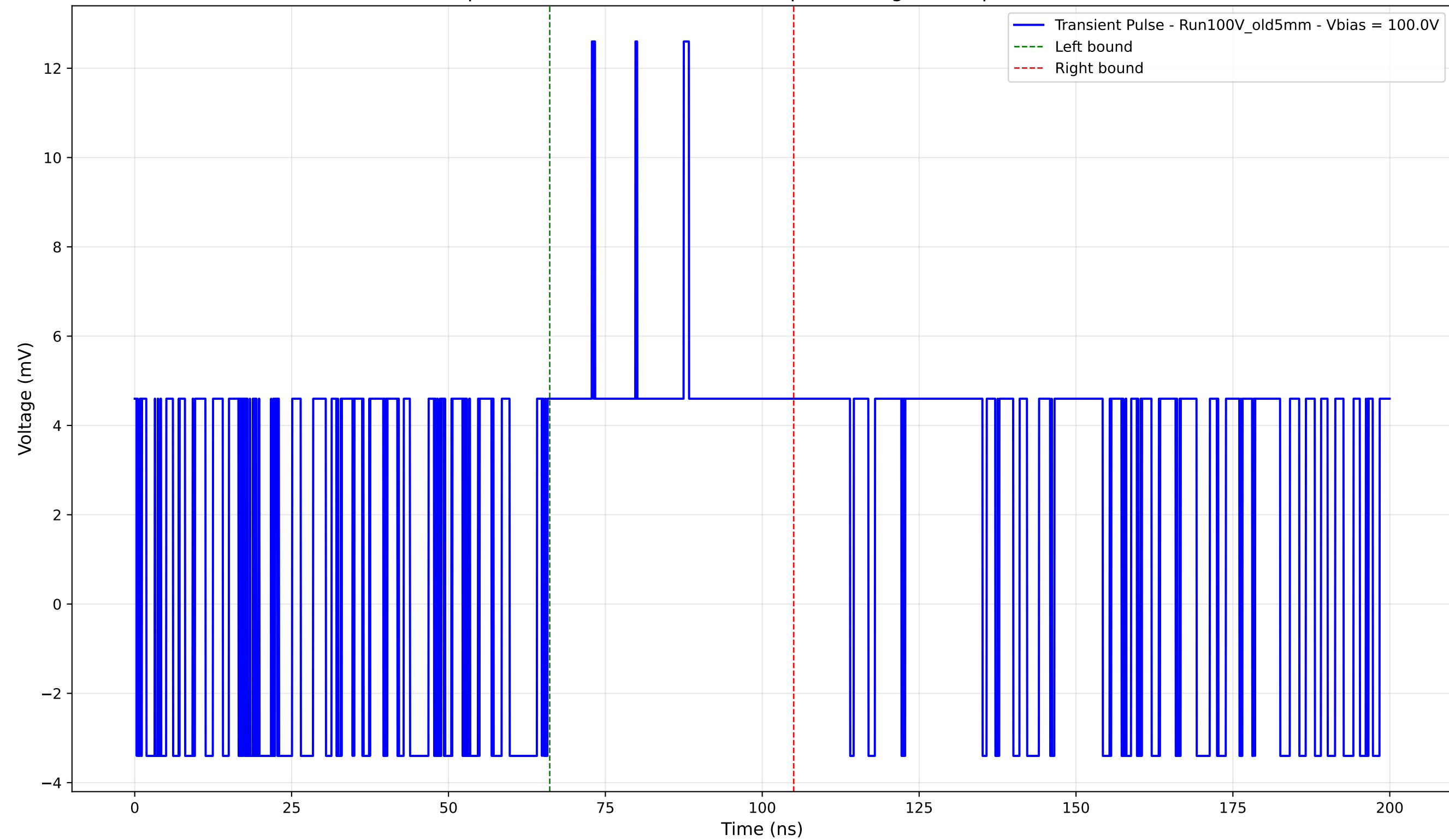
Transient Pulse - Sample: Old5mm - Position: 1345.0 \mu\text{m} - Charge: 3.81 pC - Rise Time: 0.00 ns (N/A)
