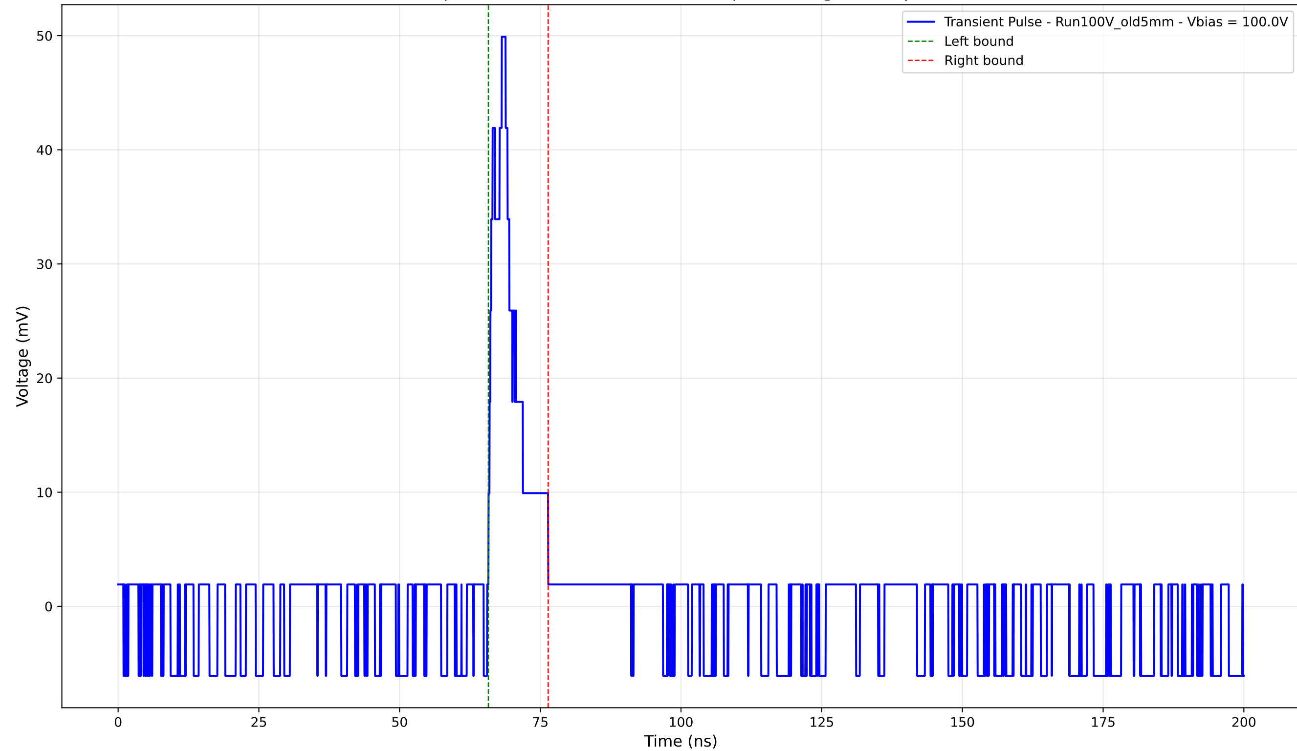
Transient Pulse - Sample: Old5mm - Position: 3460.0 \mu\text{m} - Charge: 4.68 pC - Rise Time: 2.35 ns
