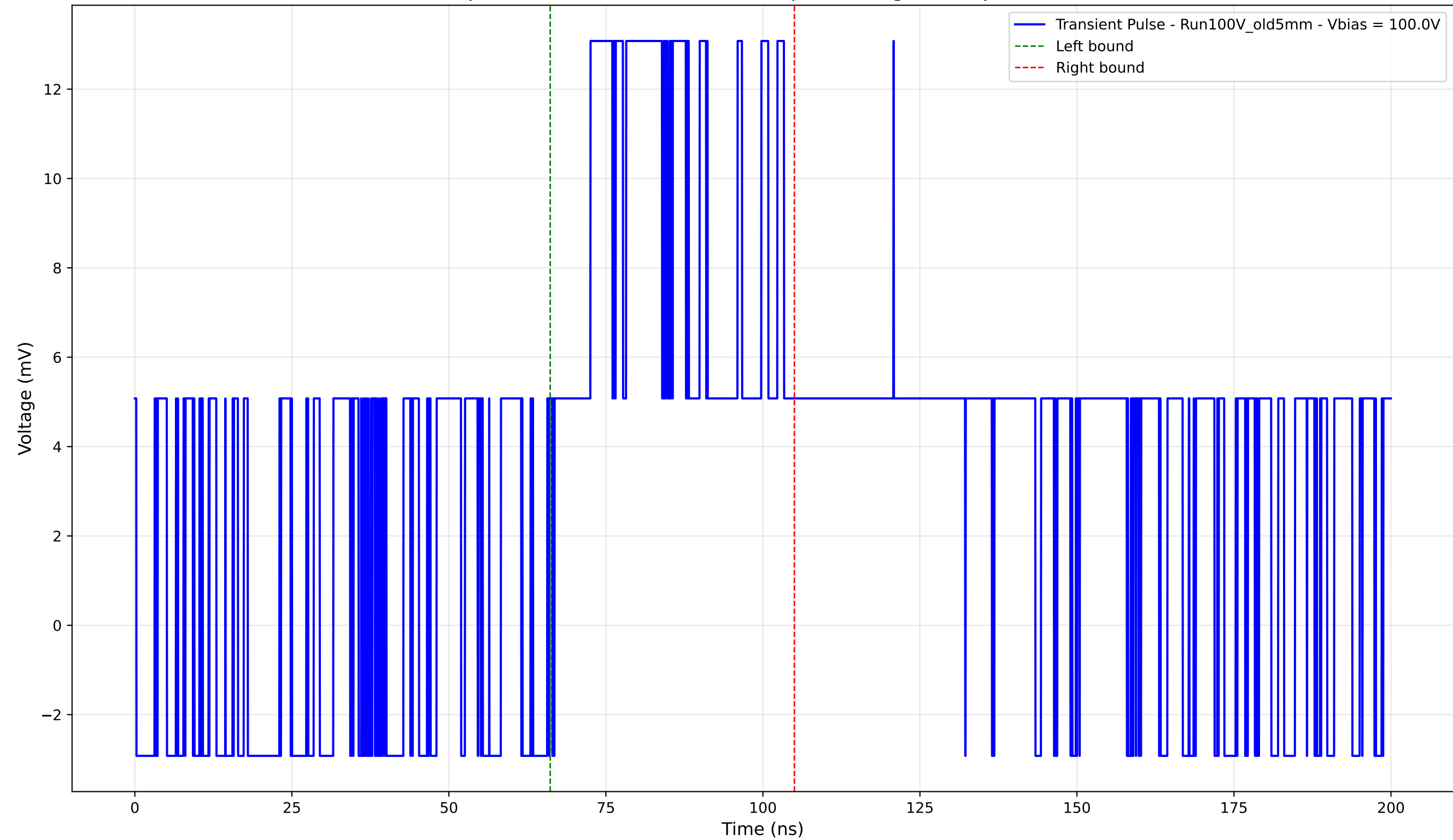
Transient Pulse - Sample: Old5mm - Position: 1060.0 \mu\text{m} - Charge: 6.75 pC - Rise Time: 0.00 ns (N/A)
