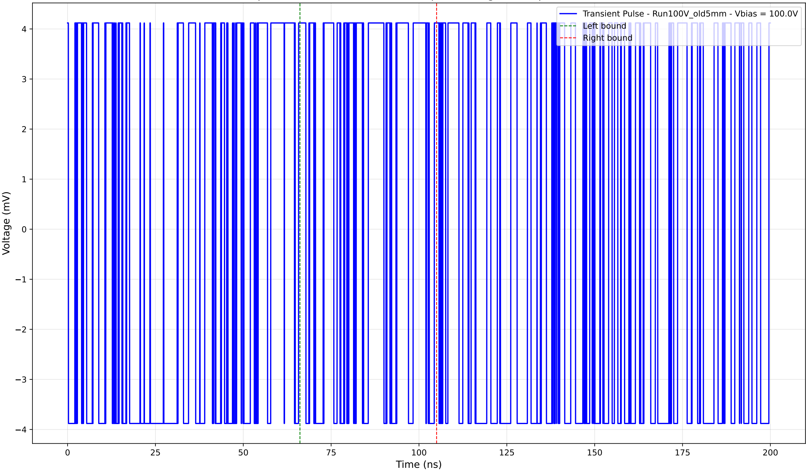
Transient Pulse - Sample: Old5mm - Position: 145.0 \mu\text{m} - Charge: 1.06 pC - Rise Time: 0.00 ns (N/A)
