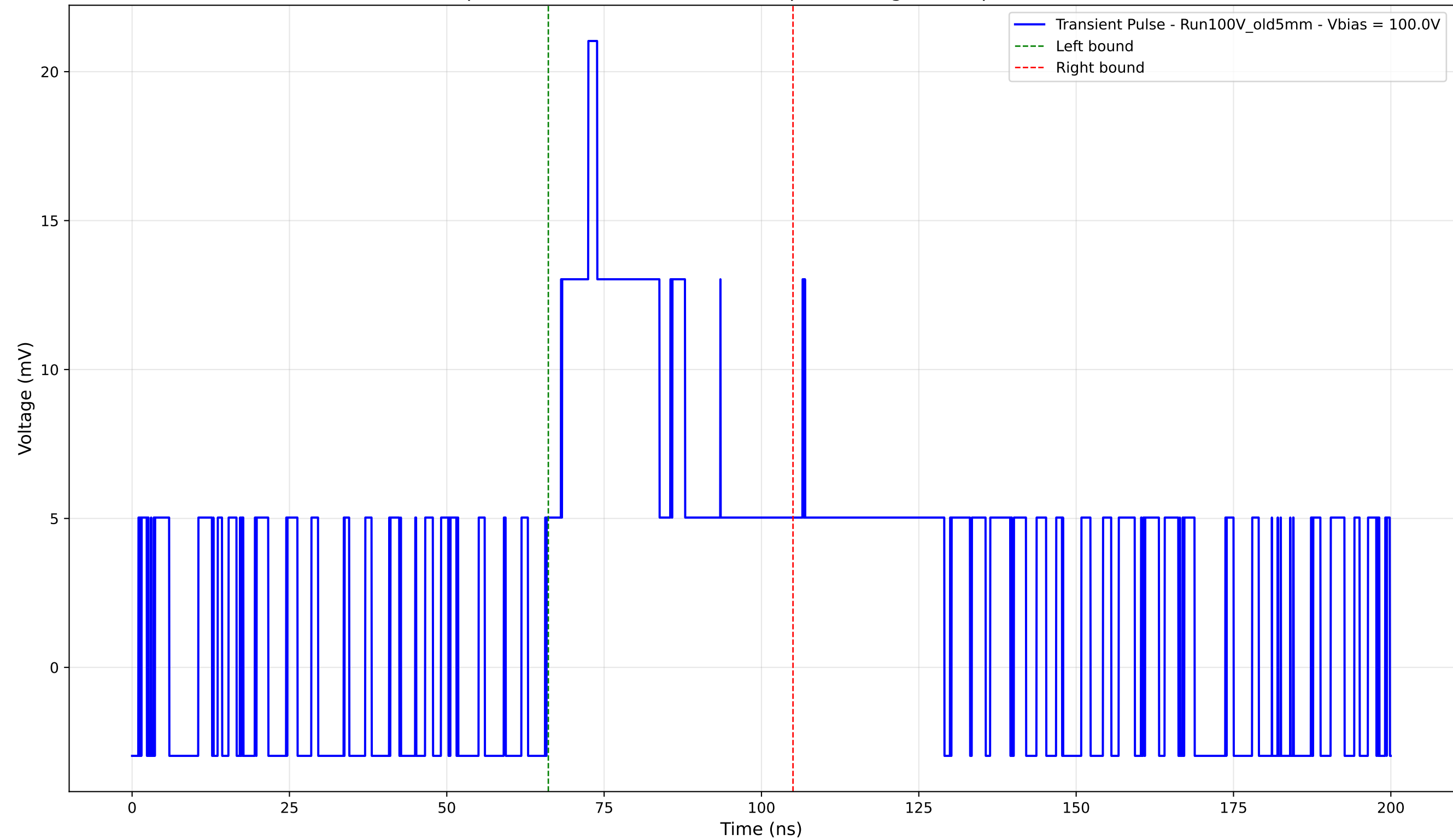
Transient Pulse - Sample: Old5mm - Position: 2475.0 \mu\text{m} - Charge: 7.00 pC - Rise Time: 0.00 ns (N/A)
