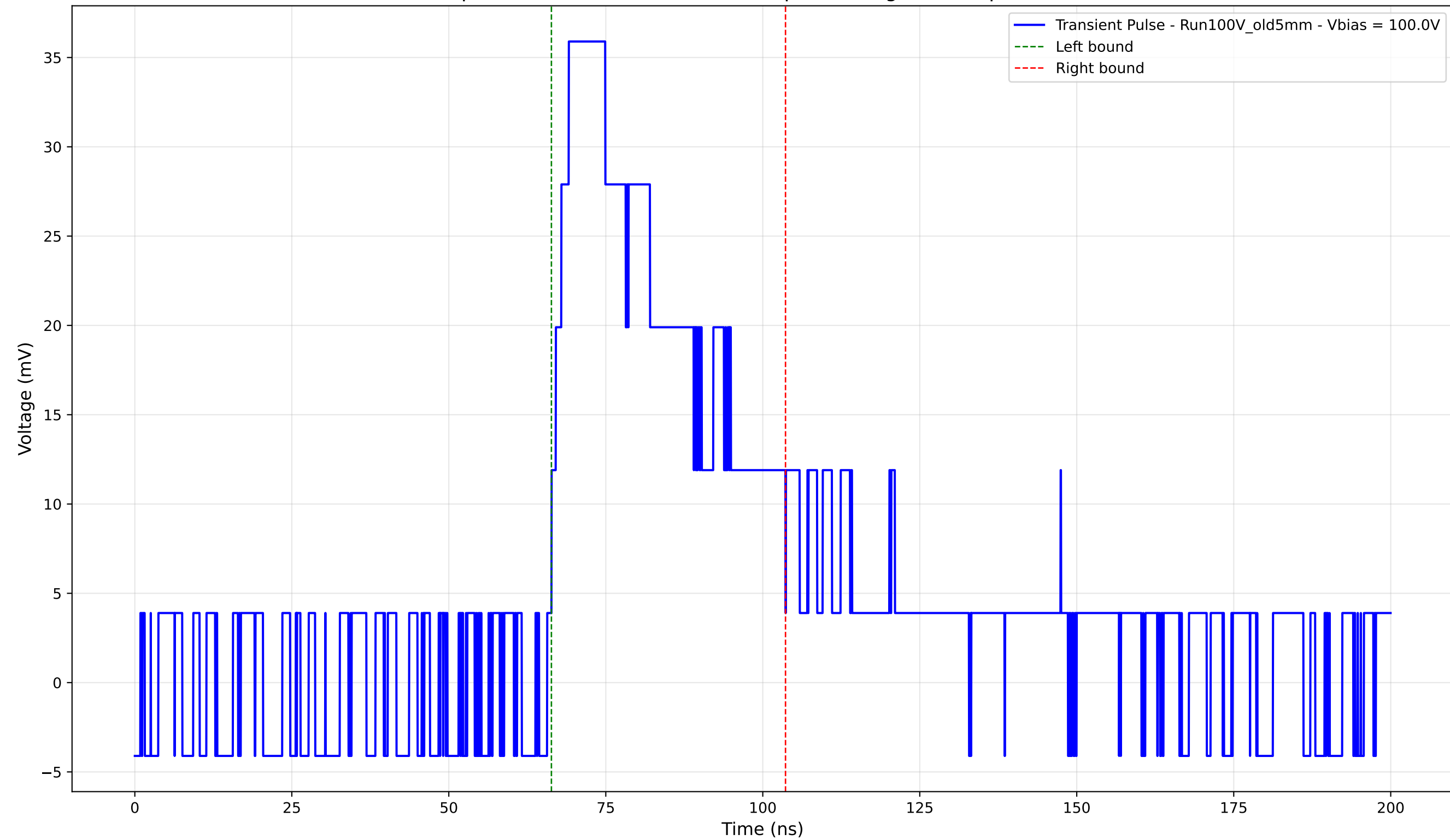
Transient Pulse - Sample: Old5mm - Position: 4940.0 \mu\text{m} - Charge: 16.03 pC - Rise Time: 0.00 ns (N/A)
