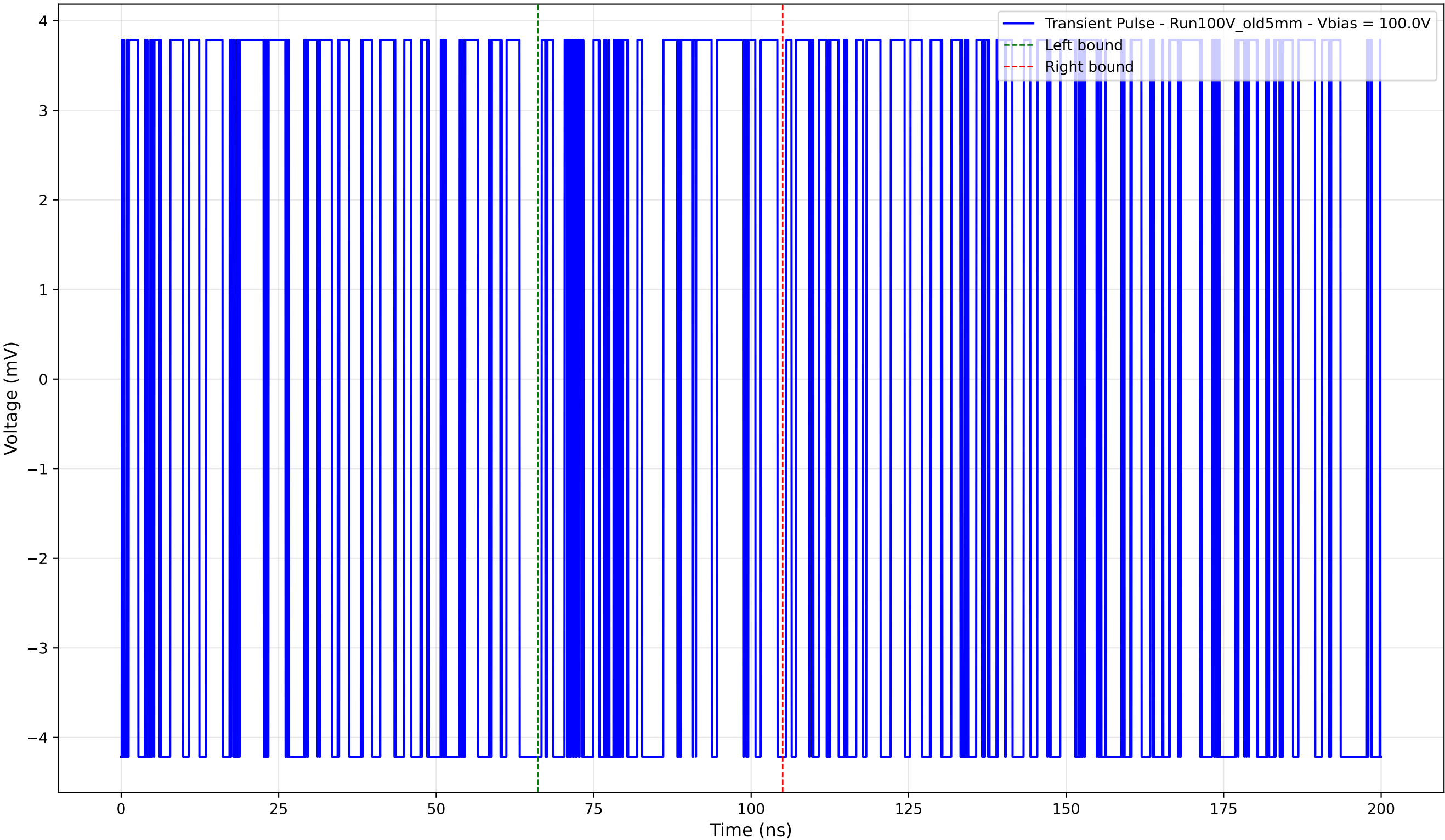
Transient Pulse - Sample: Old5mm - Position: 110.0 \mu\text{m} - Charge: 0.28 pC - Rise Time: 0.00 ns (N/A)
