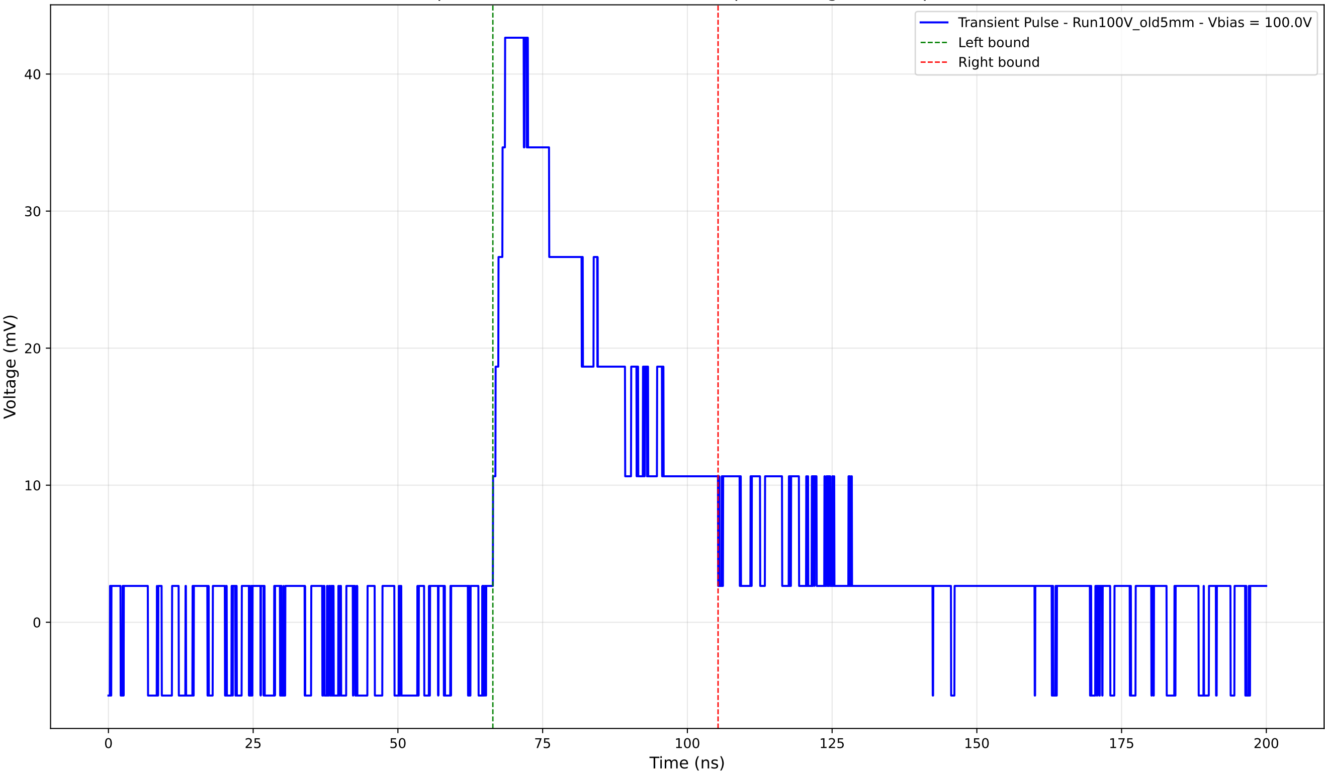
Transient Pulse - Sample: Old5mm - Position: 4835.0 \mu\text{m} - Charge: 16.63 pC - Rise Time: 2.10 ns
