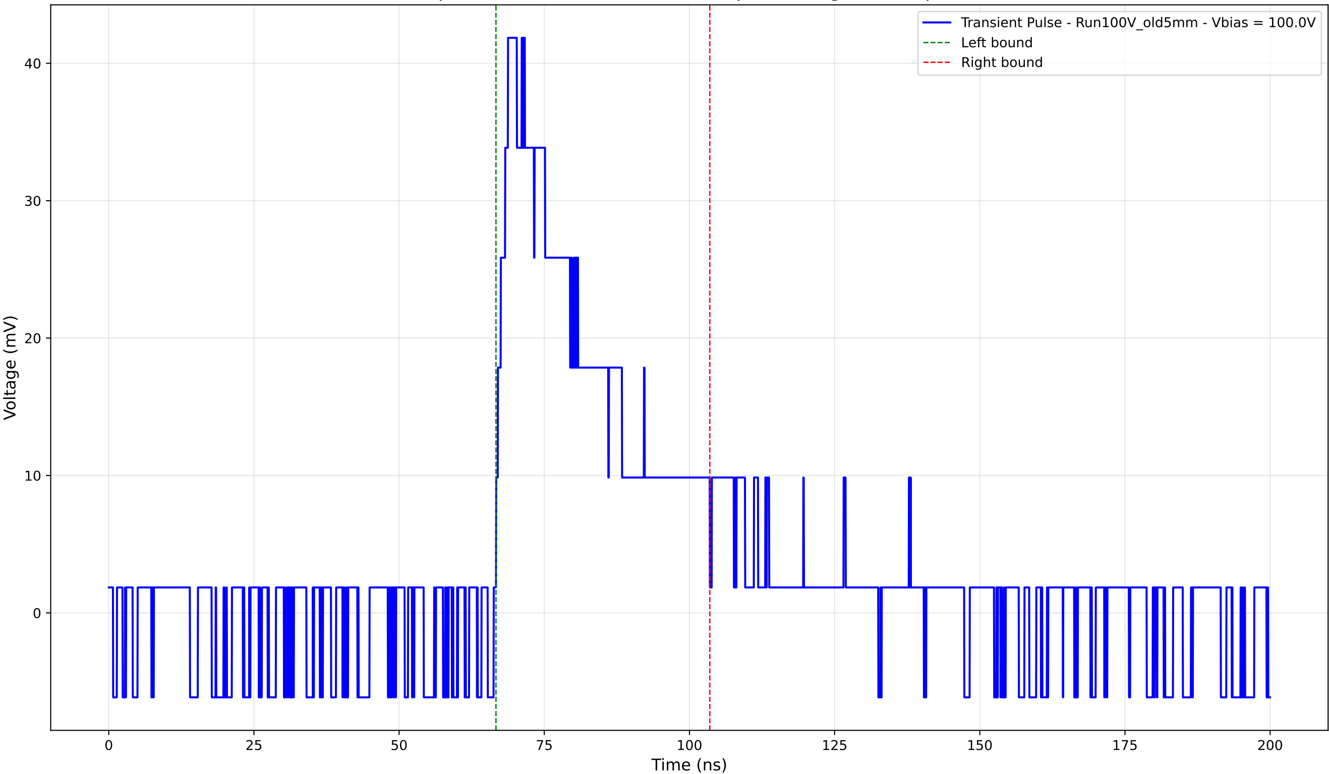
Transient Pulse - Sample: Old5mm - Position: 2645.0 \mu\text{m} - Charge: 14.06 pC - Rise Time: 2.05 ns
