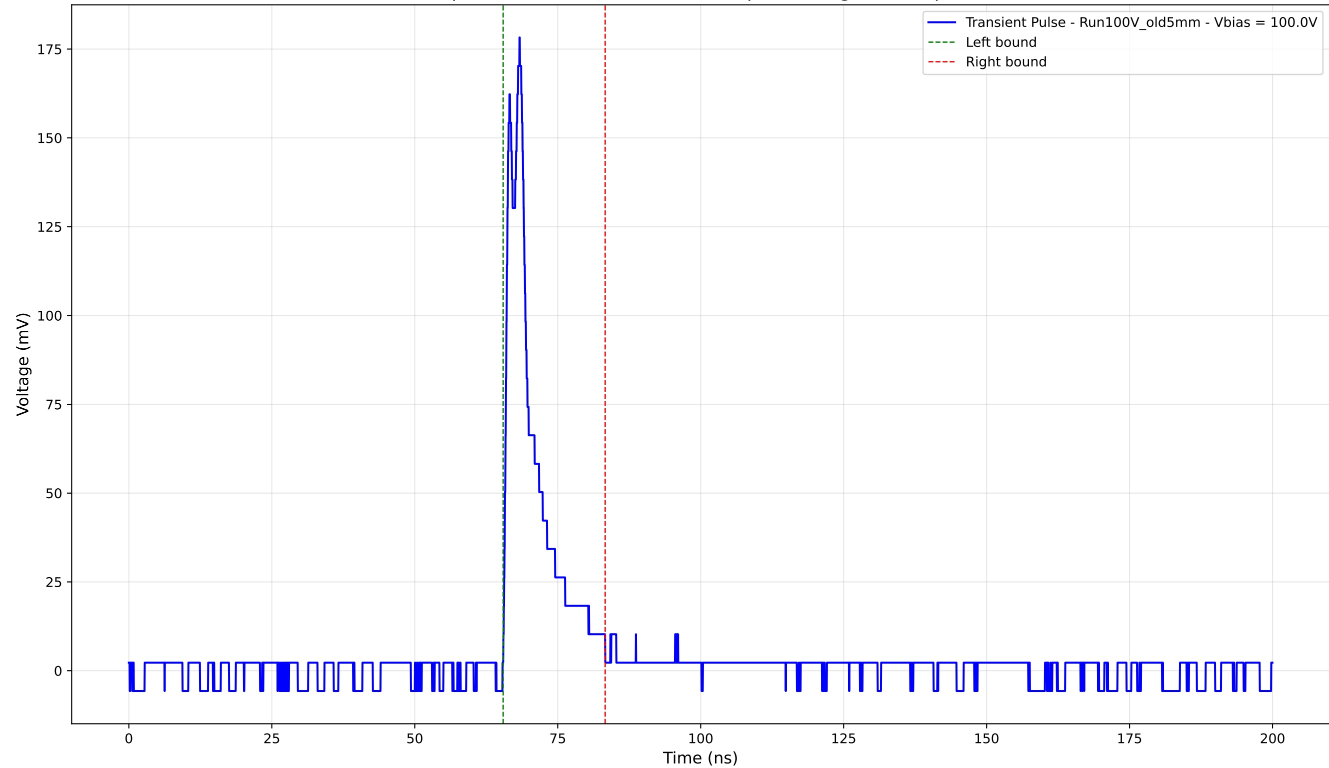
Transient Pulse - Sample: Old5mm - Position: 3890.0 \mu\text{m} - Charge: 18.62 pC - Rise Time: 0.98 ns
