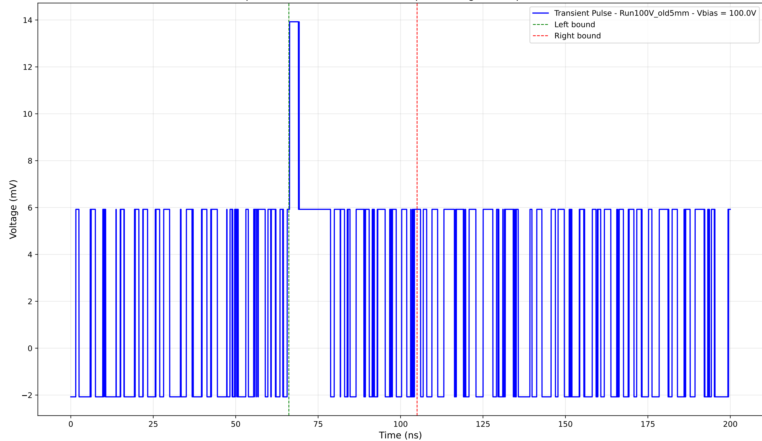
Transient Pulse - Sample: Old5mm - Position: 3985.0 \mu\text{m} - Charge: 3.18 pC - Rise Time: 0.00 ns (N/A)
