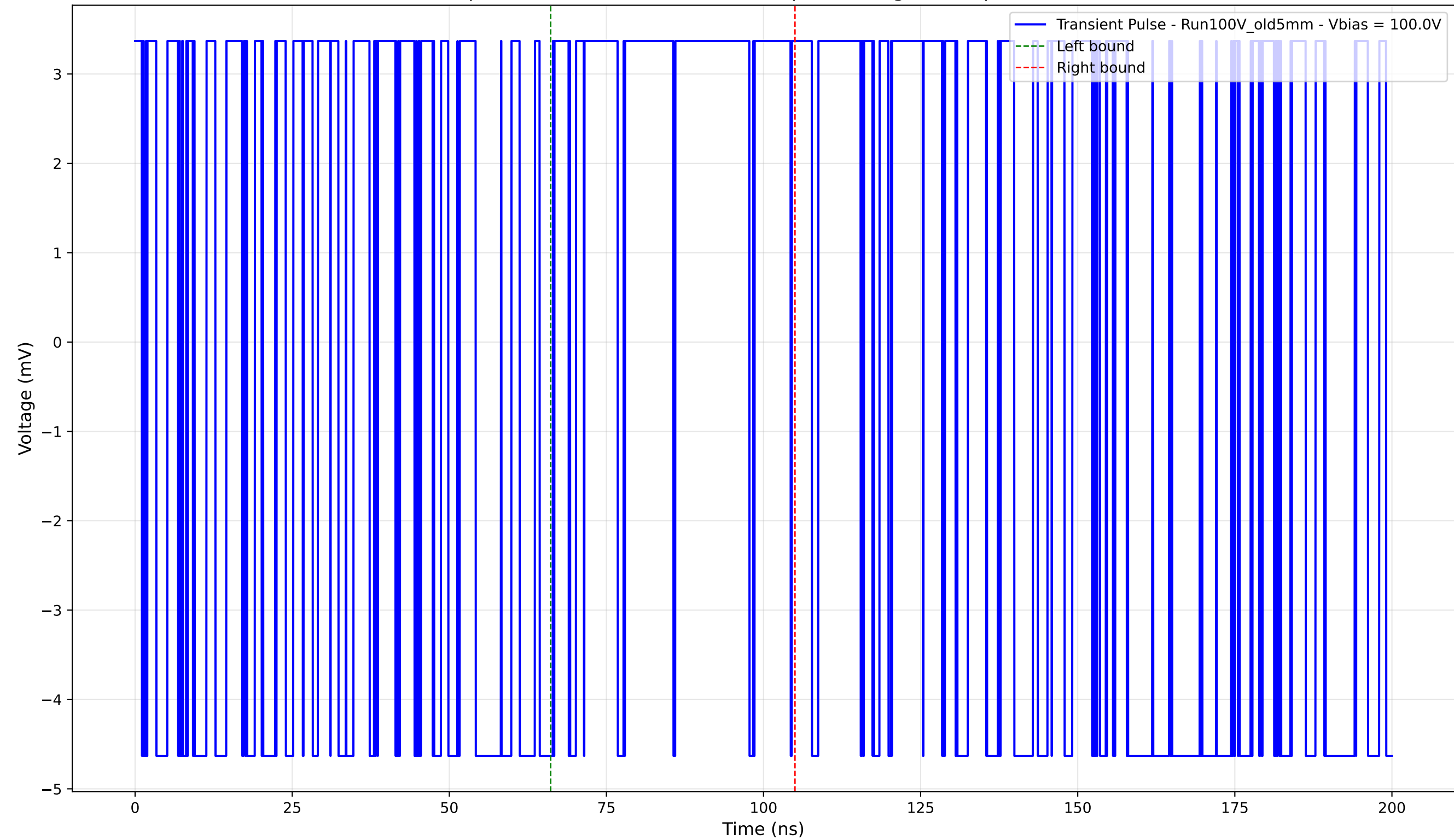
Transient Pulse - Sample: Old5mm - Position: 1930.0 \mu\text{m} - Charge: 1.99 pC - Rise Time: 0.00 ns (N/A)
