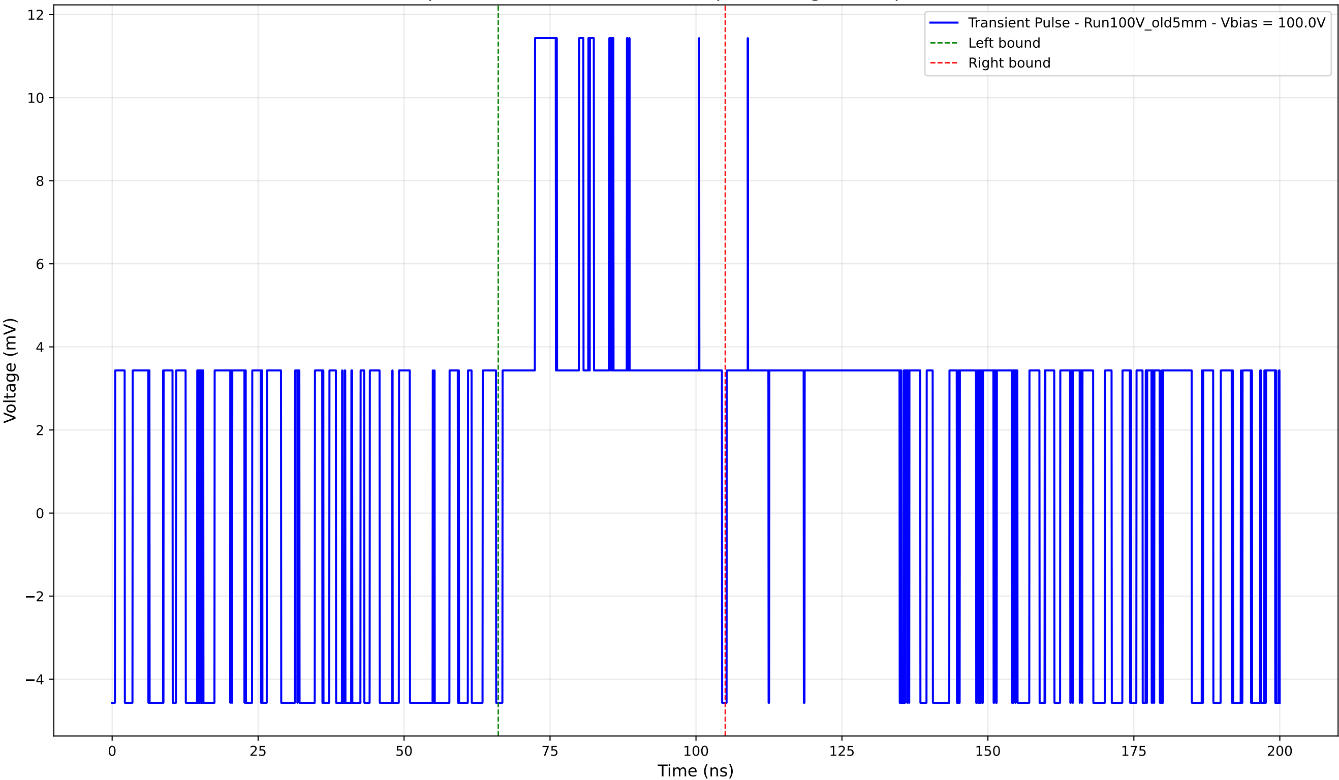
Transient Pulse - Sample: Old5mm - Position: 840.0 \mu\text{m} - Charge: 3.42 pC - Rise Time: 0.00 ns (N/A)
