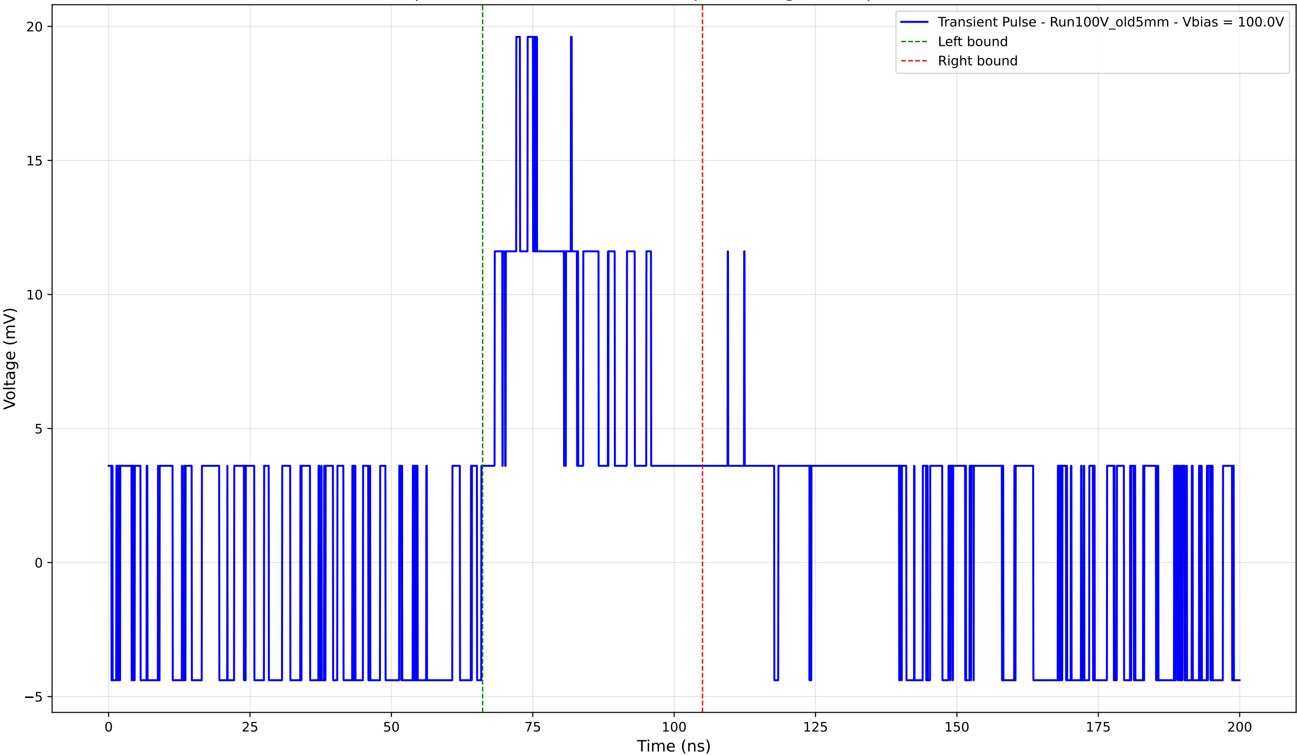
Transient Pulse - Sample: Old5mm - Position: 345.0 \mu\text{m} - Charge: 6.40 pC - Rise Time: 0.00 ns (N/A)
