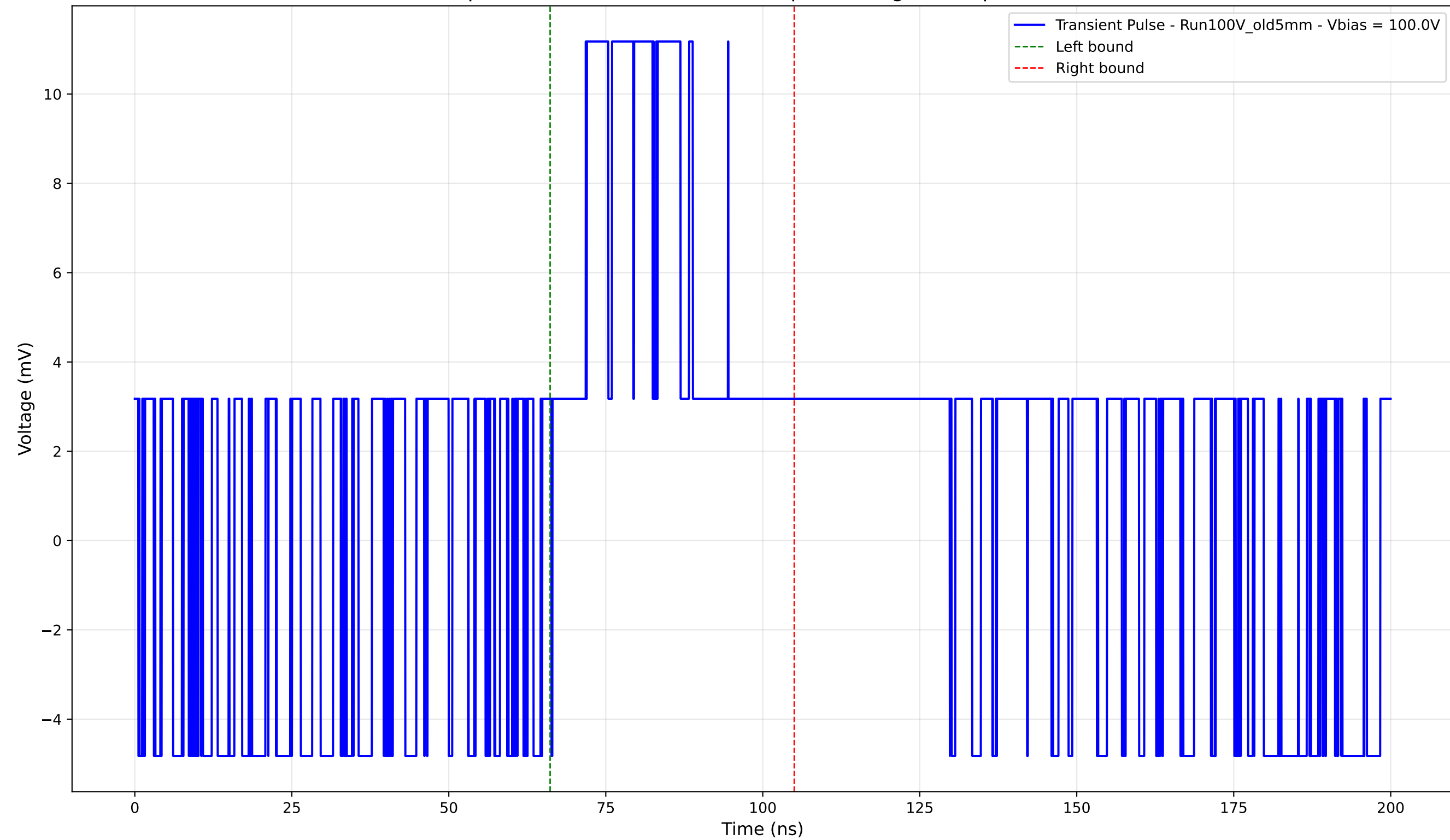
Transient Pulse - Sample: Old5mm - Position: 1360.0 \mu\text{m} - Charge: 4.74 pC - Rise Time: 0.00 ns (N/A)
