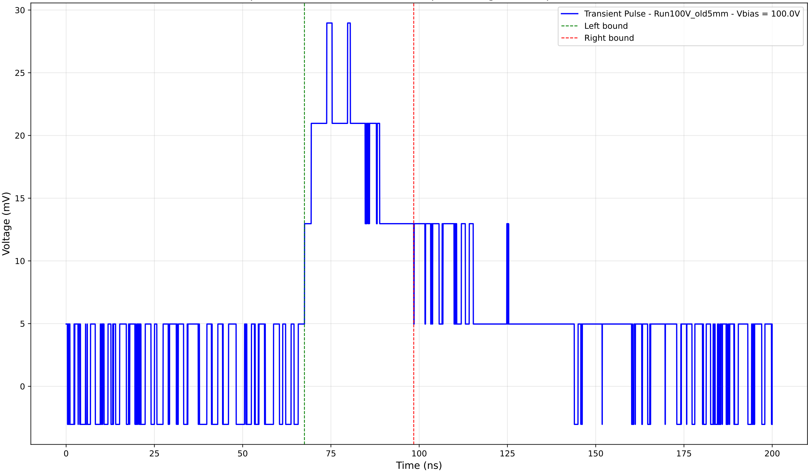
Transient Pulse - Sample: Old5mm - Position: 2205.0 \mu\text{m} - Charge: 11.36 pC - Rise Time: 0.00 ns (N/A)
