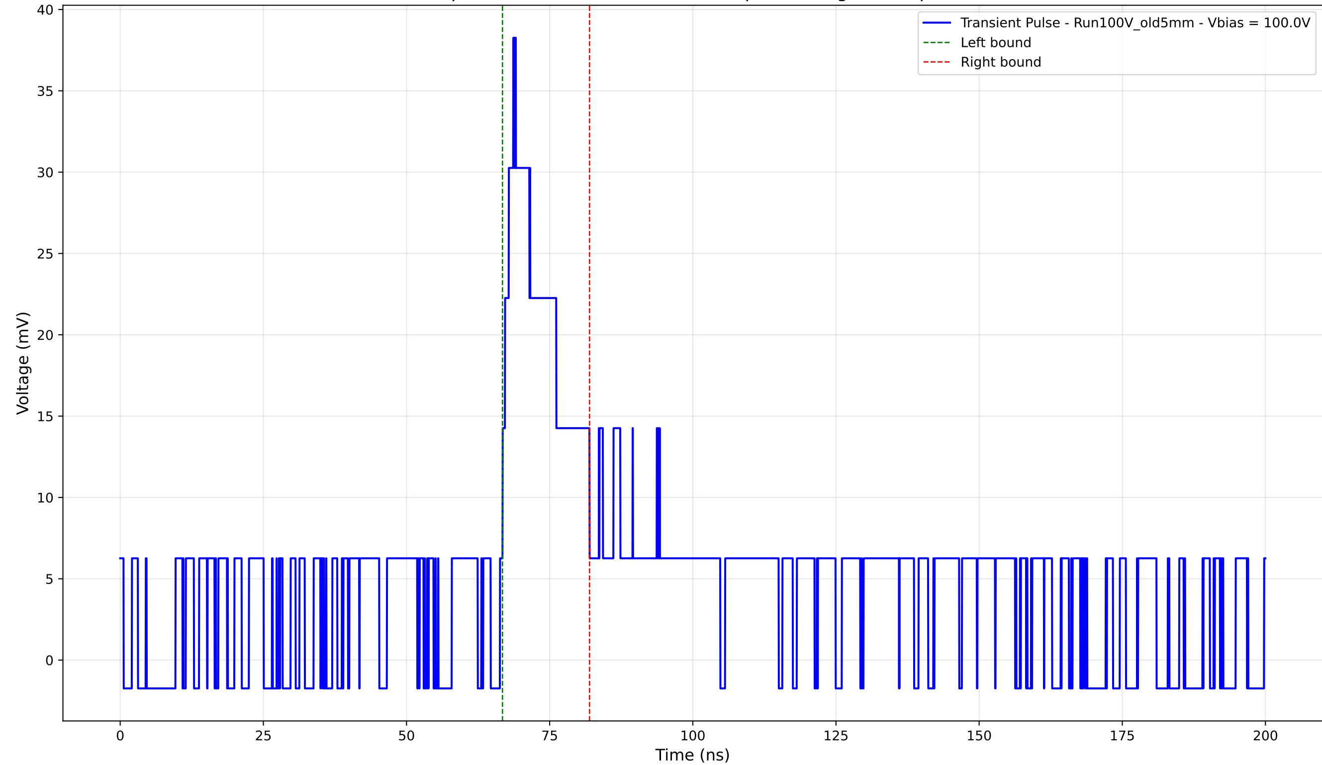
Transient Pulse - Sample: Old5mm - Position: 2870.0 \mu\text{m} - Charge: 6.39 pC - Rise Time: 2.33 ns
