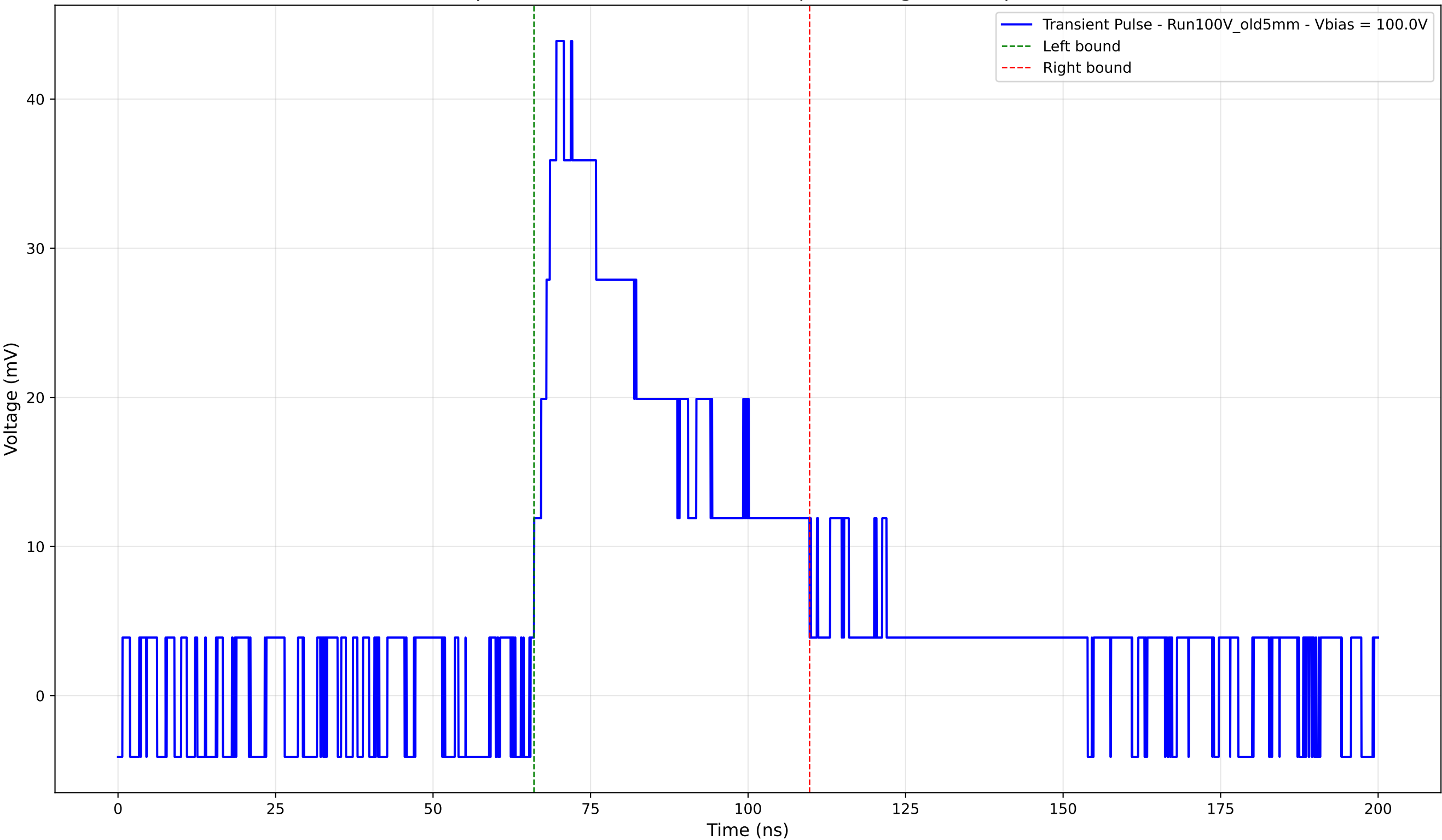
Transient Pulse - Sample: Old5mm - Position: 4910.0 \mu\text{m} - Charge: 18.26 pC - Rise Time: 3.54 ns
