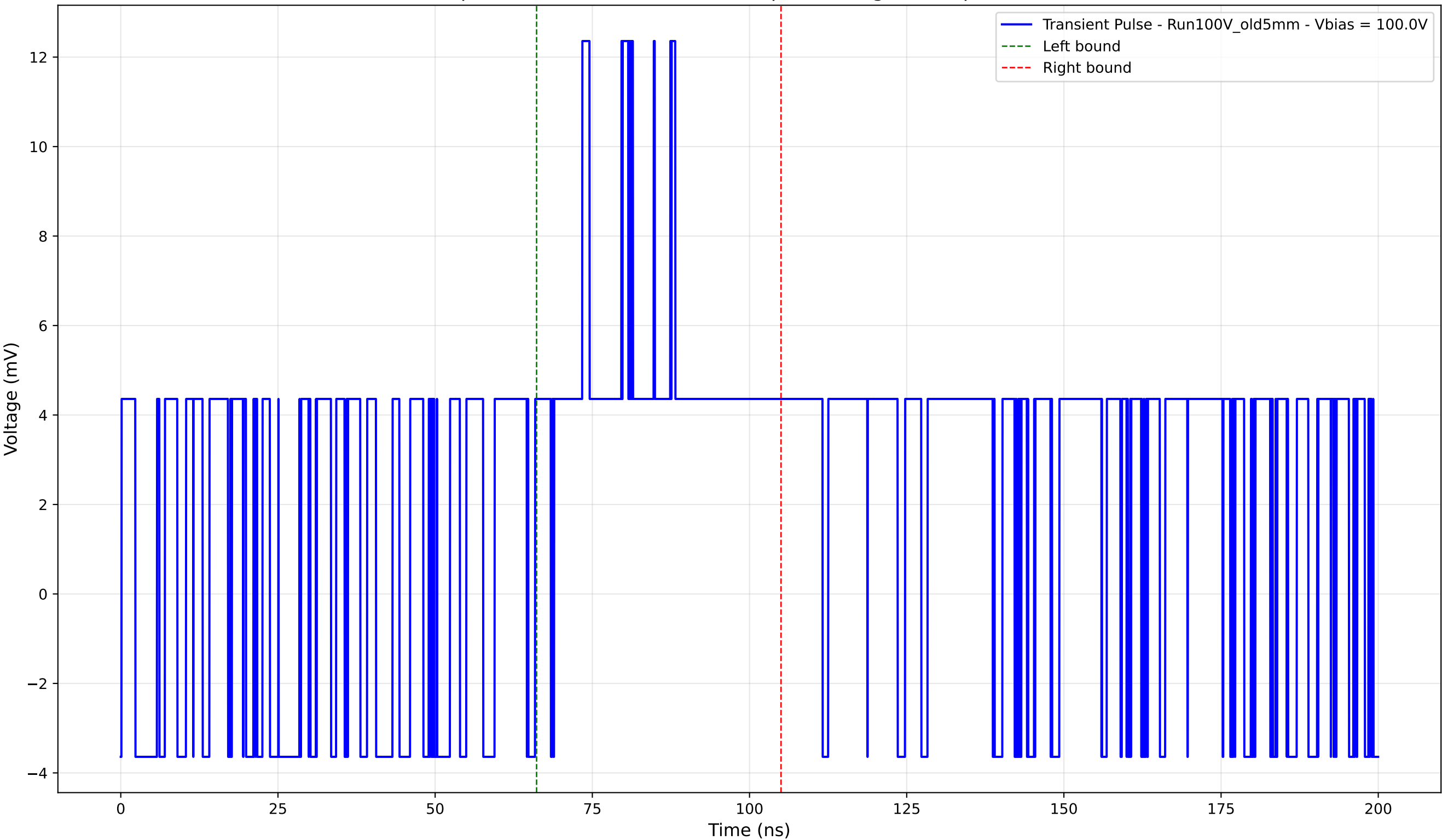
Transient Pulse - Sample: Old5mm - Position: 630.0 \mu\text{m} - Charge: 3.87 pC - Rise Time: 0.00 ns (N/A)
