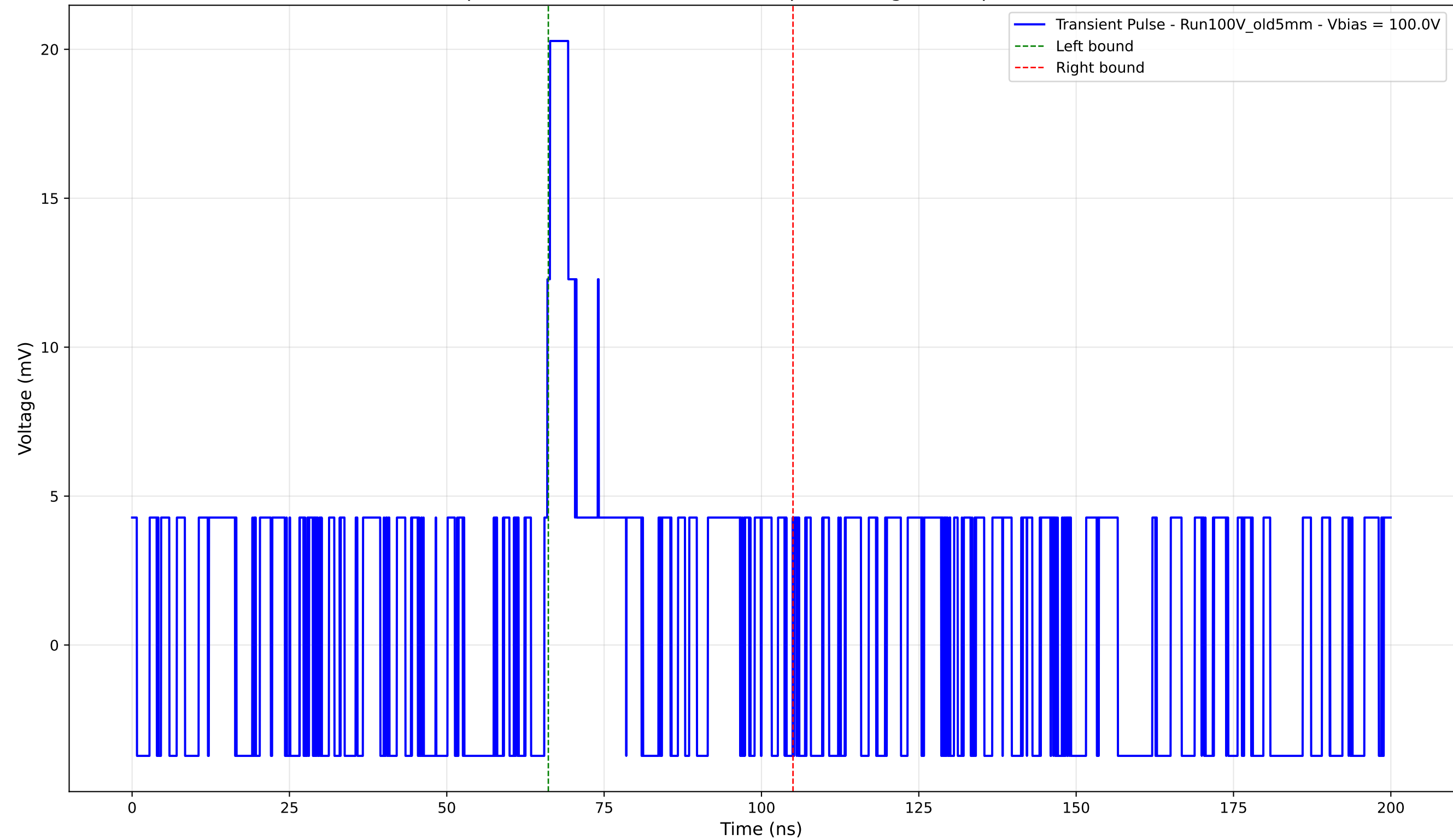
Transient Pulse - Sample: Old5mm - Position: 3975.0 \mu\text{m} - Charge: 2.94 pC - Rise Time: 0.00 ns (N/A)
