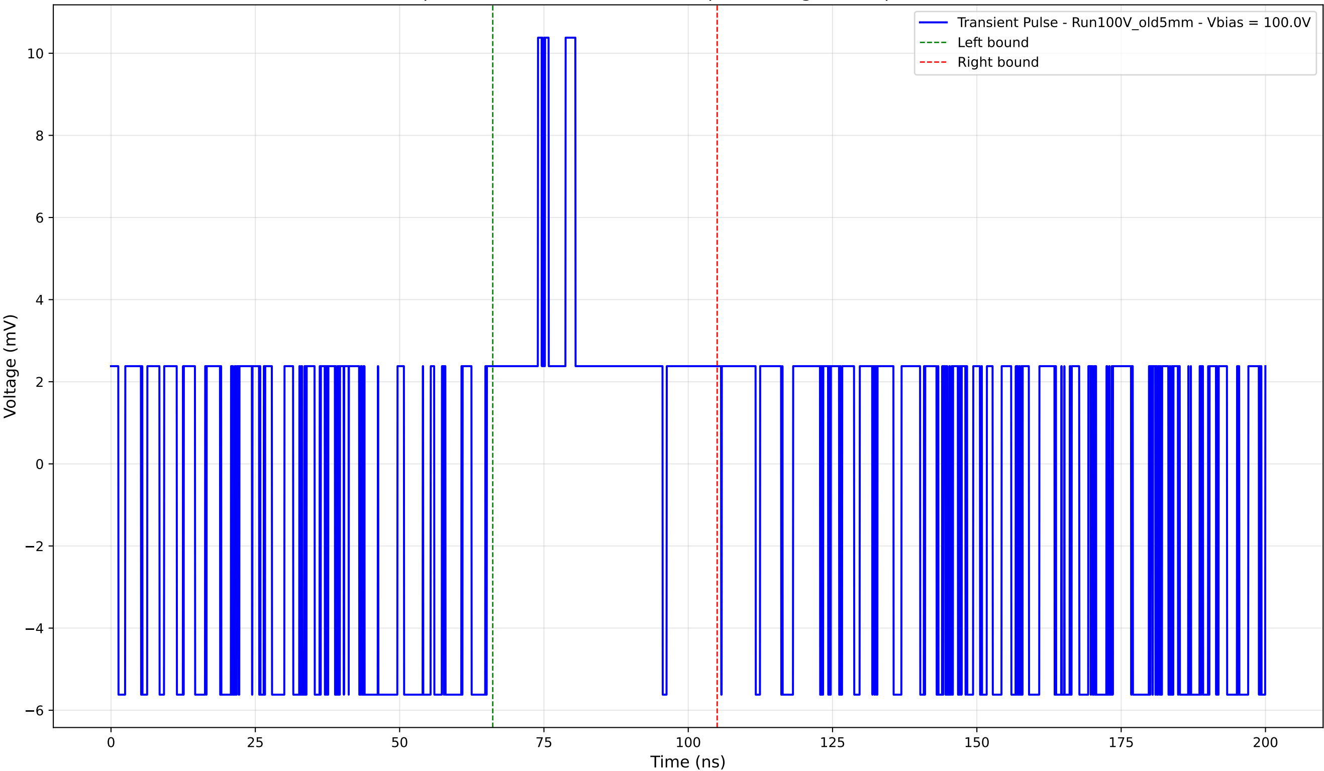
Transient Pulse - Sample: Old5mm - Position: 715.0 \mu\text{m} - Charge: 2.25 pC - Rise Time: 0.00 ns (N/A)
