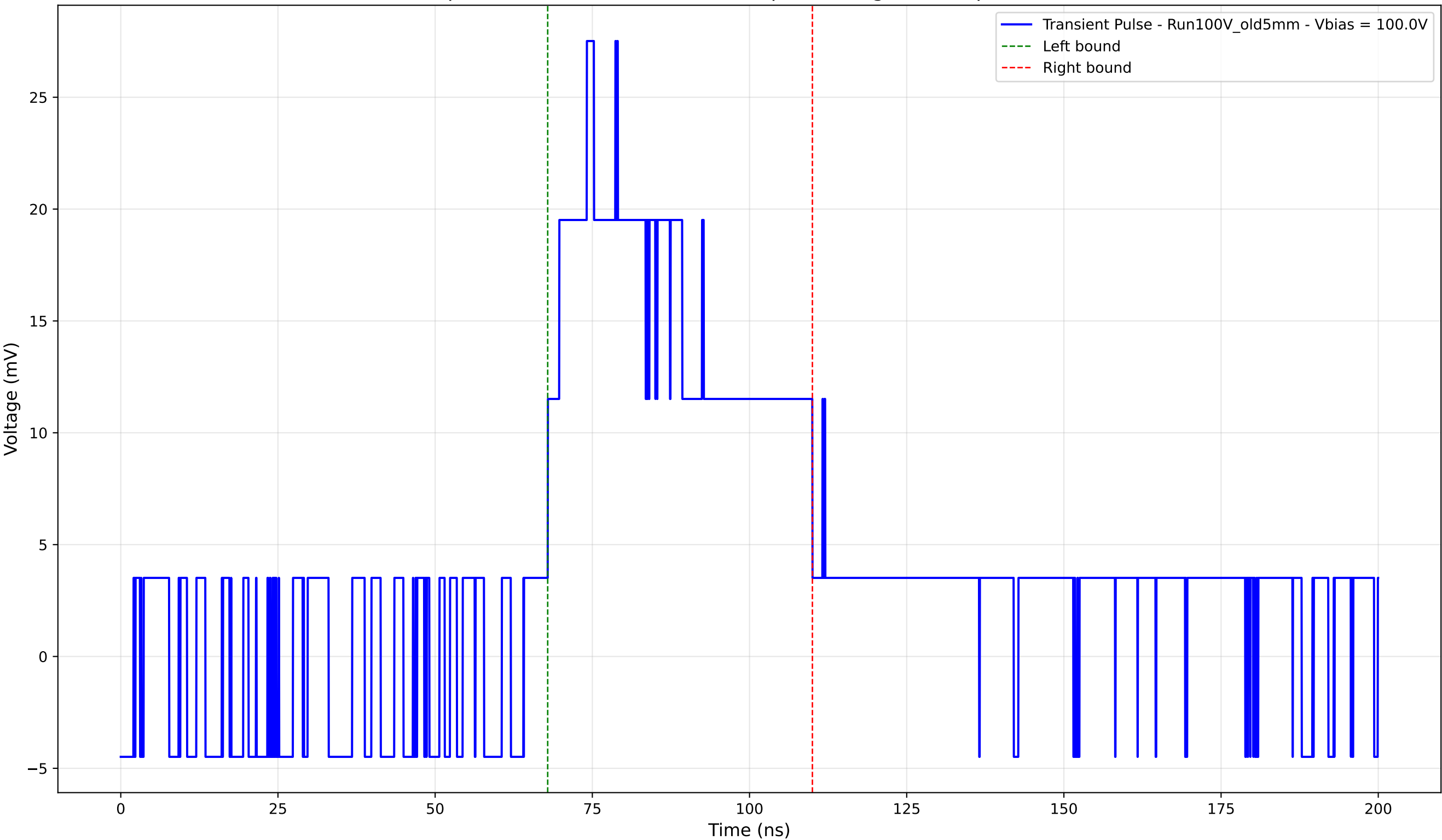
Transient Pulse - Sample: Old5mm - Position: 2210.0 \mu\text{m} - Charge: 13.01 pC - Rise Time: 0.00 ns (N/A)
