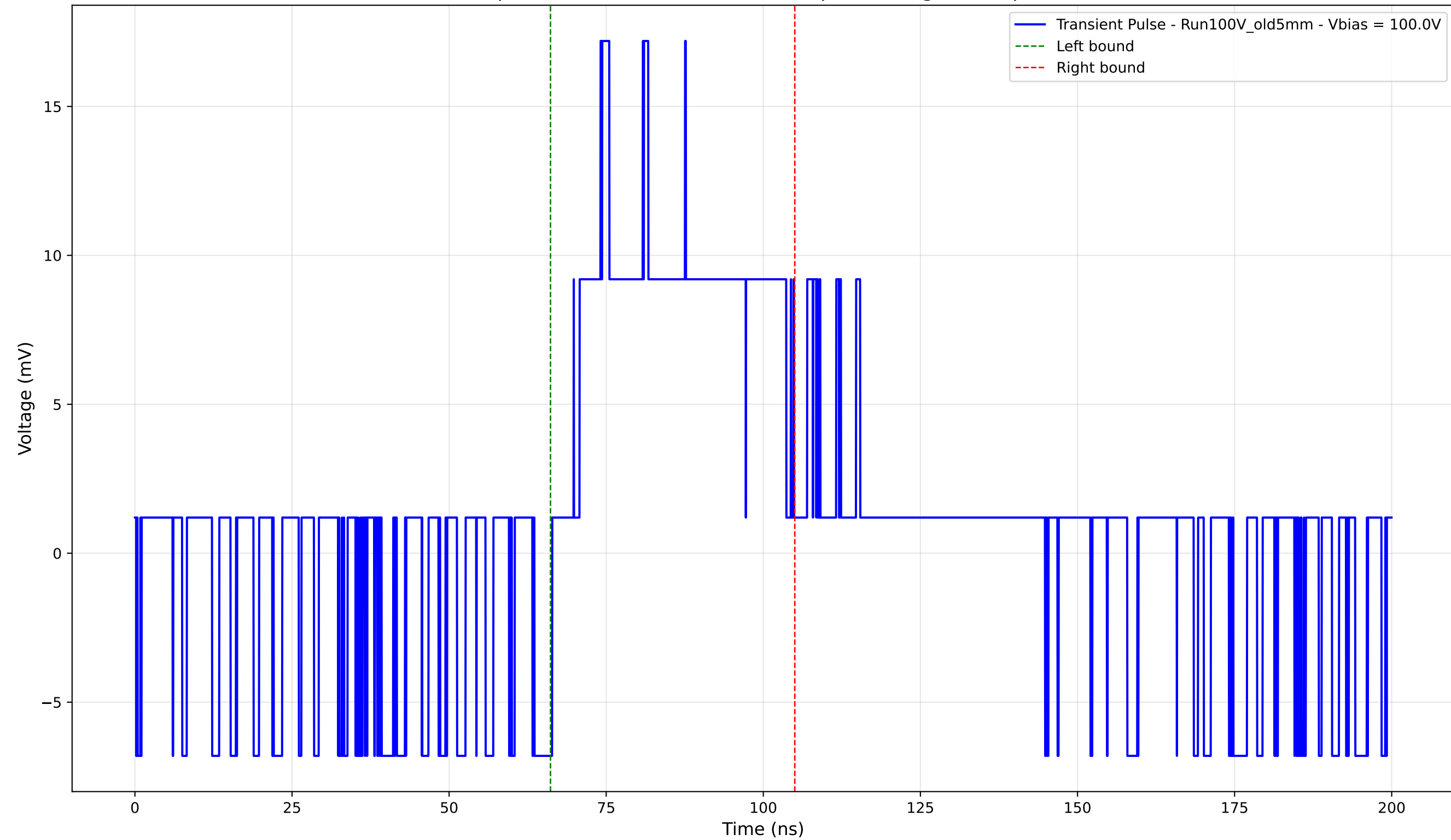
Transient Pulse - Sample: Old5mm - Position: 1580.0 \mu\text{m} - Charge: 6.53 pC - Rise Time: 3.36 ns
