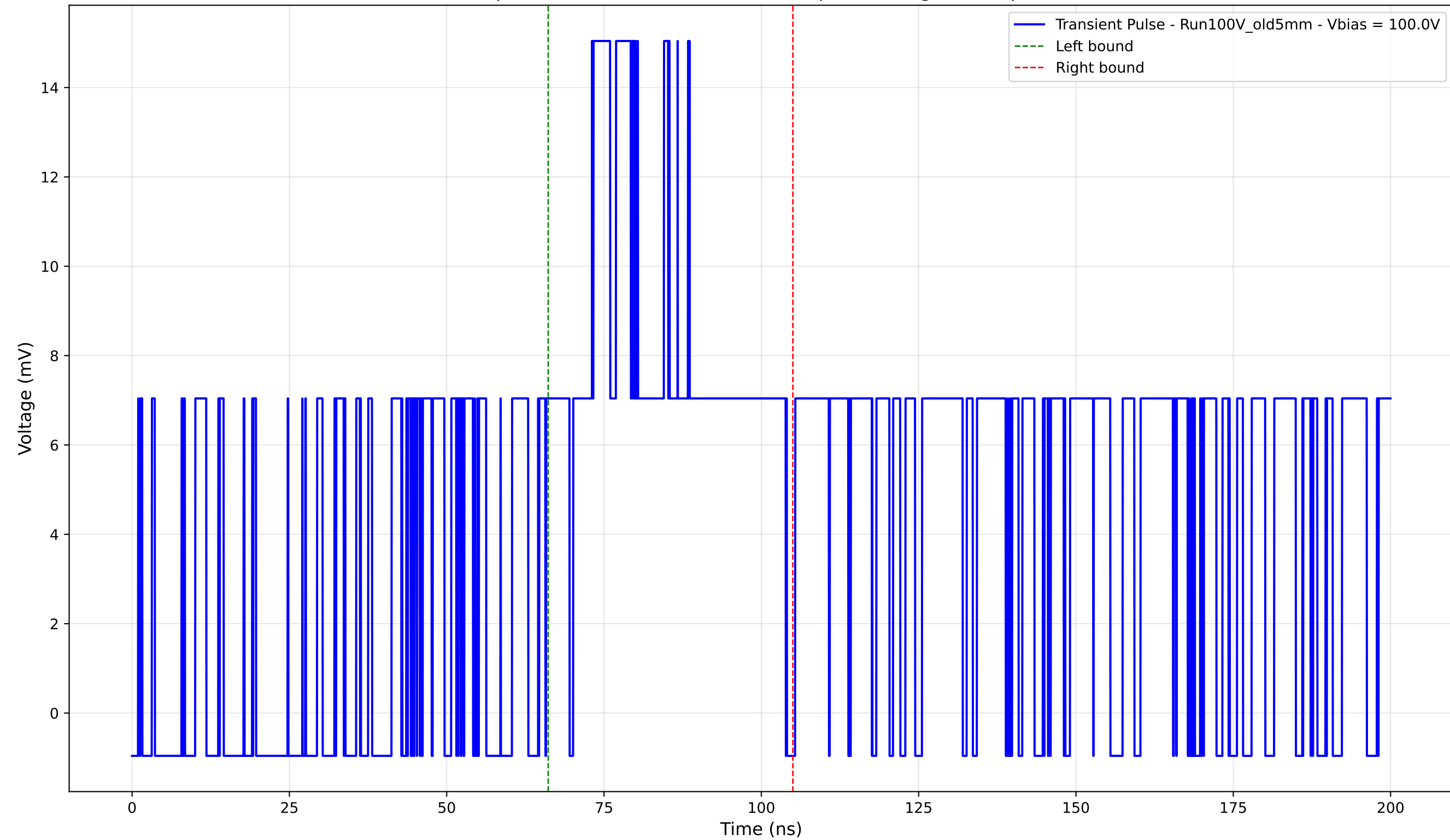
Transient Pulse - Sample: Old5mm - Position: 1015.0 \mu\text{m} - Charge: 6.26 pC - Rise Time: 3.02 ns
