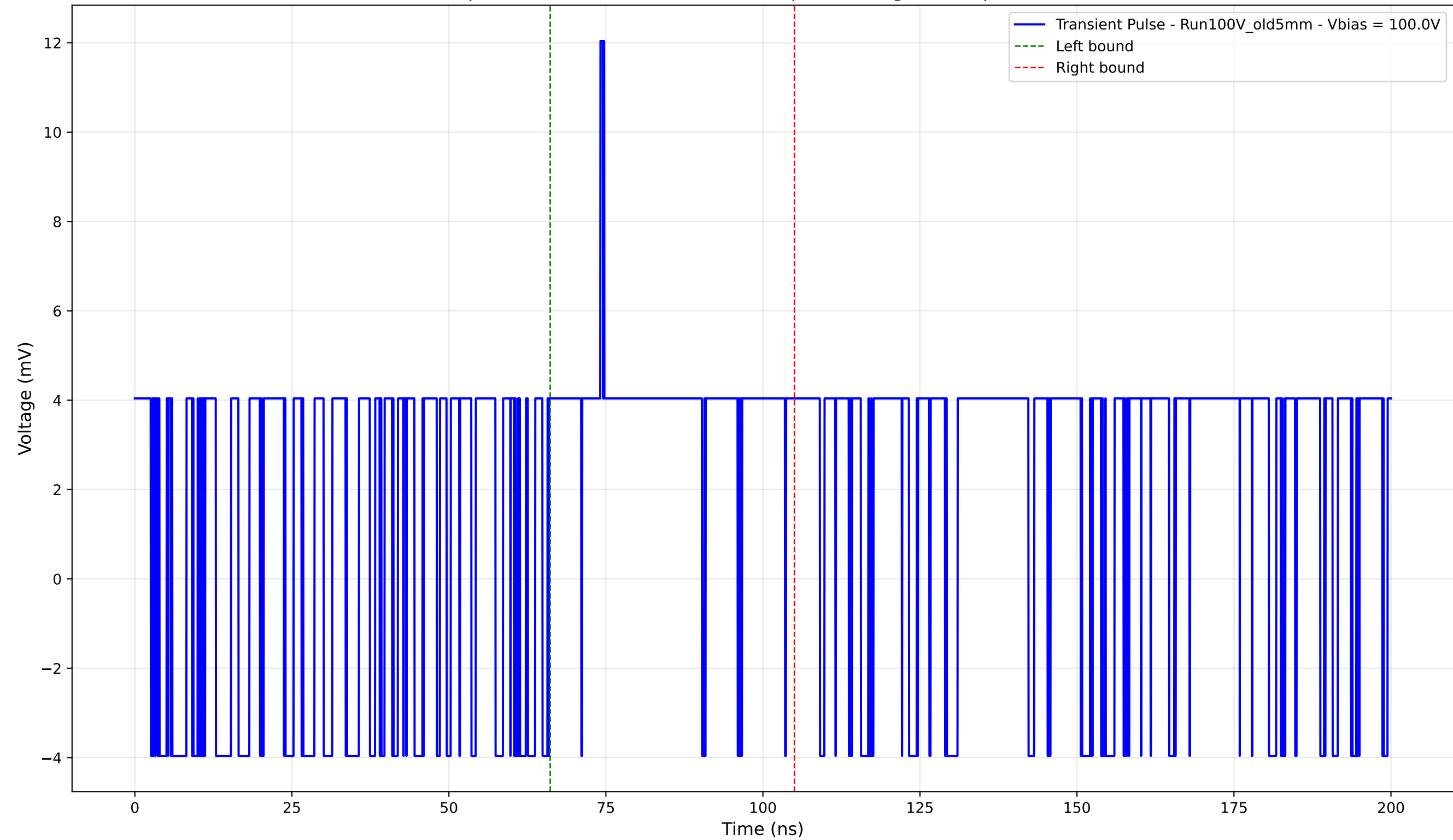
Transient Pulse - Sample: Old5mm - Position: 2100.0 \mu\text{m} - Charge: 3.03 pC - Rise Time: 0.00 ns (N/A)
