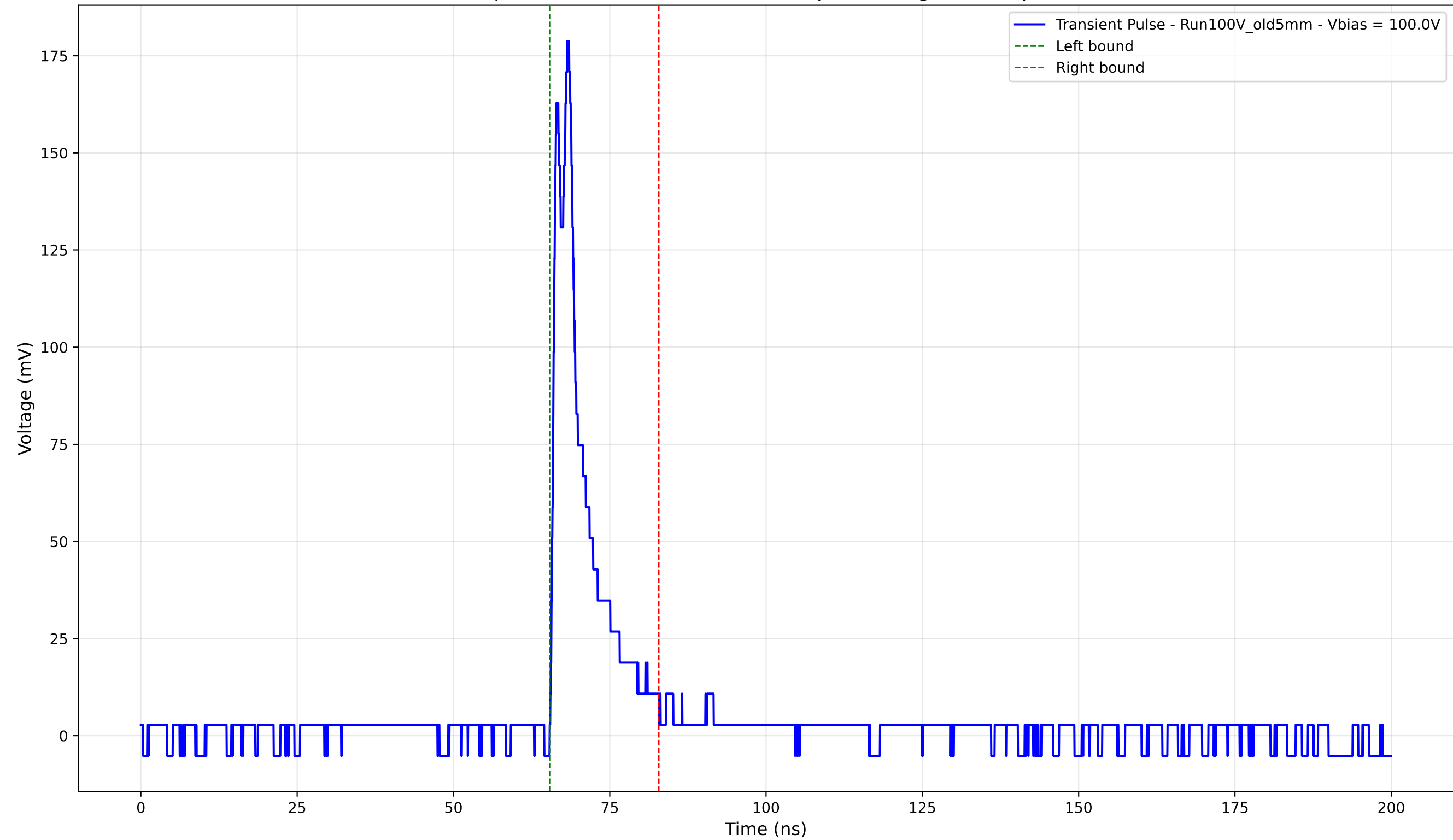
Transient Pulse - Sample: Old5mm - Position: 3530.0 \mu\text{m} - Charge: 19.10 pC - Rise Time: 0.88 ns
