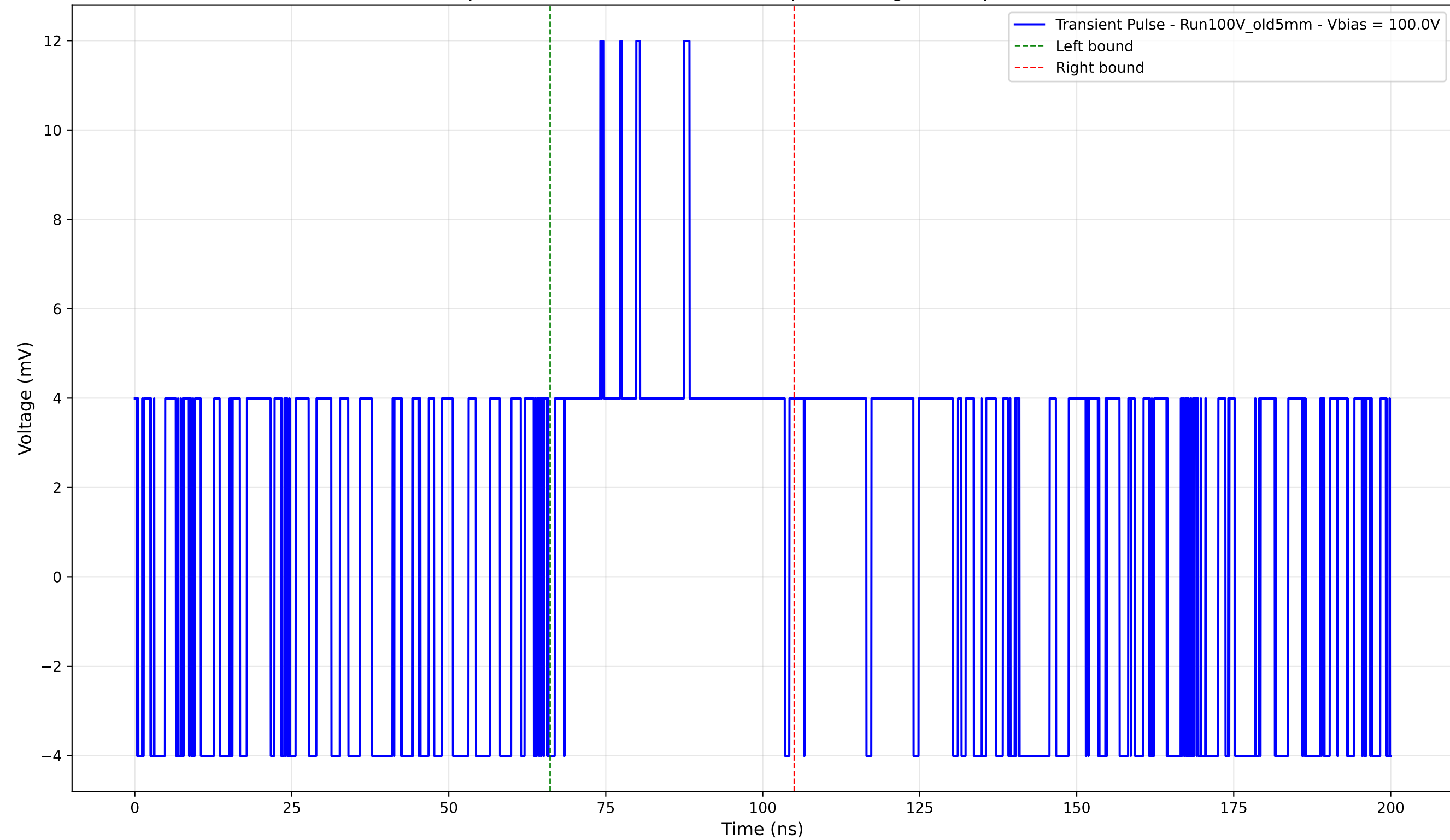
Transient Pulse - Sample: Old5mm - Position: 2090.0 \mu\text{m} - Charge: 3.22 pC - Rise Time: 0.00 ns (N/A)
