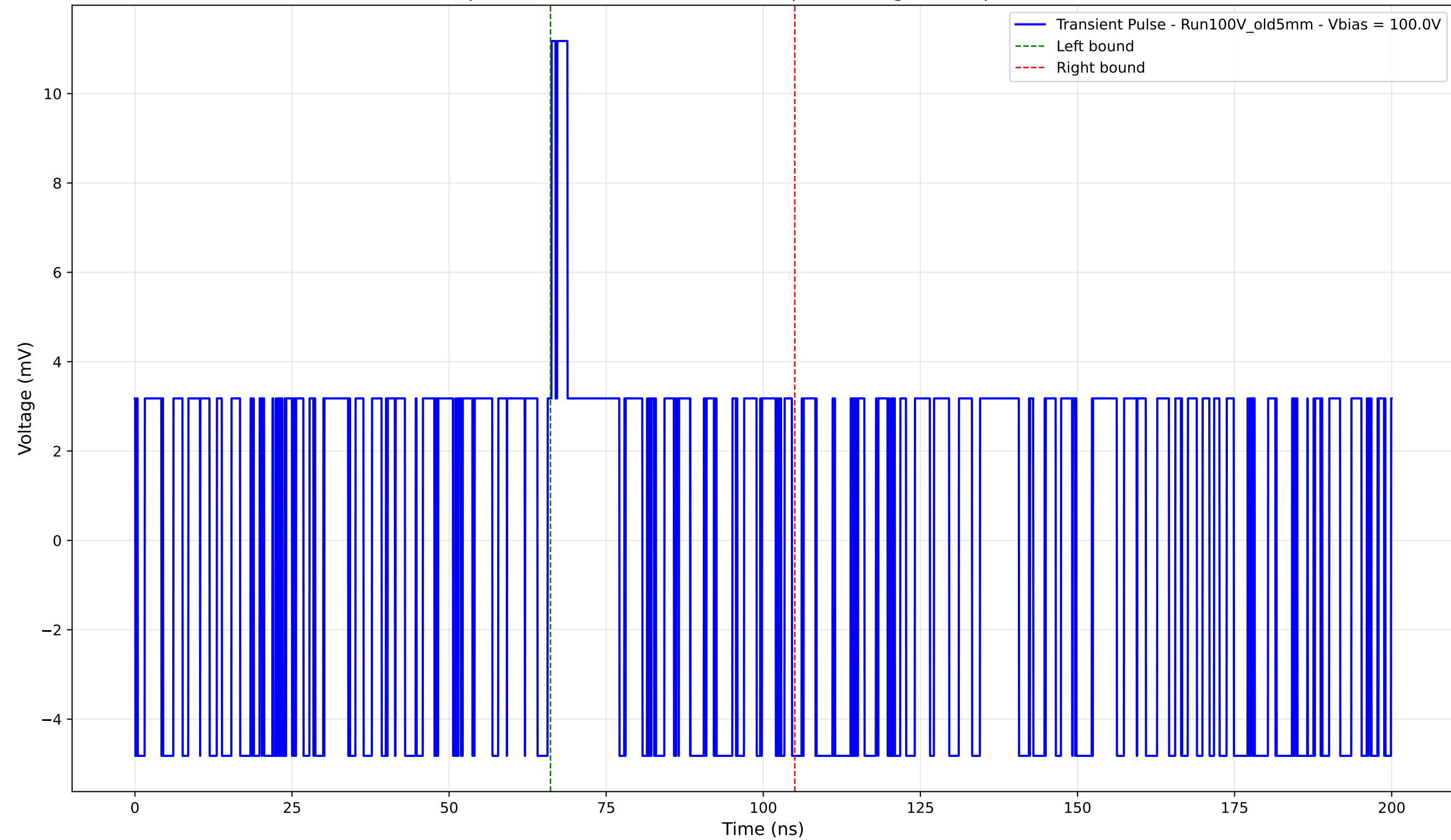
Transient Pulse - Sample: Old5mm - Position: 3705.0 \mu\text{m} - Charge: 0.88 pC - Rise Time: 0.00 ns (N/A)
