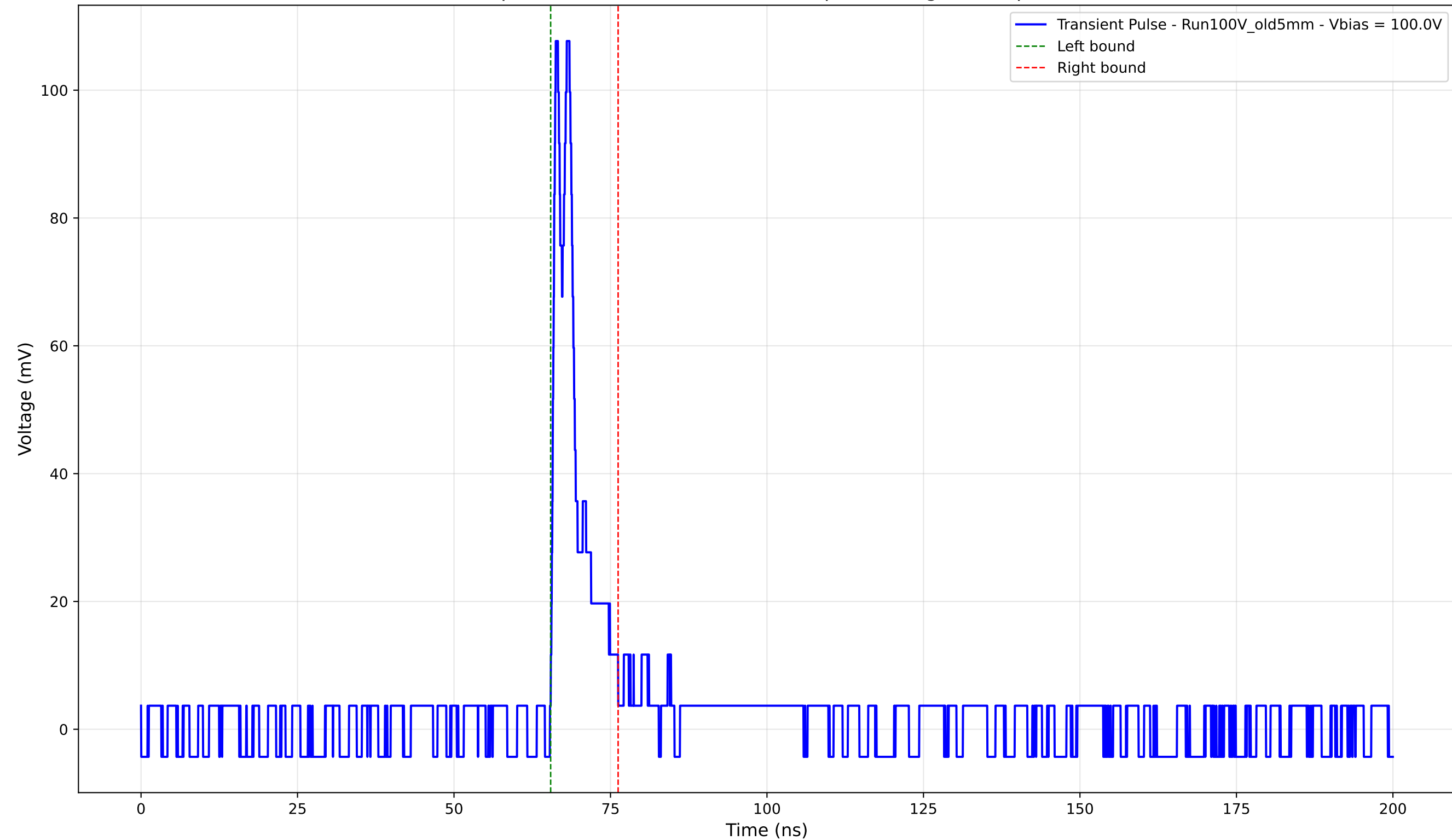
Transient Pulse - Sample: Old5mm - Position: 3640.0 \mu\text{m} - Charge: 9.37 pC - Rise Time: 0.70 ns
