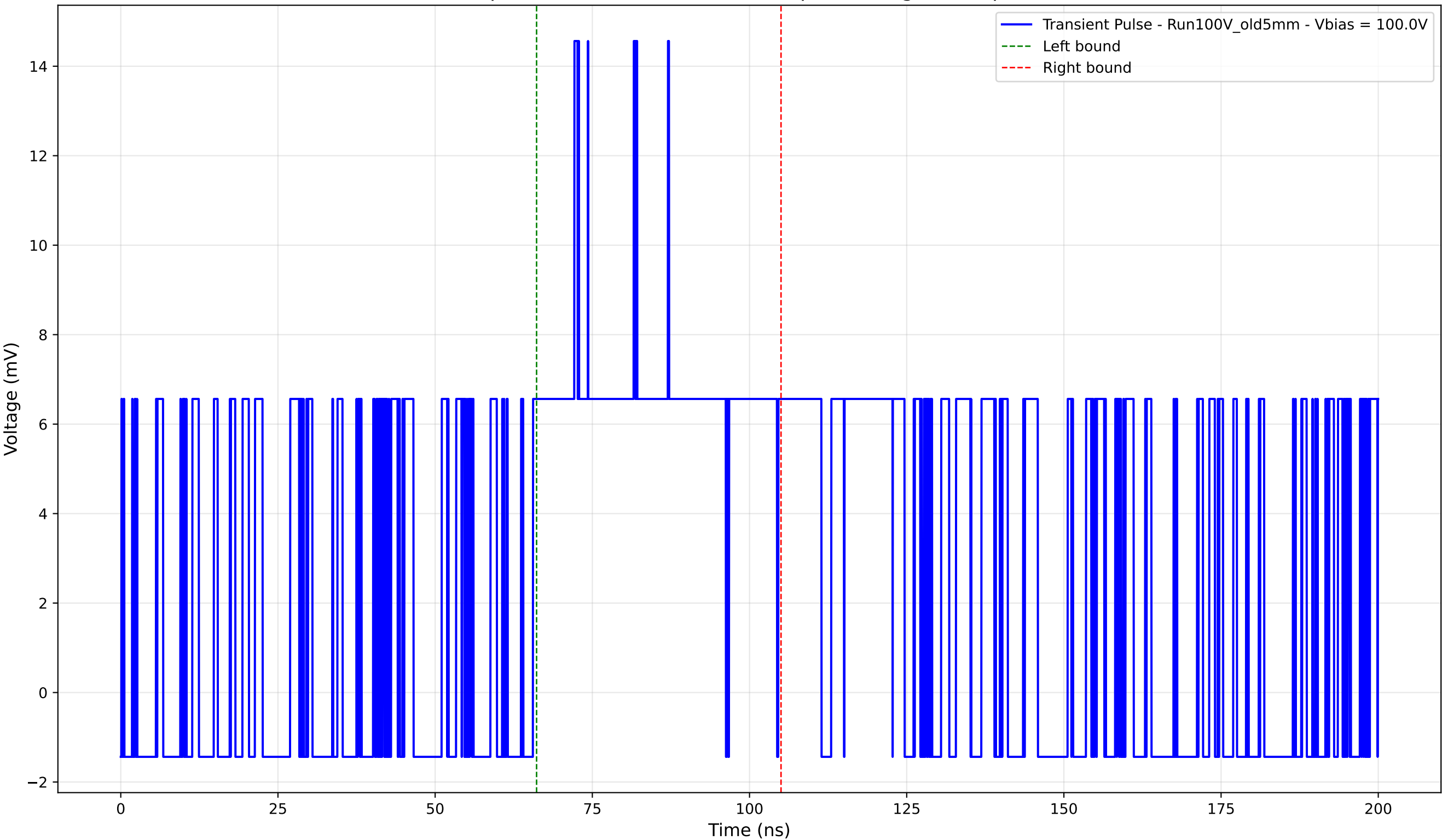
Transient Pulse - Sample: Old5mm - Position: 535.0 \mu\text{m} - Charge: 5.22 pC - Rise Time: 6.60 ns
