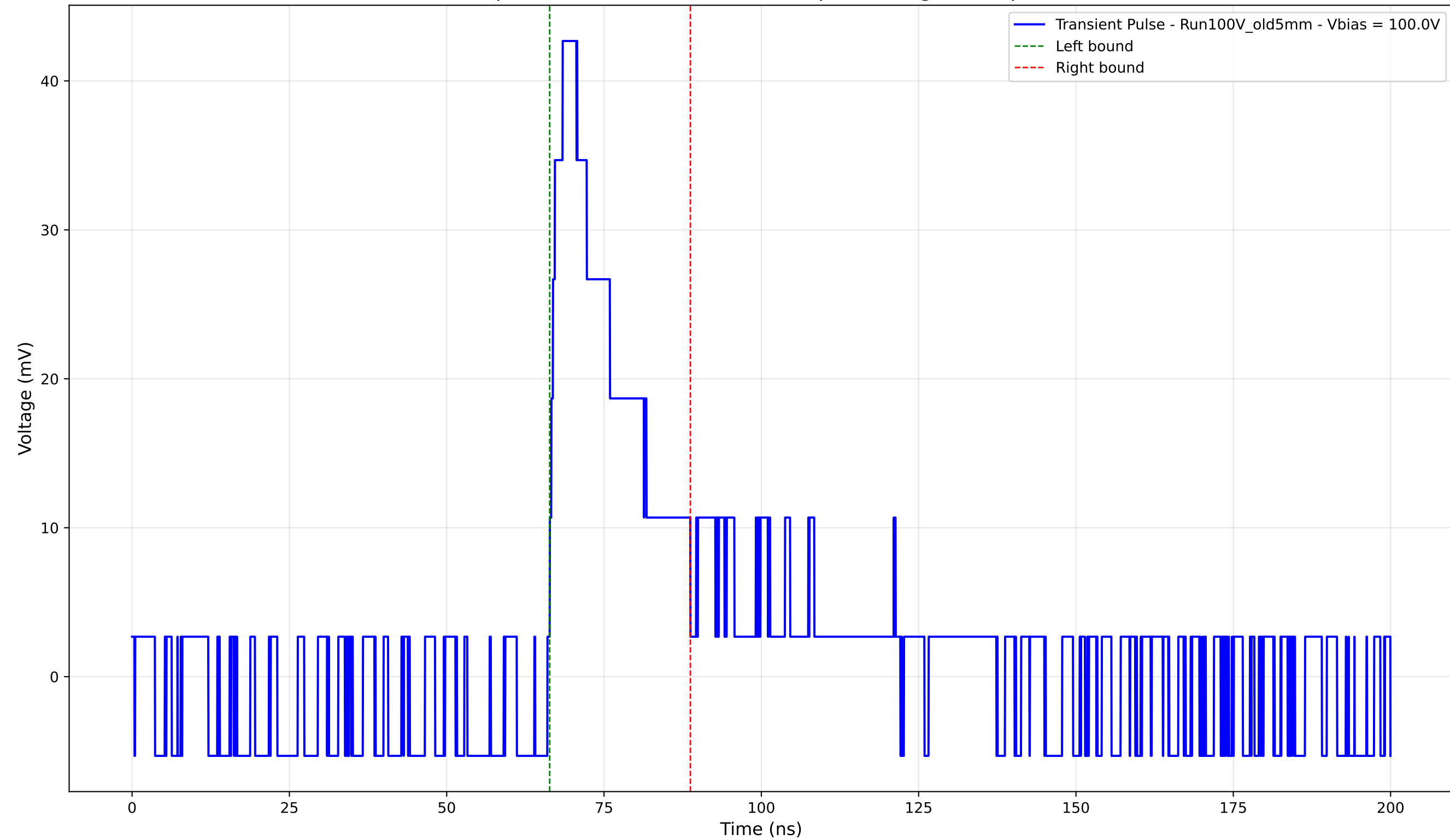
Transient Pulse - Sample: Old5mm - Position: 2890.0 \mu\text{m} - Charge: 9.81 pC - Rise Time: 2.06 ns
