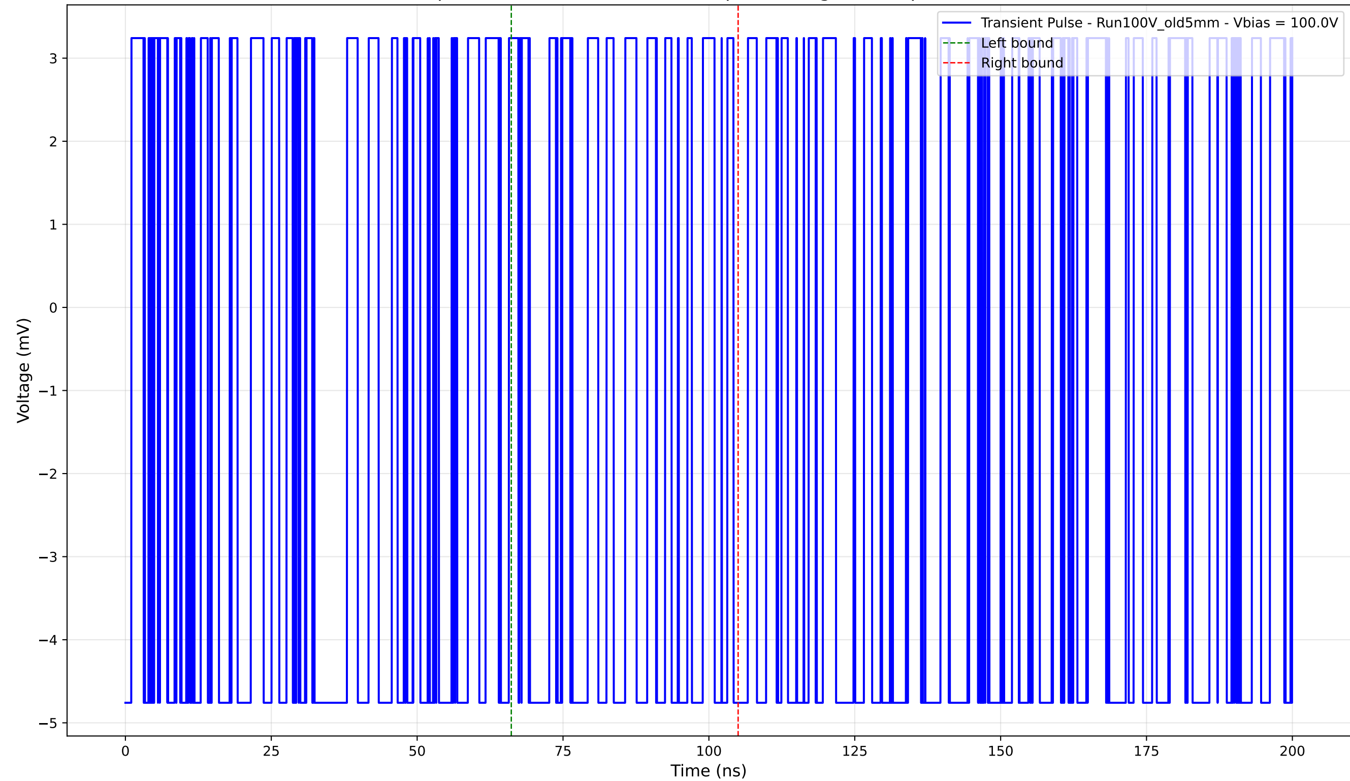
Transient Pulse - Sample: Old5mm - Position: 165.0 \mu\text{m} - Charge: -0.91 pC - Rise Time: 0.00 ns (N/A)
