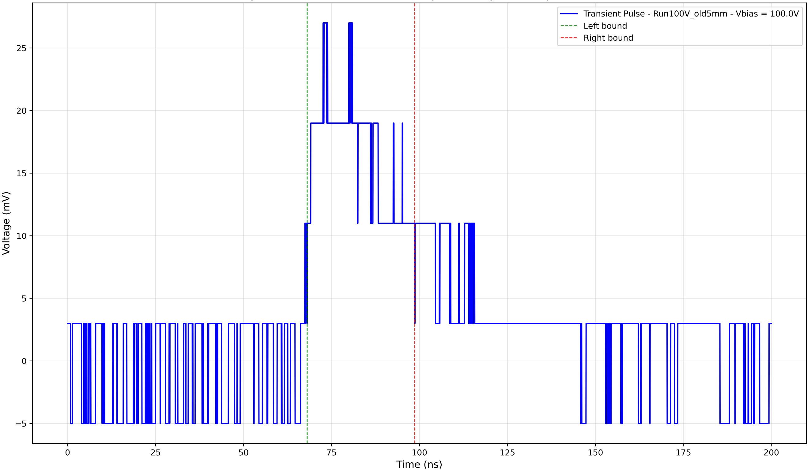
Transient Pulse - Sample: Old5mm - Position: 2230.0 \mu\text{m} - Charge: 10.02 pC - Rise Time: 0.00 ns (N/A)
