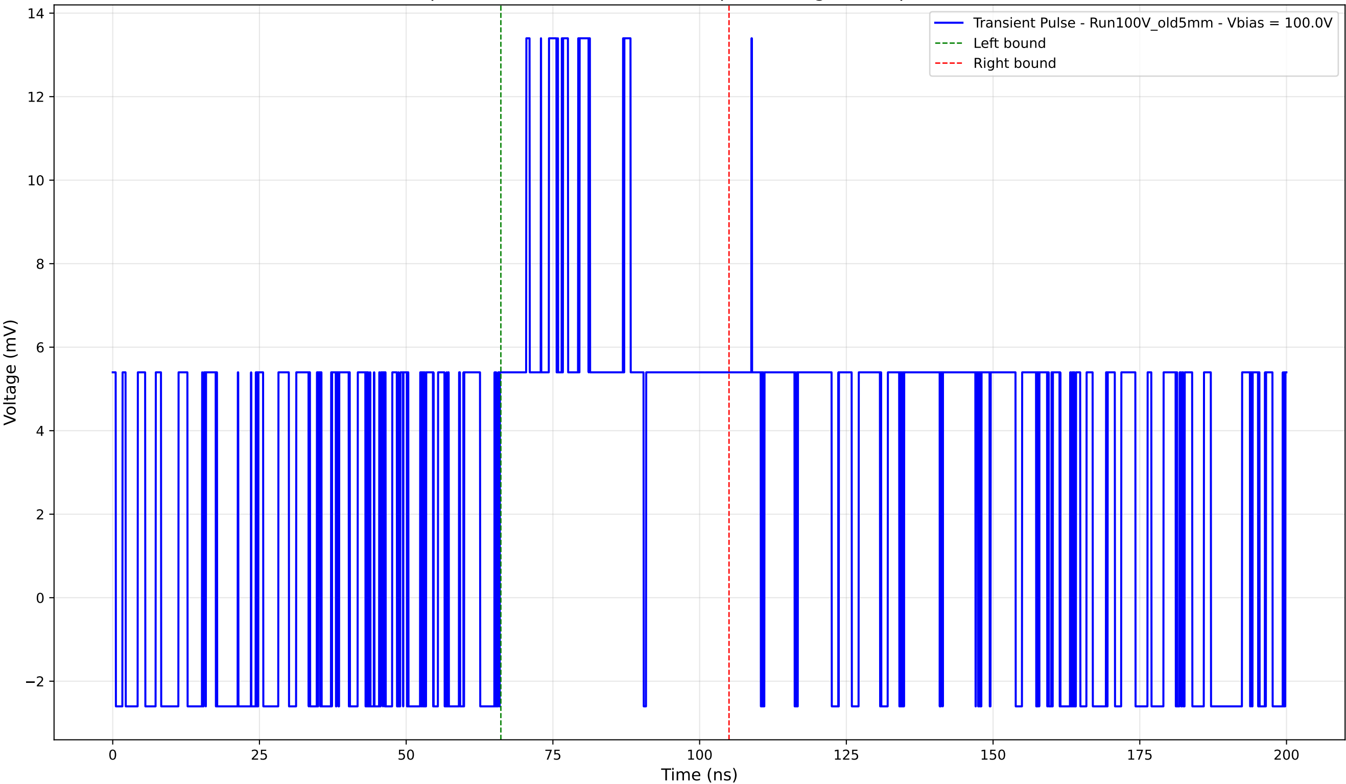
Transient Pulse - Sample: Old5mm - Position: 750.0 \mu\text{m} - Charge: 5.09 pC - Rise Time: 0.00 ns (N/A)
