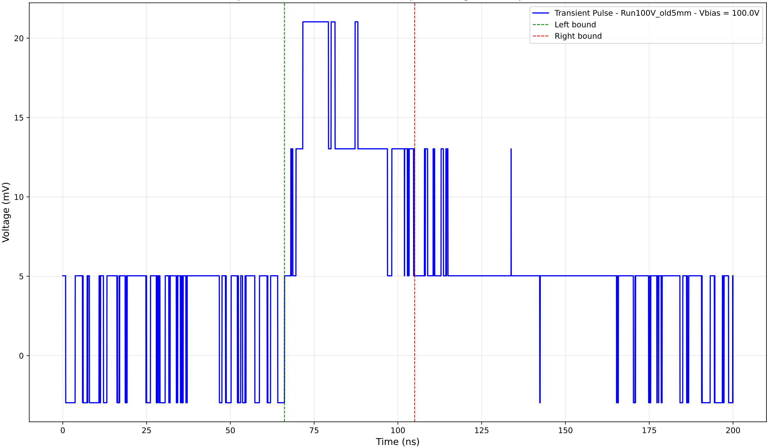
Transient Pulse - Sample: Old5mm - Position: 2045.0 \mu\text{m} - Charge: 10.90 pC - Rise Time: 0.00 ns (N/A)
