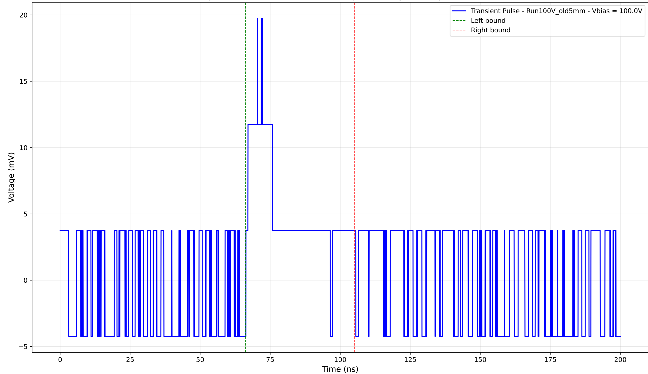
Transient Pulse - Sample: Old5mm - Position: 2850.0 \mu\text{m} - Charge: 4.19 pC - Rise Time: 0.00 ns (N/A)
