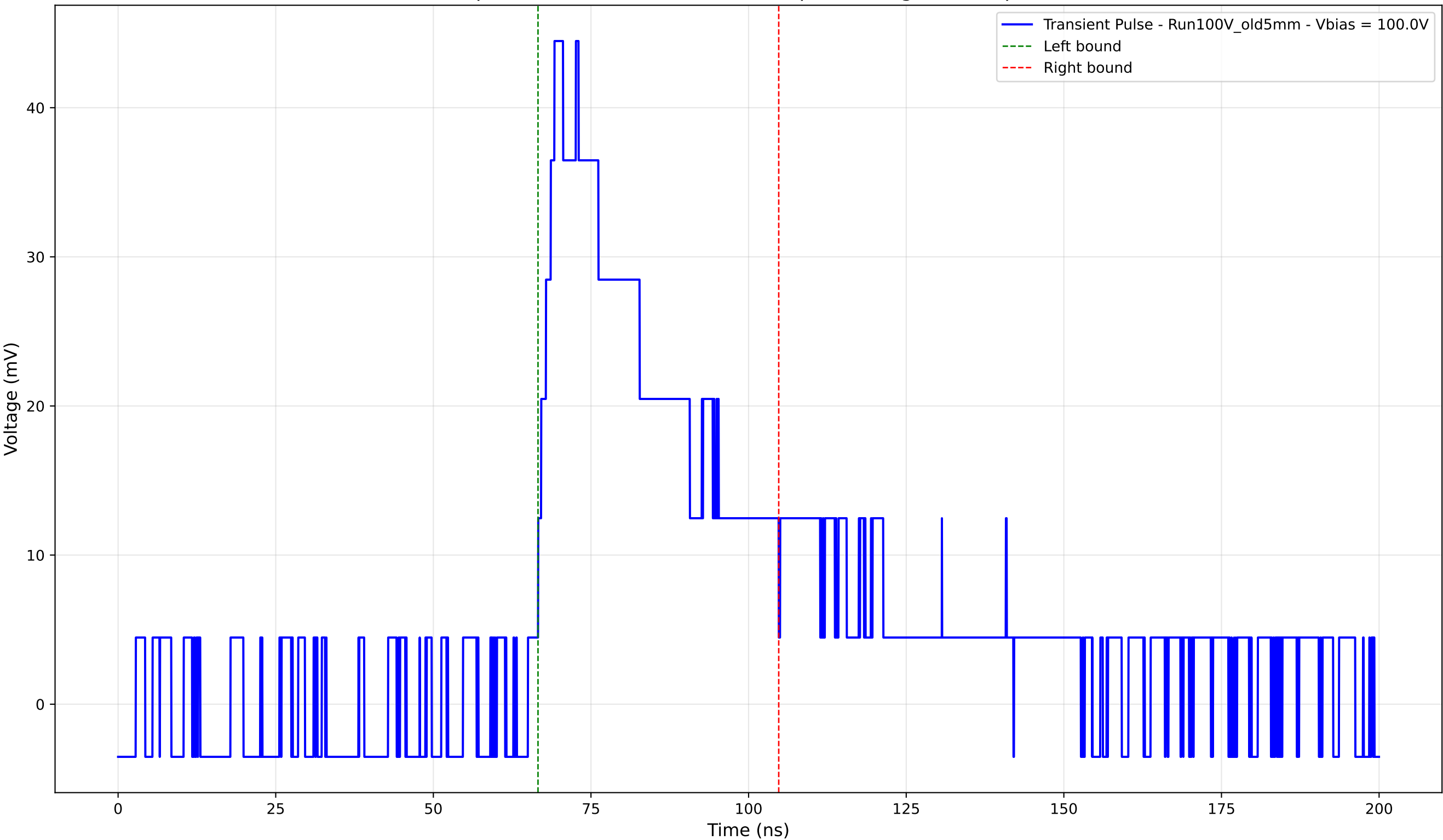
Transient Pulse - Sample: Old5mm - Position: 4905.0 \mu\text{m} - Charge: 17.48 pC - Rise Time: 4.20 ns
