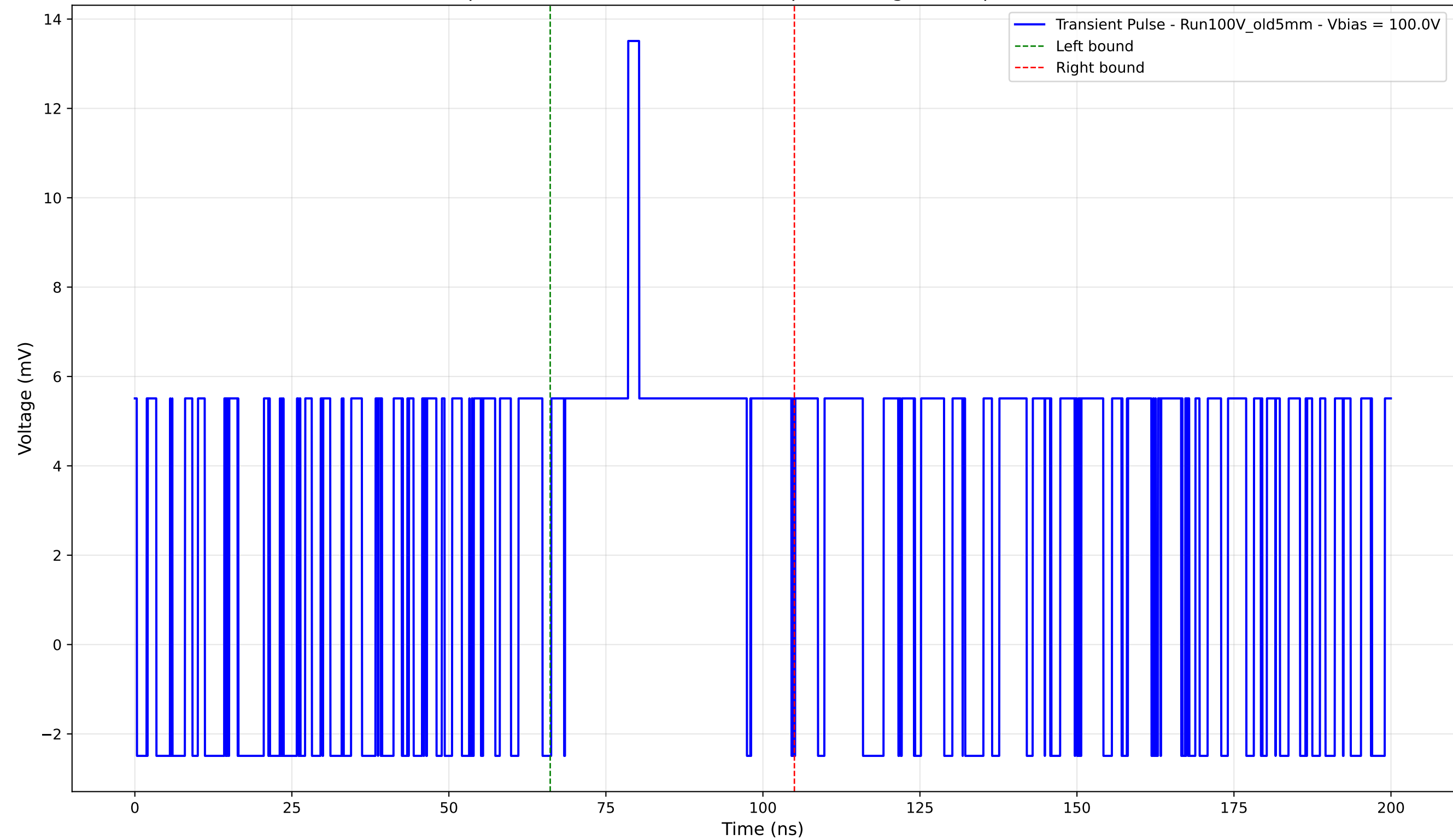
Transient Pulse - Sample: Old5mm - Position: 1280.0 \mu\text{m} - Charge: 4.35 pC - Rise Time: 0.00 ns (N/A)
