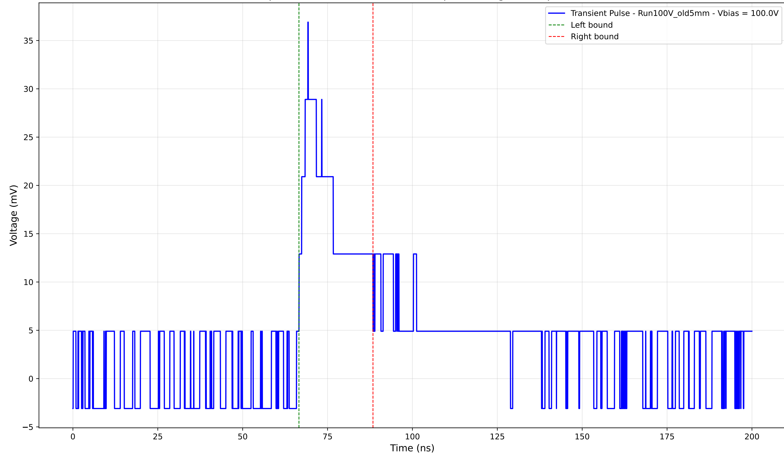
Transient Pulse - Sample: Old5mm - Position: 2715.0 \mu\text{m} - Charge: 7.67 pC - Rise Time: 3.35 ns
