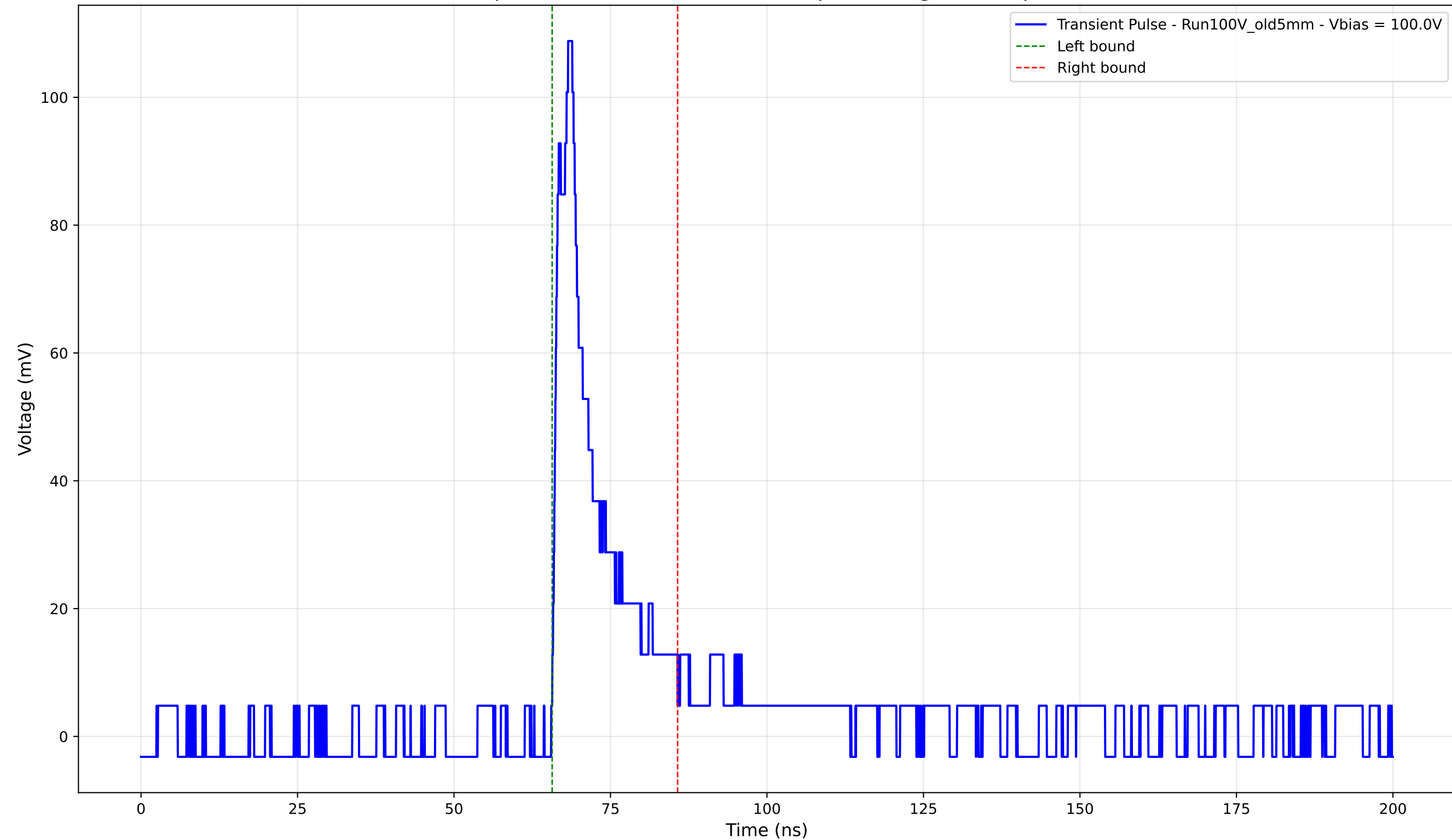
Transient Pulse - Sample: Old5mm - Position: 3305.0 \mu\text{m} - Charge: 14.99 pC - Rise Time: 2.28 ns
