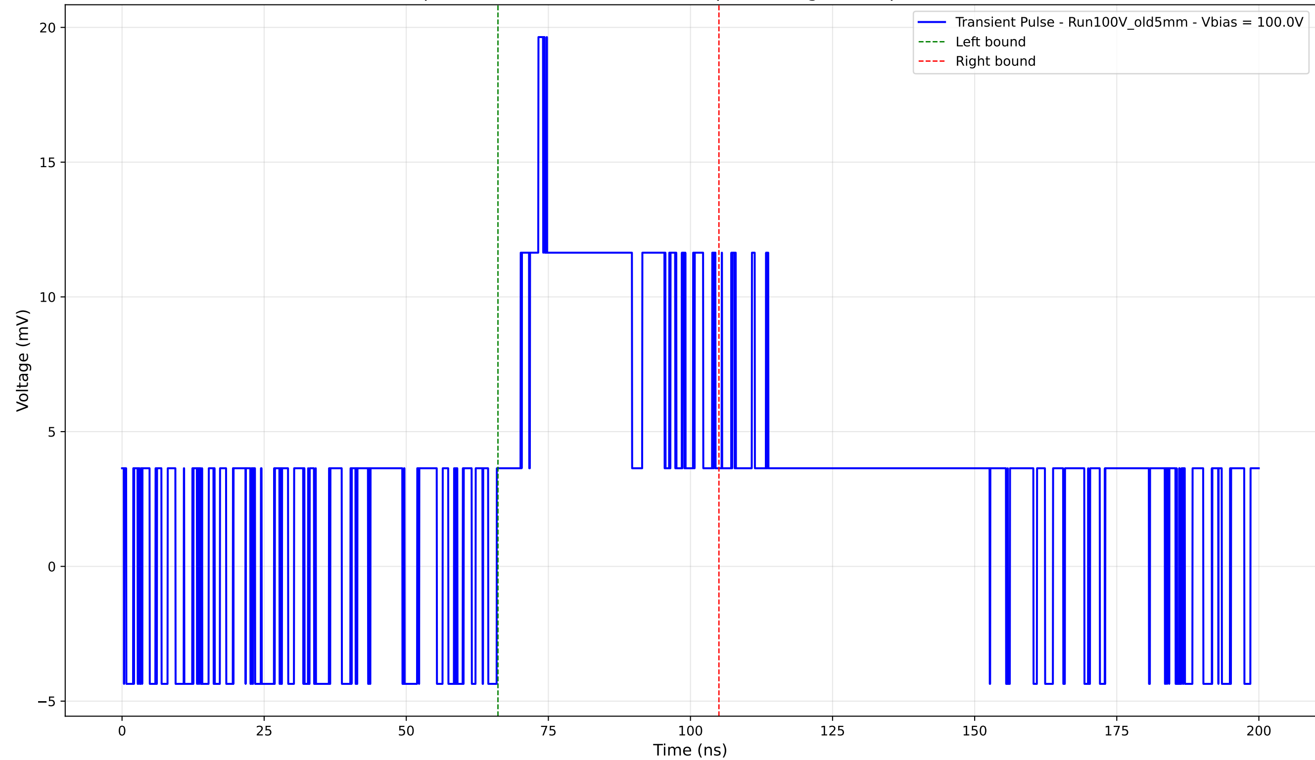
Transient Pulse - Sample: Old5mm - Position: 1970.0 \mu\text{m} - Charge: 7.32 pC - Rise Time: 0.00 ns (N/A)
