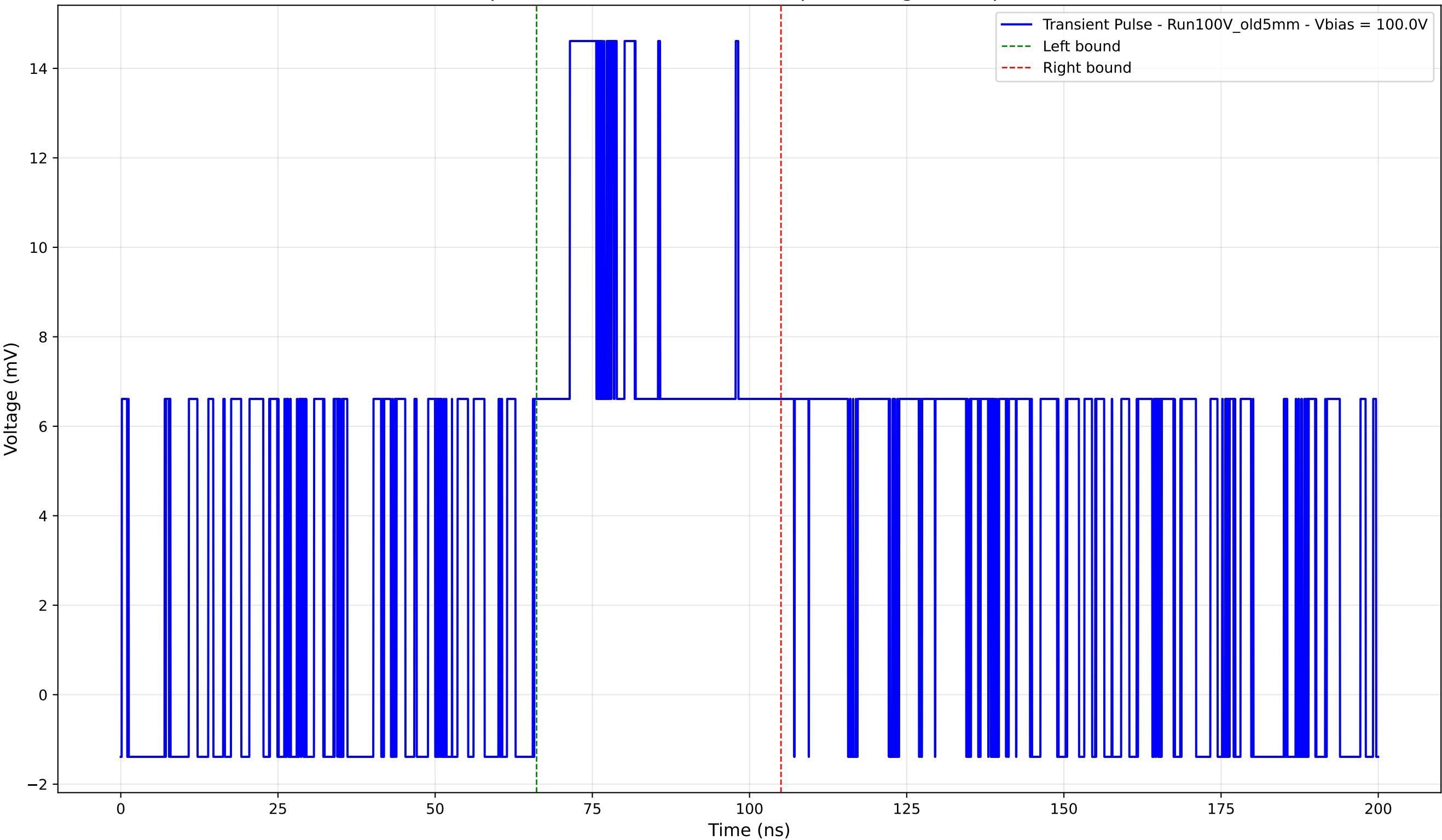
Transient Pulse - Sample: Old5mm - Position: 460.0 \mu\text{m} - Charge: 6.47 pC - Rise Time: 5.66 ns
