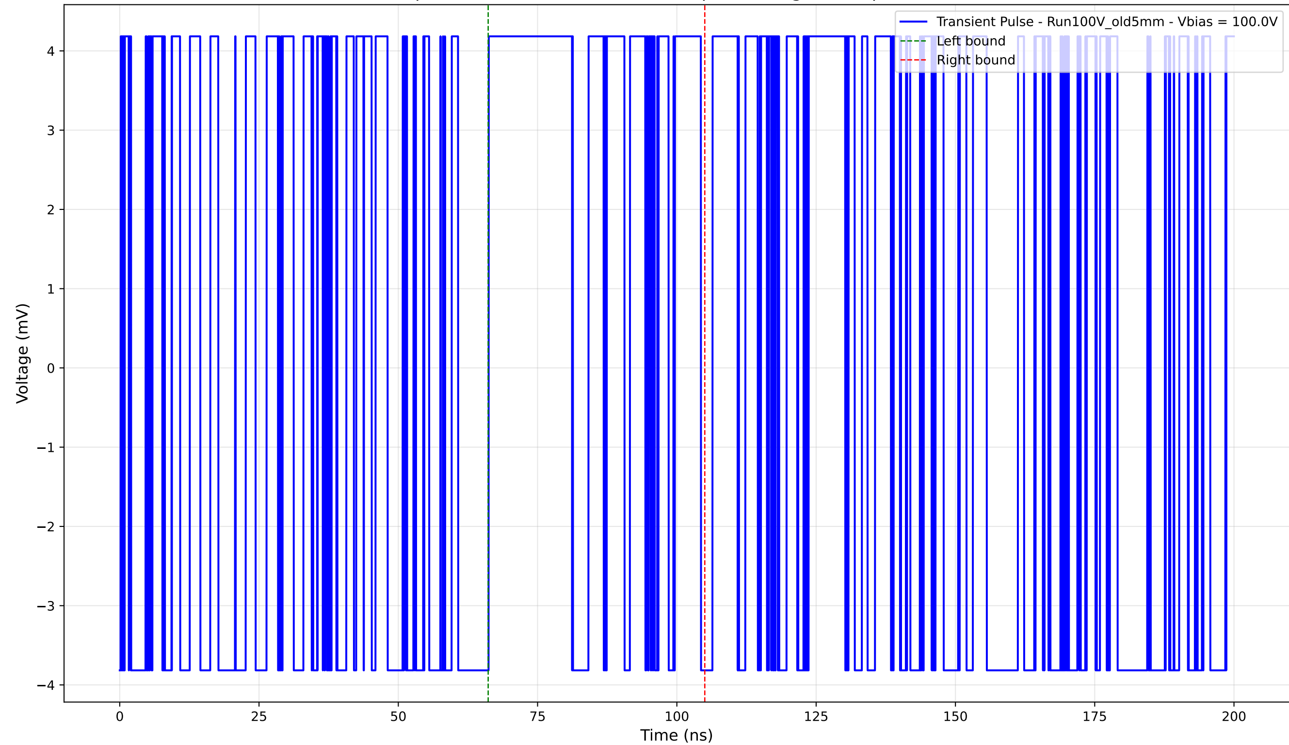
Transient Pulse - Sample: Old5mm - Position: 2825.0 \mu\text{m} - Charge: 2.12 pC - Rise Time: 0.00 ns (N/A)
