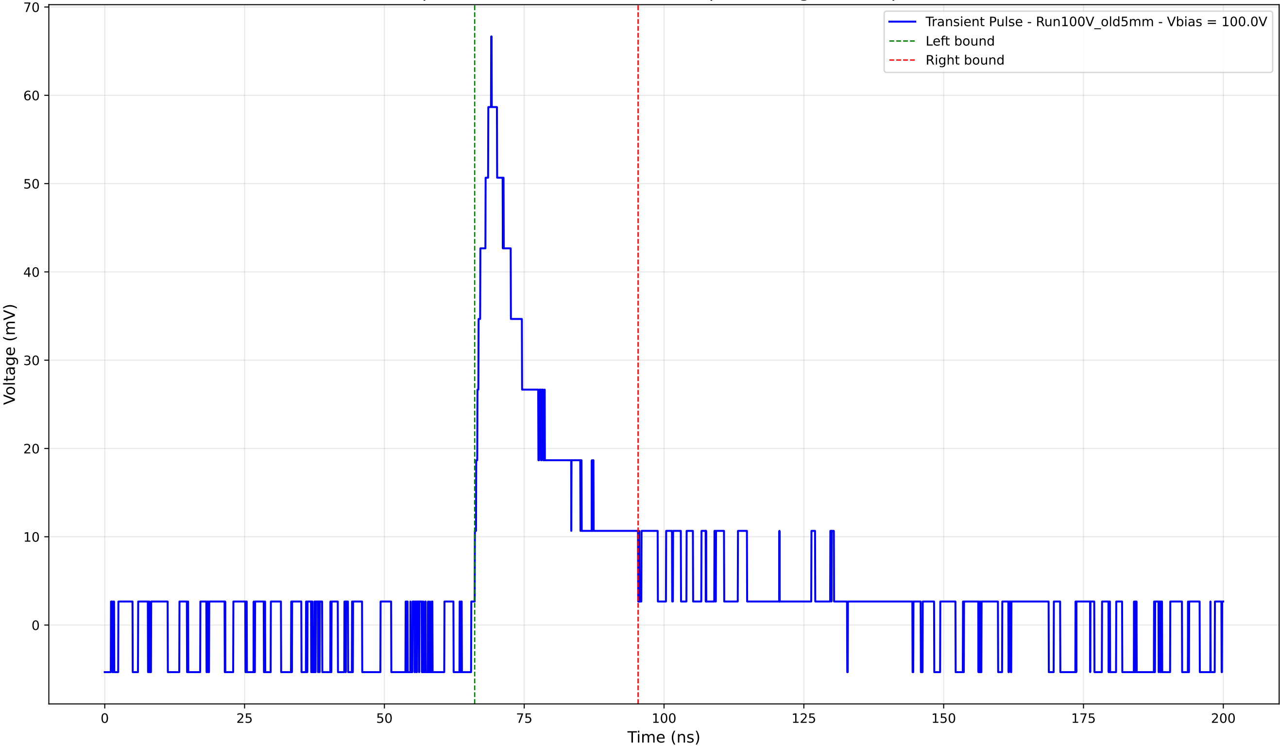
Transient Pulse - Sample: Old5mm - Position: 4500.0 \mu\text{m} - Charge: 14.00 pC - Rise Time: 2.93 ns
