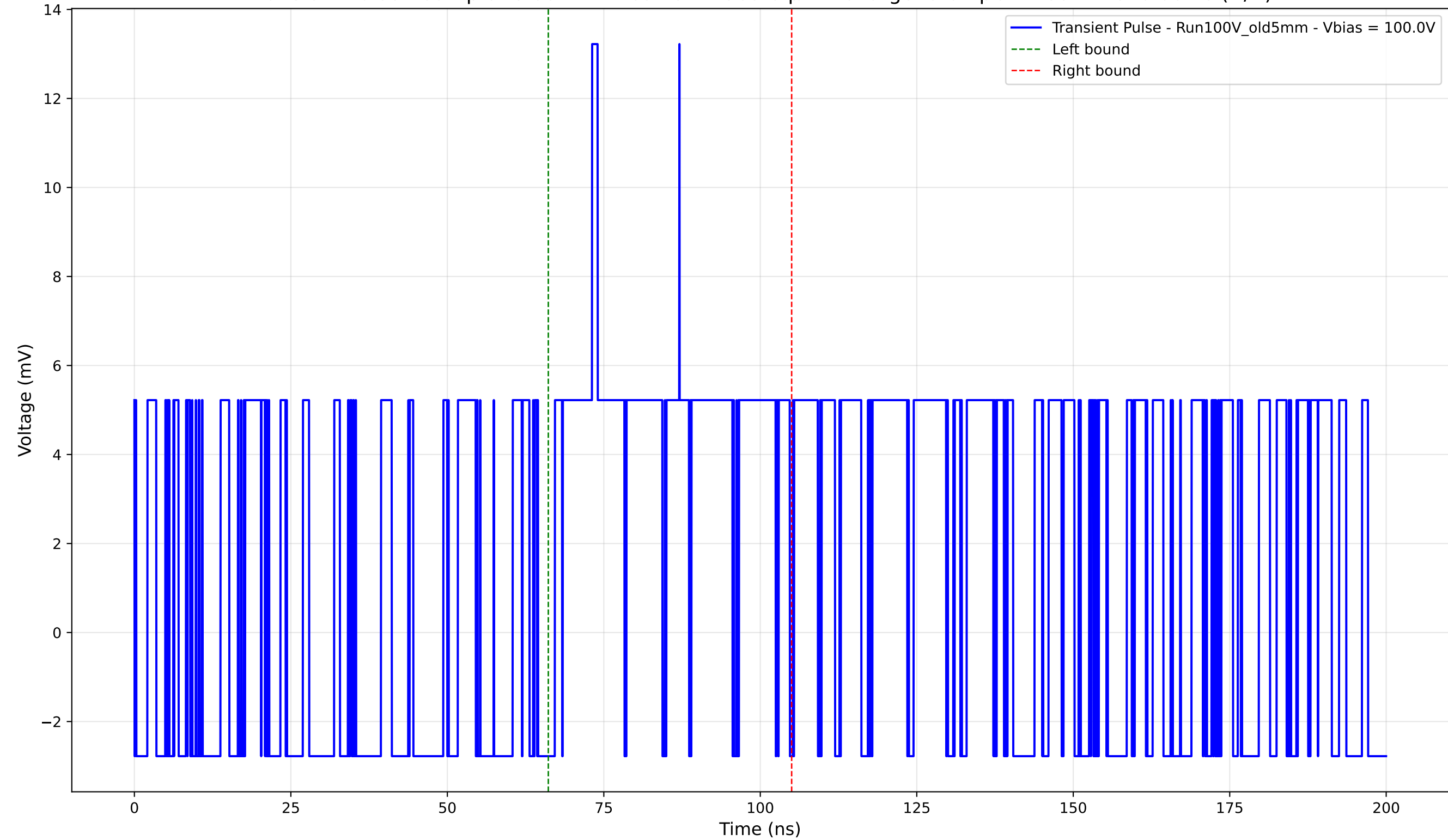
Transient Pulse - Sample: Old5mm - Position: 2305.0 \mu\text{m} - Charge: 3.64 pC - Rise Time: 0.00 ns (N/A)
