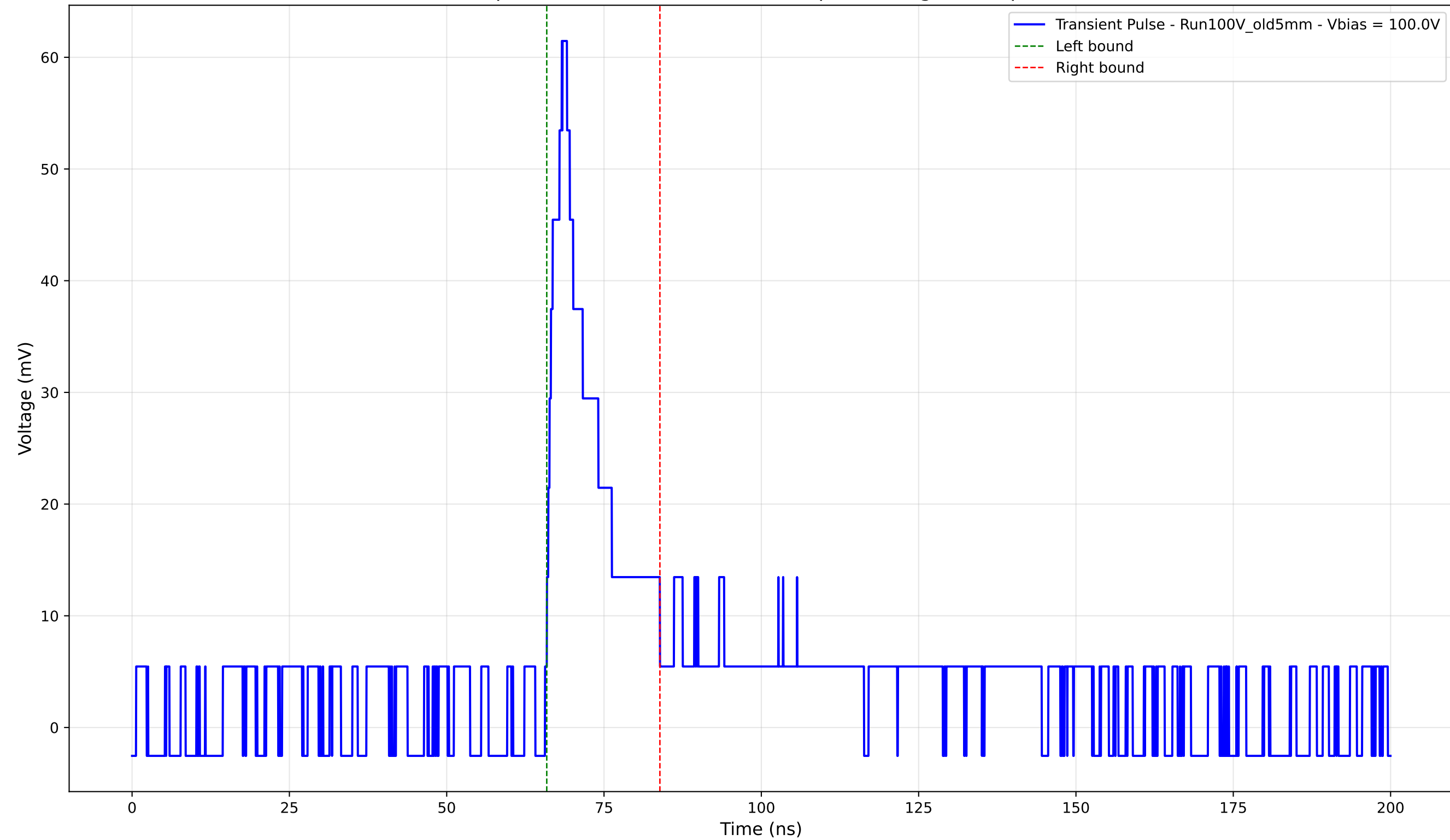
Transient Pulse - Sample: Old5mm - Position: 4230.0 \mu\text{m} - Charge: 9.41 pC - Rise Time: 2.38 ns
