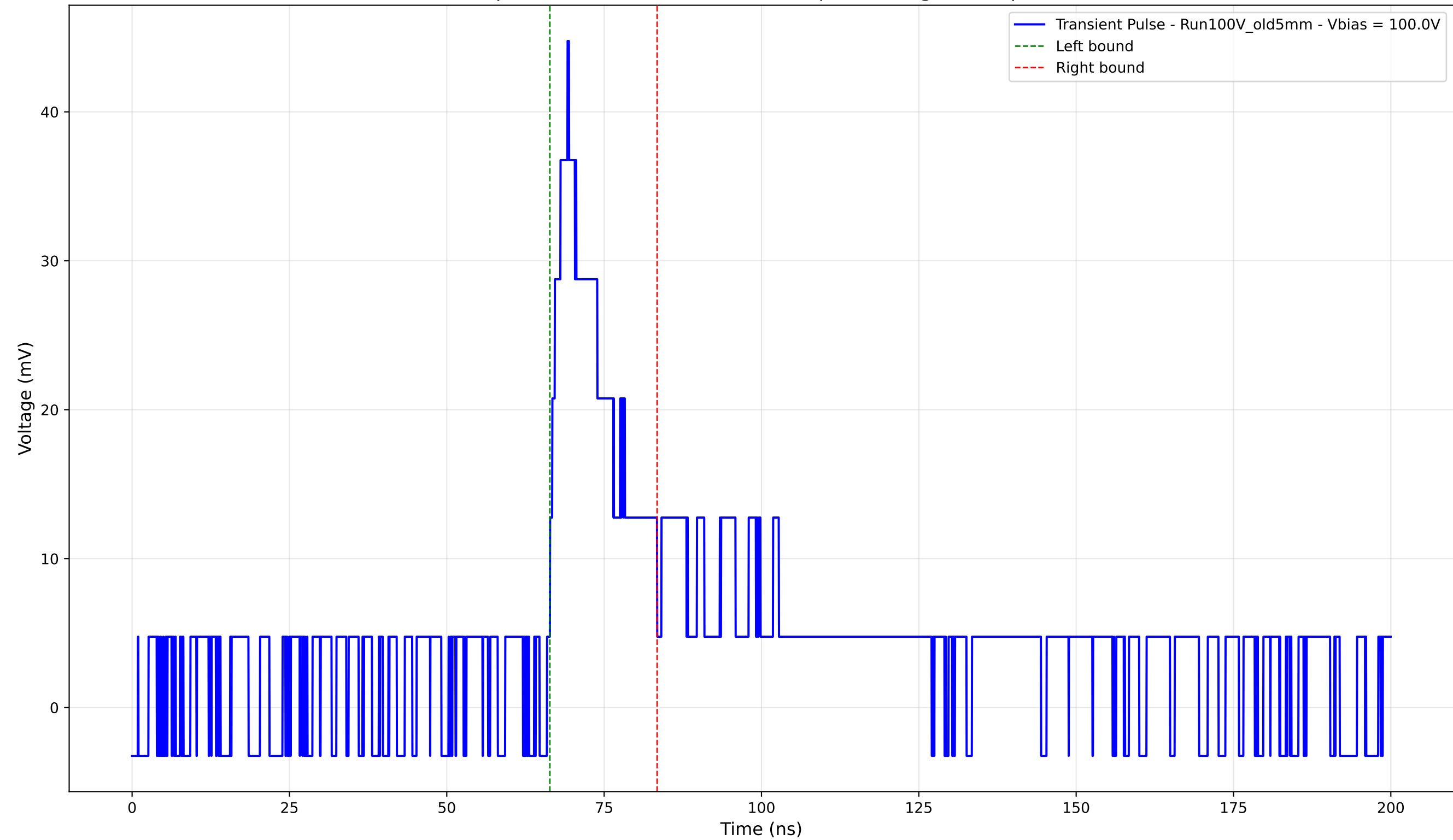
Transient Pulse - Sample: Old5mm - Position: 4540.0 \mu\text{m} - Charge: 7.52 pC - Rise Time: 3.26 ns
