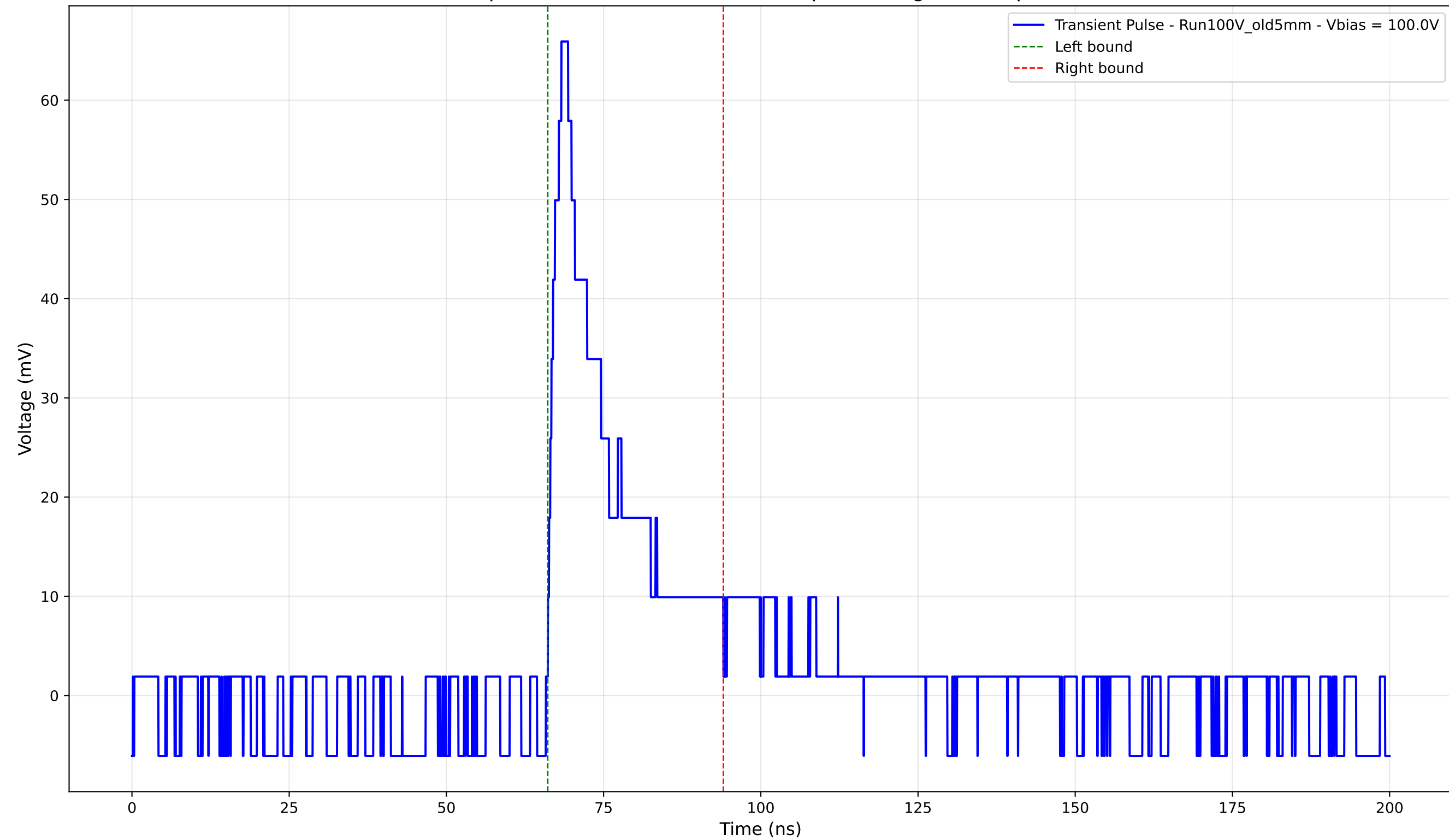
Transient Pulse - Sample: Old5mm - Position: 4420.0 \mu\text{m} - Charge: 12.89 pC - Rise Time: 2.15 ns
