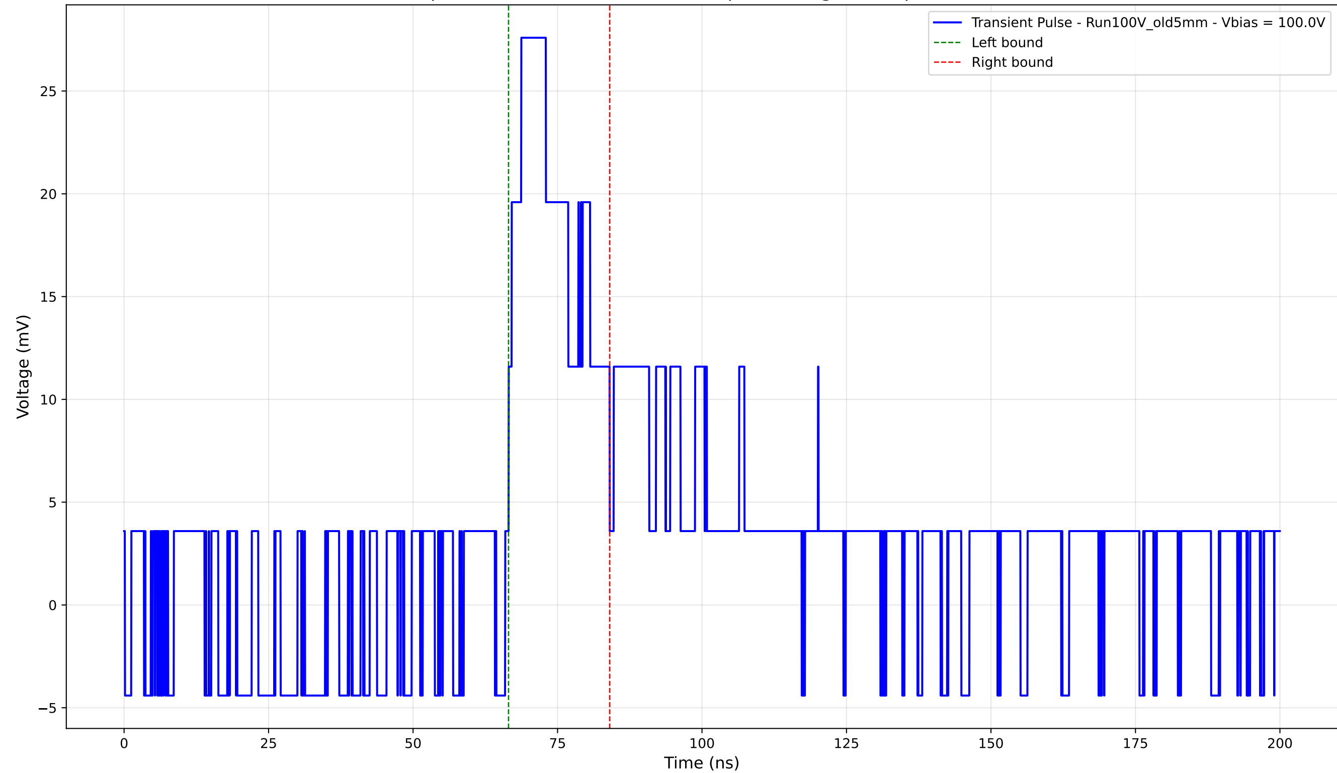
Transient Pulse - Sample: Old5mm - Position: 2720.0 \mu\text{m} - Charge: 6.55 pC - Rise Time: 0.00 ns (N/A)
