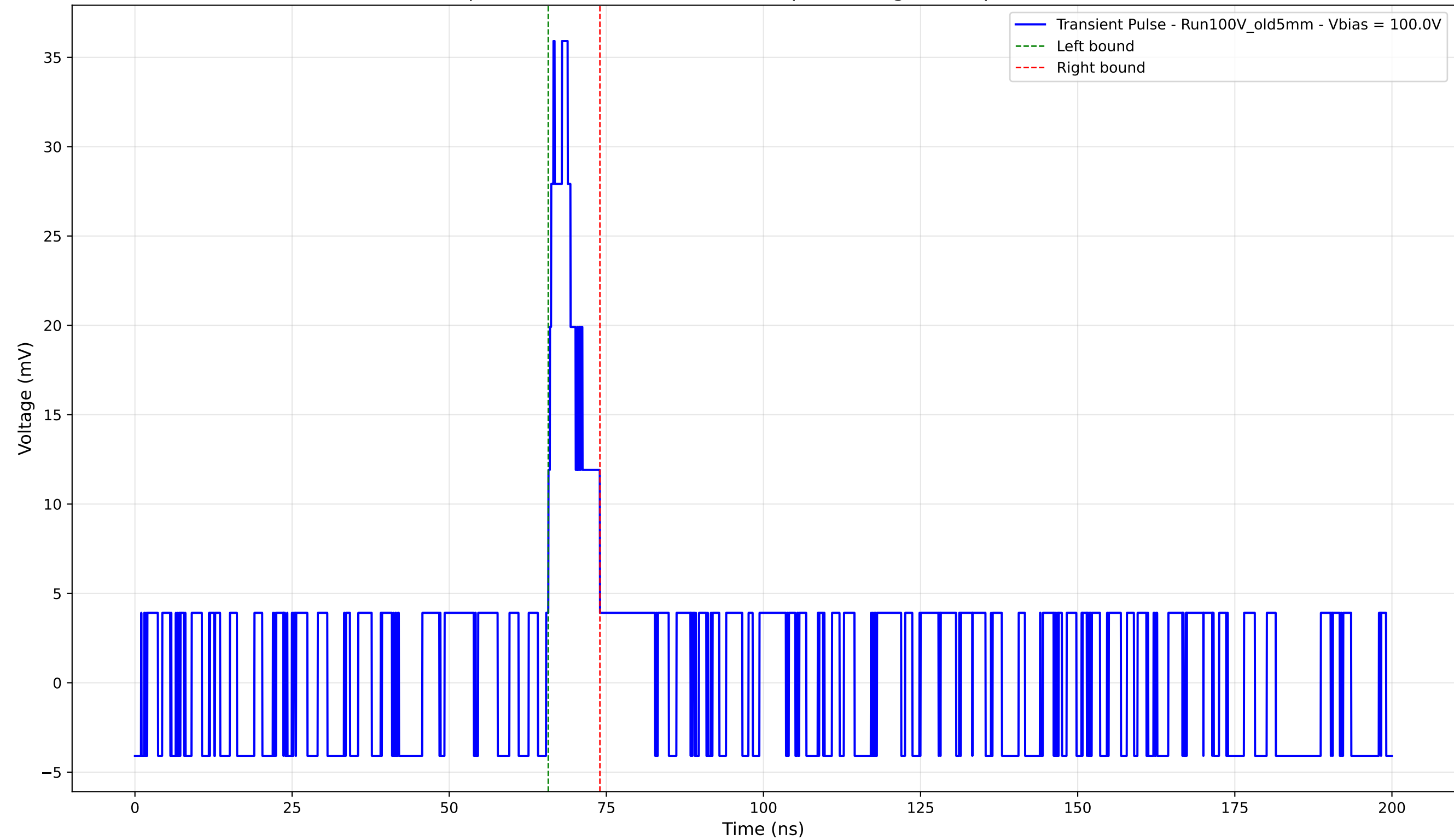
Transient Pulse - Sample: Old5mm - Position: 3965.0 \mu\text{m} - Charge: 3.35 pC - Rise Time: 0.00 ns (N/A)
