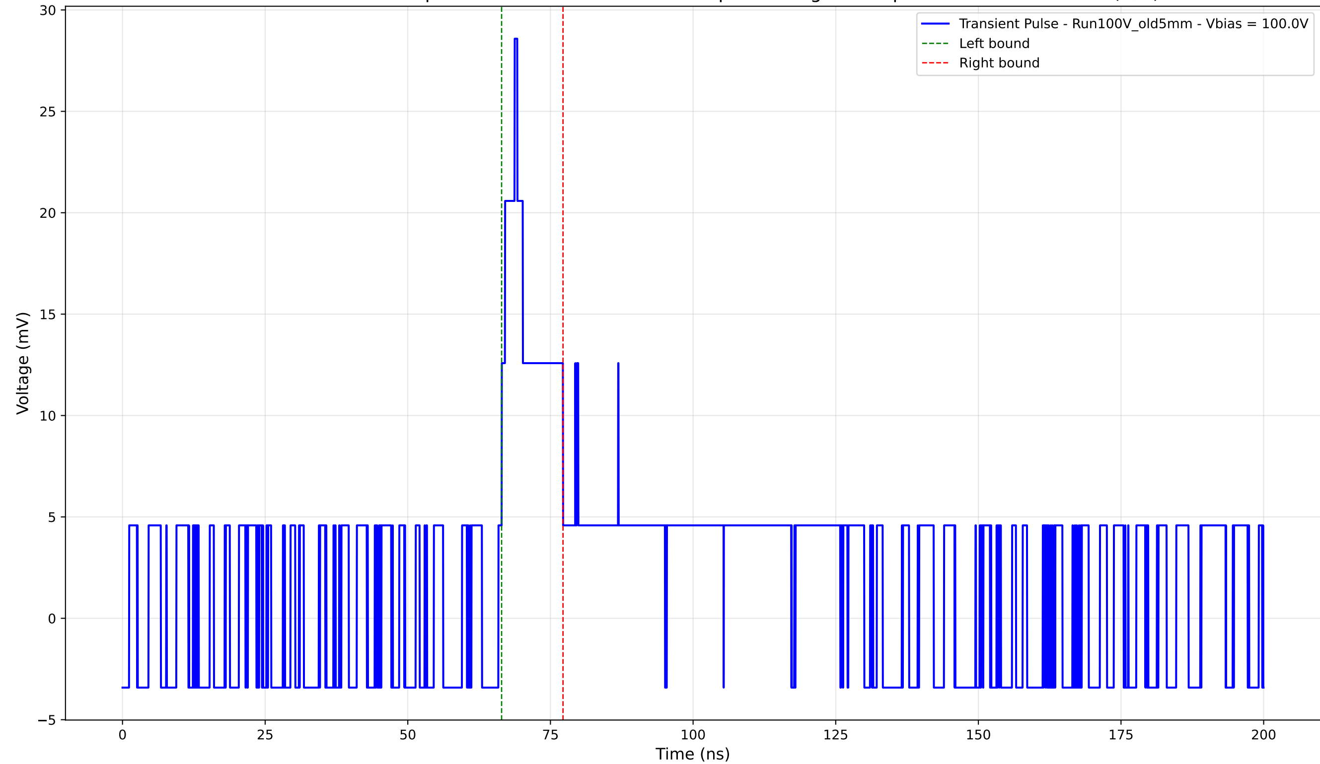
Transient Pulse - Sample: Old5mm - Position: 4365.0 \mu\text{m} - Charge: 3.28 pC - Rise Time: 0.00 ns (N/A)
