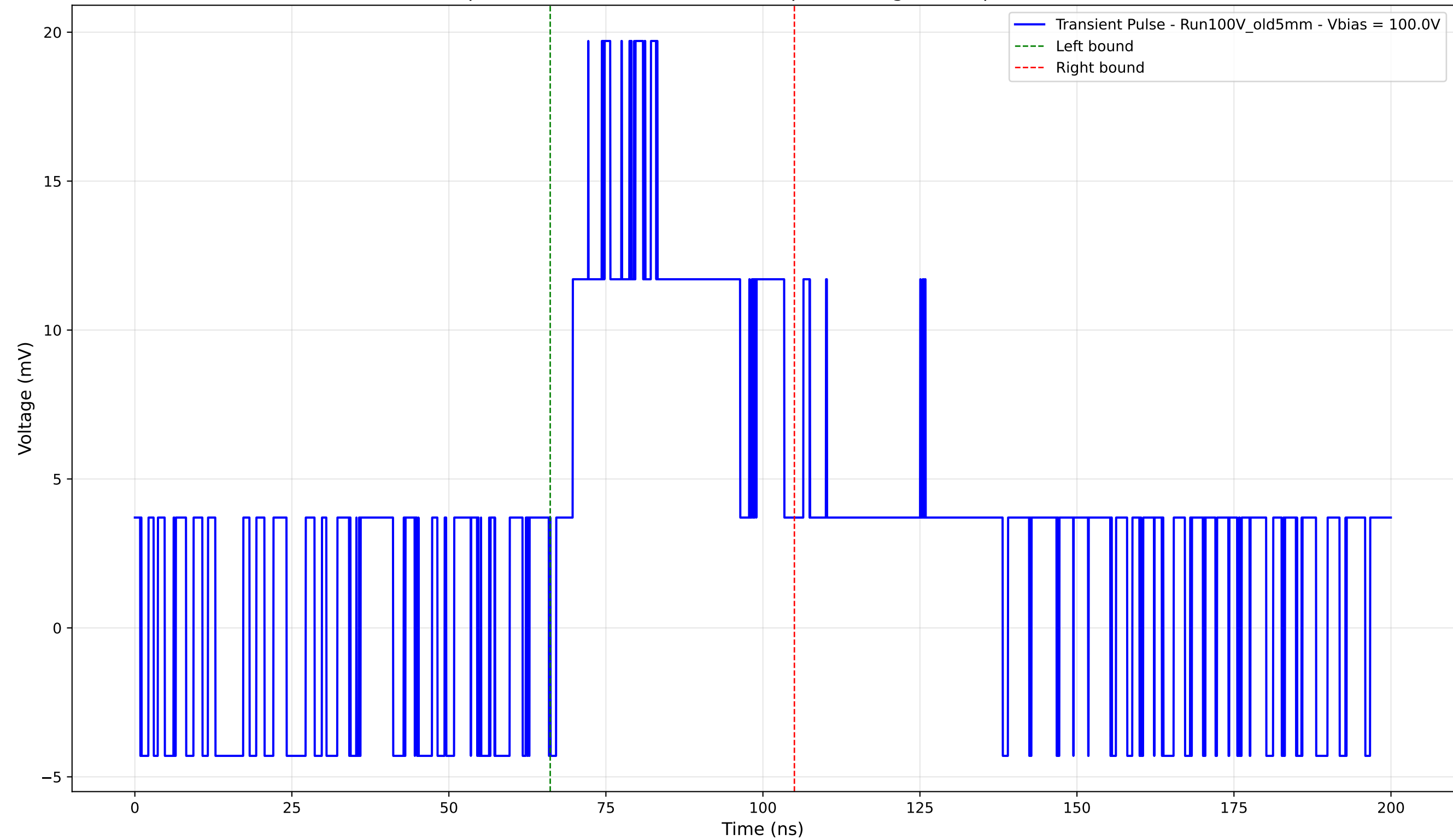
Transient Pulse - Sample: Old5mm - Position: 1210.0 \mu\text{m} - Charge: 8.45 pC - Rise Time: 0.00 ns (N/A)
