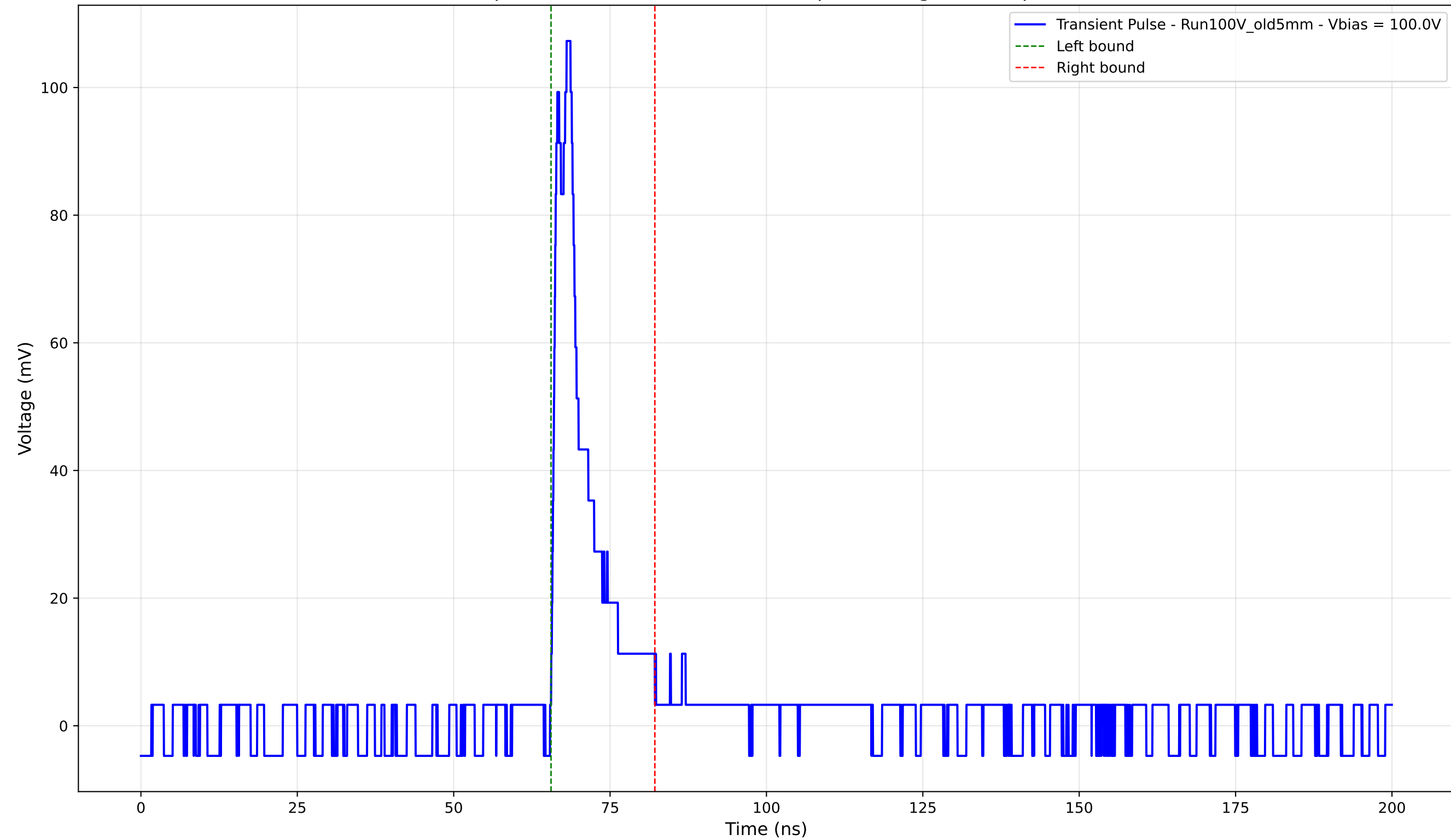
Transient Pulse - Sample: Old5mm - Position: 3930.0 \mu\text{m} - Charge: 12.04 pC - Rise Time: 0.98 ns
