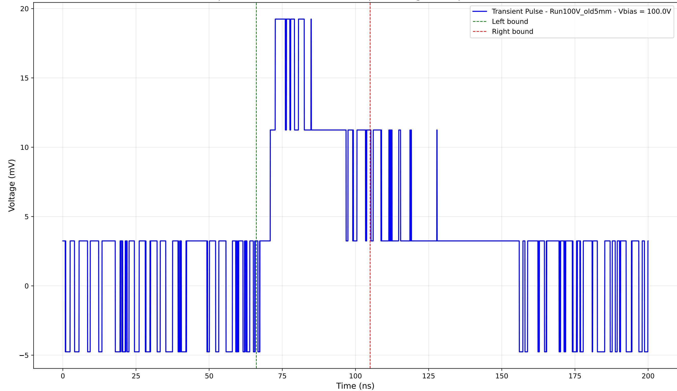
Transient Pulse - Sample: Old5mm - Position: 1620.0 \mu\text{m} - Charge: 8.85 pC - Rise Time: 0.00 ns (N/A)
