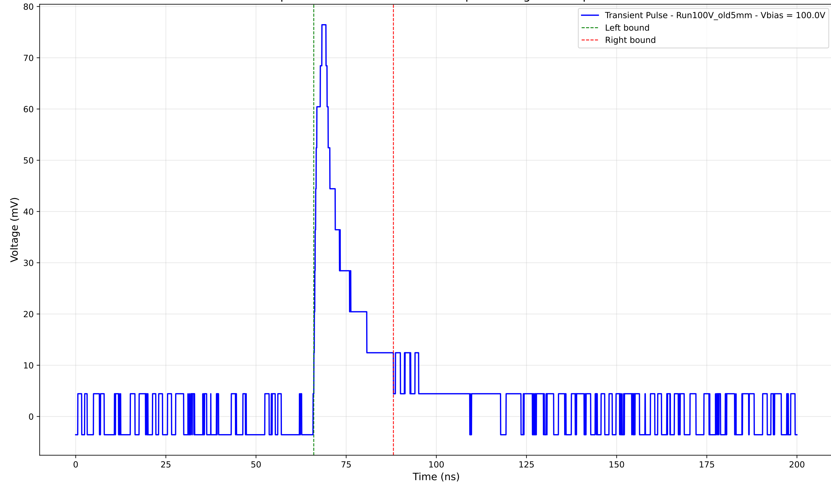
Transient Pulse - Sample: Old5mm - Position: 4215.0 \mu\text{m} - Charge: 12.93 pC - Rise Time: 2.23 ns
