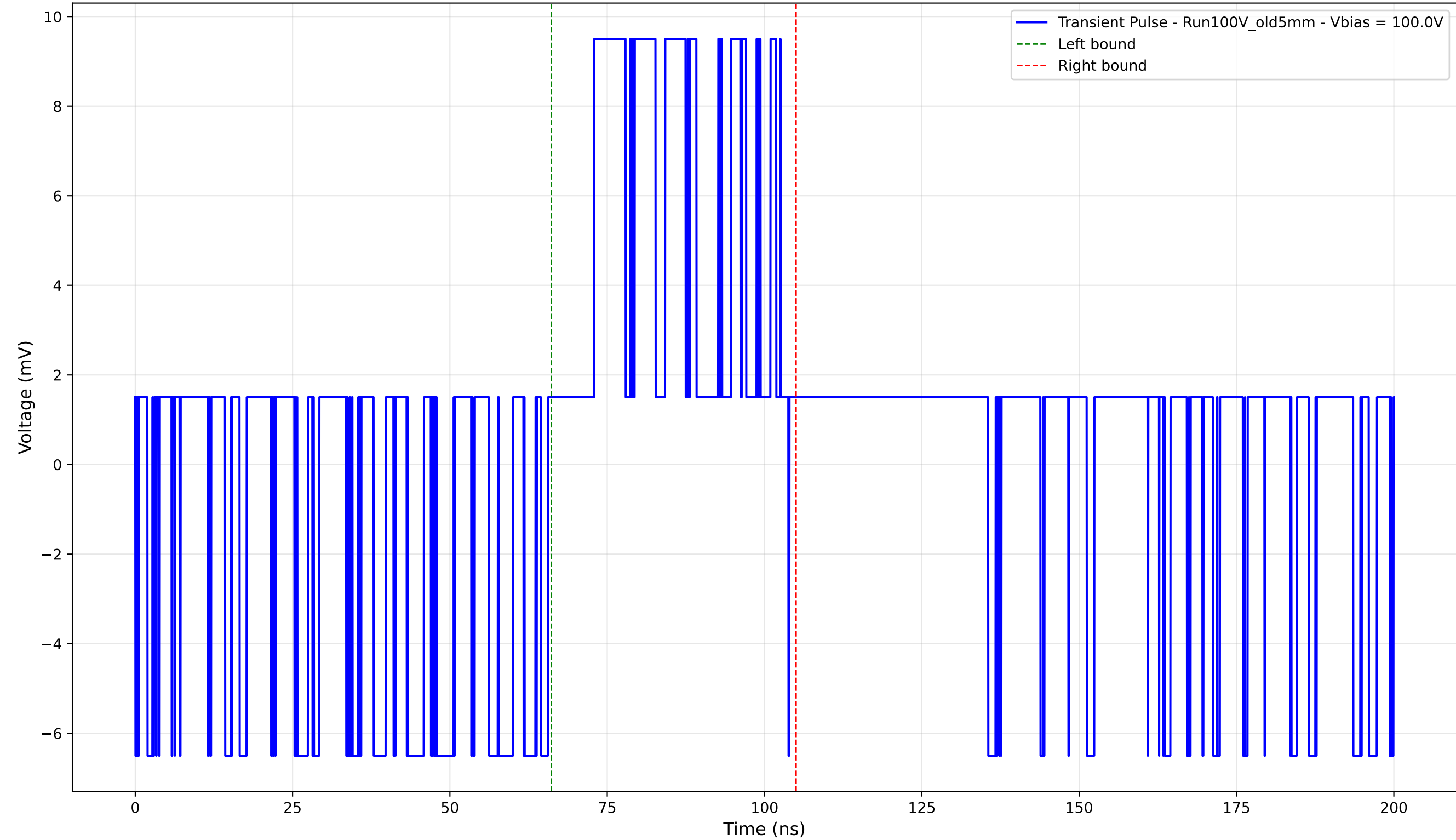
Transient Pulse - Sample: Old5mm - Position: 1100.0 \mu\text{m} - Charge: 3.92 pC - Rise Time: 0.00 ns (N/A)
