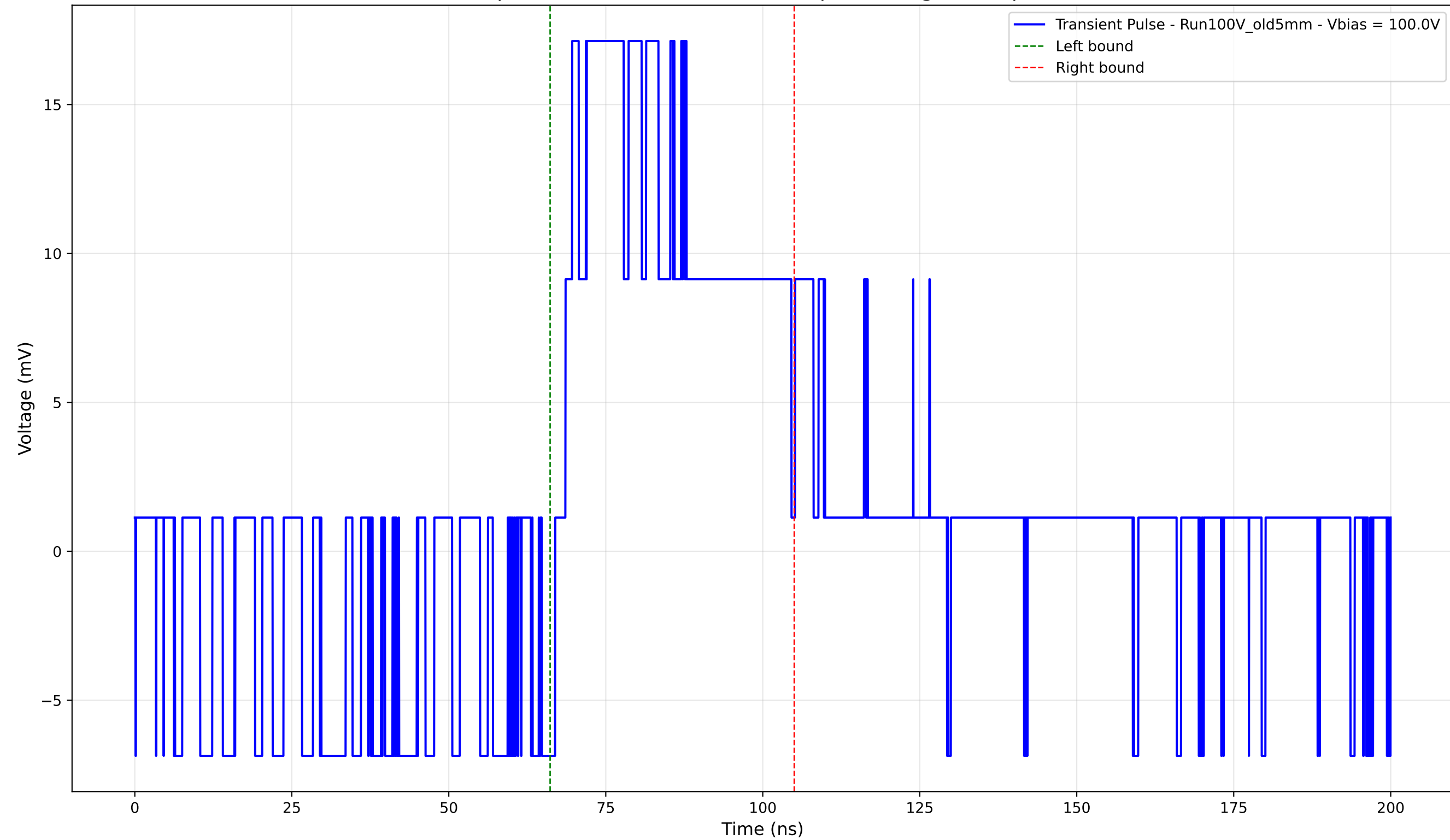
Transient Pulse - Sample: Old5mm - Position: 2185.0 \mu\text{m} - Charge: 8.48 pC - Rise Time: 1.08 ns
