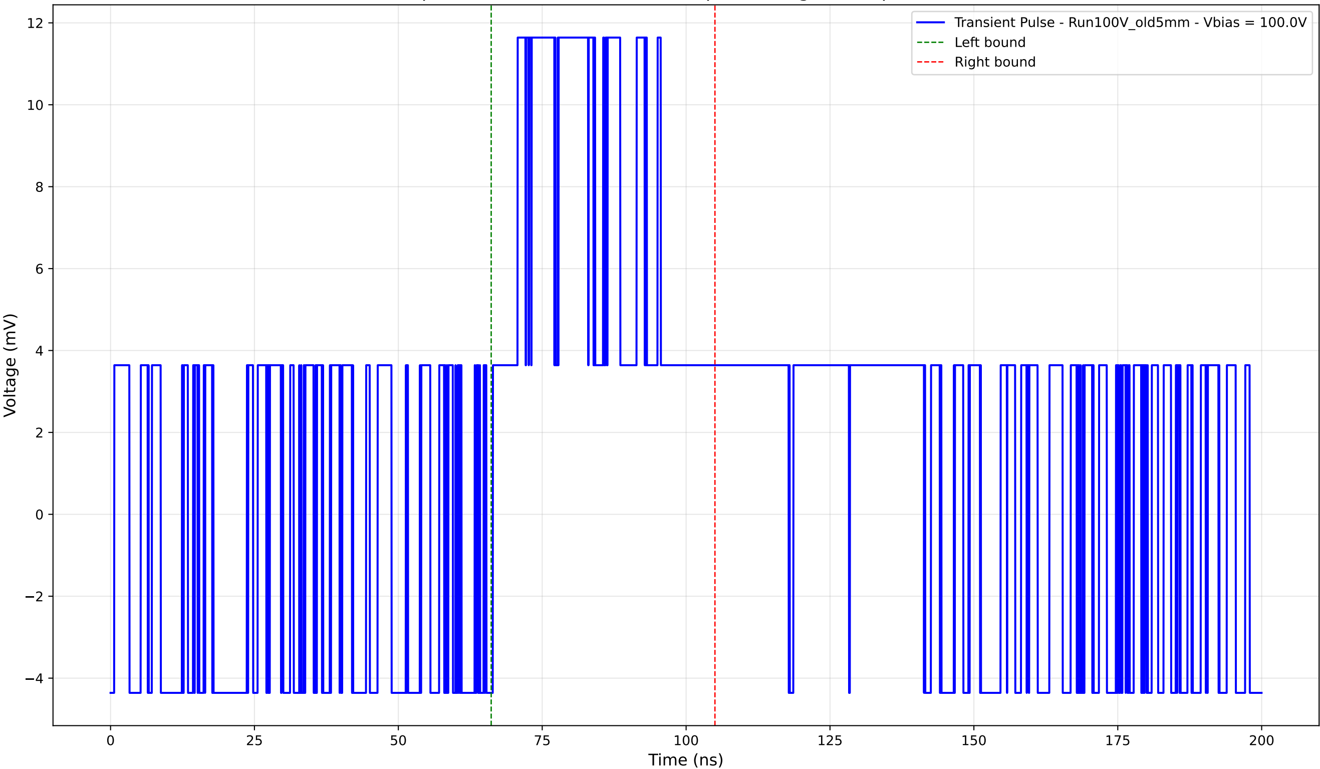
Transient Pulse - Sample: Old5mm - Position: 680.0 \mu\text{m} - Charge: 5.54 pC - Rise Time: 0.00 ns (N/A)
