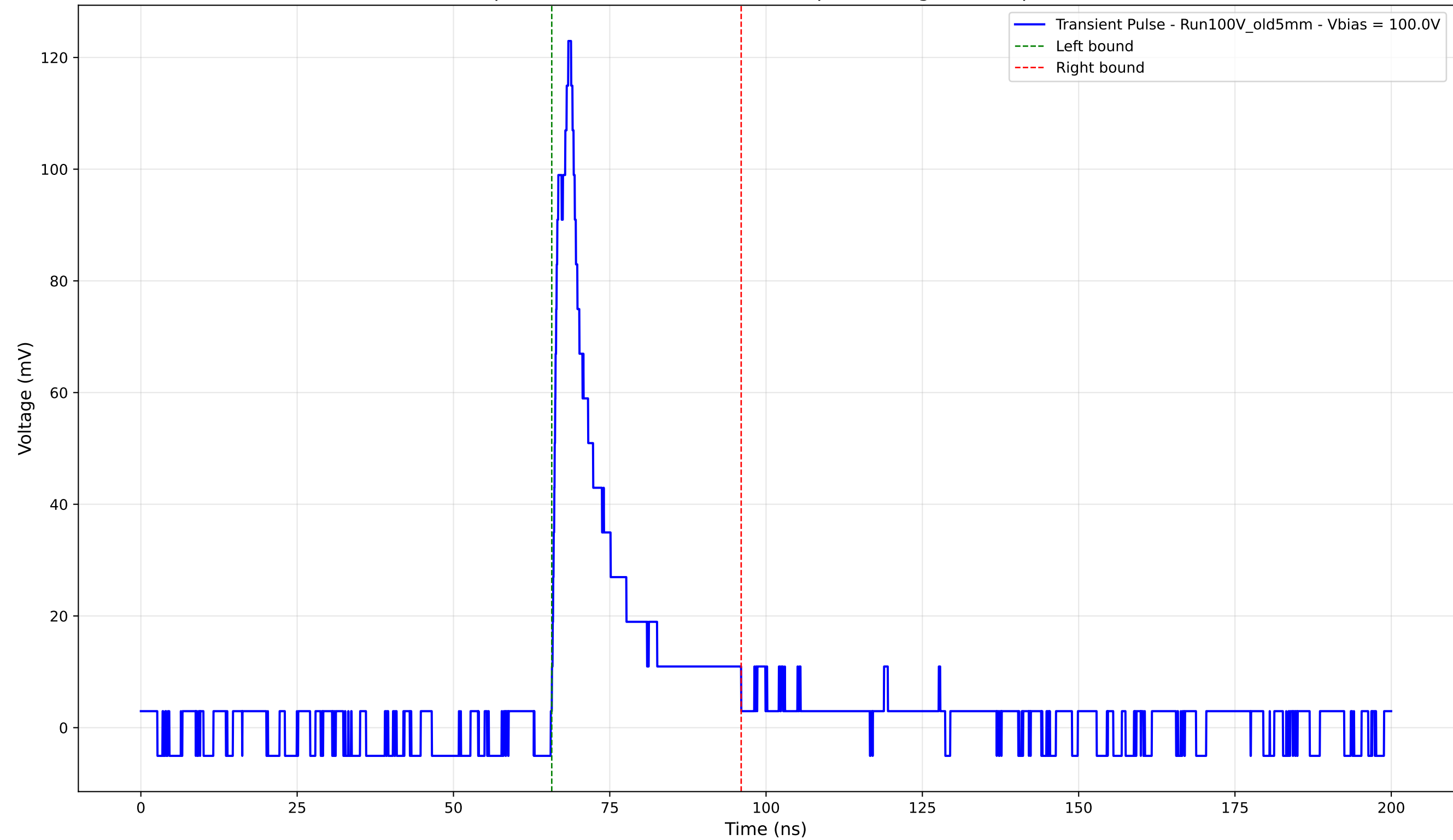
Transient Pulse - Sample: Old5mm - Position: 3265.0 \mu\text{m} - Charge: 18.80 pC - Rise Time: 2.26 ns
