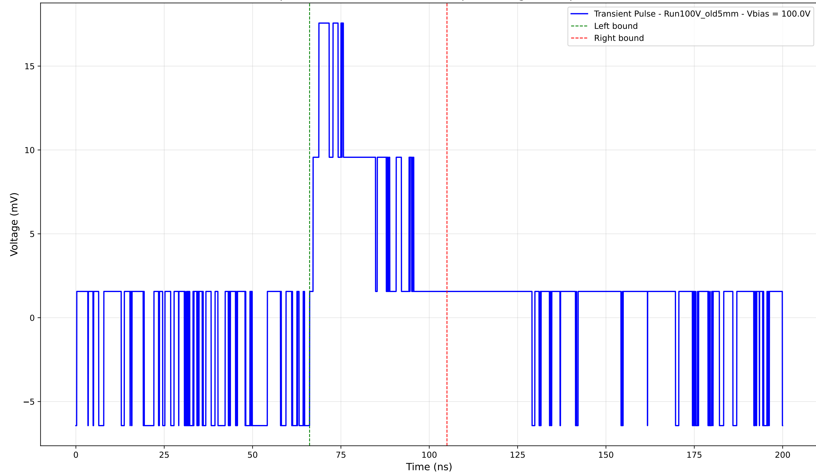
Transient Pulse - Sample: Old5mm - Position: 2565.0 \mu\text{m} - Charge: 5.67 pC - Rise Time: 1.66 ns
