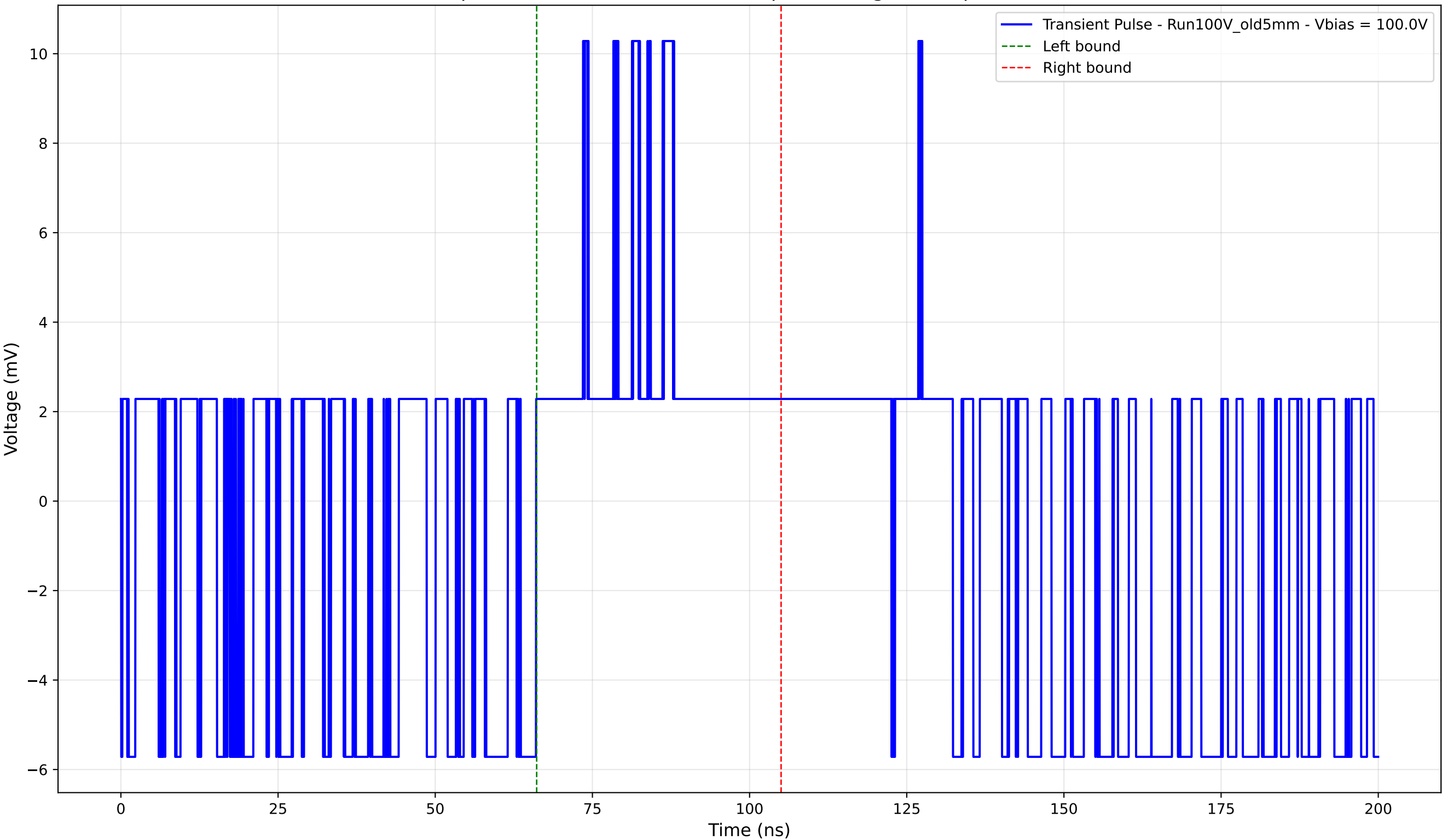
Transient Pulse - Sample: Old5mm - Position: 810.0 \mu\text{m} - Charge: 2.49 pC - Rise Time: 0.00 ns (N/A)
