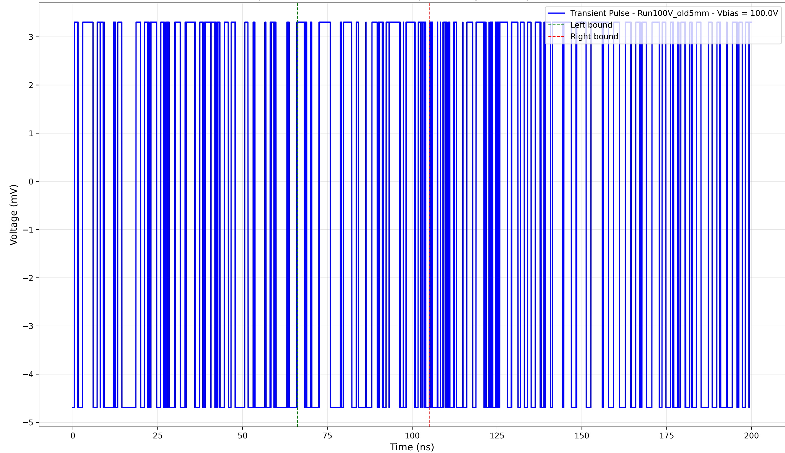
Transient Pulse - Sample: Old5mm - Position: 60.0 \mu\text{m} - Charge: -0.31 pC - Rise Time: 0.00 ns (N/A)
