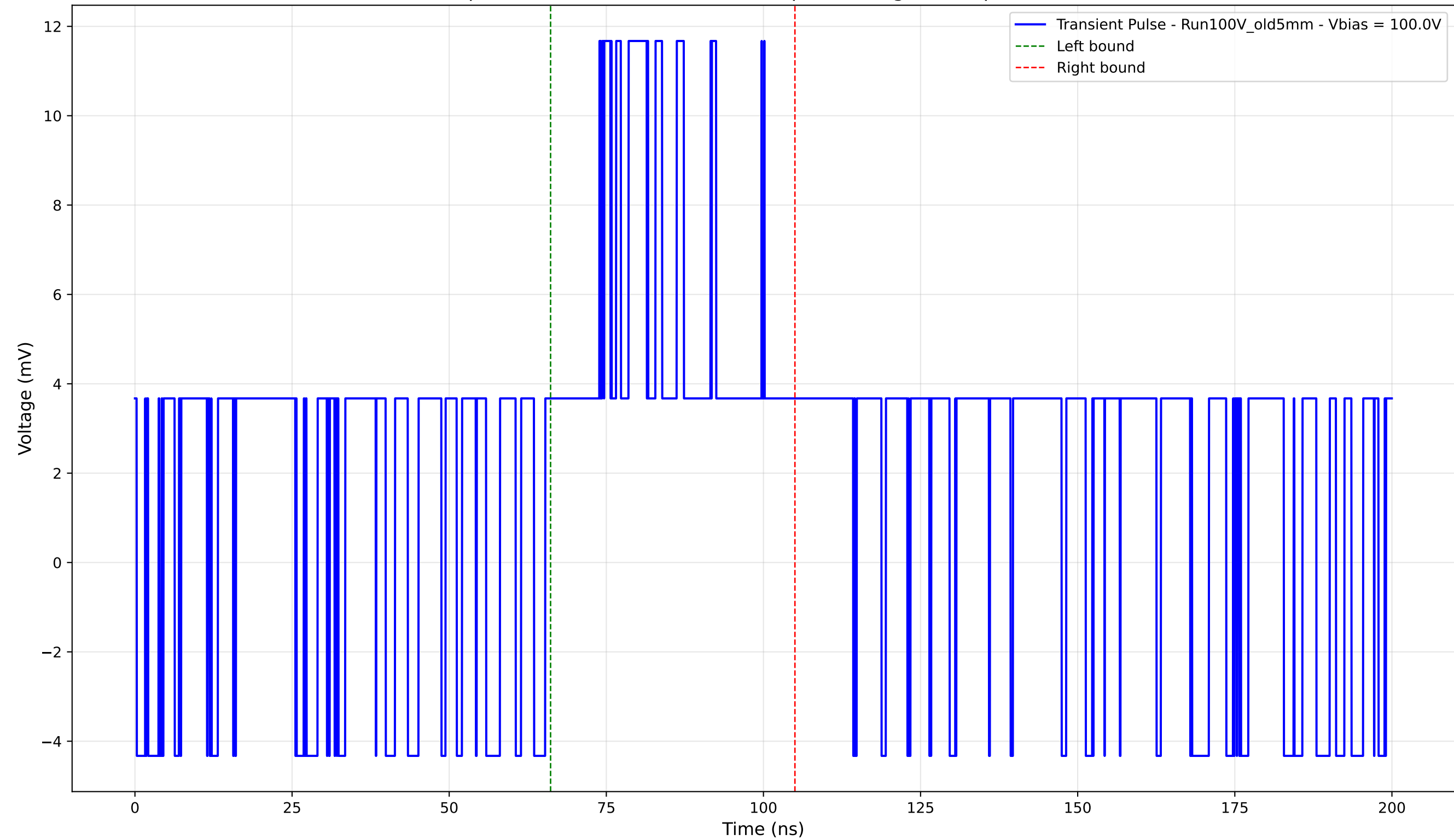
Transient Pulse - Sample: Old5mm - Position: 1555.0 \mu\text{m} - Charge: 4.19 pC - Rise Time: 0.00 ns (N/A)
