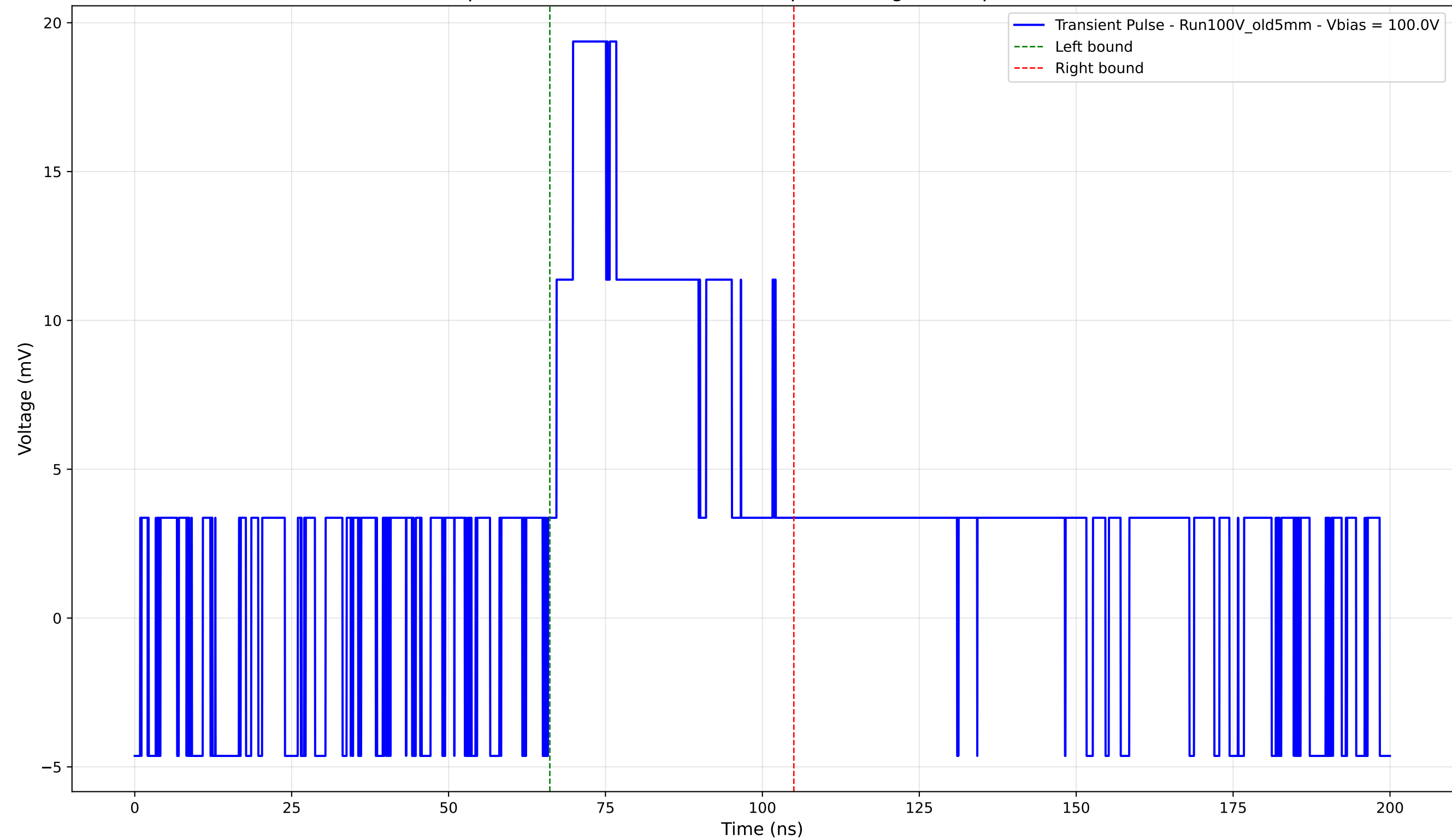
Transient Pulse - Sample: Old5mm - Position: 2470.0 \mu\text{m} - Charge: 8.02 pC - Rise Time: 0.00 ns (N/A)
