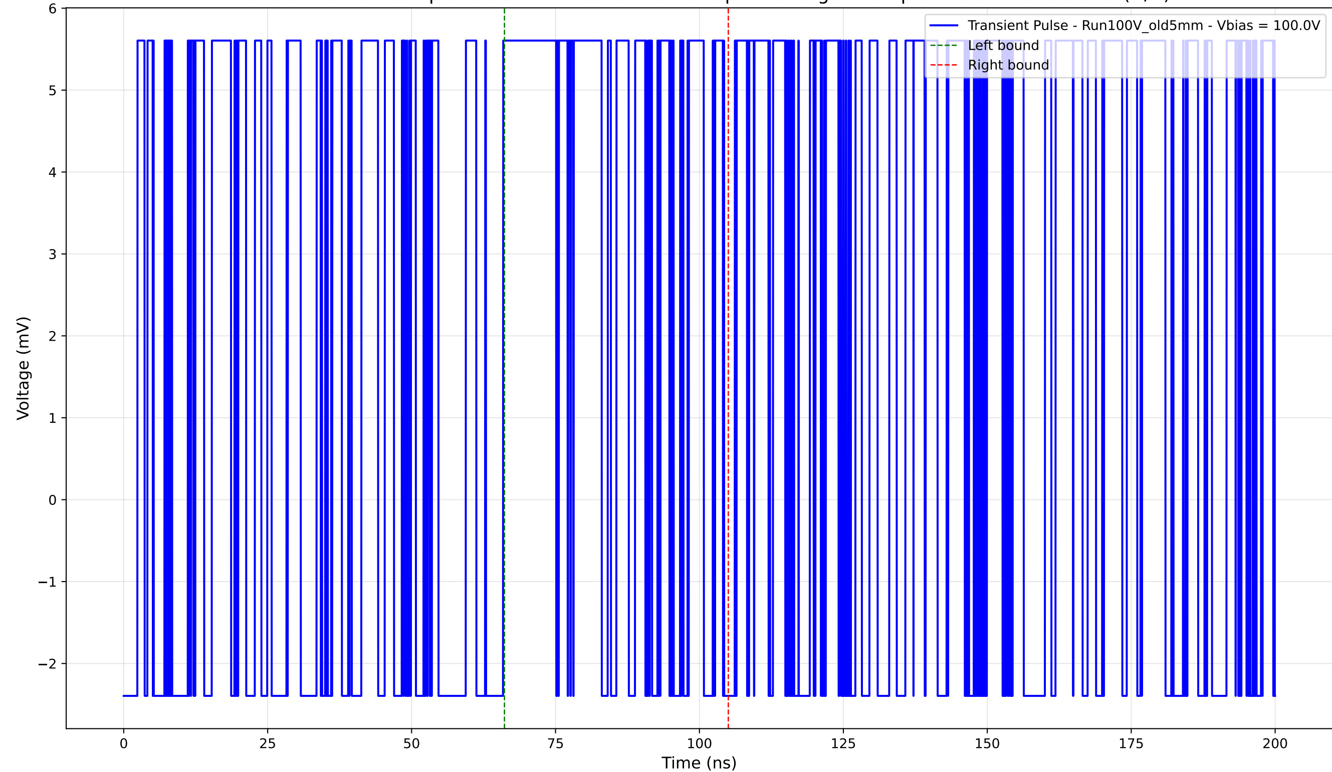
Transient Pulse - Sample: Old5mm - Position: 3110.0 \mu\text{m} - Charge: 2.67 pC - Rise Time: 0.00 ns (N/A)
