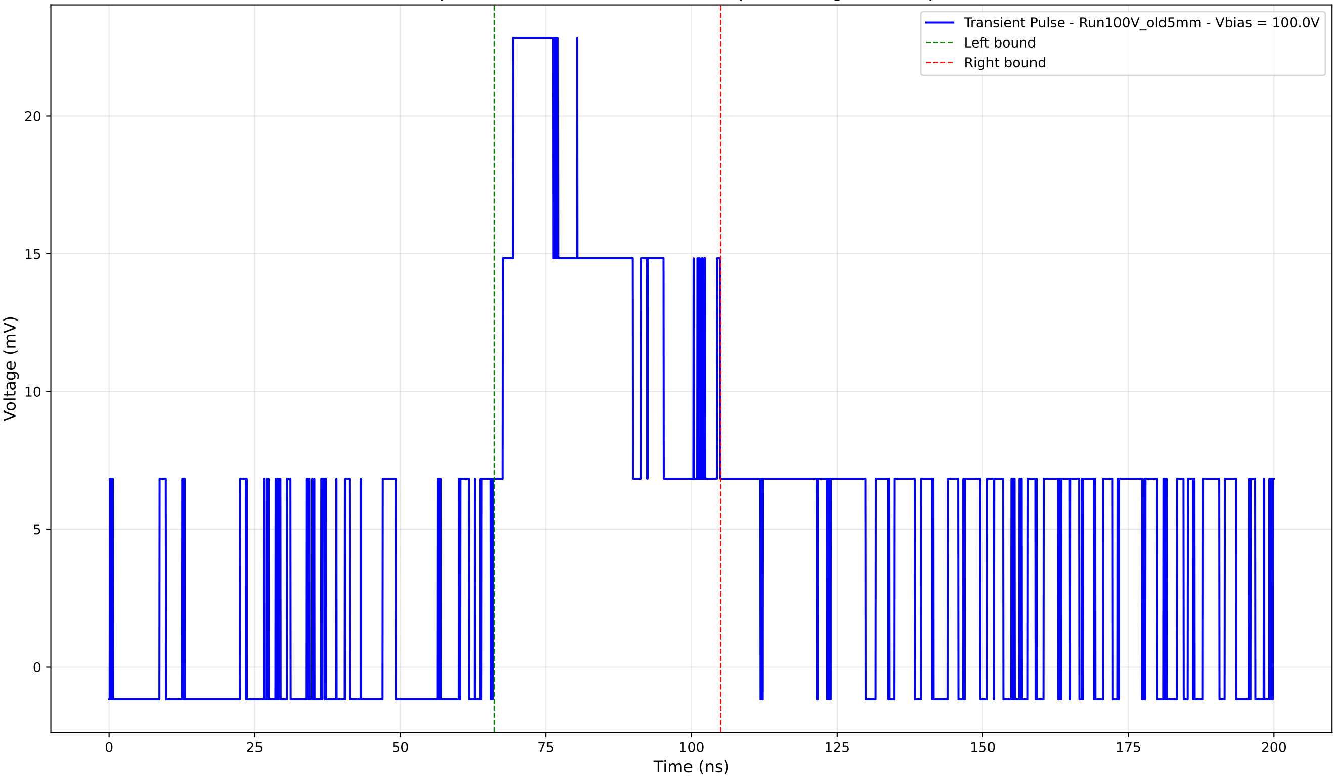
Transient Pulse - Sample: Old5mm - Position: 2465.0 \mu\text{m} - Charge: 10.86 pC - Rise Time: 3.52 ns
