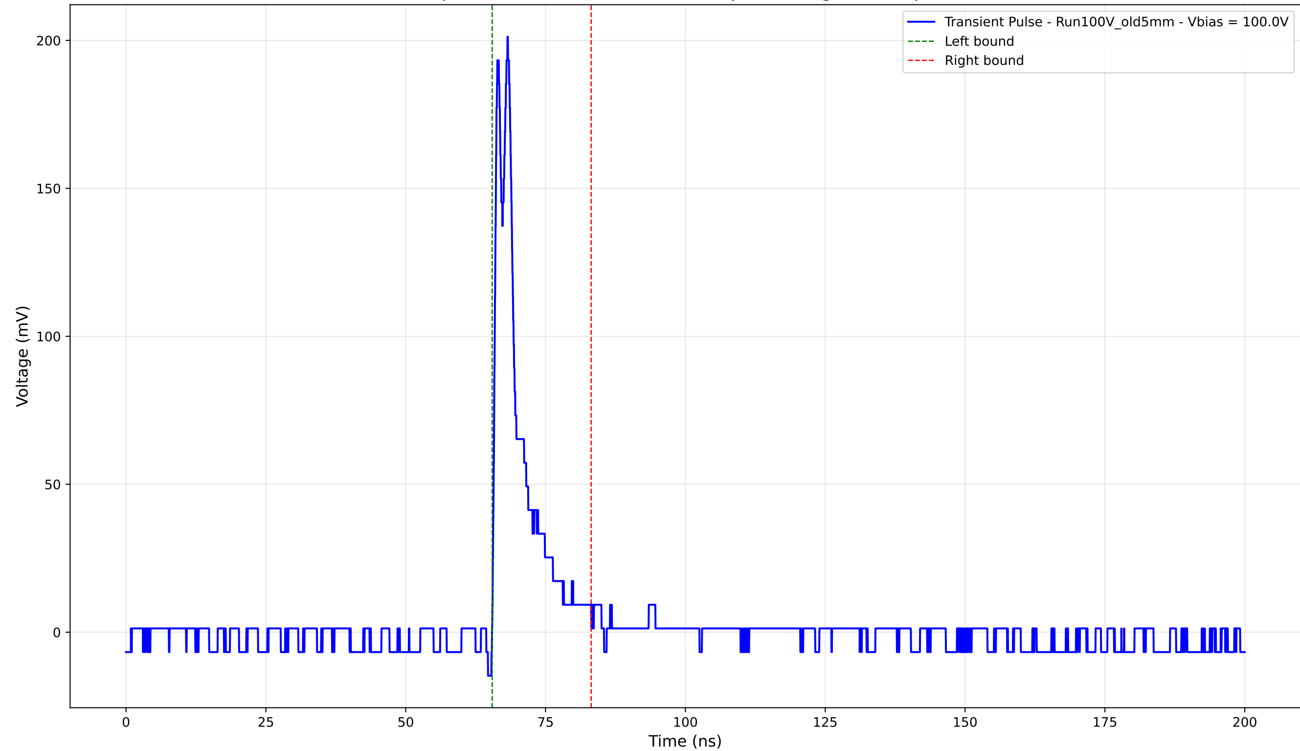
Transient Pulse - Sample: Old5mm - Position: 3575.0 \mu\text{m} - Charge: 19.42 pC - Rise Time: 0.73 ns
