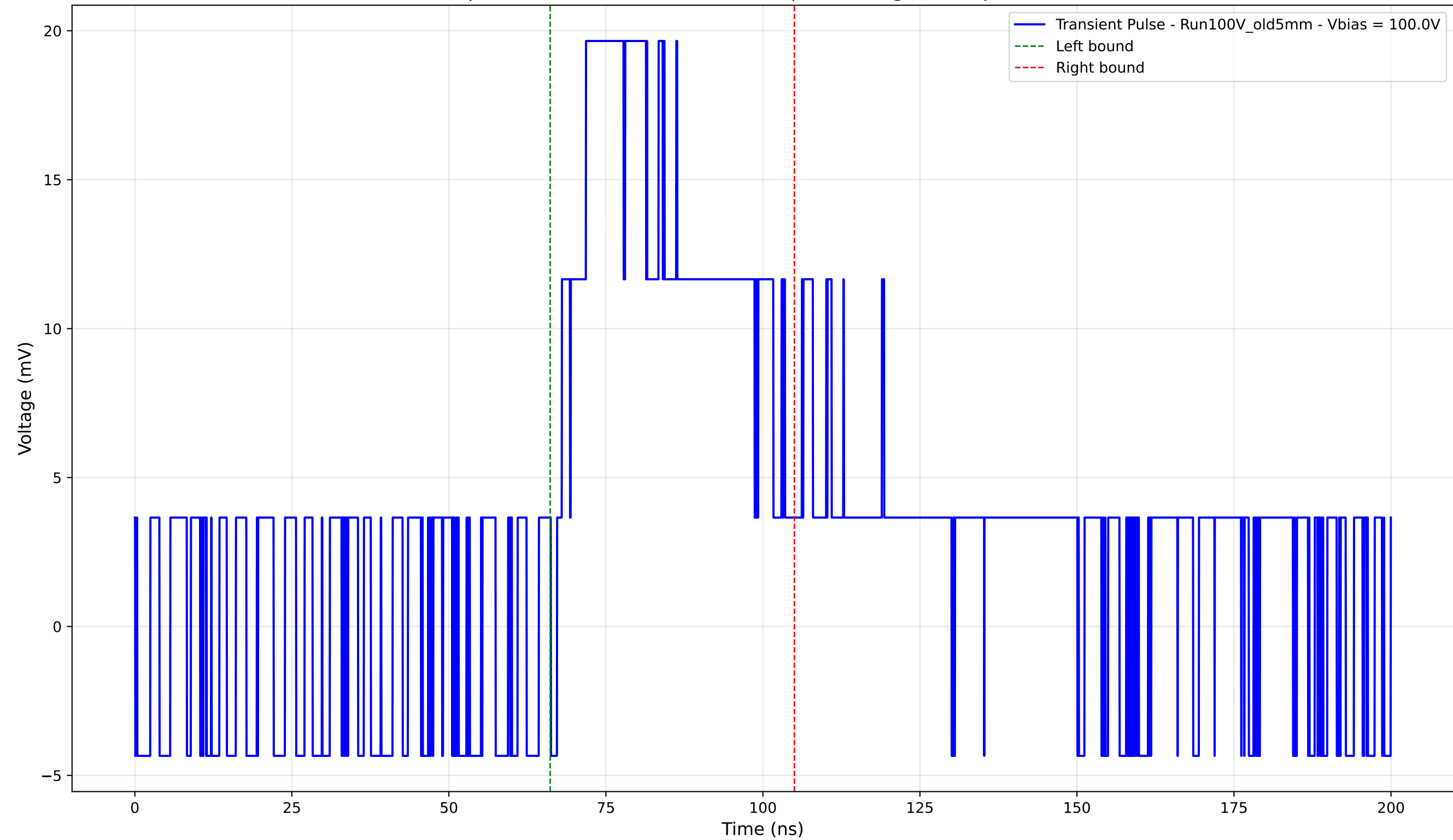
Transient Pulse - Sample: Old5mm - Position: 1990.0 \mu\text{m} - Charge: 9.75 pC - Rise Time: 0.00 ns (N/A)
