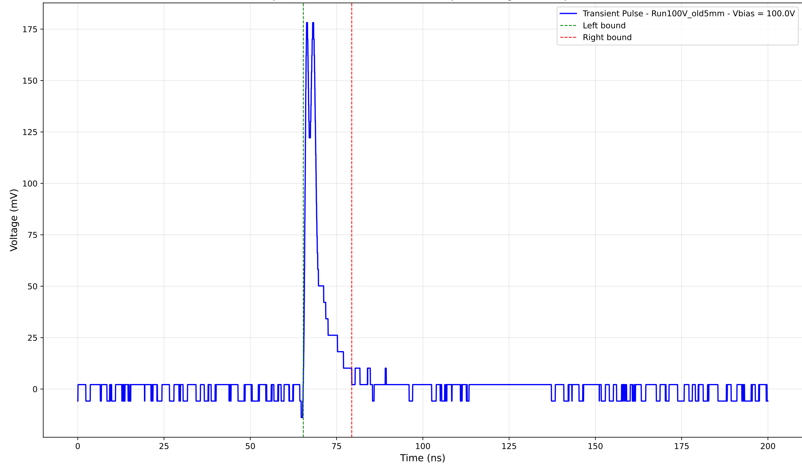
Transient Pulse - Sample: Old5mm - Position: 3610.0 \mu\text{m} - Charge: 15.97 pC - Rise Time: 0.72 ns
