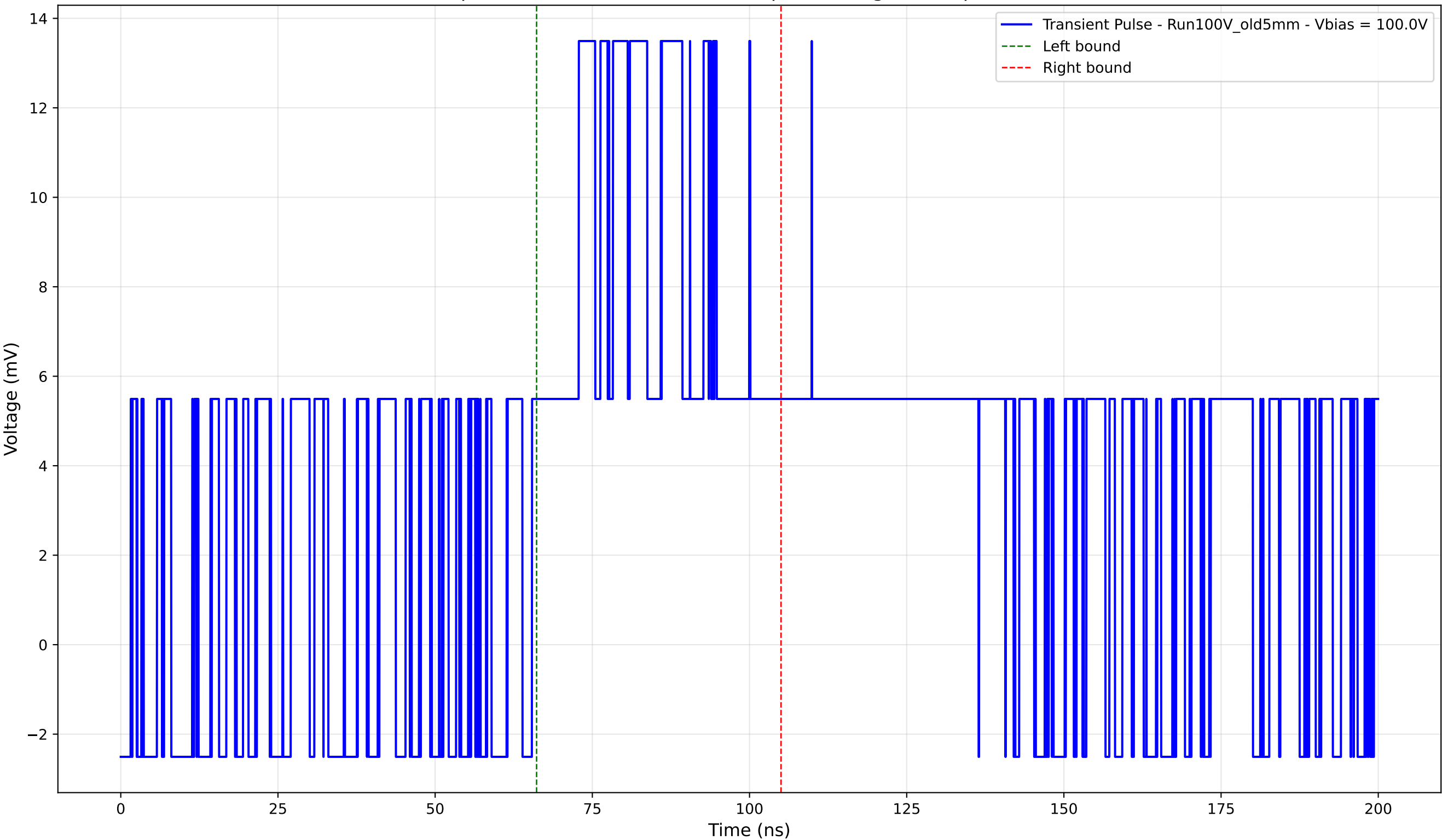
Transient Pulse - Sample: Old5mm - Position: 900.0 \mu\text{m} - Charge: 6.55 pC - Rise Time: 0.00 ns (N/A)
