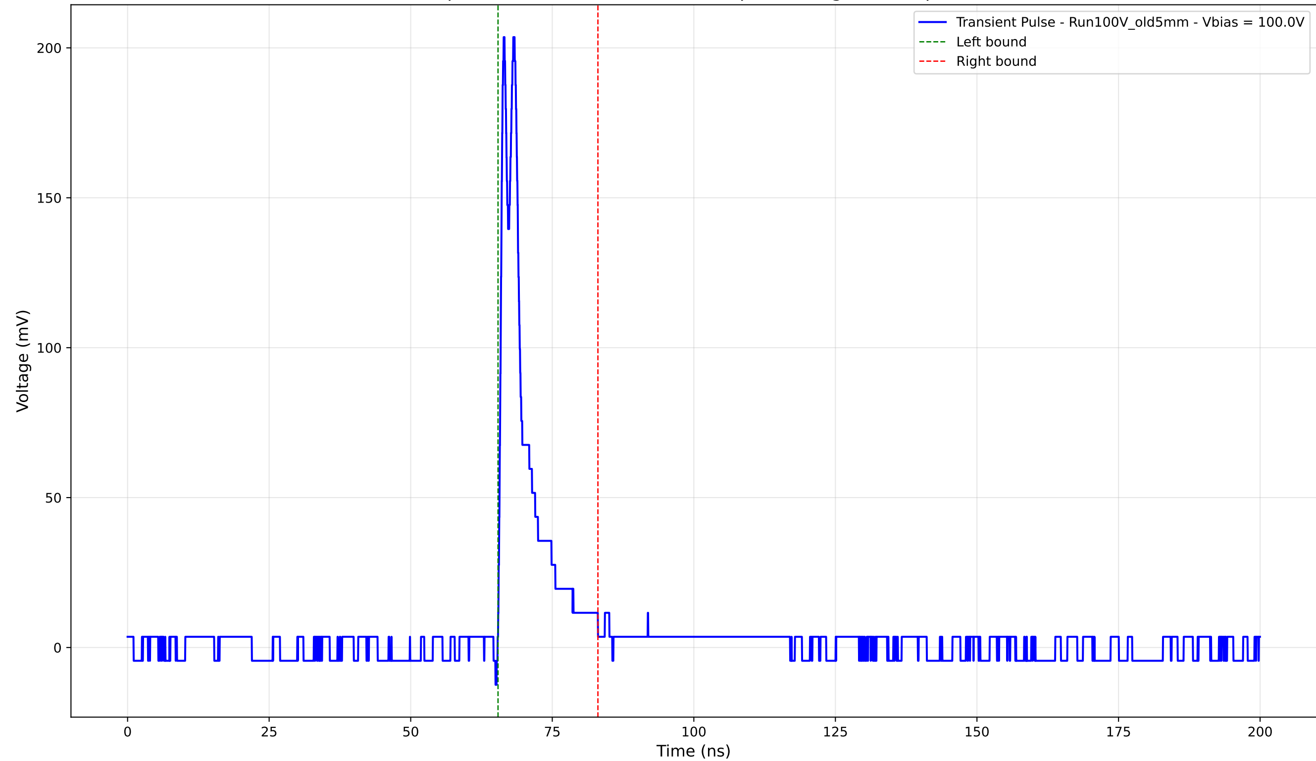
Transient Pulse - Sample: Old5mm - Position: 3590.0 \mu\text{m} - Charge: 20.02 pC - Rise Time: 0.72 ns
