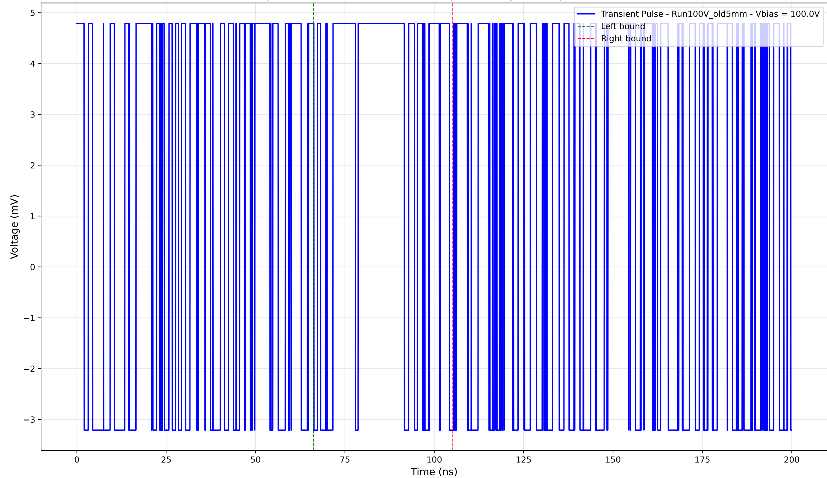
Transient Pulse - Sample: Old5mm - Position: 1715.0 \mu\text{m} - Charge: 2.18 pC - Rise Time: 0.00 ns (N/A)
