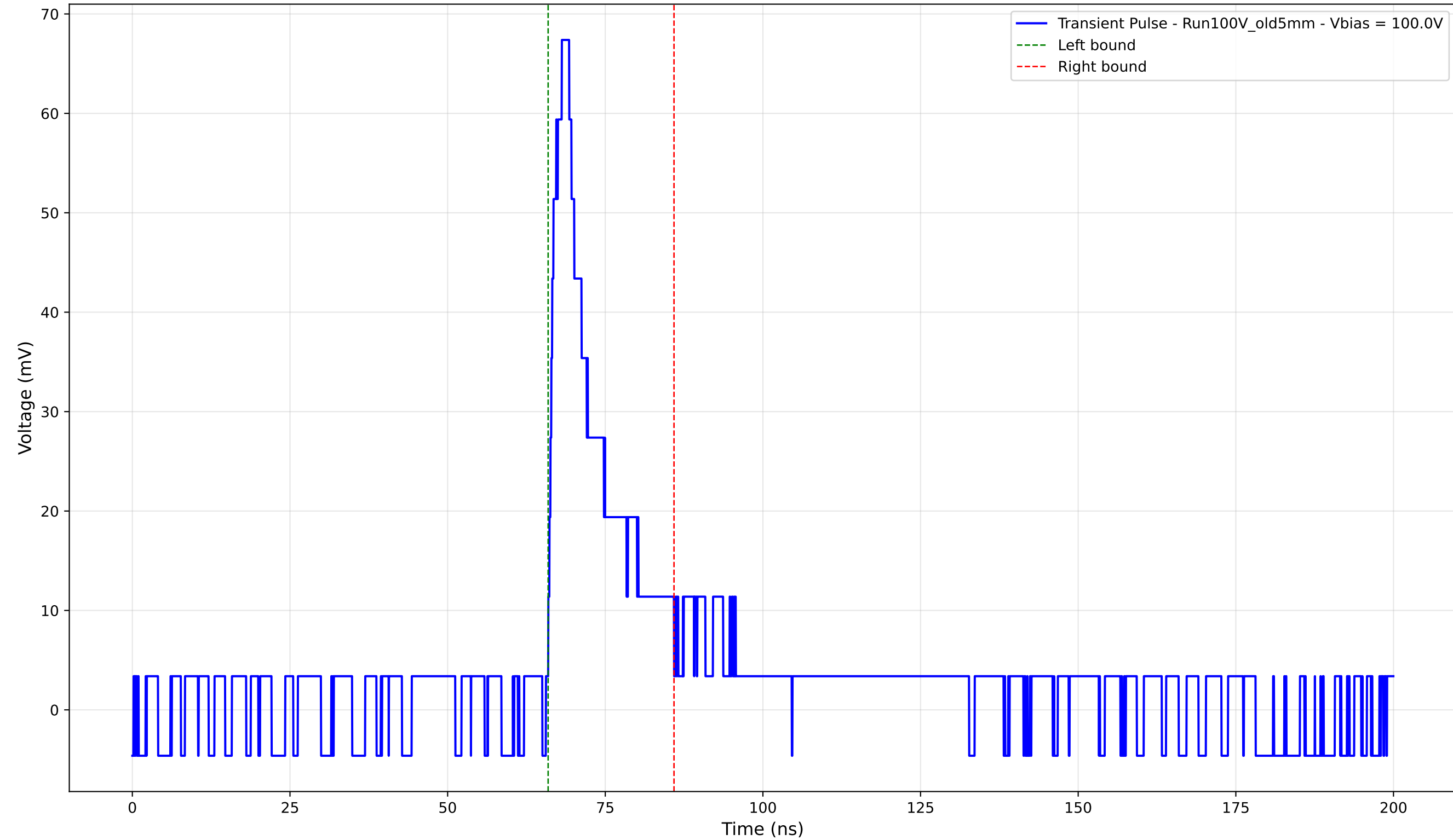
Transient Pulse - Sample: Old5mm - Position: 4220.0 \mu\text{m} - Charge: 10.85 pC - Rise Time: 2.15 ns
