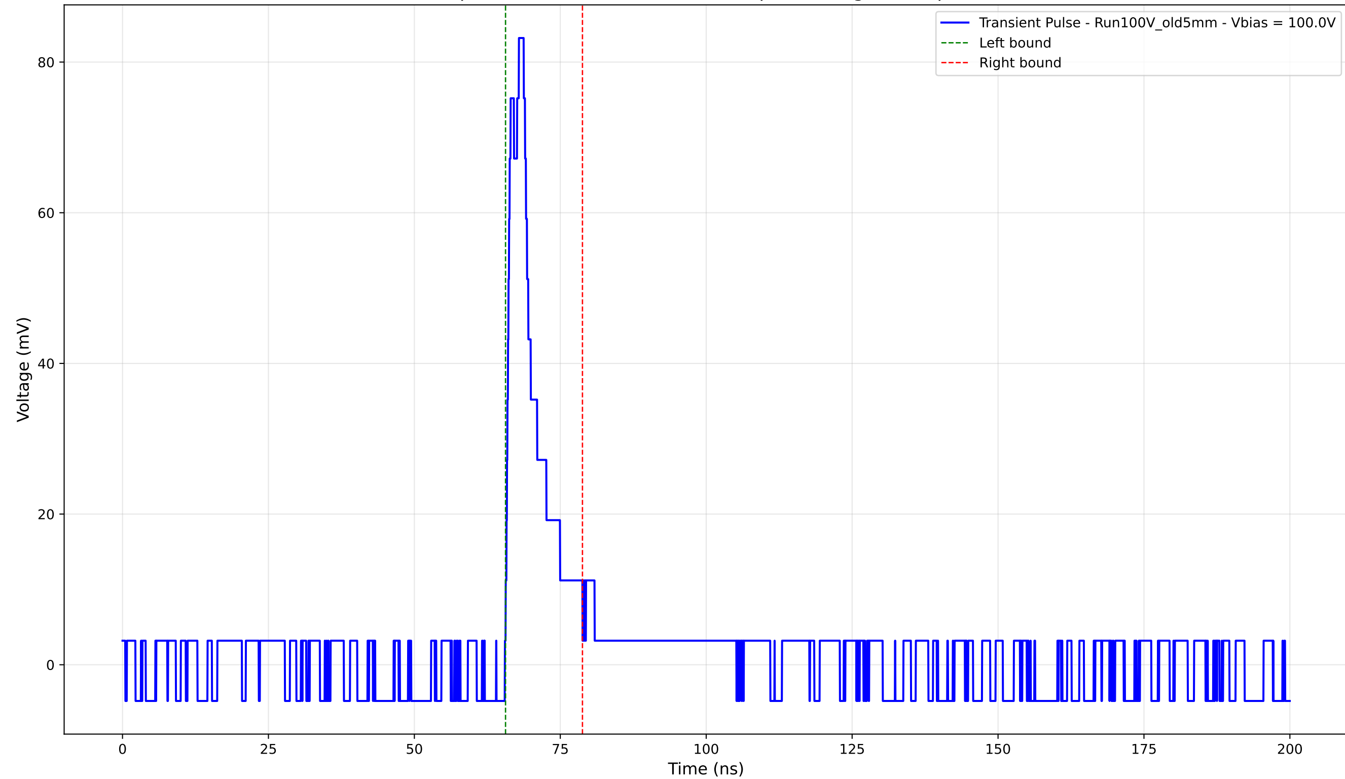
Transient Pulse - Sample: Old5mm - Position: 3940.0 \mu\text{m} - Charge: 8.87 pC - Rise Time: 0.85 ns
