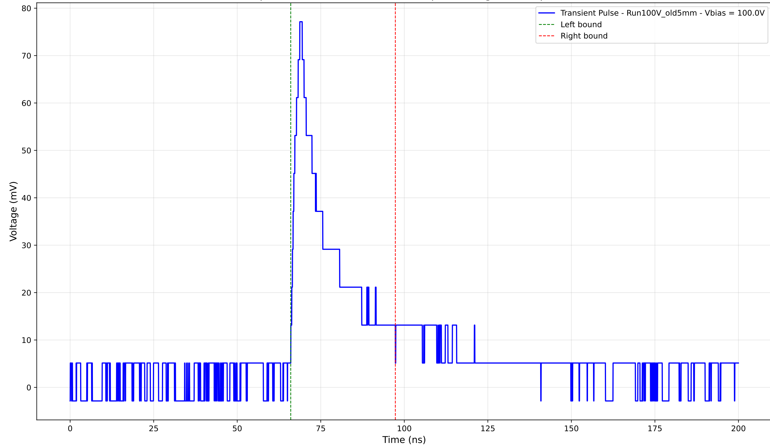
Transient Pulse - Sample: Old5mm - Position: 4470.0 \mu\text{m} - Charge: 18.14 pC - Rise Time: 2.69 ns
