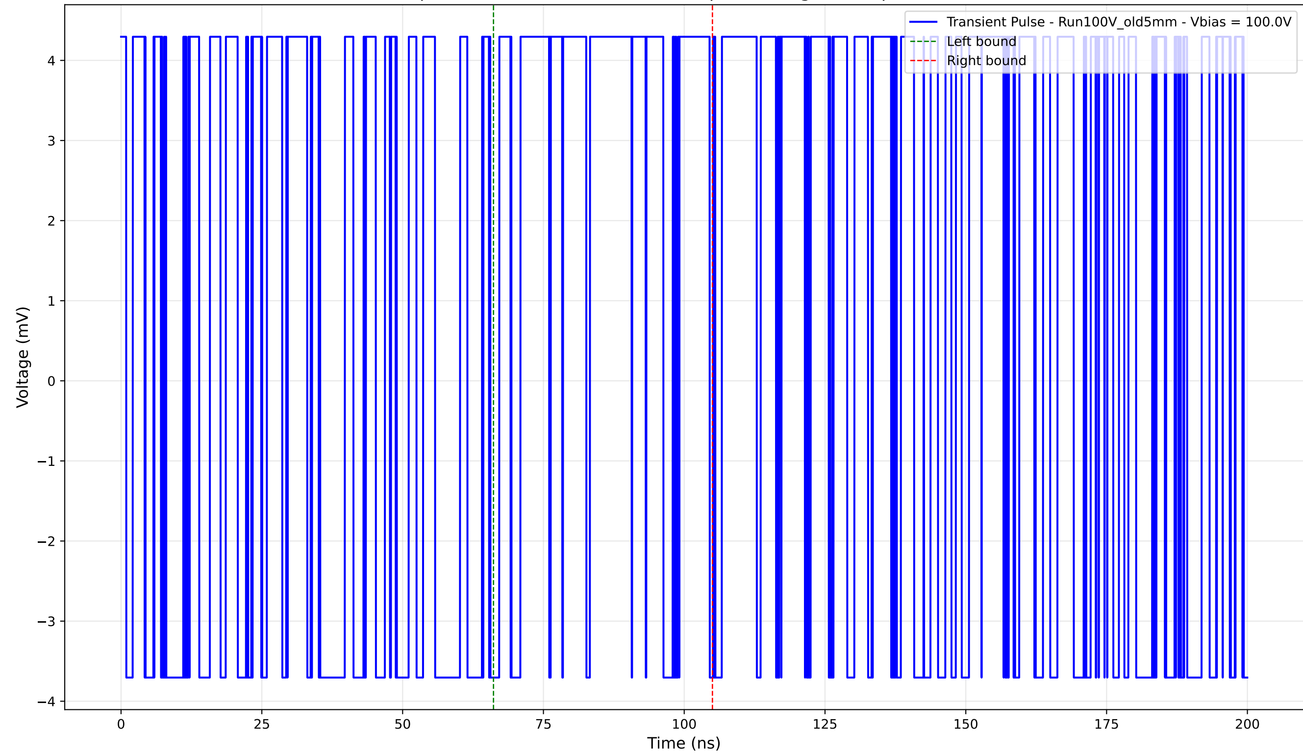
Transient Pulse - Sample: Old5mm - Position: 1530.0 \mu\text{m} - Charge: 2.28 pC - Rise Time: 0.00 ns (N/A)
