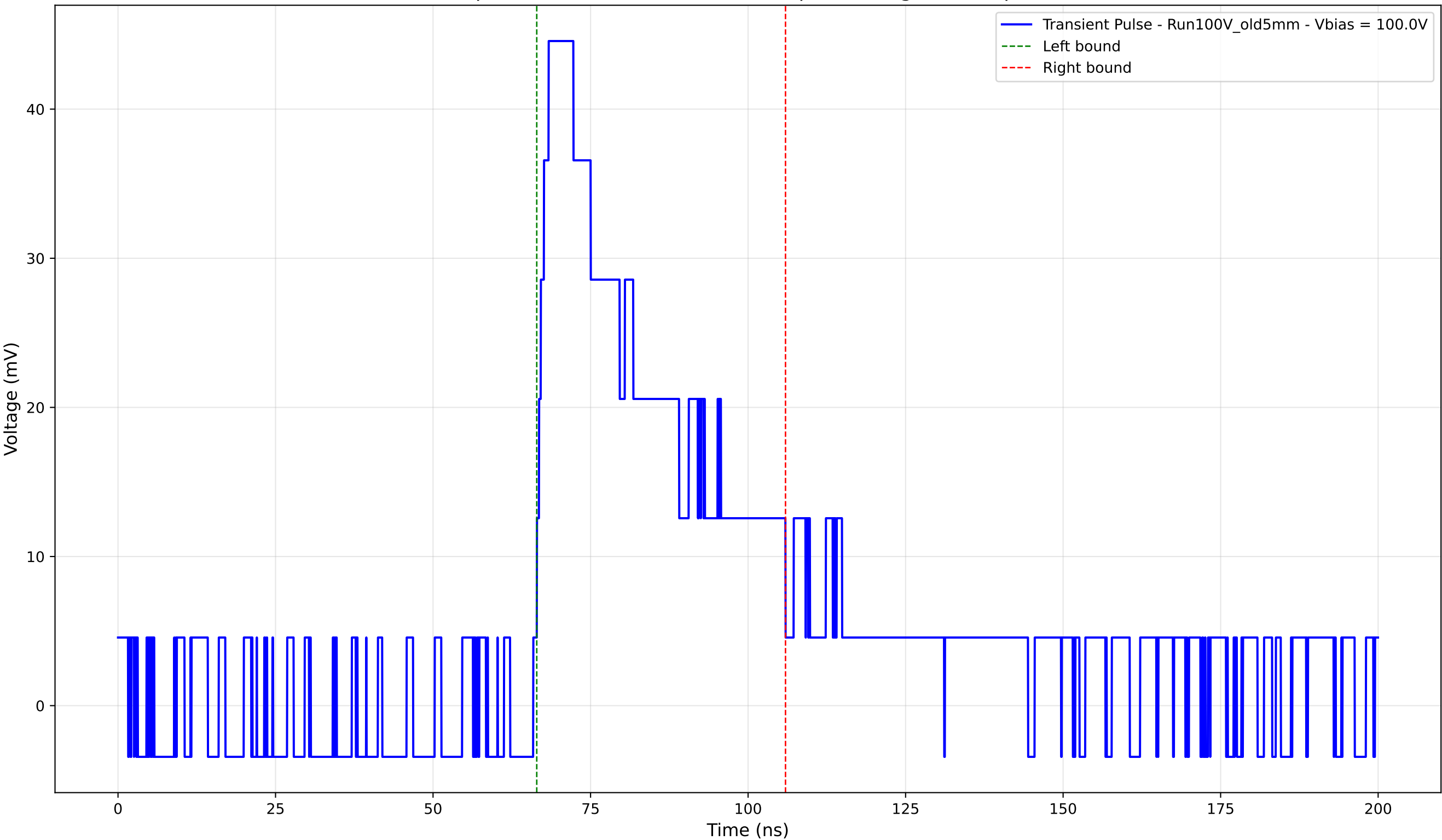
Transient Pulse - Sample: Old5mm - Position: 4770.0 \mu\text{m} - Charge: 17.92 pC - Rise Time: 2.44 ns
