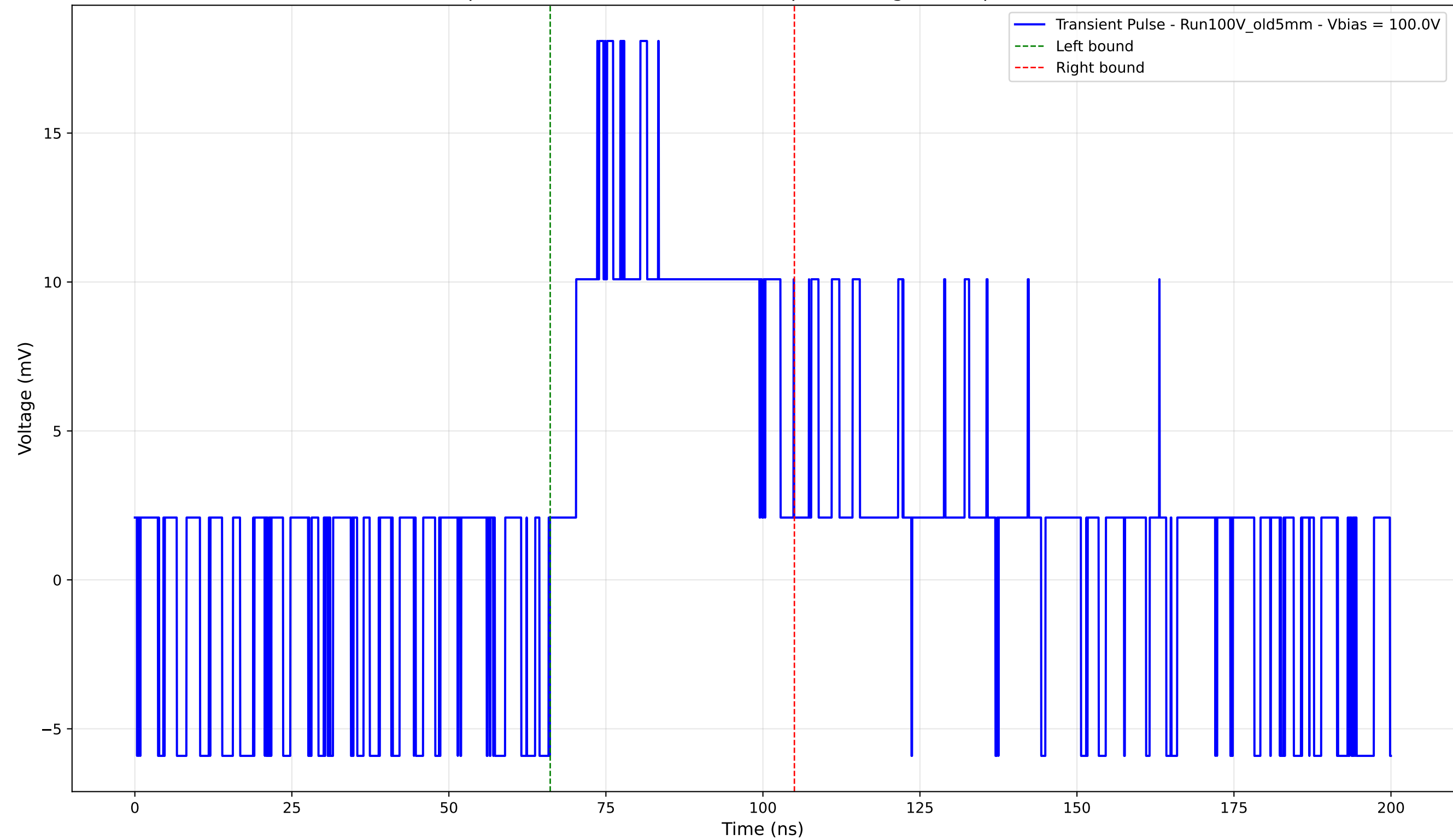
Transient Pulse - Sample: Old5mm - Position: 1430.0 \mu\text{m} - Charge: 7.33 pC - Rise Time: 0.00 ns (N/A)
