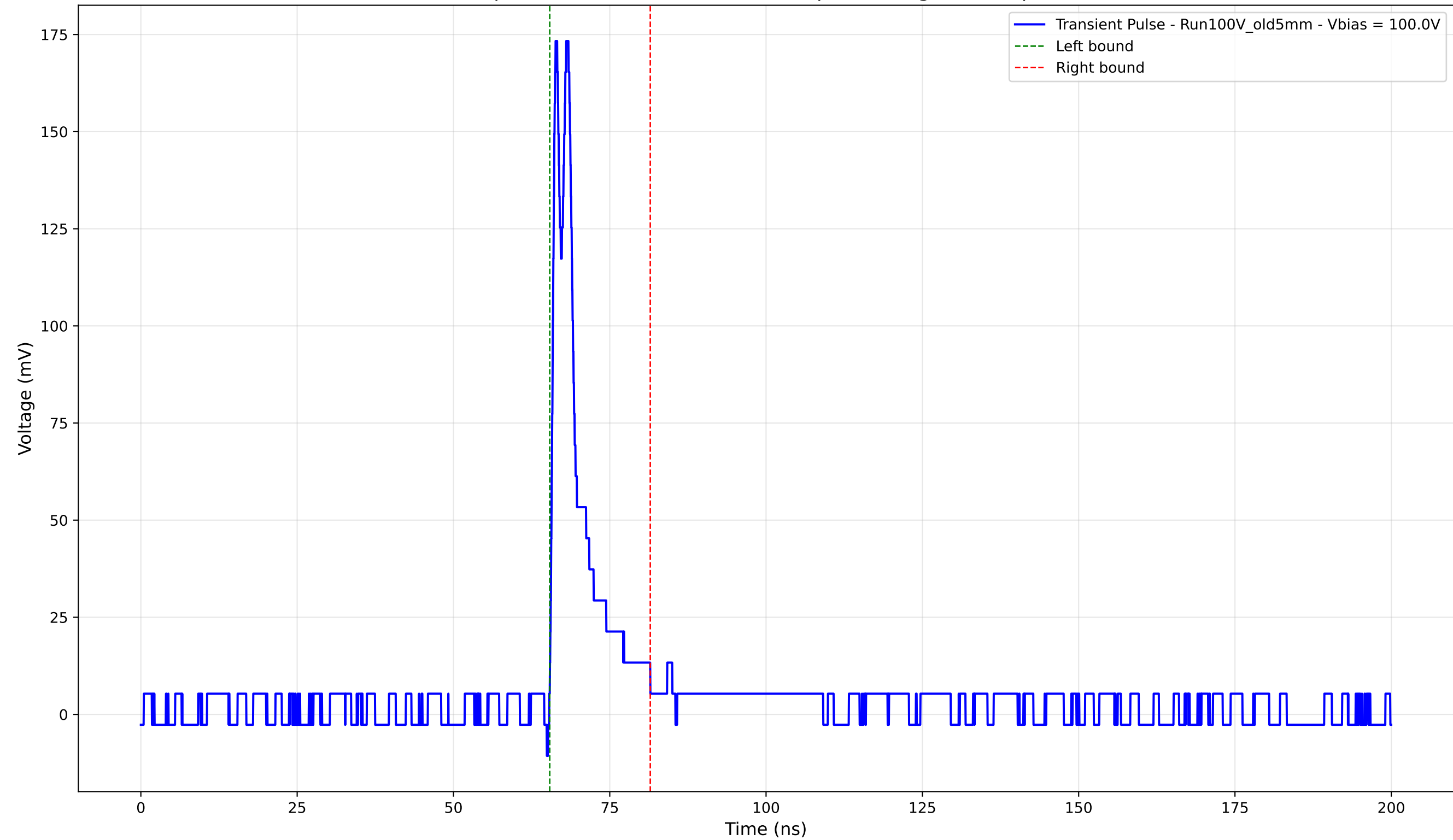
Transient Pulse - Sample: Old5mm - Position: 3800.0 \mu\text{m} - Charge: 16.84 pC - Rise Time: 0.71 ns
