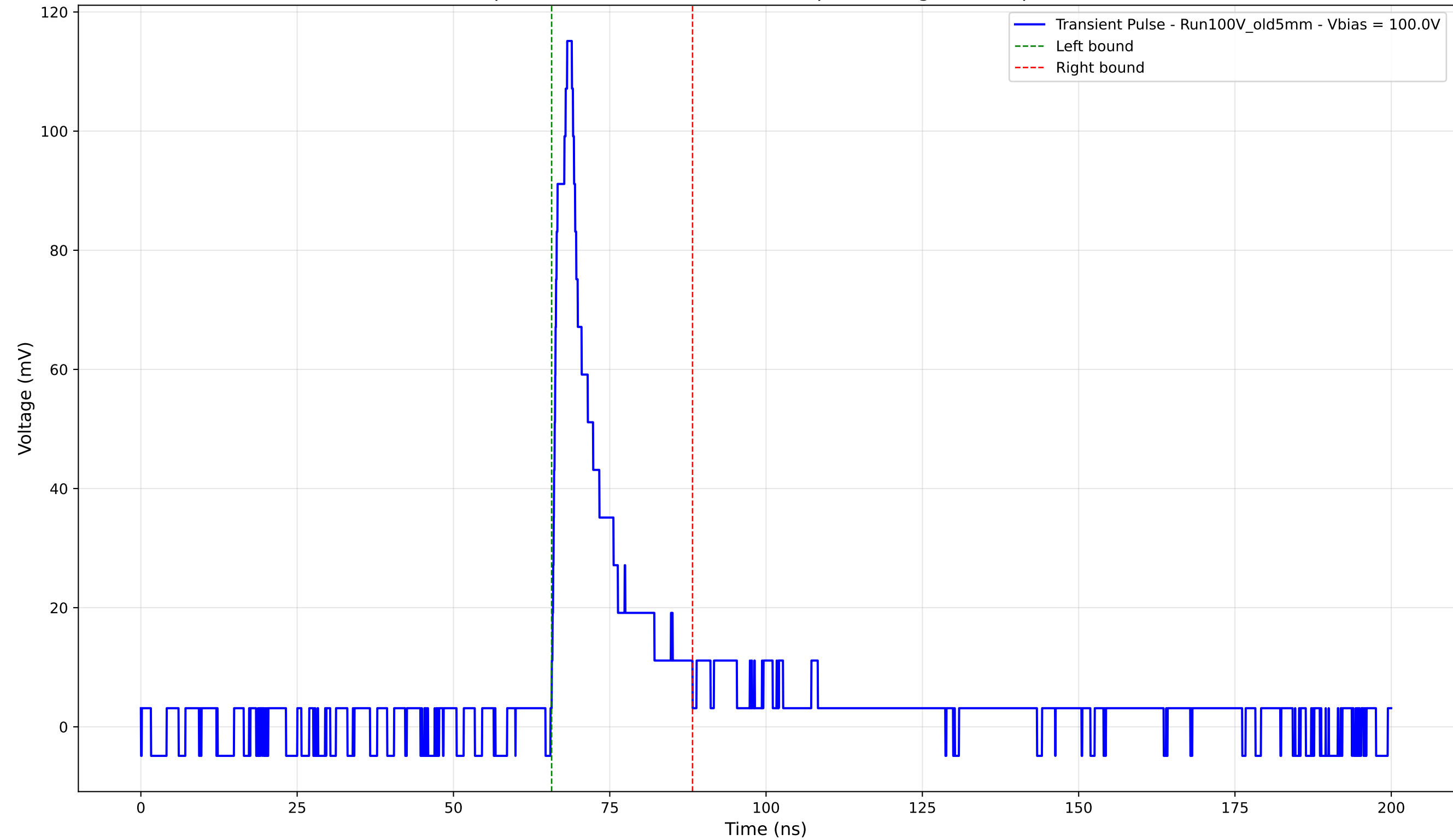
Transient Pulse - Sample: Old5mm - Position: 4125.0 \mu\text{m} - Charge: 16.58 pC - Rise Time: 2.12 ns
