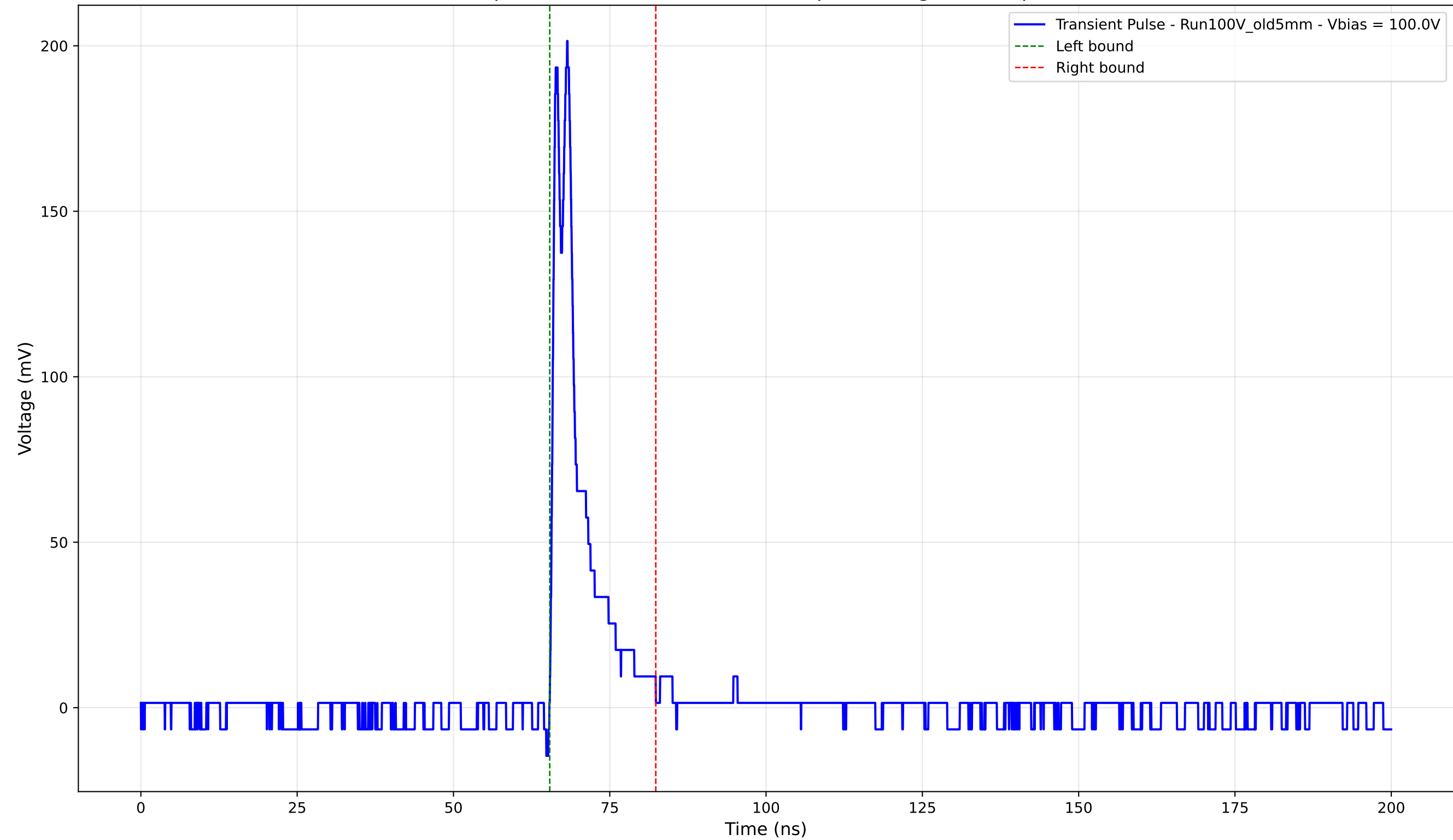
Transient Pulse - Sample: Old5mm - Position: 3830.0 \mu\text{m} - Charge: 19.20 pC - Rise Time: 0.73 ns
