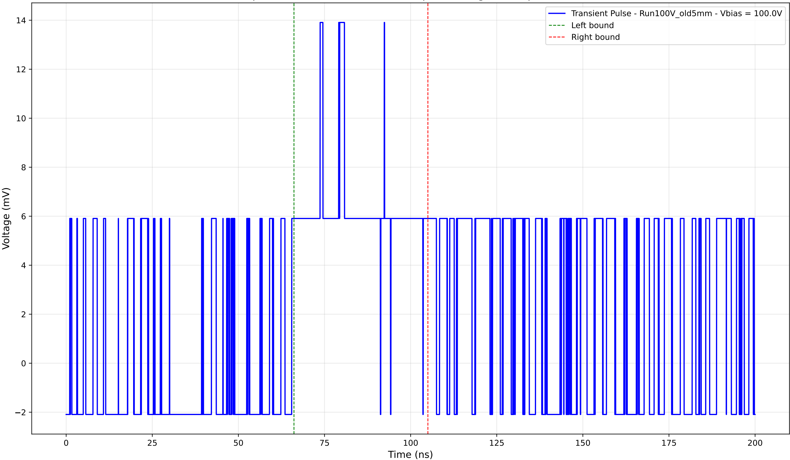
Transient Pulse - Sample: Old5mm - Position: 635.0 \mu\text{m} - Charge: 4.95 pC - Rise Time: 0.00 ns (N/A)
