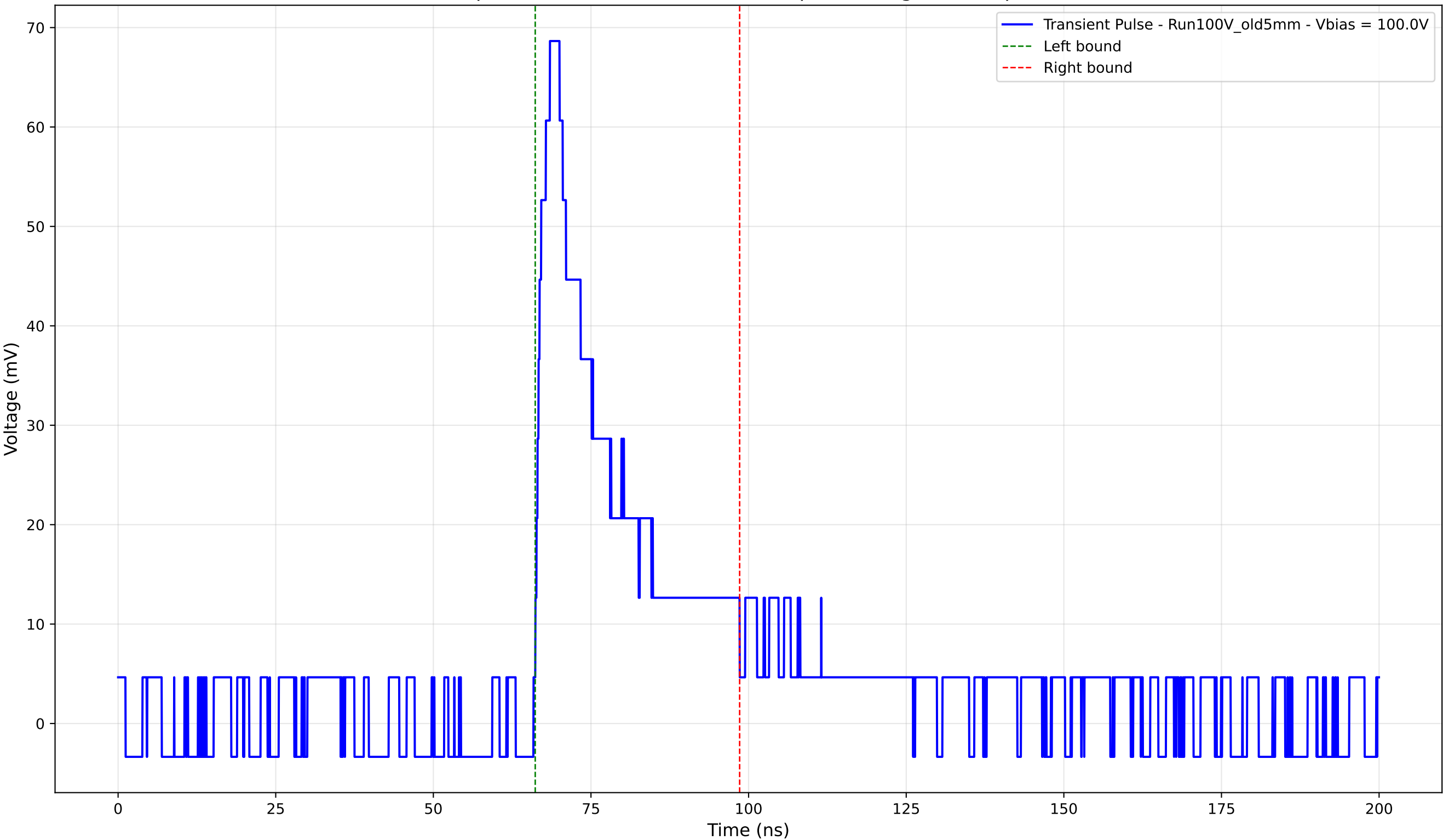
Transient Pulse - Sample: Old5mm - Position: 4465.0 \mu\text{m} - Charge: 16.72 pC - Rise Time: 2.31 ns
