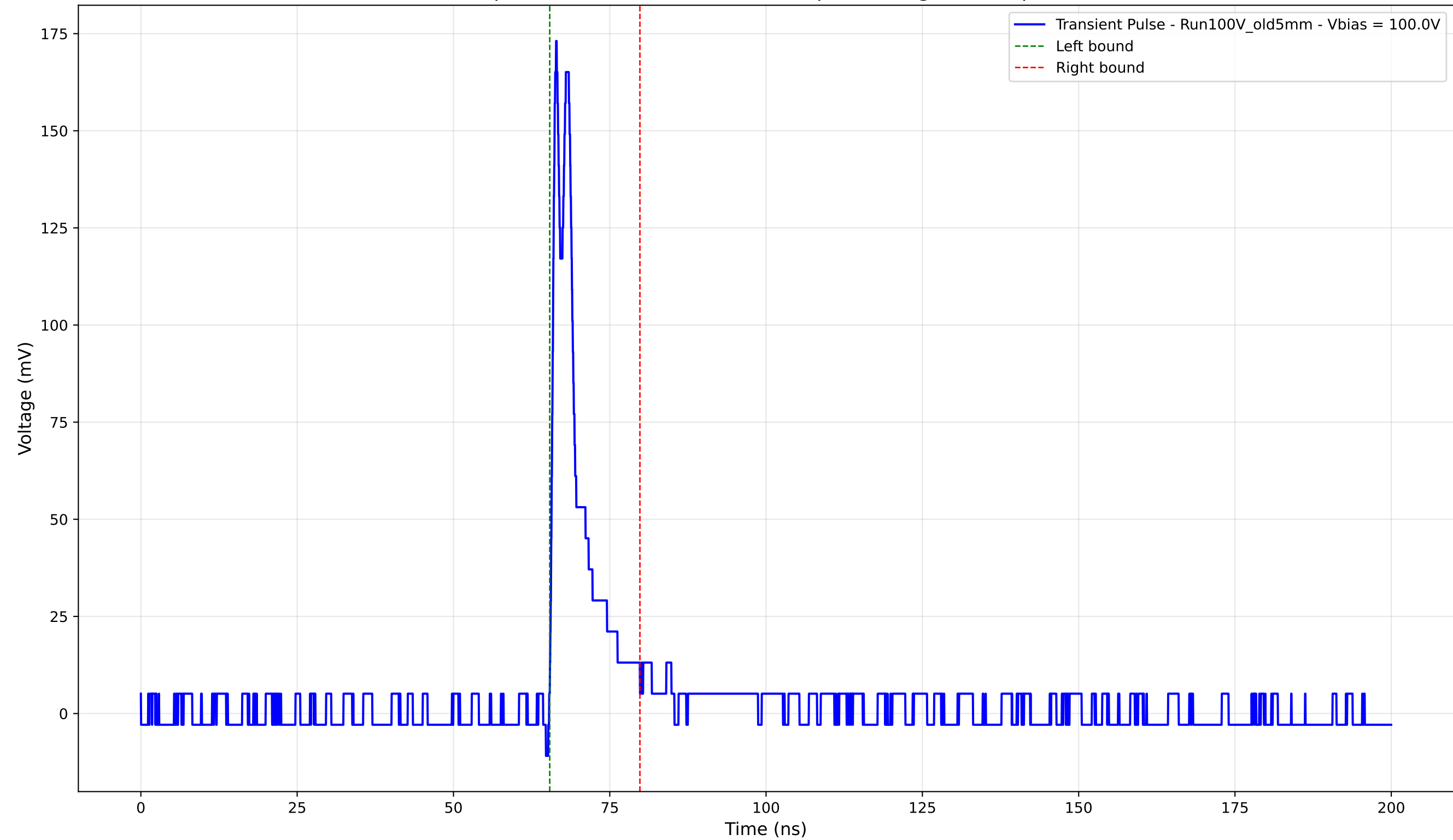
Transient Pulse - Sample: Old5mm - Position: 3620.0 \mu\text{m} - Charge: 15.80 pC - Rise Time: 0.73 ns
