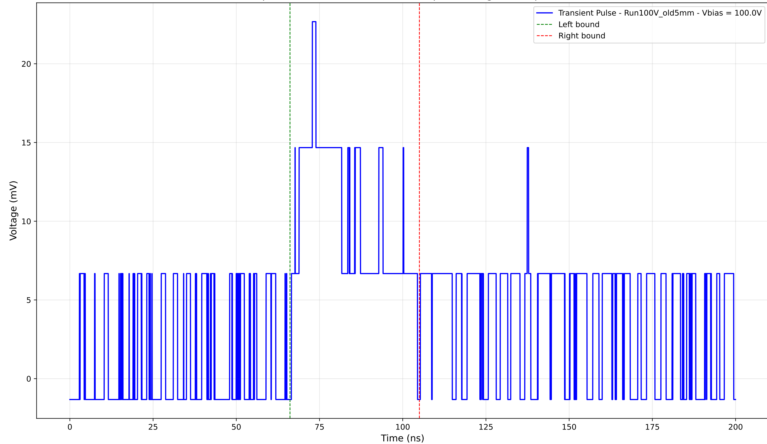
Transient Pulse - Sample: Old5mm - Position: 2360.0 \mu\text{m} - Charge: 7.83 pC - Rise Time: 6.30 ns
