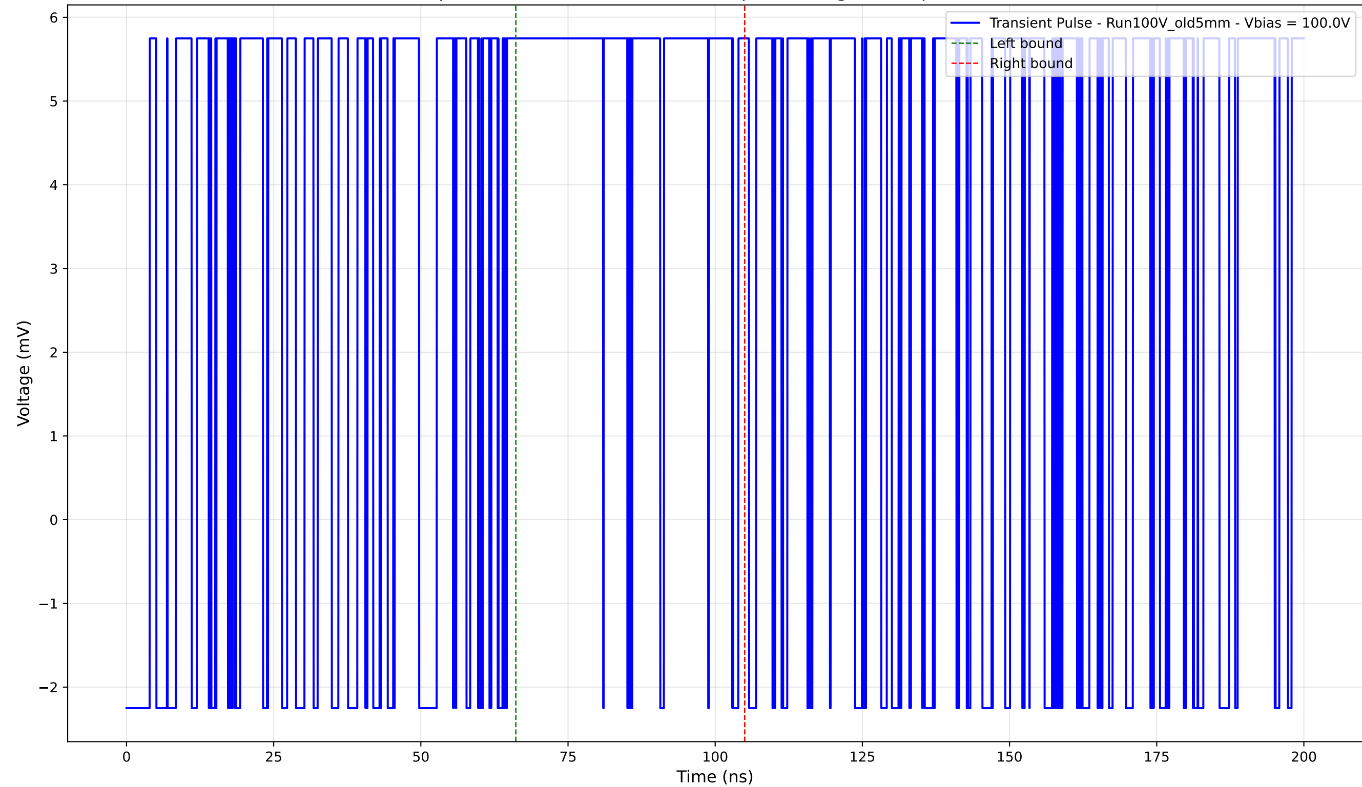
Transient Pulse - Sample: Old5mm - Position: 4330.0 \mu\text{m} - Charge: 4.11 pC - Rise Time: 0.00 ns (N/A)
