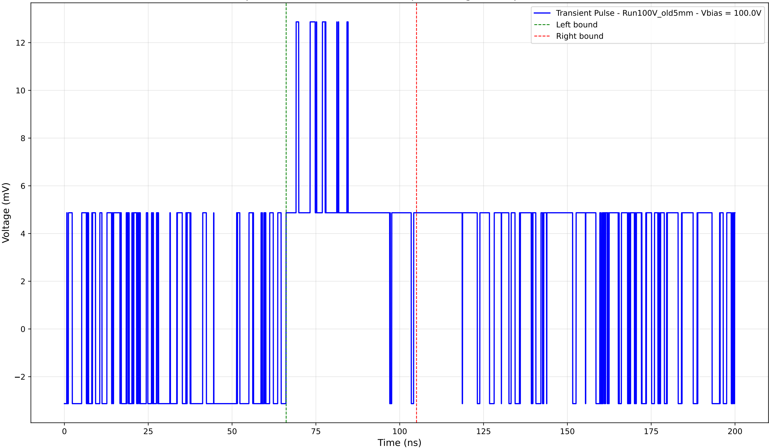
Transient Pulse - Sample: Old5mm - Position: 405.0 \mu\text{m} - Charge: 4.18 pC - Rise Time: 0.00 ns (N/A)
