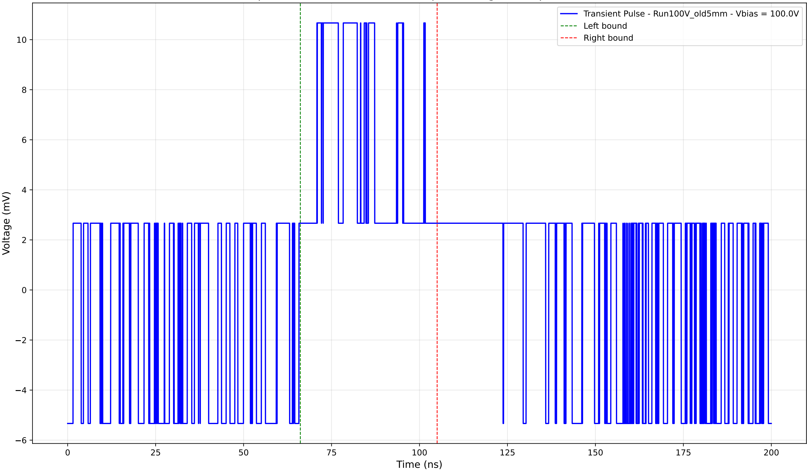
Transient Pulse - Sample: Old5mm - Position: 660.0 \mu\text{m} - Charge: 4.34 pC - Rise Time: 0.00 ns (N/A)
