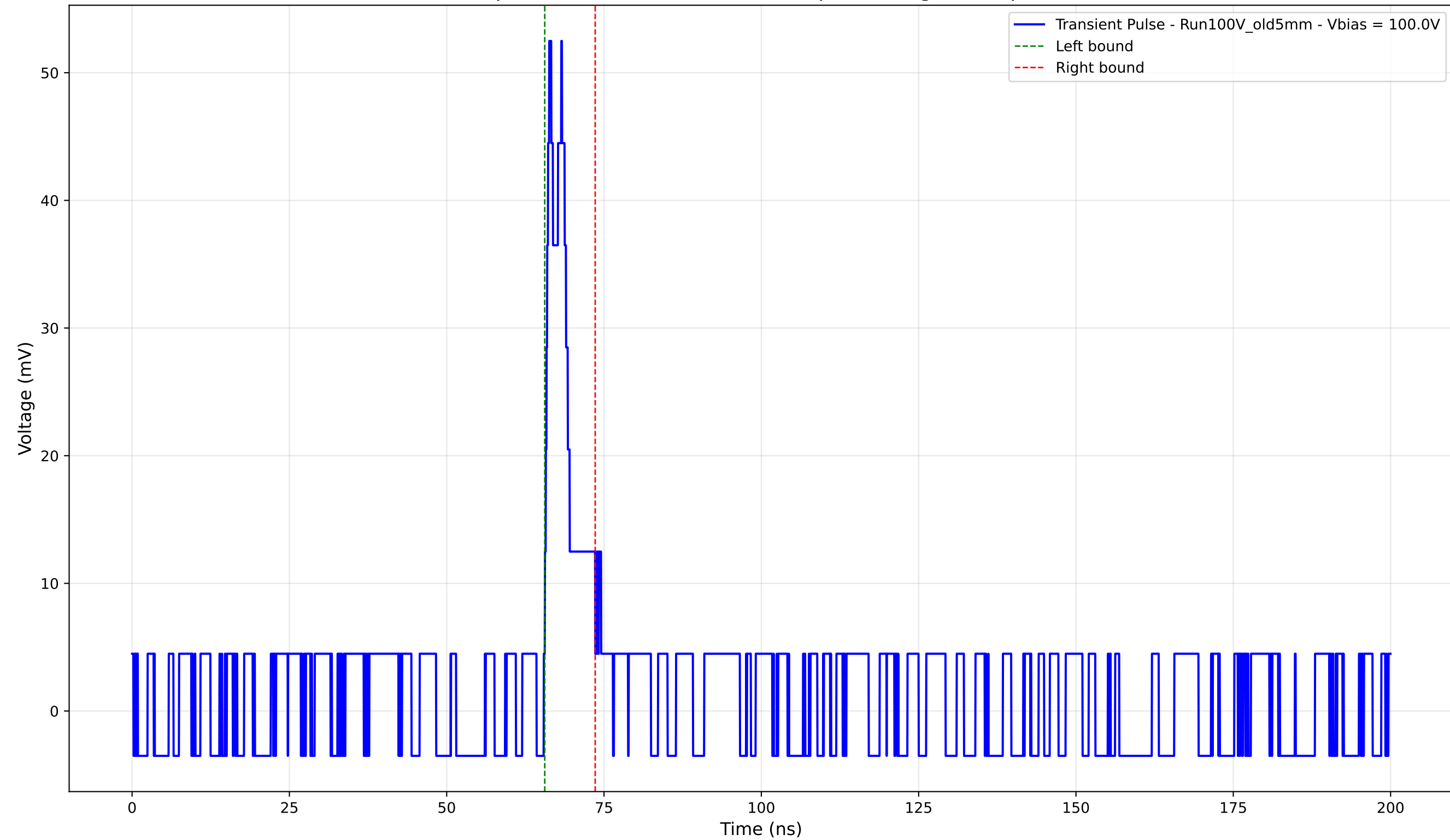
Transient Pulse - Sample: Old5mm - Position: 3660.0 \mu\text{m} - Charge: 4.00 pC - Rise Time: 0.70 ns
