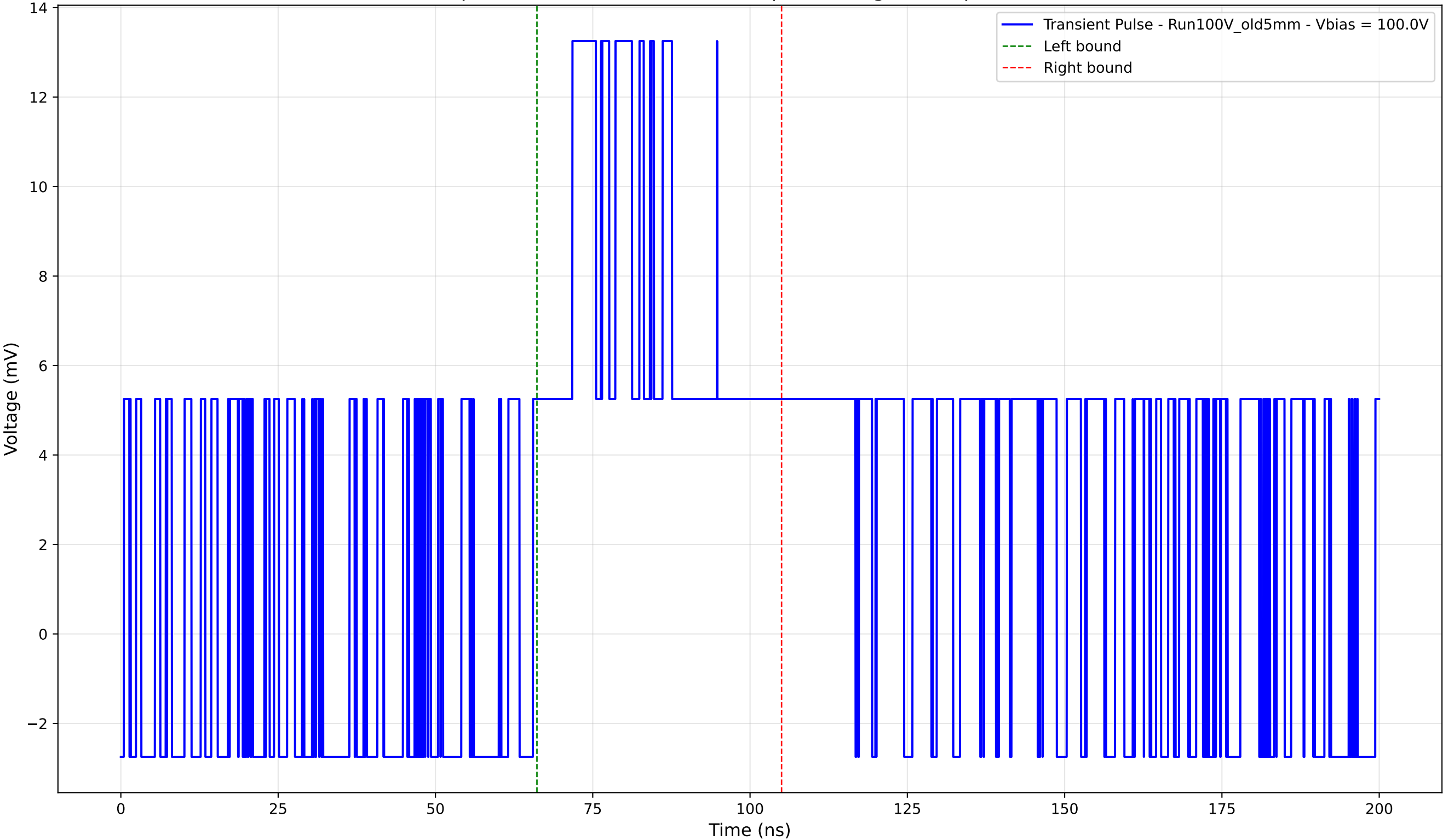
Transient Pulse - Sample: Old5mm - Position: 580.0 \mu\text{m} - Charge: 5.75 pC - Rise Time: 0.00 ns (N/A)
