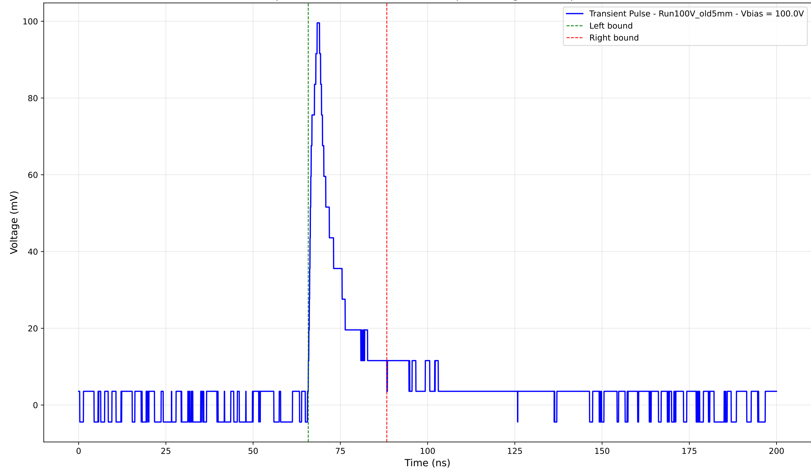
Transient Pulse - Sample: Old5mm - Position: 4195.0 \mu\text{m} - Charge: 15.27 pC - Rise Time: 2.16 ns
