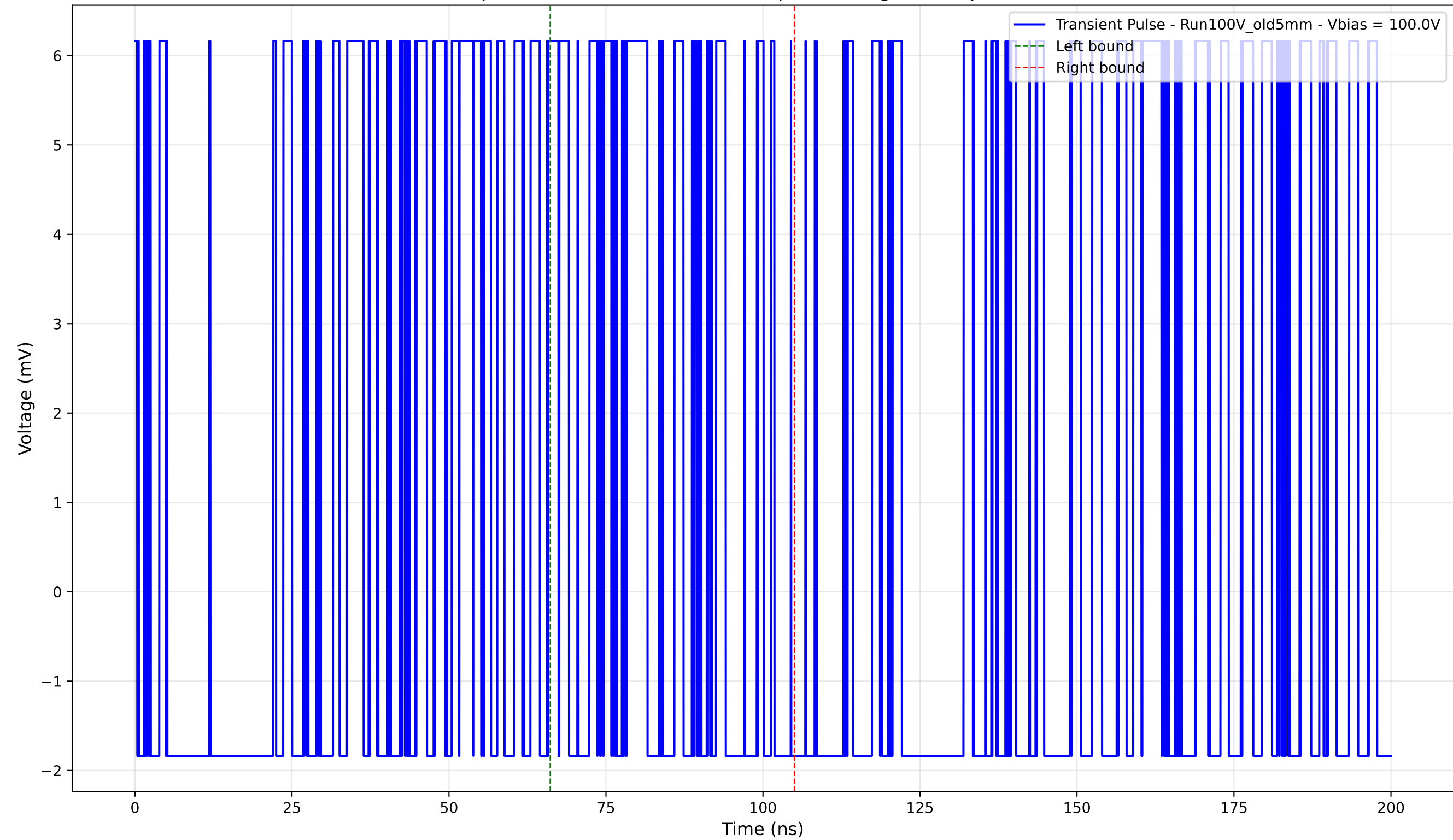
Transient Pulse - Sample: Old5mm - Position: 70.0 \mu\text{m} - Charge: 1.27 pC - Rise Time: 0.00 ns (N/A)
