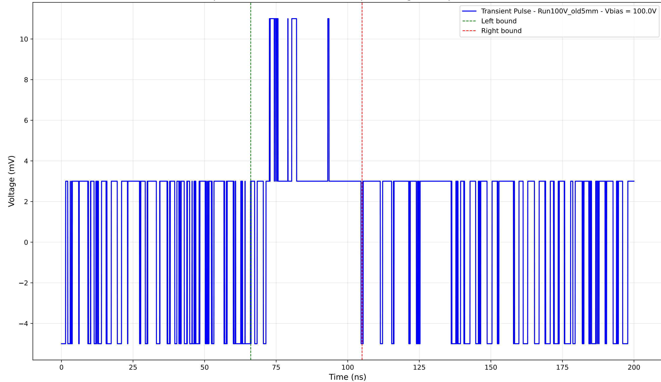
Transient Pulse - Sample: Old5mm - Position: 1545.0 \mu\text{m} - Charge: 2.76 pC - Rise Time: 0.00 ns (N/A)
