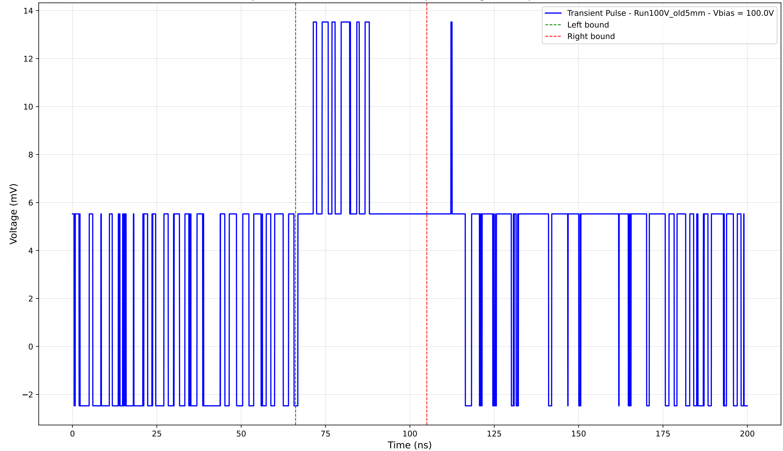
Transient Pulse - Sample: Old5mm - Position: 1465.0 \mu\text{m} - Charge: 5.54 pC - Rise Time: 0.00 ns (N/A)
