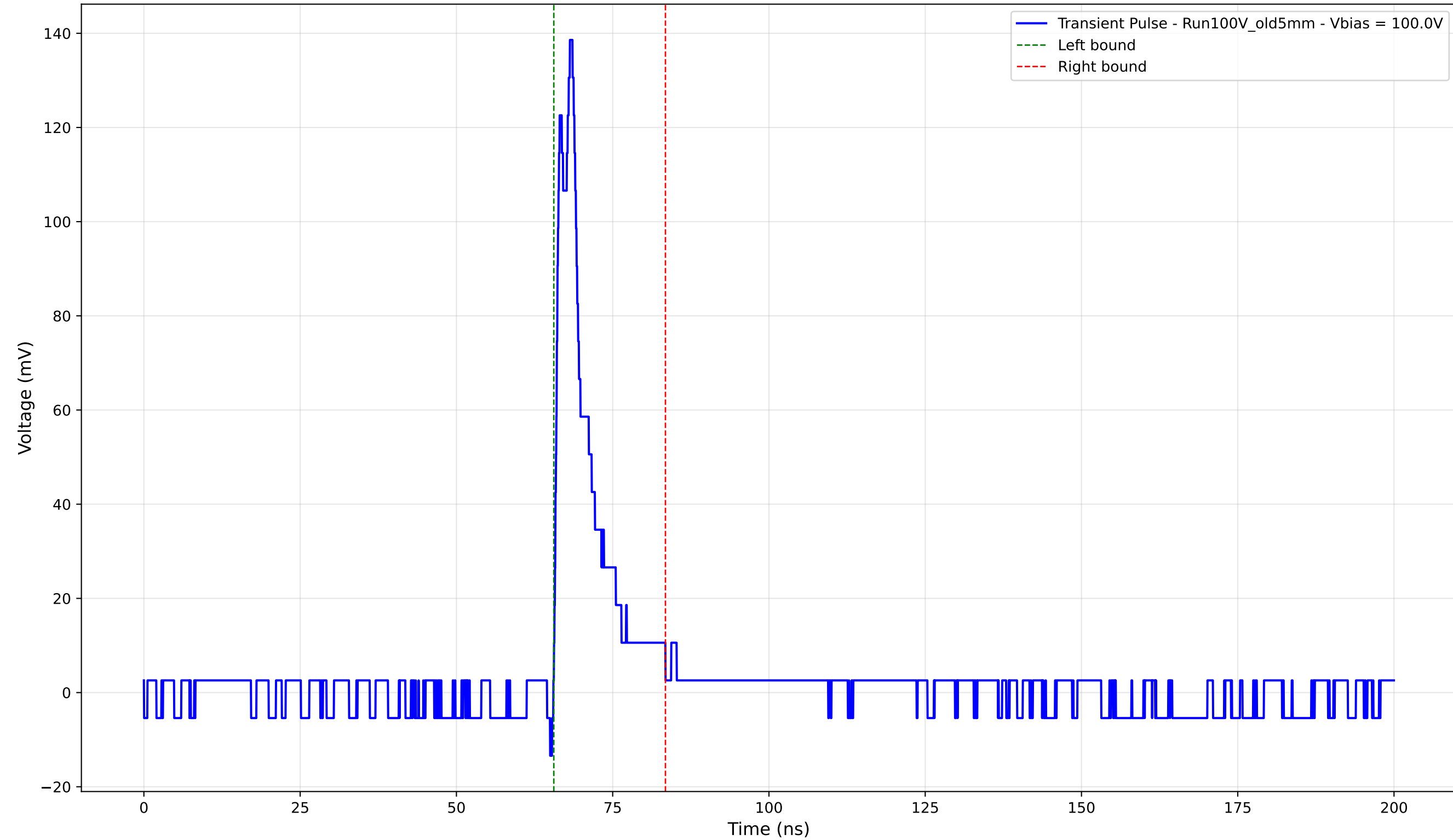
Transient Pulse - Sample: Old5mm - Position: 3500.0 \mu\text{m} - Charge: 14.93 pC - Rise Time: 2.29 ns
