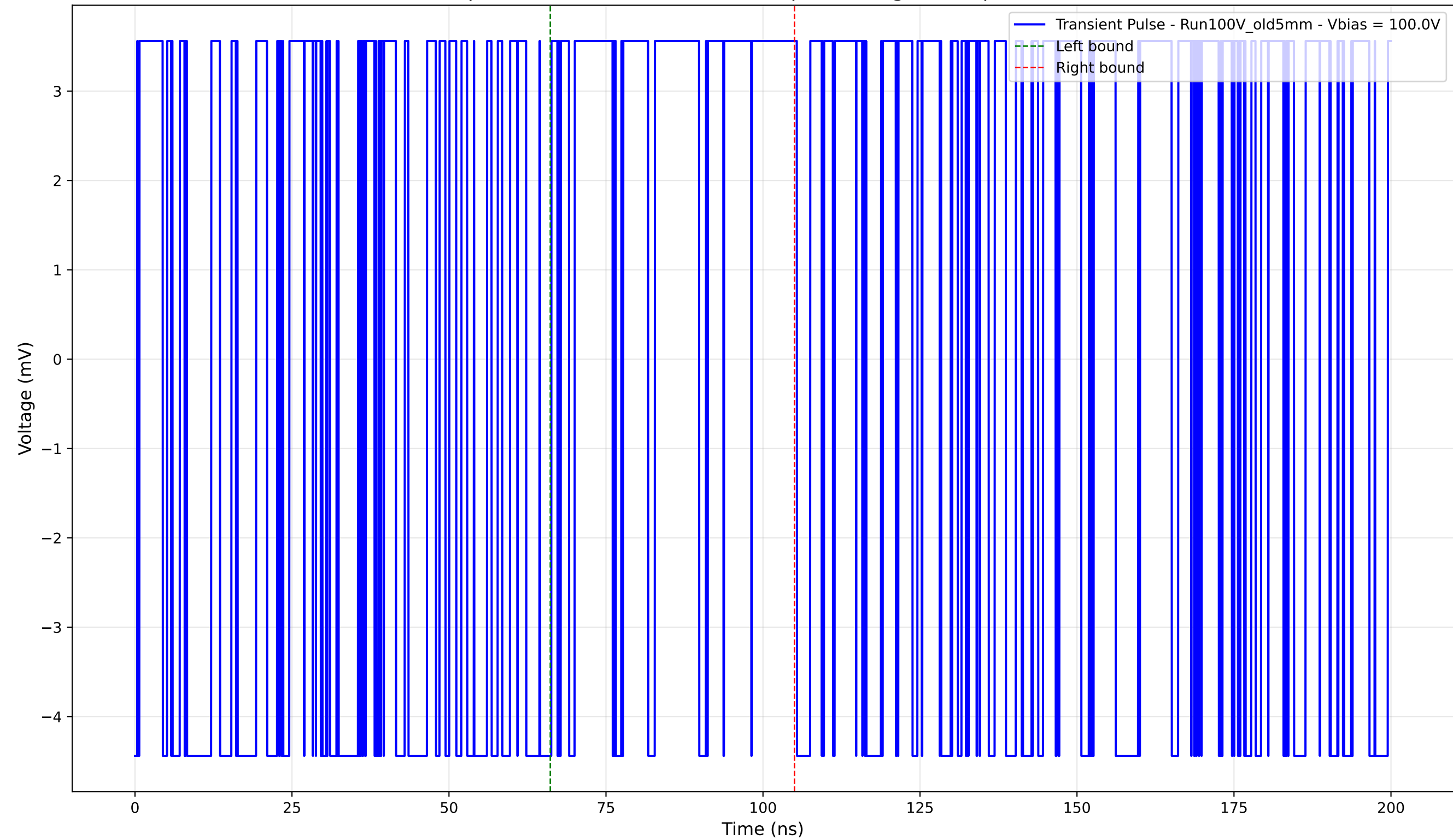
Transient Pulse - Sample: Old5mm - Position: 1305.0 \mu\text{m} - Charge: 1.93 pC - Rise Time: 0.00 ns (N/A)
