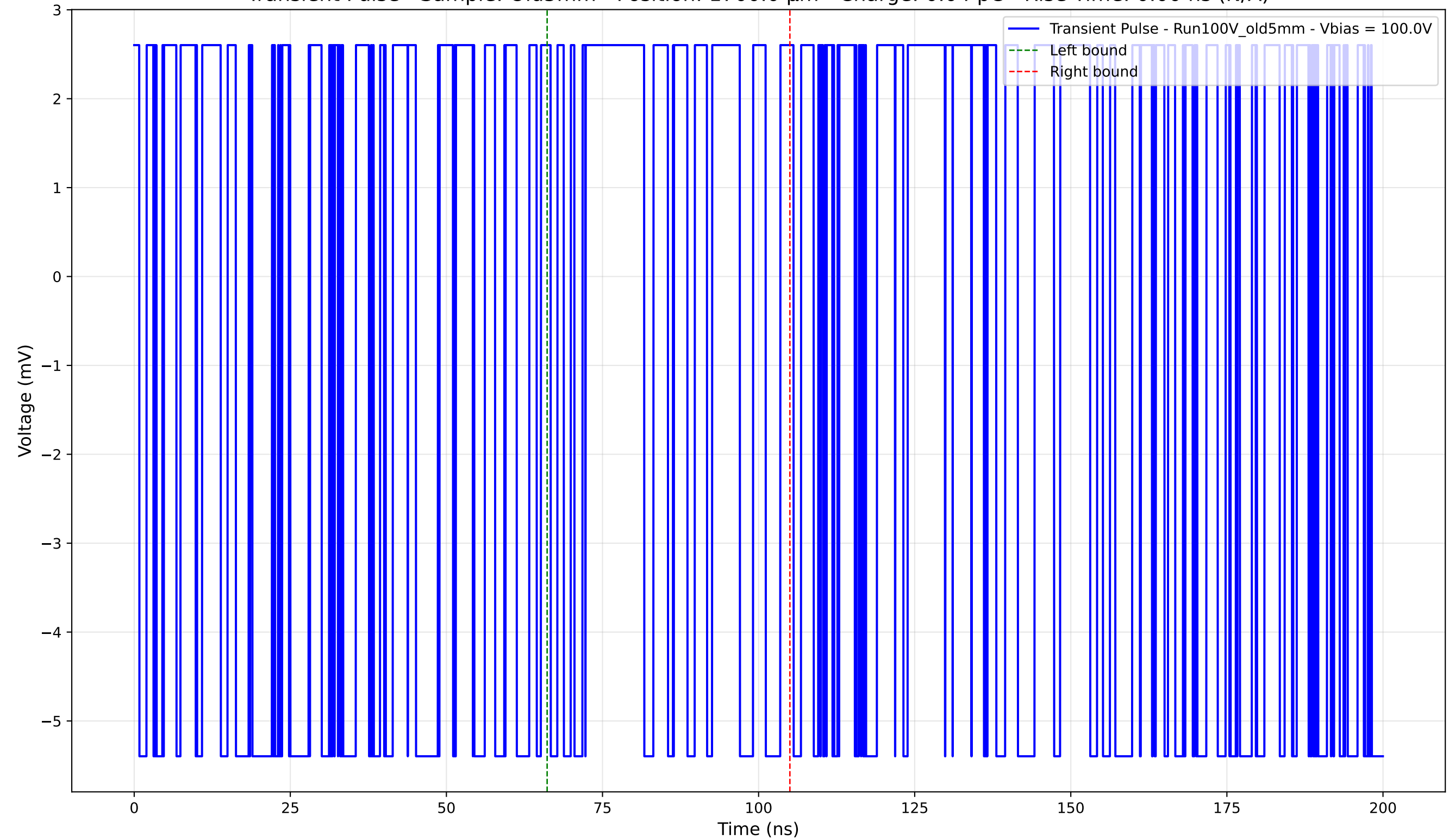
Transient Pulse - Sample: Old5mm - Position: 1700.0 \mu\text{m} - Charge: 0.04 pC - Rise Time: 0.00 ns (N/A)
