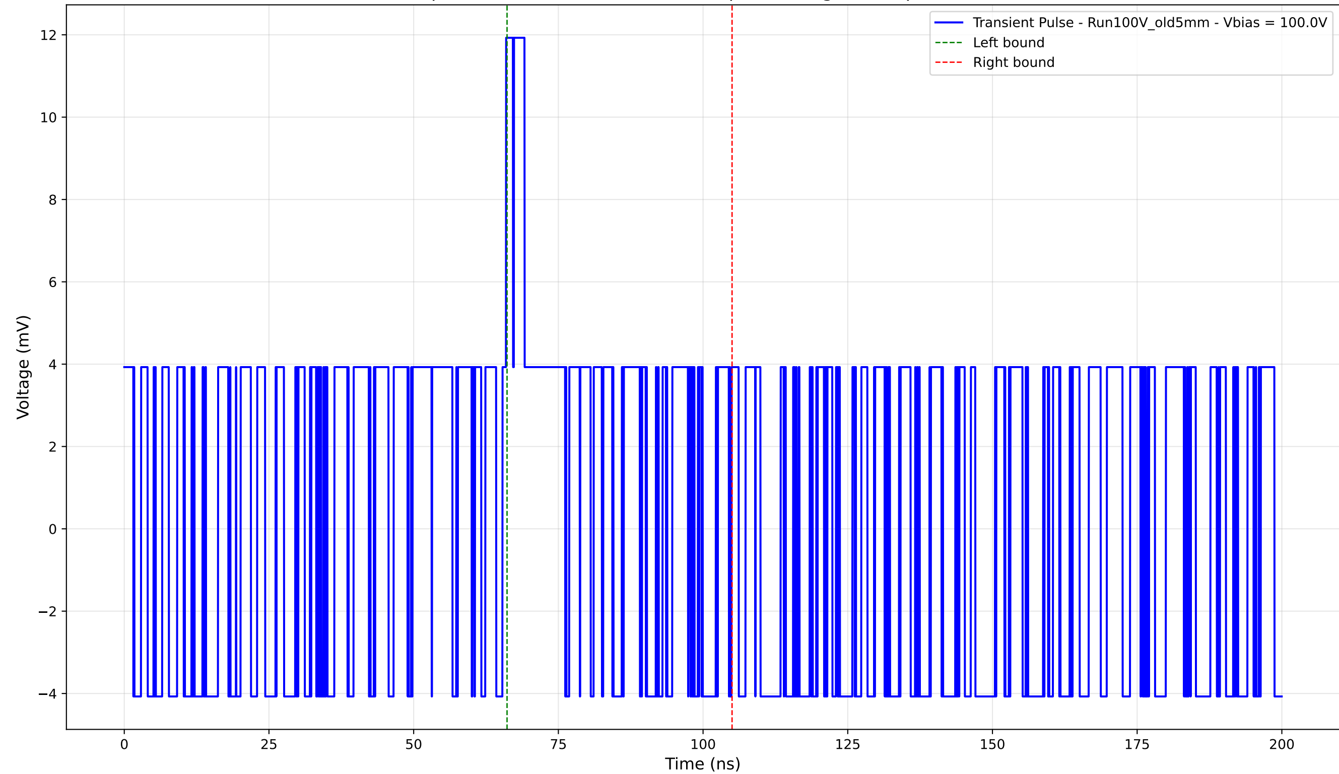
Transient Pulse - Sample: Old5mm - Position: 3690.0 \mu\text{m} - Charge: 1.82 pC - Rise Time: 0.00 ns (N/A)
