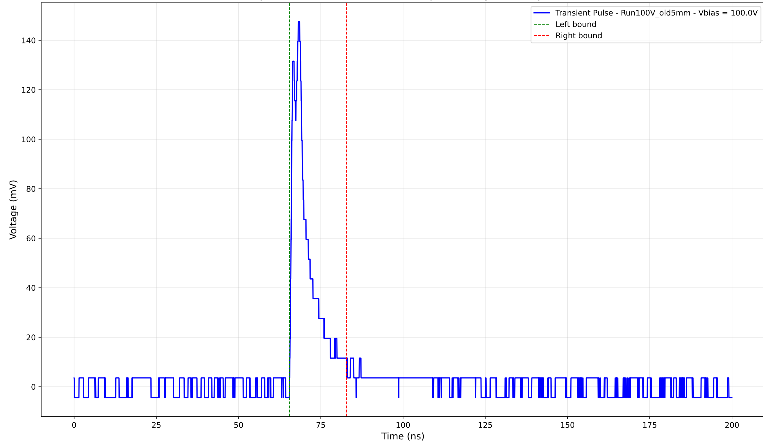
Transient Pulse - Sample: Old5mm - Position: 3505.0 \mu\text{m} - Charge: 16.50 pC - Rise Time: 2.35 ns
