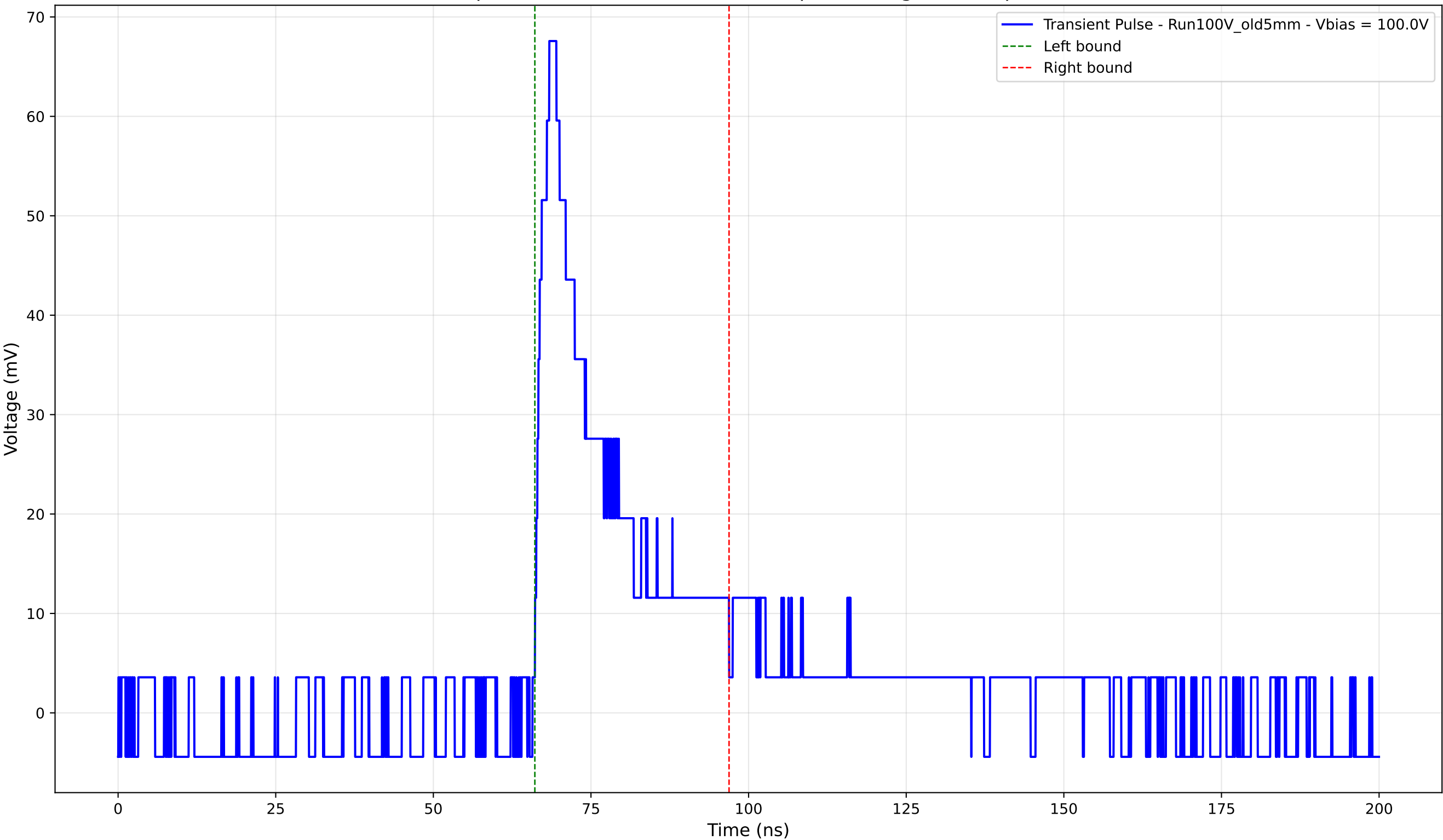
Transient Pulse - Sample: Old5mm - Position: 2990.0 \mu\text{m} - Charge: 14.86 pC - Rise Time: 2.27 ns
