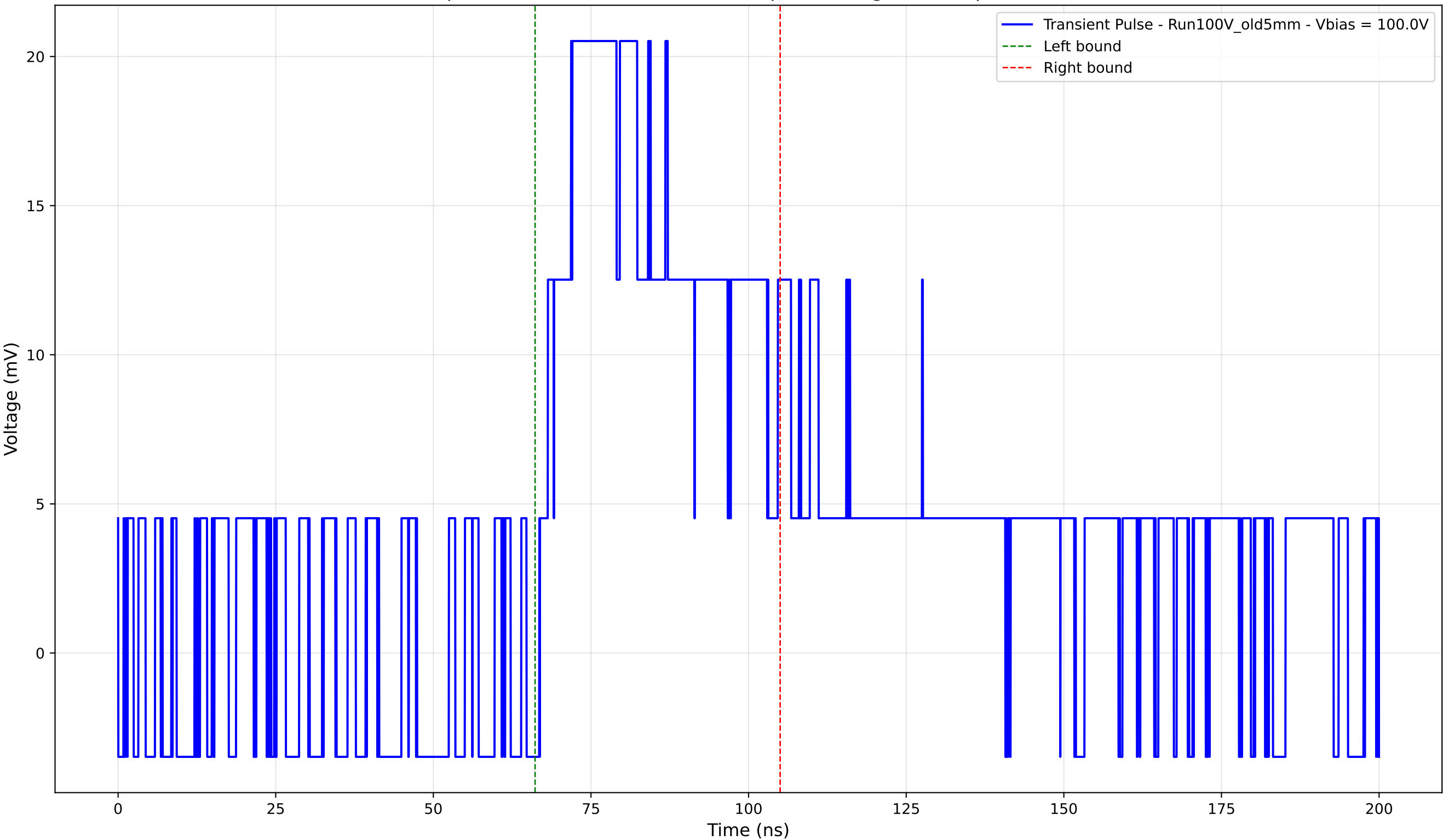
Transient Pulse - Sample: Old5mm - Position: 2005.0 \mu\text{m} - Charge: 10.64 pC - Rise Time: 0.00 ns (N/A)
