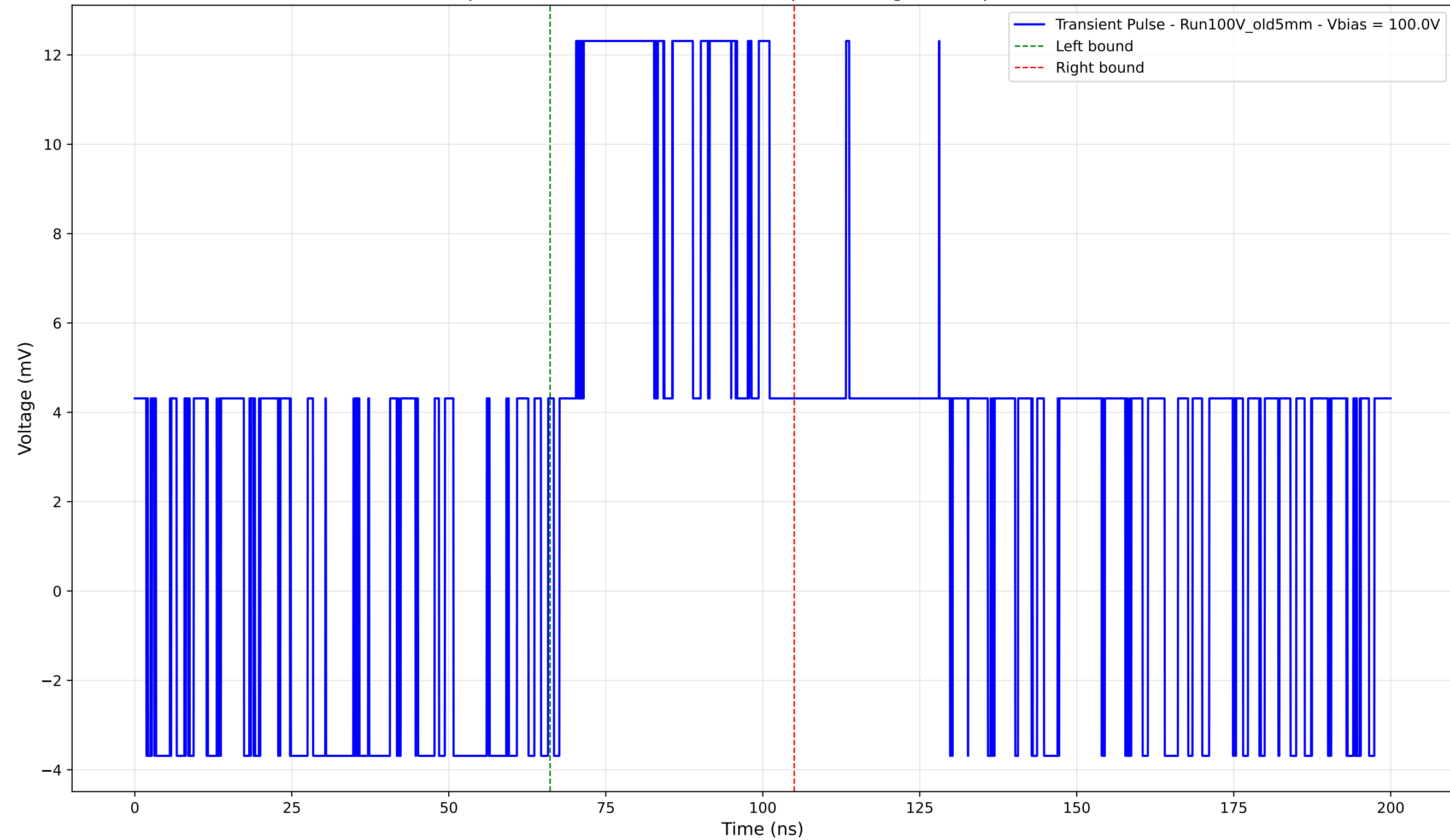
Transient Pulse - Sample: Old5mm - Position: 1860.0 \mu\text{m} - Charge: 7.01 pC - Rise Time: 0.00 ns (N/A)
