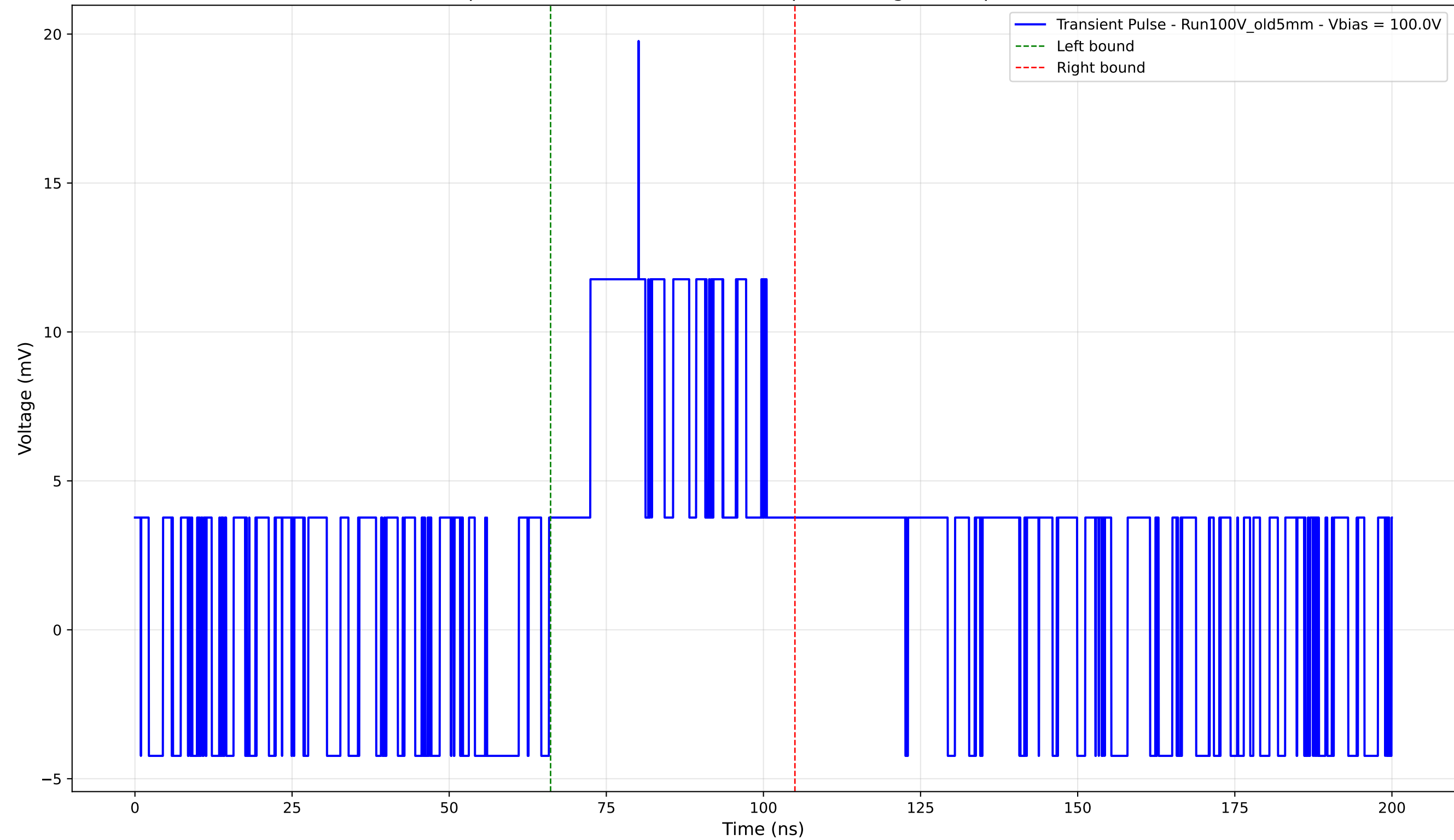
Transient Pulse - Sample: Old5mm - Position: 1250.0 \mu\text{m} - Charge: 5.99 pC - Rise Time: 0.00 ns (N/A)
