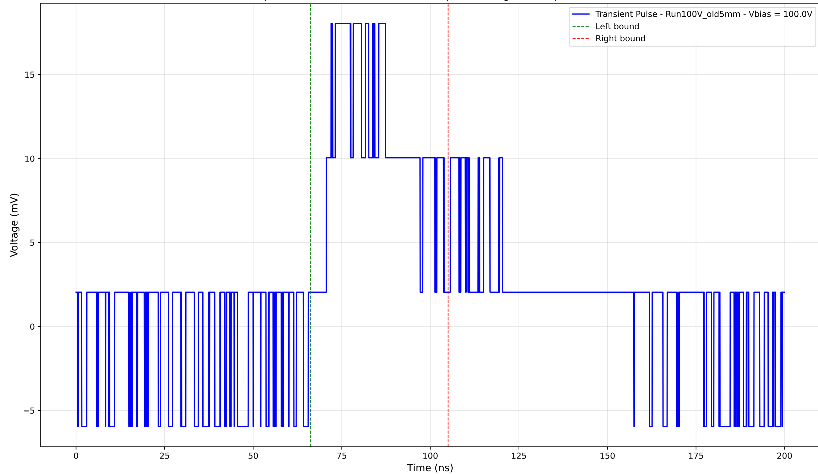
Transient Pulse - Sample: Old5mm - Position: 1825.0 \mu\text{m} - Charge: 8.34 pC - Rise Time: 0.00 ns (N/A)
