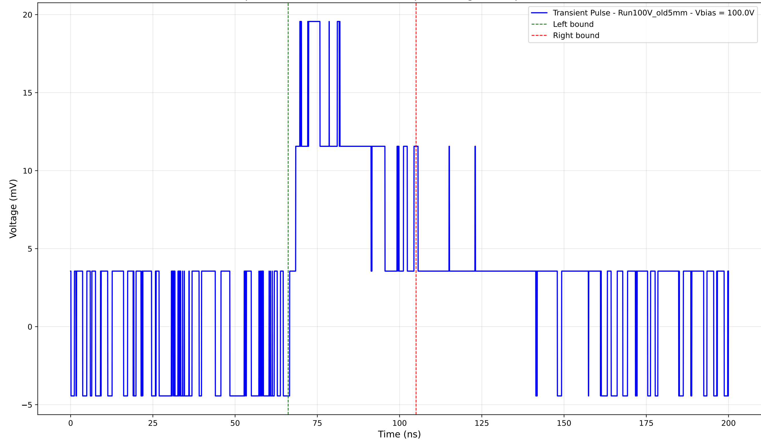
Transient Pulse - Sample: Old5mm - Position: 2260.0 \mu\text{m} - Charge: 8.14 pC - Rise Time: 0.00 ns (N/A)
