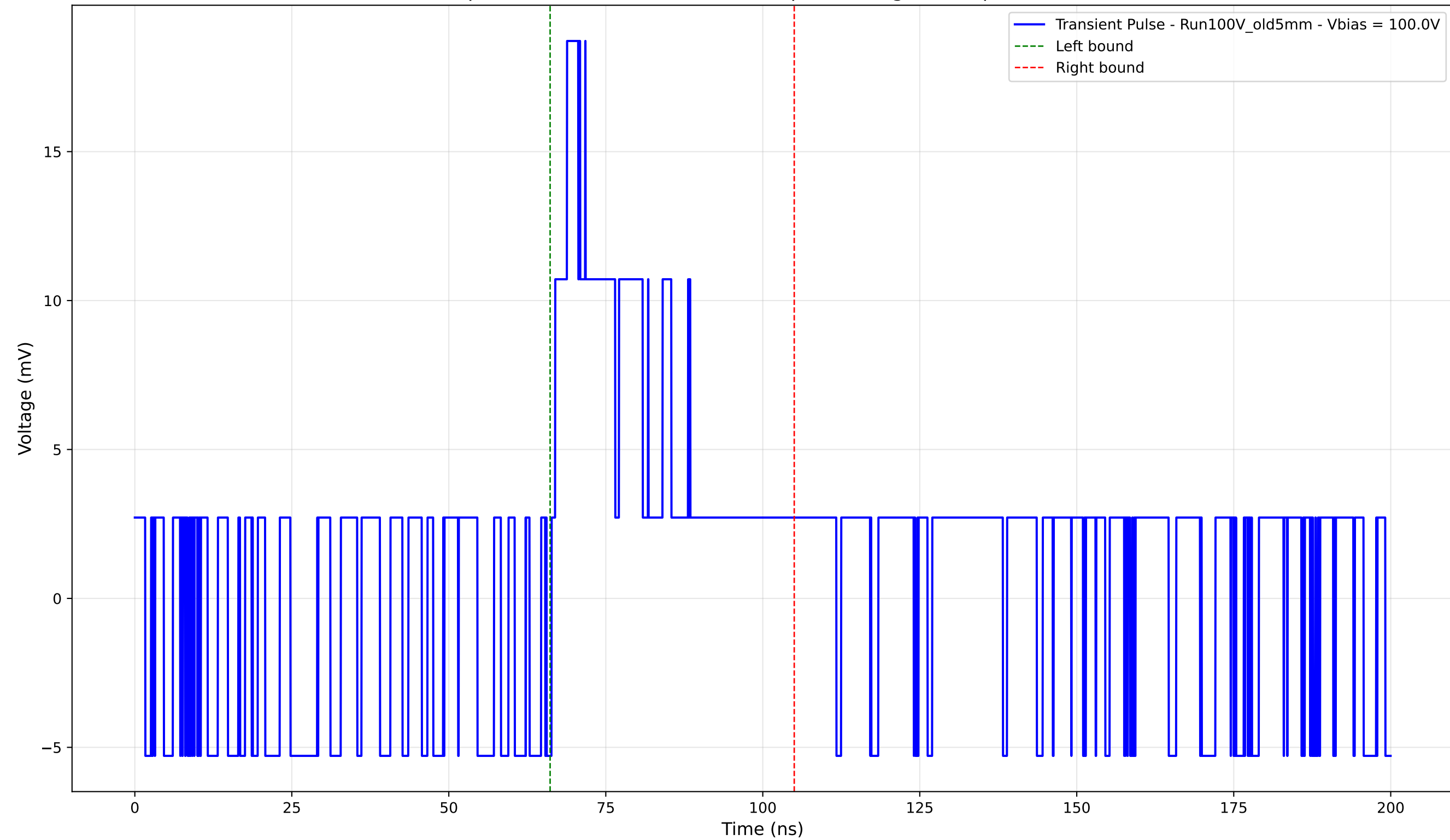
Transient Pulse - Sample: Old5mm - Position: 2735.0 \mu\text{m} - Charge: 4.81 pC - Rise Time: 0.00 ns (N/A)
