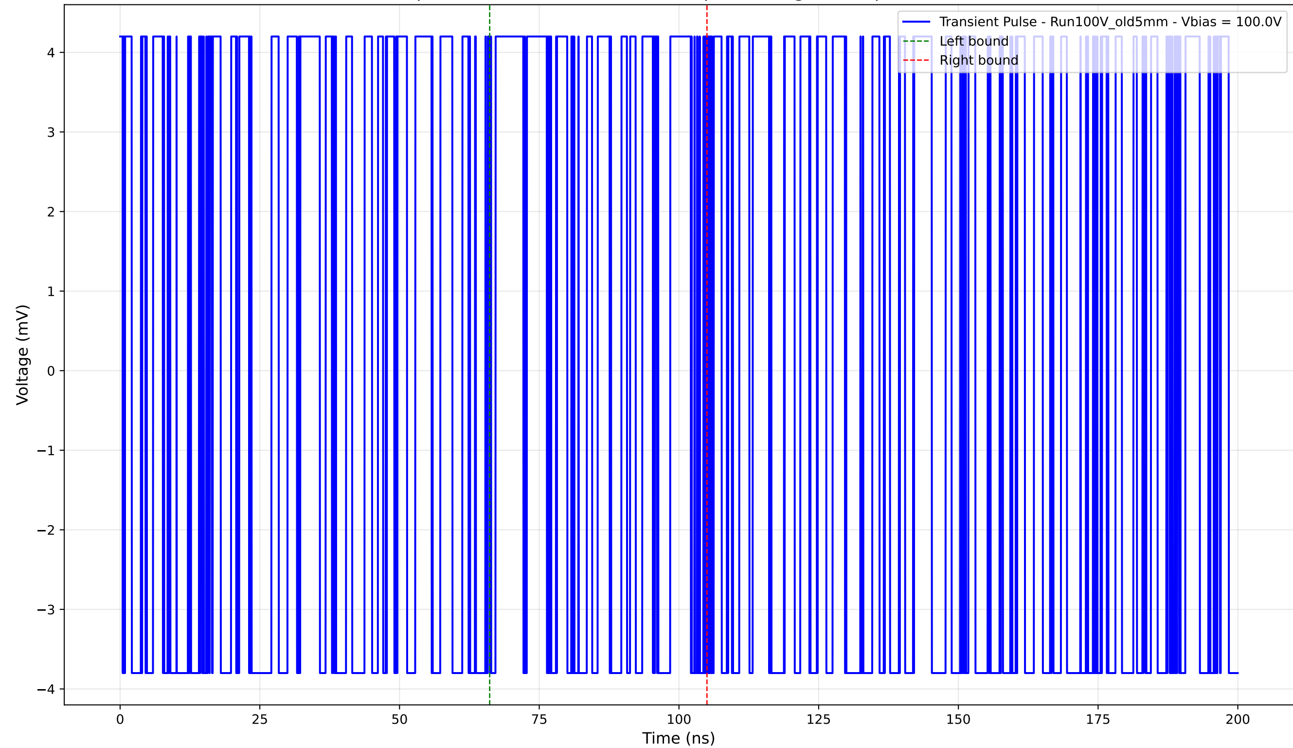
Transient Pulse - Sample: Old5mm - Position: 4600.0 \mu\text{m} - Charge: 0.77 pC - Rise Time: 0.00 ns (N/A)
