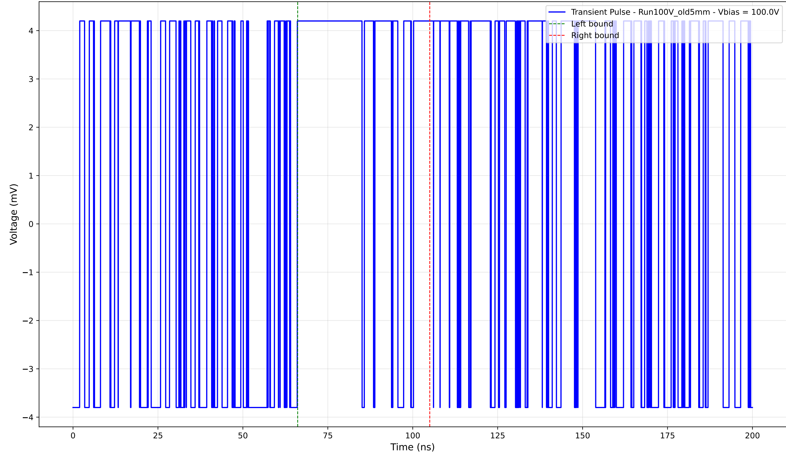
Transient Pulse - Sample: Old5mm - Position: 2535.0 \mu\text{m} - Charge: 2.67 pC - Rise Time: 0.00 ns (N/A)
