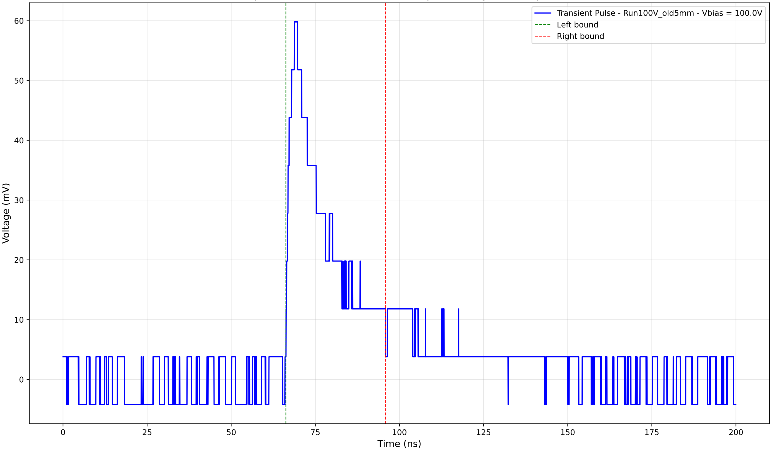
Transient Pulse - Sample: Old5mm - Position: 2915.0 \mu\text{m} - Charge: 14.70 pC - Rise Time: 2.47 ns
