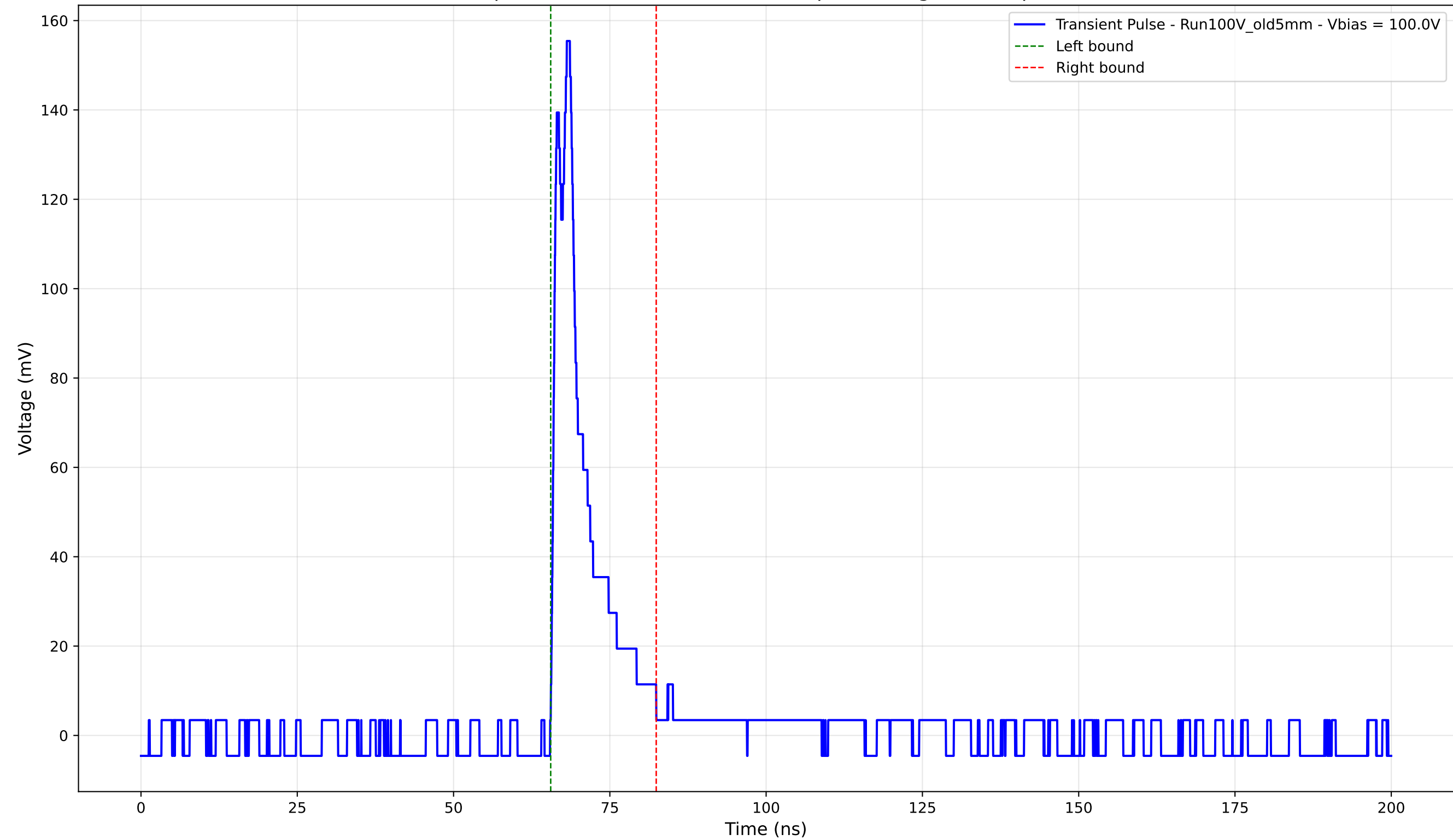
Transient Pulse - Sample: Old5mm - Position: 3510.0 \mu\text{m} - Charge: 17.15 pC - Rise Time: 2.33 ns
