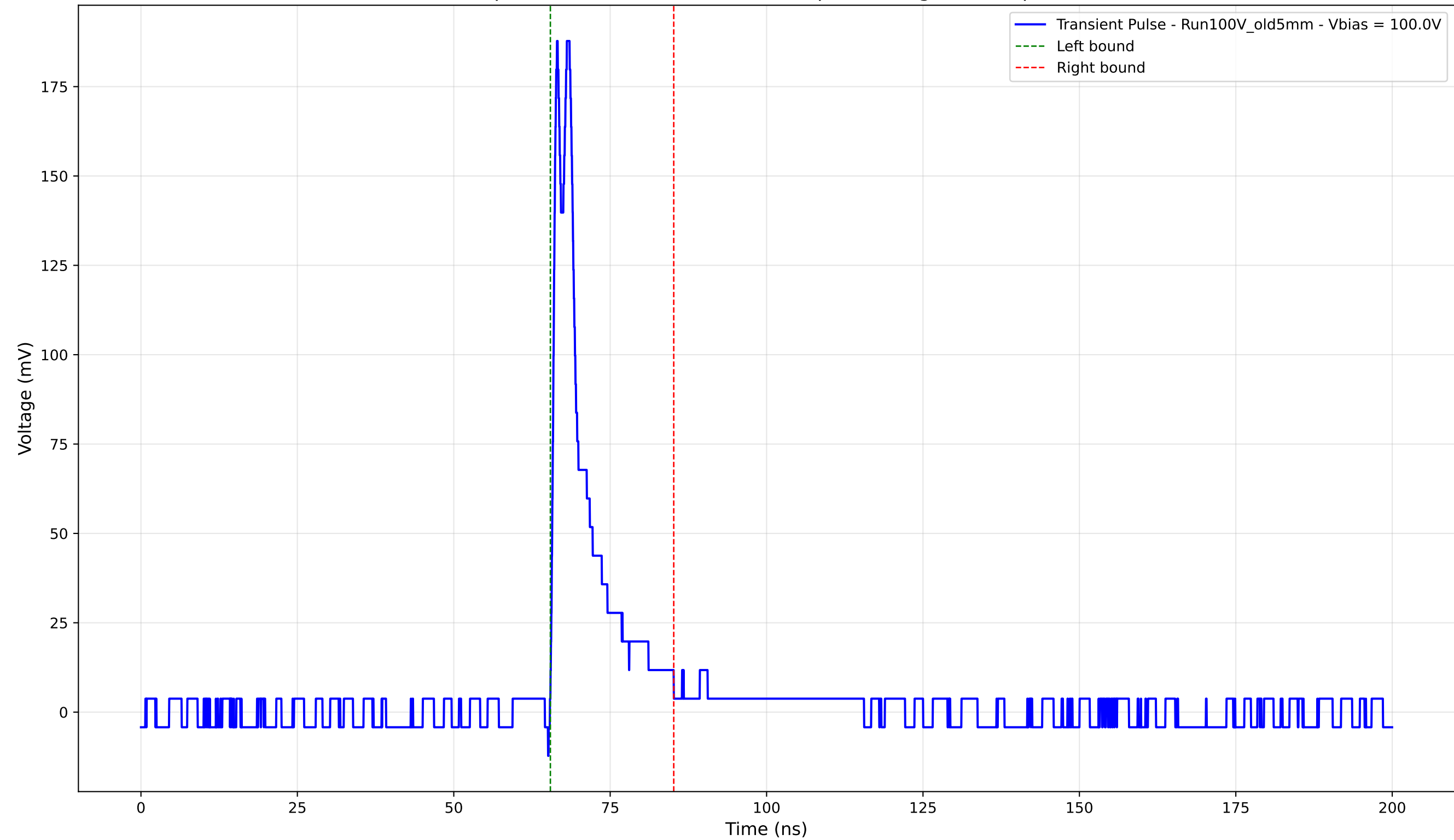
Transient Pulse - Sample: Old5mm - Position: 3860.0 \mu\text{m} - Charge: 20.93 pC - Rise Time: 0.78 ns
