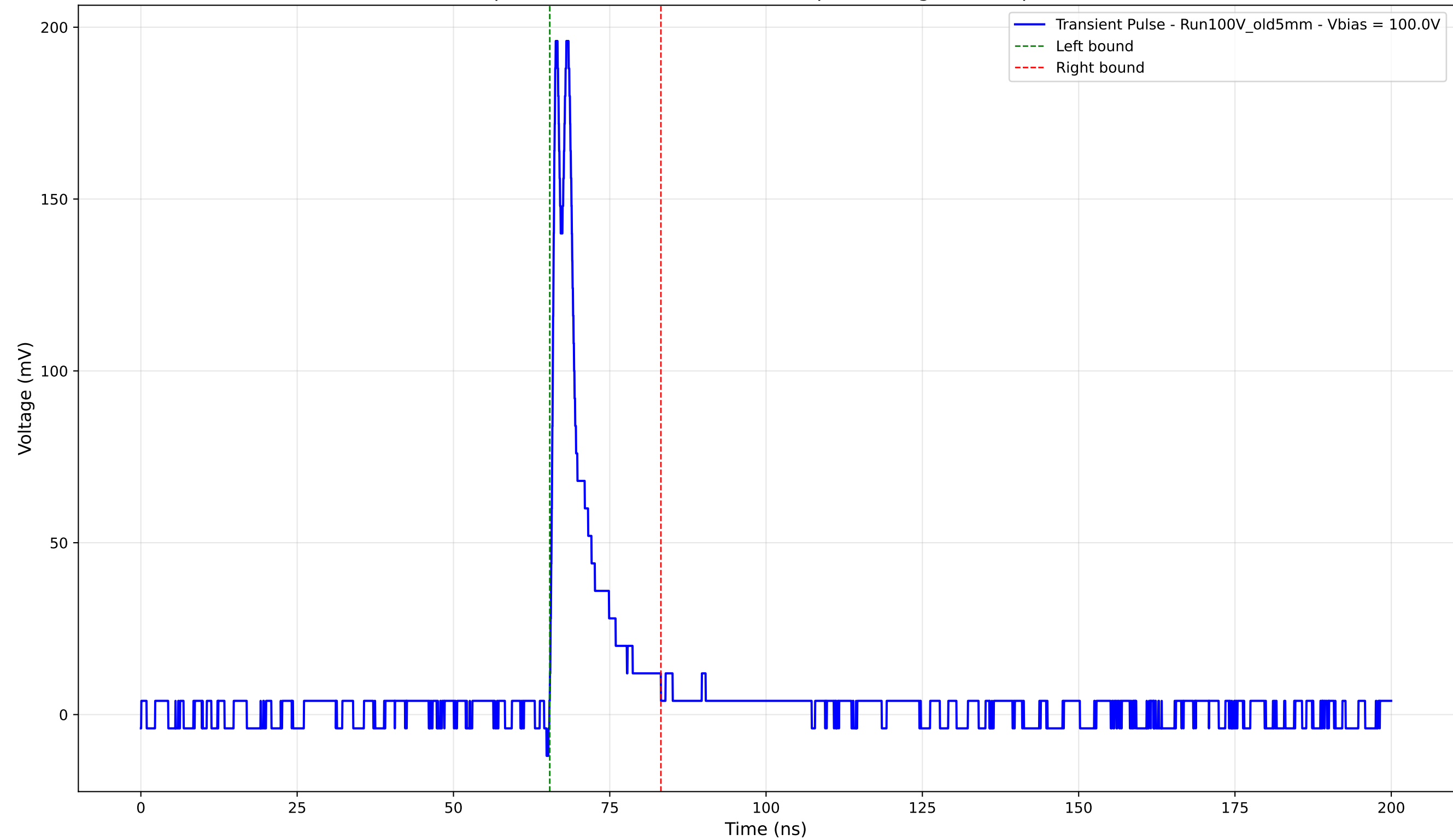
Transient Pulse - Sample: Old5mm - Position: 3835.0 \mu\text{m} - Charge: 20.16 pC - Rise Time: 0.74 ns
