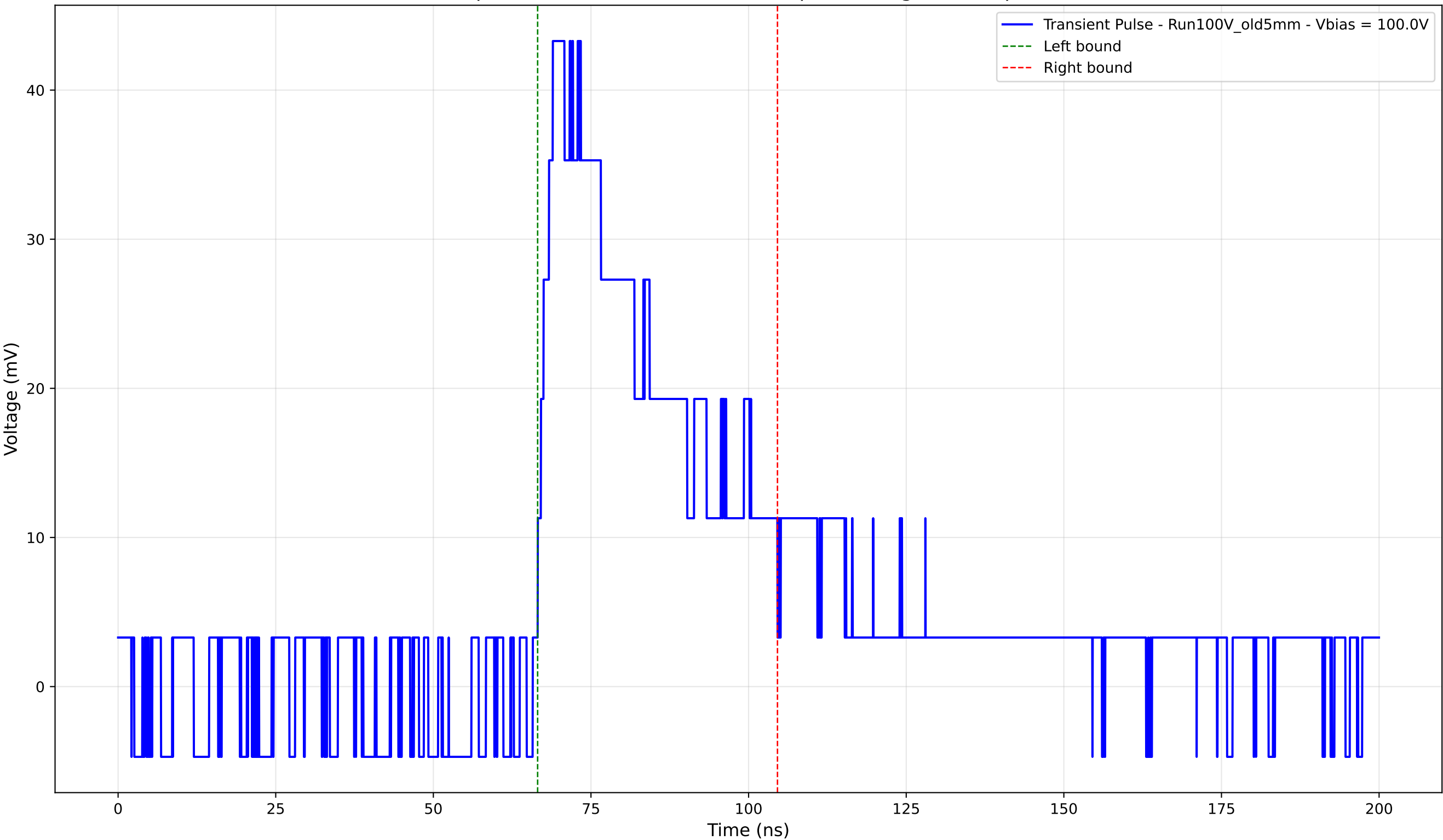
Transient Pulse - Sample: Old5mm - Position: 4890.0 \mu\text{m} - Charge: 17.04 pC - Rise Time: 2.40 ns
