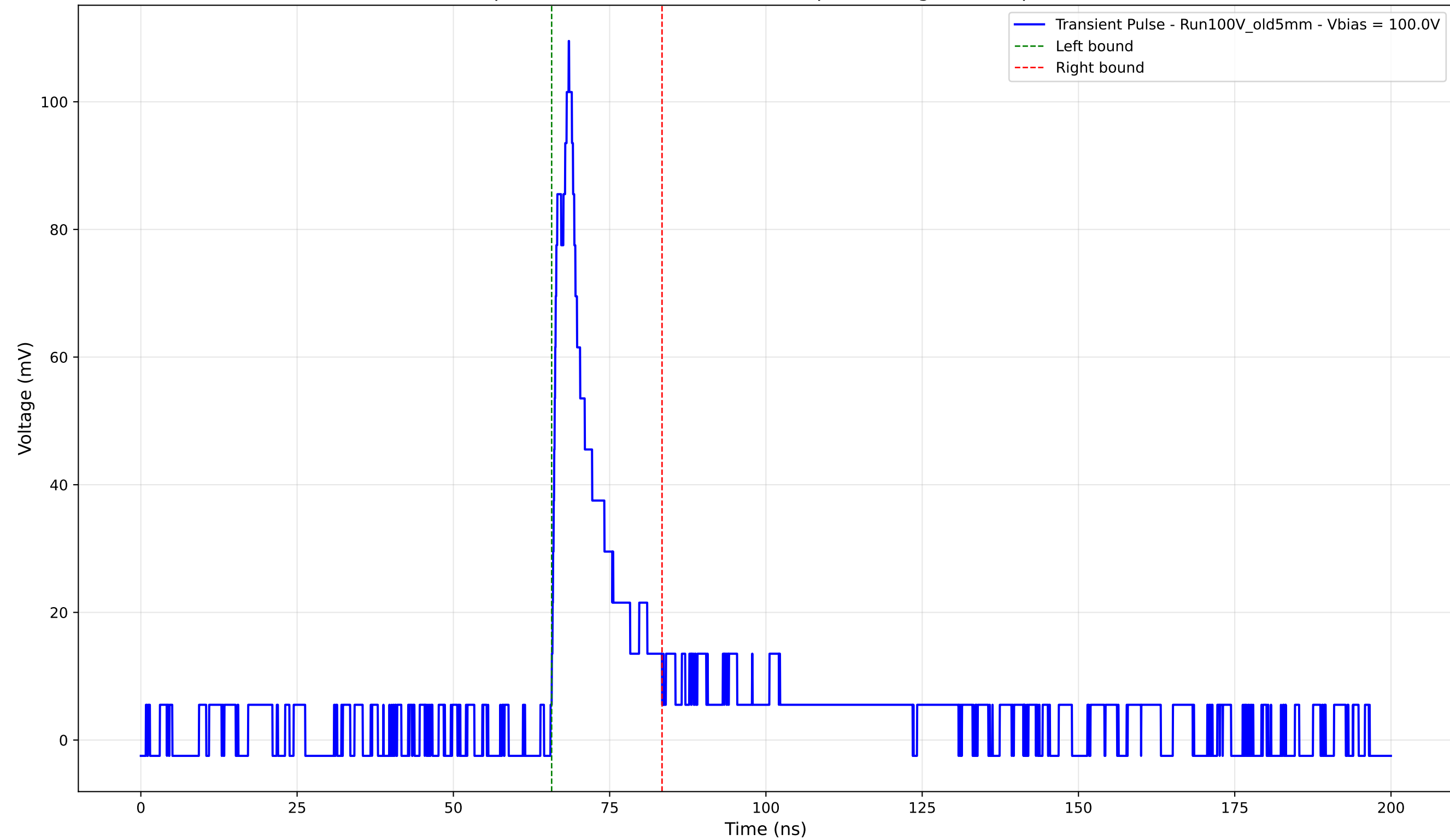
Transient Pulse - Sample: Old5mm - Position: 3310.0 \mu\text{m} - Charge: 13.95 pC - Rise Time: 2.39 ns
