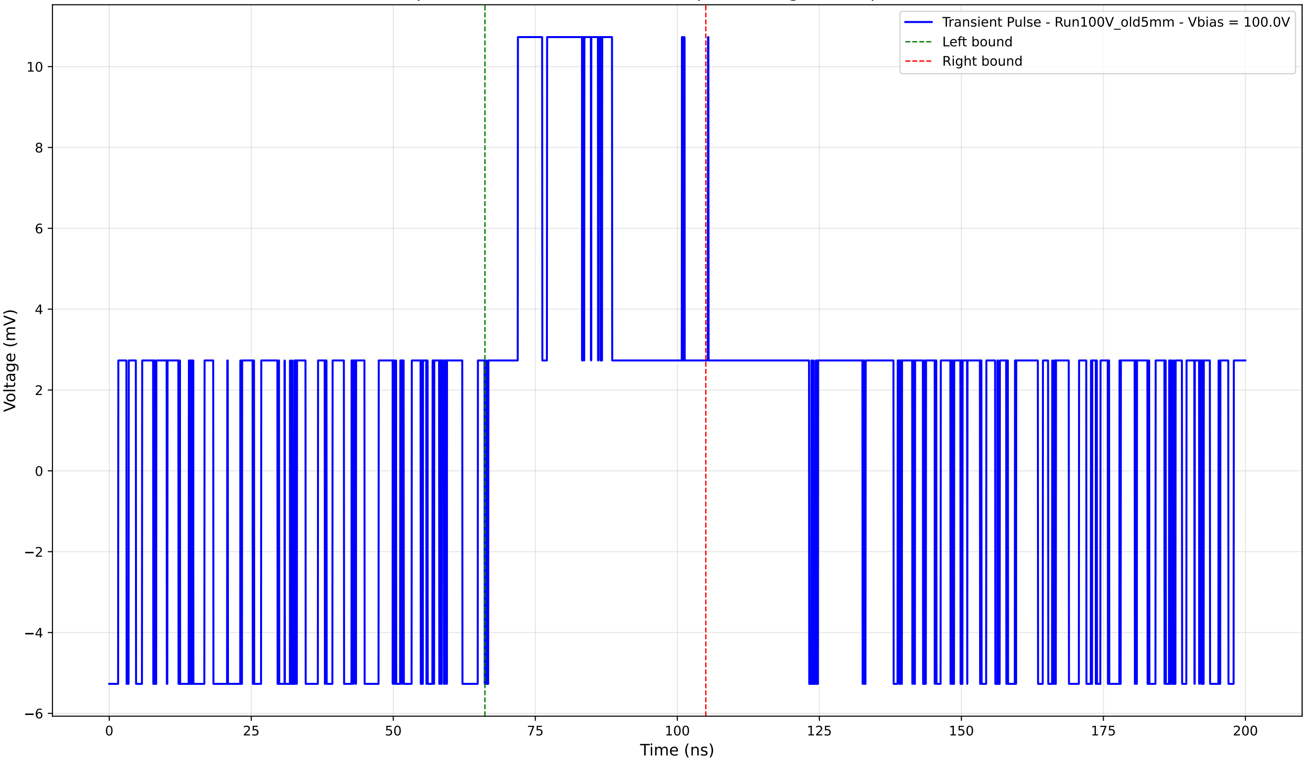
Transient Pulse - Sample: Old5mm - Position: 790.0 \mu\text{m} - Charge: 4.52 pC - Rise Time: 0.00 ns (N/A)
