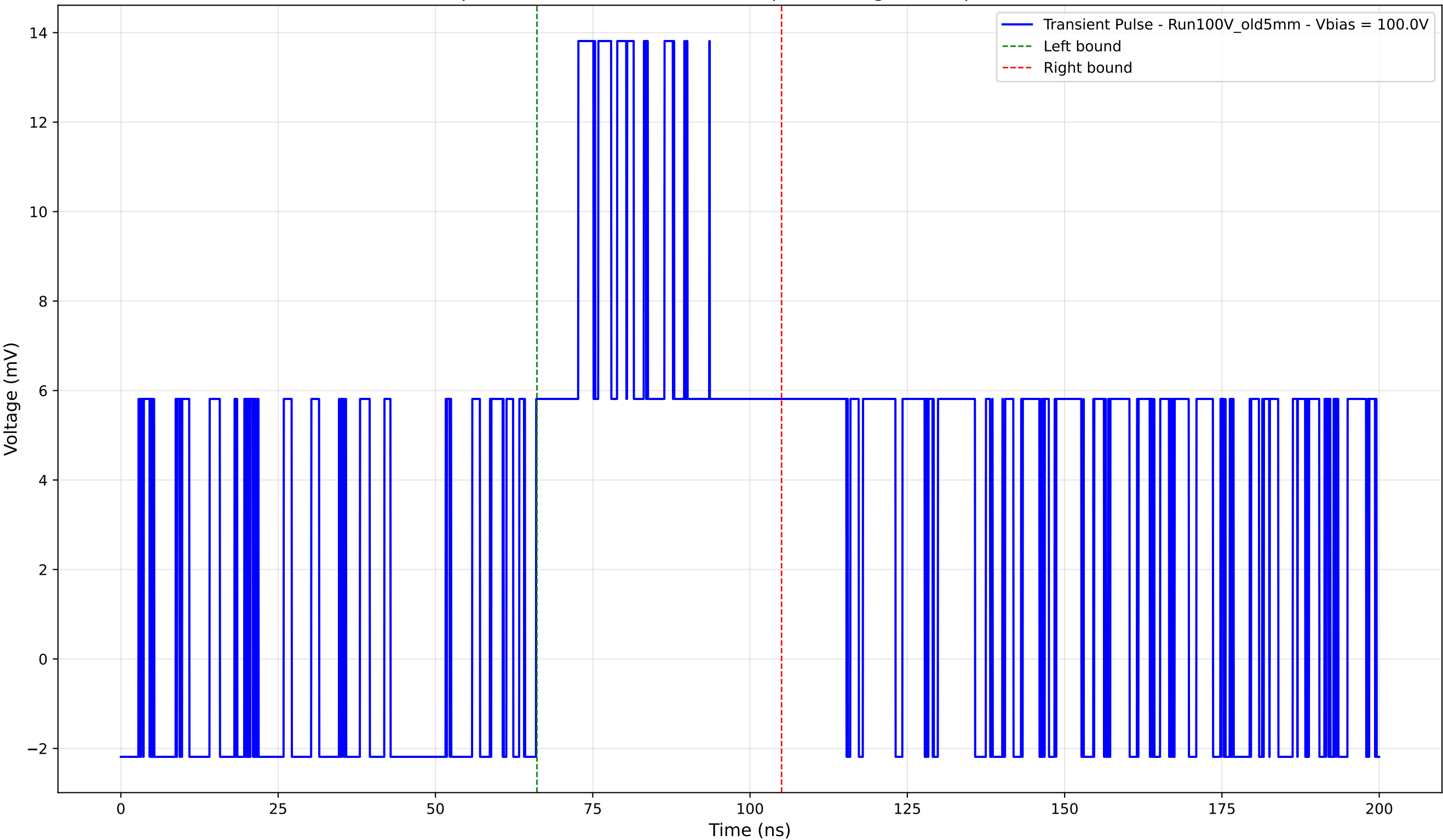
Transient Pulse - Sample: Old5mm - Position: 595.0 \mu\text{m} - Charge: 6.01 pC - Rise Time: 0.00 ns (N/A)
