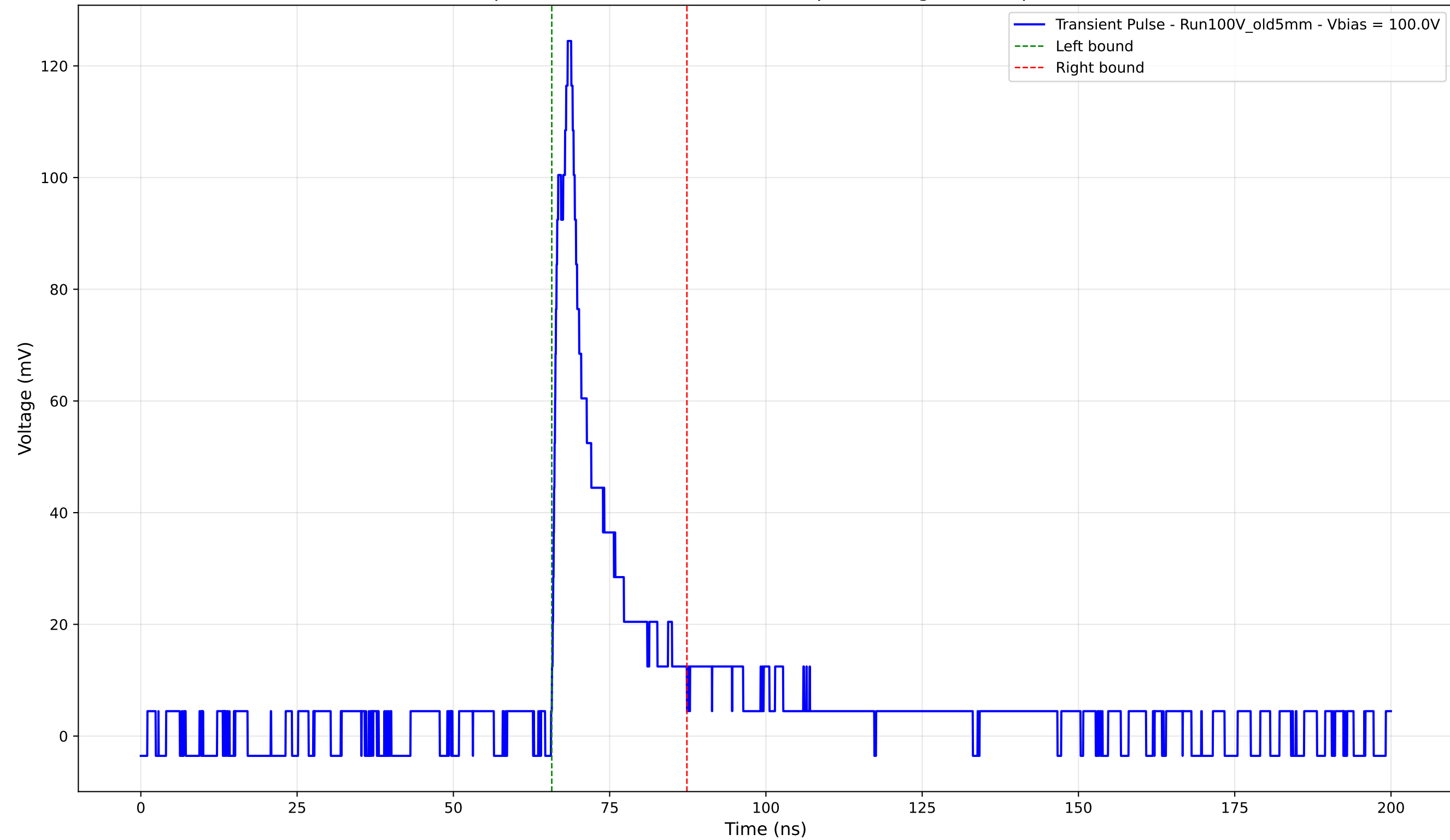
Transient Pulse - Sample: Old5mm - Position: 3280.0 \mu\text{m} - Charge: 17.64 pC - Rise Time: 2.28 ns
