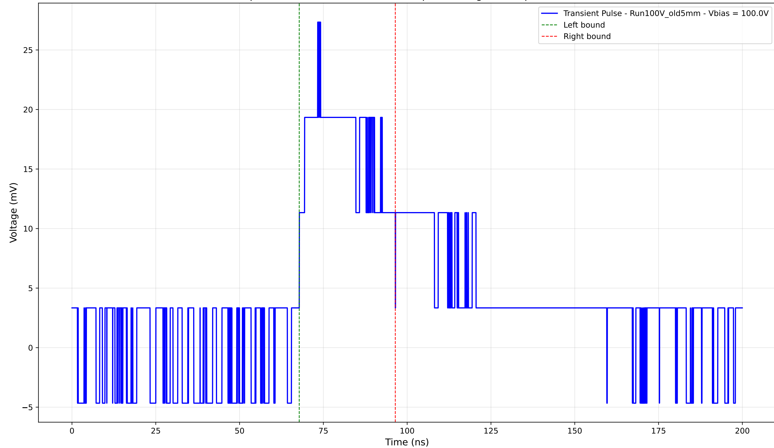
Transient Pulse - Sample: Old5mm - Position: 2240.0 \mu\text{m} - Charge: 9.65 pC - Rise Time: 0.00 ns (N/A)
