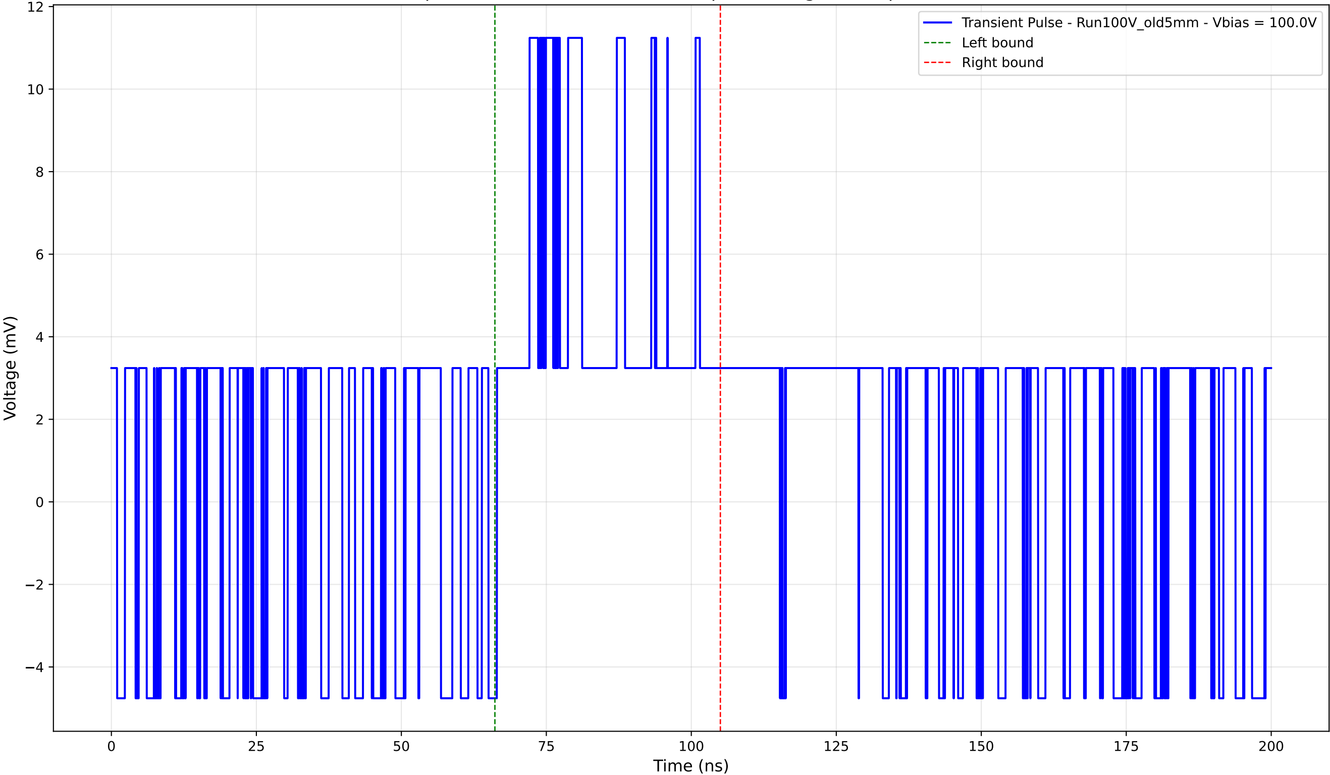
Transient Pulse - Sample: Old5mm - Position: 705.0 \mu\text{m} - Charge: 4.01 pC - Rise Time: 0.00 ns (N/A)
