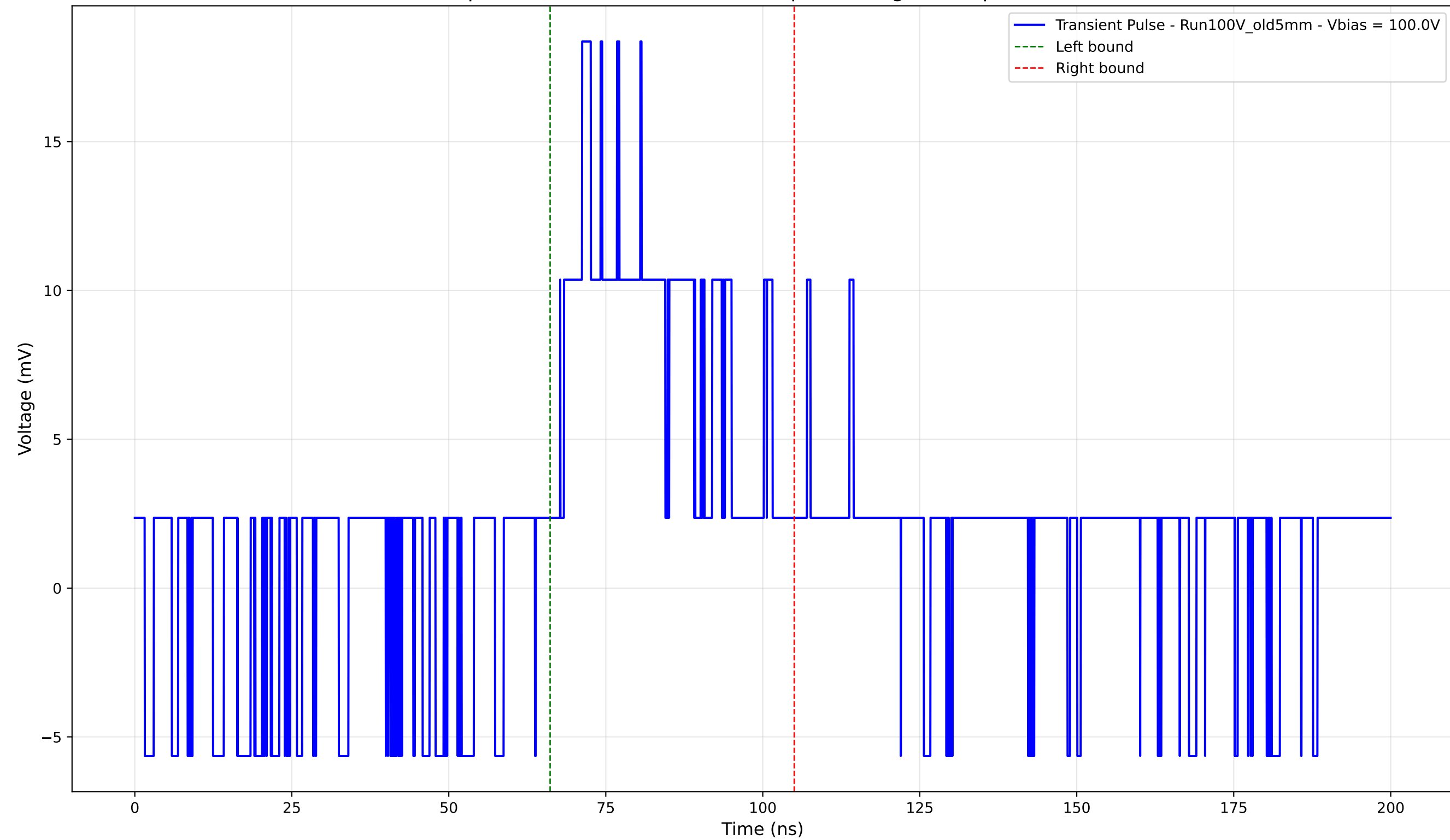
Transient Pulse - Sample: Old5mm - Position: 2265.0 \mu\text{m} - Charge: 6.16 pC - Rise Time: 0.00 ns (N/A)
