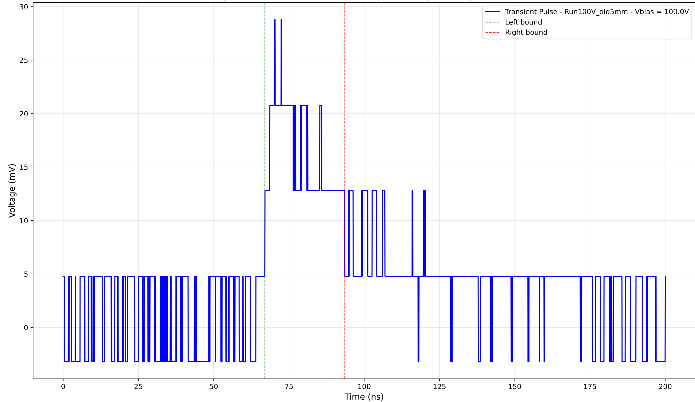
Transient Pulse - Sample: Old5mm - Position: 4995.0 \mu\text{m} - Charge: 8.55 pC - Rise Time: 0.00 ns (N/A)
