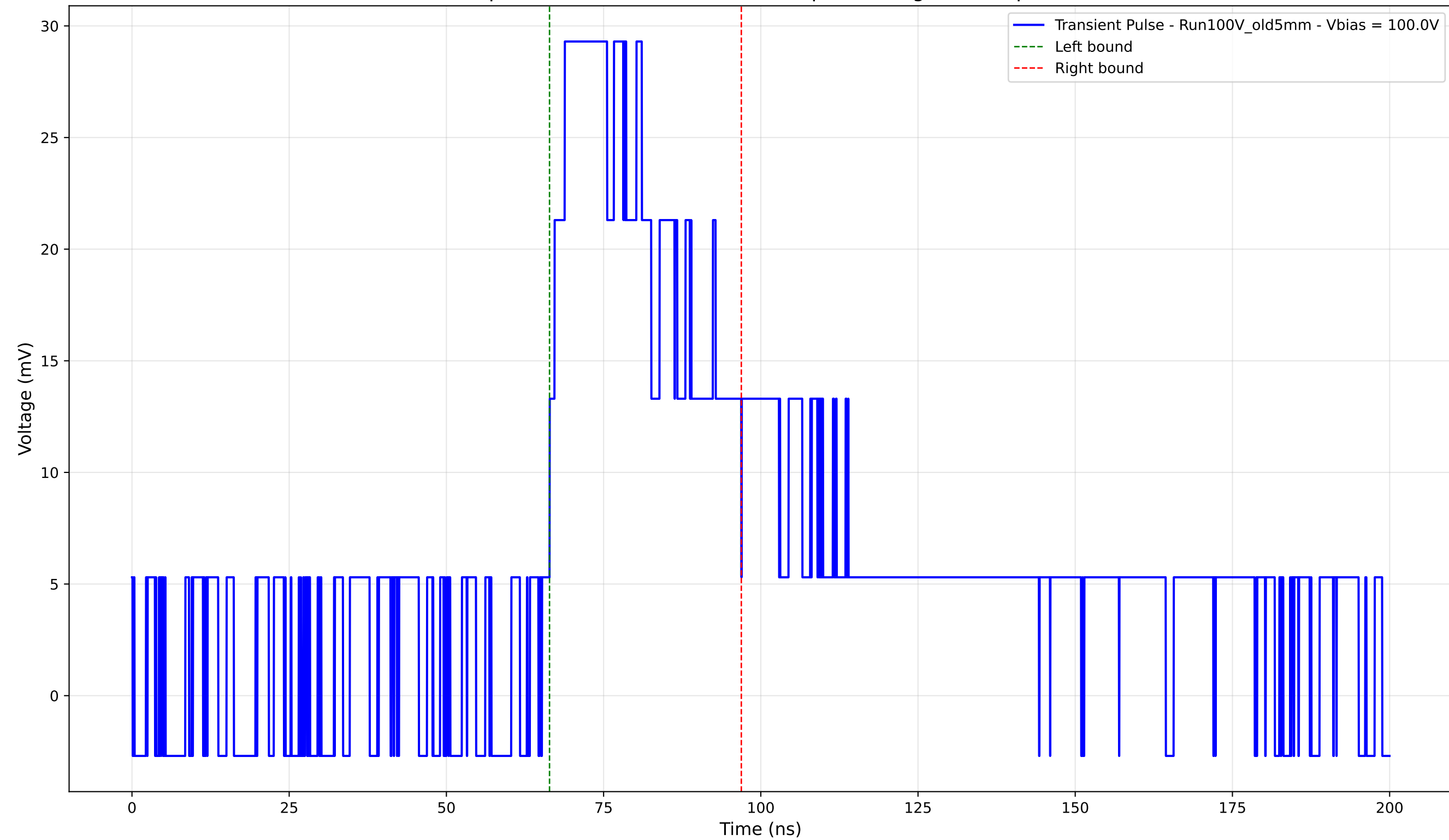
Transient Pulse - Sample: Old5mm - Position: 4980.0 \mu\text{m} - Charge: 12.71 pC - Rise Time: 3.64 ns
