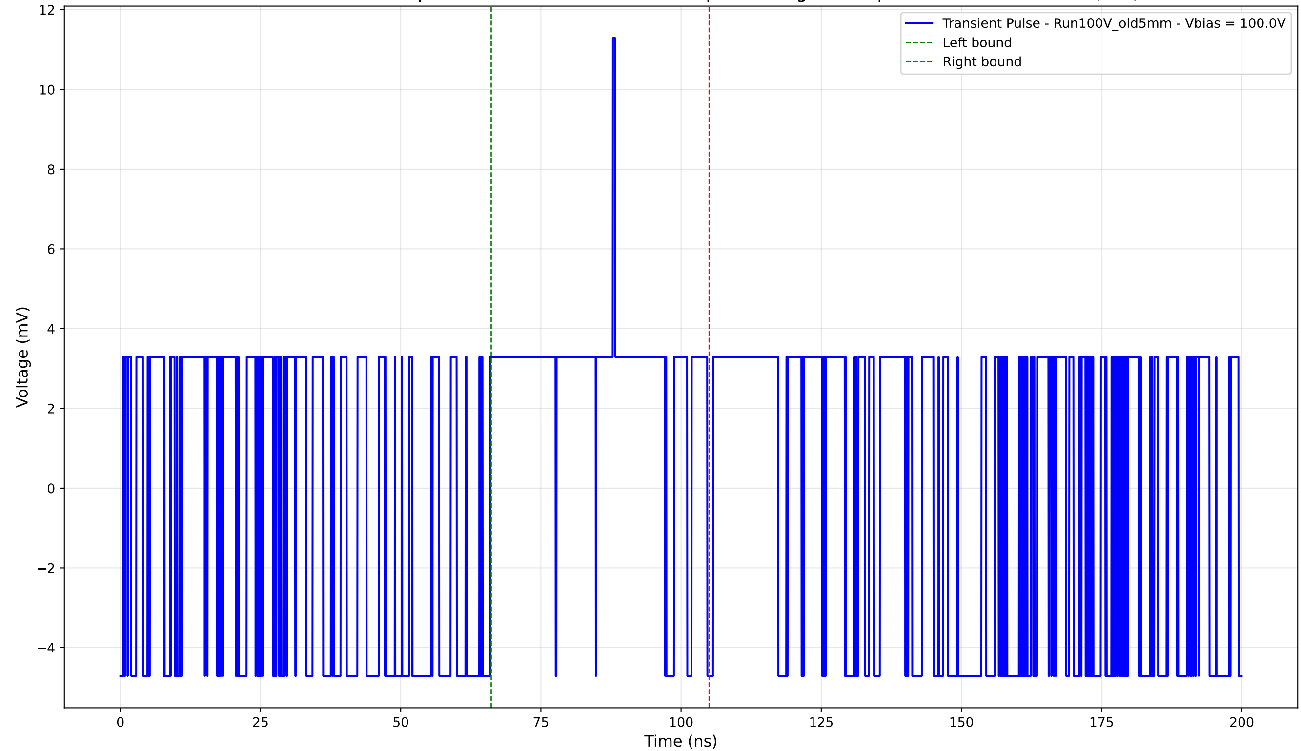
Transient Pulse - Sample: Old5mm - Position: 2300.0 \mu\text{m} - Charge: 2.19 pC - Rise Time: 0.00 ns (N/A)
