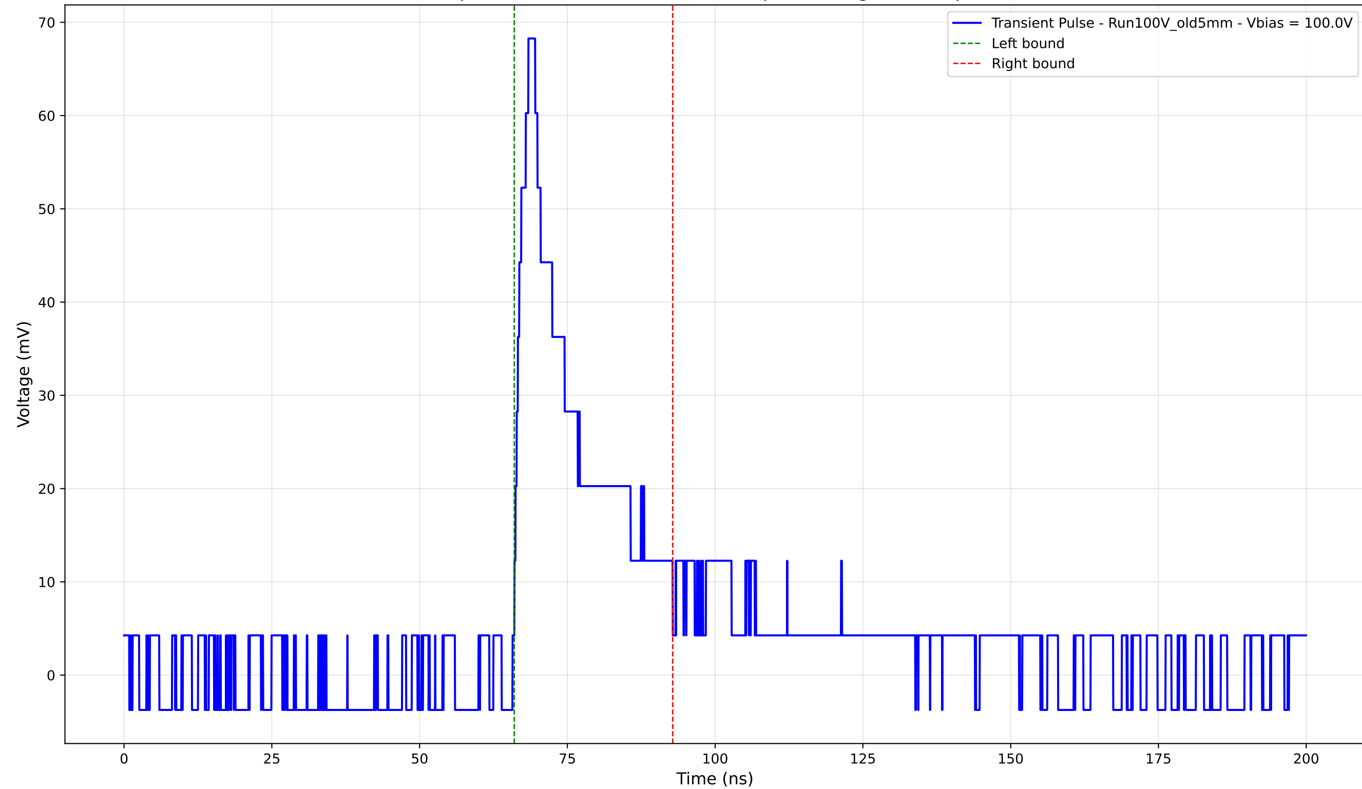
Transient Pulse - Sample: Old5mm - Position: 2995.0 \mu\text{m} - Charge: 14.63 pC - Rise Time: 2.37 ns
