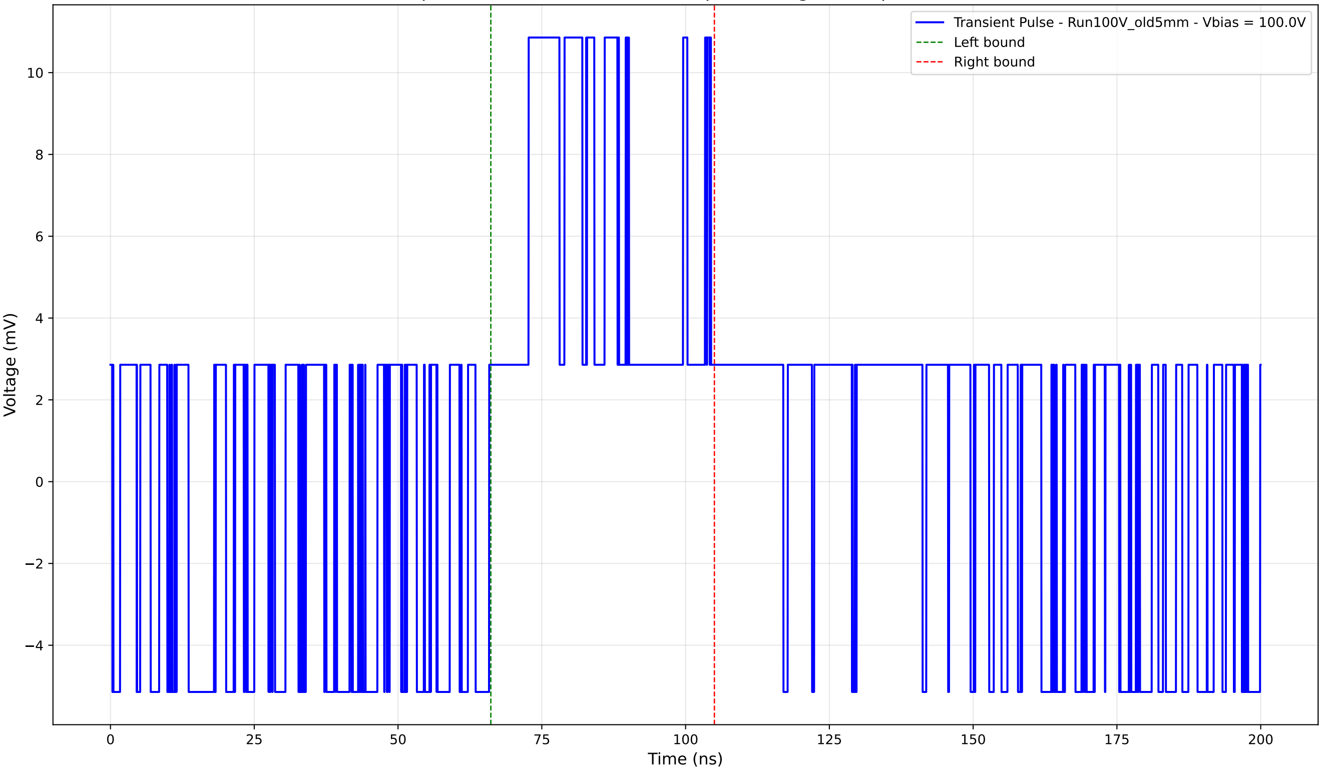
Transient Pulse - Sample: Old5mm - Position: 890.0 \mu\text{m} - Charge: 4.46 pC - Rise Time: 0.00 ns (N/A)
