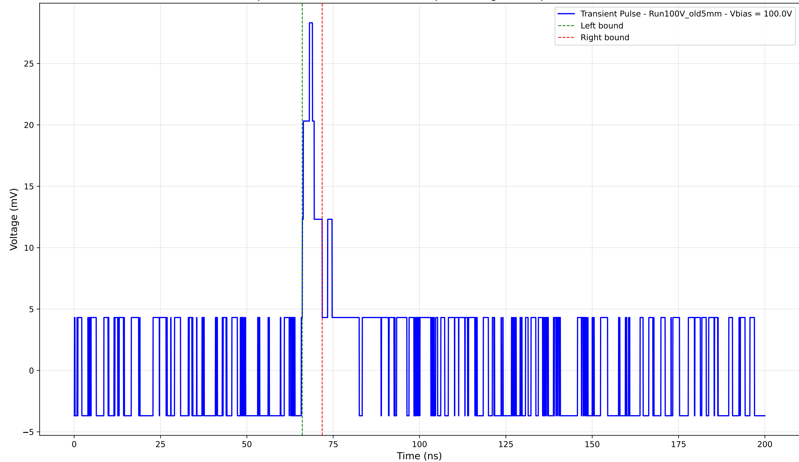
Transient Pulse - Sample: Old5mm - Position: 3365.0 \mu\text{m} - Charge: 2.07 pC - Rise Time: 0.00 ns (N/A)
