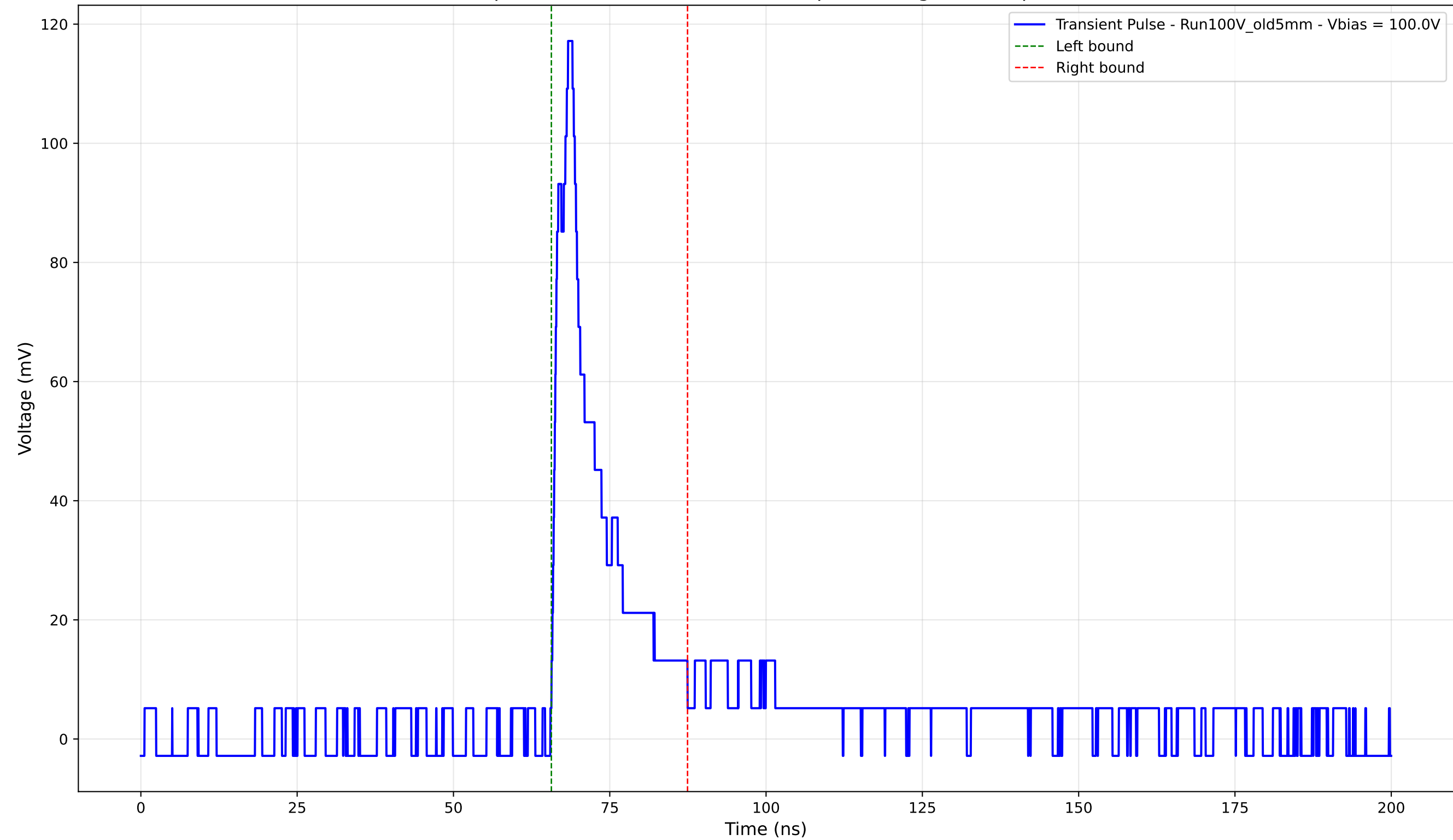
Transient Pulse - Sample: Old5mm - Position: 4150.0 \mu\text{m} - Charge: 17.26 pC - Rise Time: 2.44 ns
