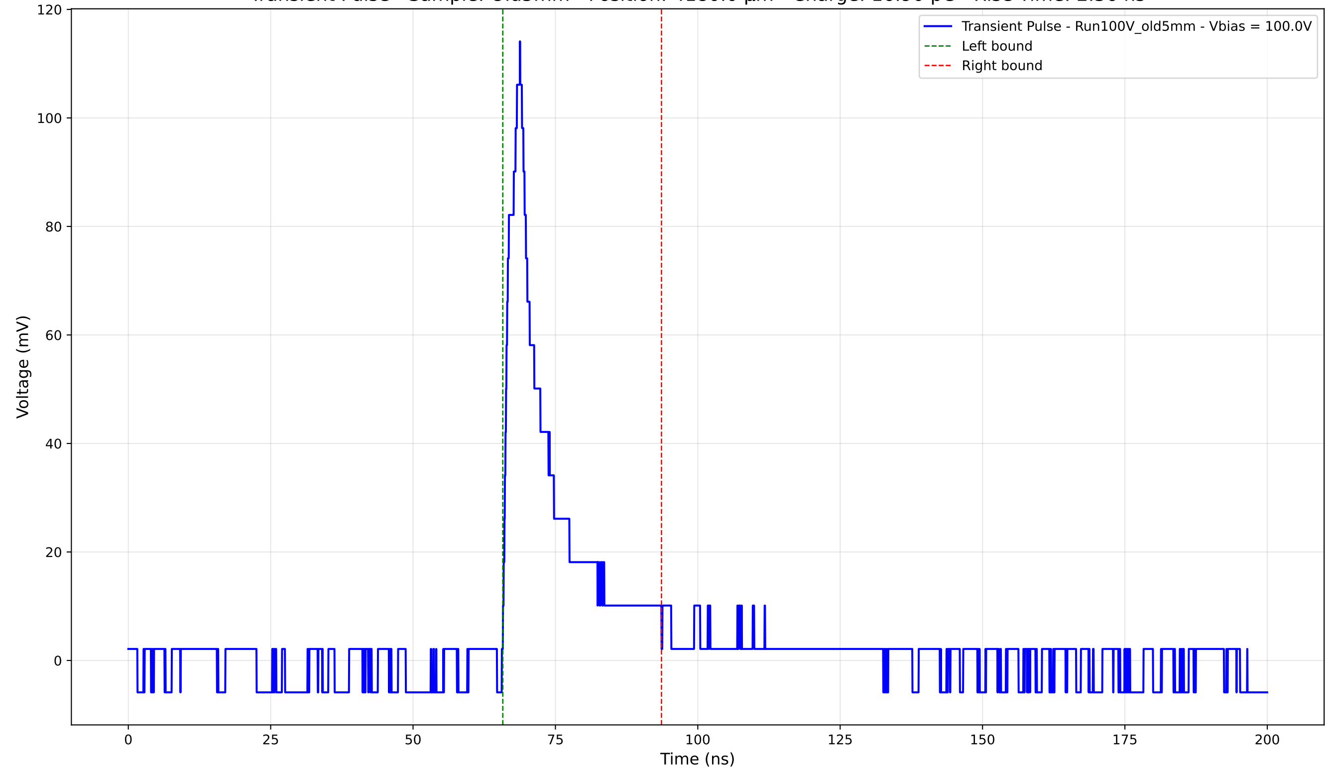
Transient Pulse - Sample: Old5mm - Position: 4180.0 \mu\text{m} - Charge: 16.90 pC - Rise Time: 2.36 ns
