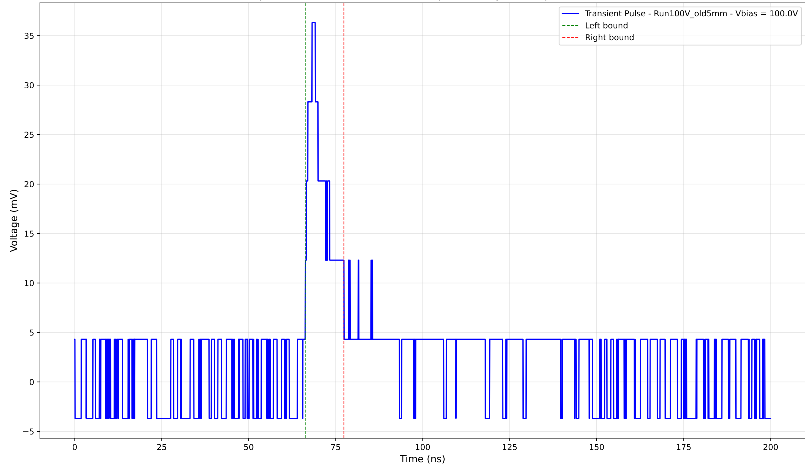
Transient Pulse - Sample: Old5mm - Position: 3160.0 \mu\text{m} - Charge: 4.35 pC - Rise Time: 0.00 ns (N/A)
