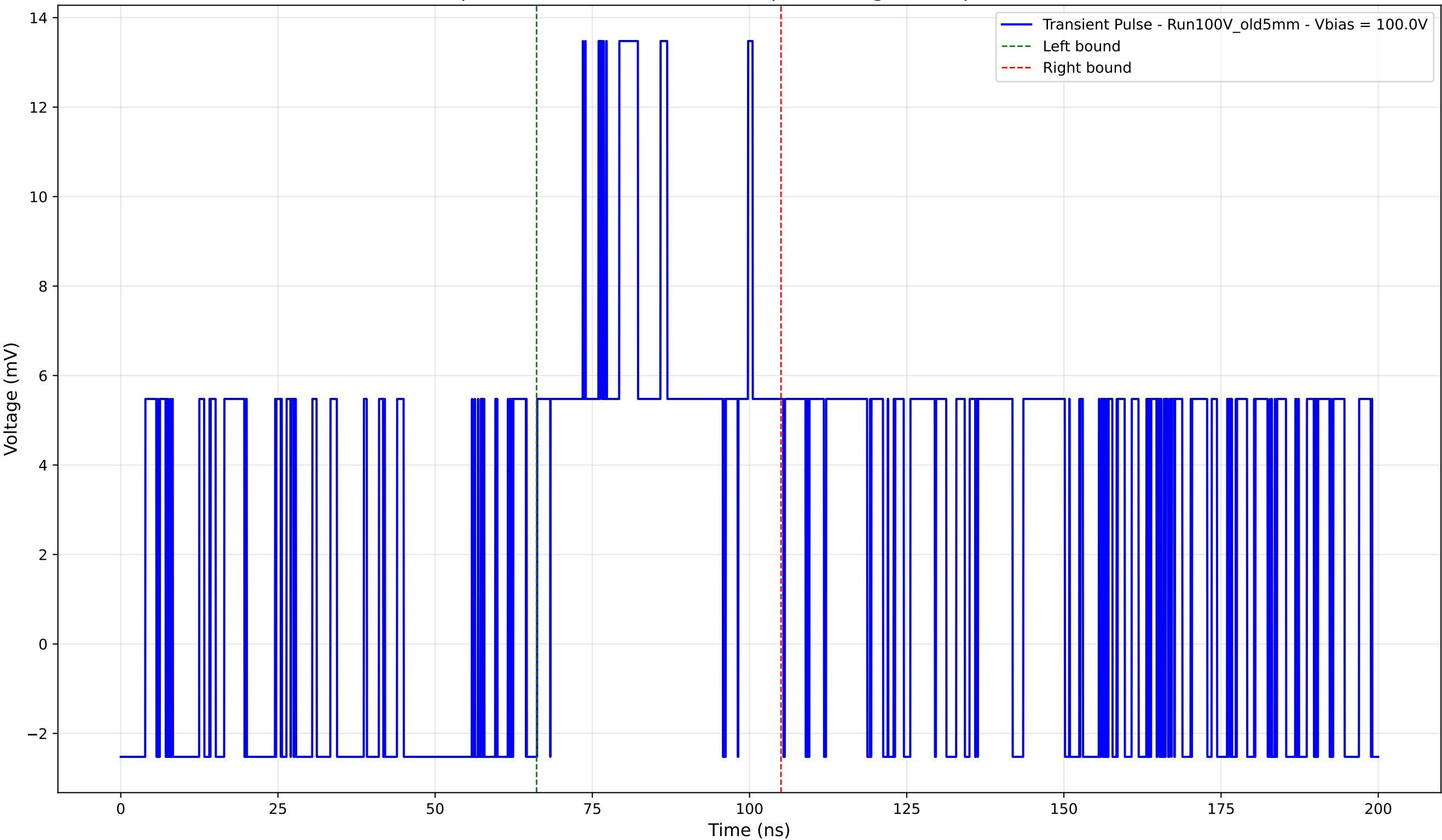
Transient Pulse - Sample: Old5mm - Position: 740.0 \mu\text{m} - Charge: 5.05 pC - Rise Time: 0.00 ns (N/A)
