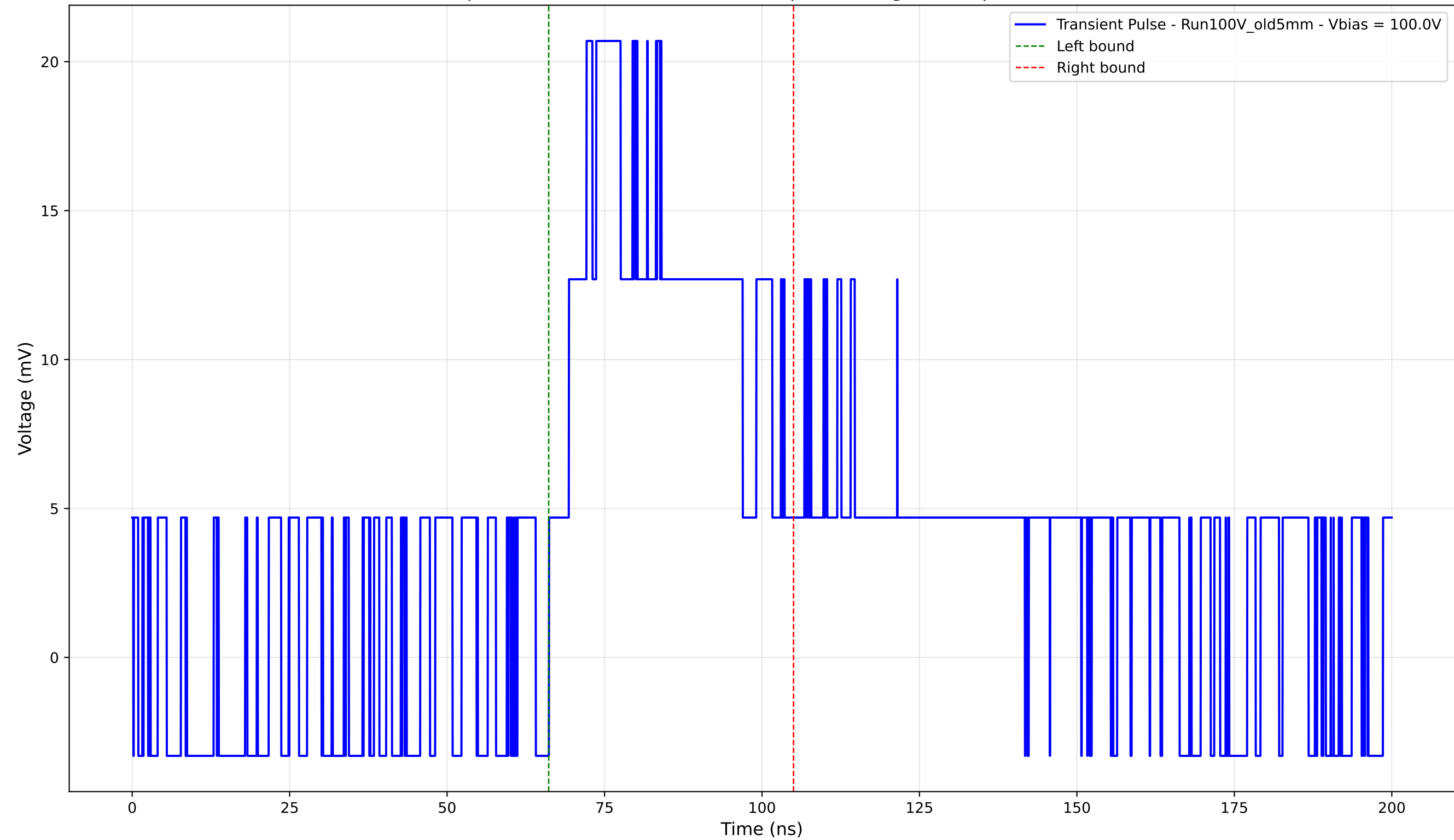
Transient Pulse - Sample: Old5mm - Position: 2050.0 \mu\text{m} - Charge: 9.53 pC - Rise Time: 0.00 ns (N/A)
