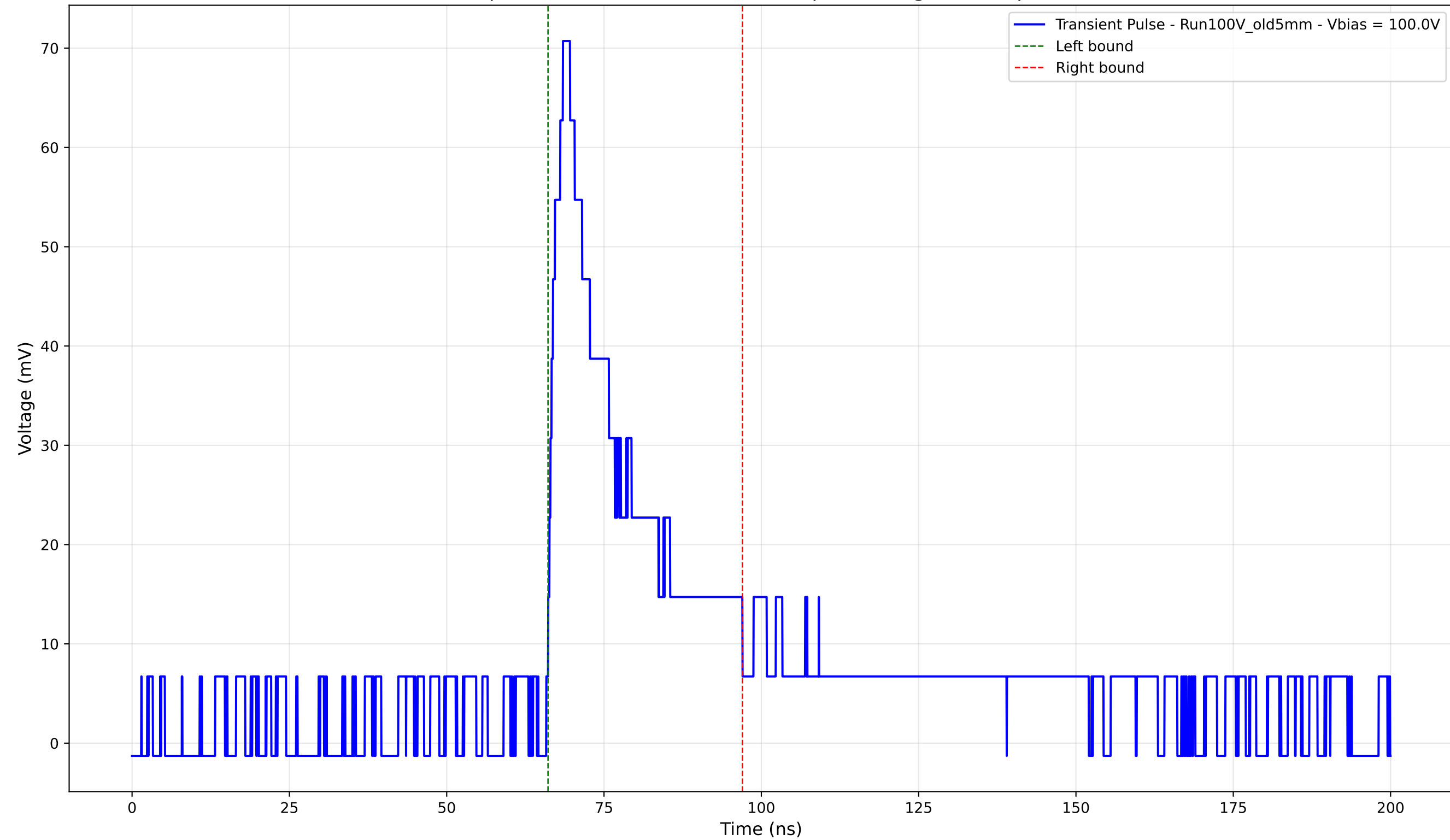
Transient Pulse - Sample: Old5mm - Position: 4460.0 \mu\text{m} - Charge: 17.53 pC - Rise Time: 2.36 ns
