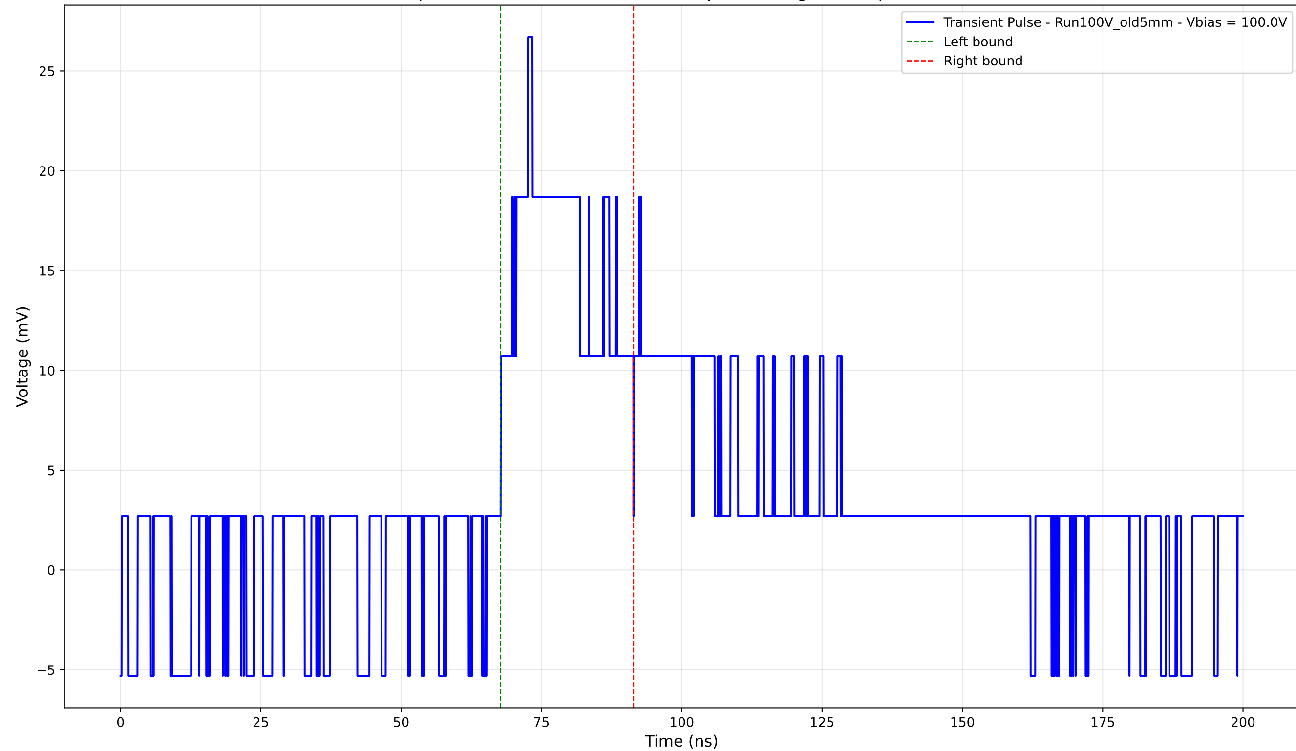
Transient Pulse - Sample: Old5mm - Position: 2190.0 \mu\text{m} - Charge: 7.26 pC - Rise Time: 0.00 ns (N/A)
