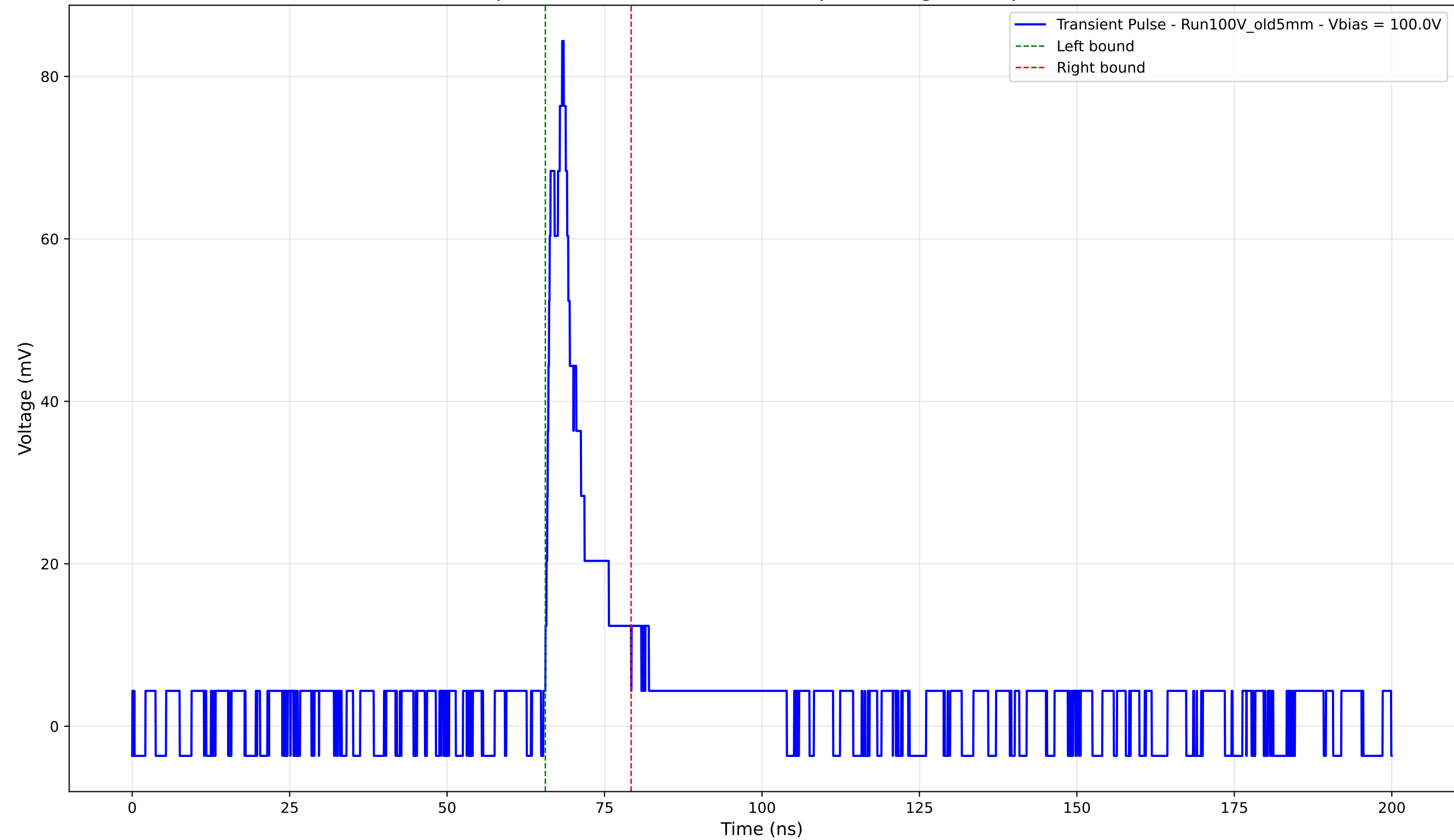
Transient Pulse - Sample: Old5mm - Position: 3475.0 \mu\text{m} - Charge: 8.97 pC - Rise Time: 2.29 ns
