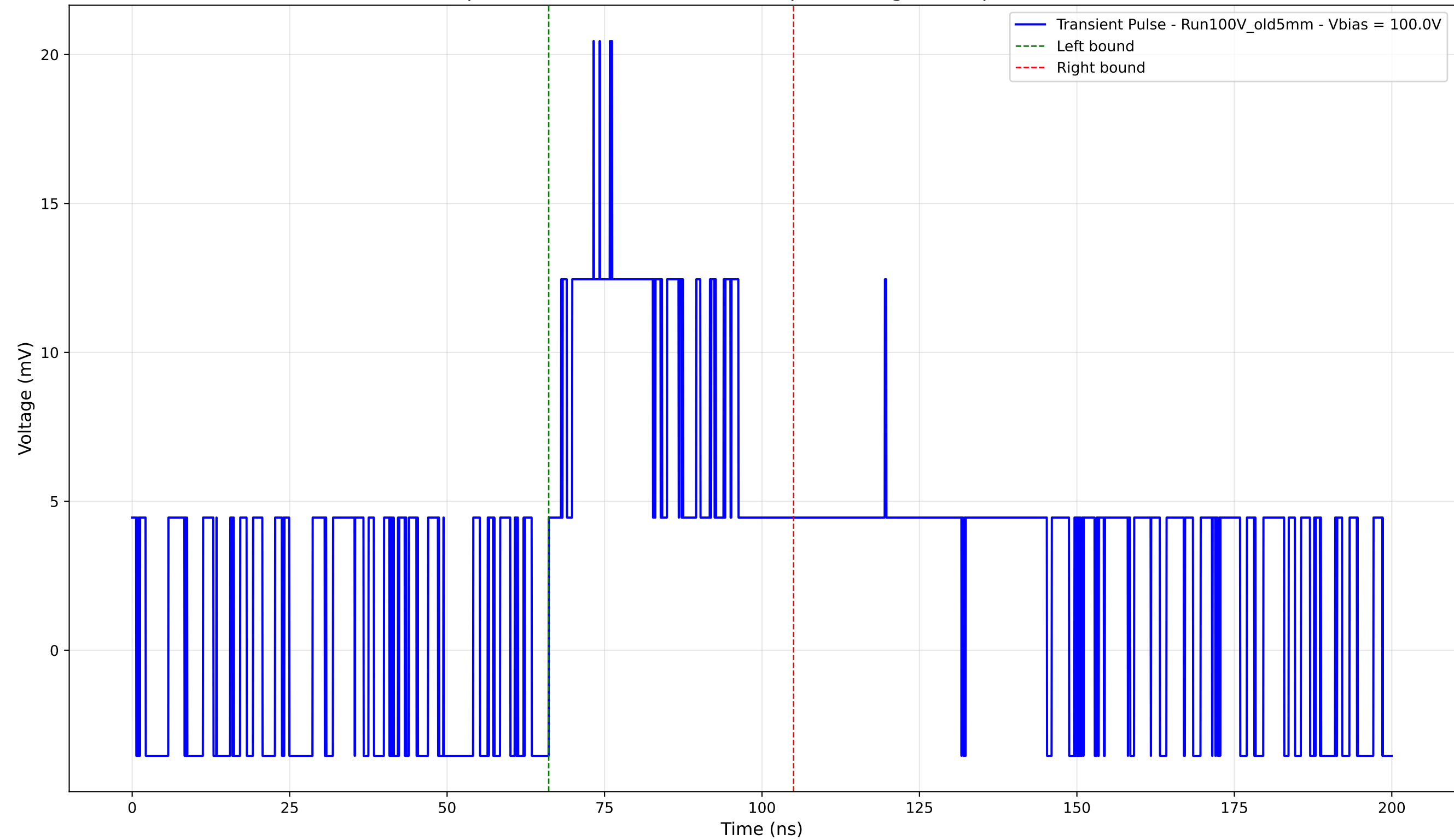
Transient Pulse - Sample: Old5mm - Position: 2165.0 \mu\text{m} - Charge: 6.81 pC - Rise Time: 0.00 ns (N/A)
