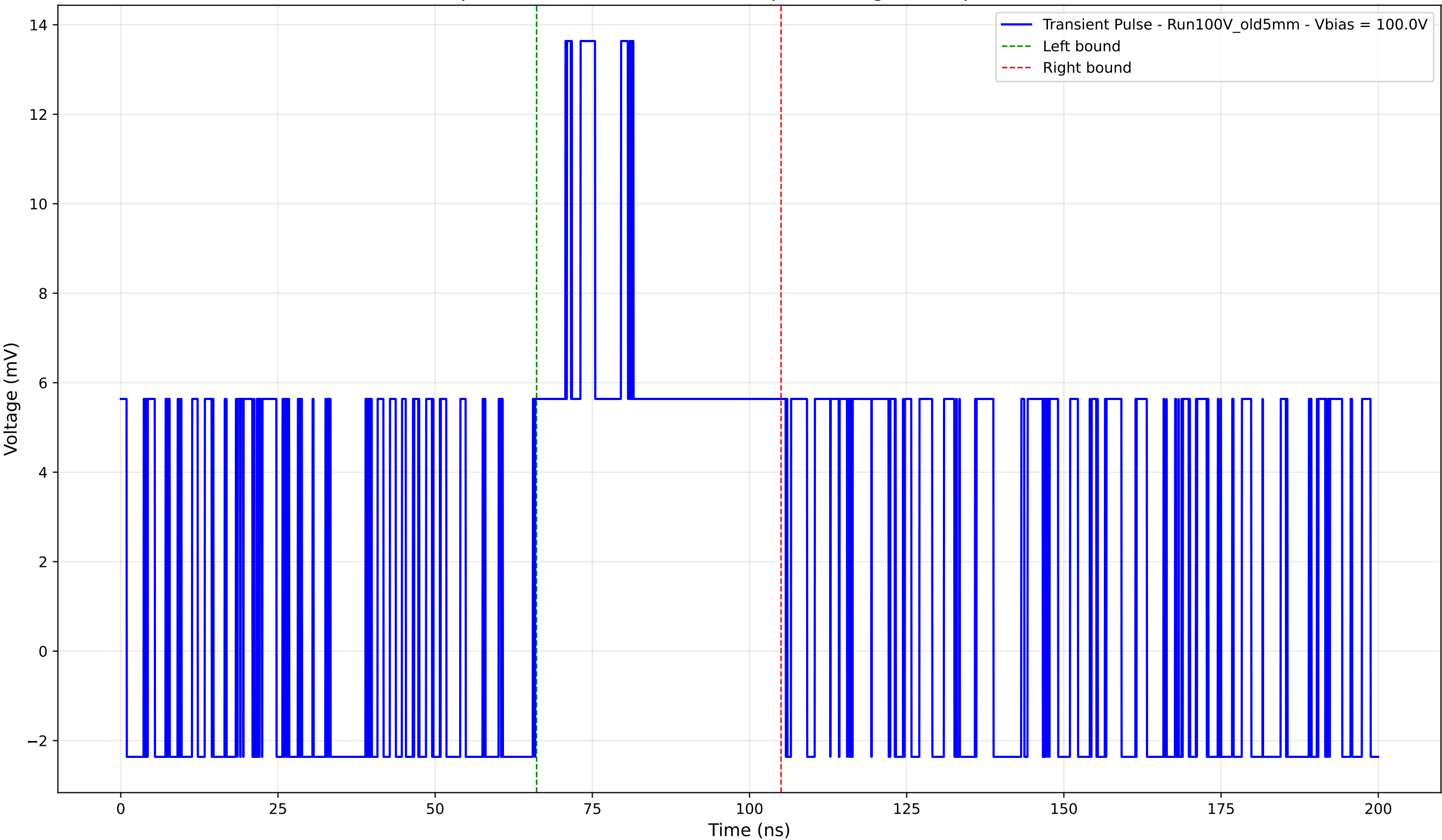
Transient Pulse - Sample: Old5mm - Position: 600.0 \mu\text{m} - Charge: 5.14 pC - Rise Time: 0.00 ns (N/A)
