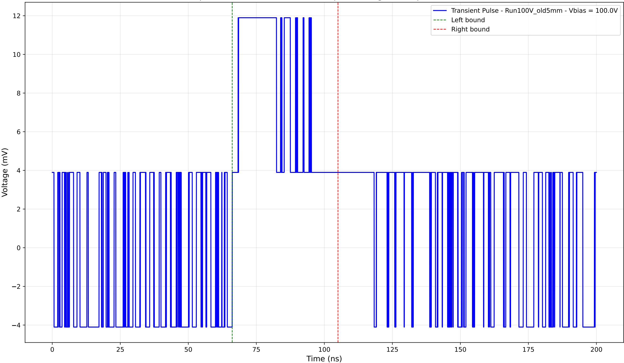
Transient Pulse - Sample: Old5mm - Position: 380.0 \mu\text{m} - Charge: 5.87 pC - Rise Time: 0.00 ns (N/A)
