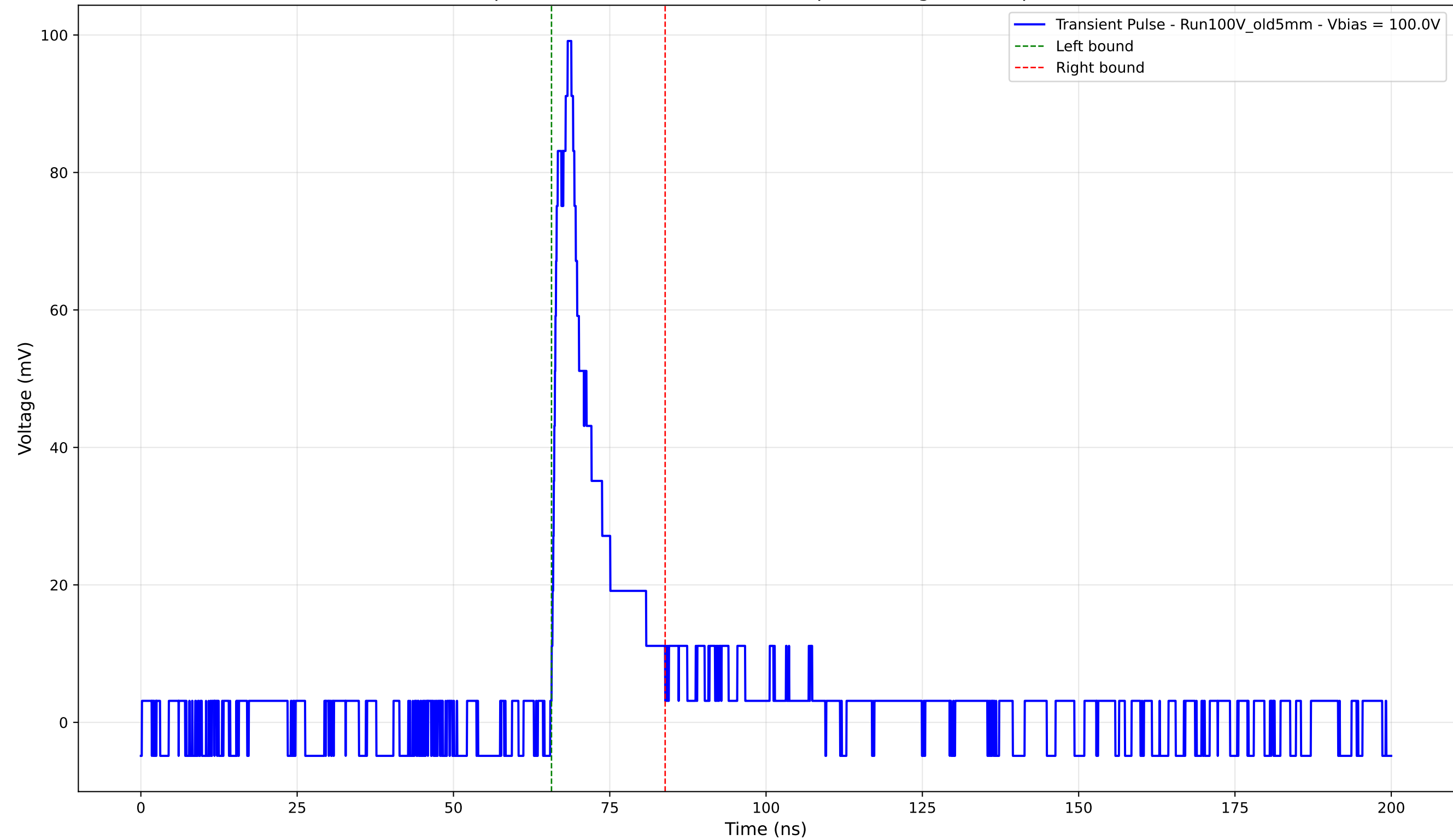
Transient Pulse - Sample: Old5mm - Position: 4105.0 \mu\text{m} - Charge: 13.20 pC - Rise Time: 2.24 ns
