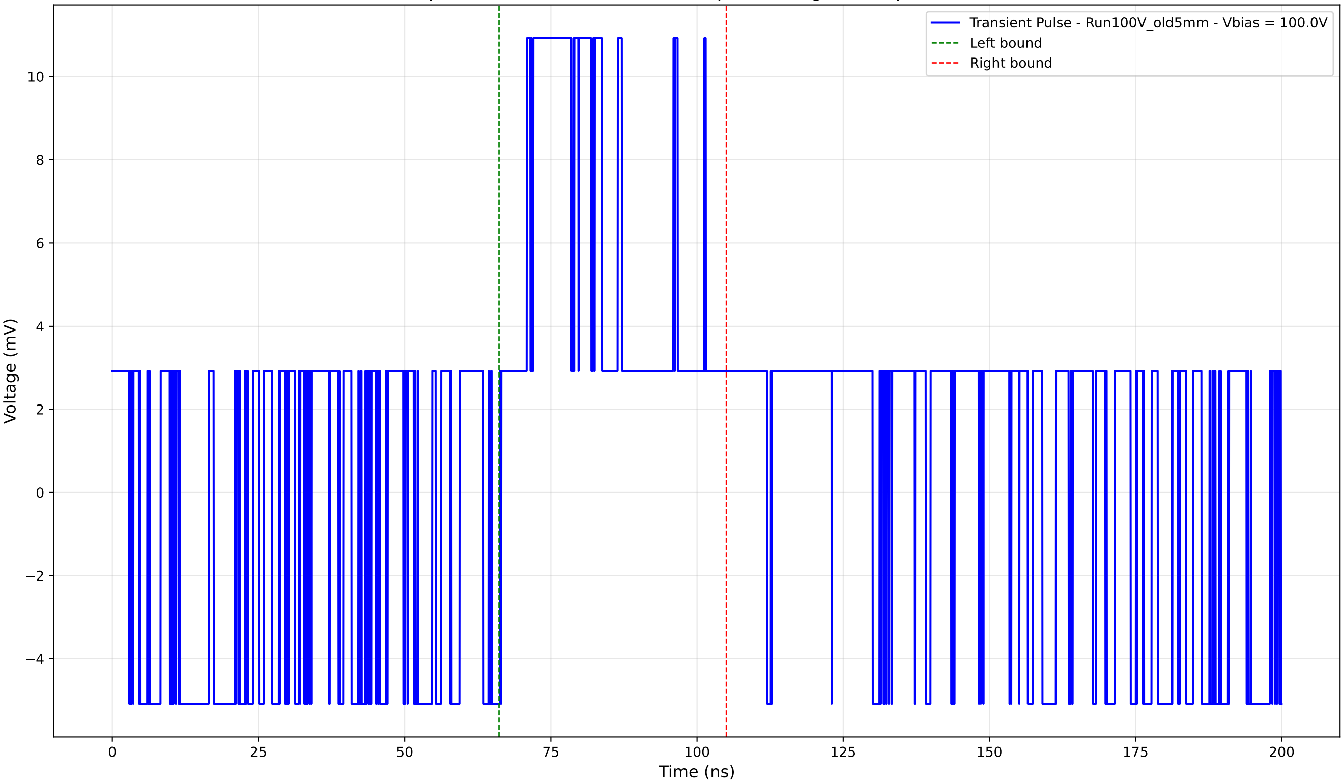
Transient Pulse - Sample: Old5mm - Position: 675.0 \mu\text{m} - Charge: 4.36 pC - Rise Time: 0.00 ns (N/A)
