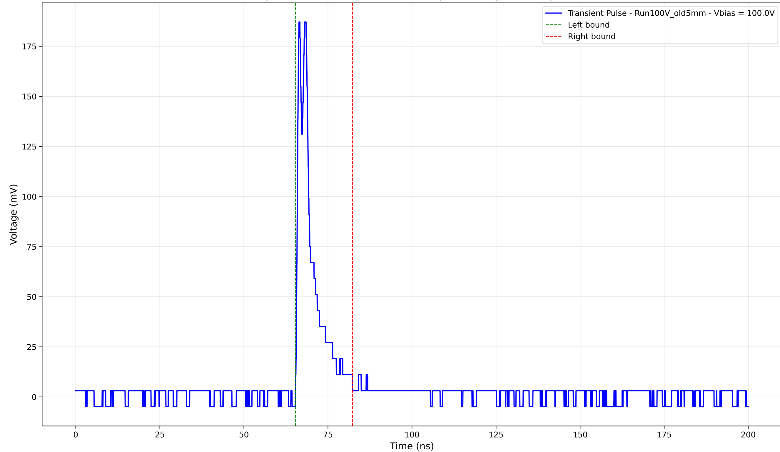
Transient Pulse - Sample: Old5mm - Position: 3840.0 \mu\text{m} - Charge: 19.09 pC - Rise Time: 0.74 ns
