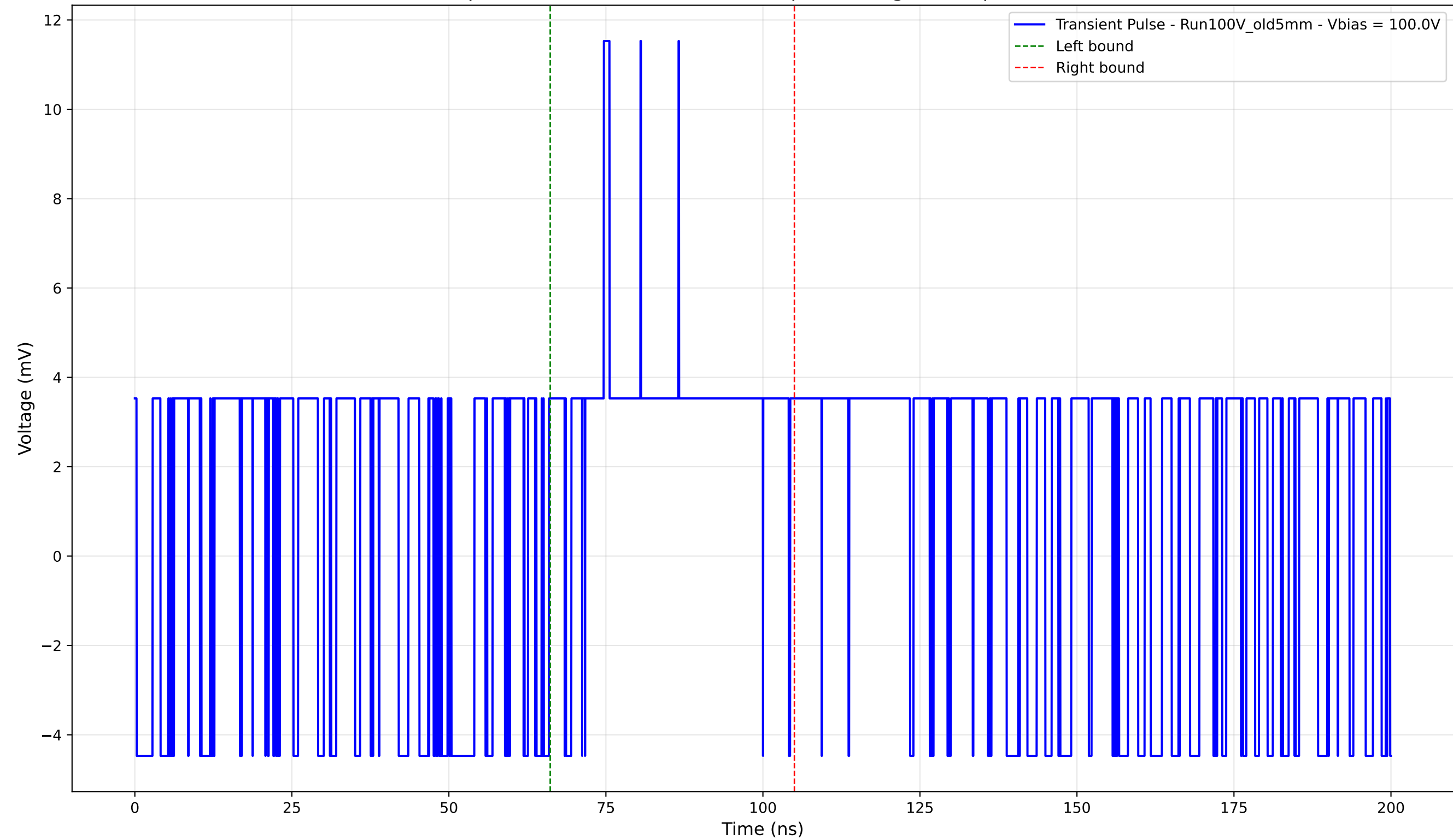
Transient Pulse - Sample: Old5mm - Position: 1890.0 \mu\text{m} - Charge: 2.73 pC - Rise Time: 0.00 ns (N/A)
