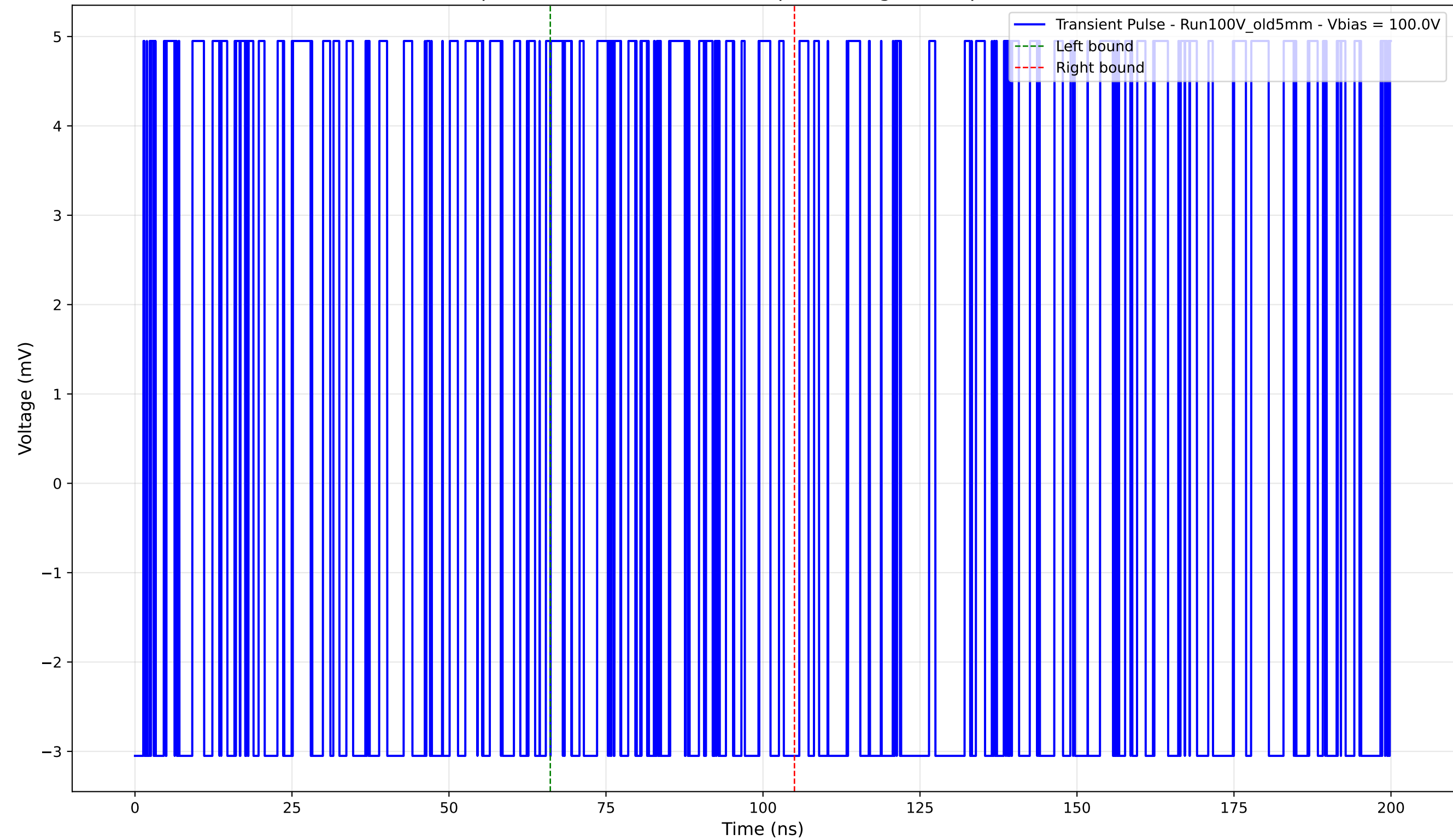
Transient Pulse - Sample: Old5mm - Position: 55.0 \mu\text{m} - Charge: 0.84 pC - Rise Time: 0.00 ns (N/A)
