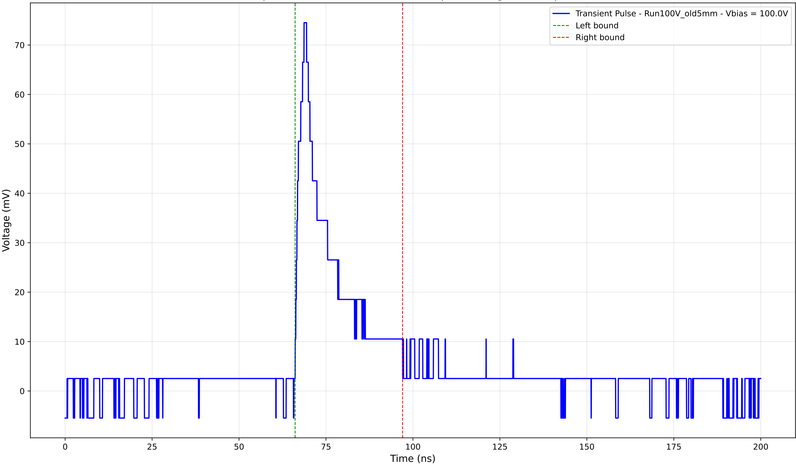
Transient Pulse - Sample: Old5mm - Position: 4425.0 \mu\text{m} - Charge: 15.29 pC - Rise Time: 2.55 ns
