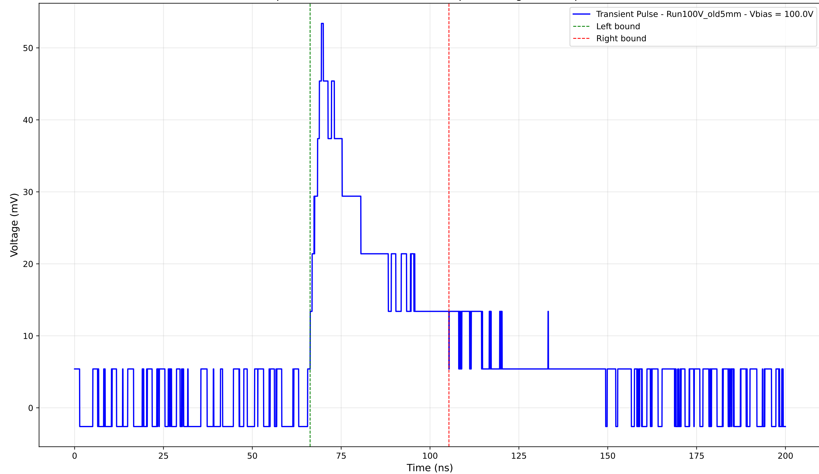
Transient Pulse - Sample: Old5mm - Position: 4830.0 \mu\text{m} - Charge: 18.29 pC - Rise Time: 3.88 ns
