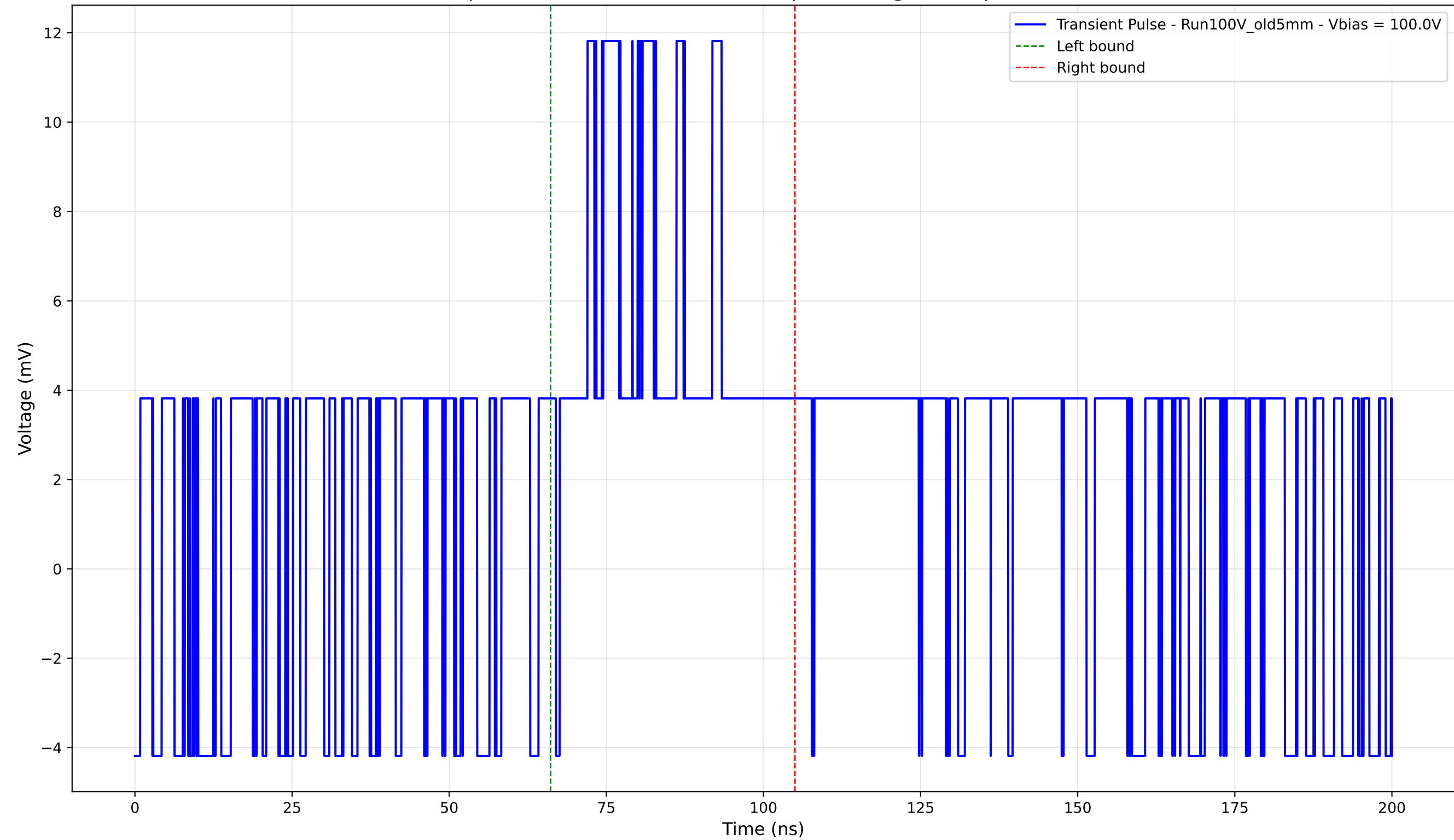
Transient Pulse - Sample: Old5mm - Position: 1670.0 \mu\text{m} - Charge: 4.33 pC - Rise Time: 0.00 ns (N/A)
