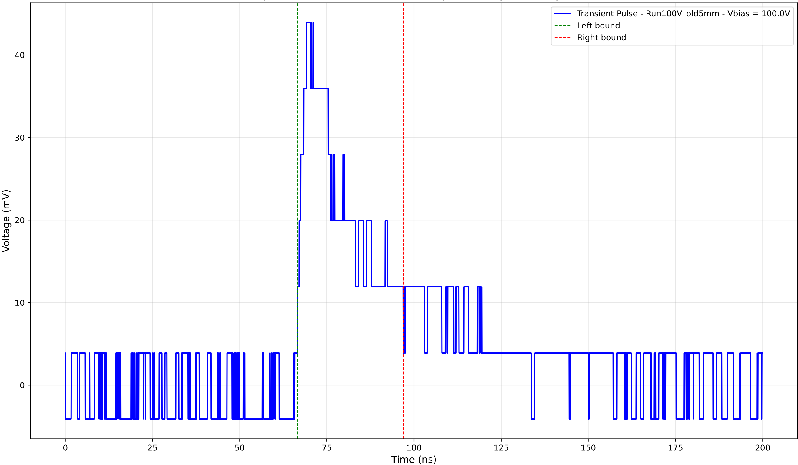
Transient Pulse - Sample: Old5mm - Position: 2650.0 \mu\text{m} - Charge: 13.22 pC - Rise Time: 2.64 ns
