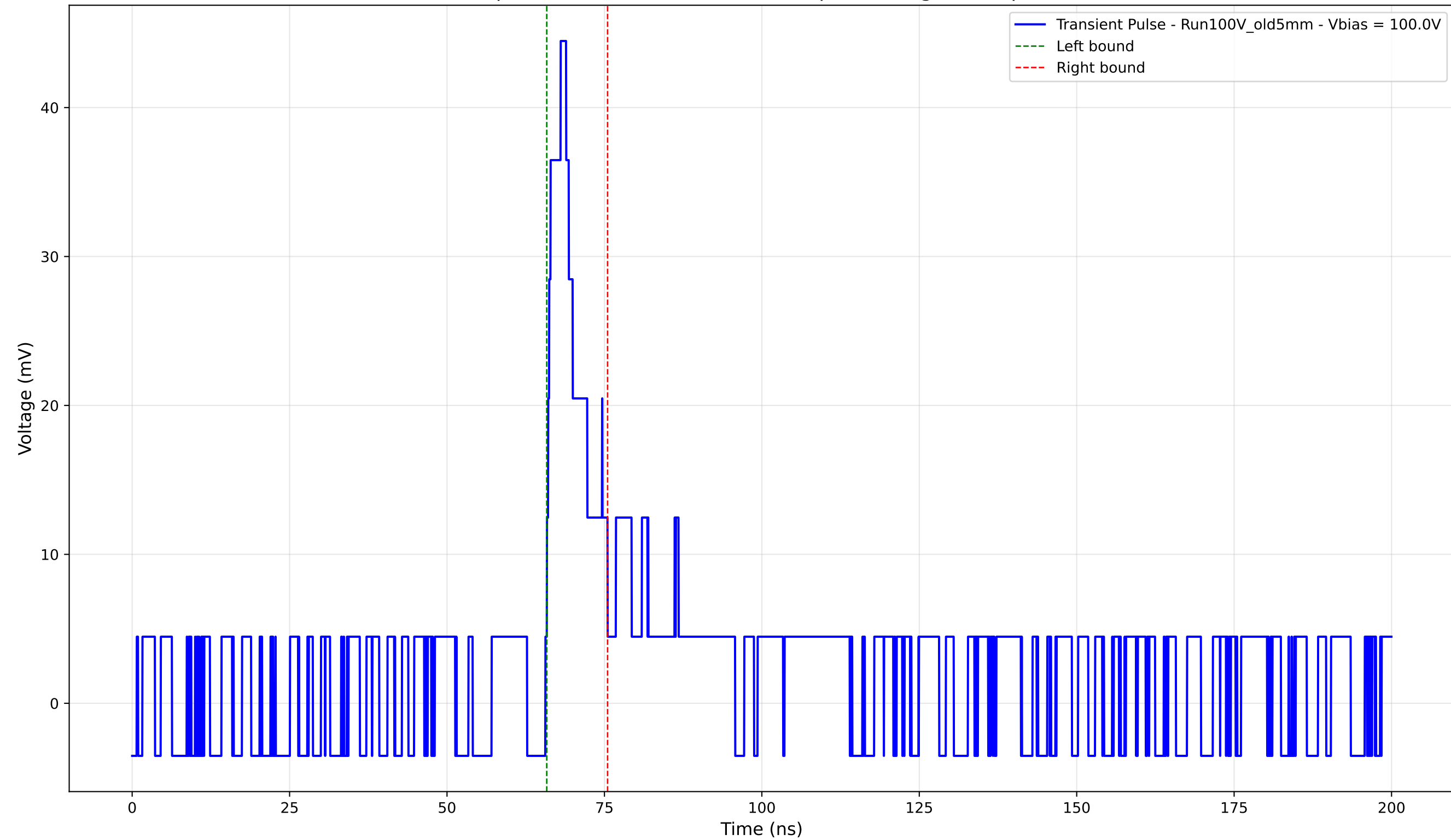
Transient Pulse - Sample: Old5mm - Position: 3350.0 \mu\text{m} - Charge: 4.61 pC - Rise Time: 2.42 ns
