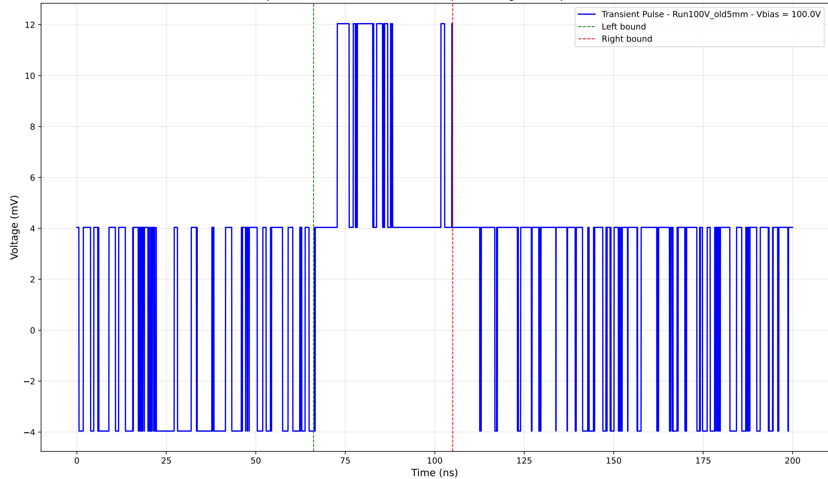
Transient Pulse - Sample: Old5mm - Position: 1005.0 \mu\text{m} - Charge: 5.14 pC - Rise Time: 0.00 ns (N/A)
