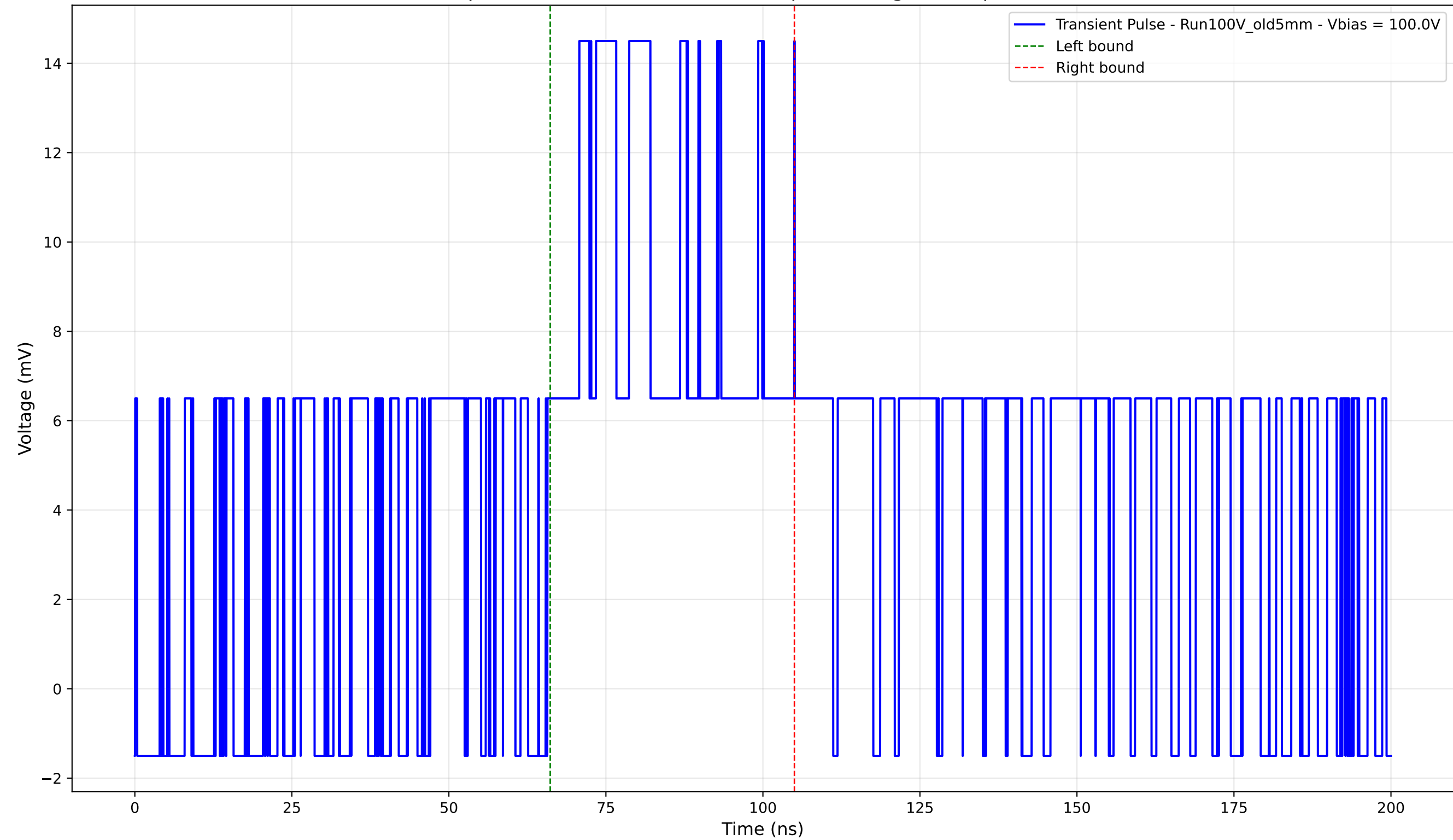
Transient Pulse - Sample: Old5mm - Position: 1955.0 \mu\text{m} - Charge: 6.80 pC - Rise Time: 0.00 ns (N/A)
