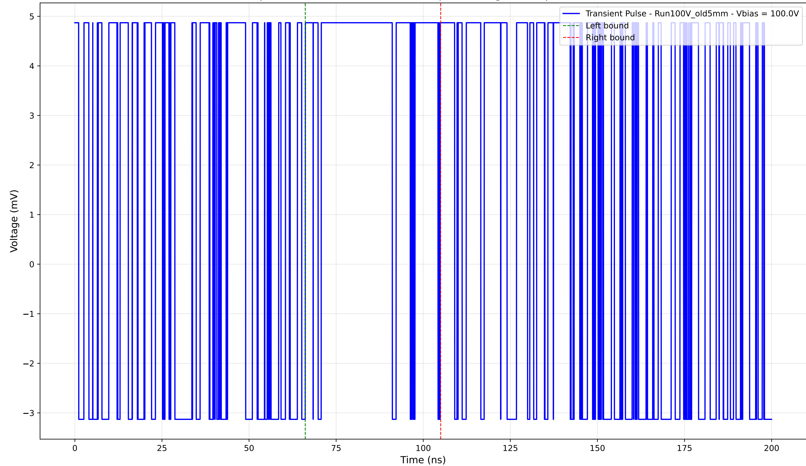
Transient Pulse - Sample: Old5mm - Position: 2320.0 \mu\text{m} - Charge: 3.29 pC - Rise Time: 0.00 ns (N/A)
