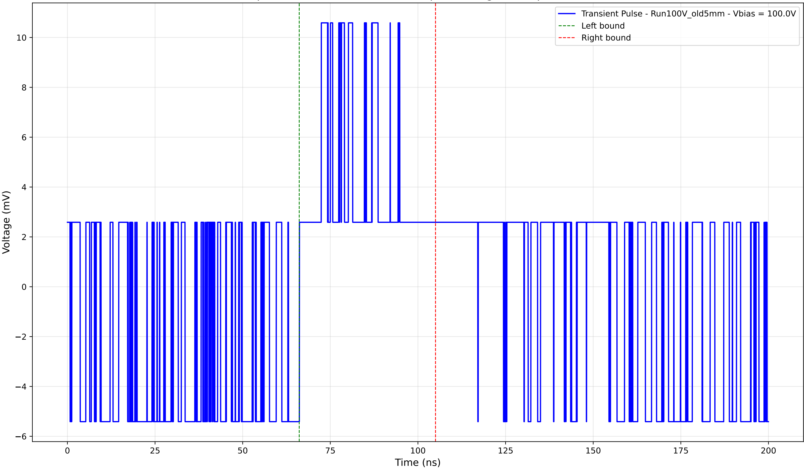
Transient Pulse - Sample: Old5mm - Position: 655.0 \mu\text{m} - Charge: 3.25 pC - Rise Time: 0.00 ns (N/A)
