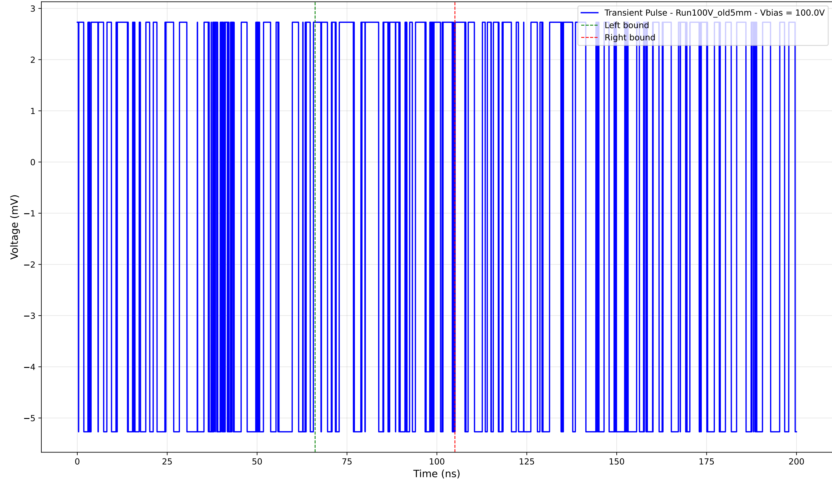
Transient Pulse - Sample: Old5mm - Position: 15.0 \mu\text{m} - Charge: 0.24 pC - Rise Time: 0.00 ns (N/A)
