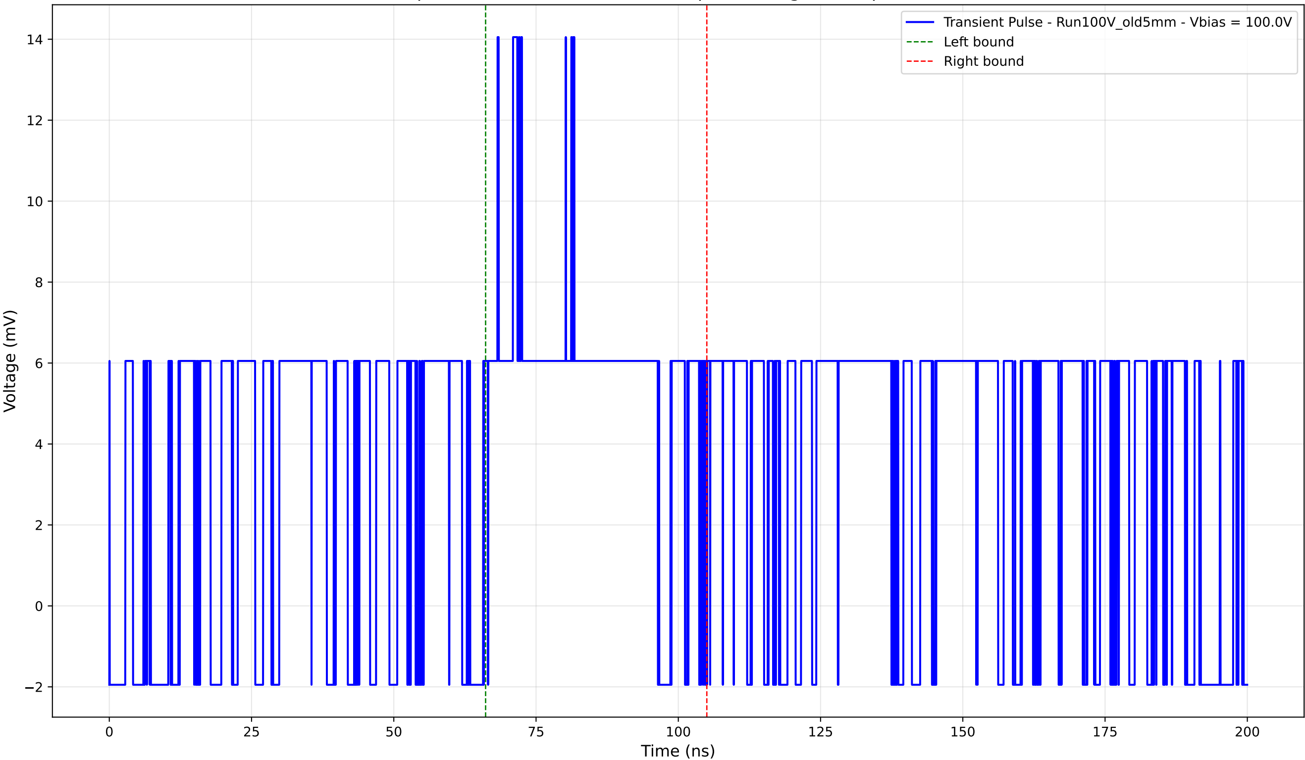
Transient Pulse - Sample: Old5mm - Position: 295.0 \mu\text{m} - Charge: 4.41 pC - Rise Time: 0.00 ns (N/A)
