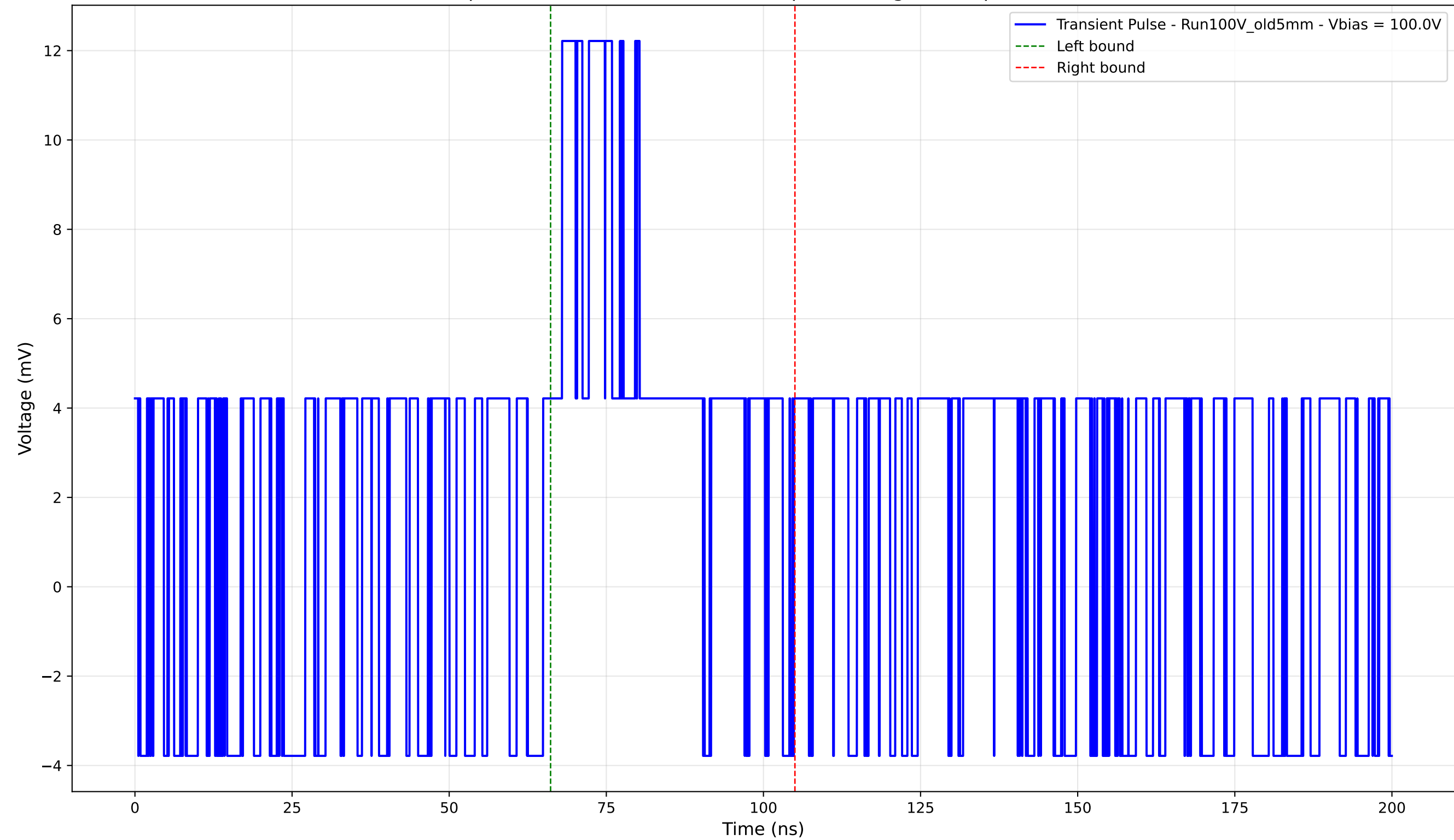
Transient Pulse - Sample: Old5mm - Position: 2845.0 \mu\text{m} - Charge: 3.96 pC - Rise Time: 0.00 ns (N/A)
