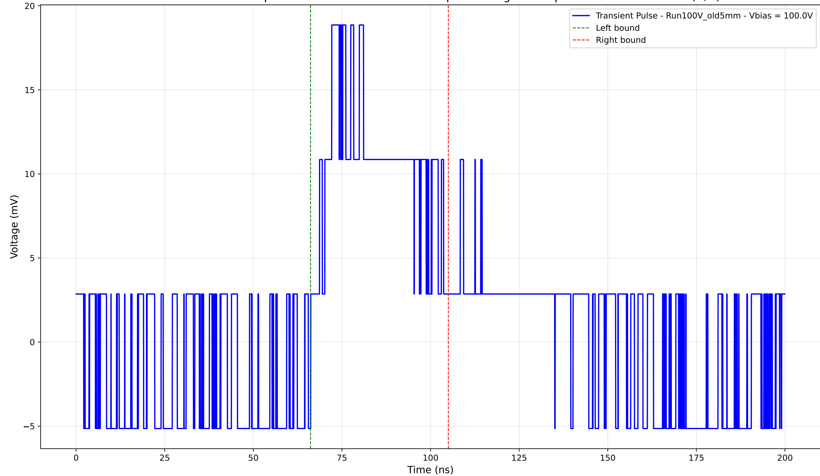
Transient Pulse - Sample: Old5mm - Position: 1985.0 \mu\text{m} - Charge: 8.24 pC - Rise Time: 0.00 ns (N/A)
