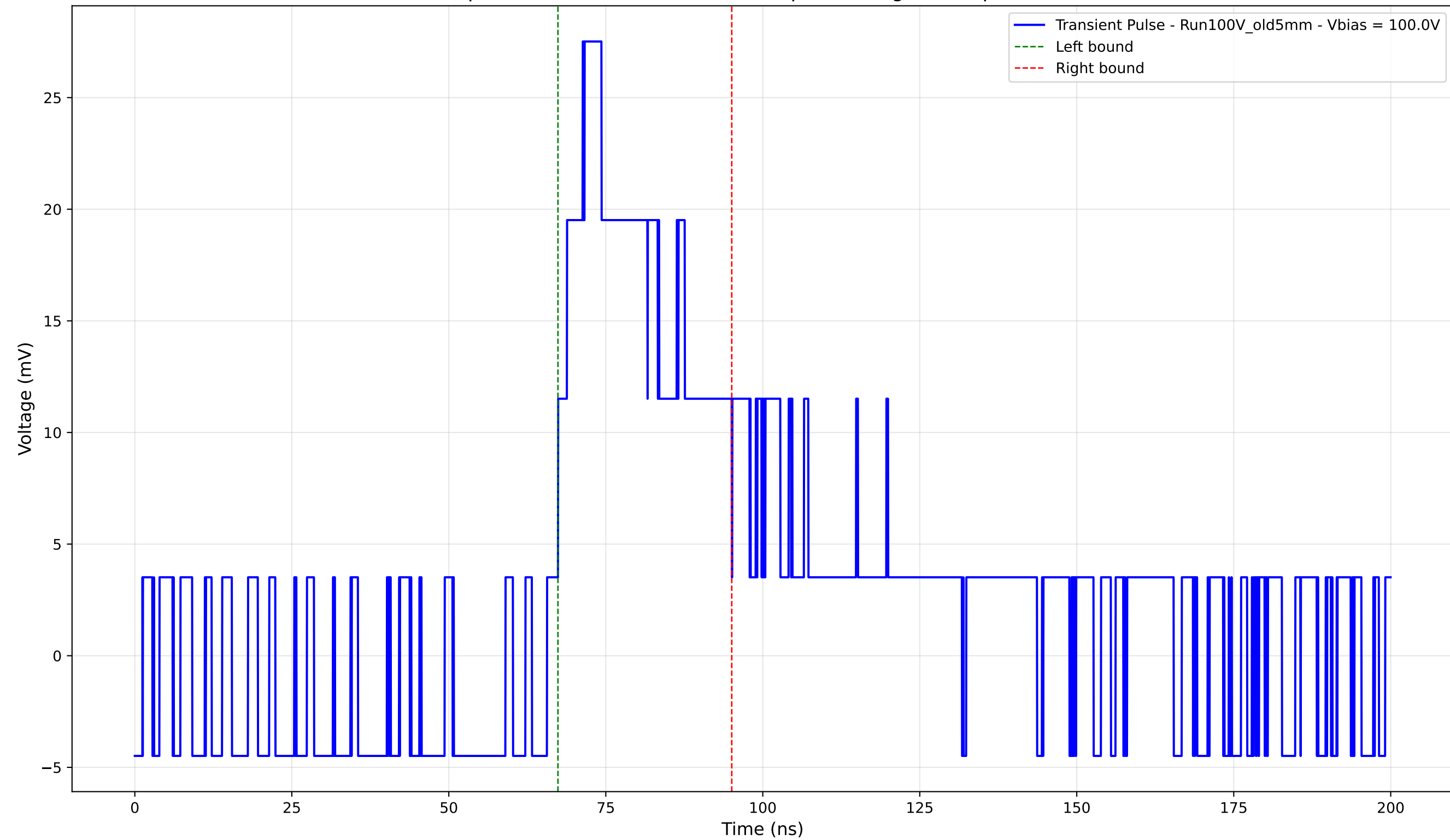
Transient Pulse - Sample: Old5mm - Position: 2395.0 \mu\text{m} - Charge: 9.34 pC - Rise Time: 0.00 ns (N/A)
