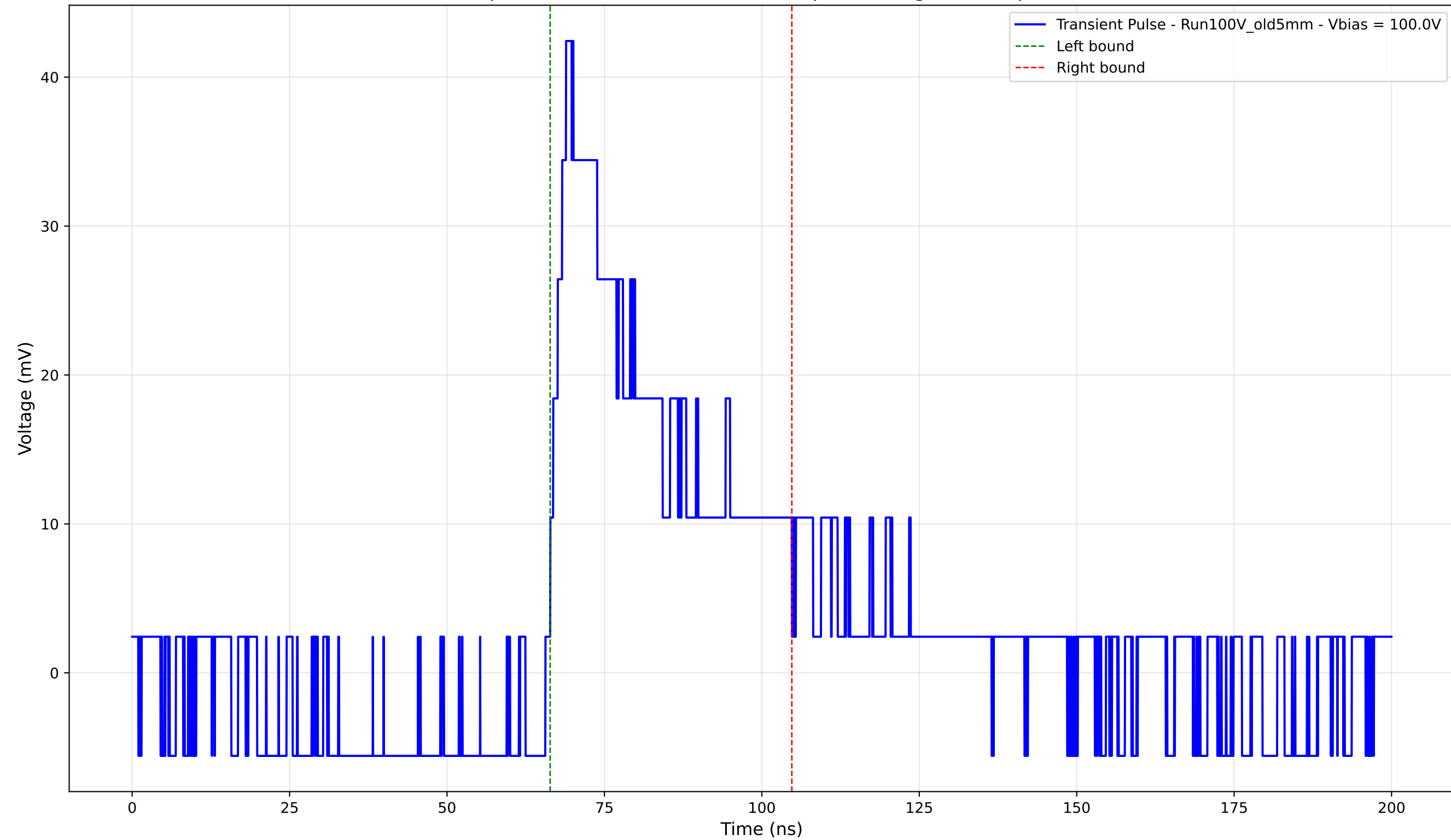
Transient Pulse - Sample: Old5mm - Position: 2655.0 \mu\text{m} - Charge: 14.05 pC - Rise Time: 2.52 ns
