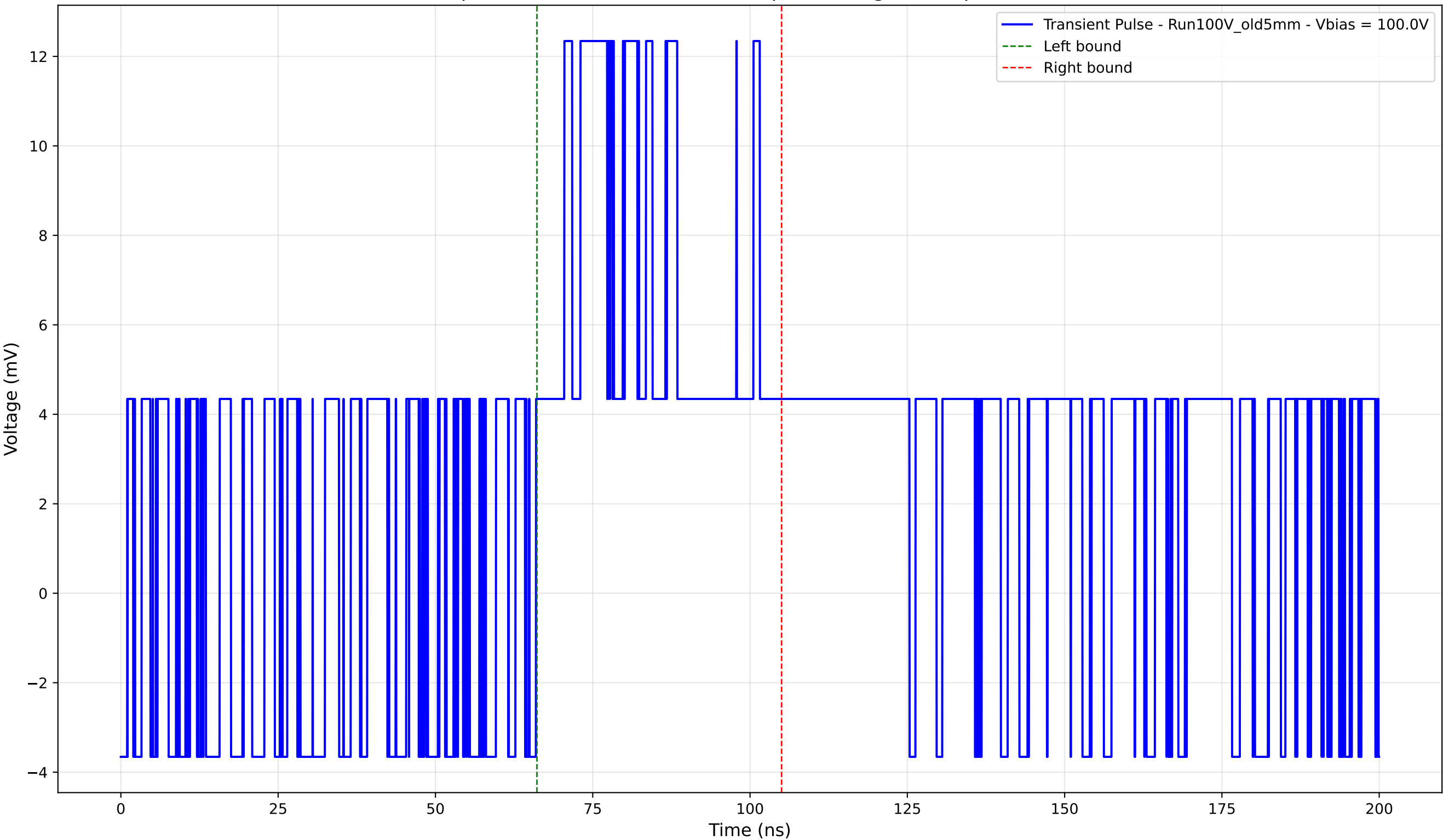
Transient Pulse - Sample: Old5mm - Position: 700.0 \mu\text{m} - Charge: 5.36 pC - Rise Time: 0.00 ns (N/A)
