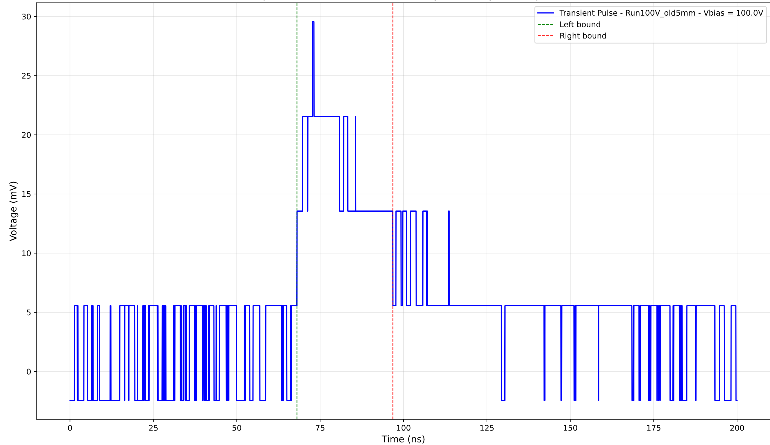
Transient Pulse - Sample: Old5mm - Position: 2245.0 \mu\text{m} - Charge: 9.82 pC - Rise Time: 6.30 ns
