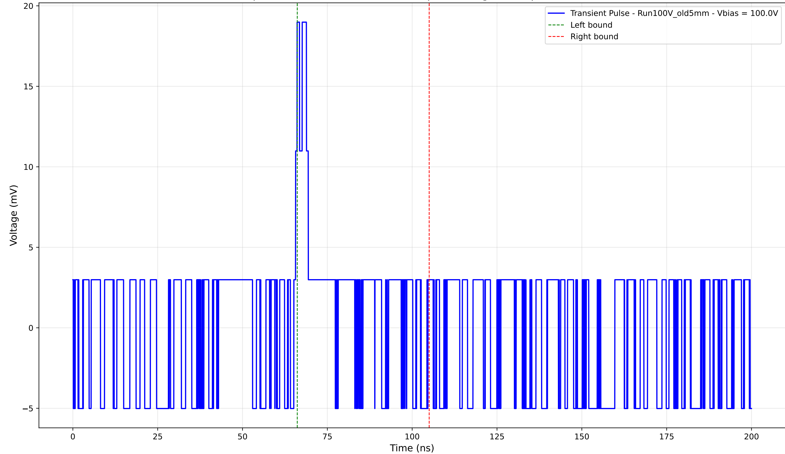
Transient Pulse - Sample: Old5mm - Position: 3680.0 \mu\text{m} - Charge: 1.99 pC - Rise Time: 0.00 ns (N/A)
