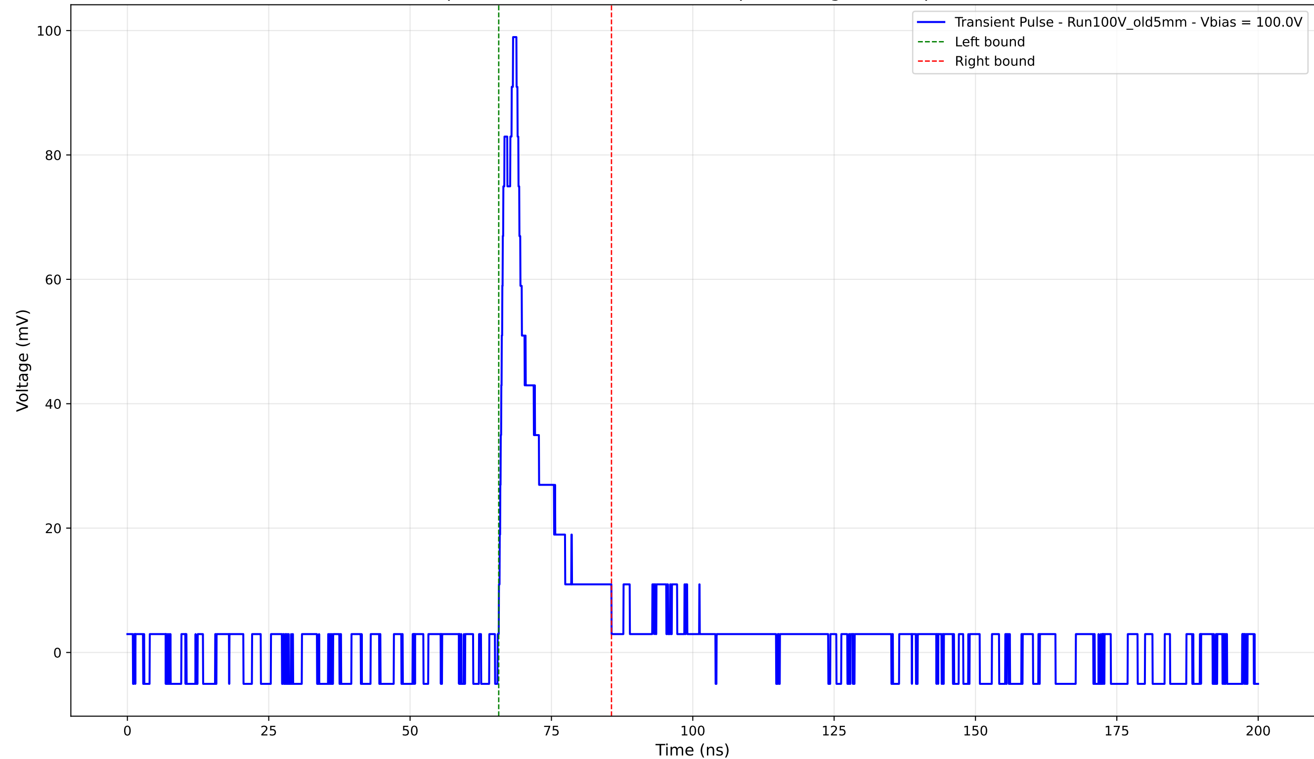
Transient Pulse - Sample: Old5mm - Position: 3315.0 \mu\text{m} - Charge: 12.54 pC - Rise Time: 2.26 ns
