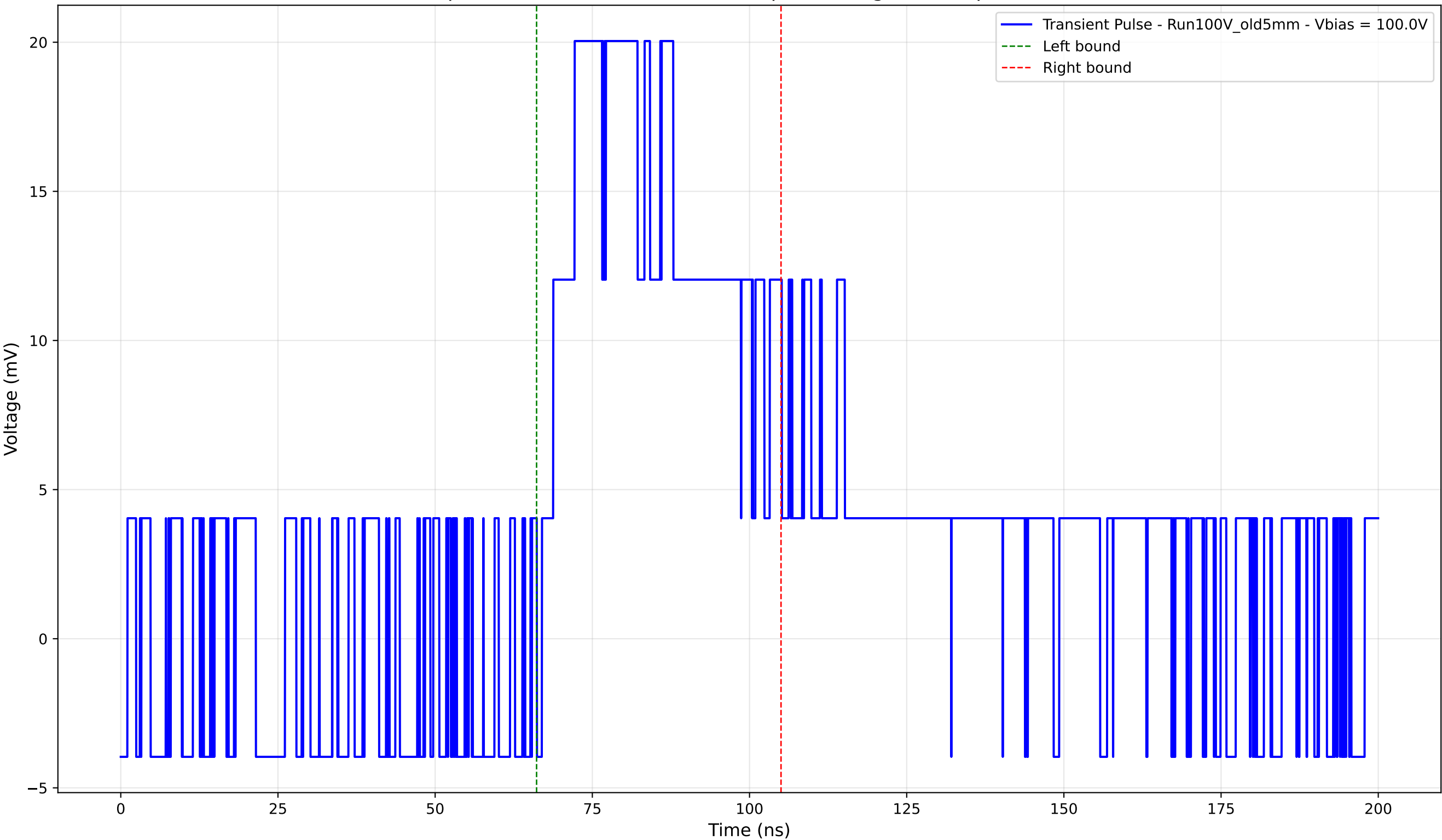
Transient Pulse - Sample: Old5mm - Position: 2000.0 \mu\text{m} - Charge: 10.58 pC - Rise Time: 0.00 ns (N/A)
