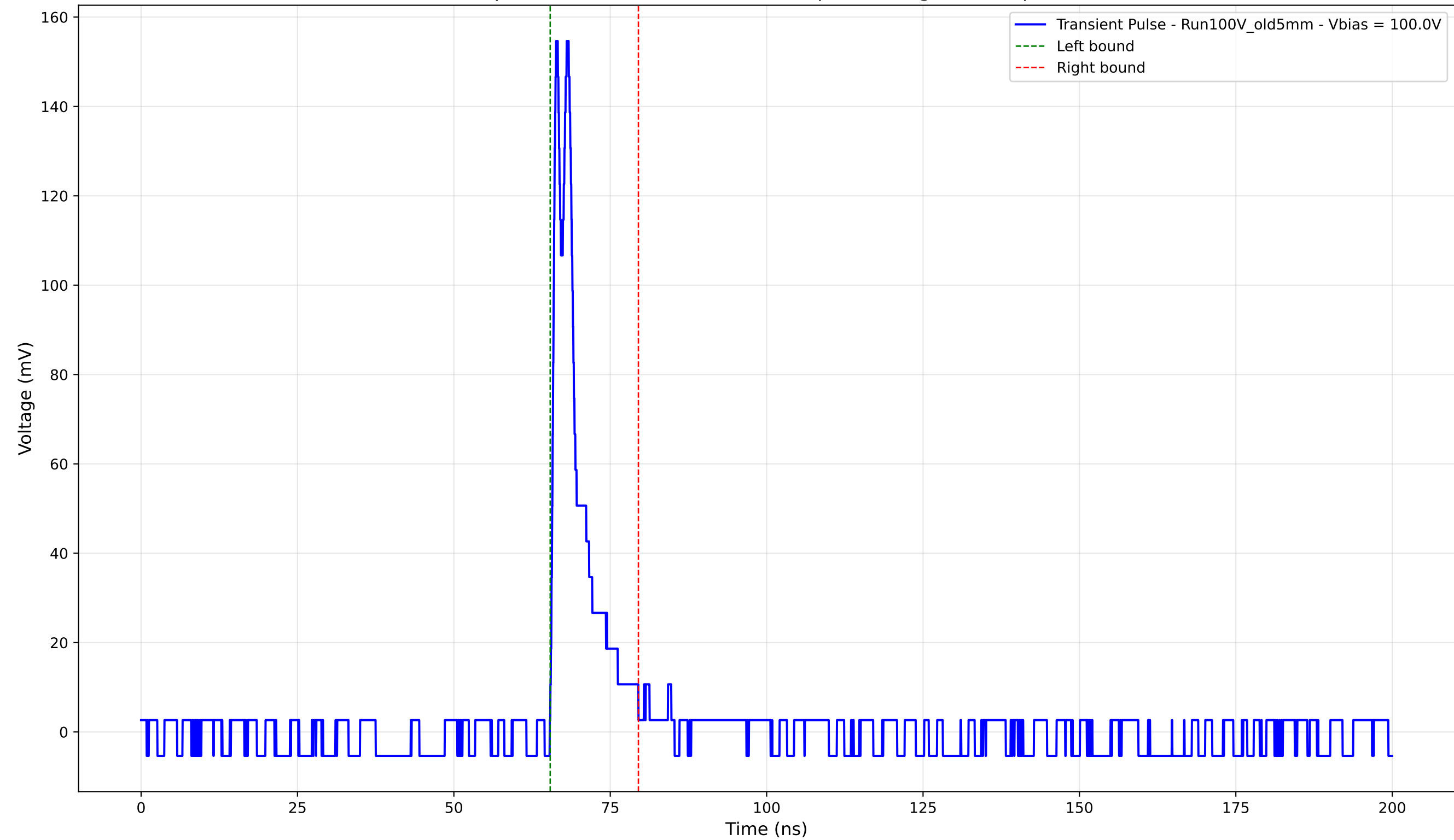
Transient Pulse - Sample: Old5mm - Position: 3795.0 \mu\text{m} - Charge: 14.27 pC - Rise Time: 0.75 ns
