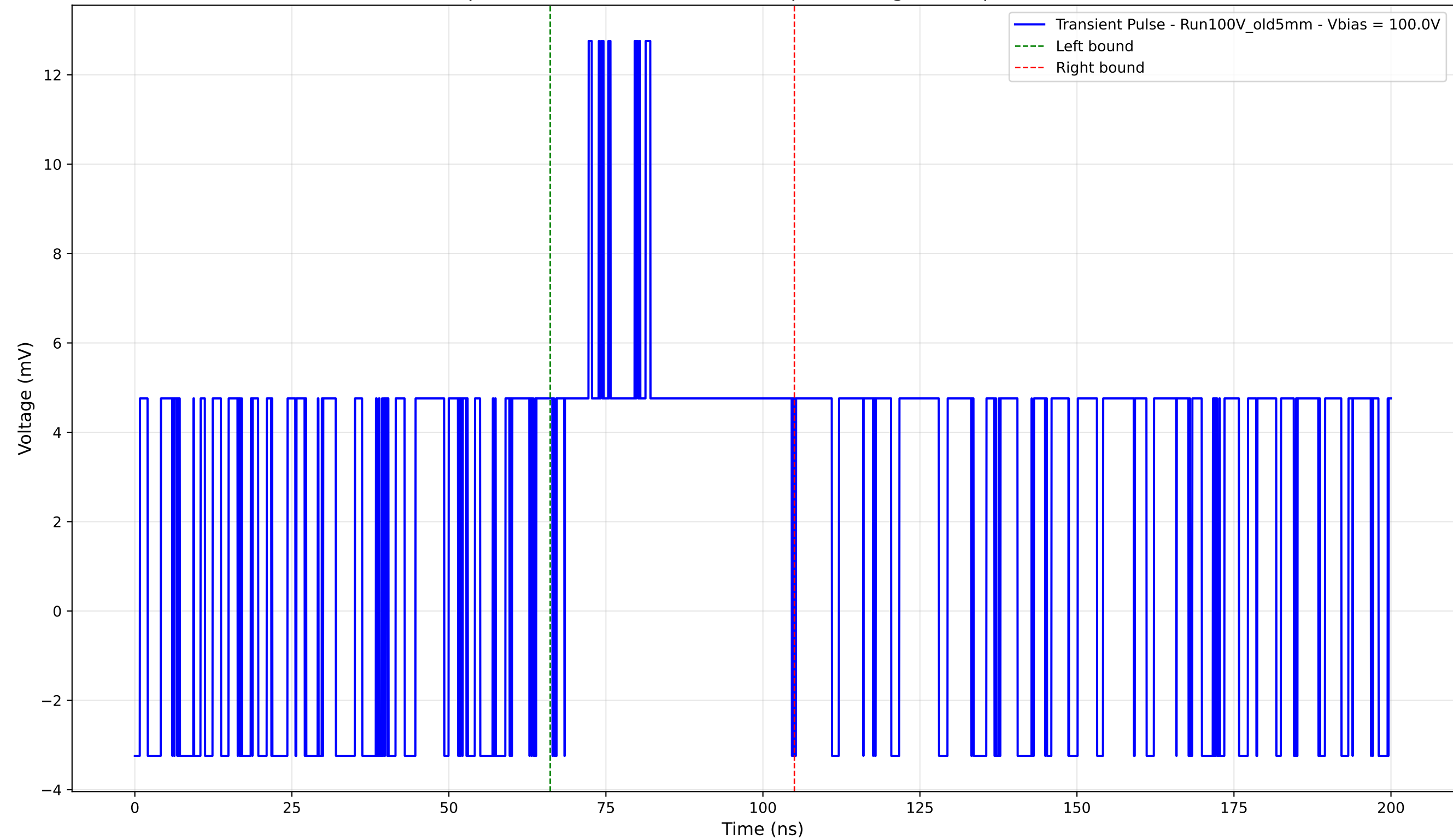
Transient Pulse - Sample: Old5mm - Position: 1885.0 \mu\text{m} - Charge: 3.99 pC - Rise Time: 0.00 ns (N/A)
