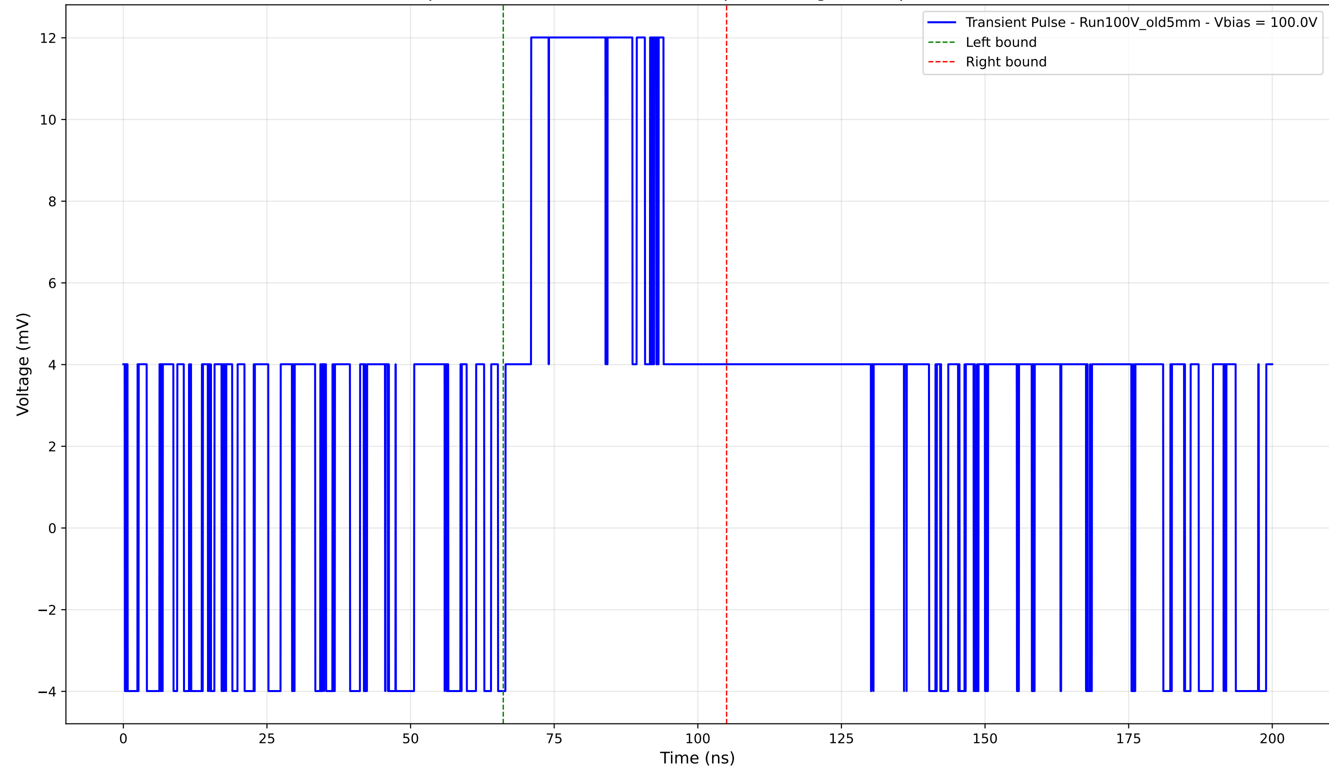
Transient Pulse - Sample: Old5mm - Position: 1765.0 \mu\text{m} - Charge: 6.39 pC - Rise Time: 0.00 ns (N/A)
