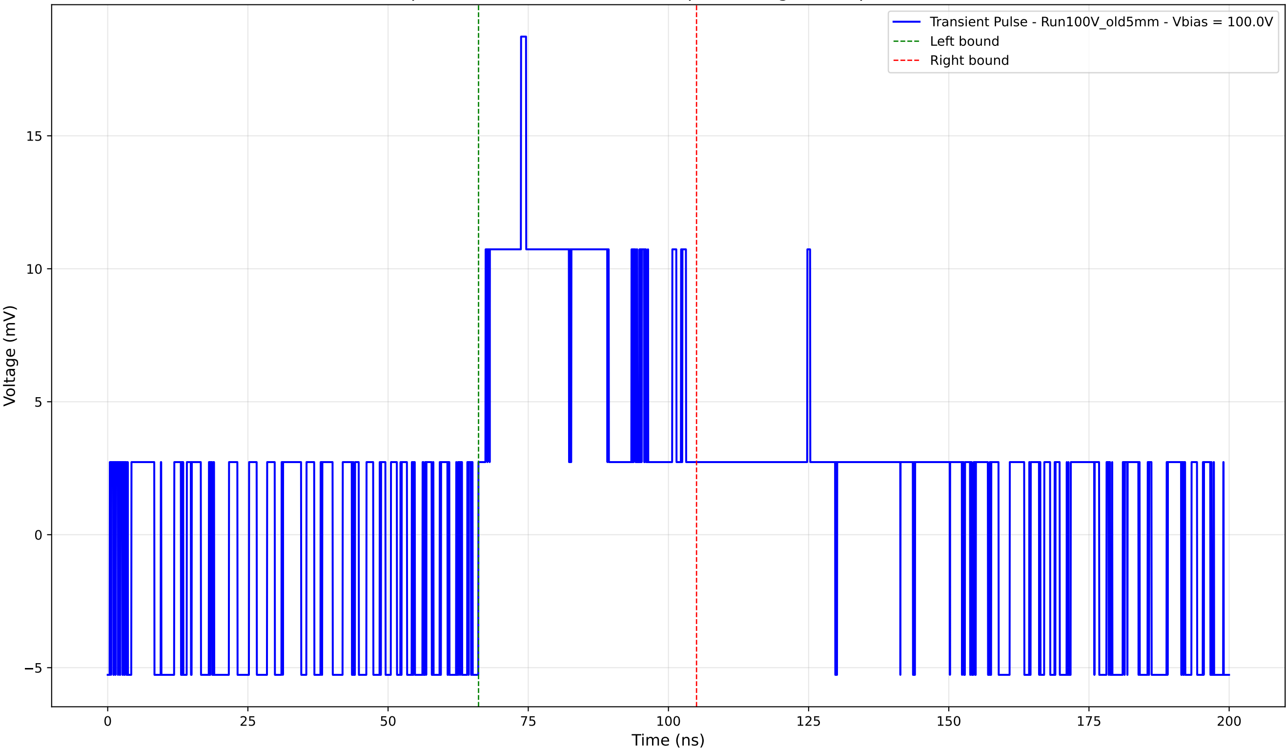
Transient Pulse - Sample: Old5mm - Position: 360.0 \mu\text{m} - Charge: 6.22 pC - Rise Time: 0.00 ns (N/A)
