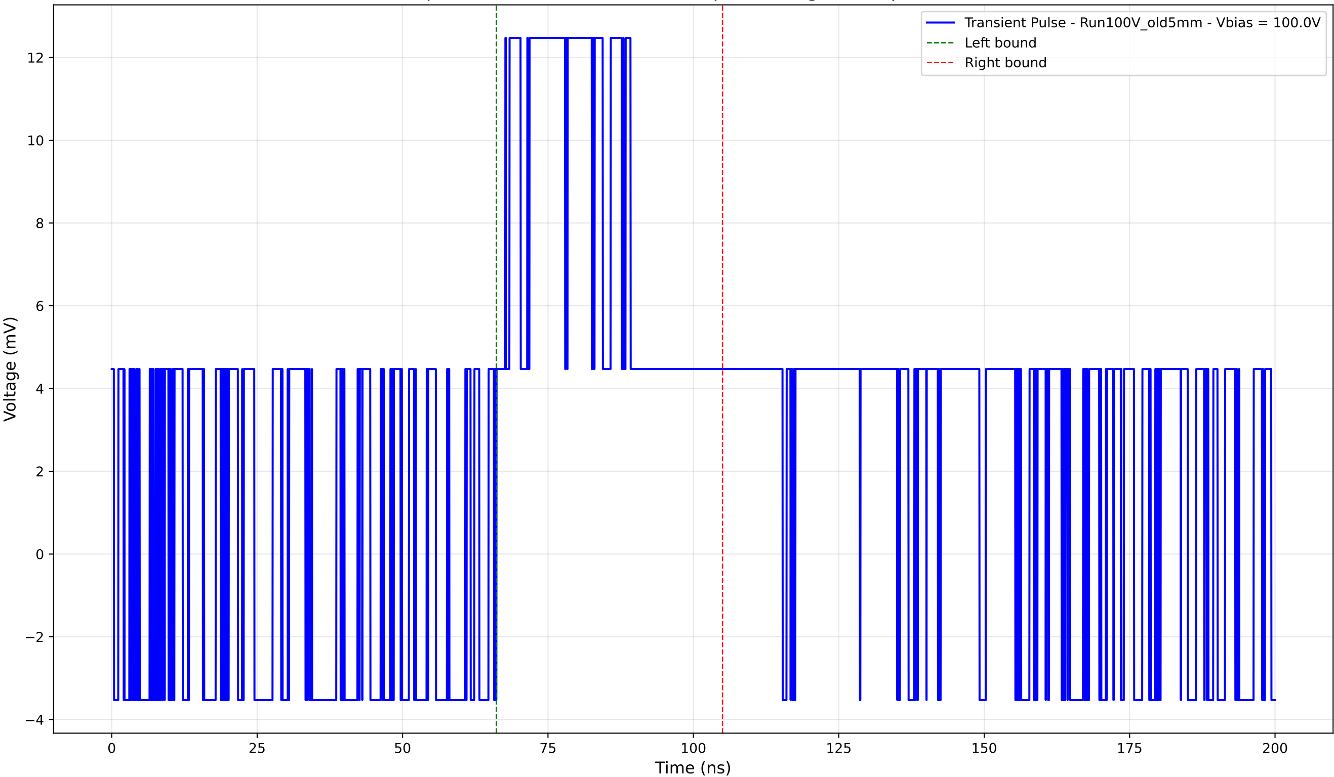
Transient Pulse - Sample: Old5mm - Position: 325.0 \mu\text{m} - Charge: 6.22 pC - Rise Time: 0.00 ns (N/A)
