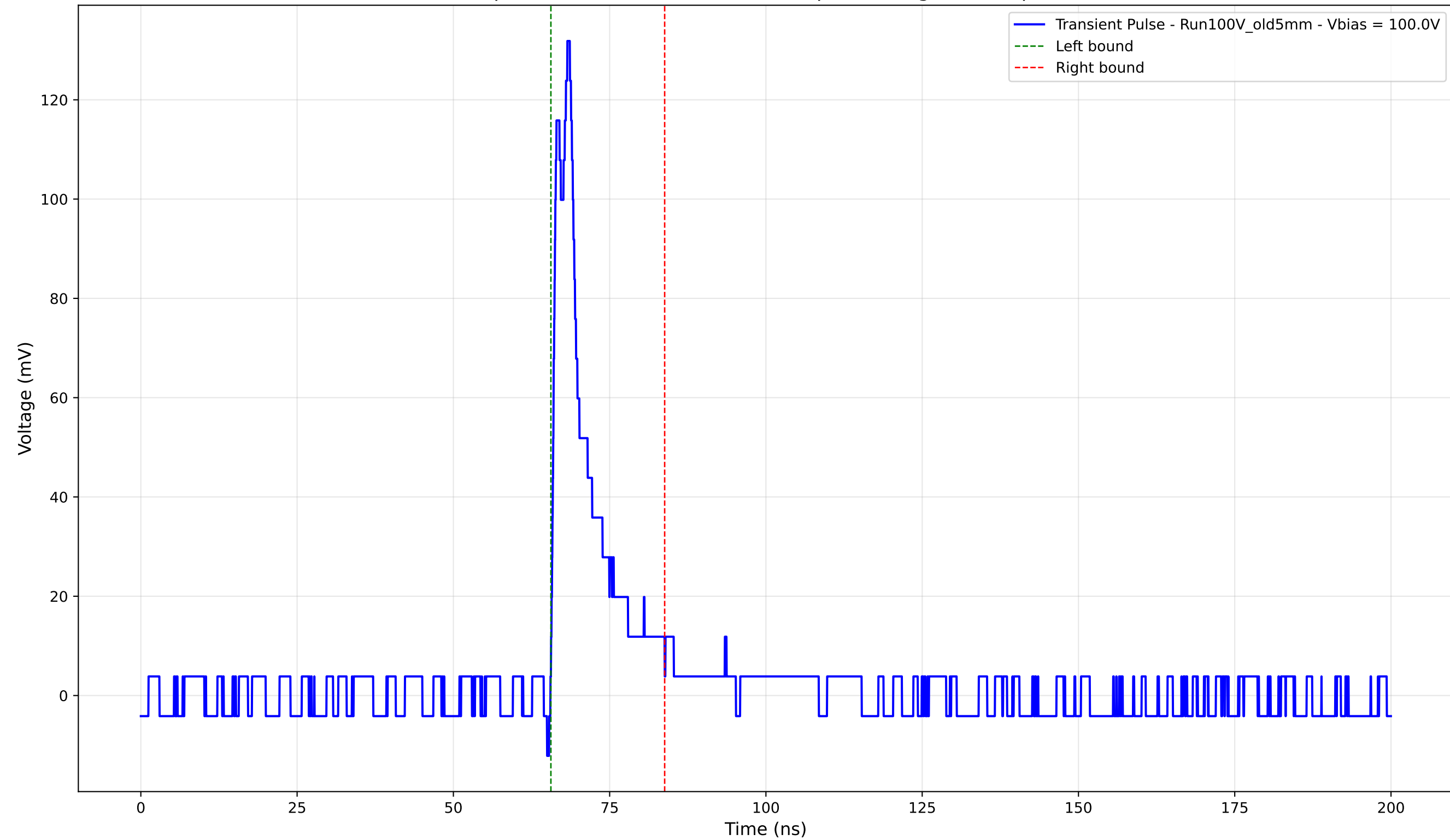
Transient Pulse - Sample: Old5mm - Position: 3495.0 \mu\text{m} - Charge: 15.15 pC - Rise Time: 2.32 ns
