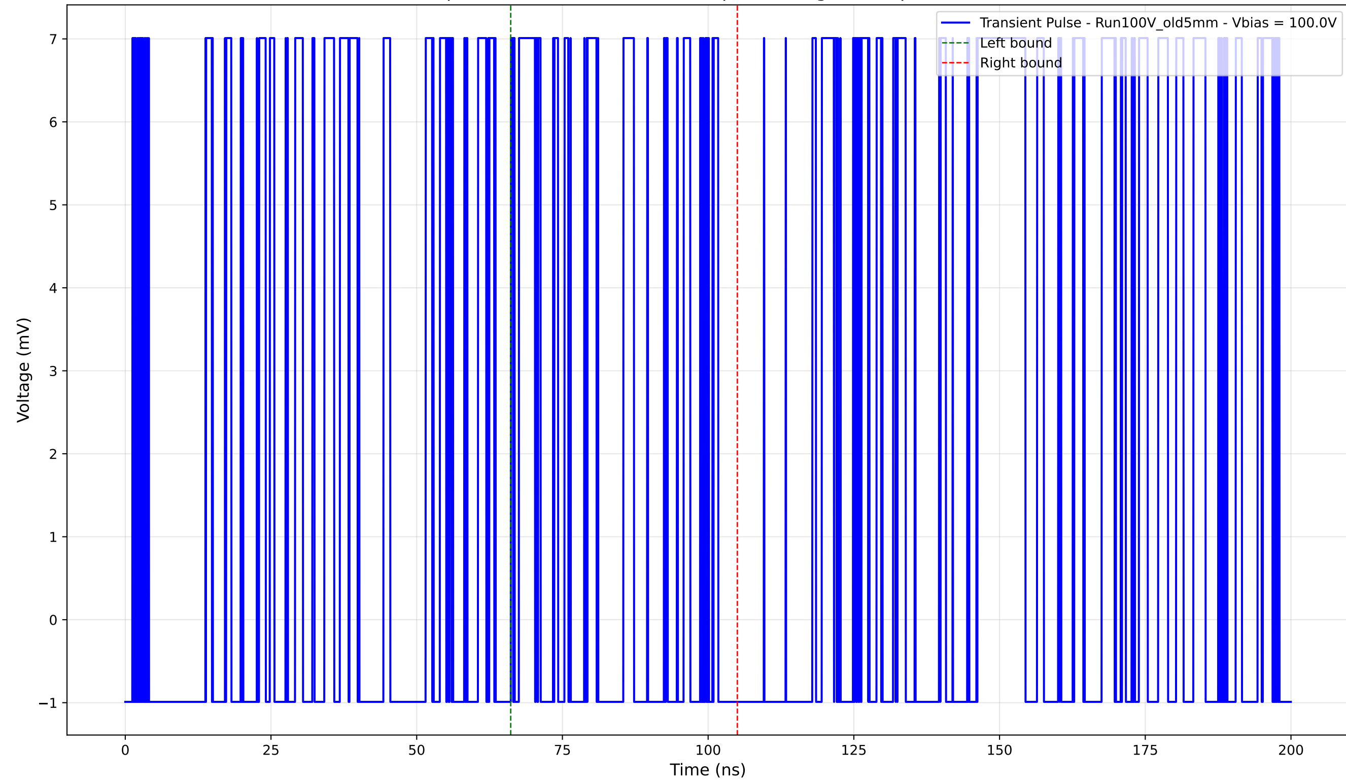
Transient Pulse - Sample: Old5mm - Position: 20.0 \mu\text{m} - Charge: 1.23 pC - Rise Time: 0.00 ns (N/A)
