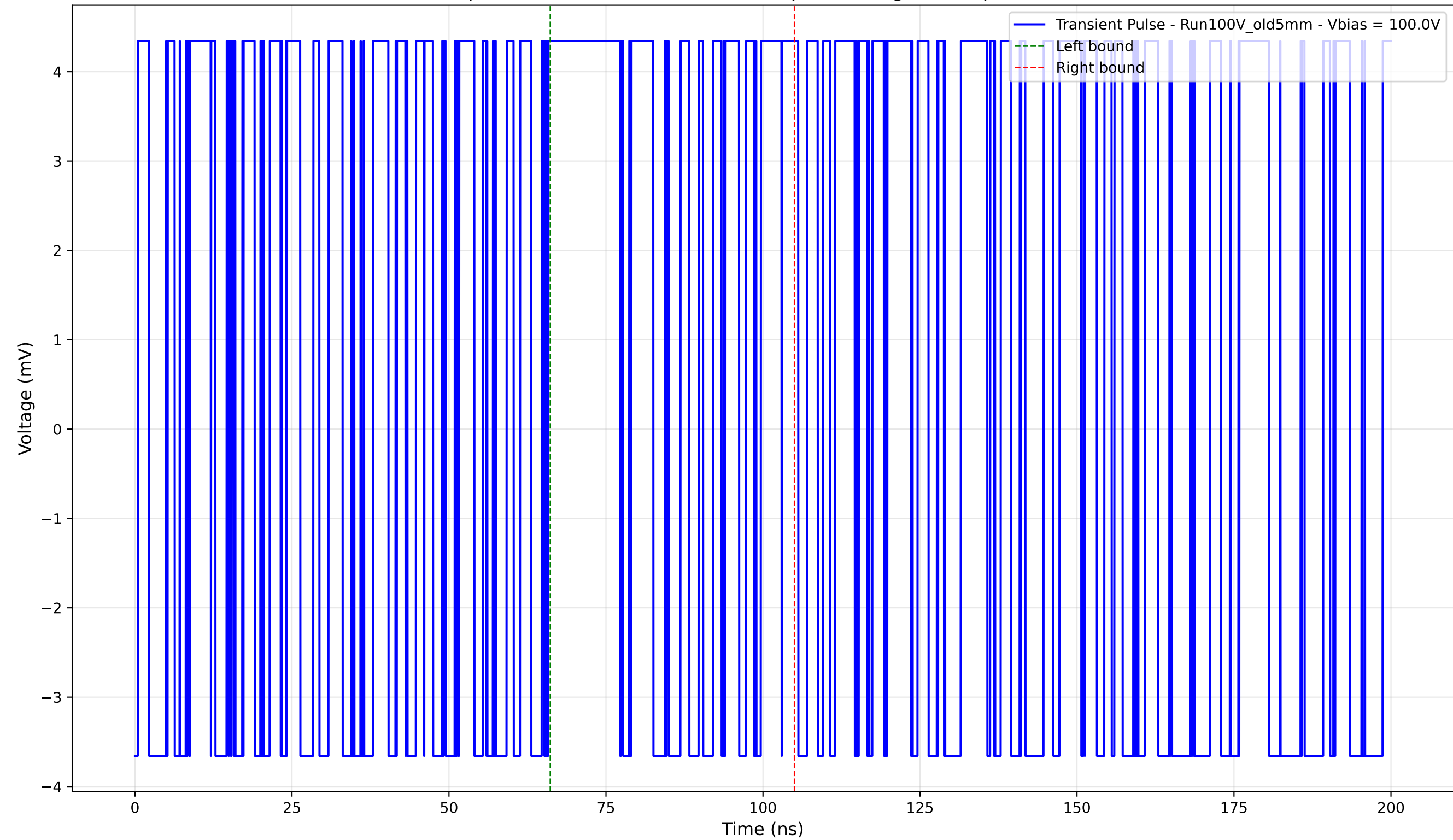
Transient Pulse - Sample: Old5mm - Position: 4295.0 \mu\text{m} - Charge: 1.64 pC - Rise Time: 0.00 ns (N/A)
