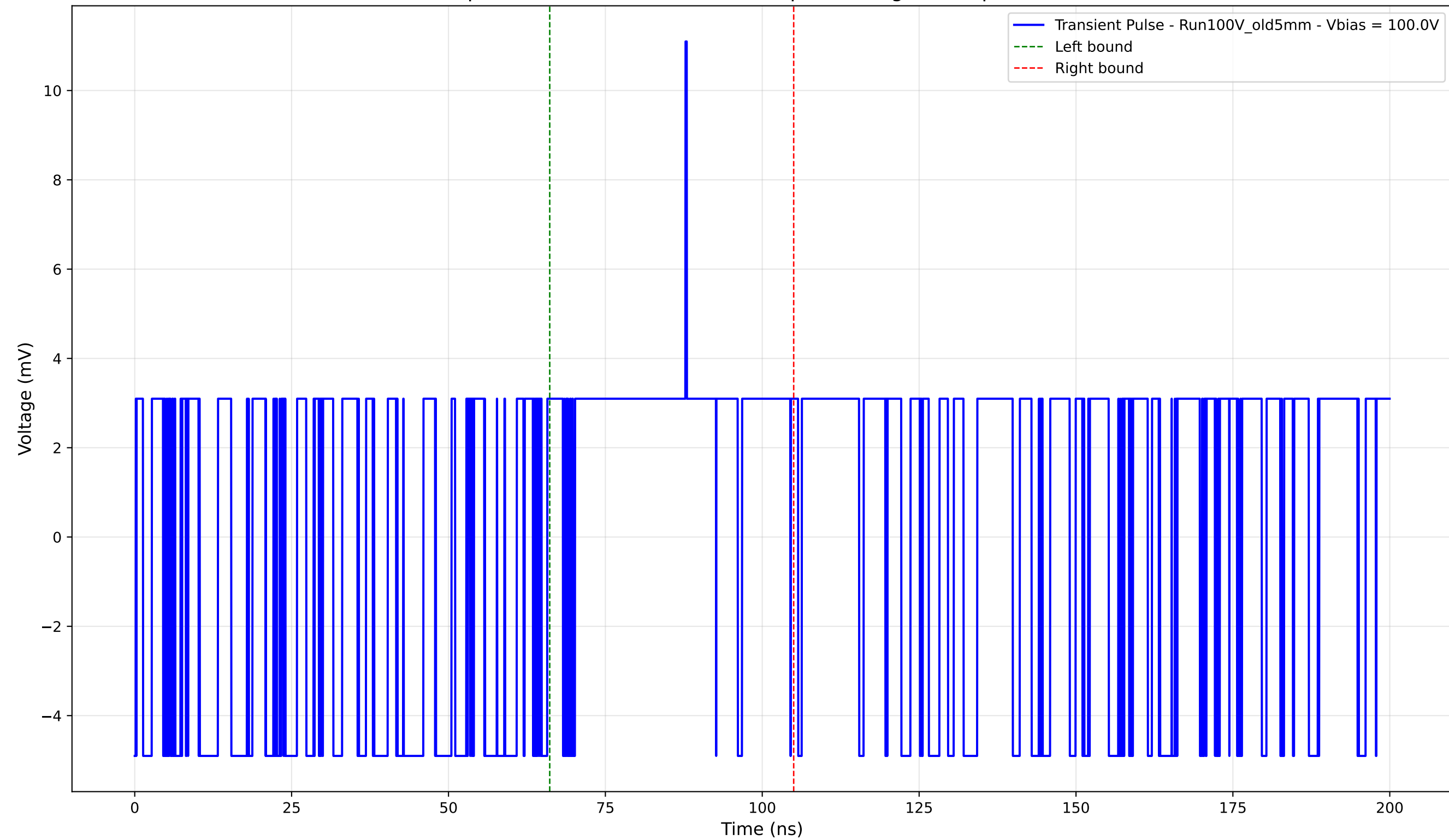
Transient Pulse - Sample: Old5mm - Position: 1535.0 \mu\text{m} - Charge: 2.11 pC - Rise Time: 0.00 ns (N/A)
