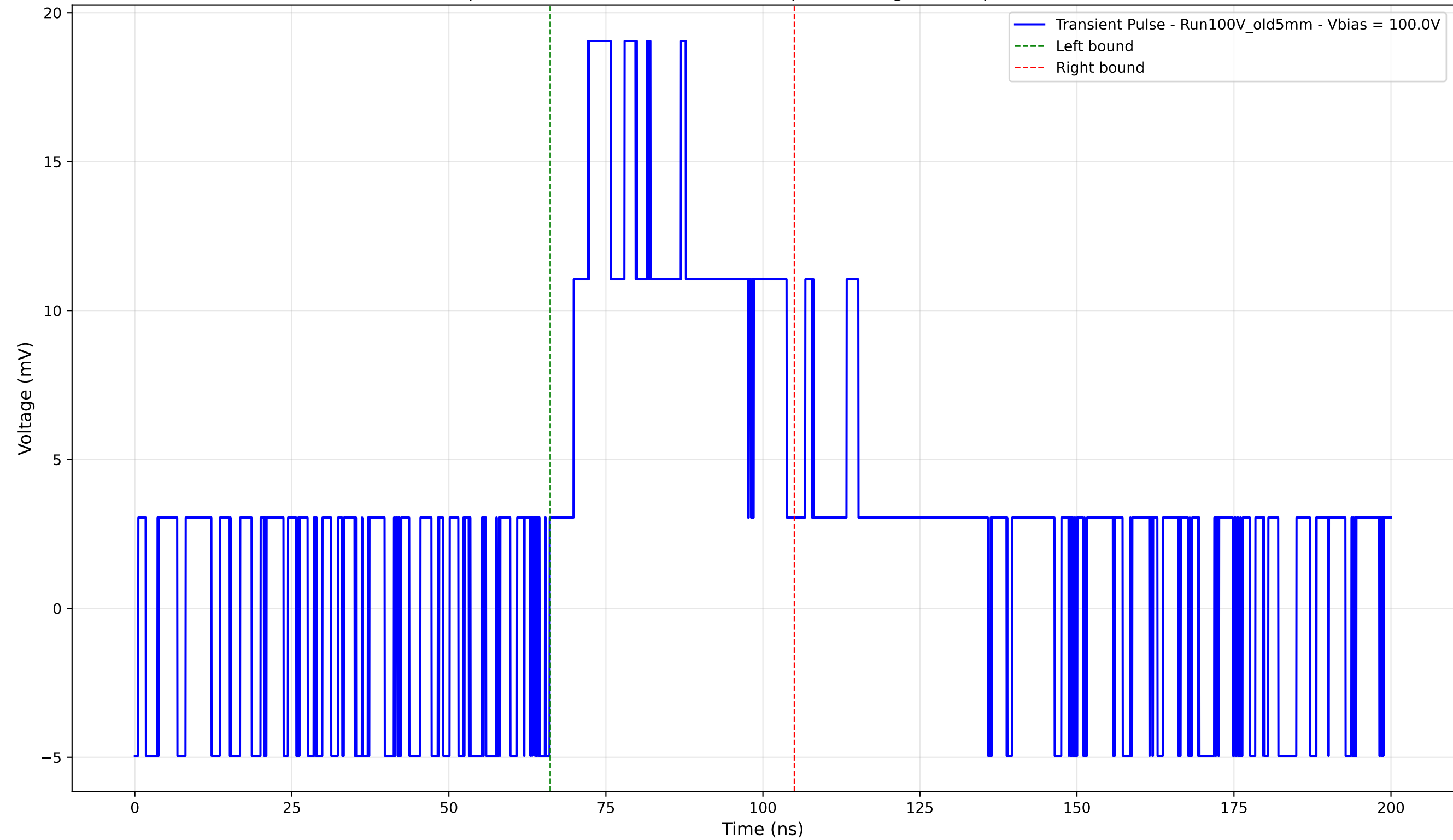
Transient Pulse - Sample: Old5mm - Position: 1840.0 \mu\text{m} - Charge: 8.80 pC - Rise Time: 0.00 ns (N/A)
