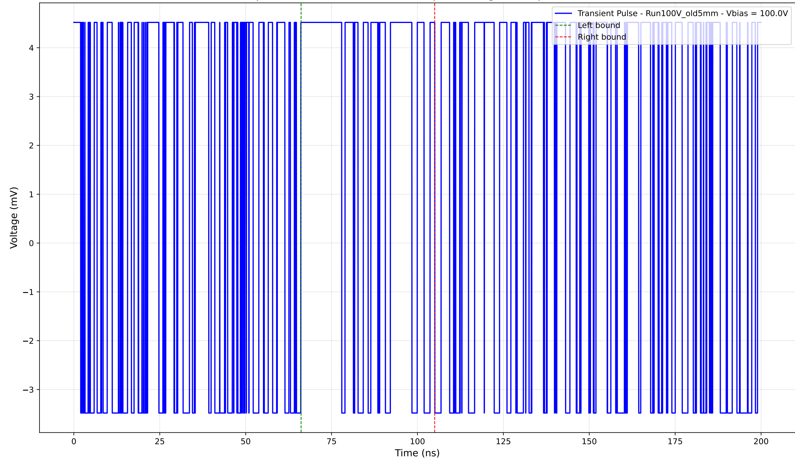
Transient Pulse - Sample: Old5mm - Position: 3405.0 \mu\text{m} - Charge: 2.08 pC - Rise Time: 0.00 ns (N/A)
