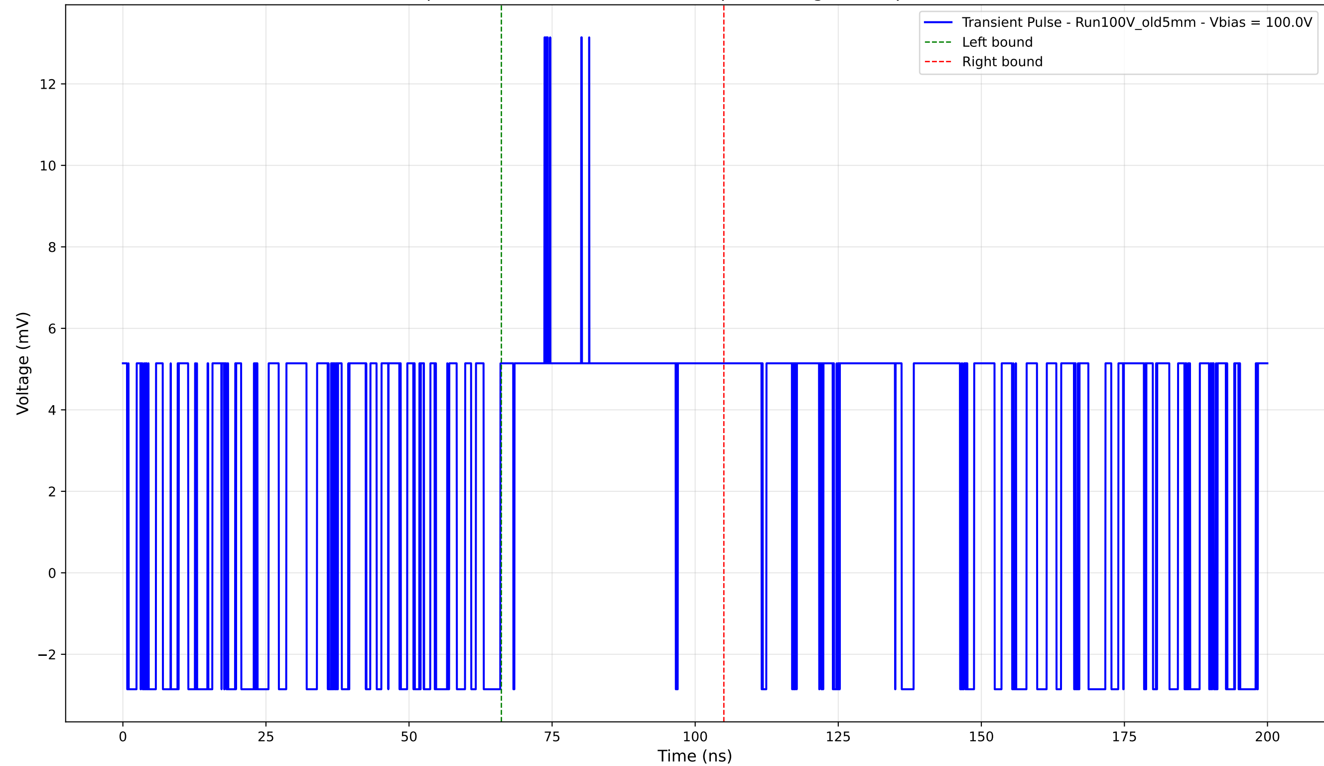
Transient Pulse - Sample: Old5mm - Position: 1735.0 \mu\text{m} - Charge: 4.01 pC - Rise Time: 0.00 ns (N/A)
