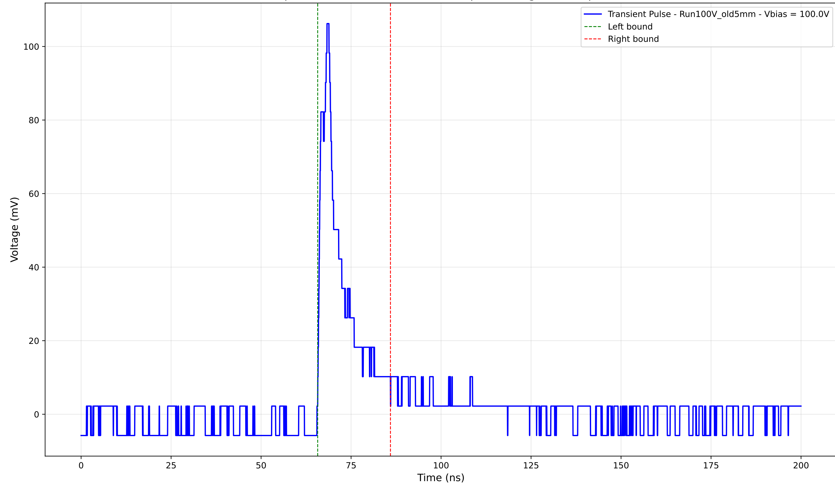
Transient Pulse - Sample: Old5mm - Position: 4110.0 \mu\text{m} - Charge: 13.84 pC - Rise Time: 2.26 ns
