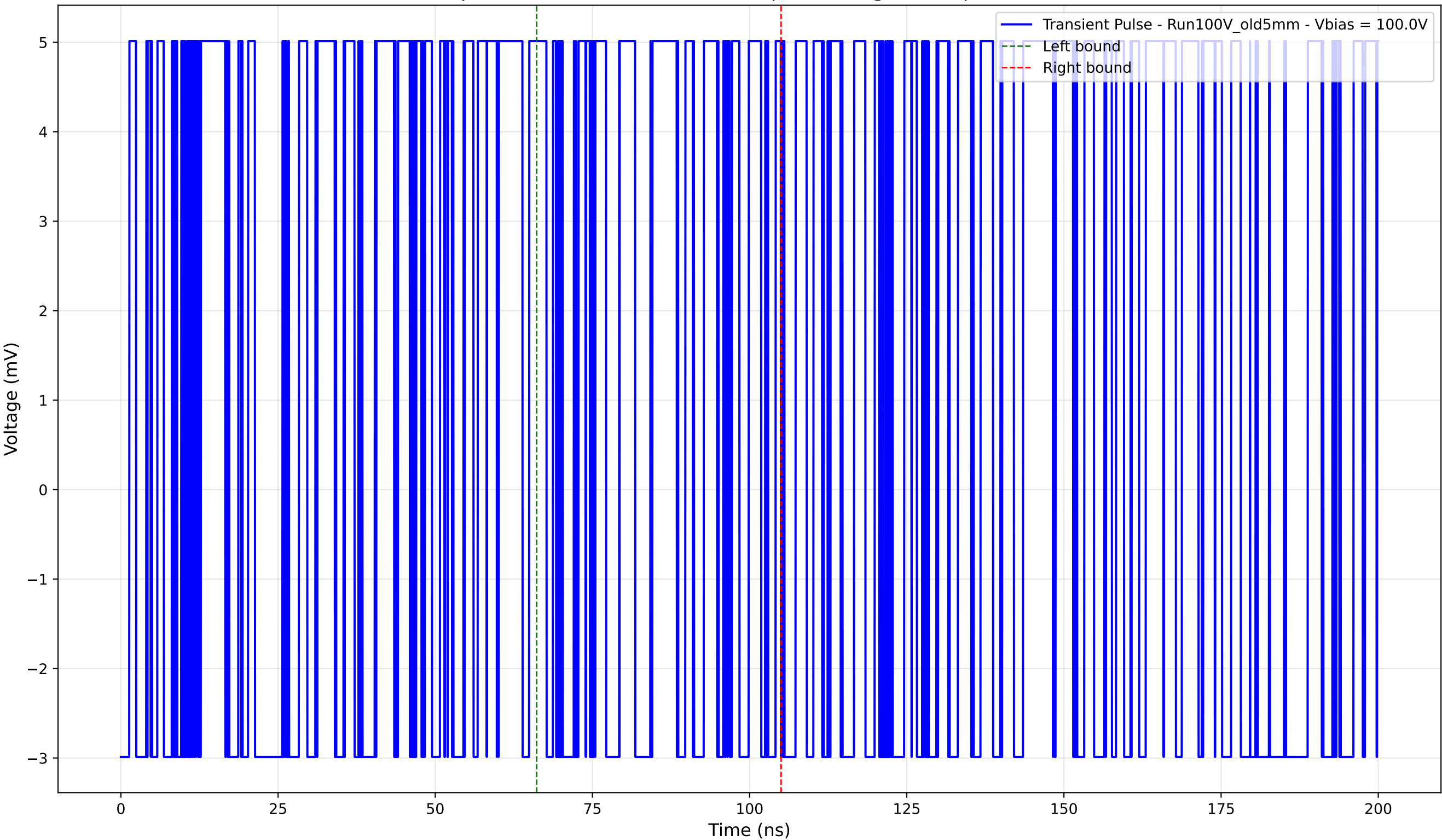
Transient Pulse - Sample: Old5mm - Position: 220.0 \mu\text{m} - Charge: 1.19 pC - Rise Time: 0.00 ns (N/A)
