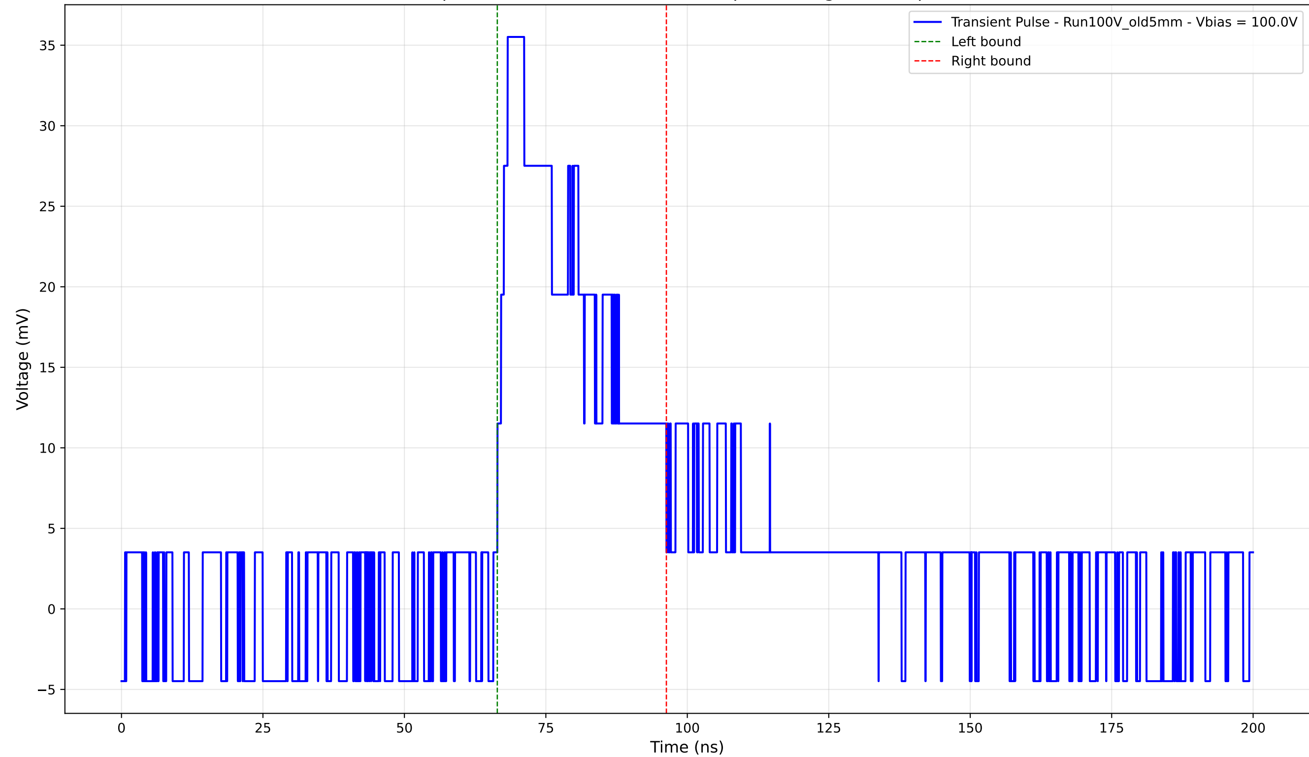
Transient Pulse - Sample: Old5mm - Position: 2695.0 \mu\text{m} - Charge: 11.88 pC - Rise Time: 1.82 ns
