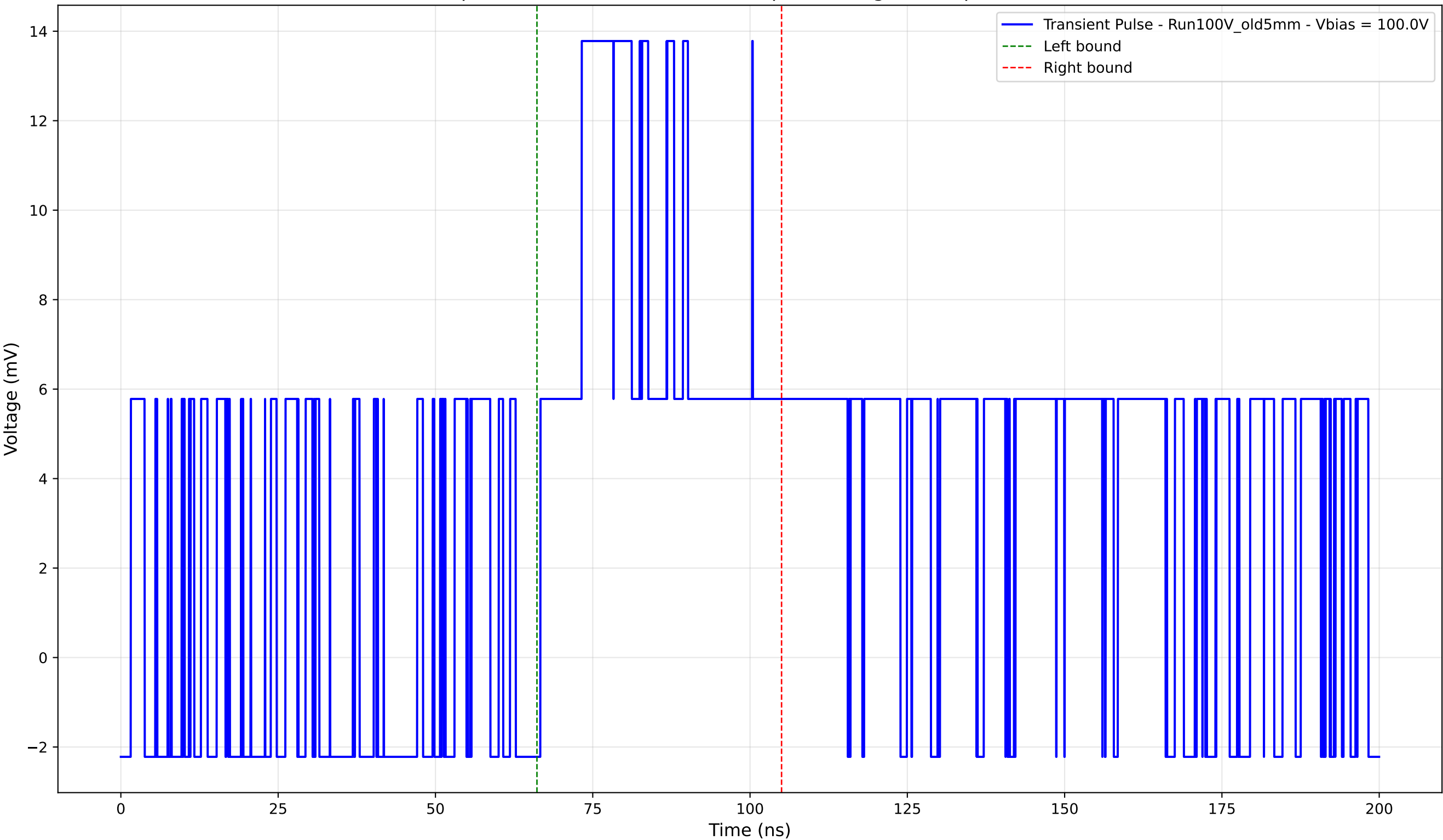
Transient Pulse - Sample: Old5mm - Position: 755.0 \mu\text{m} - Charge: 6.20 pC - Rise Time: 0.00 ns (N/A)
