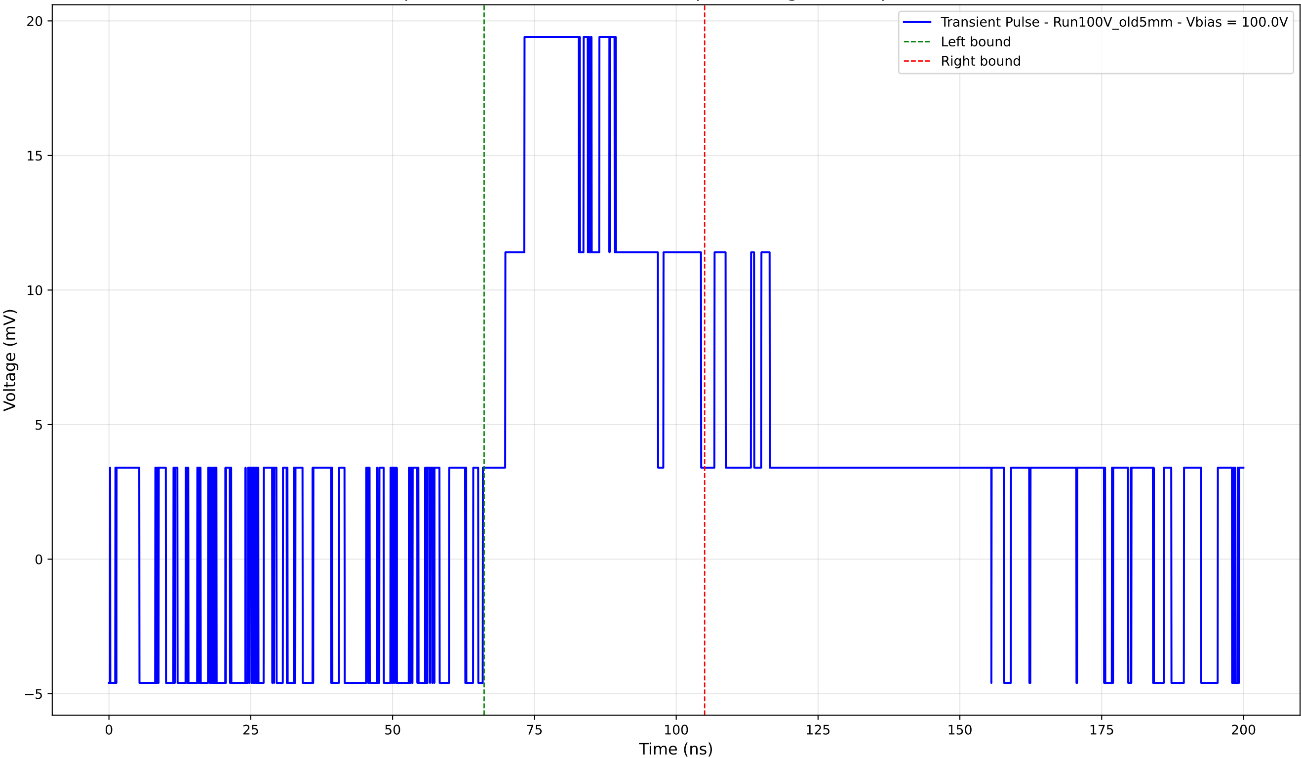
Transient Pulse - Sample: Old5mm - Position: 1820.0 \mu\text{m} - Charge: 10.19 pC - Rise Time: 0.00 ns (N/A)
