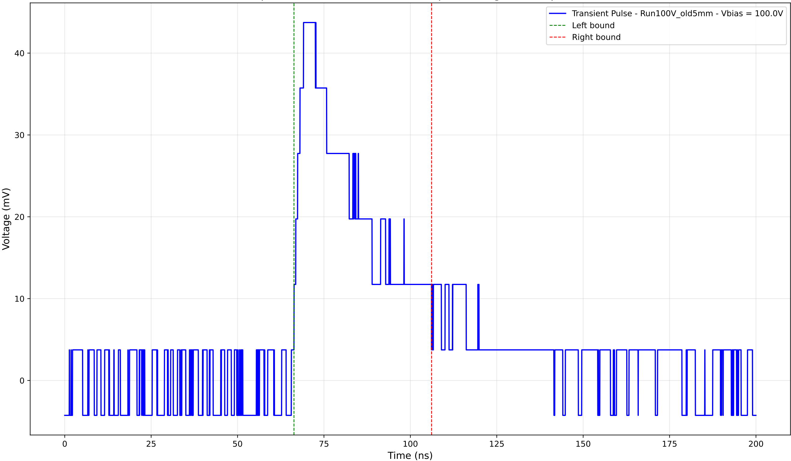
Transient Pulse - Sample: Old5mm - Position: 4870.0 \mu\text{m} - Charge: 17.45 pC - Rise Time: 2.76 ns
