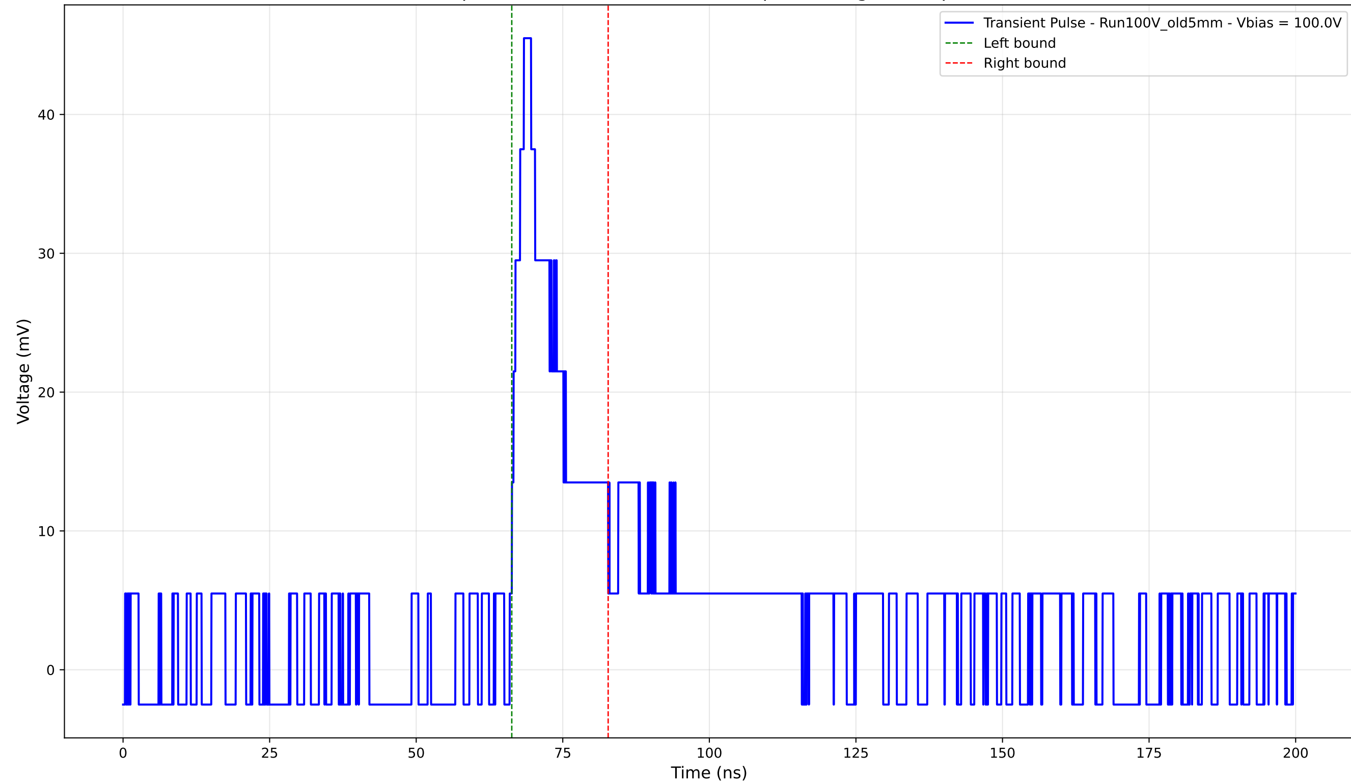
Transient Pulse - Sample: Old5mm - Position: 4385.0 \mu\text{m} - Charge: 7.45 pC - Rise Time: 2.43 ns
