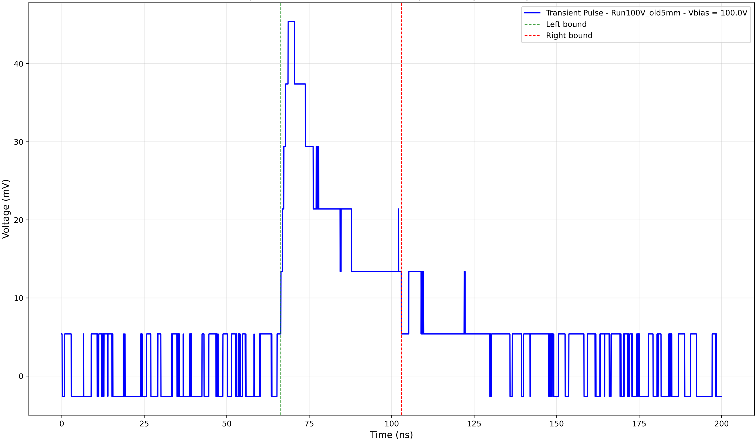
Transient Pulse - Sample: Old5mm - Position: 4720.0 \mu\text{m} - Charge: 15.89 pC - Rise Time: 3.37 ns
