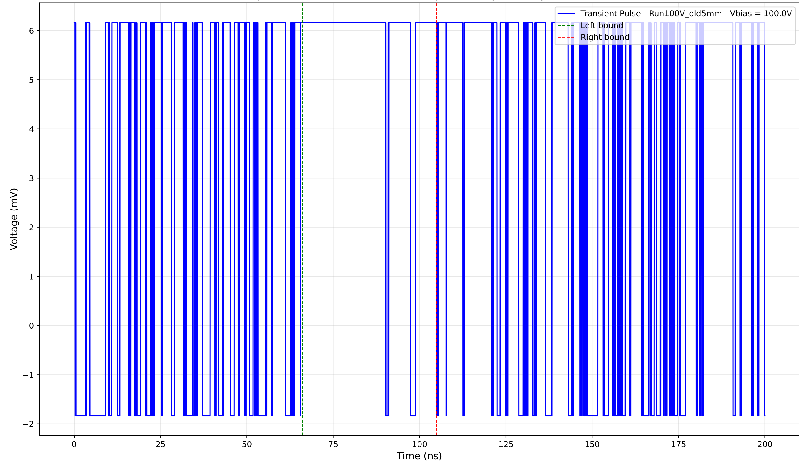
Transient Pulse - Sample: Old5mm - Position: 2330.0 \mu\text{m} - Charge: 4.43 pC - Rise Time: 0.00 ns (N/A)
