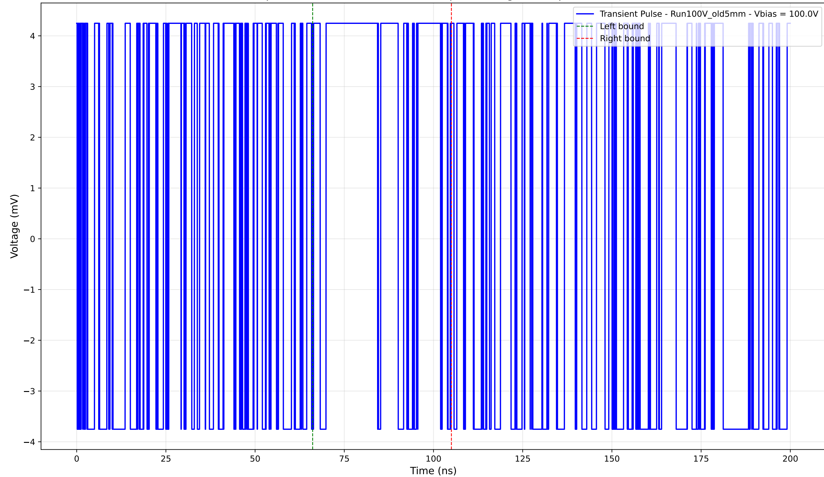
Transient Pulse - Sample: Old5mm - Position: 1905.0 \mu\text{m} - Charge: 2.10 pC - Rise Time: 0.00 ns (N/A)
