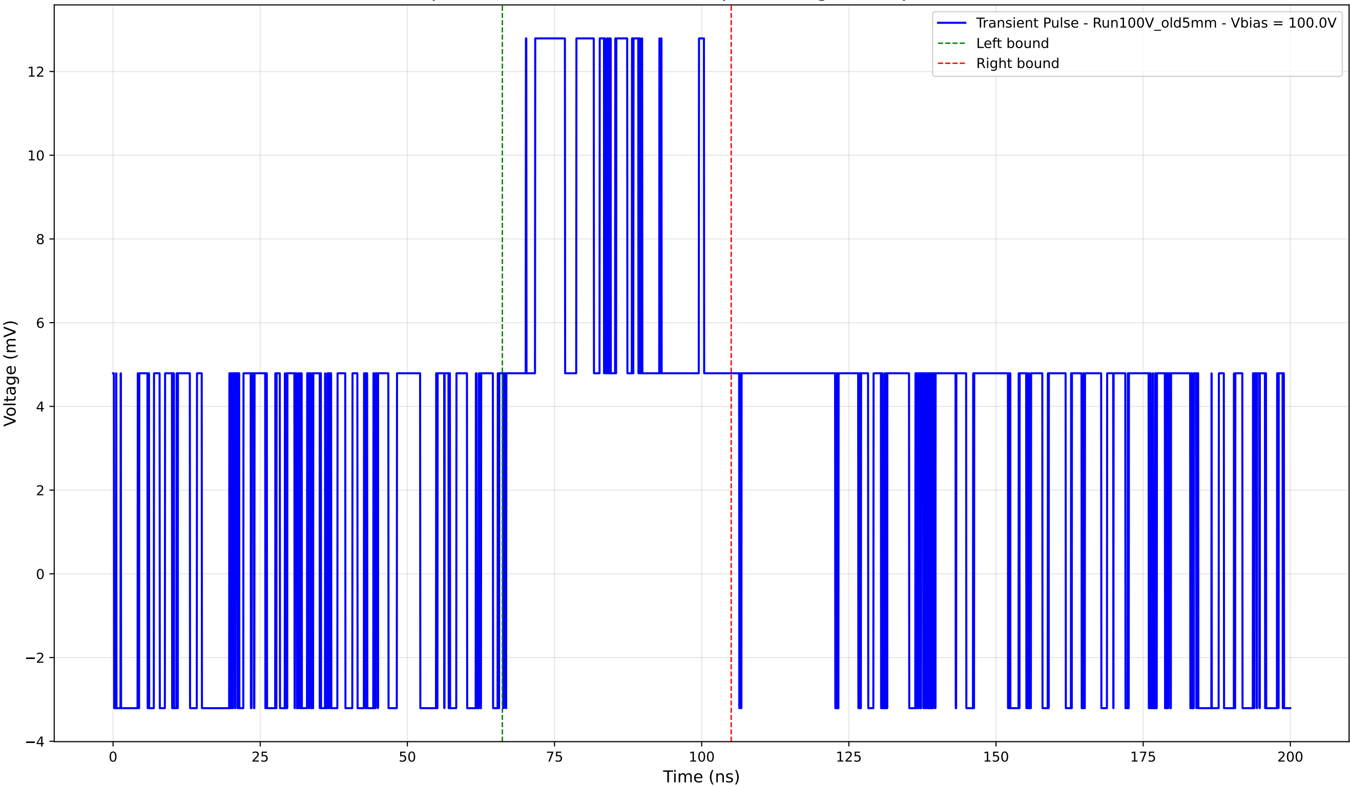
Transient Pulse - Sample: Old5mm - Position: 895.0 \mu\text{m} - Charge: 5.86 pC - Rise Time: 0.00 ns (N/A)
