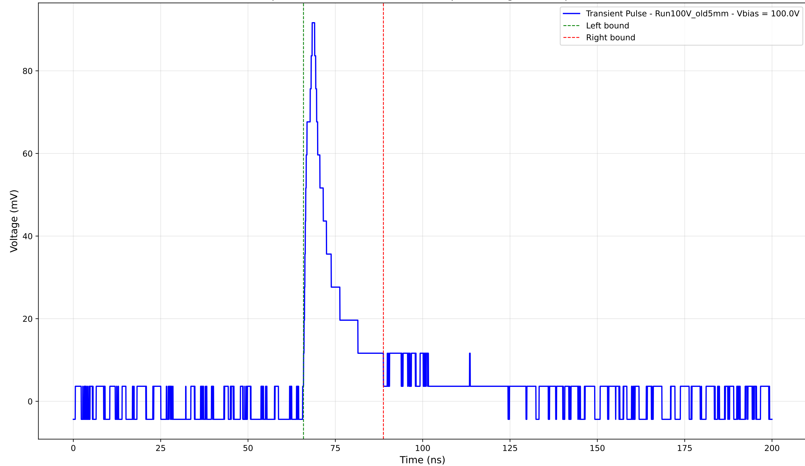
Transient Pulse - Sample: Old5mm - Position: 4205.0 \mu\text{m} - Charge: 14.12 pC - Rise Time: 2.19 ns
