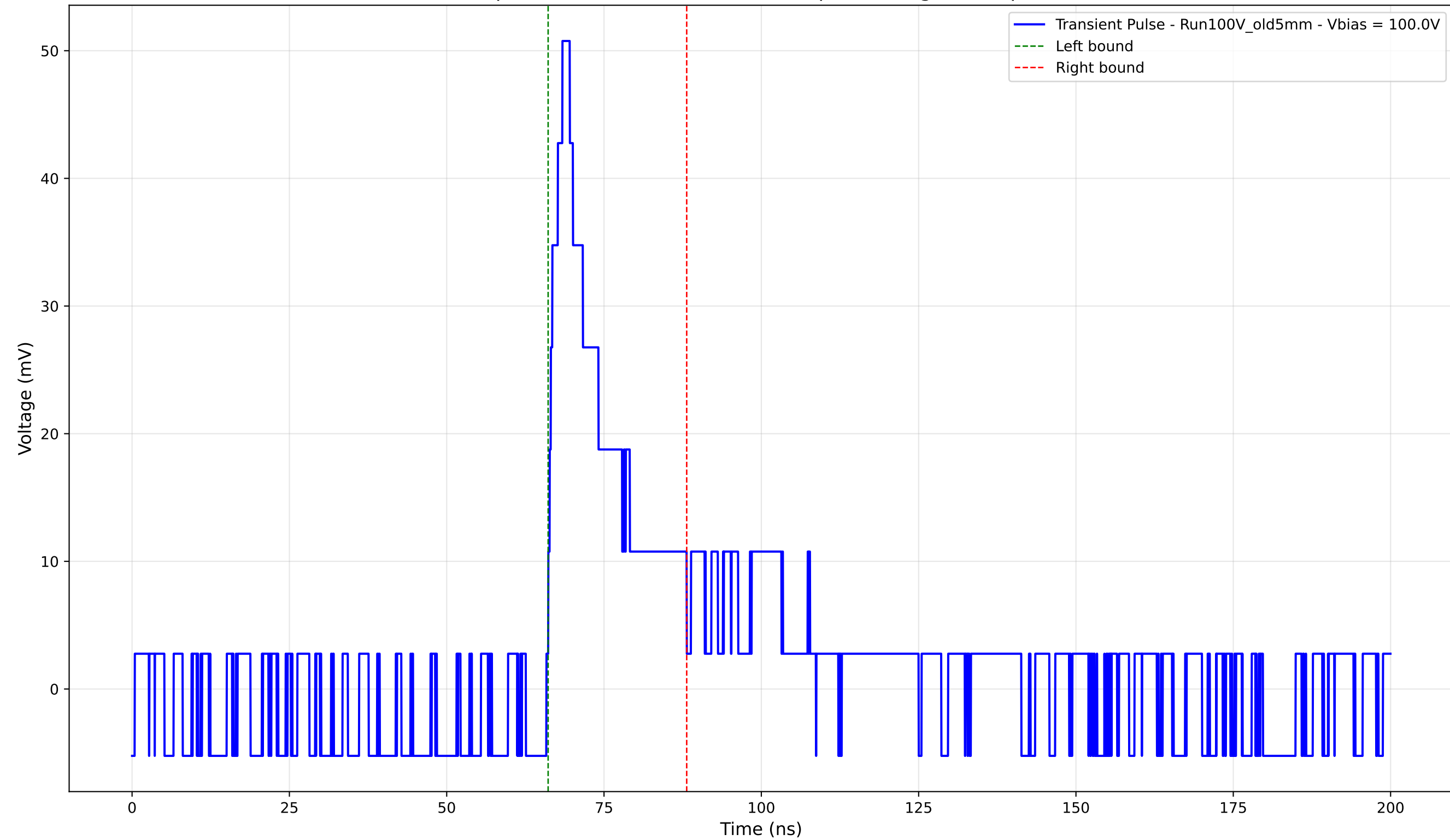
Transient Pulse - Sample: Old5mm - Position: 4395.0 \mu\text{m} - Charge: 9.27 pC - Rise Time: 2.25 ns
