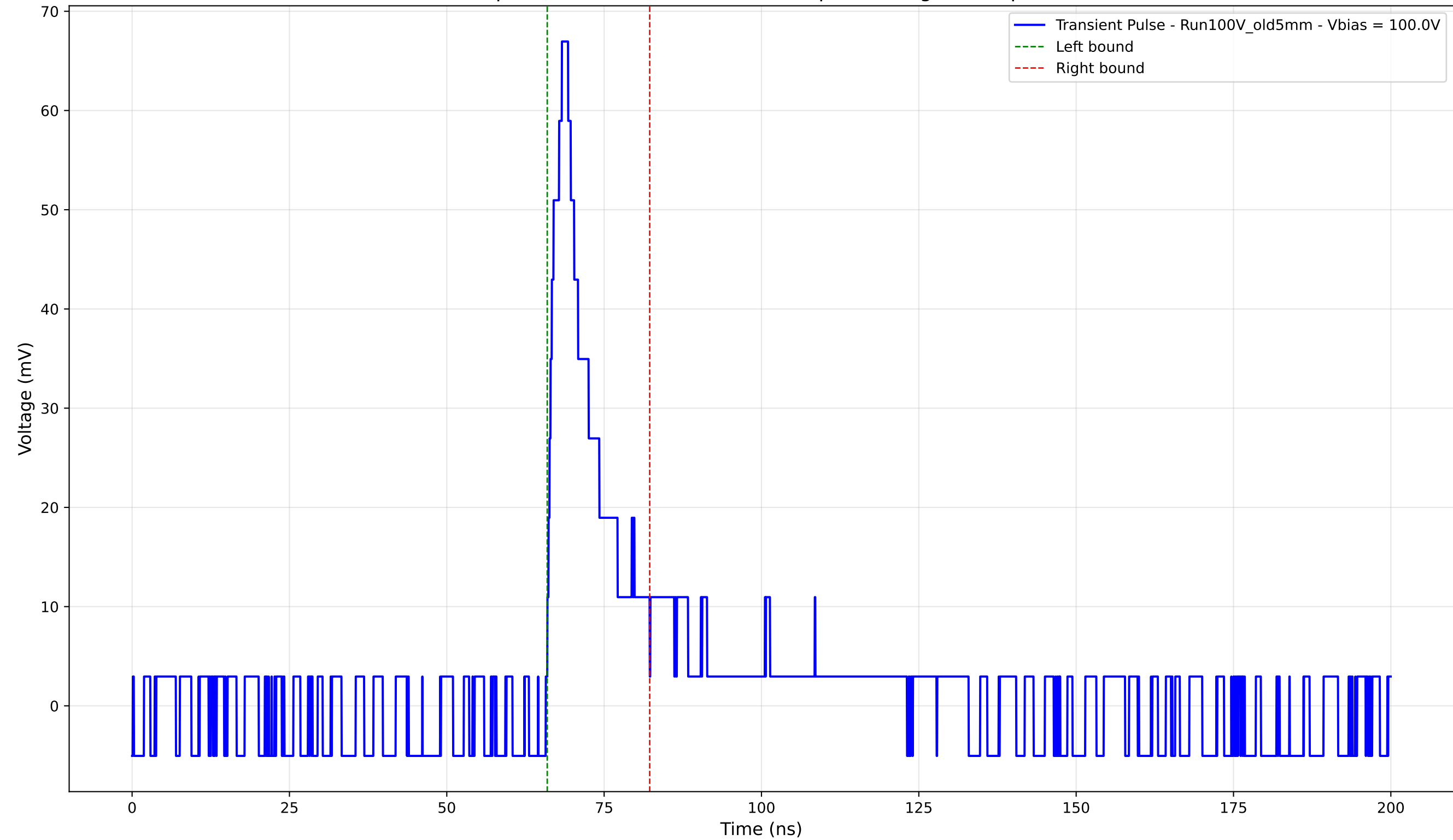
Transient Pulse - Sample: Old5mm - Position: 3185.0 \mu\text{m} - Charge: 9.25 pC - Rise Time: 2.31 ns
