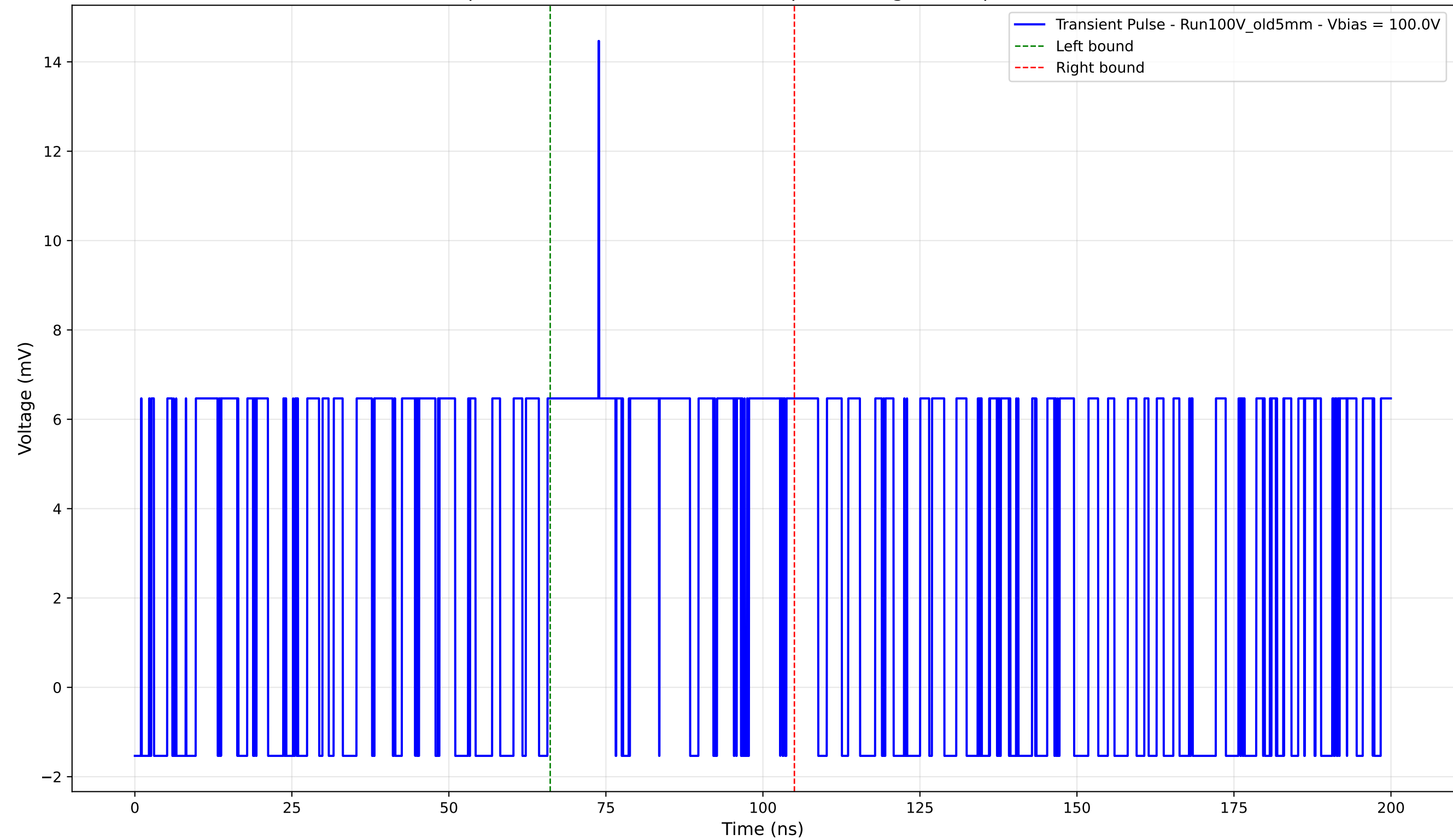
Transient Pulse - Sample: Old5mm - Position: 4645.0 \mu\text{m} - Charge: 4.26 pC - Rise Time: 0.00 ns (N/A)
