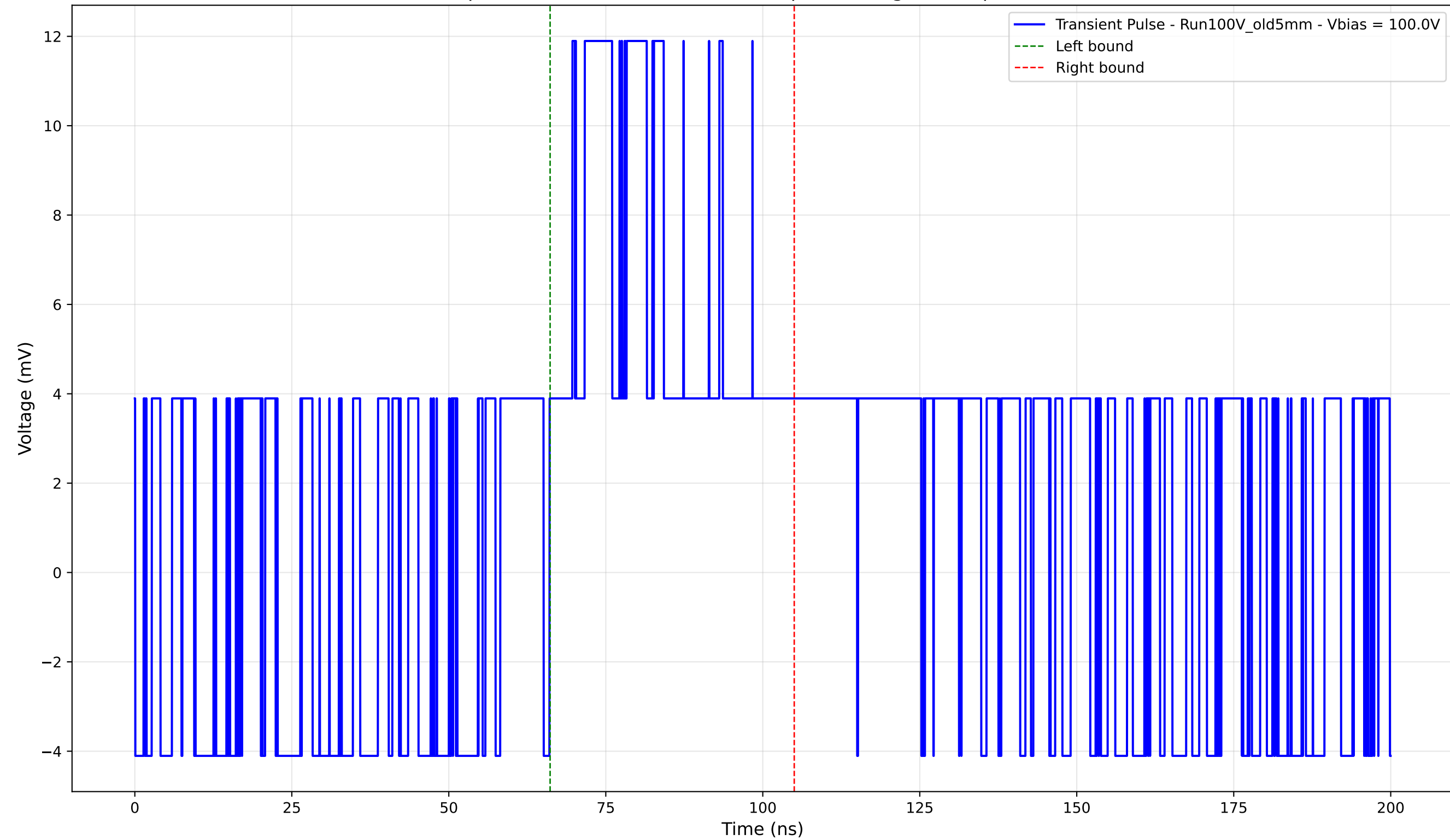
Transient Pulse - Sample: Old5mm - Position: 2150.0 \mu\text{m} - Charge: 4.77 pC - Rise Time: 0.00 ns (N/A)
