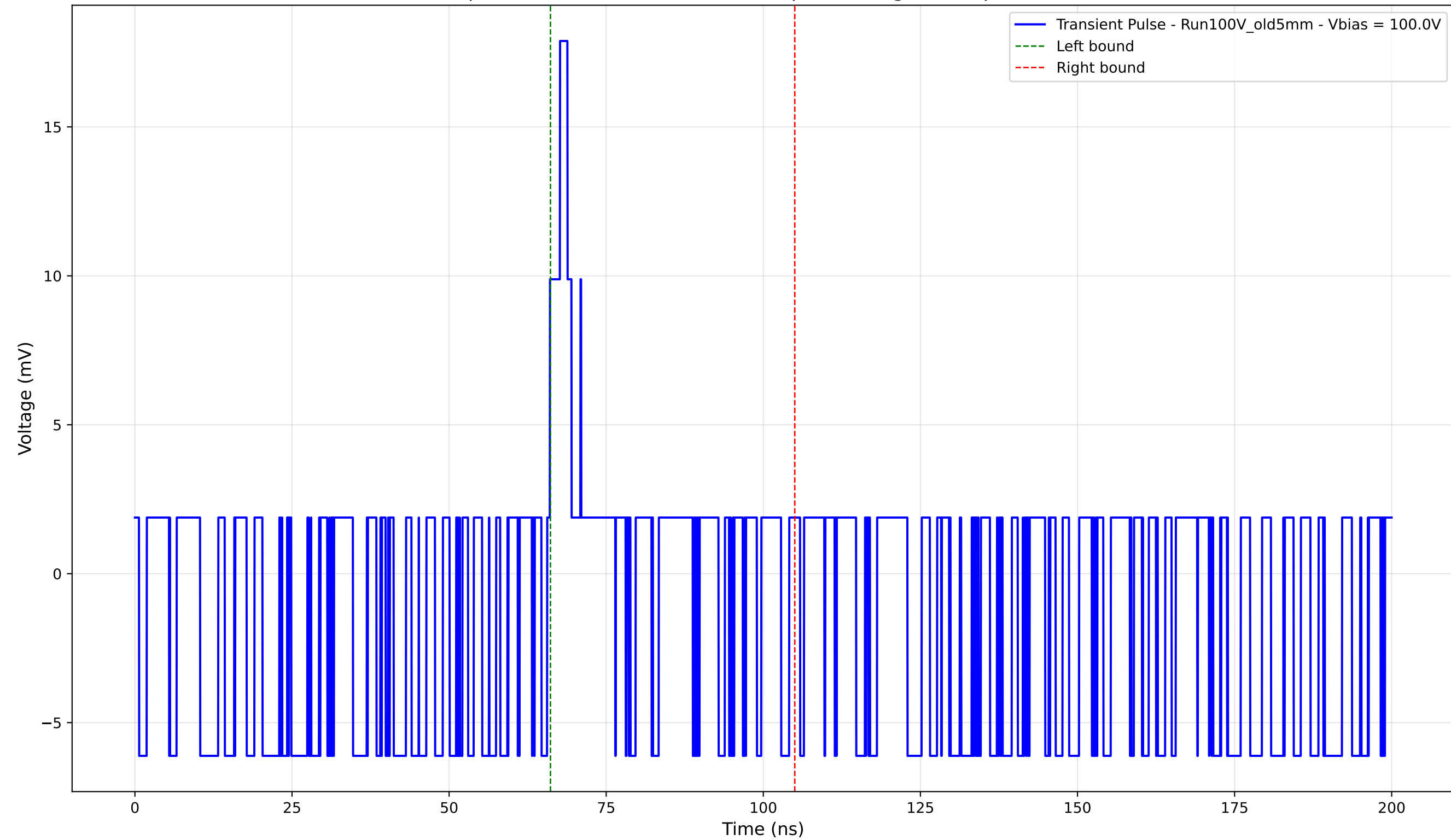
Transient Pulse - Sample: Old5mm - Position: 3980.0 \mu\text{m} - Charge: 1.14 pC - Rise Time: 0.00 ns (N/A)
