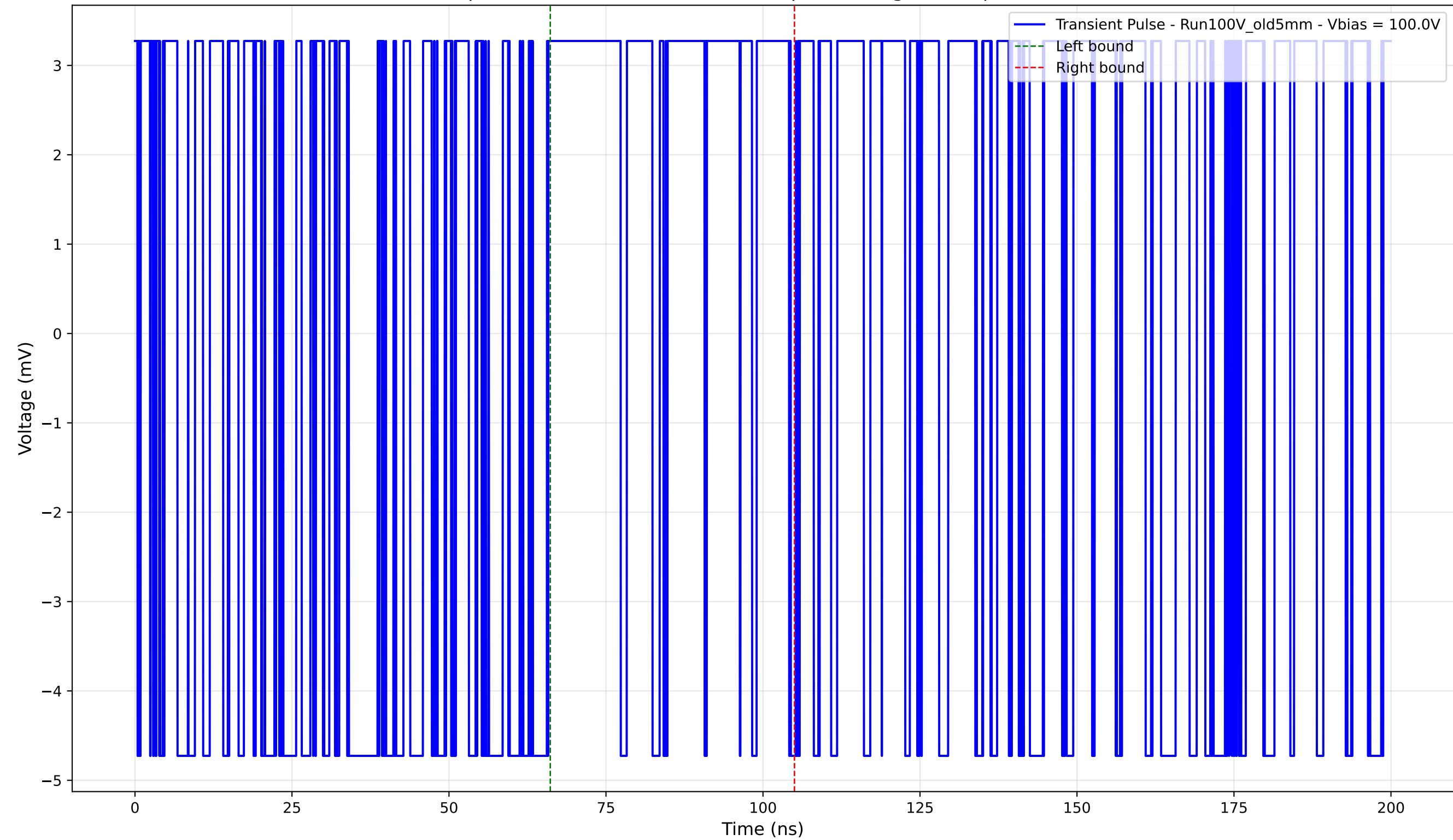
Transient Pulse - Sample: Old5mm - Position: 2765.0 \mu\text{m} - Charge: 1.84 pC - Rise Time: 0.00 ns (N/A)
