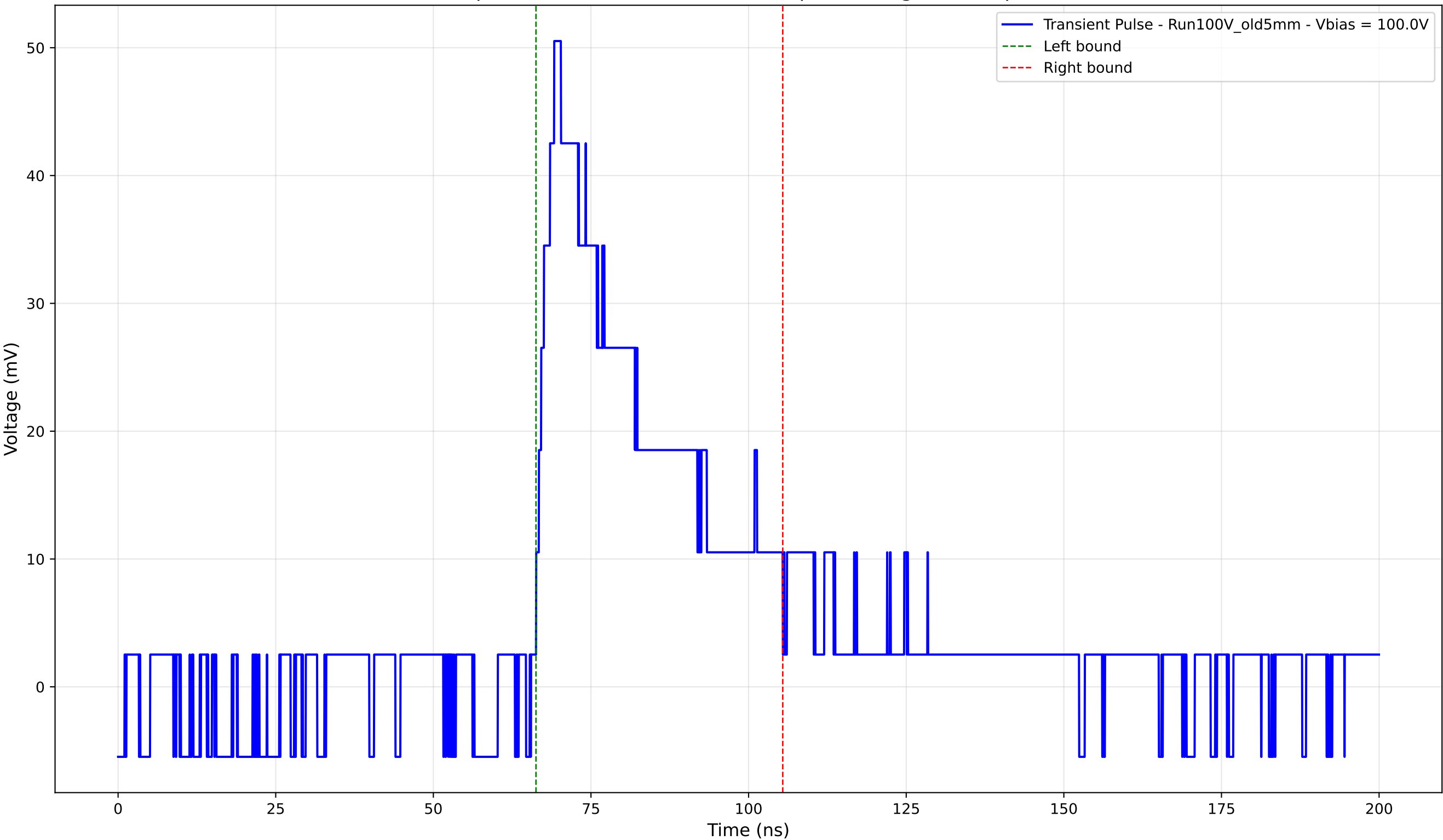
Transient Pulse - Sample: Old5mm - Position: 4795.0 \mu\text{m} - Charge: 17.17 pC - Rise Time: 2.87 ns
