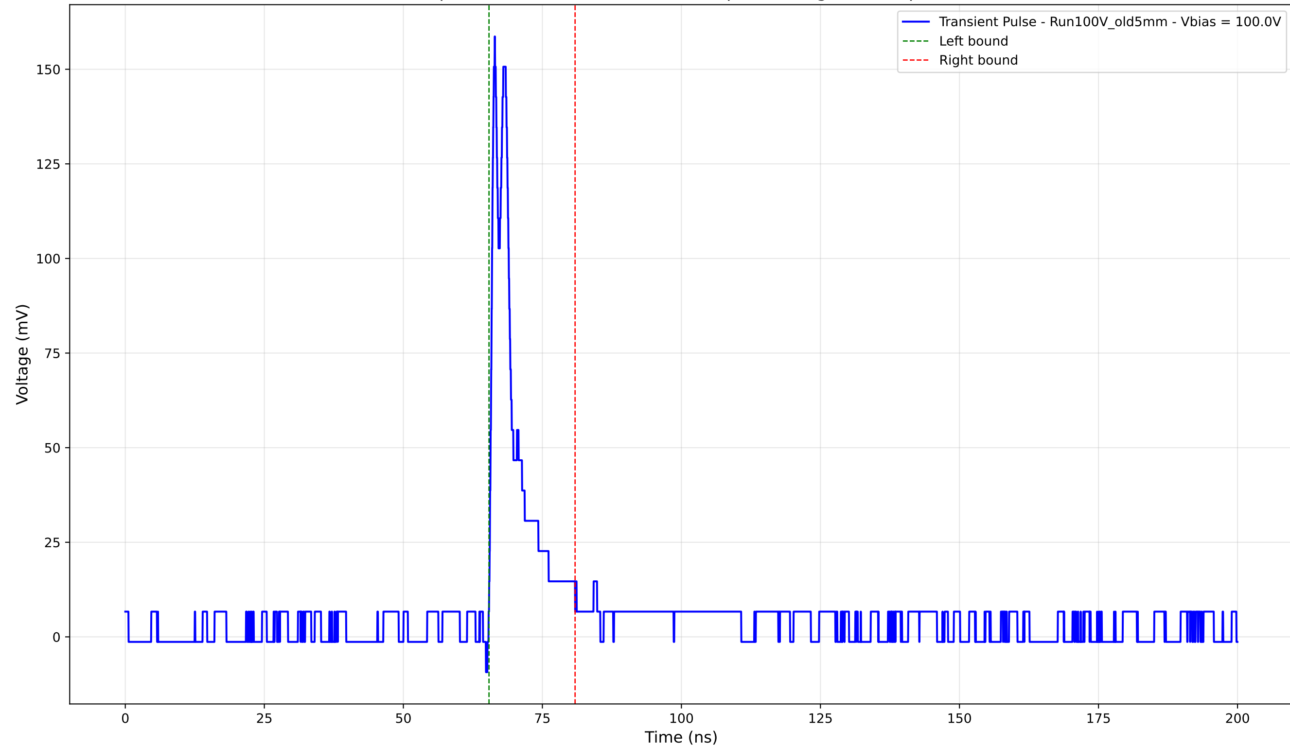
Transient Pulse - Sample: Old5mm - Position: 3625.0 \mu\text{m} - Charge: 15.12 pC - Rise Time: 0.78 ns
