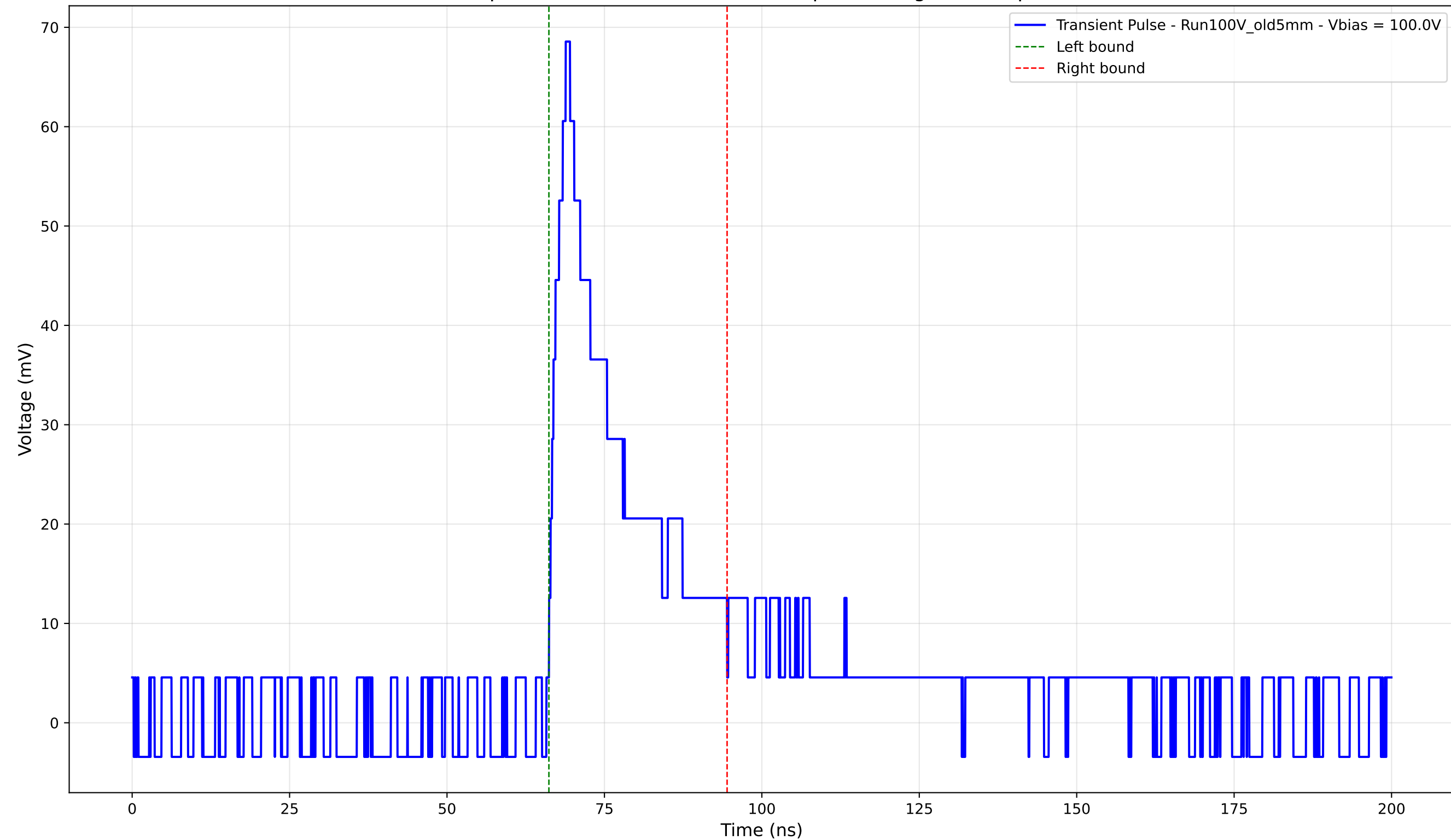
Transient Pulse - Sample: Old5mm - Position: 4495.0 \mu\text{m} - Charge: 15.32 pC - Rise Time: 2.65 ns
