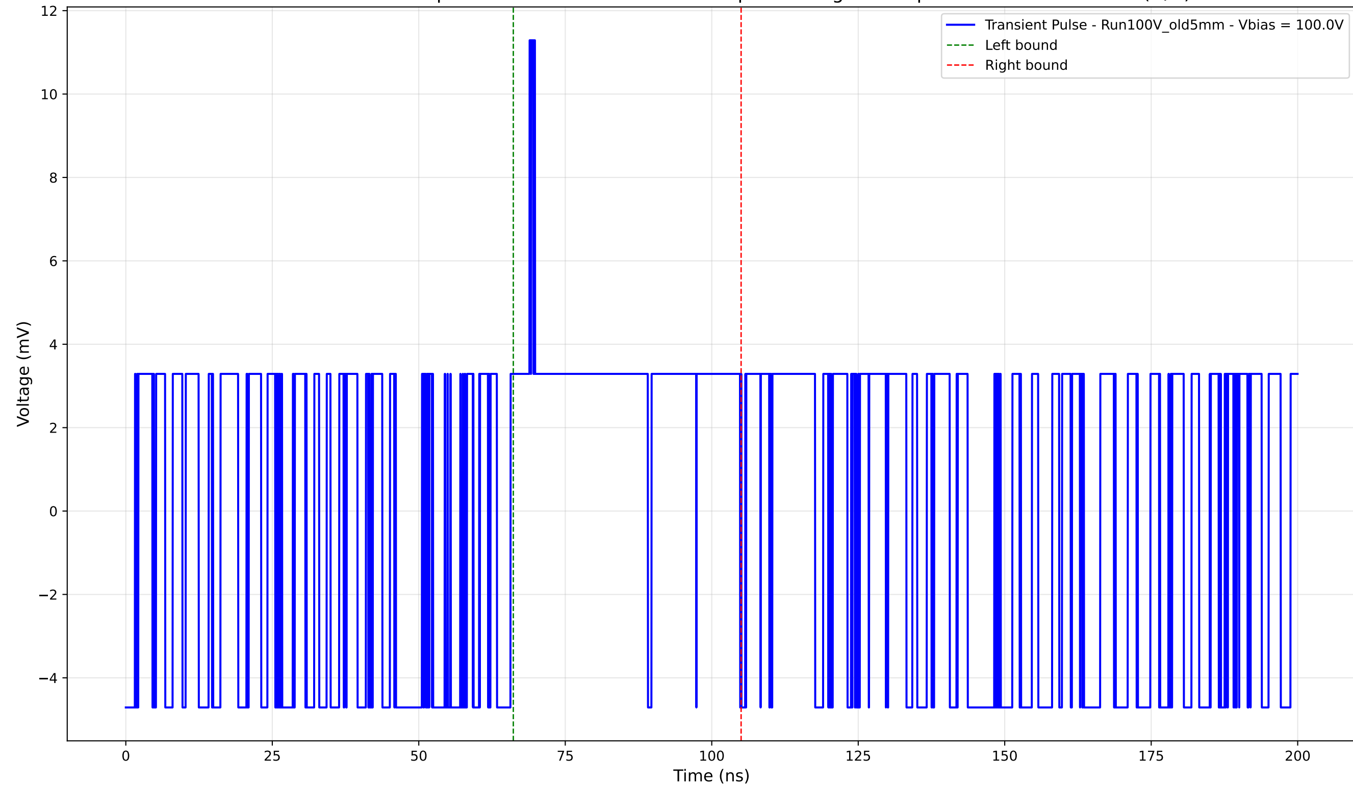
Transient Pulse - Sample: Old5mm - Position: 4655.0 \mu\text{m} - Charge: 2.54 pC - Rise Time: 0.00 ns (N/A)
