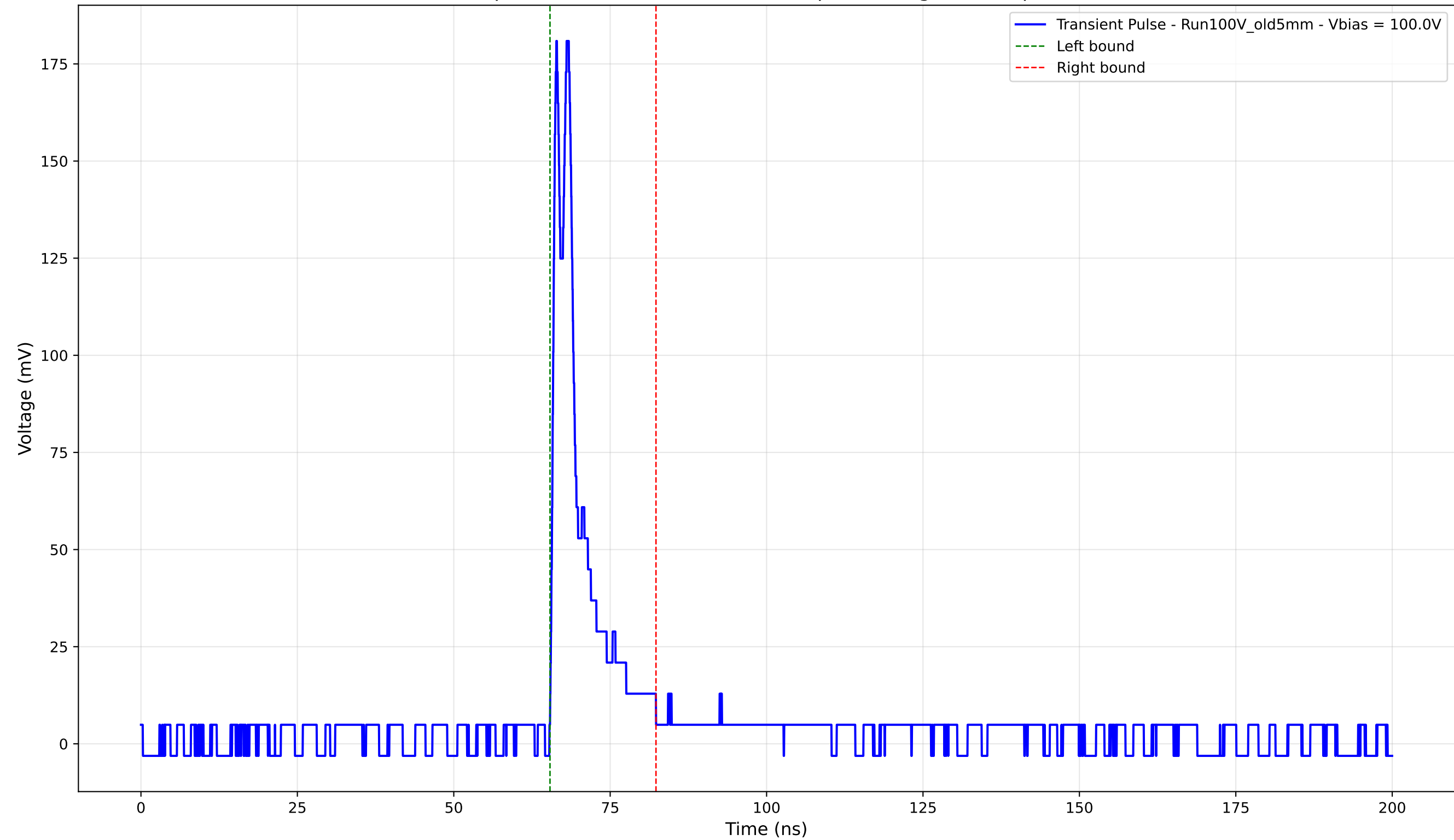
Transient Pulse - Sample: Old5mm - Position: 3805.0 \mu\text{m} - Charge: 17.63 pC - Rise Time: 0.77 ns
