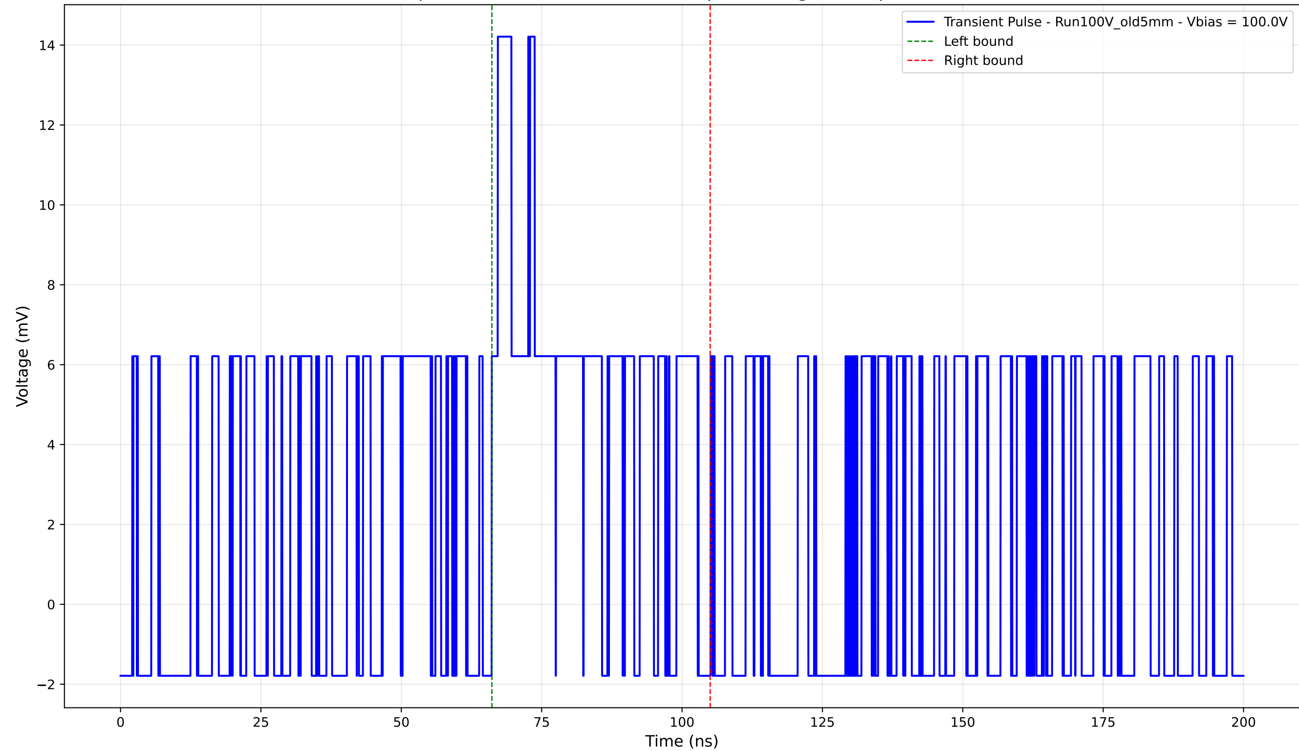
Transient Pulse - Sample: Old5mm - Position: 4345.0 \mu\text{m} - Charge: 4.24 pC - Rise Time: 0.00 ns (N/A)
