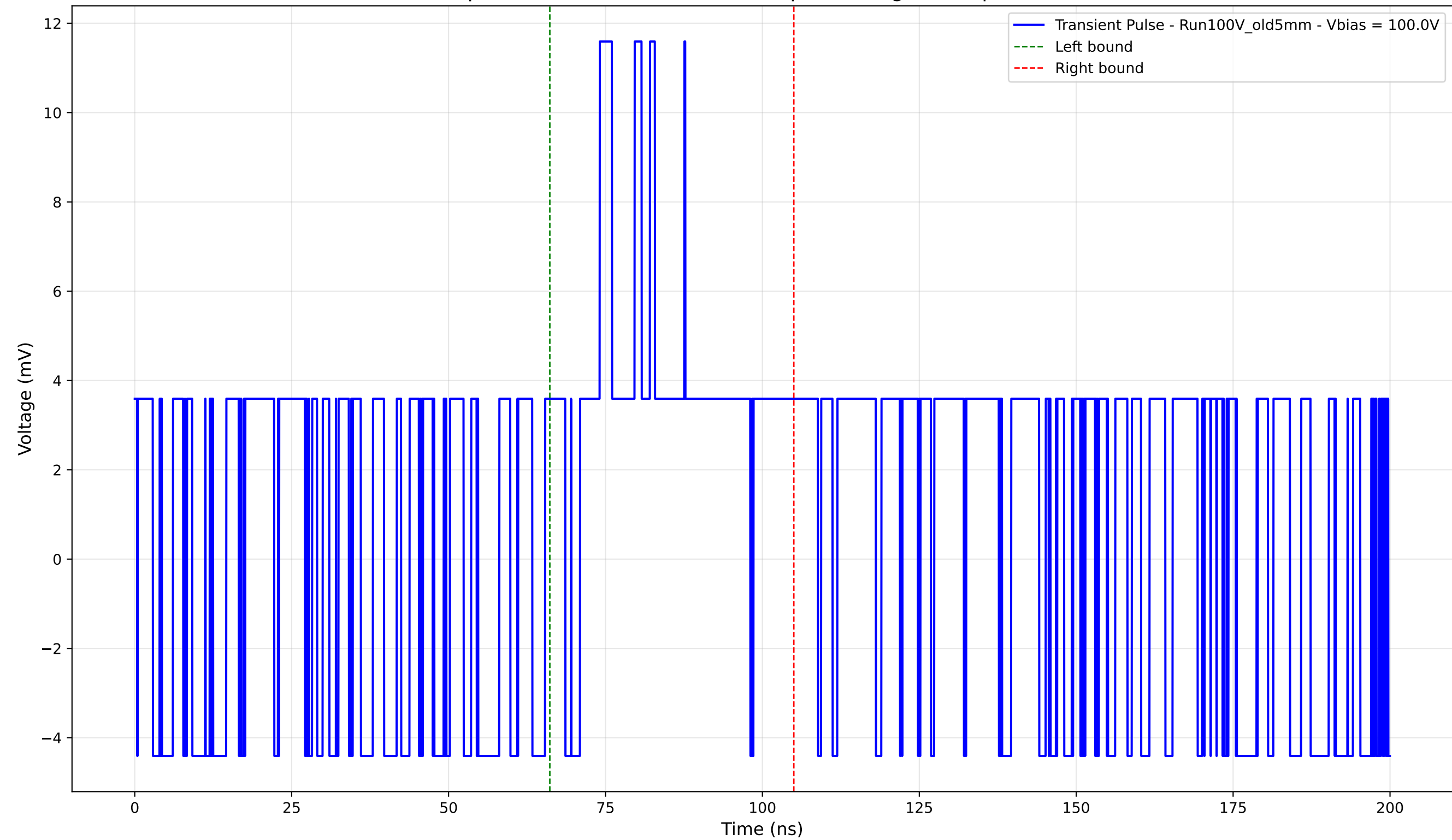
Transient Pulse - Sample: Old5mm - Position: 1745.0 \mu\text{m} - Charge: 3.00 pC - Rise Time: 0.00 ns (N/A)
