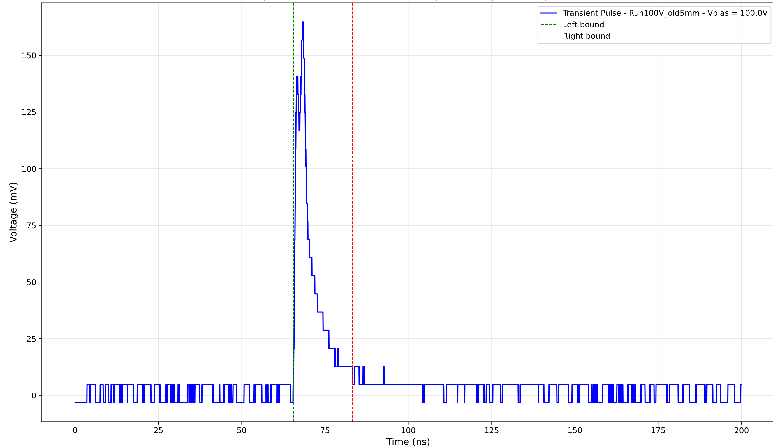
Transient Pulse - Sample: Old5mm - Position: 3905.0 \mu\text{m} - Charge: 17.58 pC - Rise Time: 2.29 ns
