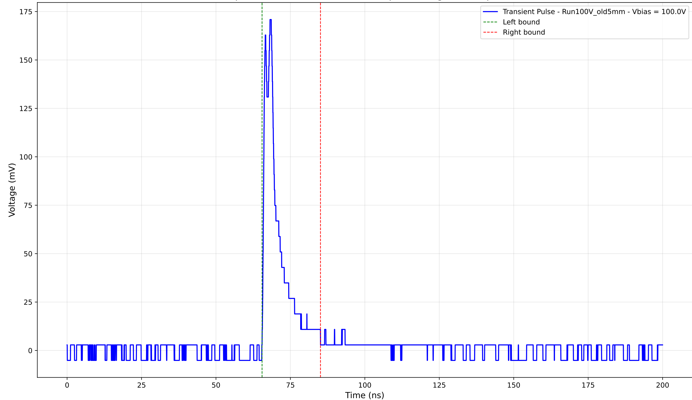
Transient Pulse - Sample: Old5mm - Position: 3525.0 \mu\text{m} - Charge: 18.81 pC - Rise Time: 0.82 ns
