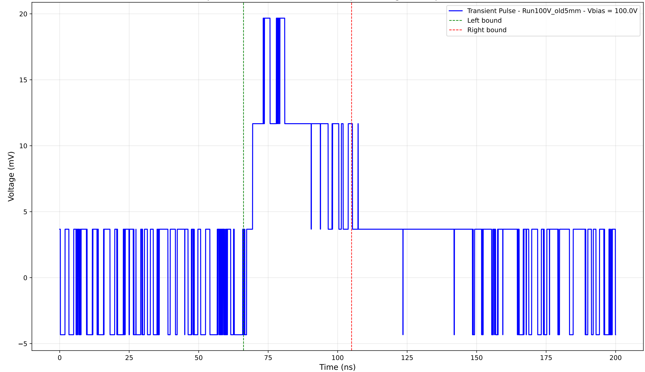
Transient Pulse - Sample: Old5mm - Position: 2055.0 \mu\text{m} - Charge: 8.49 pC - Rise Time: 0.00 ns (N/A)
