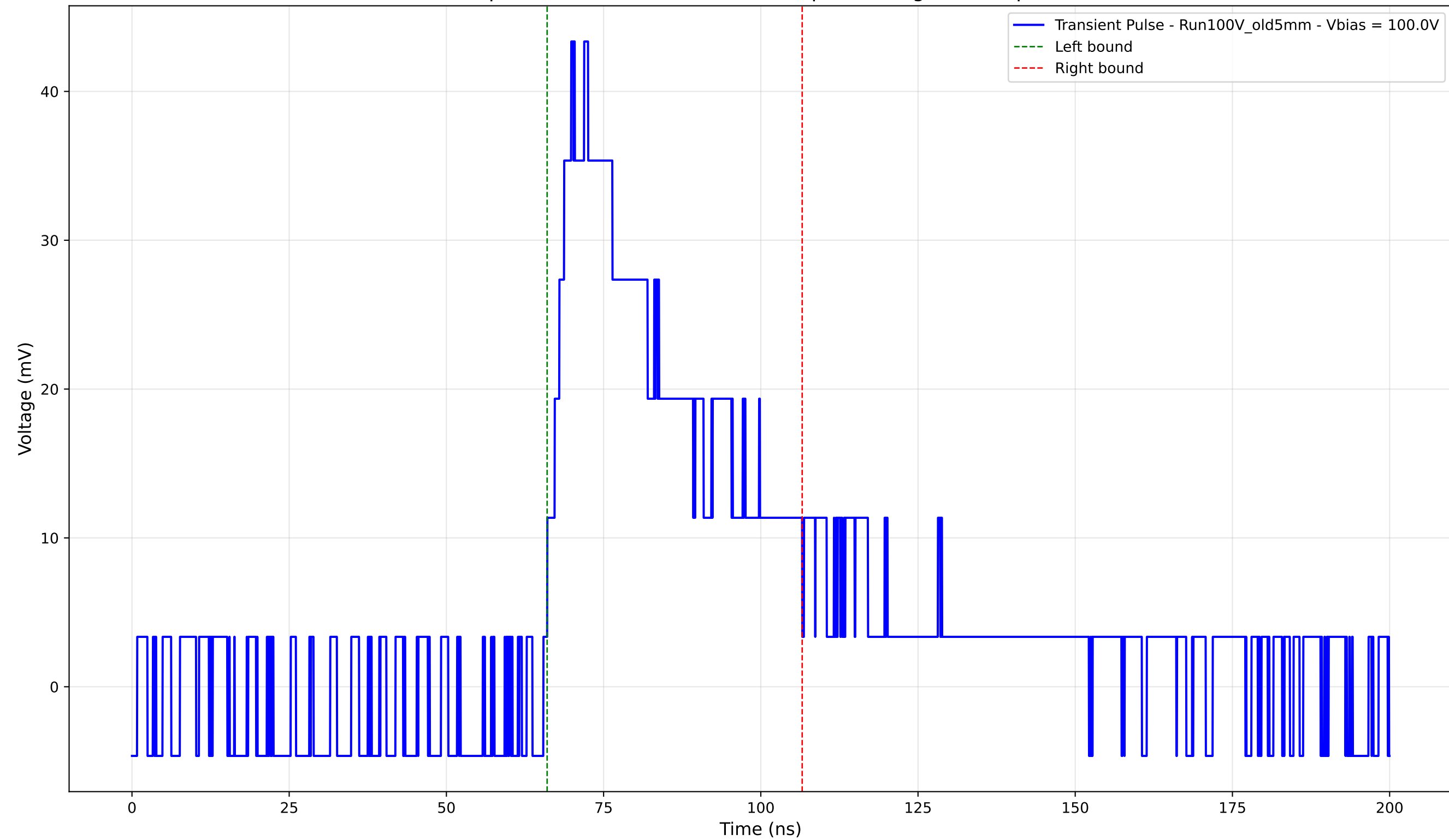
Transient Pulse - Sample: Old5mm - Position: 4925.0 \mu\text{m} - Charge: 17.31 pC - Rise Time: 3.82 ns
