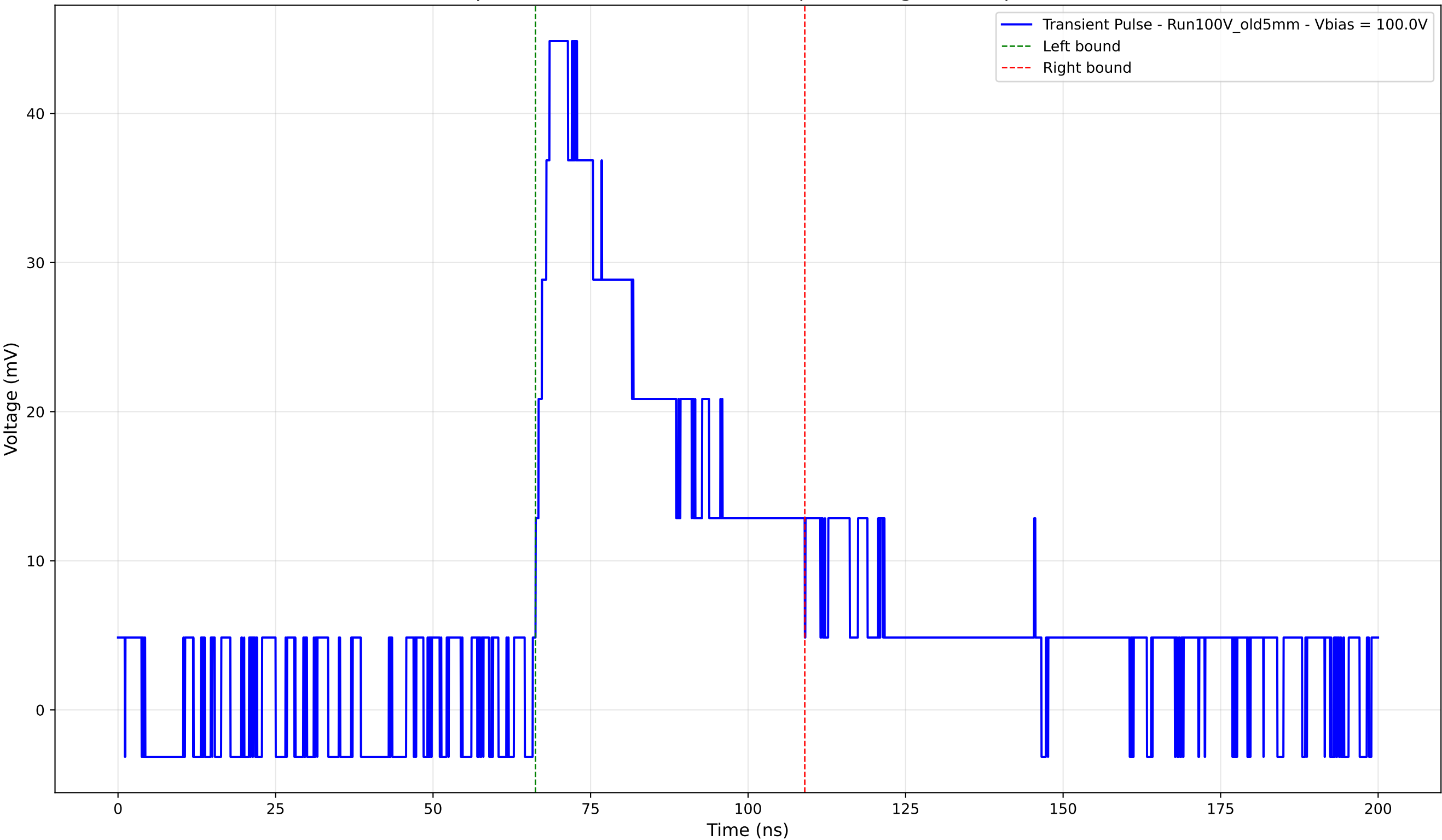
Transient Pulse - Sample: Old5mm - Position: 4810.0 \mu\text{m} - Charge: 19.10 pC - Rise Time: 2.66 ns
