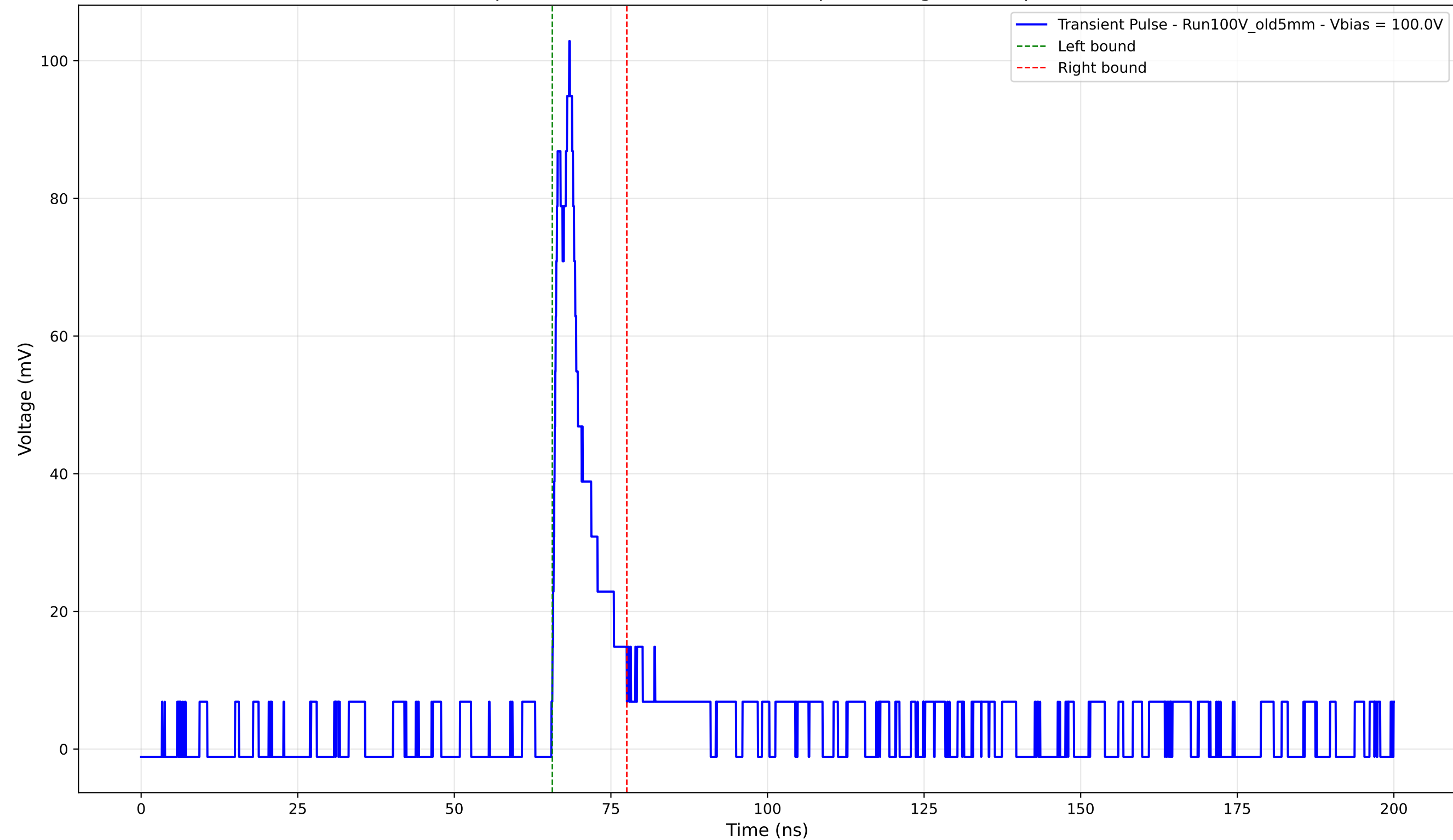
Transient Pulse - Sample: Old5mm - Position: 3480.0 \mu\text{m} - Charge: 10.26 pC - Rise Time: 2.35 ns
