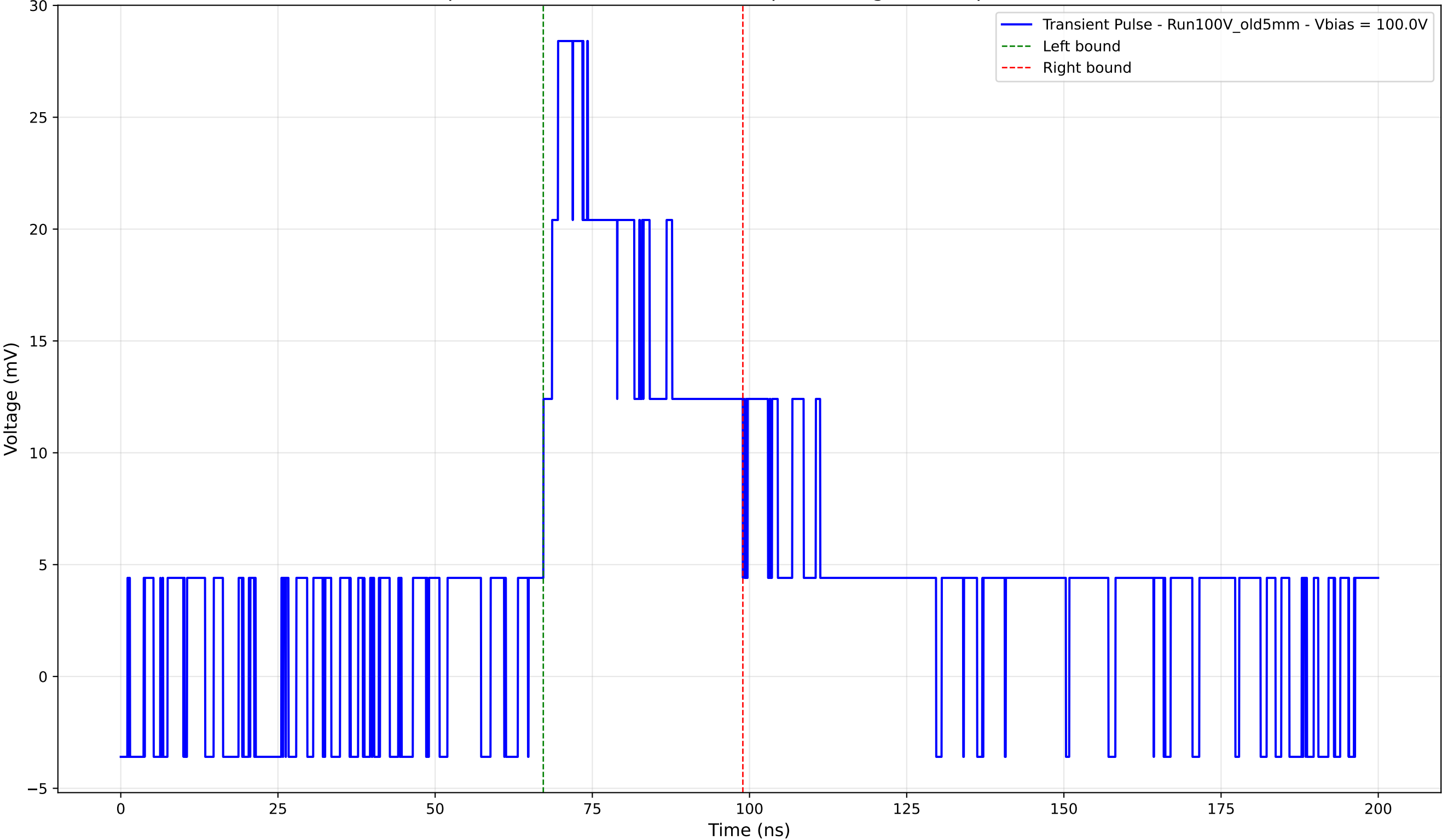
Transient Pulse - Sample: Old5mm - Position: 2455.0 \mu\text{m} - Charge: 10.96 pC - Rise Time: 0.00 ns (N/A)
