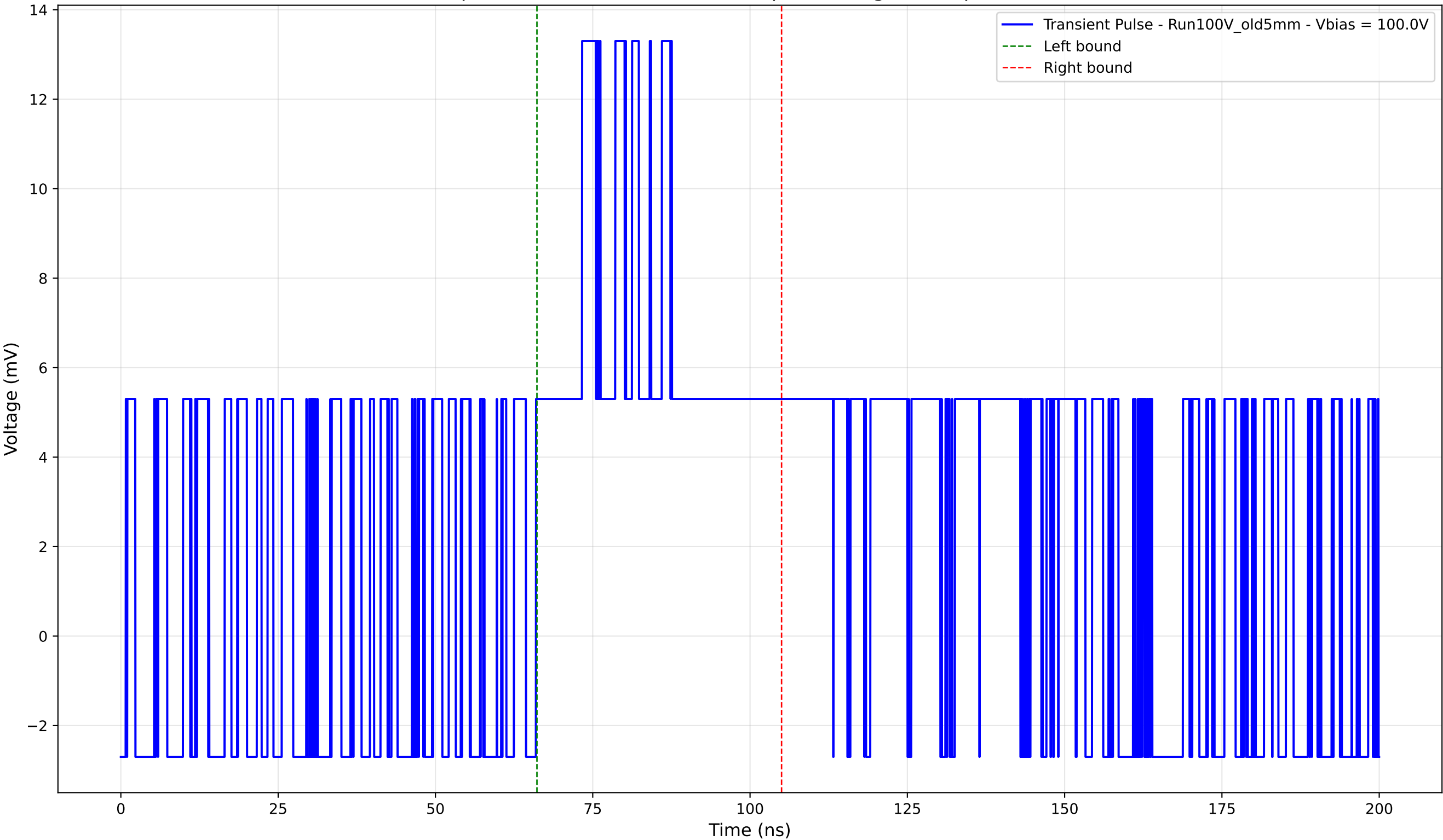
Transient Pulse - Sample: Old5mm - Position: 950.0 \mu\text{m} - Charge: 5.24 pC - Rise Time: 0.00 ns (N/A)
