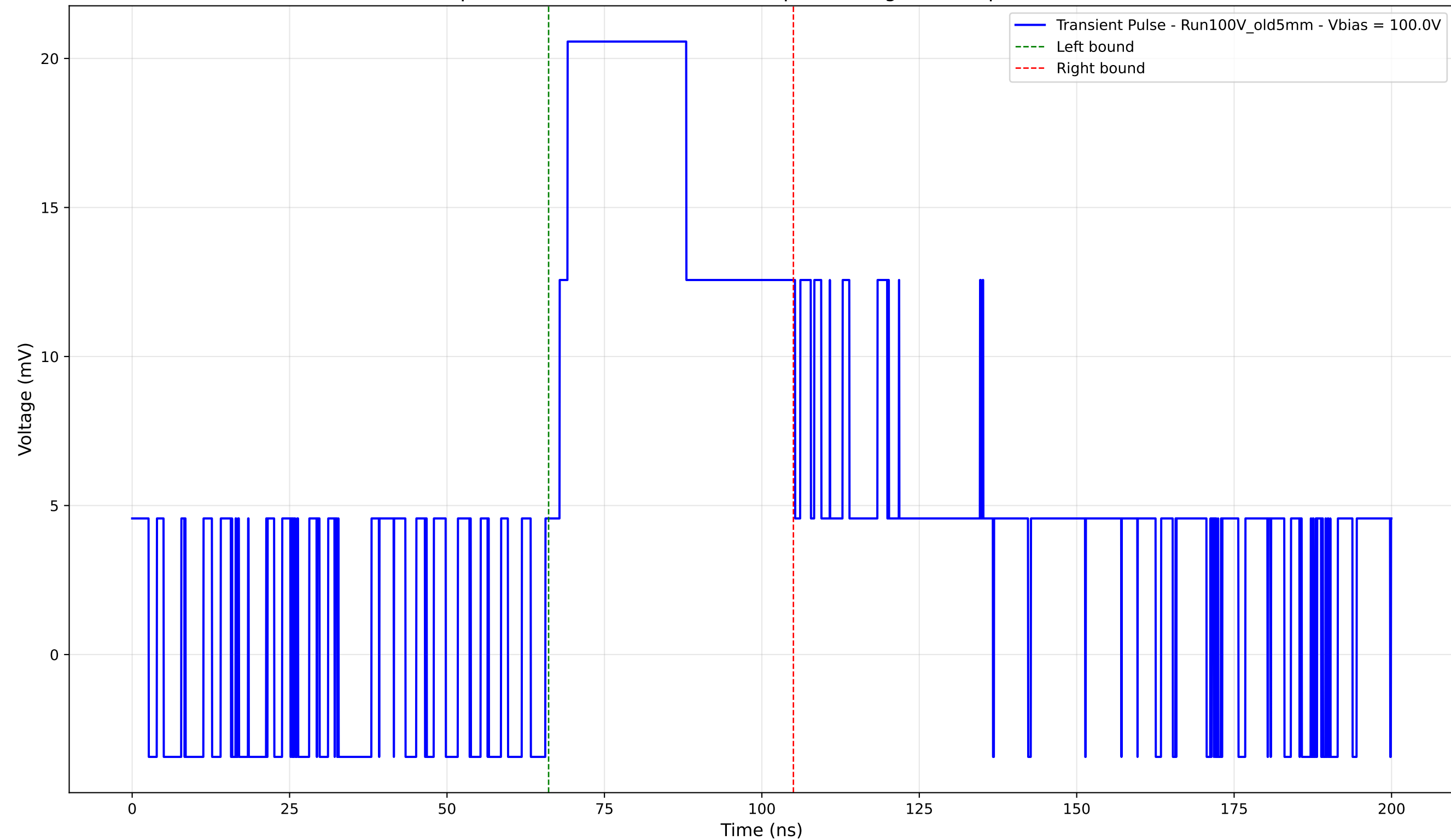
Transient Pulse - Sample: Old5mm - Position: 2215.0 \mu\text{m} - Charge: 12.51 pC - Rise Time: 0.00 ns (N/A)
