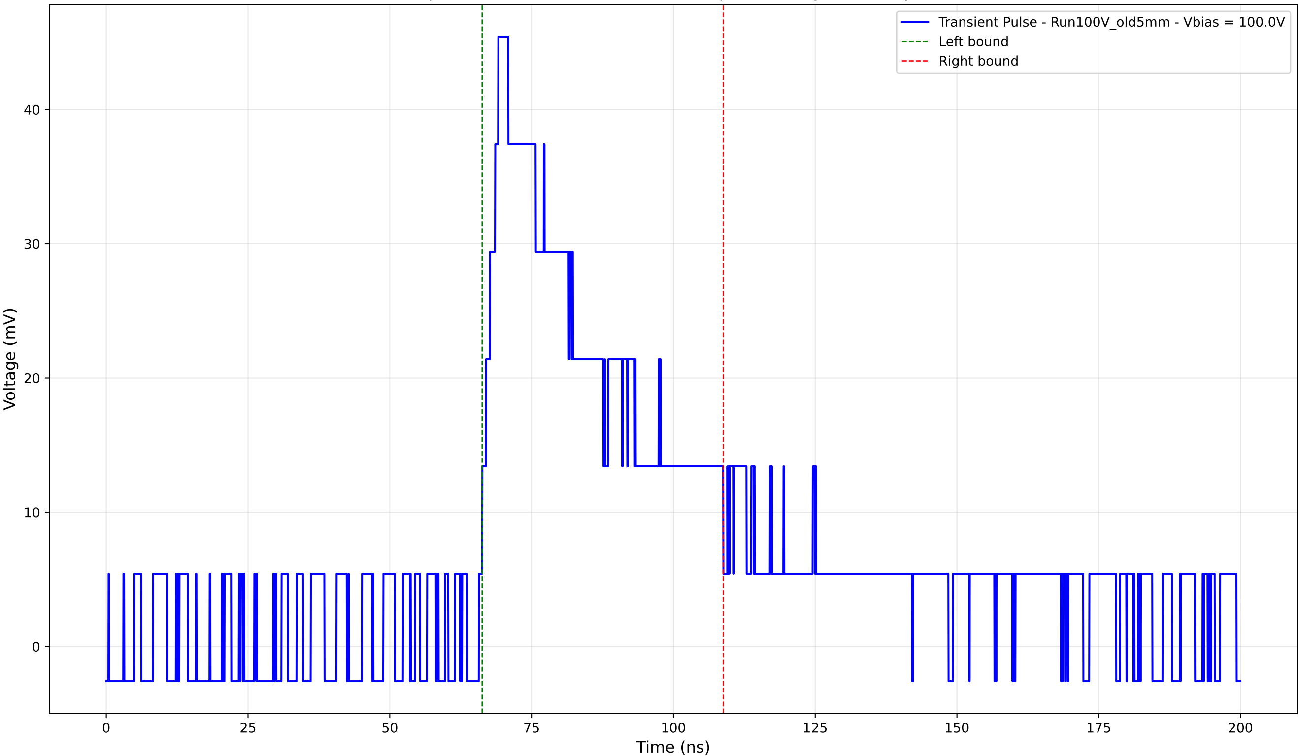
Transient Pulse - Sample: Old5mm - Position: 4885.0 \mu\text{m} - Charge: 19.21 pC - Rise Time: 3.43 ns
