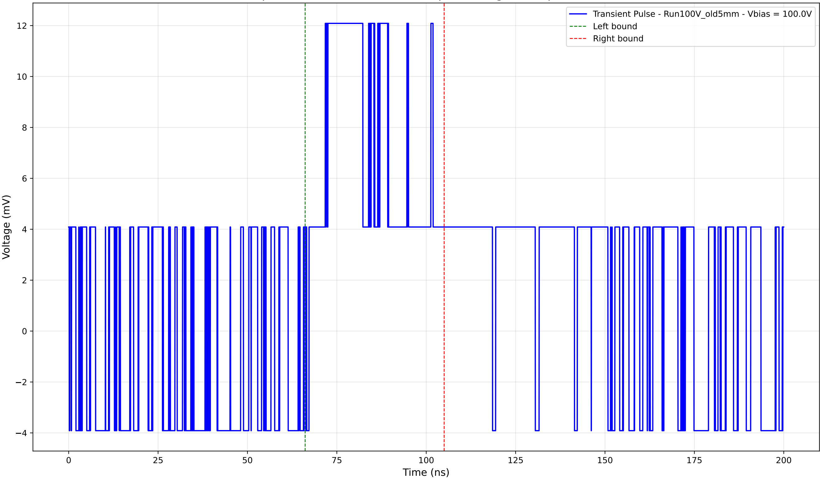
Transient Pulse - Sample: Old5mm - Position: 780.0 \mu\text{m} - Charge: 5.47 pC - Rise Time: 0.00 ns (N/A)
