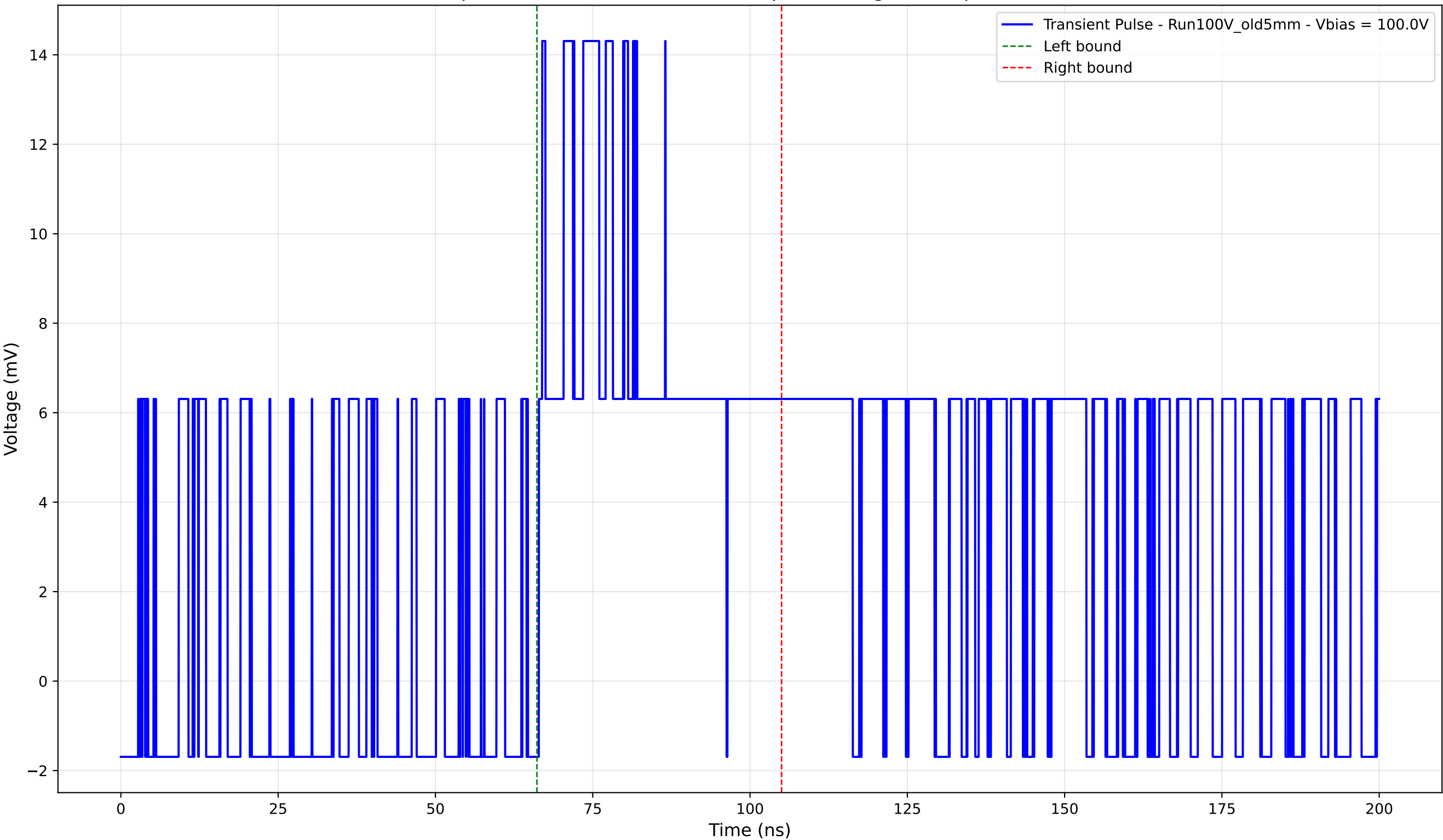
Transient Pulse - Sample: Old5mm - Position: 455.0 \mu\text{m} - Charge: 5.96 pC - Rise Time: 0.00 ns (N/A)
