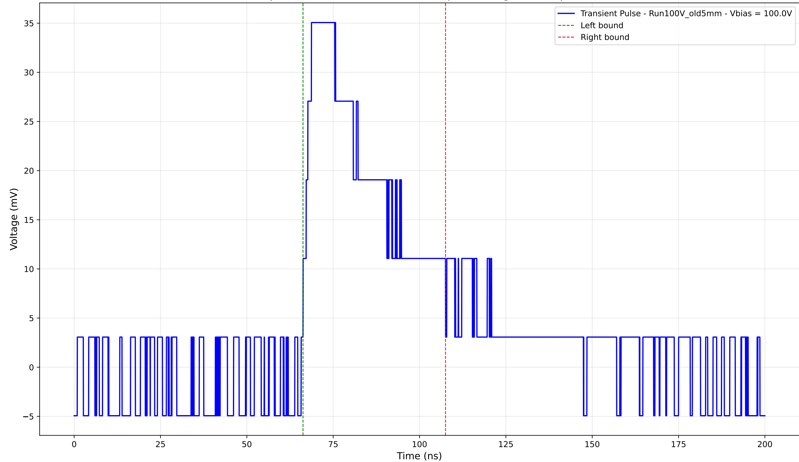
Transient Pulse - Sample: Old5mm - Position: 4935.0 \mu\text{m} - Charge: 16.43 pC - Rise Time: 2.44 ns
