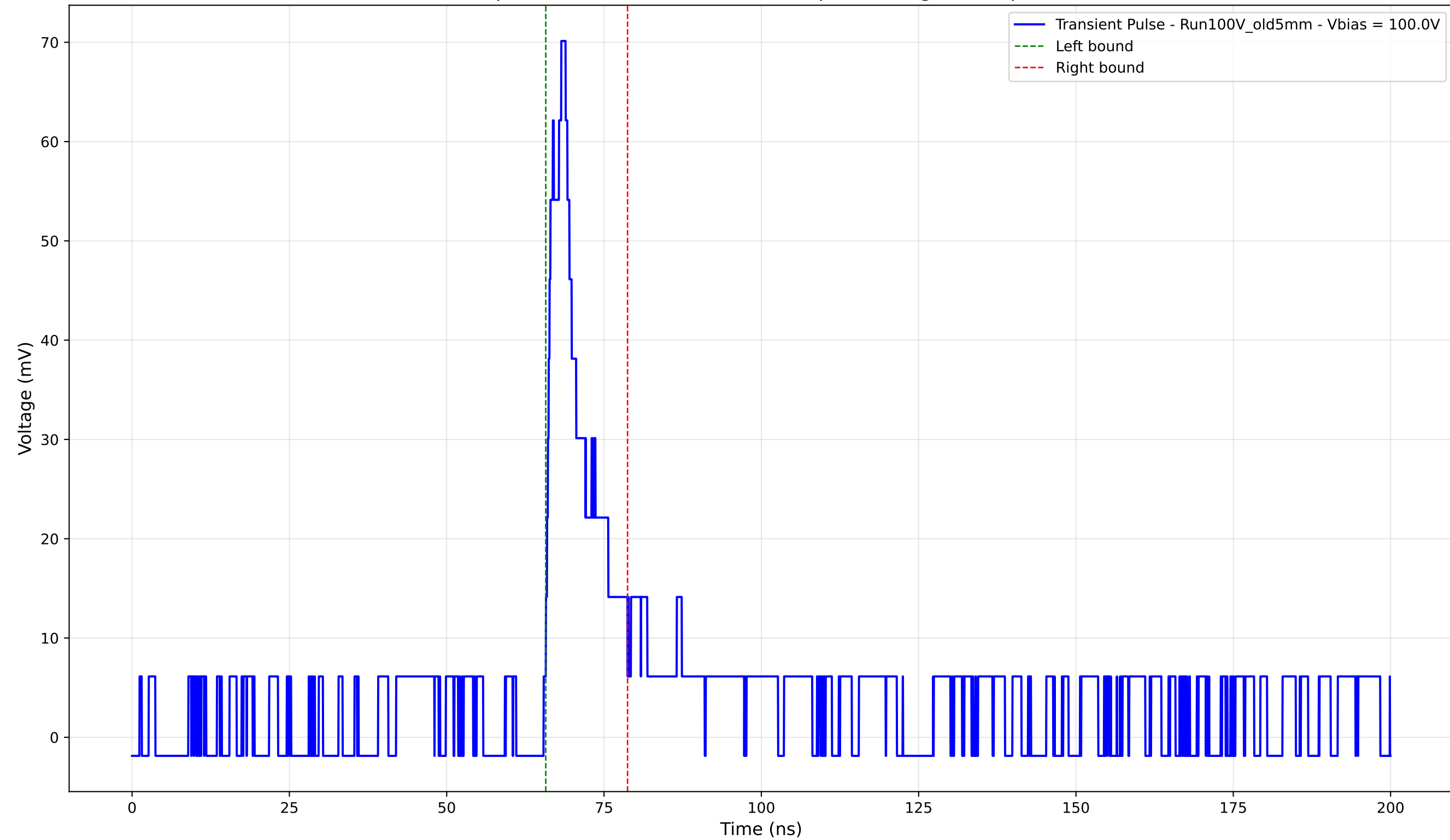
Transient Pulse - Sample: Old5mm - Position: 3335.0 \mu\text{m} - Charge: 8.35 pC - Rise Time: 2.46 ns
