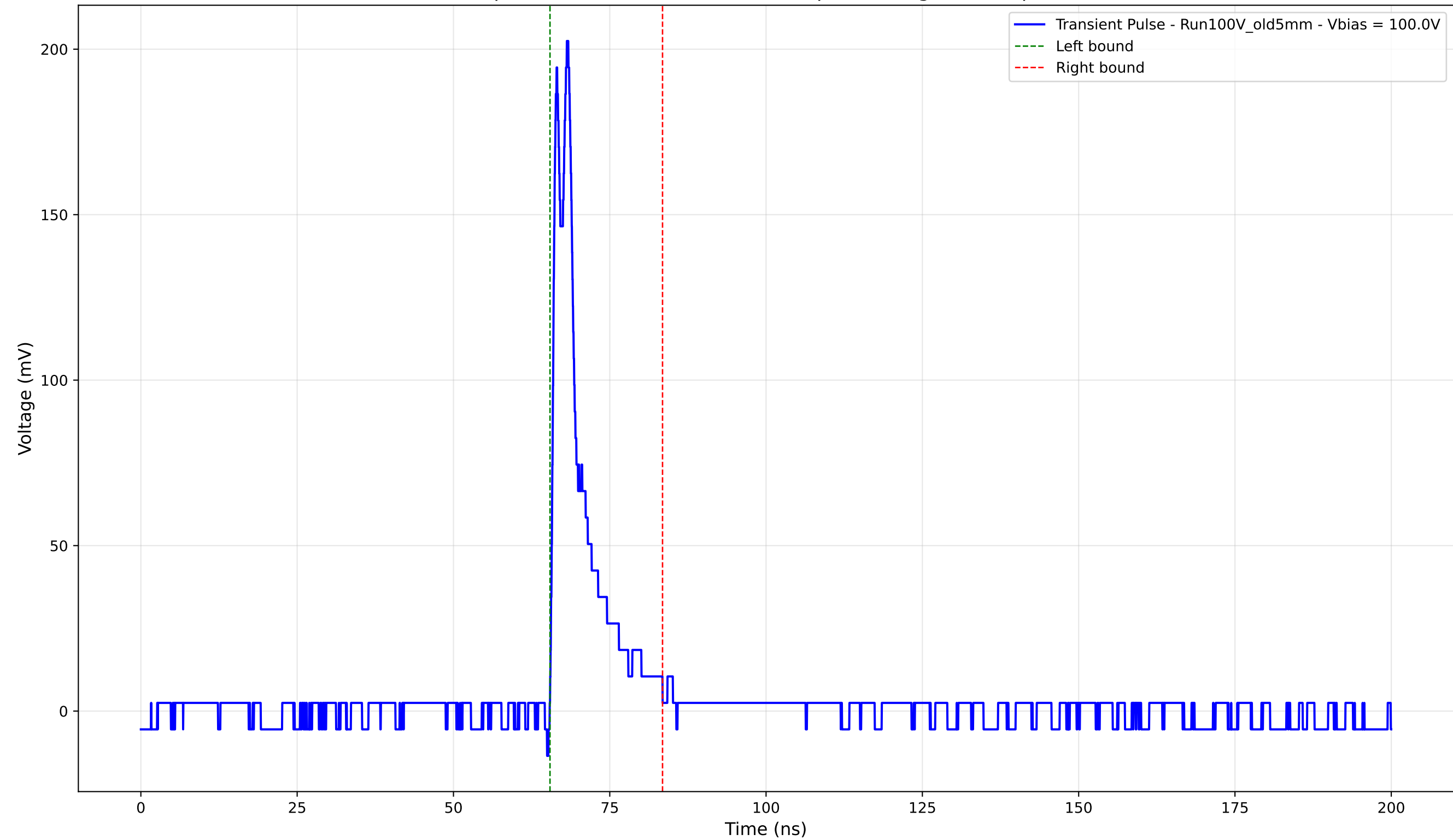
Transient Pulse - Sample: Old5mm - Position: 3570.0 \mu\text{m} - Charge: 20.06 pC - Rise Time: 0.80 ns
