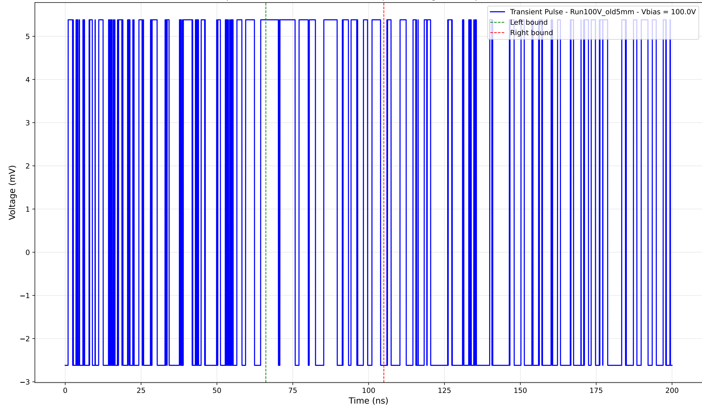
Transient Pulse - Sample: Old5mm - Position: 4595.0 \mu\text{m} - Charge: 2.25 pC - Rise Time: 0.00 ns (N/A)
