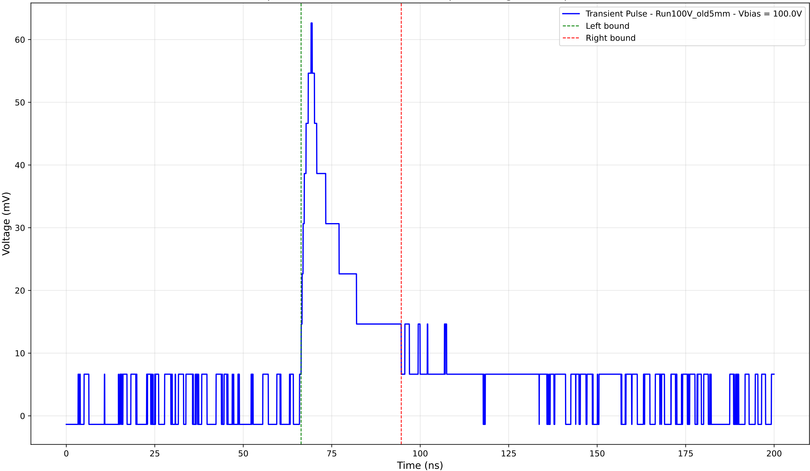
Transient Pulse - Sample: Old5mm - Position: 4515.0 \mu\text{m} - Charge: 14.16 pC - Rise Time: 3.26 ns
