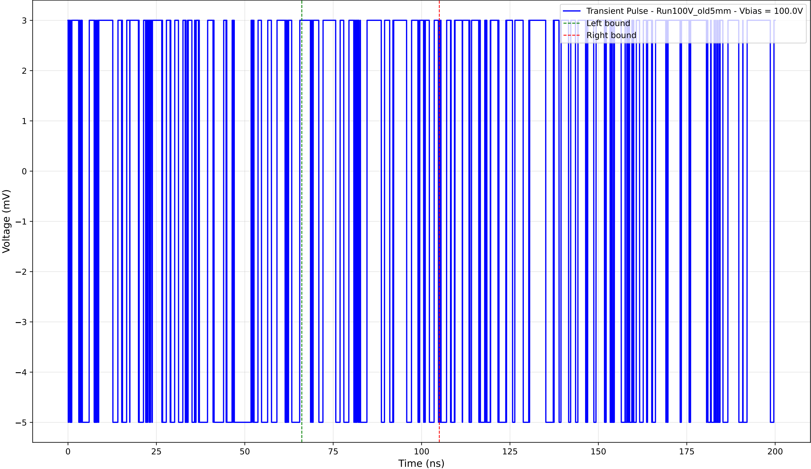
Transient Pulse - Sample: Old5mm - Position: 255.0 \mu\text{m} - Charge: 0.37 pC - Rise Time: 0.00 ns (N/A)
