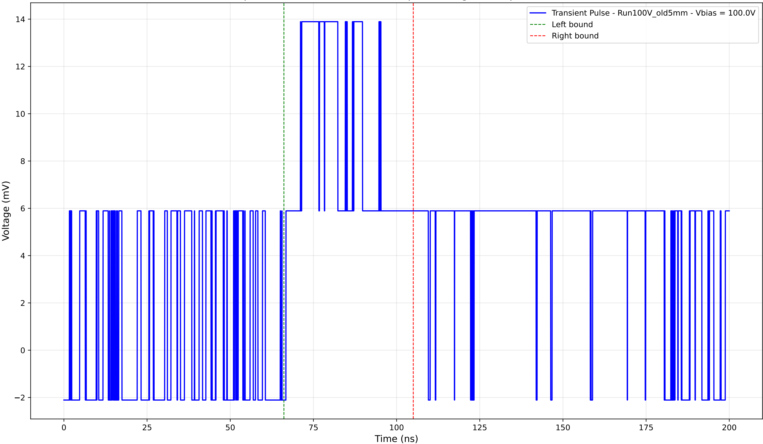
Transient Pulse - Sample: Old5mm - Position: 965.0 \mu\text{m} - Charge: 6.75 pC - Rise Time: 0.00 ns (N/A)
