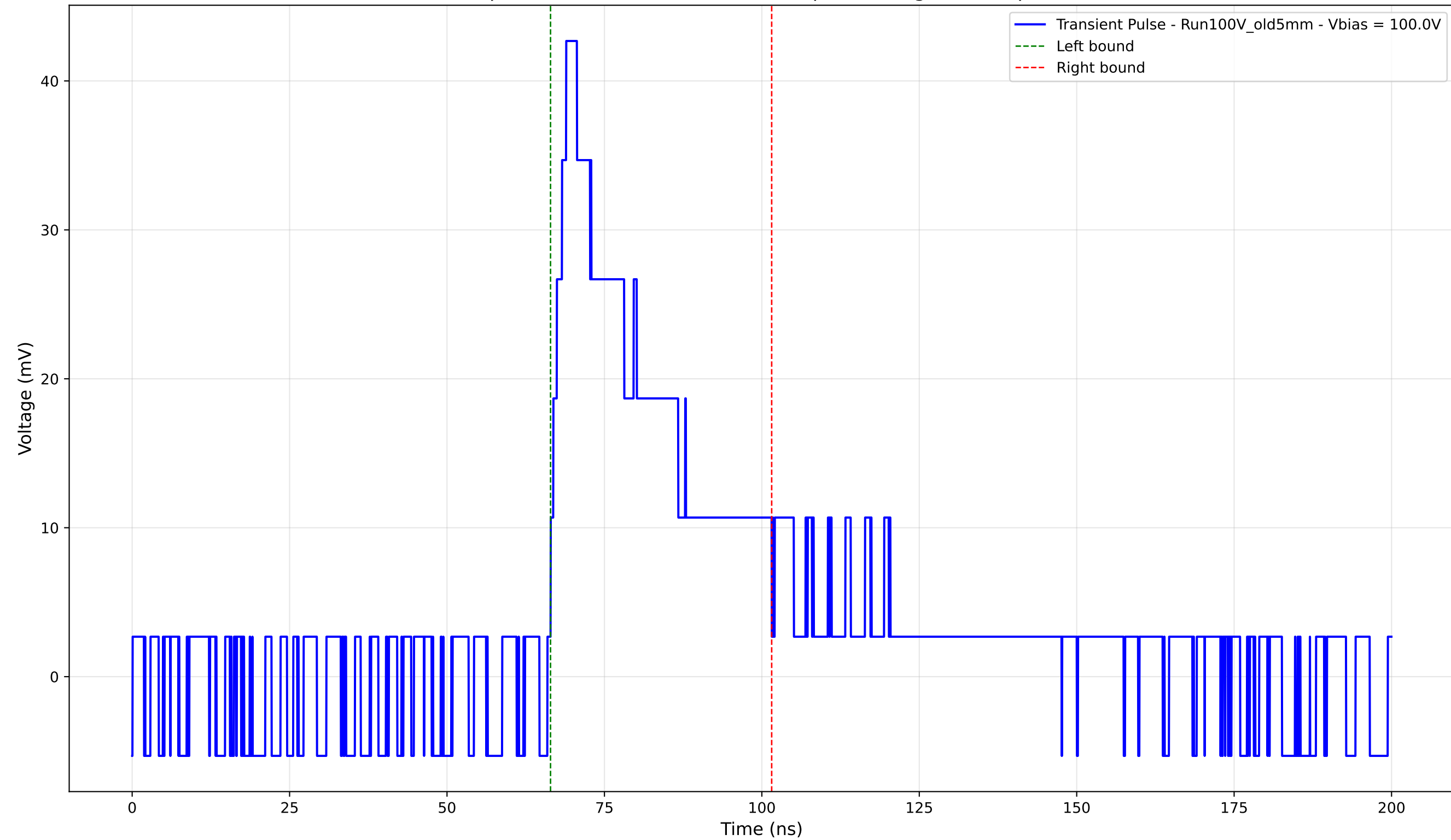
Transient Pulse - Sample: Old5mm - Position: 2685.0 \mu\text{m} - Charge: 13.49 pC - Rise Time: 2.48 ns
