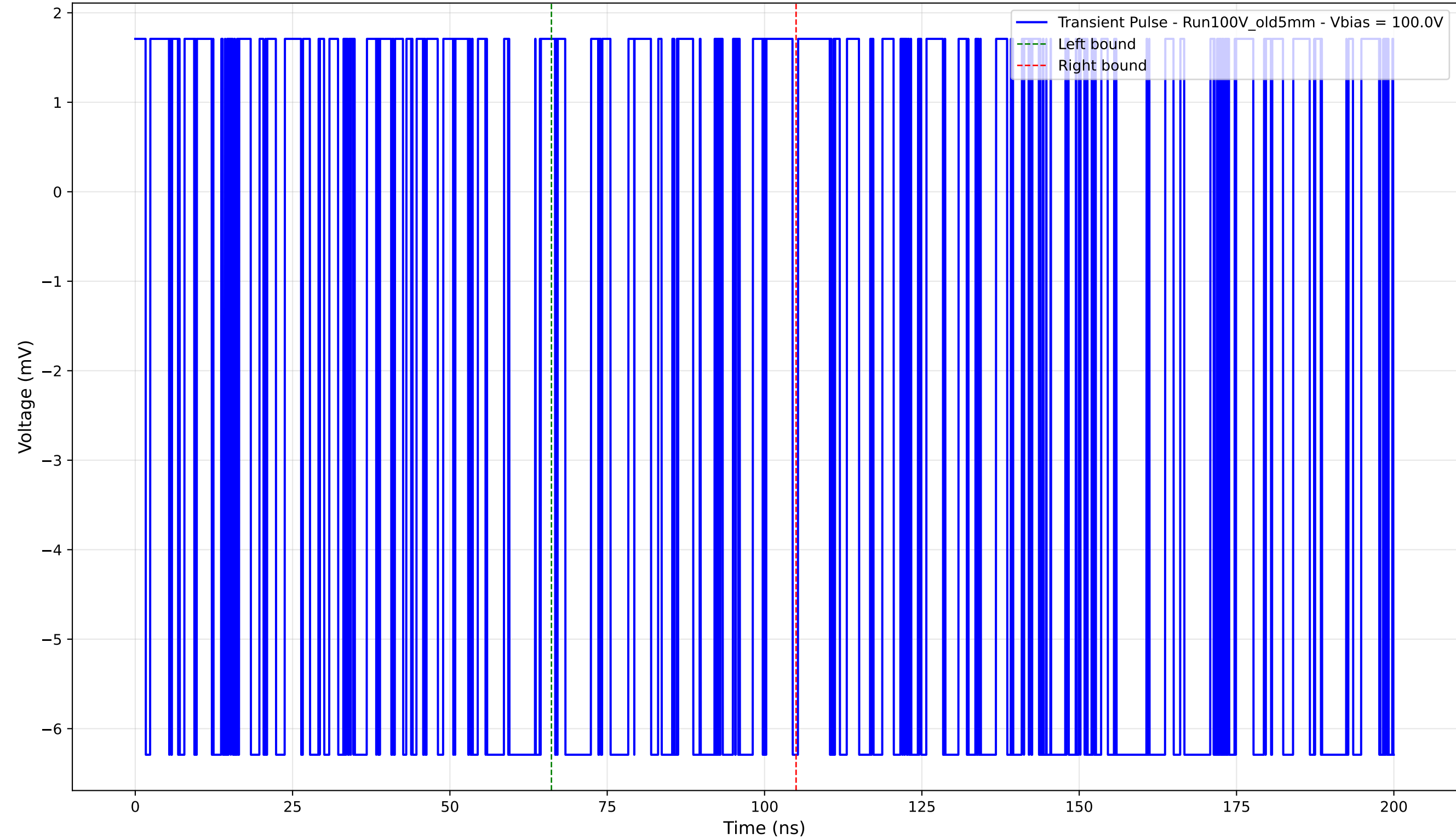
Transient Pulse - Sample: Old5mm - Position: 150.0 \mu\text{m} - Charge: -1.81 pC - Rise Time: 0.00 ns (N/A)
