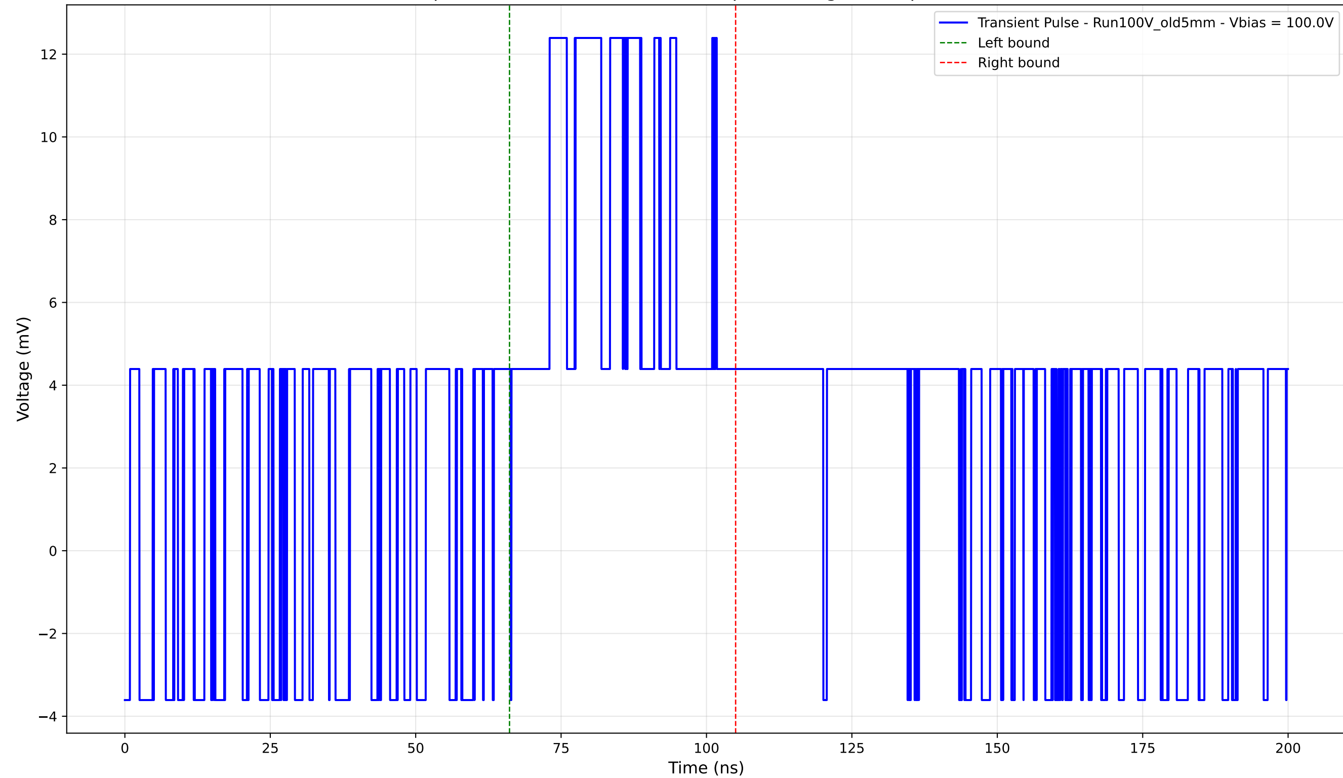
Transient Pulse - Sample: Old5mm - Position: 1665.0 \mu\text{m} - Charge: 5.81 pC - Rise Time: 0.00 ns (N/A)
