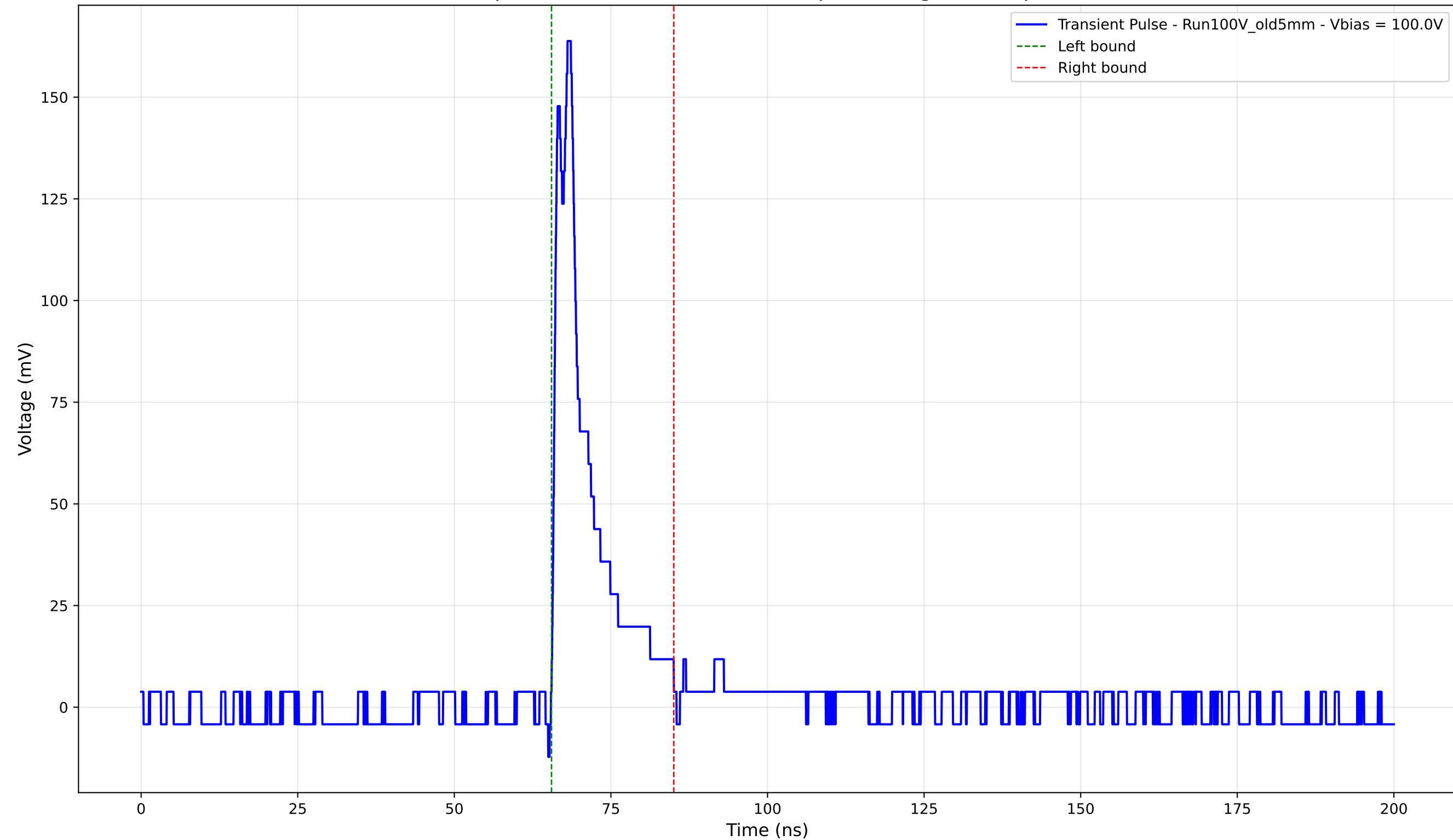
Transient Pulse - Sample: Old5mm - Position: 3515.0 \mu\text{m} - Charge: 19.22 pC - Rise Time: 0.87 ns
