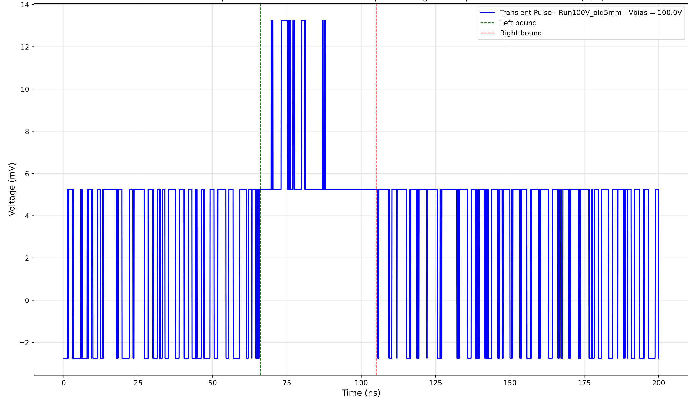
Transient Pulse - Sample: Old5mm - Position: 2345.0 \mu\text{m} - Charge: 4.89 pC - Rise Time: 0.00 ns (N/A)
