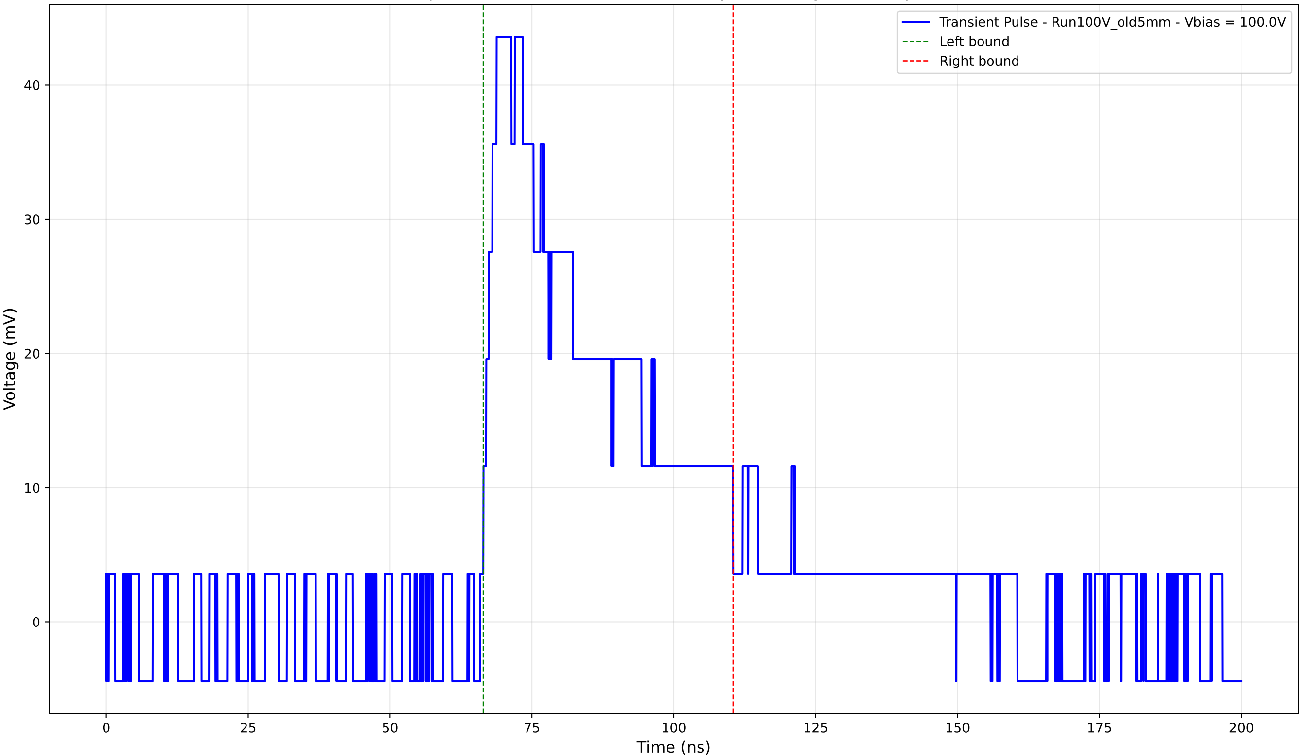
Transient Pulse - Sample: Old5mm - Position: 4865.0 \mu\text{m} - Charge: 18.88 pC - Rise Time: 2.36 ns
