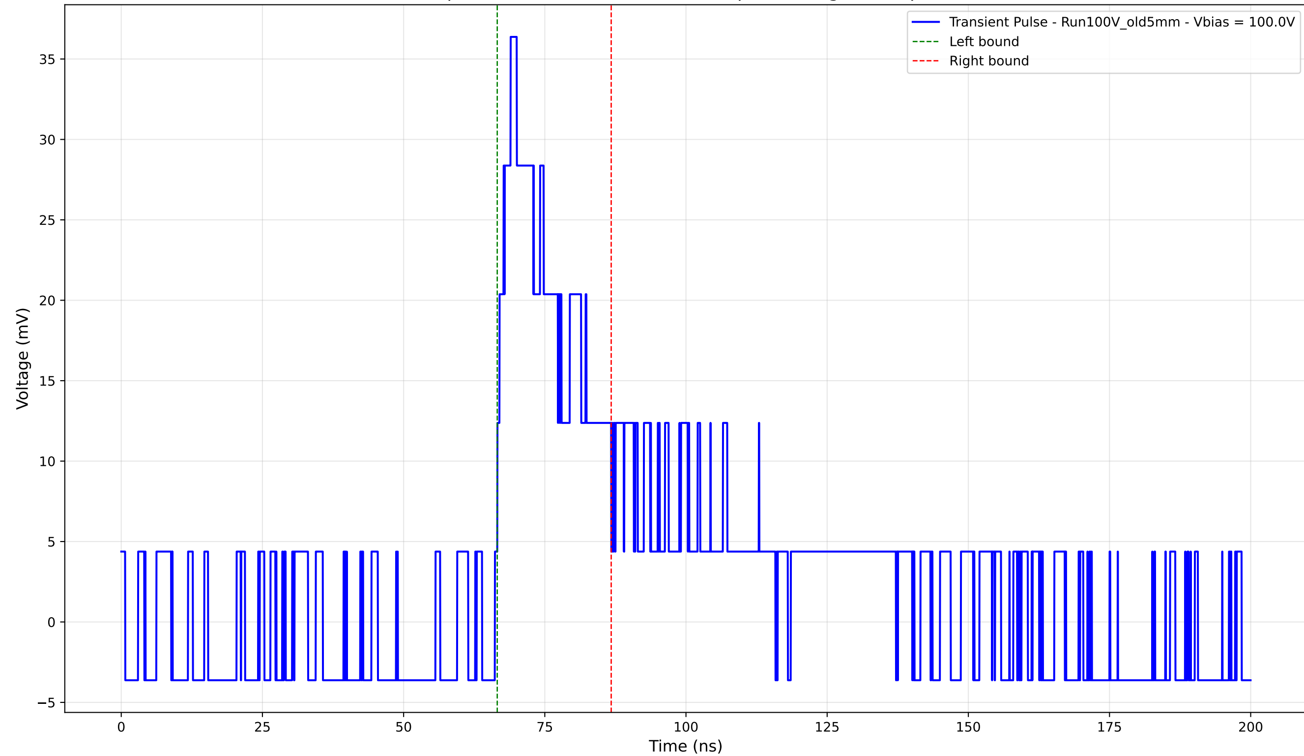
Transient Pulse - Sample: Old5mm - Position: 4700.0 \mu\text{m} - Charge: 8.19 pC - Rise Time: 2.80 ns
