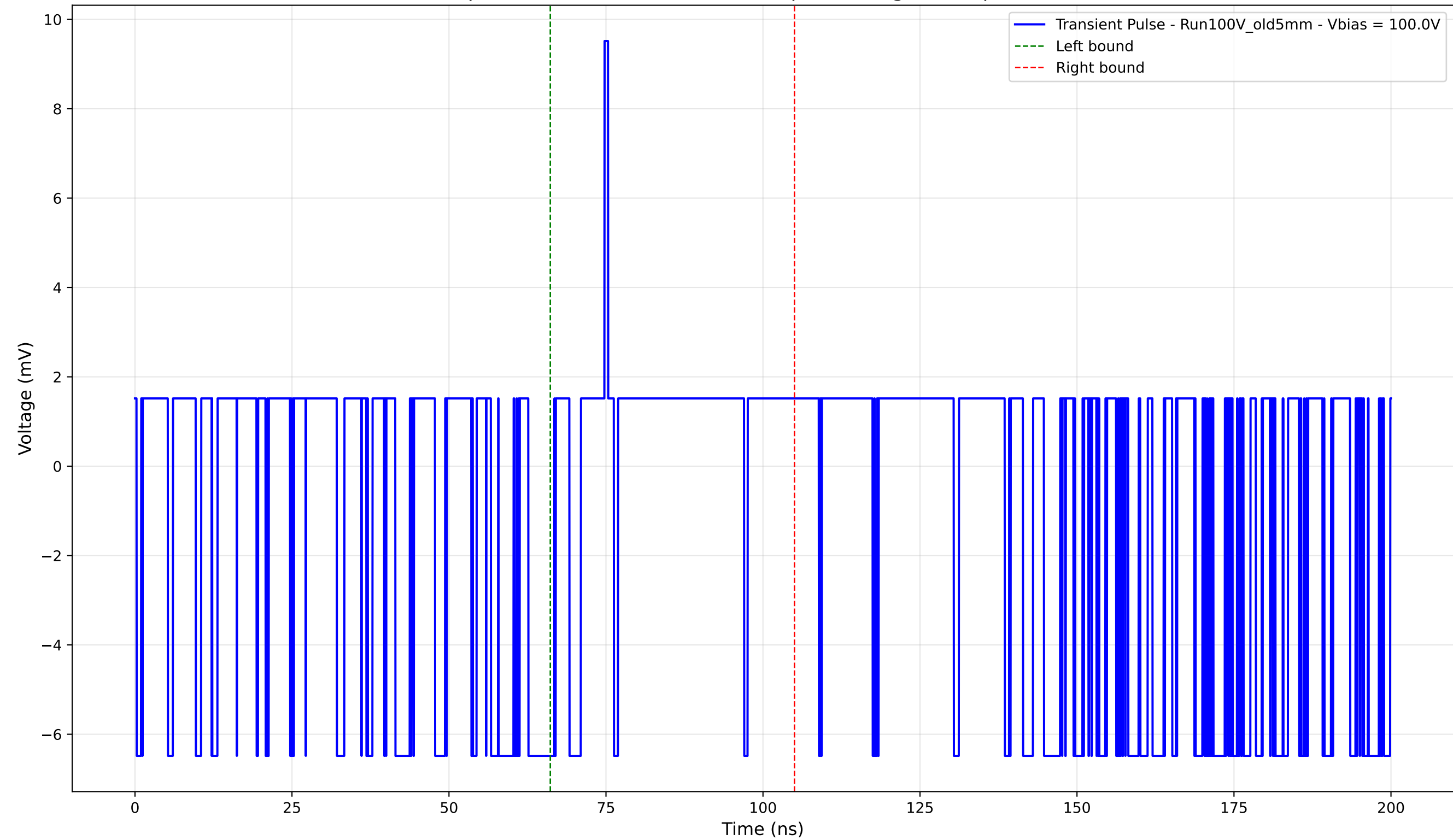
Transient Pulse - Sample: Old5mm - Position: 2125.0 \mu\text{m} - Charge: 0.65 pC - Rise Time: 0.00 ns (N/A)
