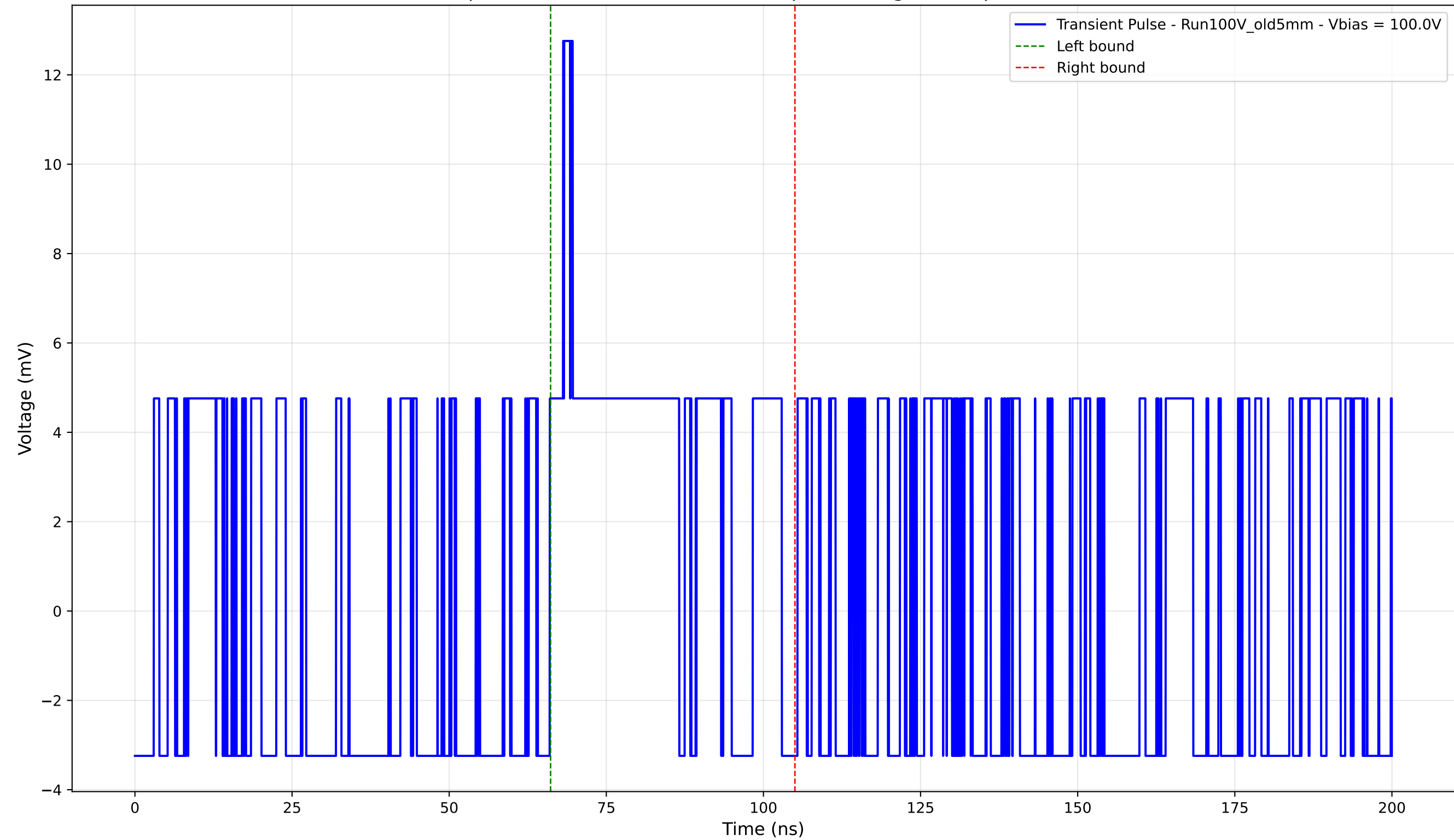
Transient Pulse - Sample: Old5mm - Position: 3130.0 \mu\text{m} - Charge: 2.75 pC - Rise Time: 0.00 ns (N/A)
