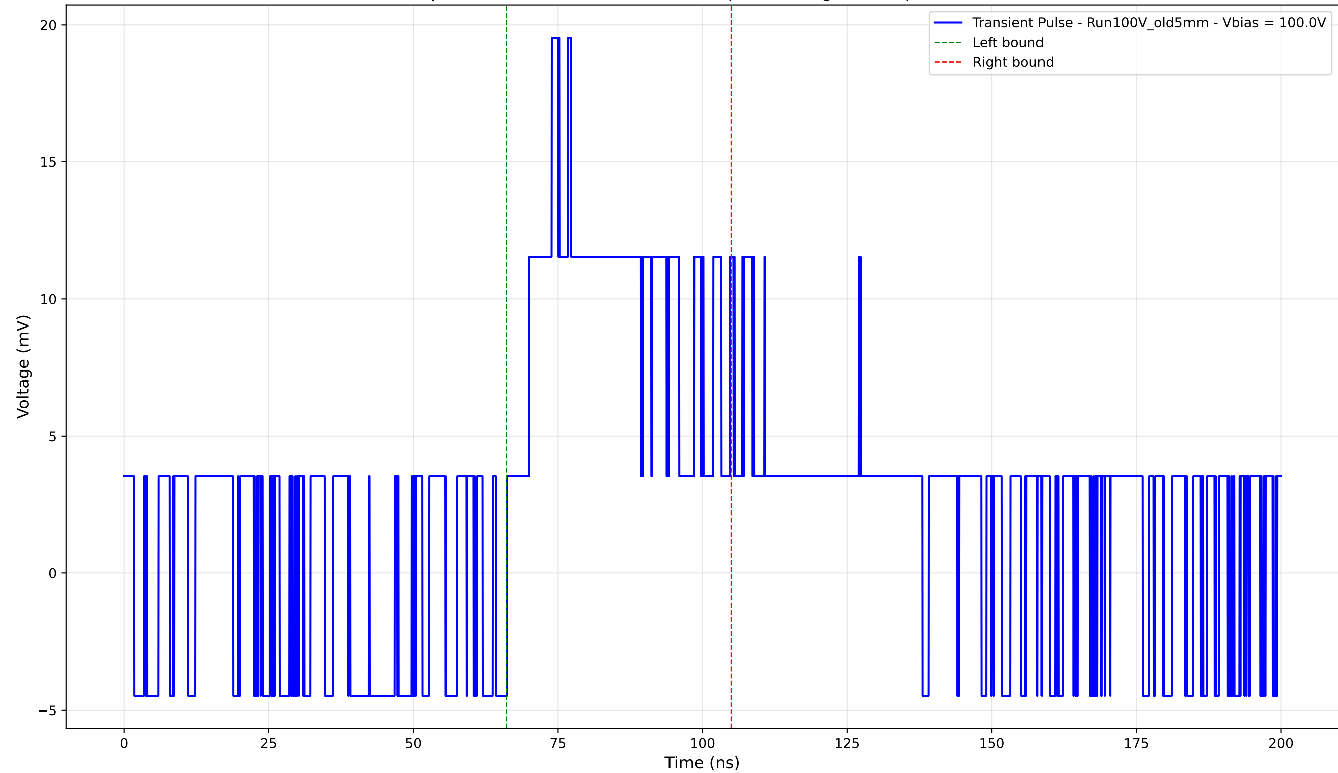
Transient Pulse - Sample: Old5mm - Position: 2065.0 \mu\text{m} - Charge: 7.59 pC - Rise Time: 0.00 ns (N/A)
