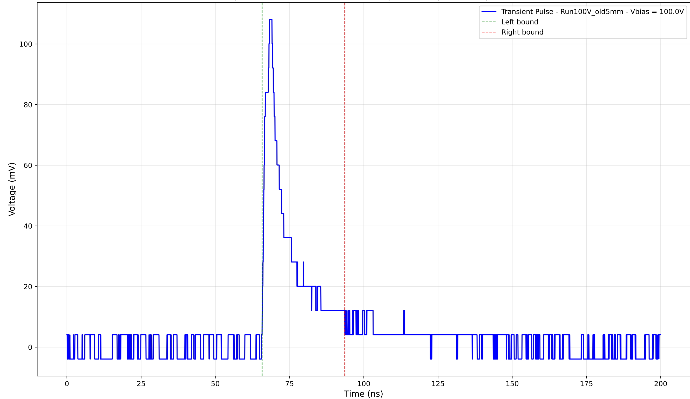
Transient Pulse - Sample: Old5mm - Position: 3230.0 \mu\text{m} - Charge: 18.32 pC - Rise Time: 2.30 ns
