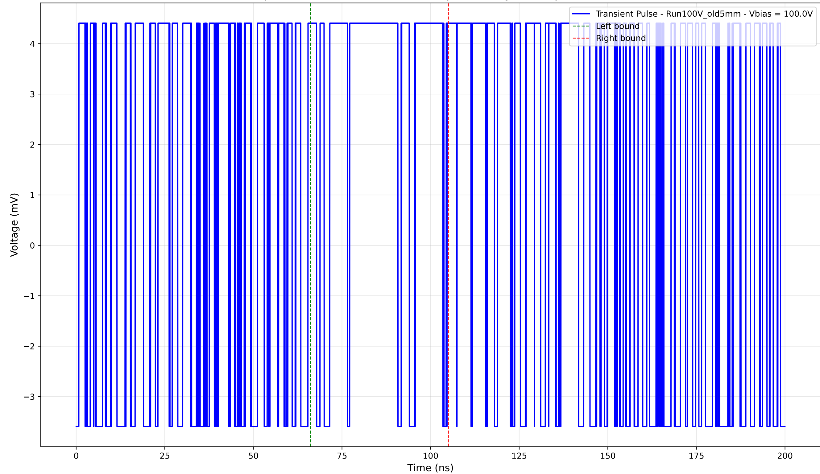
Transient Pulse - Sample: Old5mm - Position: 1500.0 \mu\text{m} - Charge: 2.33 pC - Rise Time: 0.00 ns (N/A)
