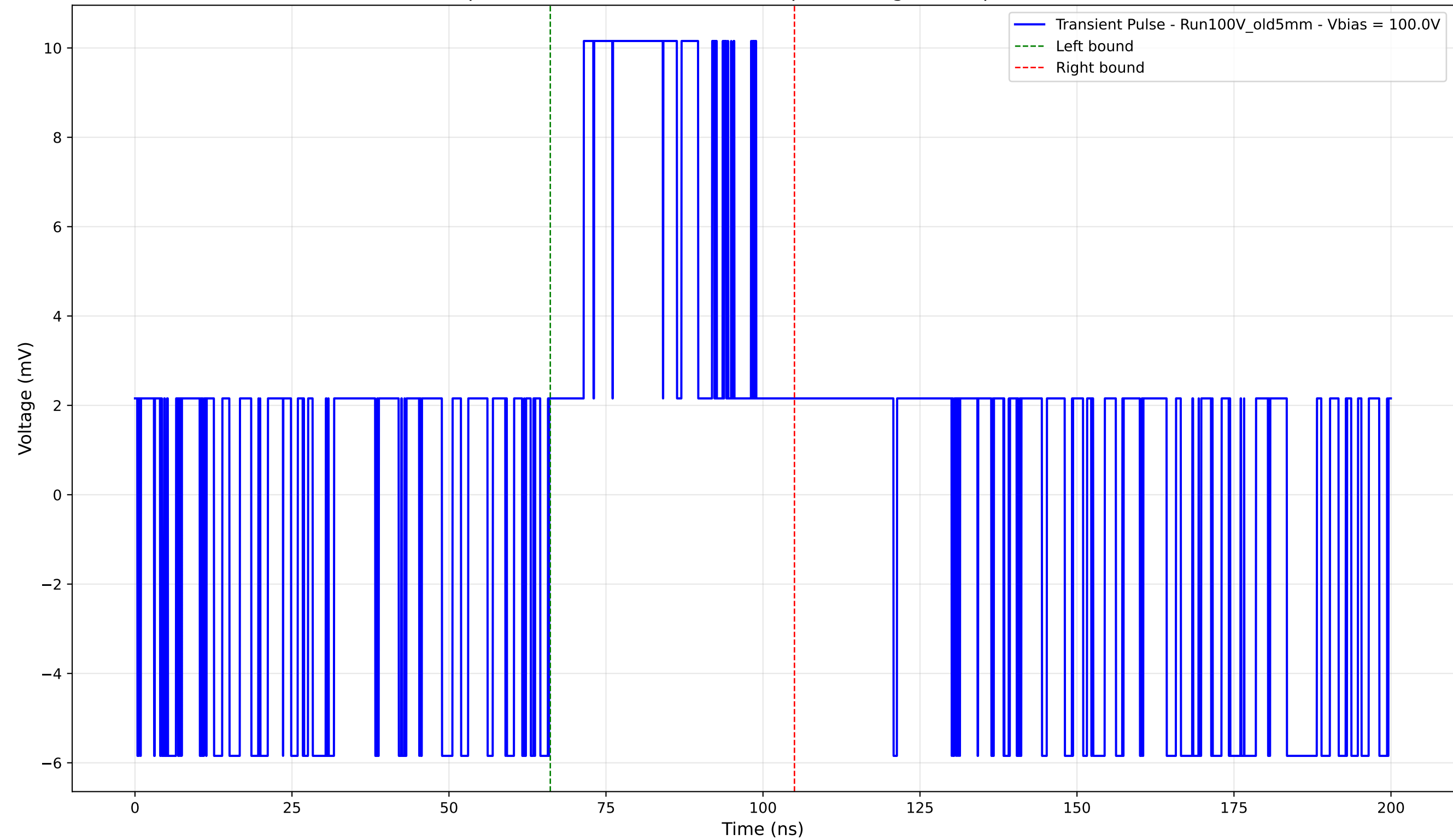
Transient Pulse - Sample: Old5mm - Position: 1960.0 \mu\text{m} - Charge: 4.69 pC - Rise Time: 0.00 ns (N/A)
