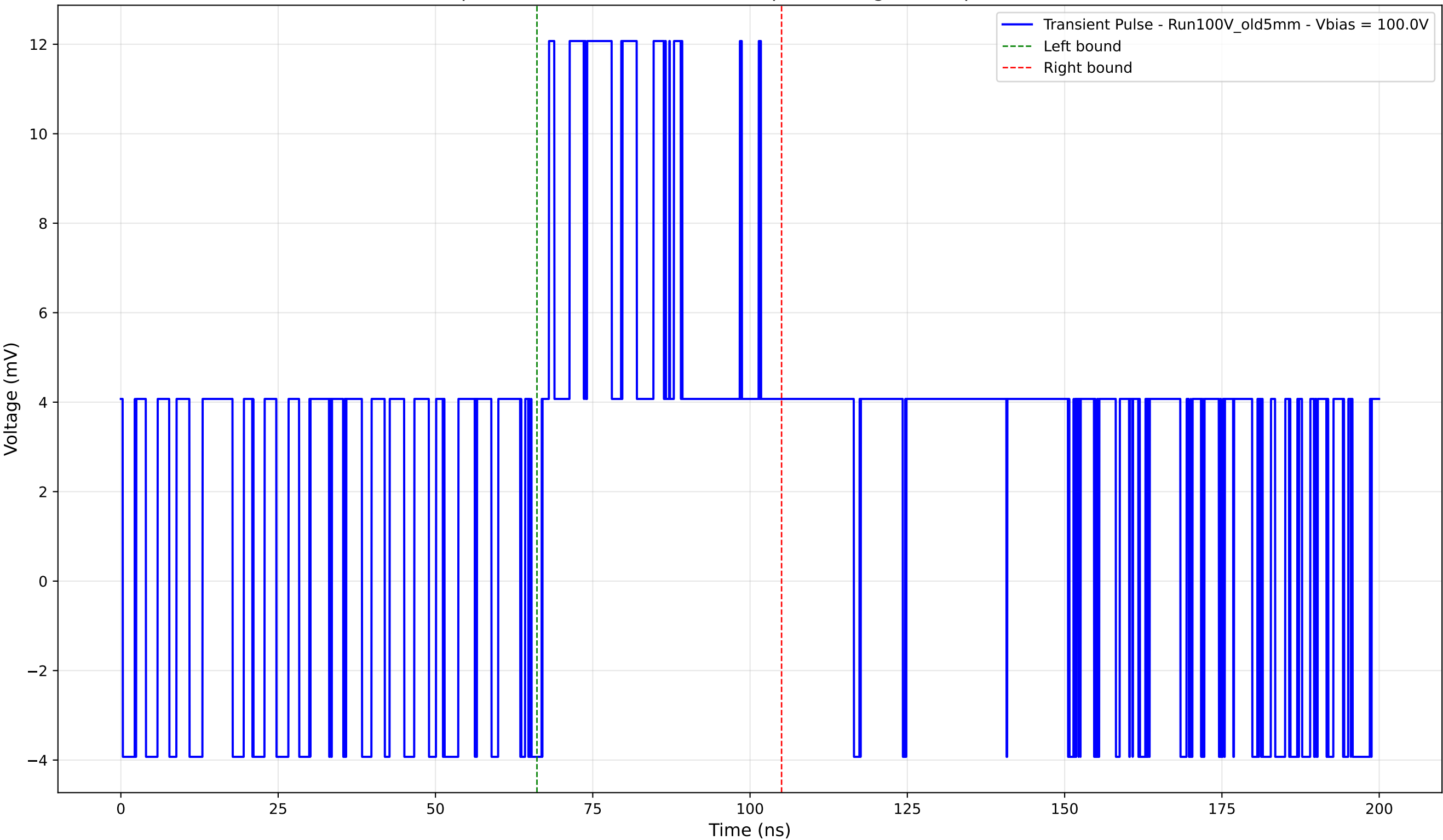
Transient Pulse - Sample: Old5mm - Position: 695.0 \mu\text{m} - Charge: 5.16 pC - Rise Time: 0.00 ns (N/A)
