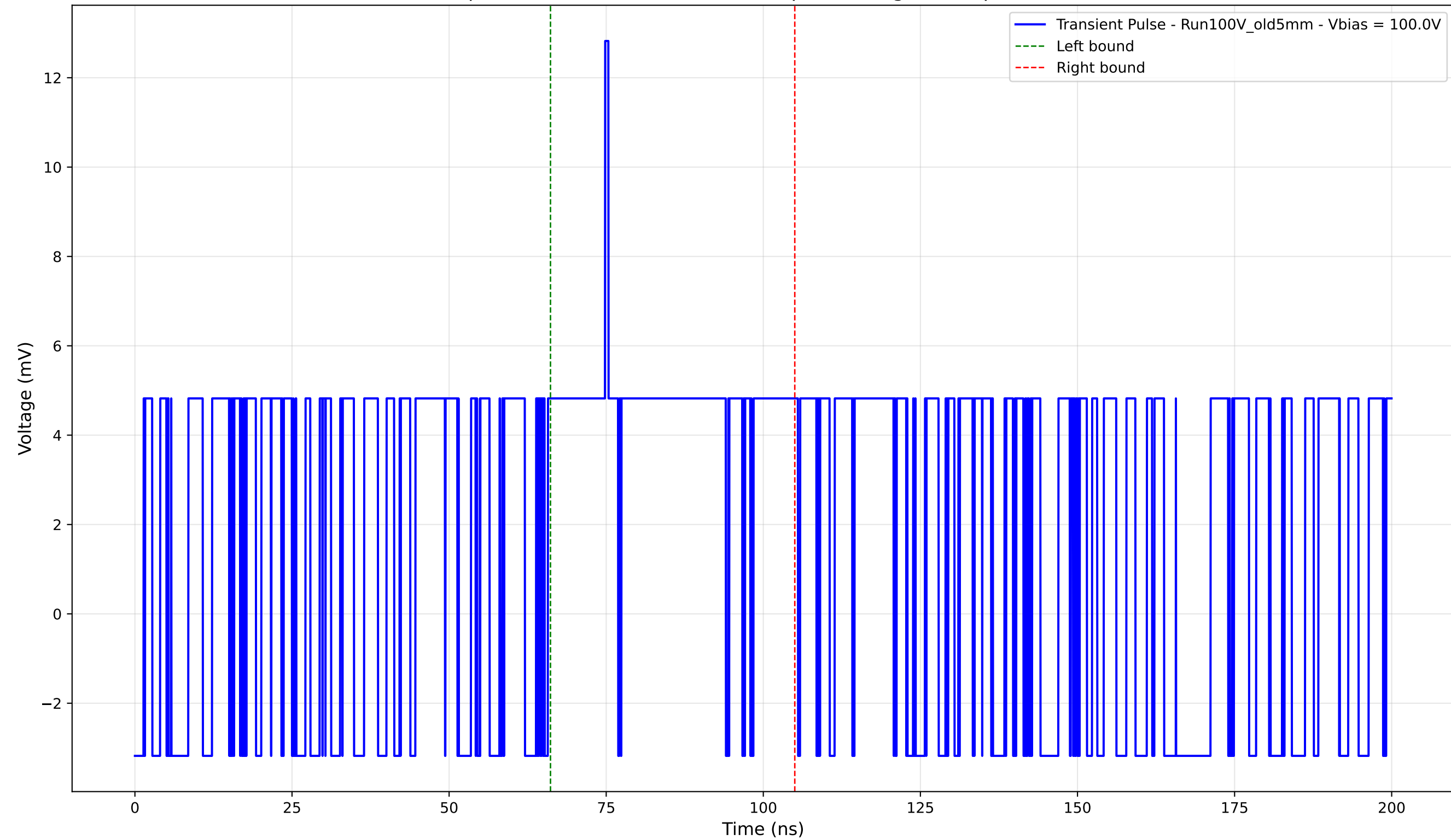
Transient Pulse - Sample: Old5mm - Position: 2130.0 \mu\text{m} - Charge: 3.62 pC - Rise Time: 0.00 ns (N/A)
