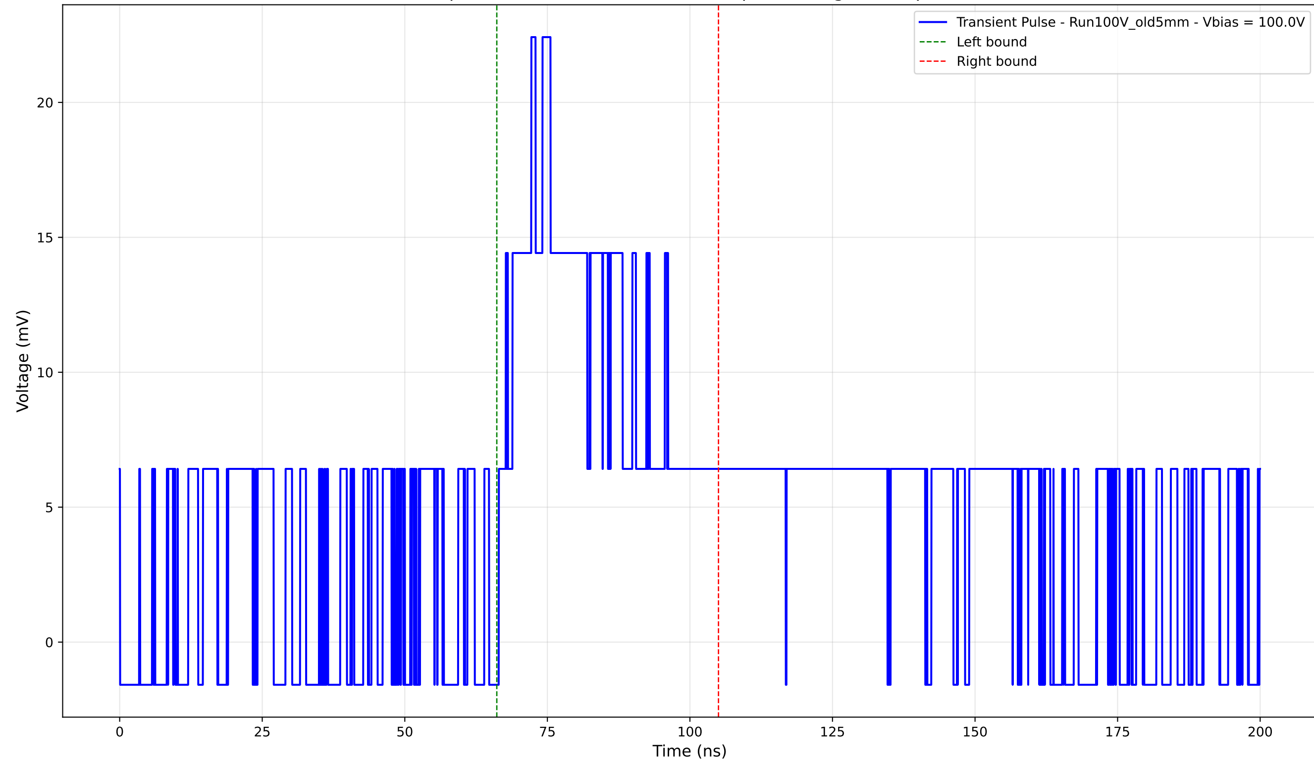
Transient Pulse - Sample: Old5mm - Position: 2365.0 \mu\text{m} - Charge: 8.56 pC - Rise Time: 5.72 ns
