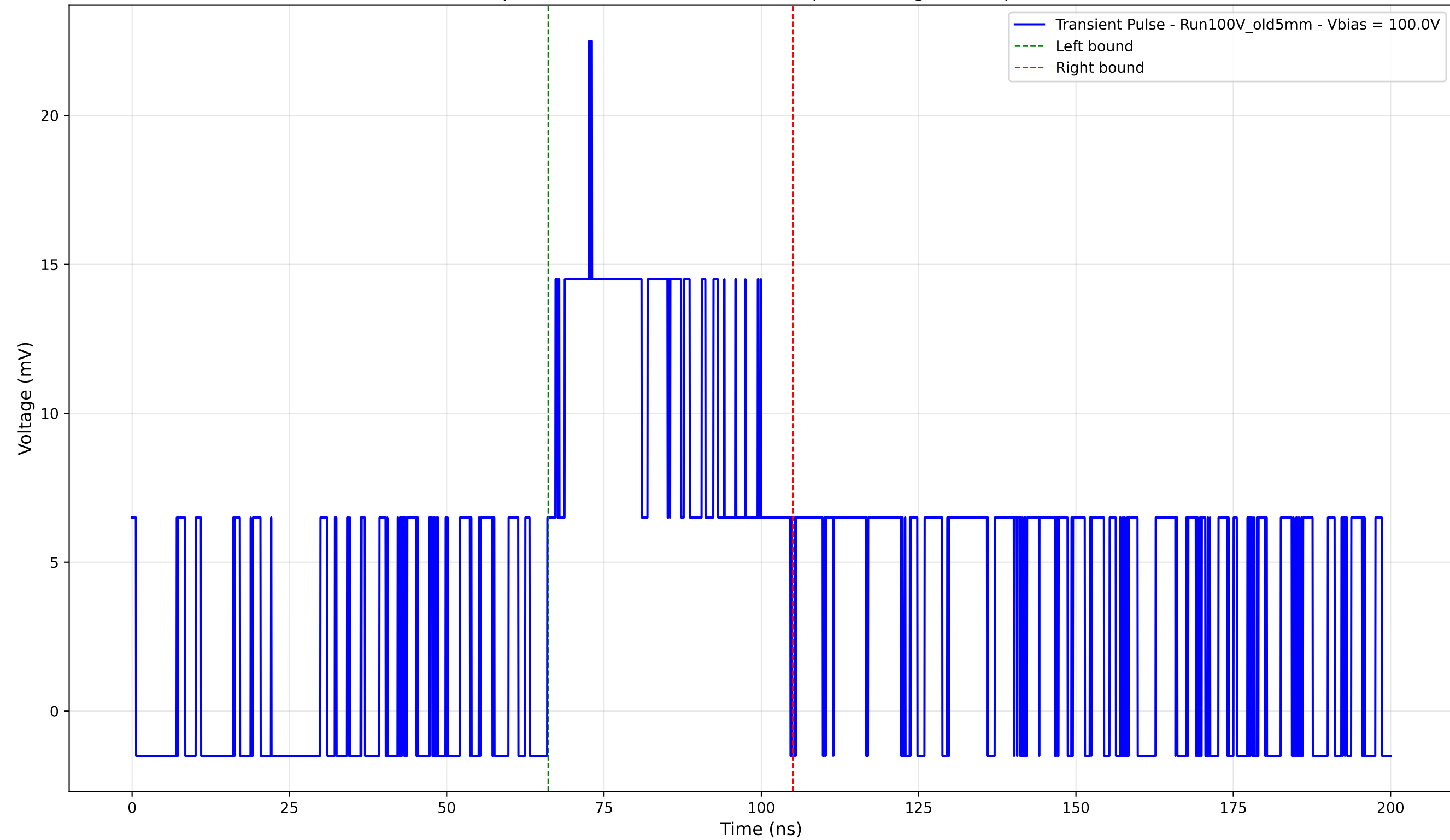
Transient Pulse - Sample: Old5mm - Position: 340.0 \mu\text{m} - Charge: 8.32 pC - Rise Time: 6.66 ns
