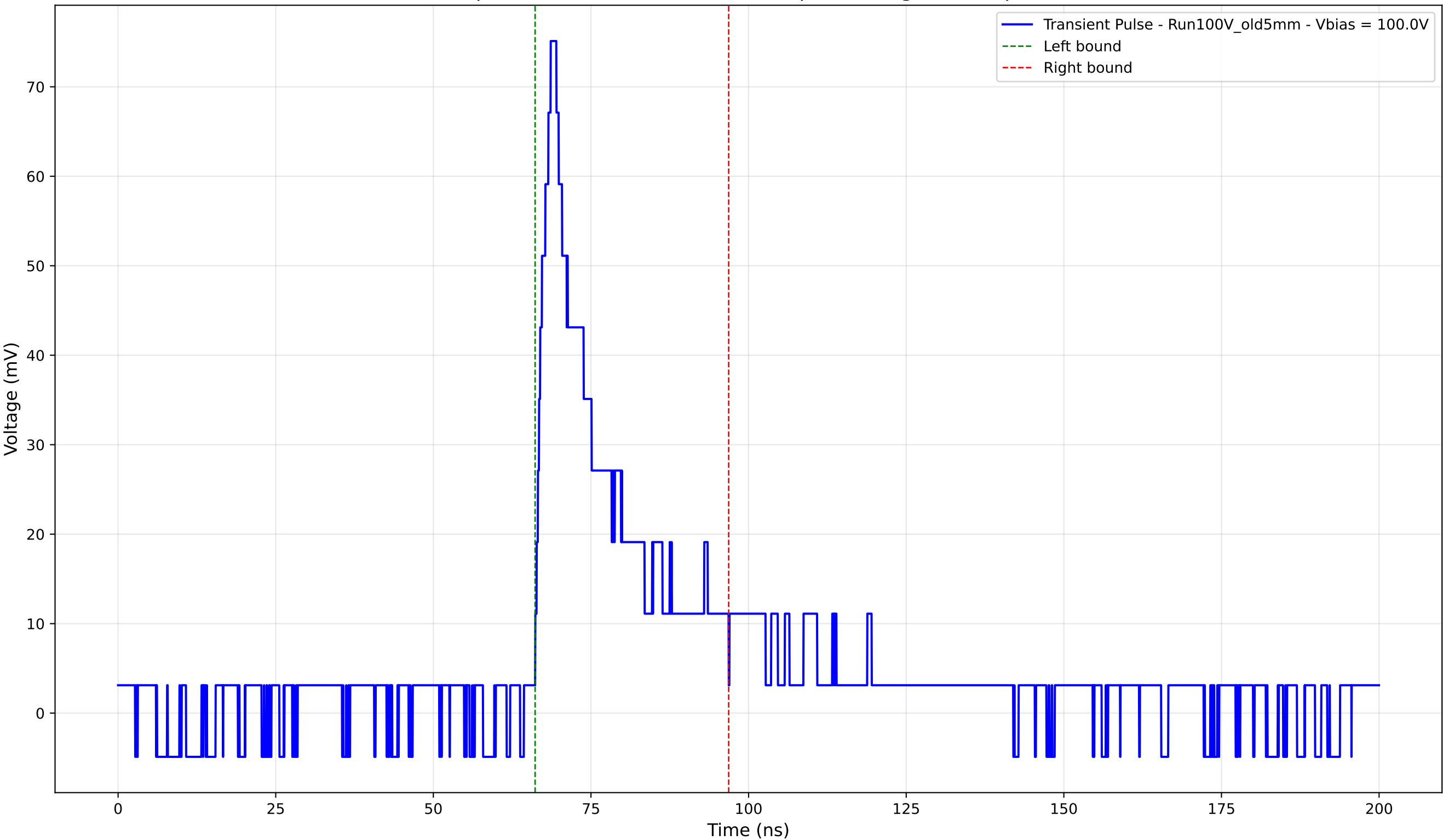
Transient Pulse - Sample: Old5mm - Position: 4450.0 \mu\text{m} - Charge: 15.91 pC - Rise Time: 2.45 ns
