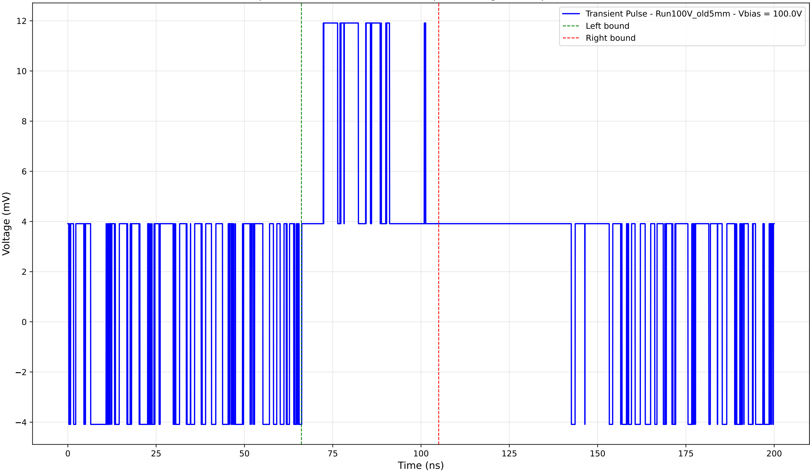
Transient Pulse - Sample: Old5mm - Position: 865.0 \mu\text{m} - Charge: 5.27 pC - Rise Time: 0.00 ns (N/A)
