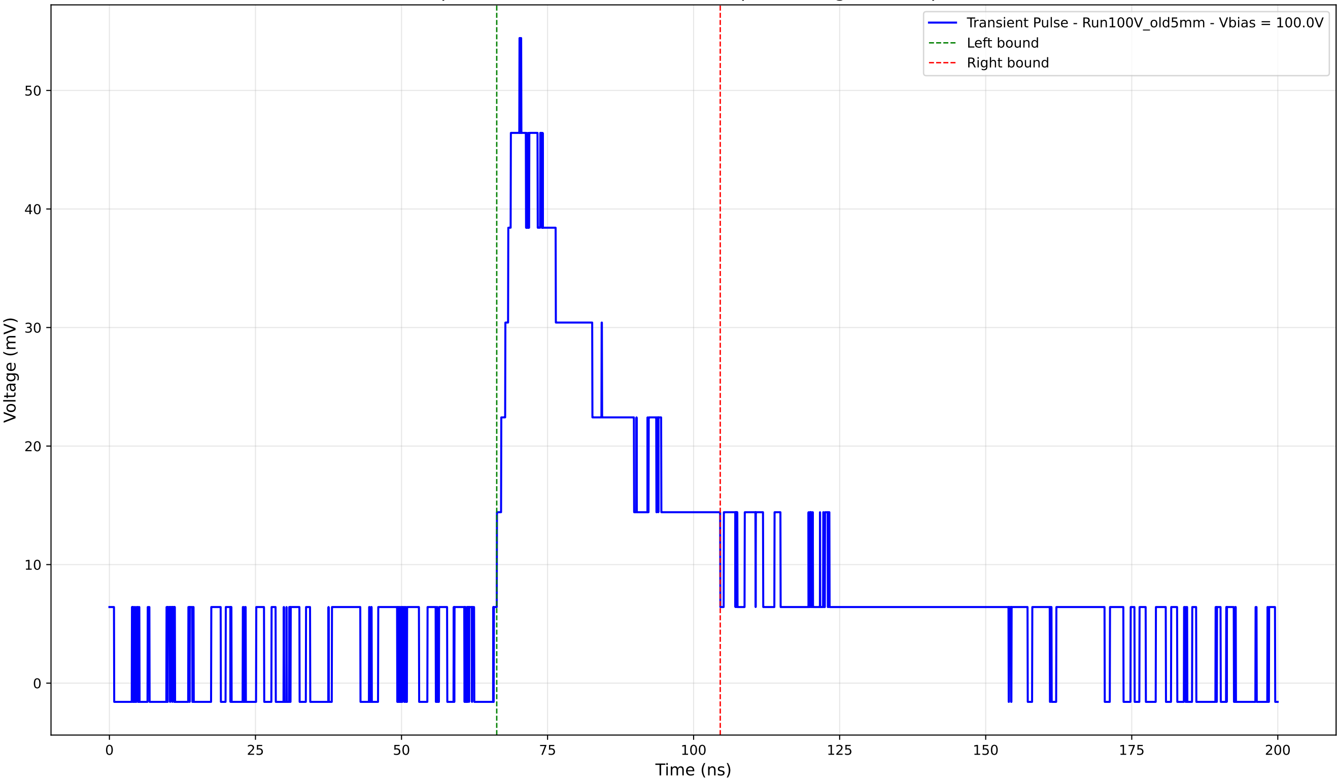
Transient Pulse - Sample: Old5mm - Position: 4845.0 \mu\text{m} - Charge: 19.43 pC - Rise Time: 4.38 ns
