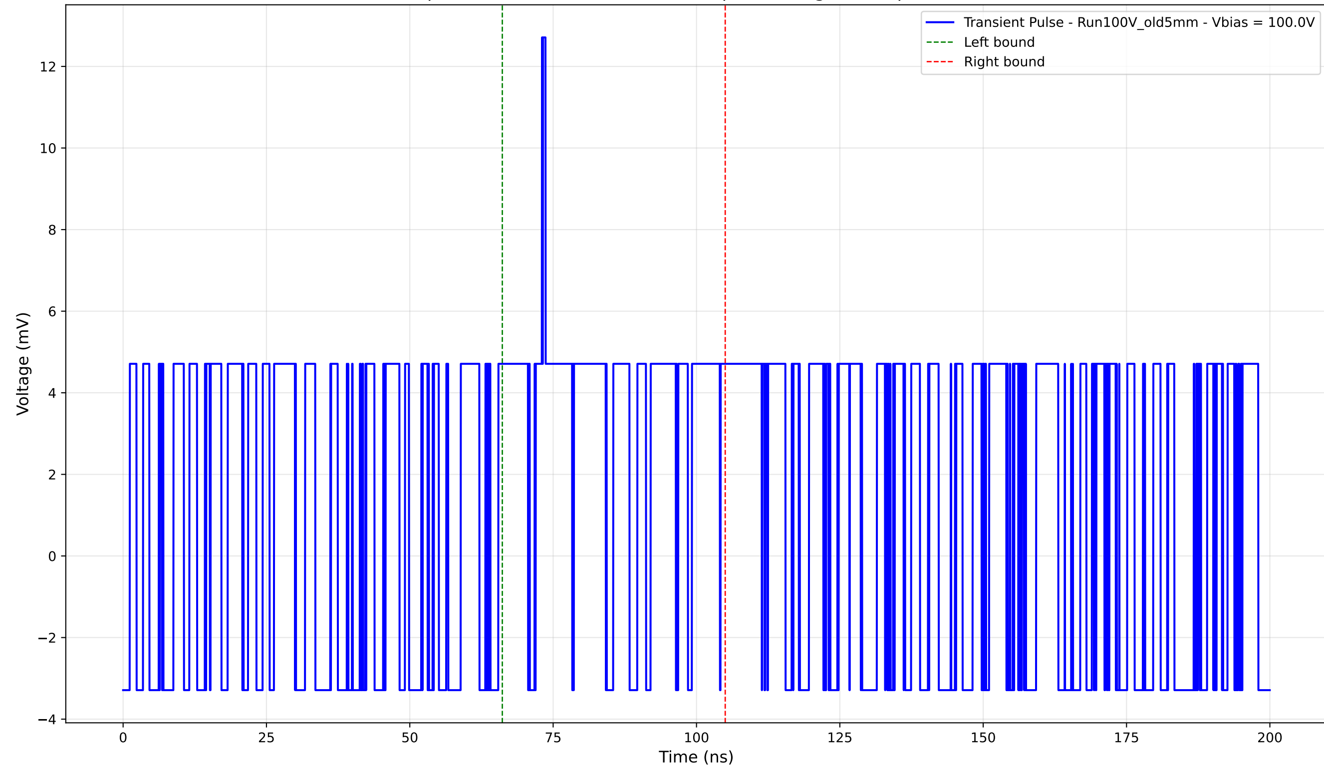
Transient Pulse - Sample: Old5mm - Position: 2315.0 \mu\text{m} - Charge: 2.81 pC - Rise Time: 0.00 ns (N/A)
