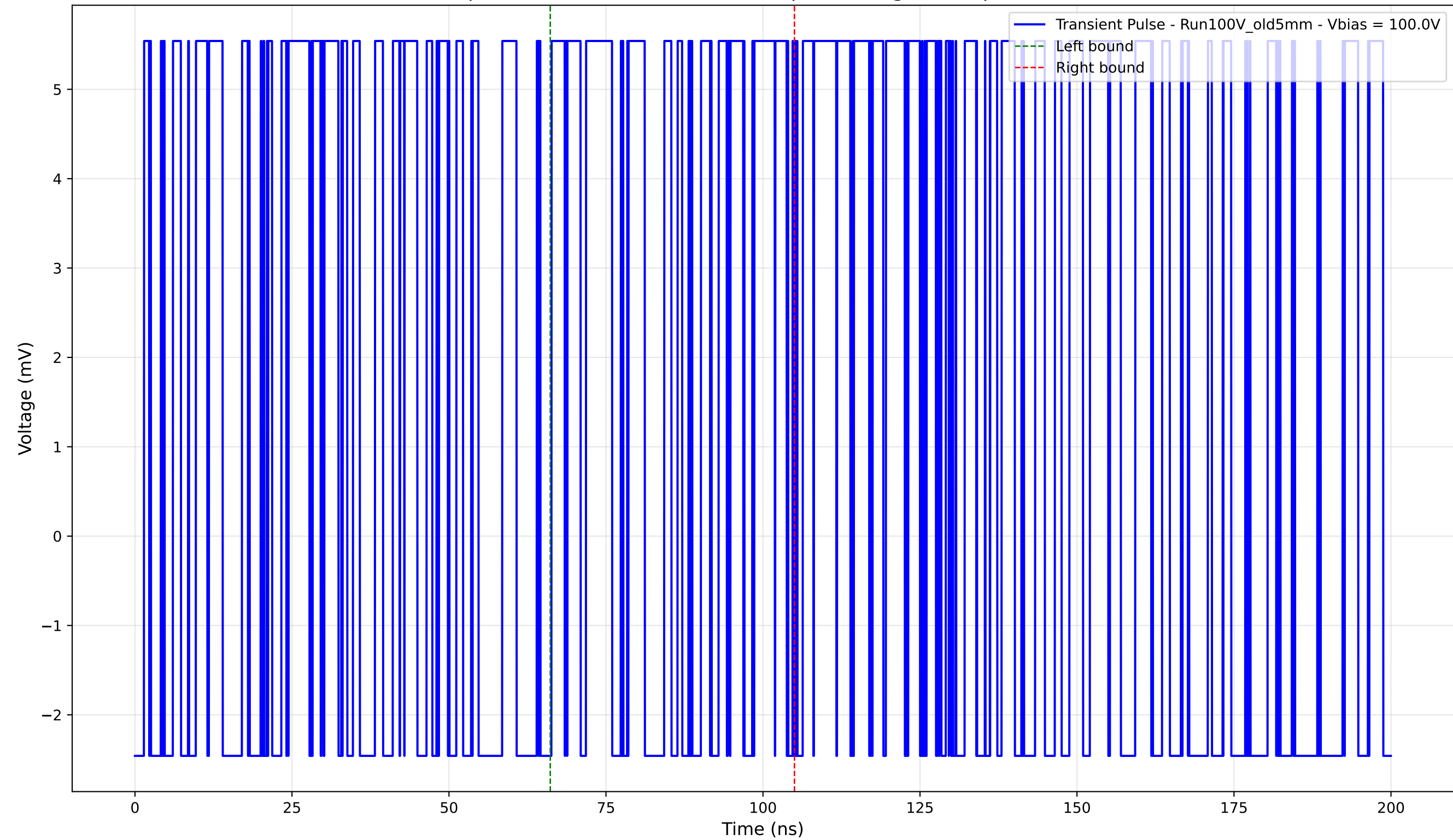
Transient Pulse - Sample: Old5mm - Position: 2785.0 \mu\text{m} - Charge: 2.06 pC - Rise Time: 0.00 ns (N/A)
