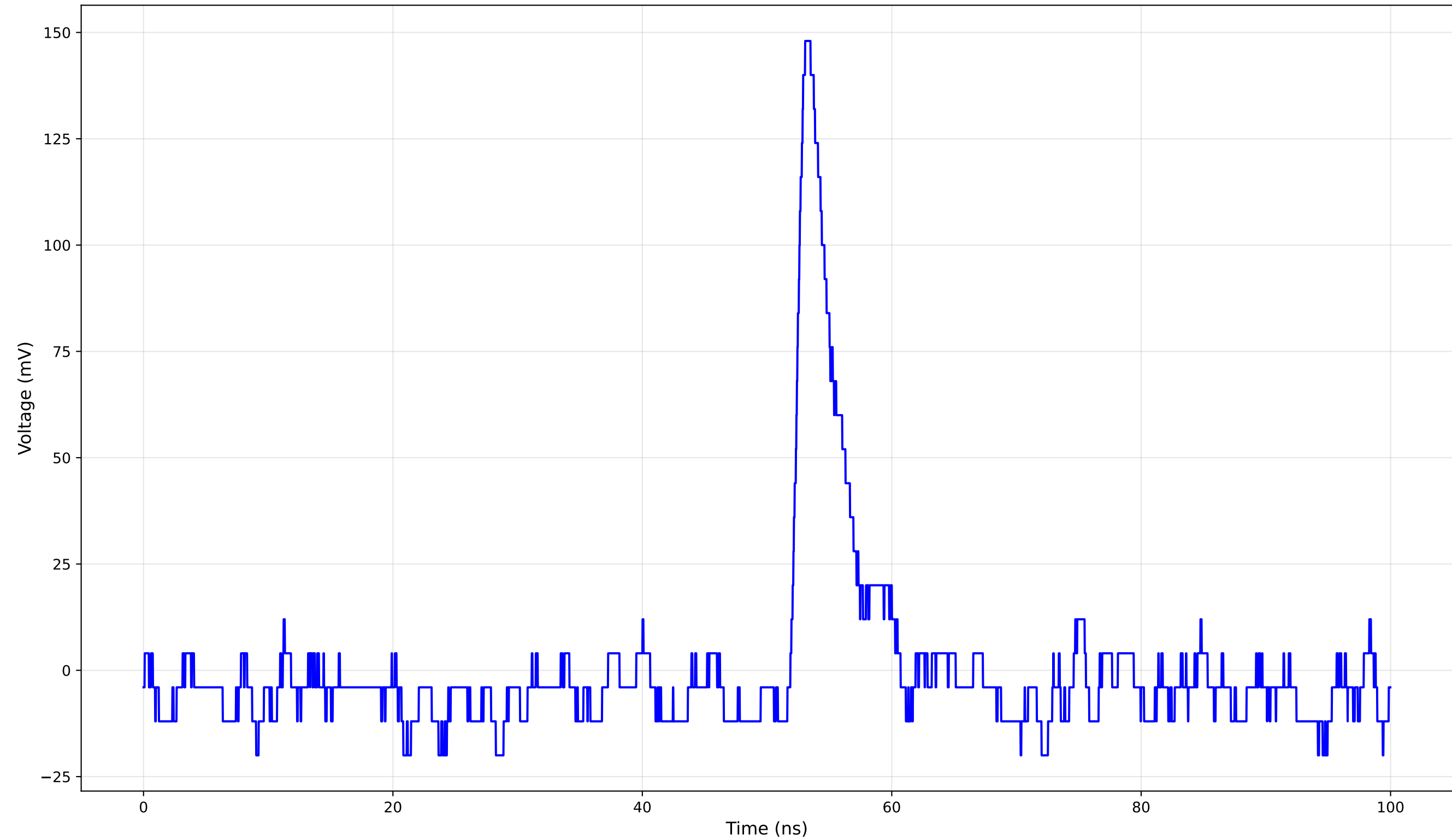
TCT Pulse Waveform - Run 13: 31 (450.0 V)
