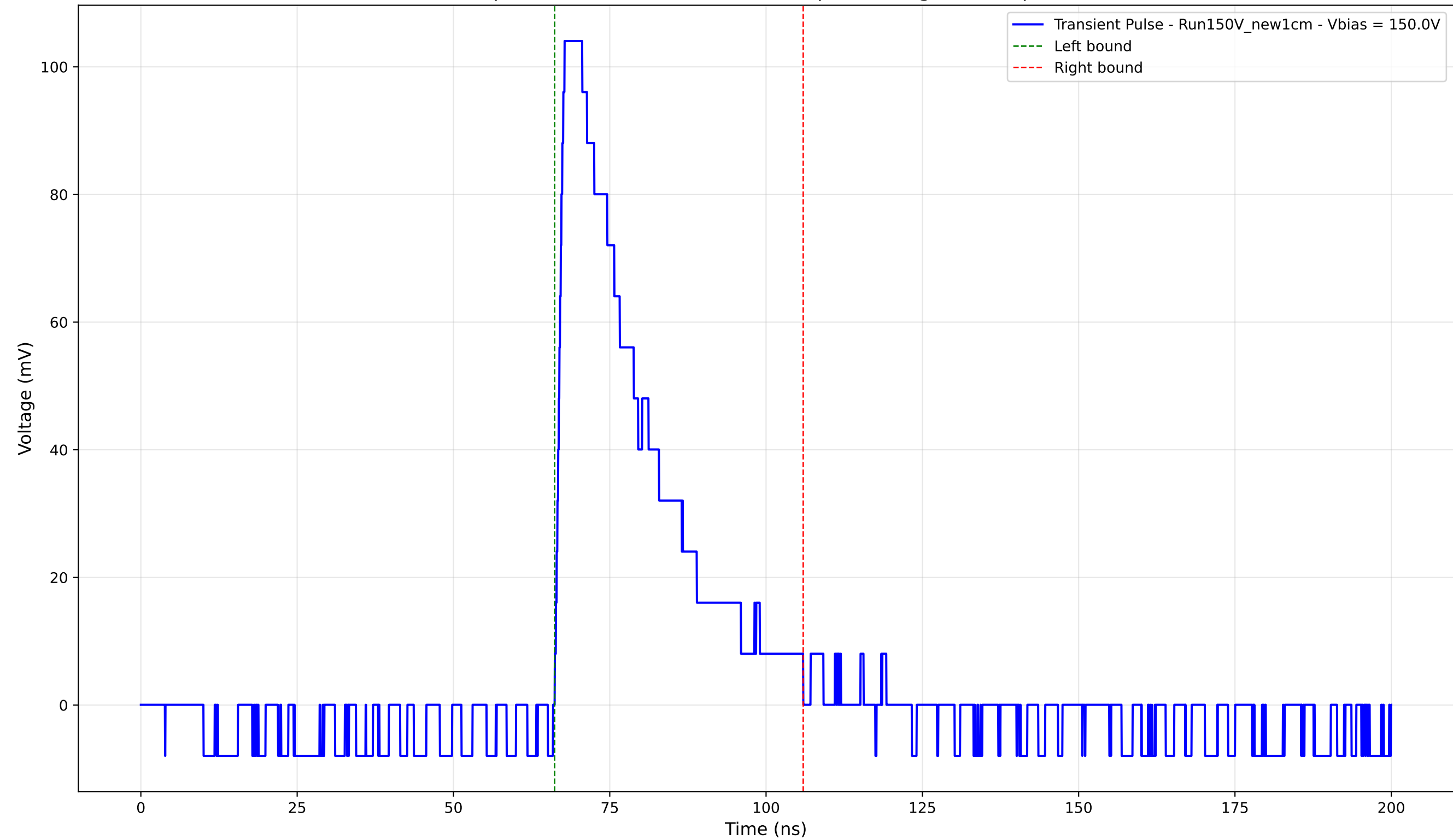
Transient Pulse - Sample: New1cm - Position: 1260.0 \mu\text{m} - Charge: 30.66 pC - Rise Time: 1.19 ns
