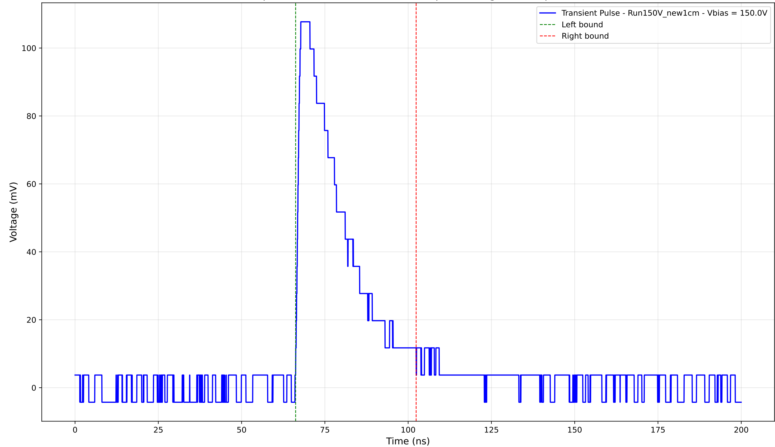
Transient Pulse - Sample: New1cm - Position: 1320.0 \mu\text{m} - Charge: 32.62 pC - Rise Time: 1.30 ns
