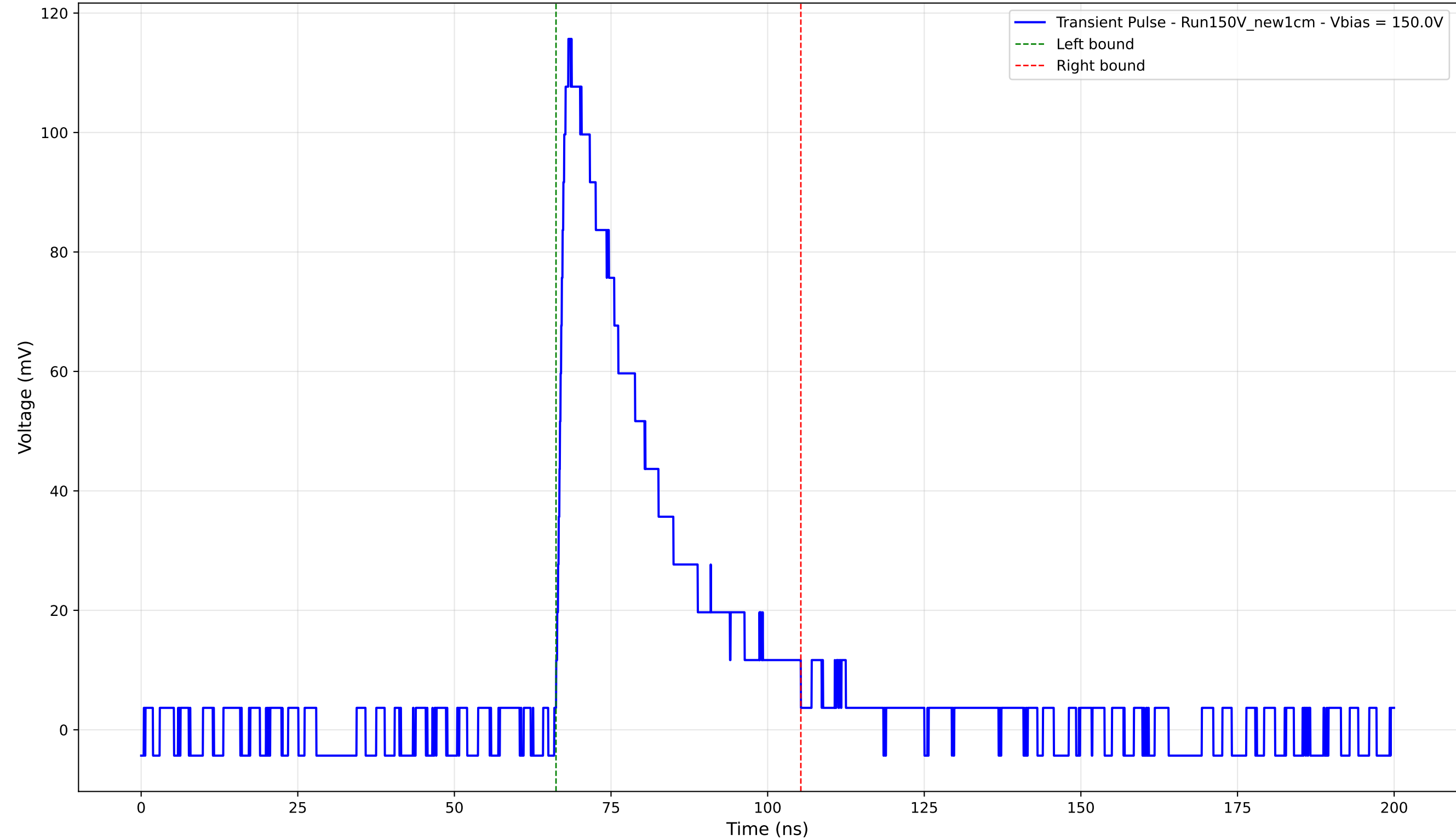
Transient Pulse - Sample: New1cm - Position: 1280.0 \mu\text{m} - Charge: 32.97 pC - Rise Time: 1.50 ns
