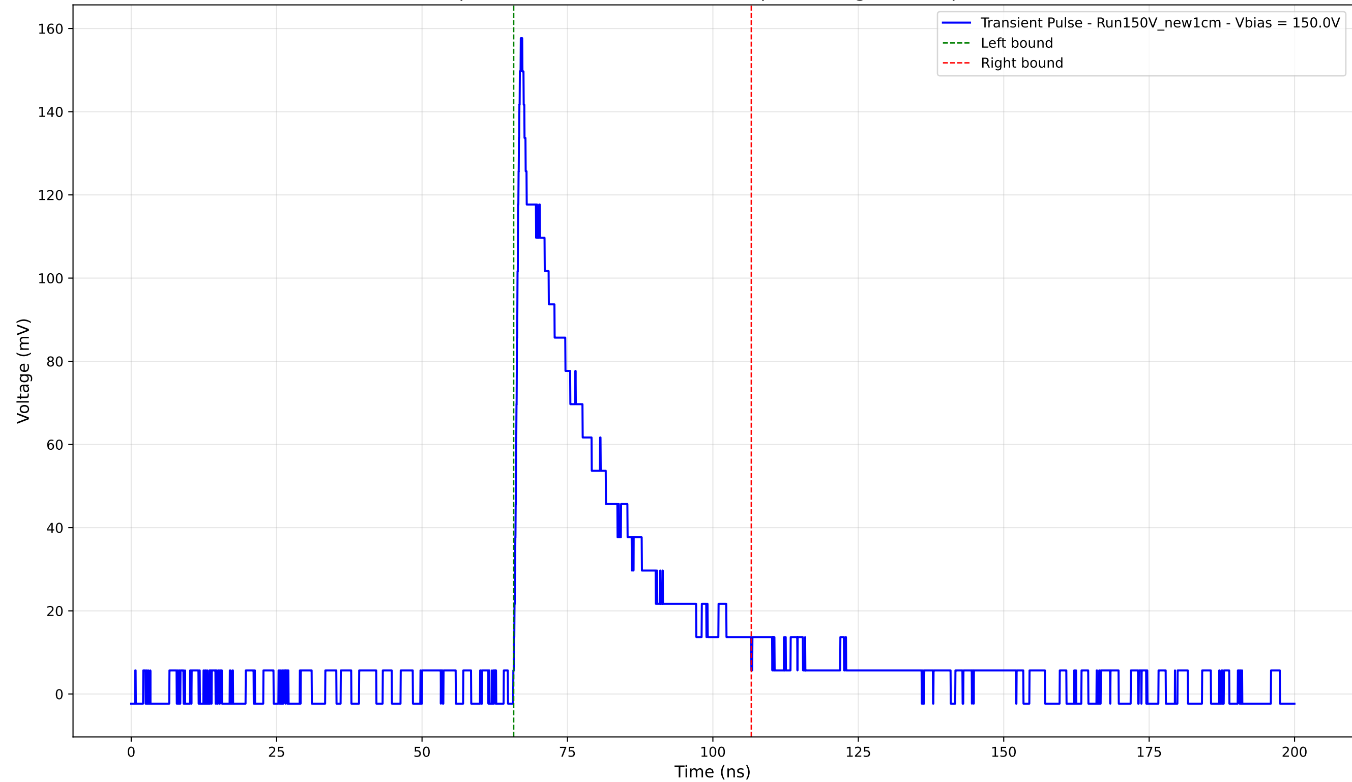
Transient Pulse - Sample: New1cm - Position: 2955.0 \mu\text{m} - Charge: 39.99 pC - Rise Time: 0.93 ns
