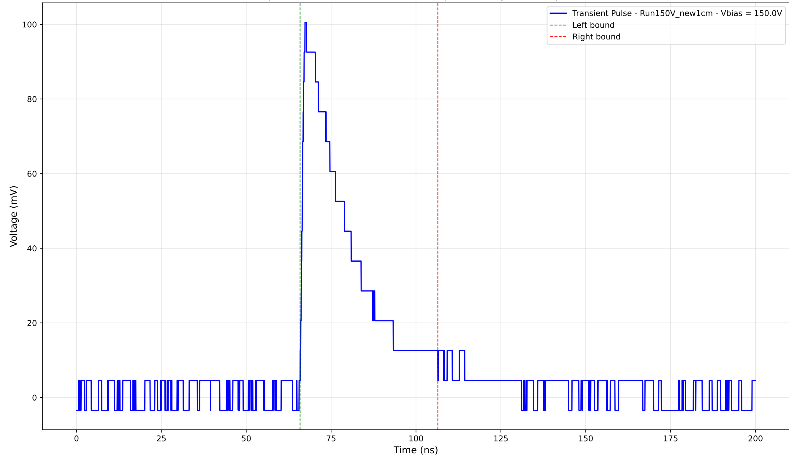
Transient Pulse - Sample: New1cm - Position: 1900.0 \mu\text{m} - Charge: 30.31 pC - Rise Time: 1.17 ns
