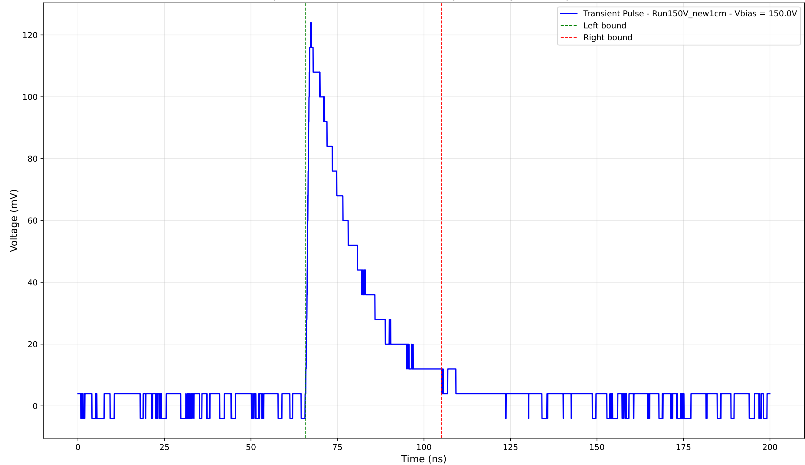
Transient Pulse - Sample: New1cm - Position: 3145.0 \mu\text{m} - Charge: 34.16 pC - Rise Time: 1.04 ns
