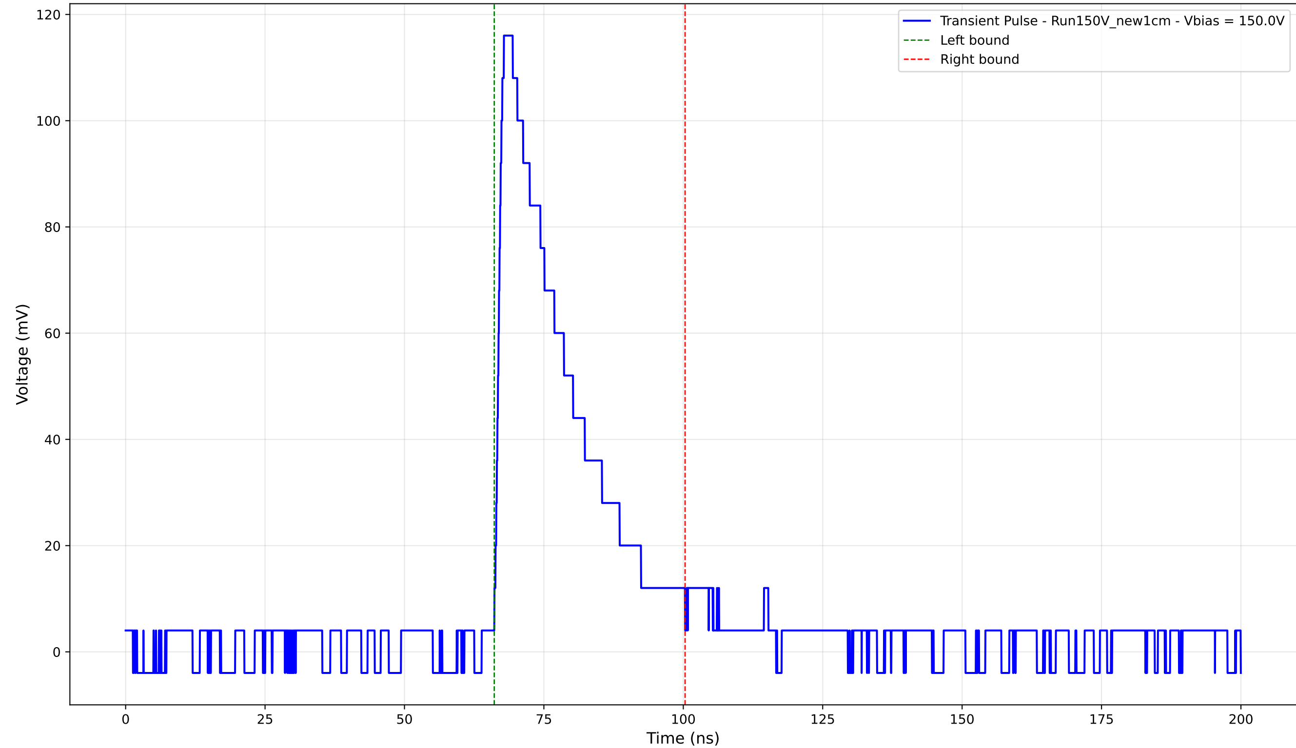
Transient Pulse - Sample: New1cm - Position: 860.0 \mu\text{m} - Charge: 31.69 pC - Rise Time: 1.42 ns
