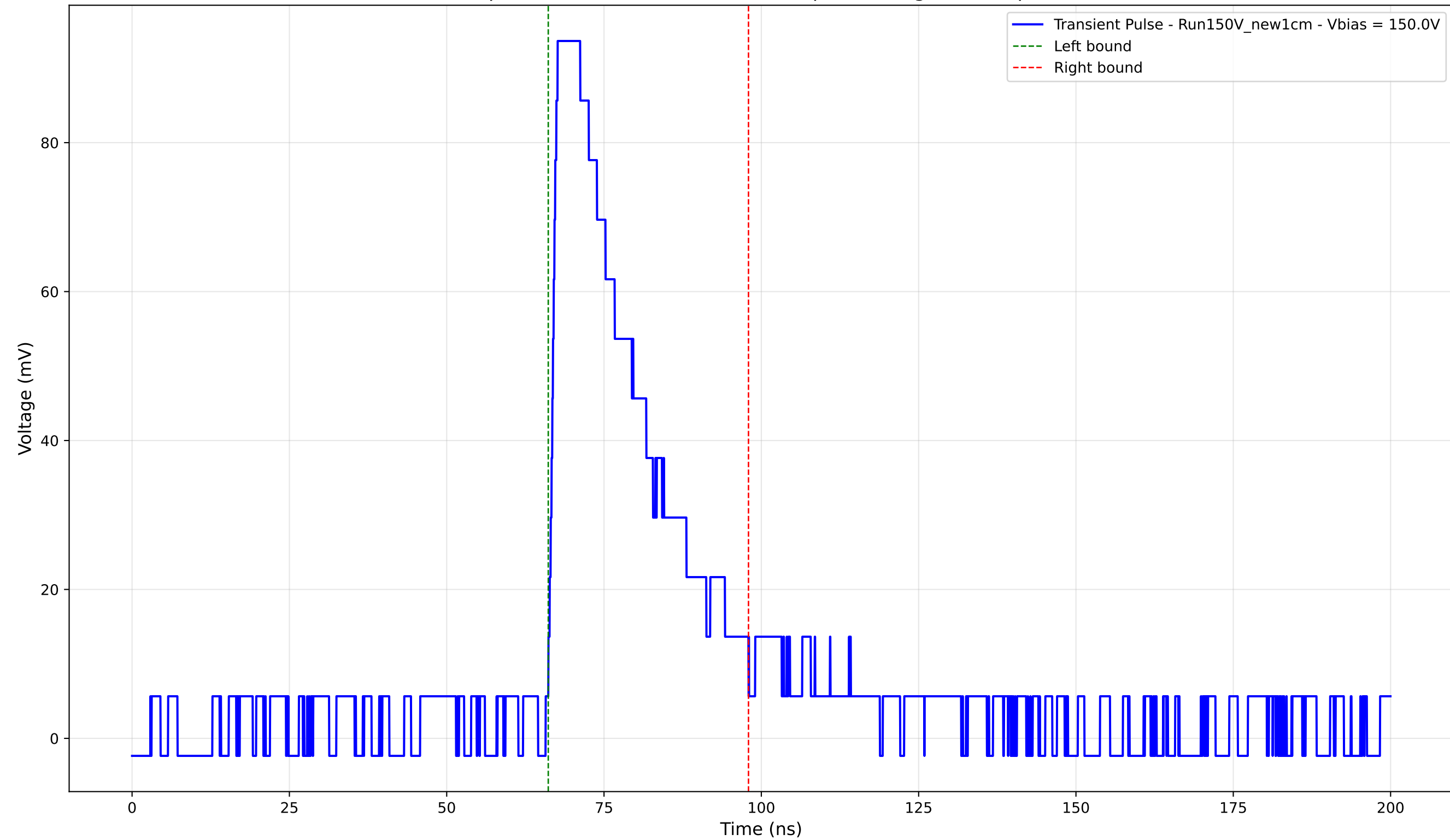
Transient Pulse - Sample: New1cm - Position: 1450.0 \mu\text{m} - Charge: 28.97 pC - Rise Time: 1.27 ns
