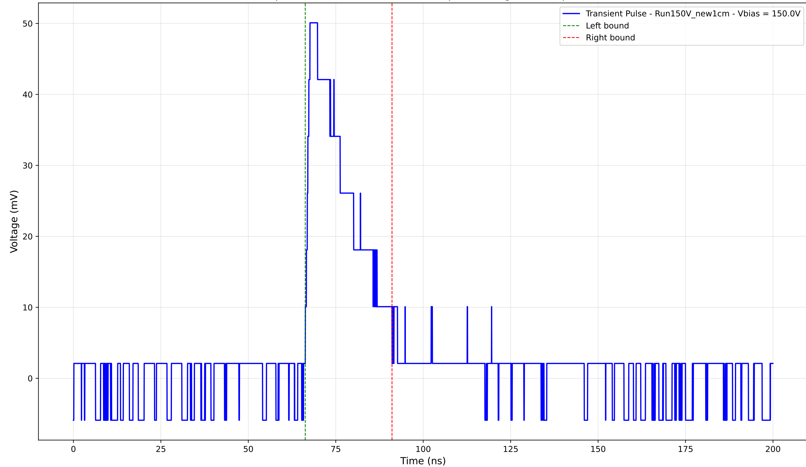
Transient Pulse - Sample: New1cm - Position: 985.0 \mu\text{m} - Charge: 13.11 pC - Rise Time: 1.33 ns
