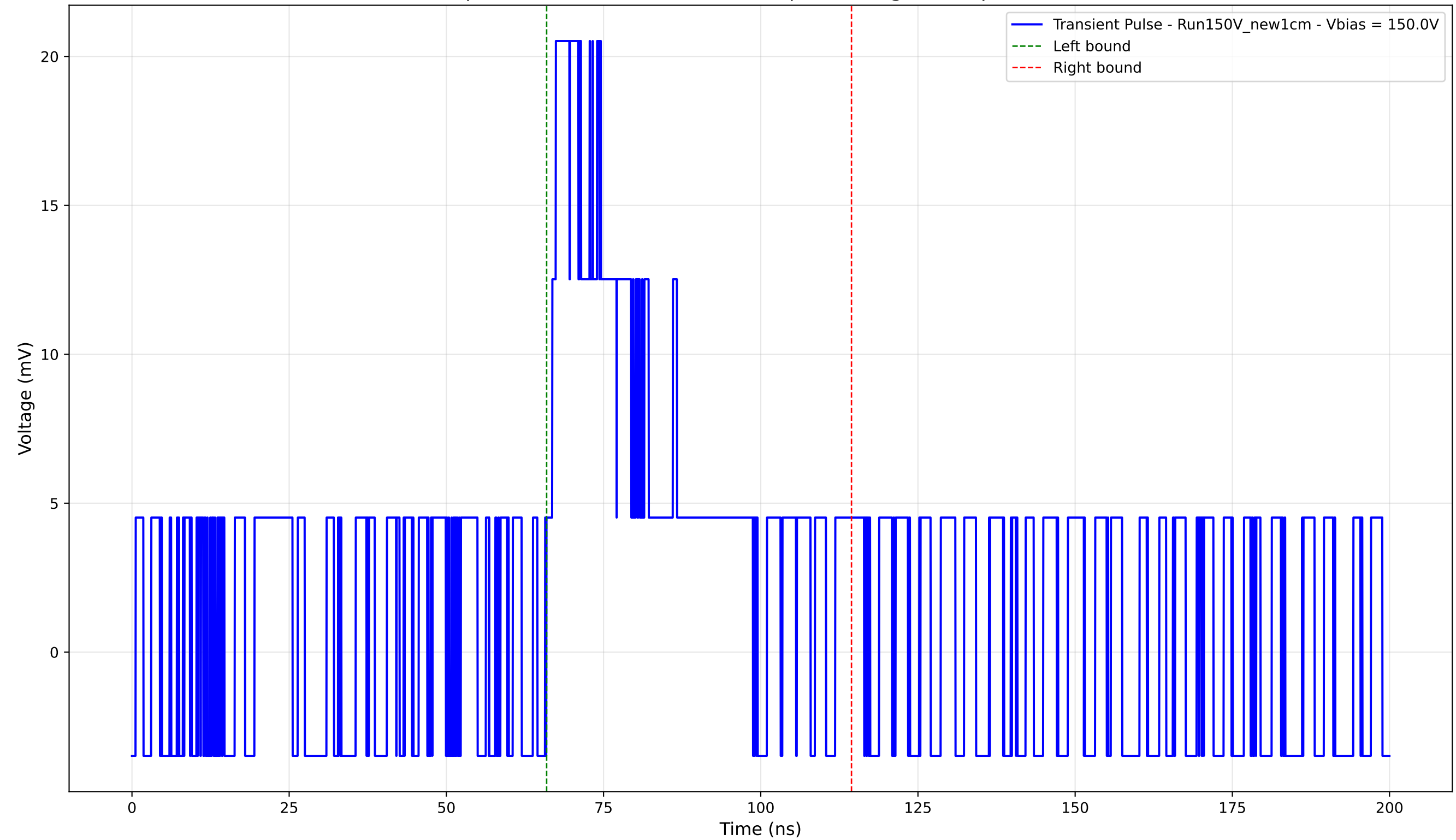
Transient Pulse - Sample: New1cm - Position: 4075.0 \mu\text{m} - Charge: 6.76 pC - Rise Time: 0.00 ns (N/A)
