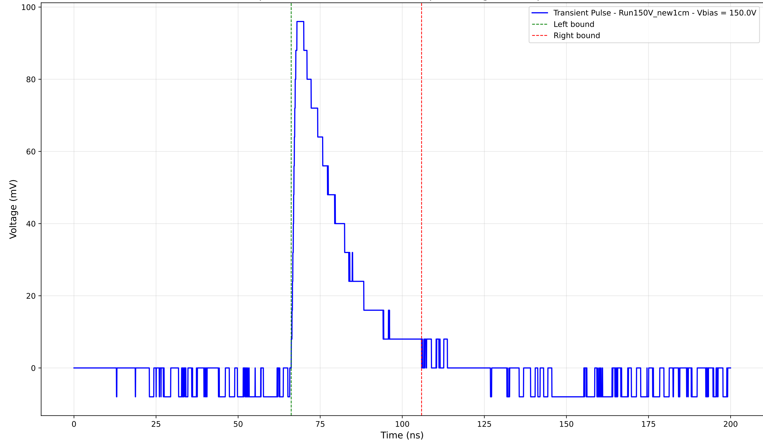
Transient Pulse - Sample: New1cm - Position: 1140.0 \mu\text{m} - Charge: 27.42 pC - Rise Time: 1.18 ns
