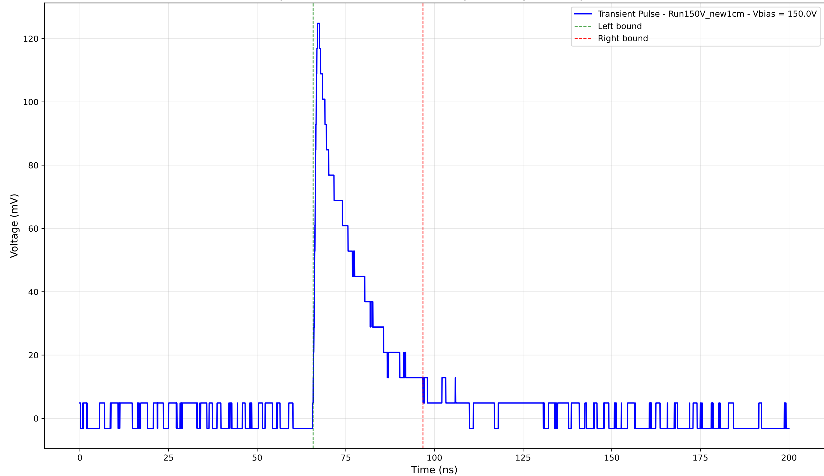
Transient Pulse - Sample: New1cm - Position: 4660.0 \mu\text{m} - Charge: 27.23 pC - Rise Time: 1.04 ns
