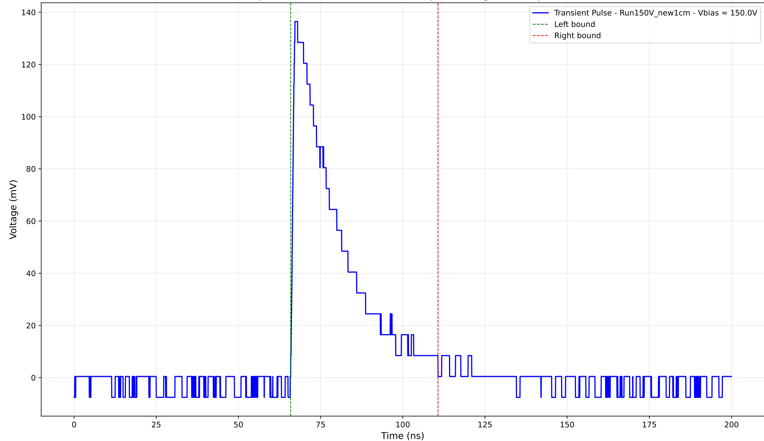
Transient Pulse - Sample: New1cm - Position: 3225.0 \mu\text{m} - Charge: 40.47 pC - Rise Time: 1.03 ns
