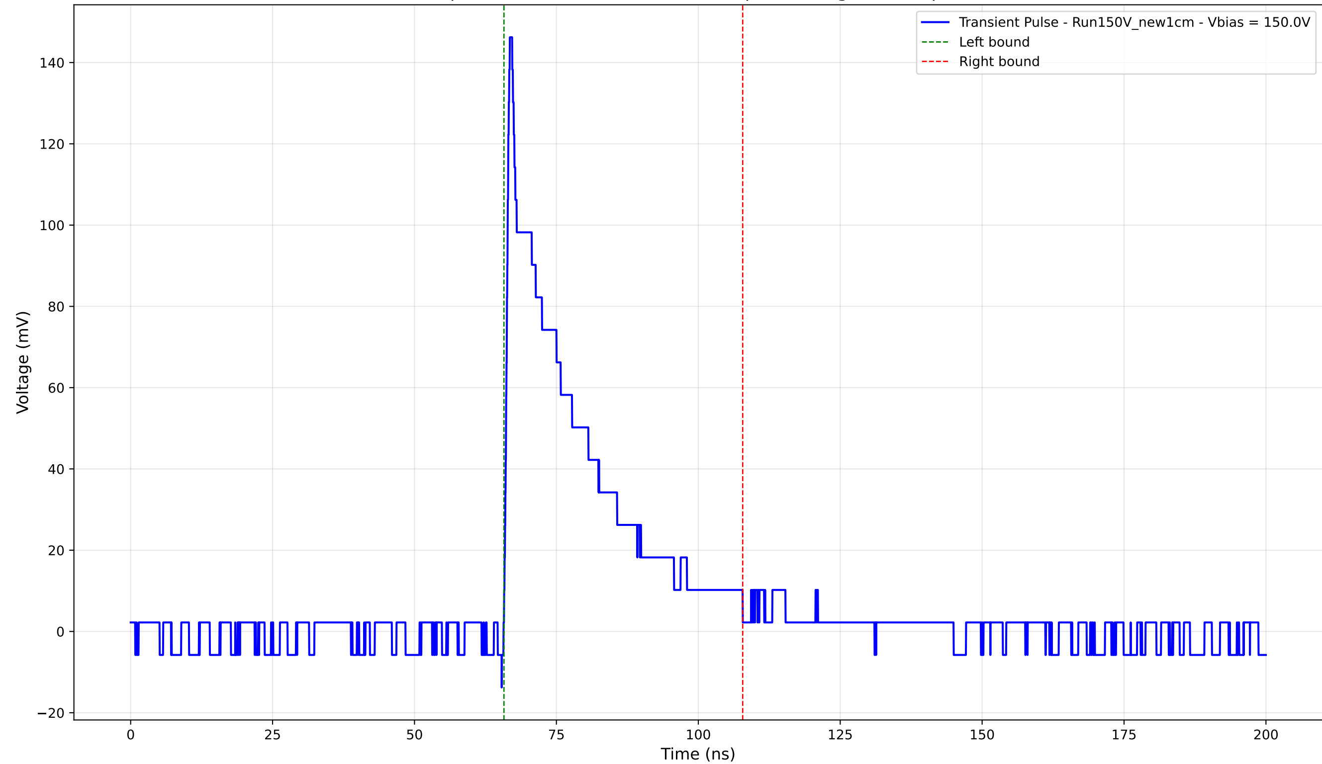
Transient Pulse - Sample: New1cm - Position: 2210.0 \mu\text{m} - Charge: 33.67 pC - Rise Time: 0.83 ns
