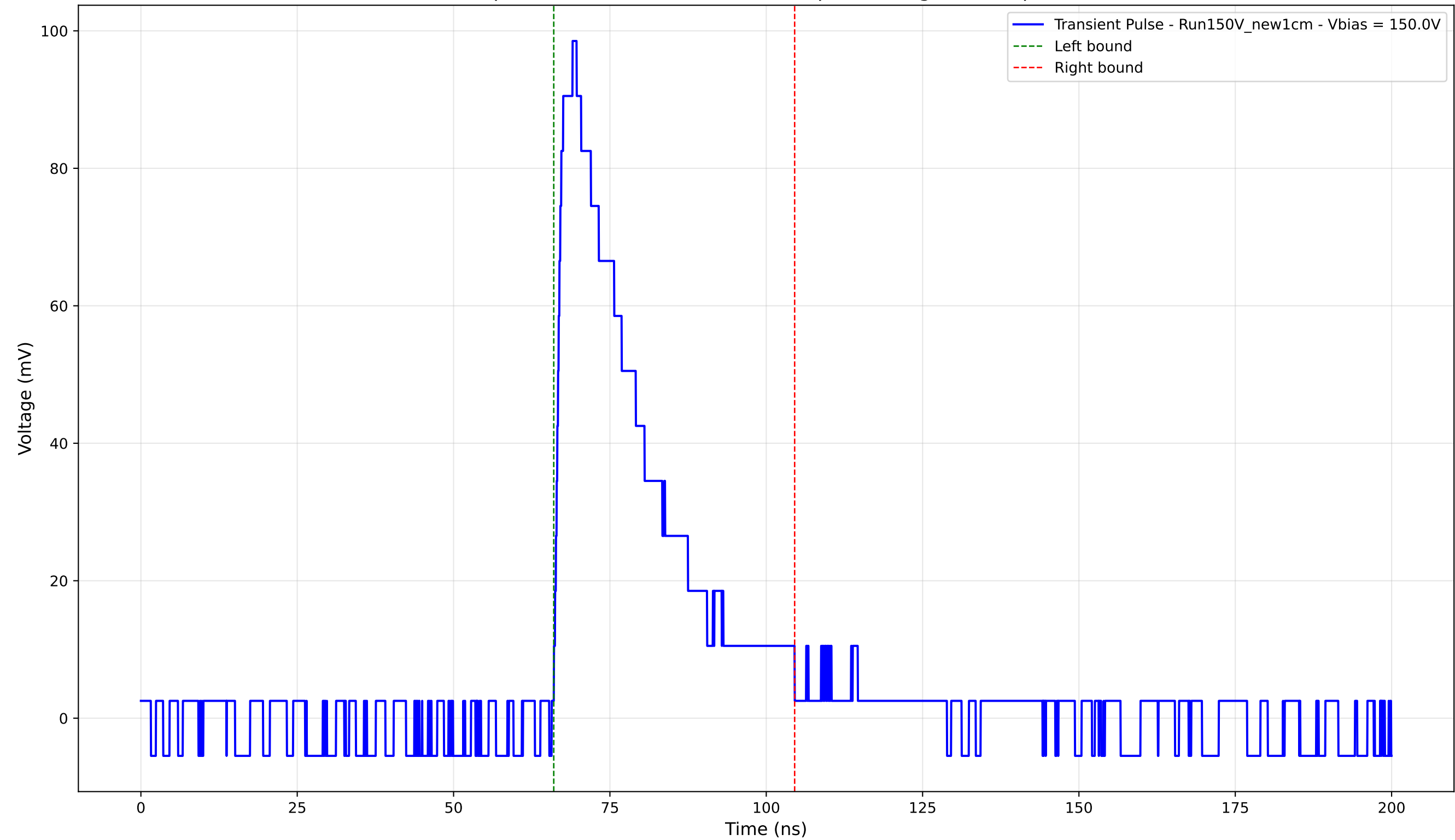
Transient Pulse - Sample: New1cm - Position: 1640.0 \mu\text{m} - Charge: 27.90 pC - Rise Time: 1.48 ns
