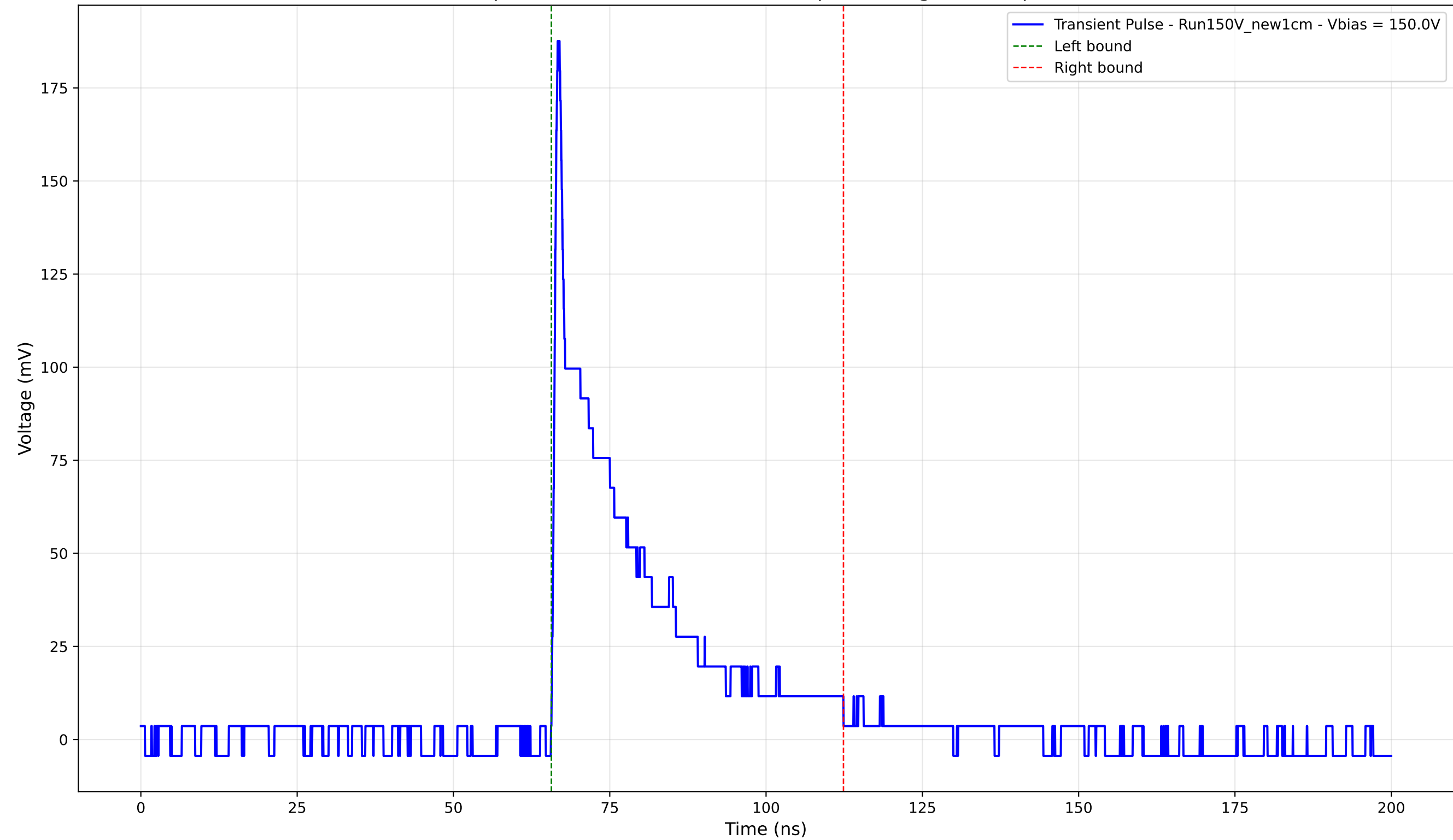
Transient Pulse - Sample: New1cm - Position: 2390.0 \mu\text{m} - Charge: 36.81 pC - Rise Time: 0.76 ns
