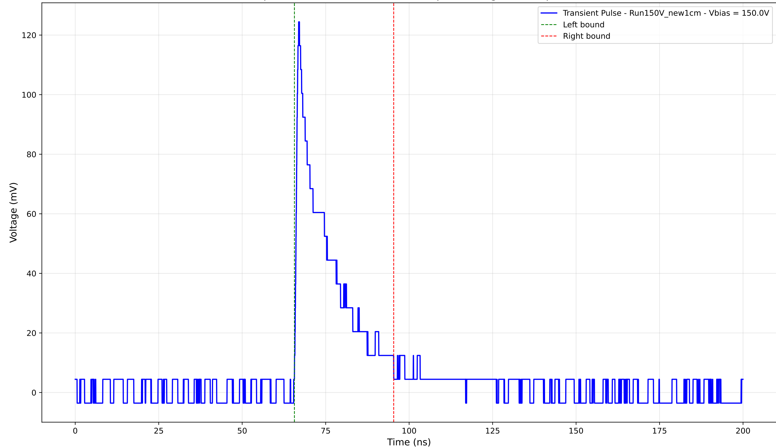
Transient Pulse - Sample: New1cm - Position: 4825.0 \mu\text{m} - Charge: 23.85 pC - Rise Time: 0.92 ns
