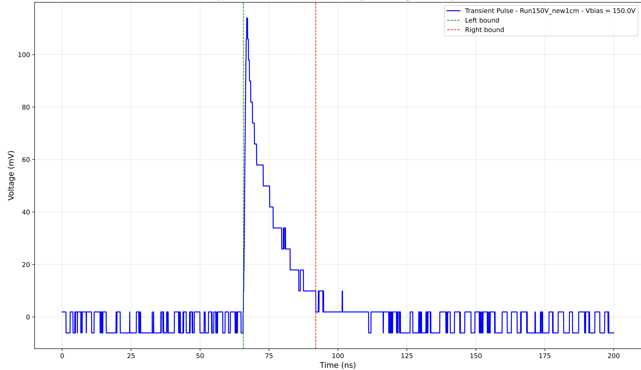
Transient Pulse - Sample: New1cm - Position: 4830.0 \mu\text{m} - Charge: 20.04 pC - Rise Time: 0.88 ns
