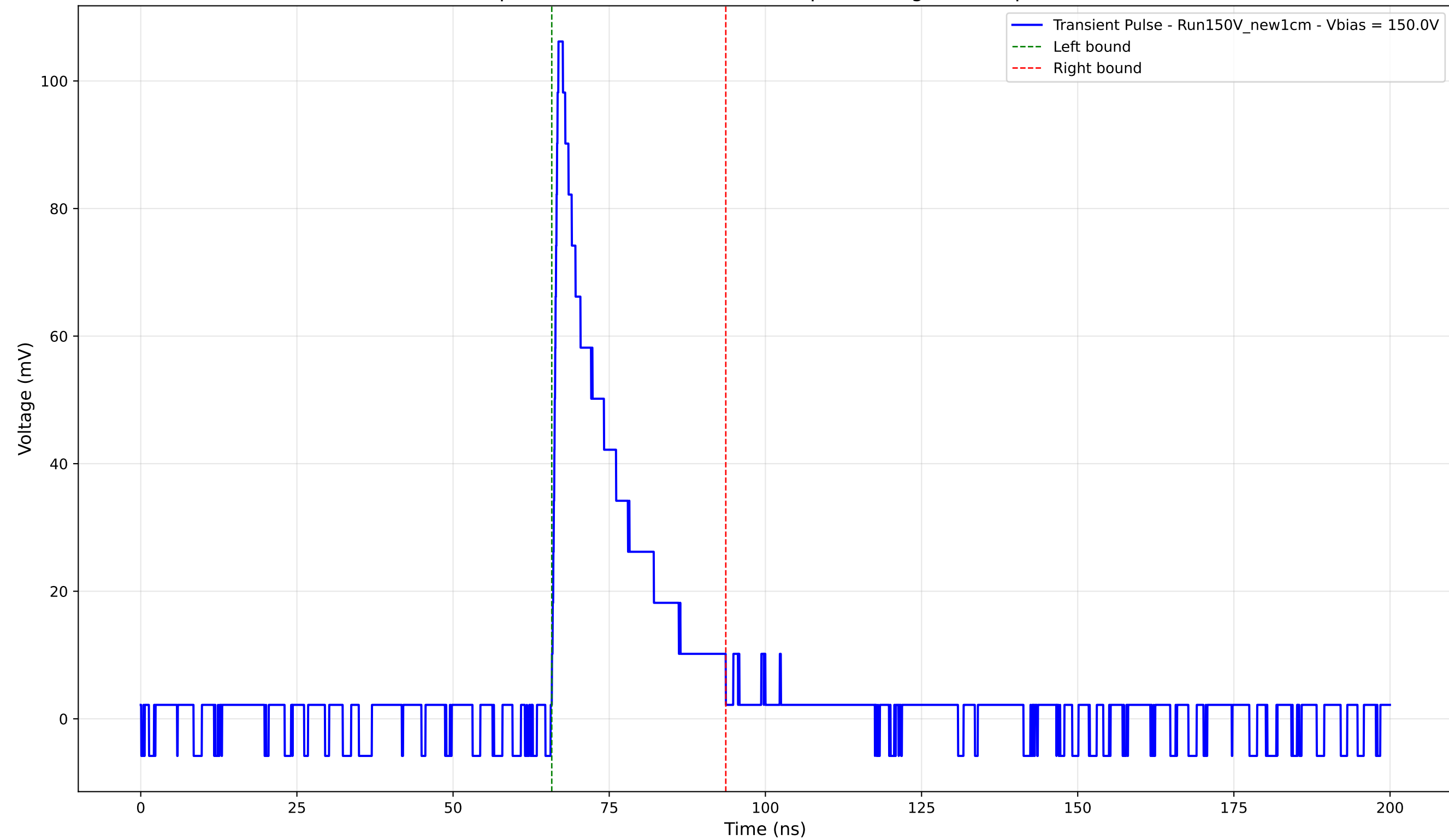
Transient Pulse - Sample: New1cm - Position: 120.0 \mu\text{m} - Charge: 19.33 pC - Rise Time: 0.80 ns
