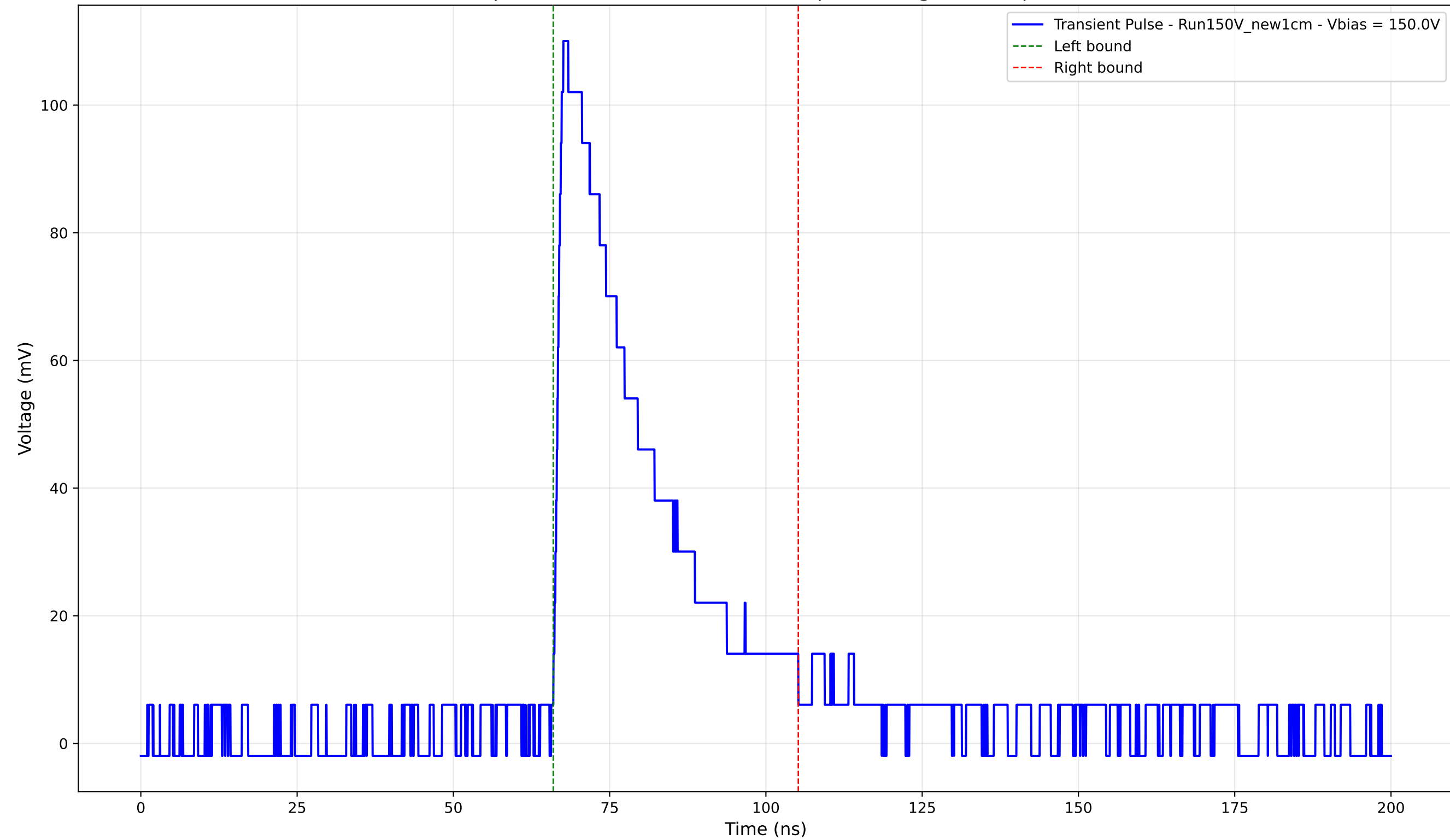
Transient Pulse - Sample: New1cm - Position: 3490.0 \mu\text{m} - Charge: 33.42 pC - Rise Time: 1.33 ns
