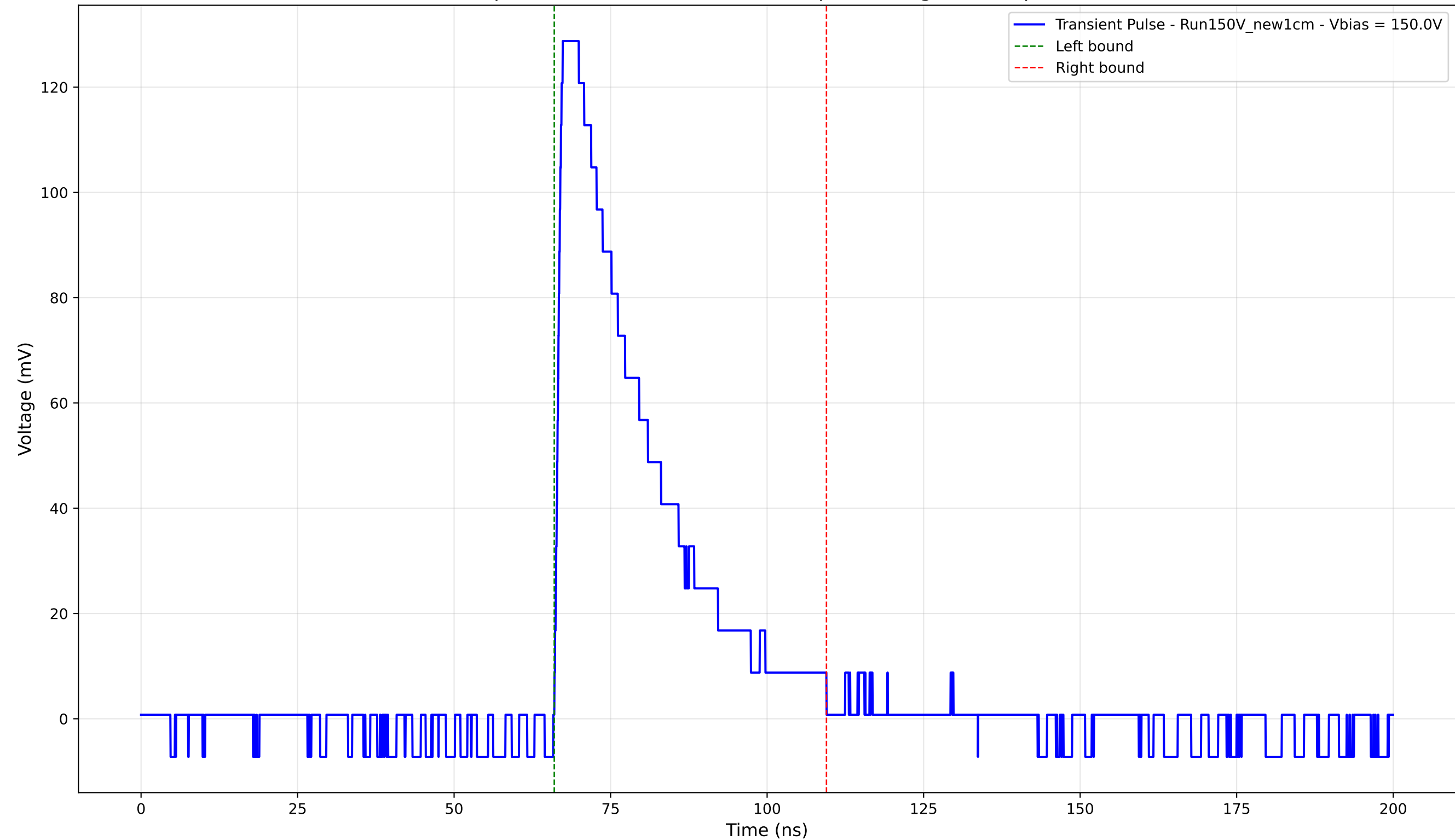
Transient Pulse - Sample: New1cm - Position: 3395.0 \mu\text{m} - Charge: 38.85 pC - Rise Time: 1.05 ns
