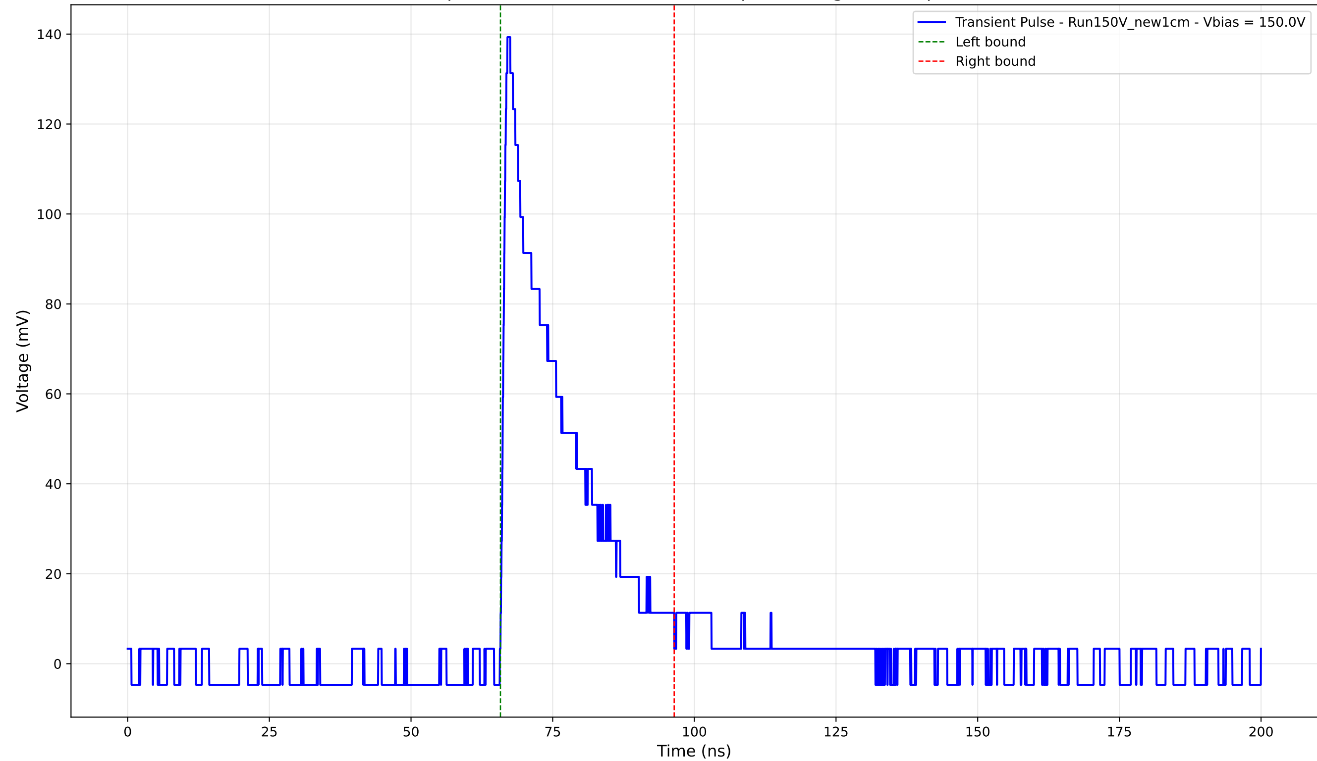
Transient Pulse - Sample: New1cm - Position: 4705.0 \mu\text{m} - Charge: 29.71 pC - Rise Time: 0.95 ns
