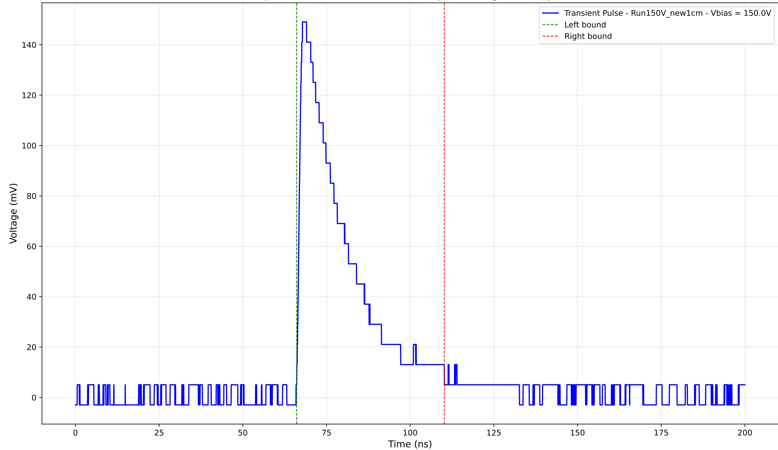
Transient Pulse - Sample: New1cm - Position: 3850.0 \mu\text{m} - Charge: 44.56 pC - Rise Time: 1.36 ns
