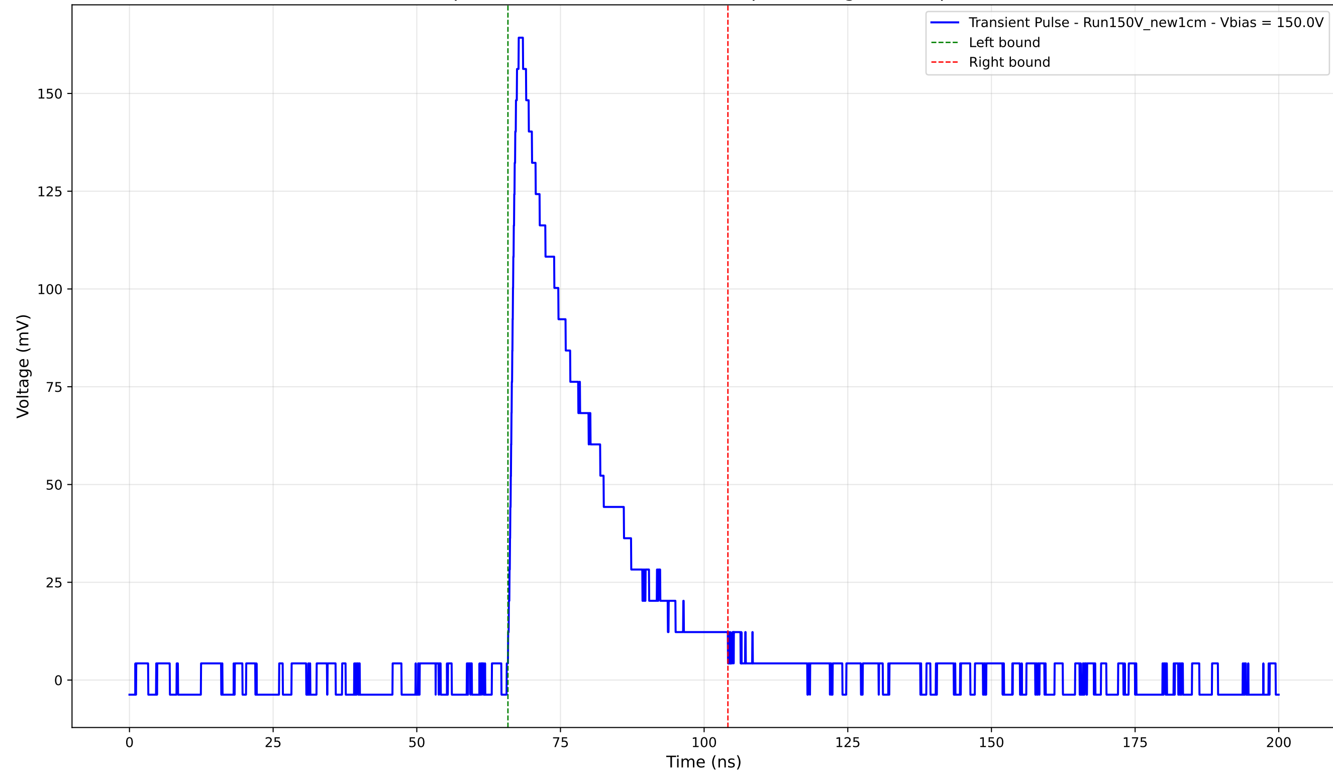
Transient Pulse - Sample: New1cm - Position: 4330.0 \mu\text{m} - Charge: 42.47 pC - Rise Time: 1.25 ns
