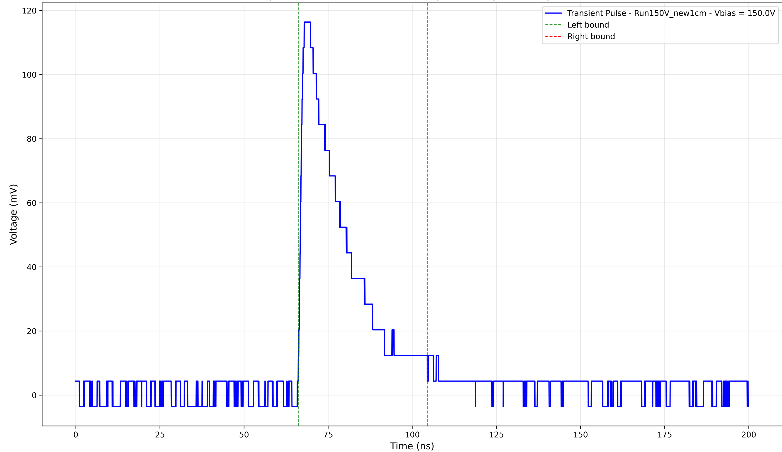
Transient Pulse - Sample: New1cm - Position: 895.0 \mu\text{m} - Charge: 33.09 pC - Rise Time: 1.44 ns
