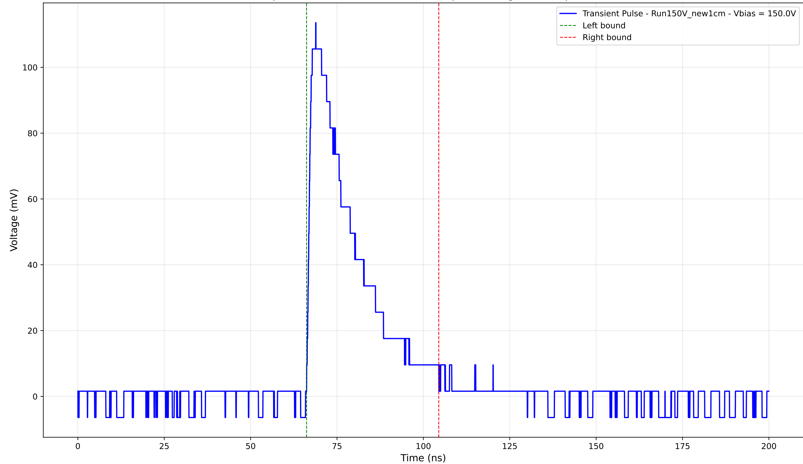
Transient Pulse - Sample: New1cm - Position: 1340.0 \mu\text{m} - Charge: 31.28 pC - Rise Time: 1.48 ns
