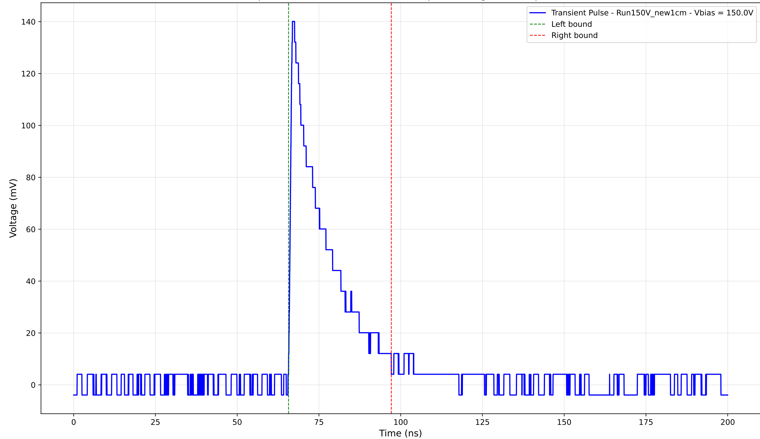
Transient Pulse - Sample: New1cm - Position: 4730.0 \mu\text{m} - Charge: 31.12 pC - Rise Time: 0.96 ns
