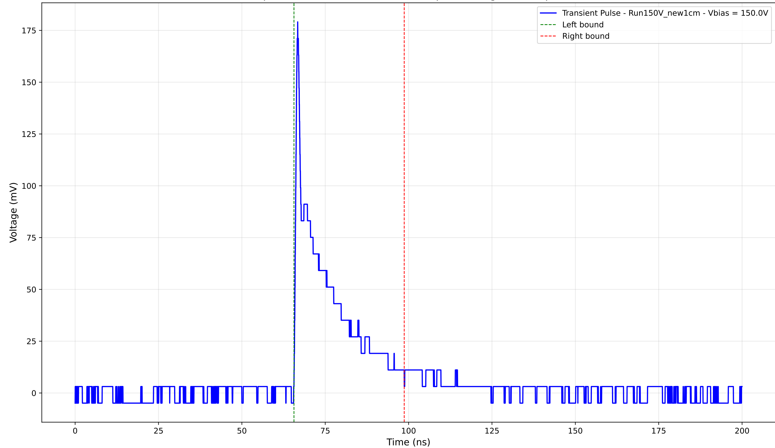
Transient Pulse - Sample: New1cm - Position: 2635.0 \mu\text{m} - Charge: 28.25 pC - Rise Time: 0.80 ns
