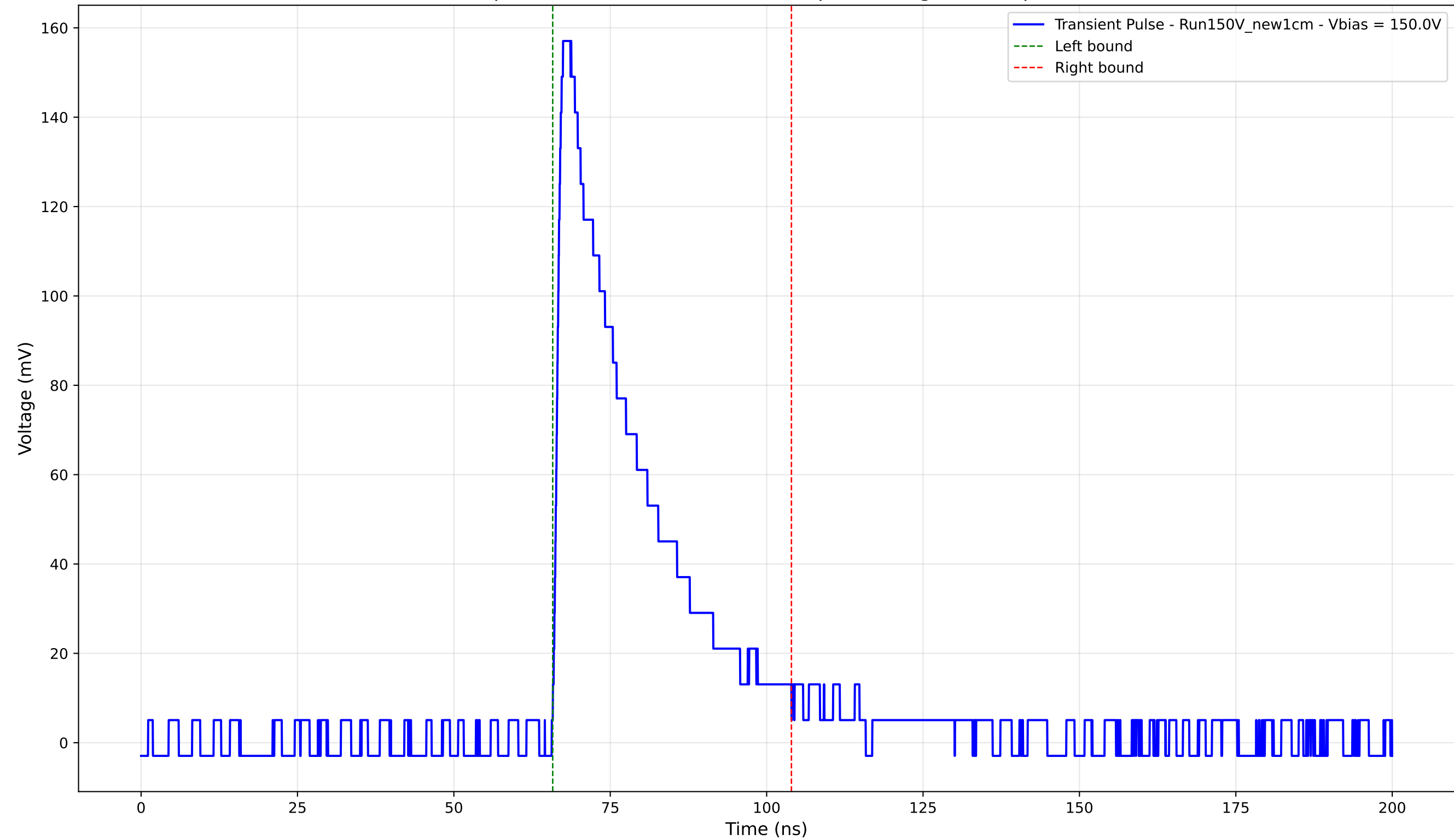
Transient Pulse - Sample: New1cm - Position: 4370.0 \mu\text{m} - Charge: 42.51 pC - Rise Time: 1.27 ns
