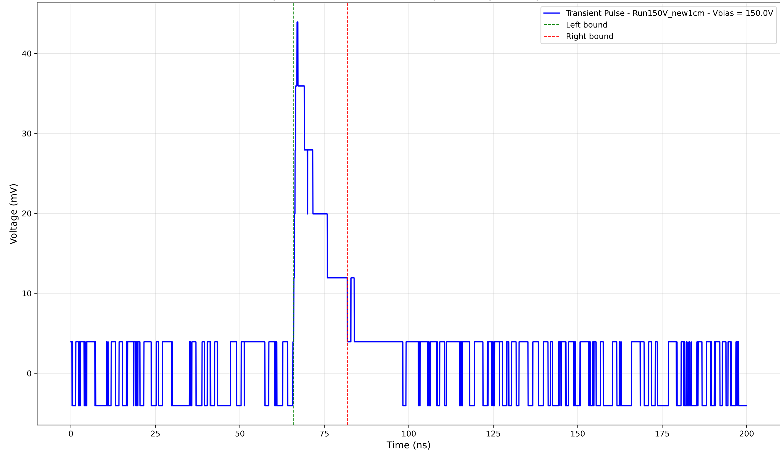
Transient Pulse - Sample: New1cm - Position: 65.0 \mu\text{m} - Charge: 6.61 pC - Rise Time: 0.96 ns
