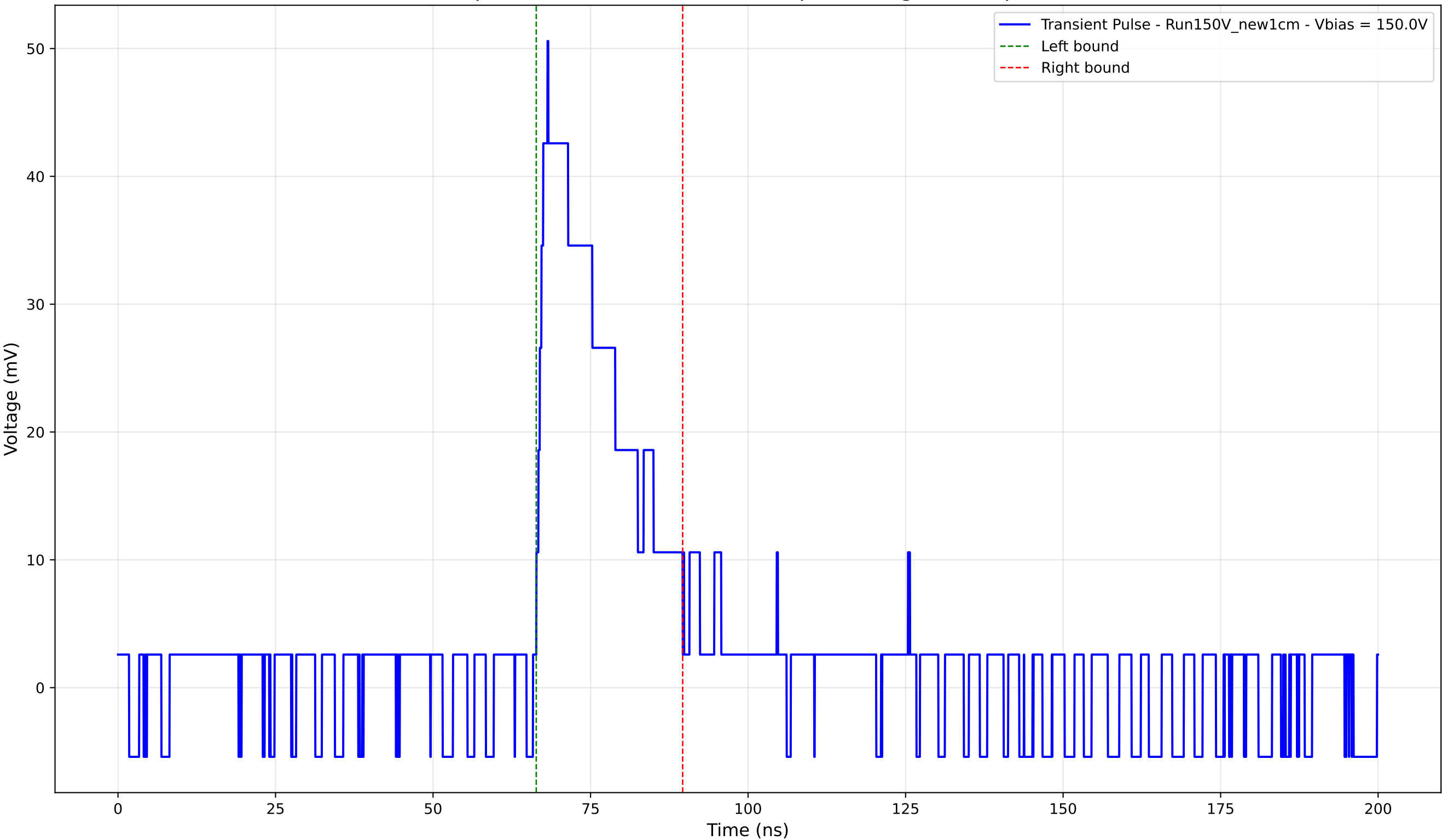
Transient Pulse - Sample: New1cm - Position: 1080.0 \mu\text{m} - Charge: 11.56 pC - Rise Time: 1.77 ns
