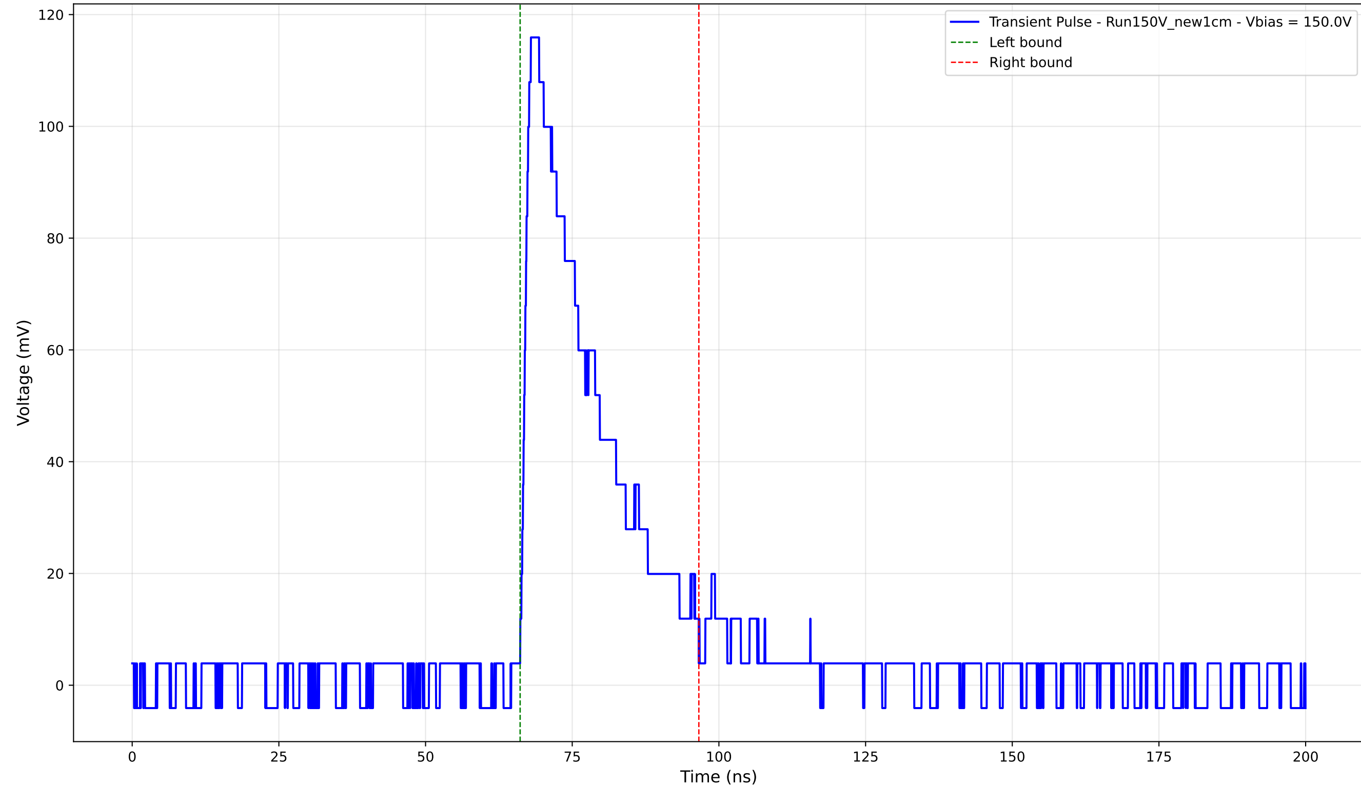
Transient Pulse - Sample: New1cm - Position: 910.0 \mu\text{m} - Charge: 30.34 pC - Rise Time: 1.52 ns
