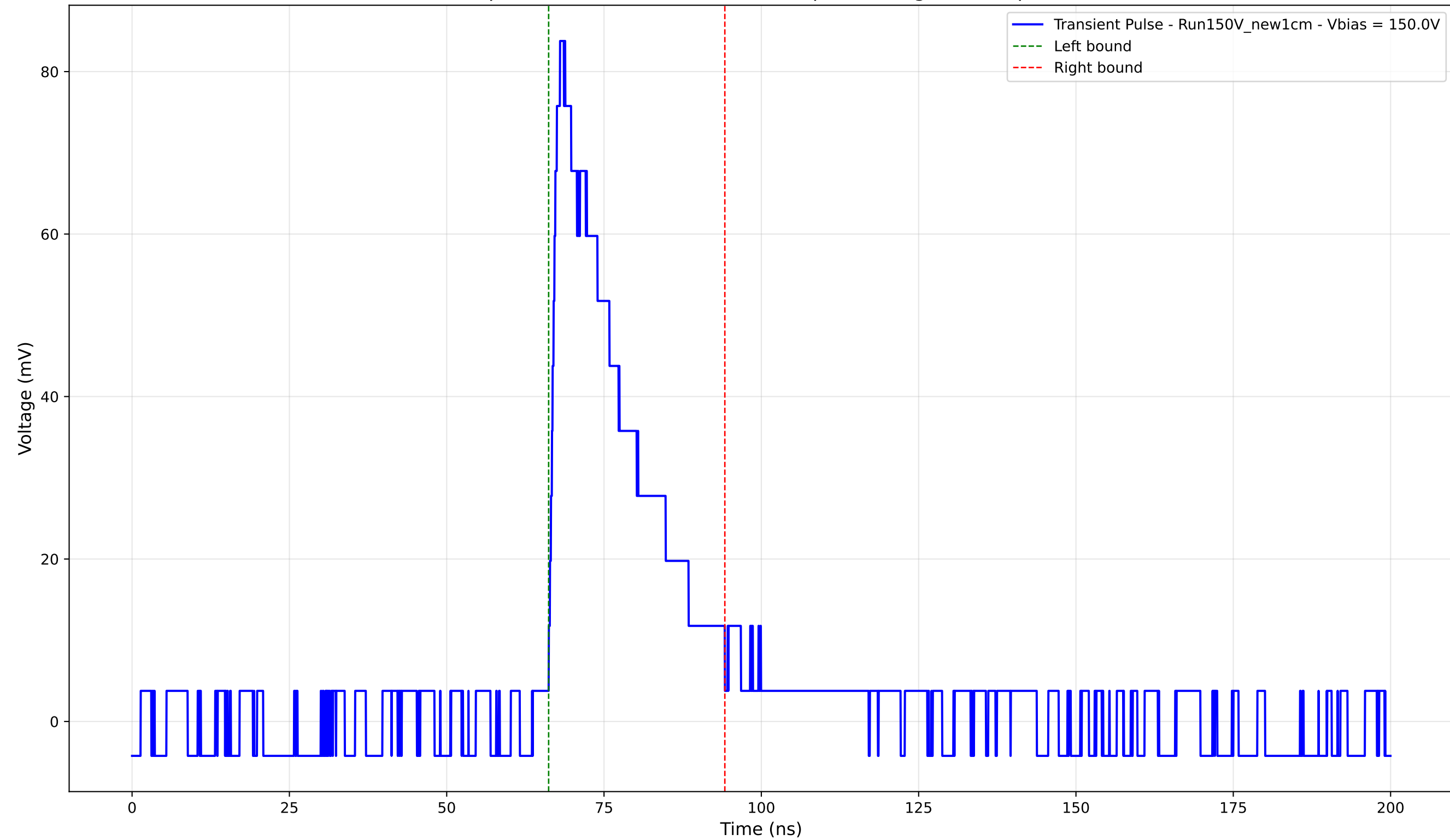
Transient Pulse - Sample: New1cm - Position: 4010.0 \mu\text{m} - Charge: 20.63 pC - Rise Time: 1.29 ns
