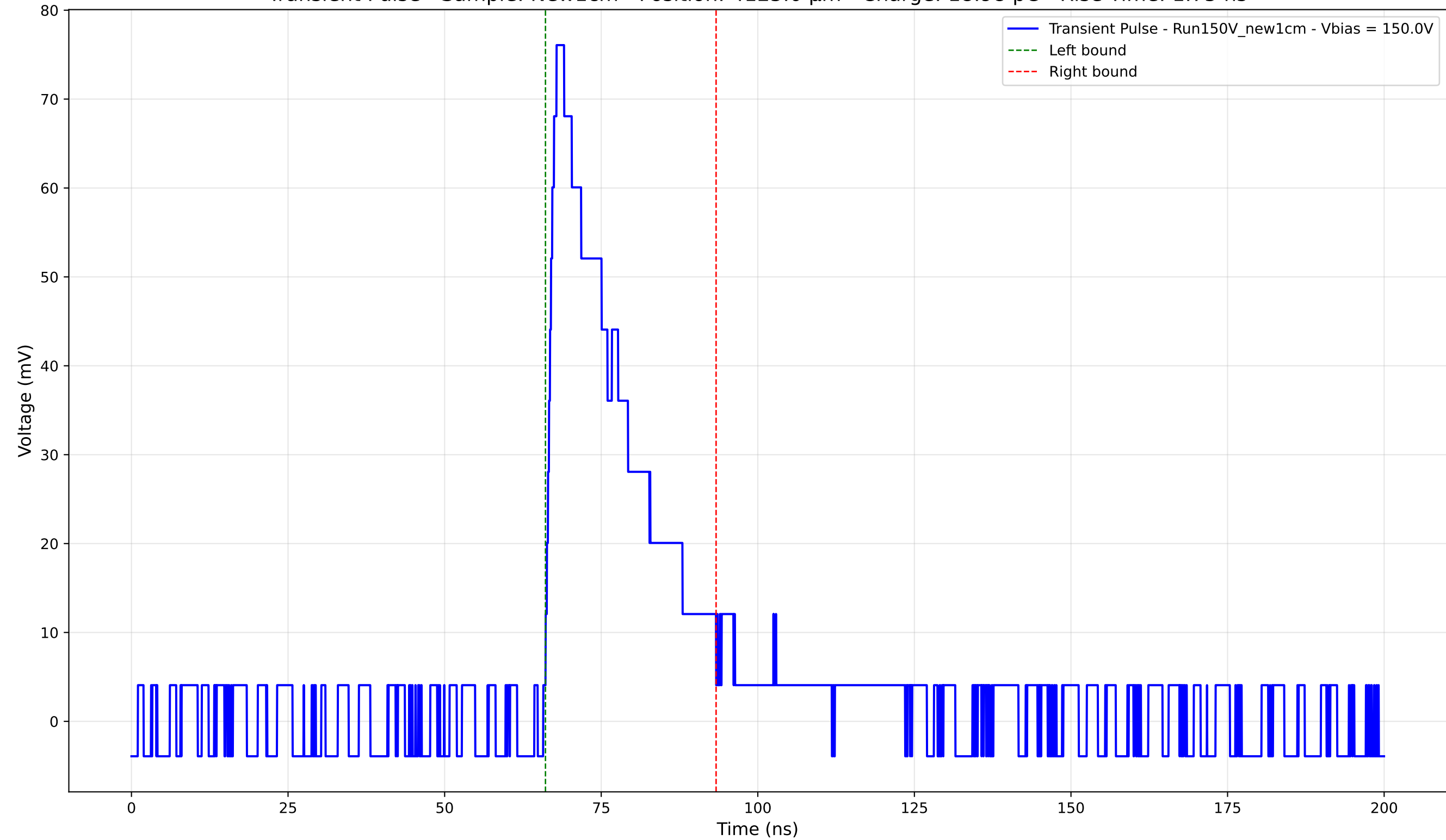
Transient Pulse - Sample: New1cm - Position: 4125.0 \mu\text{m} - Charge: 18.98 pC - Rise Time: 1.75 ns
