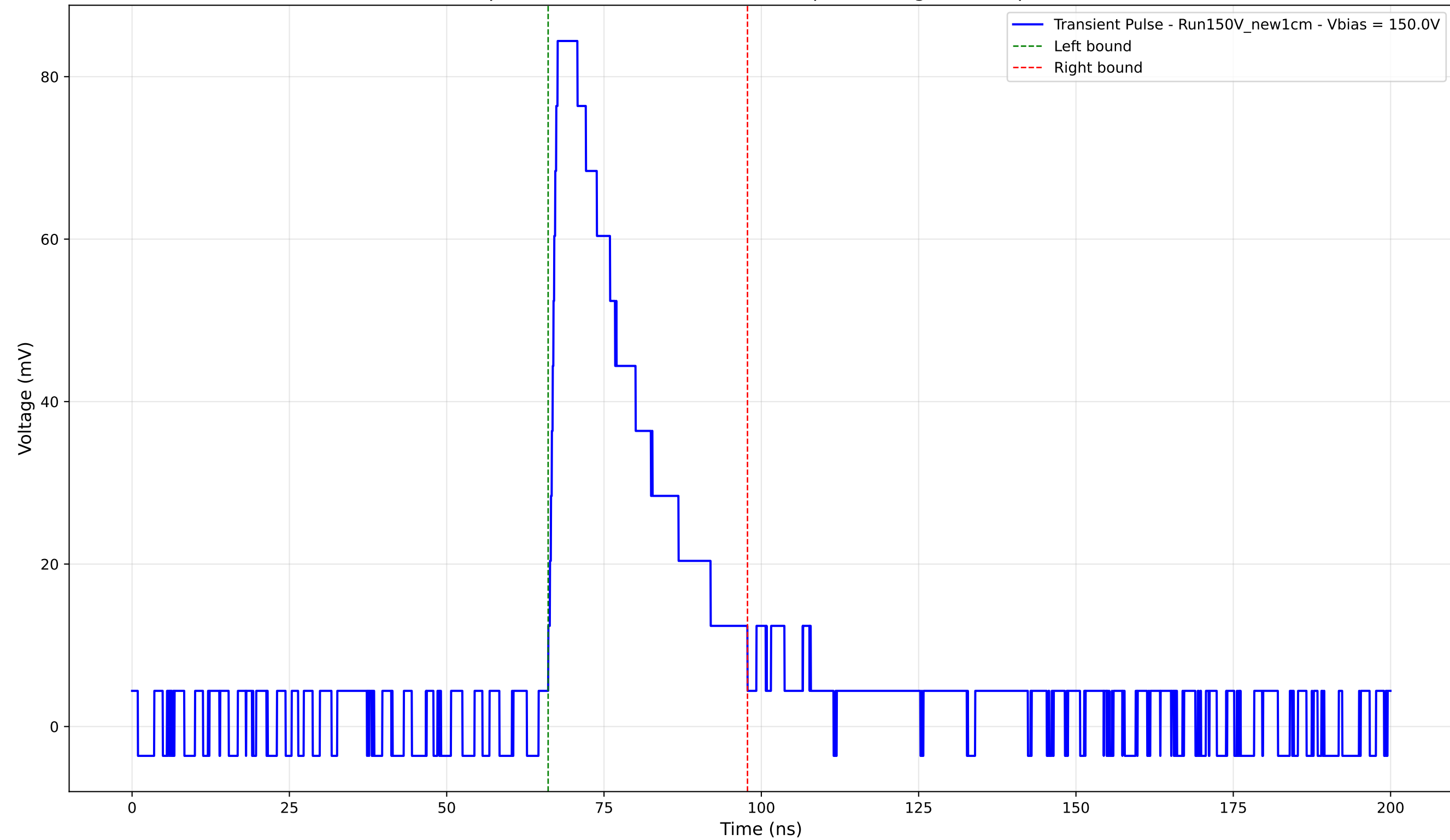
Transient Pulse - Sample: New1cm - Position: 1460.0 \mu\text{m} - Charge: 25.15 pC - Rise Time: 1.27 ns
