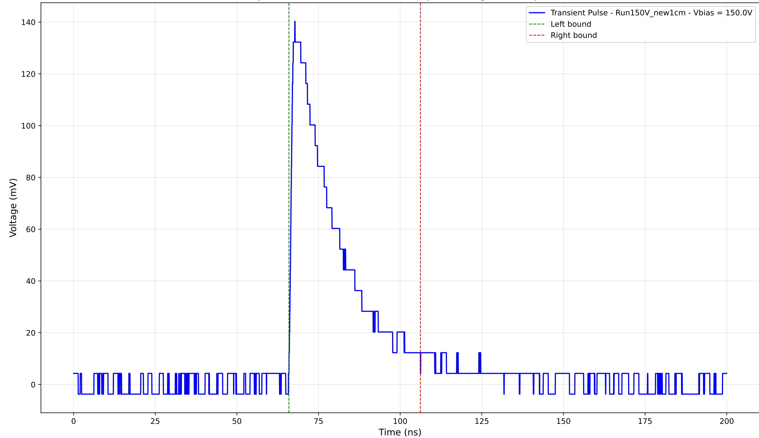
Transient Pulse - Sample: New1cm - Position: 3340.0 \mu\text{m} - Charge: 41.69 pC - Rise Time: 1.20 ns
