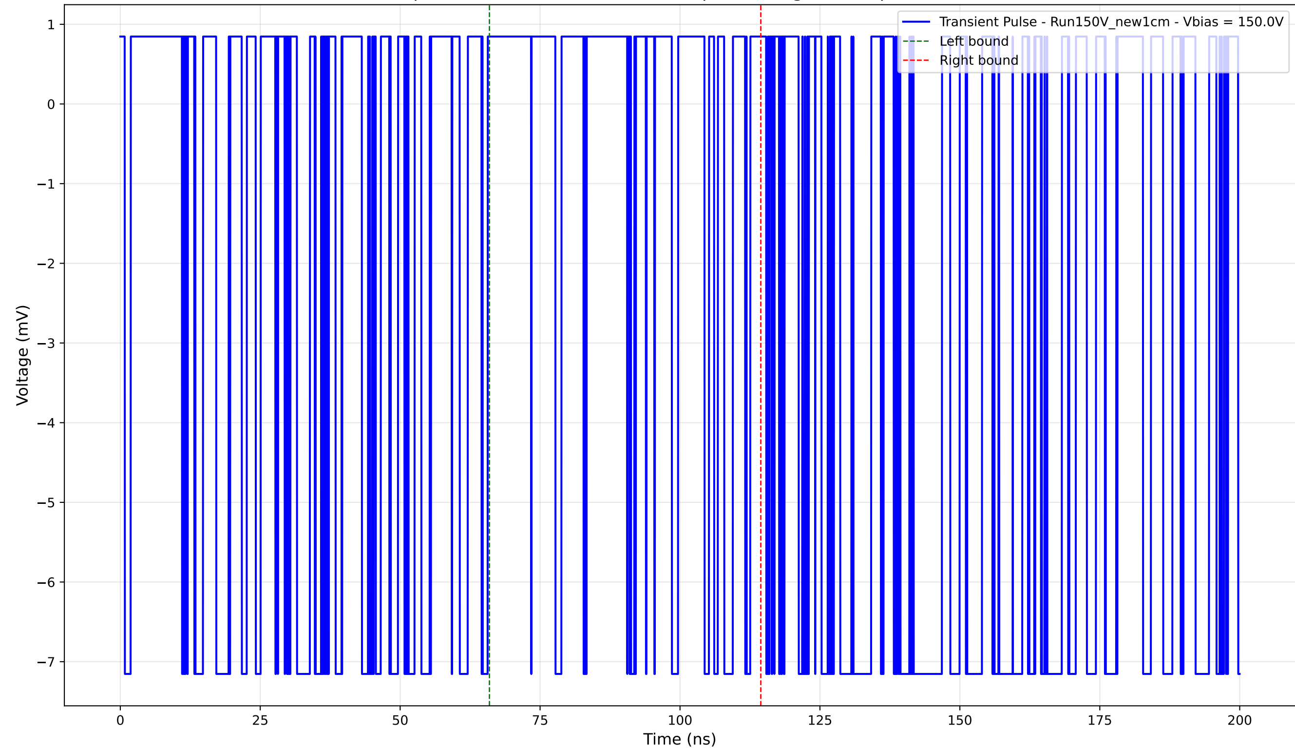
Transient Pulse - Sample: New1cm - Position: 4940.0 \mu\text{m} - Charge: -0.39 pC - Rise Time: 0.00 ns (N/A)
