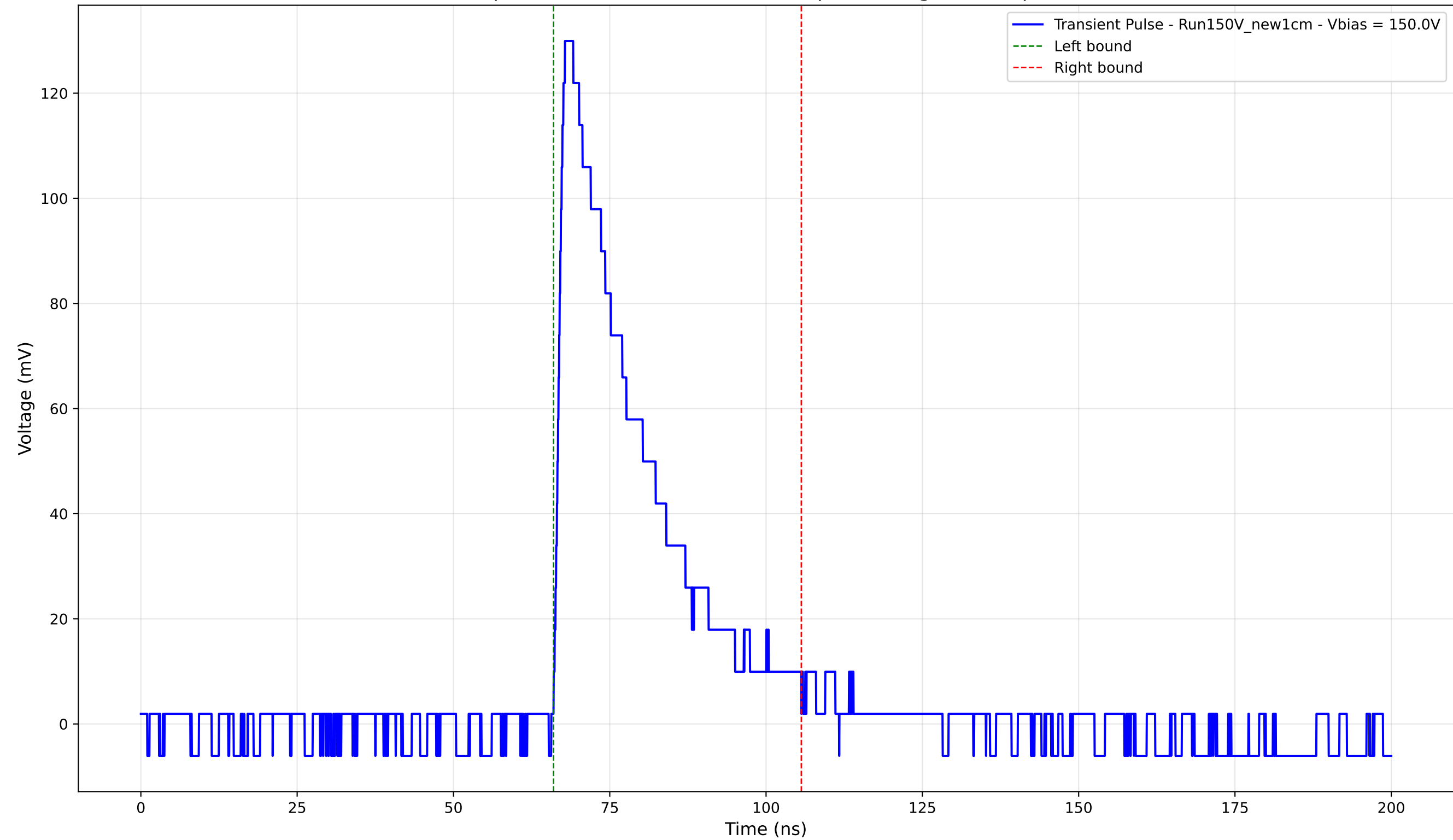
Transient Pulse - Sample: New1cm - Position: 3970.0 \mu\text{m} - Charge: 36.08 pC - Rise Time: 1.41 ns
