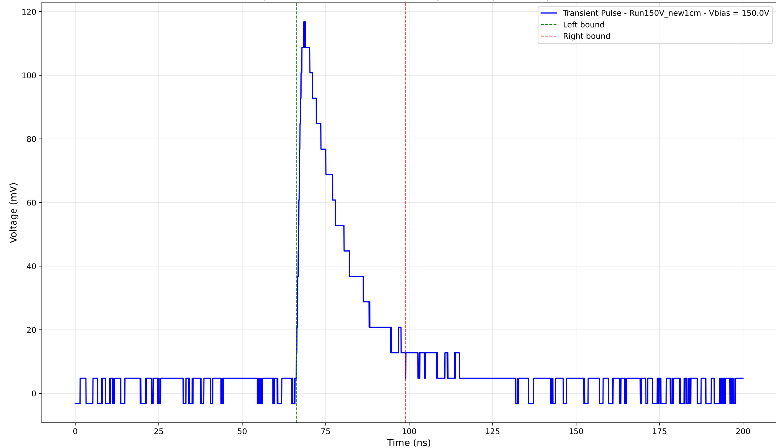
Transient Pulse - Sample: New1cm - Position: 1175.0 \mu\text{m} - Charge: 31.60 pC - Rise Time: 1.68 ns
