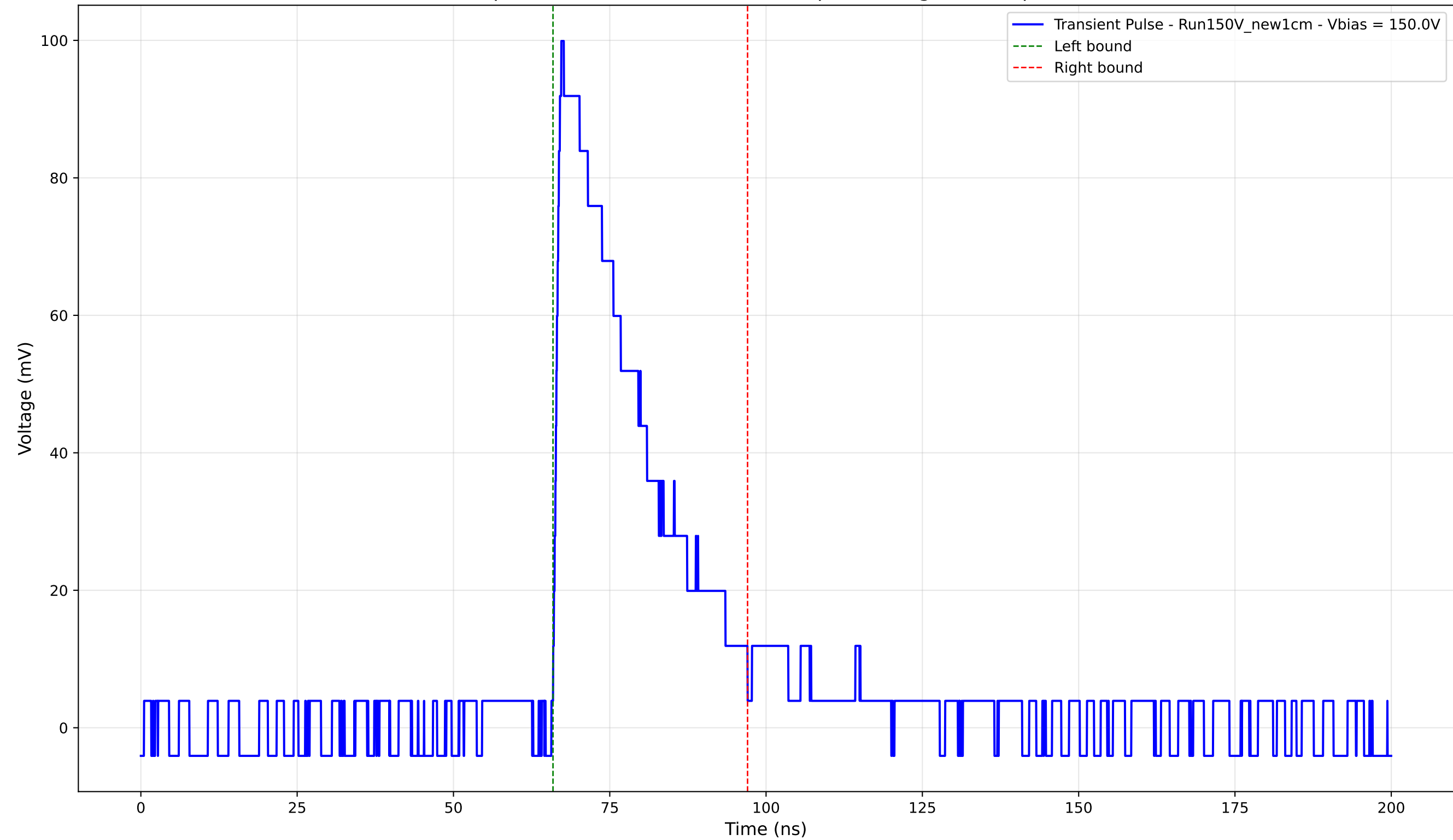
Transient Pulse - Sample: New1cm - Position: 1895.0 \mu\text{m} - Charge: 27.89 pC - Rise Time: 1.08 ns
