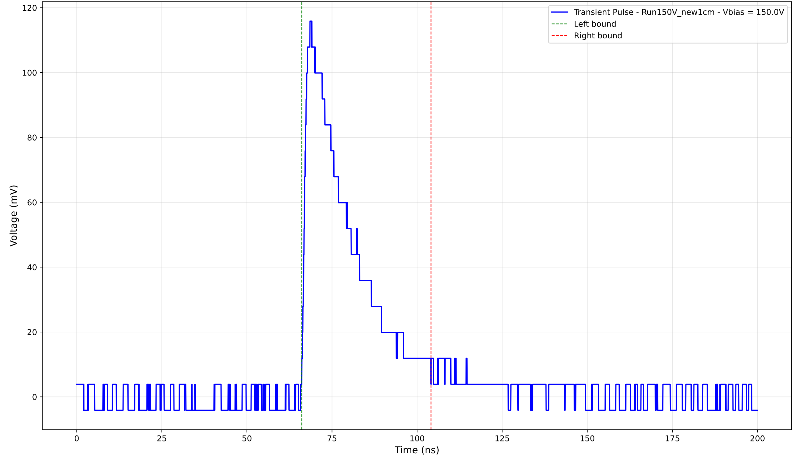
Transient Pulse - Sample: New1cm - Position: 1390.0 \mu\text{m} - Charge: 33.65 pC - Rise Time: 1.66 ns
