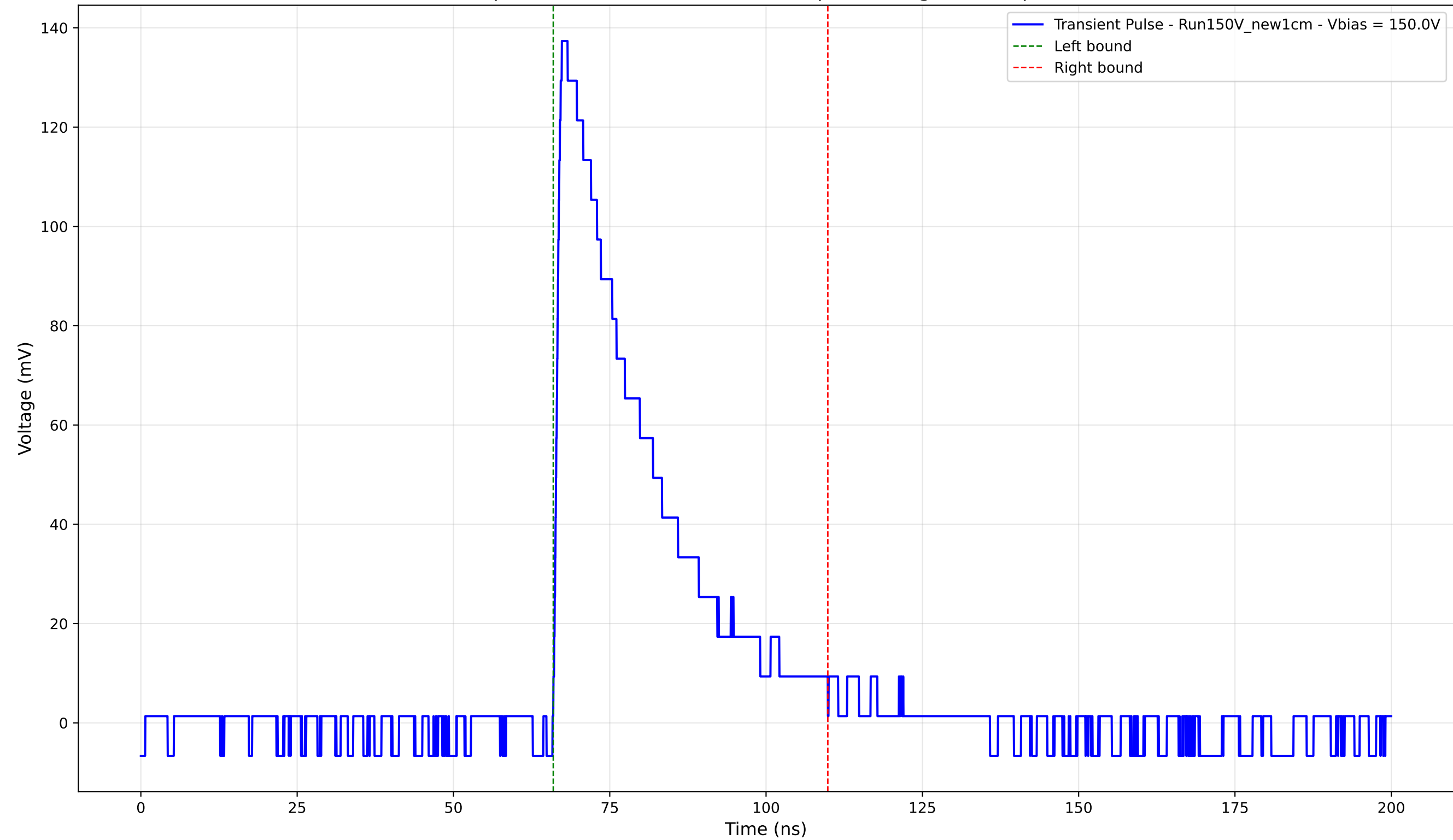
Transient Pulse - Sample: New1cm - Position: 3290.0 \mu\text{m} - Charge: 40.75 pC - Rise Time: 1.05 ns
