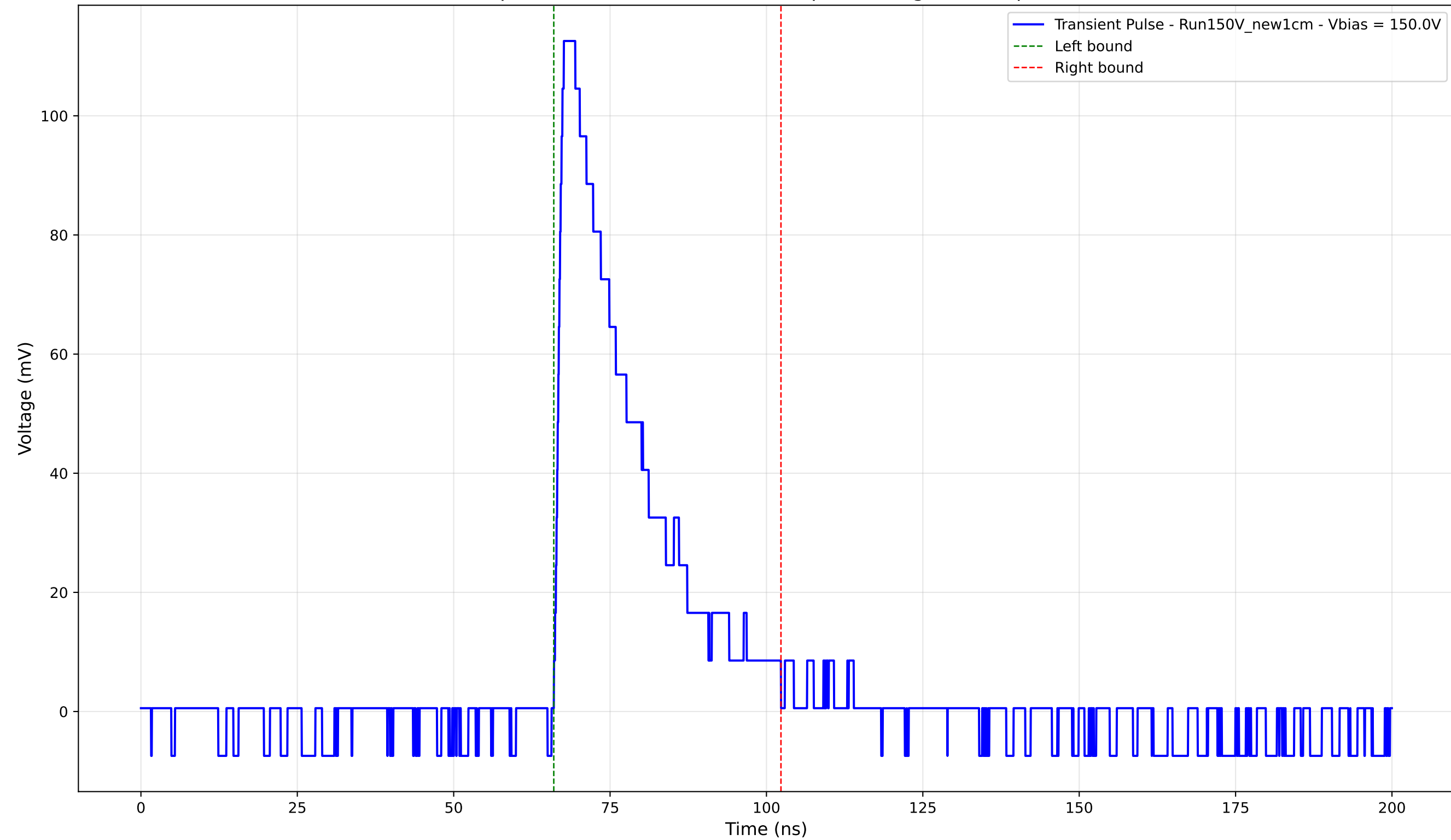
Transient Pulse - Sample: New1cm - Position: 710.0 \mu\text{m} - Charge: 29.19 pC - Rise Time: 1.19 ns
