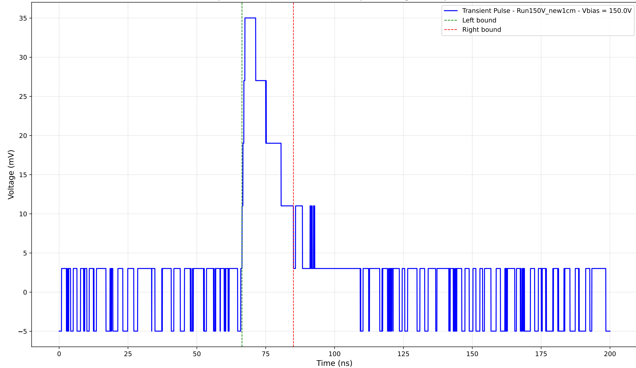
Transient Pulse - Sample: New1cm - Position: 1505.0 \mu\text{m} - Charge: 8.25 pC - Rise Time: 1.06 ns
