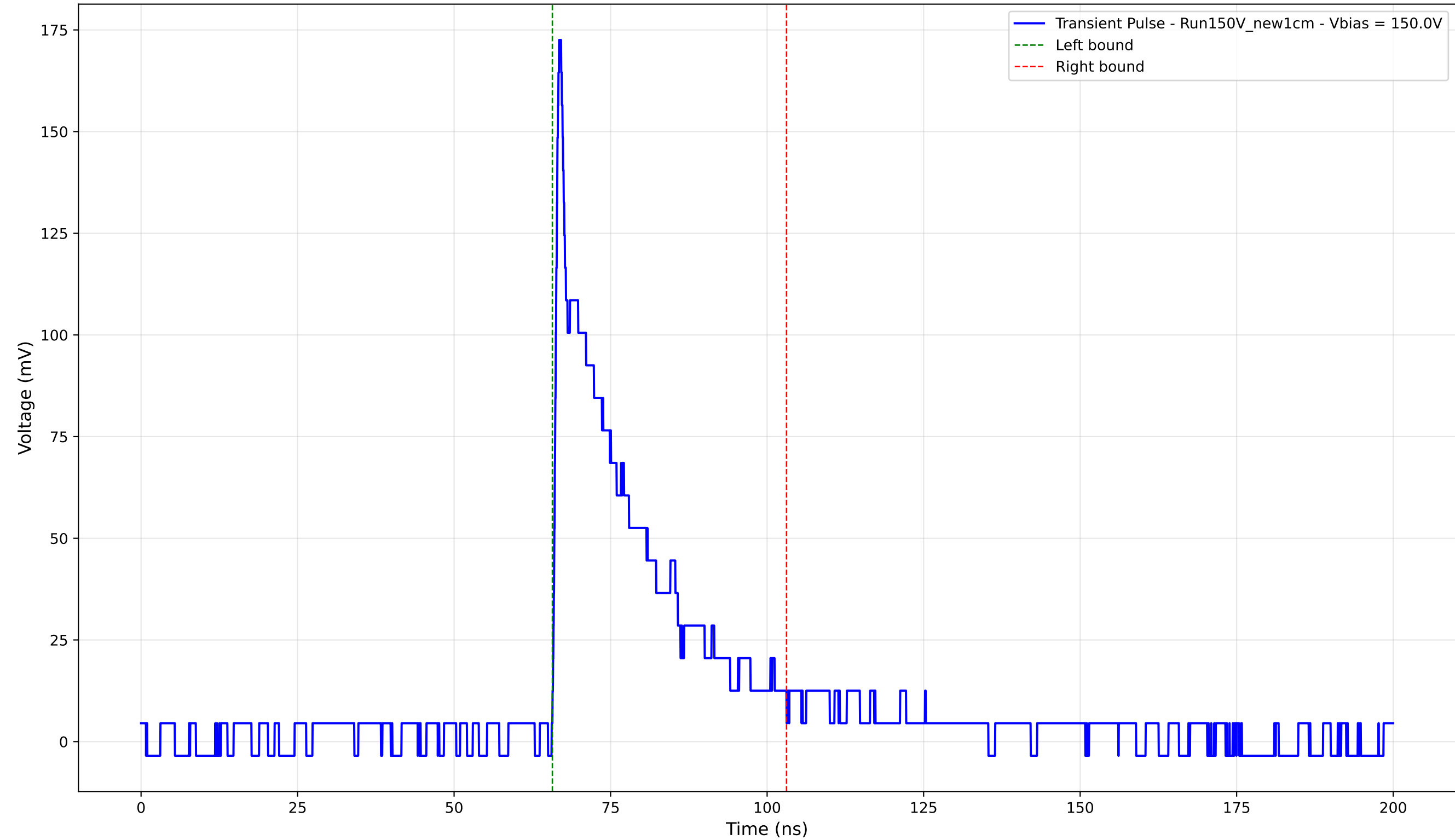
Transient Pulse - Sample: New1cm - Position: 2290.0 \mu\text{m} - Charge: 36.04 pC - Rise Time: 0.79 ns
