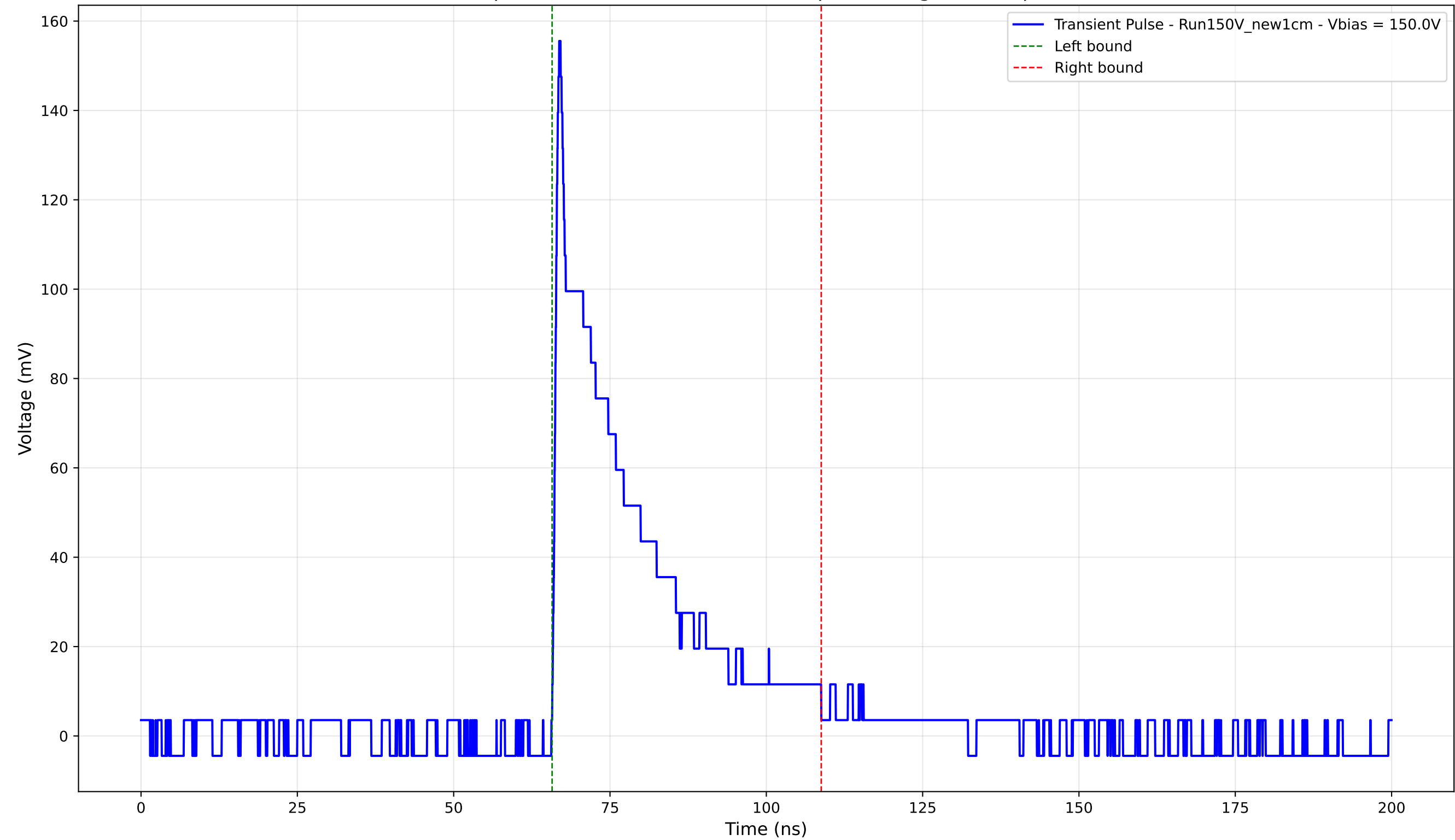
Transient Pulse - Sample: New1cm - Position: 2225.0 \mu\text{m} - Charge: 34.61 pC - Rise Time: 0.91 ns
