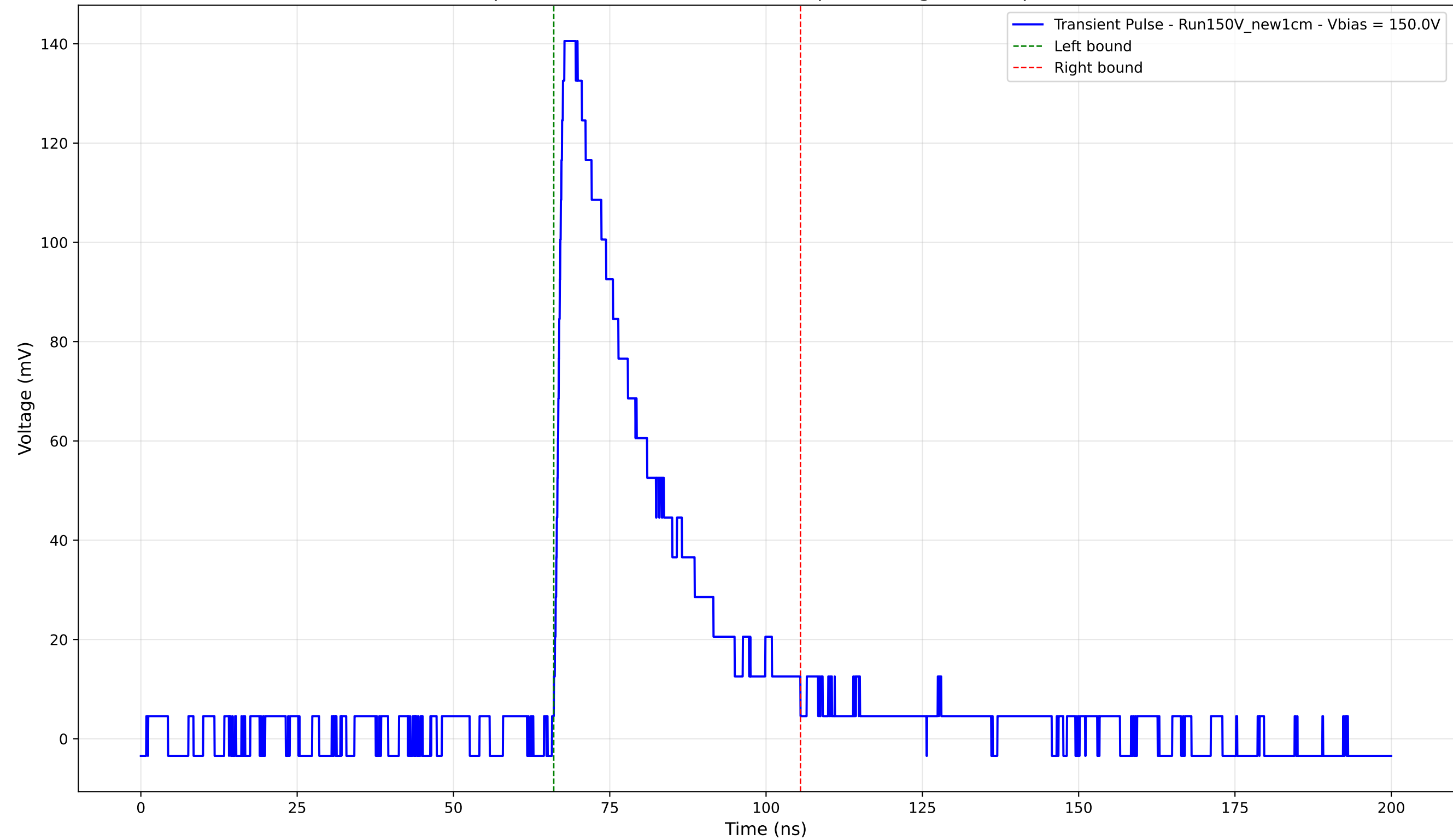
Transient Pulse - Sample: New1cm - Position: 3750.0 \mu\text{m} - Charge: 41.52 pC - Rise Time: 1.30 ns
