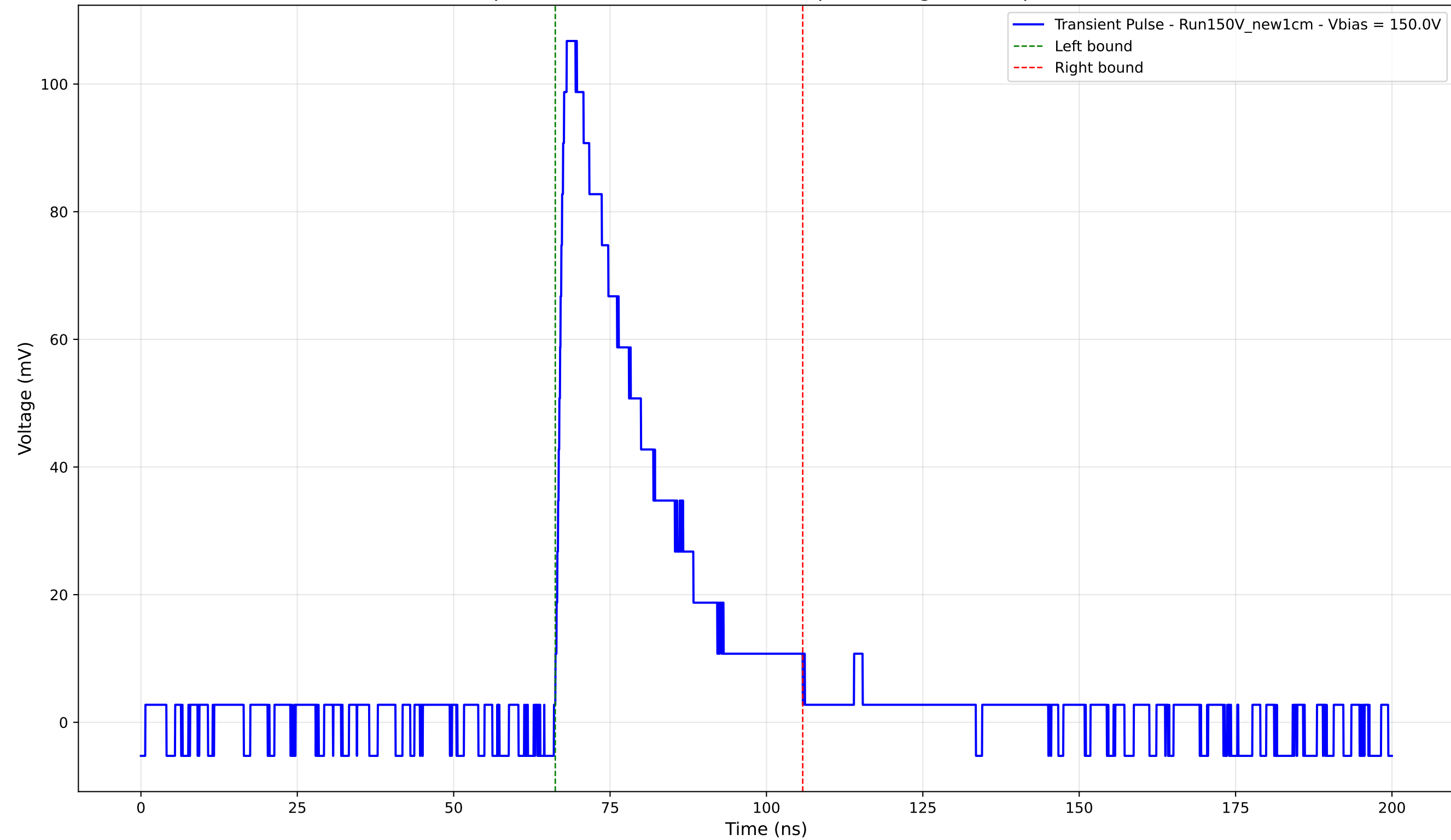
Transient Pulse - Sample: New1cm - Position: 1165.0 \mu\text{m} - Charge: 30.63 pC - Rise Time: 1.38 ns
