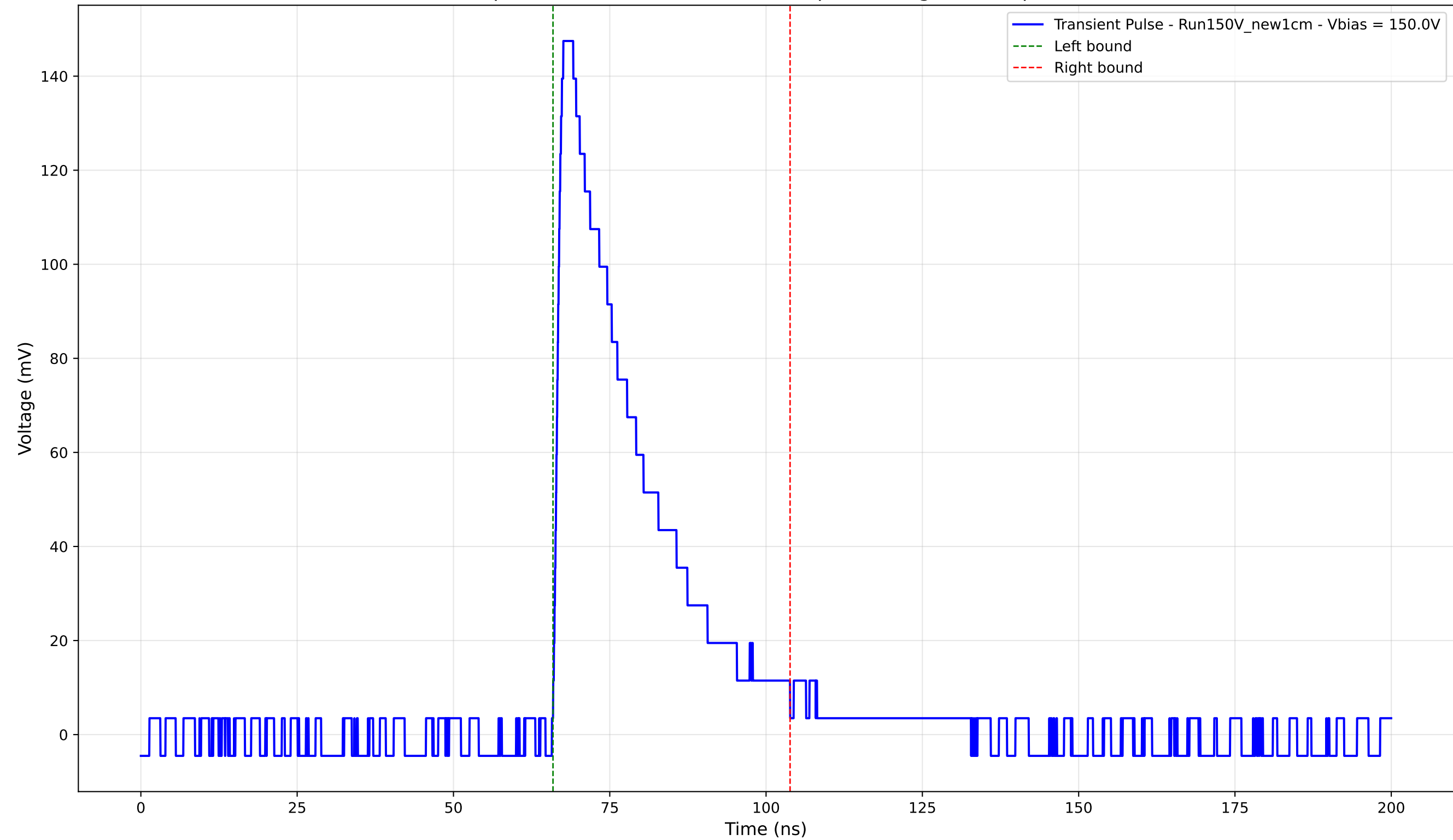
Transient Pulse - Sample: New1cm - Position: 4260.0 \mu\text{m} - Charge: 40.20 pC - Rise Time: 1.29 ns
