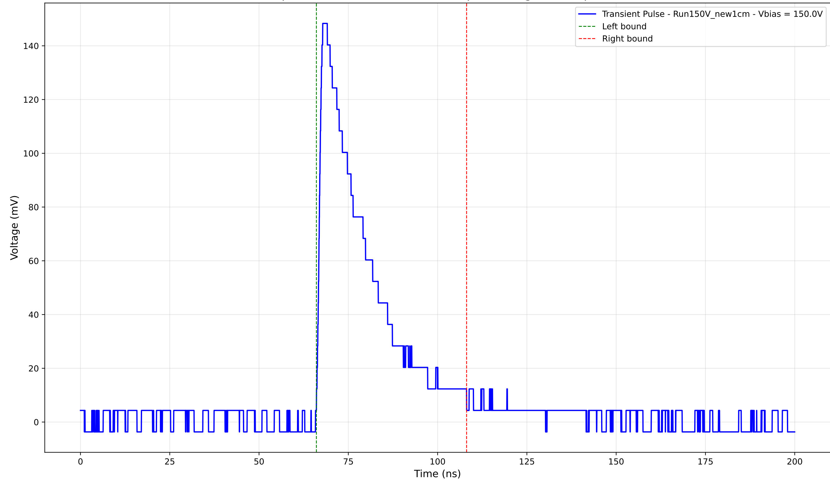
Transient Pulse - Sample: New1cm - Position: 3885.0 \mu\text{m} - Charge: 42.74 pC - Rise Time: 1.39 ns
