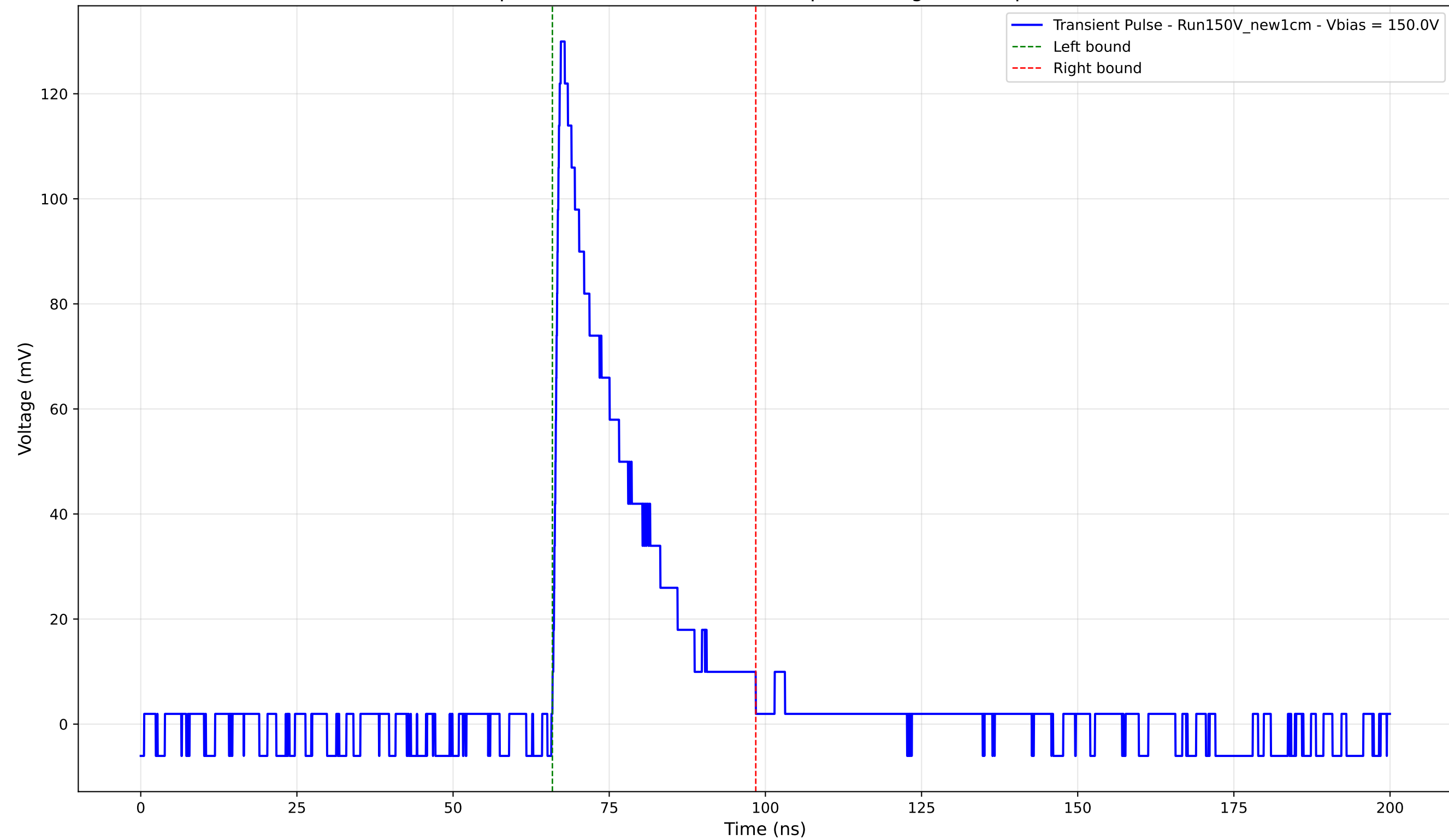
Transient Pulse - Sample: New1cm - Position: 365.0 \mu\text{m} - Charge: 27.60 pC - Rise Time: 1.01 ns
