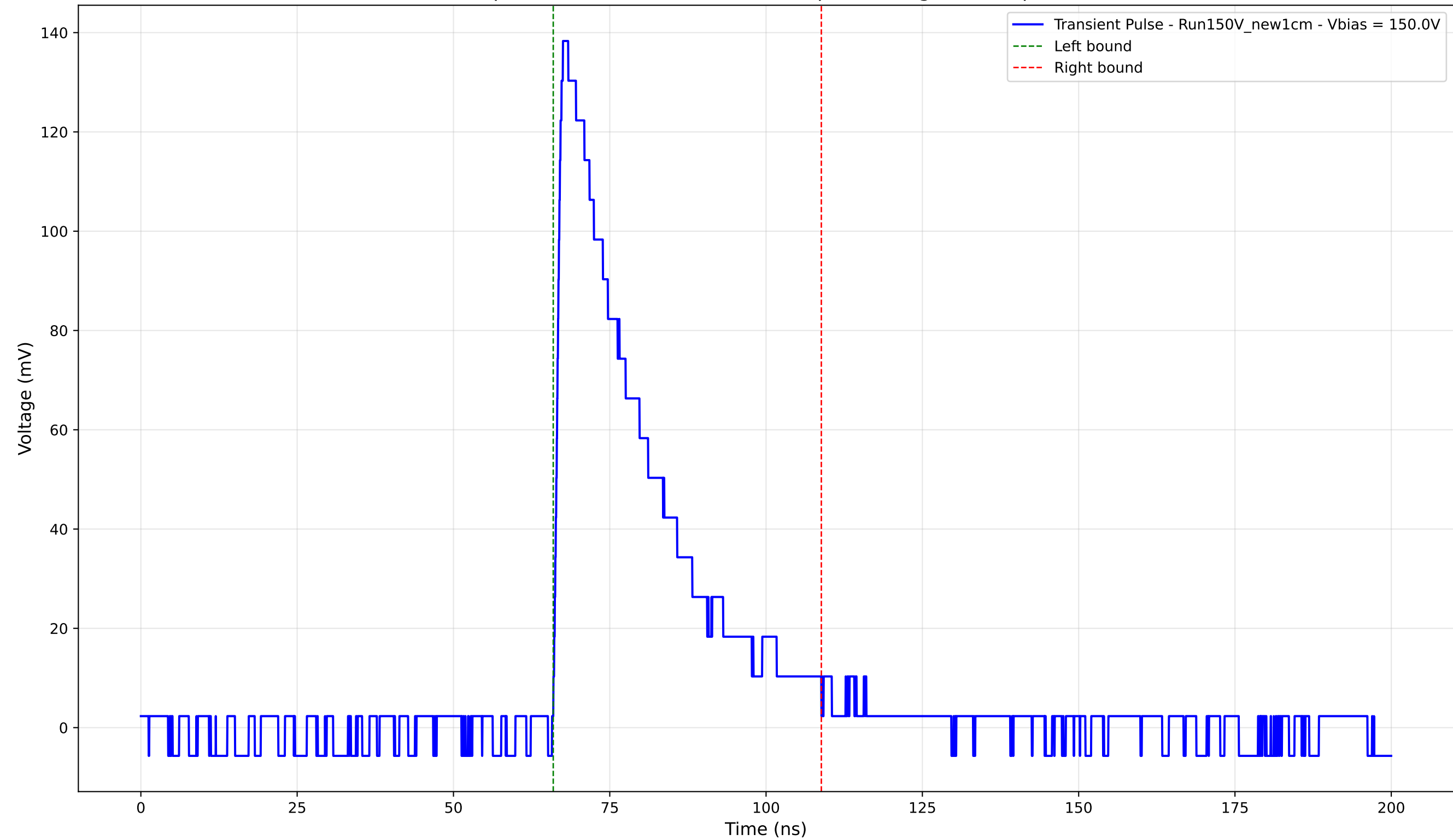
Transient Pulse - Sample: New1cm - Position: 3380.0 \mu\text{m} - Charge: 40.76 pC - Rise Time: 1.19 ns
