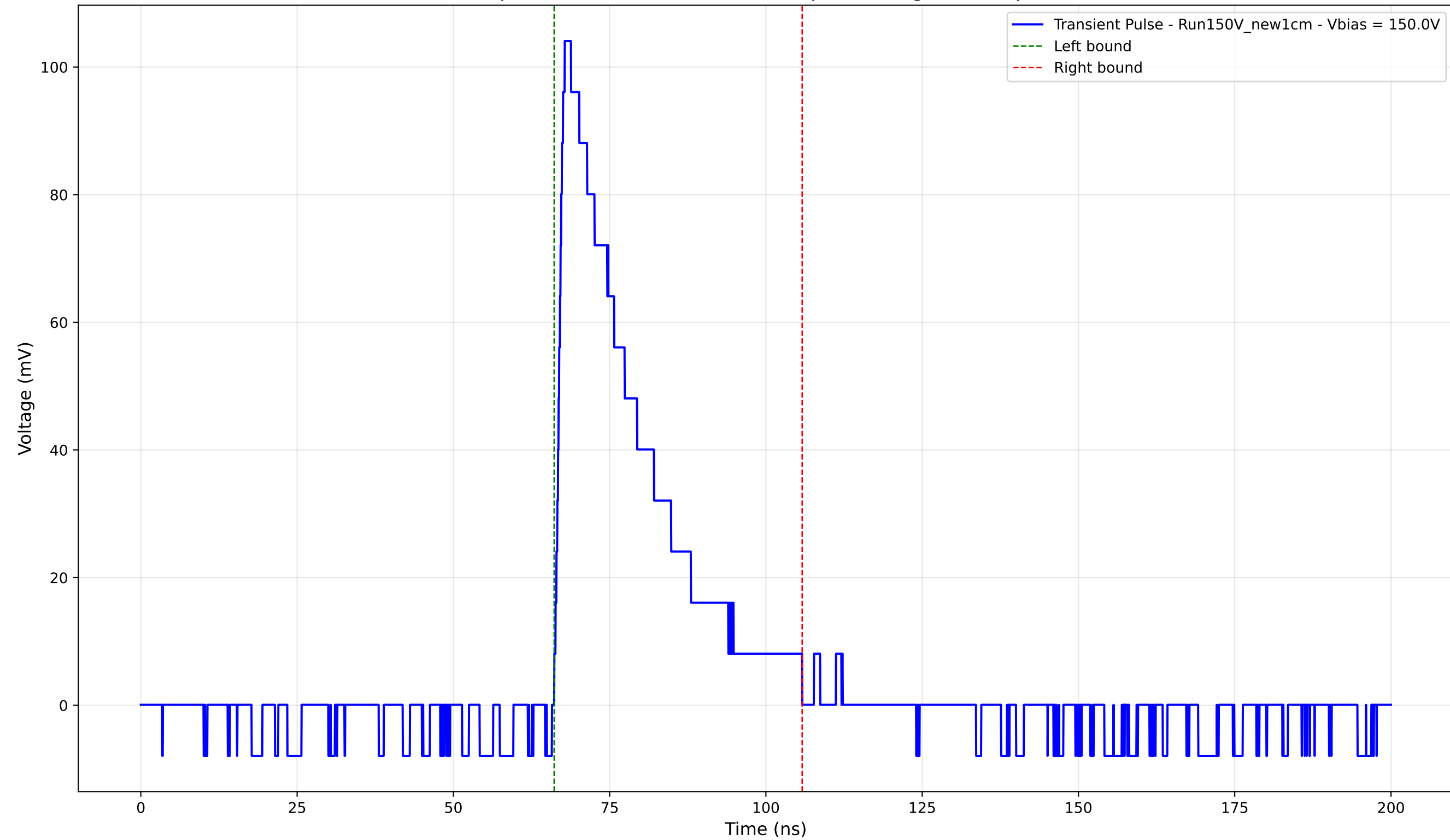
Transient Pulse - Sample: New1cm - Position: 935.0 \mu\text{m} - Charge: 28.06 pC - Rise Time: 1.21 ns
