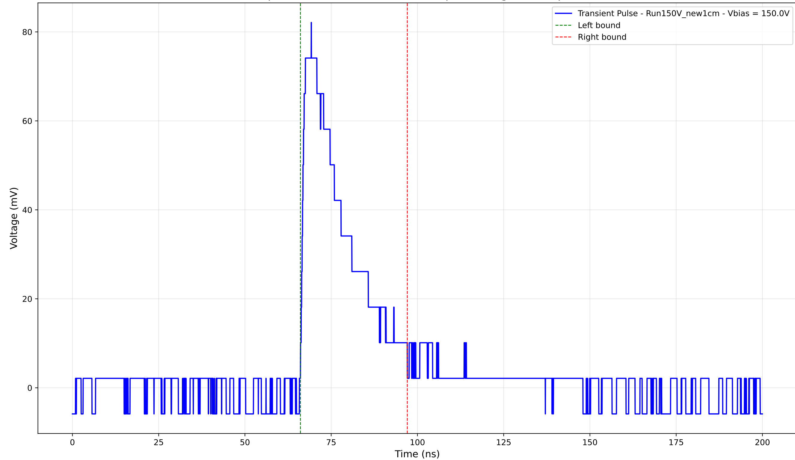
Transient Pulse - Sample: New1cm - Position: 1615.0 \mu\text{m} - Charge: 21.49 pC - Rise Time: 1.42 ns
