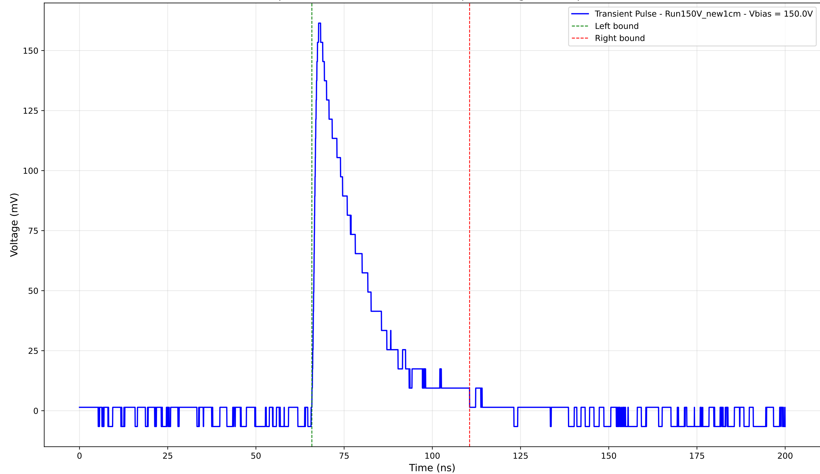
Transient Pulse - Sample: New1cm - Position: 4310.0 \mu\text{m} - Charge: 41.95 pC - Rise Time: 1.28 ns
