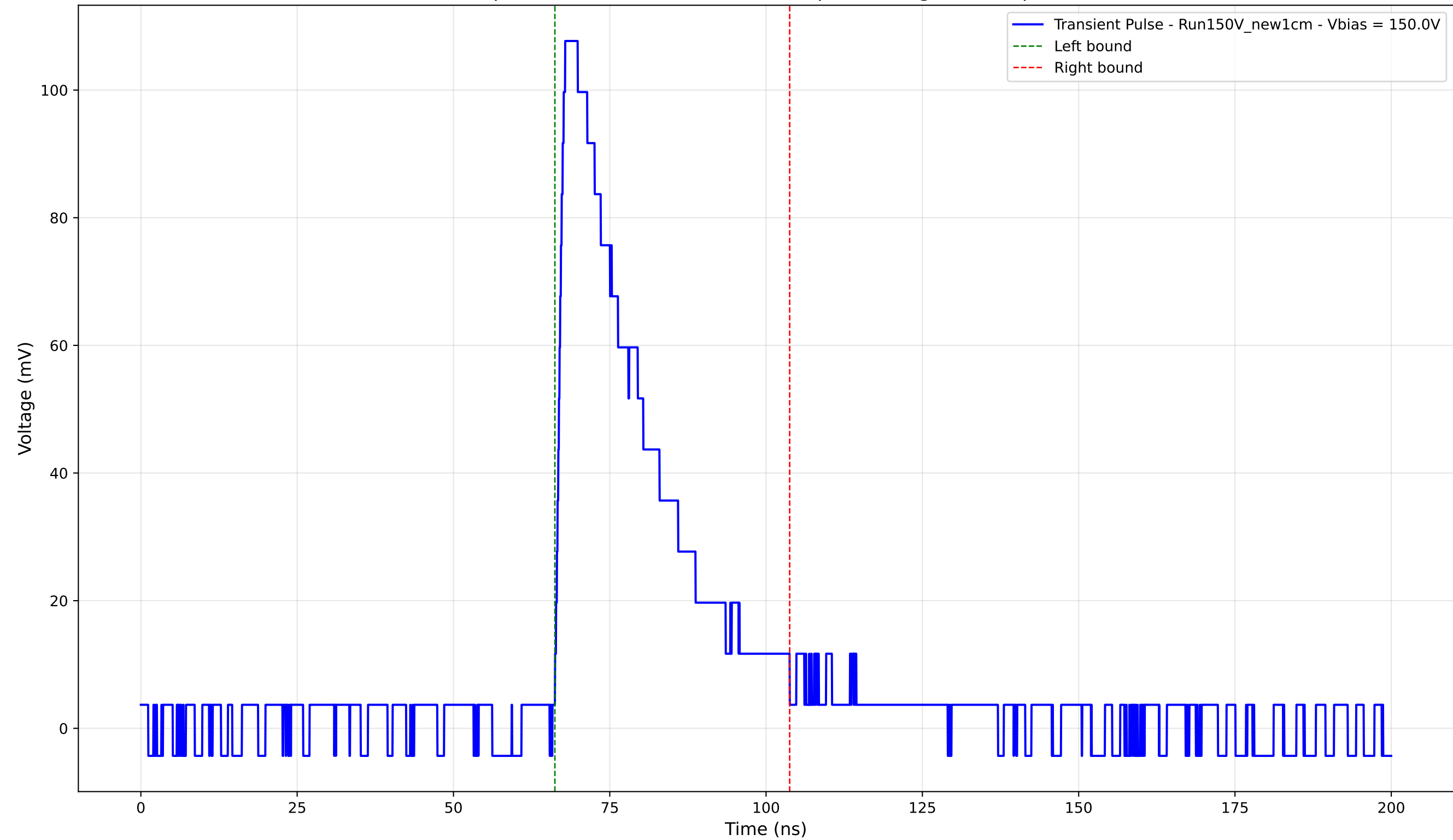
Transient Pulse - Sample: New1cm - Position: 1285.0 \mu\text{m} - Charge: 32.20 pC - Rise Time: 1.38 ns
