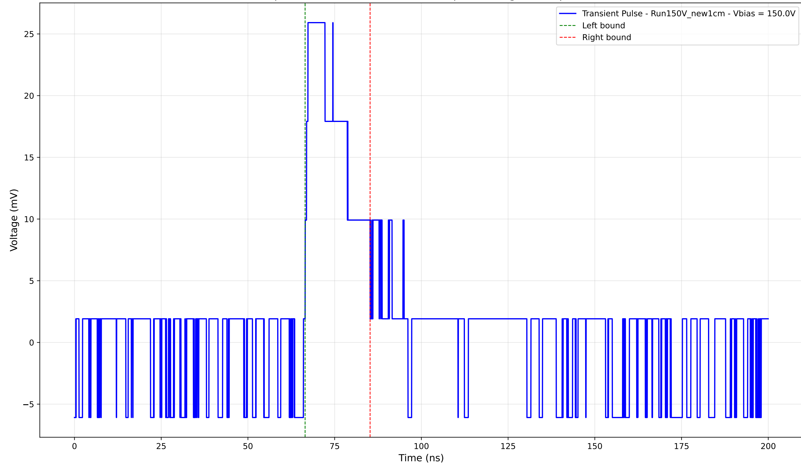
Transient Pulse - Sample: New1cm - Position: 1065.0 \mu\text{m} - Charge: 6.39 pC - Rise Time: 0.82 ns
