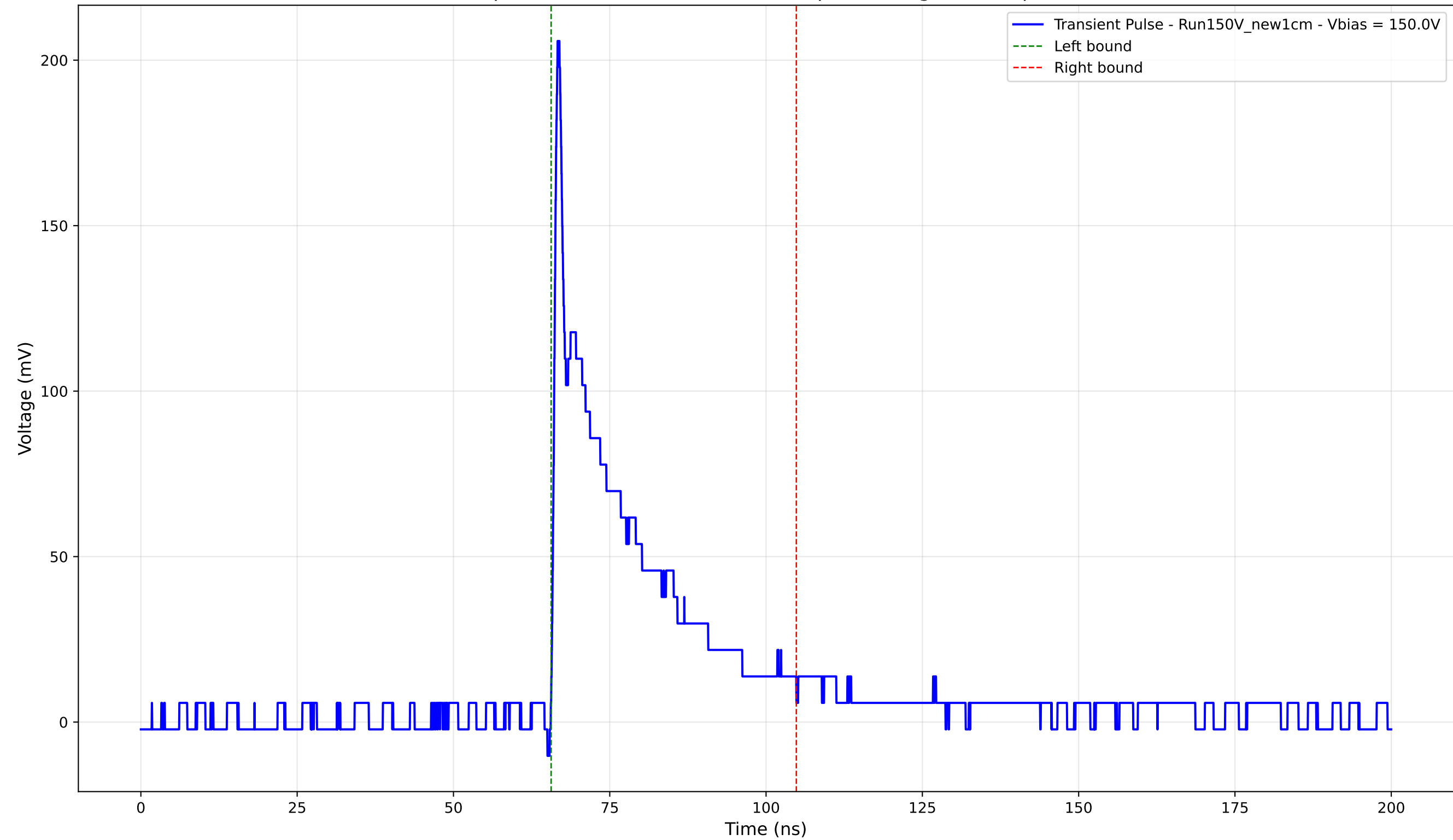
Transient Pulse - Sample: New1cm - Position: 2695.0 \mu\text{m} - Charge: 38.92 pC - Rise Time: 0.82 ns
