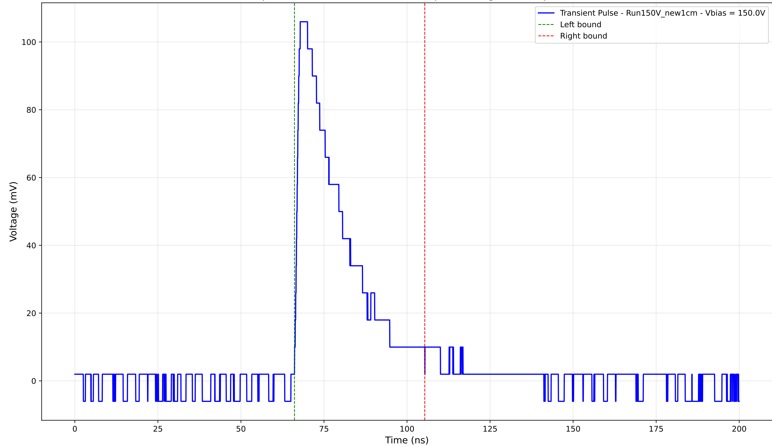
Transient Pulse - Sample: New1cm - Position: 1365.0 \mu\text{m} - Charge: 31.73 pC - Rise Time: 1.22 ns
