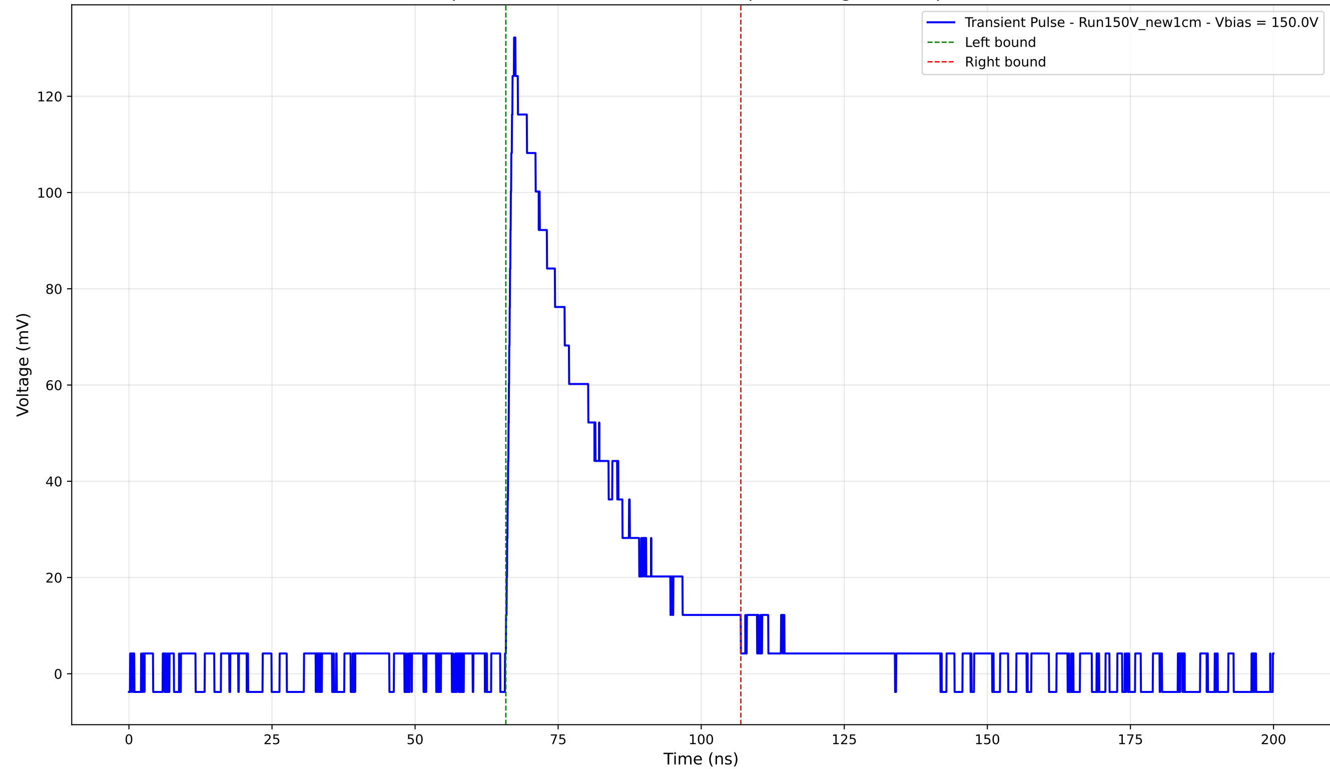
Transient Pulse - Sample: New1cm - Position: 3155.0 \mu\text{m} - Charge: 37.15 pC - Rise Time: 1.04 ns
