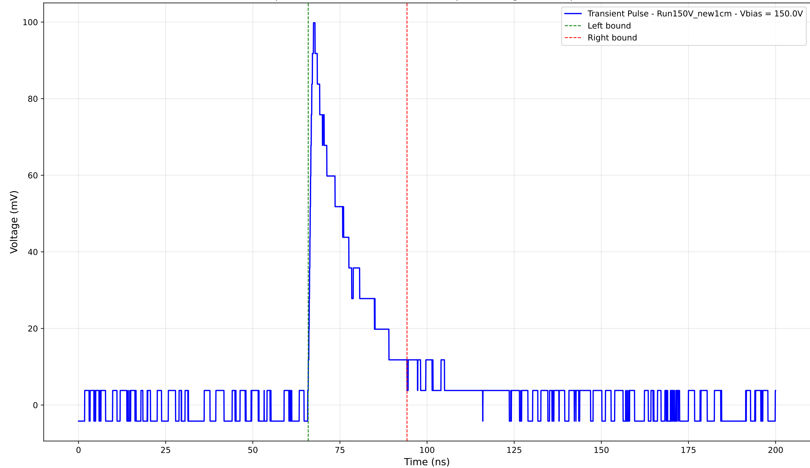
Transient Pulse - Sample: New1cm - Position: 4510.0 \mu\text{m} - Charge: 21.97 pC - Rise Time: 1.18 ns
