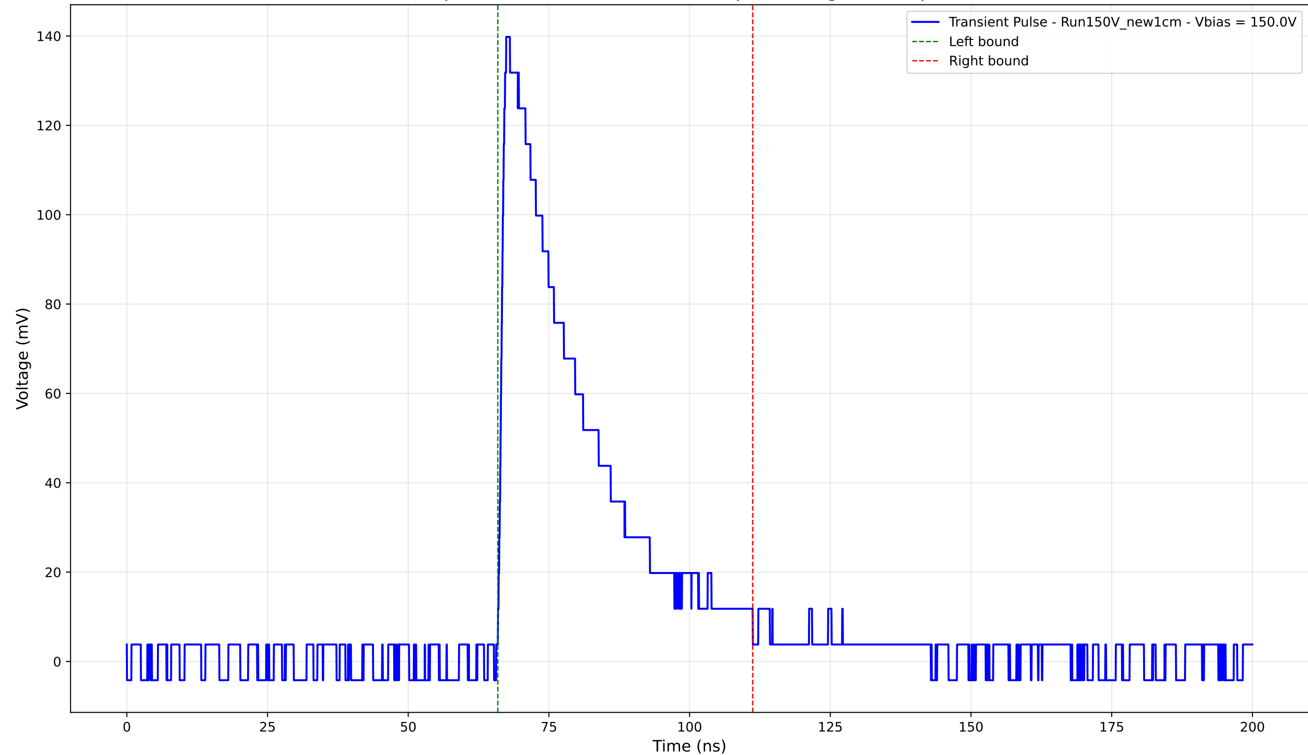
Transient Pulse - Sample: New1cm - Position: 3320.0 \mu\text{m} - Charge: 43.09 pC - Rise Time: 1.15 ns
