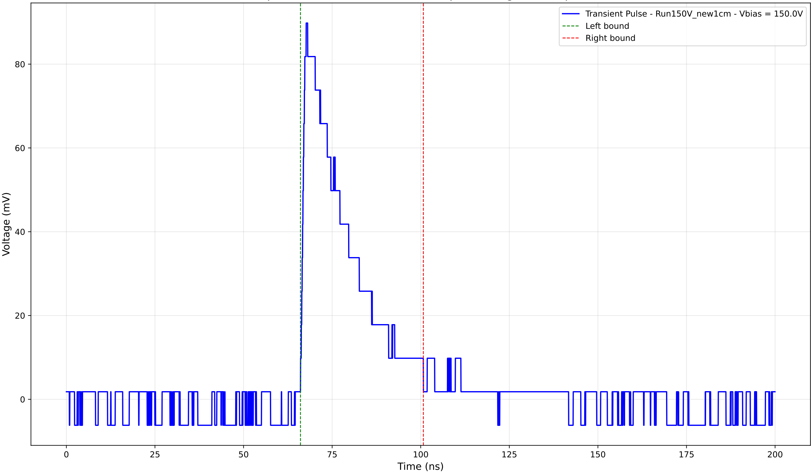
Transient Pulse - Sample: New1cm - Position: 3500.0 \mu\text{m} - Charge: 23.96 pC - Rise Time: 1.20 ns
