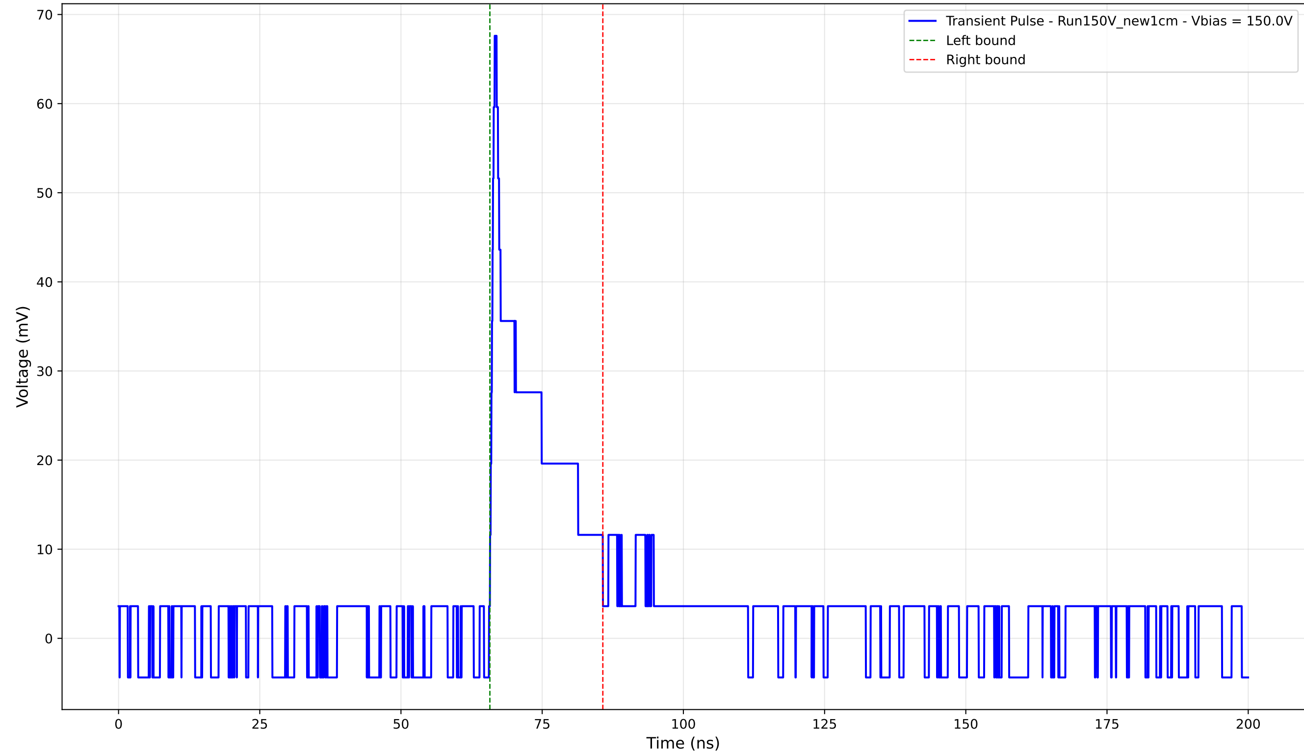
Transient Pulse - Sample: New1cm - Position: 2585.0 \mu\text{m} - Charge: 9.80 pC - Rise Time: 0.83 ns
