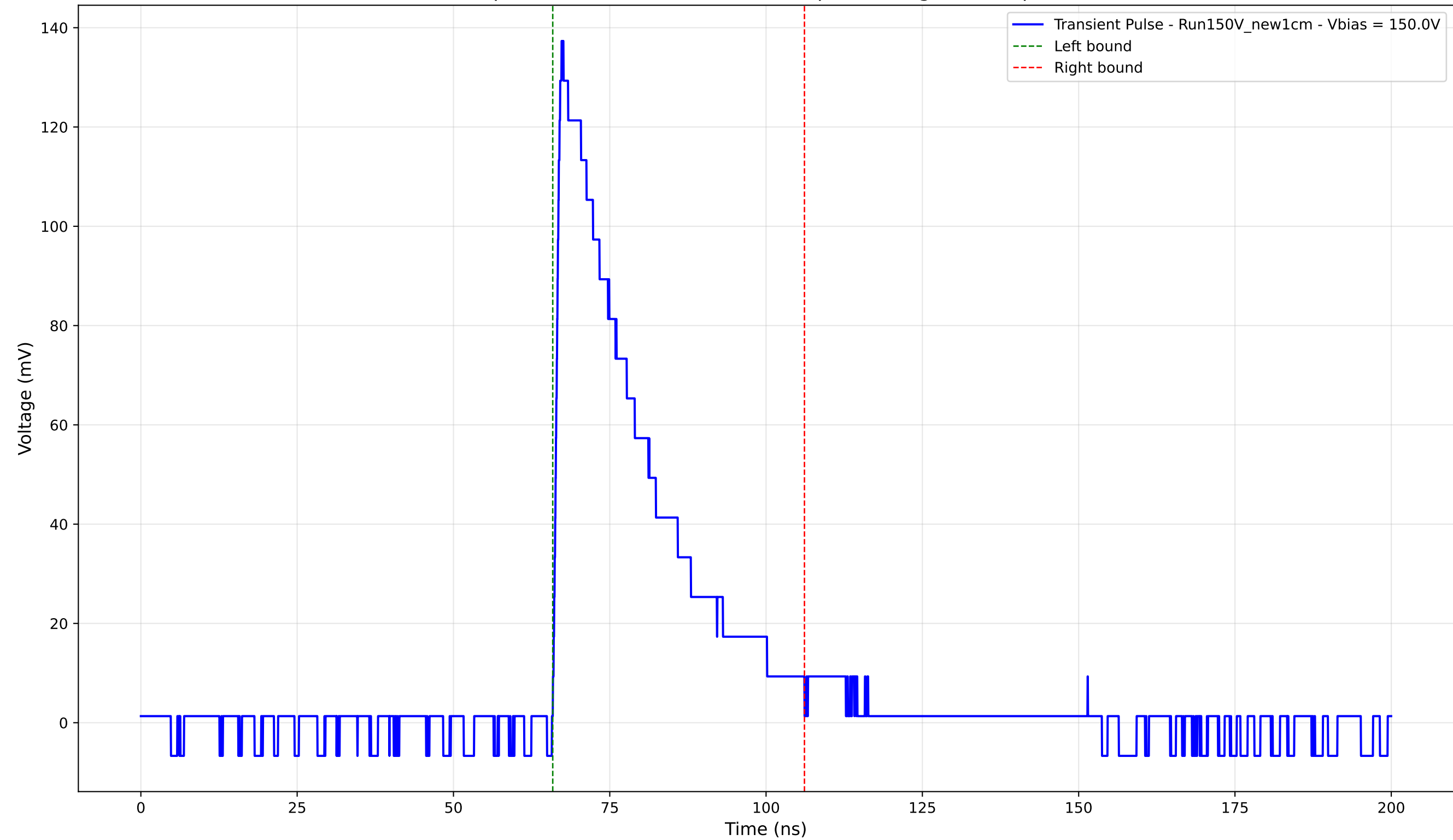
Transient Pulse - Sample: New1cm - Position: 3230.0 \mu\text{m} - Charge: 38.94 pC - Rise Time: 1.05 ns
