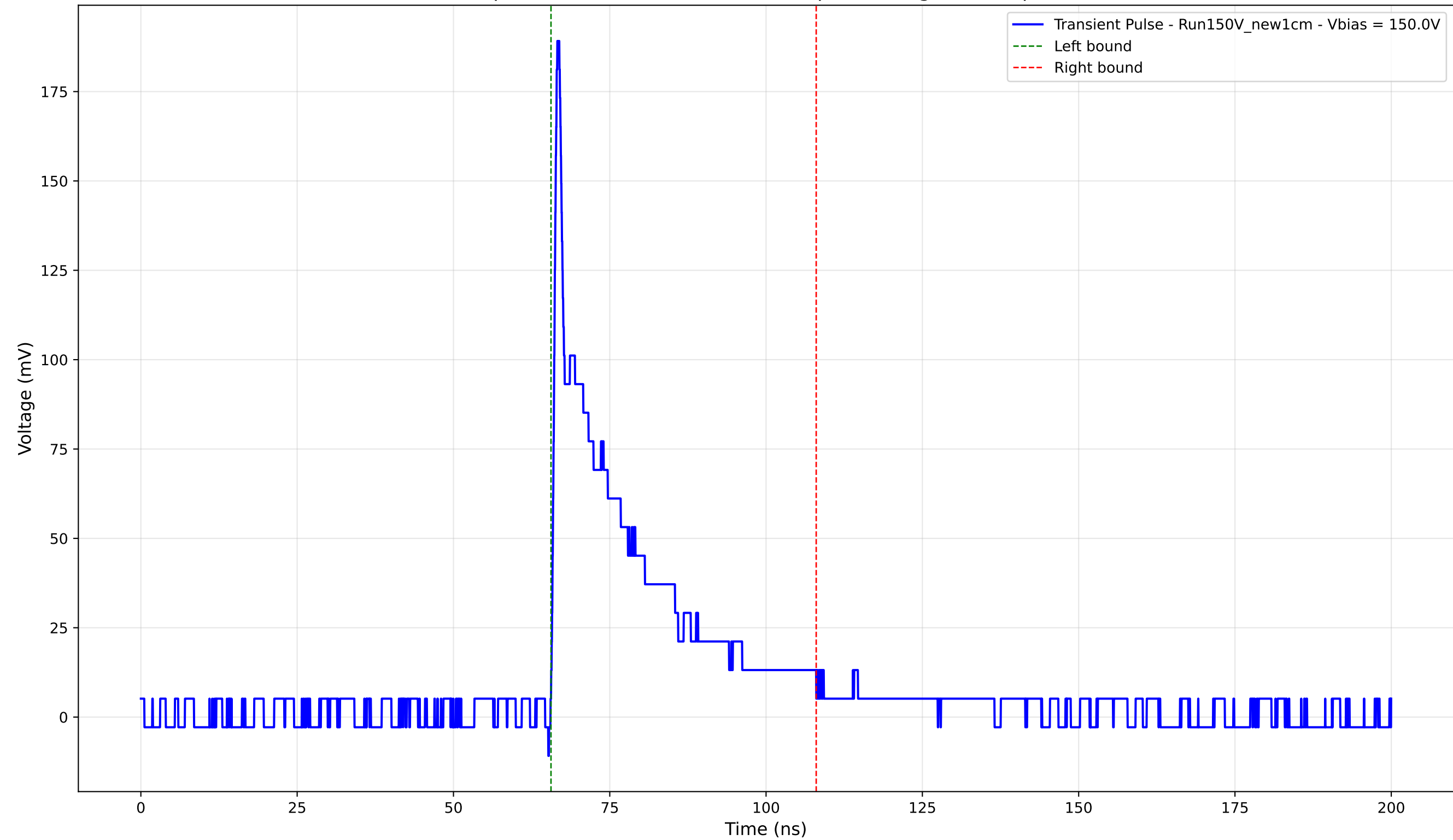
Transient Pulse - Sample: New1cm - Position: 2450.0 \mu\text{m} - Charge: 34.79 pC - Rise Time: 0.79 ns
