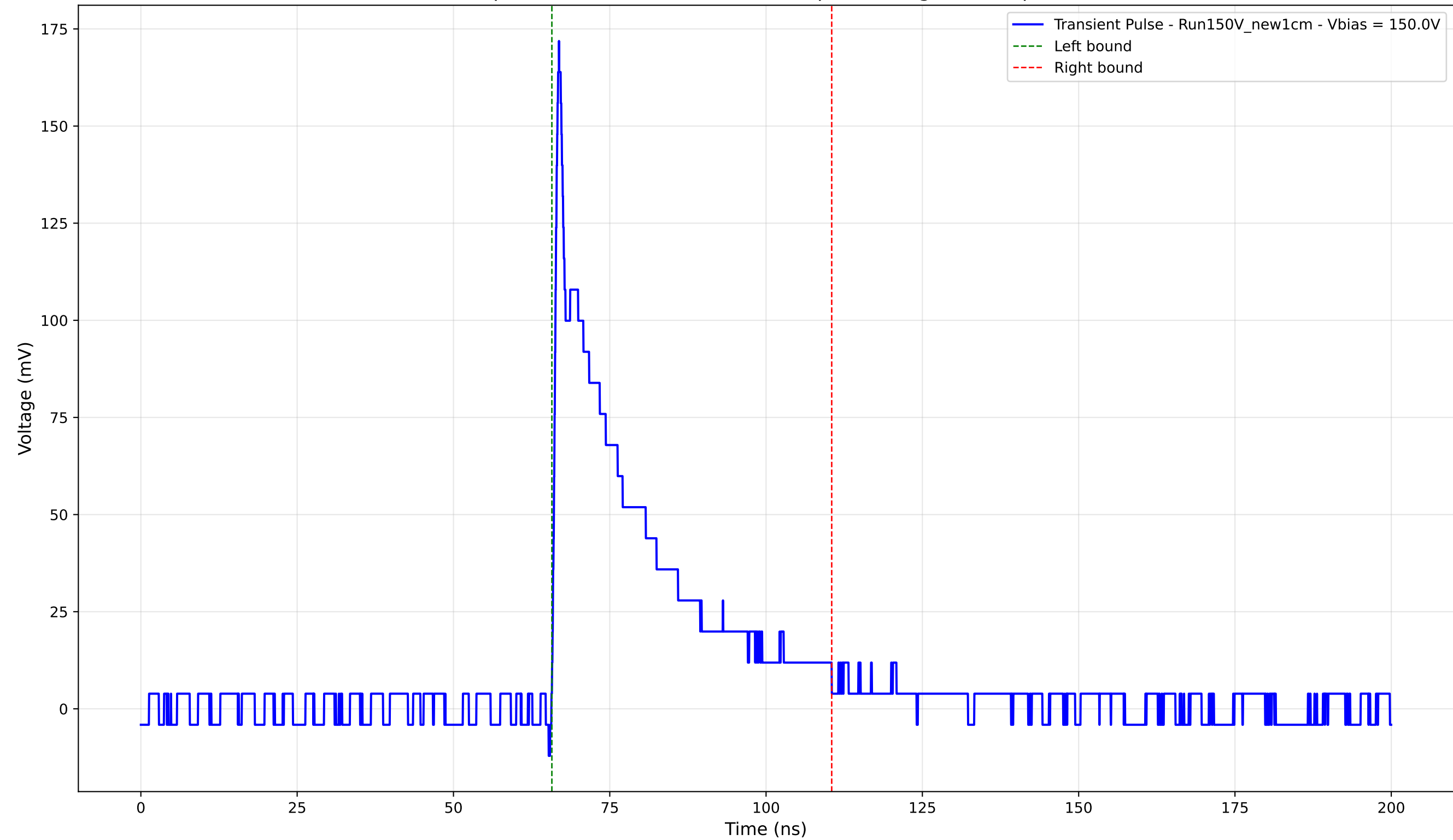
Transient Pulse - Sample: New1cm - Position: 2275.0 \mu\text{m} - Charge: 36.88 pC - Rise Time: 0.81 ns
