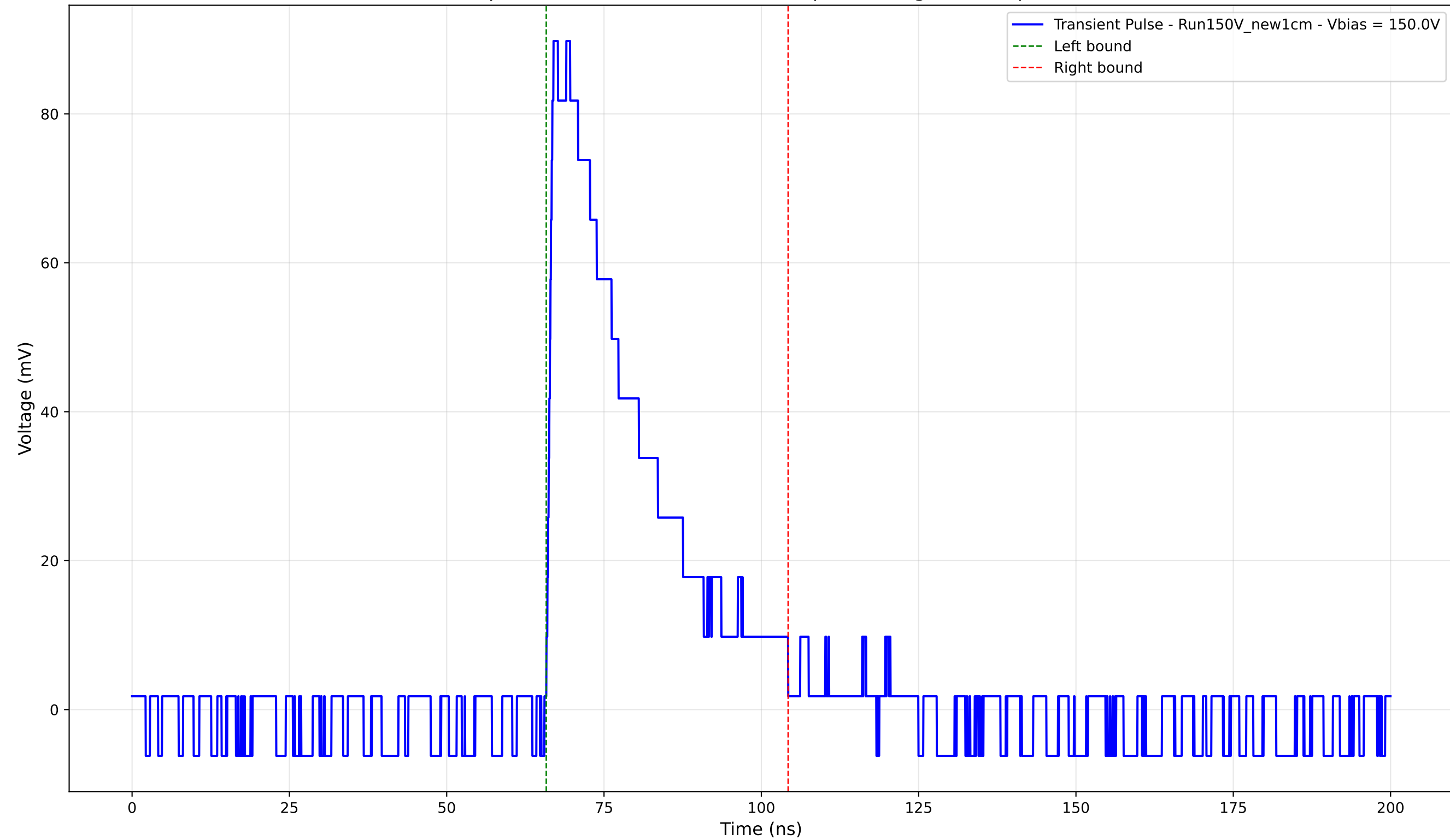
Transient Pulse - Sample: New1cm - Position: 1950.0 \mu\text{m} - Charge: 26.71 pC - Rise Time: 0.94 ns
