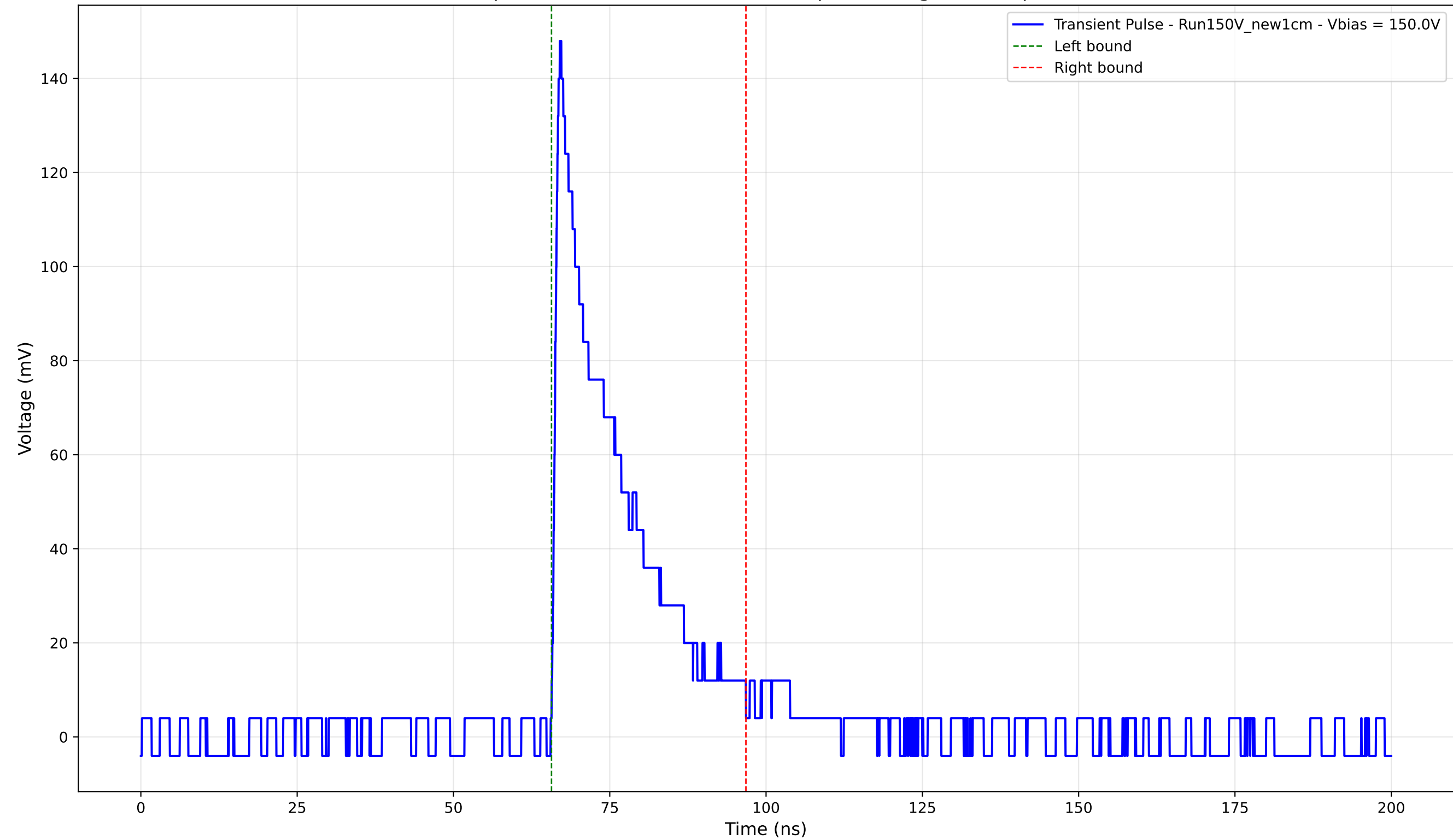
Transient Pulse - Sample: New1cm - Position: 4765.0 \mu\text{m} - Charge: 29.82 pC - Rise Time: 1.01 ns
