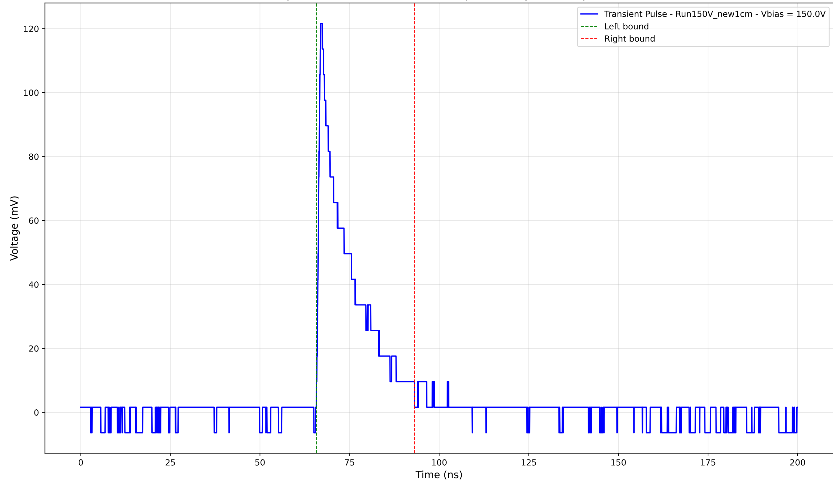
Transient Pulse - Sample: New1cm - Position: 145.0 \mu\text{m} - Charge: 21.21 pC - Rise Time: 0.93 ns
