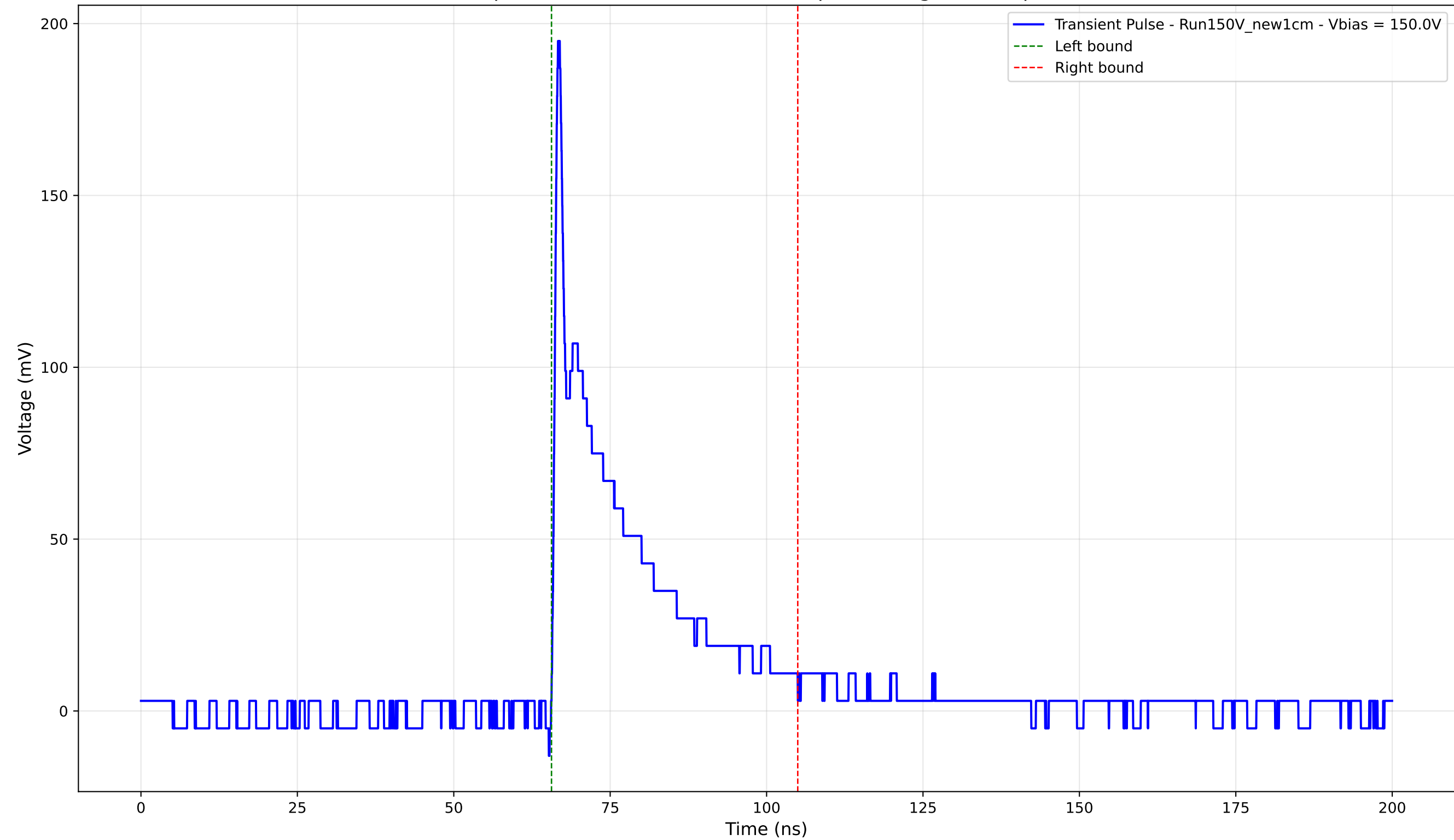
Transient Pulse - Sample: New1cm - Position: 2420.0 \mu\text{m} - Charge: 34.86 pC - Rise Time: 0.76 ns
