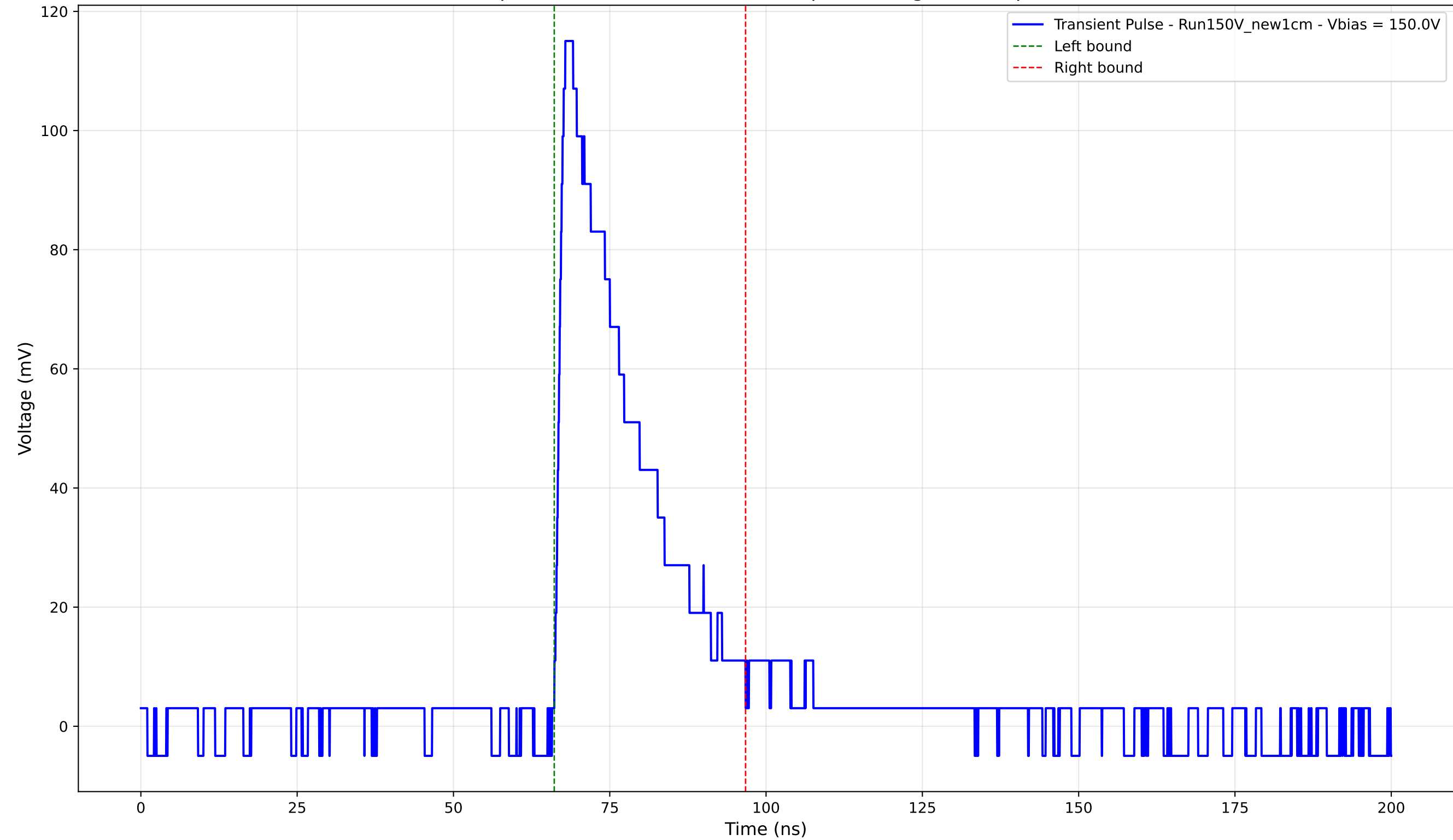
Transient Pulse - Sample: New1cm - Position: 875.0 \mu\text{m} - Charge: 29.04 pC - Rise Time: 1.32 ns
