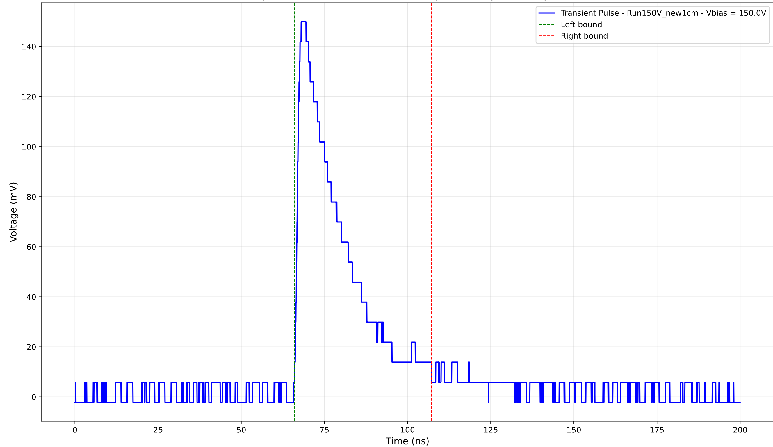
Transient Pulse - Sample: New1cm - Position: 3795.0 \mu\text{m} - Charge: 44.28 pC - Rise Time: 1.46 ns
