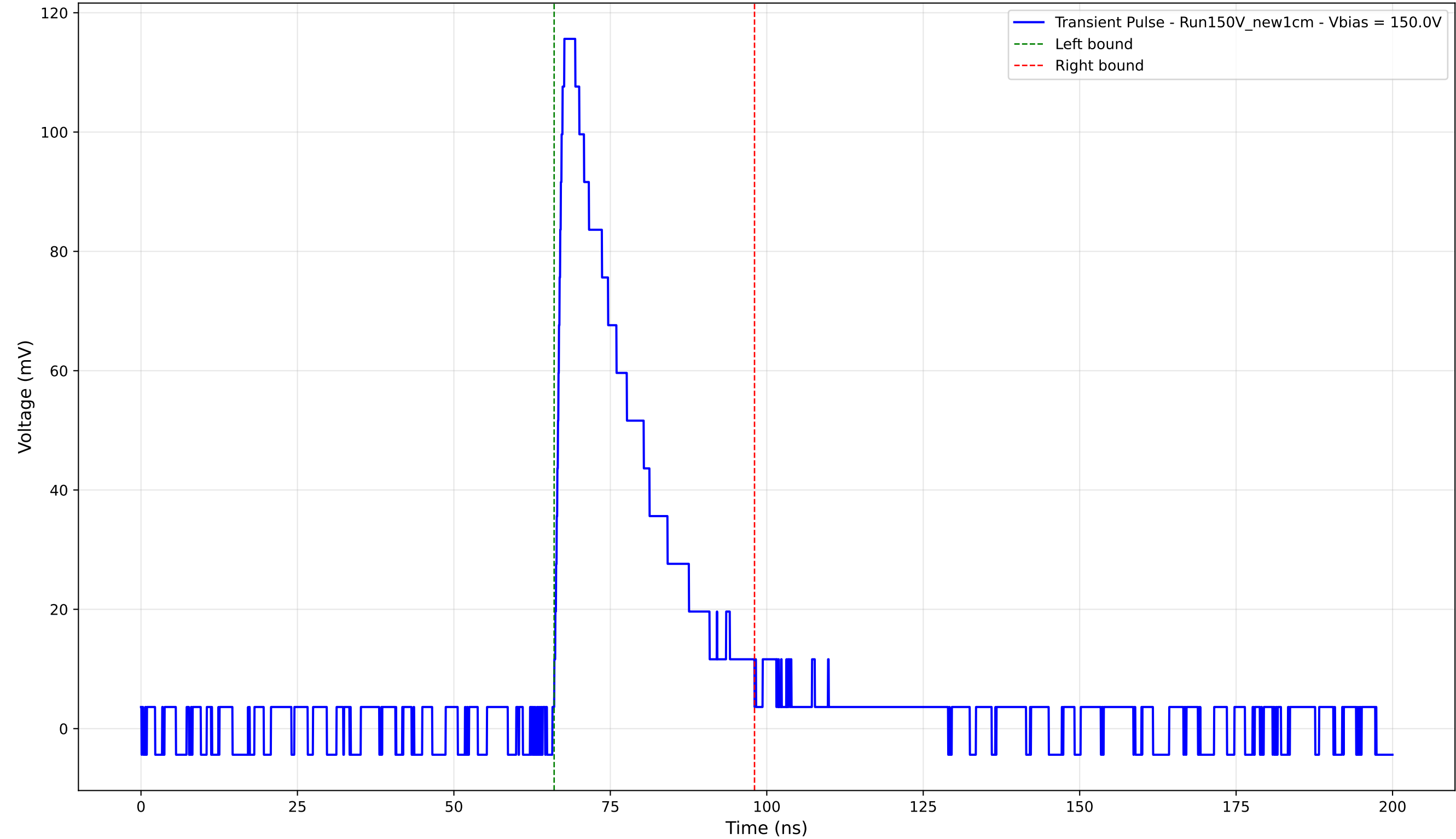
Transient Pulse - Sample: New1cm - Position: 700.0 \mu\text{m} - Charge: 29.82 pC - Rise Time: 1.32 ns
