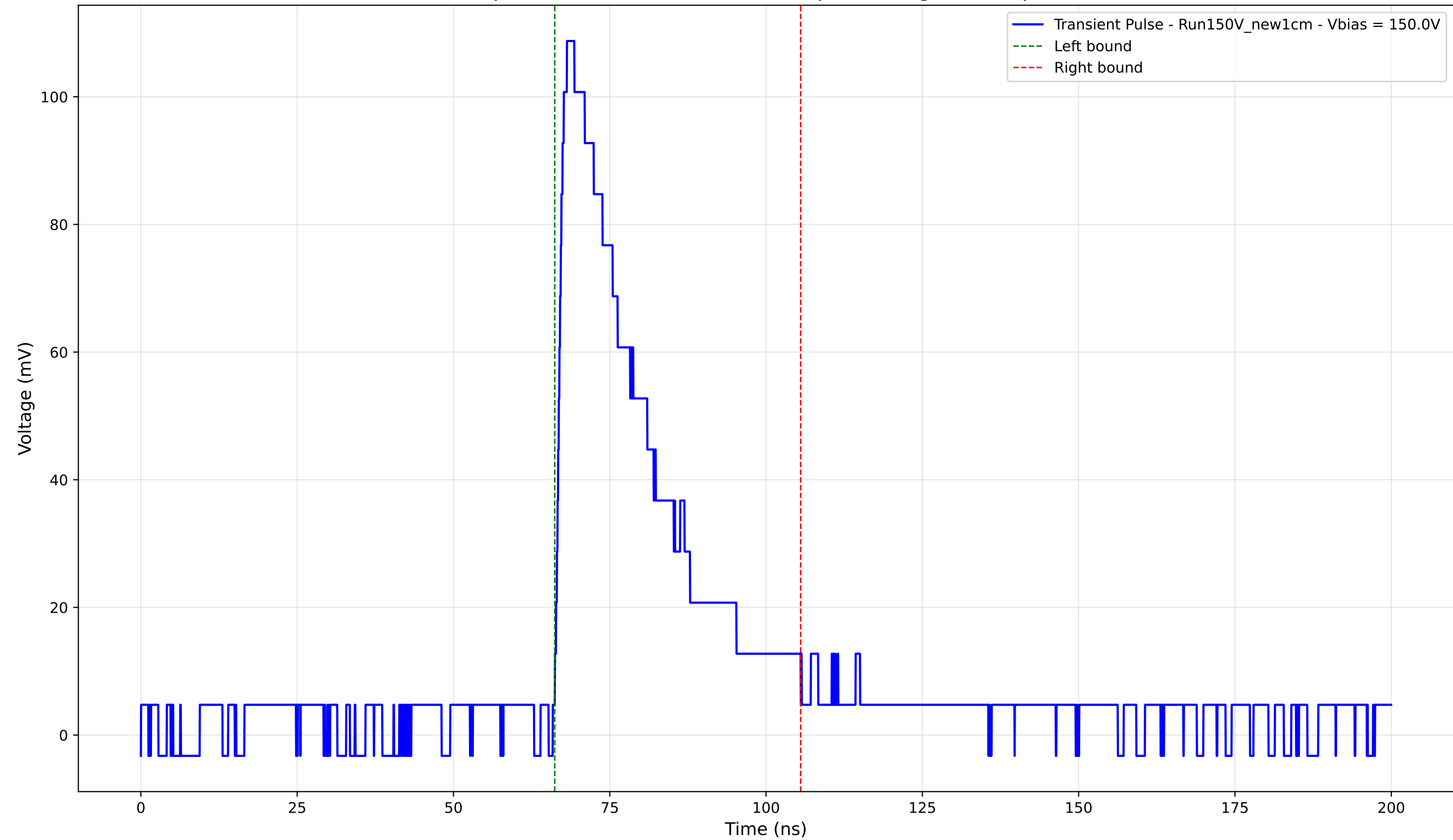
Transient Pulse - Sample: New1cm - Position: 1315.0 \mu\text{m} - Charge: 33.13 pC - Rise Time: 1.42 ns
