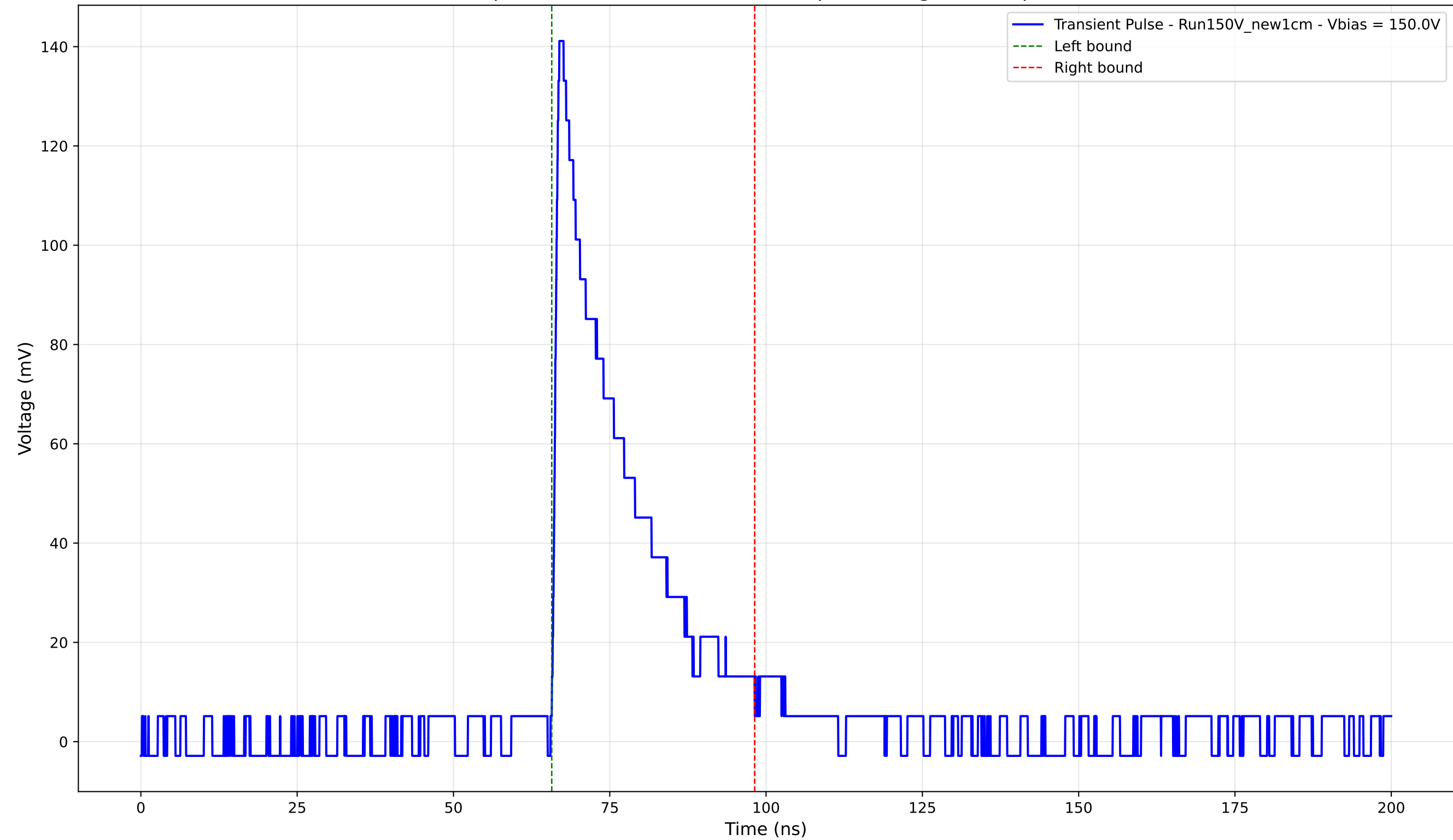
Transient Pulse - Sample: New1cm - Position: 4720.0 \mu\text{m} - Charge: 31.84 pC - Rise Time: 0.94 ns
