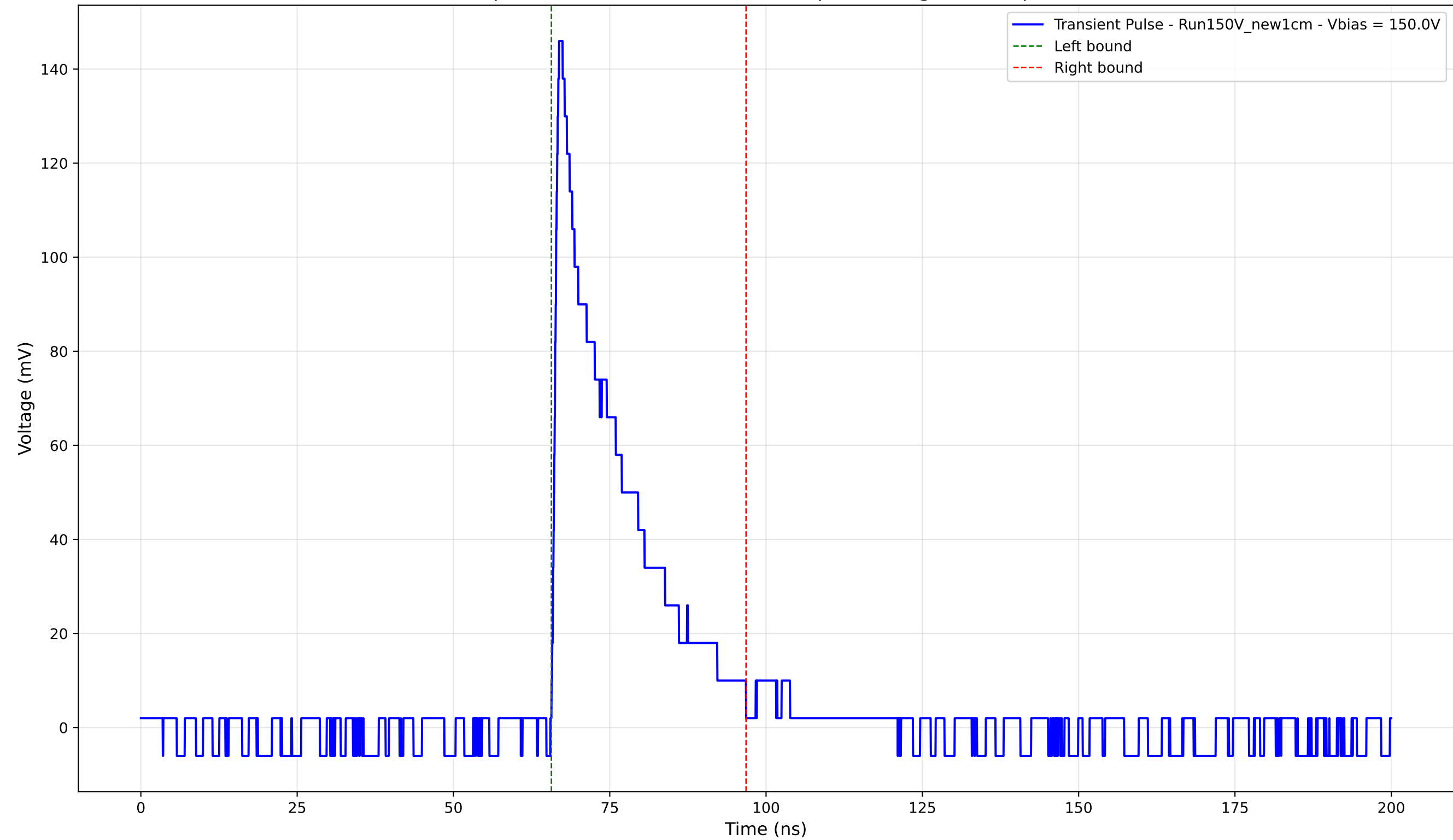
Transient Pulse - Sample: New1cm - Position: 4740.0 \mu\text{m} - Charge: 29.69 pC - Rise Time: 0.99 ns
