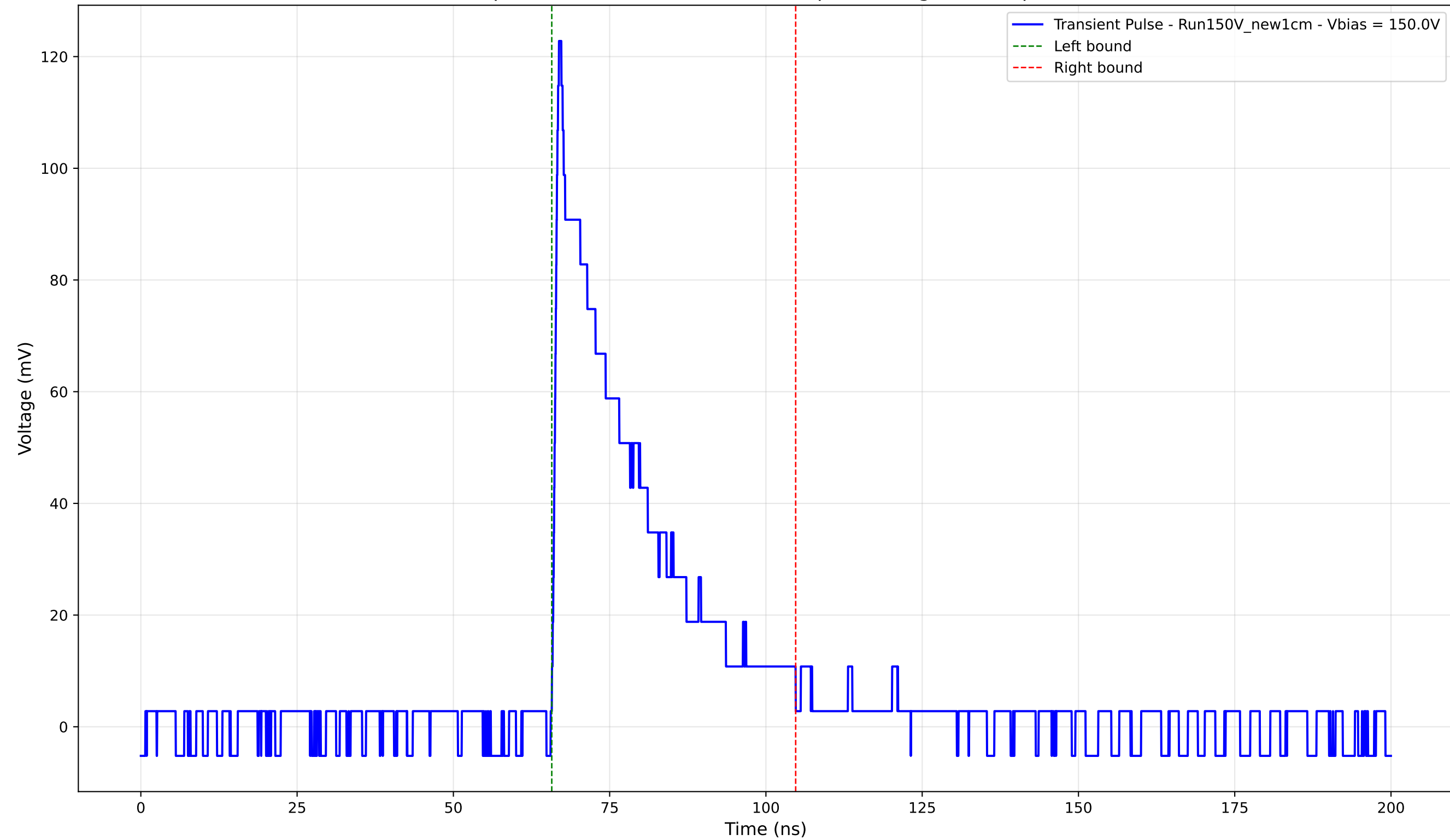
Transient Pulse - Sample: New1cm - Position: 2160.0 \mu\text{m} - Charge: 29.71 pC - Rise Time: 0.88 ns
