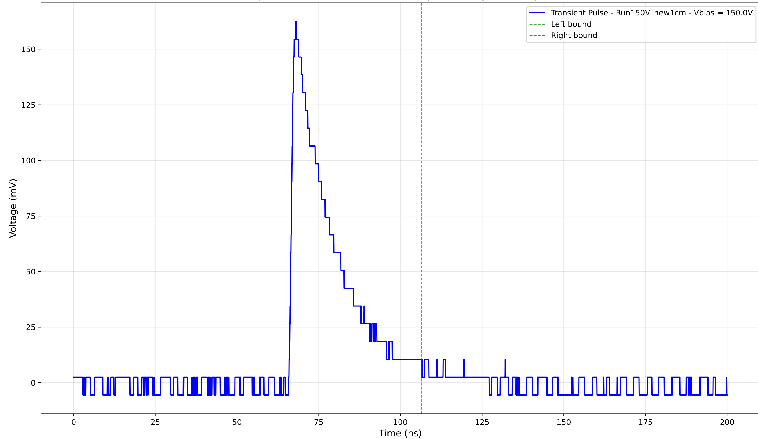
Transient Pulse - Sample: New1cm - Position: 4280.0 \mu\text{m} - Charge: 42.03 pC - Rise Time: 1.29 ns
