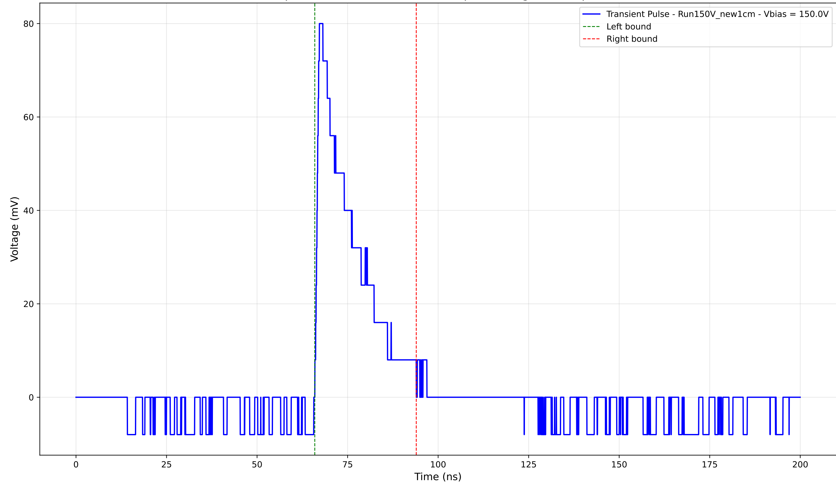
Transient Pulse - Sample: New1cm - Position: 460.0 \mu\text{m} - Charge: 16.82 pC - Rise Time: 0.84 ns
