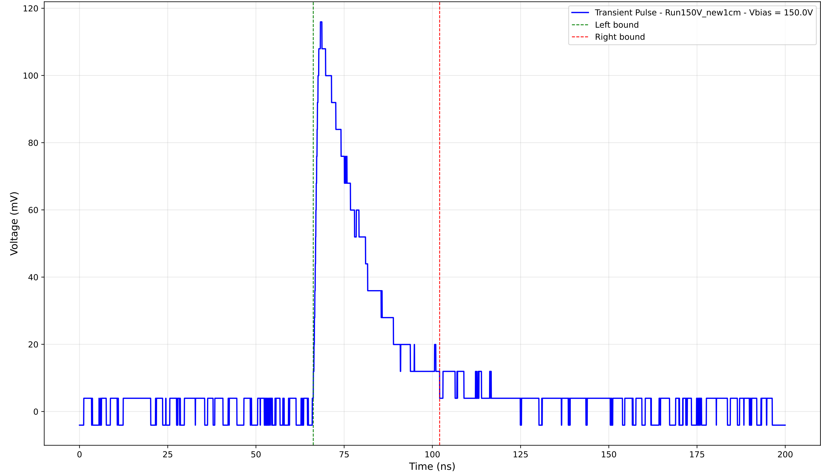
Transient Pulse - Sample: New1cm - Position: 1215.0 \mu\text{m} - Charge: 31.87 pC - Rise Time: 1.54 ns
