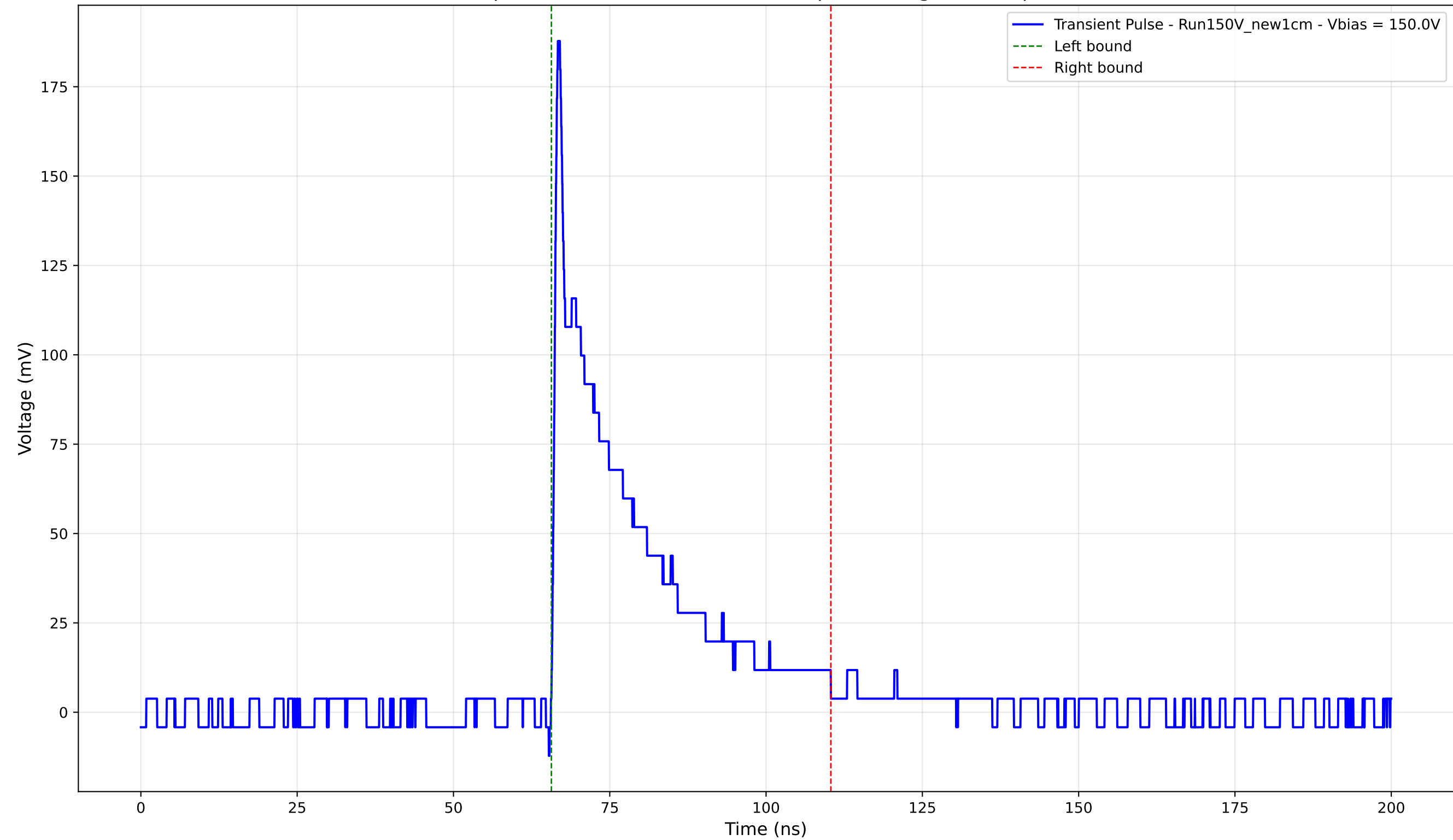
Transient Pulse - Sample: New1cm - Position: 2760.0 \mu\text{m} - Charge: 38.62 pC - Rise Time: 0.78 ns
