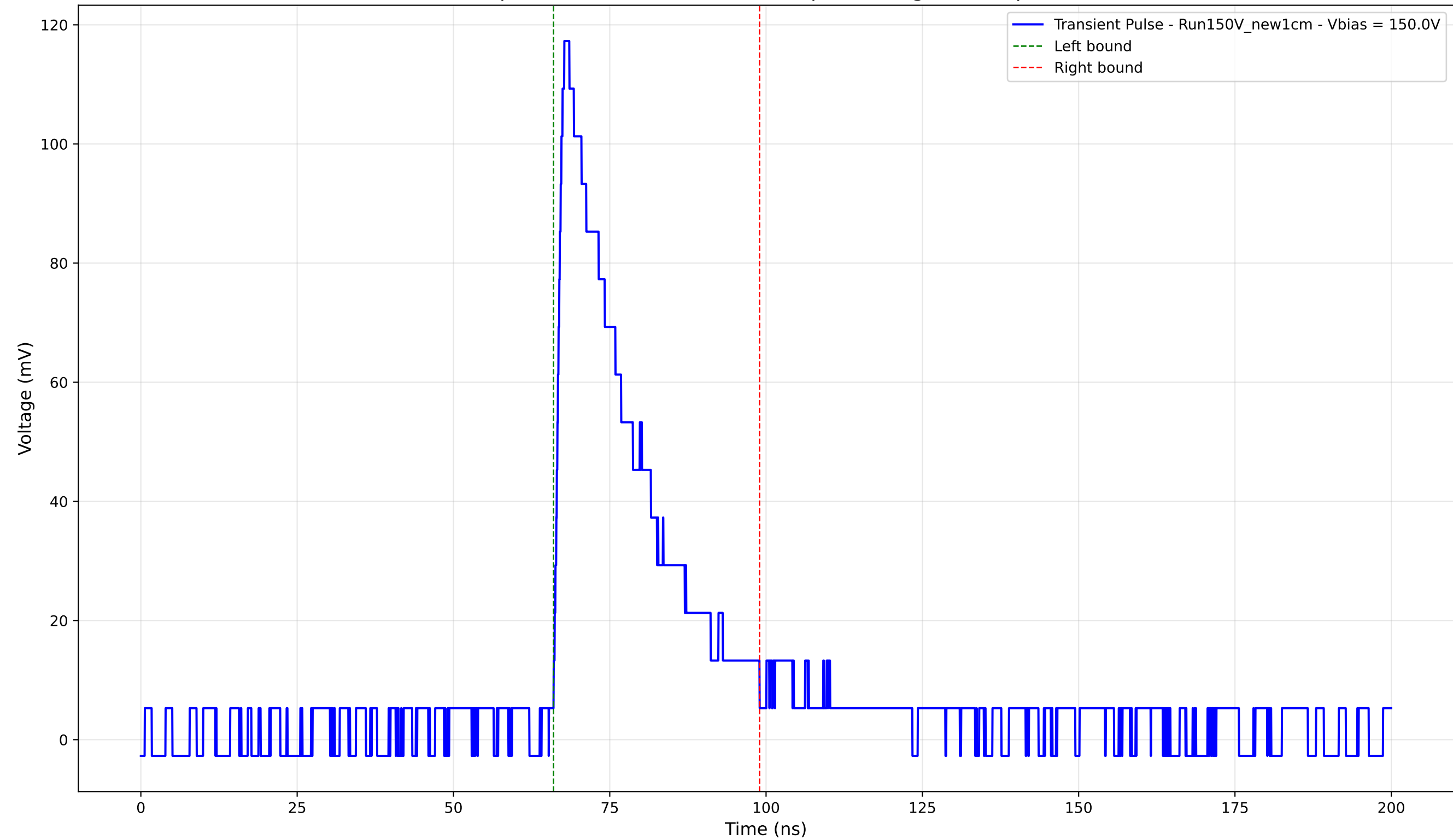
Transient Pulse - Sample: New1cm - Position: 650.0 \mu\text{m} - Charge: 30.02 pC - Rise Time: 1.42 ns
