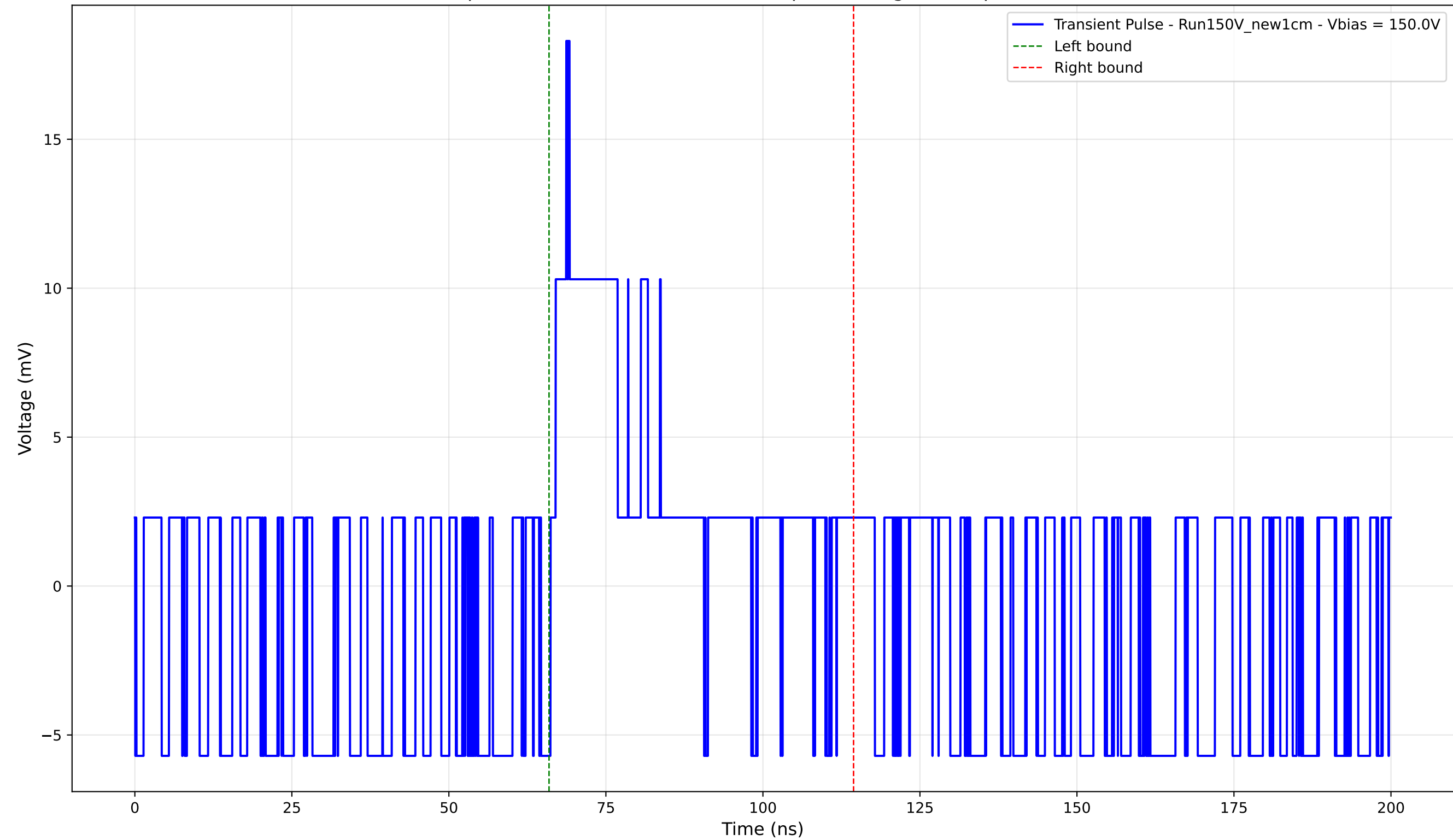
Transient Pulse - Sample: New1cm - Position: 1030.0 \mu\text{m} - Charge: 3.68 pC - Rise Time: 0.00 ns (N/A)
