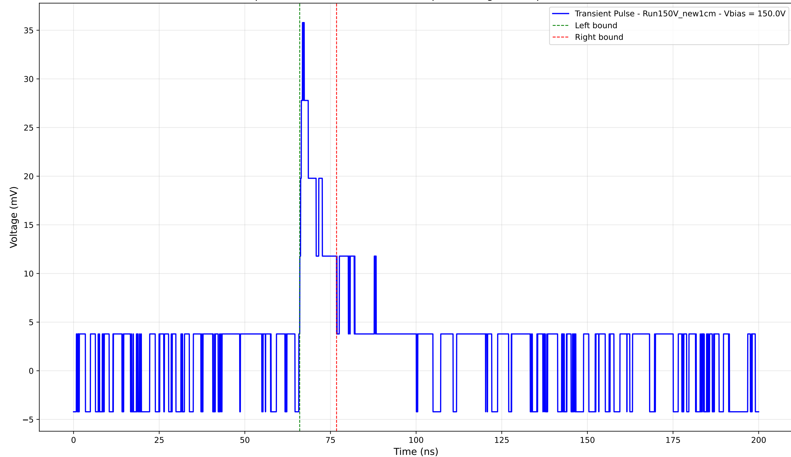
Transient Pulse - Sample: New1cm - Position: 4880.0 \mu\text{m} - Charge: 3.82 pC - Rise Time: 0.00 ns (N/A)
