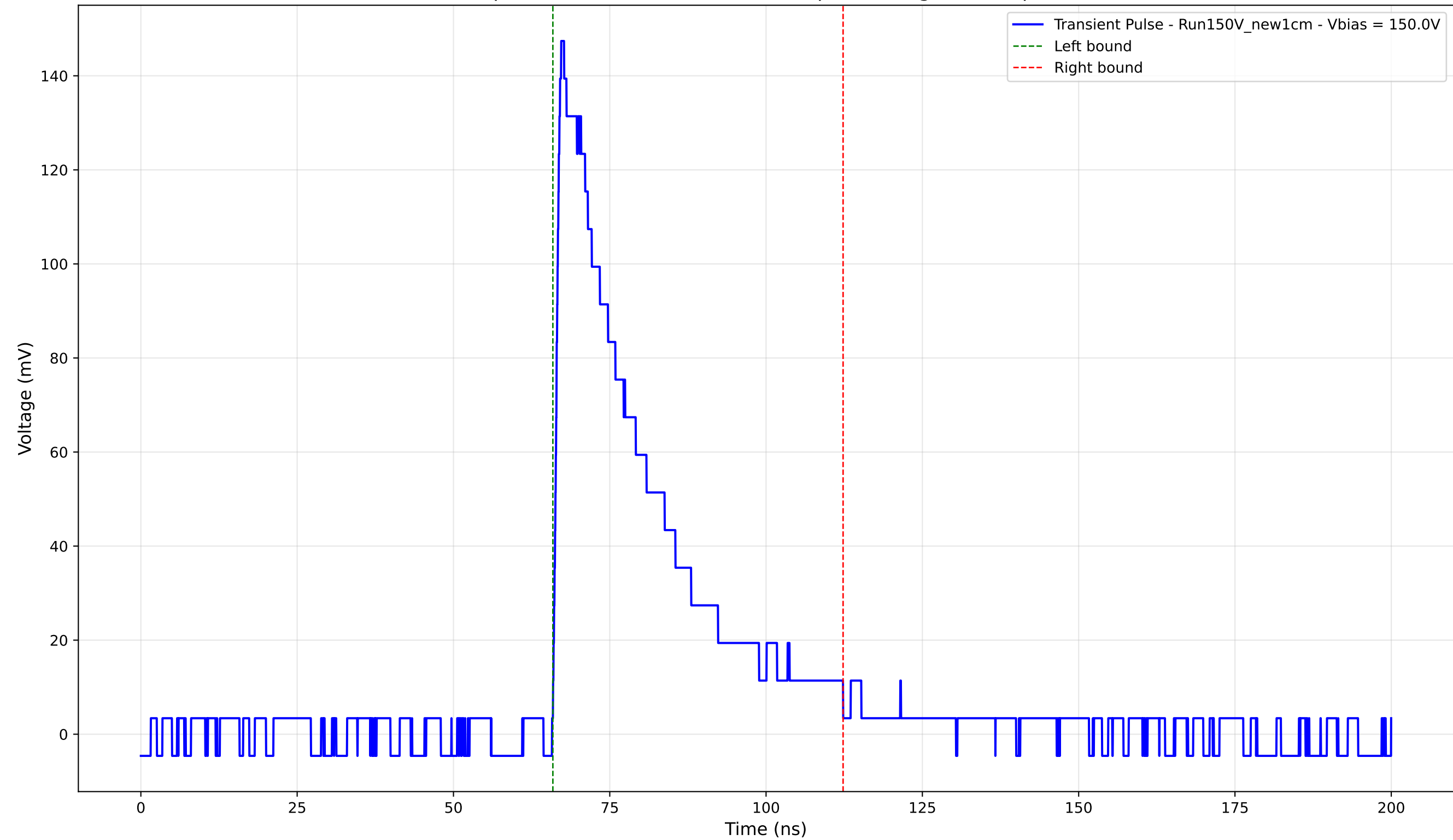
Transient Pulse - Sample: New1cm - Position: 3200.0 \mu\text{m} - Charge: 42.79 pC - Rise Time: 1.05 ns
