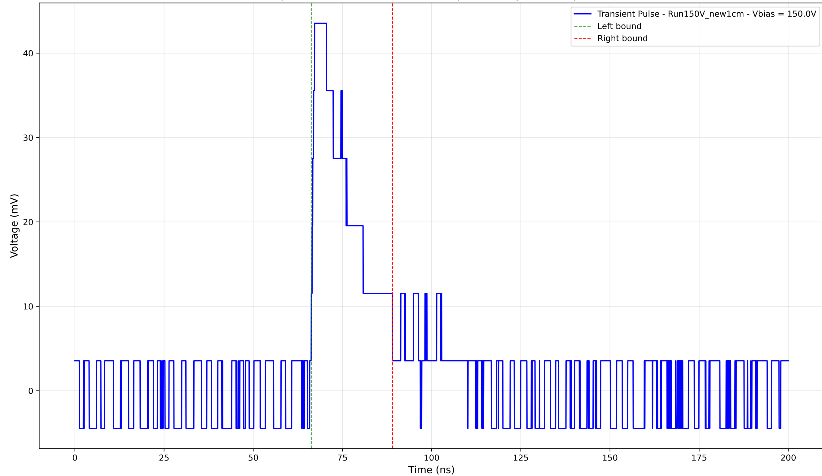
Transient Pulse - Sample: New1cm - Position: 570.0 \mu\text{m} - Charge: 10.54 pC - Rise Time: 0.94 ns
