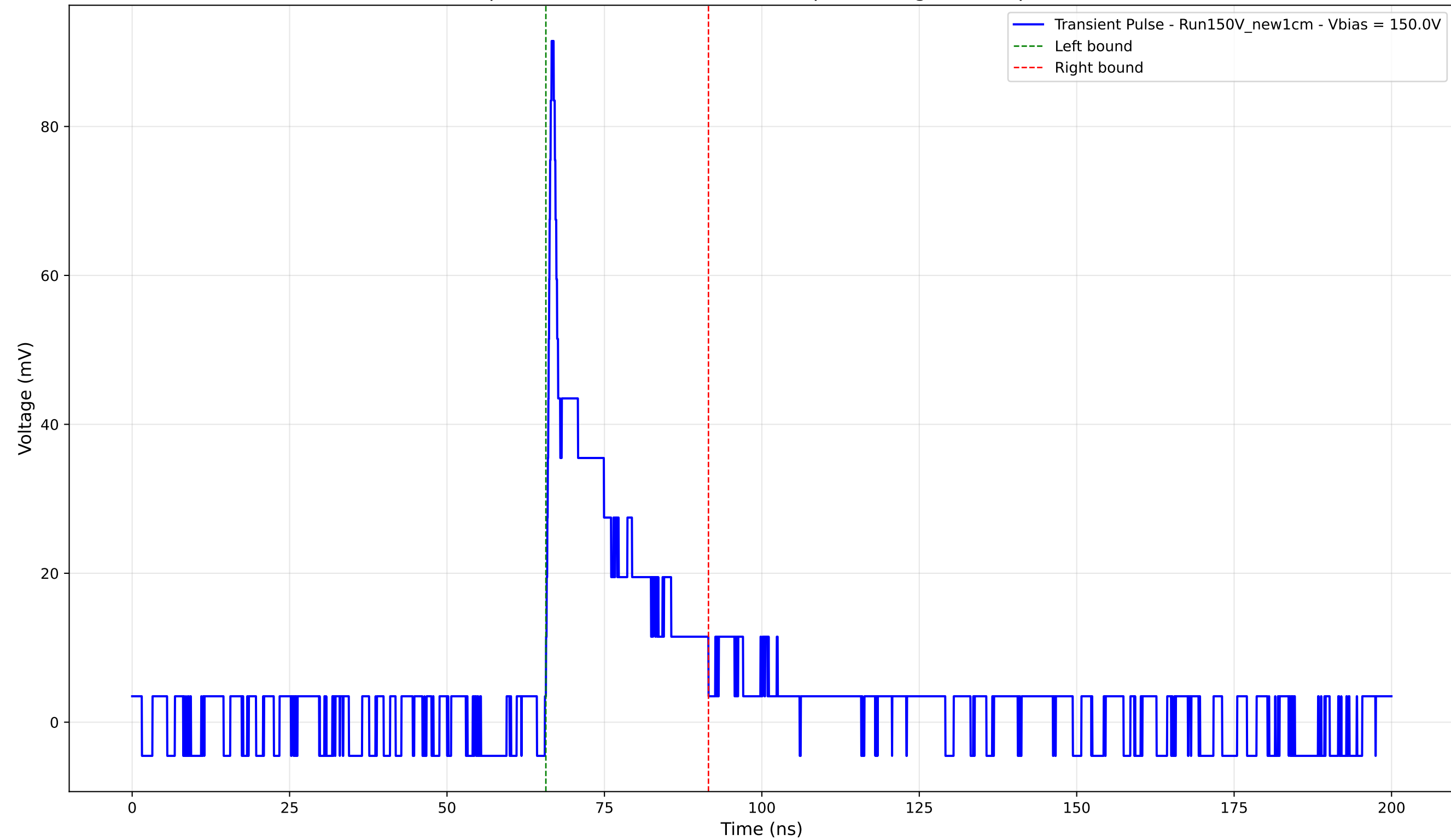
Transient Pulse - Sample: New1cm - Position: 2505.0 \mu\text{m} - Charge: 13.78 pC - Rise Time: 0.75 ns
