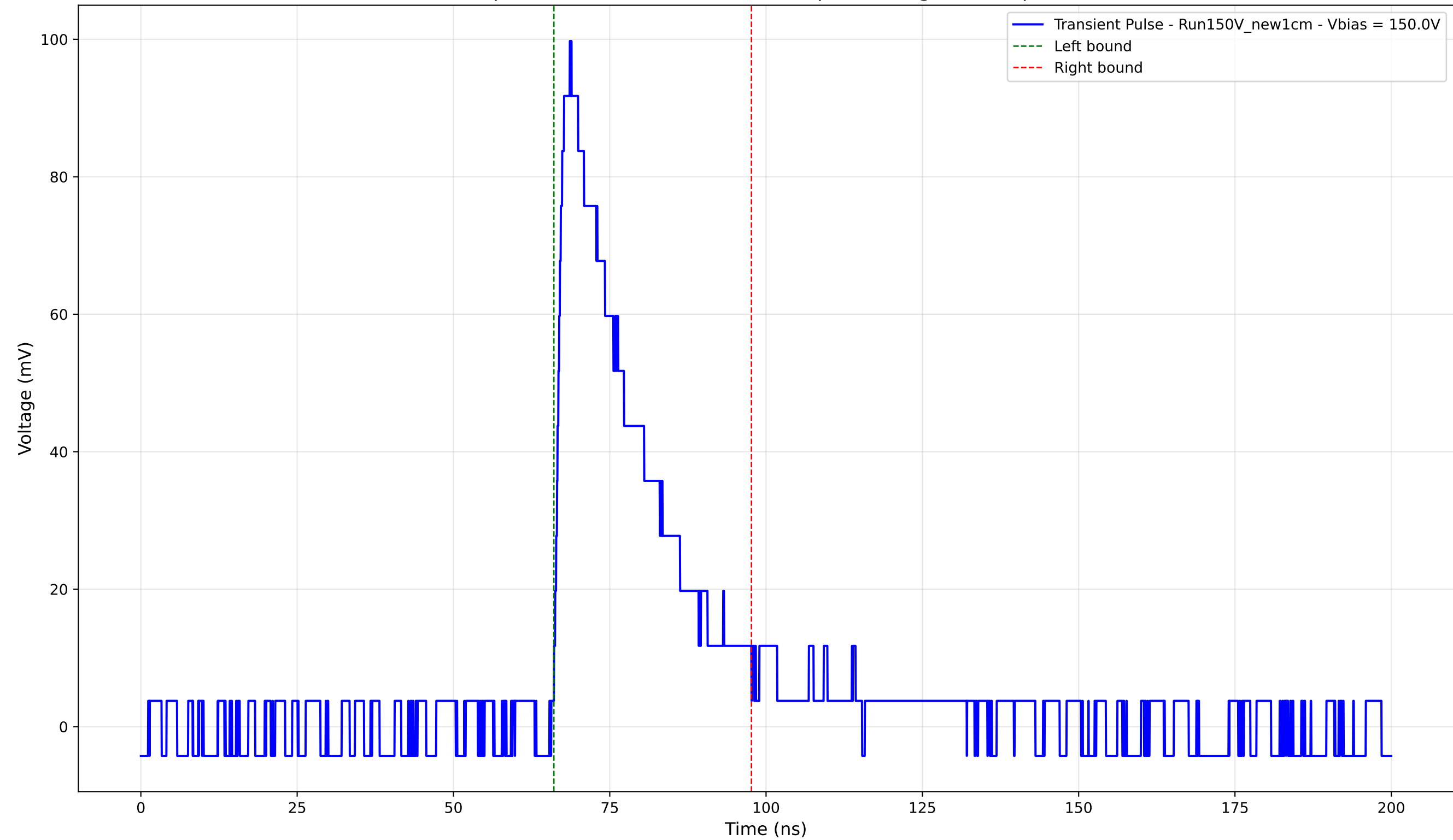
Transient Pulse - Sample: New1cm - Position: 4000.0 \mu\text{m} - Charge: 25.52 pC - Rise Time: 1.60 ns
