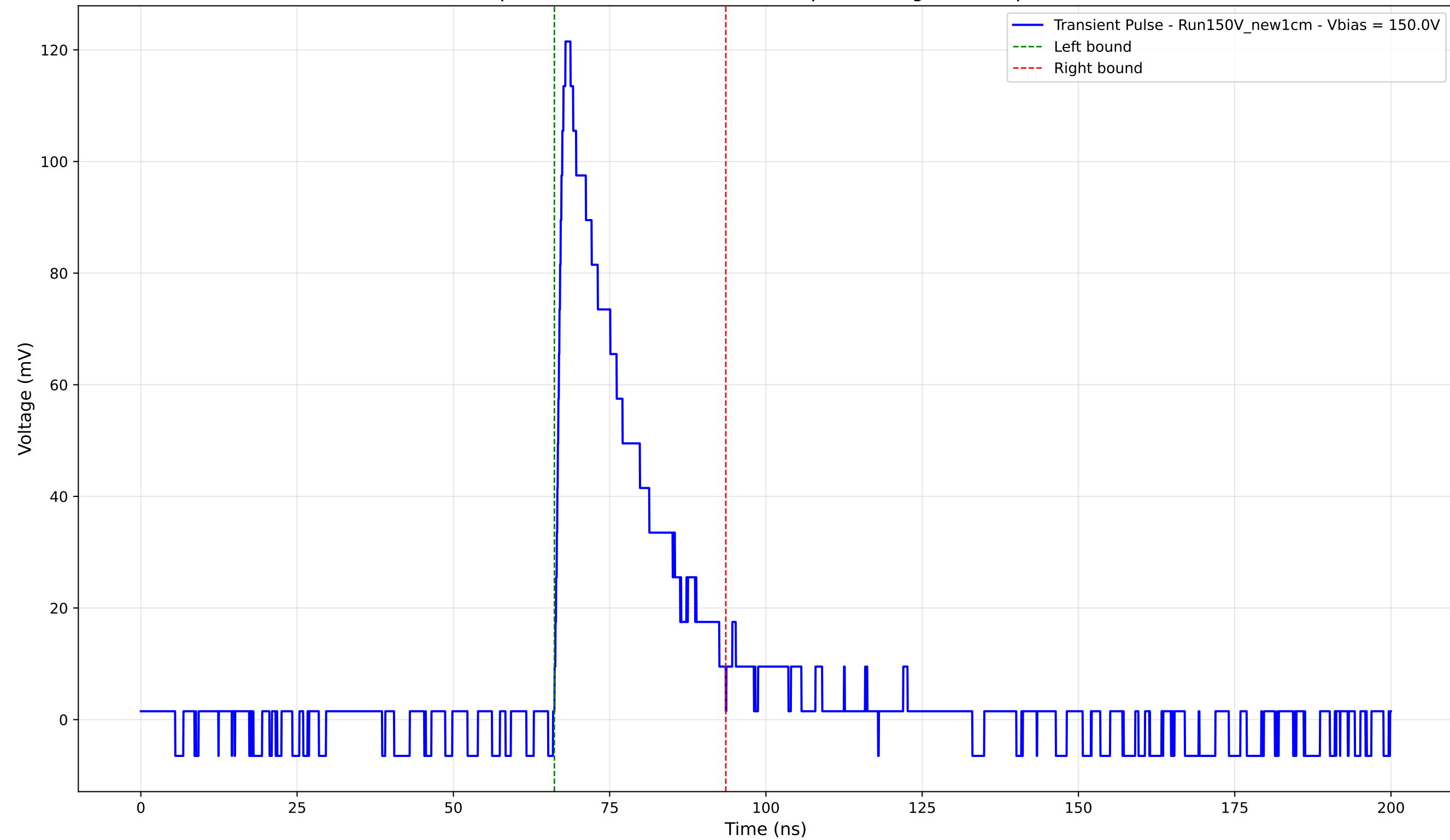
Transient Pulse - Sample: New1cm - Position: 745.0 \mu\text{m} - Charge: 27.82 pC - Rise Time: 1.29 ns
