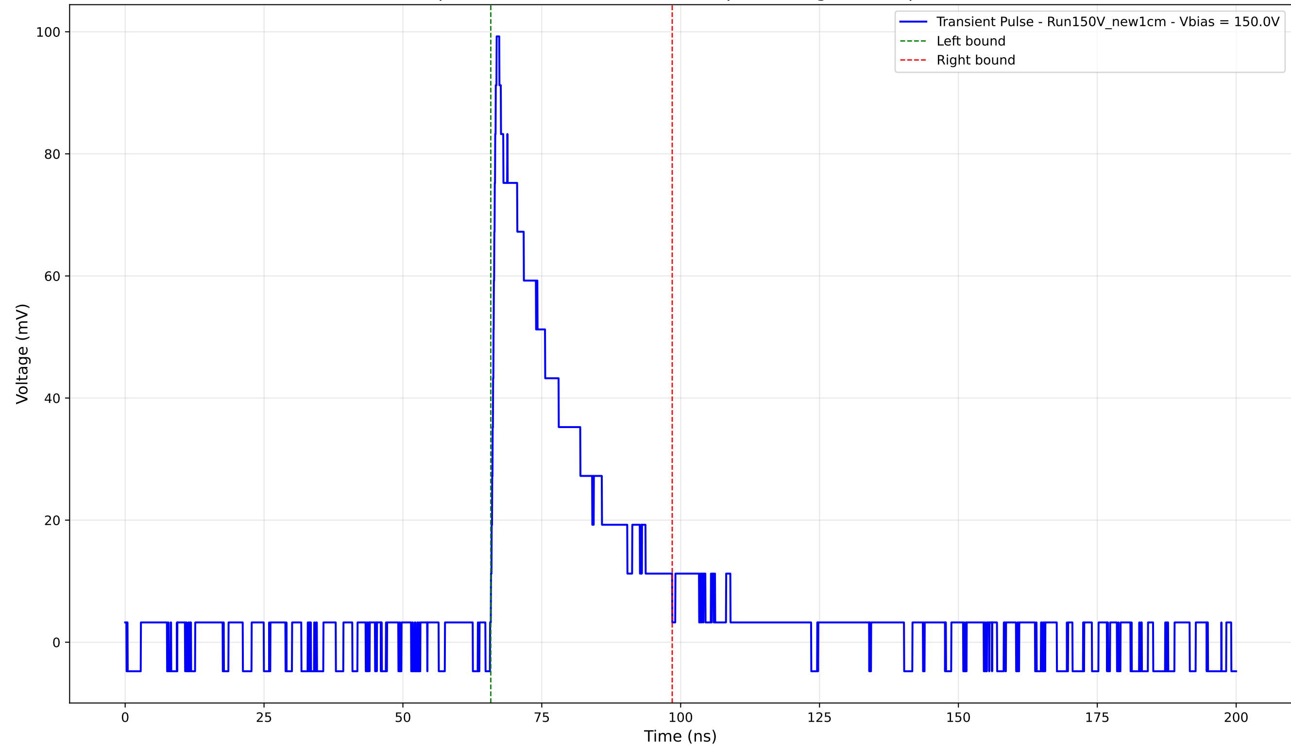
Transient Pulse - Sample: New1cm - Position: 2995.0 \mu\text{m} - Charge: 23.85 pC - Rise Time: 0.86 ns
