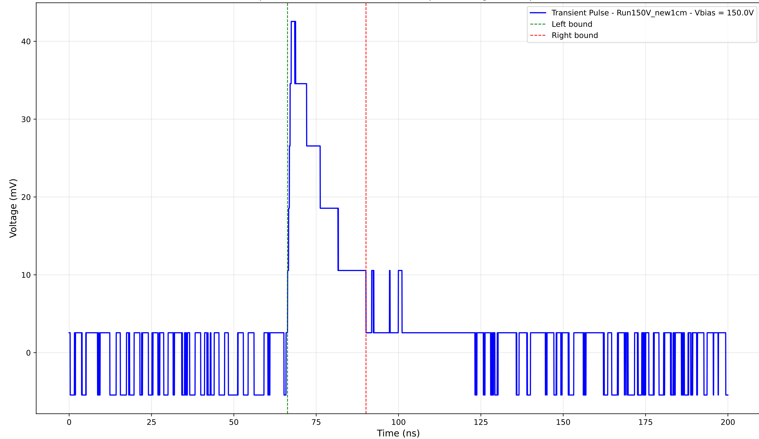
Transient Pulse - Sample: New1cm - Position: 3530.0 \mu\text{m} - Charge: 9.92 pC - Rise Time: 1.12 ns
