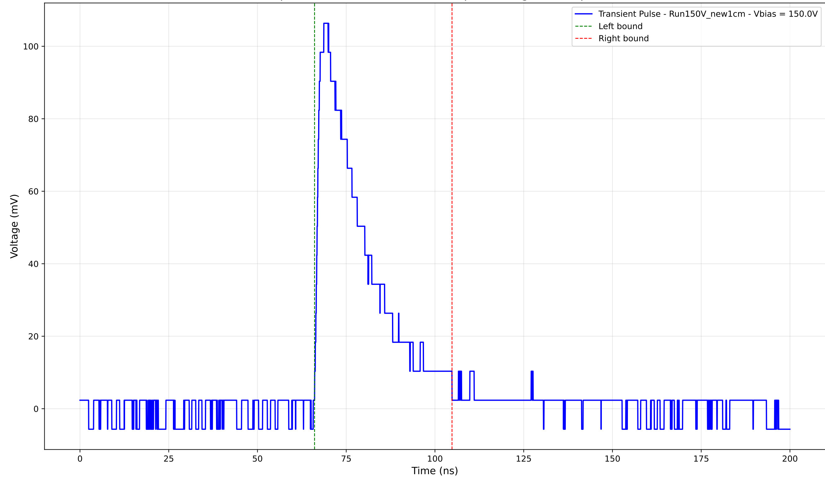
Transient Pulse - Sample: New1cm - Position: 1430.0 \mu\text{m} - Charge: 30.79 pC - Rise Time: 1.40 ns
