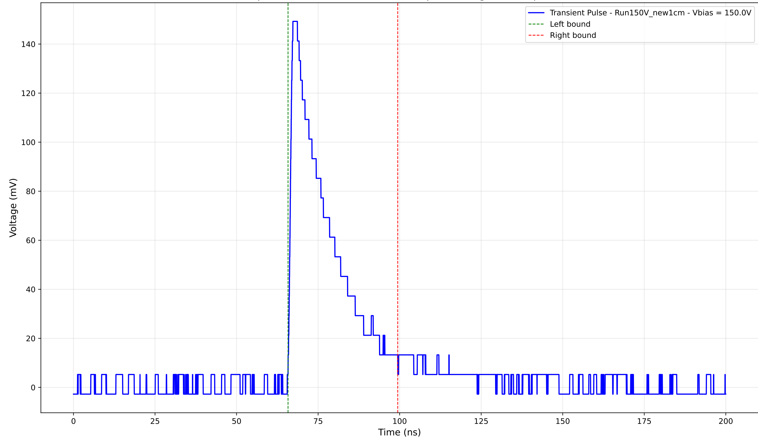
Transient Pulse - Sample: New1cm - Position: 4435.0 \mu\text{m} - Charge: 38.39 pC - Rise Time: 1.18 ns
