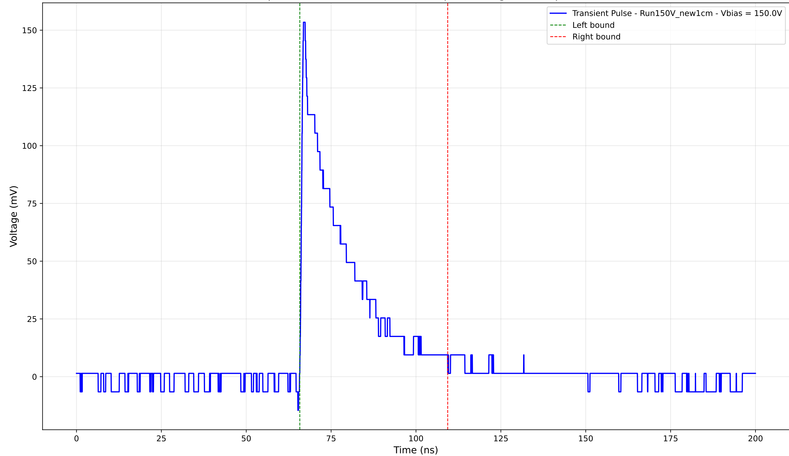
Transient Pulse - Sample: New1cm - Position: 2945.0 \mu\text{m} - Charge: 37.40 pC - Rise Time: 0.87 ns
