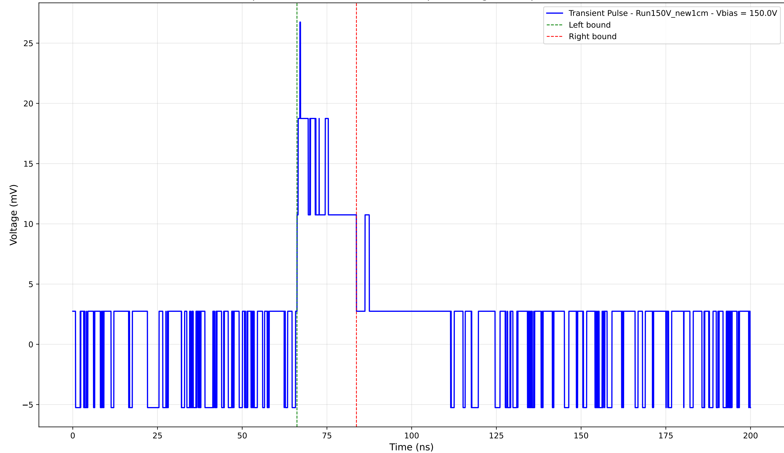
Transient Pulse - Sample: New1cm - Position: 3050.0 \mu\text{m} - Charge: 4.67 pC - Rise Time: 0.00 ns (N/A)
