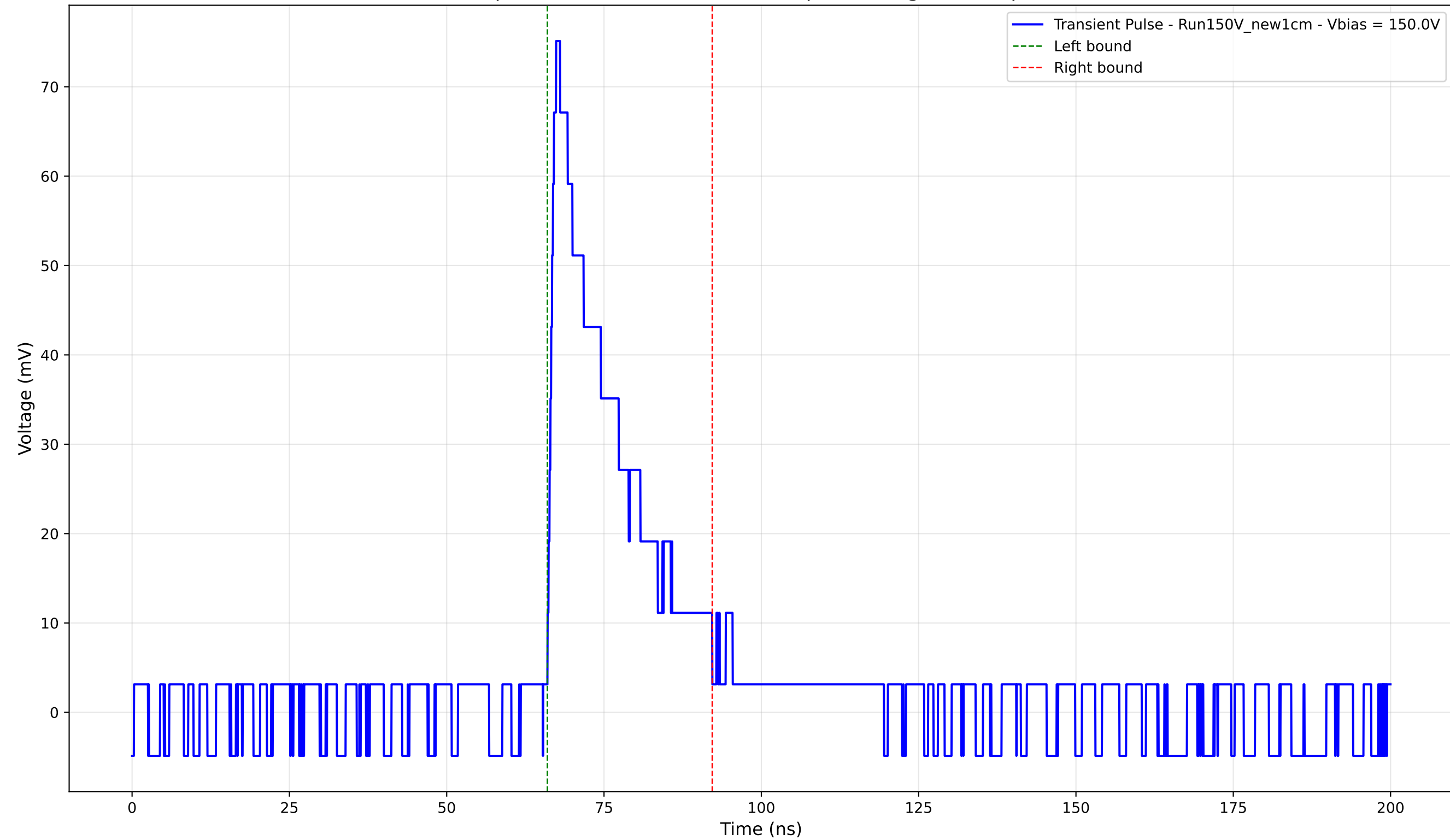
Transient Pulse - Sample: New1cm - Position: 470.0 \mu\text{m} - Charge: 15.85 pC - Rise Time: 1.37 ns
