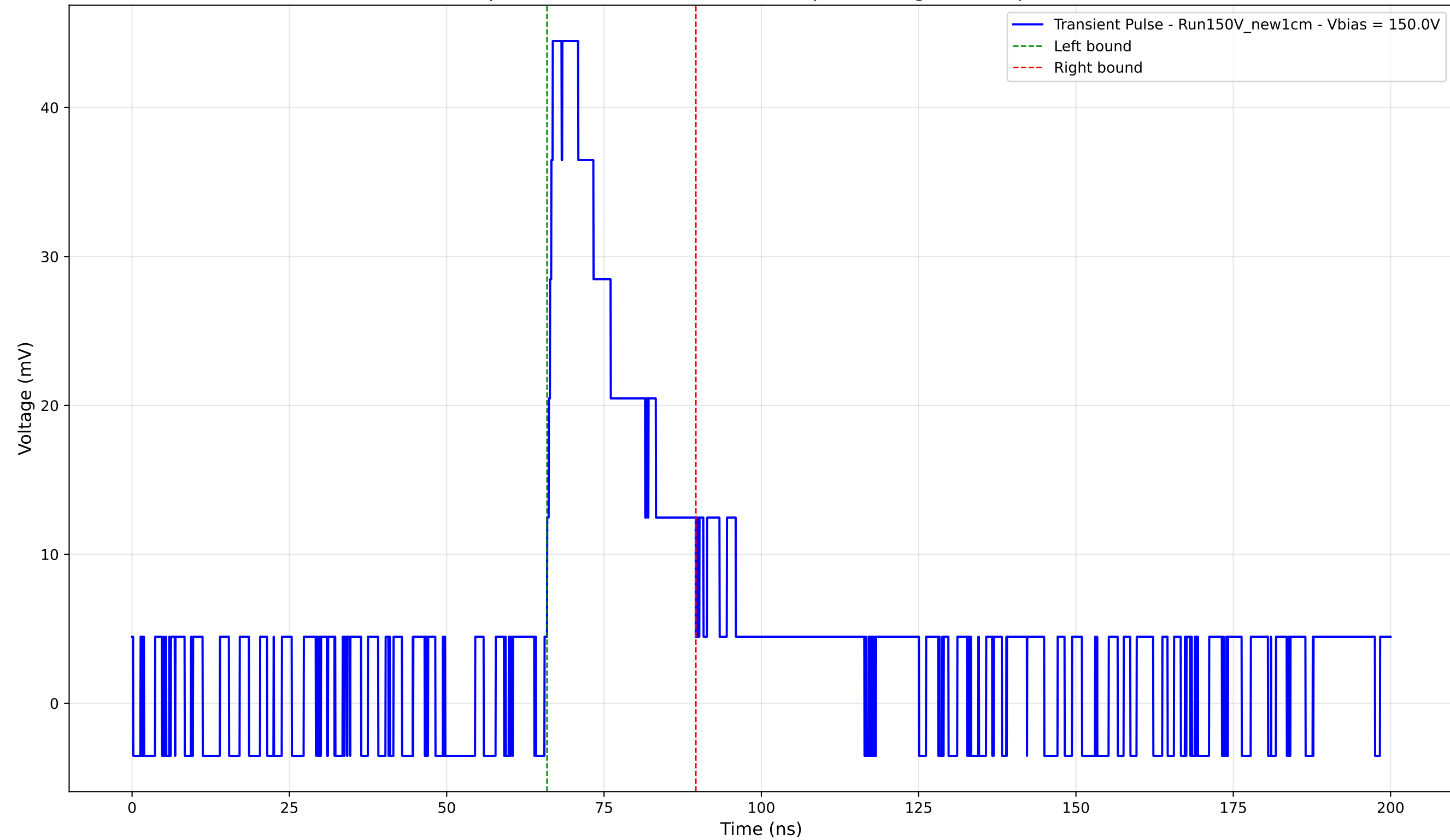
Transient Pulse - Sample: New1cm - Position: 3095.0 \mu\text{m} - Charge: 11.82 pC - Rise Time: 1.30 ns
