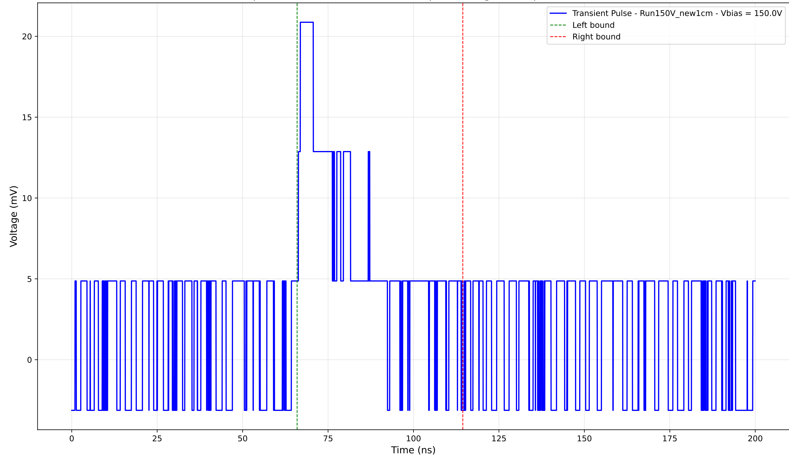
Transient Pulse - Sample: New1cm - Position: 4565.0 \mu\text{m} - Charge: 7.02 pC - Rise Time: 0.00 ns (N/A)
