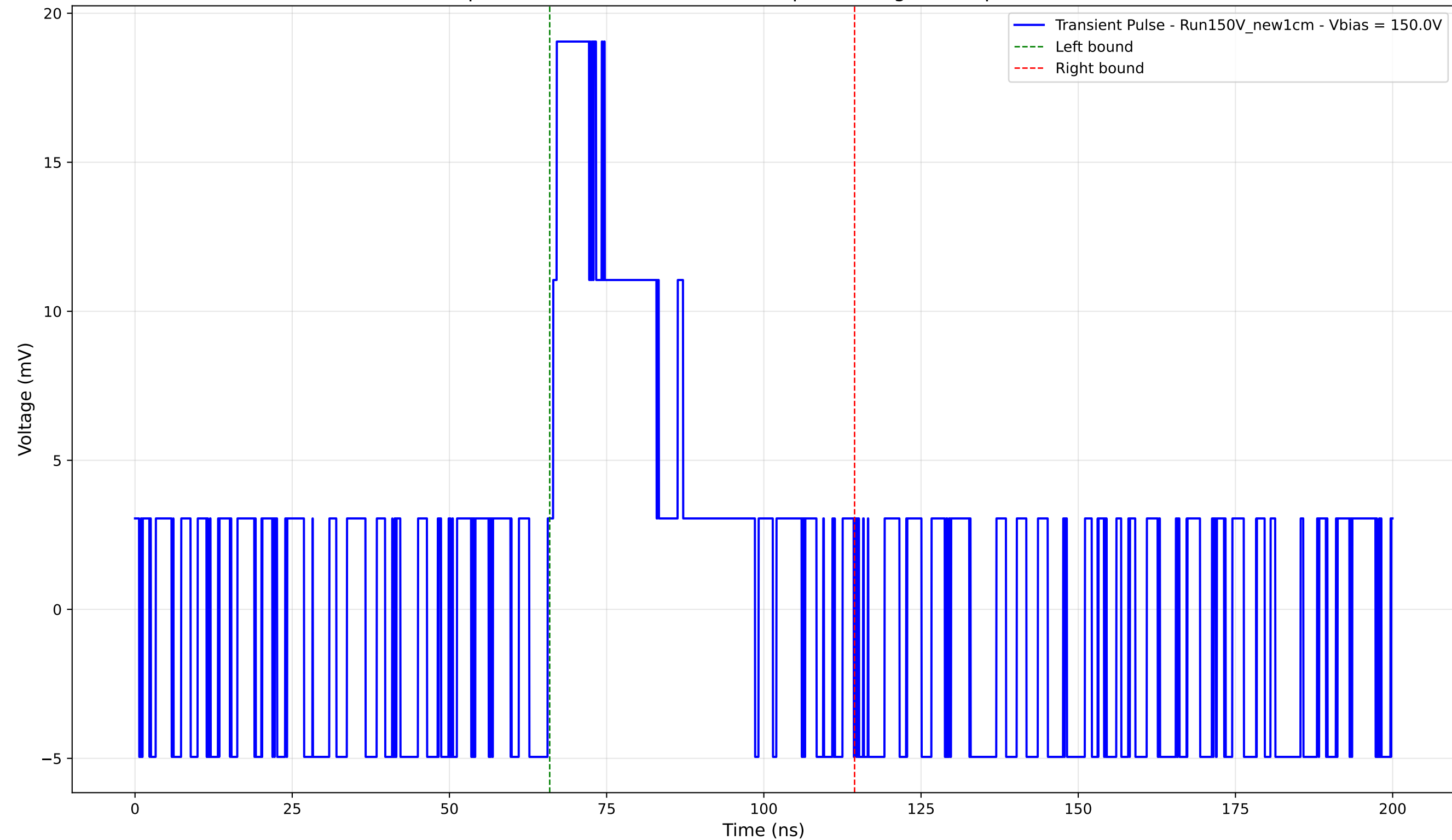
Transient Pulse - Sample: New1cm - Position: 4055.0 \mu\text{m} - Charge: 5.90 pC - Rise Time: 0.00 ns (N/A)
