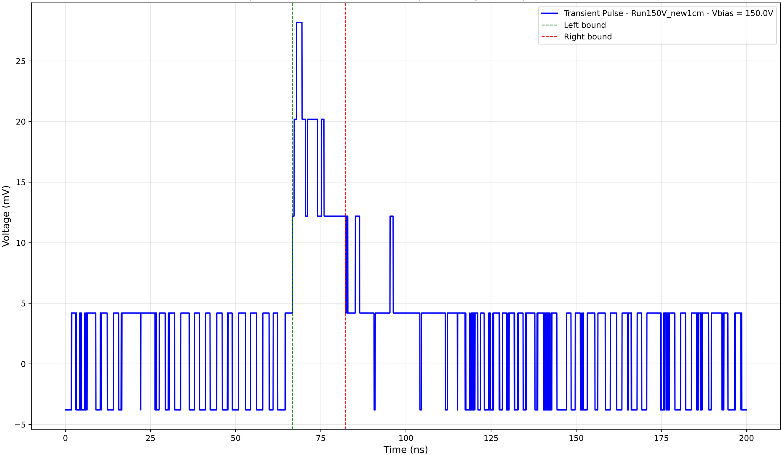
Transient Pulse - Sample: New1cm - Position: 550.0 \mu\text{m} - Charge: 5.17 pC - Rise Time: 0.00 ns (N/A)
