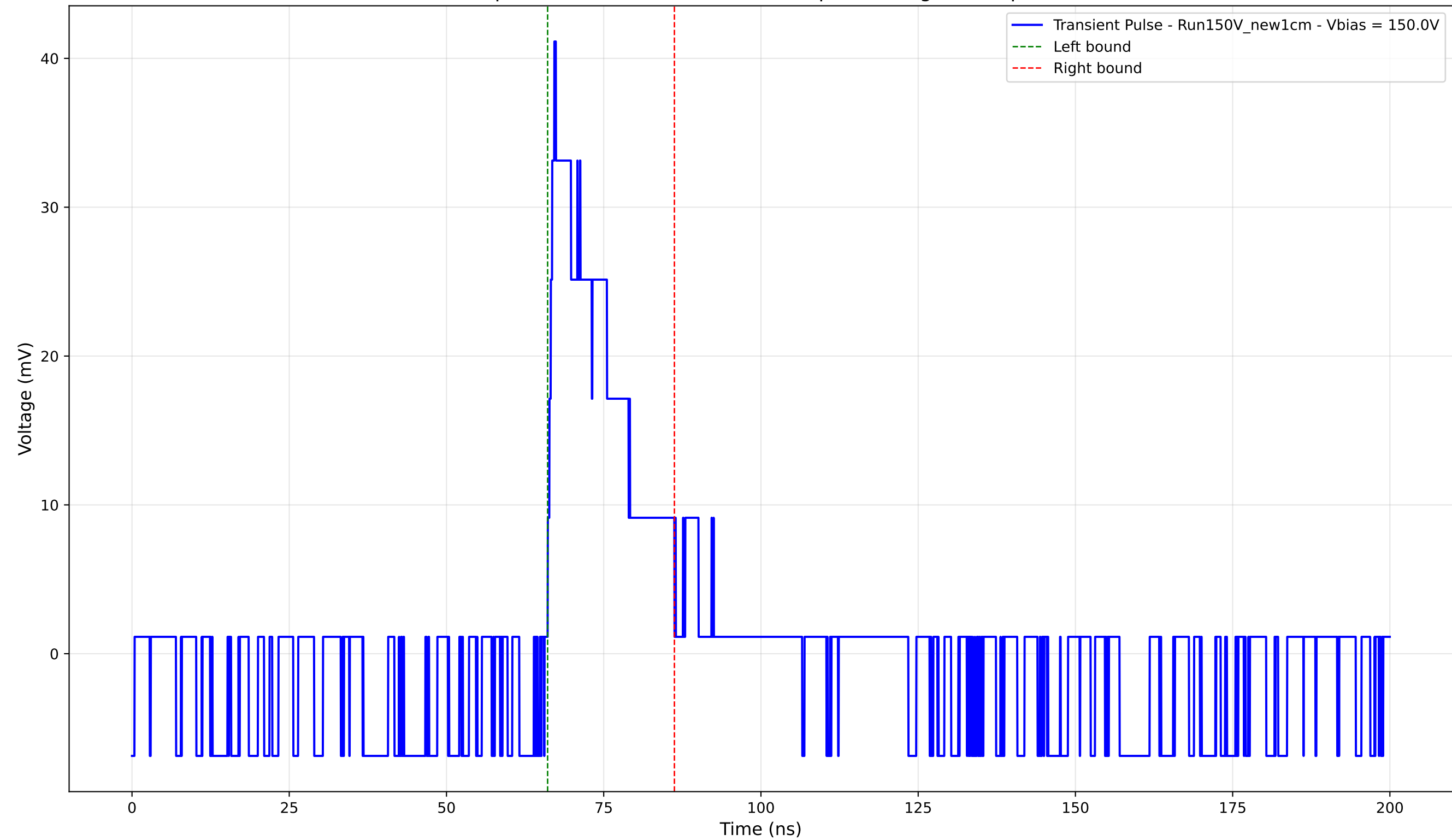
Transient Pulse - Sample: New1cm - Position: 3090.0 \mu\text{m} - Charge: 7.65 pC - Rise Time: 1.05 ns
