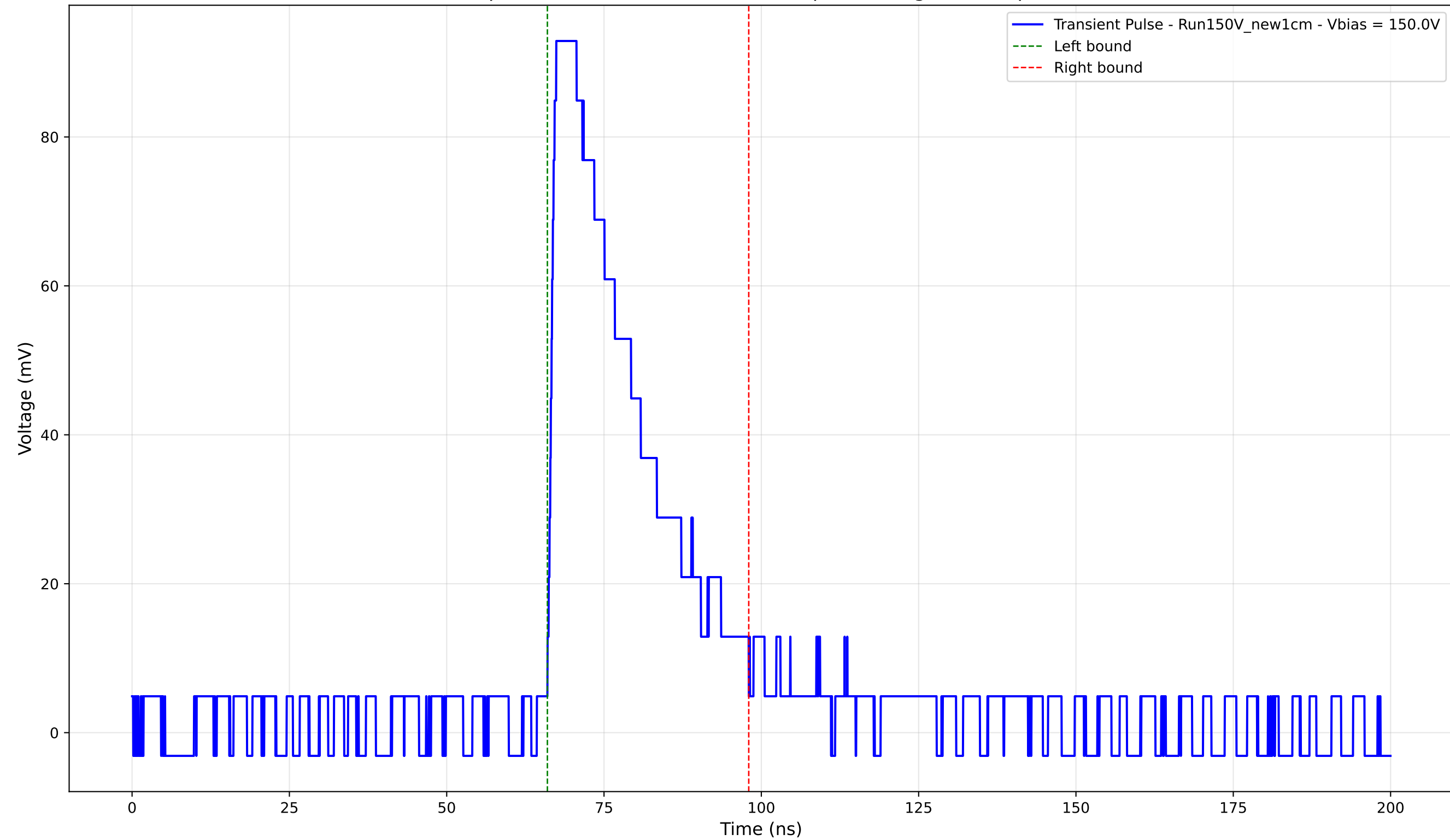
Transient Pulse - Sample: New1cm - Position: 1775.0 \mu\text{m} - Charge: 28.02 pC - Rise Time: 1.13 ns
