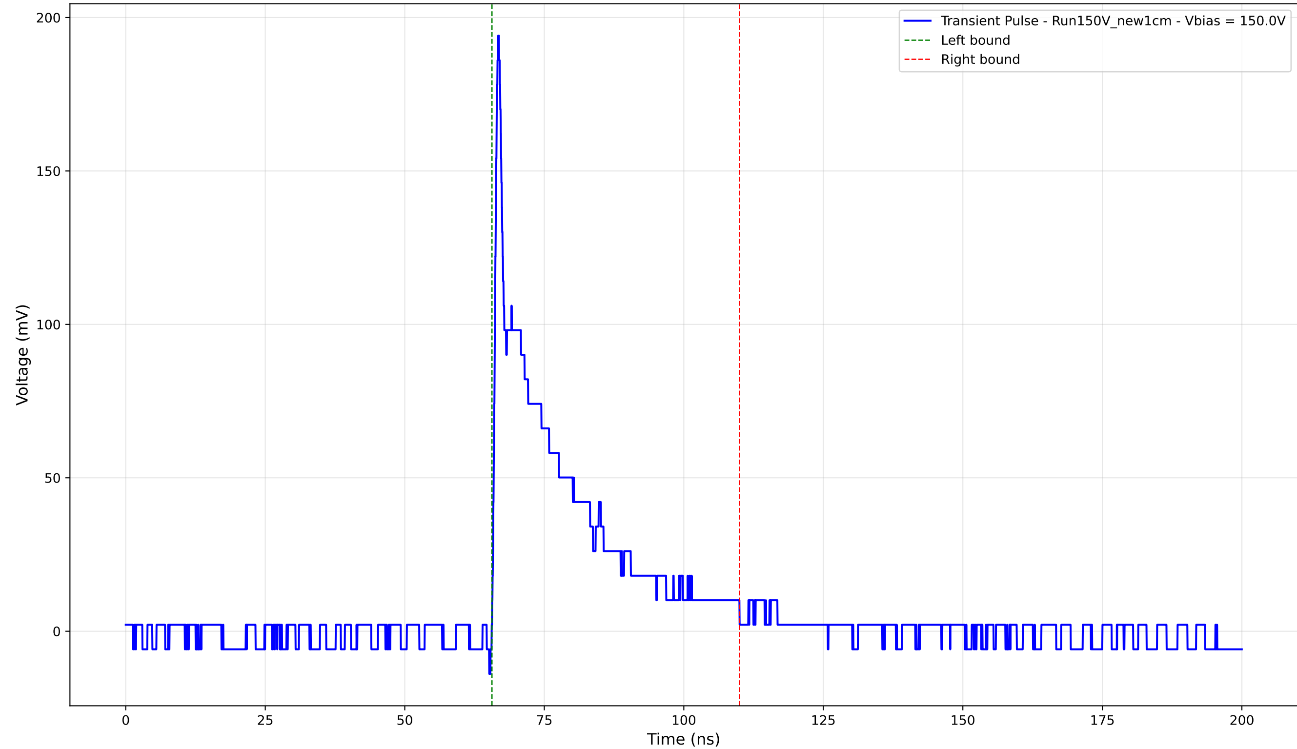
Transient Pulse - Sample: New1cm - Position: 2405.0 \mu\text{m} - Charge: 35.33 pC - Rise Time: 0.78 ns
