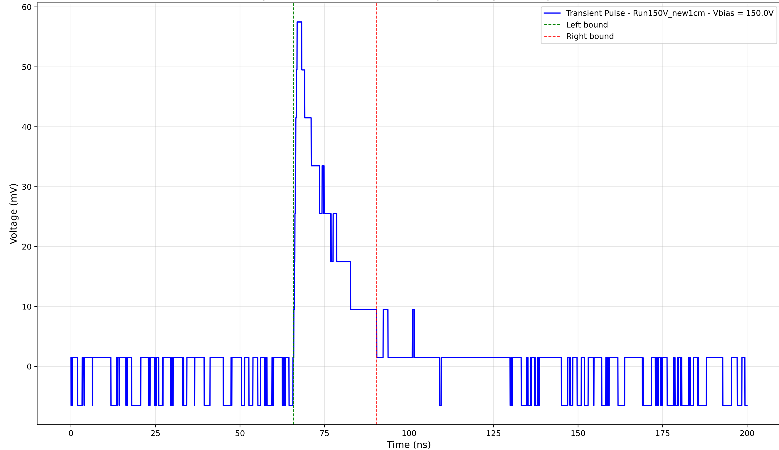
Transient Pulse - Sample: New1cm - Position: 4610.0 \mu\text{m} - Charge: 11.78 pC - Rise Time: 0.97 ns
