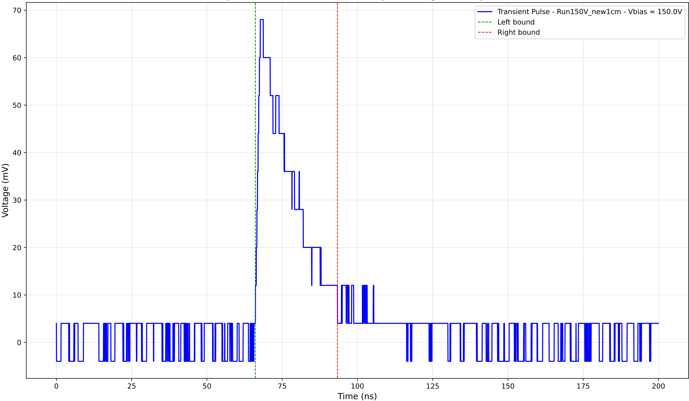
Transient Pulse - Sample: New1cm - Position: 4020.0 \mu\text{m} - Charge: 17.44 pC - Rise Time: 1.61 ns
