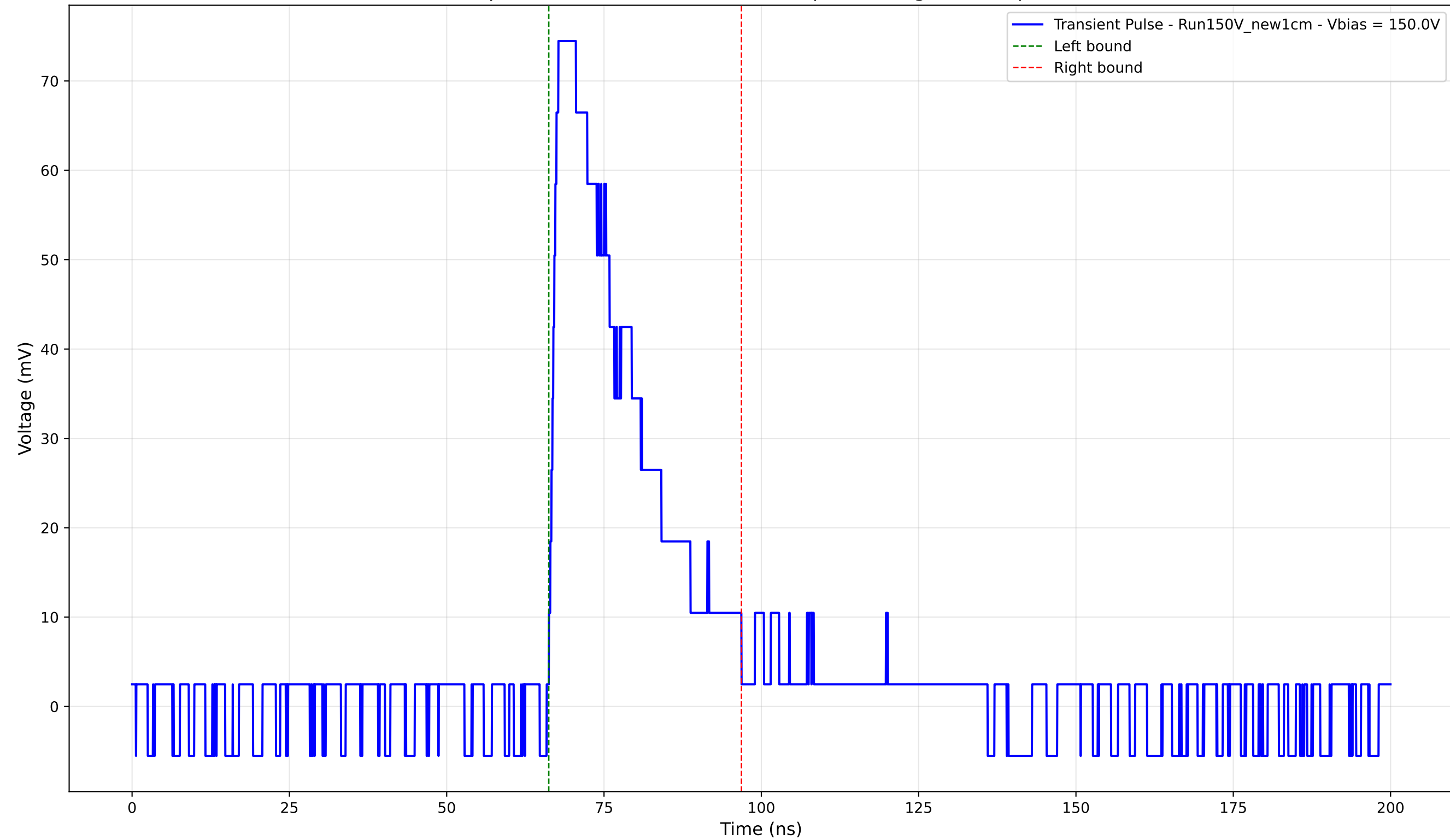
Transient Pulse - Sample: New1cm - Position: 1110.0 \mu\text{m} - Charge: 20.66 pC - Rise Time: 1.51 ns
