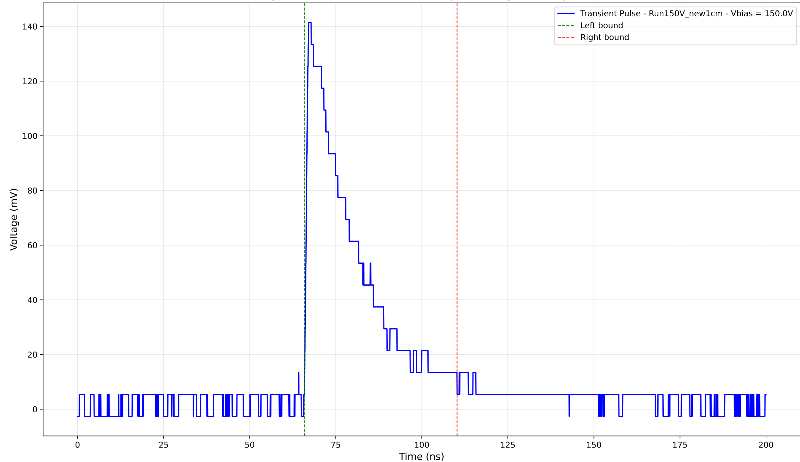
Transient Pulse - Sample: New1cm - Position: 3195.0 \mu\text{m} - Charge: 43.59 pC - Rise Time: 1.00 ns
