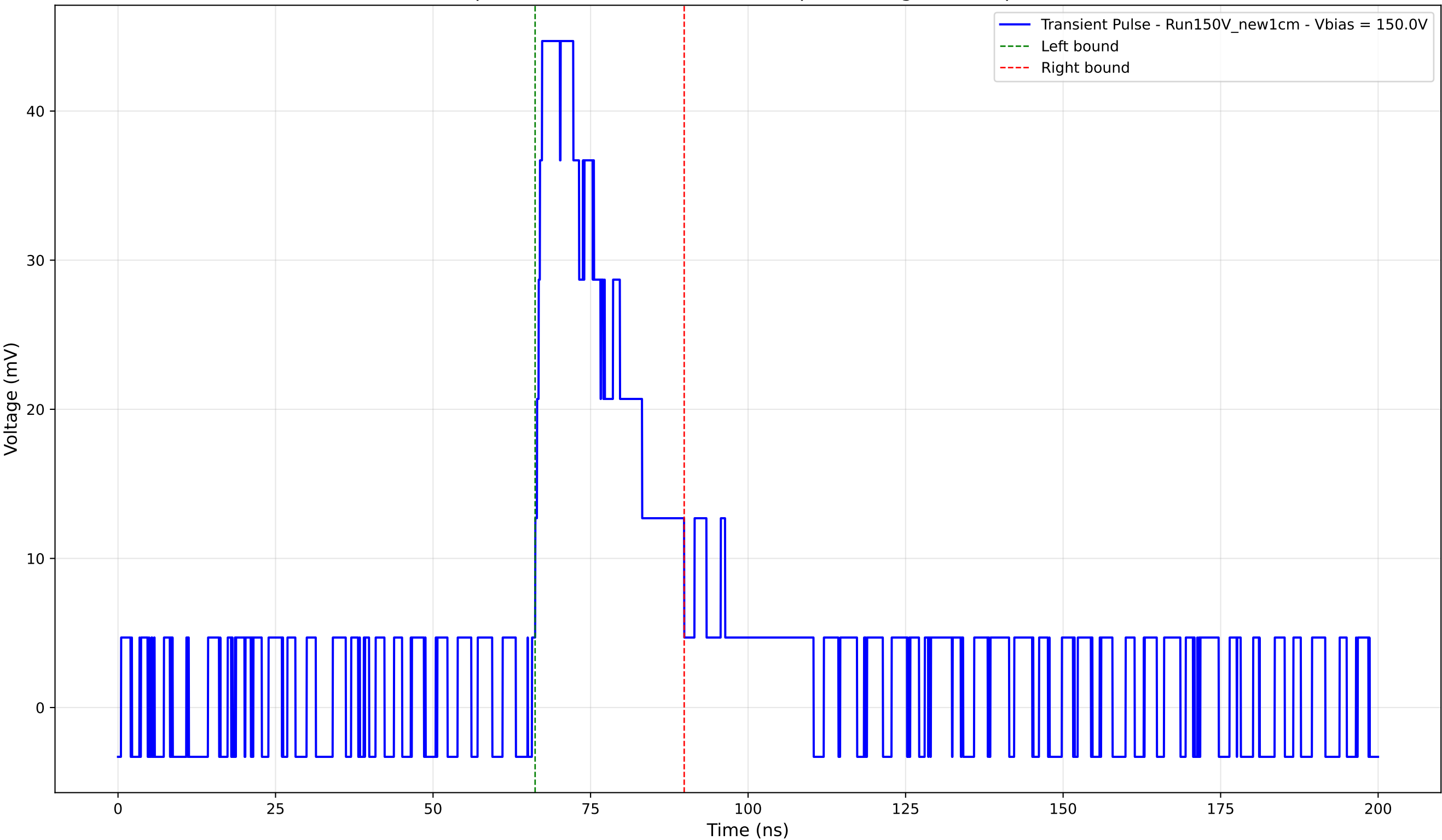
Transient Pulse - Sample: New1cm - Position: 1585.0 \mu\text{m} - Charge: 12.49 pC - Rise Time: 1.60 ns
