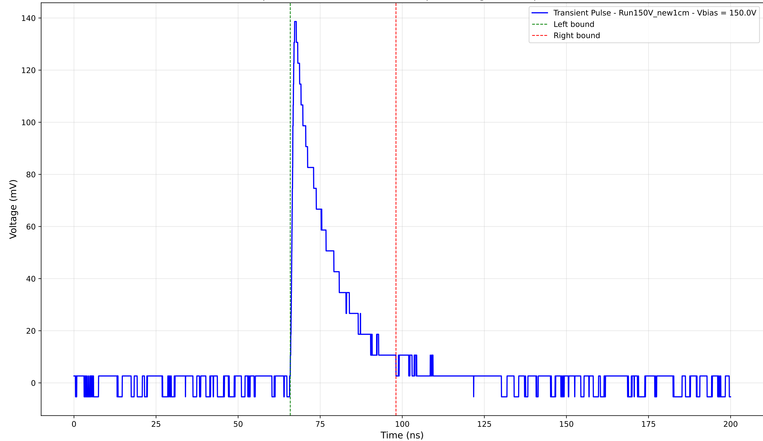
Transient Pulse - Sample: New1cm - Position: 335.0 \mu\text{m} - Charge: 29.36 pC - Rise Time: 1.01 ns
