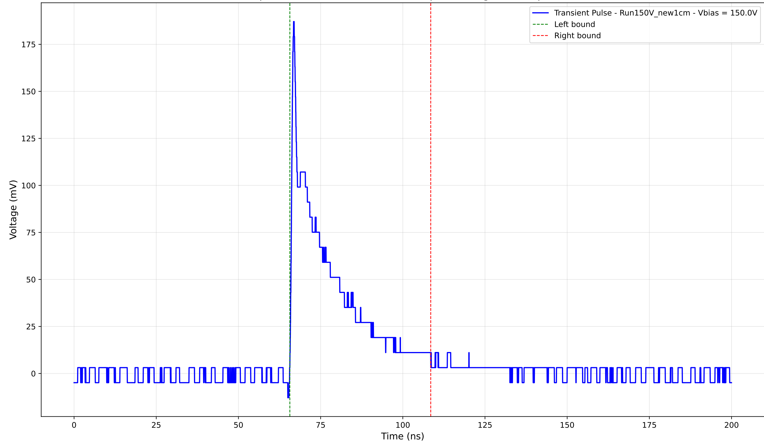
Transient Pulse - Sample: New1cm - Position: 2355.0 \mu\text{m} - Charge: 36.39 pC - Rise Time: 0.82 ns
