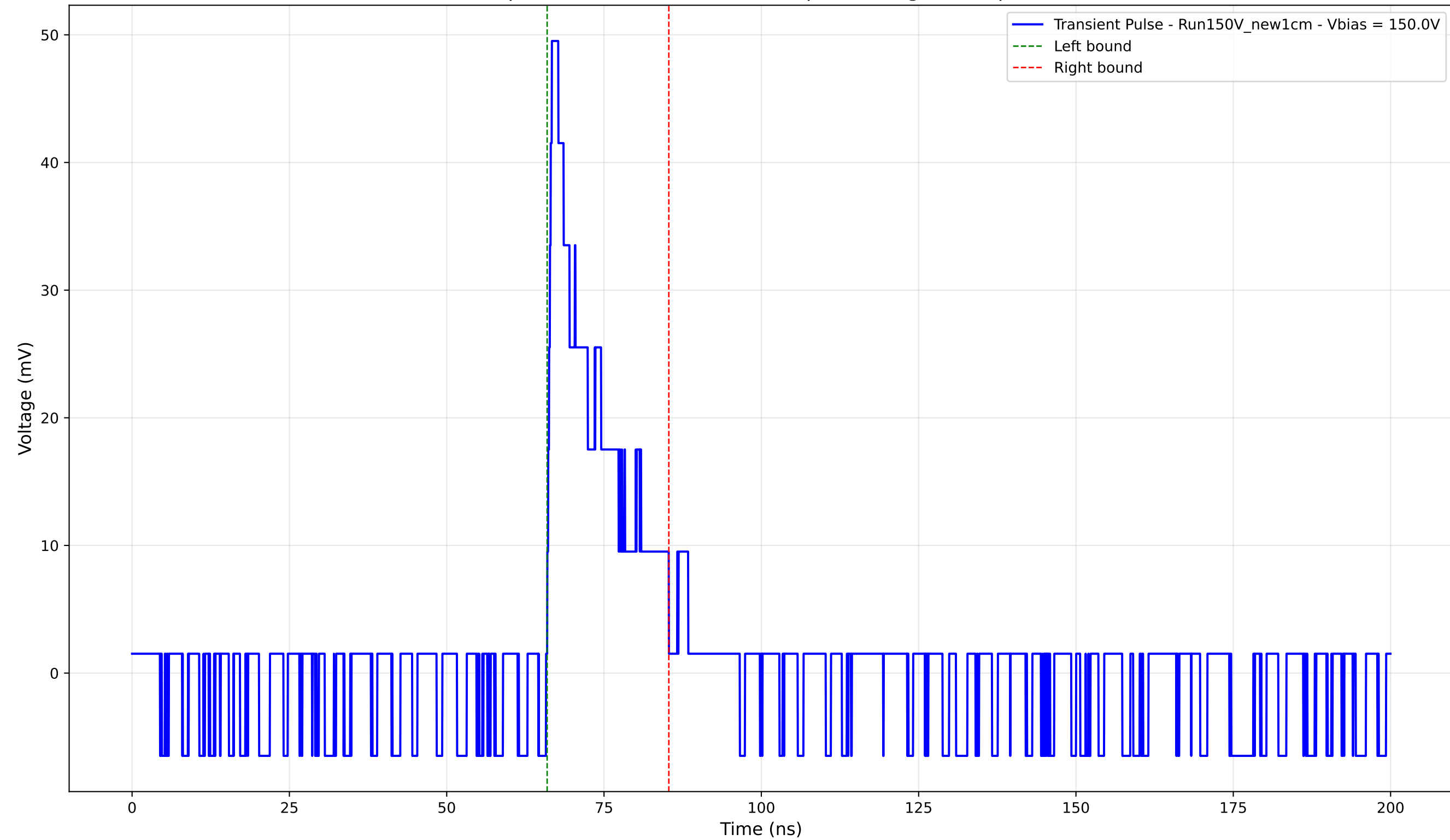
Transient Pulse - Sample: New1cm - Position: 70.0 \mu\text{m} - Charge: 7.79 pC - Rise Time: 0.73 ns
