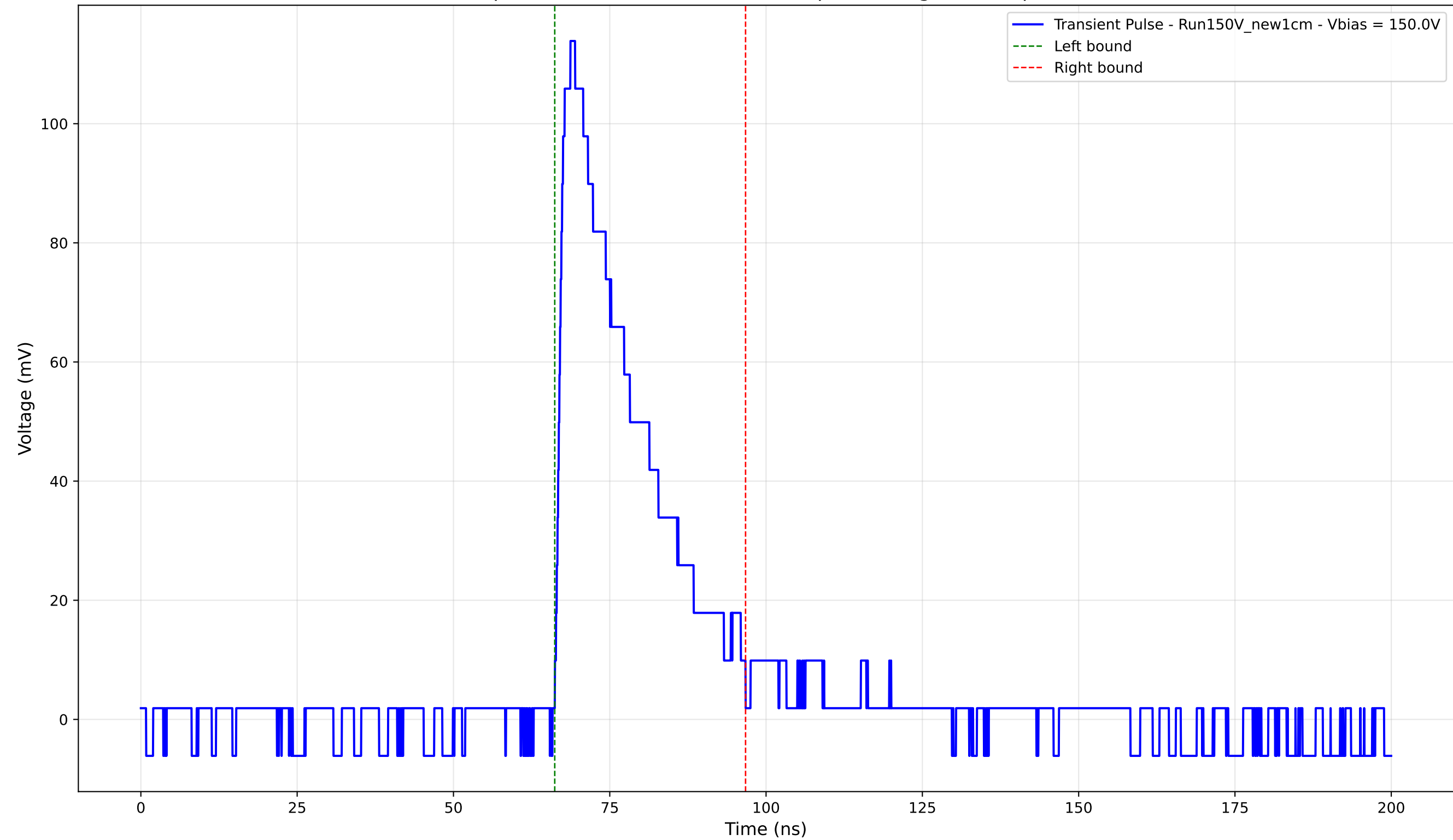
Transient Pulse - Sample: New1cm - Position: 1220.0 \mu\text{m} - Charge: 29.95 pC - Rise Time: 1.40 ns
