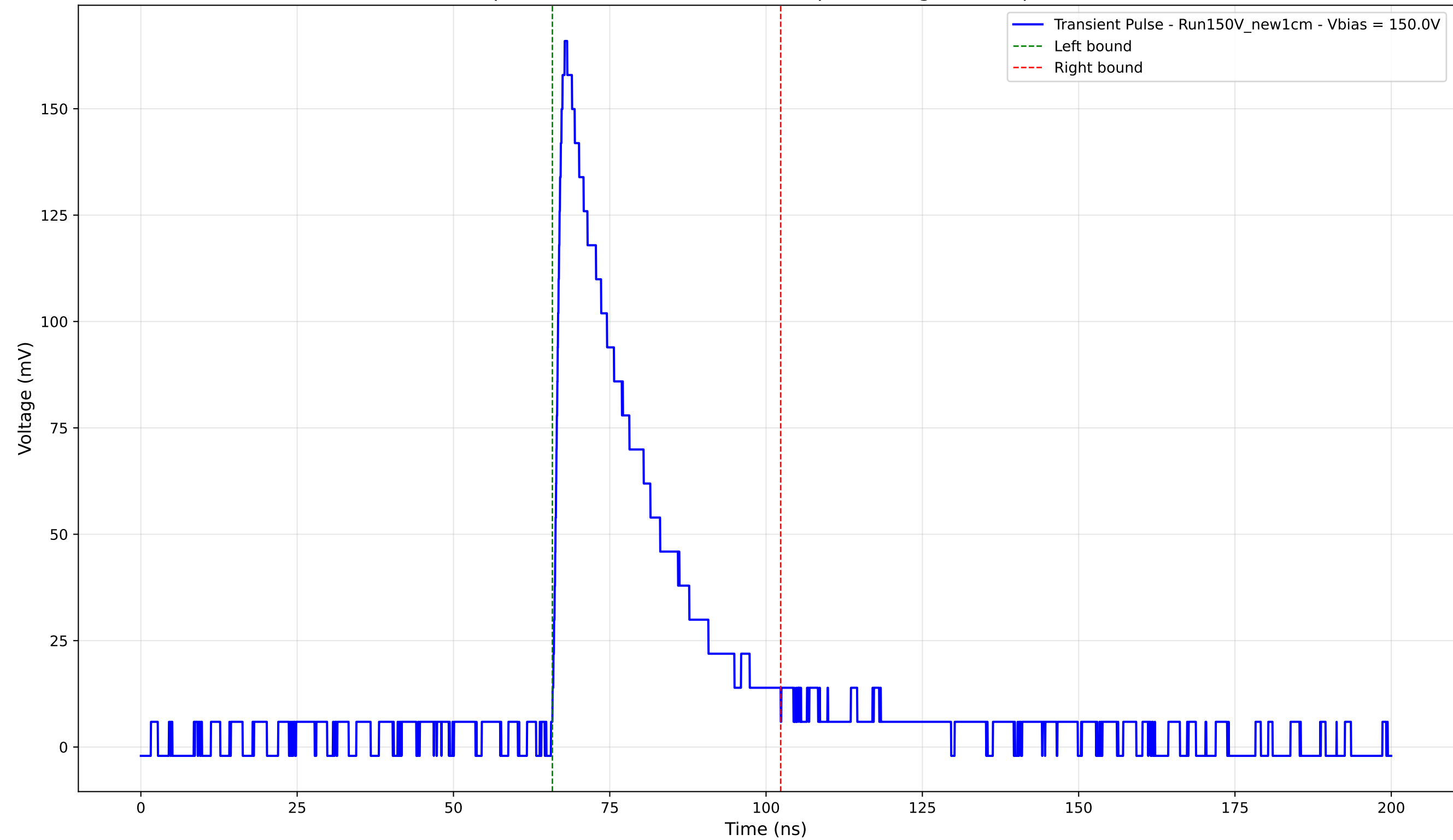
Transient Pulse - Sample: New1cm - Position: 4320.0 \mu\text{m} - Charge: 43.61 pC - Rise Time: 1.31 ns
