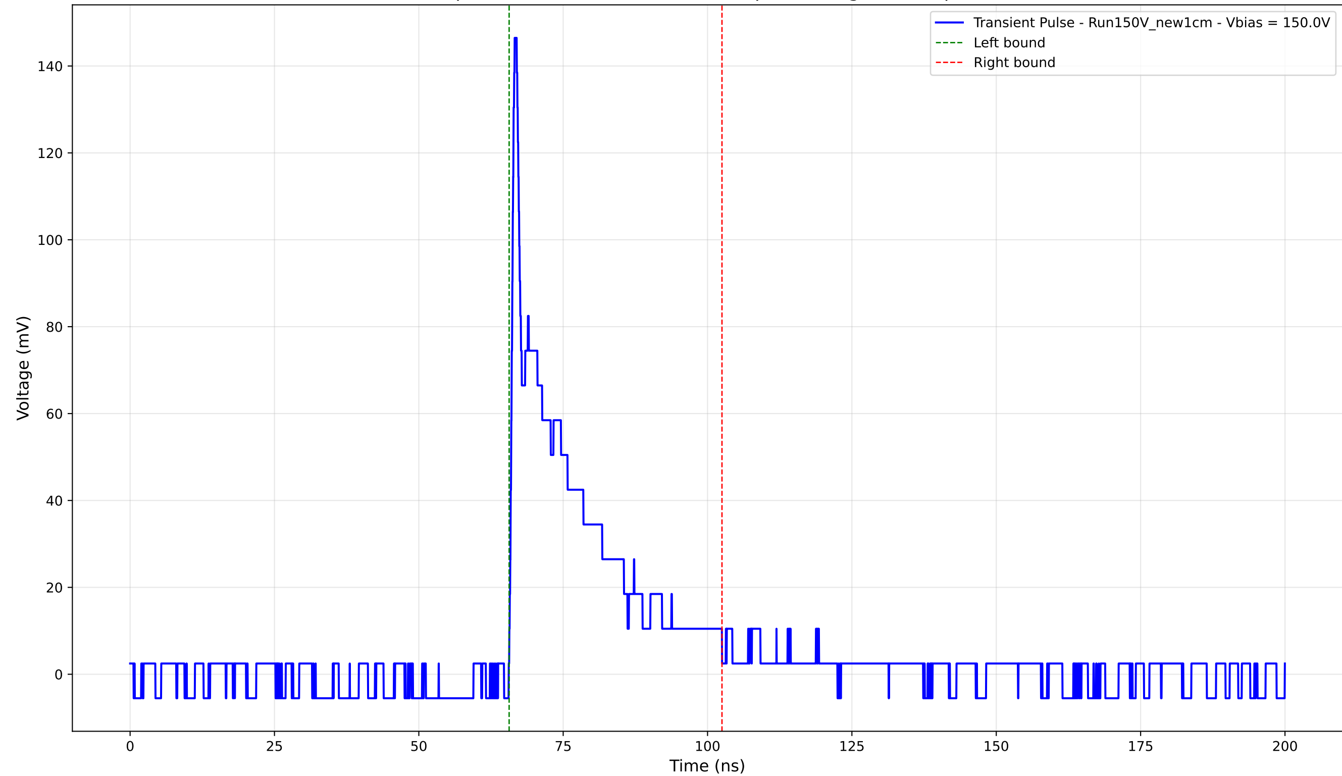
Transient Pulse - Sample: New1cm - Position: 2625.0 \mu\text{m} - Charge: 25.16 pC - Rise Time: 0.77 ns
