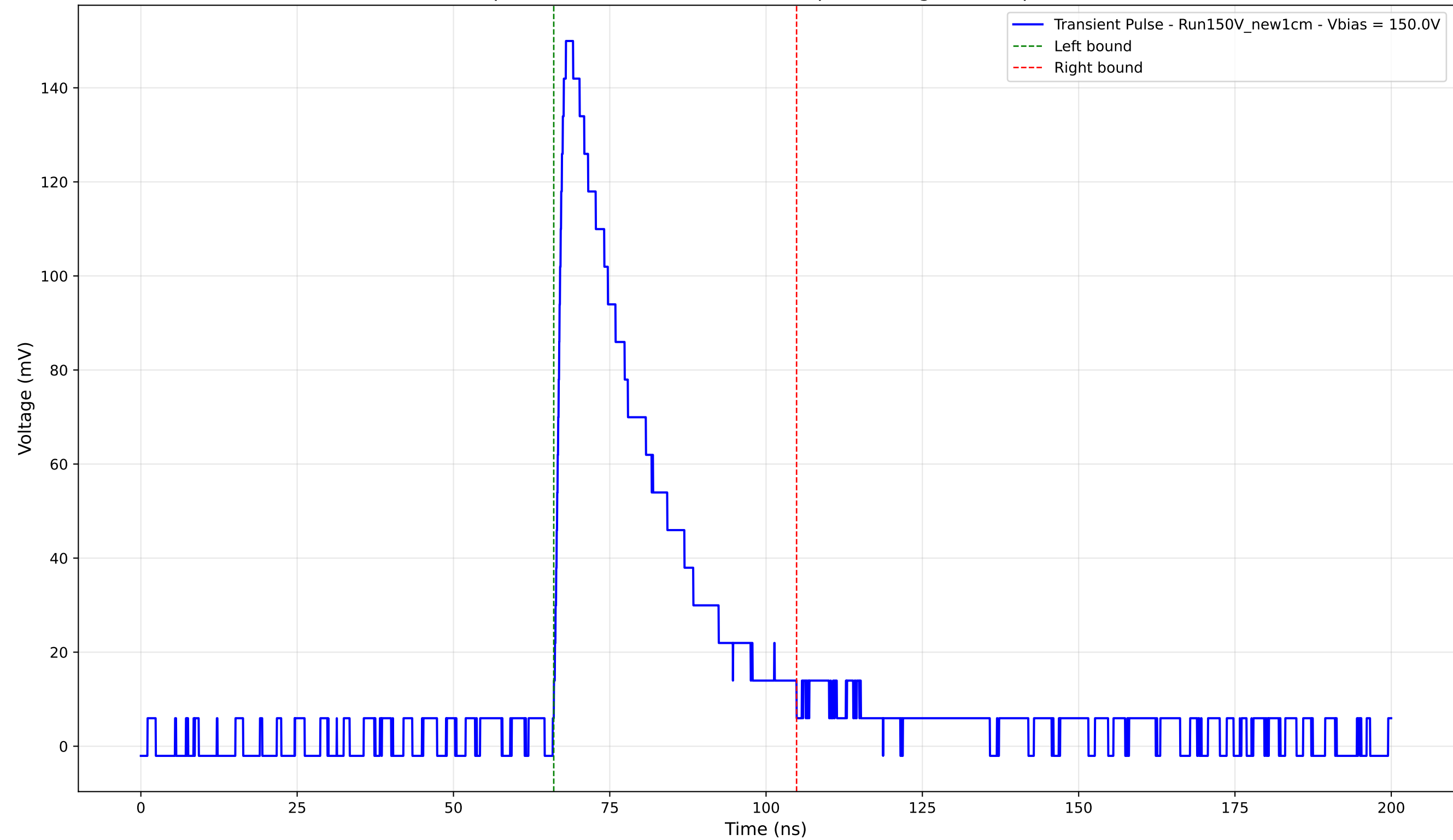
Transient Pulse - Sample: New1cm - Position: 3815.0 \mu\text{m} - Charge: 44.26 pC - Rise Time: 1.44 ns
