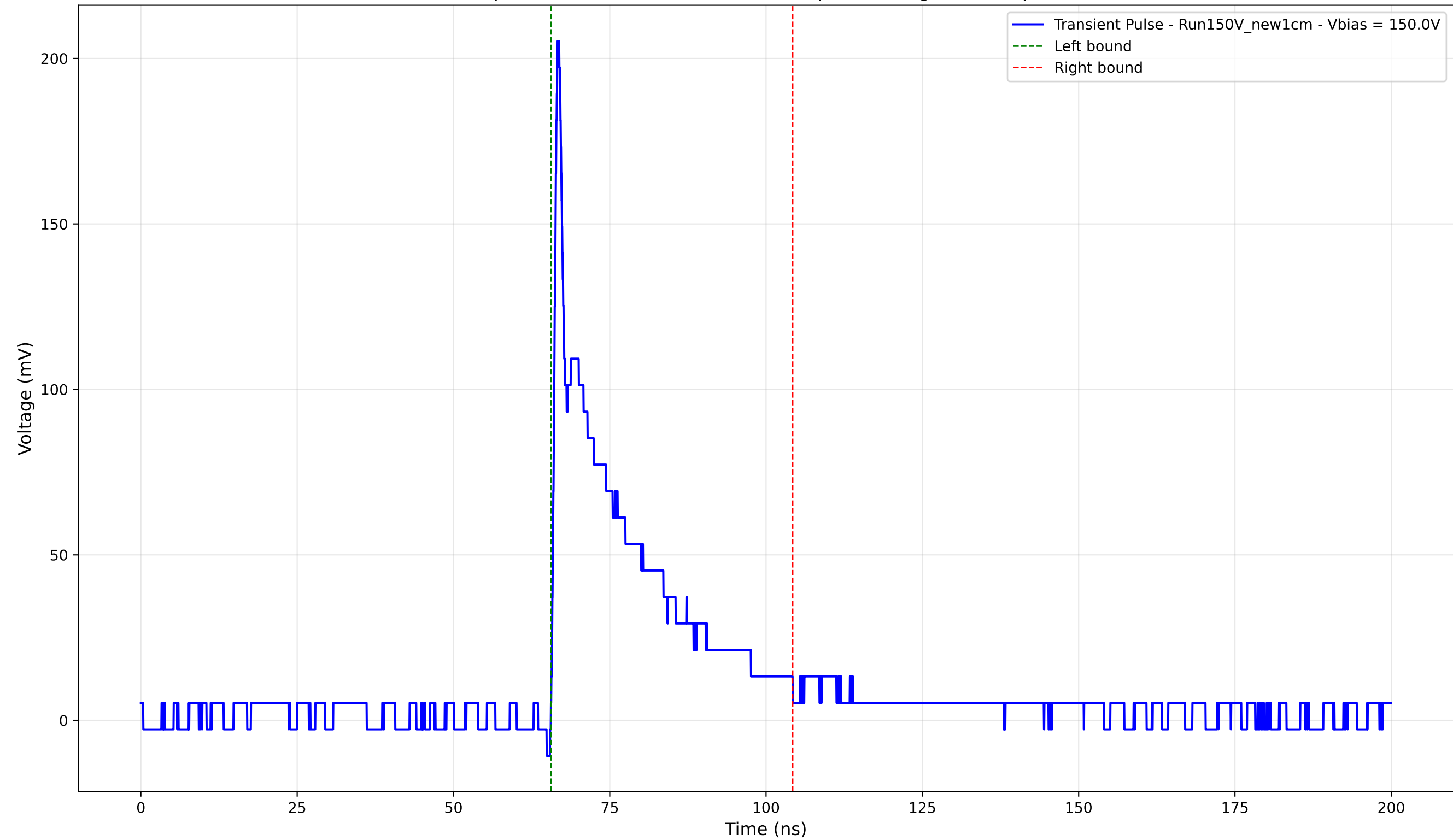
Transient Pulse - Sample: New1cm - Position: 2680.0 \mu\text{m} - Charge: 37.13 pC - Rise Time: 0.80 ns
