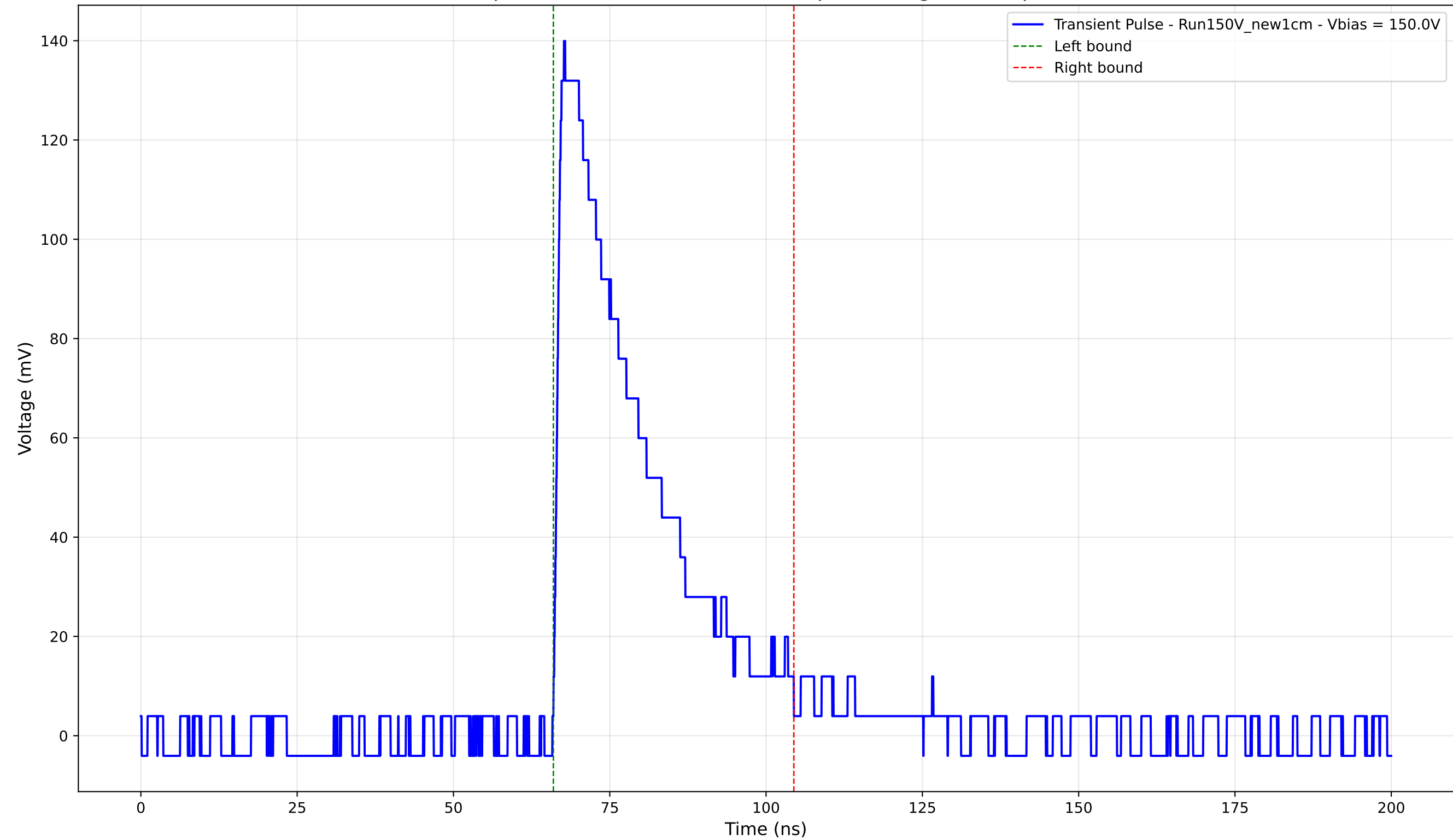
Transient Pulse - Sample: New1cm - Position: 3375.0 \mu\text{m} - Charge: 40.55 pC - Rise Time: 1.17 ns
