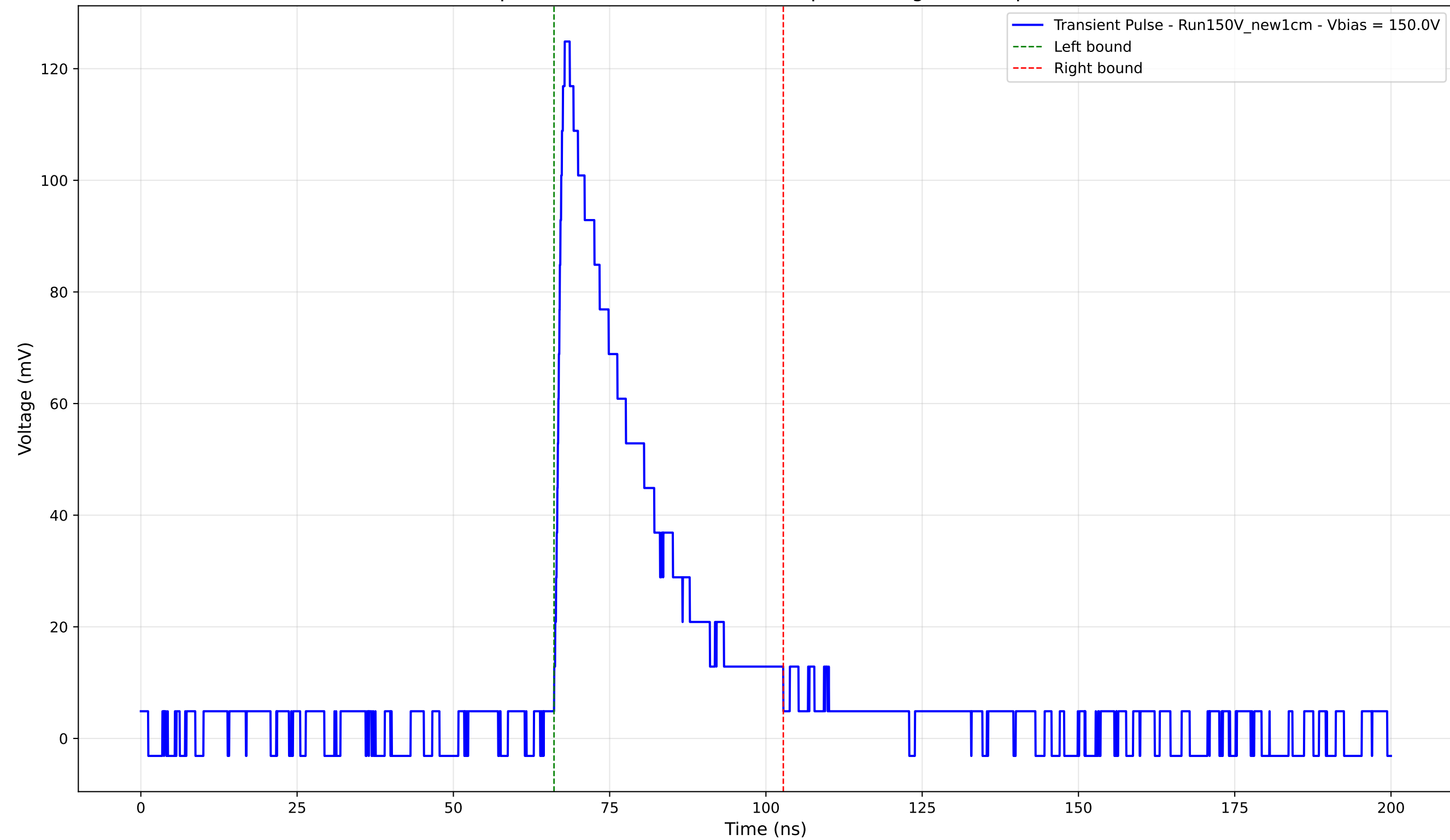
Transient Pulse - Sample: New1cm - Position: 740.0 \mu\text{m} - Charge: 32.47 pC - Rise Time: 1.40 ns
