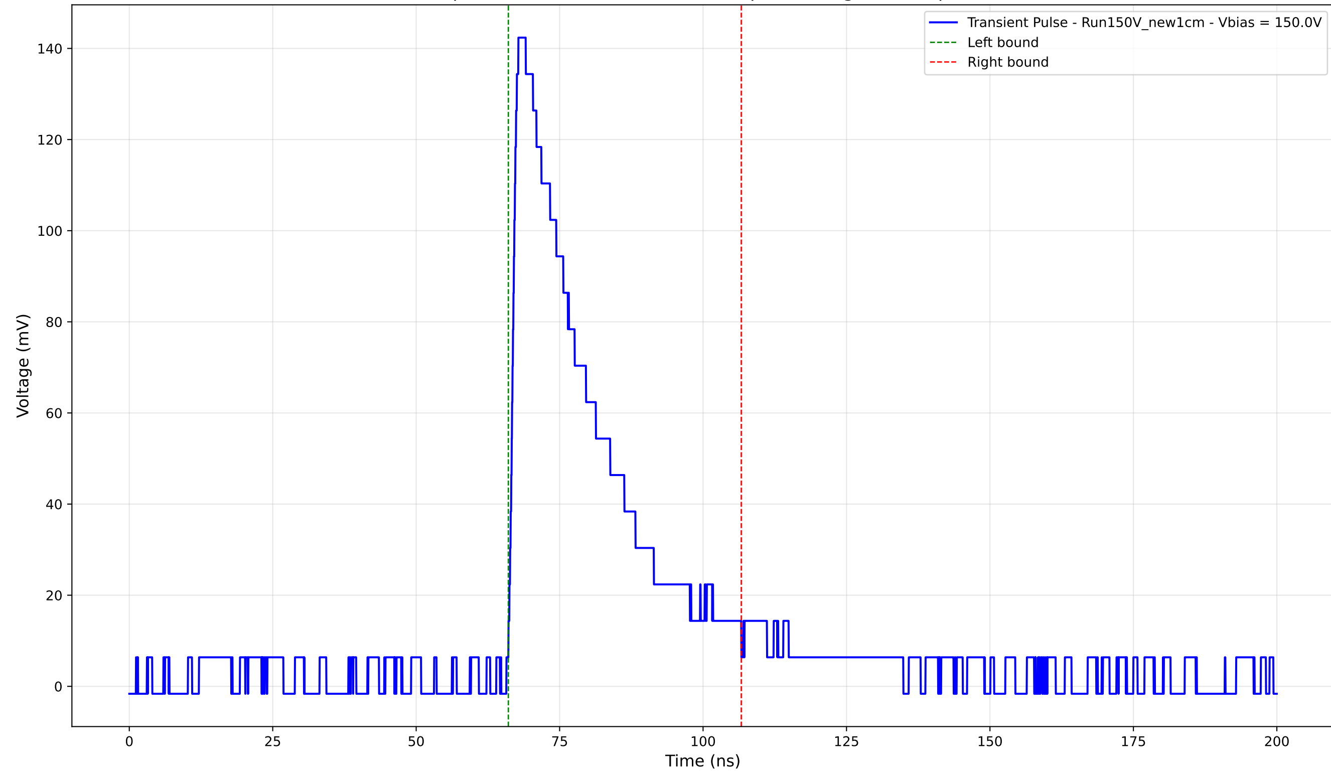
Transient Pulse - Sample: New1cm - Position: 3730.0 \mu\text{m} - Charge: 43.47 pC - Rise Time: 1.46 ns
