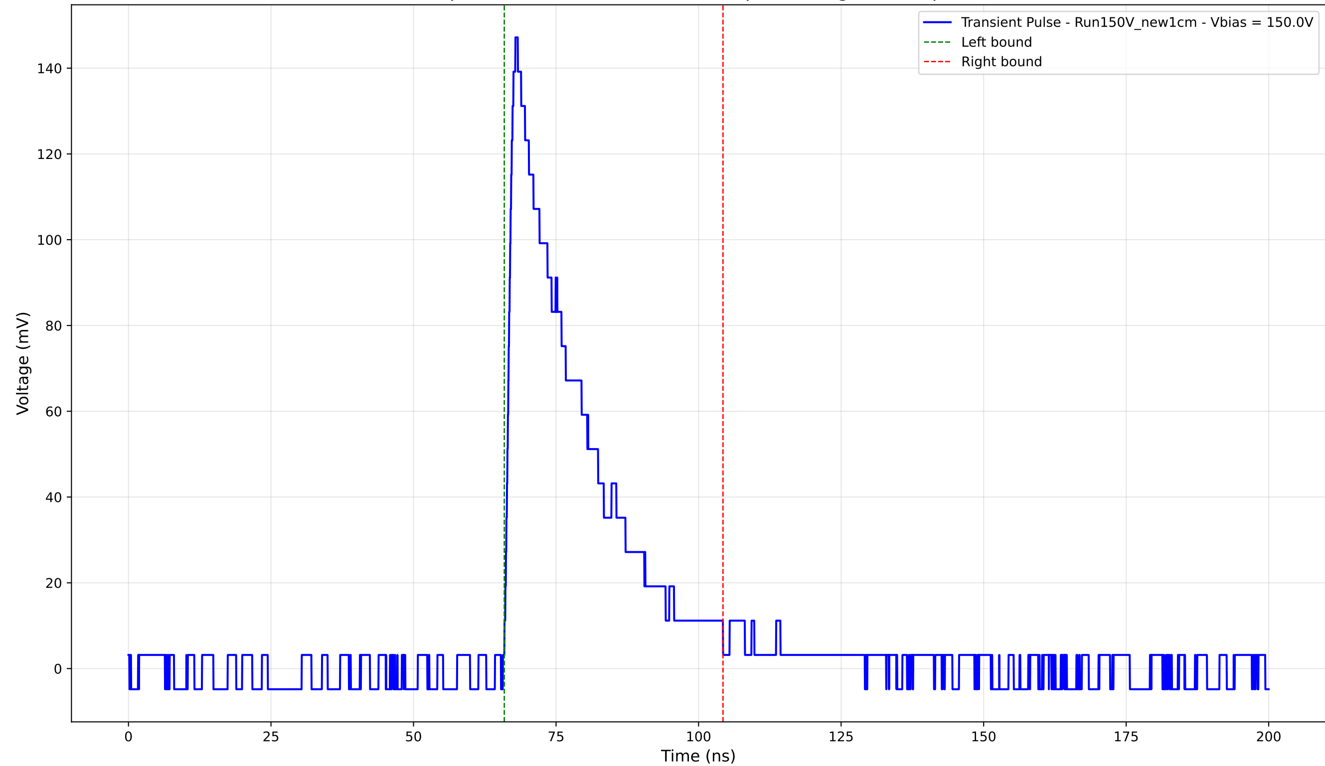
Transient Pulse - Sample: New1cm - Position: 4230.0 \mu\text{m} - Charge: 38.04 pC - Rise Time: 1.43 ns
