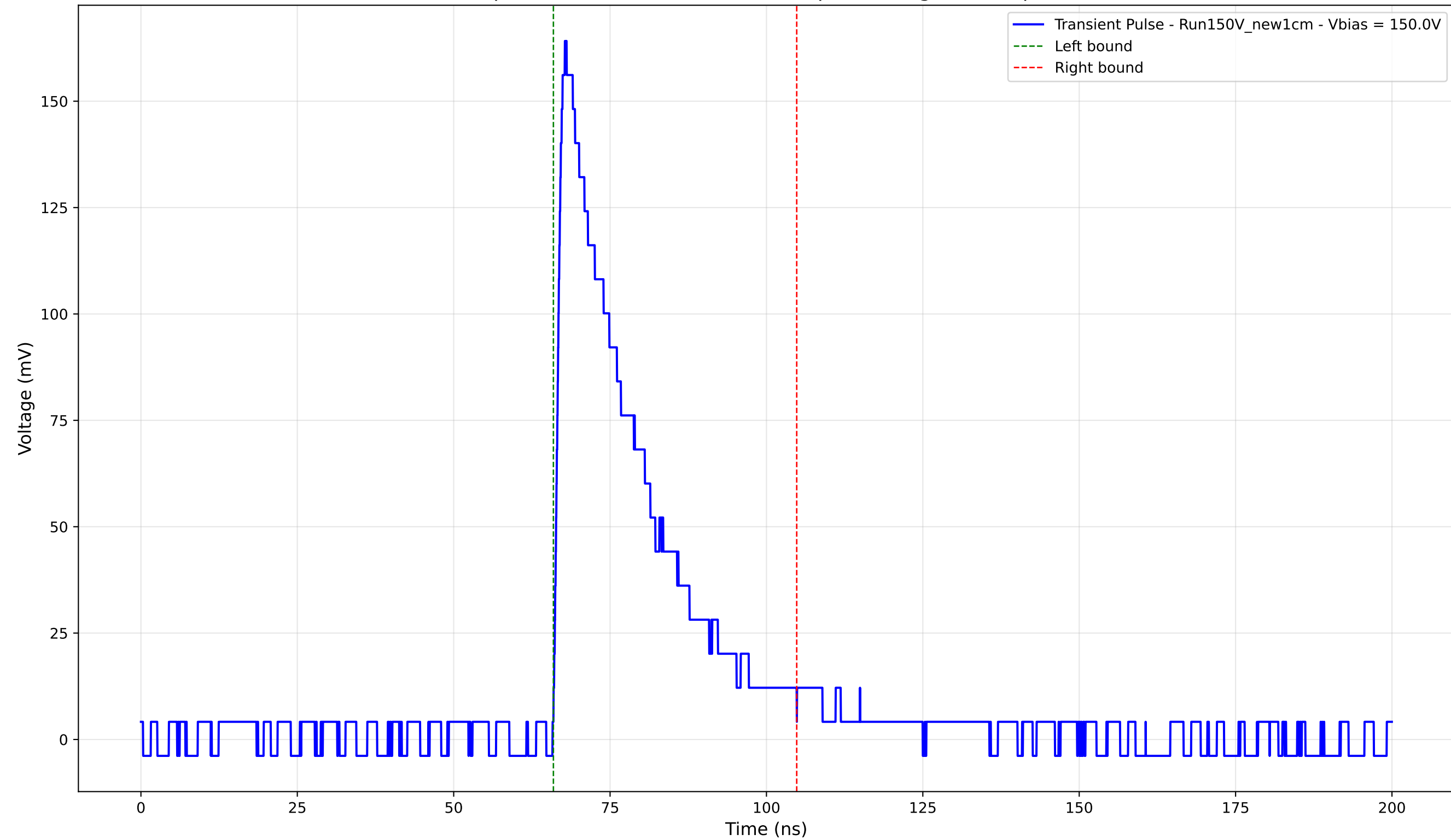
Transient Pulse - Sample: New1cm - Position: 4315.0 \mu\text{m} - Charge: 43.19 pC - Rise Time: 1.21 ns
