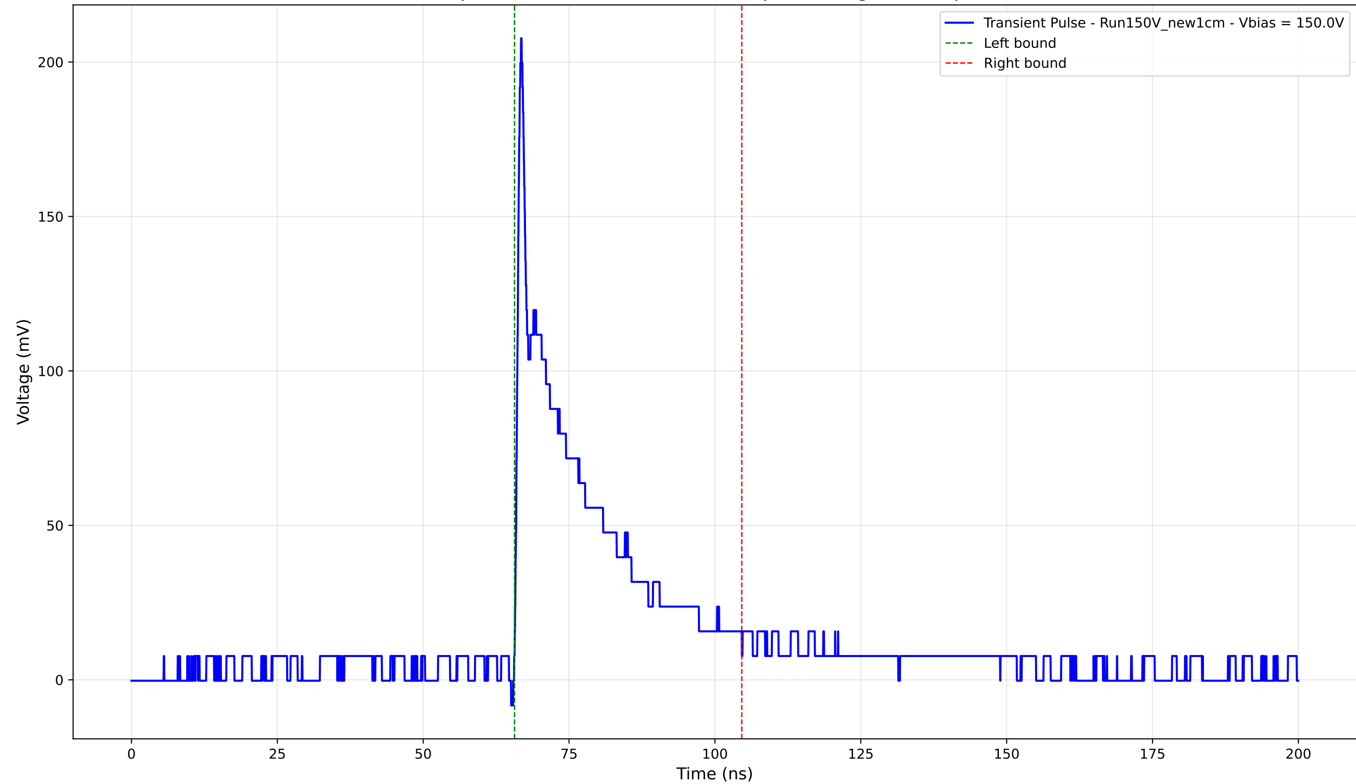
Transient Pulse - Sample: New1cm - Position: 2710.0 \mu\text{m} - Charge: 39.73 pC - Rise Time: 0.83 ns
