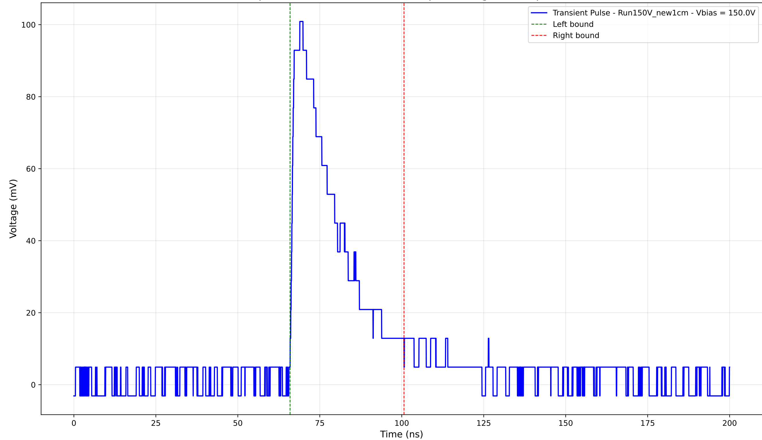
Transient Pulse - Sample: New1cm - Position: 1770.0 \mu\text{m} - Charge: 30.04 pC - Rise Time: 1.23 ns
