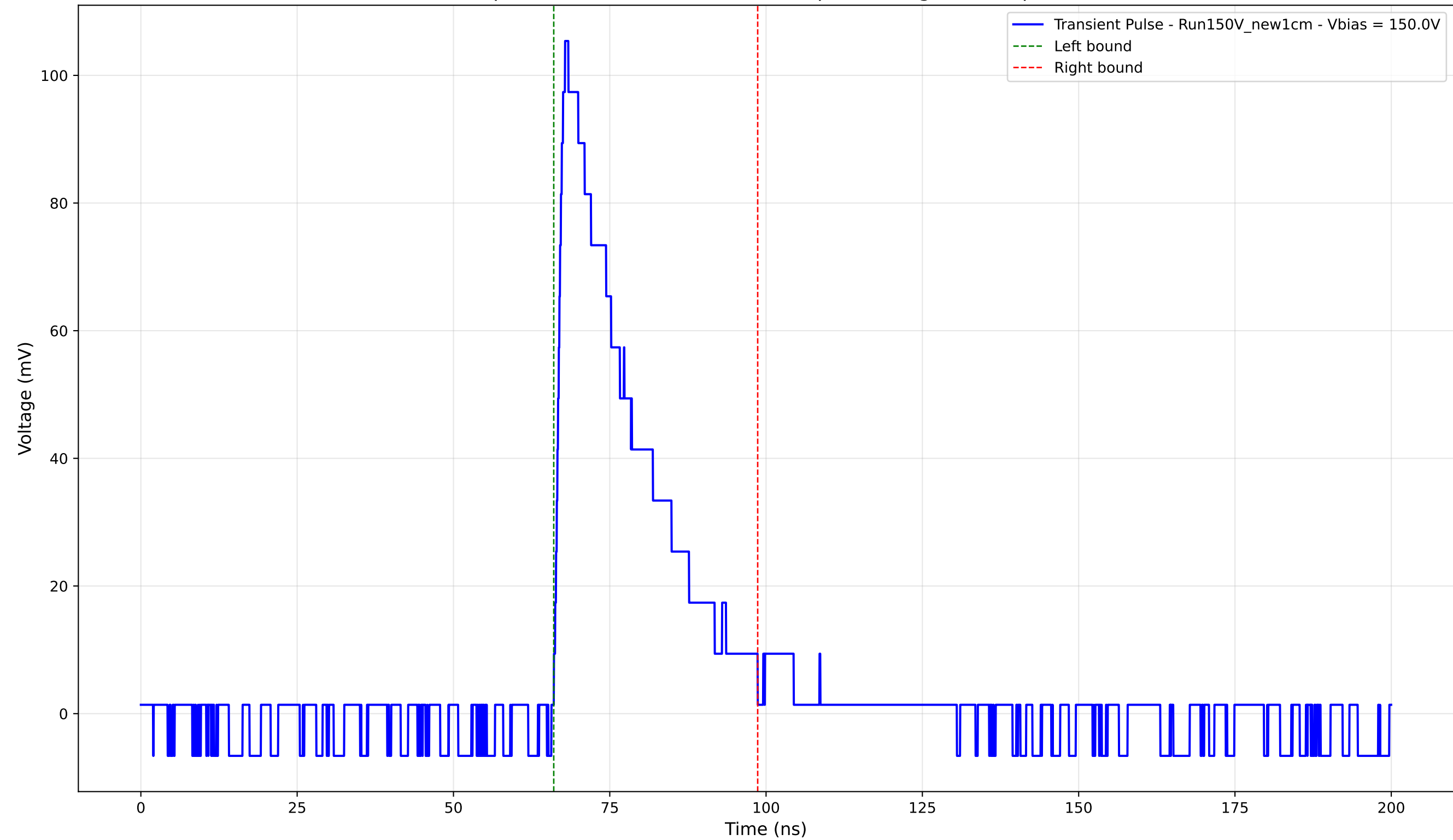
Transient Pulse - Sample: New1cm - Position: 3995.0 \mu\text{m} - Charge: 26.90 pC - Rise Time: 1.28 ns
