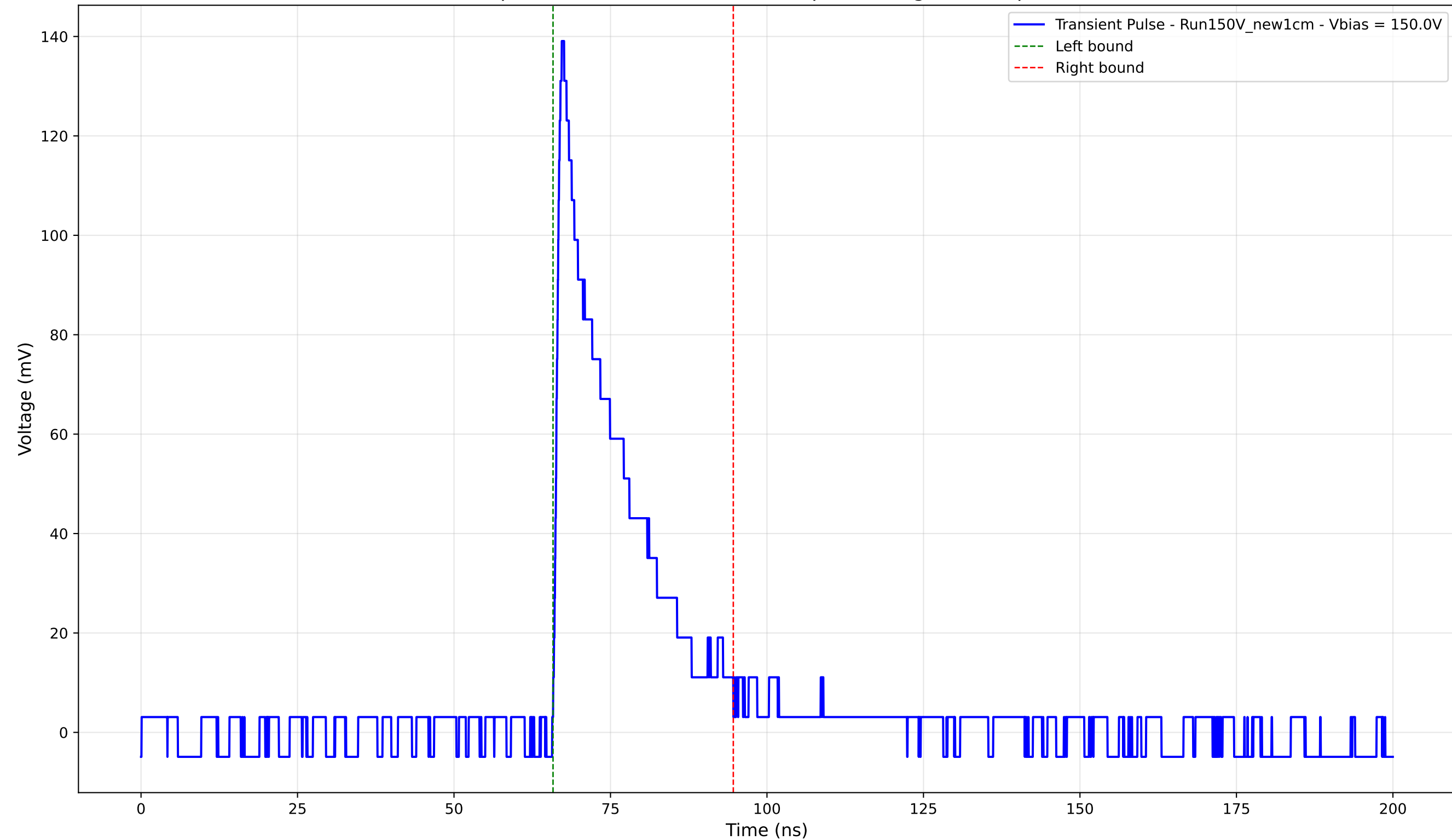
Transient Pulse - Sample: New1cm - Position: 265.0 \mu\text{m} - Charge: 27.53 pC - Rise Time: 1.05 ns
