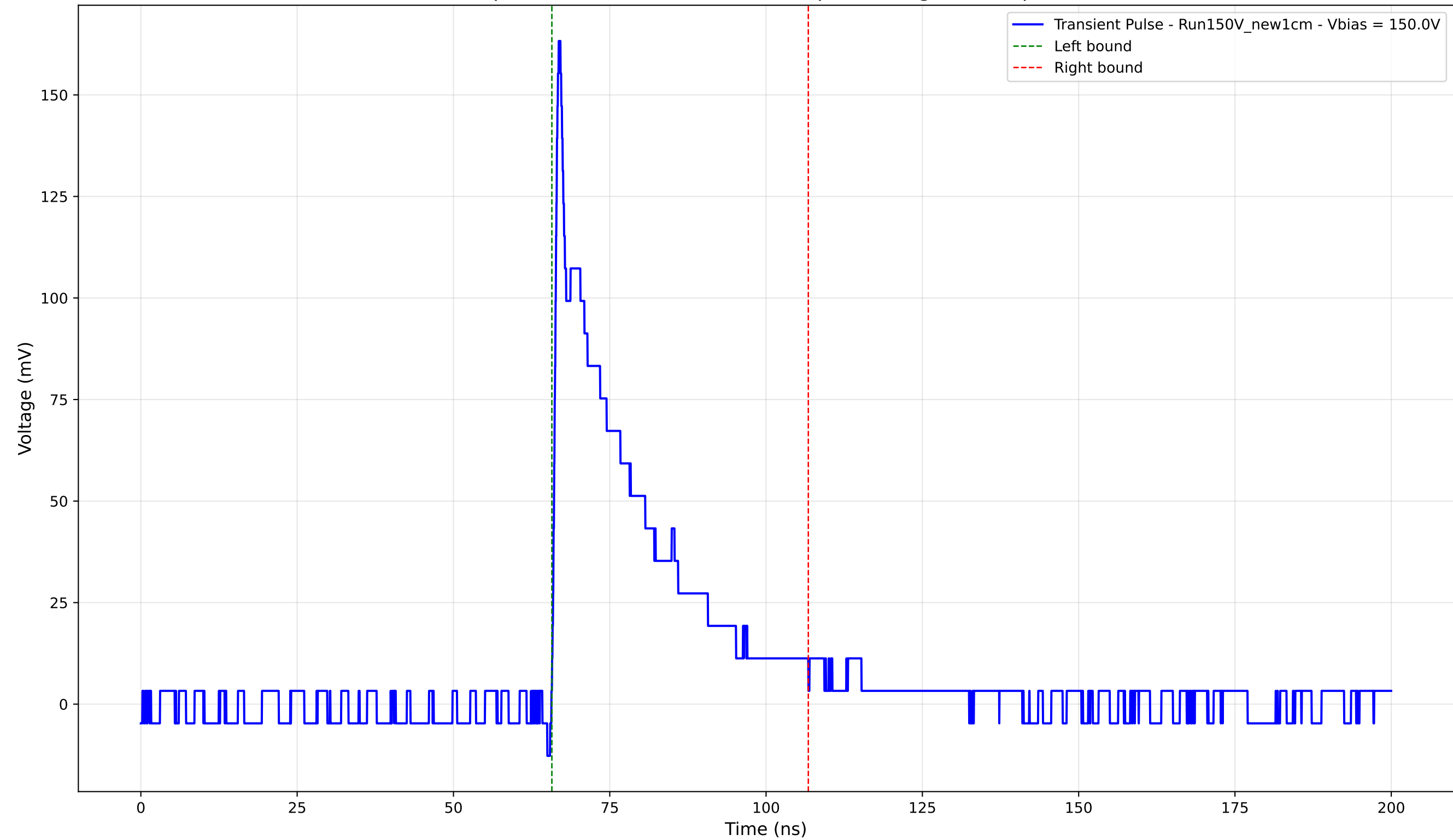
Transient Pulse - Sample: New1cm - Position: 2240.0 \mu\text{m} - Charge: 35.37 pC - Rise Time: 0.79 ns
