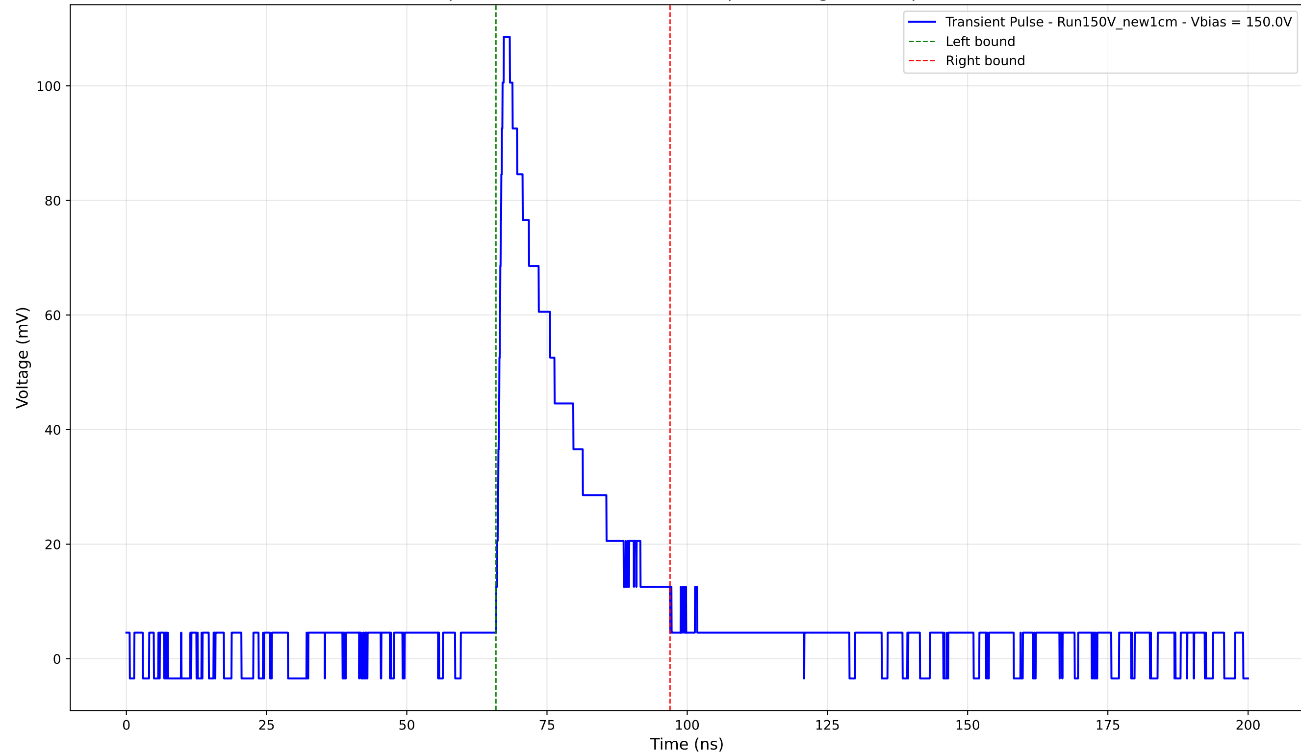
Transient Pulse - Sample: New1cm - Position: 440.0 \mu\text{m} - Charge: 25.81 pC - Rise Time: 1.14 ns
