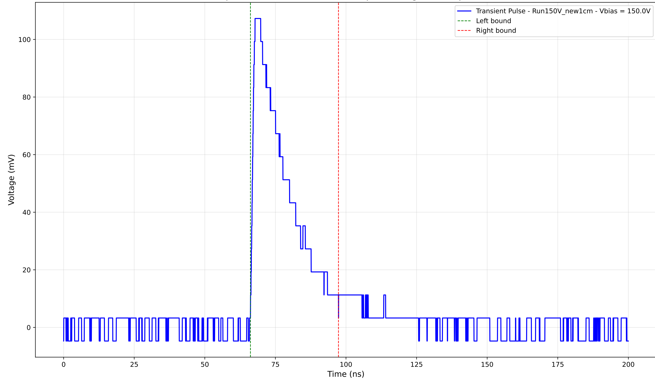
Transient Pulse - Sample: New1cm - Position: 925.0 \mu\text{m} - Charge: 29.19 pC - Rise Time: 1.36 ns
