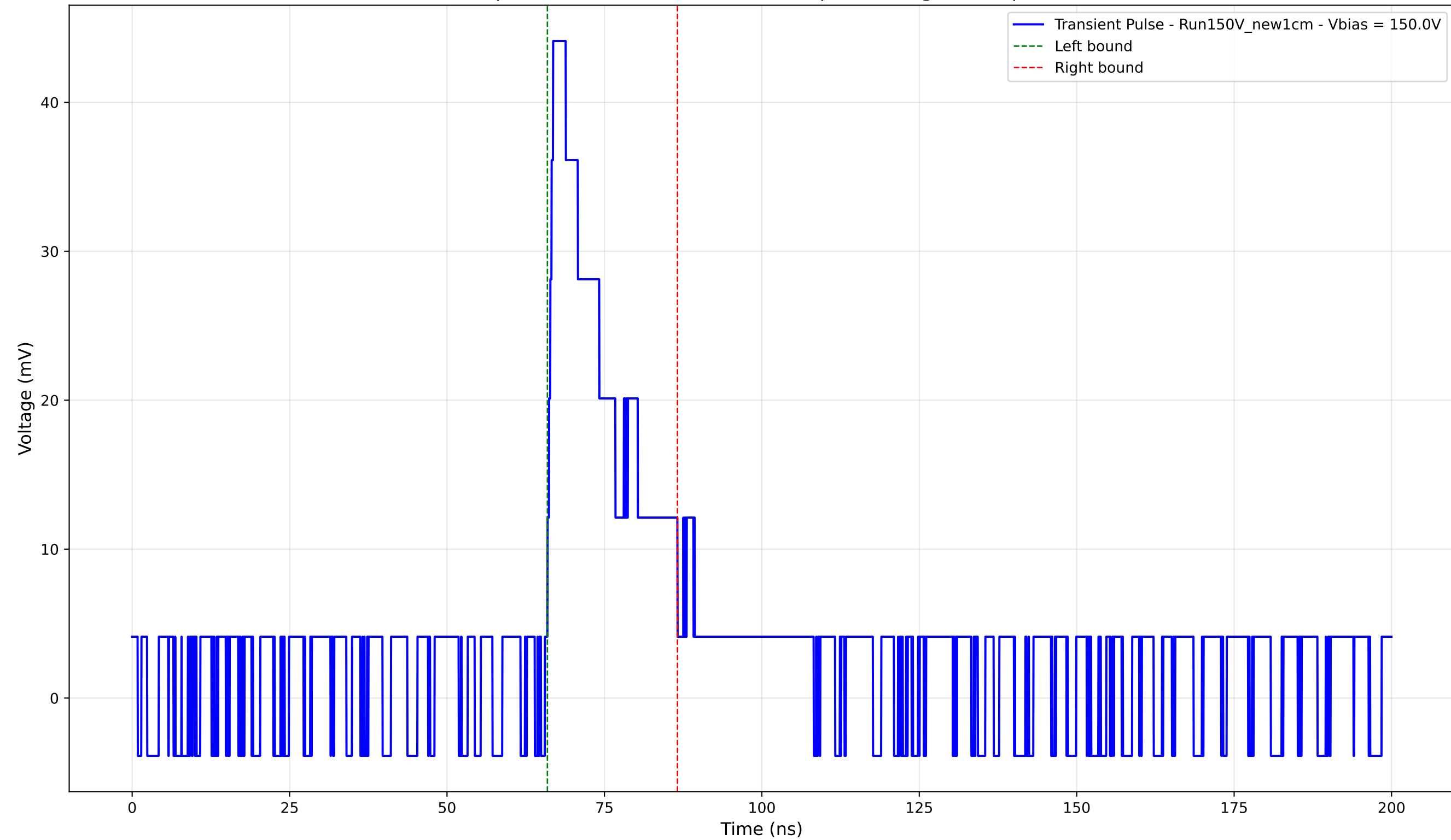
Transient Pulse - Sample: New1cm - Position: 4600.0 \mu\text{m} - Charge: 9.23 pC - Rise Time: 0.90 ns
