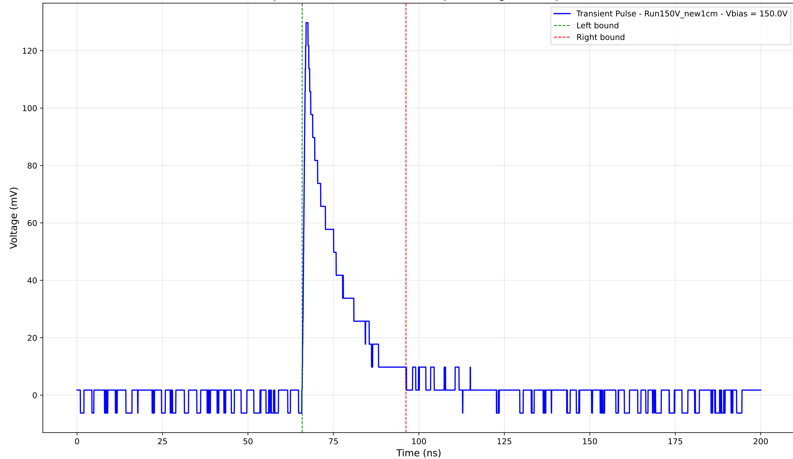
Transient Pulse - Sample: New1cm - Position: 175.0 \mu\text{m} - Charge: 23.67 pC - Rise Time: 0.91 ns
