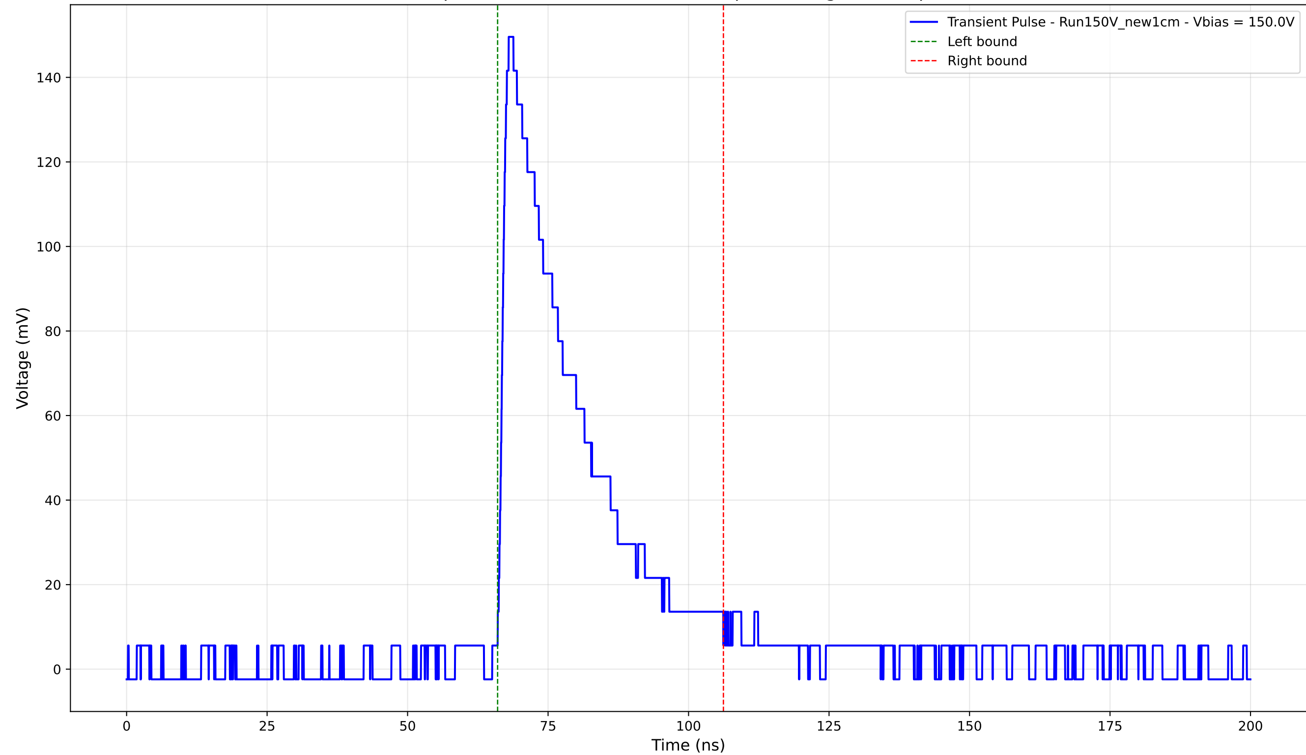
Transient Pulse - Sample: New1cm - Position: 3930.0 \mu\text{m} - Charge: 42.54 pC - Rise Time: 1.46 ns
