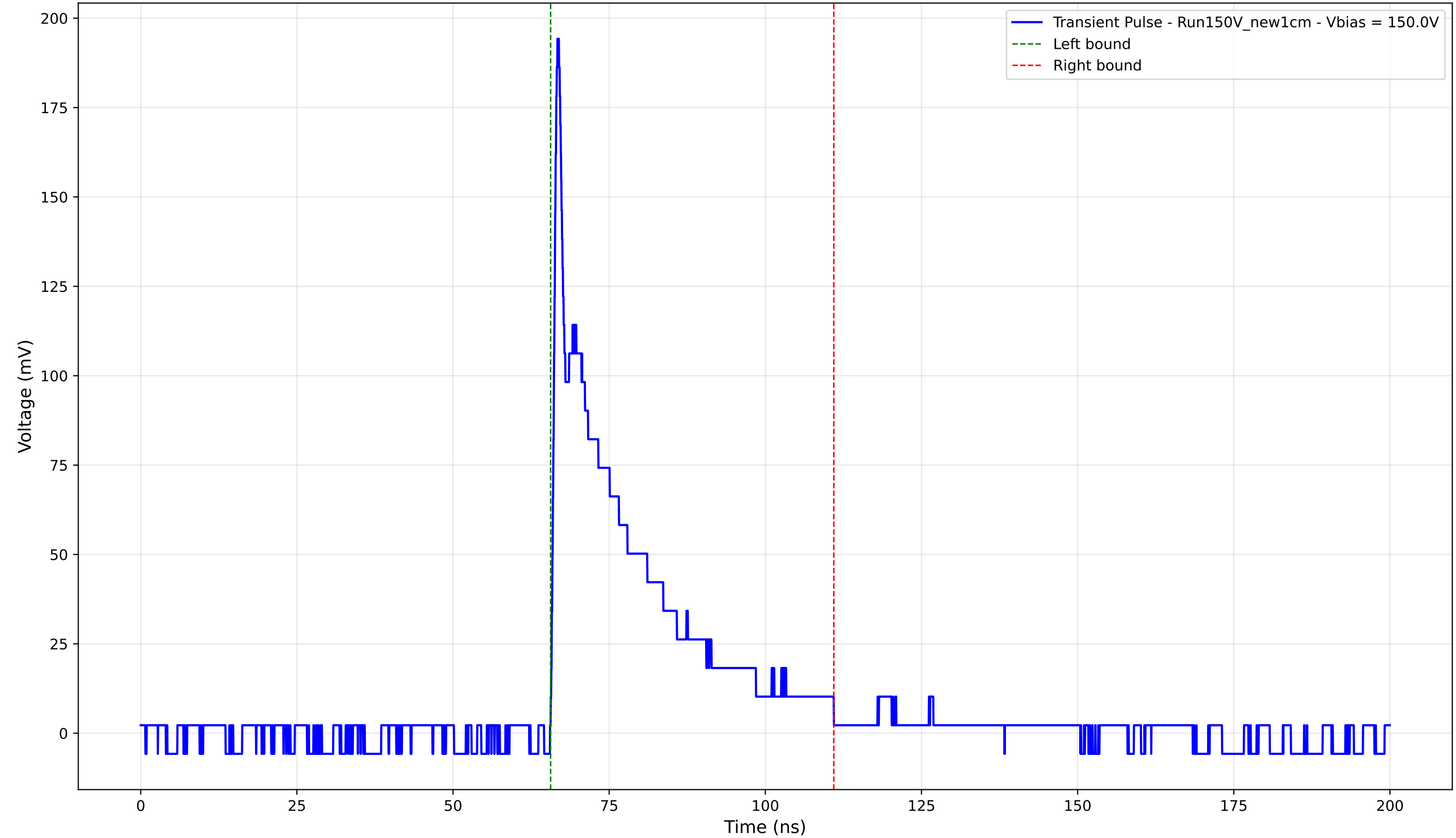
Transient Pulse - Sample: New1cm - Position: 2720.0 \mu\text{m} - Charge: 37.42 pC - Rise Time: 0.78 ns
