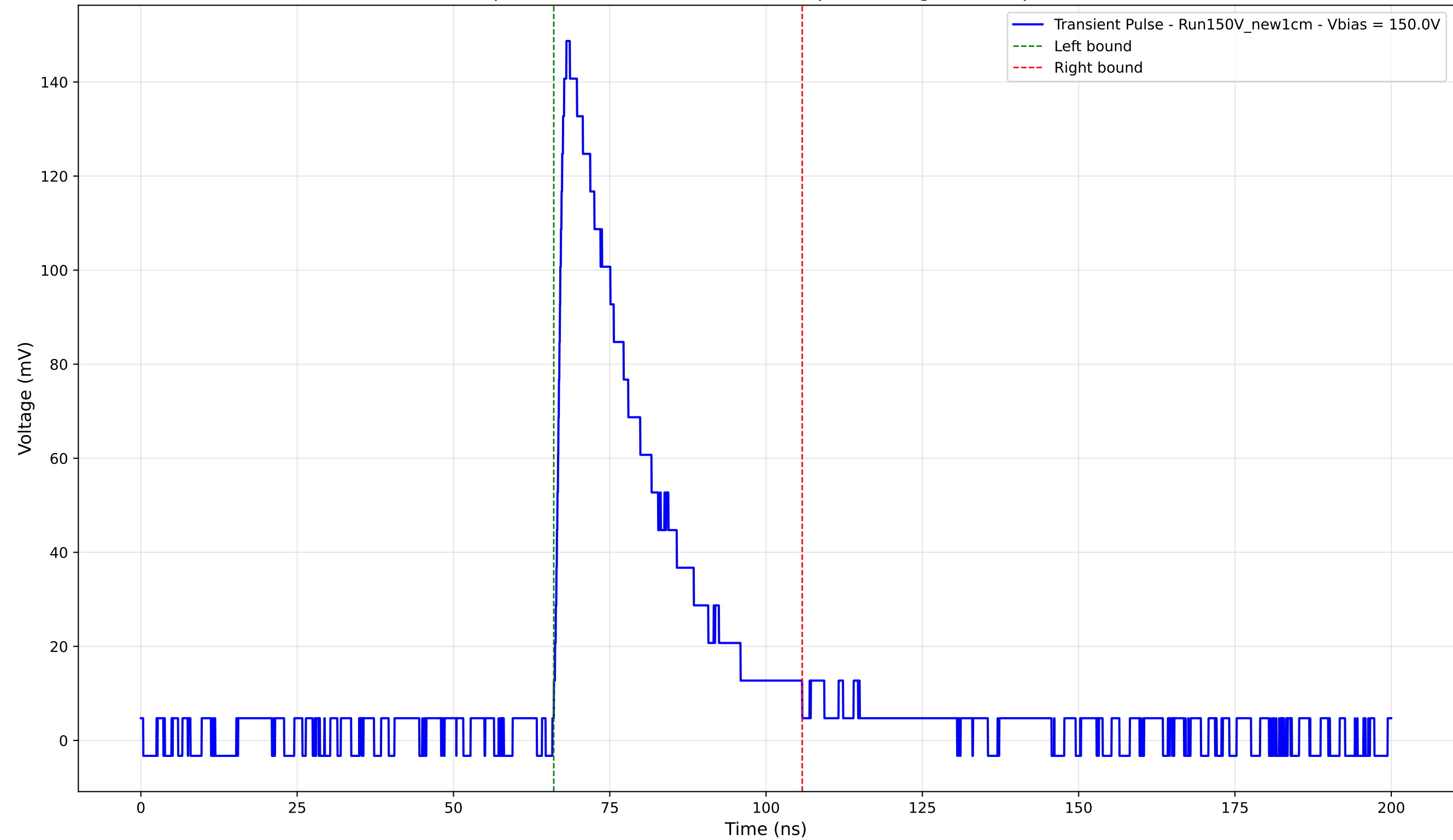
Transient Pulse - Sample: New1cm - Position: 3785.0 \mu\text{m} - Charge: 42.21 pC - Rise Time: 1.47 ns
