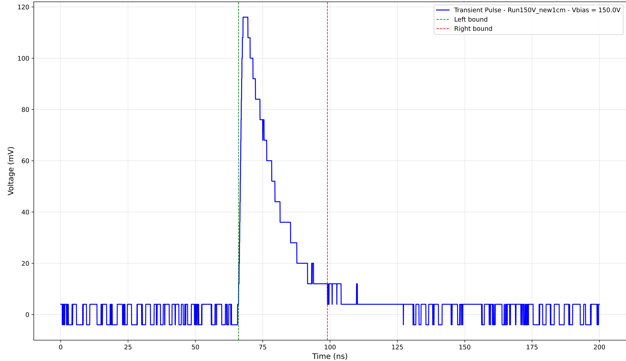
Transient Pulse - Sample: New1cm - Position: 795.0 \mu\text{m} - Charge: 31.05 pC - Rise Time: 1.40 ns
