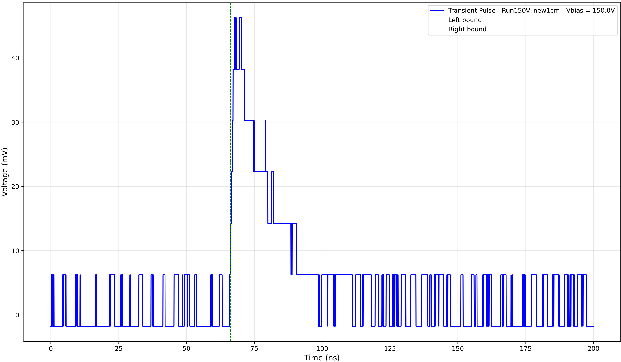
Transient Pulse - Sample: New1cm - Position: 4035.0 \mu\text{m} - Charge: 10.71 pC - Rise Time: 1.95 ns
