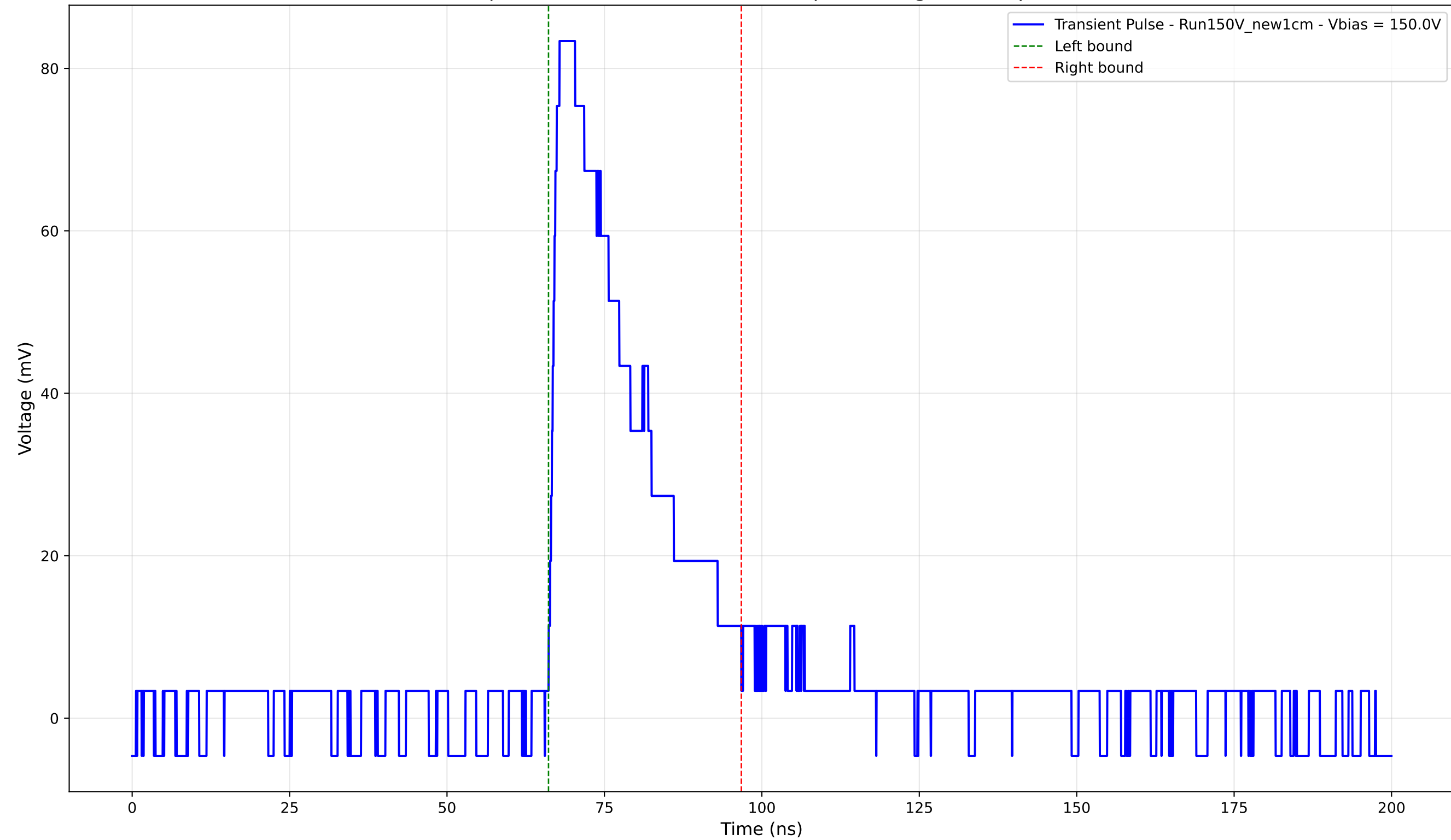
Transient Pulse - Sample: New1cm - Position: 1465.0 \mu\text{m} - Charge: 24.25 pC - Rise Time: 1.29 ns
