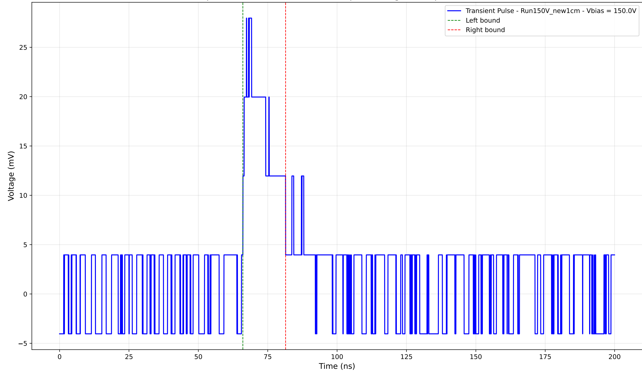
Transient Pulse - Sample: New1cm - Position: 4560.0 \mu\text{m} - Charge: 5.12 pC - Rise Time: 0.00 ns (N/A)
