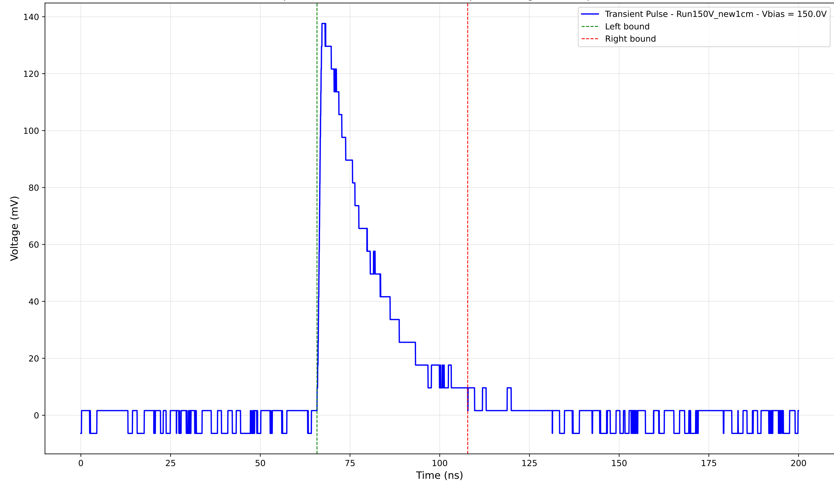
Transient Pulse - Sample: New1cm - Position: 3260.0 \mu\text{m} - Charge: 40.77 pC - Rise Time: 1.07 ns
