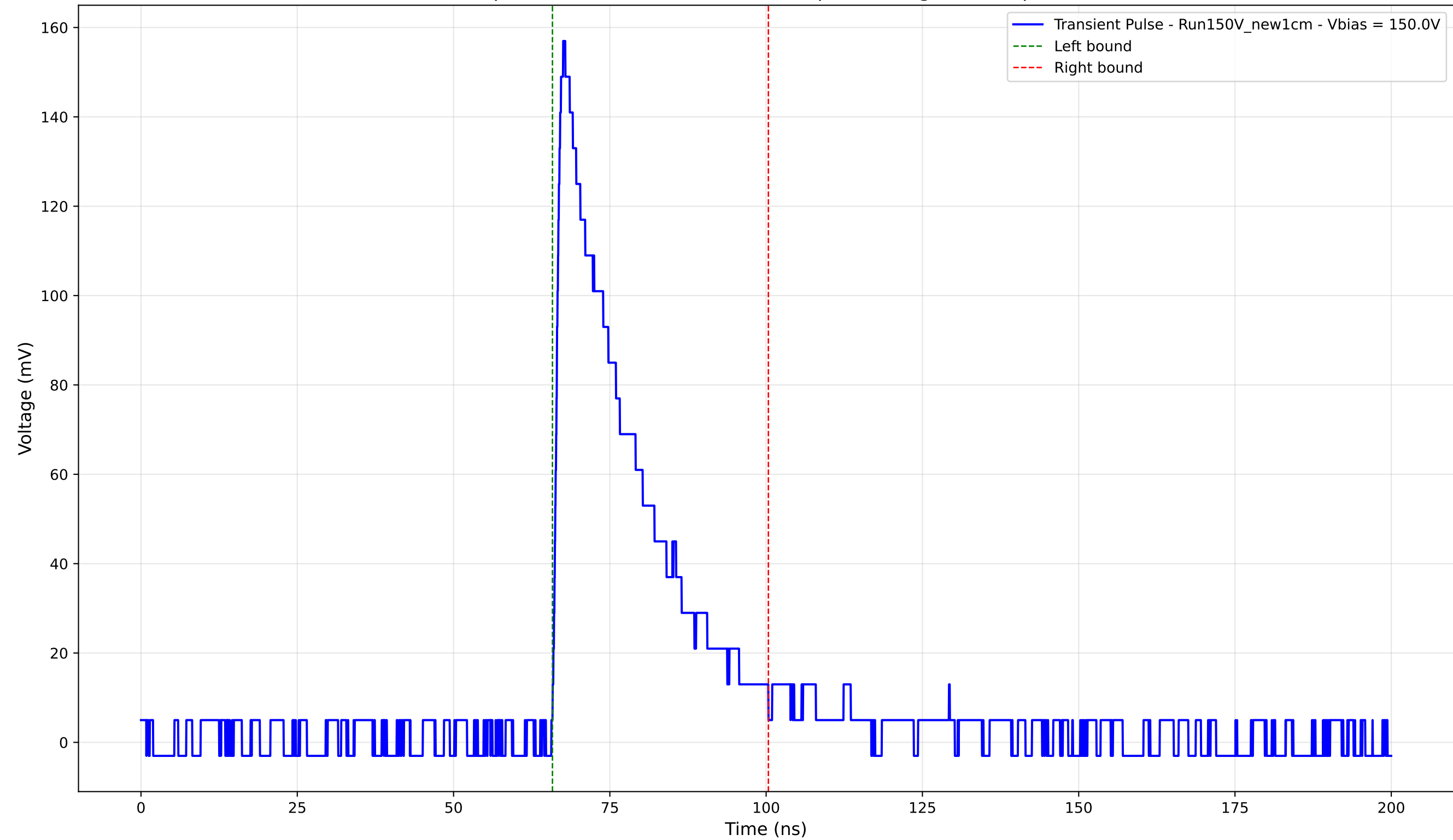
Transient Pulse - Sample: New1cm - Position: 4445.0 \mu\text{m} - Charge: 39.35 pC - Rise Time: 1.23 ns
