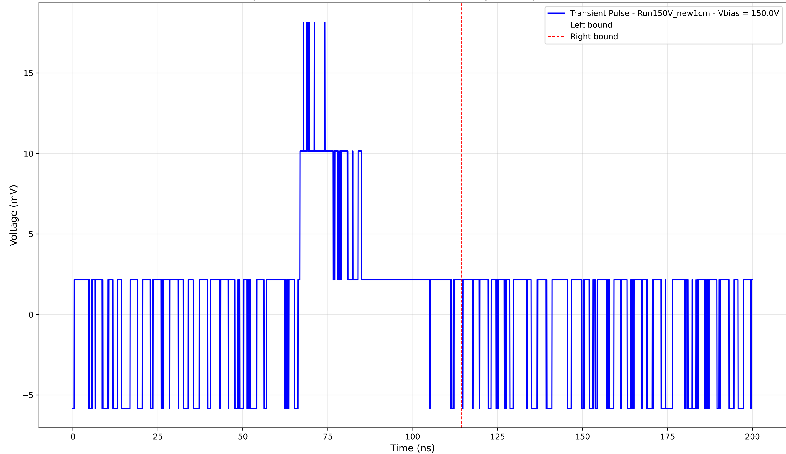
Transient Pulse - Sample: New1cm - Position: 1550.0 \mu\text{m} - Charge: 4.28 pC - Rise Time: 0.00 ns (N/A)
