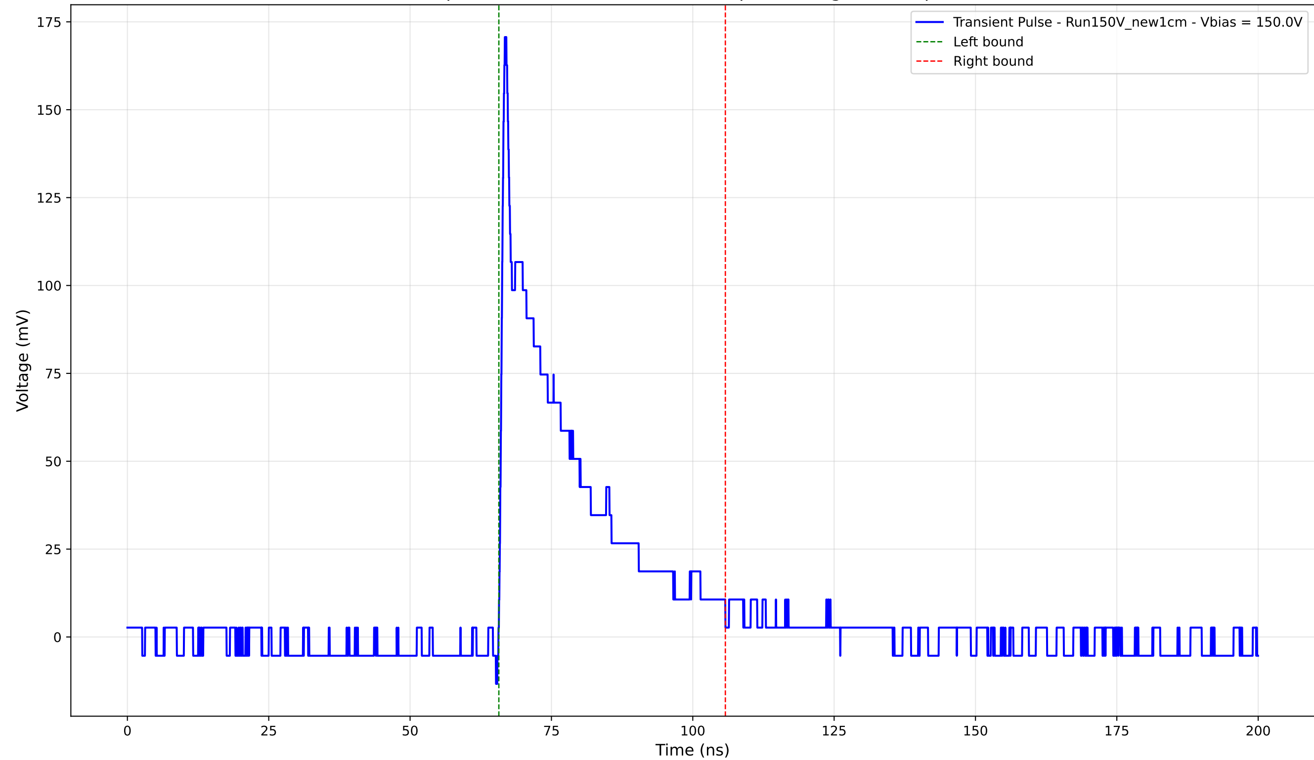
Transient Pulse - Sample: New1cm - Position: 2295.0 \mu\text{m} - Charge: 35.08 pC - Rise Time: 0.78 ns
