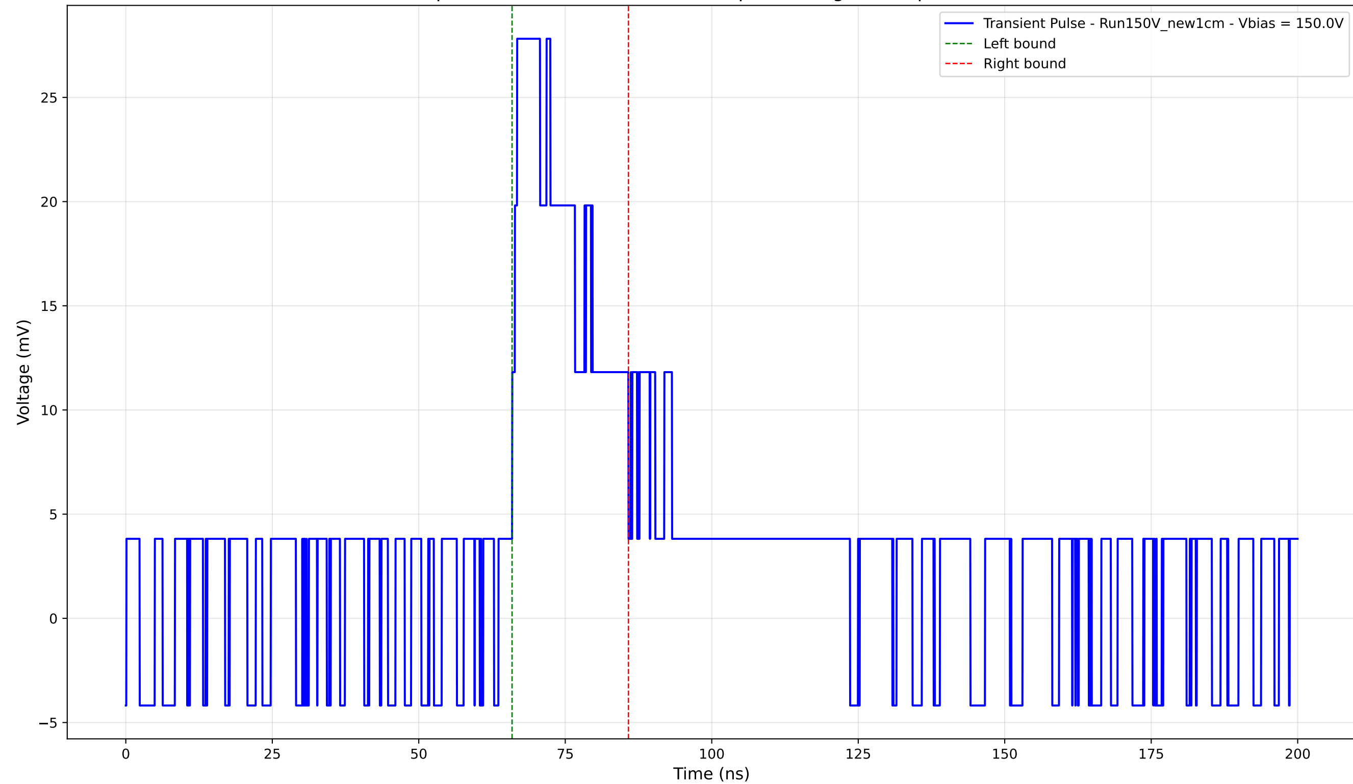
Transient Pulse - Sample: New1cm - Position: 3080.0 \mu\text{m} - Charge: 7.24 pC - Rise Time: 0.00 ns (N/A)
