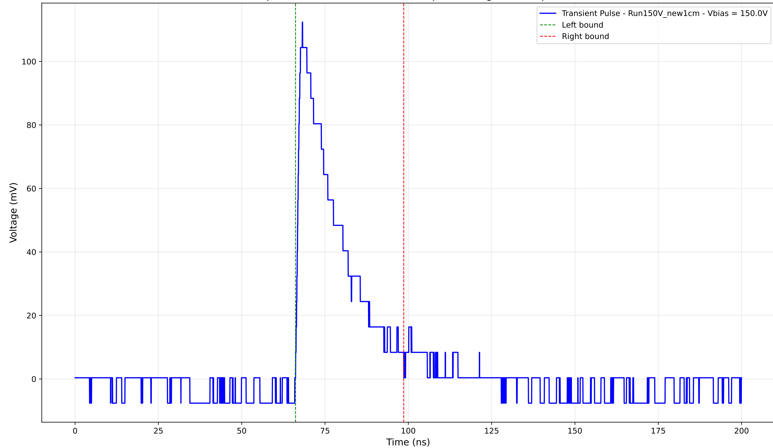
Transient Pulse - Sample: New1cm - Position: 810.0 \mu\text{m} - Charge: 27.98 pC - Rise Time: 1.31 ns
