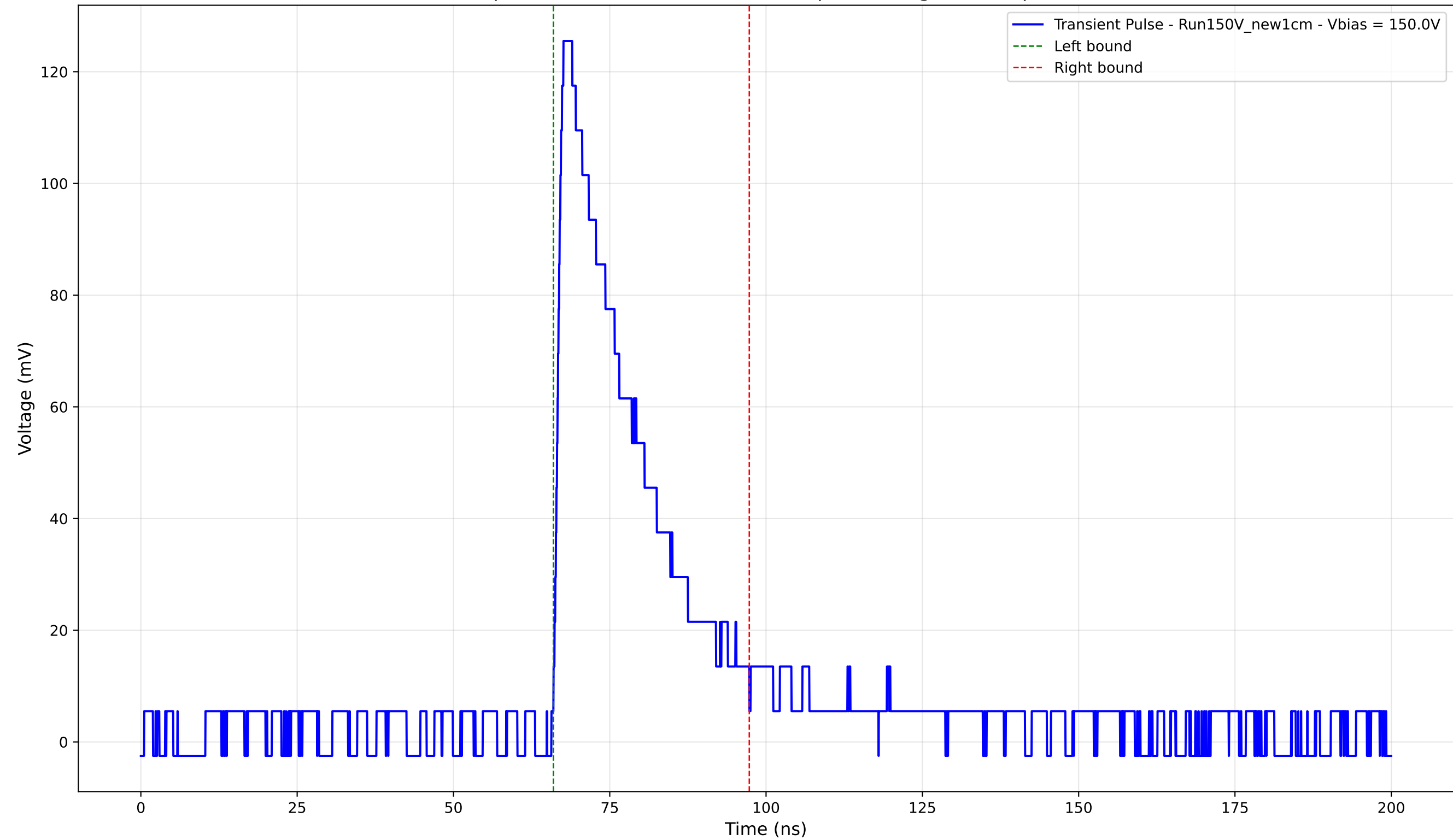
Transient Pulse - Sample: New1cm - Position: 4190.0 \mu\text{m} - Charge: 32.86 pC - Rise Time: 1.36 ns
