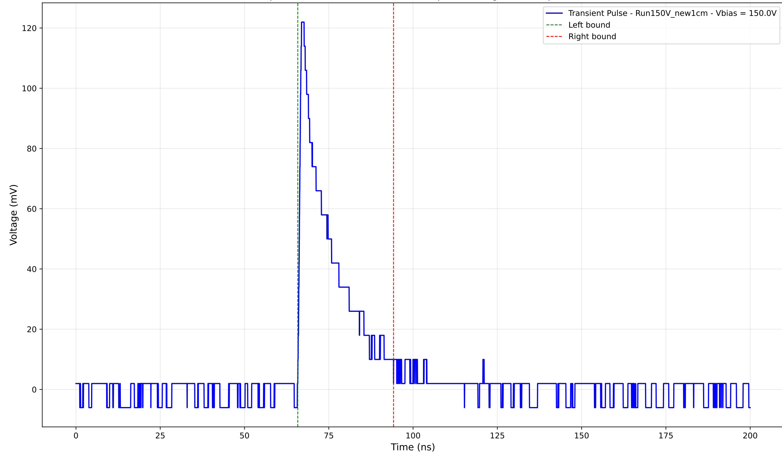
Transient Pulse - Sample: New1cm - Position: 165.0 \mu\text{m} - Charge: 23.43 pC - Rise Time: 0.87 ns
