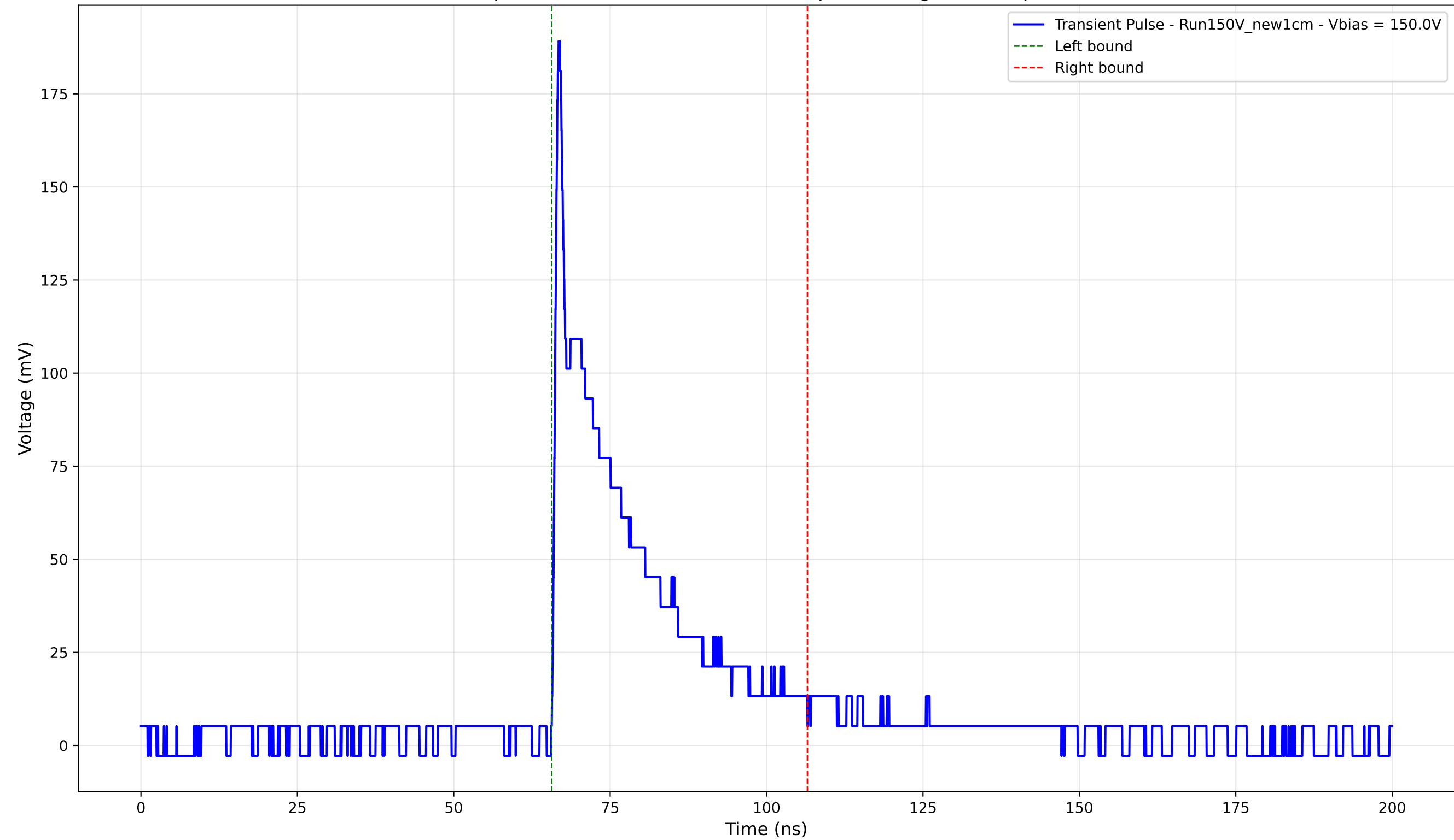
Transient Pulse - Sample: New1cm - Position: 2340.0 \mu\text{m} - Charge: 38.19 pC - Rise Time: 0.81 ns
