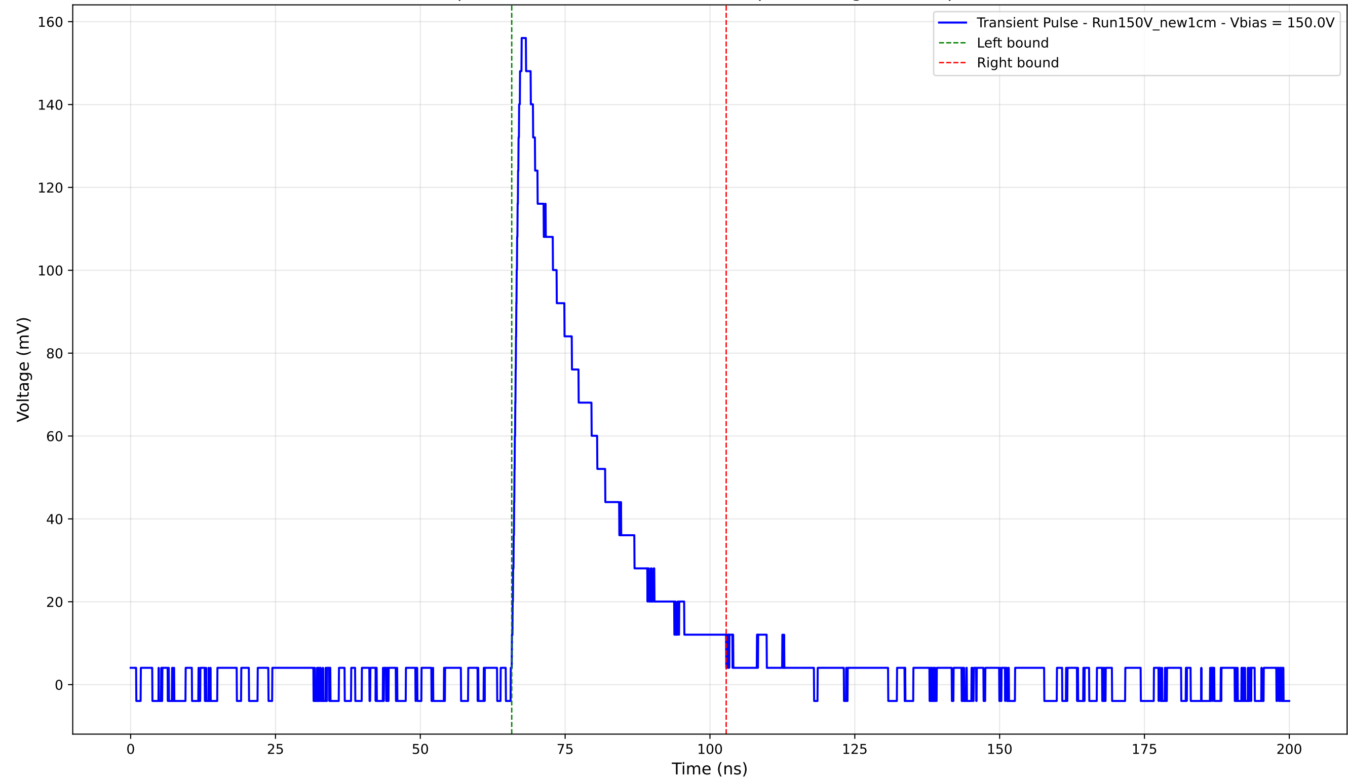
Transient Pulse - Sample: New1cm - Position: 4440.0 \mu\text{m} - Charge: 39.77 pC - Rise Time: 1.29 ns
