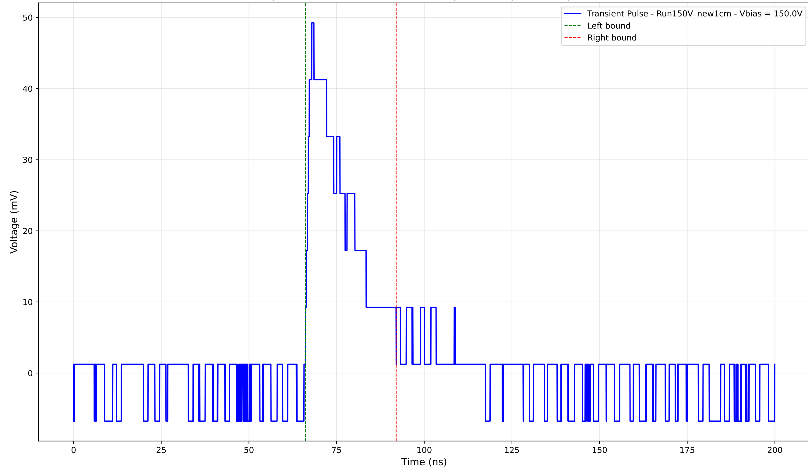
Transient Pulse - Sample: New1cm - Position: 3525.0 \mu\text{m} - Charge: 11.79 pC - Rise Time: 1.81 ns
