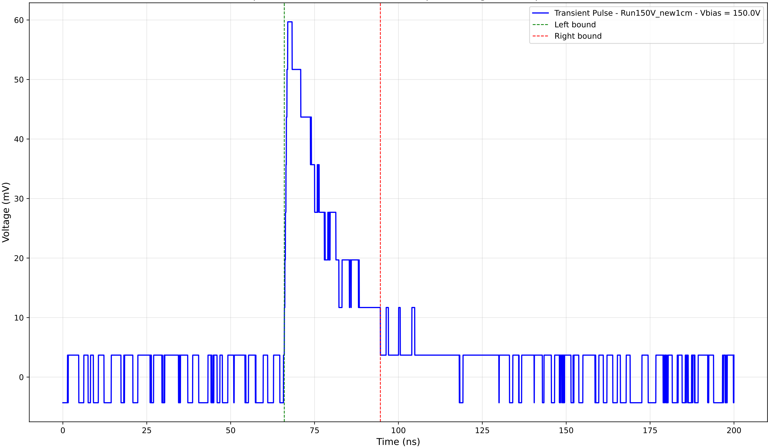
Transient Pulse - Sample: New1cm - Position: 3105.0 \mu\text{m} - Charge: 15.70 pC - Rise Time: 1.01 ns
