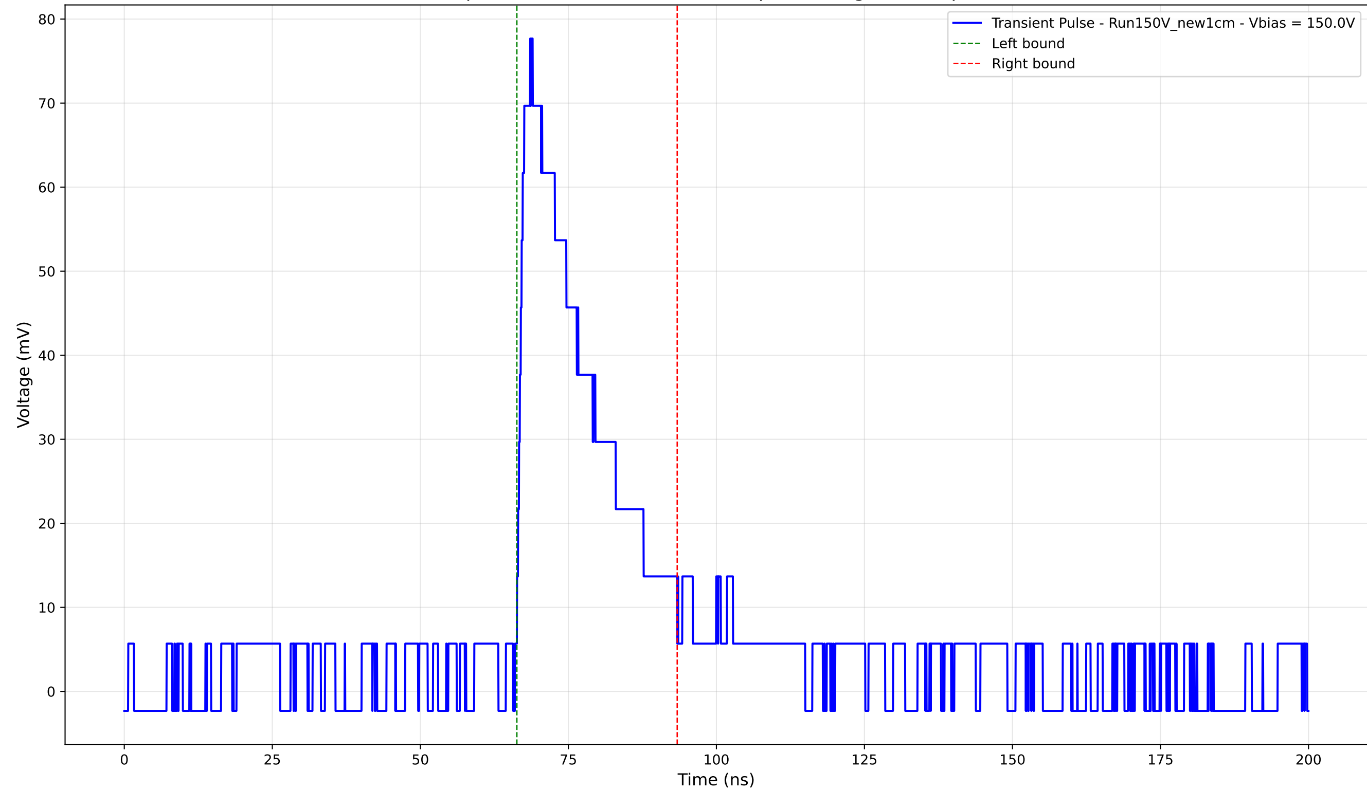
Transient Pulse - Sample: New1cm - Position: 970.0 \mu\text{m} - Charge: 19.59 pC - Rise Time: 2.23 ns
