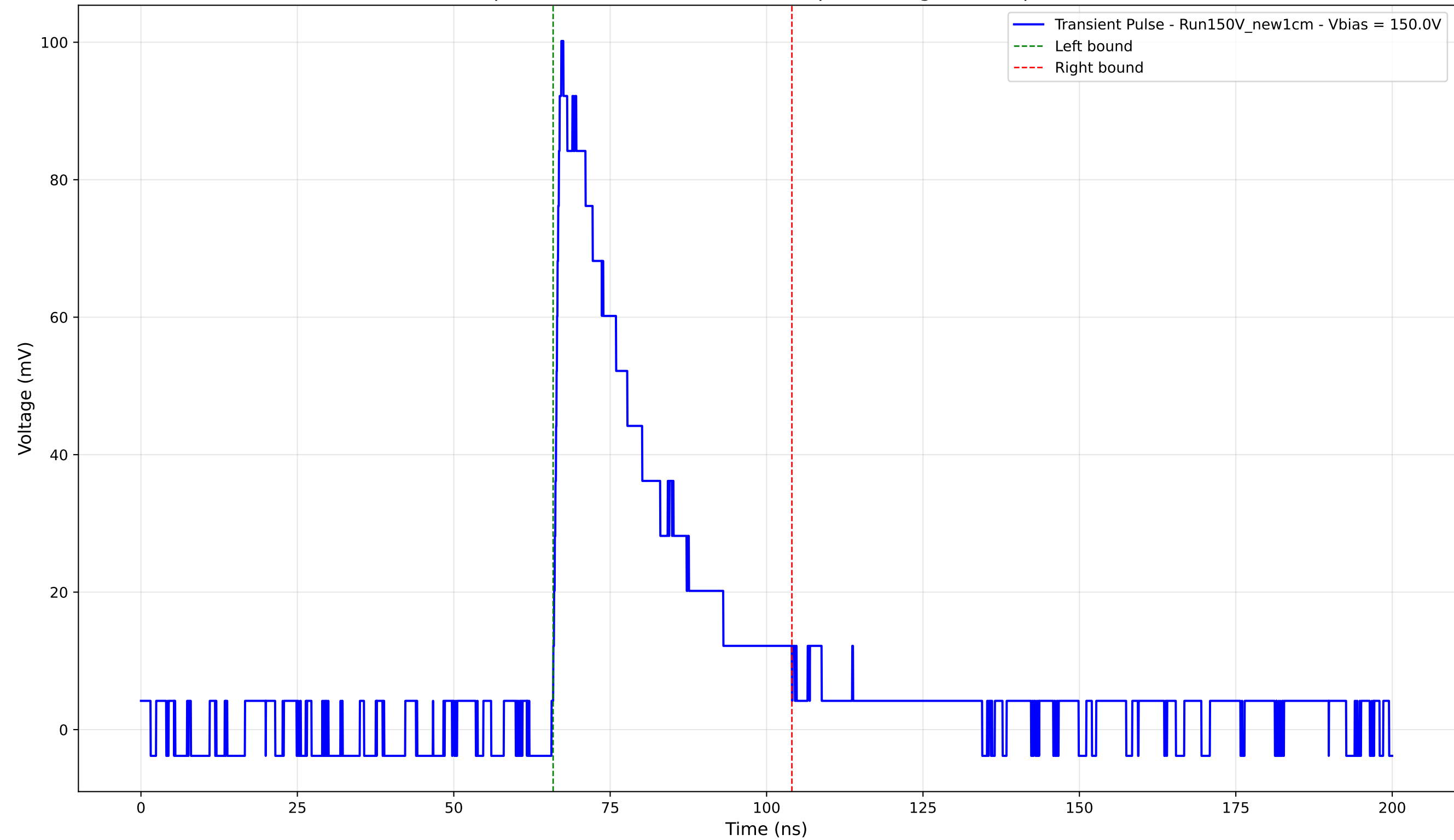
Transient Pulse - Sample: New1cm - Position: 1940.0 \mu\text{m} - Charge: 28.39 pC - Rise Time: 1.03 ns
