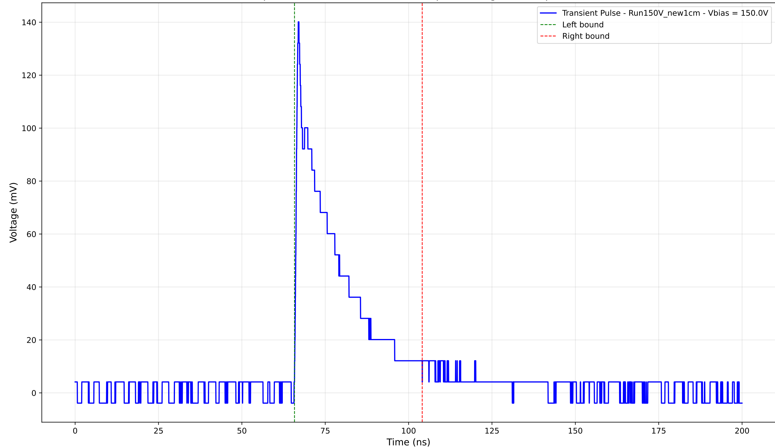
Transient Pulse - Sample: New1cm - Position: 2185.0 \mu\text{m} - Charge: 32.66 pC - Rise Time: 0.88 ns
