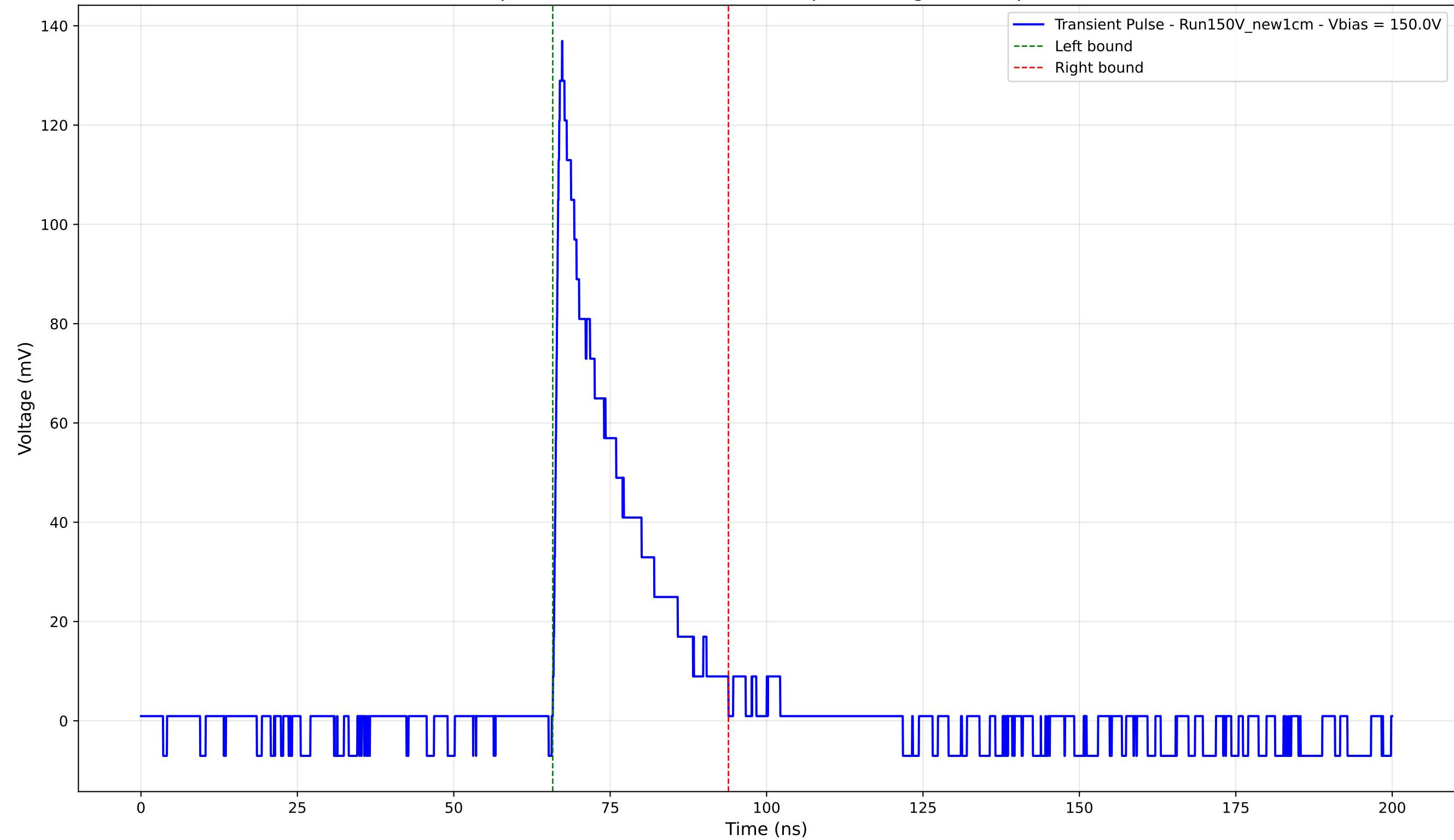
Transient Pulse - Sample: New1cm - Position: 220.0 \mu\text{m} - Charge: 25.05 pC - Rise Time: 0.99 ns
