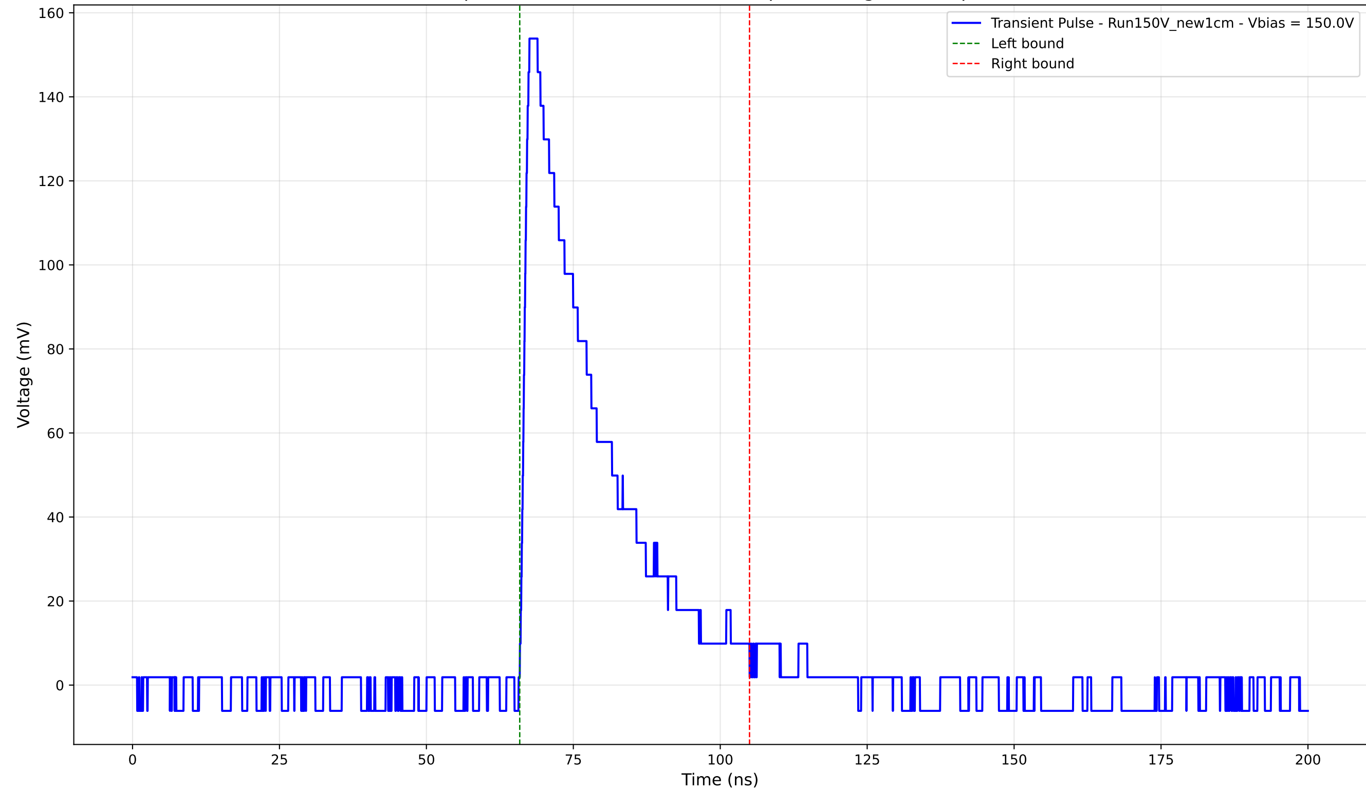
Transient Pulse - Sample: New1cm - Position: 4285.0 \mu\text{m} - Charge: 41.07 pC - Rise Time: 1.33 ns
