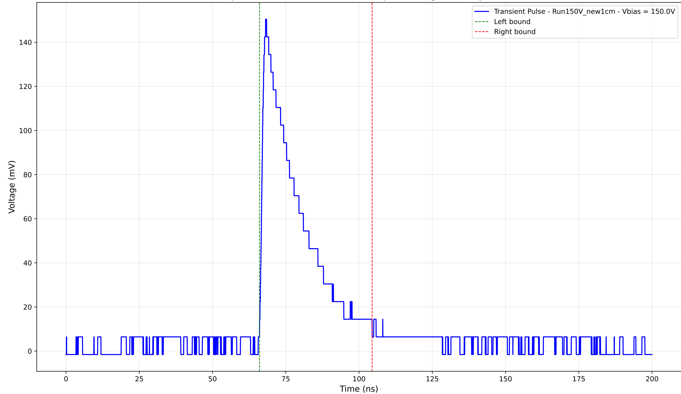
Transient Pulse - Sample: New1cm - Position: 3955.0 \mu\text{m} - Charge: 41.76 pC - Rise Time: 1.58 ns
