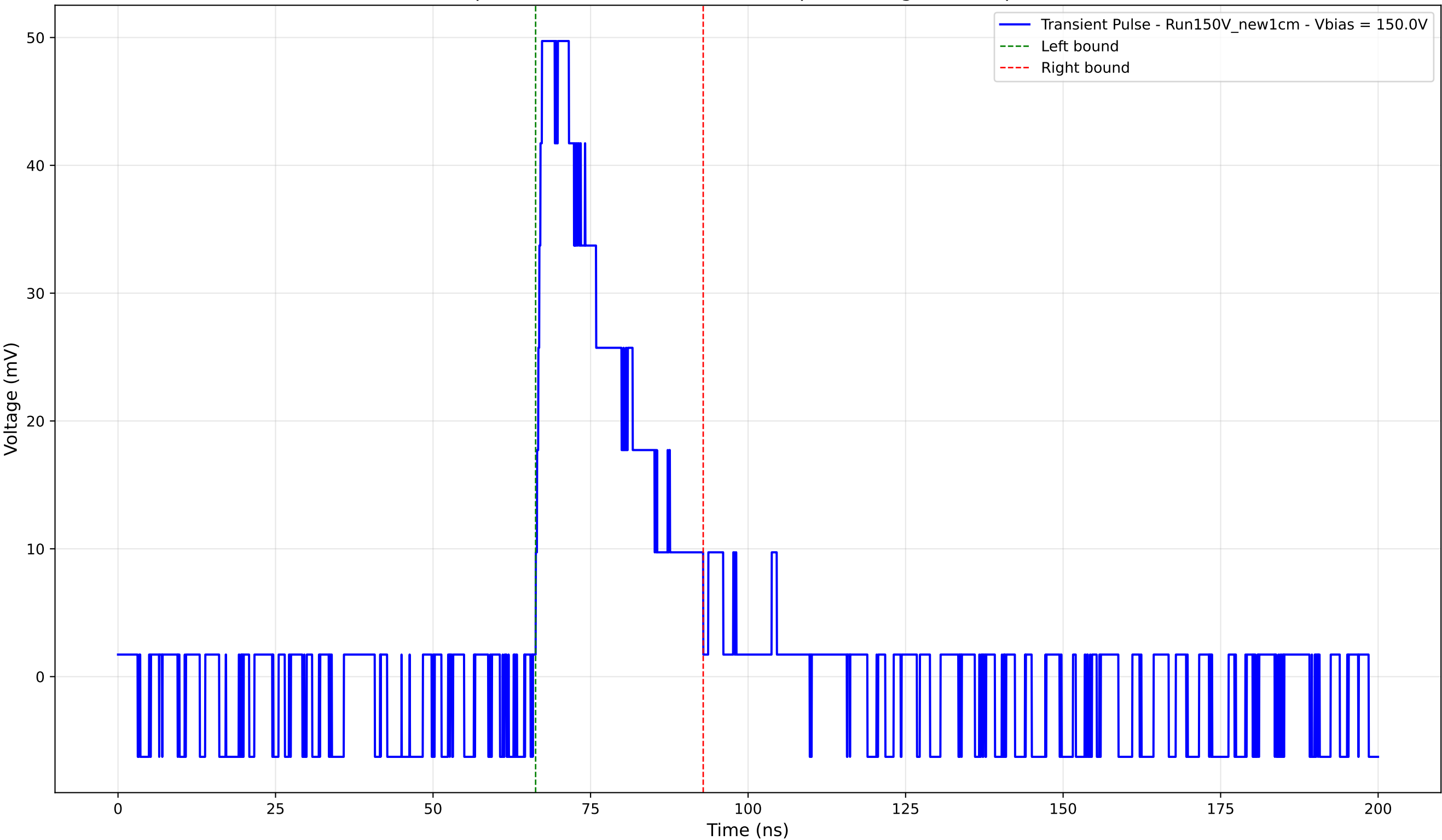
Transient Pulse - Sample: New1cm - Position: 3520.0 \mu\text{m} - Charge: 13.49 pC - Rise Time: 0.99 ns
