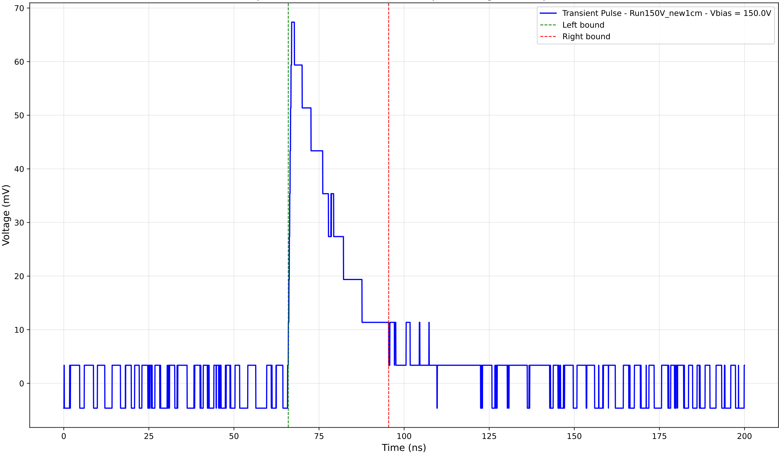
Transient Pulse - Sample: New1cm - Position: 3110.0 \mu\text{m} - Charge: 17.79 pC - Rise Time: 0.97 ns
