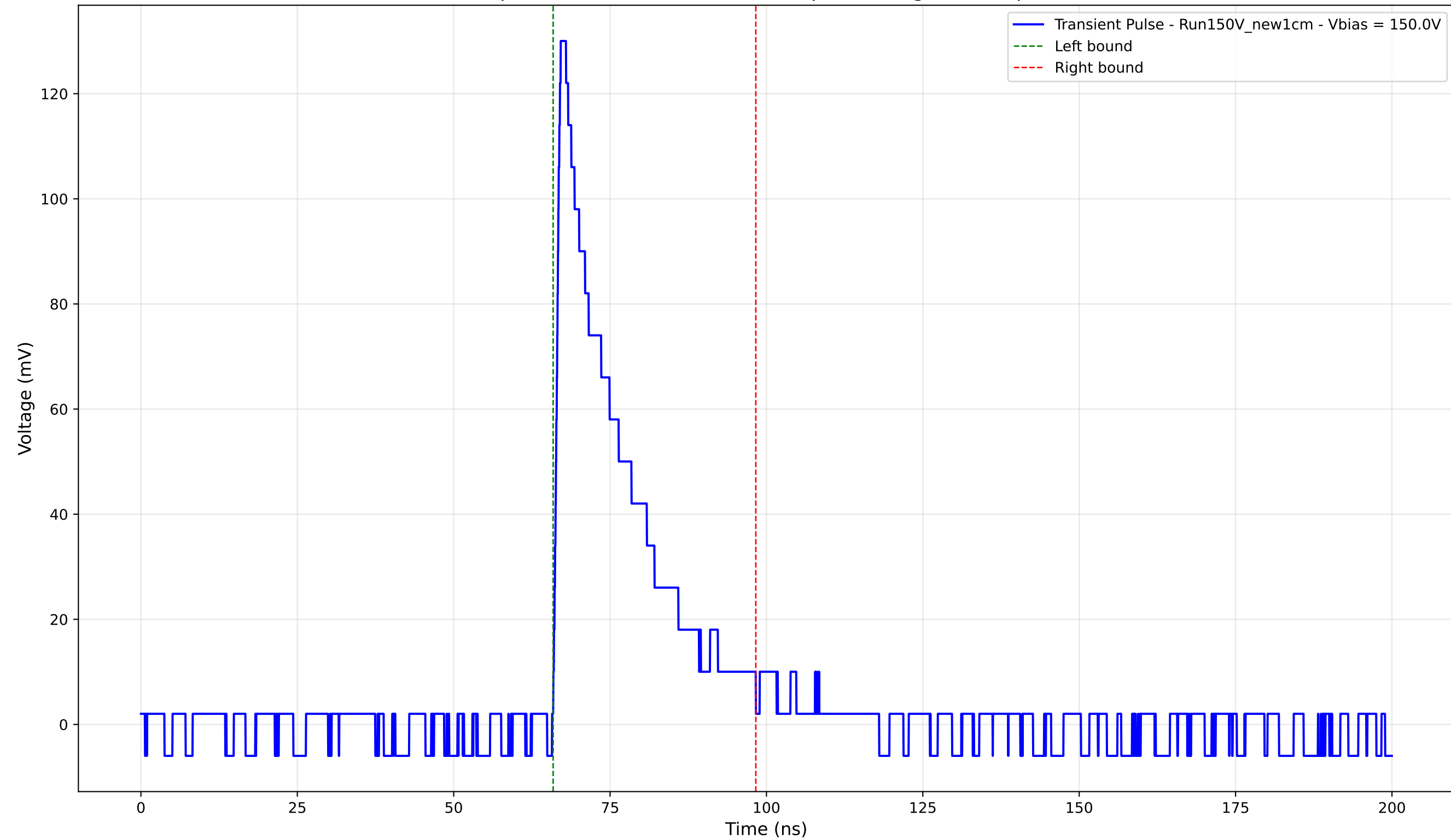
Transient Pulse - Sample: New1cm - Position: 330.0 \mu\text{m} - Charge: 27.58 pC - Rise Time: 0.97 ns
