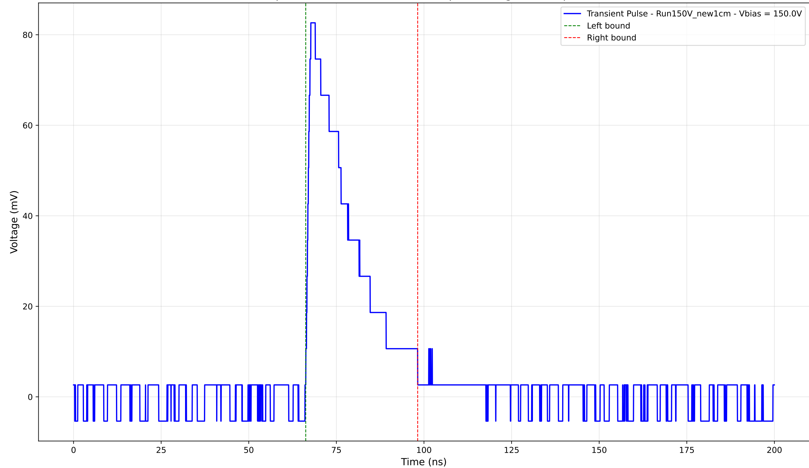
Transient Pulse - Sample: New1cm - Position: 960.0 \mu\text{m} - Charge: 21.98 pC - Rise Time: 1.19 ns
