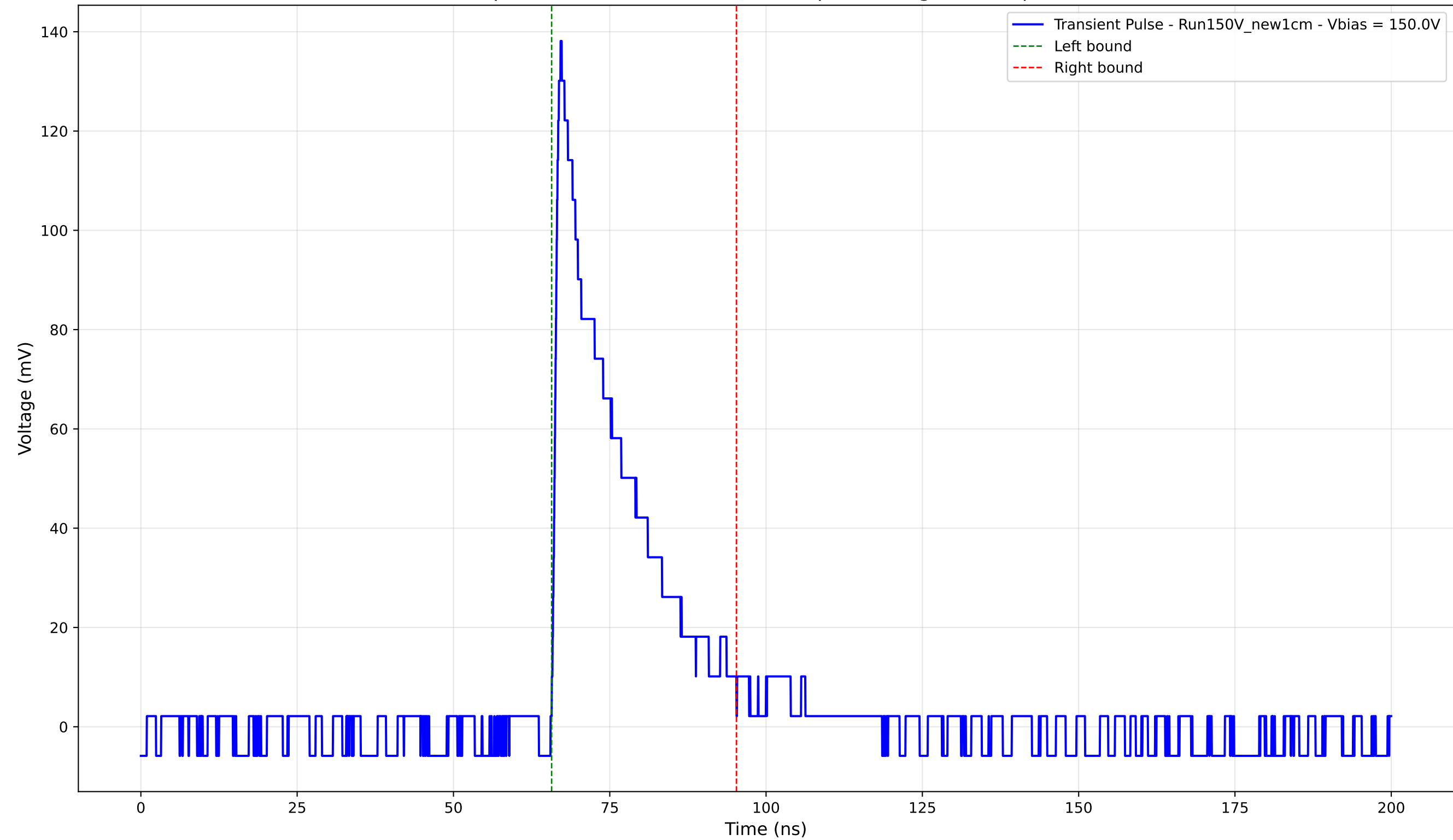
Transient Pulse - Sample: New1cm - Position: 4700.0 \mu\text{m} - Charge: 28.51 pC - Rise Time: 1.03 ns
