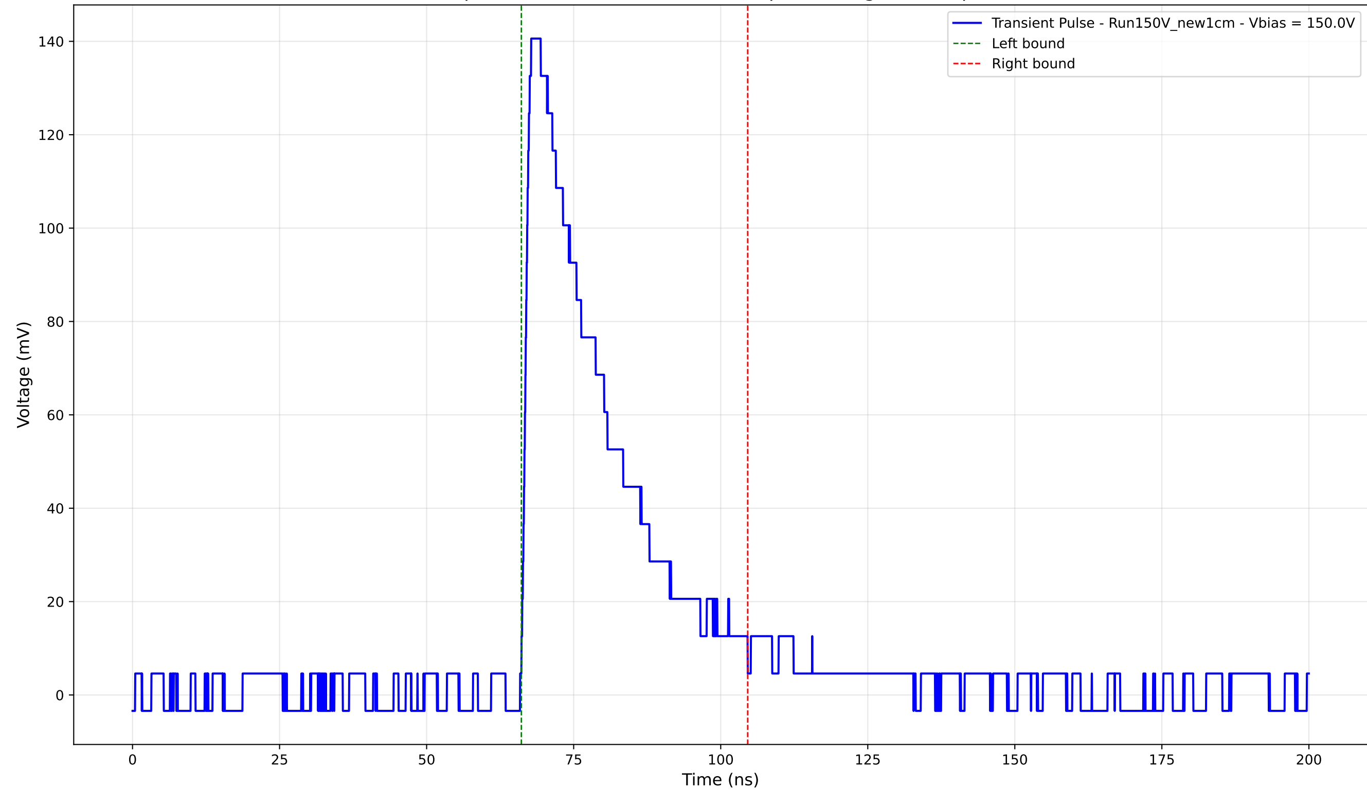
Transient Pulse - Sample: New1cm - Position: 3715.0 \mu\text{m} - Charge: 41.53 pC - Rise Time: 1.30 ns
