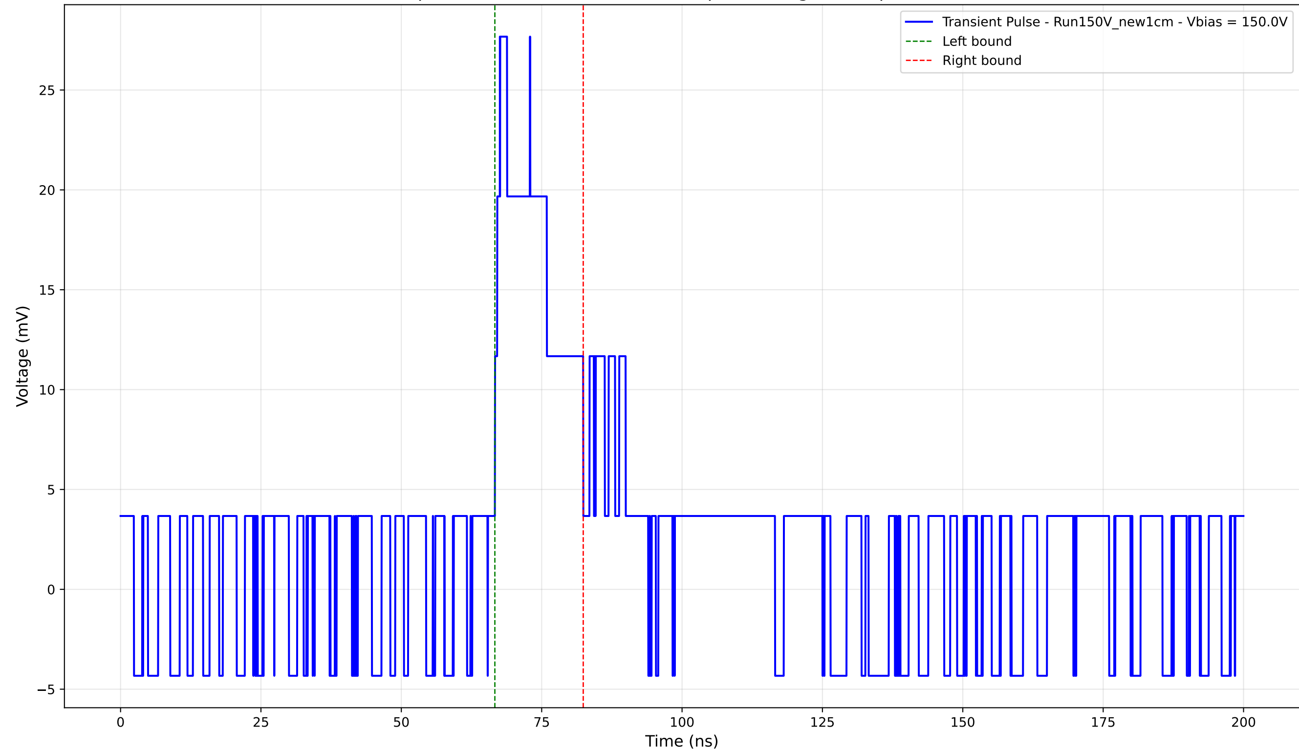
Transient Pulse - Sample: New1cm - Position: 1055.0 \mu\text{m} - Charge: 5.30 pC - Rise Time: 0.00 ns (N/A)
