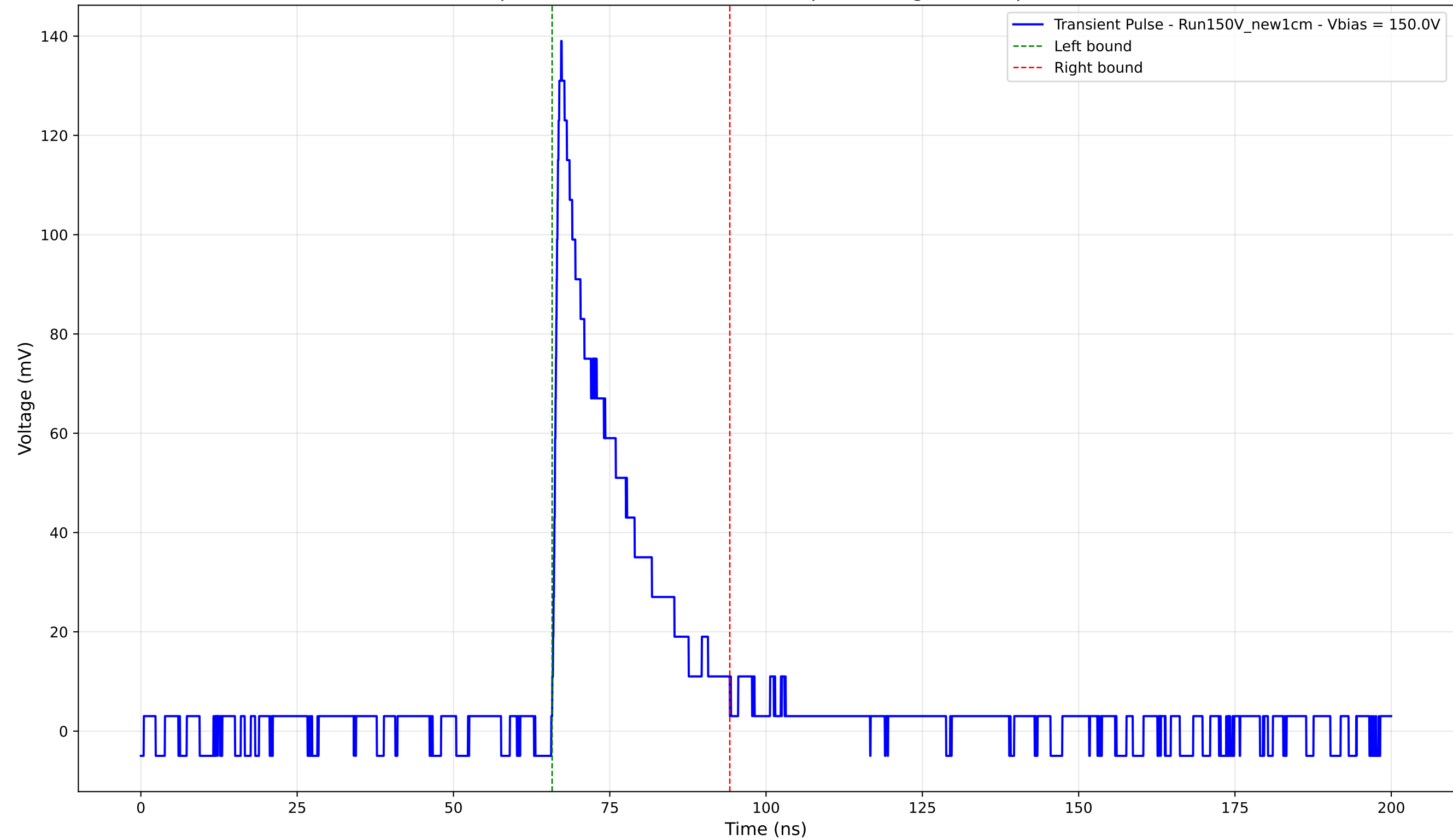
Transient Pulse - Sample: New1cm - Position: 205.0 \mu\text{m} - Charge: 26.02 pC - Rise Time: 1.01 ns
