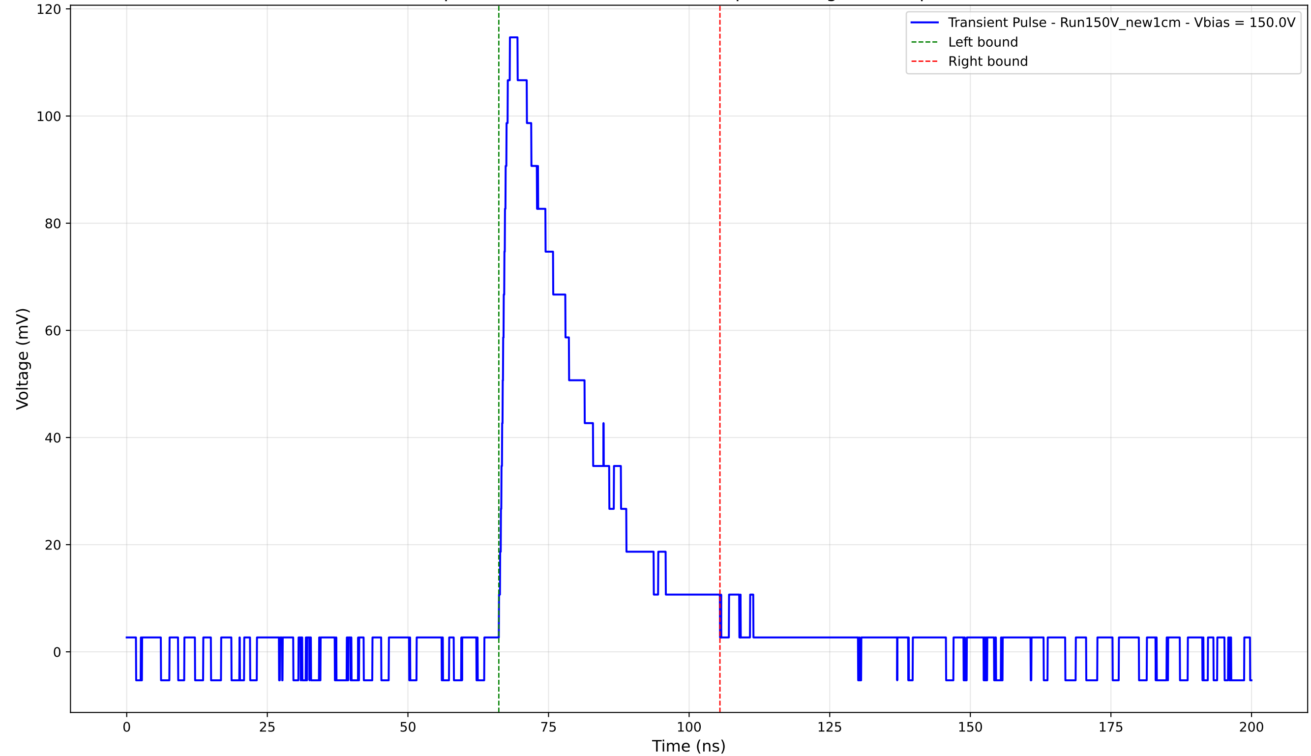
Transient Pulse - Sample: New1cm - Position: 1335.0 \mu\text{m} - Charge: 33.30 pC - Rise Time: 1.38 ns
