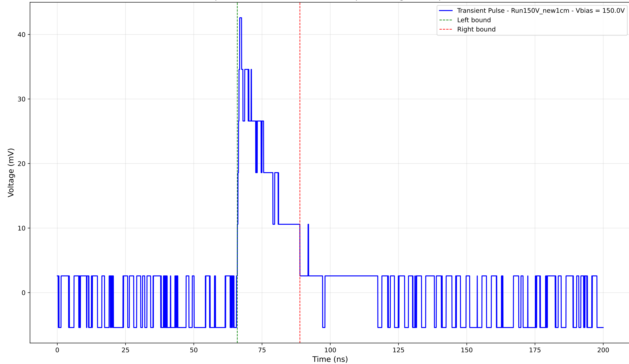
Transient Pulse - Sample: New1cm - Position: 2075.0 \mu\text{m} - Charge: 9.07 pC - Rise Time: 0.88 ns
