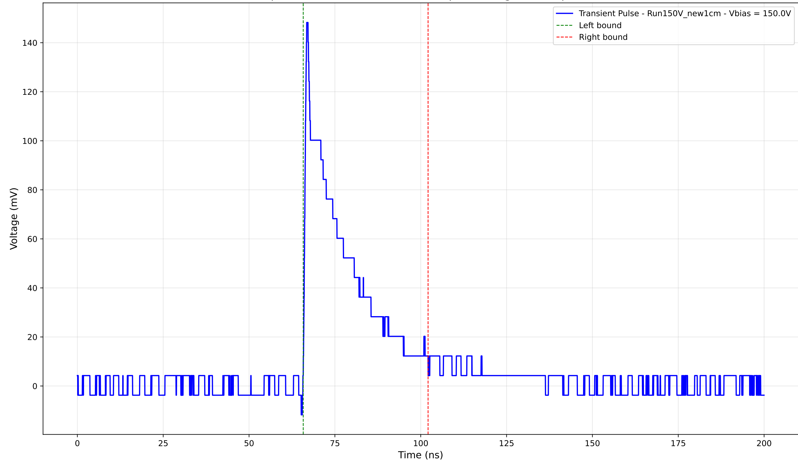
Transient Pulse - Sample: New1cm - Position: 2215.0 \mu\text{m} - Charge: 33.54 pC - Rise Time: 0.83 ns
