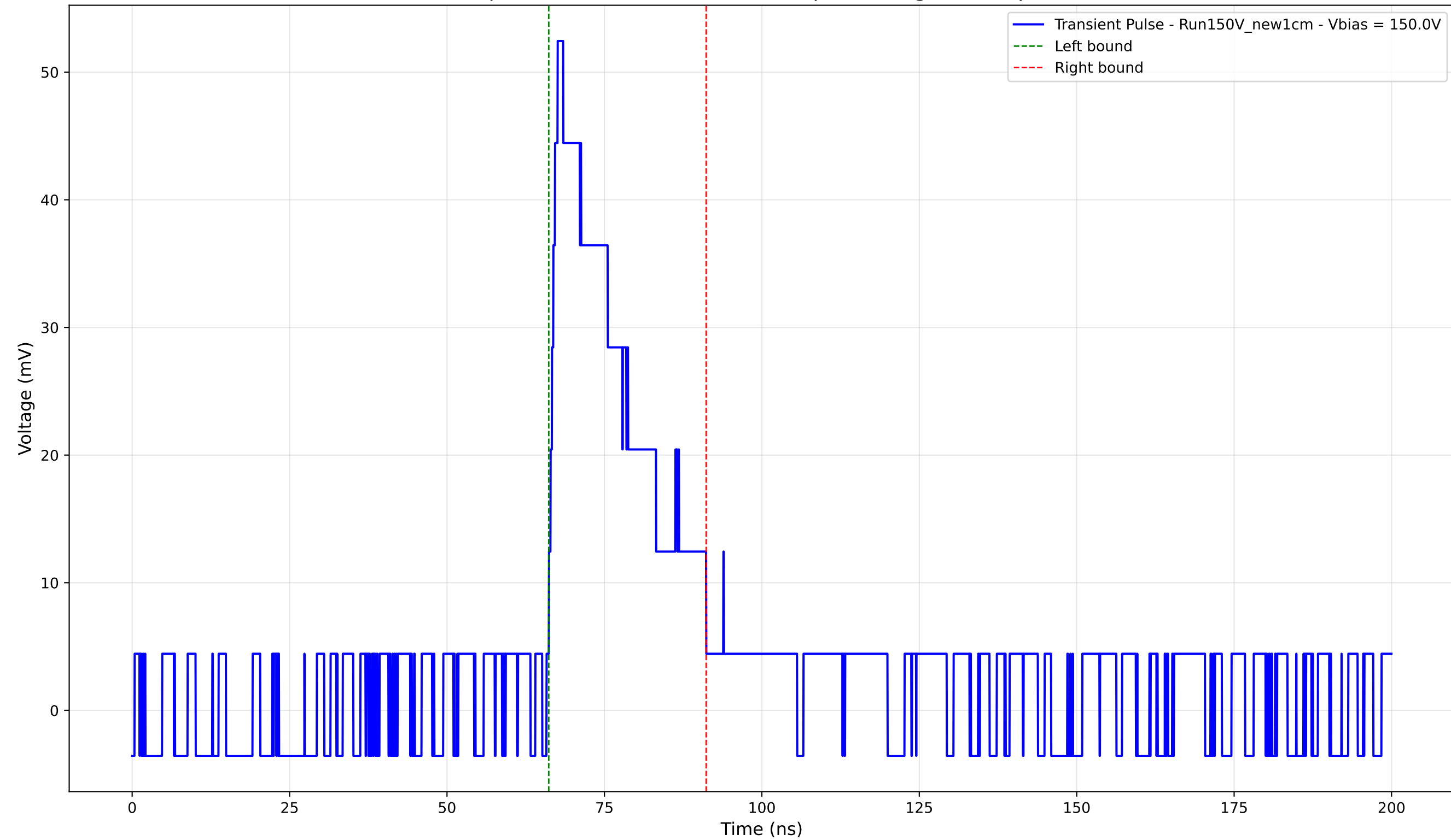
Transient Pulse - Sample: New1cm - Position: 4105.0 \mu\text{m} - Charge: 13.05 pC - Rise Time: 1.40 ns
