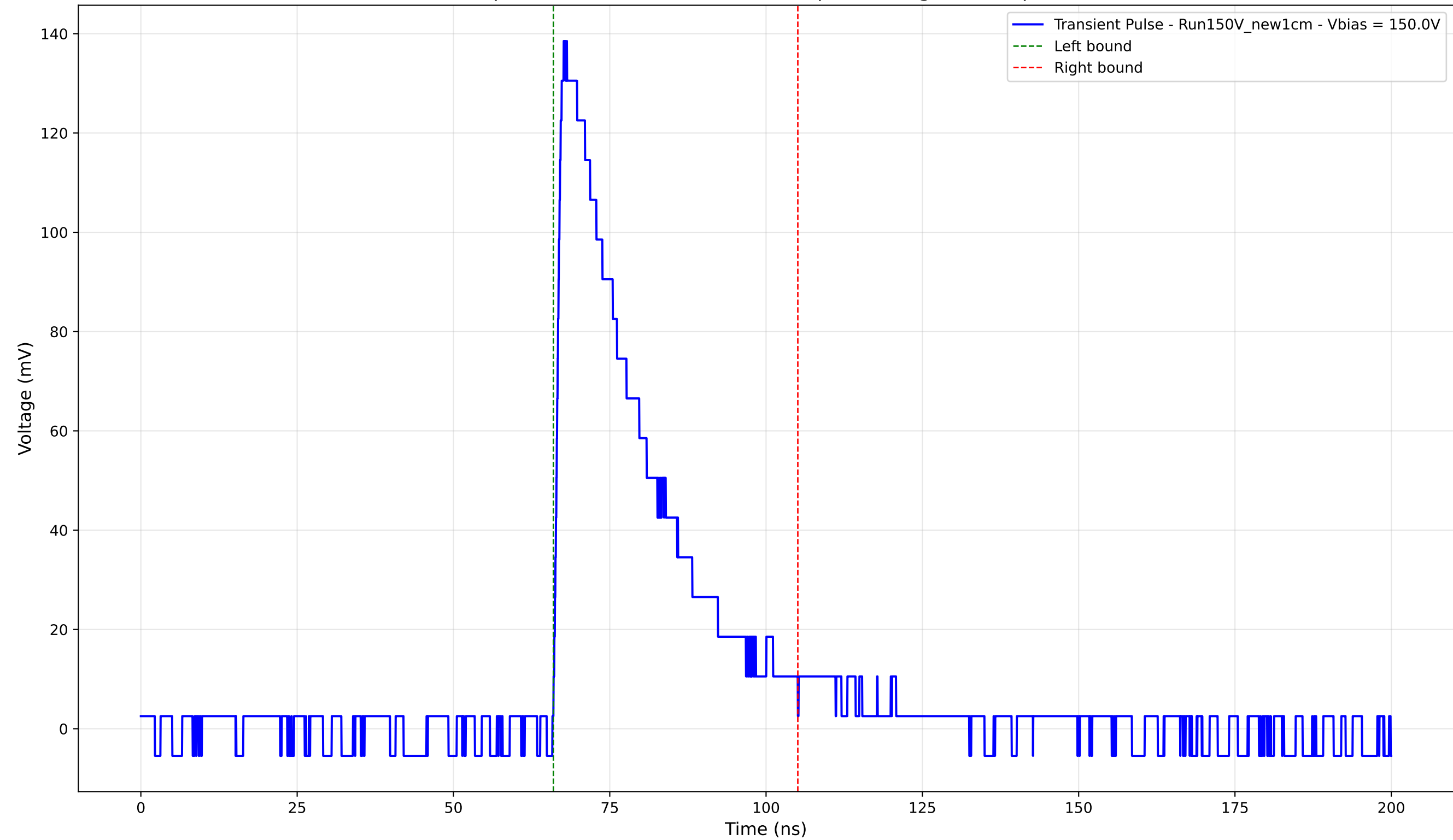
Transient Pulse - Sample: New1cm - Position: 3390.0 \mu\text{m} - Charge: 39.90 pC - Rise Time: 1.19 ns
