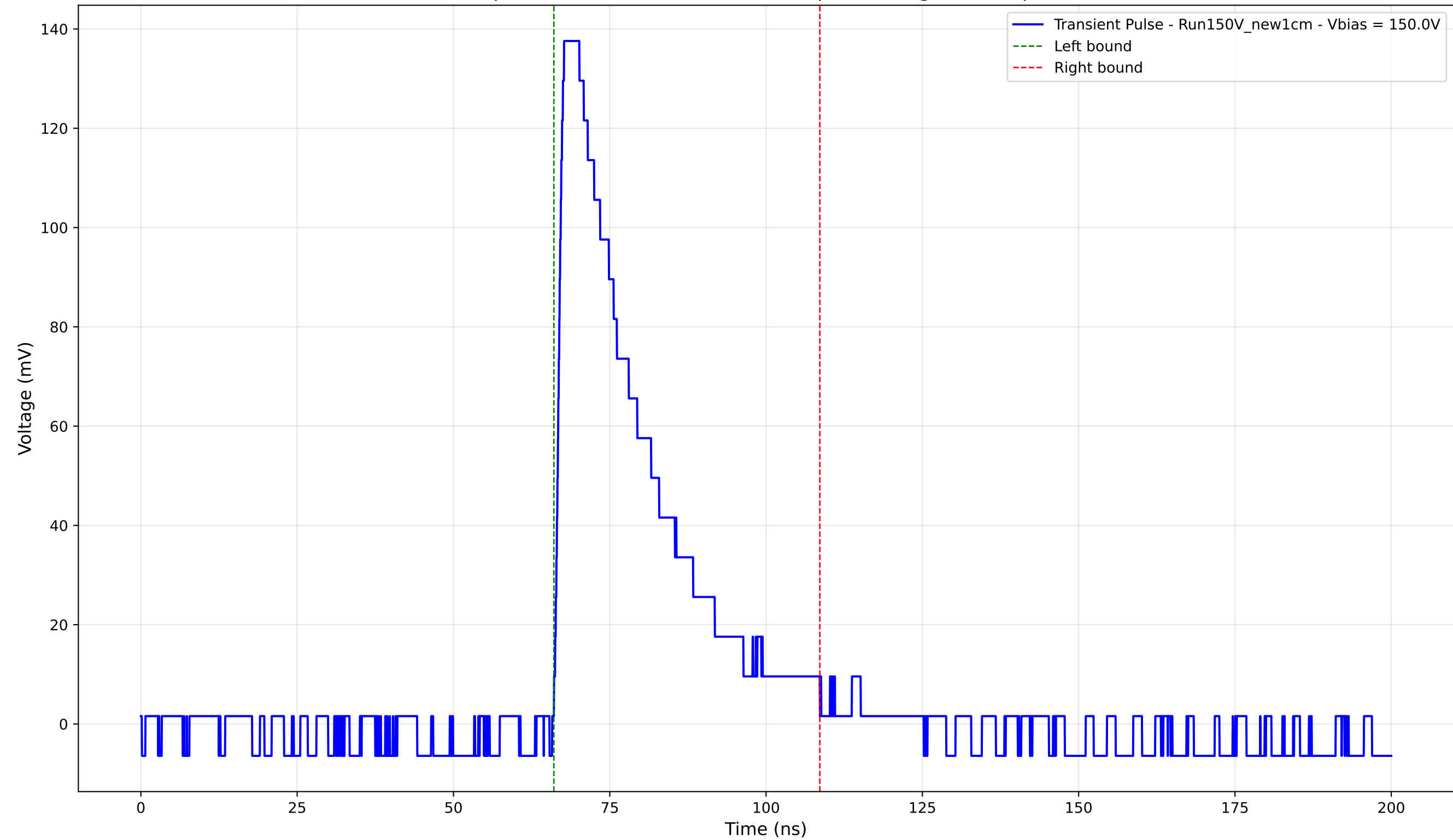
Transient Pulse - Sample: New1cm - Position: 3760.0 \mu\text{m} - Charge: 40.06 pC - Rise Time: 1.25 ns
