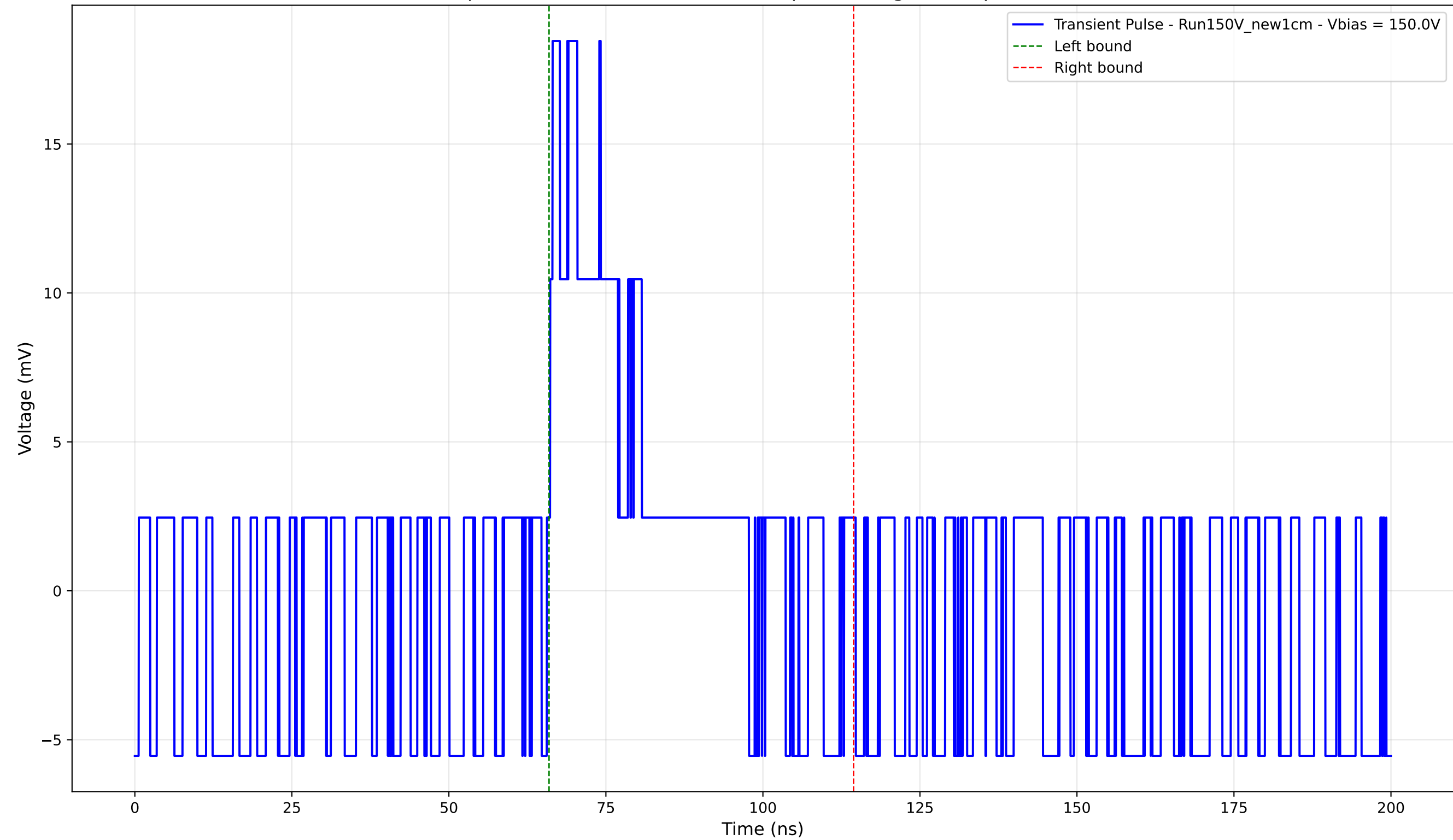
Transient Pulse - Sample: New1cm - Position: 3055.0 \mu\text{m} - Charge: 3.73 pC - Rise Time: 0.00 ns (N/A)
