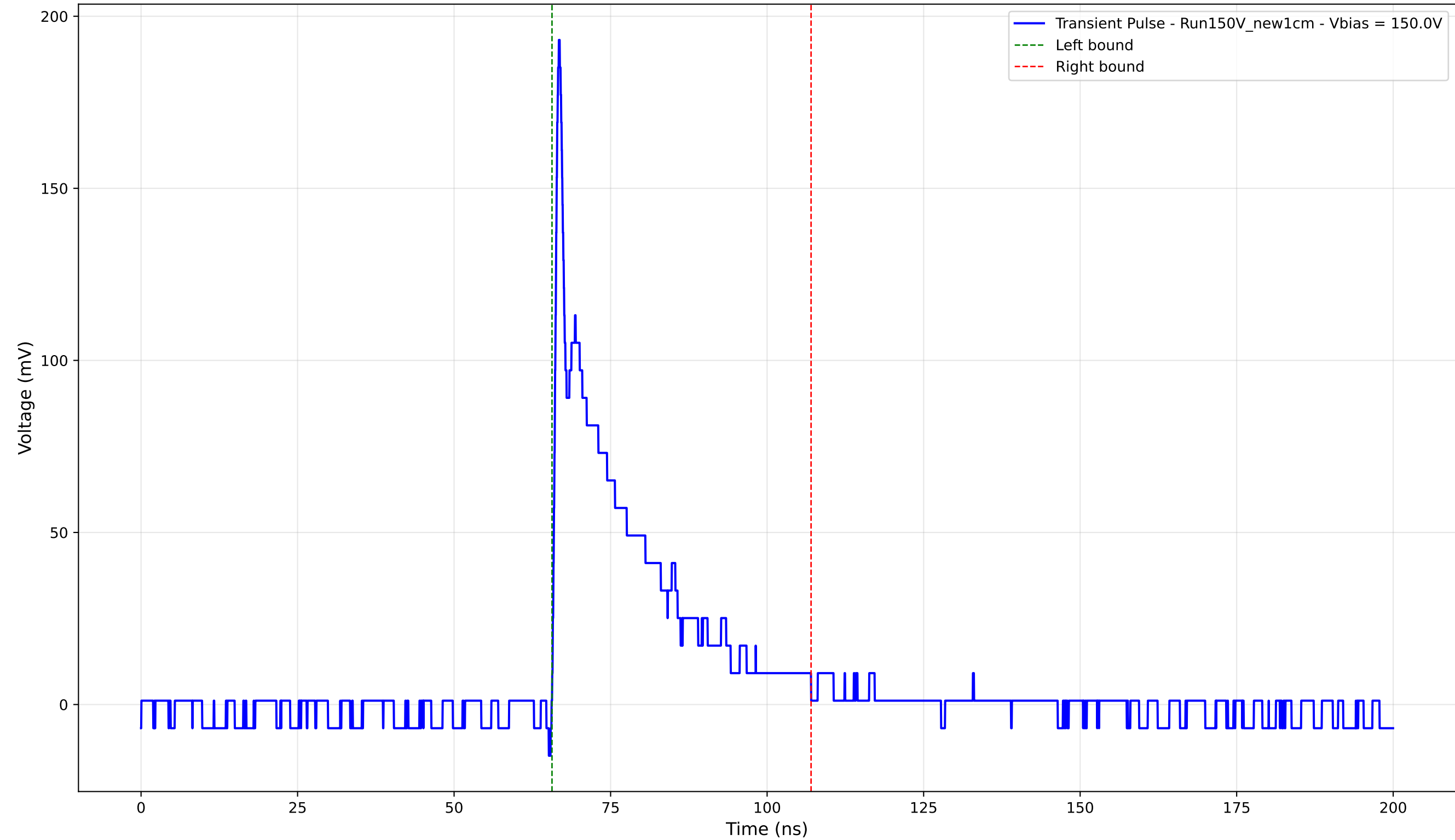
Transient Pulse - Sample: New1cm - Position: 2395.0 \mu\text{m} - Charge: 33.89 pC - Rise Time: 0.77 ns
