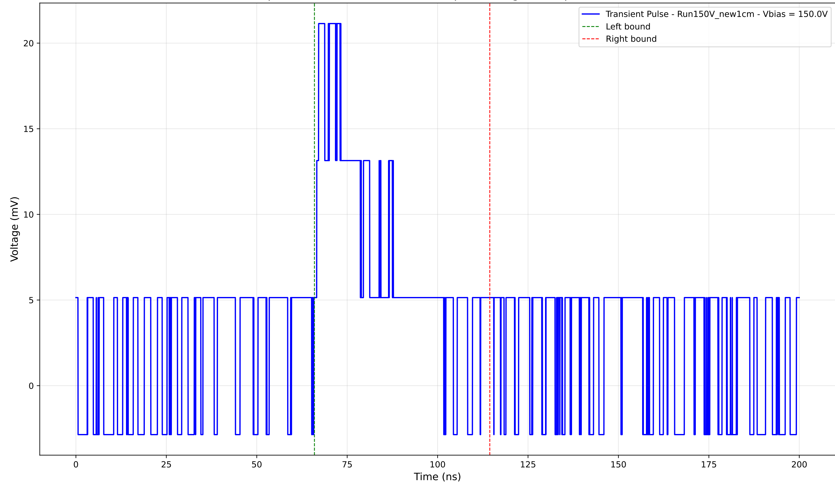
Transient Pulse - Sample: New1cm - Position: 1525.0 \mu\text{m} - Charge: 7.67 pC - Rise Time: 0.00 ns (N/A)
