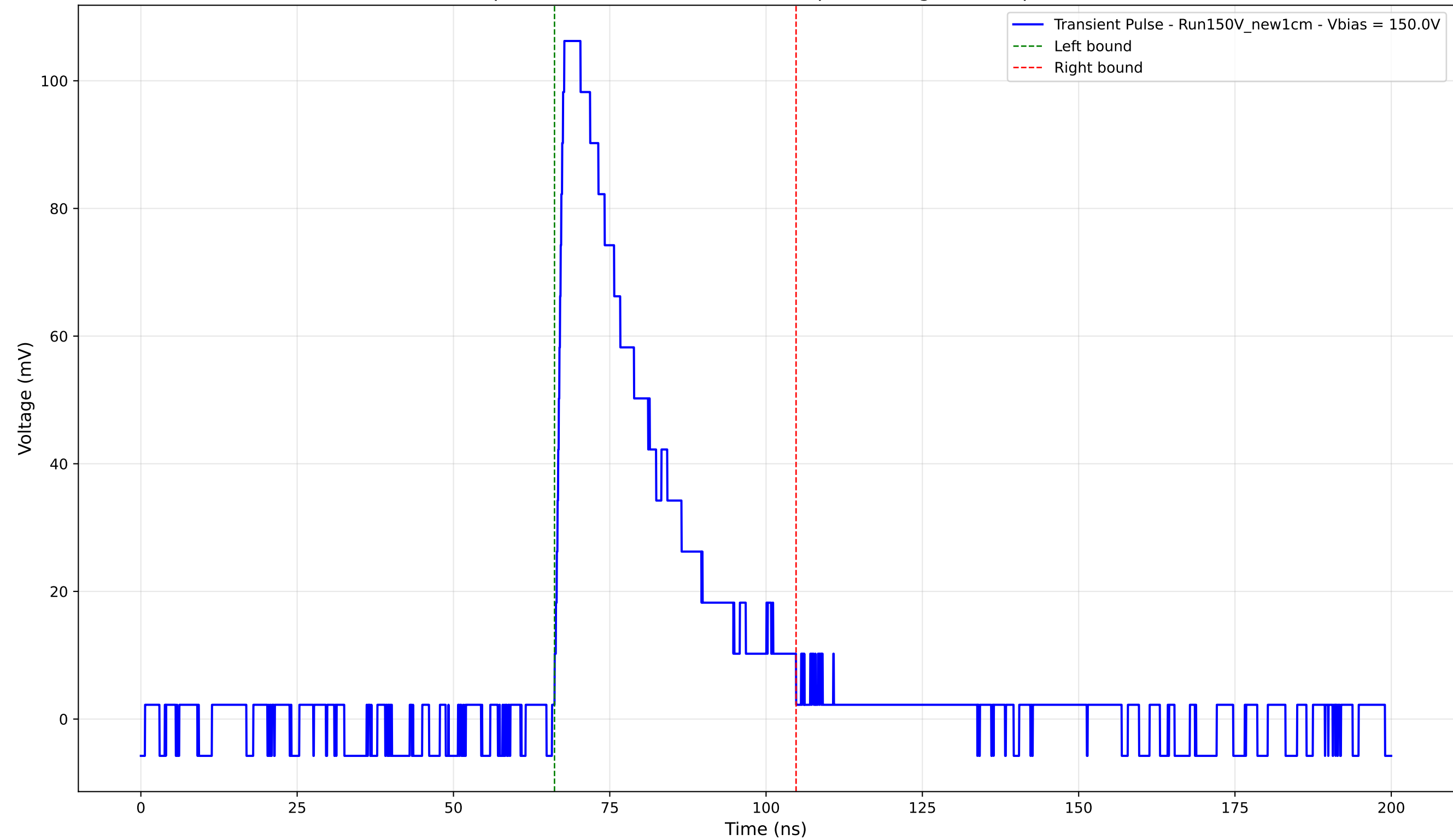
Transient Pulse - Sample: New1cm - Position: 1270.0 \mu\text{m} - Charge: 32.59 pC - Rise Time: 1.16 ns
