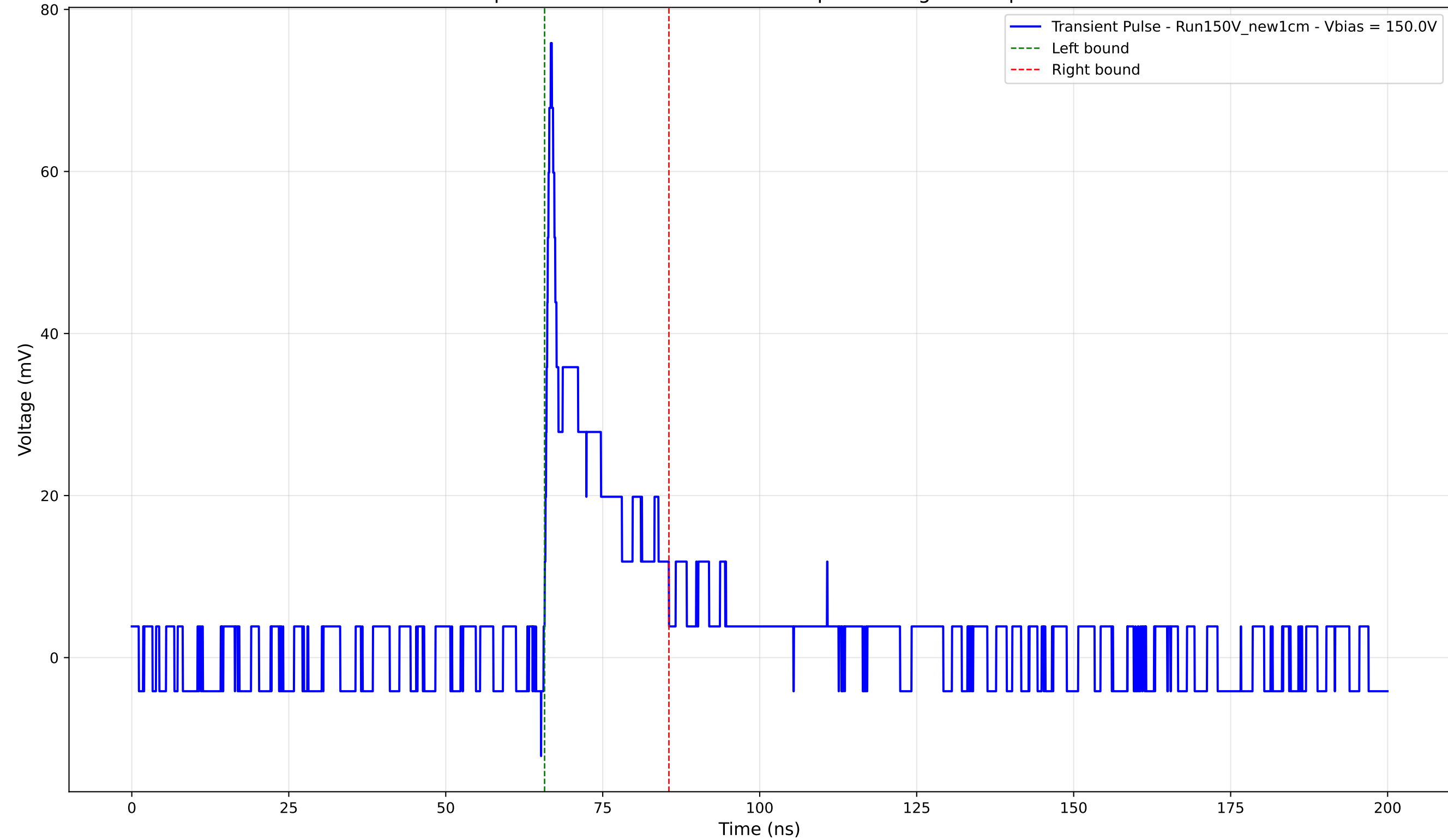
Transient Pulse - Sample: New1cm - Position: 2515.0 \mu\text{m} - Charge: 9.76 pC - Rise Time: 0.97 ns
