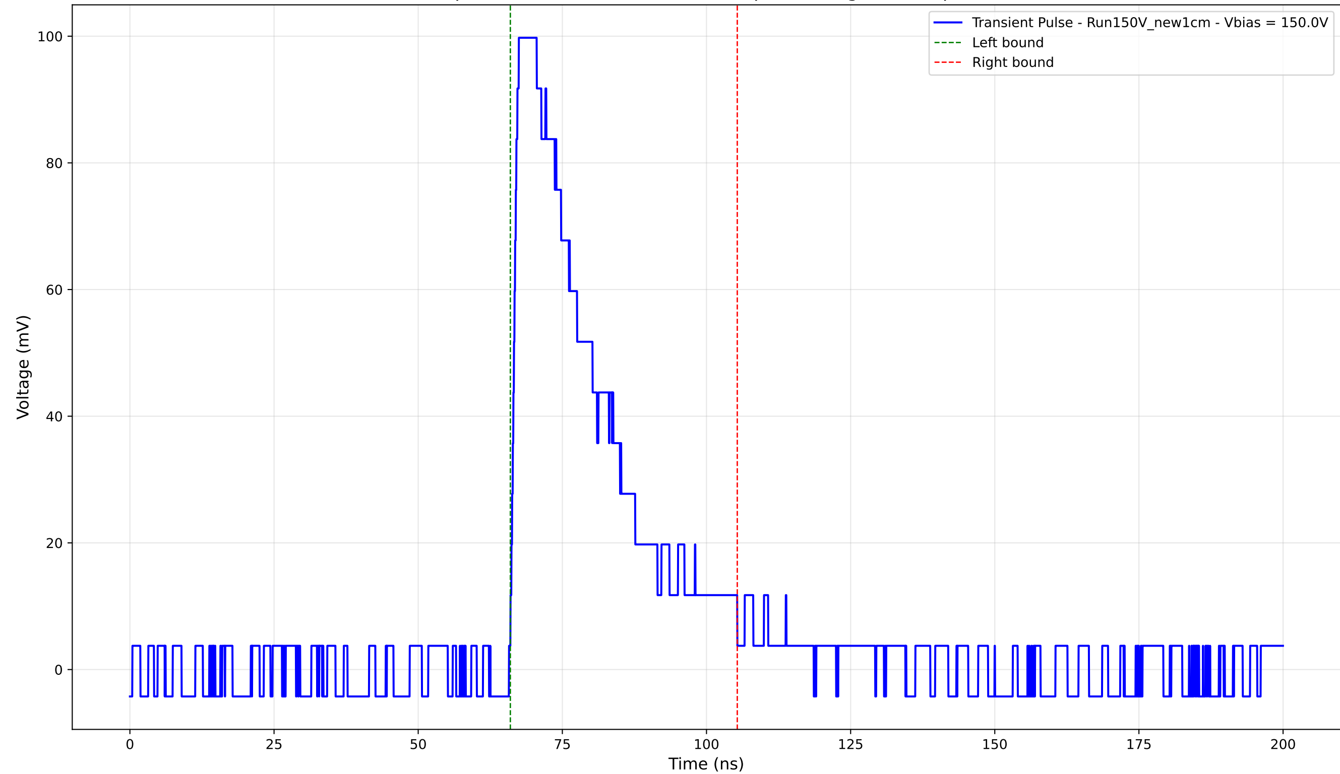
Transient Pulse - Sample: New1cm - Position: 1730.0 \mu\text{m} - Charge: 31.81 pC - Rise Time: 1.20 ns
