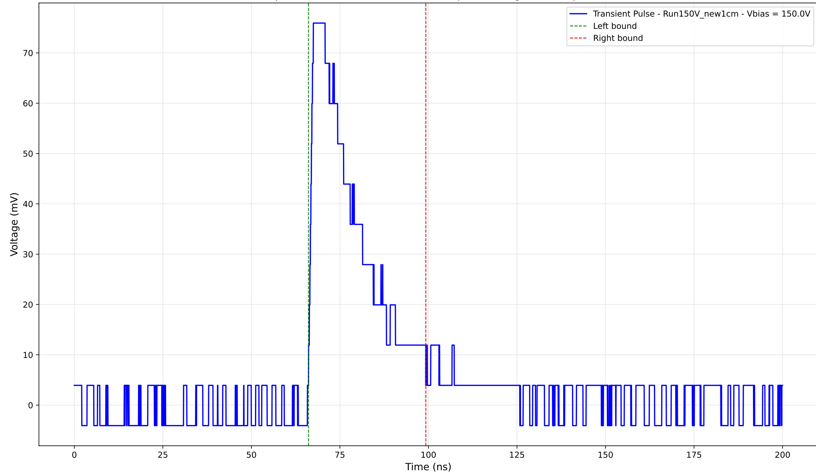
Transient Pulse - Sample: New1cm - Position: 3620.0 \mu\text{m} - Charge: 22.69 pC - Rise Time: 1.35 ns
