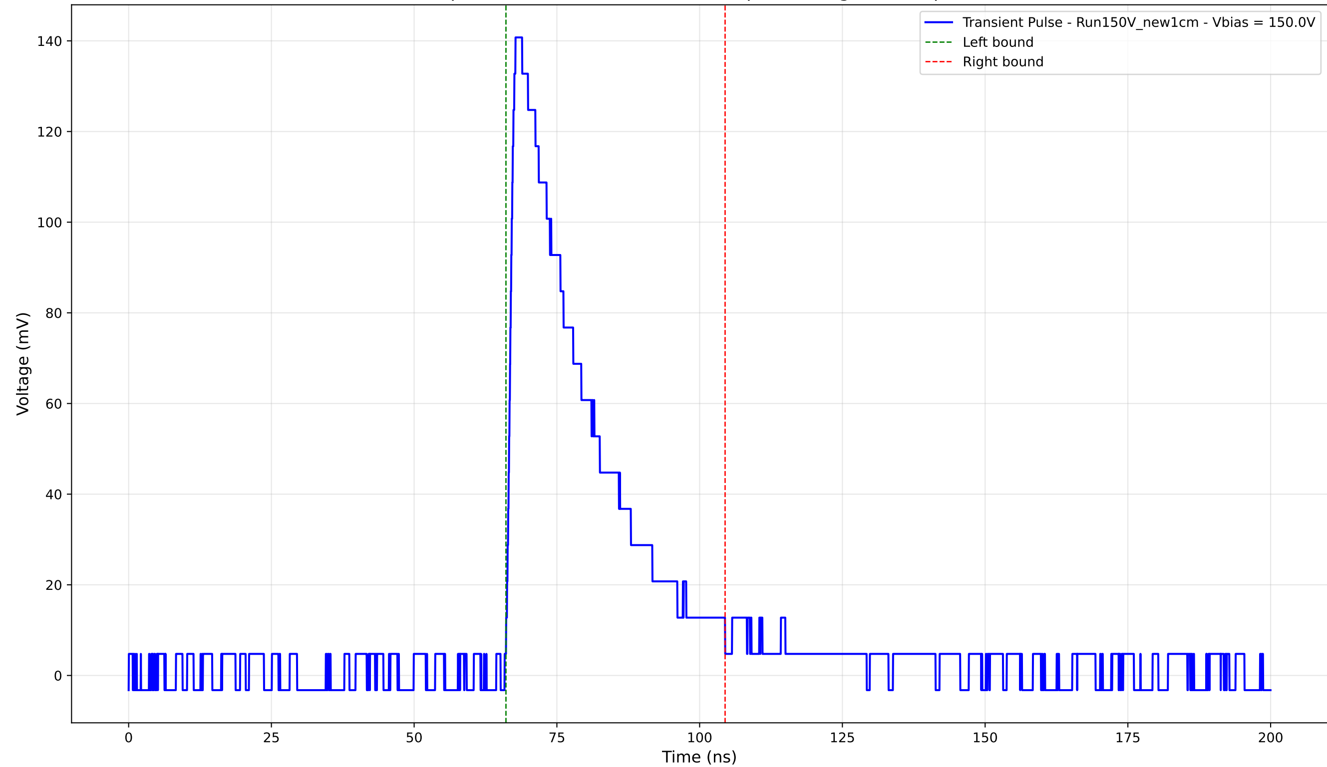
Transient Pulse - Sample: New1cm - Position: 3700.0 \mu\text{m} - Charge: 40.71 pC - Rise Time: 1.30 ns
