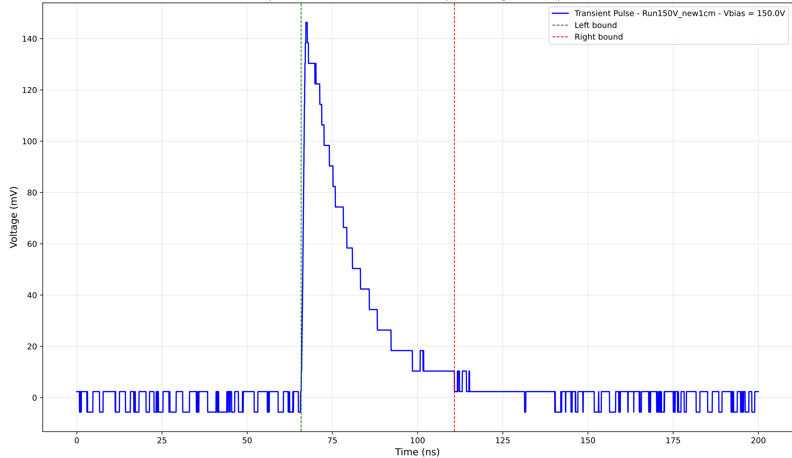
Transient Pulse - Sample: New1cm - Position: 3210.0 \mu\text{m} - Charge: 41.70 pC - Rise Time: 1.07 ns
