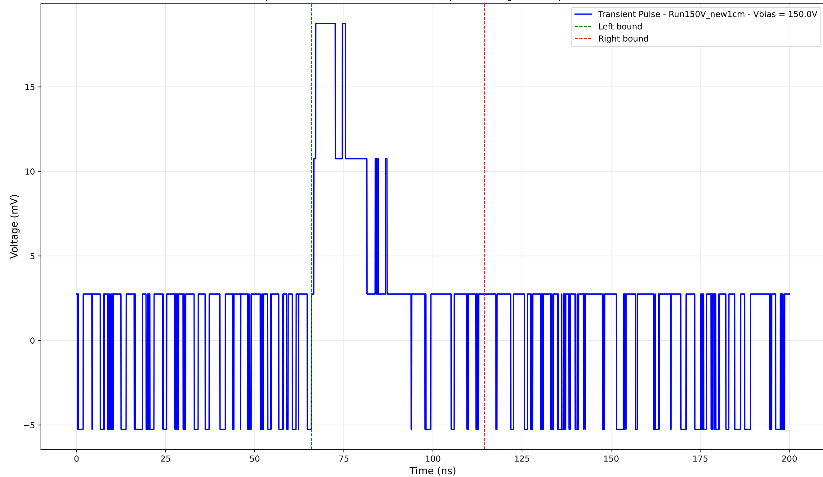
Transient Pulse - Sample: New1cm - Position: 1050.0 \mu\text{m} - Charge: 5.72 pC - Rise Time: 0.00 ns (N/A)
