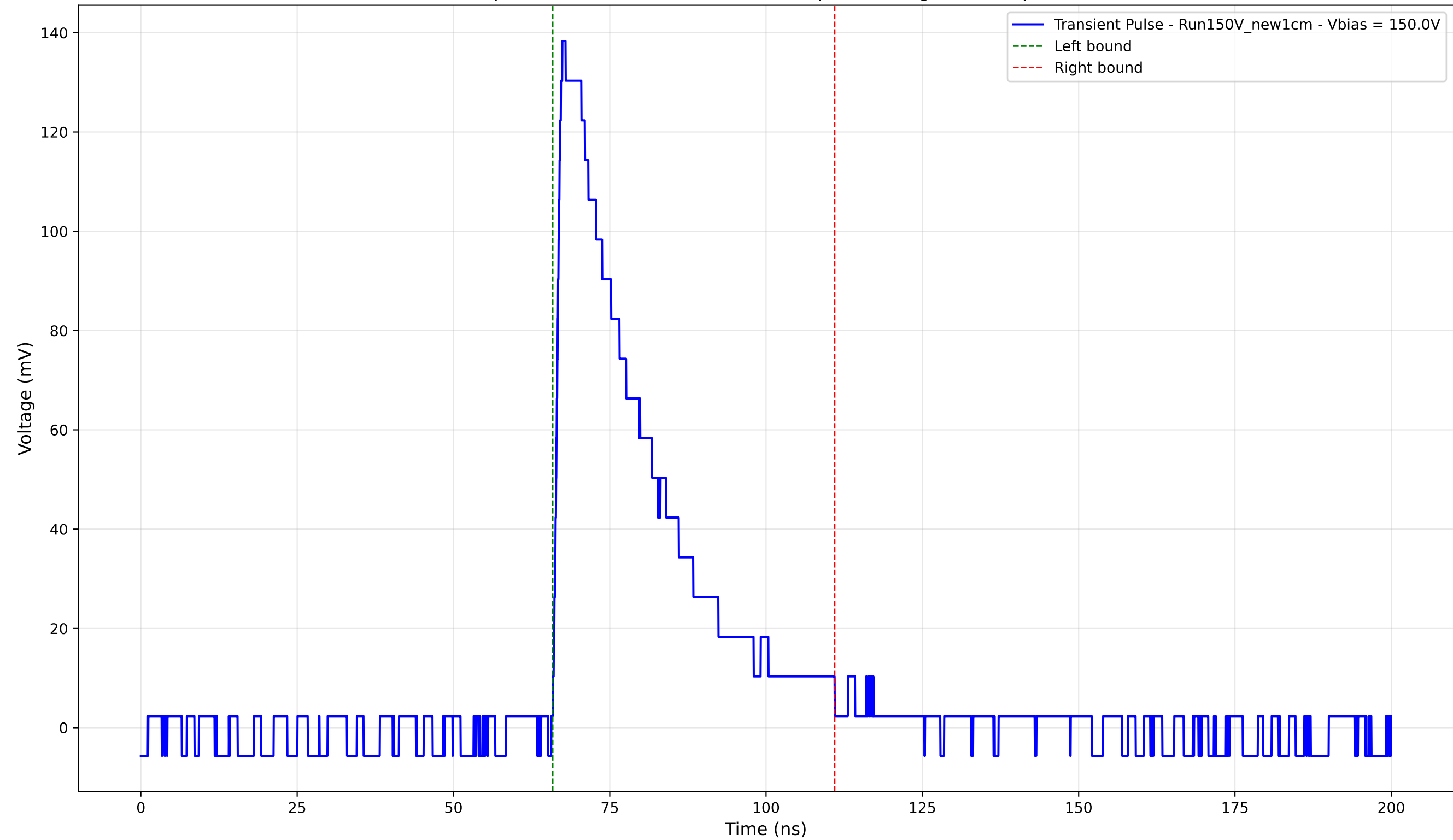
Transient Pulse - Sample: New1cm - Position: 3325.0 \mu\text{m} - Charge: 41.63 pC - Rise Time: 1.15 ns
