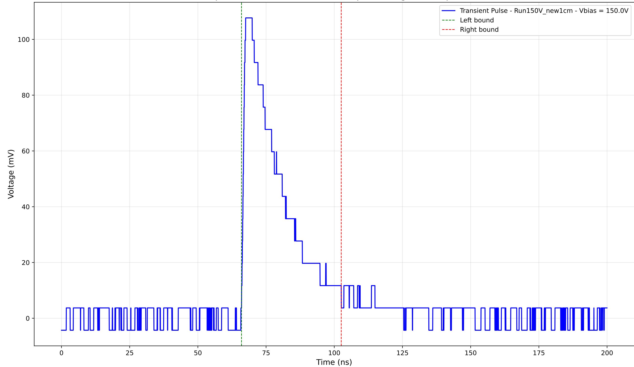
Transient Pulse - Sample: New1cm - Position: 1680.0 \mu\text{m} - Charge: 32.10 pC - Rise Time: 1.26 ns
