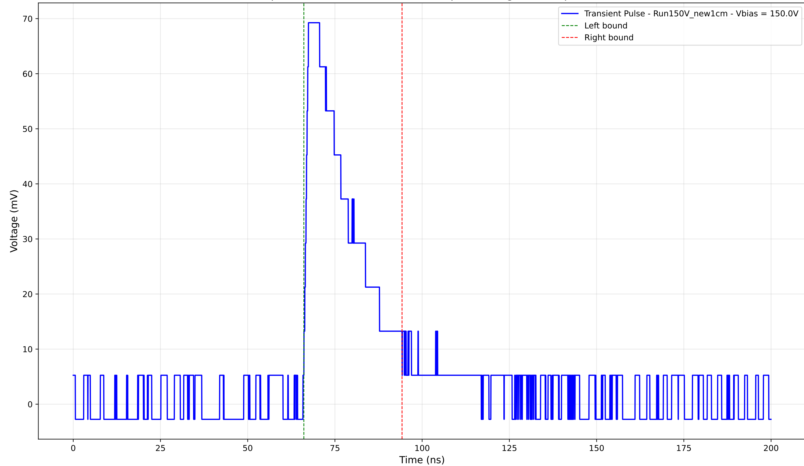
Transient Pulse - Sample: New1cm - Position: 4015.0 \mu\text{m} - Charge: 19.80 pC - Rise Time: 1.30 ns
