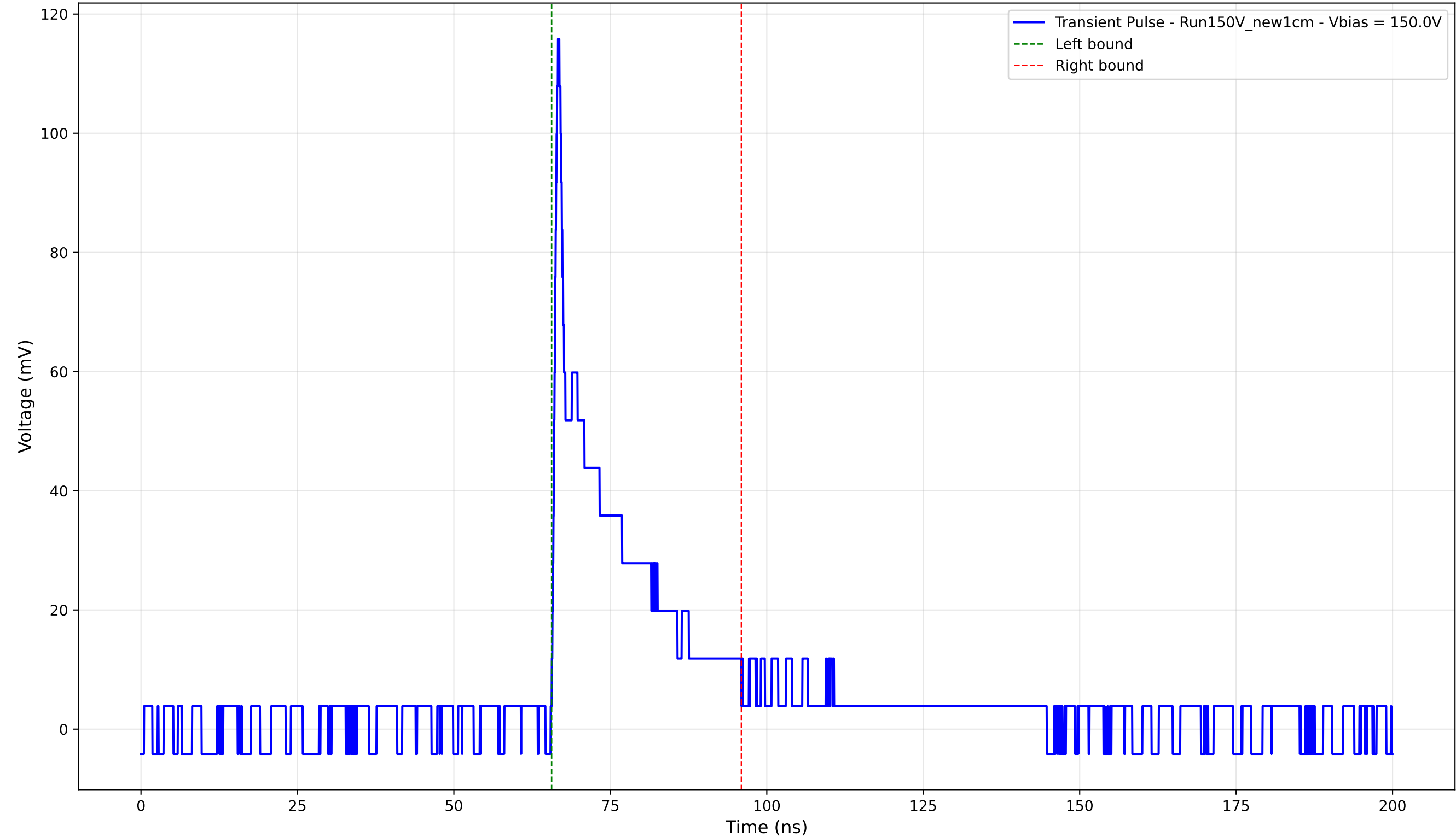
Transient Pulse - Sample: New1cm - Position: 2605.0 \mu\text{m} - Charge: 18.30 pC - Rise Time: 0.84 ns
