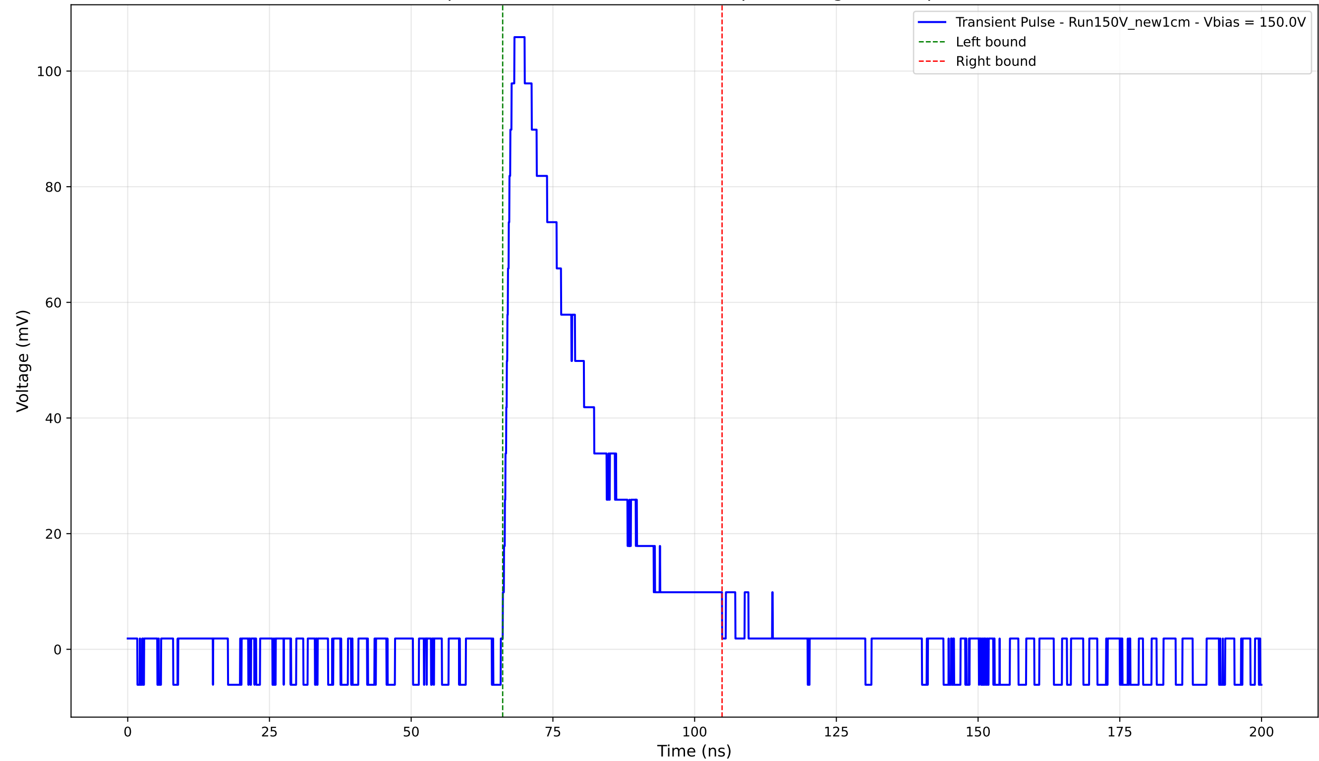
Transient Pulse - Sample: New1cm - Position: 1250.0 \mu\text{m} - Charge: 30.64 pC - Rise Time: 1.36 ns
