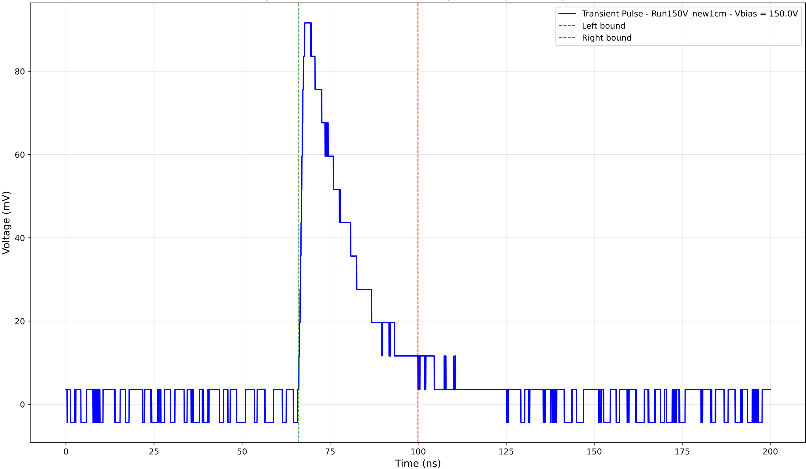
Transient Pulse - Sample: New1cm - Position: 3625.0 \mu\text{m} - Charge: 26.10 pC - Rise Time: 1.29 ns
