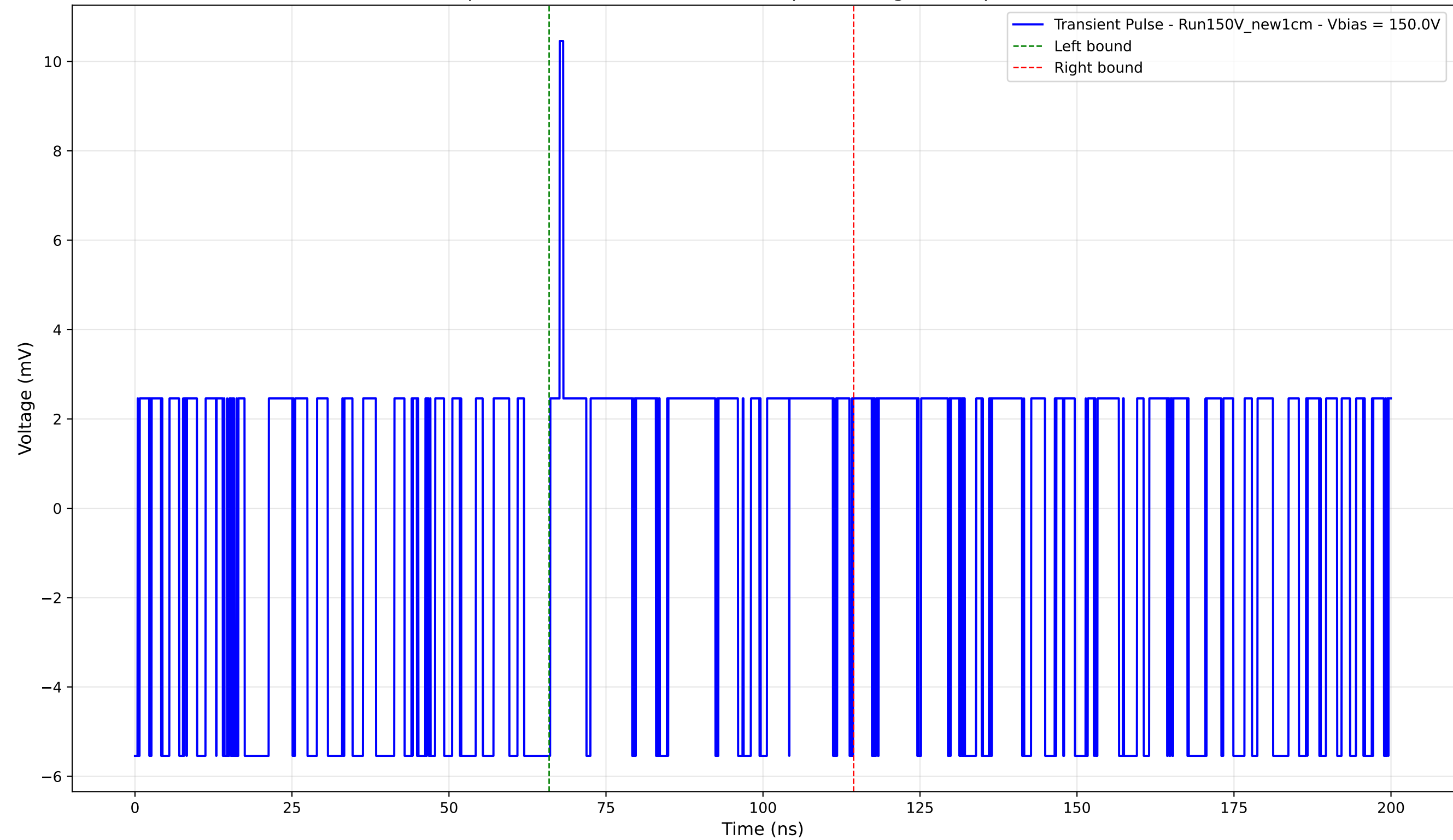
Transient Pulse - Sample: New1cm - Position: 4915.0 \mu\text{m} - Charge: 1.32 pC - Rise Time: 0.00 ns (N/A)
