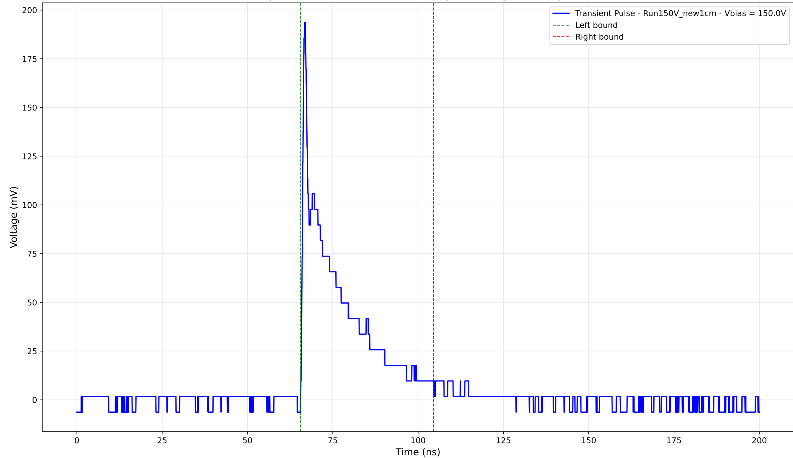
Transient Pulse - Sample: New1cm - Position: 2415.0 \mu\text{m} - Charge: 33.94 pC - Rise Time: 0.76 ns
