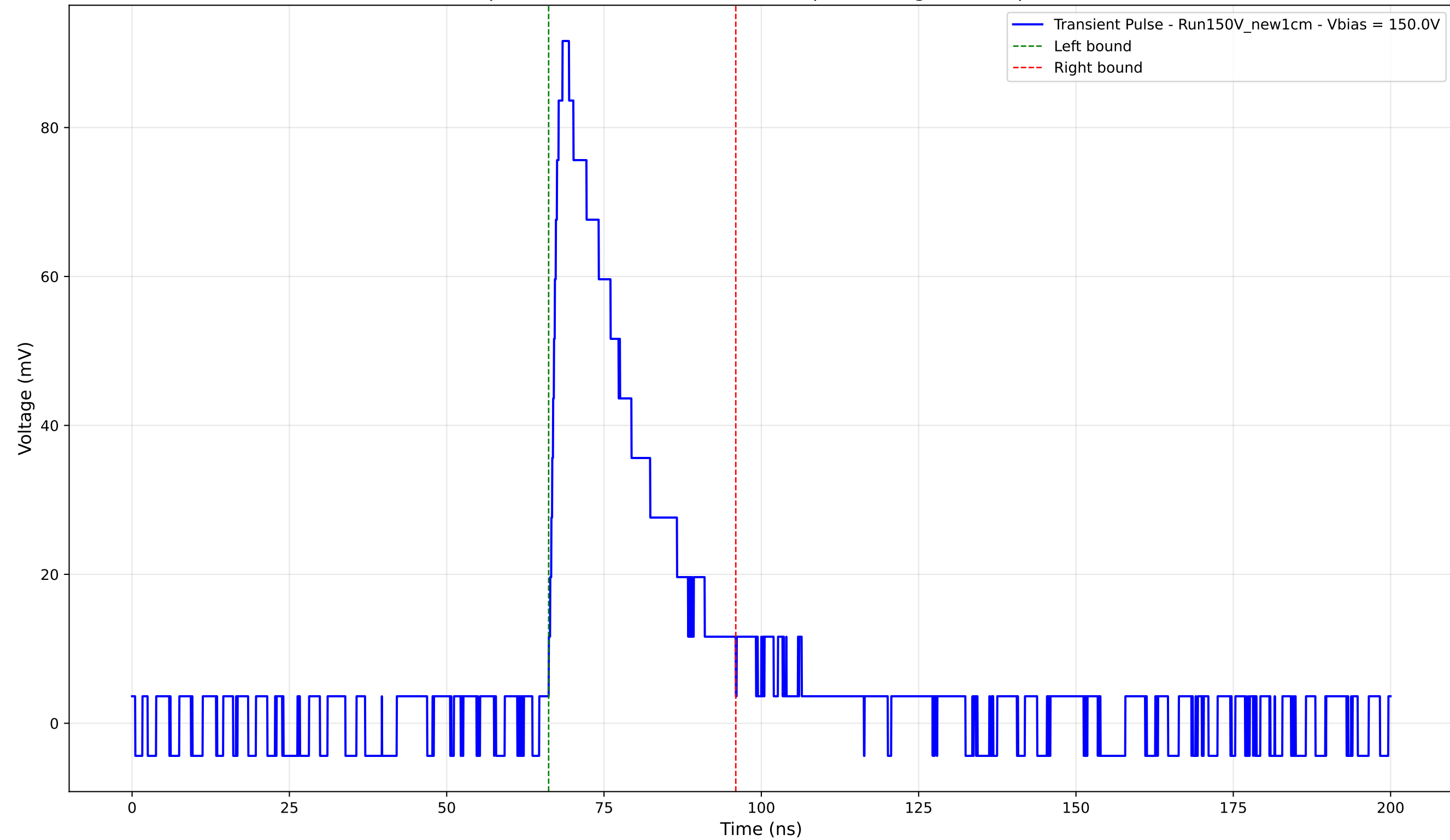
Transient Pulse - Sample: New1cm - Position: 1120.0 \mu\text{m} - Charge: 23.91 pC - Rise Time: 1.57 ns
