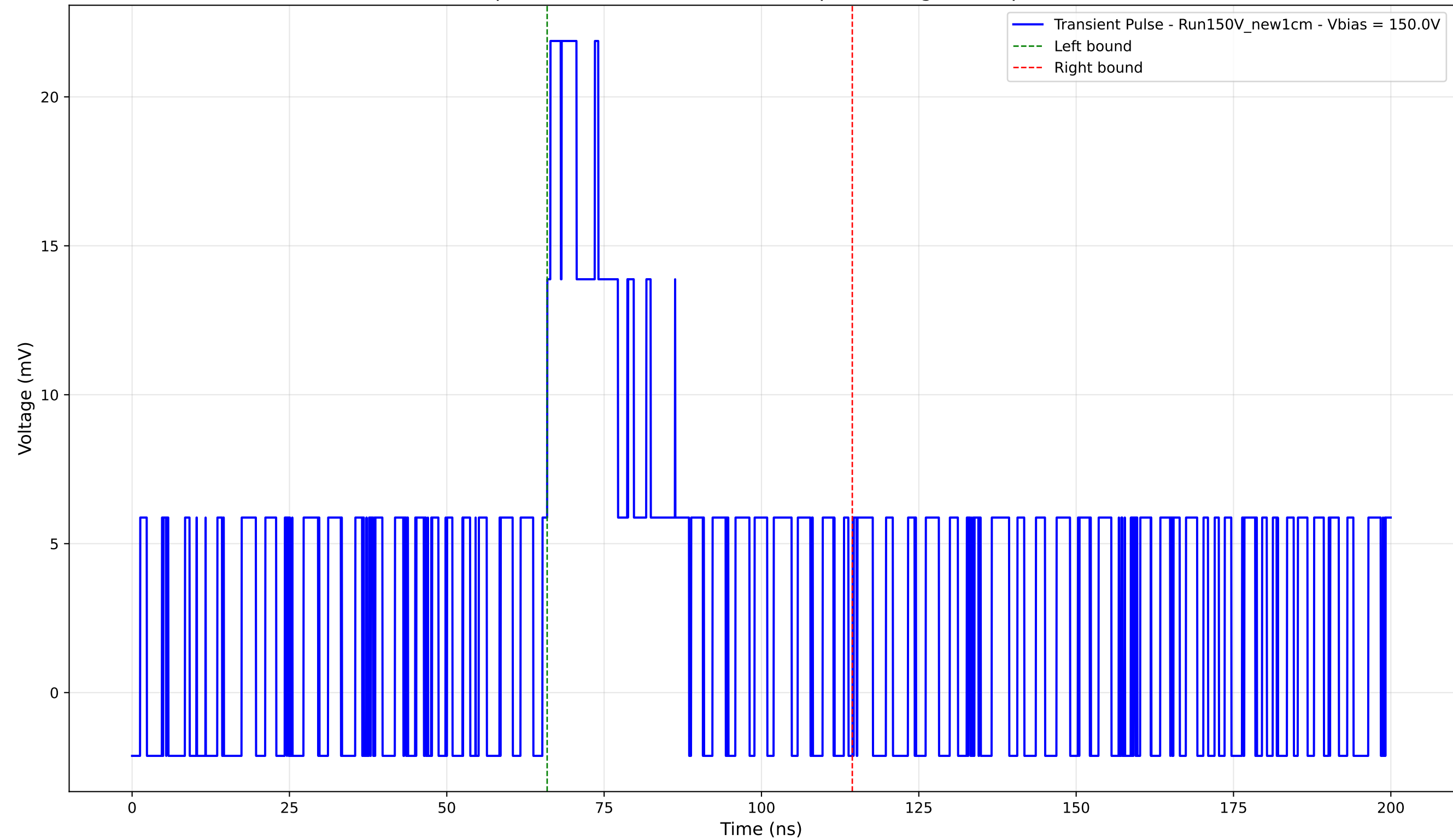
Transient Pulse - Sample: New1cm - Position: 4575.0 \mu\text{m} - Charge: 6.94 pC - Rise Time: 1.28 ns
