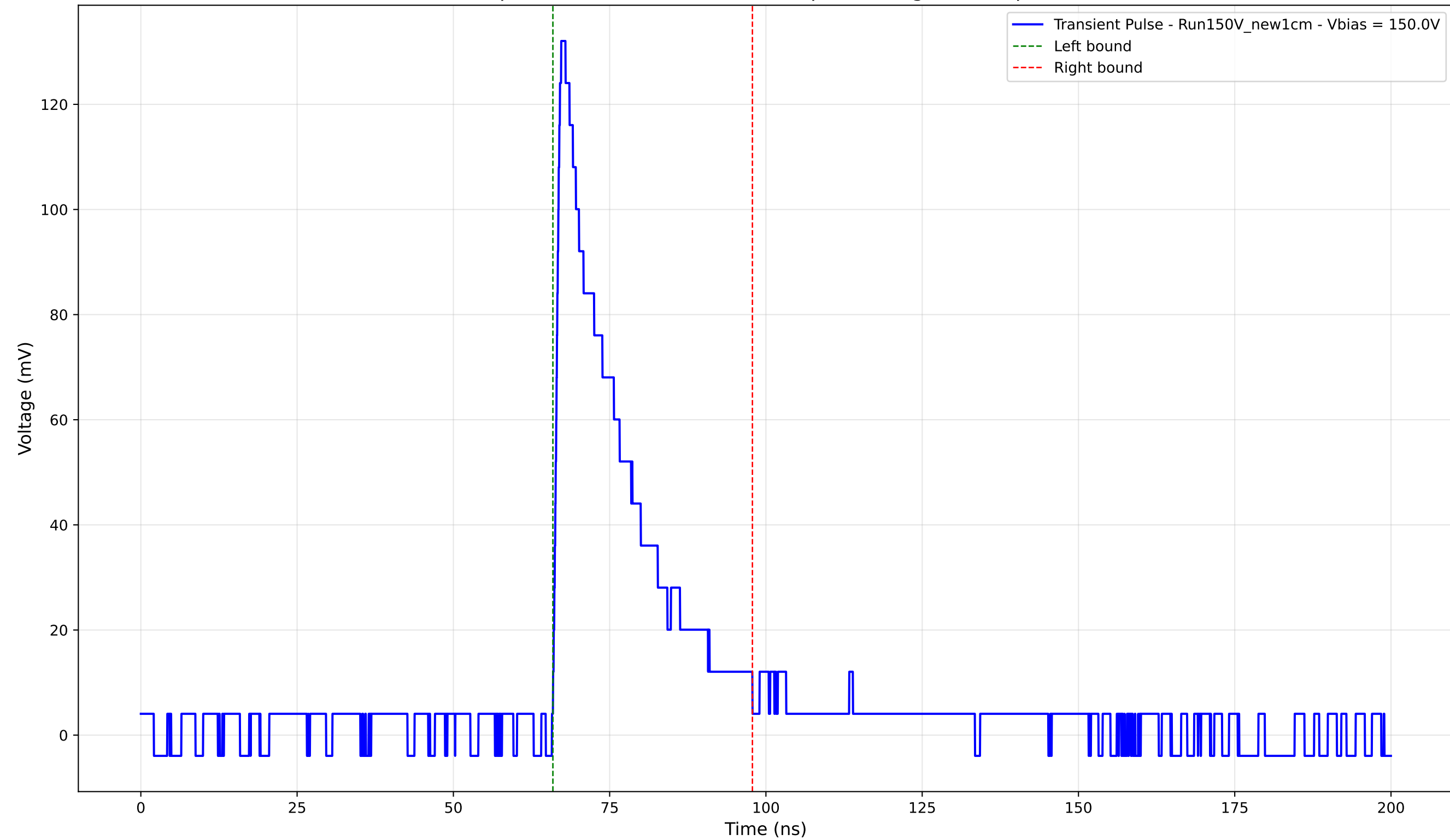
Transient Pulse - Sample: New1cm - Position: 355.0 \mu\text{m} - Charge: 29.12 pC - Rise Time: 1.02 ns
