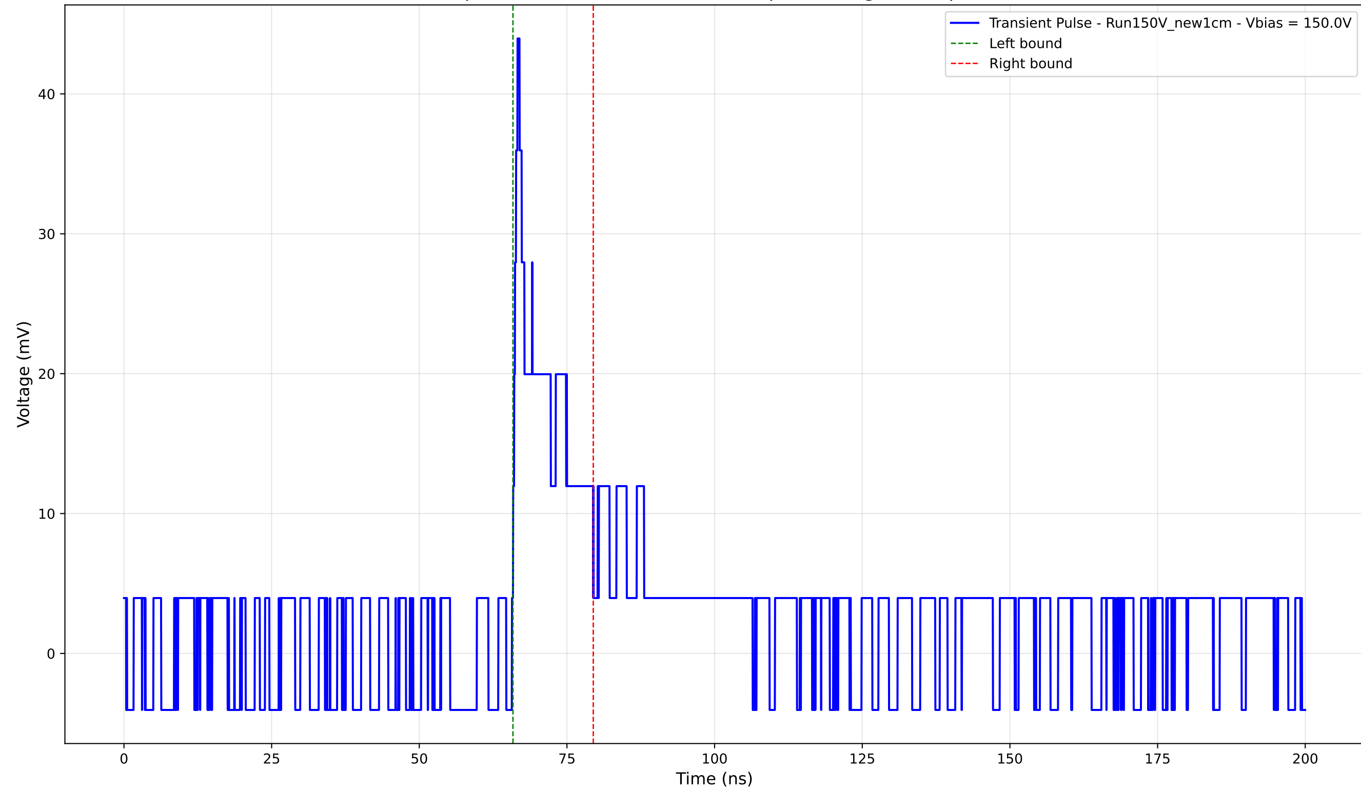
Transient Pulse - Sample: New1cm - Position: 2570.0 \mu\text{m} - Charge: 5.00 pC - Rise Time: 0.76 ns
