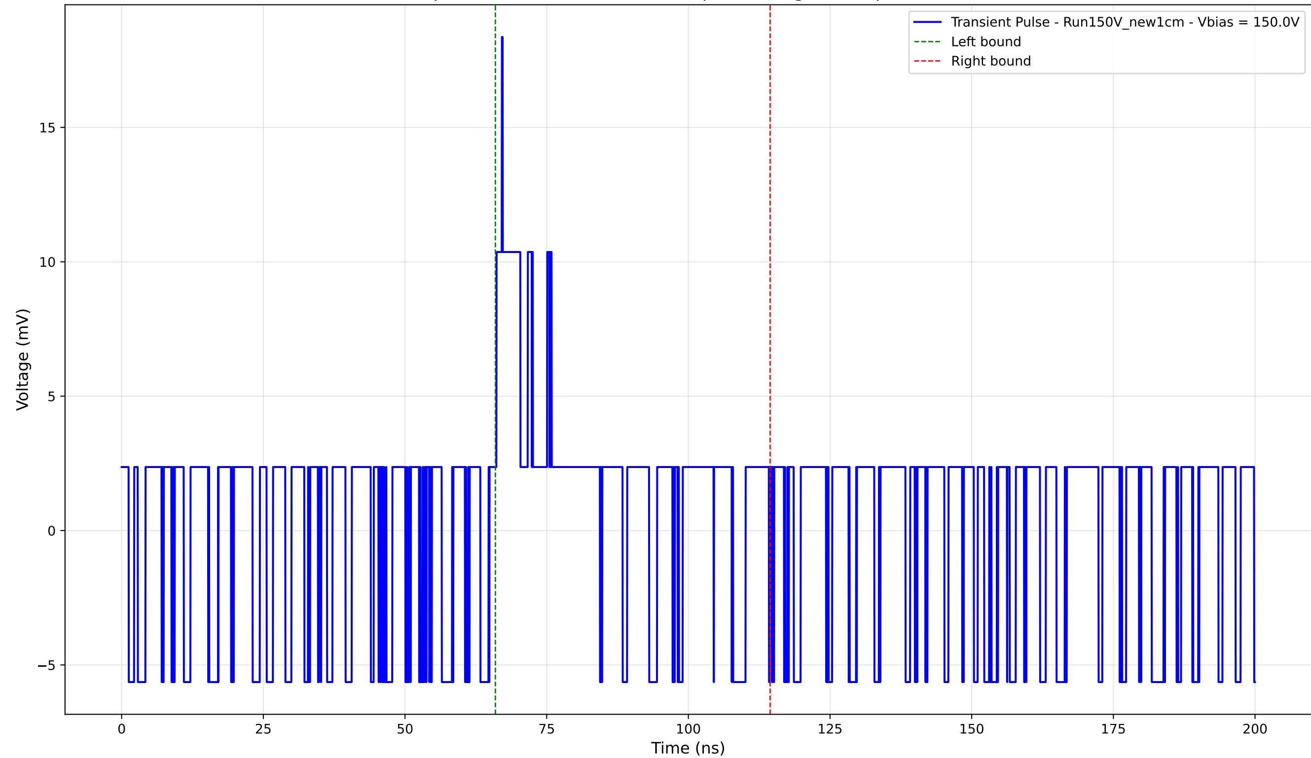
Transient Pulse - Sample: New1cm - Position: 35.0 \mu\text{m} - Charge: 2.27 pC - Rise Time: 0.00 ns (N/A)
