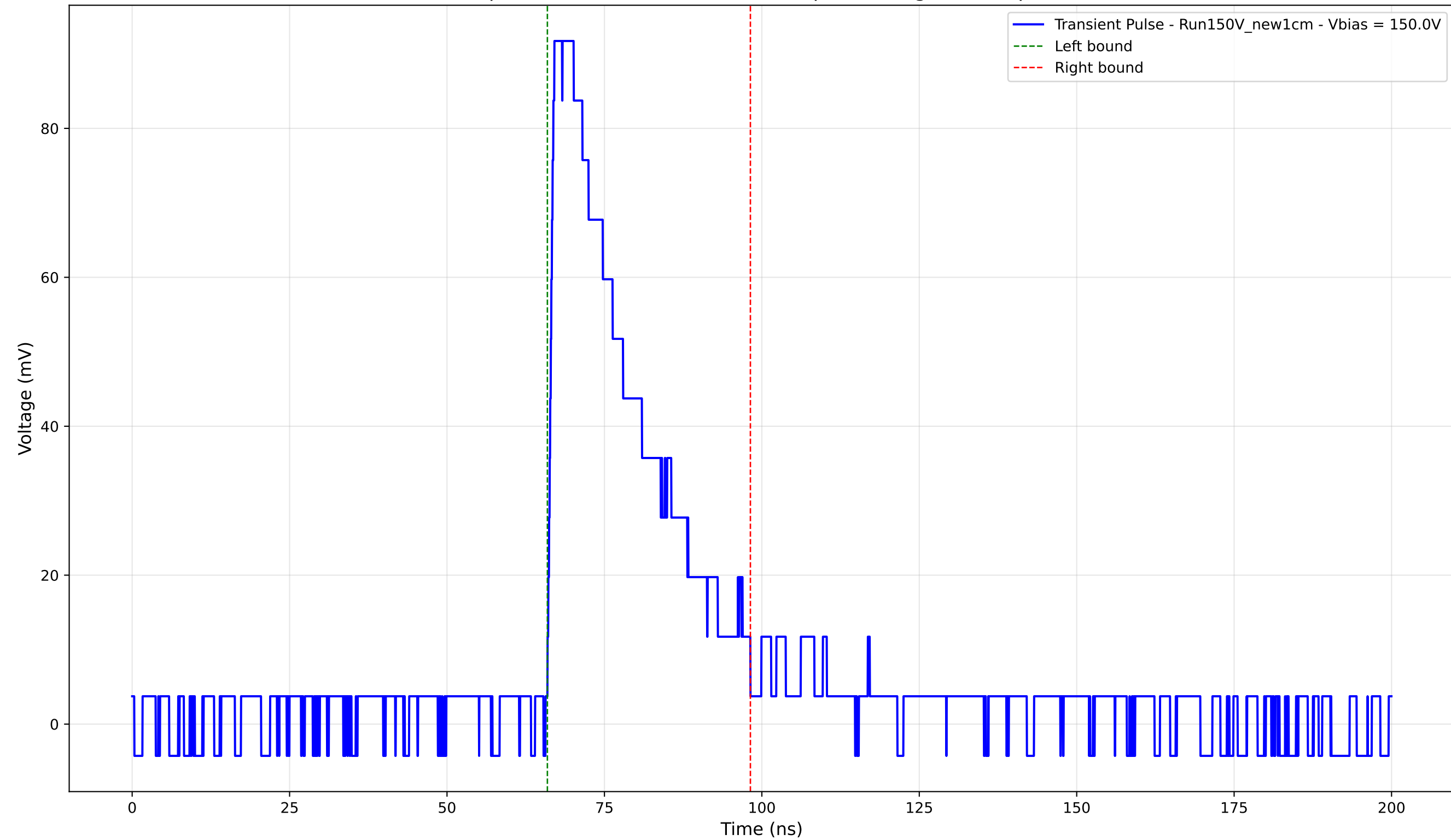
Transient Pulse - Sample: New1cm - Position: 1910.0 \mu\text{m} - Charge: 27.58 pC - Rise Time: 0.93 ns
