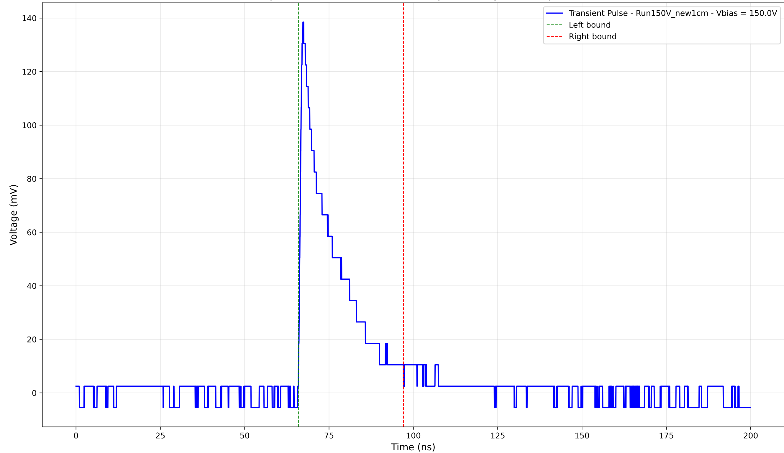
Transient Pulse - Sample: New1cm - Position: 285.0 \mu\text{m} - Charge: 27.57 pC - Rise Time: 0.99 ns
