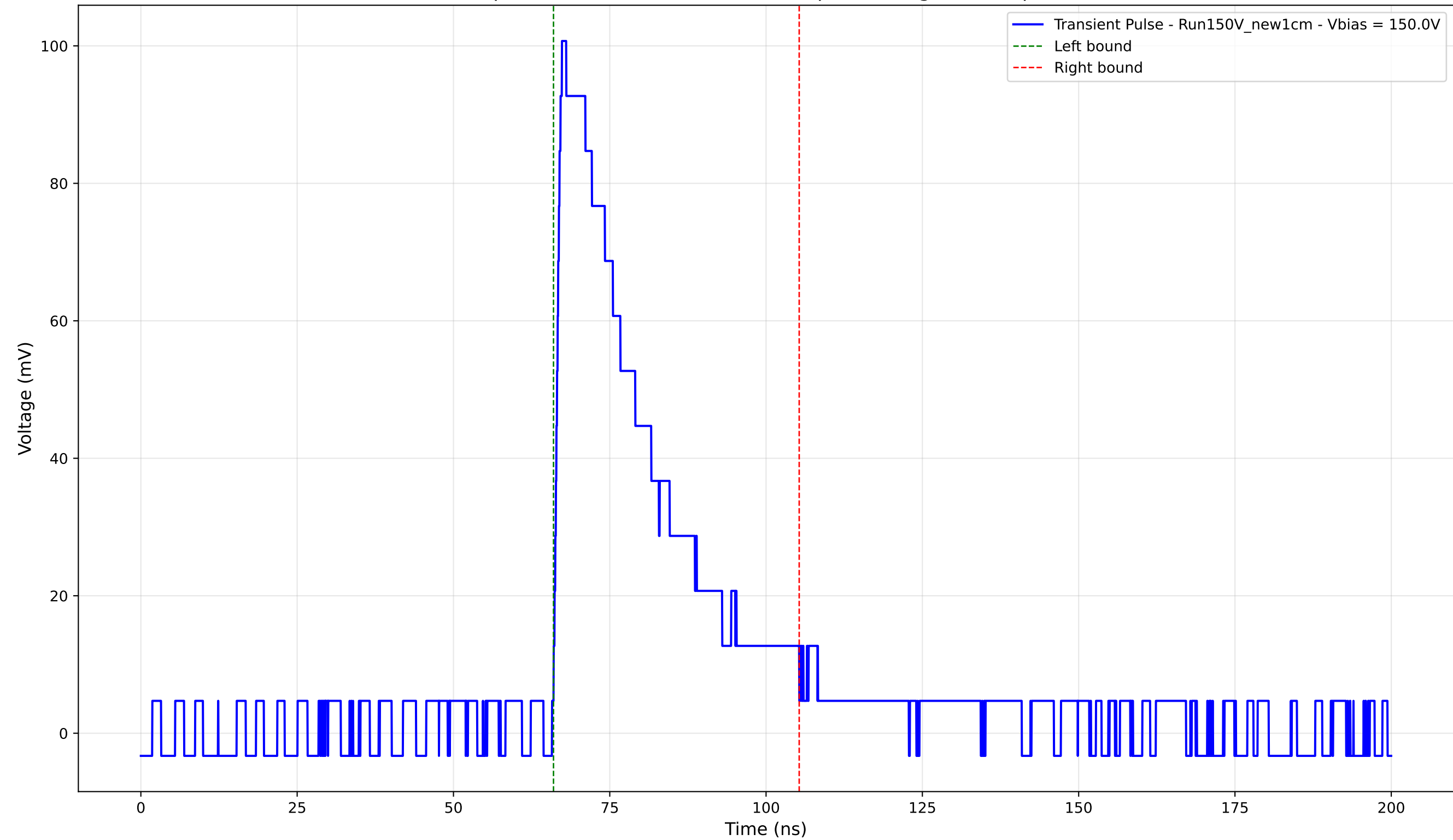
Transient Pulse - Sample: New1cm - Position: 1785.0 \mu\text{m} - Charge: 31.08 pC - Rise Time: 1.11 ns
