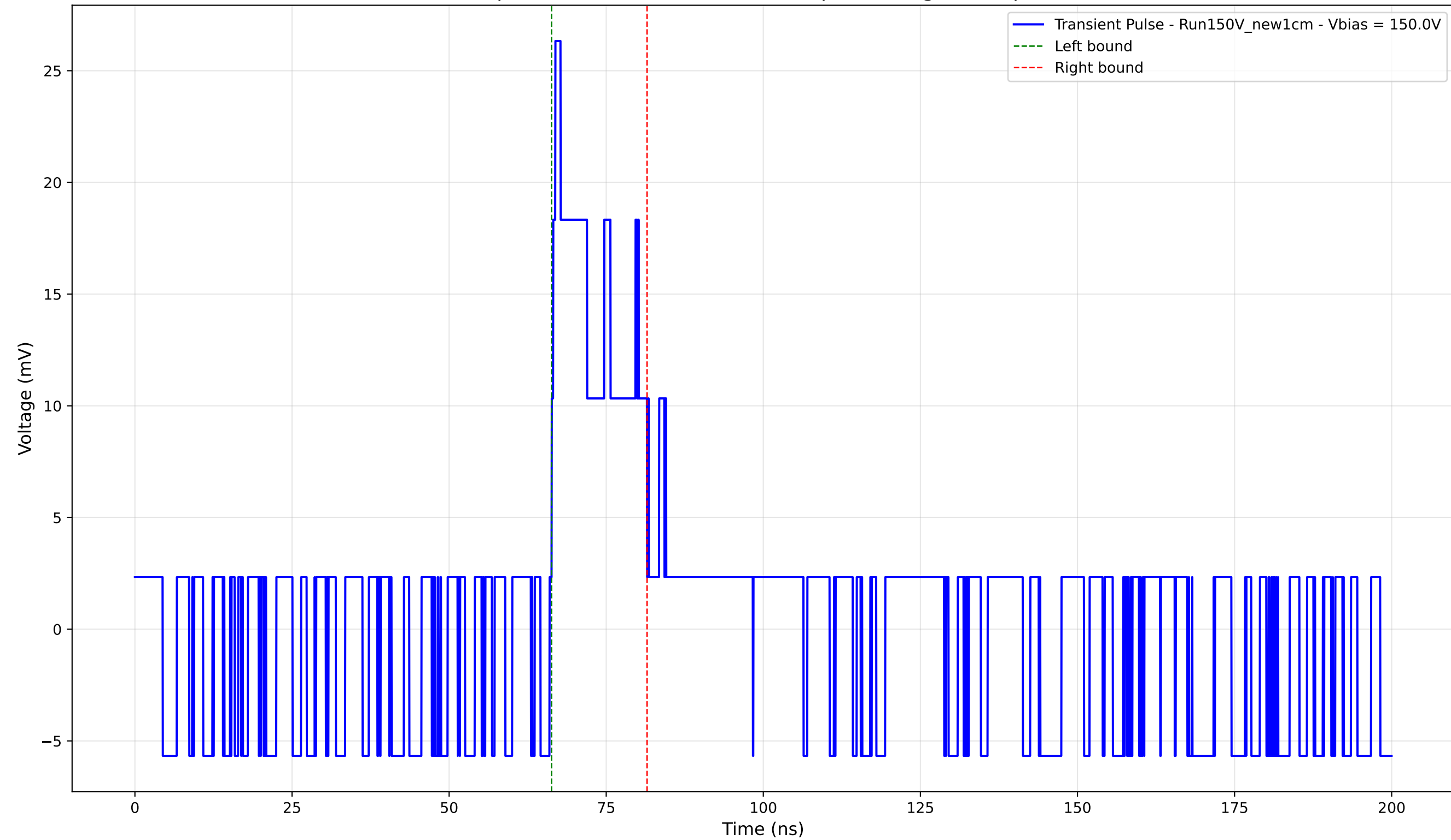
Transient Pulse - Sample: New1cm - Position: 2015.0 \mu\text{m} - Charge: 4.35 pC - Rise Time: 0.60 ns
