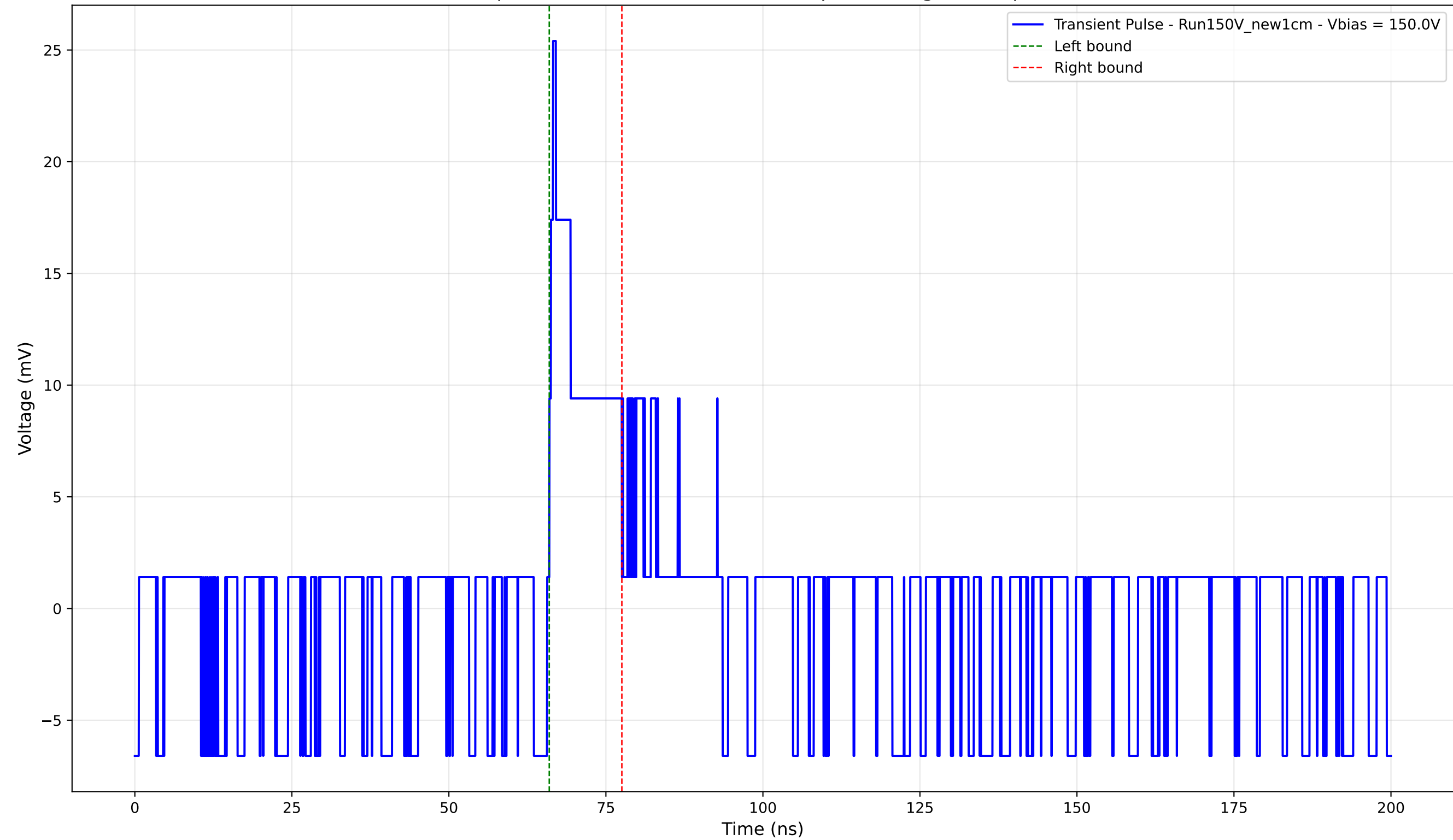
Transient Pulse - Sample: New1cm - Position: 2555.0 \mu\text{m} - Charge: 2.75 pC - Rise Time: 0.60 ns
