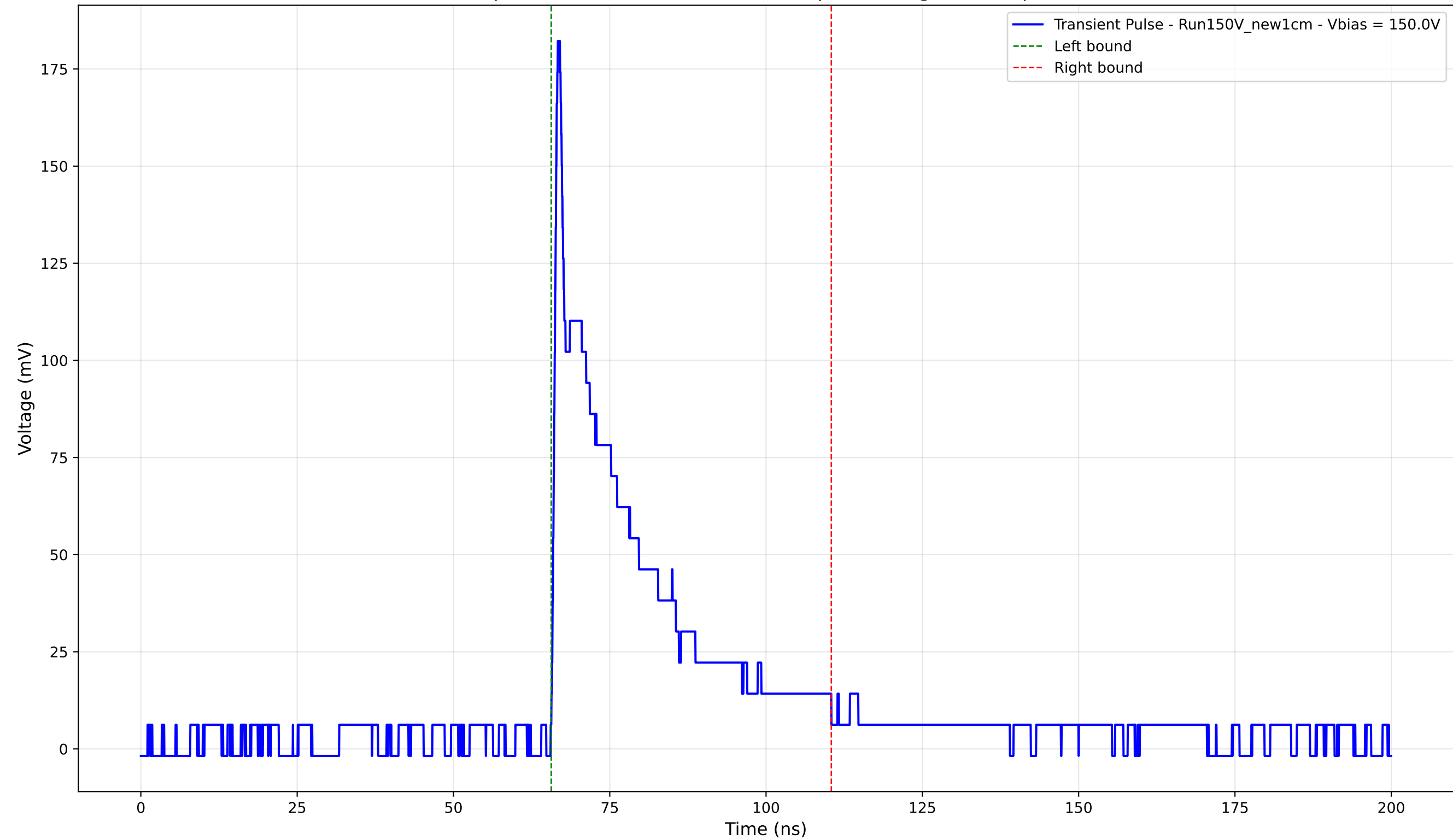
Transient Pulse - Sample: New1cm - Position: 2365.0 \mu\text{m} - Charge: 39.17 pC - Rise Time: 0.79 ns
