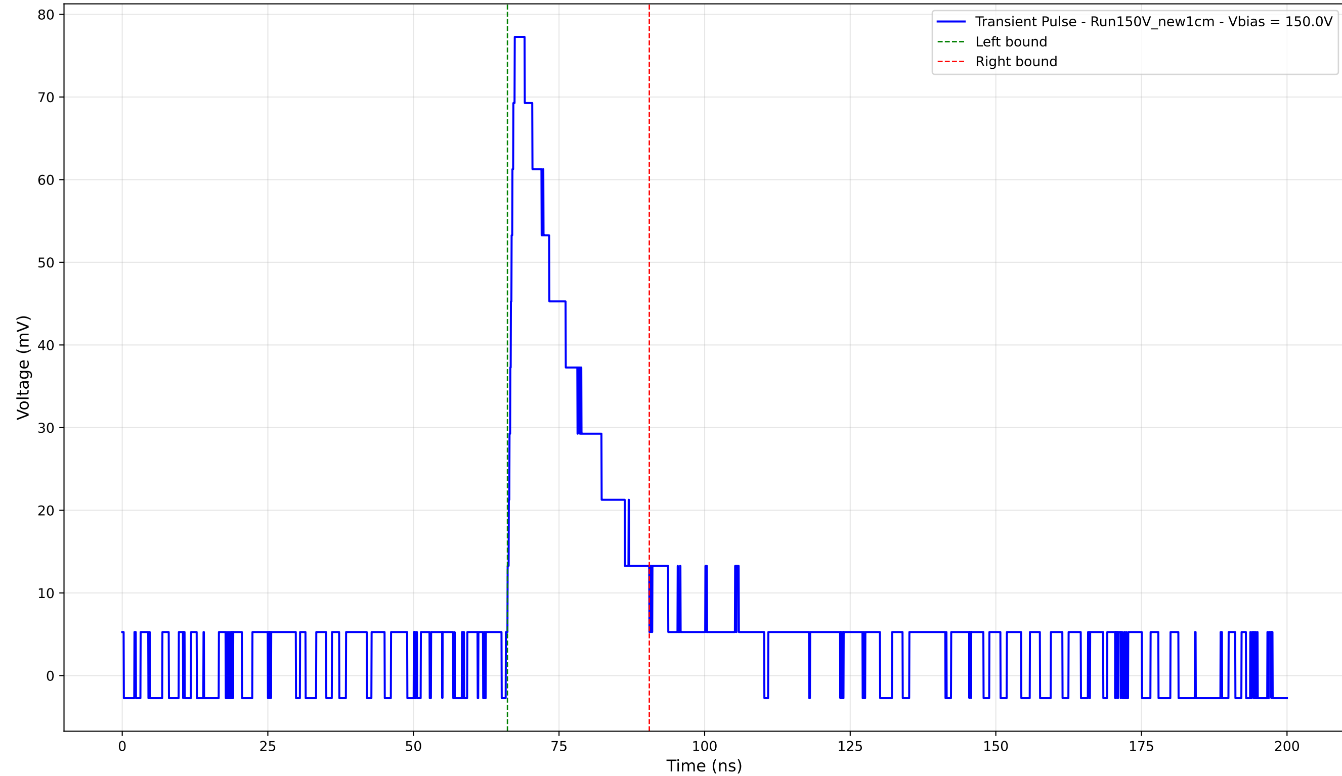
Transient Pulse - Sample: New1cm - Position: 600.0 \mu\text{m} - Charge: 18.27 pC - Rise Time: 1.23 ns
