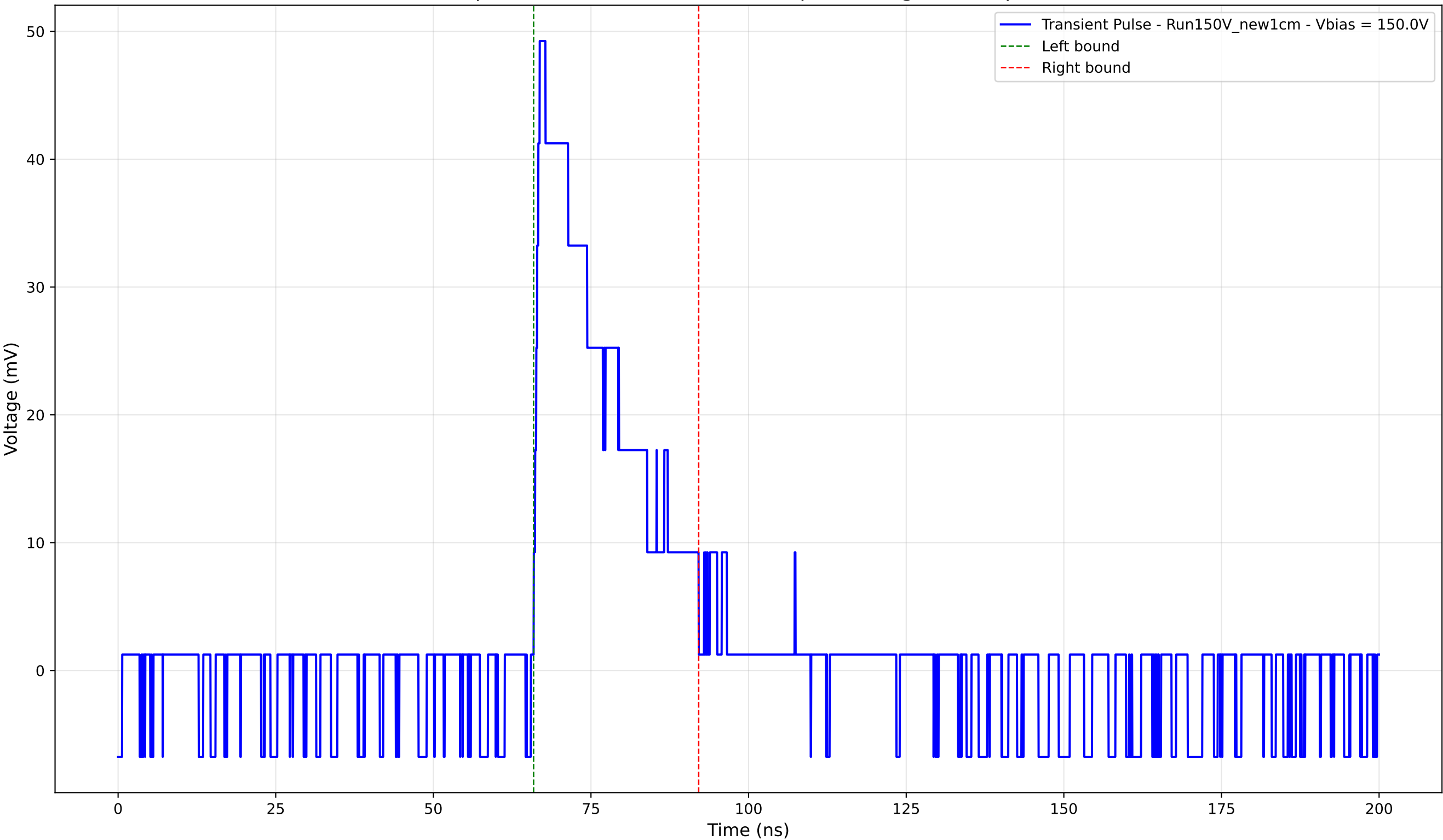
Transient Pulse - Sample: New1cm - Position: 1990.0 \mu\text{m} - Charge: 12.02 pC - Rise Time: 0.95 ns
