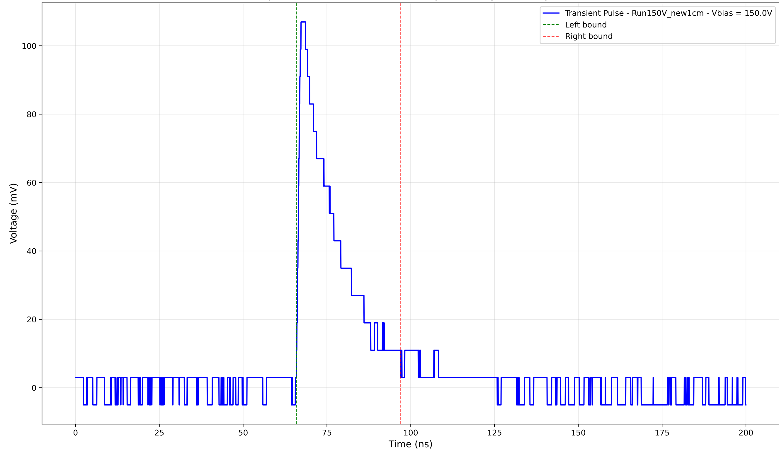
Transient Pulse - Sample: New1cm - Position: 435.0 \mu\text{m} - Charge: 25.29 pC - Rise Time: 1.16 ns
