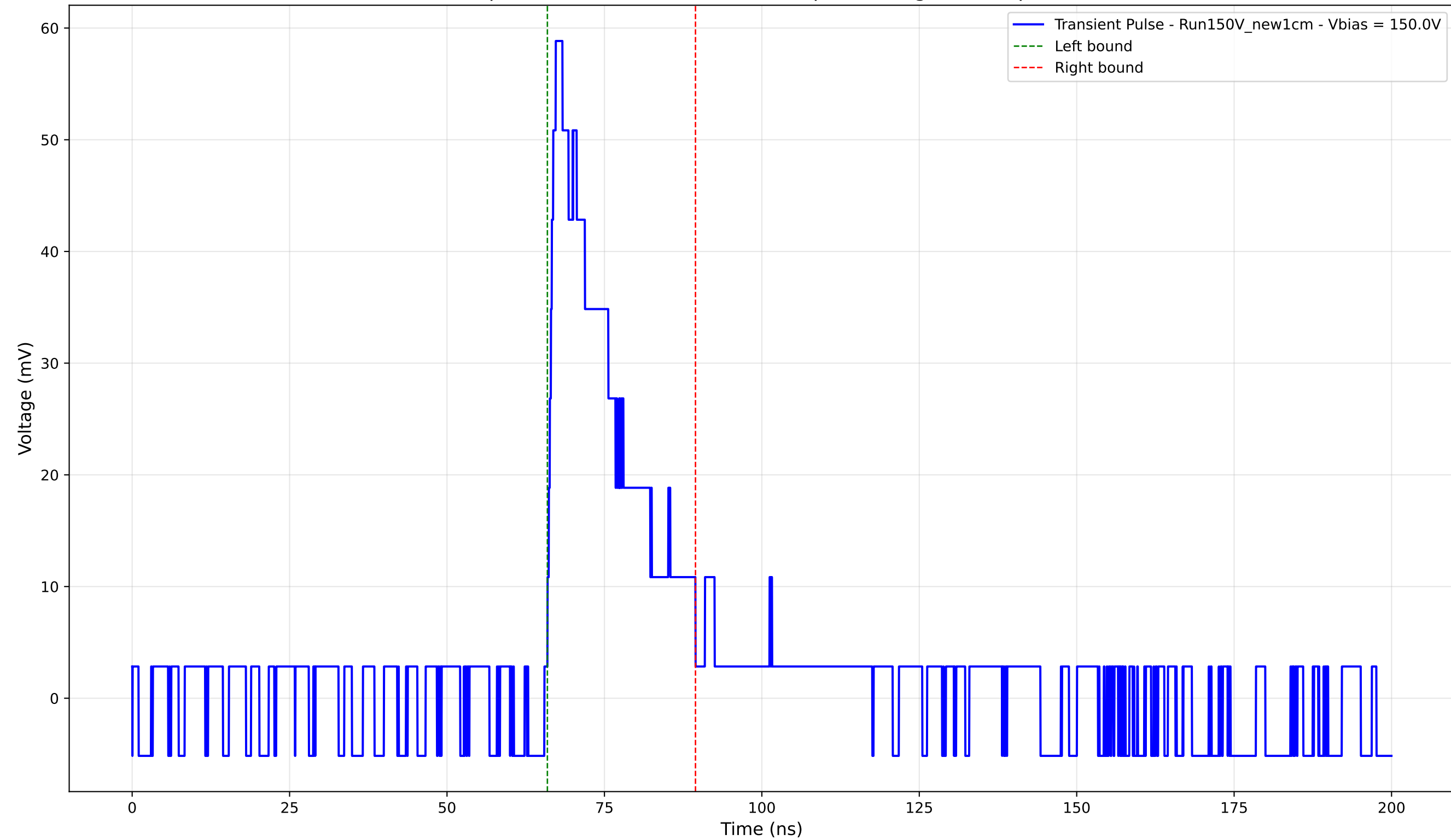
Transient Pulse - Sample: New1cm - Position: 4530.0 \mu\text{m} - Charge: 12.44 pC - Rise Time: 1.31 ns
