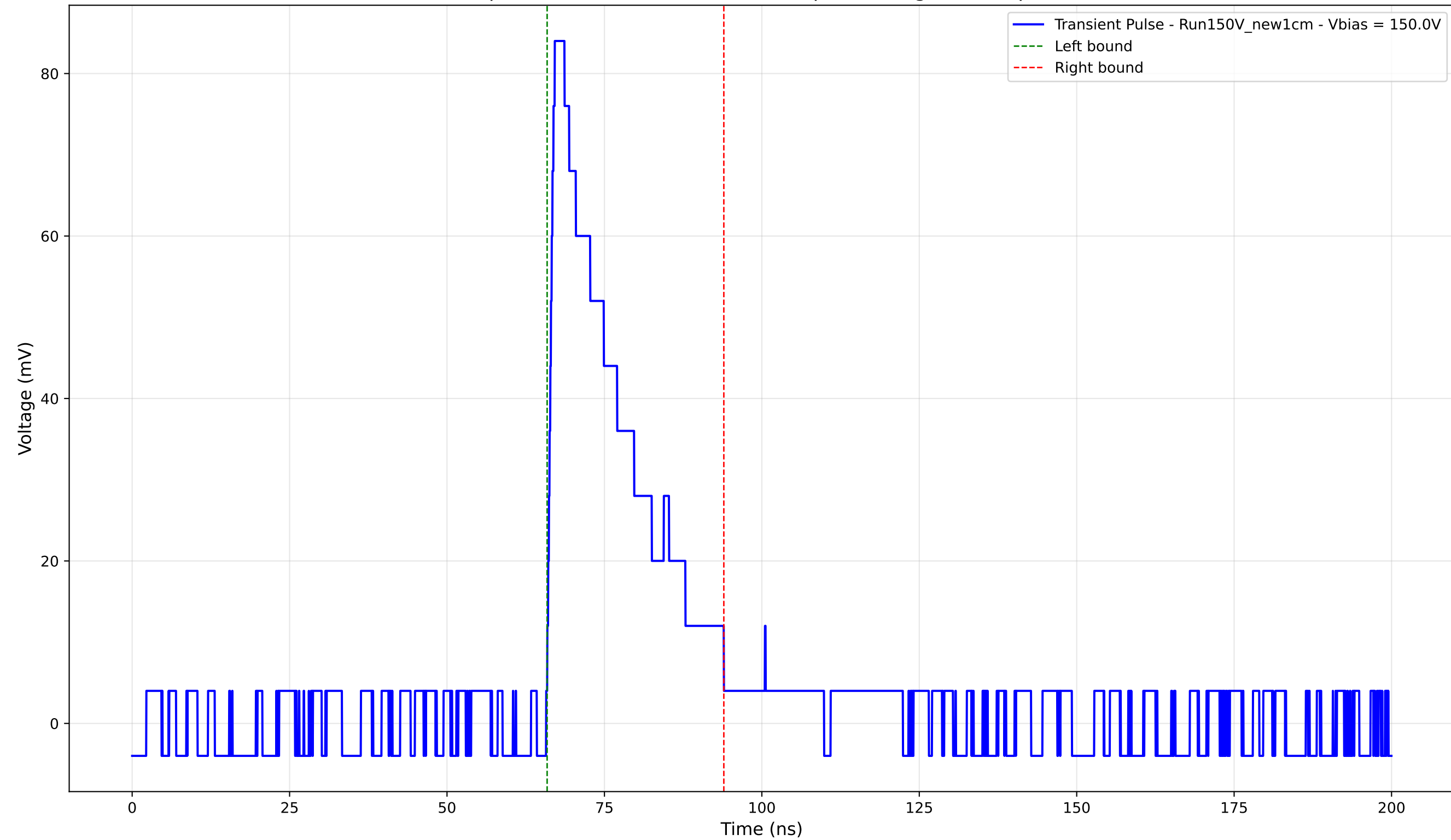
Transient Pulse - Sample: New1cm - Position: 4515.0 \mu\text{m} - Charge: 20.39 pC - Rise Time: 0.99 ns
