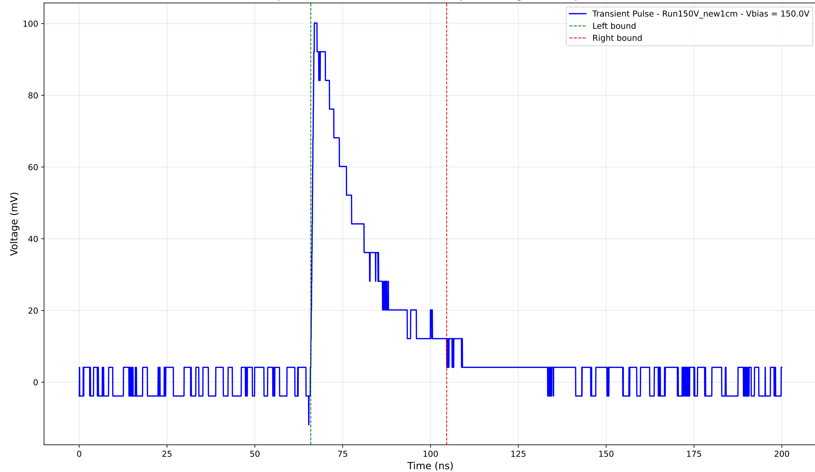
Transient Pulse - Sample: New1cm - Position: 3135.0 \mu\text{m} - Charge: 29.58 pC - Rise Time: 0.85 ns
