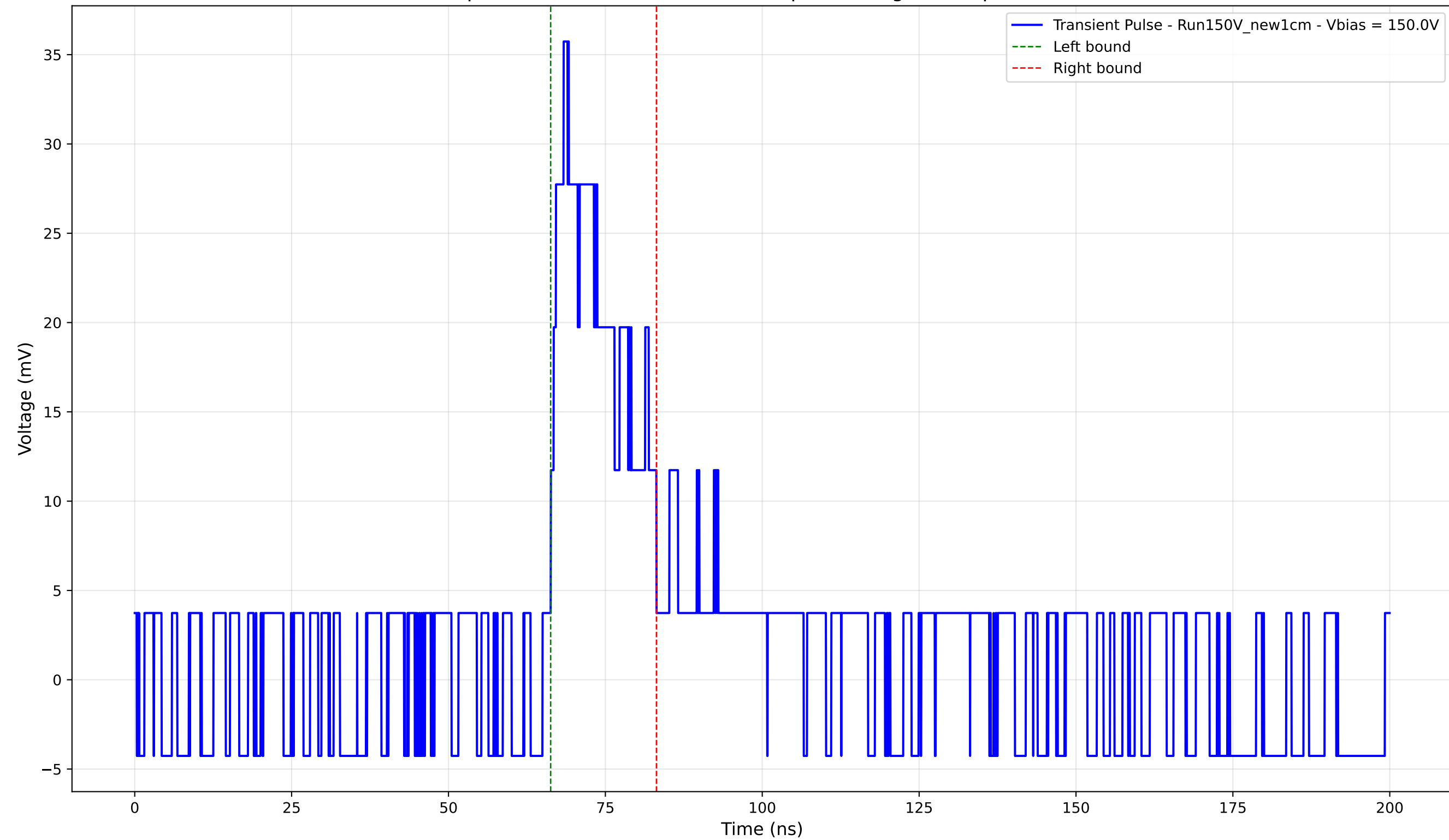
Transient Pulse - Sample: New1cm - Position: 4090.0 \mu\text{m} - Charge: 6.98 pC - Rise Time: 0.00 ns (N/A)
