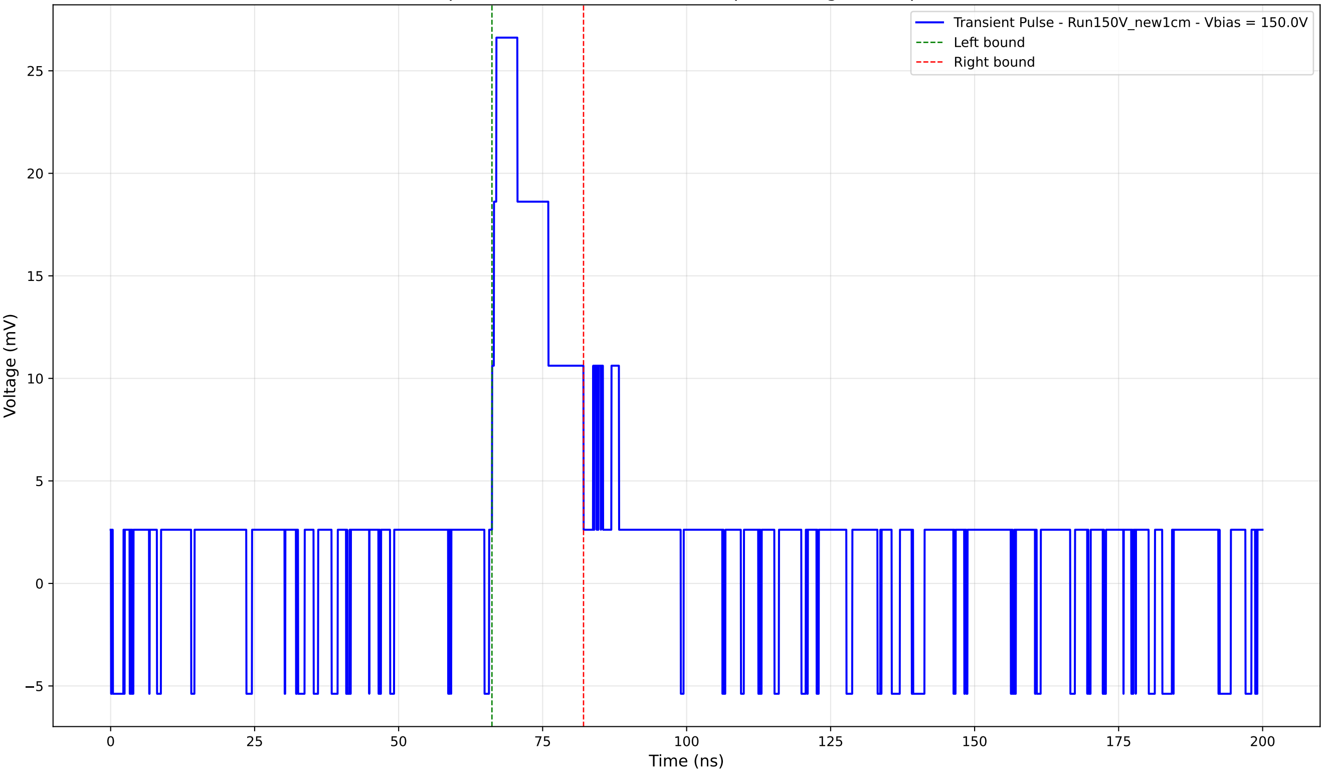
Transient Pulse - Sample: New1cm - Position: 505.0 \mu\text{m} - Charge: 5.47 pC - Rise Time: 0.76 ns
