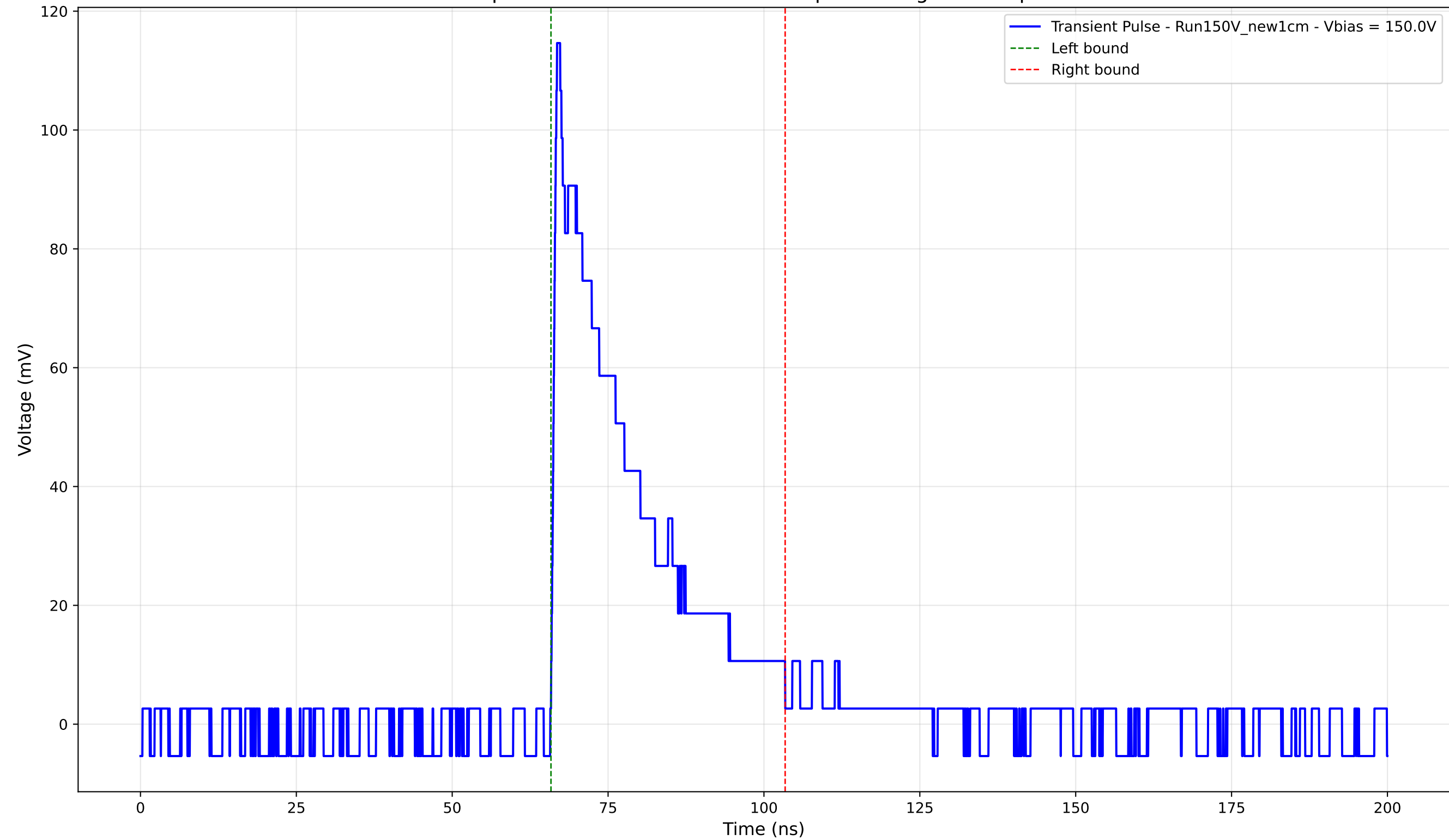
Transient Pulse - Sample: New1cm - Position: 2145.0 \mu\text{m} - Charge: 27.97 pC - Rise Time: 0.78 ns
