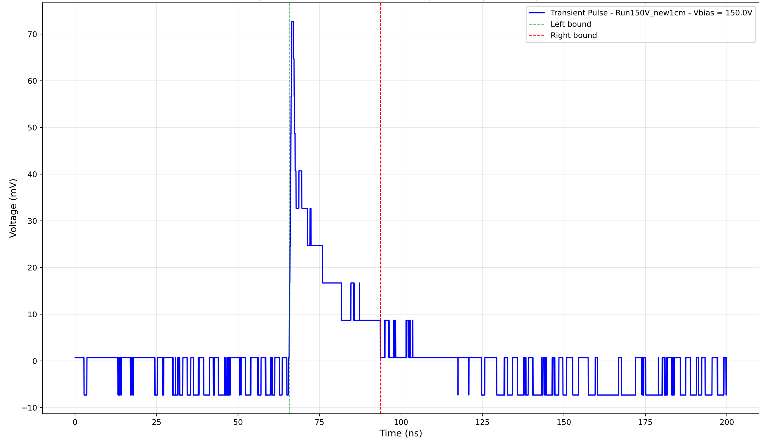
Transient Pulse - Sample: New1cm - Position: 2510.0 \mu\text{m} - Charge: 11.03 pC - Rise Time: 0.80 ns
