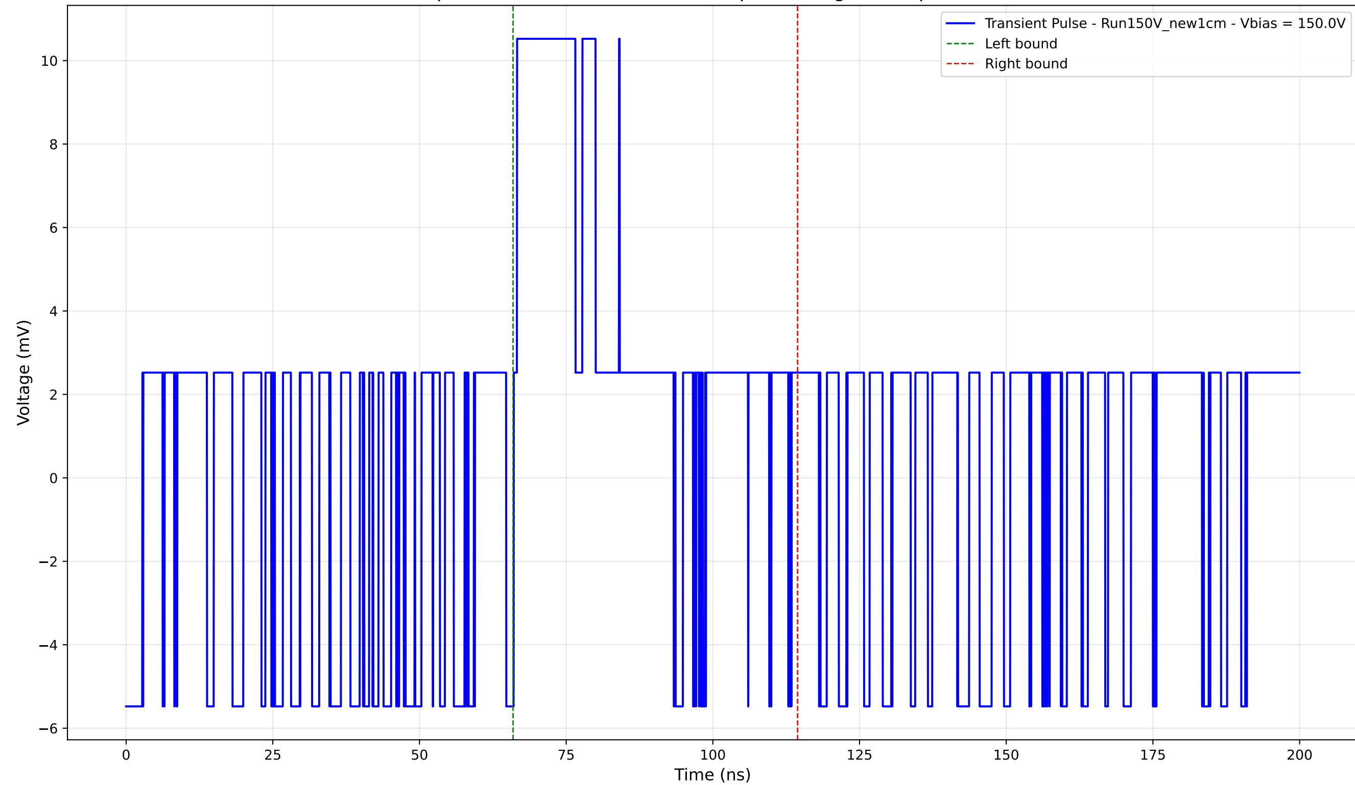
Transient Pulse - Sample: New1cm - Position: 1540.0 \mu\text{m} - Charge: 3.94 pC - Rise Time: 0.00 ns (N/A)
