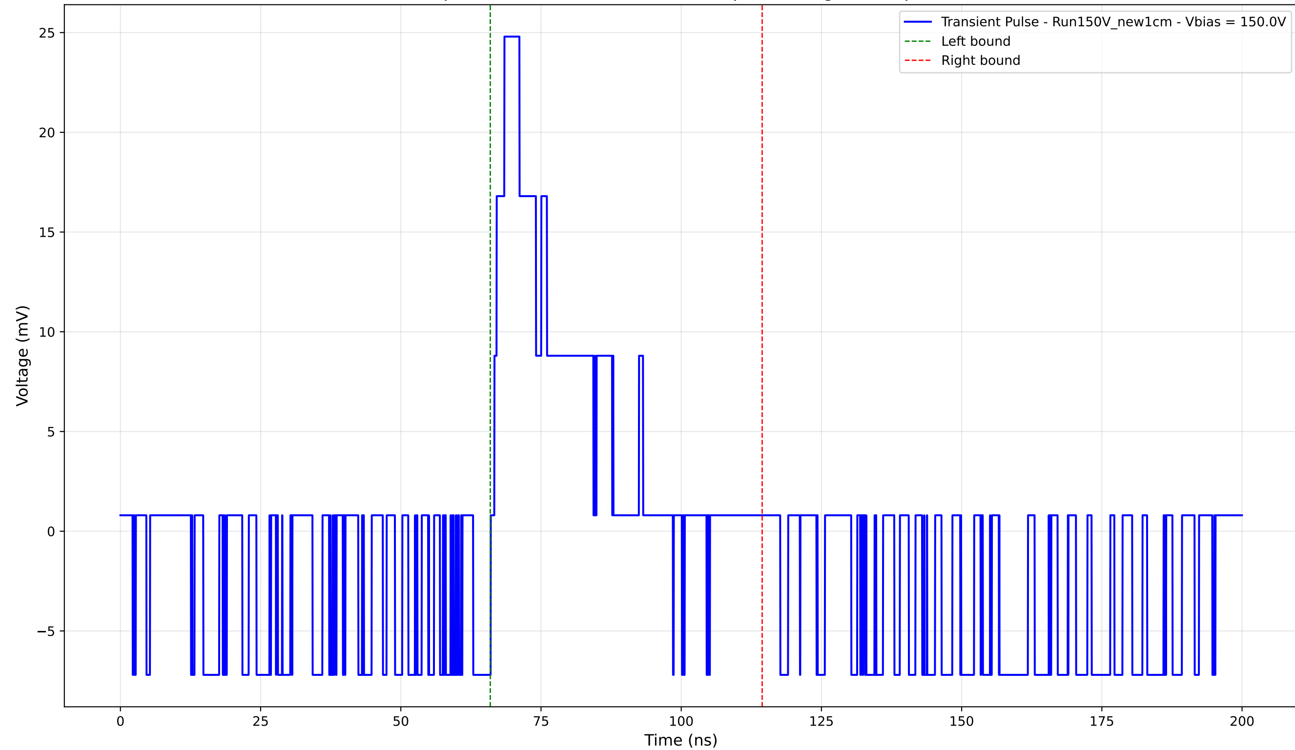
Transient Pulse - Sample: New1cm - Position: 1060.0 \mu\text{m} - Charge: 5.79 pC - Rise Time: 1.80 ns
