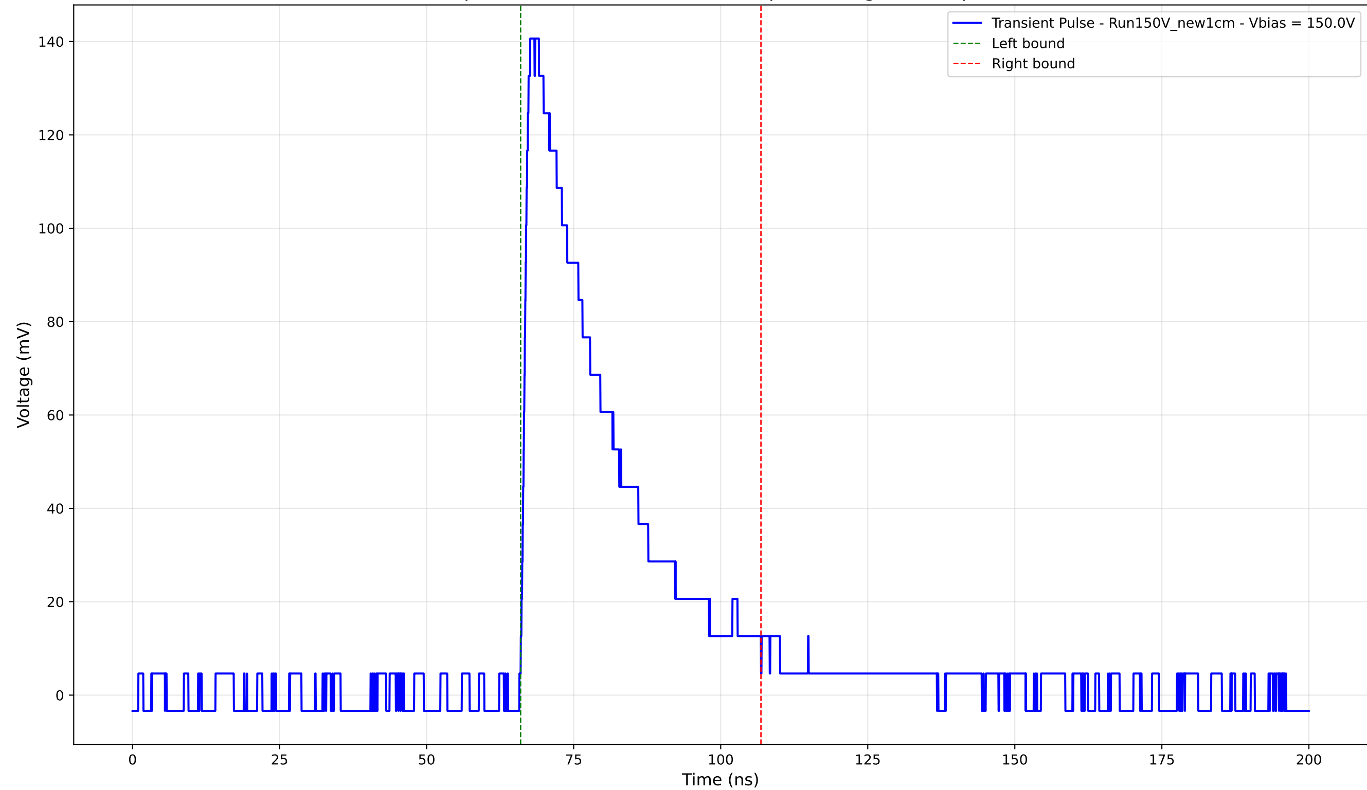
Transient Pulse - Sample: New1cm - Position: 3405.0 \mu\text{m} - Charge: 42.29 pC - Rise Time: 1.22 ns
