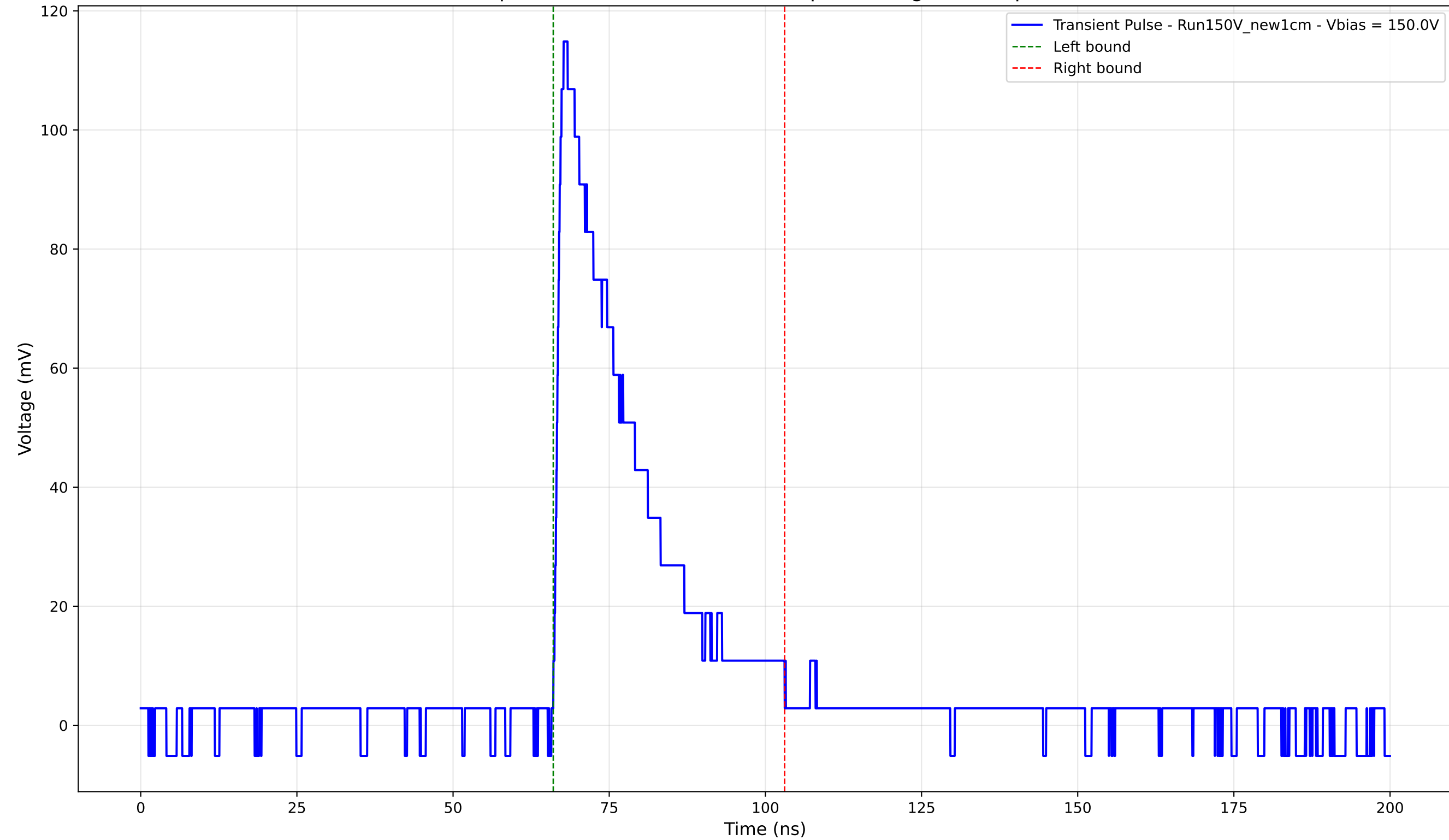
Transient Pulse - Sample: New1cm - Position: 660.0 \mu\text{m} - Charge: 29.18 pC - Rise Time: 1.14 ns
