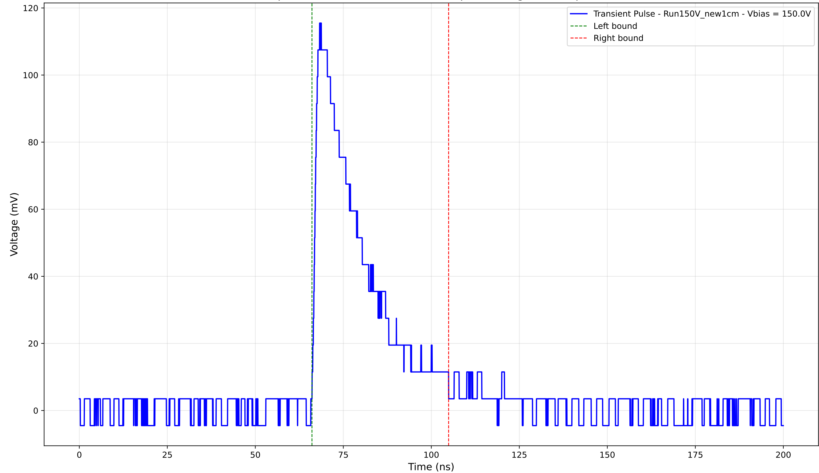
Transient Pulse - Sample: New1cm - Position: 1210.0 \mu\text{m} - Charge: 32.64 pC - Rise Time: 1.48 ns
