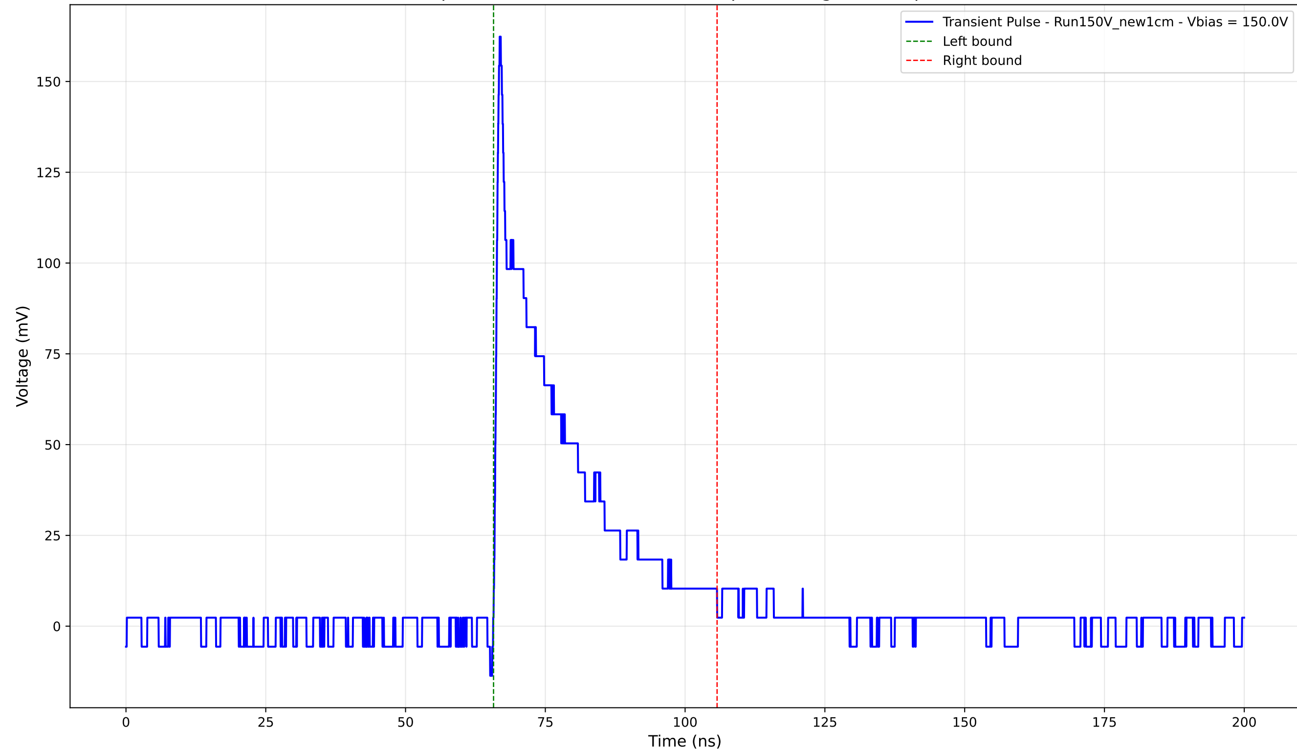
Transient Pulse - Sample: New1cm - Position: 2260.0 \mu\text{m} - Charge: 34.26 pC - Rise Time: 0.79 ns
