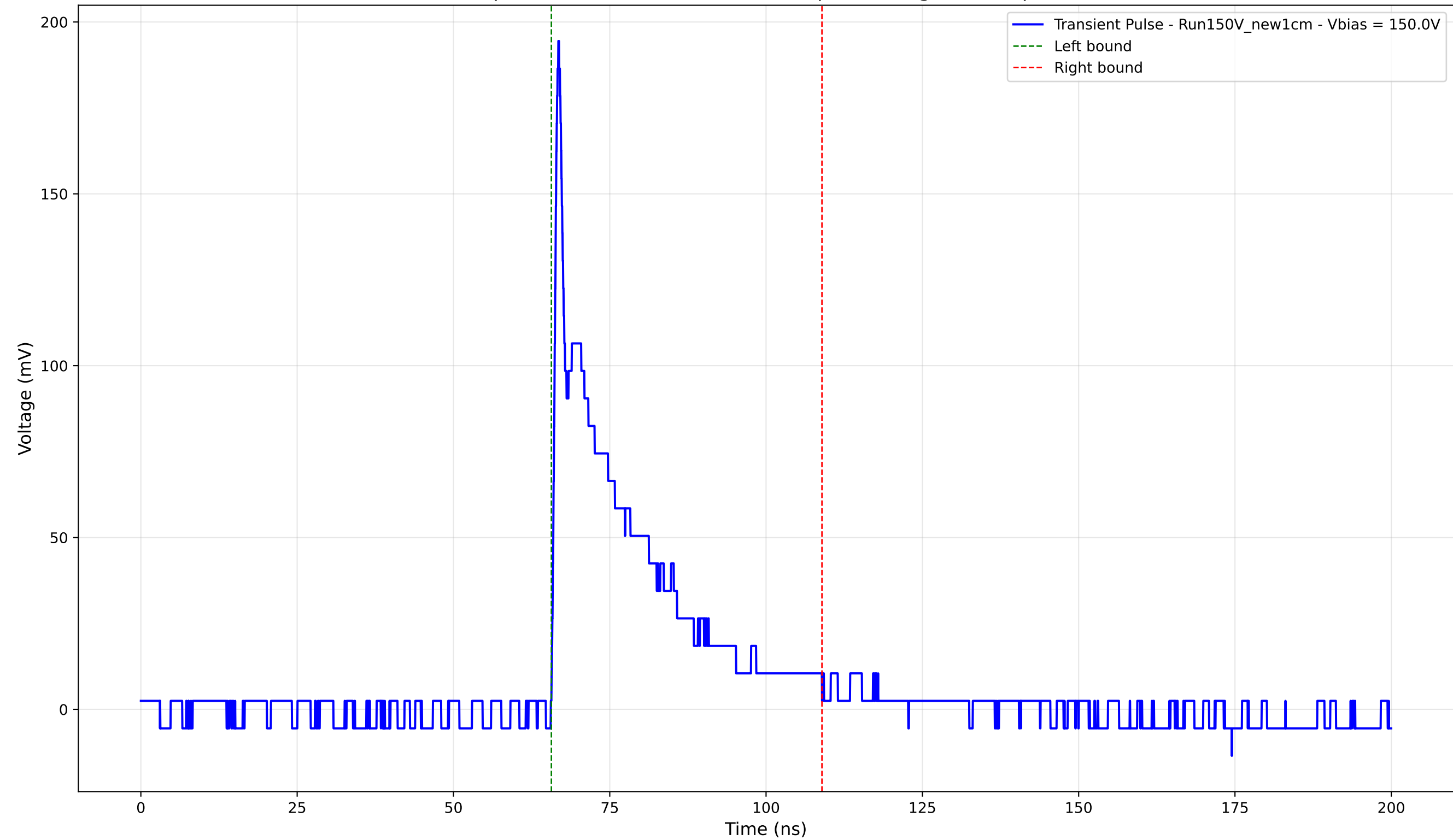
Transient Pulse - Sample: New1cm - Position: 2375.0 \mu\text{m} - Charge: 35.79 pC - Rise Time: 0.78 ns
