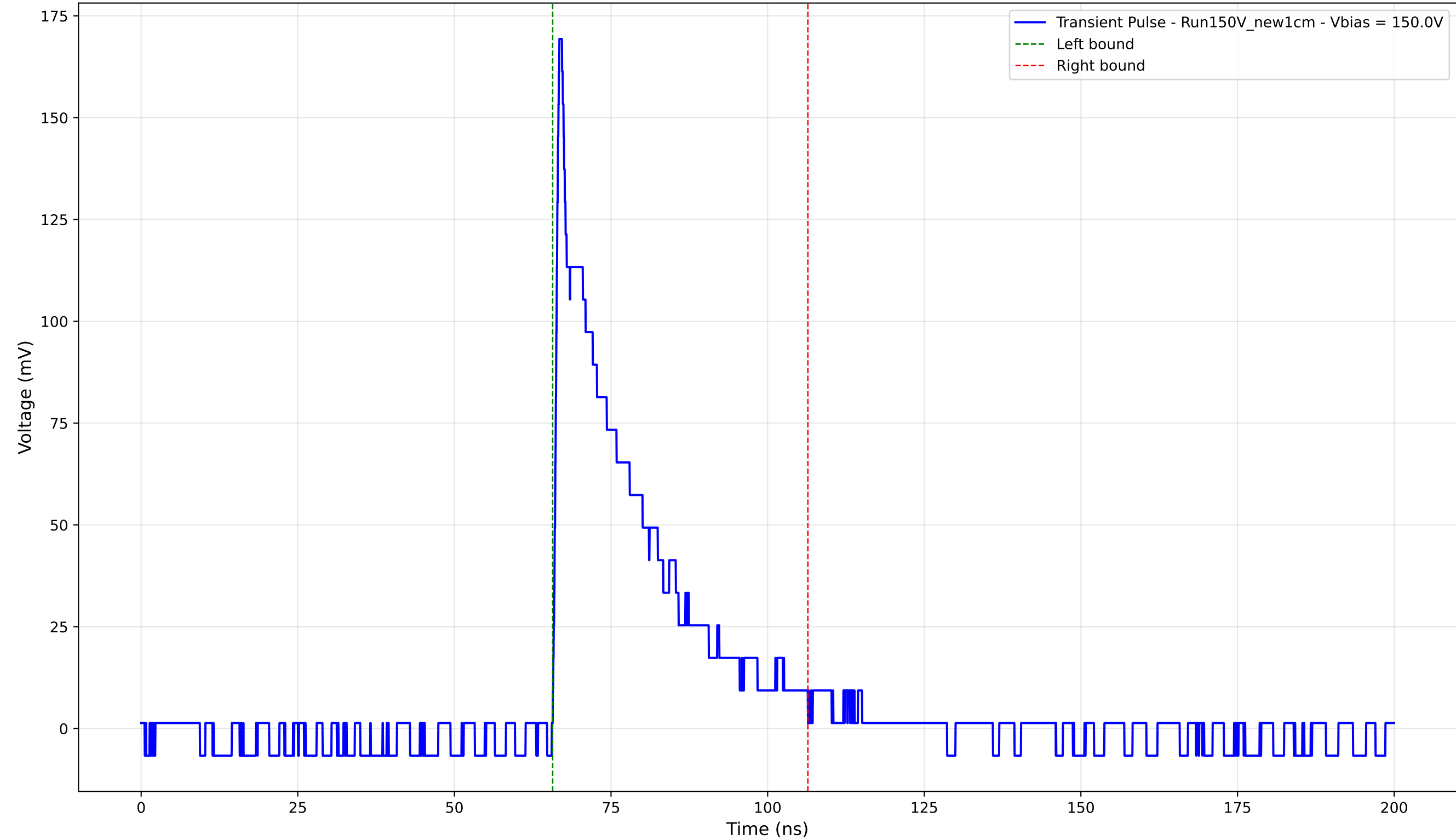
Transient Pulse - Sample: New1cm - Position: 2865.0 \mu\text{m} - Charge: 37.15 pC - Rise Time: 0.82 ns
