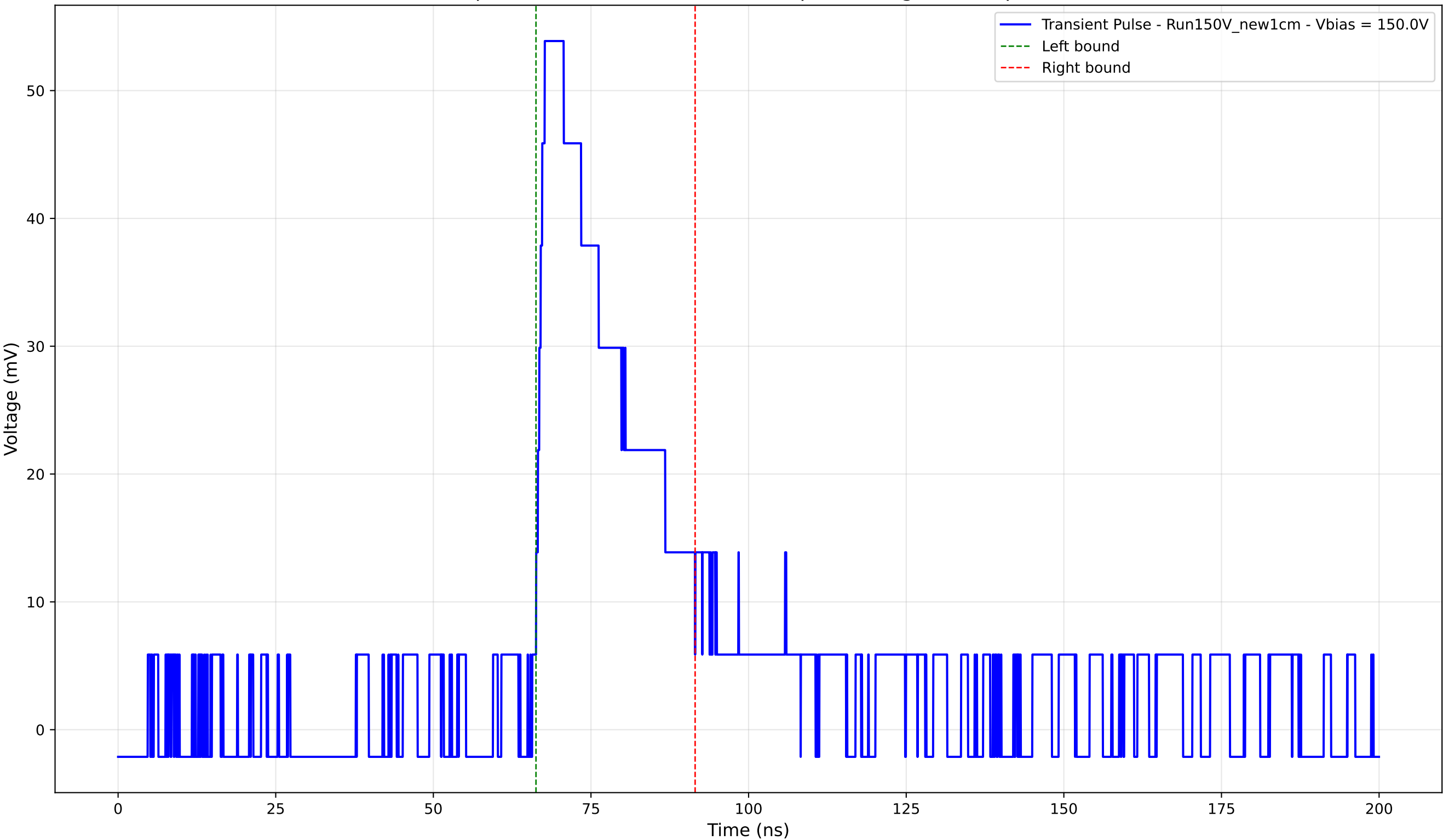
Transient Pulse - Sample: New1cm - Position: 1490.0 \mu\text{m} - Charge: 15.32 pC - Rise Time: 1.98 ns
