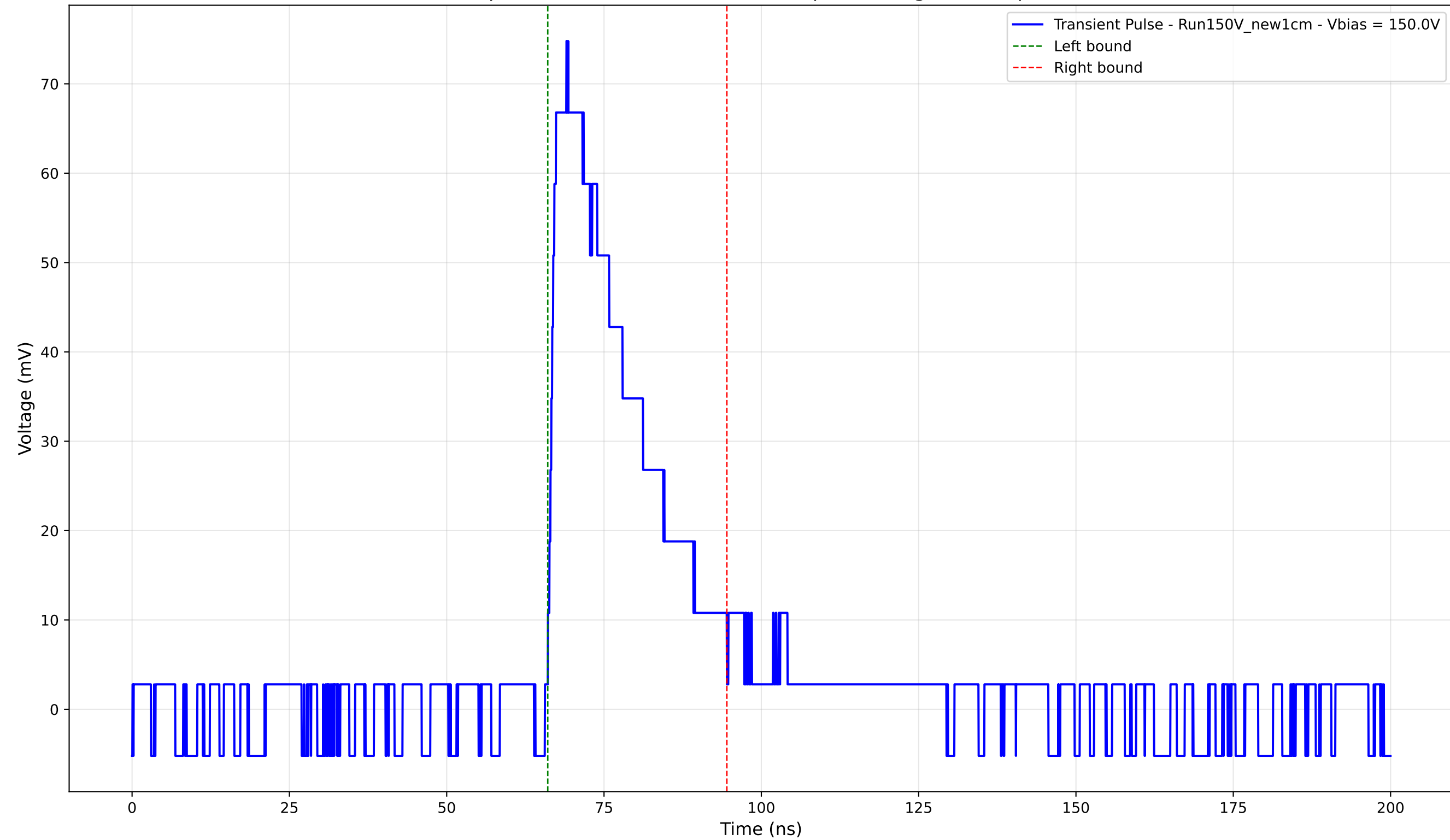
Transient Pulse - Sample: New1cm - Position: 1610.0 \mu\text{m} - Charge: 19.99 pC - Rise Time: 2.95 ns
