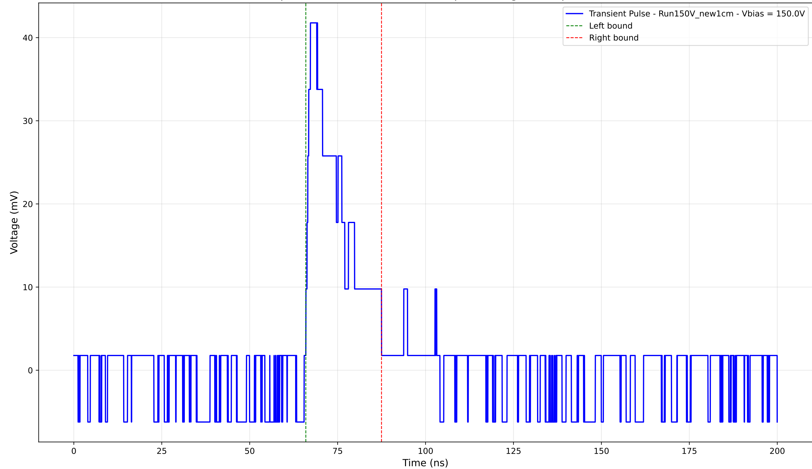
Transient Pulse - Sample: New1cm - Position: 490.0 \mu\text{m} - Charge: 8.62 pC - Rise Time: 1.29 ns
