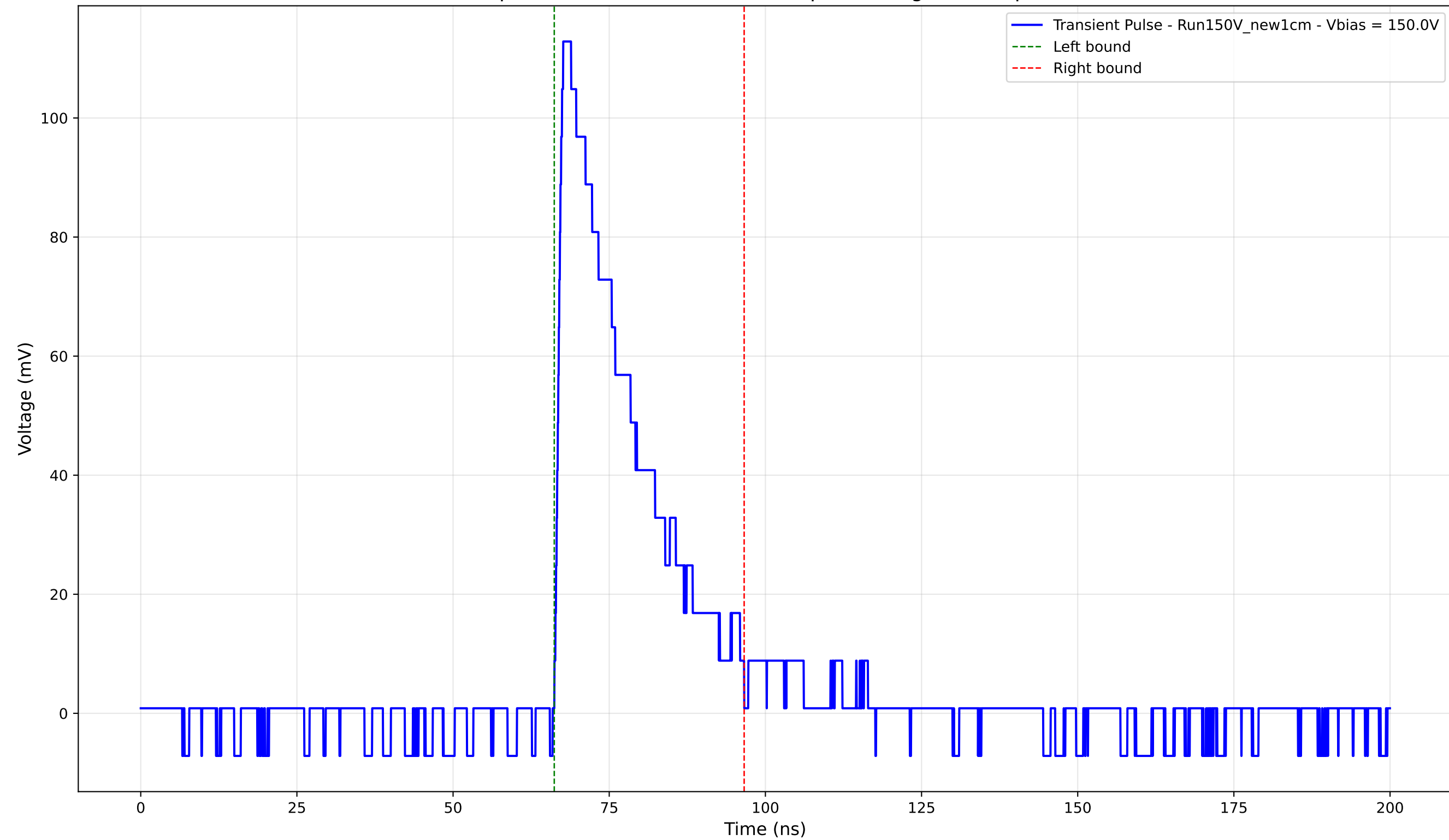
Transient Pulse - Sample: New1cm - Position: 815.0 \mu\text{m} - Charge: 28.36 pC - Rise Time: 1.07 ns
