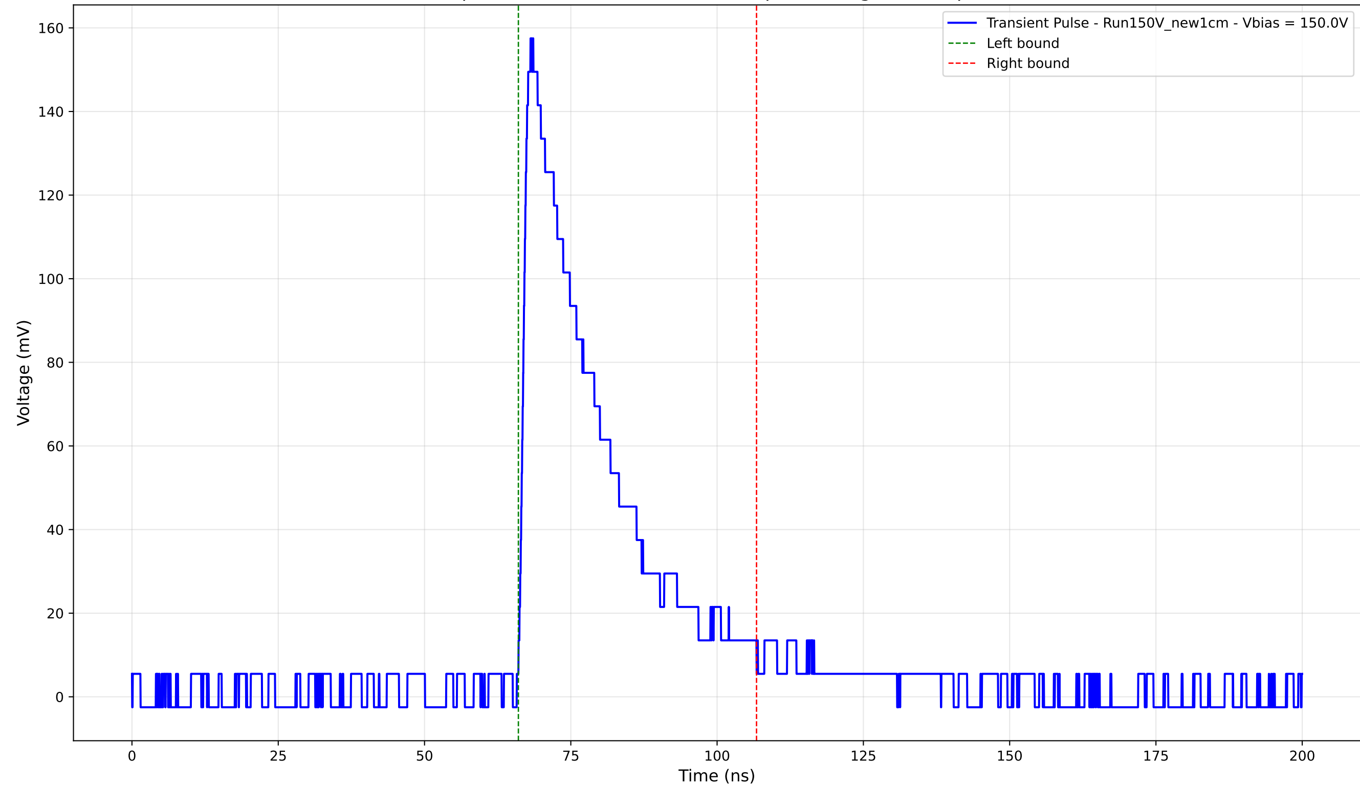
Transient Pulse - Sample: New1cm - Position: 3890.0 \mu\text{m} - Charge: 44.13 pC - Rise Time: 1.49 ns
