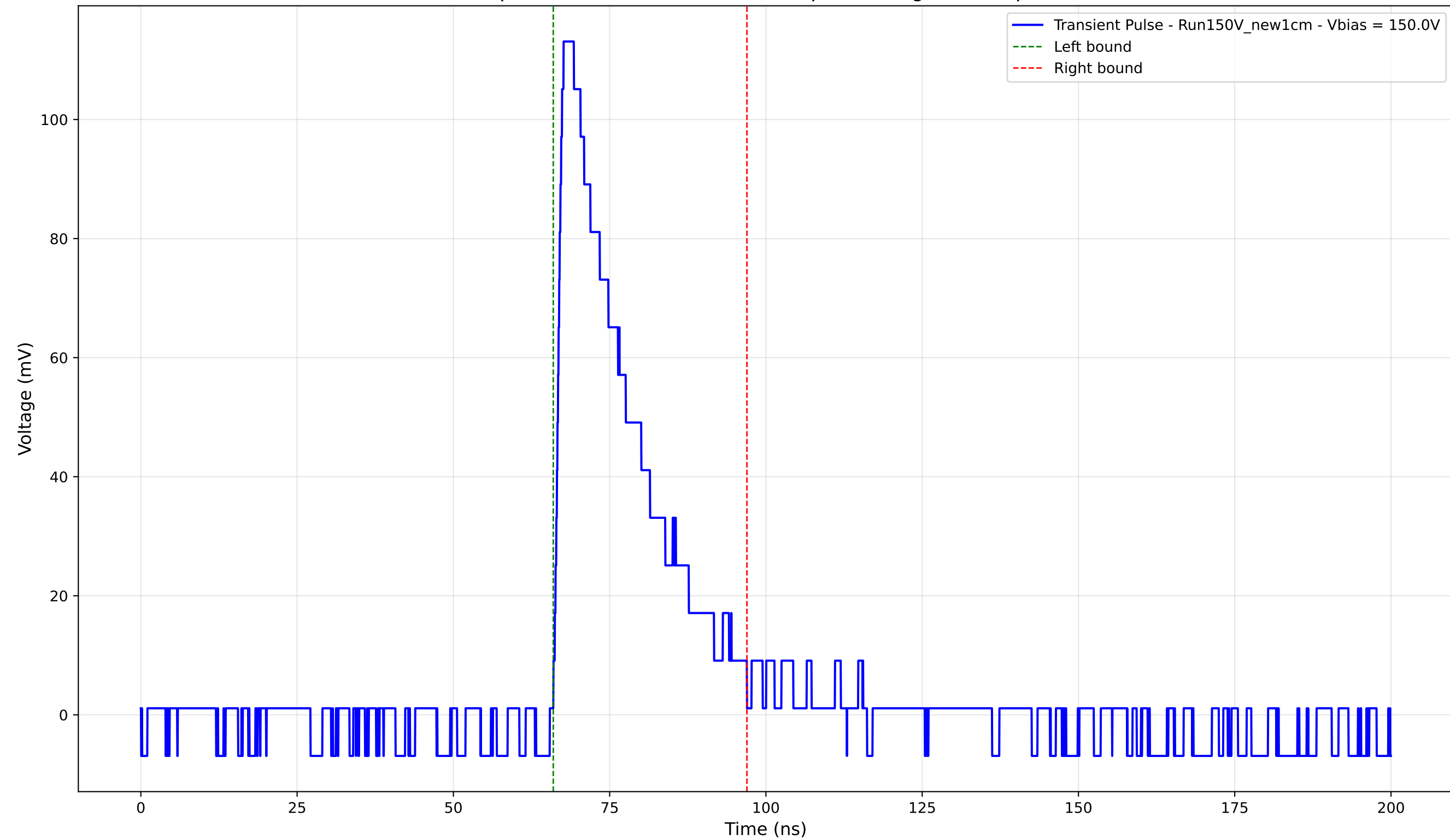
Transient Pulse - Sample: New1cm - Position: 720.0 \mu\text{m} - Charge: 28.31 pC - Rise Time: 1.17 ns
