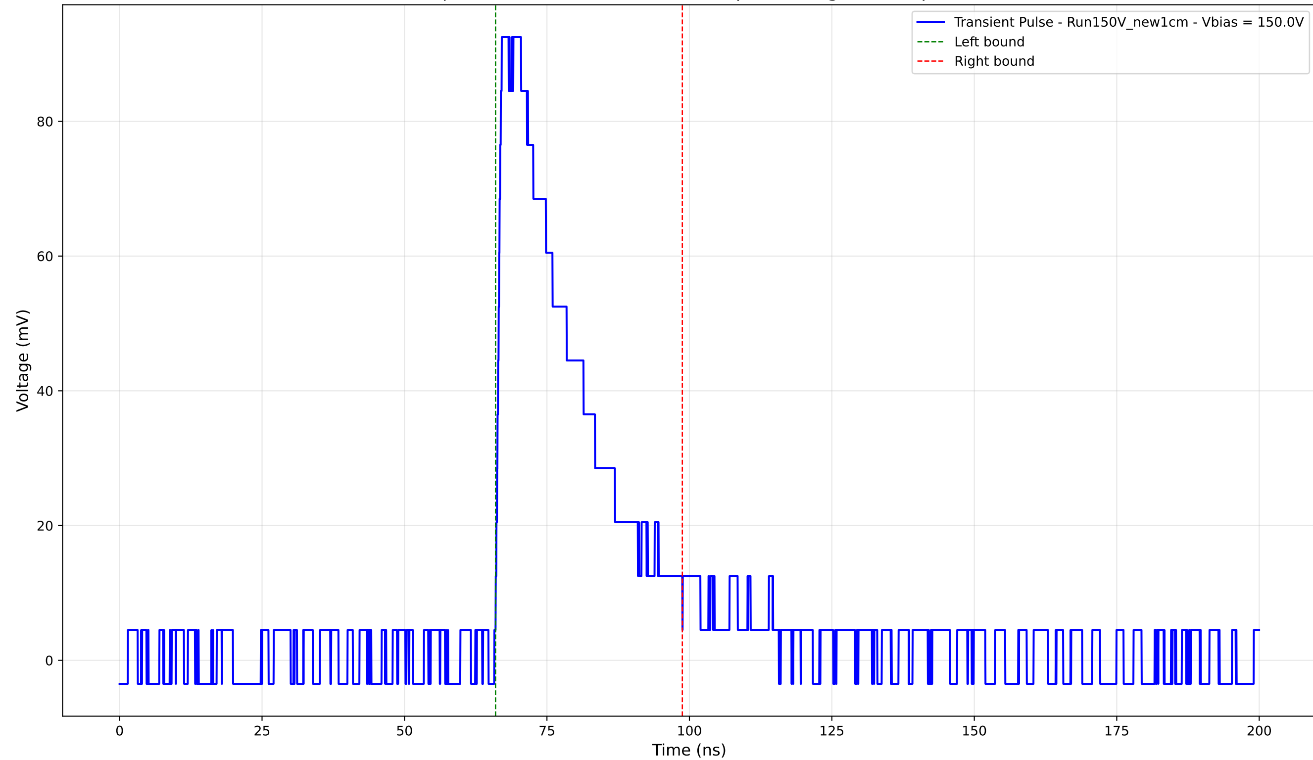
Transient Pulse - Sample: New1cm - Position: 1870.0 \mu\text{m} - Charge: 27.78 pC - Rise Time: 0.91 ns
