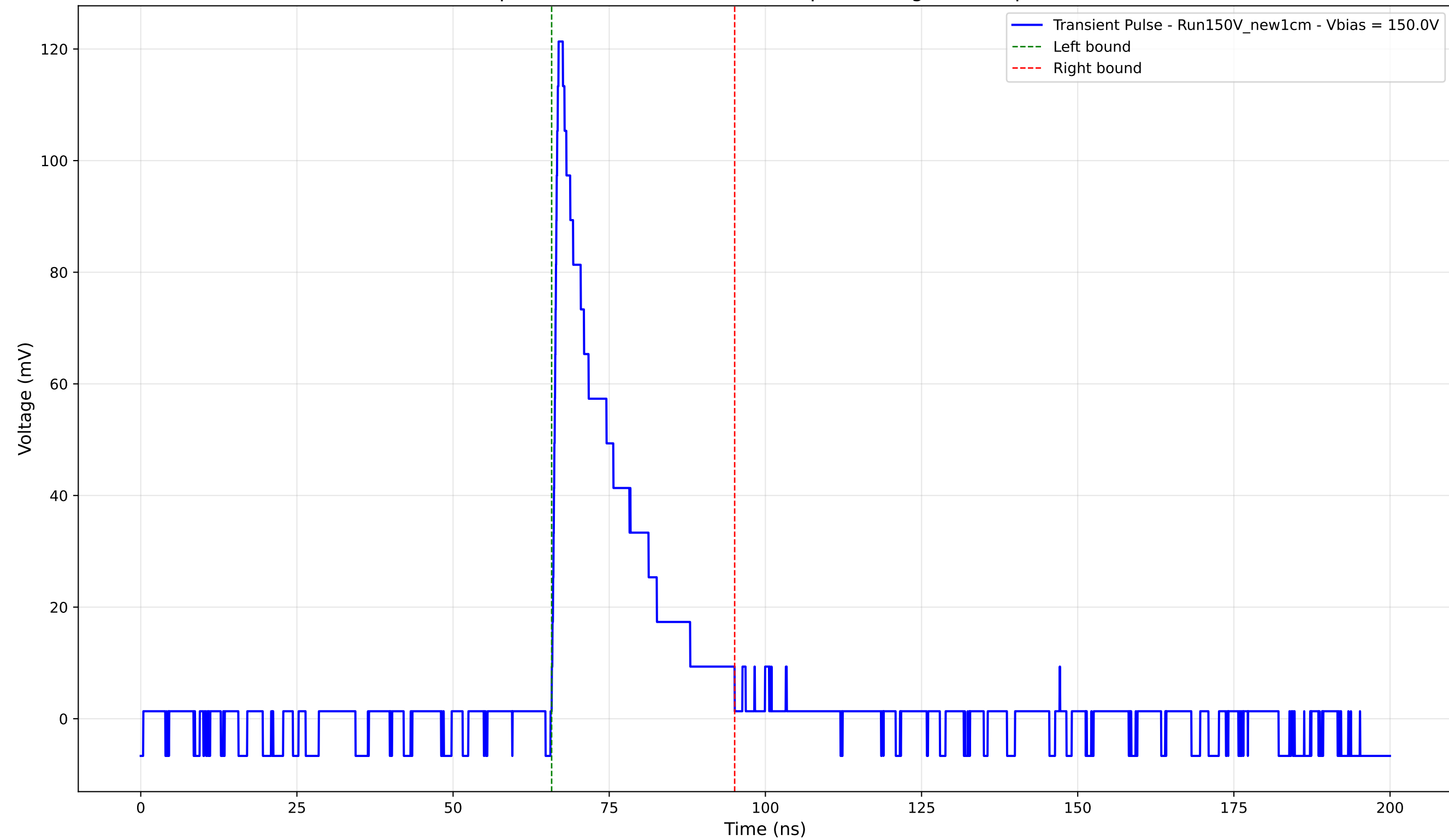
Transient Pulse - Sample: New1cm - Position: 155.0 \mu\text{m} - Charge: 22.40 pC - Rise Time: 0.87 ns
