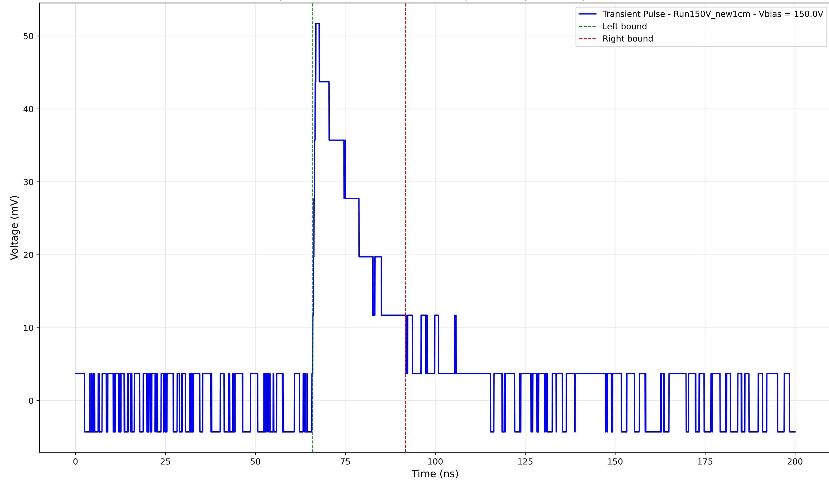
Transient Pulse - Sample: New1cm - Position: 3100.0 \mu\text{m} - Charge: 13.08 pC - Rise Time: 0.86 ns
