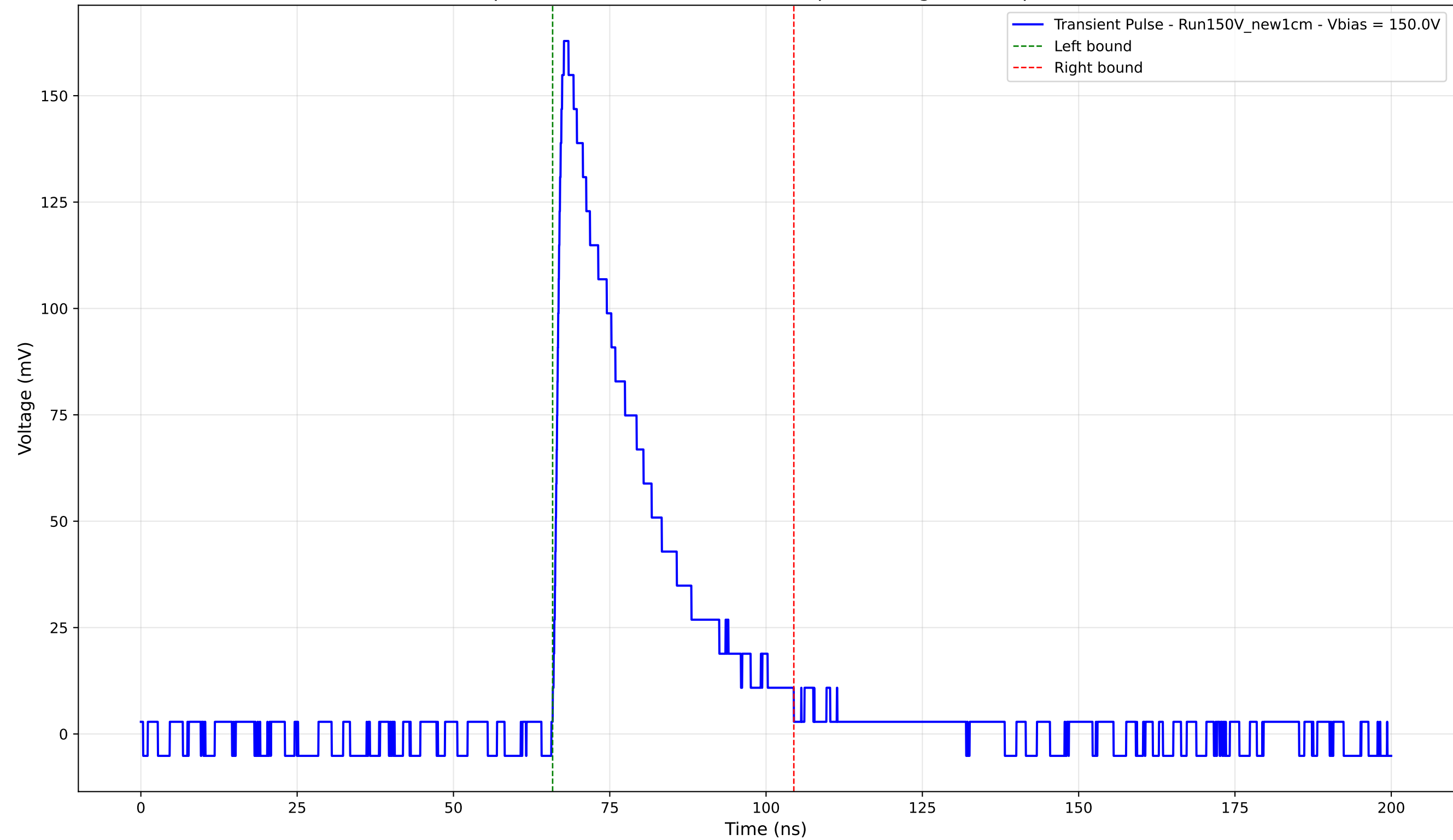
Transient Pulse - Sample: New1cm - Position: 4290.0 \mu\text{m} - Charge: 43.49 pC - Rise Time: 1.25 ns
