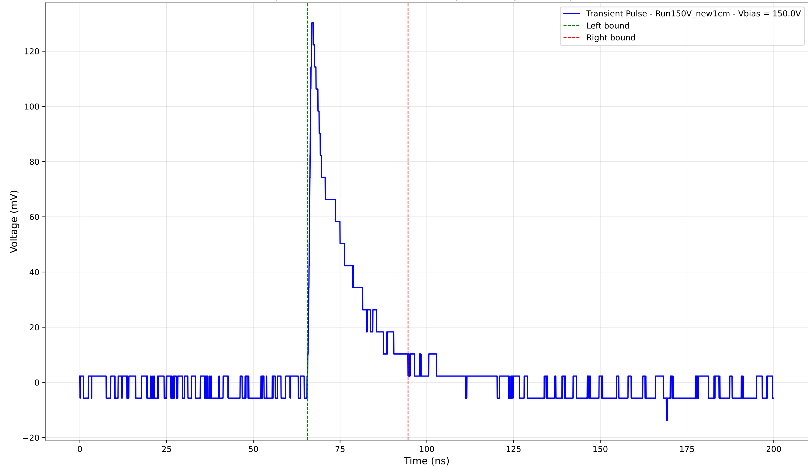
Transient Pulse - Sample: New1cm - Position: 4820.0 \mu\text{m} - Charge: 24.35 pC - Rise Time: 0.93 ns
