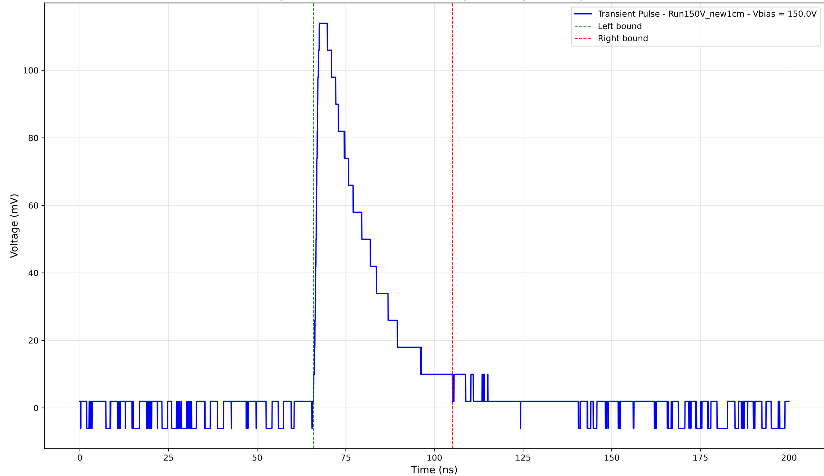
Transient Pulse - Sample: New1cm - Position: 3480.0 \mu\text{m} - Charge: 33.87 pC - Rise Time: 1.14 ns
