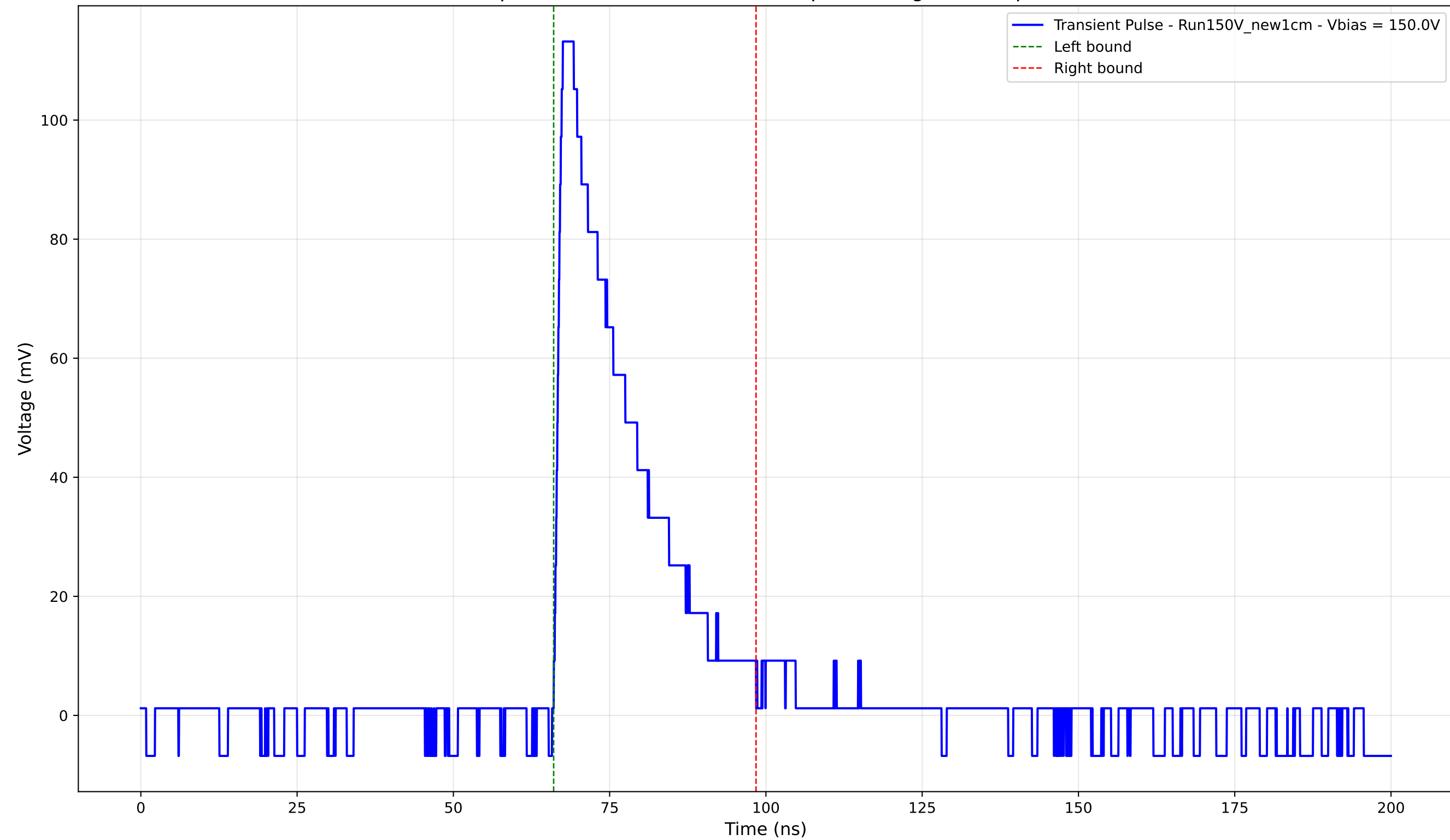
Transient Pulse - Sample: New1cm - Position: 675.0 \mu\text{m} - Charge: 27.83 pC - Rise Time: 1.11 ns
