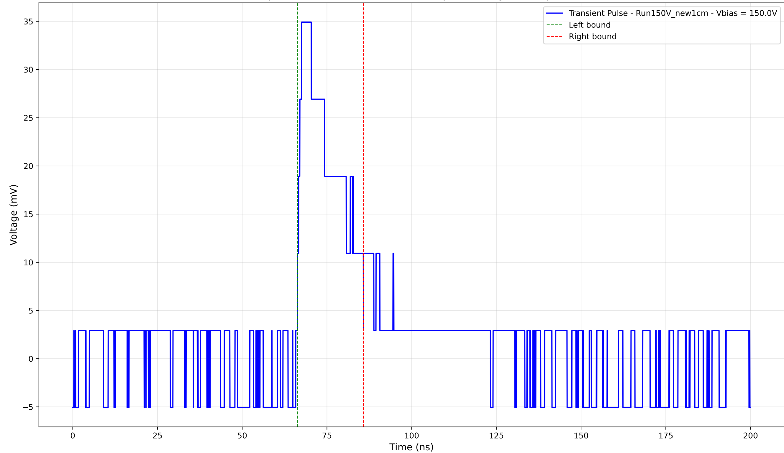
Transient Pulse - Sample: New1cm - Position: 1575.0 \mu\text{m} - Charge: 8.25 pC - Rise Time: 1.24 ns
