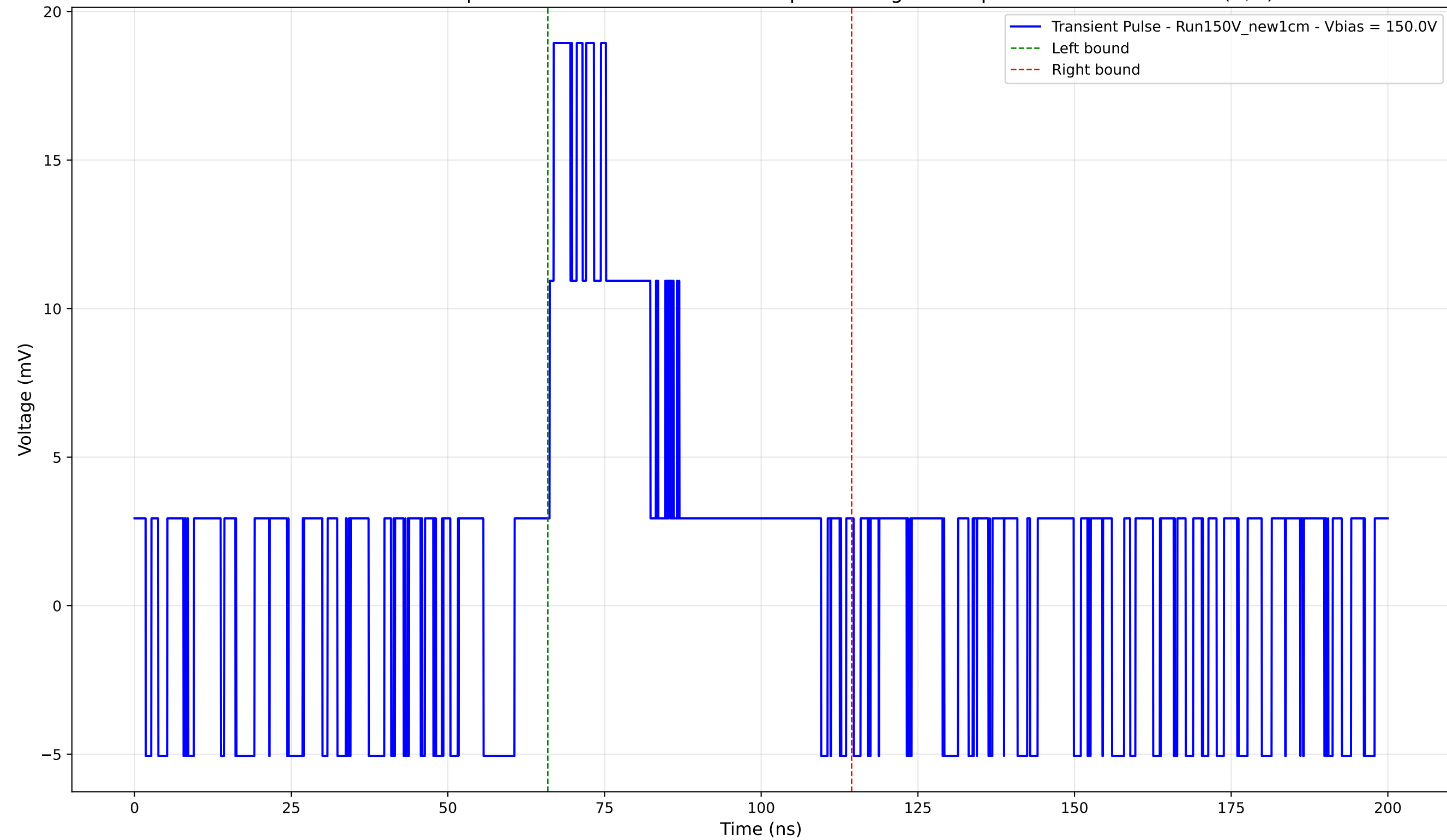
Transient Pulse - Sample: New1cm - Position: 3070.0 \mu\text{m} - Charge: 6.19 pC - Rise Time: 0.00 ns (N/A)
