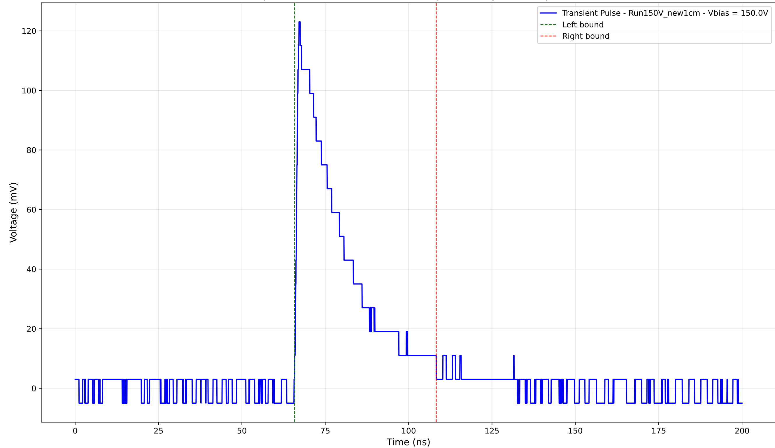
Transient Pulse - Sample: New1cm - Position: 3150.0 \mu\text{m} - Charge: 35.14 pC - Rise Time: 1.00 ns
