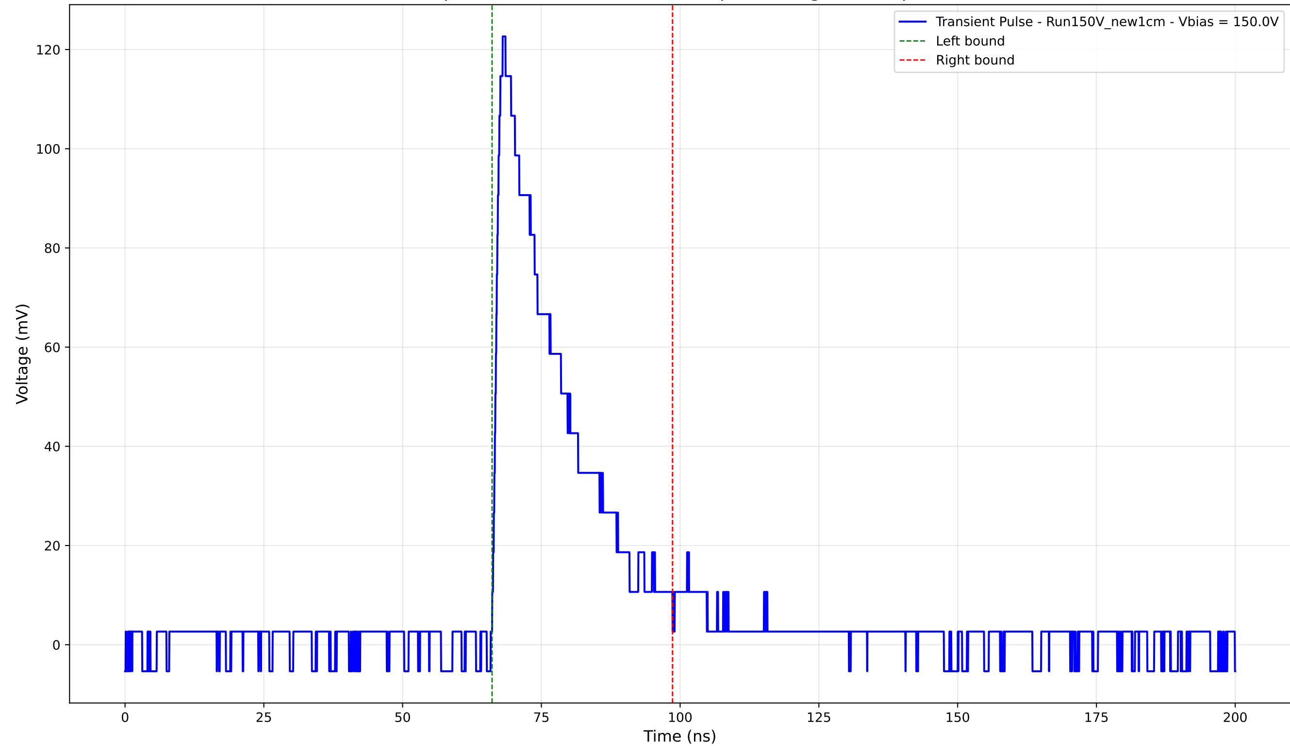
Transient Pulse - Sample: New1cm - Position: 770.0 \mu\text{m} - Charge: 30.31 pC - Rise Time: 1.32 ns
