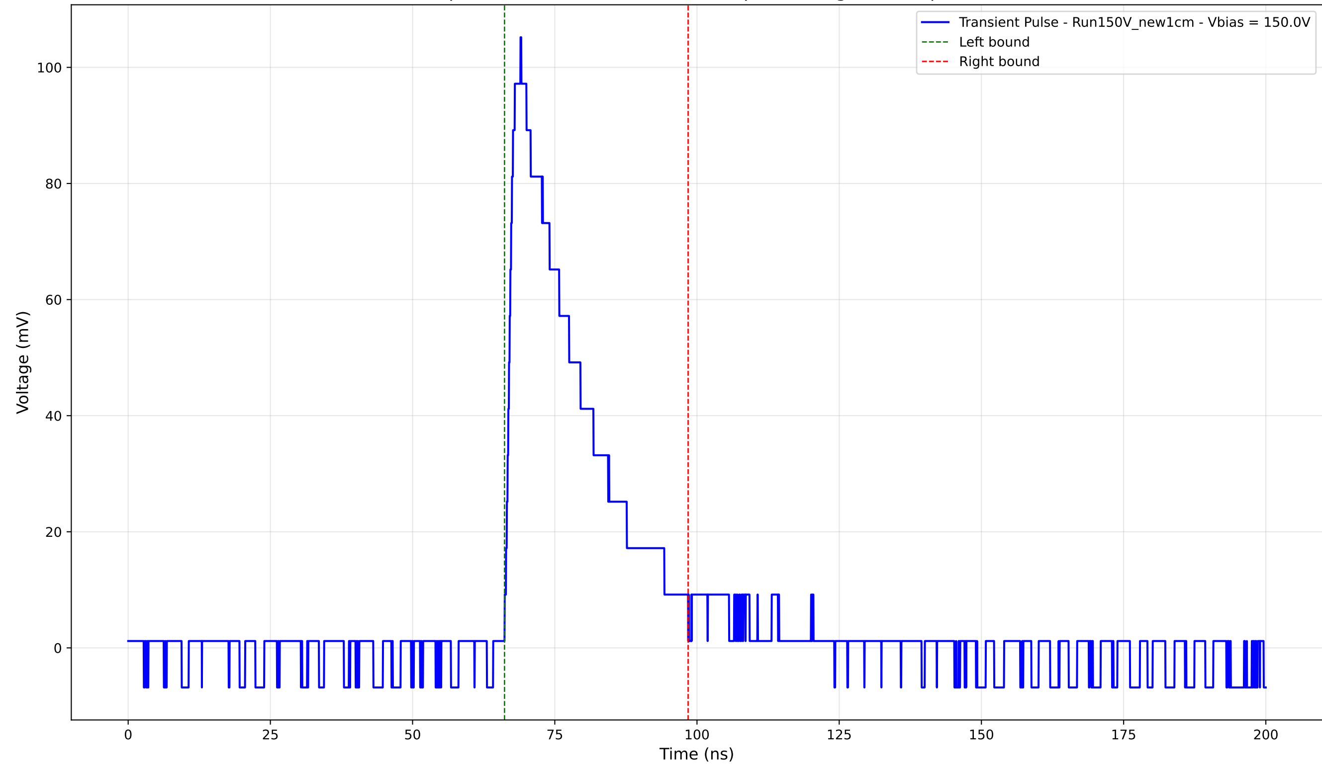
Transient Pulse - Sample: New1cm - Position: 1145.0 \mu\text{m} - Charge: 26.85 pC - Rise Time: 1.56 ns
