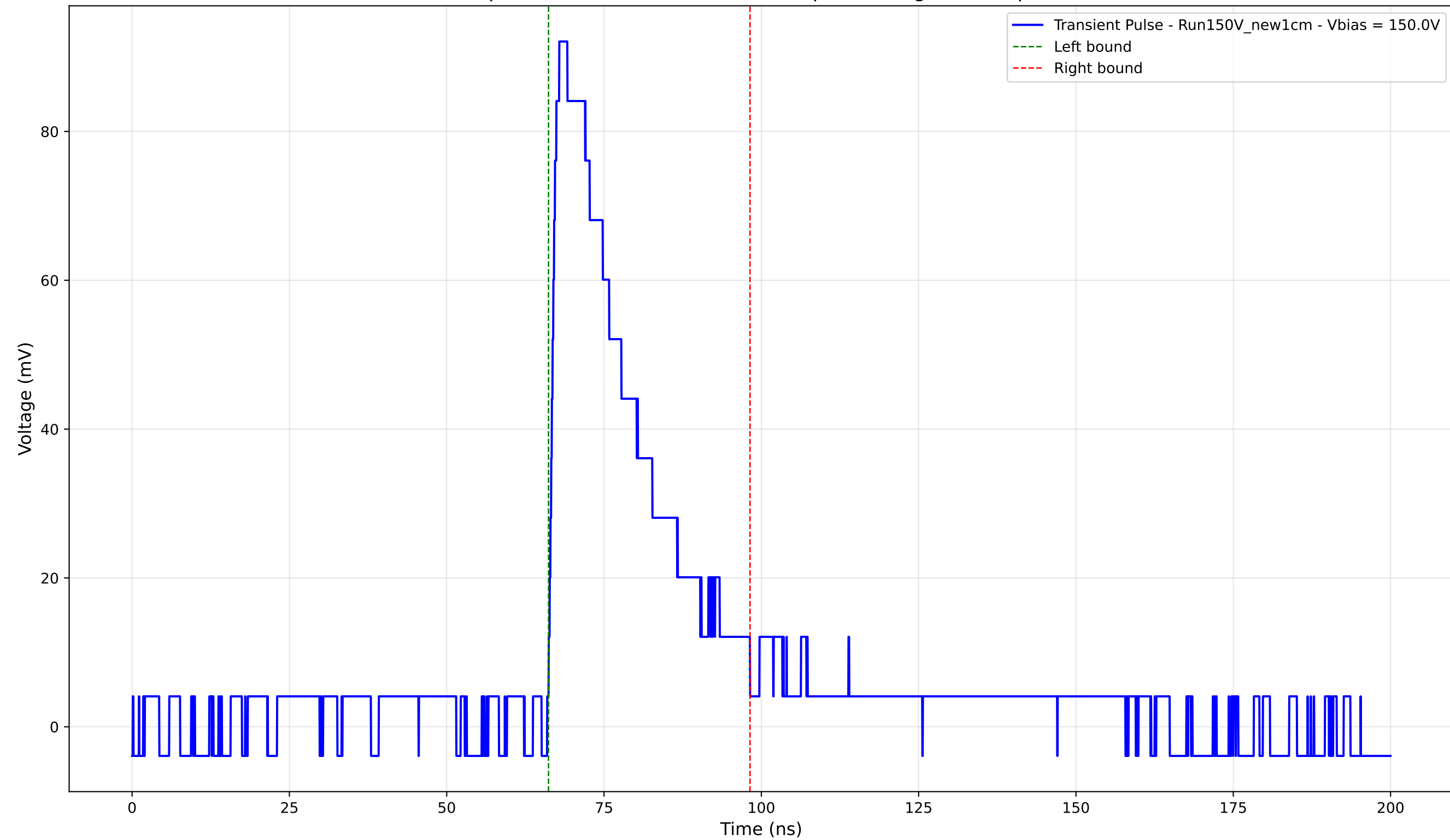
Transient Pulse - Sample: New1cm - Position: 1630.0 \mu\text{m} - Charge: 26.05 pC - Rise Time: 1.23 ns
