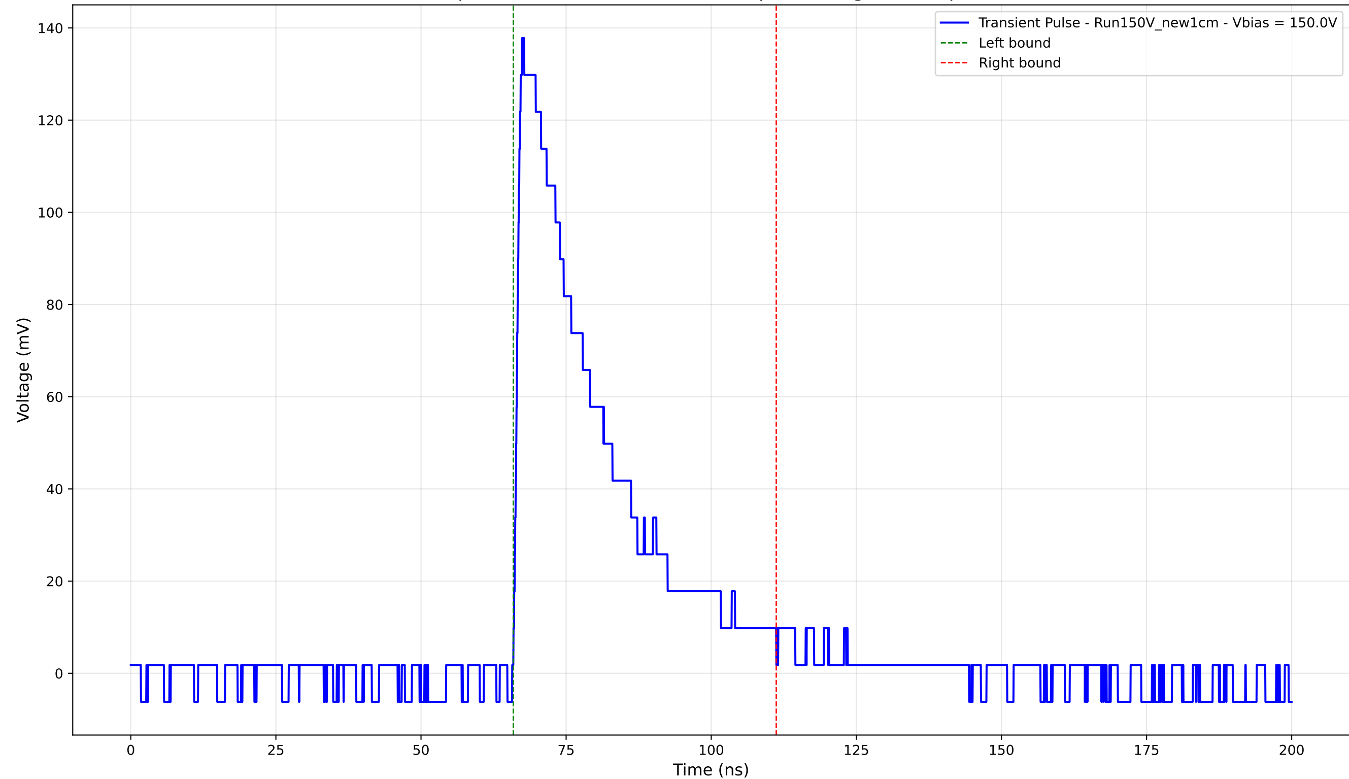
Transient Pulse - Sample: New1cm - Position: 3300.0 \mu\text{m} - Charge: 41.16 pC - Rise Time: 1.13 ns
