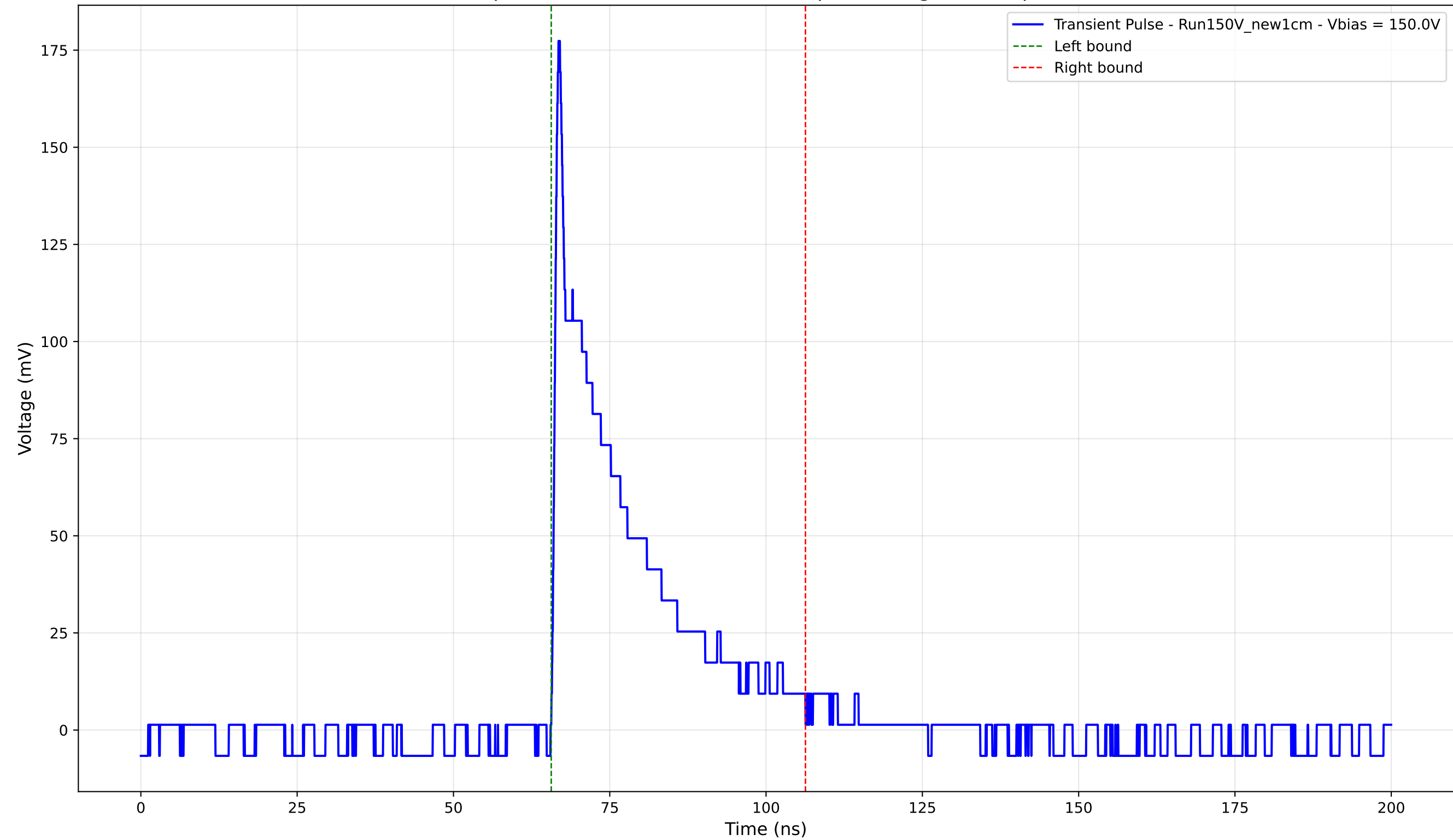
Transient Pulse - Sample: New1cm - Position: 2300.0 \mu\text{m} - Charge: 35.33 pC - Rise Time: 0.80 ns
