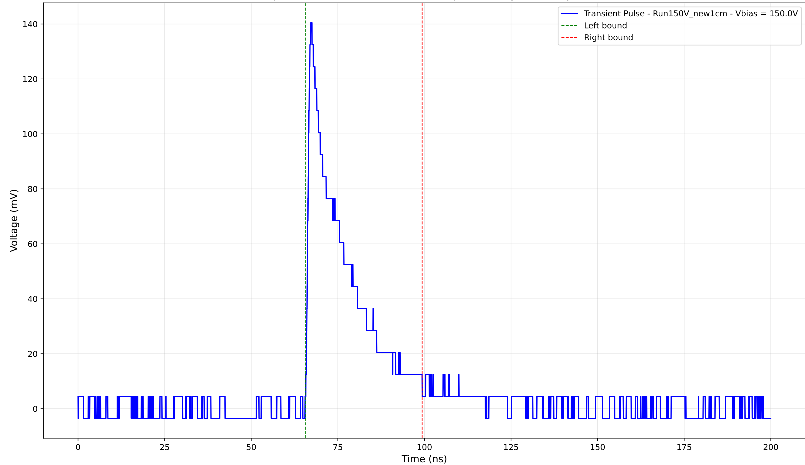
Transient Pulse - Sample: New1cm - Position: 4685.0 \mu\text{m} - Charge: 30.57 pC - Rise Time: 1.08 ns
