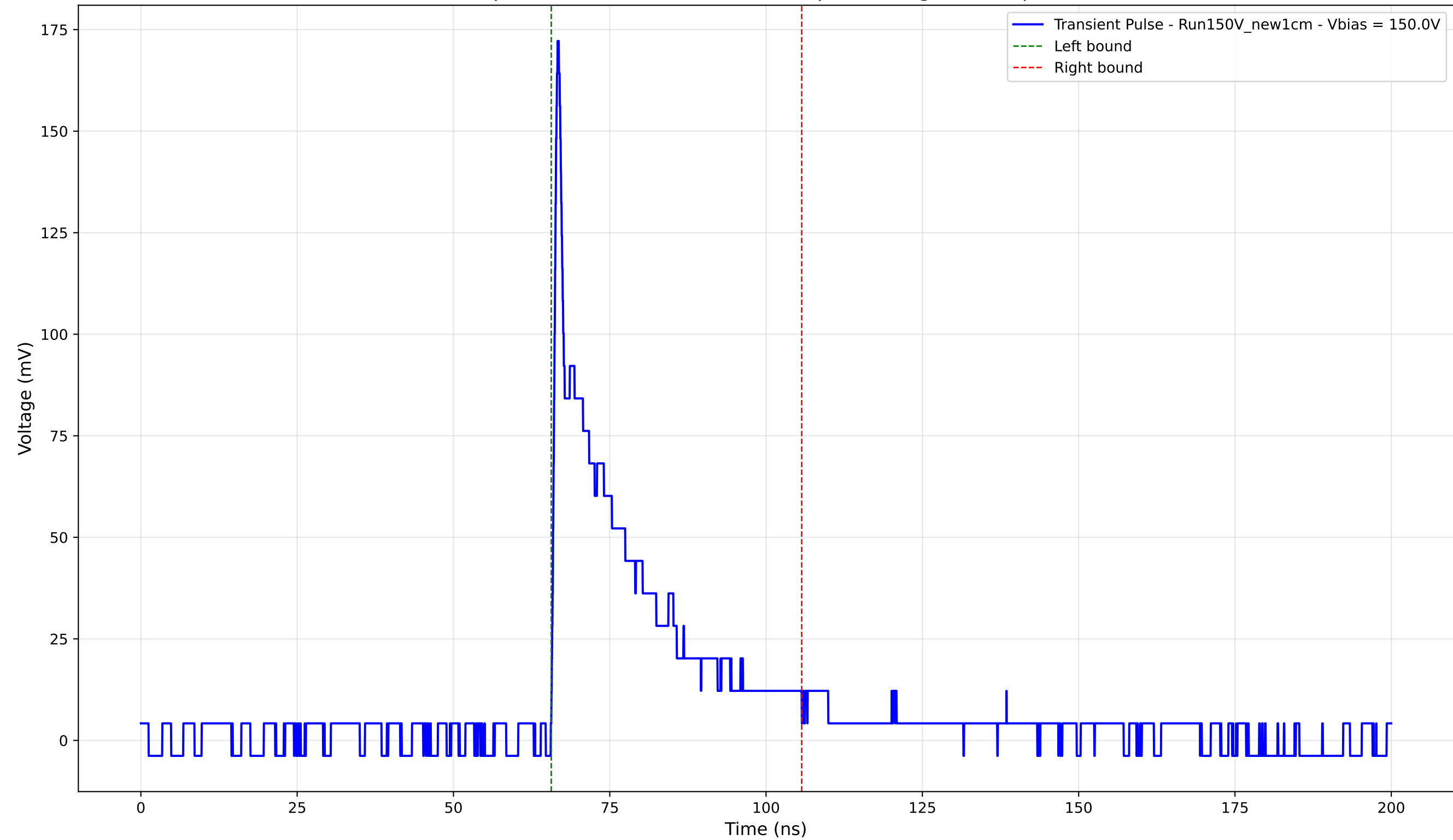
Transient Pulse - Sample: New1cm - Position: 2465.0 \mu\text{m} - Charge: 30.59 pC - Rise Time: 0.77 ns
