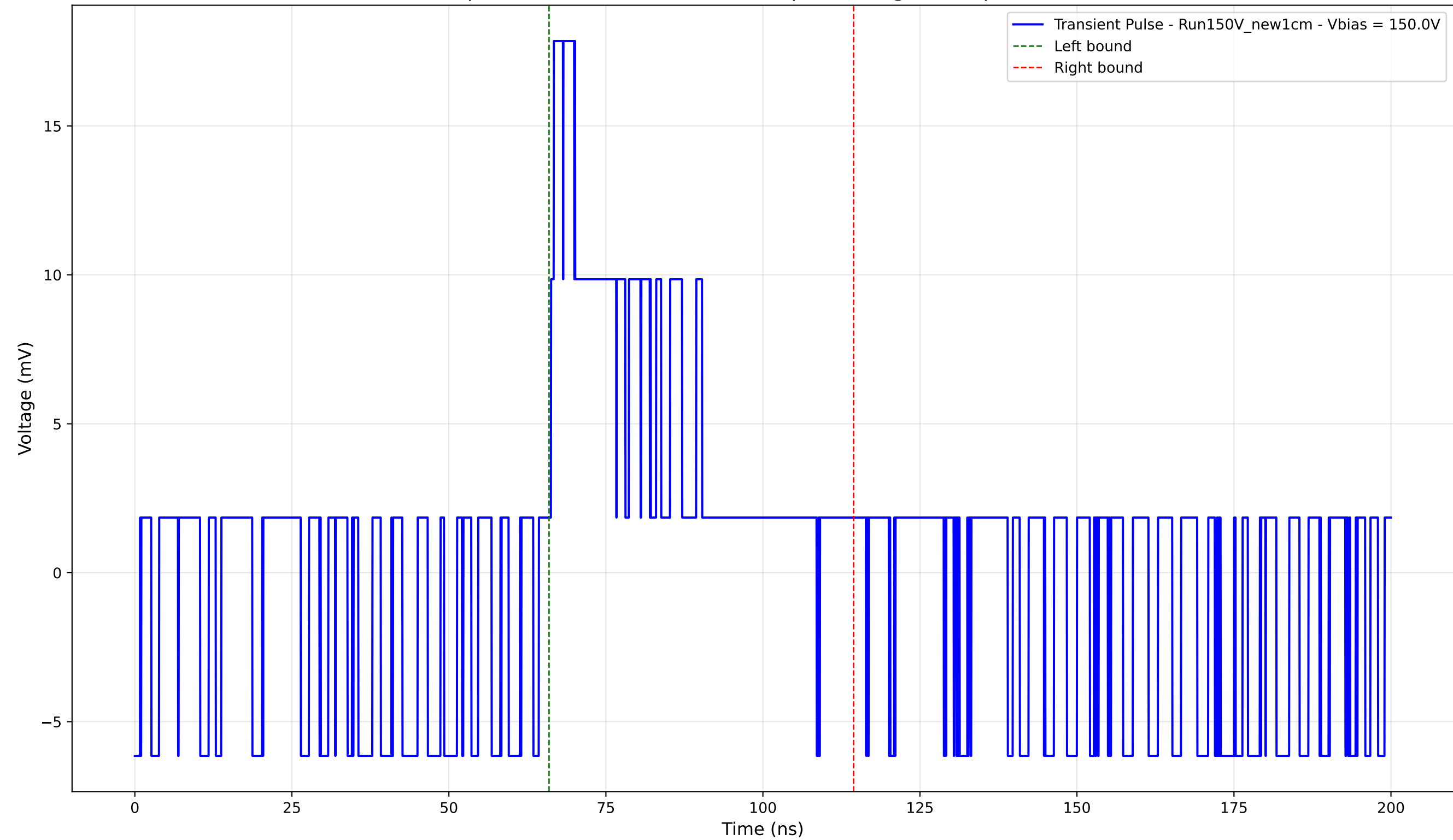
Transient Pulse - Sample: New1cm - Position: 3065.0 \mu\text{m} - Charge: 5.27 pC - Rise Time: 0.00 ns (N/A)
