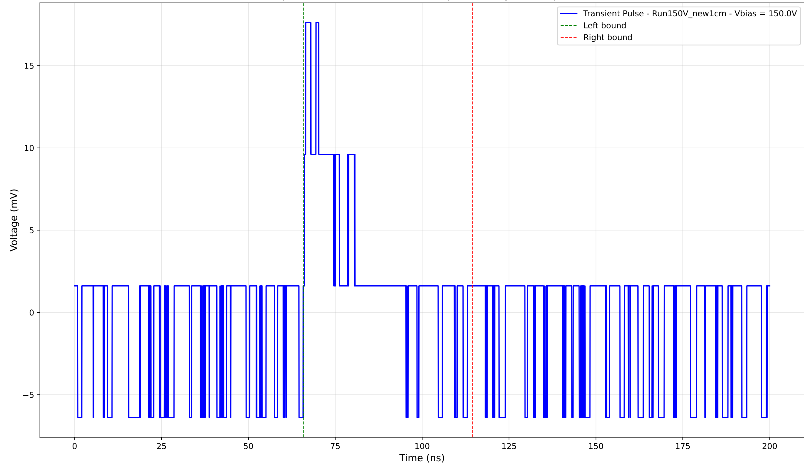
Transient Pulse - Sample: New1cm - Position: 45.0 \mu\text{m} - Charge: 3.11 pC - Rise Time: 0.34 ns
