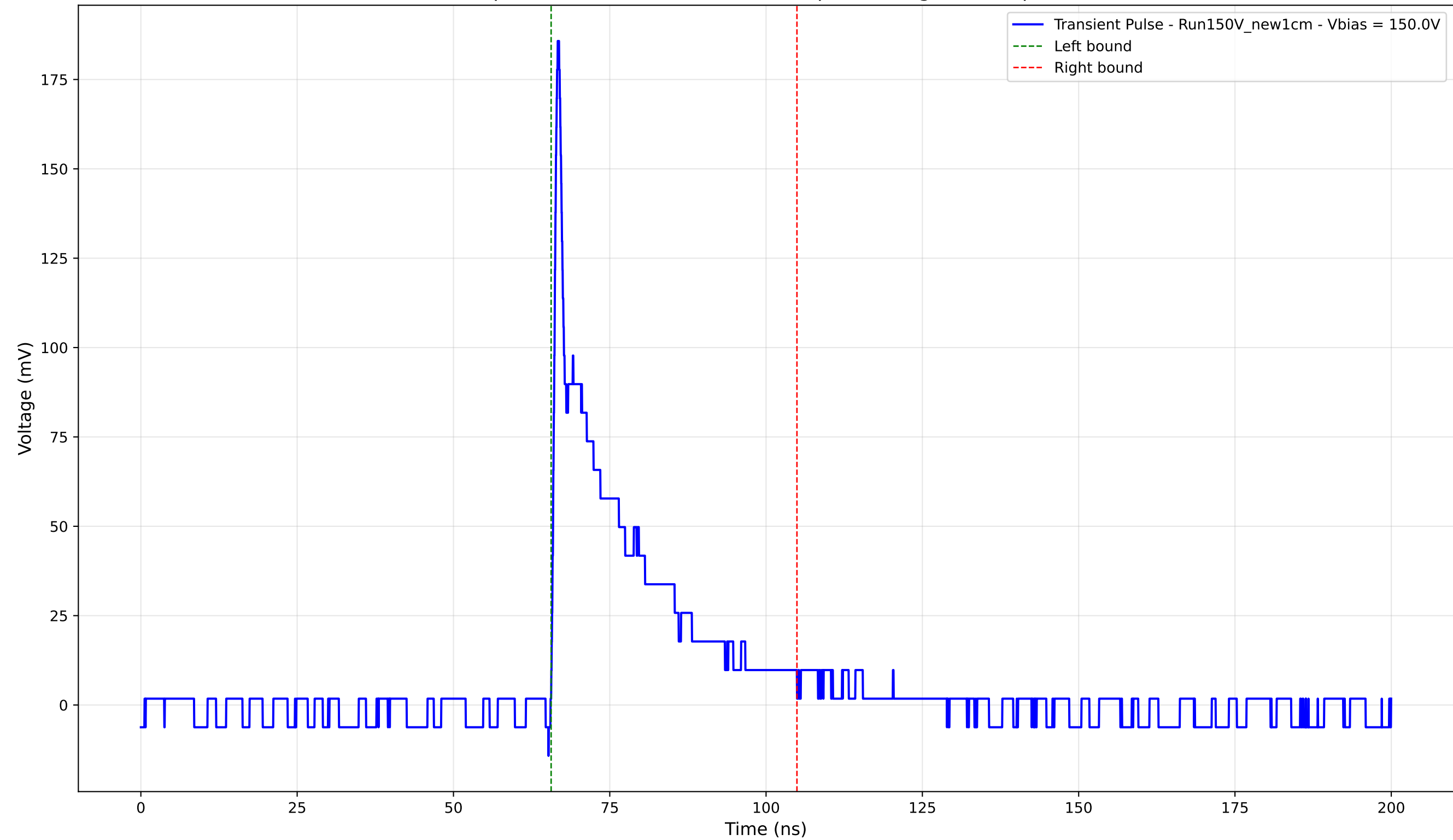
Transient Pulse - Sample: New1cm - Position: 2460.0 \mu\text{m} - Charge: 30.63 pC - Rise Time: 0.76 ns
