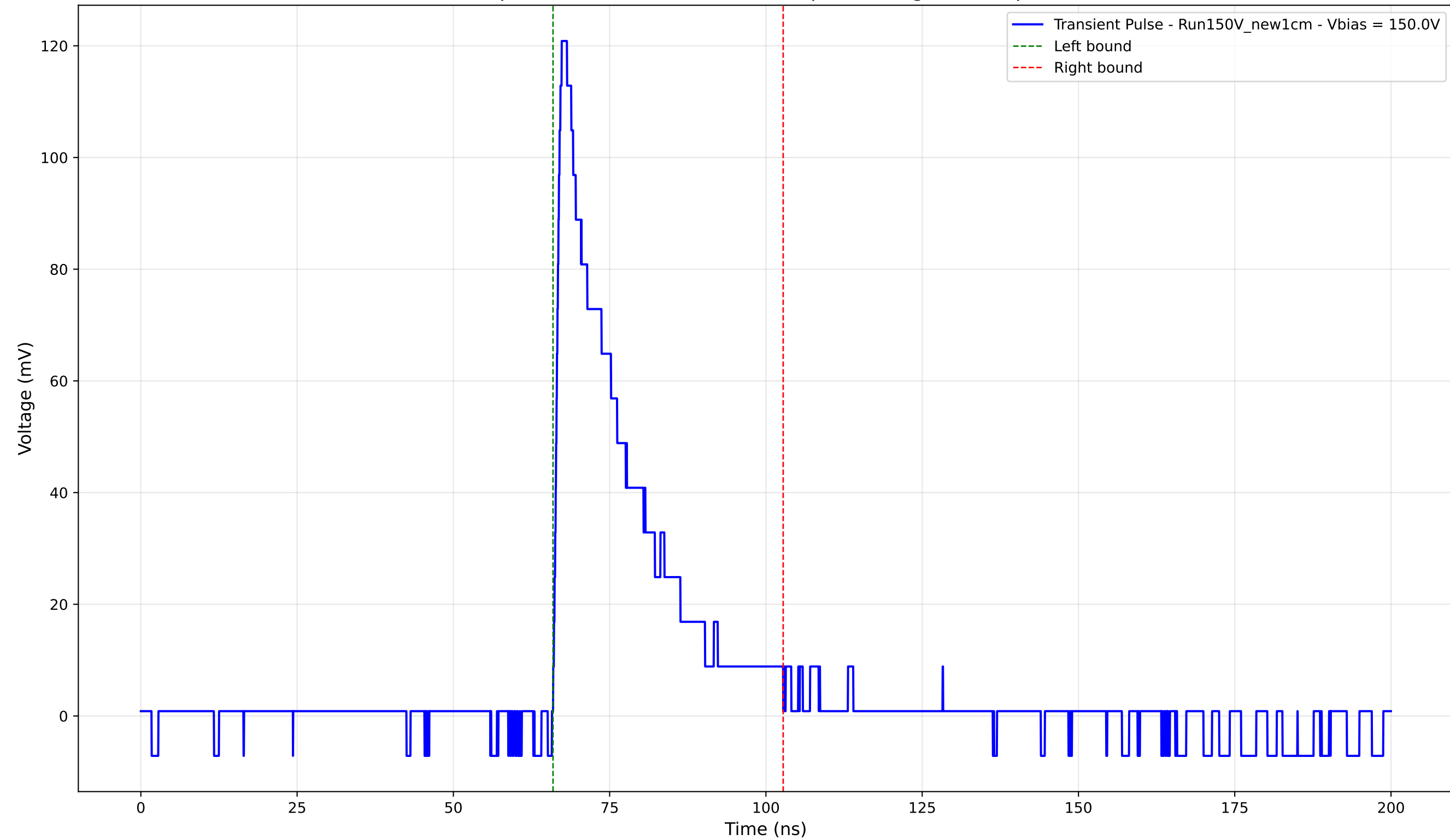
Transient Pulse - Sample: New1cm - Position: 395.0 \mu\text{m} - Charge: 27.04 pC - Rise Time: 1.05 ns
