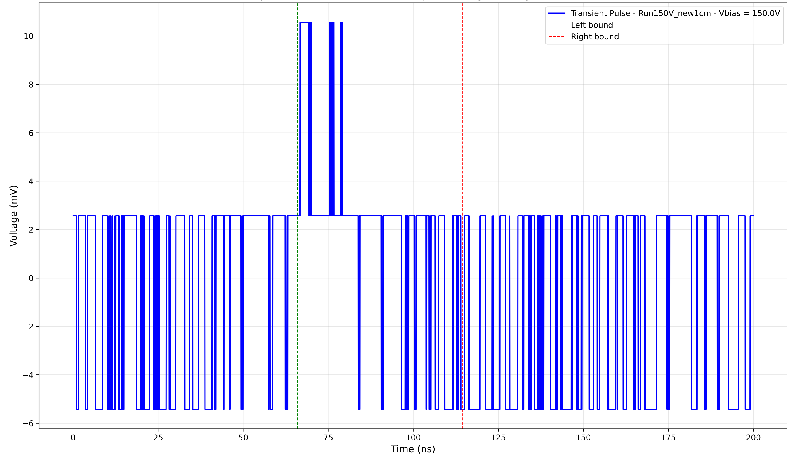
Transient Pulse - Sample: New1cm - Position: 25.0 \mu\text{m} - Charge: 1.89 pC - Rise Time: 0.00 ns (N/A)
