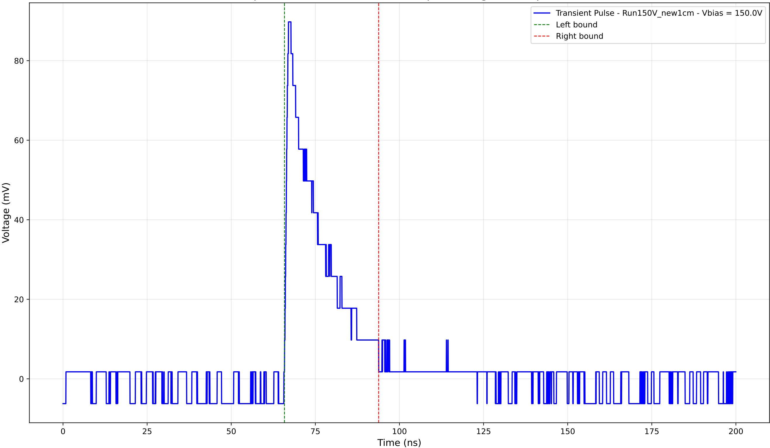
Transient Pulse - Sample: New1cm - Position: 4630.0 \mu\text{m} - Charge: 18.40 pC - Rise Time: 0.98 ns
