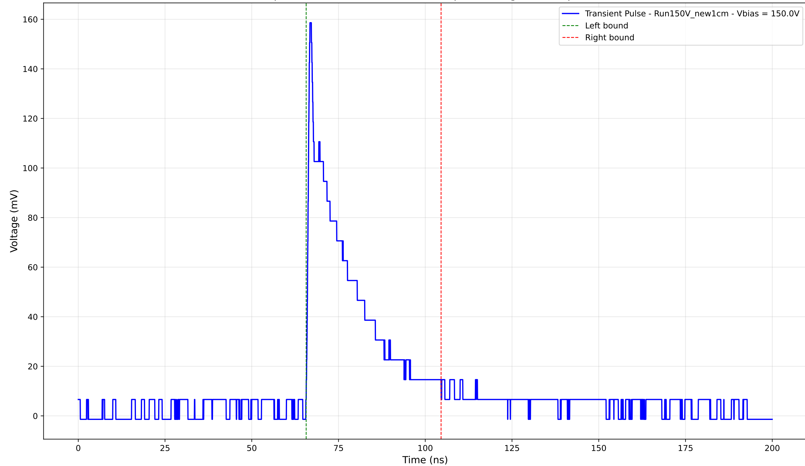
Transient Pulse - Sample: New1cm - Position: 2245.0 \mu\text{m} - Charge: 36.25 pC - Rise Time: 0.88 ns
