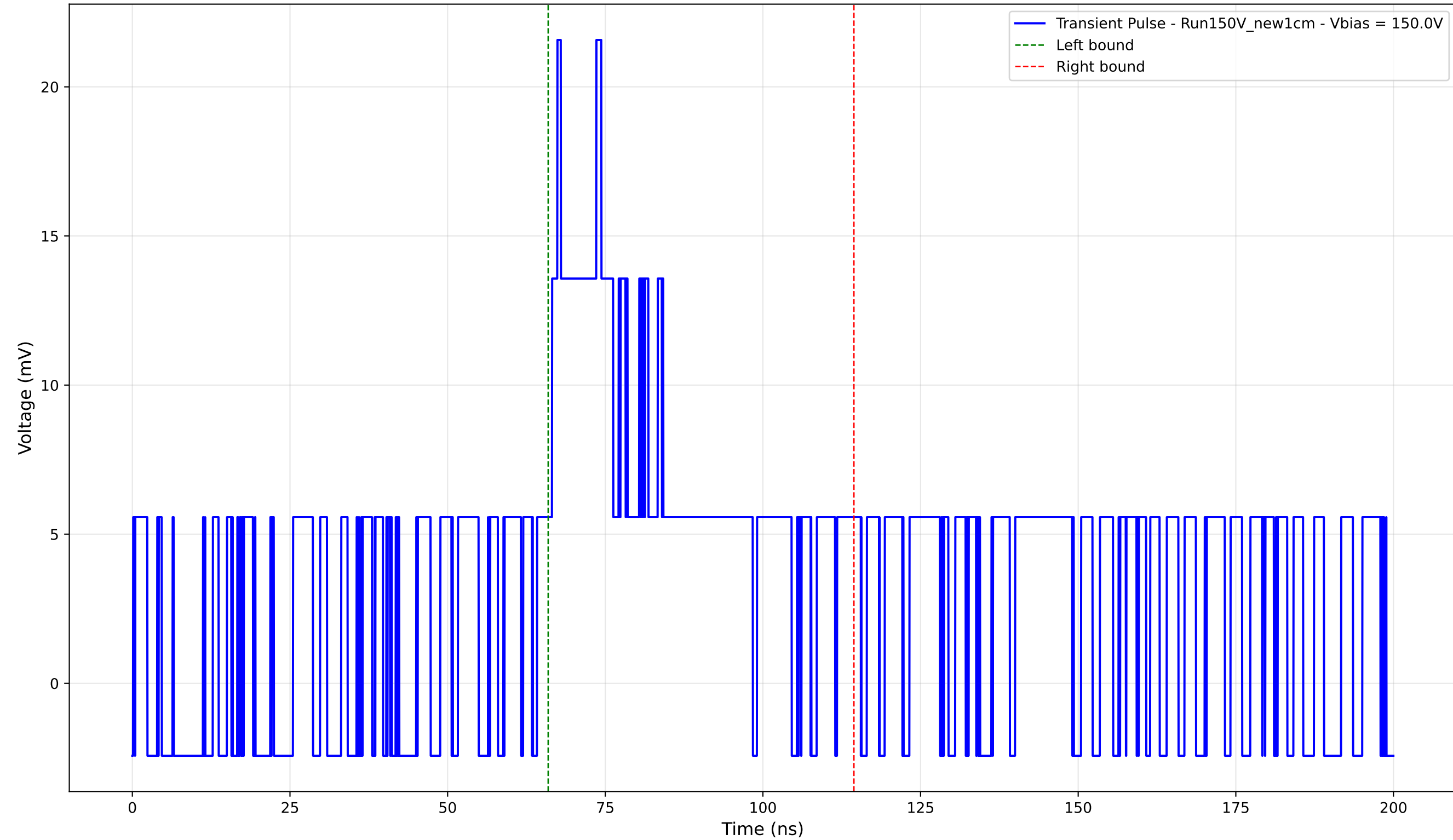
Transient Pulse - Sample: New1cm - Position: 530.0 \mu\text{m} - Charge: 7.20 pC - Rise Time: 0.00 ns (N/A)
