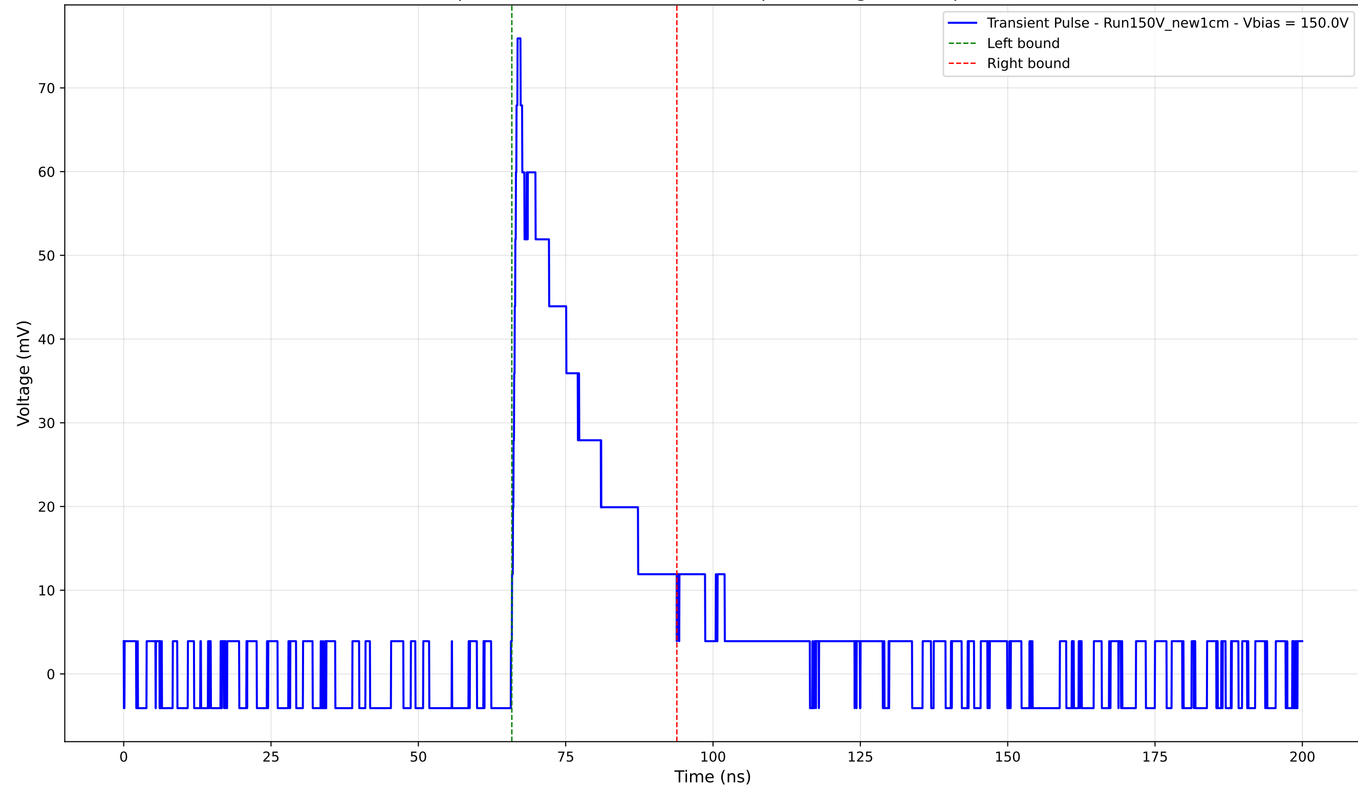
Transient Pulse - Sample: New1cm - Position: 2100.0 \mu\text{m} - Charge: 17.22 pC - Rise Time: 0.95 ns
