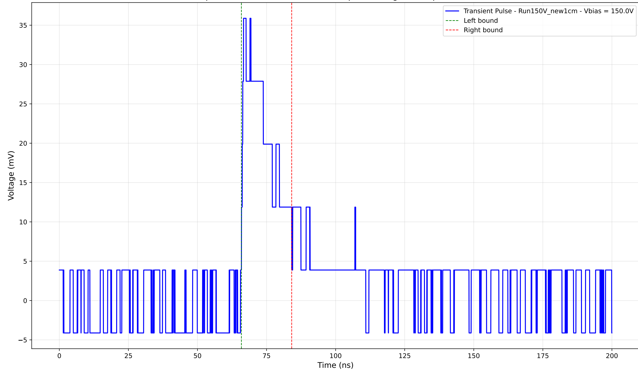
Transient Pulse - Sample: New1cm - Position: 2070.0 \mu\text{m} - Charge: 7.65 pC - Rise Time: 0.00 ns (N/A)
