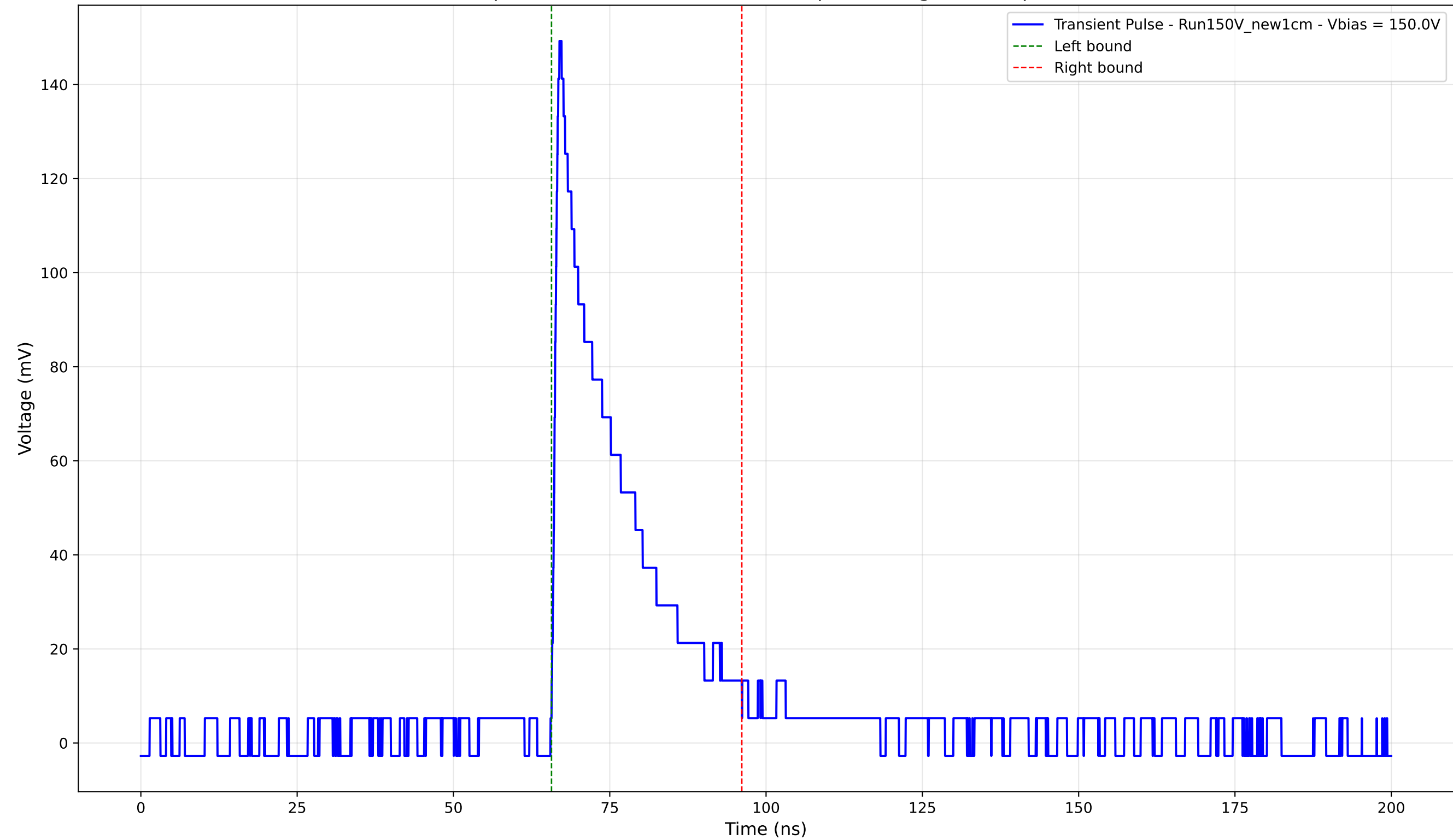
Transient Pulse - Sample: New1cm - Position: 4775.0 \mu\text{m} - Charge: 30.46 pC - Rise Time: 1.00 ns
