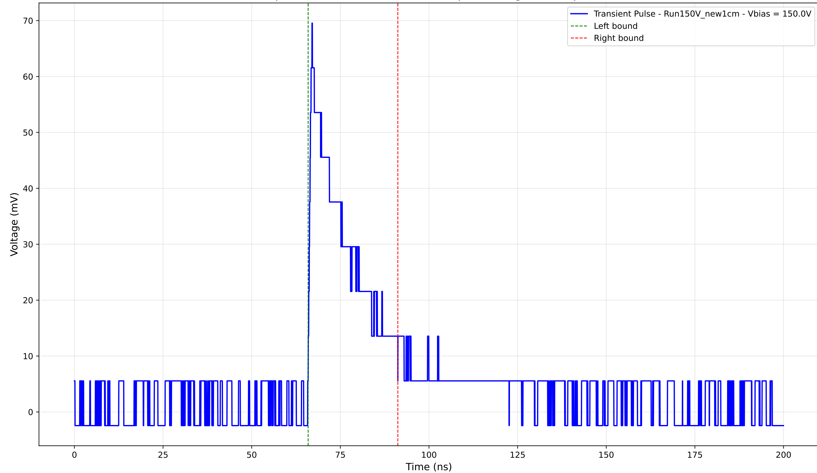
Transient Pulse - Sample: New1cm - Position: 2090.0 \mu\text{m} - Charge: 15.00 pC - Rise Time: 1.08 ns
