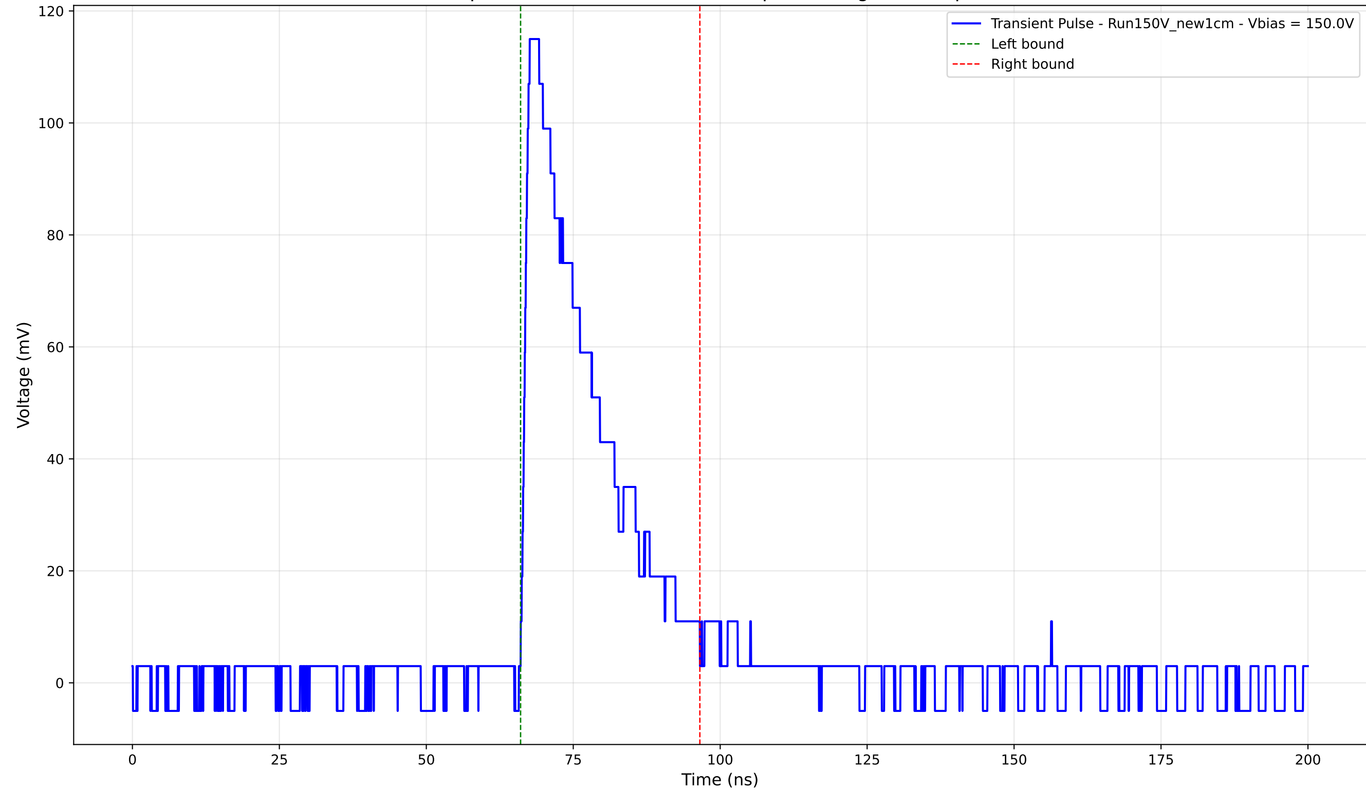
Transient Pulse - Sample: New1cm - Position: 715.0 \mu\text{m} - Charge: 29.22 pC - Rise Time: 1.18 ns
