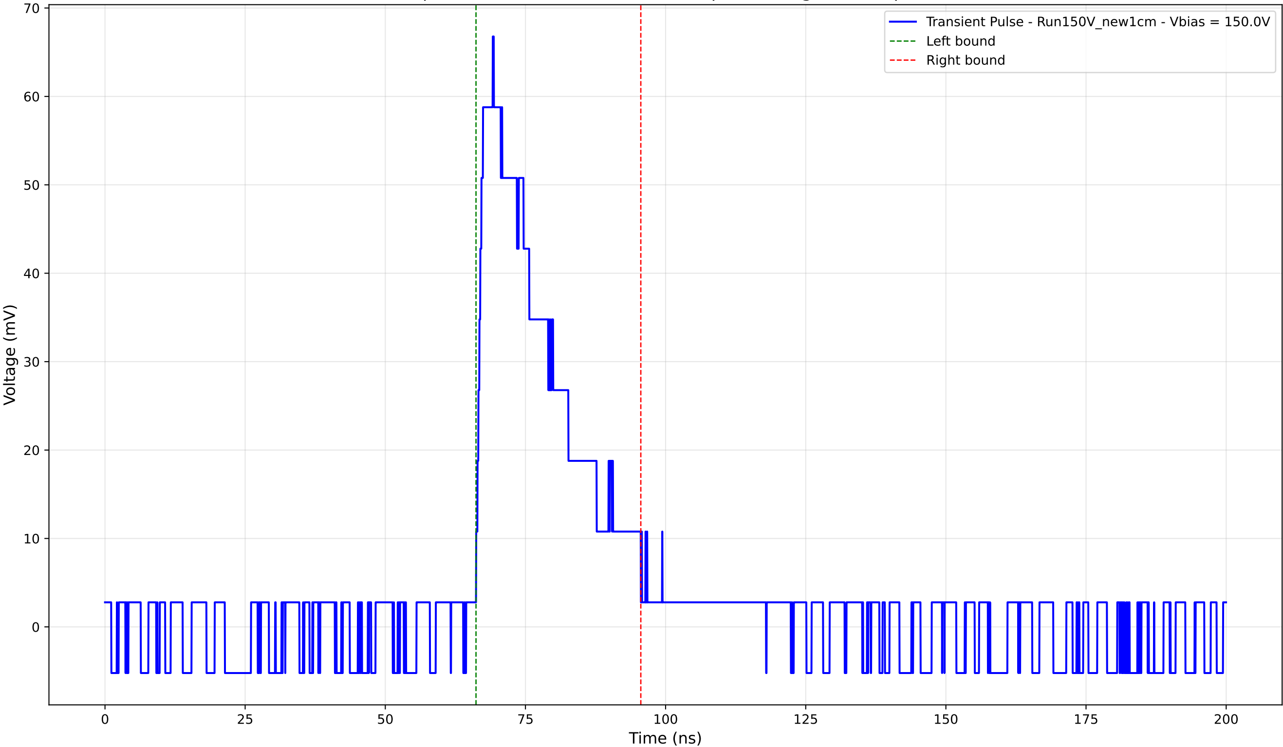
Transient Pulse - Sample: New1cm - Position: 1600.0 \mu\text{m} - Charge: 17.53 pC - Rise Time: 2.97 ns
