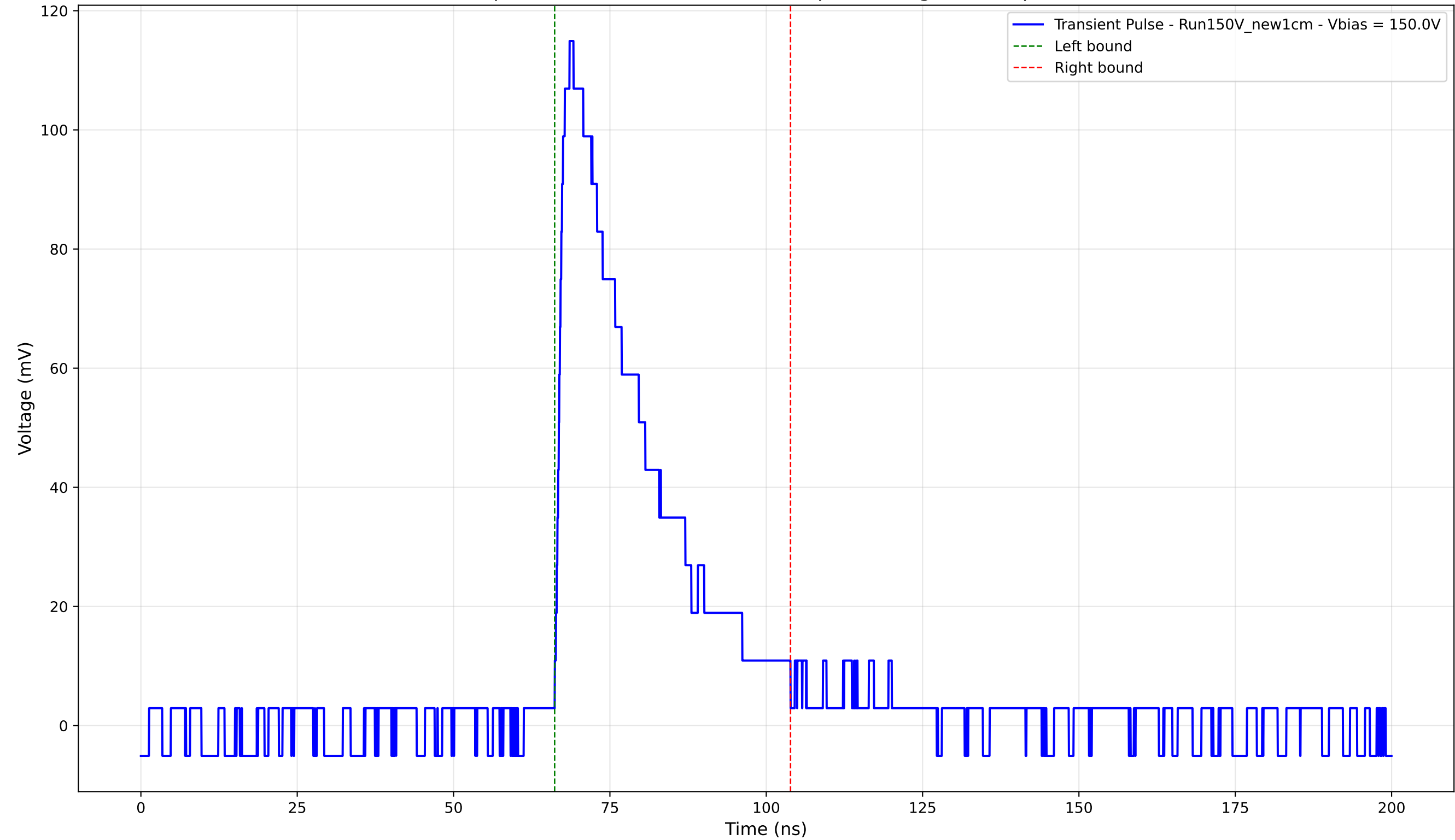
Transient Pulse - Sample: New1cm - Position: 1410.0 \mu\text{m} - Charge: 32.96 pC - Rise Time: 1.44 ns
