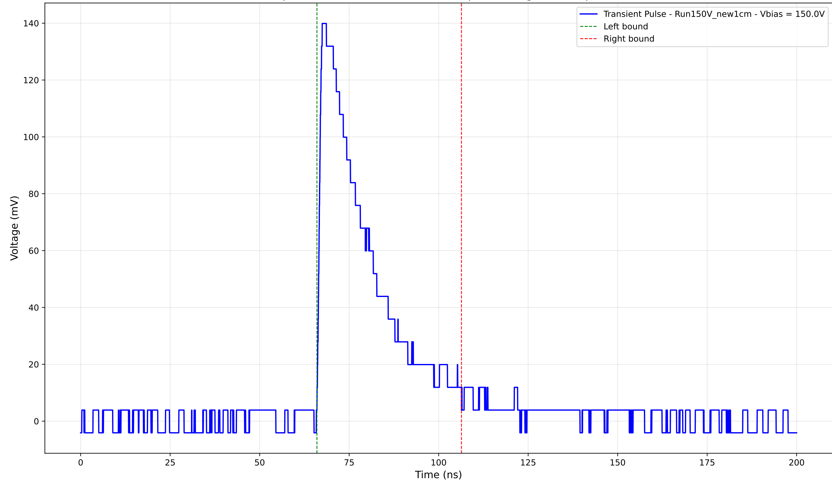
Transient Pulse - Sample: New1cm - Position: 3410.0 \mu\text{m} - Charge: 42.32 pC - Rise Time: 1.15 ns
