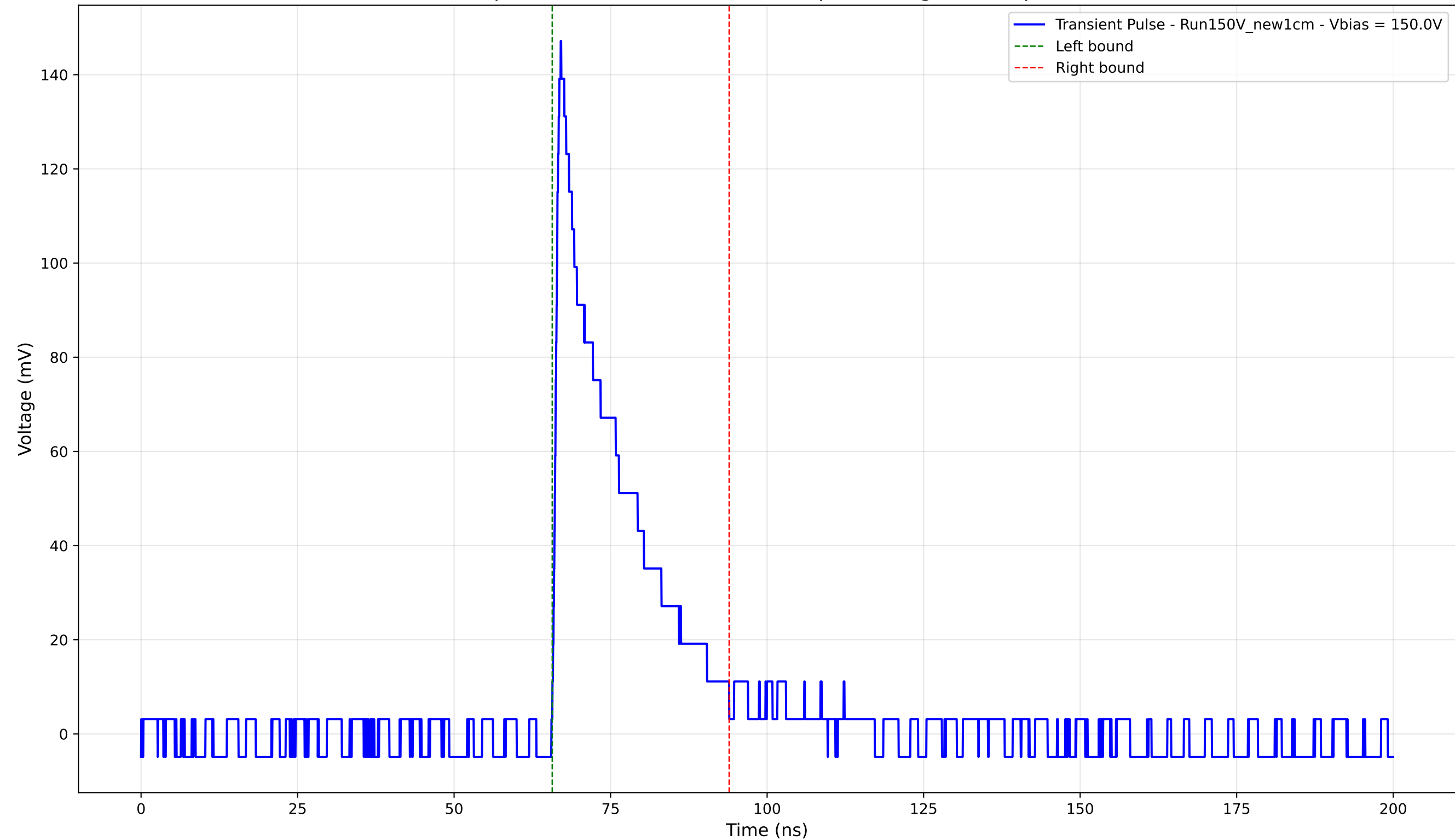
Transient Pulse - Sample: New1cm - Position: 4780.0 \mu\text{m} - Charge: 28.53 pC - Rise Time: 1.01 ns
