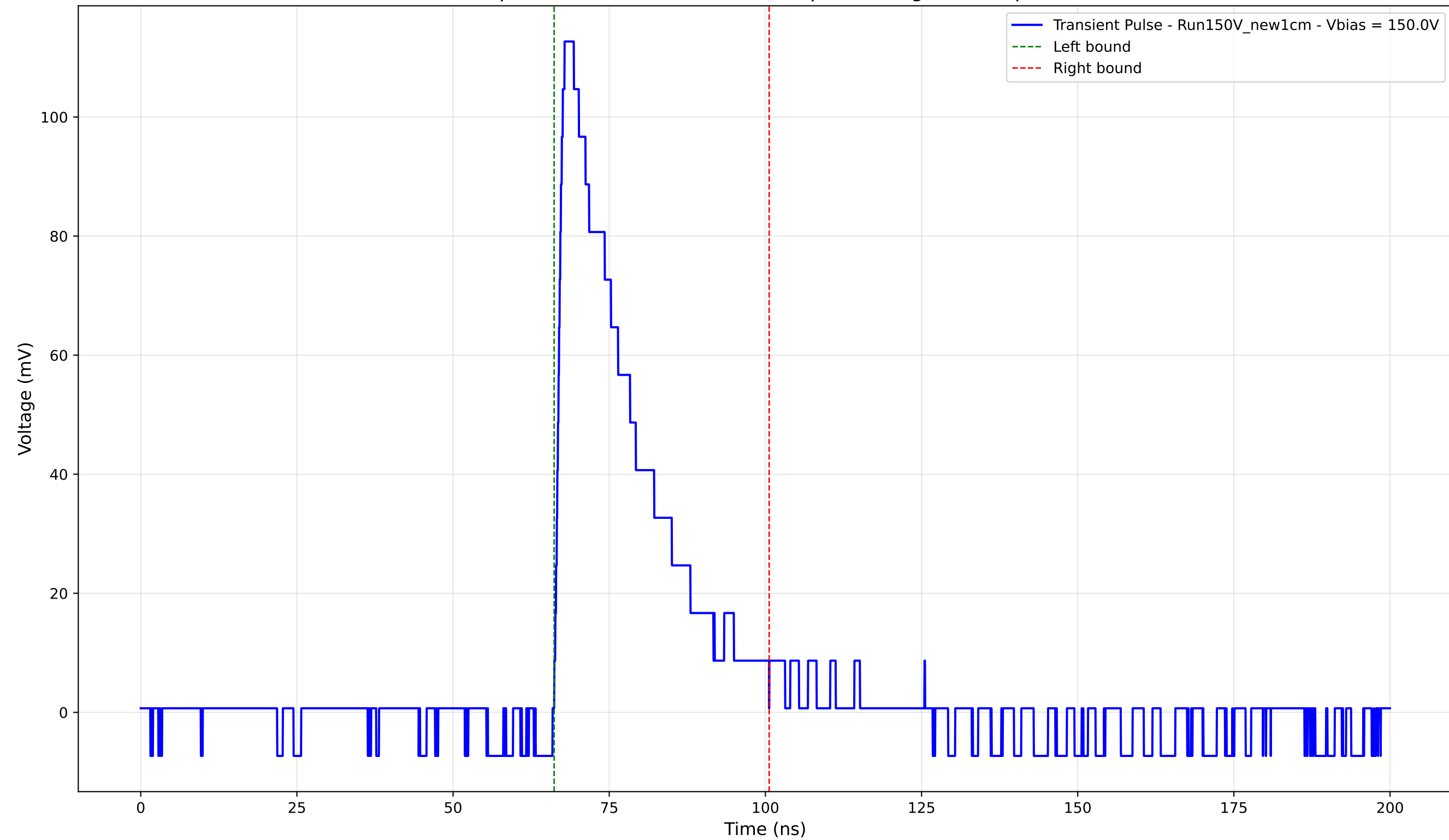
Transient Pulse - Sample: New1cm - Position: 845.0 \mu\text{m} - Charge: 28.95 pC - Rise Time: 1.21 ns
