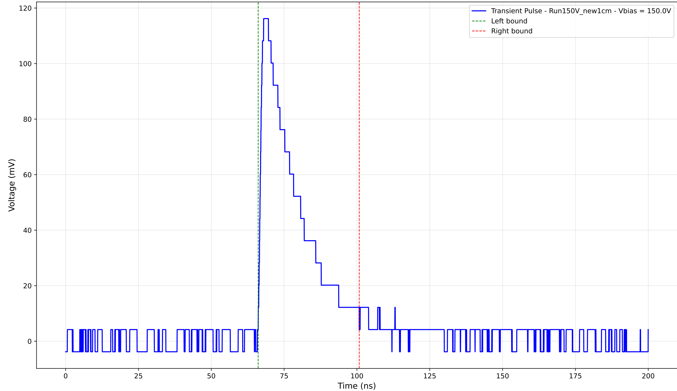
Transient Pulse - Sample: New1cm - Position: 820.0 \mu\text{m} - Charge: 32.06 pC - Rise Time: 1.44 ns
