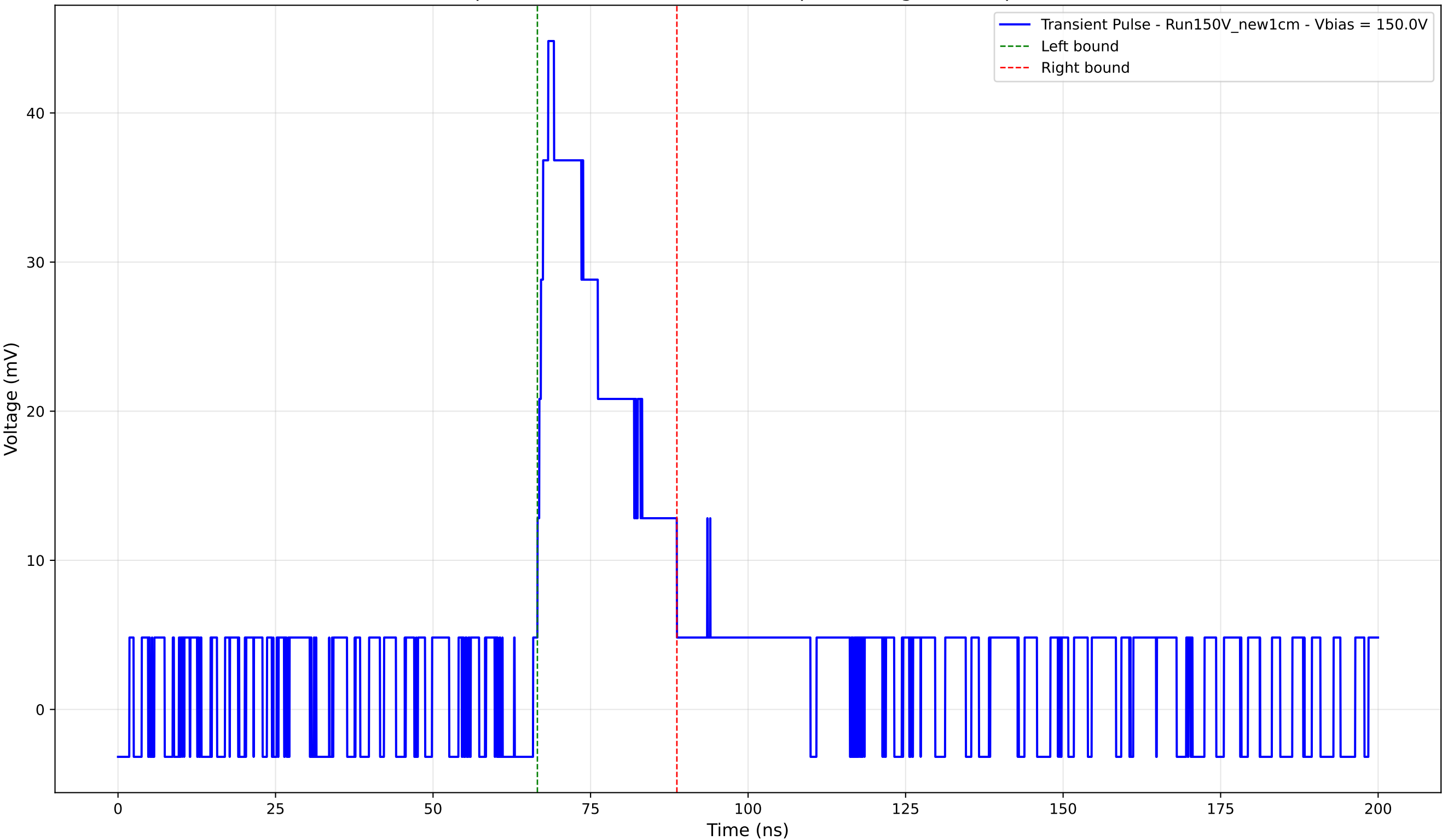
Transient Pulse - Sample: New1cm - Position: 1075.0 \mu\text{m} - Charge: 10.81 pC - Rise Time: 2.40 ns
