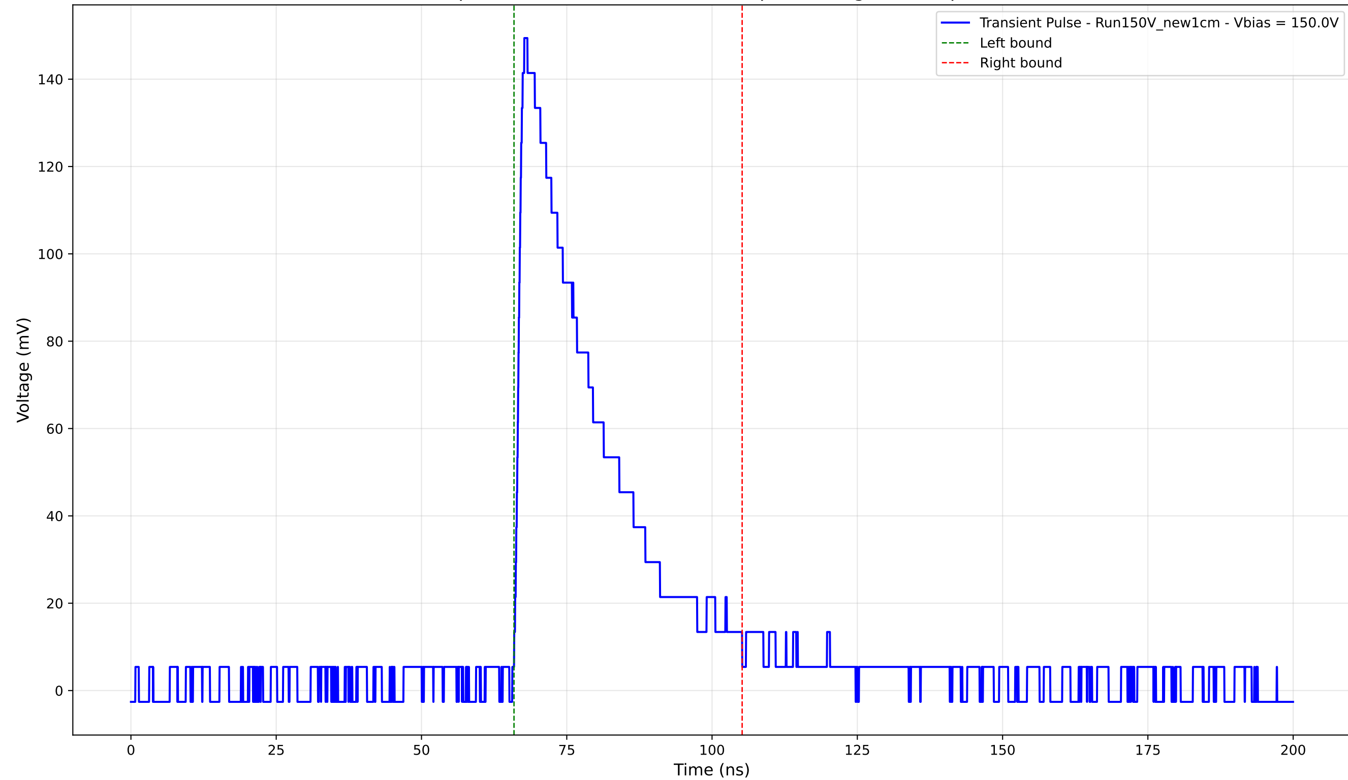
Transient Pulse - Sample: New1cm - Position: 3425.0 \mu\text{m} - Charge: 43.49 pC - Rise Time: 1.32 ns
