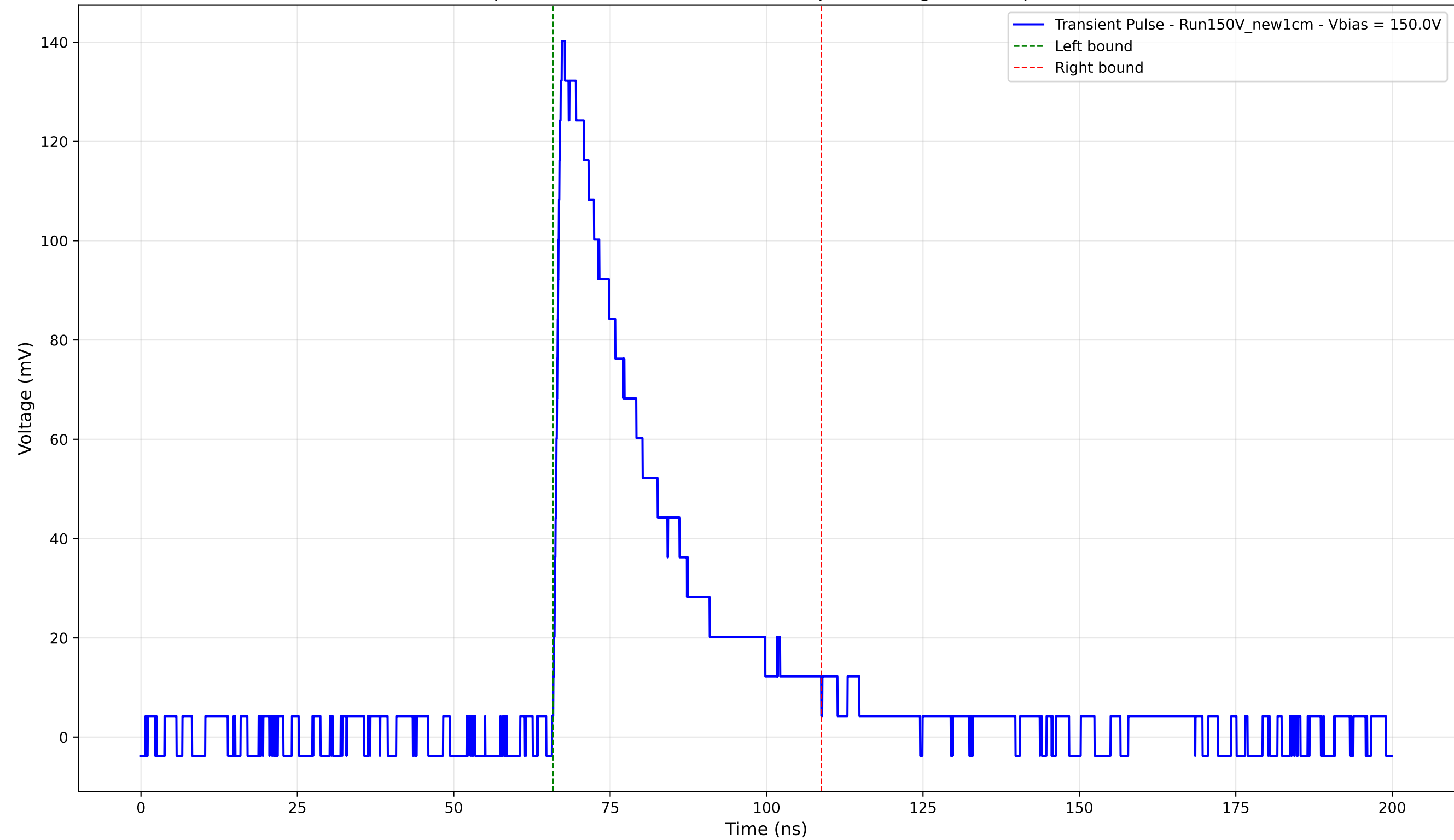
Transient Pulse - Sample: New1cm - Position: 3245.0 \mu\text{m} - Charge: 41.54 pC - Rise Time: 1.08 ns
