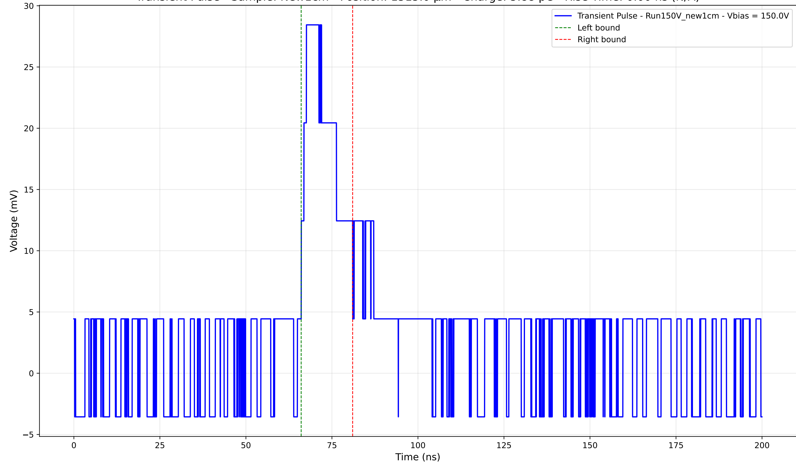
Transient Pulse - Sample: New1cm - Position: 1515.0 \mu\text{m} - Charge: 5.88 pC - Rise Time: 0.00 ns (N/A)
