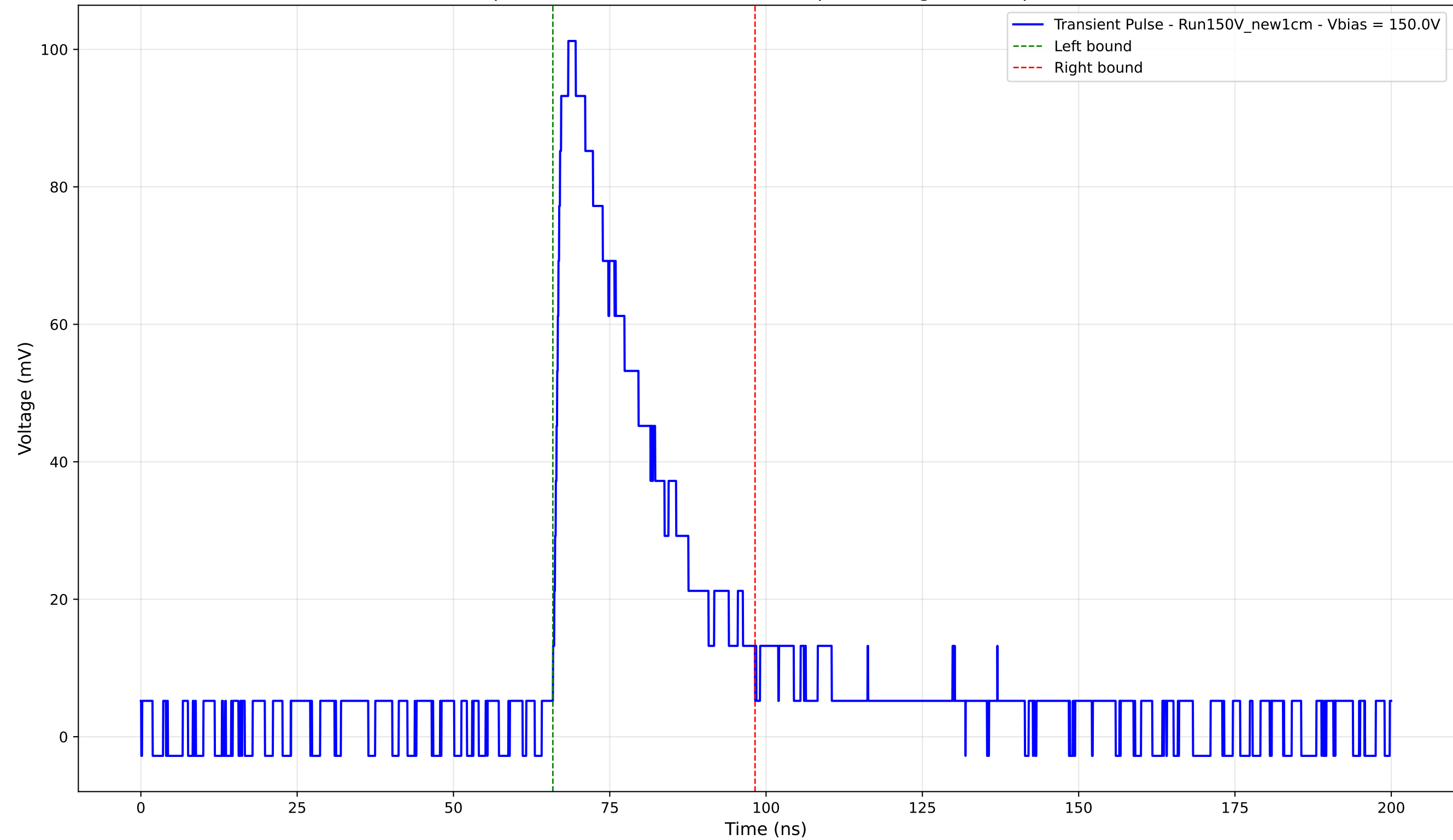
Transient Pulse - Sample: New1cm - Position: 1780.0 \mu\text{m} - Charge: 29.88 pC - Rise Time: 1.31 ns
