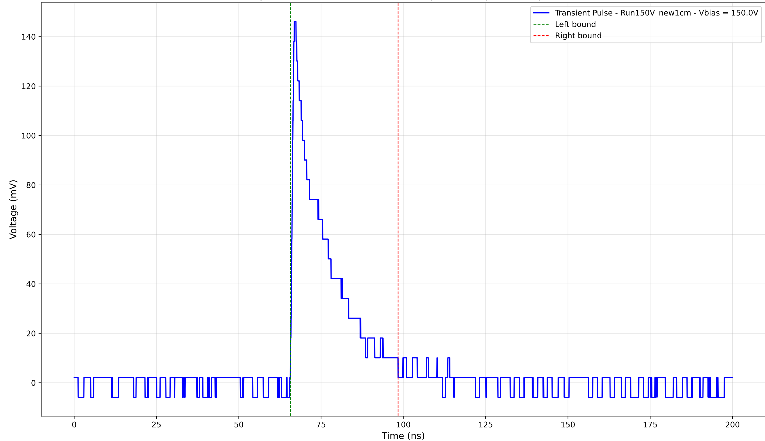
Transient Pulse - Sample: New1cm - Position: 4770.0 \mu\text{m} - Charge: 29.48 pC - Rise Time: 0.97 ns
