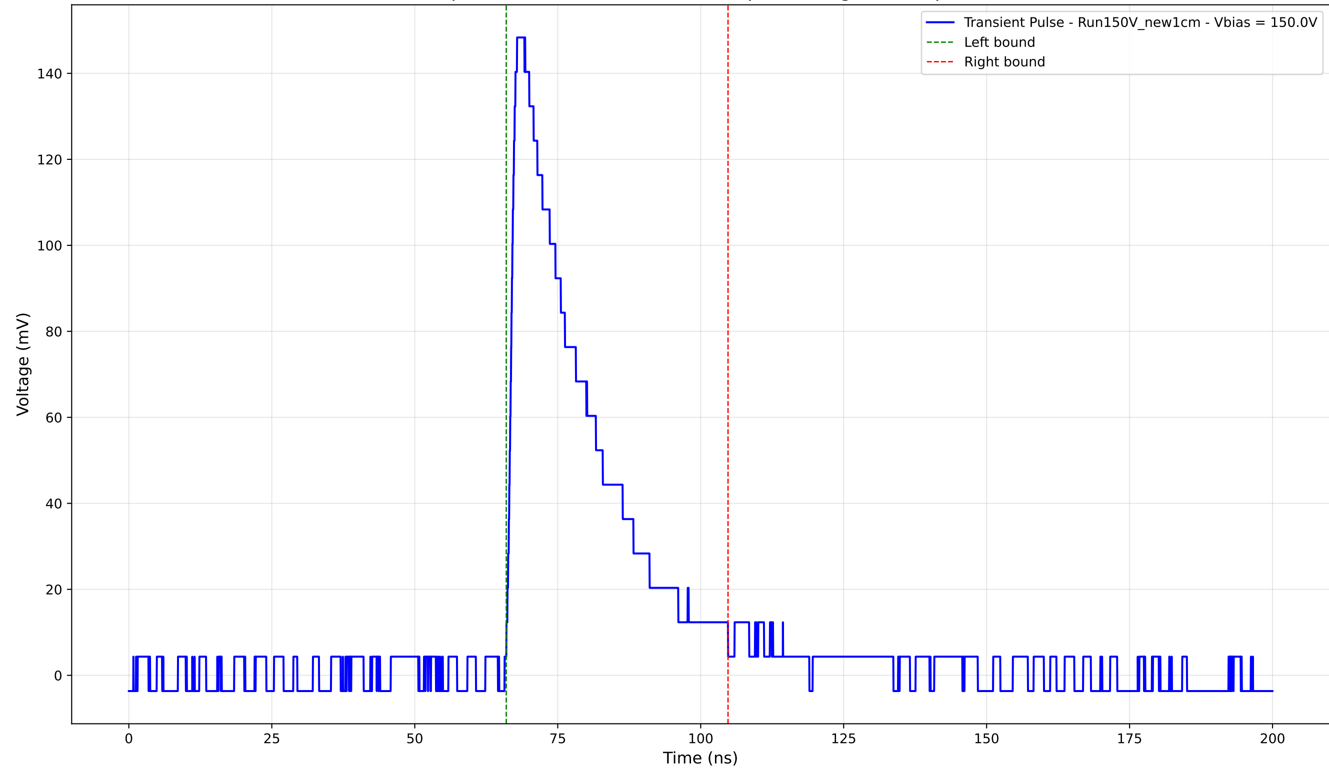
Transient Pulse - Sample: New1cm - Position: 3880.0 \mu\text{m} - Charge: 41.66 pC - Rise Time: 1.41 ns
