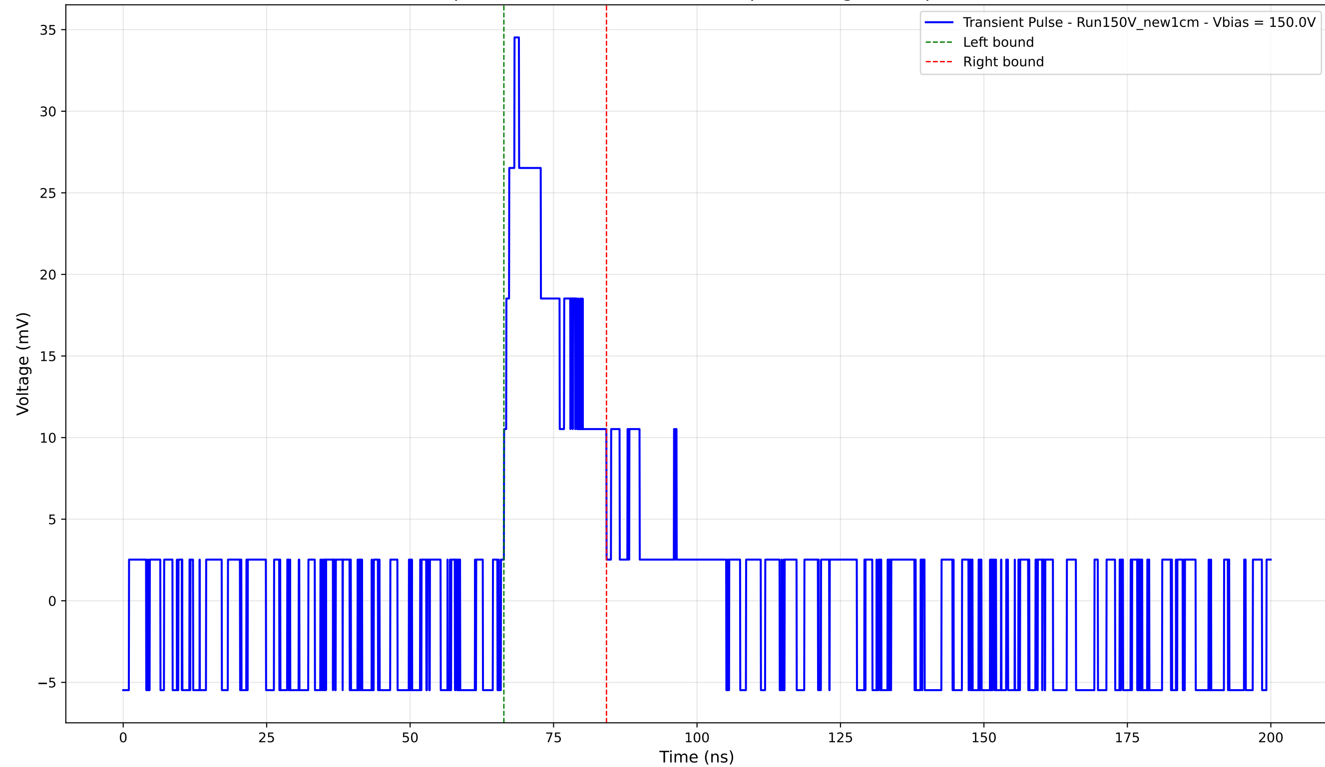
Transient Pulse - Sample: New1cm - Position: 3585.0 \mu\text{m} - Charge: 6.62 pC - Rise Time: 1.84 ns
