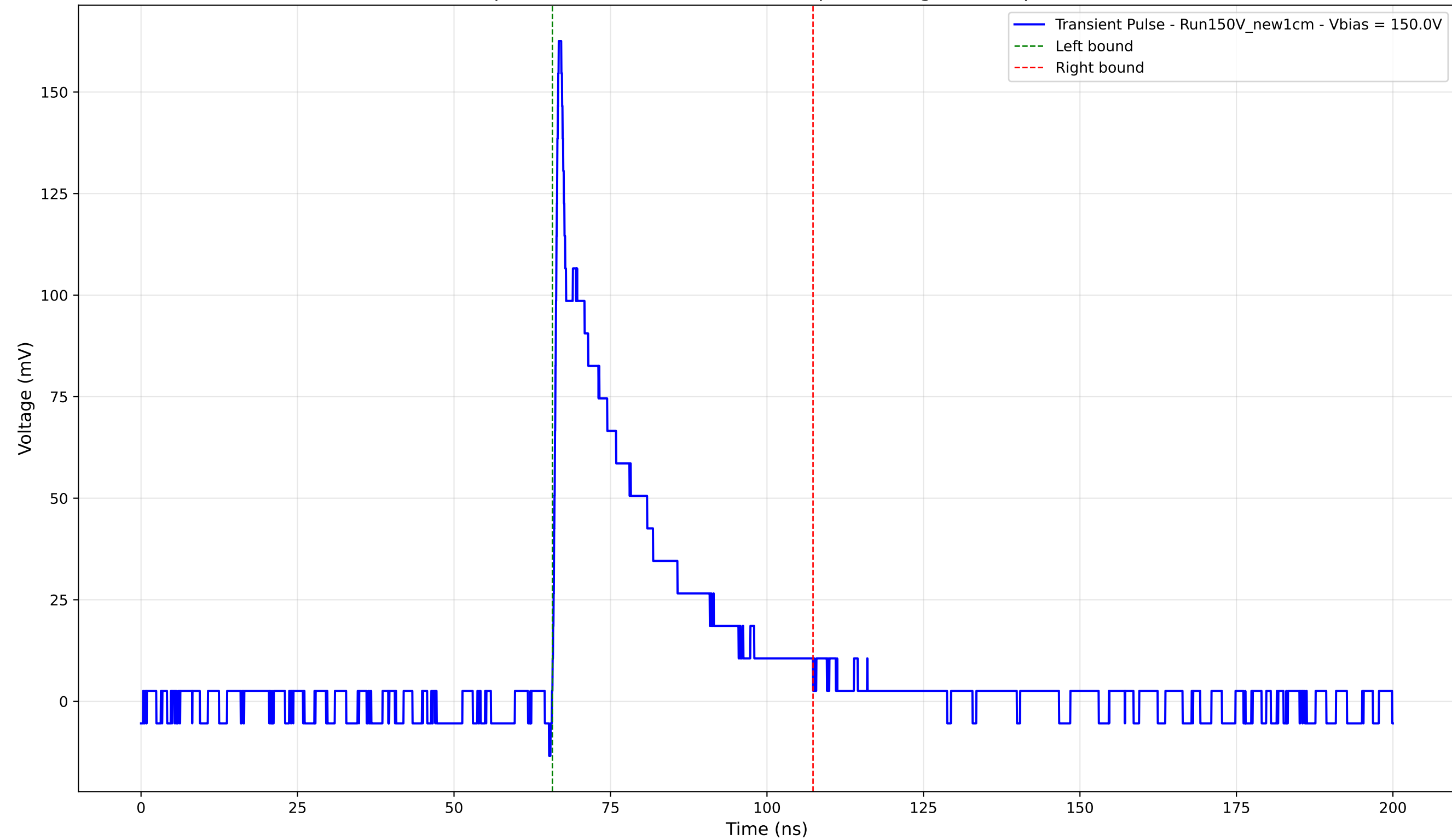
Transient Pulse - Sample: New1cm - Position: 2280.0 \mu\text{m} - Charge: 34.63 pC - Rise Time: 0.77 ns
