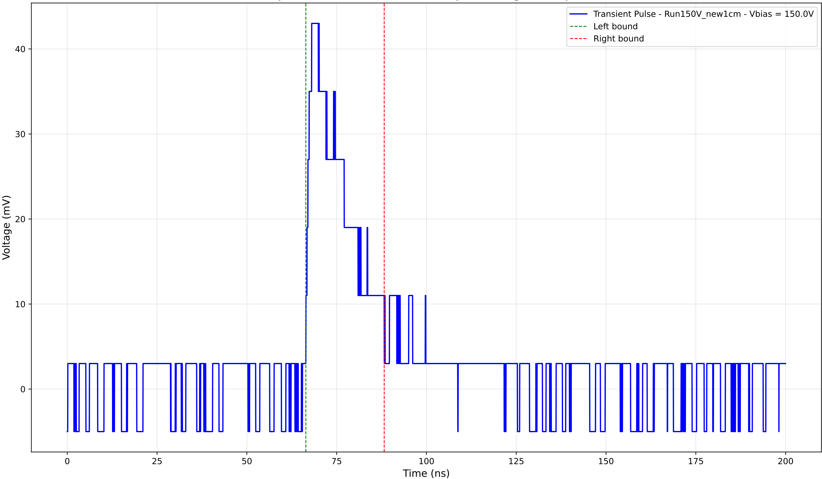
Transient Pulse - Sample: New1cm - Position: 995.0 \mu\text{m} - Charge: 9.91 pC - Rise Time: 1.62 ns
