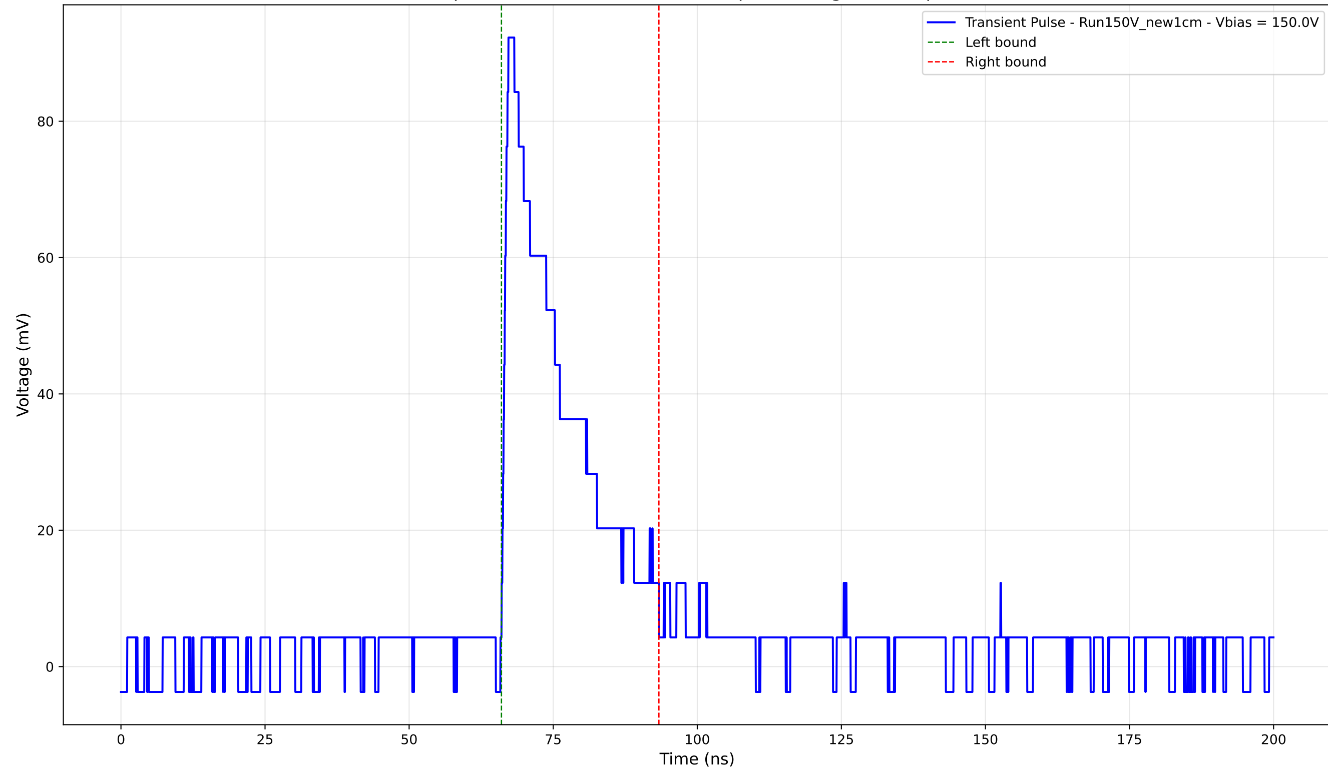
Transient Pulse - Sample: New1cm - Position: 455.0 \mu\text{m} - Charge: 20.98 pC - Rise Time: 1.03 ns
