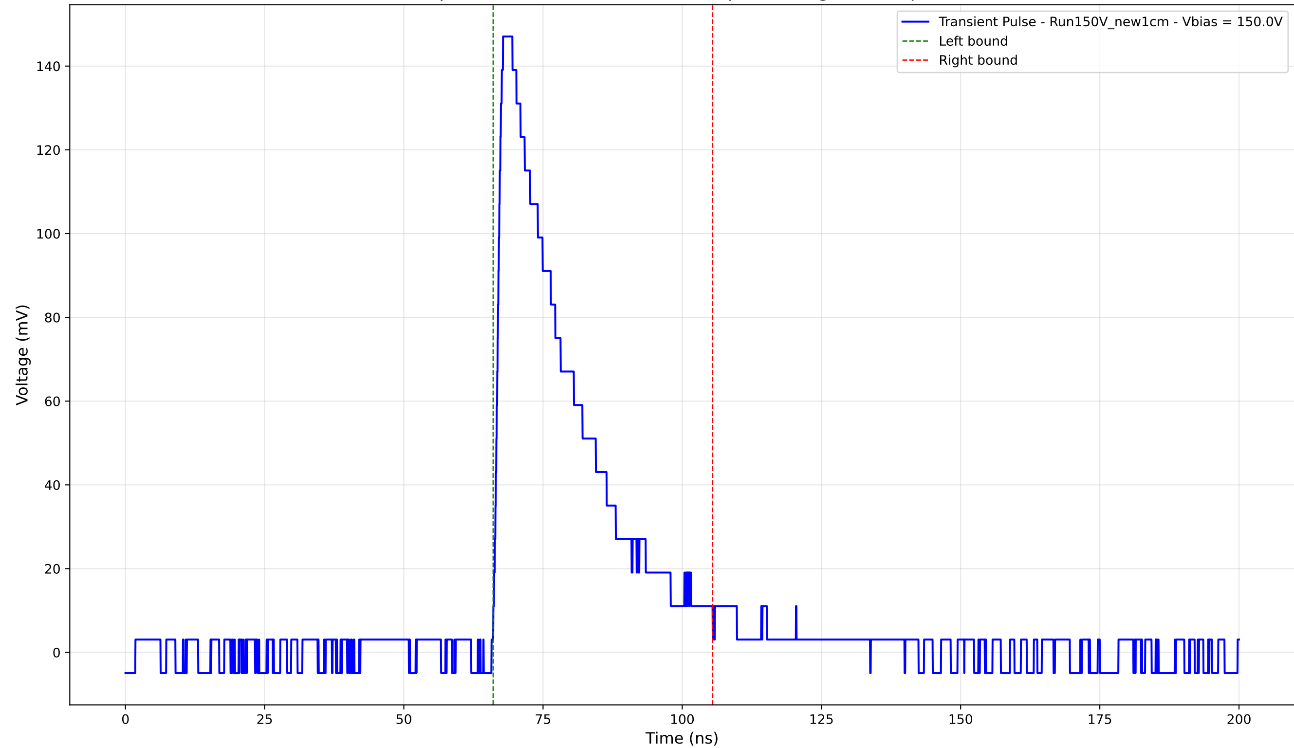
Transient Pulse - Sample: New1cm - Position: 3860.0 \mu\text{m} - Charge: 42.55 pC - Rise Time: 1.39 ns
