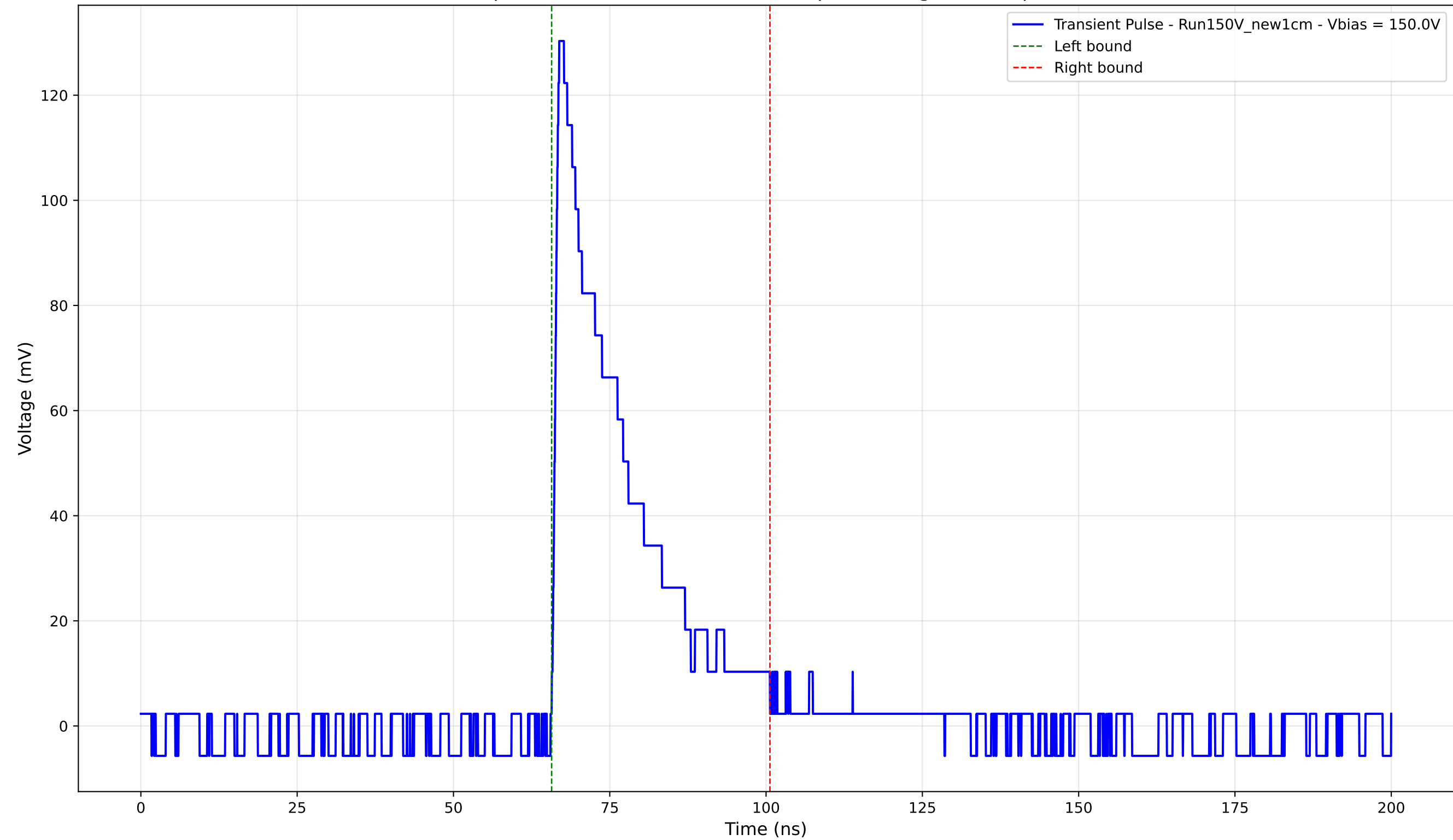
Transient Pulse - Sample: New1cm - Position: 4690.0 \mu\text{m} - Charge: 29.53 pC - Rise Time: 0.93 ns
