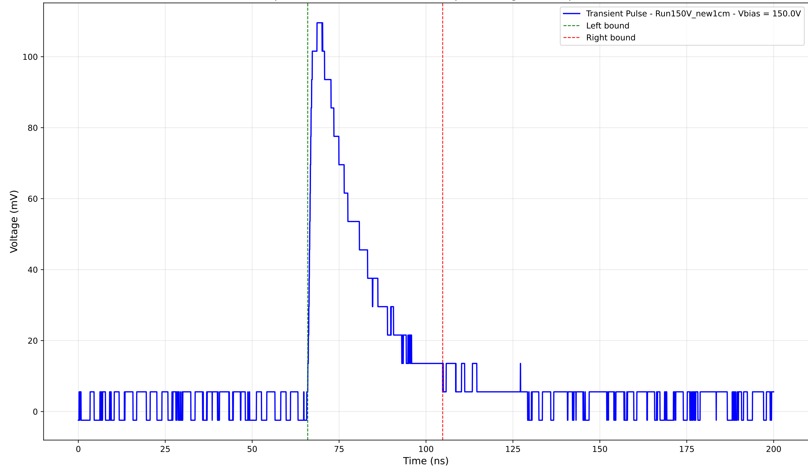
Transient Pulse - Sample: New1cm - Position: 1735.0 \mu\text{m} - Charge: 34.28 pC - Rise Time: 1.29 ns
