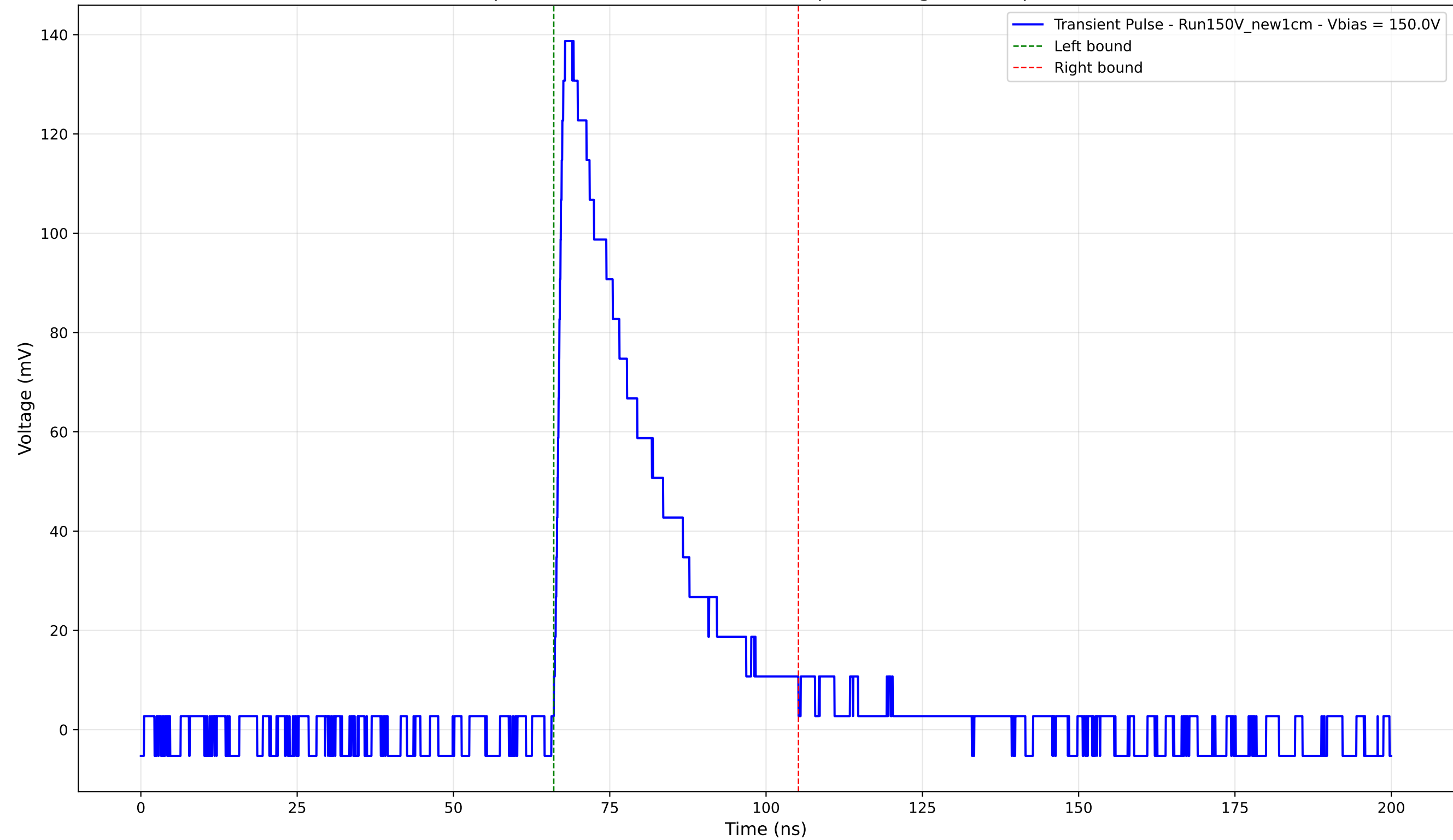
Transient Pulse - Sample: New1cm - Position: 3725.0 \mu\text{m} - Charge: 39.84 pC - Rise Time: 1.35 ns
