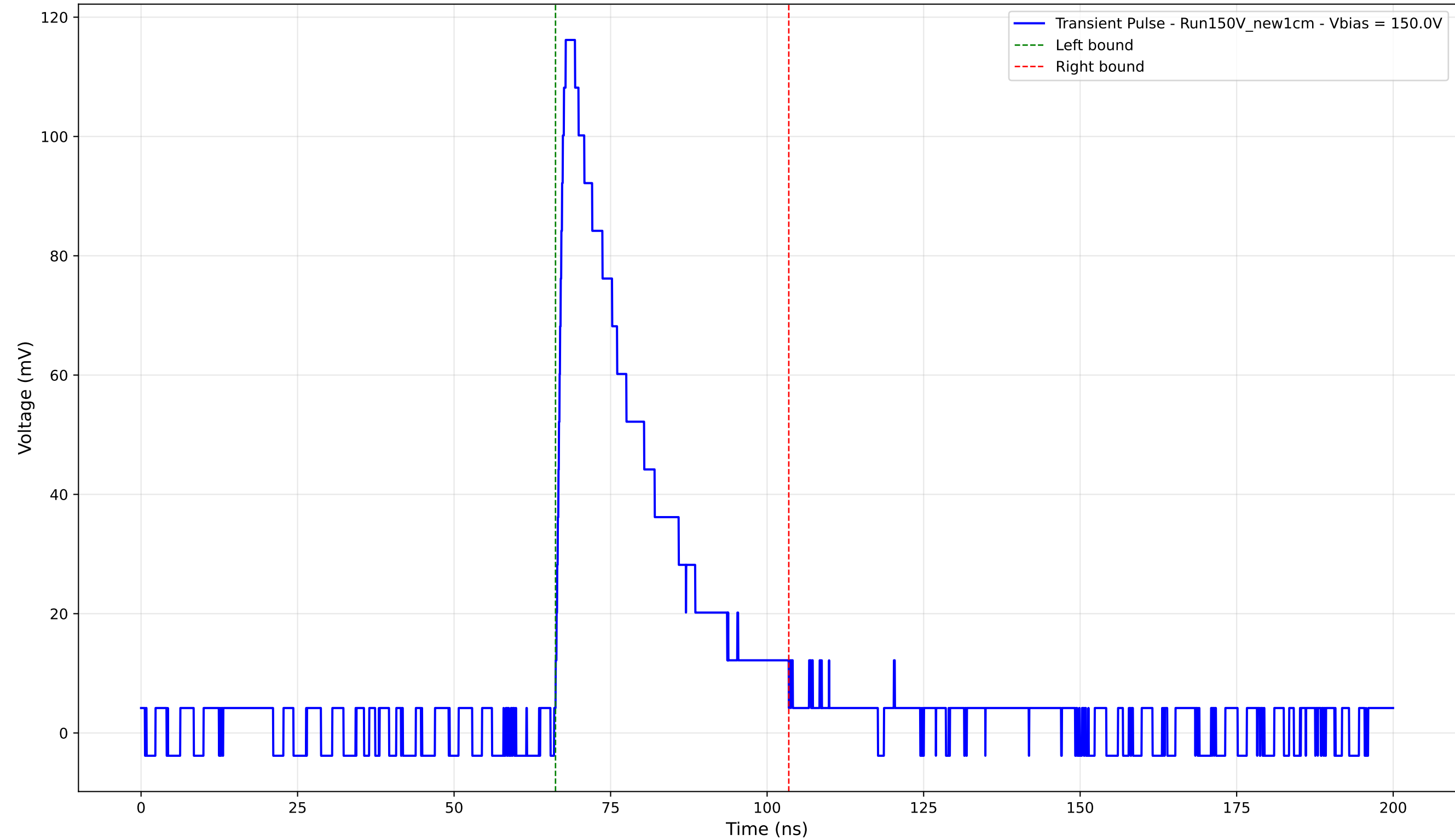
Transient Pulse - Sample: New1cm - Position: 835.0 \mu\text{m} - Charge: 32.20 pC - Rise Time: 1.32 ns
