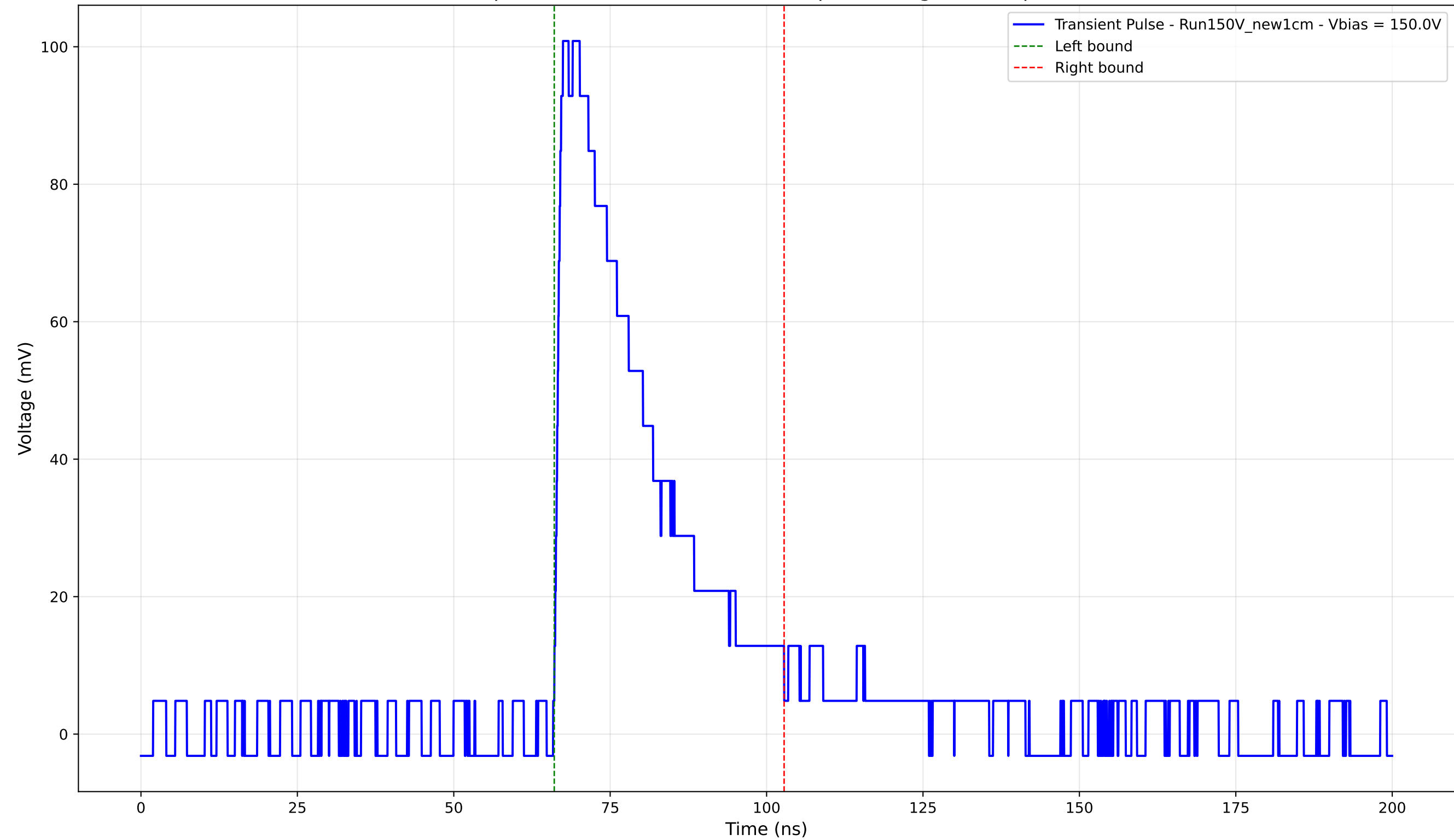
Transient Pulse - Sample: New1cm - Position: 1755.0 \mu\text{m} - Charge: 31.51 pC - Rise Time: 1.09 ns
