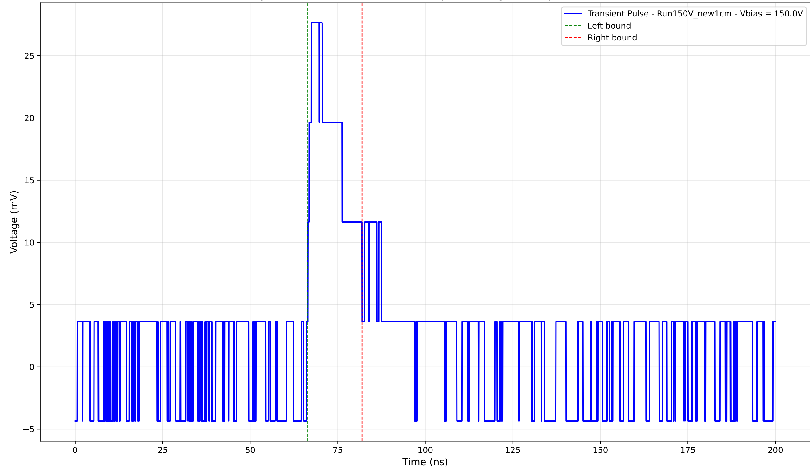
Transient Pulse - Sample: New1cm - Position: 1565.0 \mu\text{m} - Charge: 5.59 pC - Rise Time: 0.00 ns (N/A)
