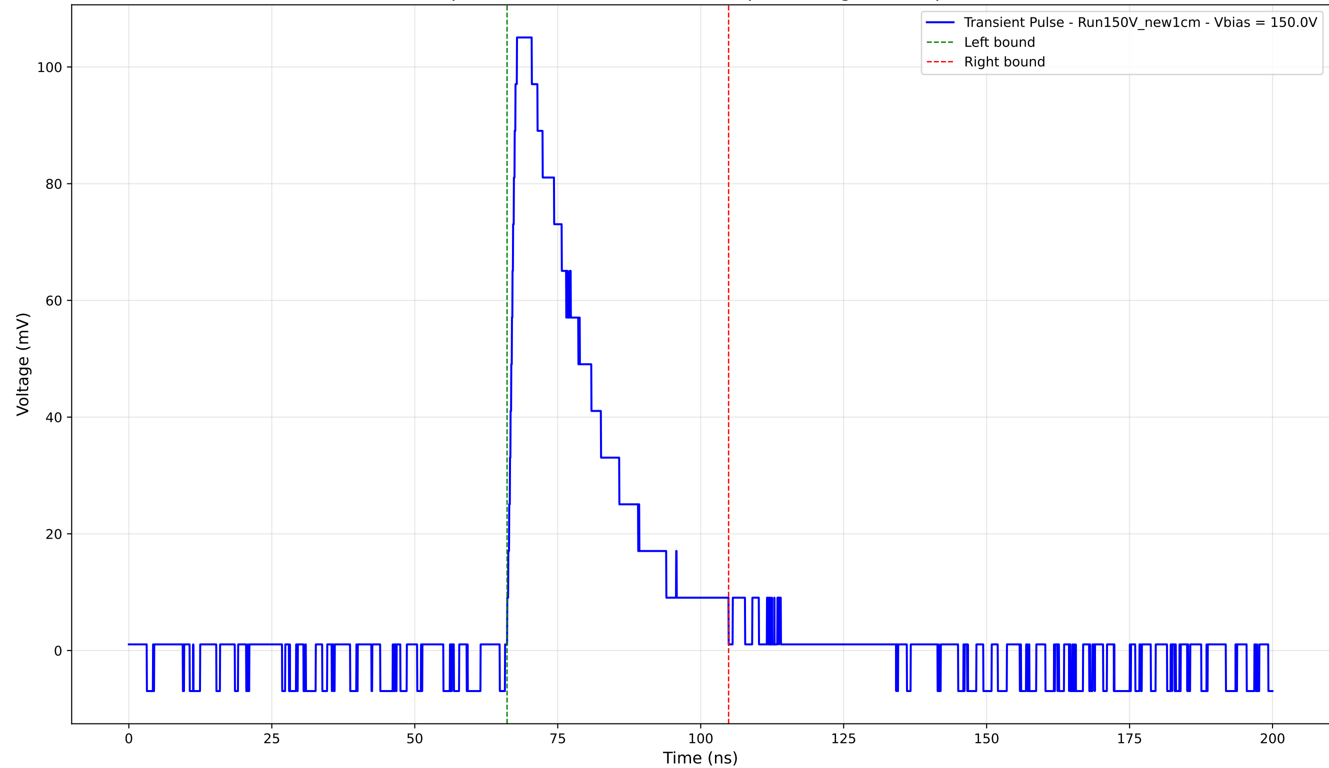
Transient Pulse - Sample: New1cm - Position: 1255.0 \mu\text{m} - Charge: 30.66 pC - Rise Time: 1.28 ns
