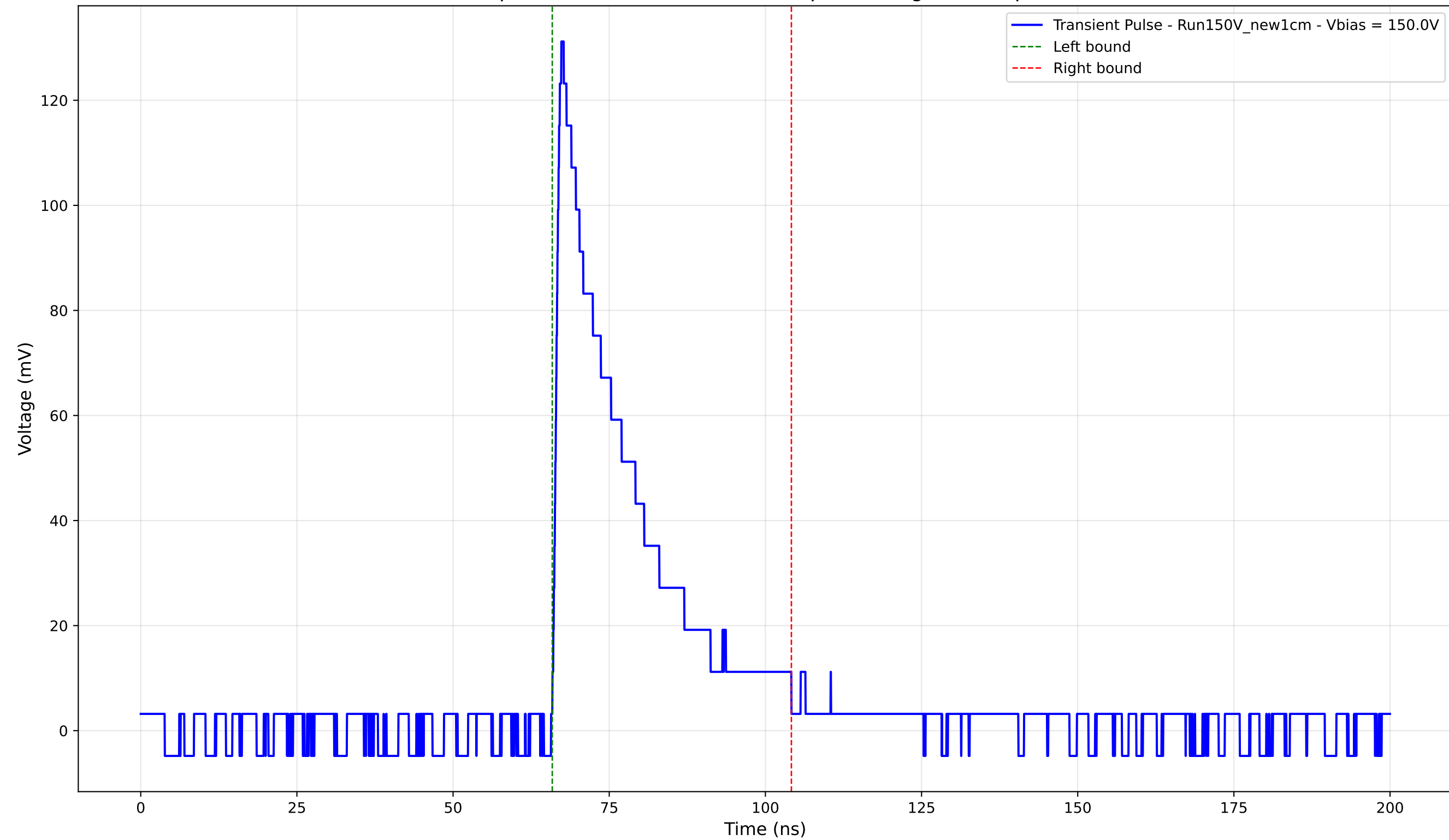
Transient Pulse - Sample: New1cm - Position: 385.0 \mu\text{m} - Charge: 30.41 pC - Rise Time: 1.06 ns
