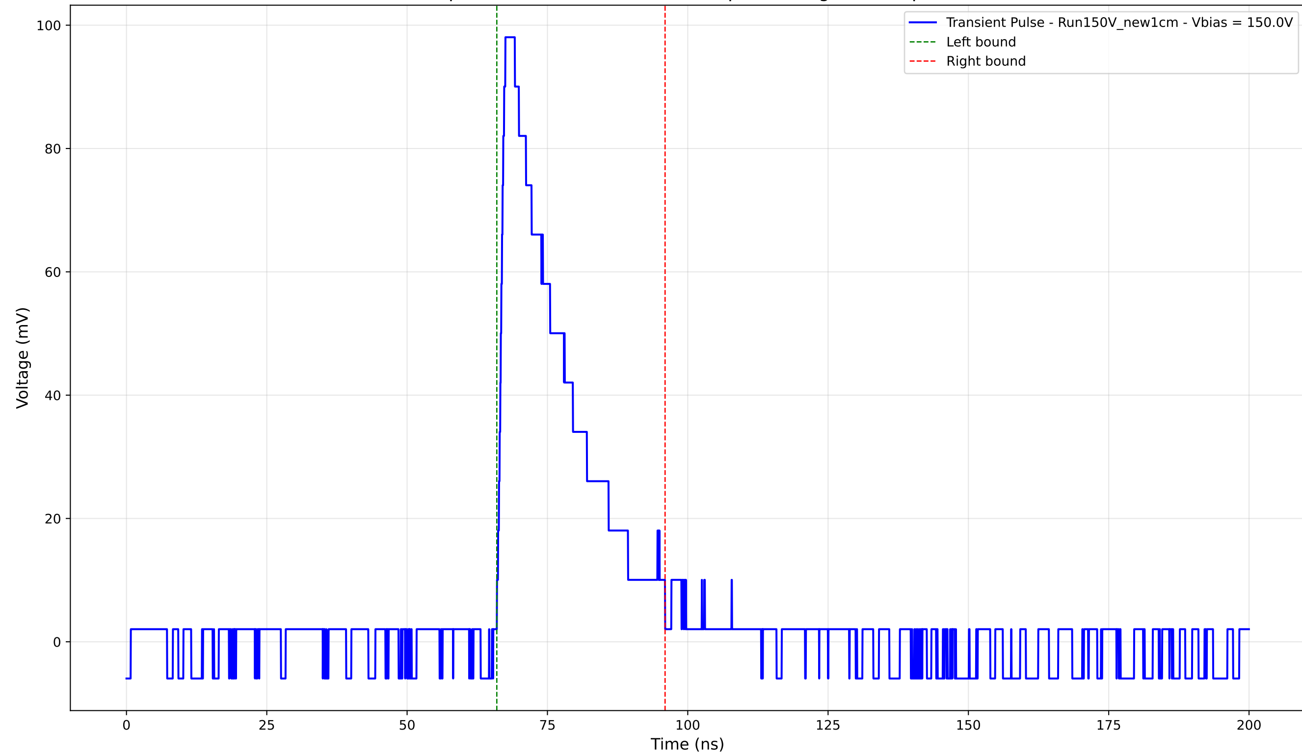
Transient Pulse - Sample: New1cm - Position: 625.0 \mu\text{m} - Charge: 23.99 pC - Rise Time: 1.28 ns
