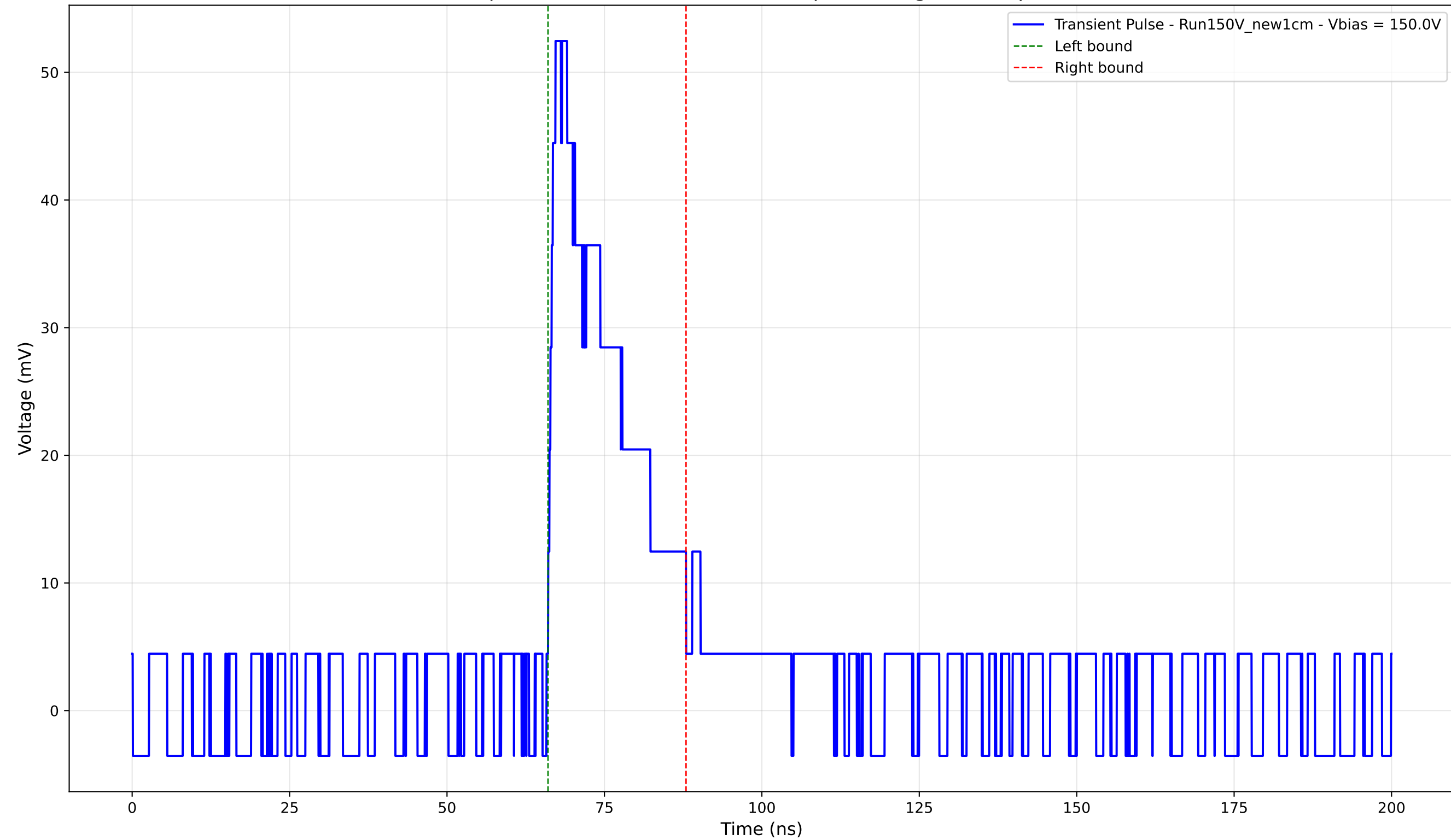
Transient Pulse - Sample: New1cm - Position: 4535.0 \mu\text{m} - Charge: 11.83 pC - Rise Time: 1.18 ns
