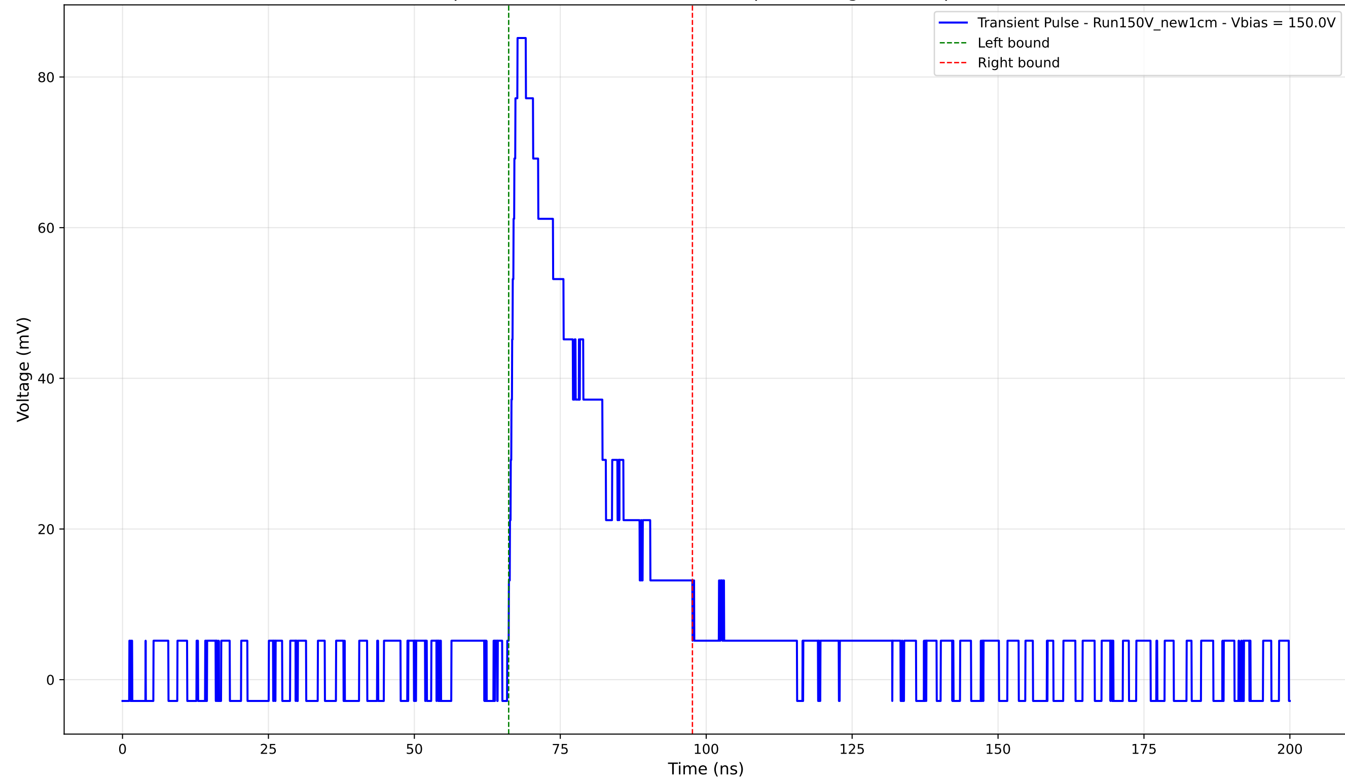
Transient Pulse - Sample: New1cm - Position: 4135.0 \mu\text{m} - Charge: 23.11 pC - Rise Time: 1.13 ns
