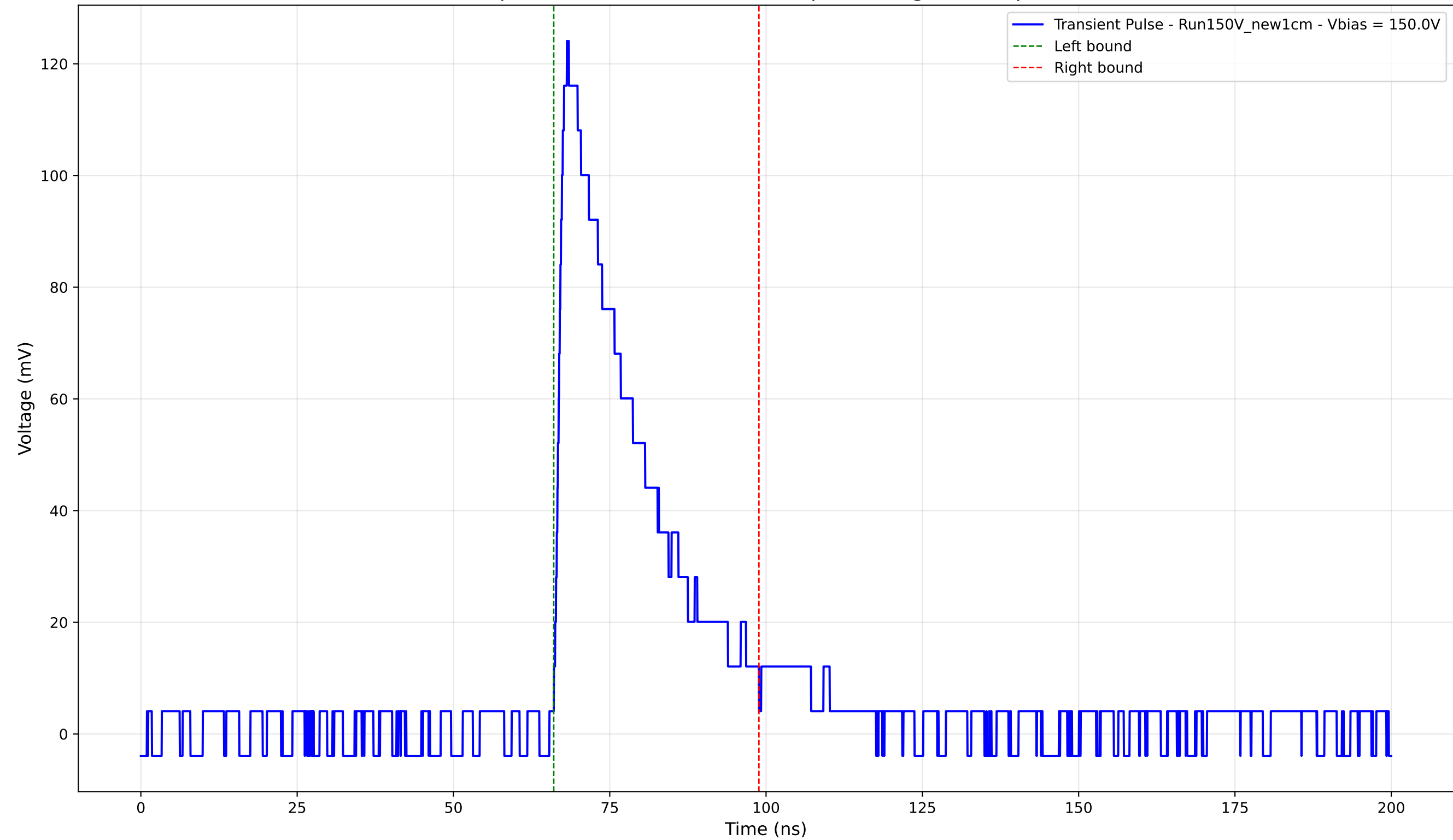
Transient Pulse - Sample: New1cm - Position: 825.0 \mu\text{m} - Charge: 32.23 pC - Rise Time: 1.44 ns
