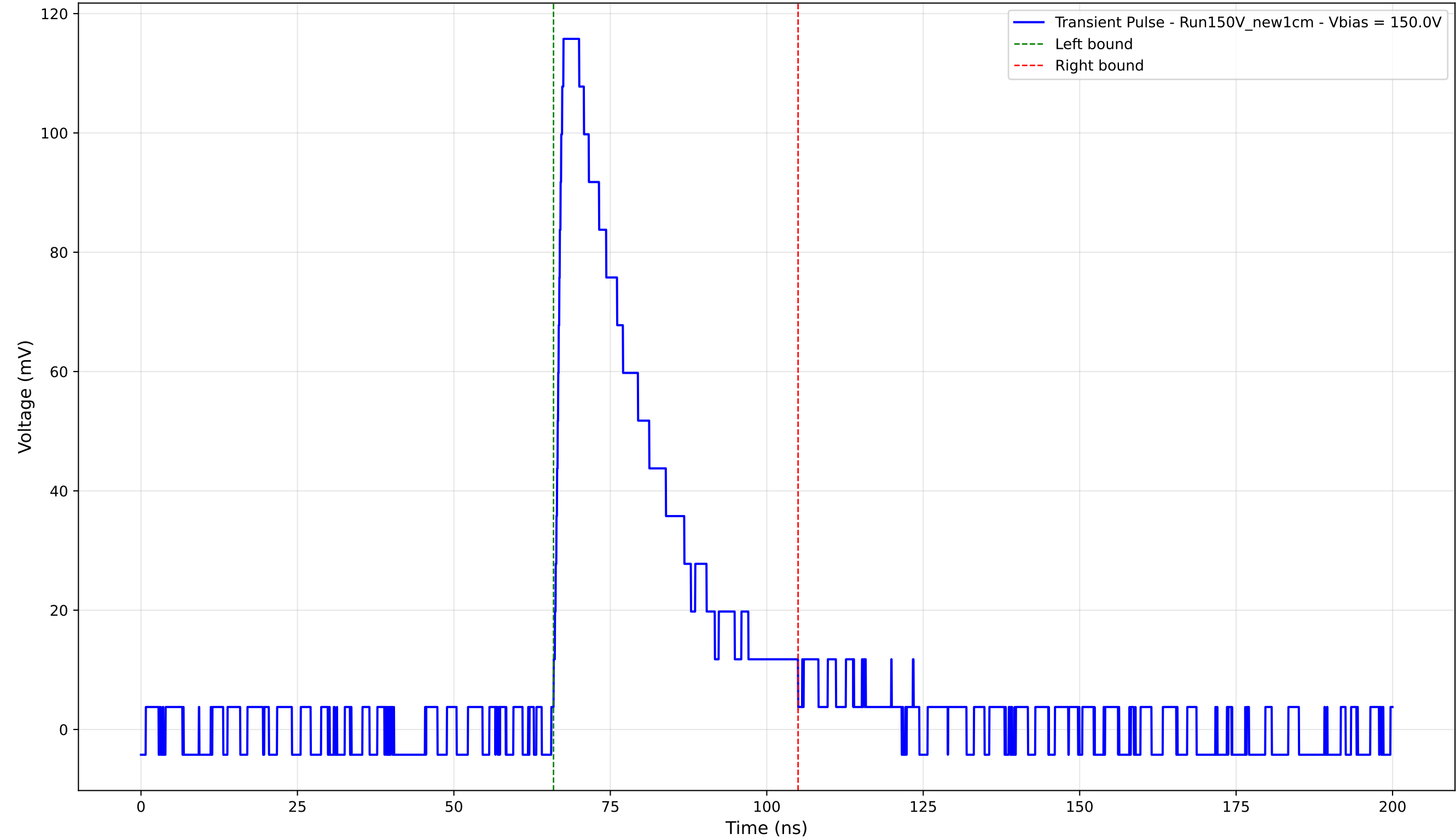
Transient Pulse - Sample: New1cm - Position: 3475.0 \mu\text{m} - Charge: 35.03 pC - Rise Time: 1.36 ns
