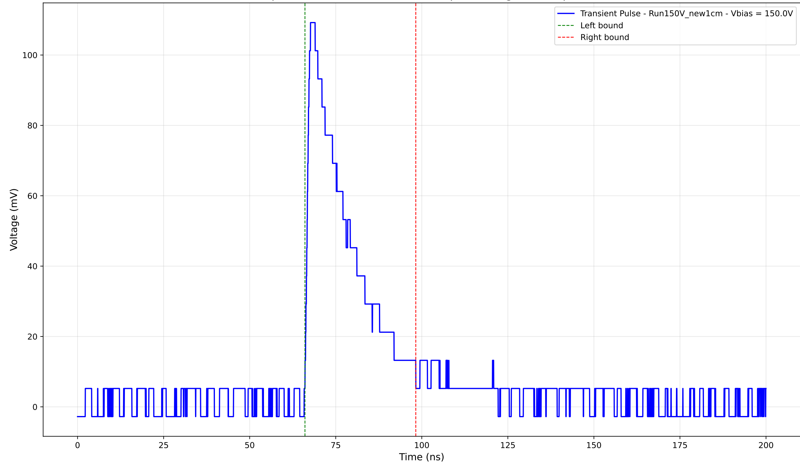
Transient Pulse - Sample: New1cm - Position: 4160.0 \mu\text{m} - Charge: 29.12 pC - Rise Time: 1.31 ns
