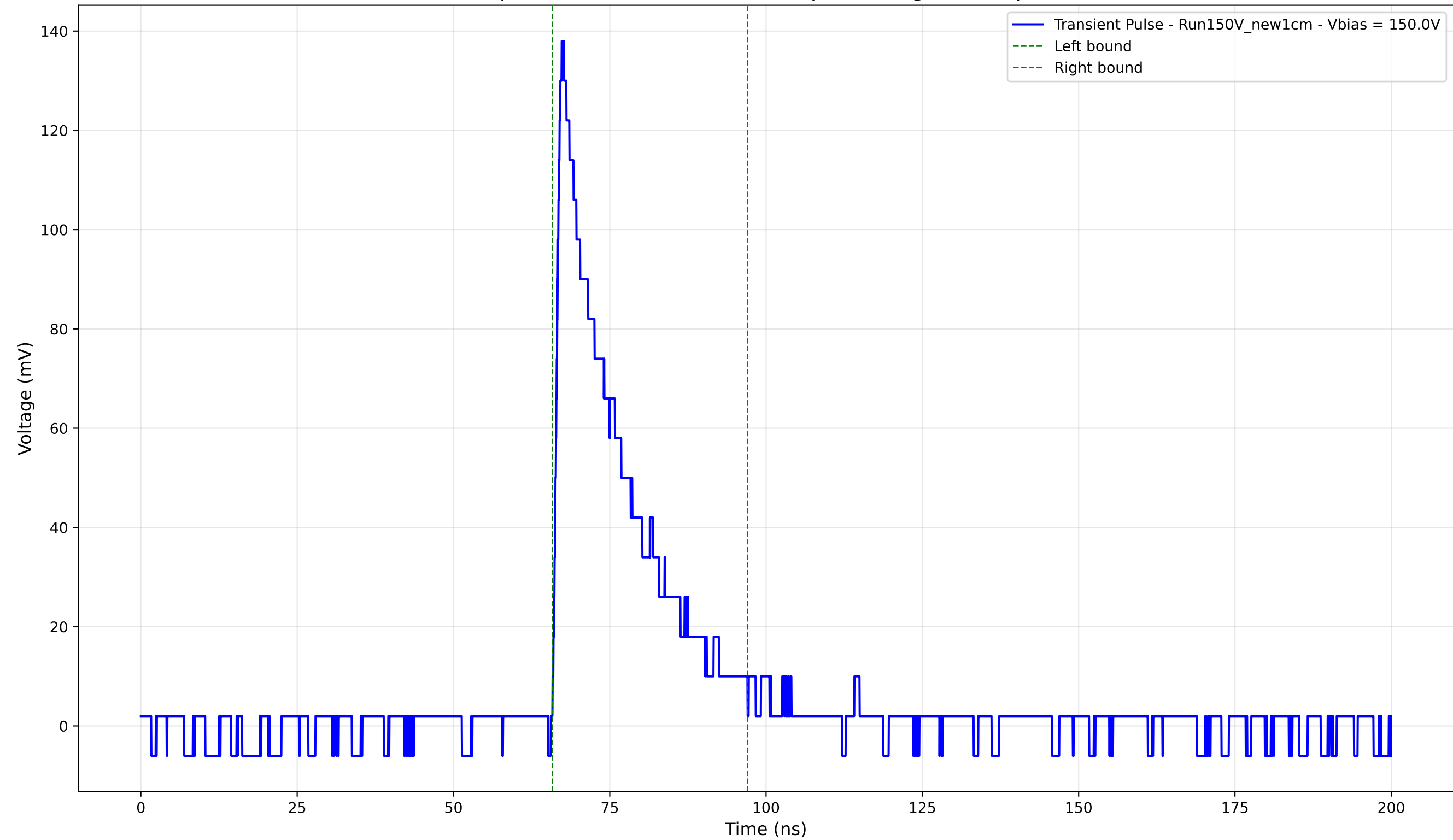
Transient Pulse - Sample: New1cm - Position: 325.0 \mu\text{m} - Charge: 28.51 pC - Rise Time: 1.11 ns
