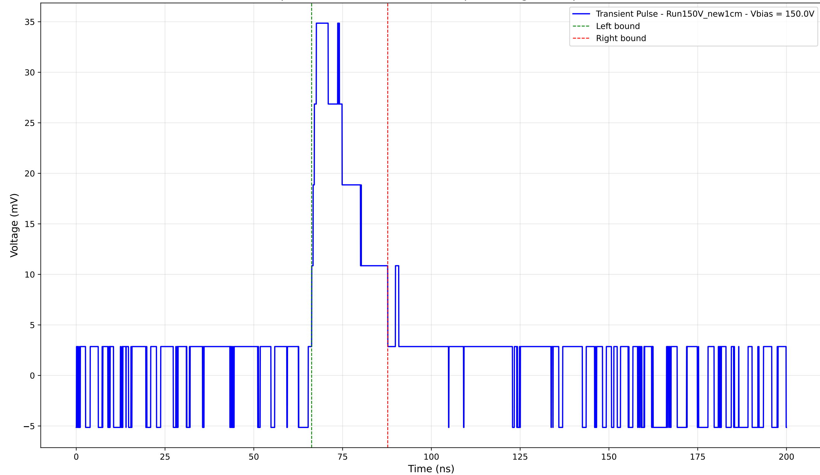
Transient Pulse - Sample: New1cm - Position: 1000.0 \mu\text{m} - Charge: 8.62 pC - Rise Time: 1.32 ns
