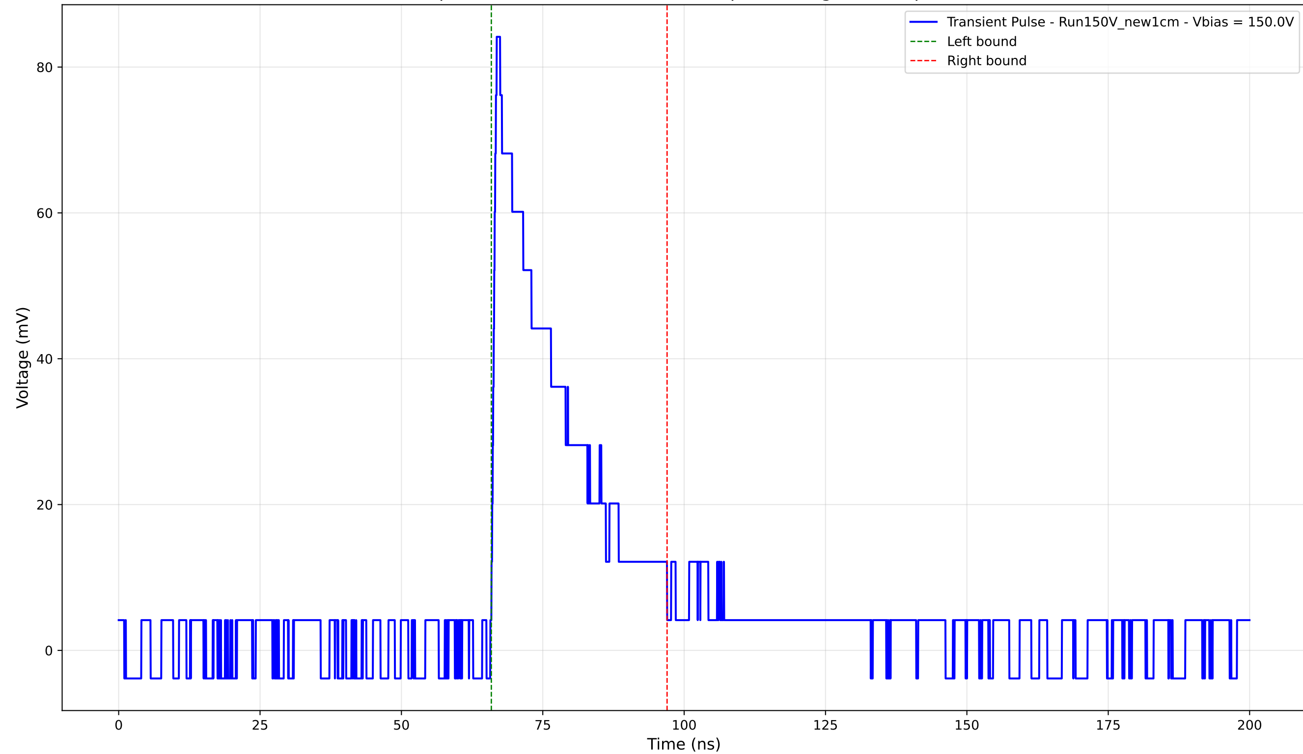
Transient Pulse - Sample: New1cm - Position: 3005.0 \mu\text{m} - Charge: 20.09 pC - Rise Time: 0.79 ns
