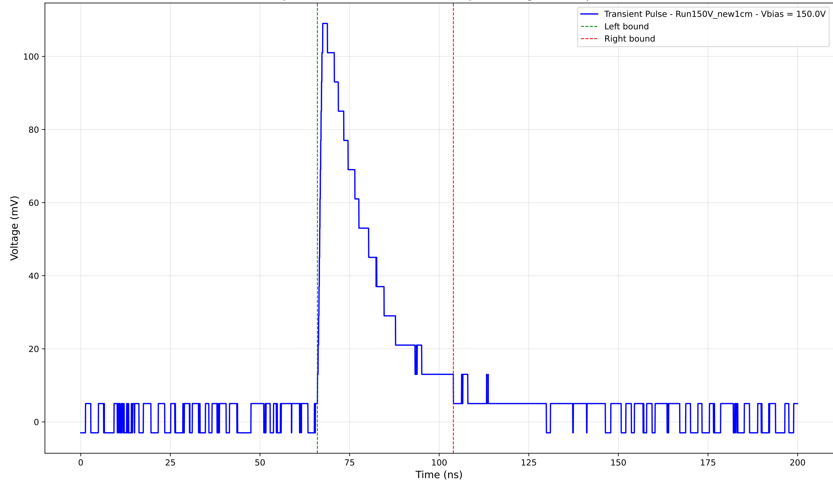
Transient Pulse - Sample: New1cm - Position: 3485.0 \mu\text{m} - Charge: 32.53 pC - Rise Time: 1.25 ns
