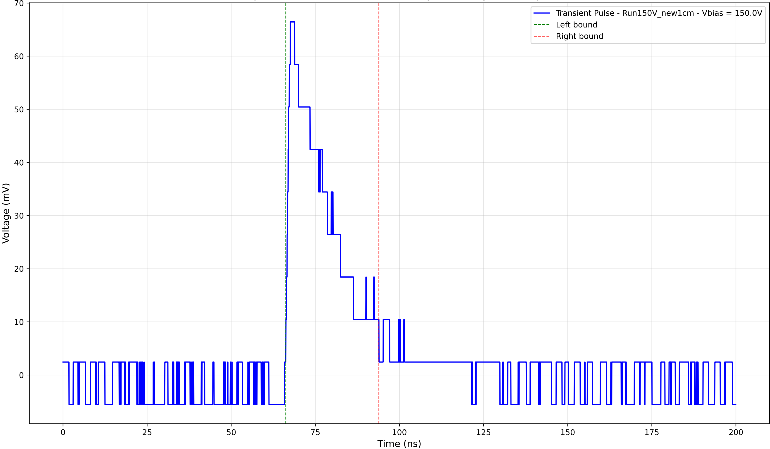
Transient Pulse - Sample: New1cm - Position: 3515.0 \mu\text{m} - Charge: 16.74 pC - Rise Time: 1.33 ns
