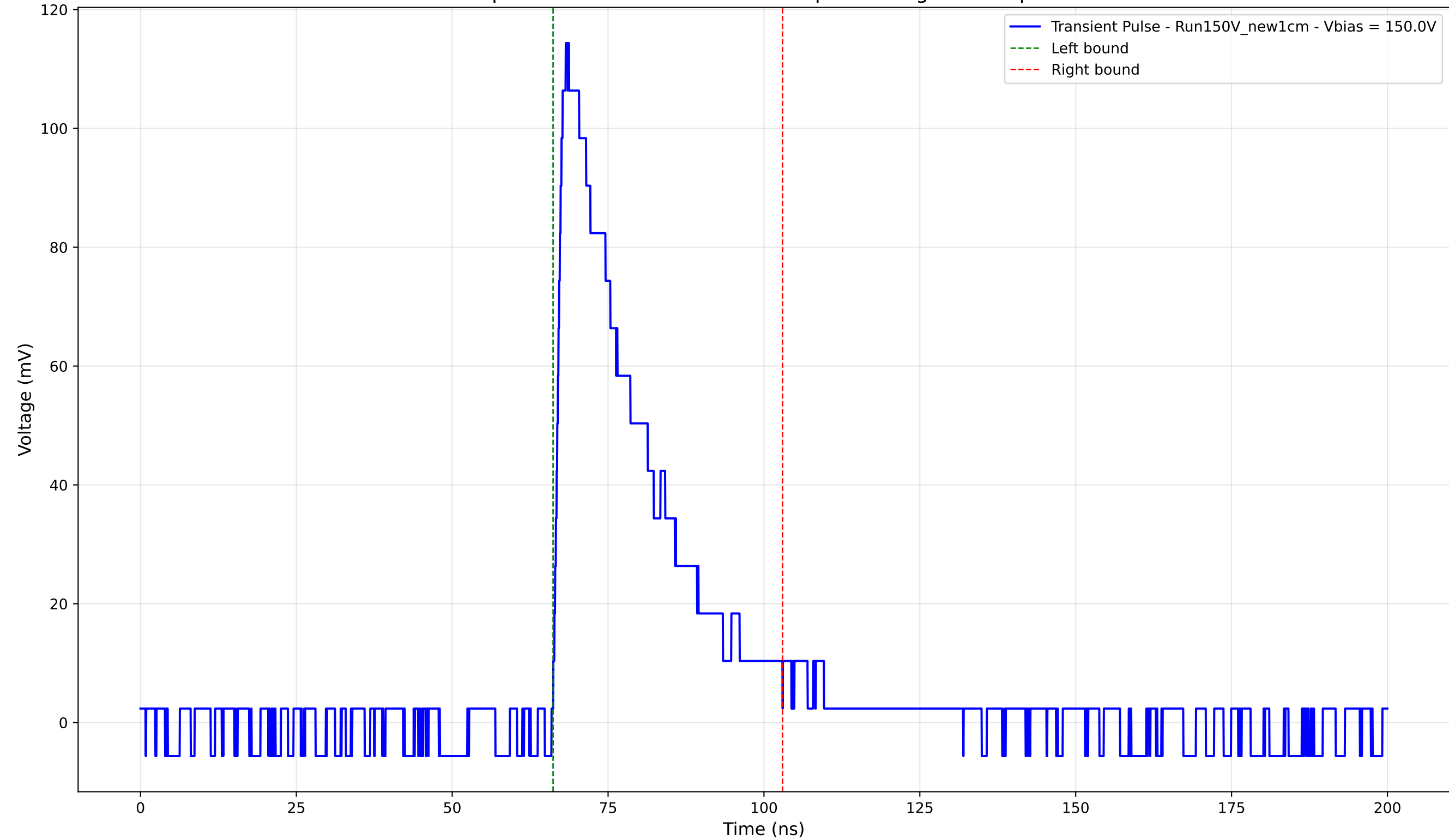
Transient Pulse - Sample: New1cm - Position: 1290.0 \mu\text{m} - Charge: 31.58 pC - Rise Time: 1.34 ns
