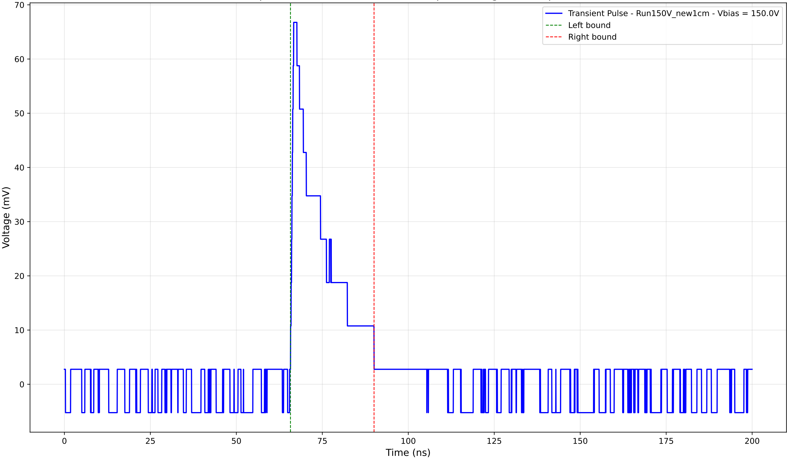
Transient Pulse - Sample: New1cm - Position: 4855.0 \mu\text{m} - Charge: 12.47 pC - Rise Time: 0.91 ns
