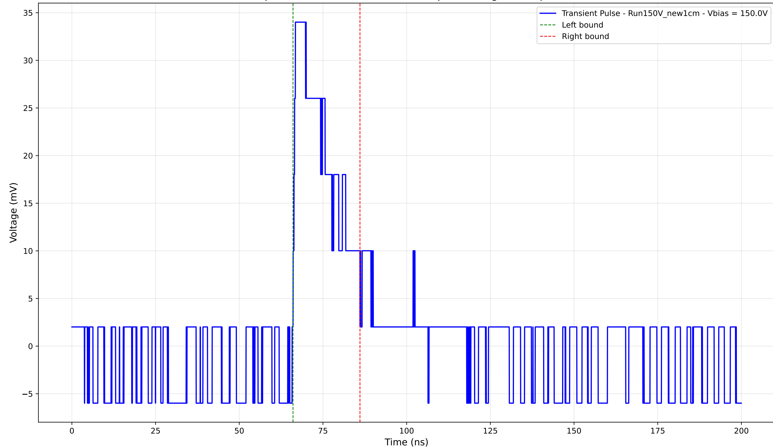
Transient Pulse - Sample: New1cm - Position: 2000.0 \mu\text{m} - Charge: 8.13 pC - Rise Time: 0.70 ns
