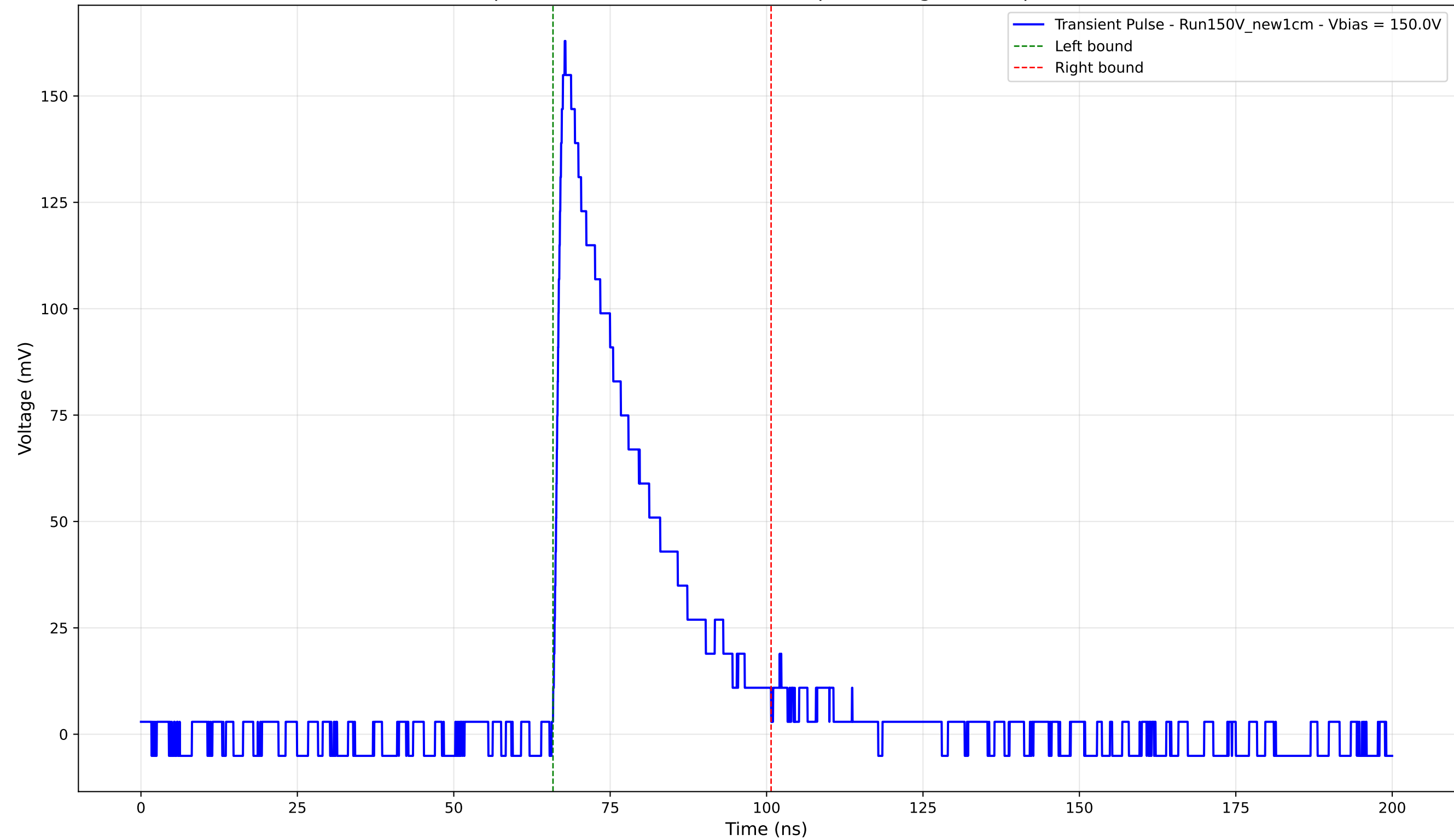
Transient Pulse - Sample: New1cm - Position: 4355.0 \mu\text{m} - Charge: 40.47 pC - Rise Time: 1.27 ns
