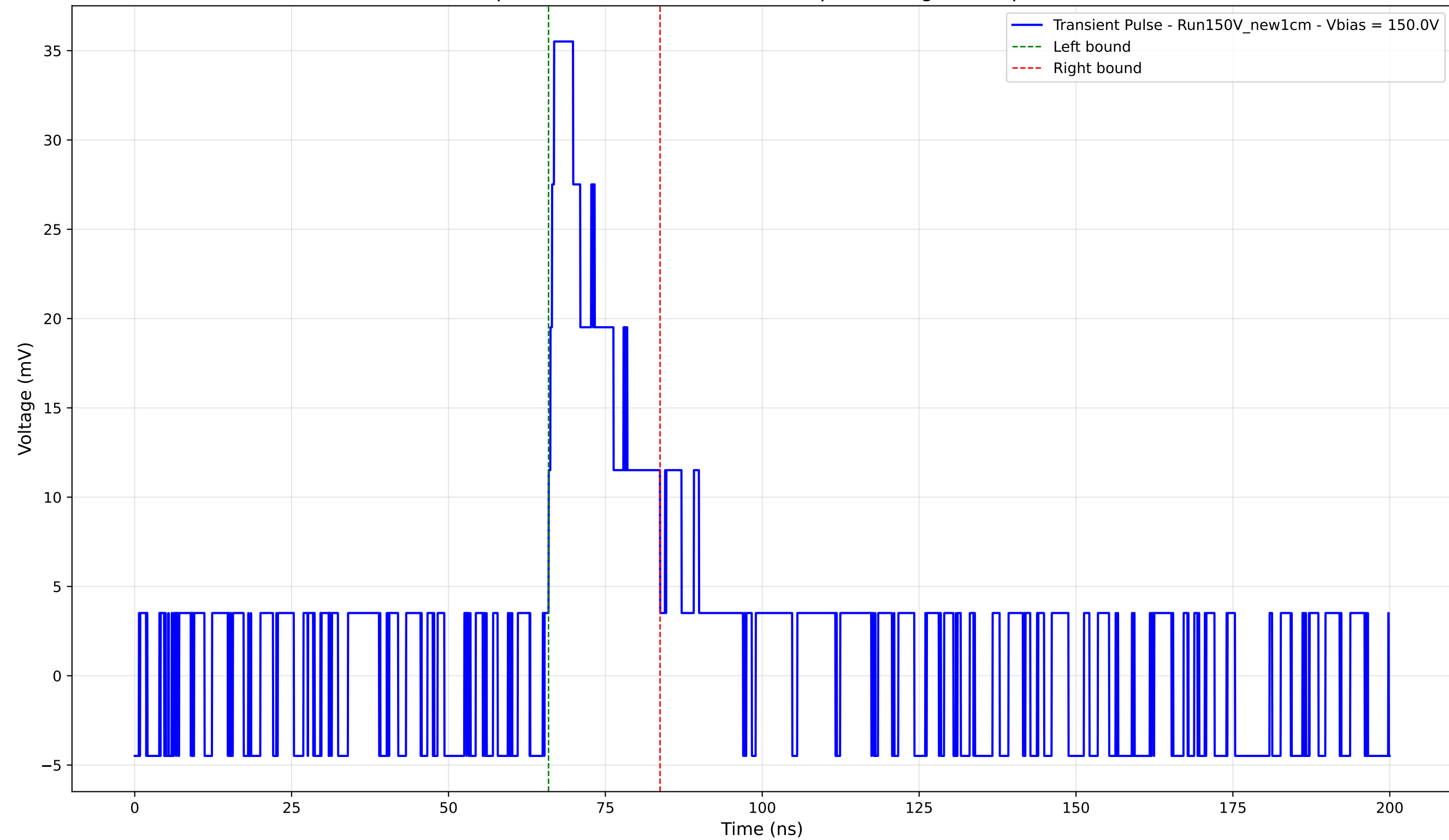
Transient Pulse - Sample: New1cm - Position: 4595.0 \mu\text{m} - Charge: 7.05 pC - Rise Time: 0.88 ns
