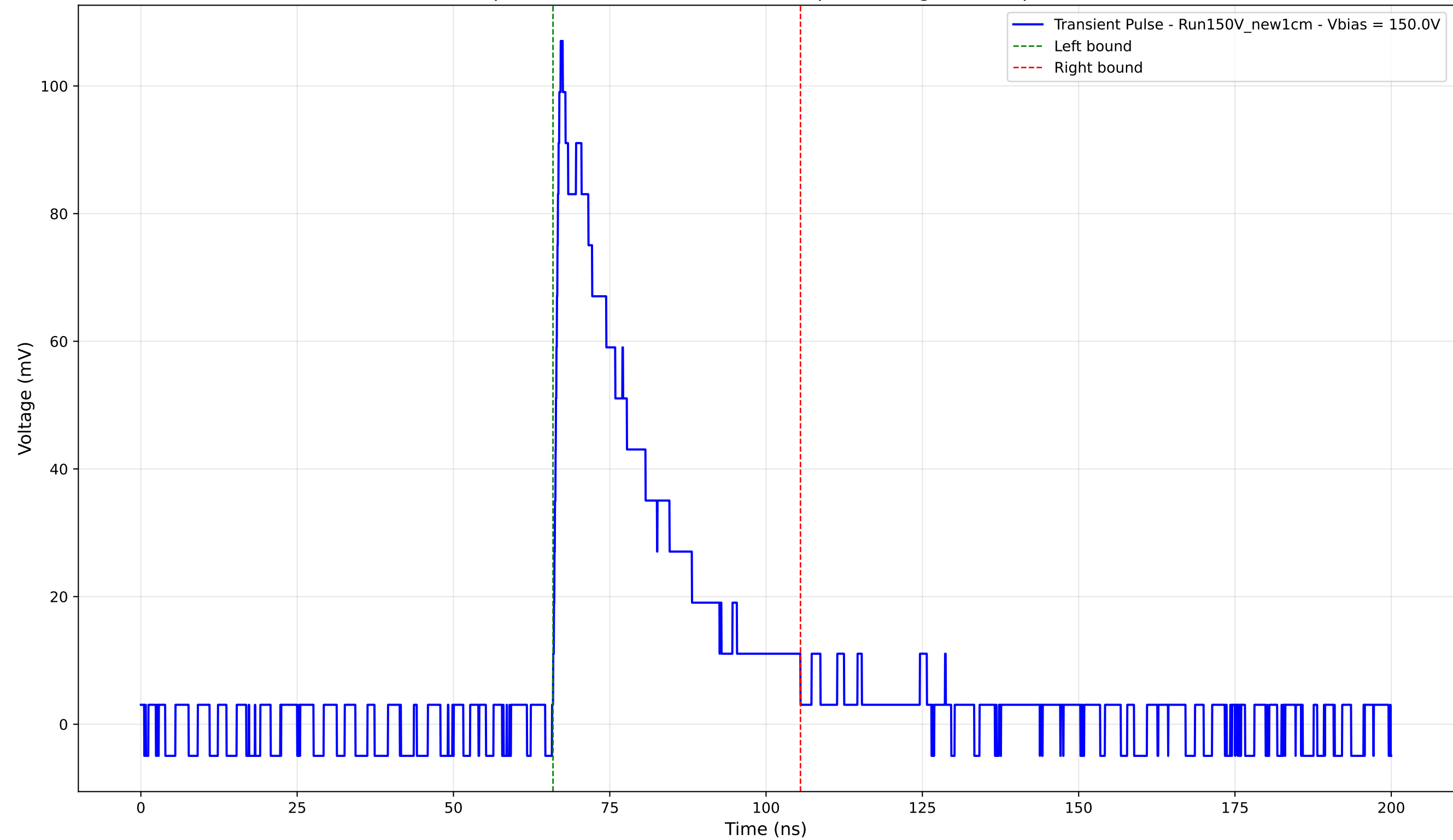
Transient Pulse - Sample: New1cm - Position: 3130.0 \mu\text{m} - Charge: 28.76 pC - Rise Time: 0.98 ns
