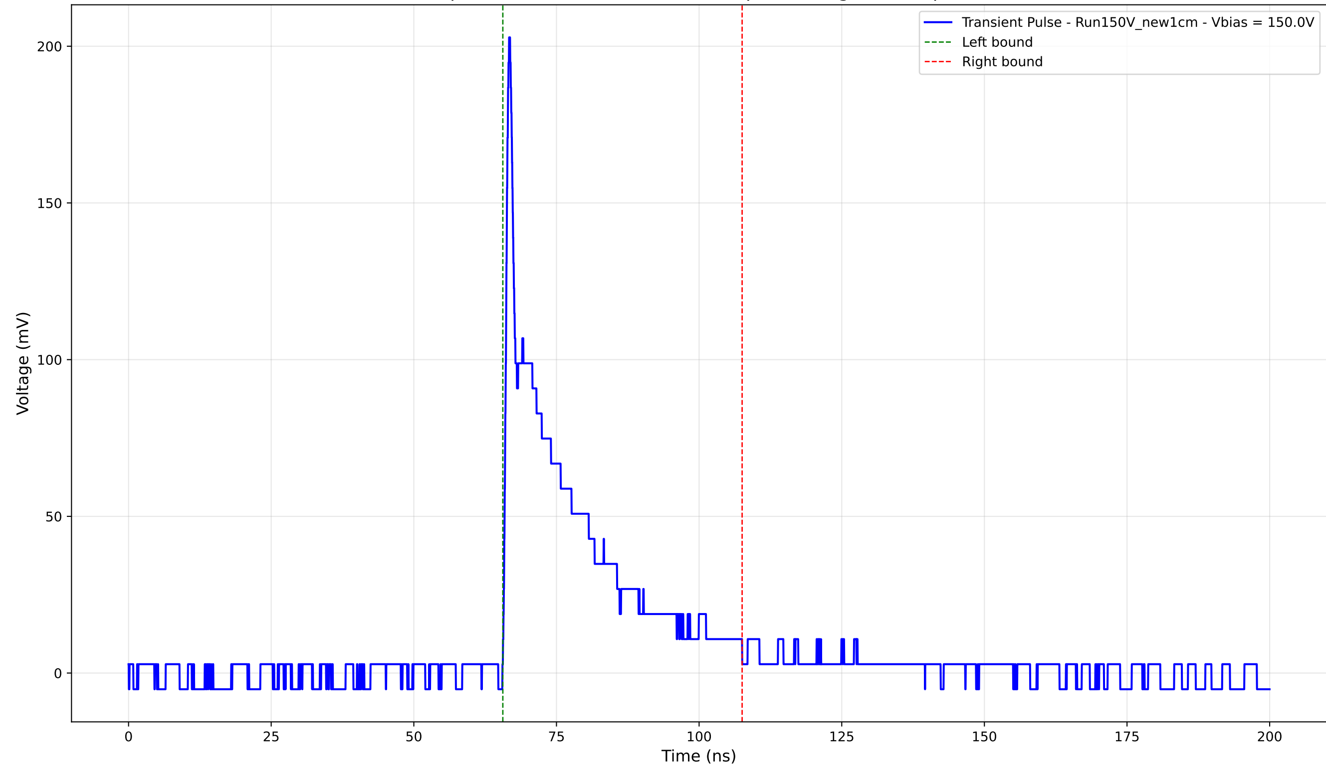
Transient Pulse - Sample: New1cm - Position: 2440.0 \mu\text{m} - Charge: 35.50 pC - Rise Time: 0.78 ns
