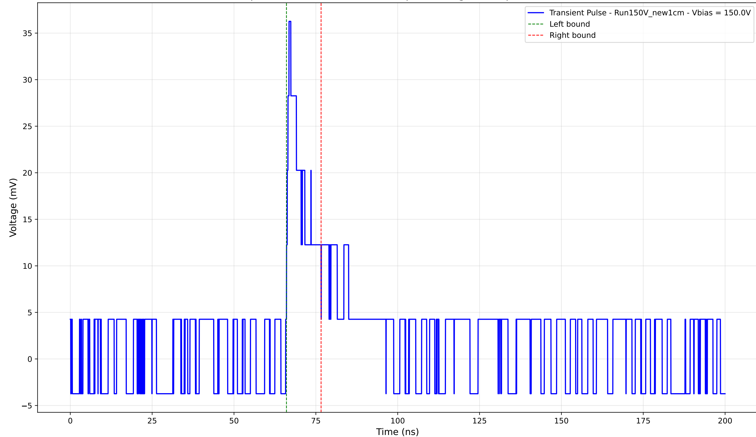
Transient Pulse - Sample: New1cm - Position: 55.0 \mu\text{m} - Charge: 3.94 pC - Rise Time: 0.00 ns (N/A)
