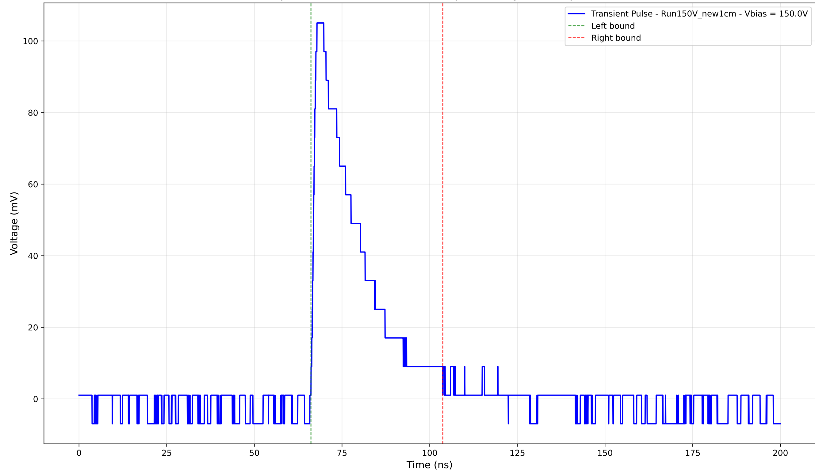
Transient Pulse - Sample: New1cm - Position: 930.0 \mu\text{m} - Charge: 28.44 pC - Rise Time: 1.18 ns
