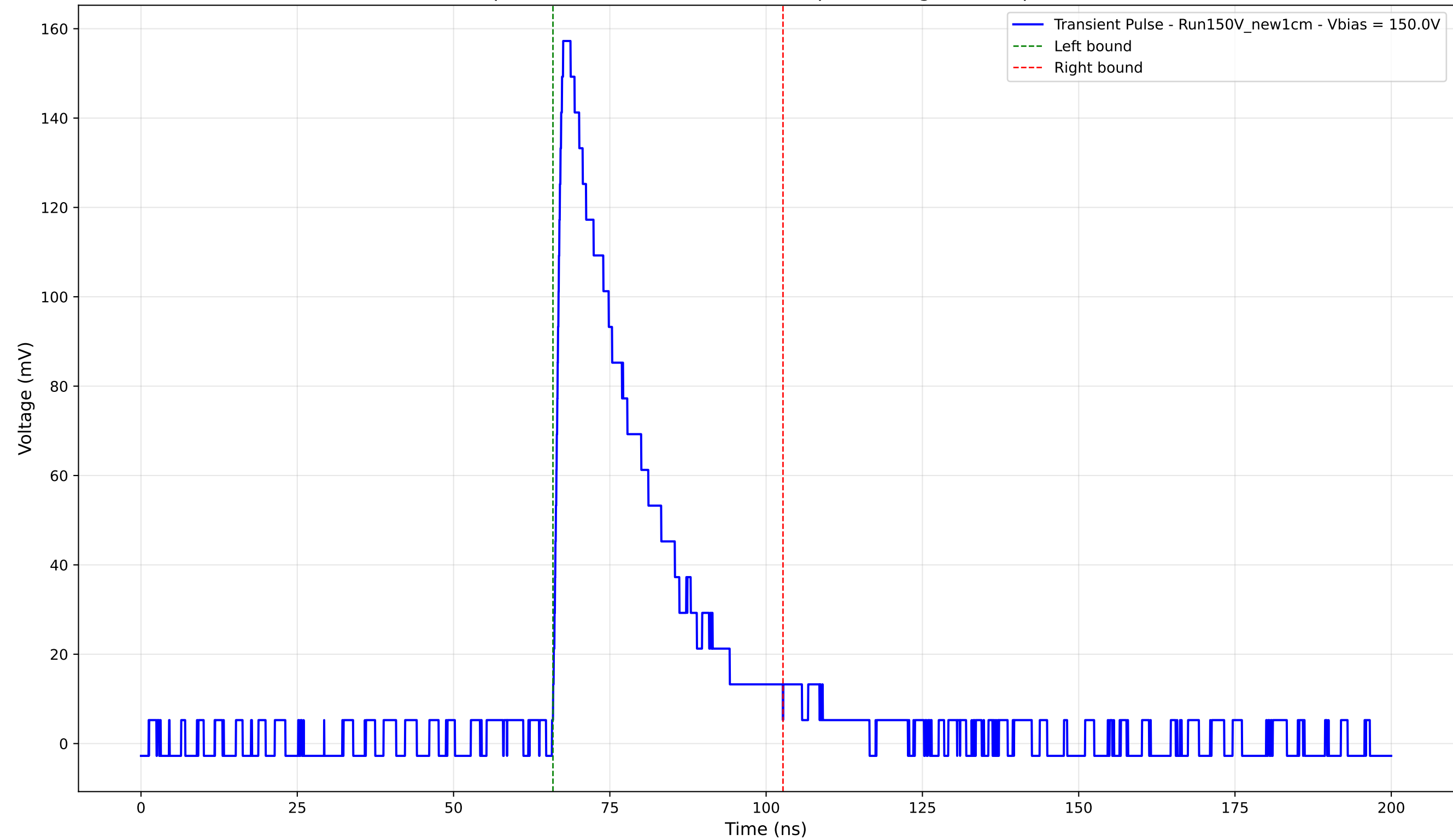
Transient Pulse - Sample: New1cm - Position: 4295.0 \mu\text{m} - Charge: 42.06 pC - Rise Time: 1.33 ns
