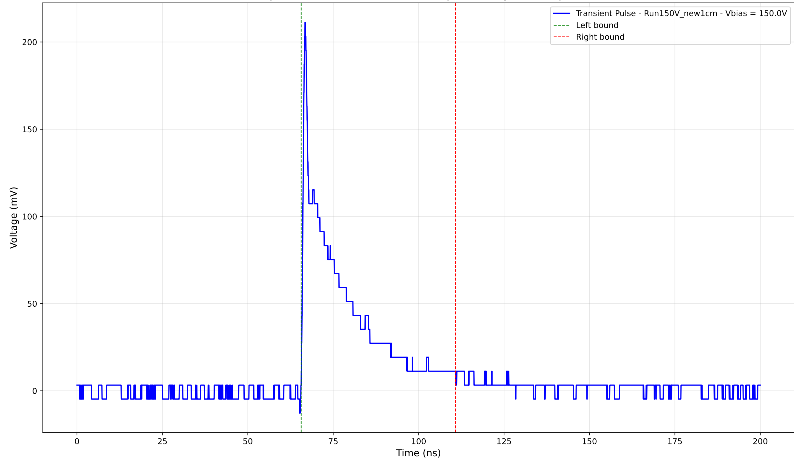
Transient Pulse - Sample: New1cm - Position: 2700.0 \mu\text{m} - Charge: 38.84 pC - Rise Time: 0.82 ns
