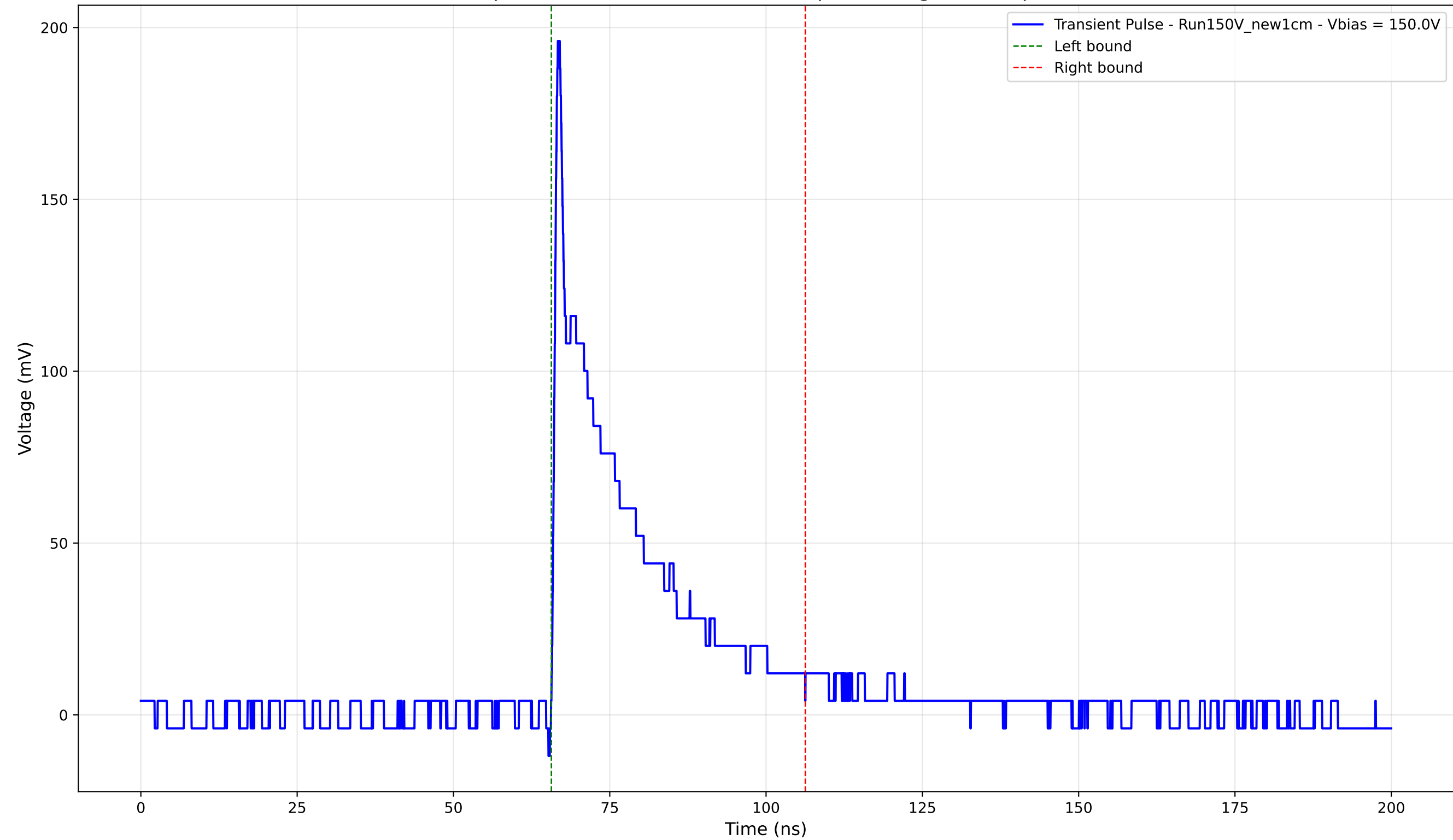
Transient Pulse - Sample: New1cm - Position: 2735.0 \mu\text{m} - Charge: 38.81 pC - Rise Time: 0.78 ns
