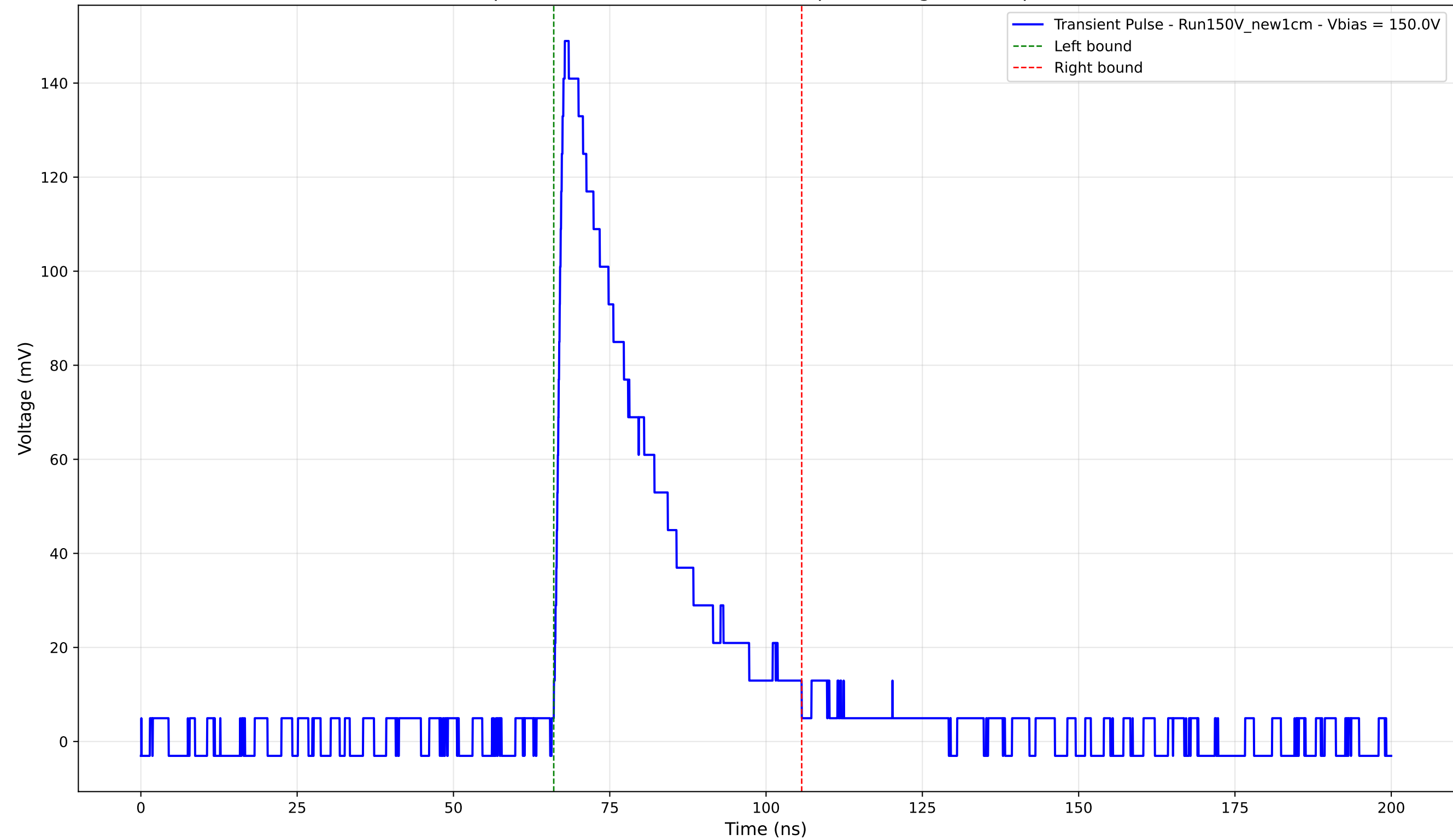
Transient Pulse - Sample: New1cm - Position: 3895.0 \mu\text{m} - Charge: 43.08 pC - Rise Time: 1.38 ns
