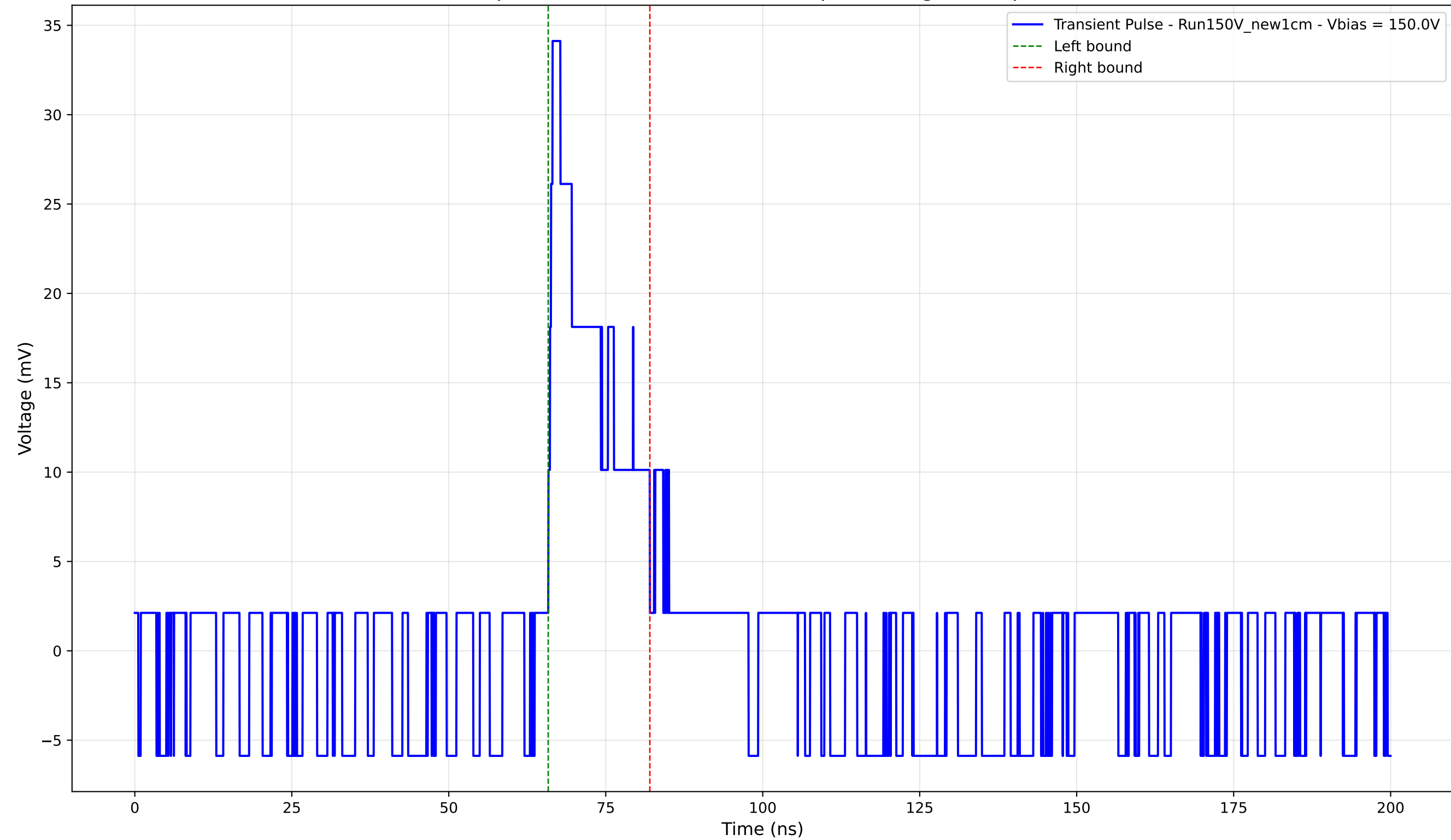
Transient Pulse - Sample: New1cm - Position: 4875.0 \mu\text{m} - Charge: 5.48 pC - Rise Time: 0.68 ns
