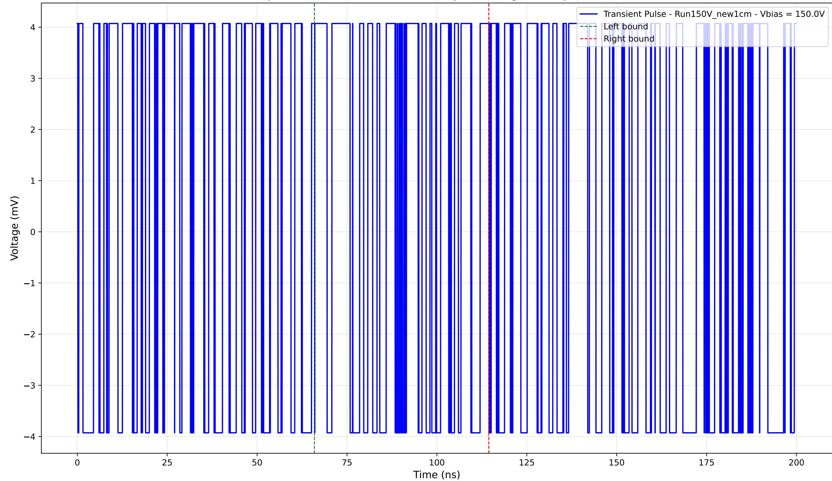
Transient Pulse - Sample: New1cm - Position: 4995.0 \mu\text{m} - Charge: 0.91 pC - Rise Time: 0.00 ns (N/A)
