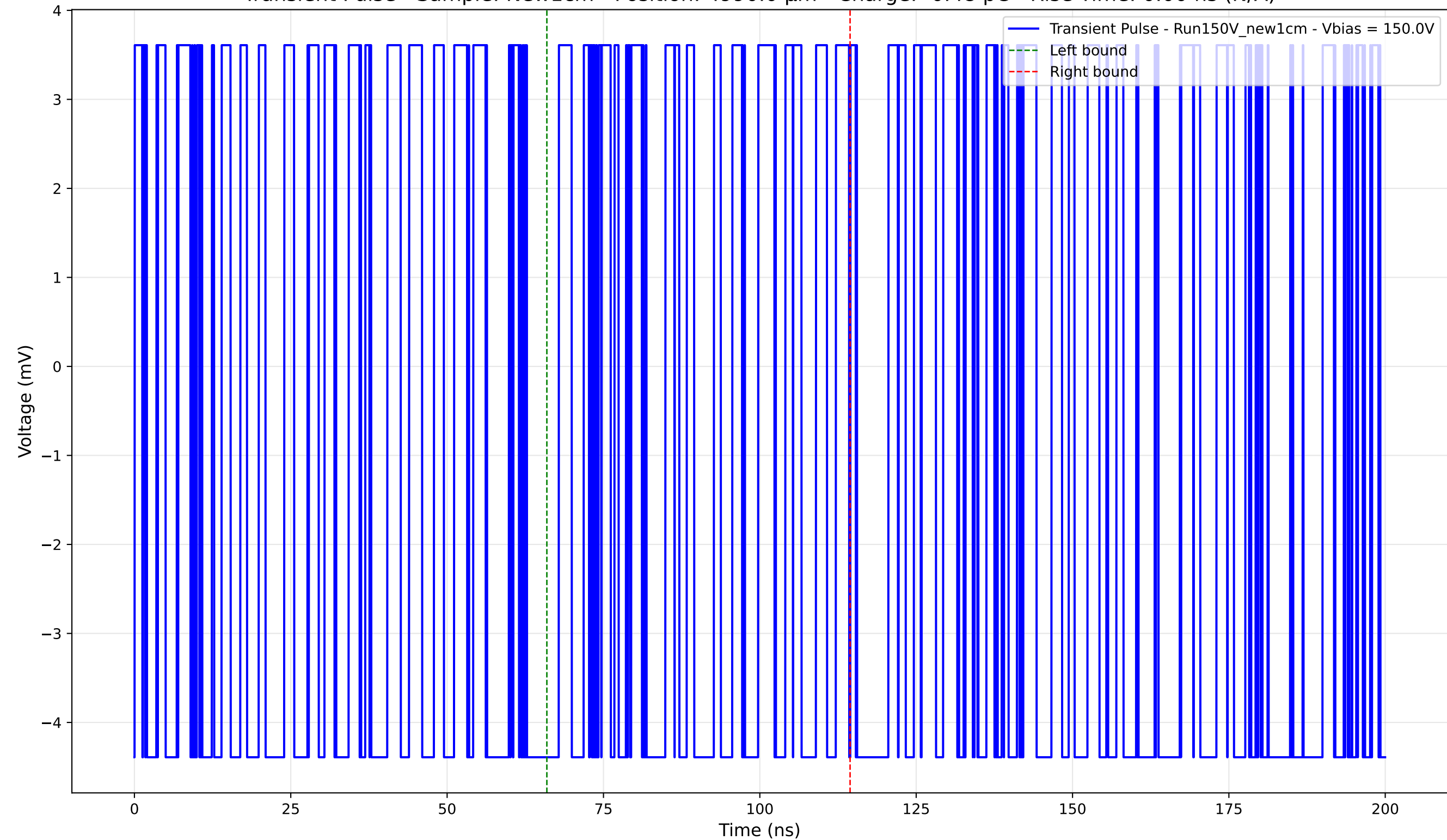
Transient Pulse - Sample: New1cm - Position: 4990.0 \mu\text{m} - Charge: -0.48 pC - Rise Time: 0.00 ns (N/A)
