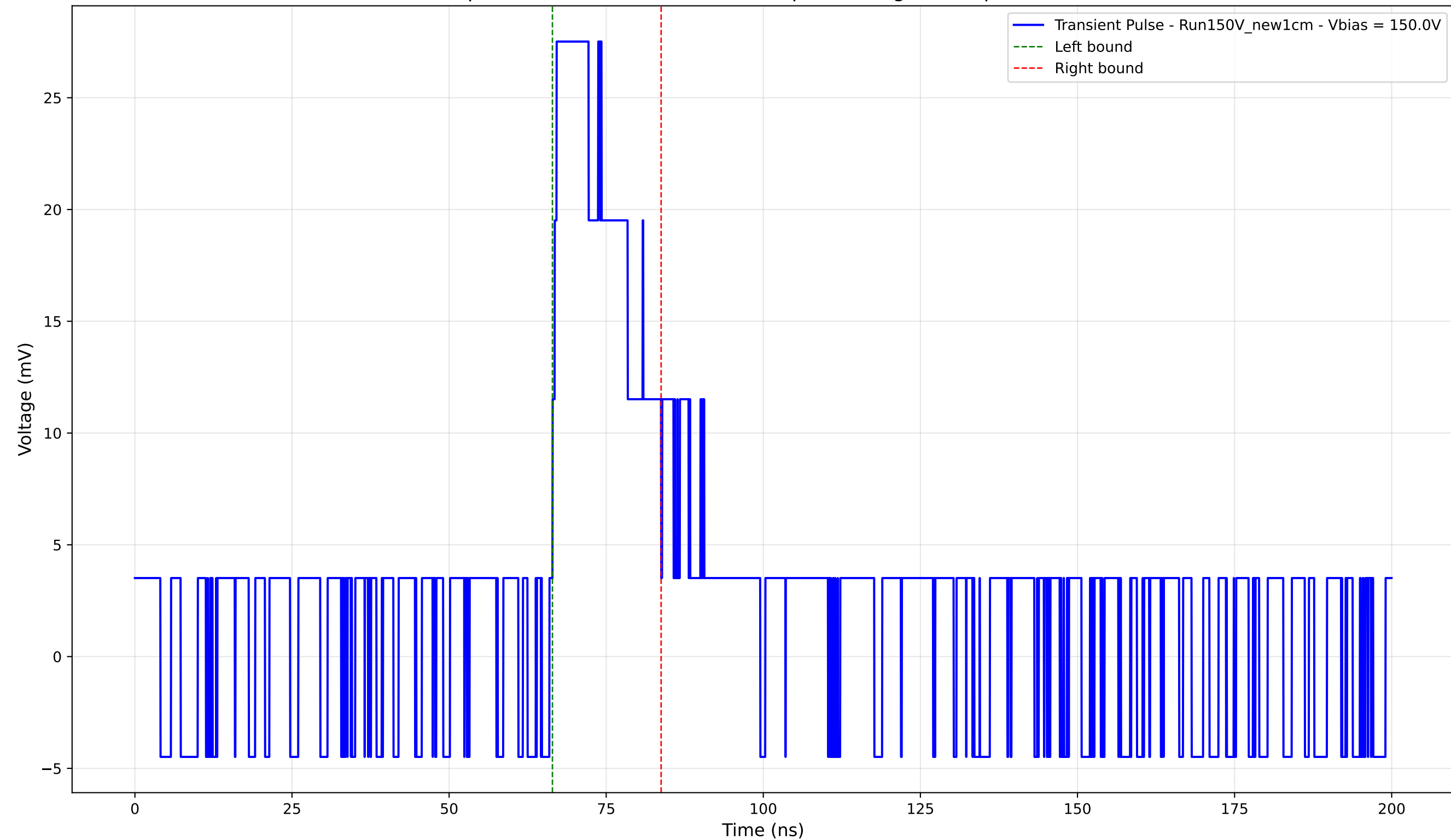
Transient Pulse - Sample: New1cm - Position: 1510.0 \mu\text{m} - Charge: 6.74 pC - Rise Time: 0.00 ns (N/A)
