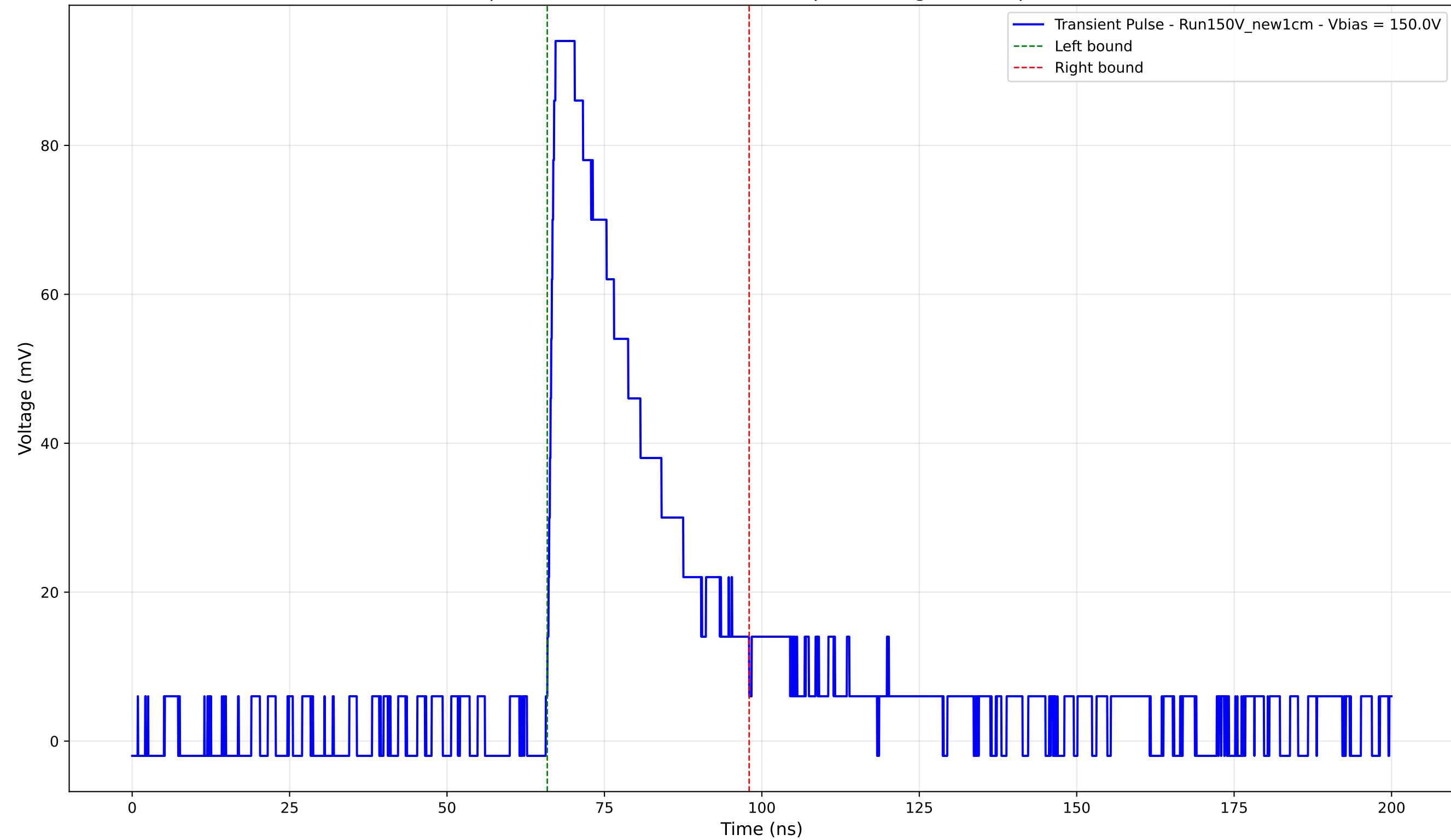
Transient Pulse - Sample: New1cm - Position: 1845.0 \mu\text{m} - Charge: 28.92 pC - Rise Time: 1.07 ns
