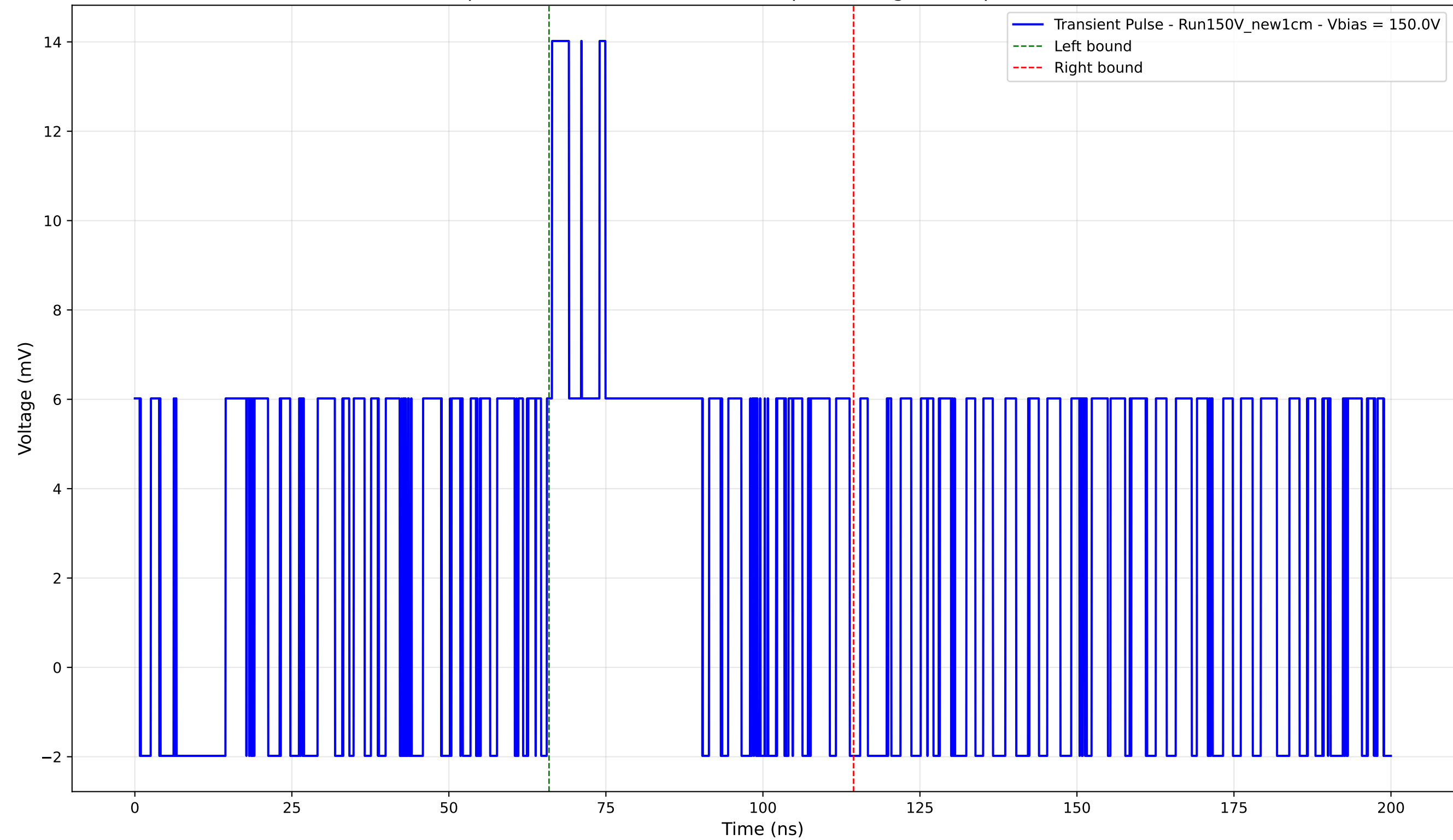
Transient Pulse - Sample: New1cm - Position: 4900.0 \mu\text{m} - Charge: 4.81 pC - Rise Time: 0.00 ns (N/A)
