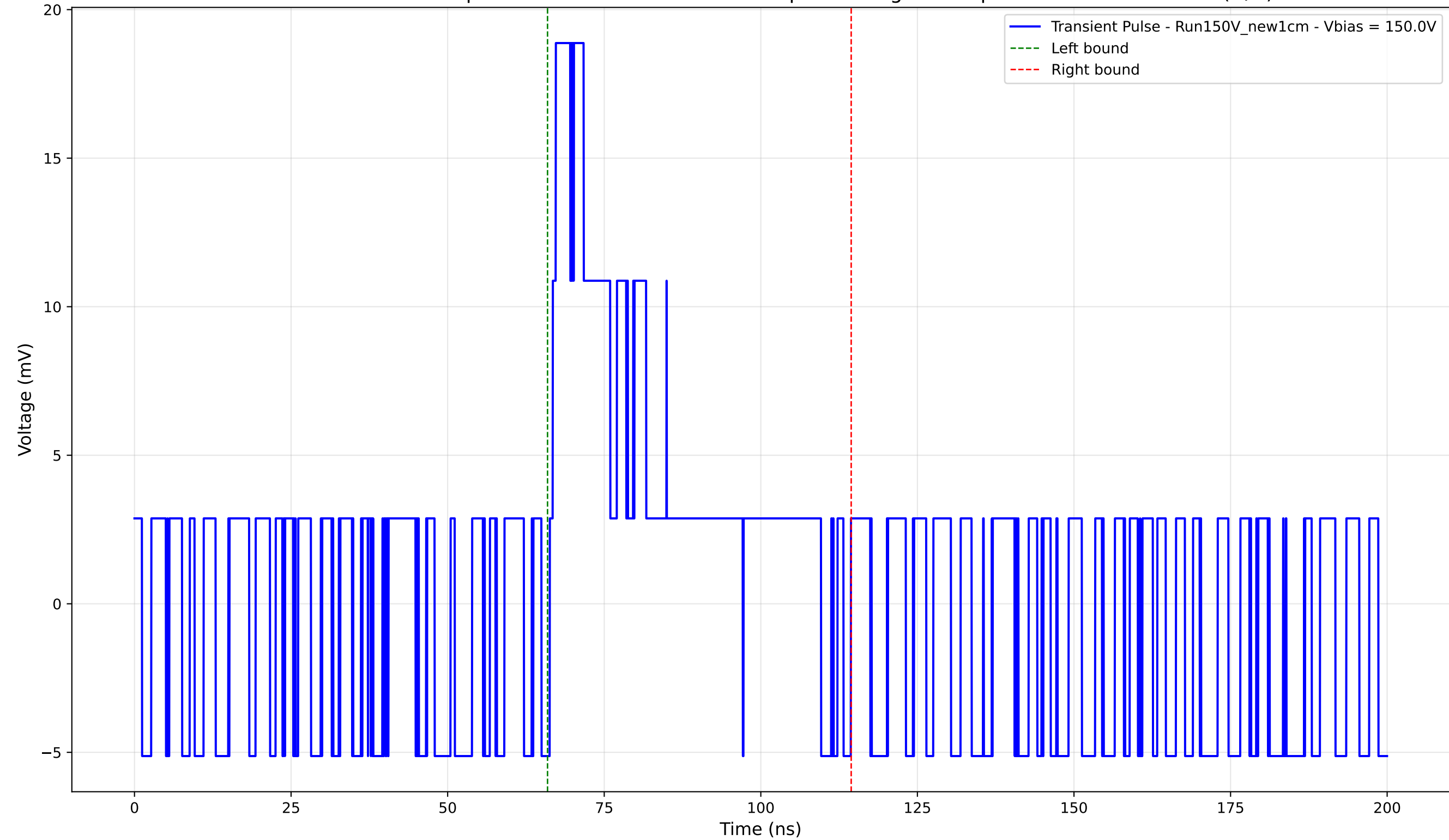
Transient Pulse - Sample: New1cm - Position: 4070.0 \mu\text{m} - Charge: 4.86 pC - Rise Time: 0.00 ns (N/A)
