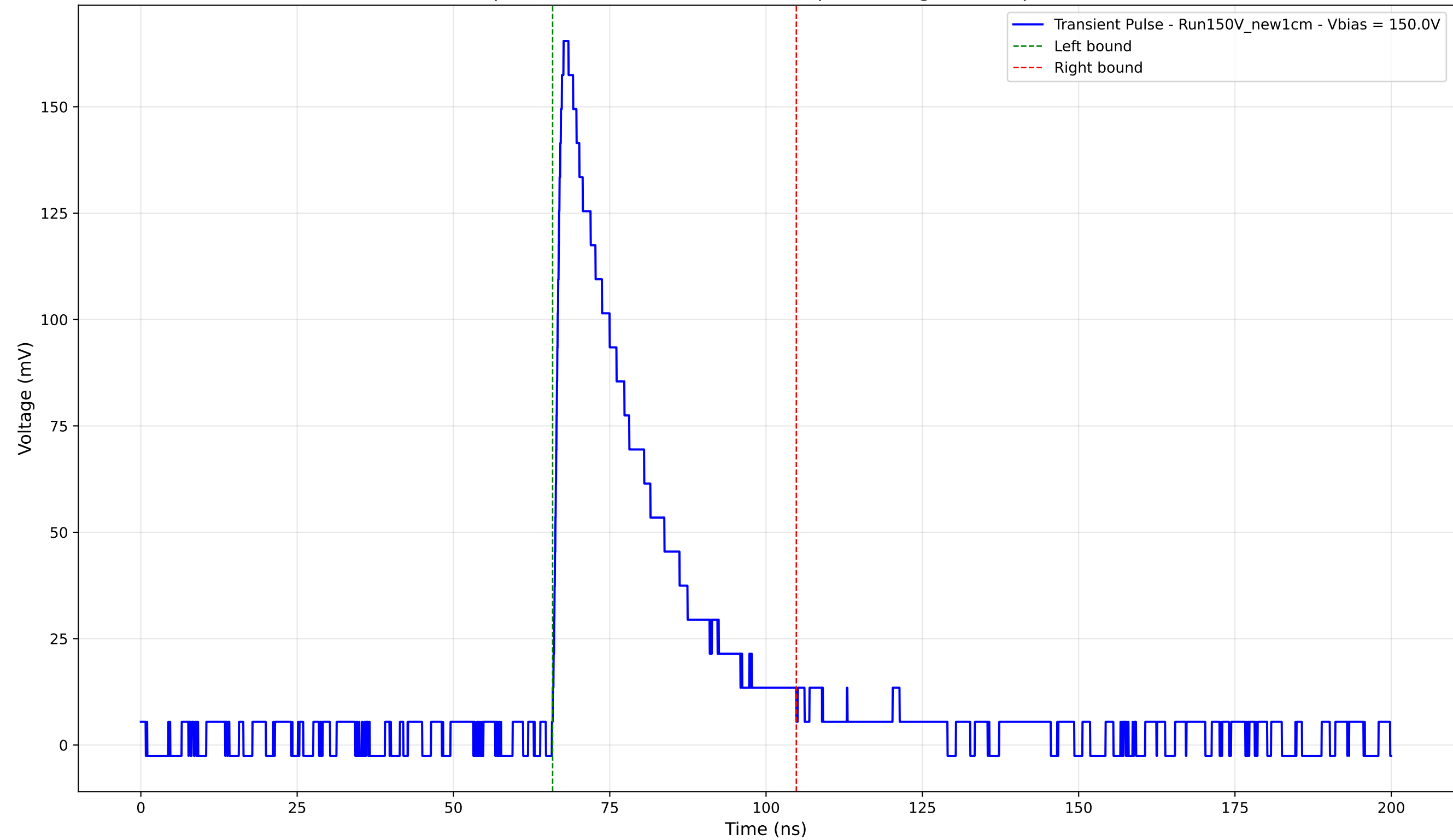
Transient Pulse - Sample: New1cm - Position: 4350.0 \mu\text{m} - Charge: 44.78 pC - Rise Time: 1.19 ns
