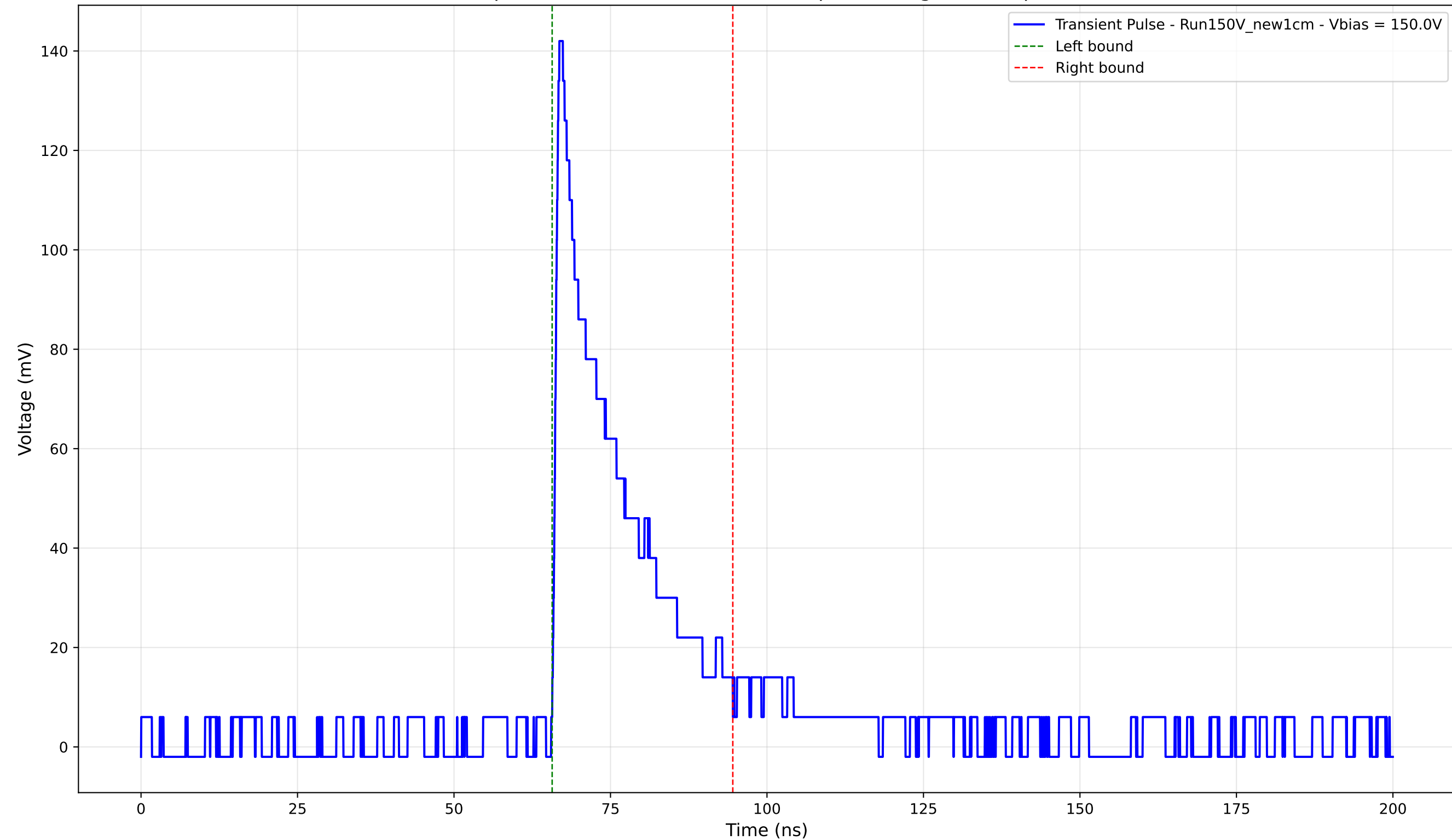
Transient Pulse - Sample: New1cm - Position: 4800.0 \mu\text{m} - Charge: 28.75 pC - Rise Time: 0.90 ns
