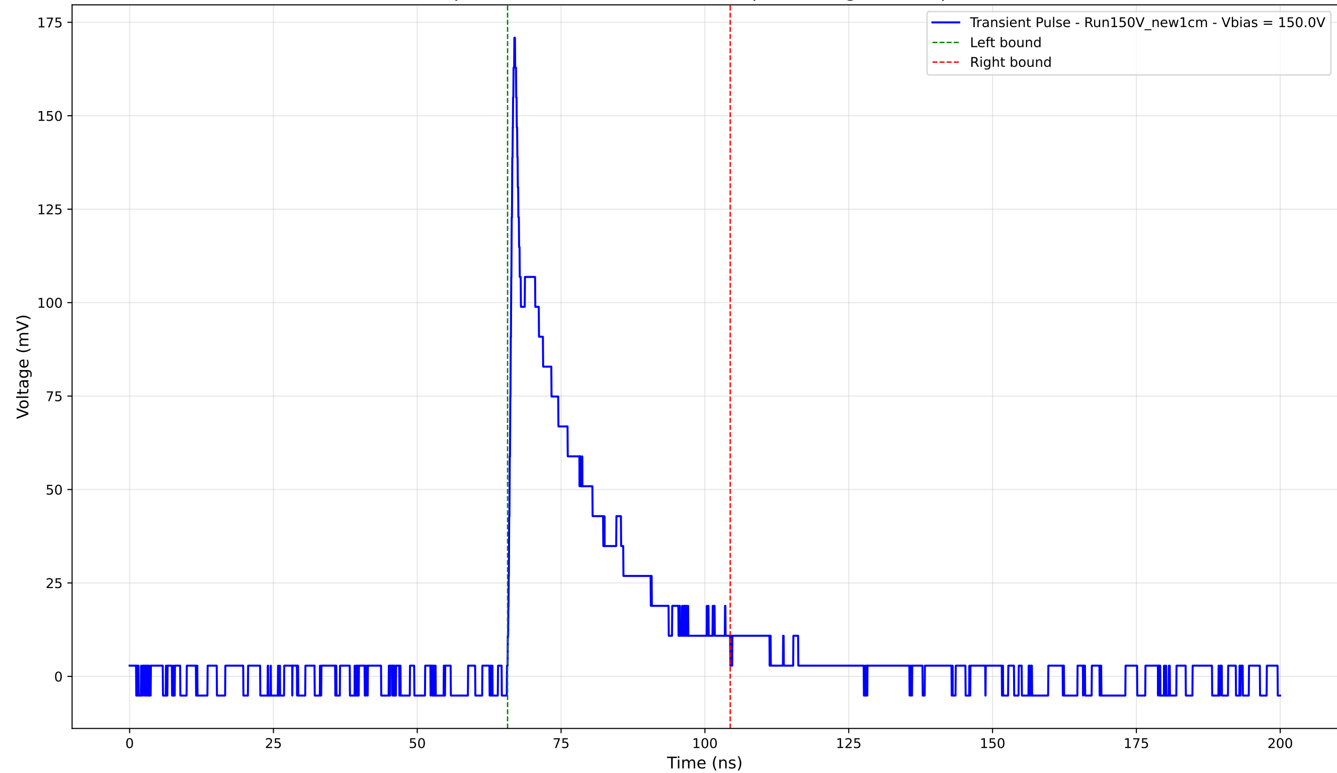
Transient Pulse - Sample: New1cm - Position: 2265.0 \mu\text{m} - Charge: 34.79 pC - Rise Time: 0.82 ns
