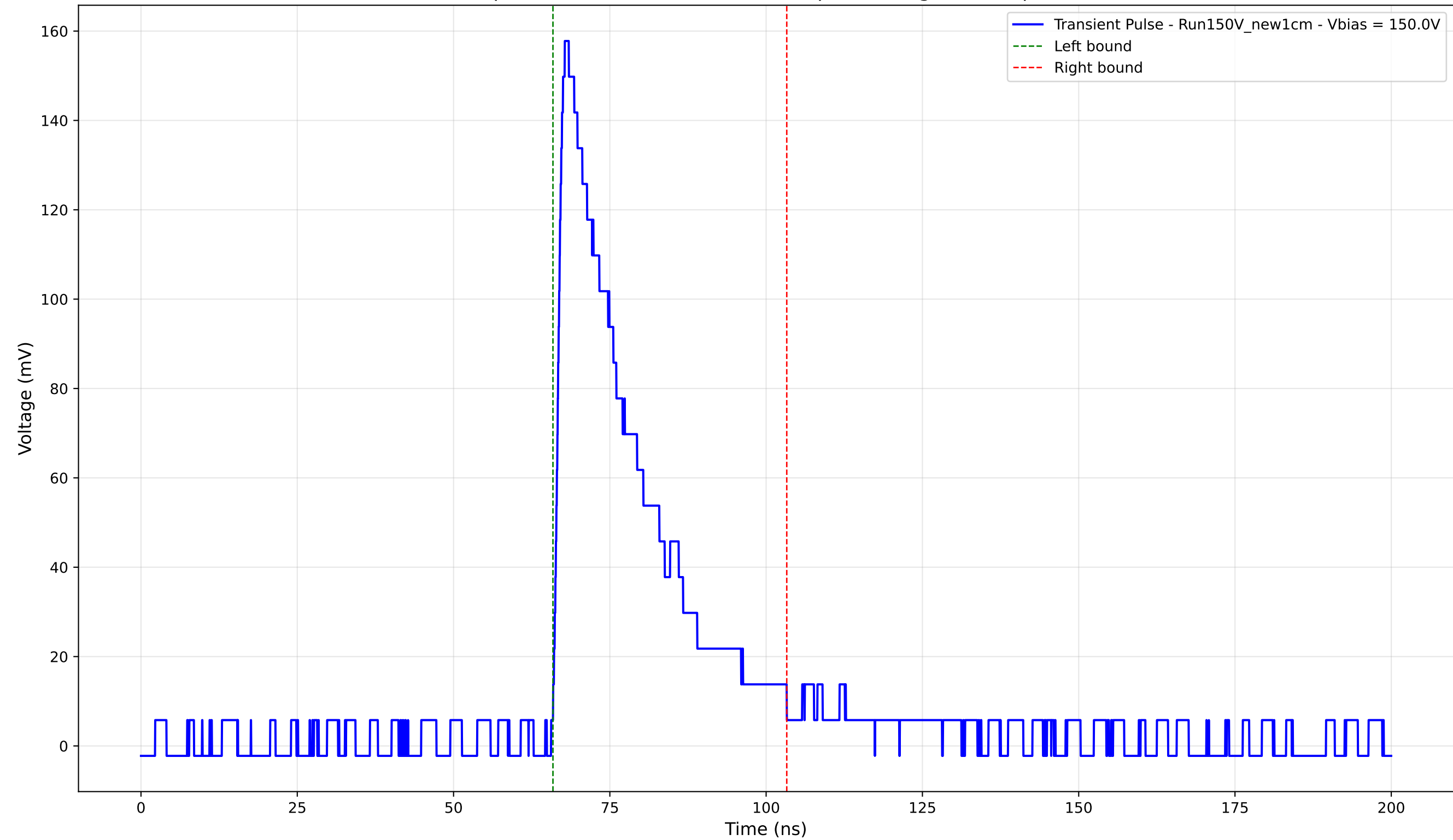
Transient Pulse - Sample: New1cm - Position: 4255.0 \mu\text{m} - Charge: 41.63 pC - Rise Time: 1.46 ns
