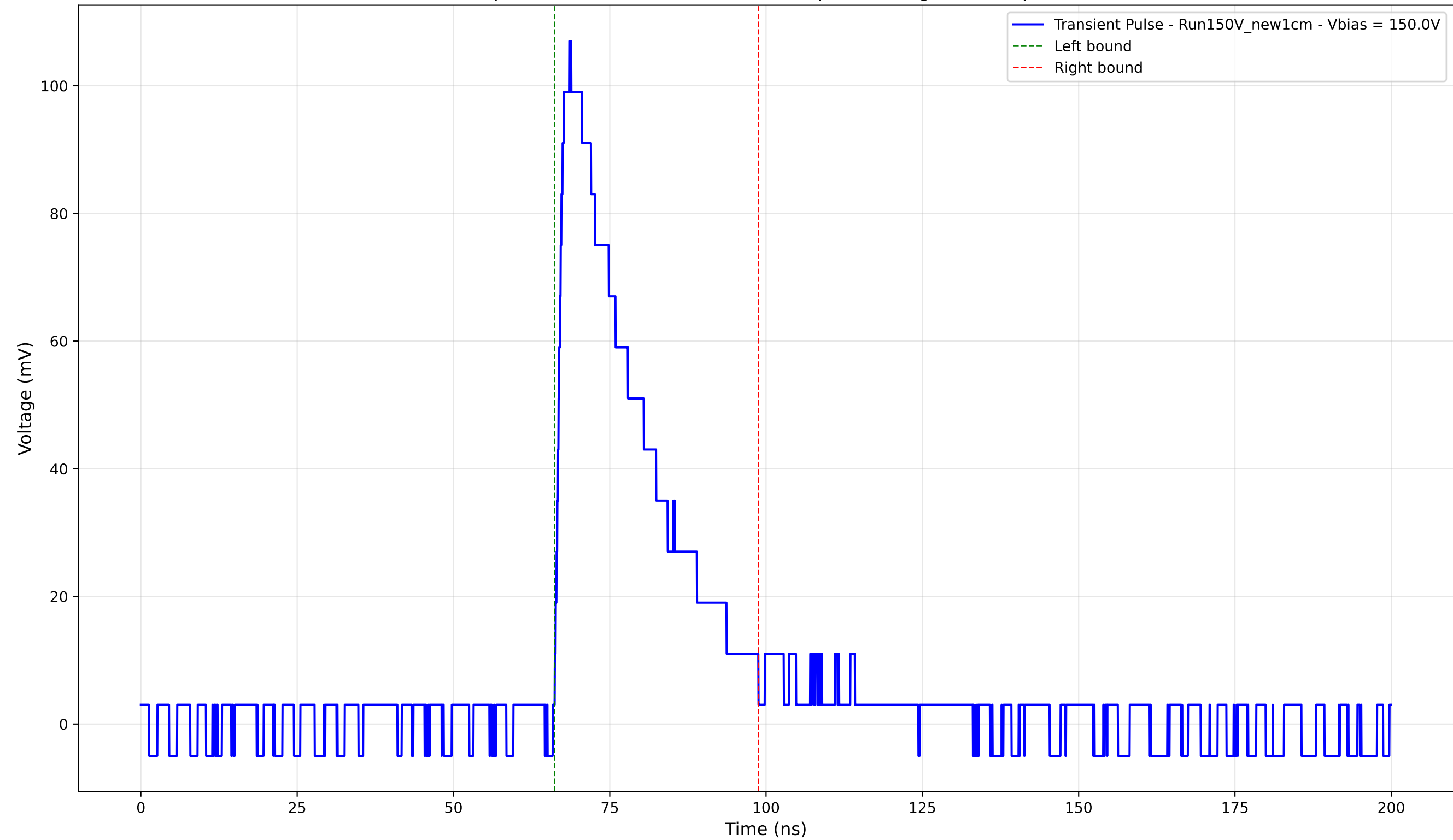
Transient Pulse - Sample: New1cm - Position: 1445.0 \mu\text{m} - Charge: 29.18 pC - Rise Time: 1.44 ns
