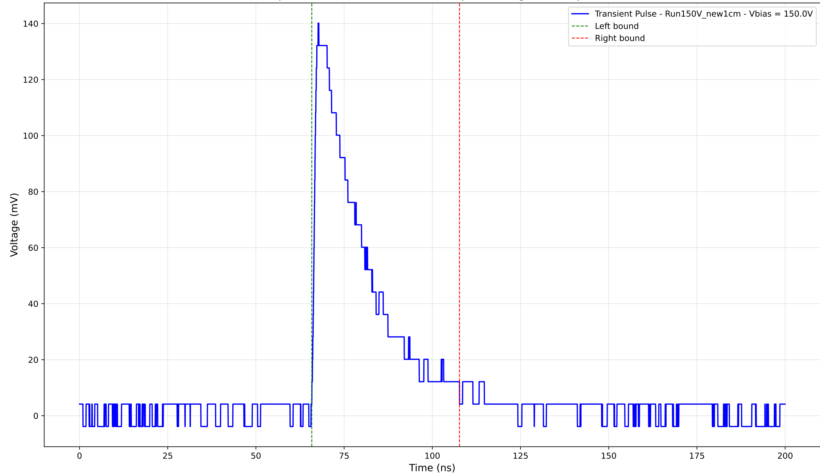
Transient Pulse - Sample: New1cm - Position: 3330.0 \mu\text{m} - Charge: 41.65 pC - Rise Time: 1.26 ns
