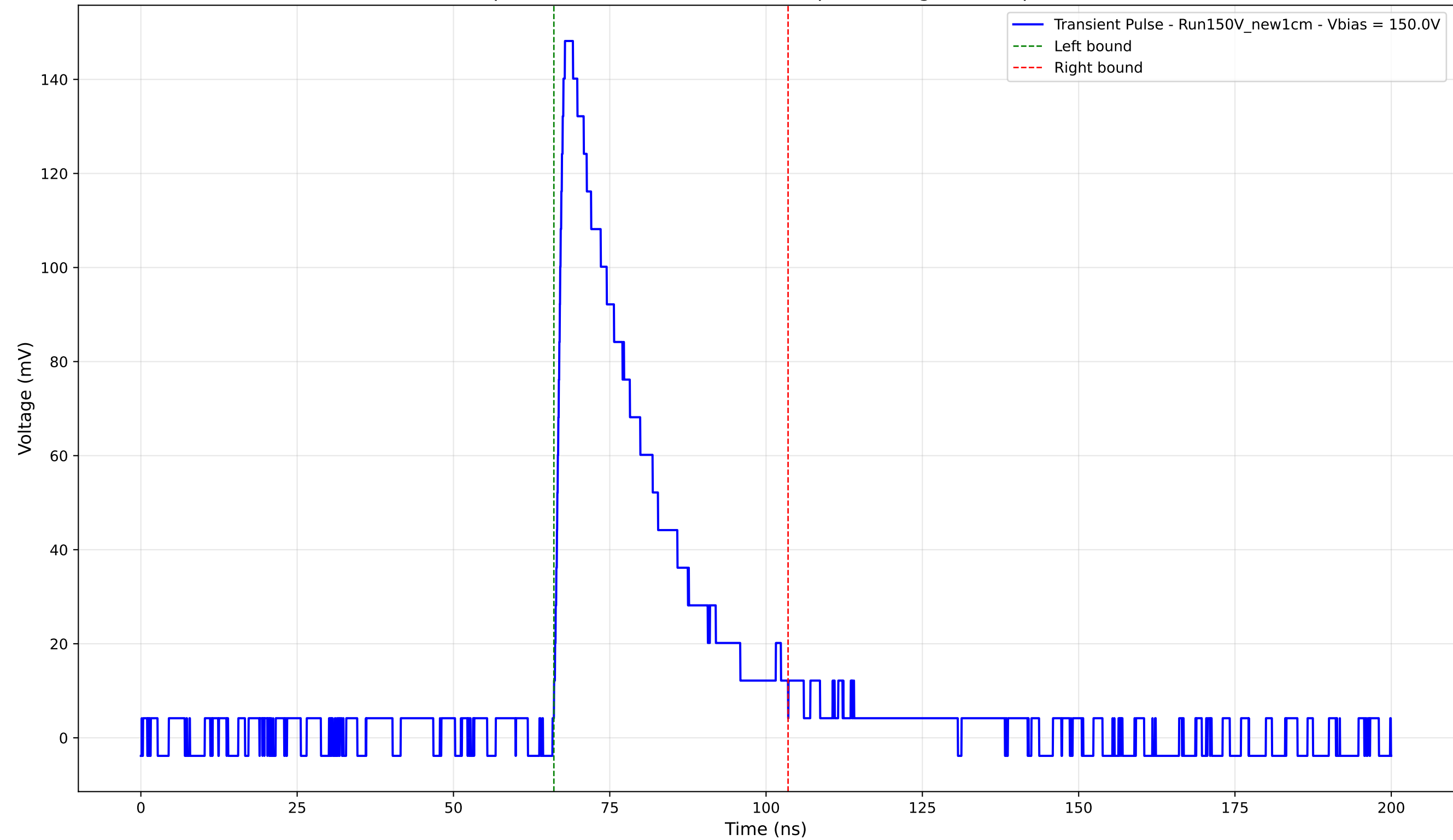
Transient Pulse - Sample: New1cm - Position: 3910.0 \mu\text{m} - Charge: 41.20 pC - Rise Time: 1.35 ns
