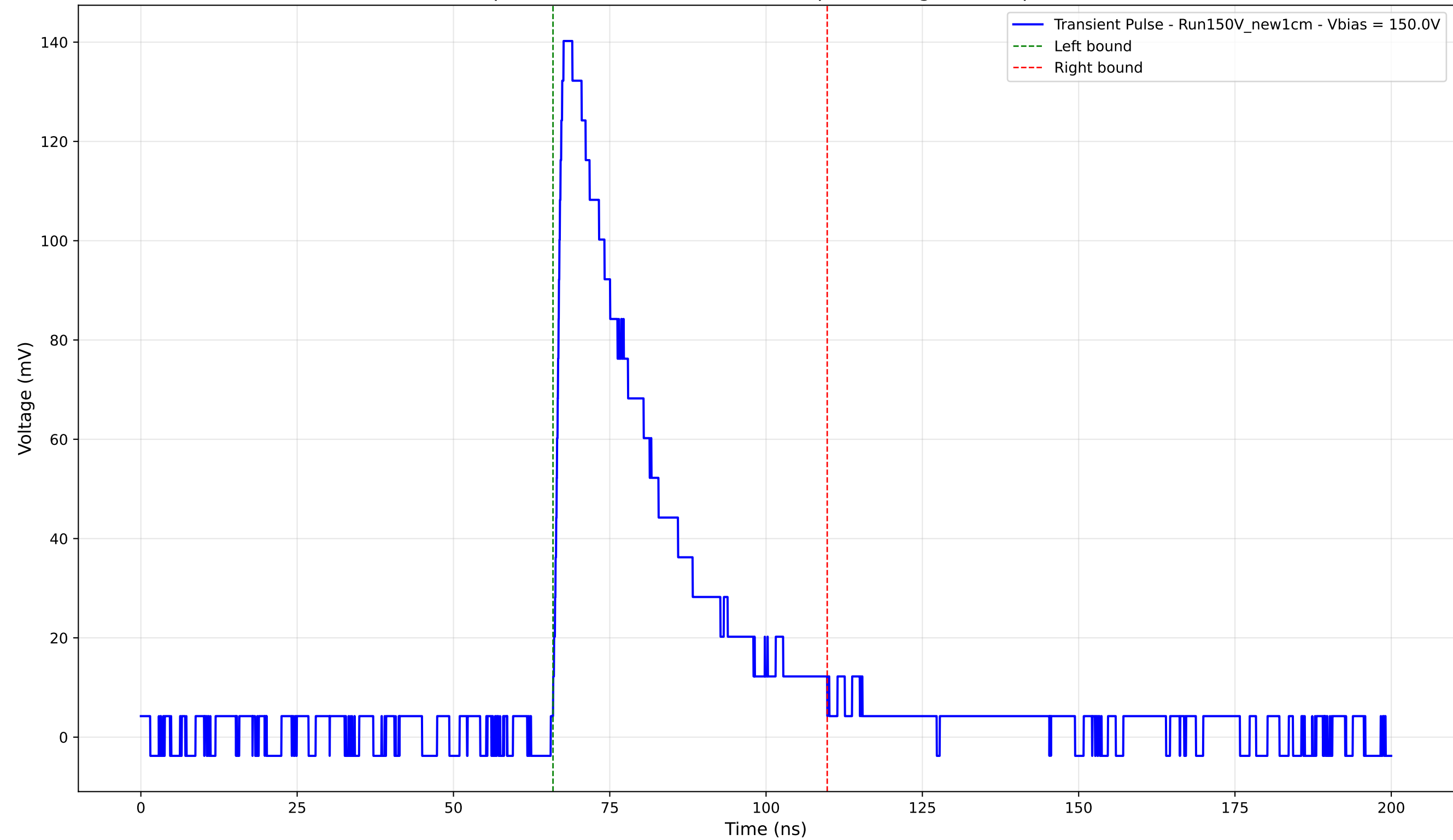
Transient Pulse - Sample: New1cm - Position: 3450.0 \mu\text{m} - Charge: 43.12 pC - Rise Time: 1.32 ns
