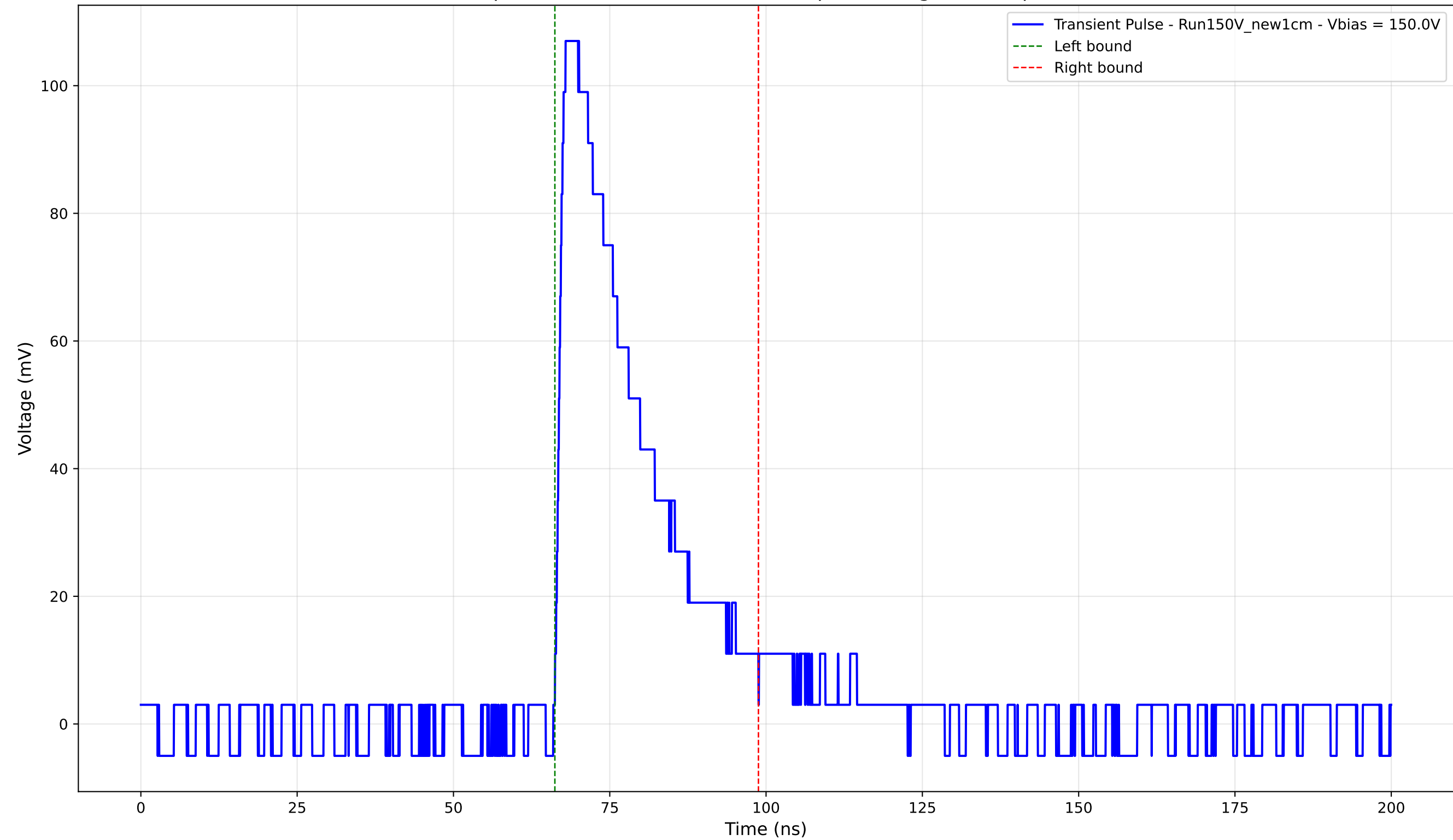
Transient Pulse - Sample: New1cm - Position: 1205.0 \mu\text{m} - Charge: 29.92 pC - Rise Time: 1.36 ns
