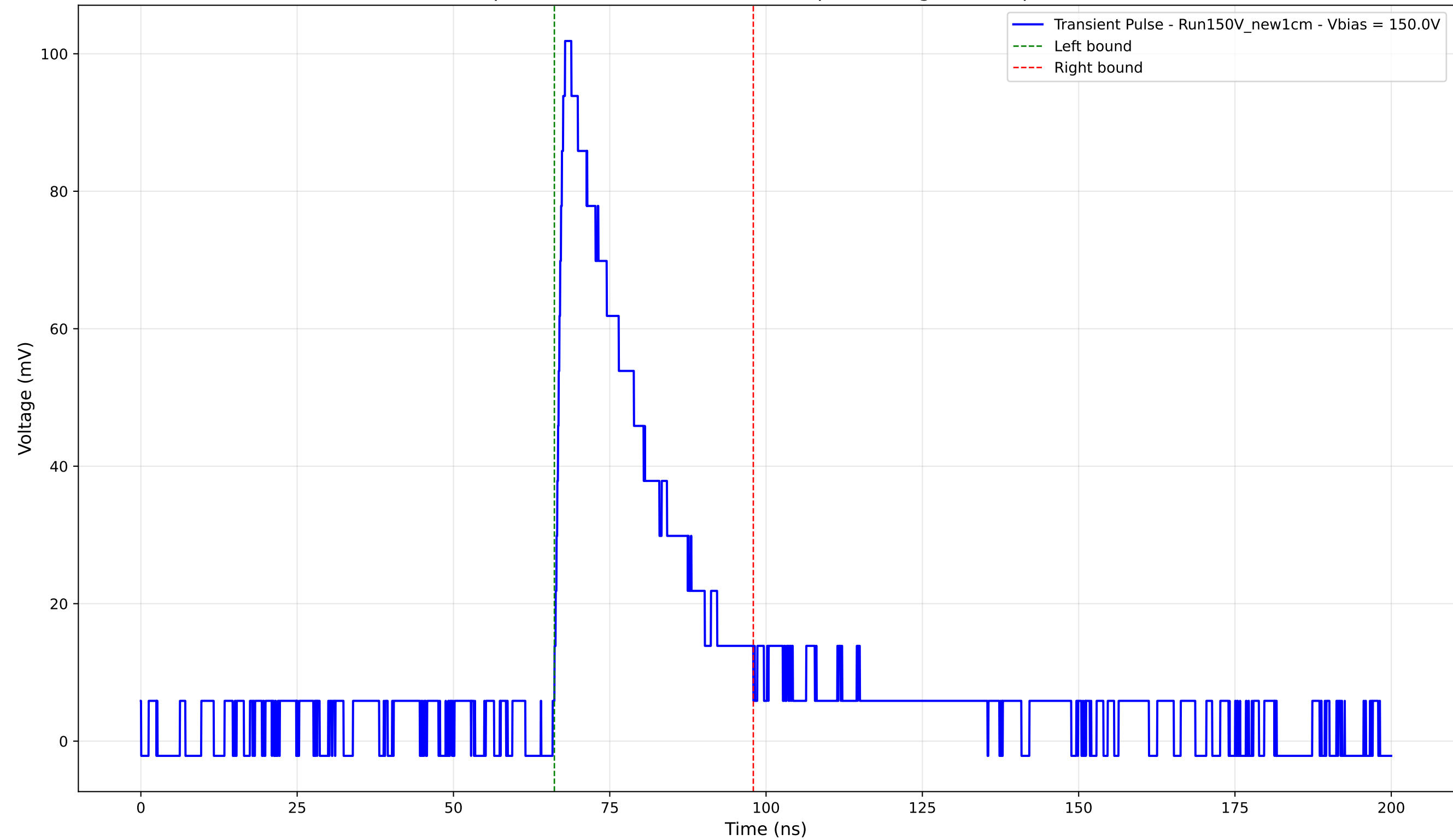
Transient Pulse - Sample: New1cm - Position: 3630.0 \mu\text{m} - Charge: 27.87 pC - Rise Time: 1.39 ns
