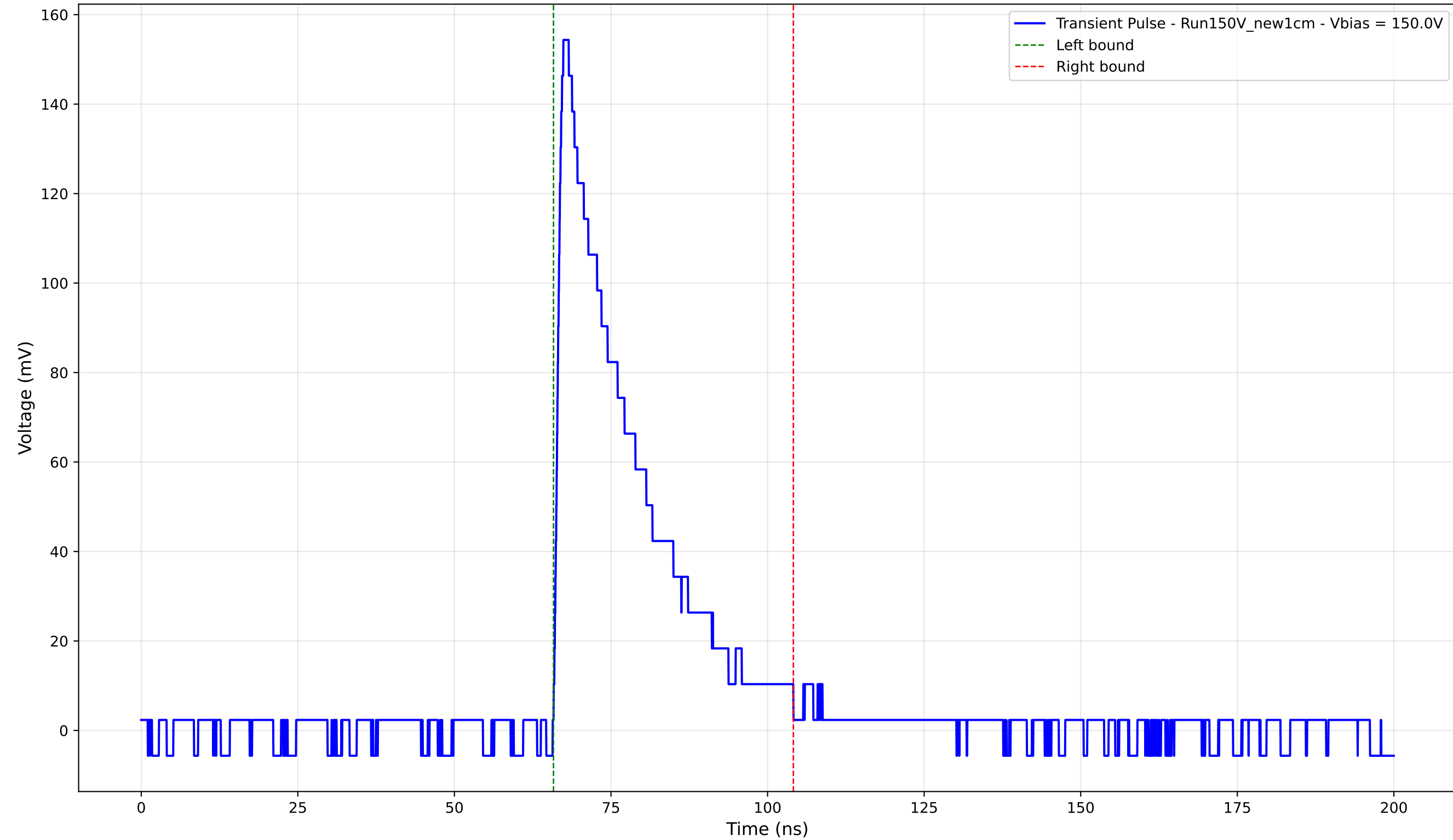
Transient Pulse - Sample: New1cm - Position: 4450.0 \mu\text{m} - Charge: 38.77 pC - Rise Time: 1.23 ns
