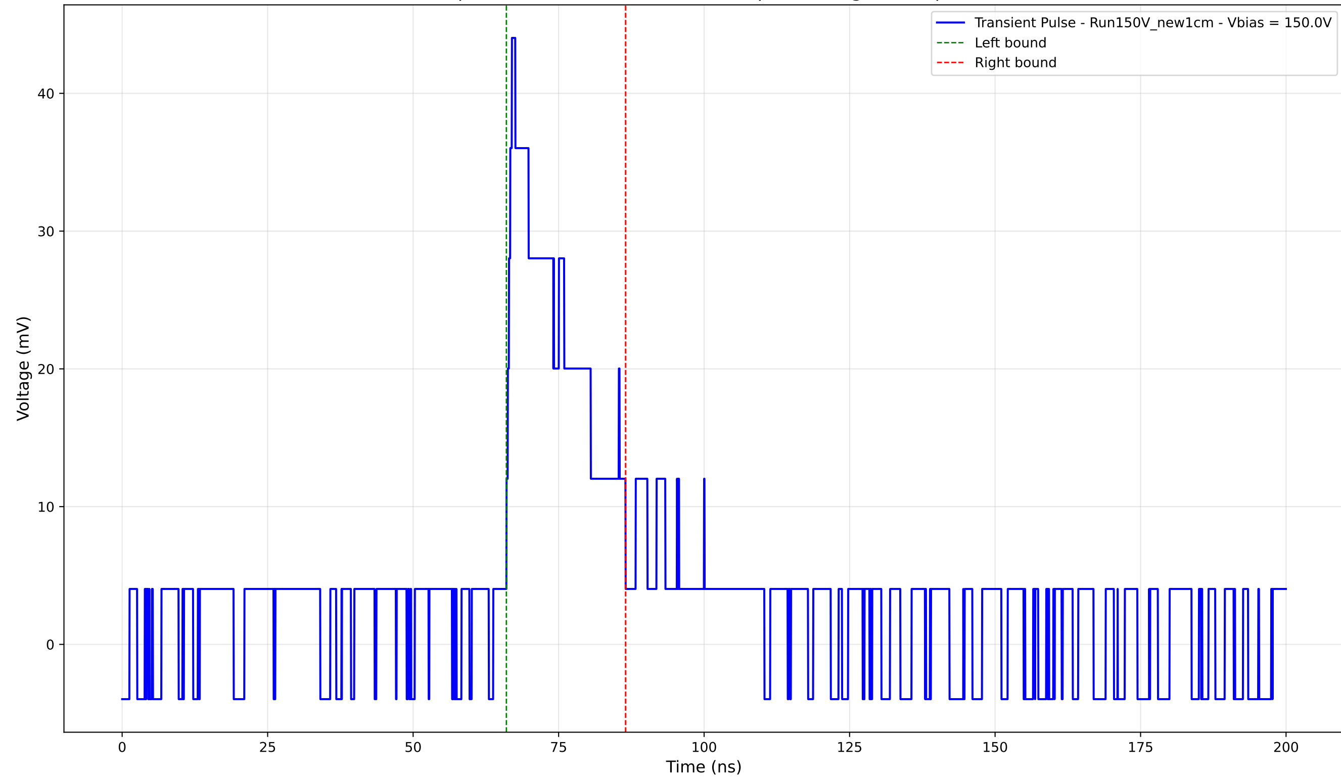
Transient Pulse - Sample: New1cm - Position: 3030.0 \mu\text{m} - Charge: 9.21 pC - Rise Time: 0.94 ns
