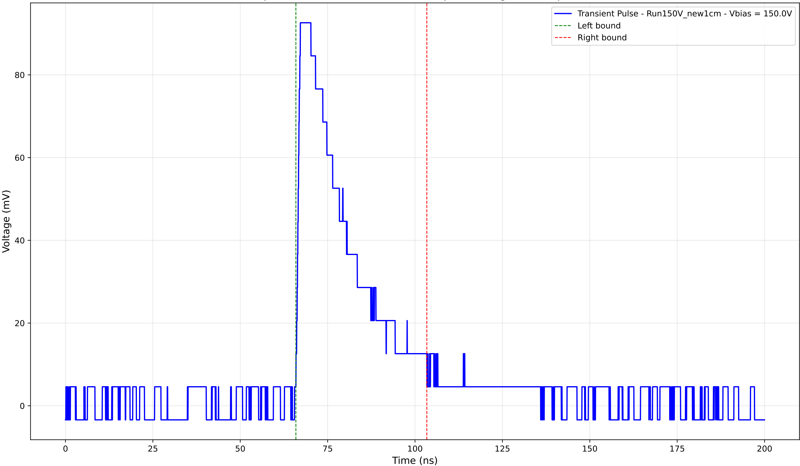
Transient Pulse - Sample: New1cm - Position: 1805.0 \mu\text{m} - Charge: 29.42 pC - Rise Time: 1.11 ns
