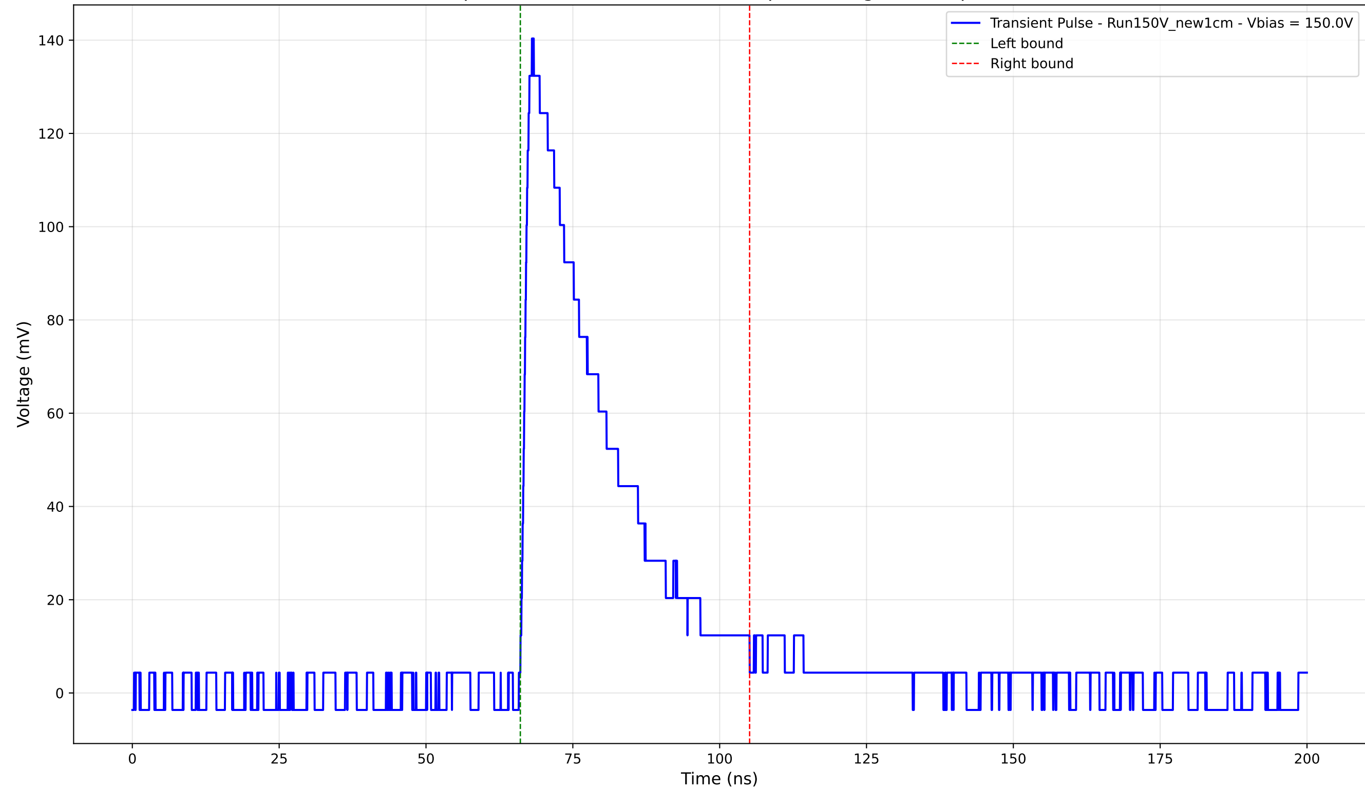
Transient Pulse - Sample: New1cm - Position: 3680.0 \mu\text{m} - Charge: 39.77 pC - Rise Time: 1.38 ns
