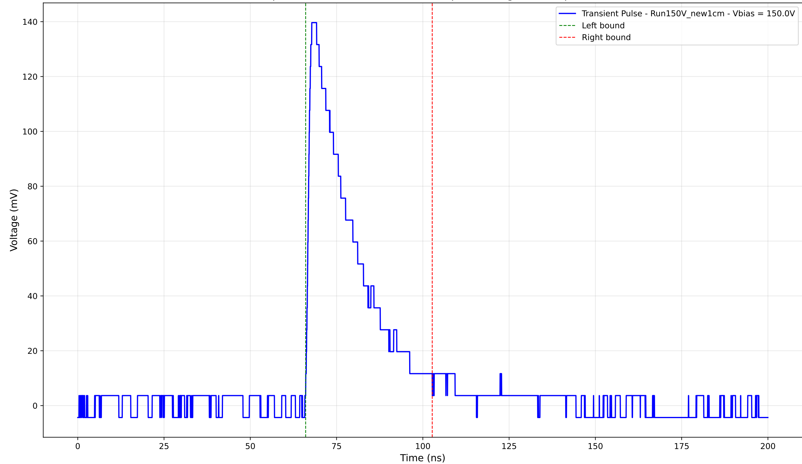
Transient Pulse - Sample: New1cm - Position: 3940.0 \mu\text{m} - Charge: 39.24 pC - Rise Time: 1.31 ns
