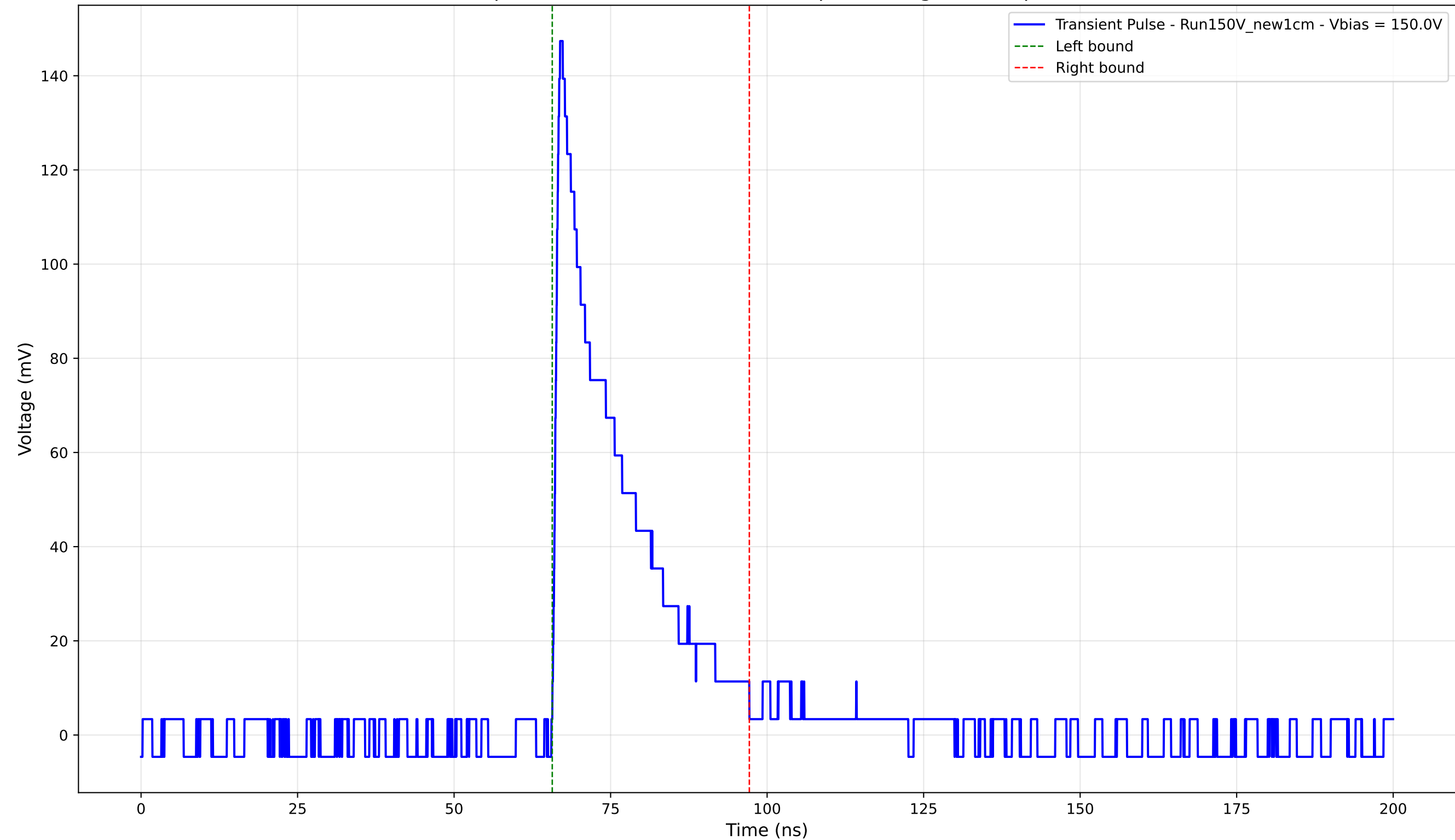
Transient Pulse - Sample: New1cm - Position: 4755.0 \mu\text{m} - Charge: 30.25 pC - Rise Time: 0.99 ns
