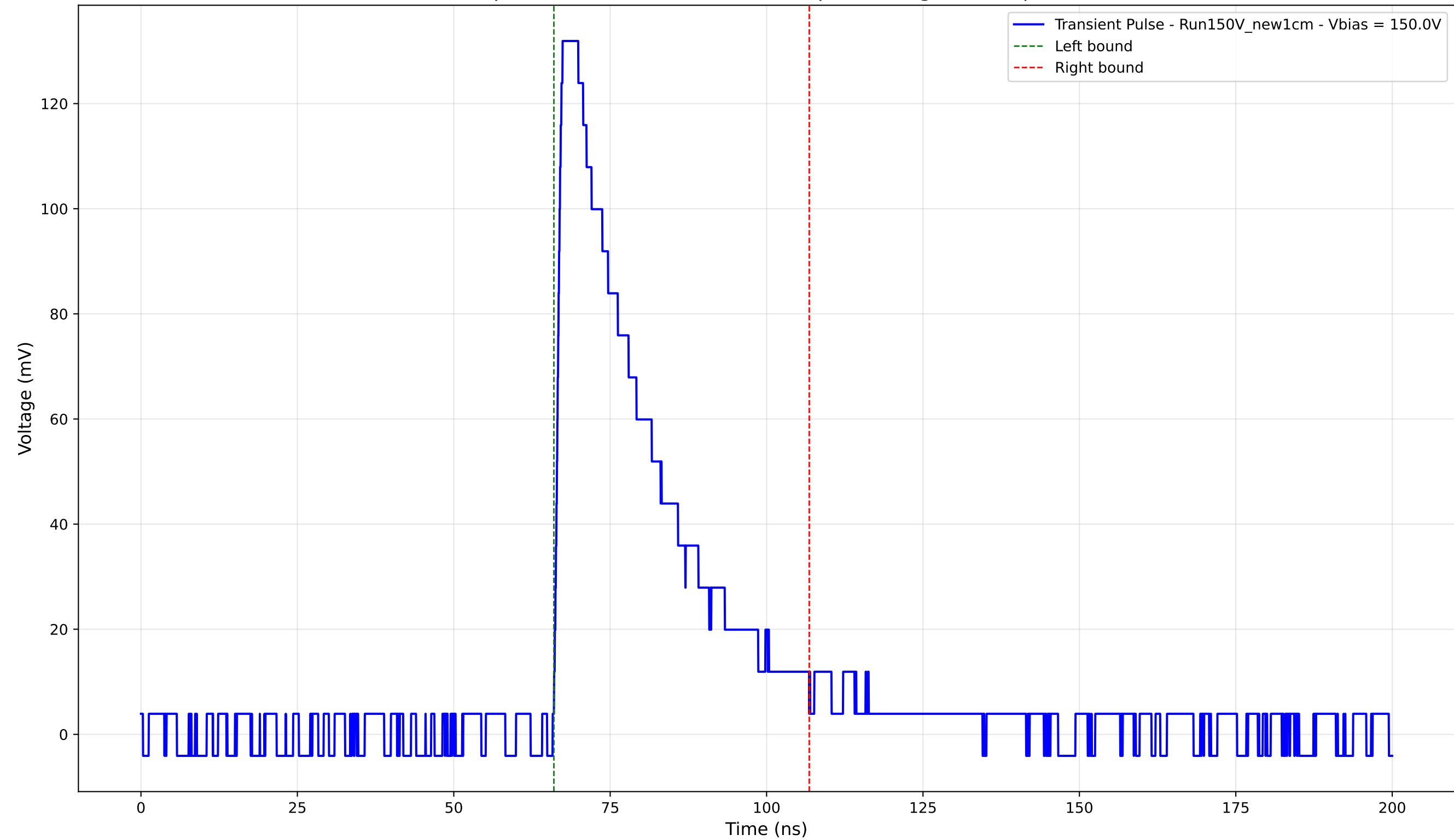
Transient Pulse - Sample: New1cm - Position: 3370.0 \mu\text{m} - Charge: 41.24 pC - Rise Time: 1.08 ns
