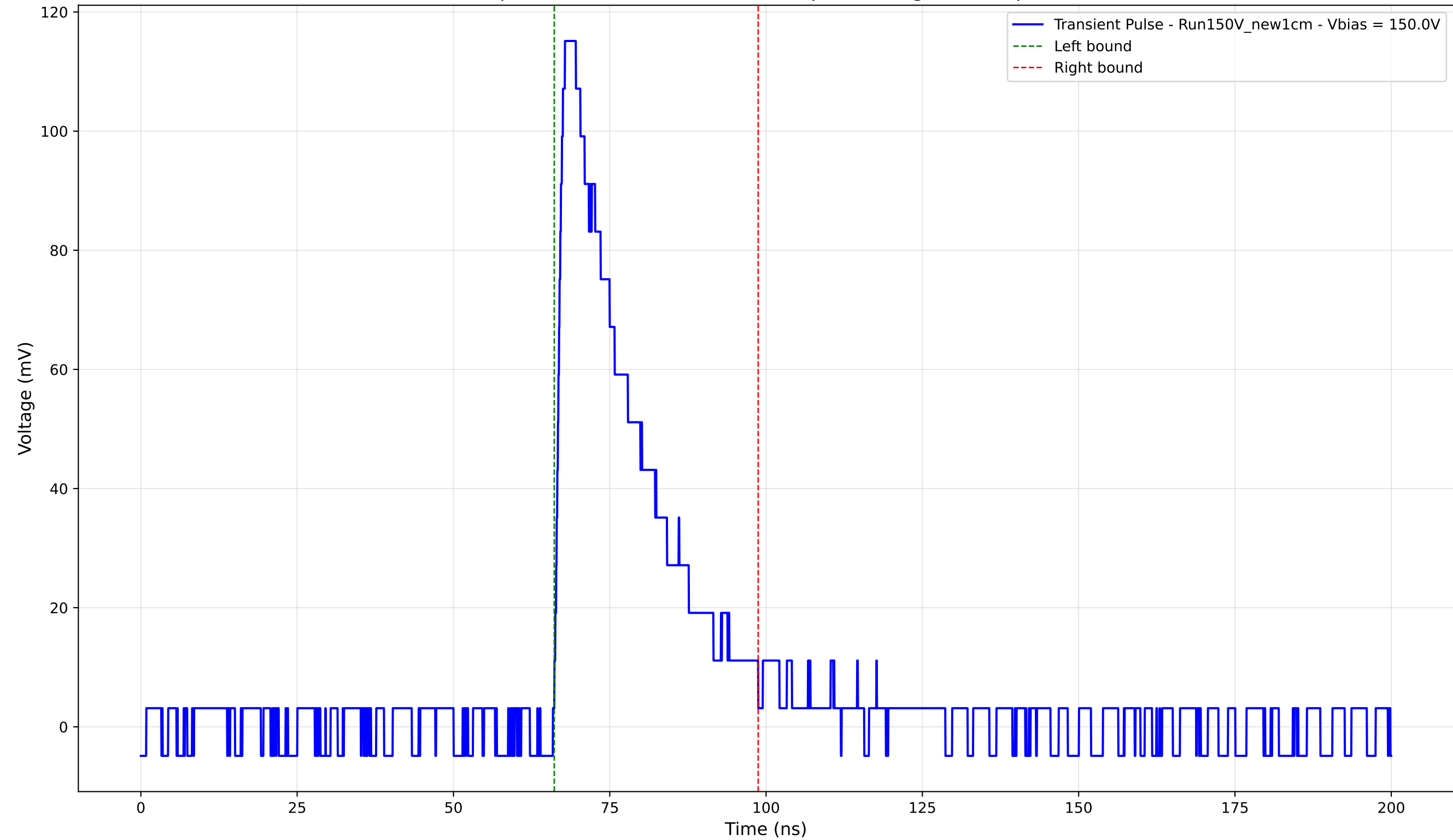
Transient Pulse - Sample: New1cm - Position: 790.0 \mu\text{m} - Charge: 30.03 pC - Rise Time: 1.24 ns
