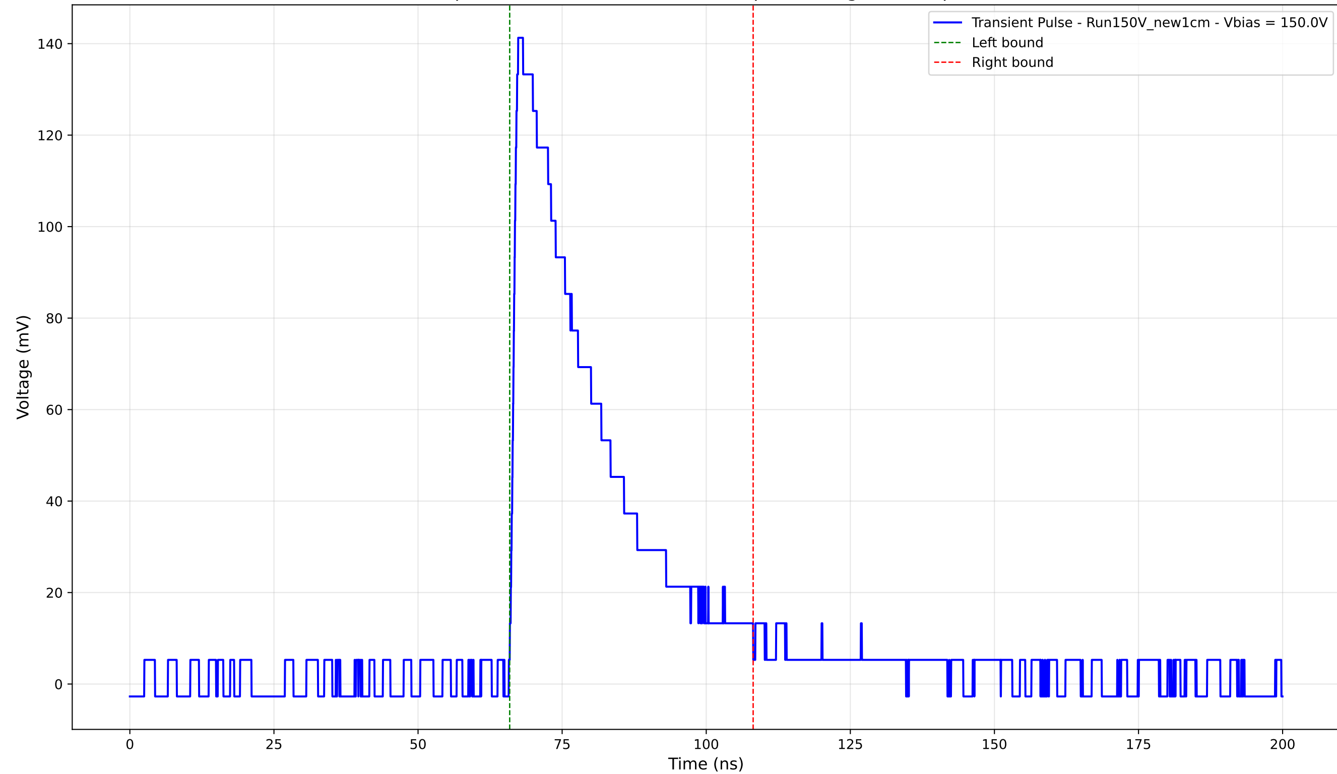
Transient Pulse - Sample: New1cm - Position: 3315.0 \mu\text{m} - Charge: 43.74 pC - Rise Time: 1.12 ns
