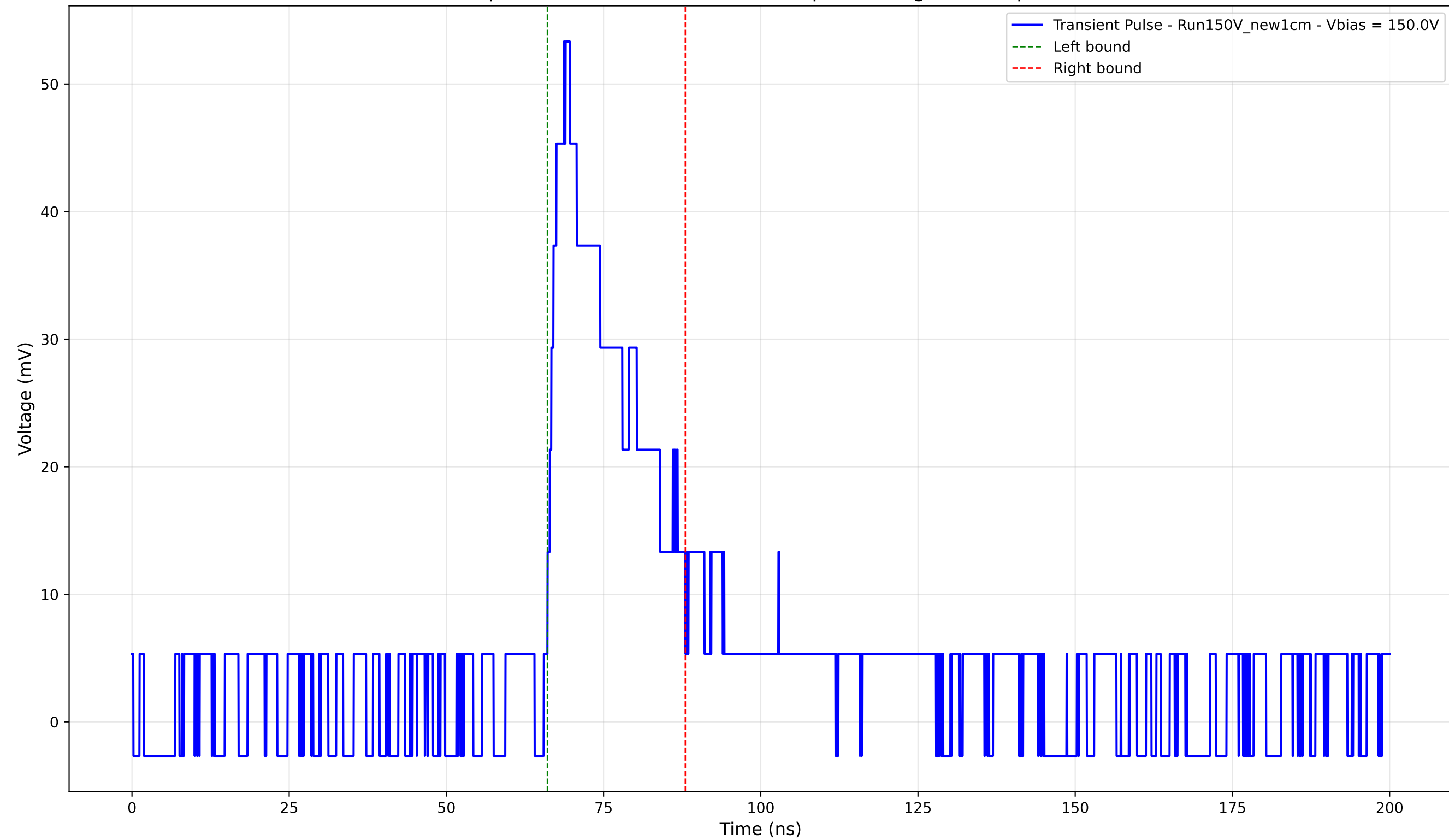
Transient Pulse - Sample: New1cm - Position: 4030.0 \mu\text{m} - Charge: 12.58 pC - Rise Time: 2.62 ns
