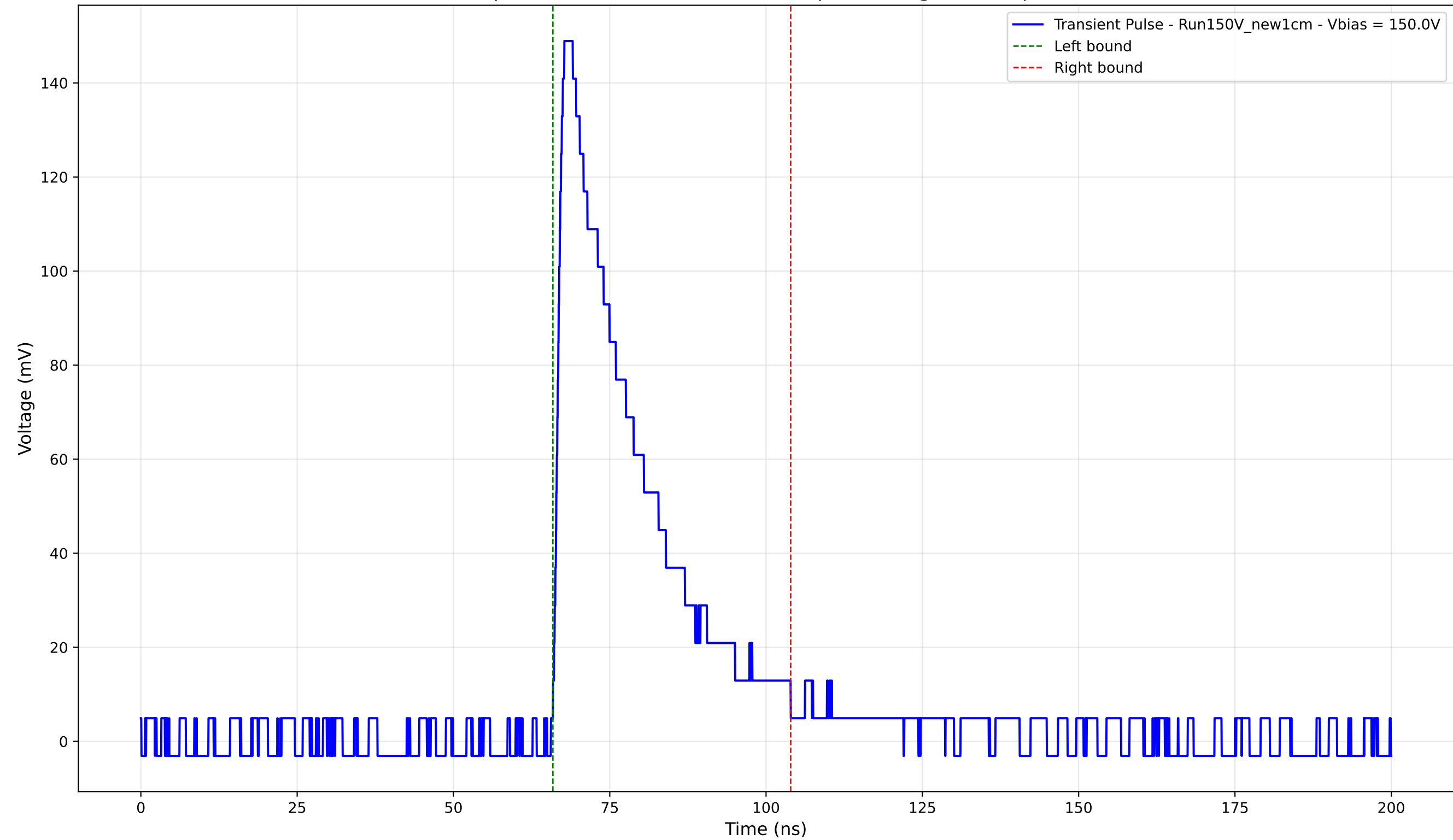
Transient Pulse - Sample: New1cm - Position: 4240.0 \mu\text{m} - Charge: 40.15 pC - Rise Time: 1.42 ns
