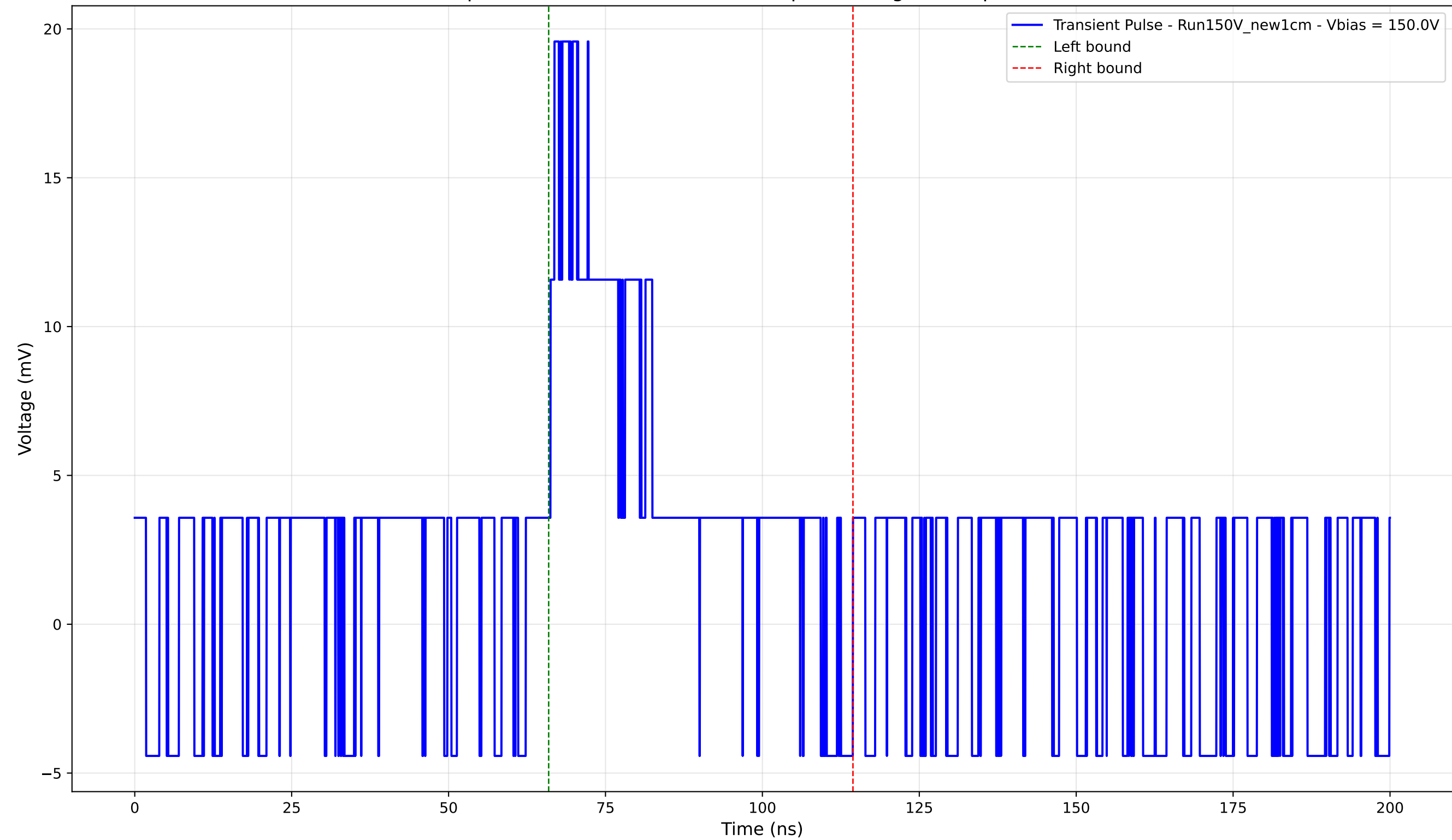
Transient Pulse - Sample: New1cm - Position: 2045.0 \mu\text{m} - Charge: 5.54 pC - Rise Time: 0.00 ns (N/A)
