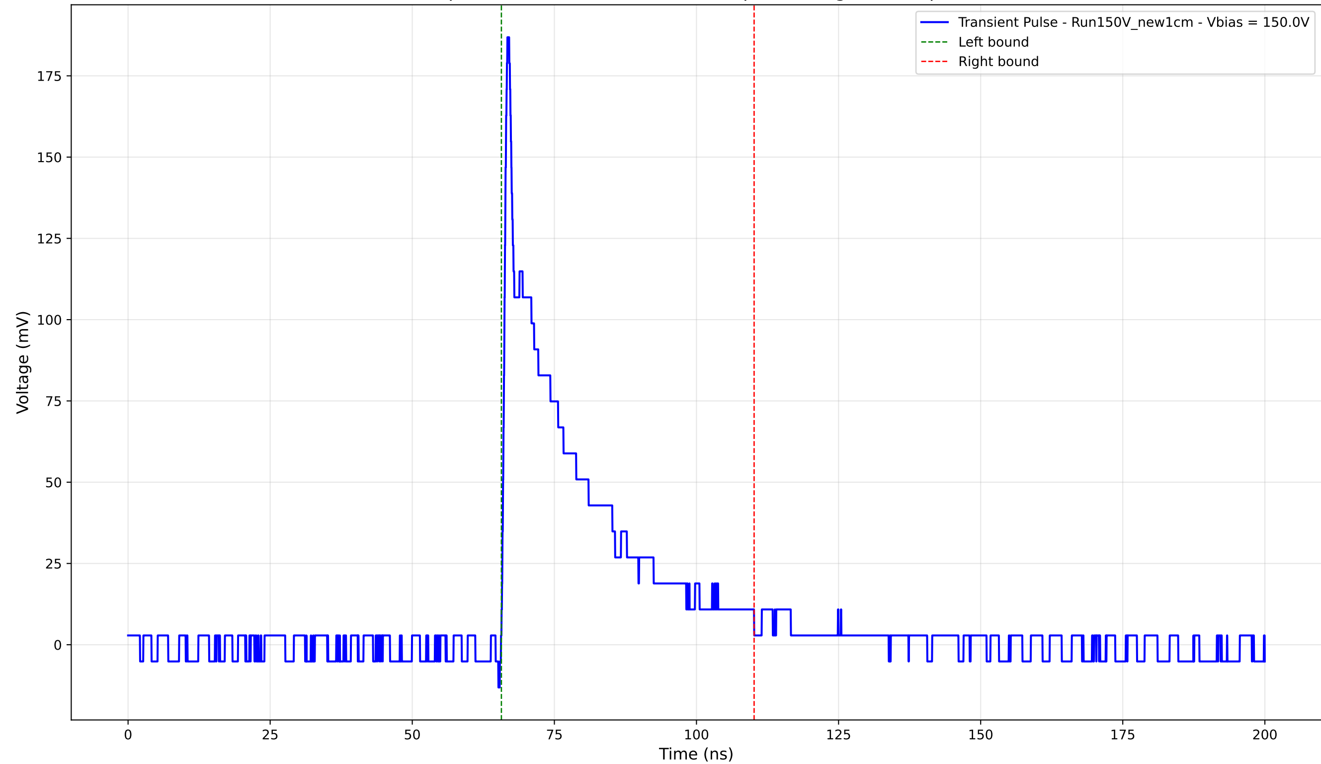
Transient Pulse - Sample: New1cm - Position: 2780.0 \mu\text{m} - Charge: 38.96 pC - Rise Time: 0.80 ns
