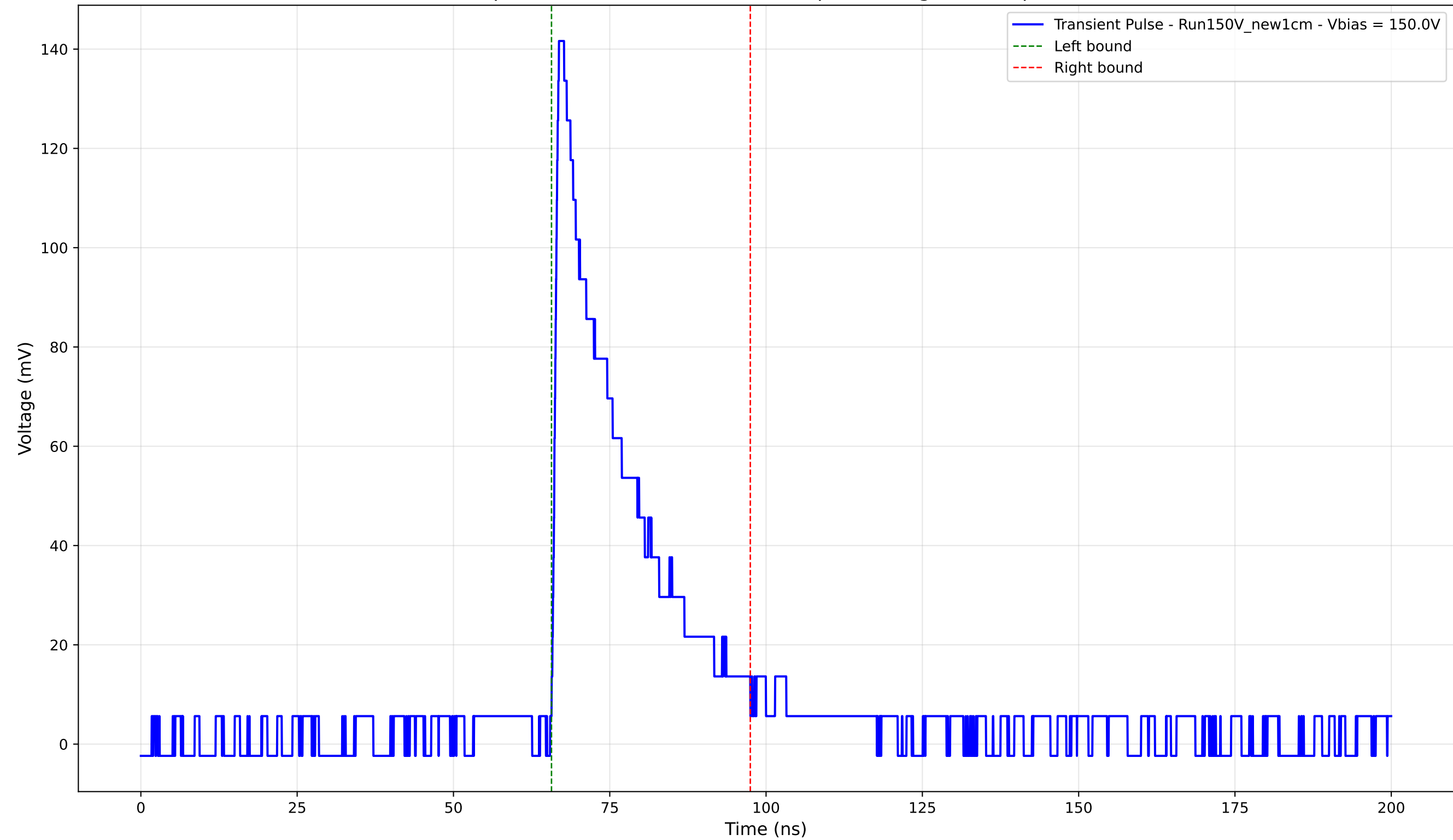
Transient Pulse - Sample: New1cm - Position: 4725.0 \mu\text{m} - Charge: 32.01 pC - Rise Time: 0.96 ns
