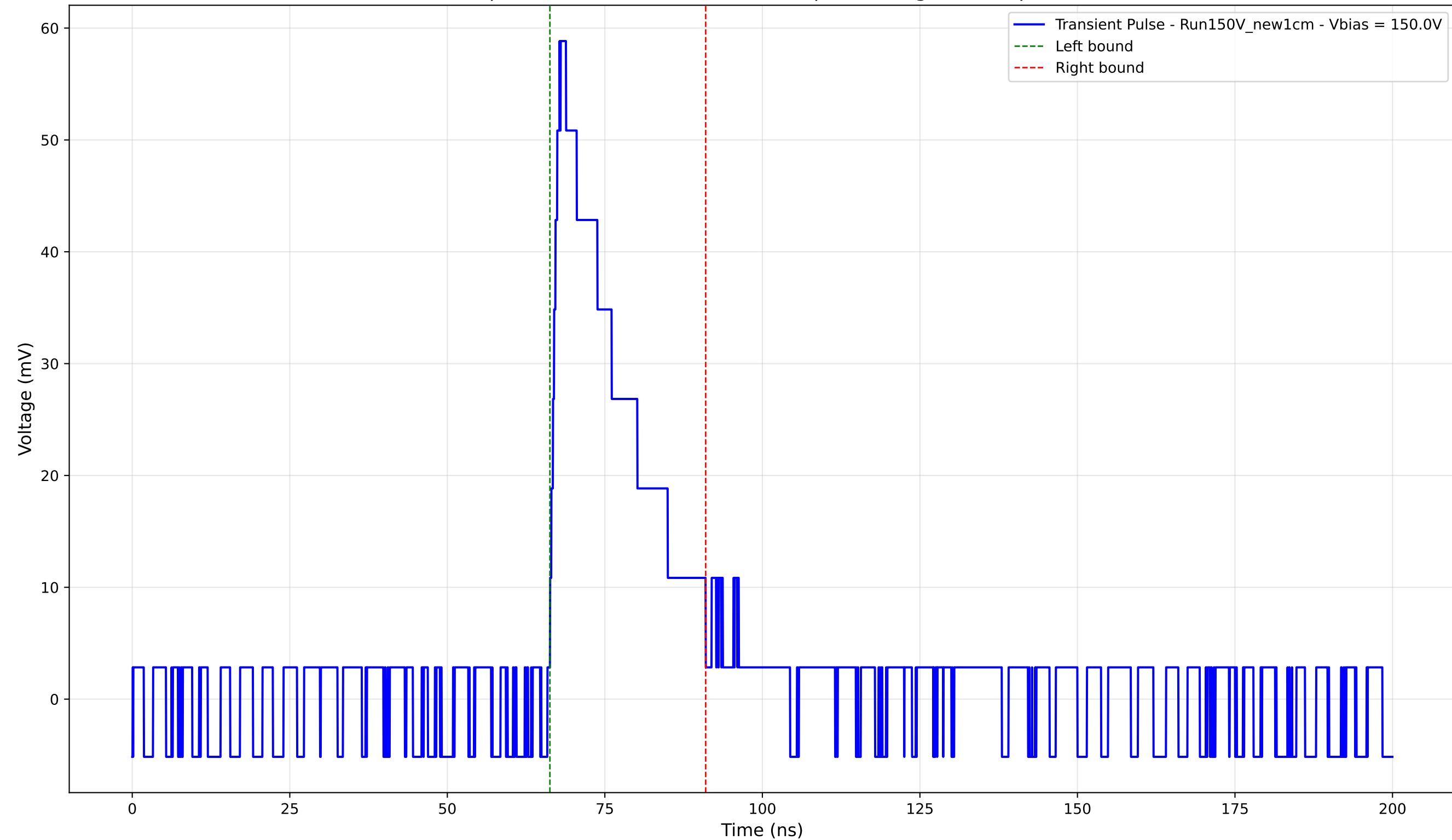
Transient Pulse - Sample: New1cm - Position: 4025.0 \mu\text{m} - Charge: 13.62 pC - Rise Time: 1.53 ns
