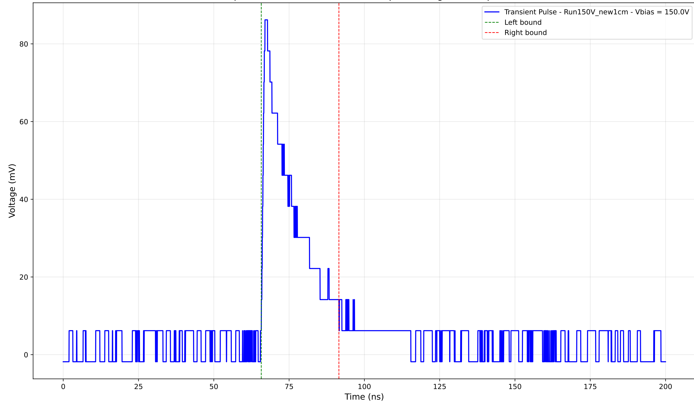
Transient Pulse - Sample: New1cm - Position: 4625.0 \mu\text{m} - Charge: 18.83 pC - Rise Time: 0.99 ns
