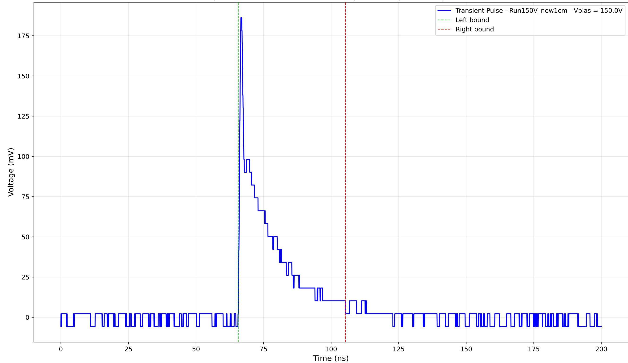
Transient Pulse - Sample: New1cm - Position: 2655.0 \mu\text{m} - Charge: 32.17 pC - Rise Time: 0.72 ns
