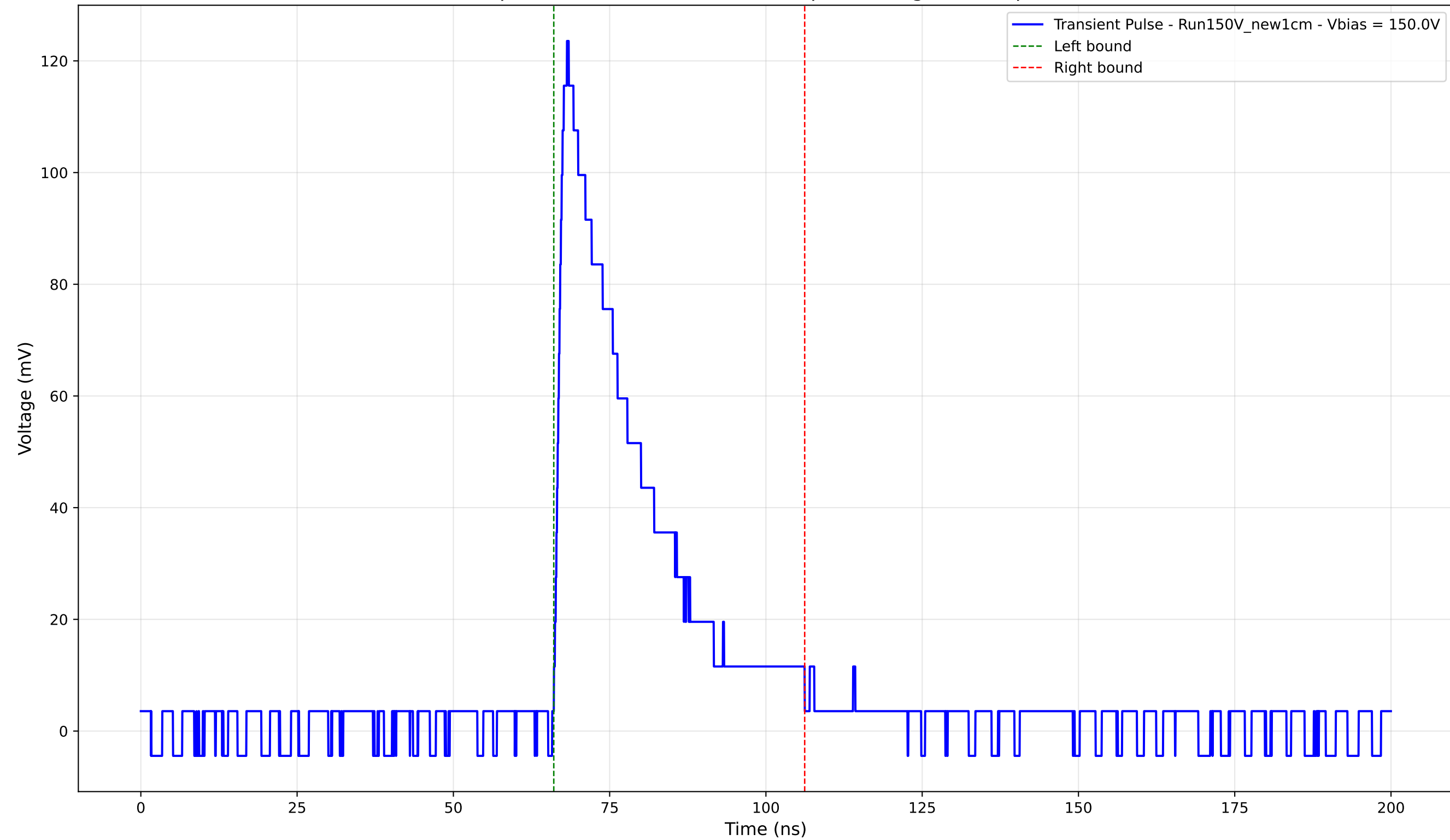
Transient Pulse - Sample: New1cm - Position: 780.0 \mu\text{m} - Charge: 32.27 pC - Rise Time: 1.44 ns
