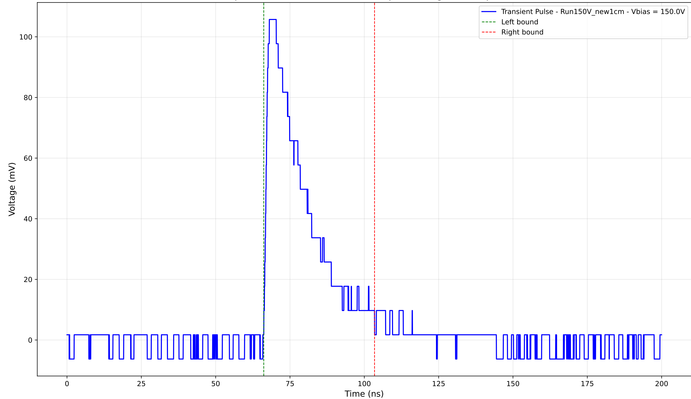
Transient Pulse - Sample: New1cm - Position: 1200.0 \mu\text{m} - Charge: 30.78 pC - Rise Time: 1.28 ns
