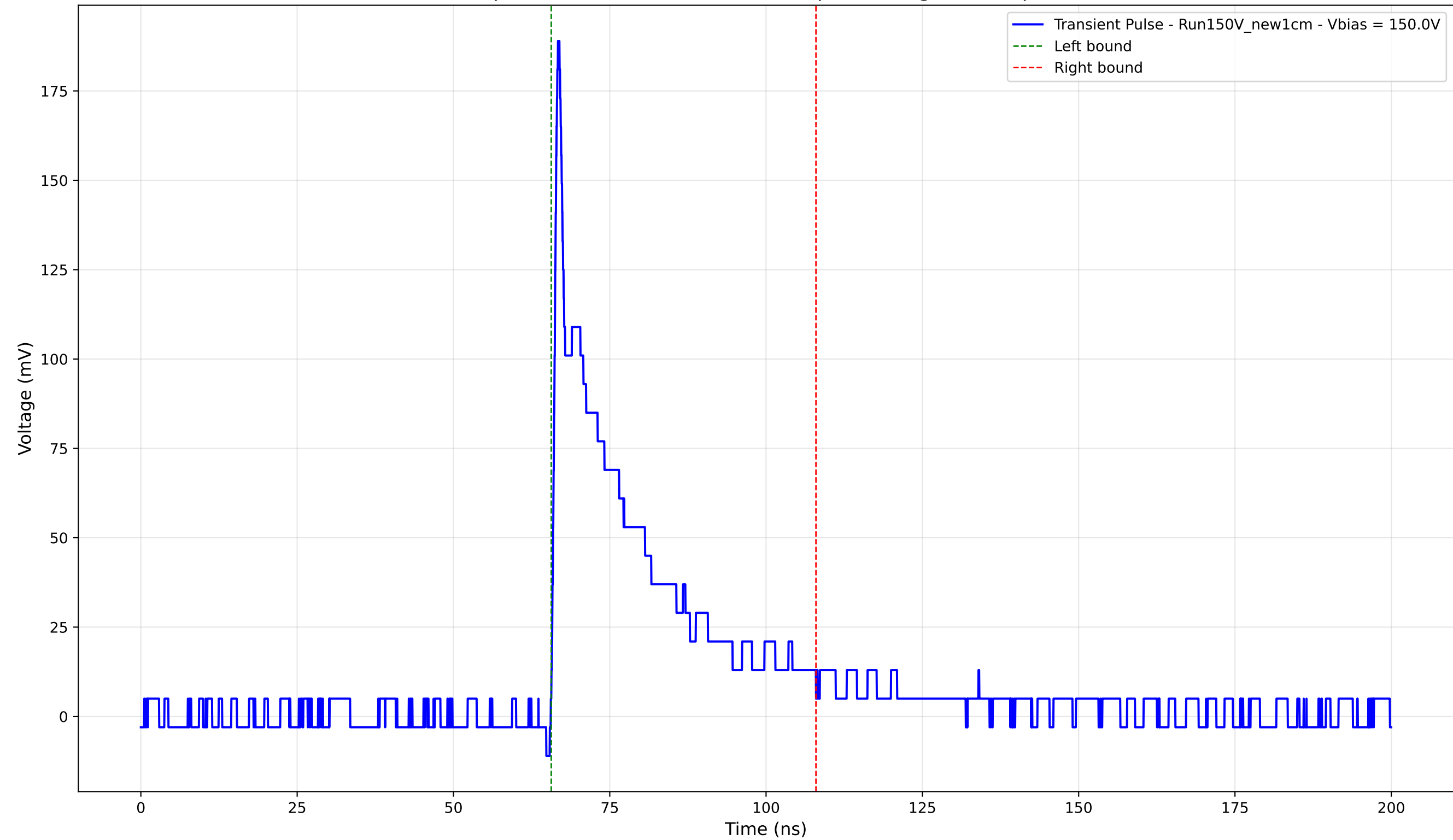
Transient Pulse - Sample: New1cm - Position: 2370.0 \mu\text{m} - Charge: 37.53 pC - Rise Time: 0.81 ns
