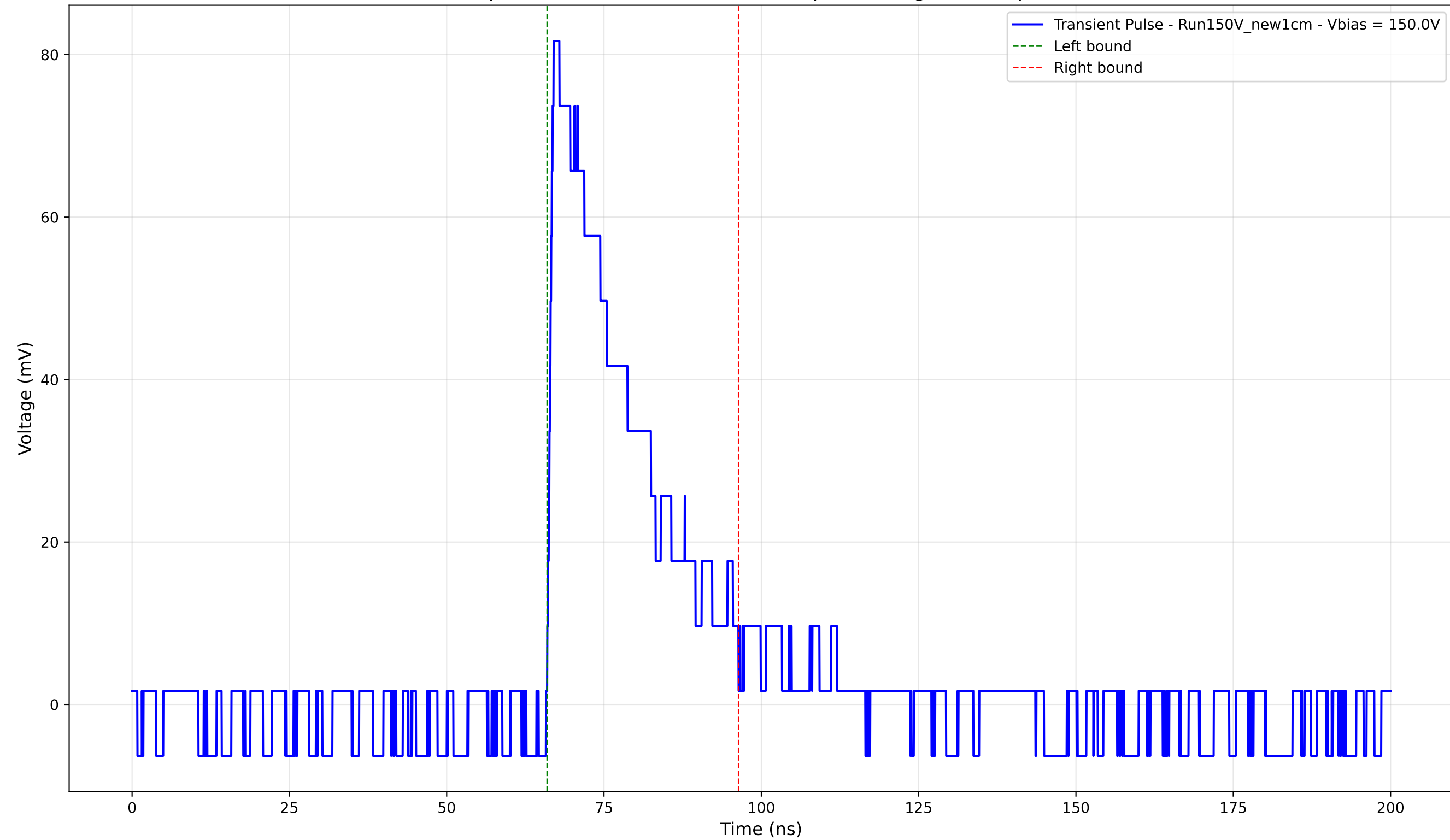
Transient Pulse - Sample: New1cm - Position: 3120.0 \mu\text{m} - Charge: 21.73 pC - Rise Time: 0.84 ns
