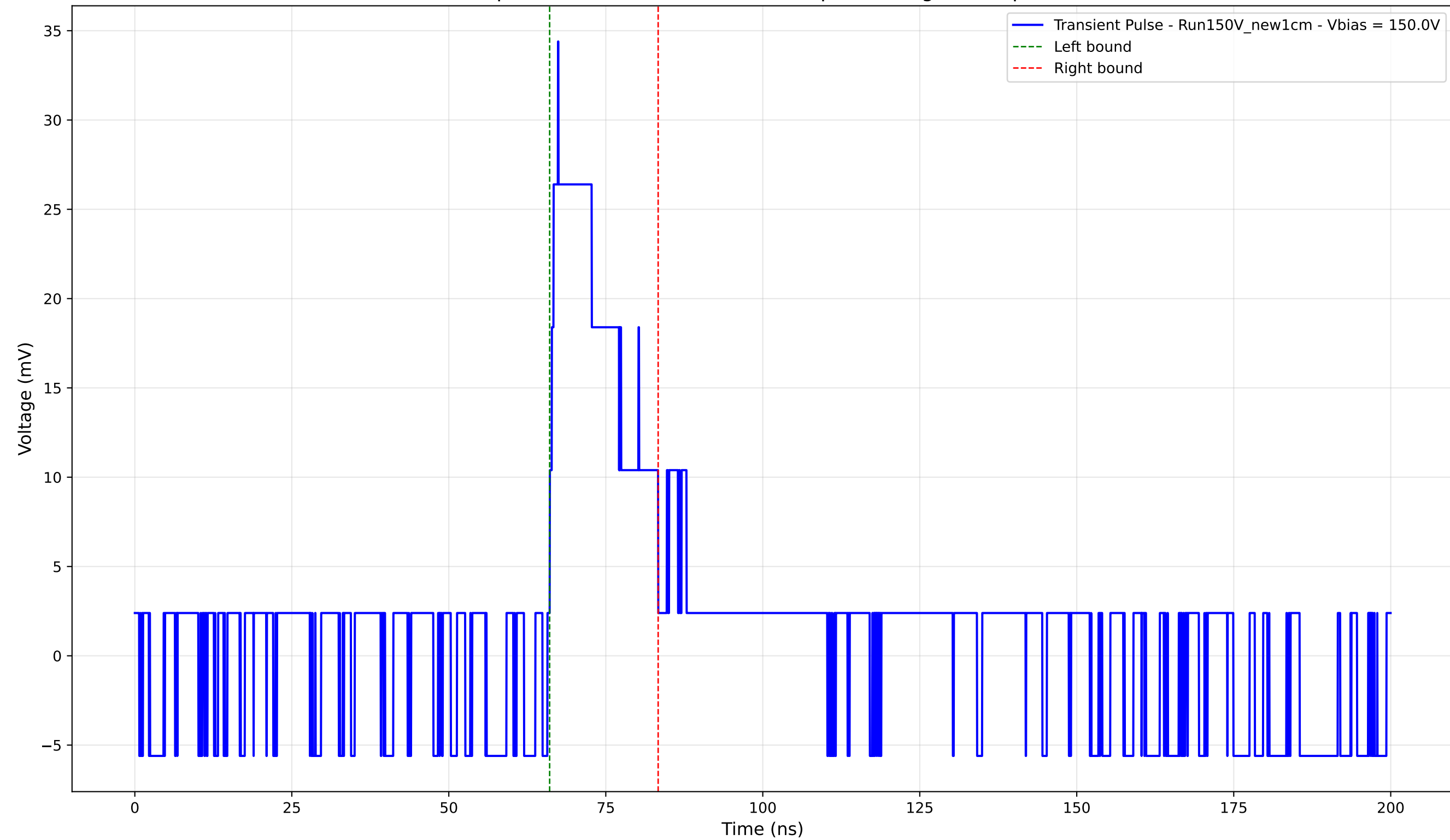
Transient Pulse - Sample: New1cm - Position: 3085.0 \mu\text{m} - Charge: 6.34 pC - Rise Time: 1.32 ns
