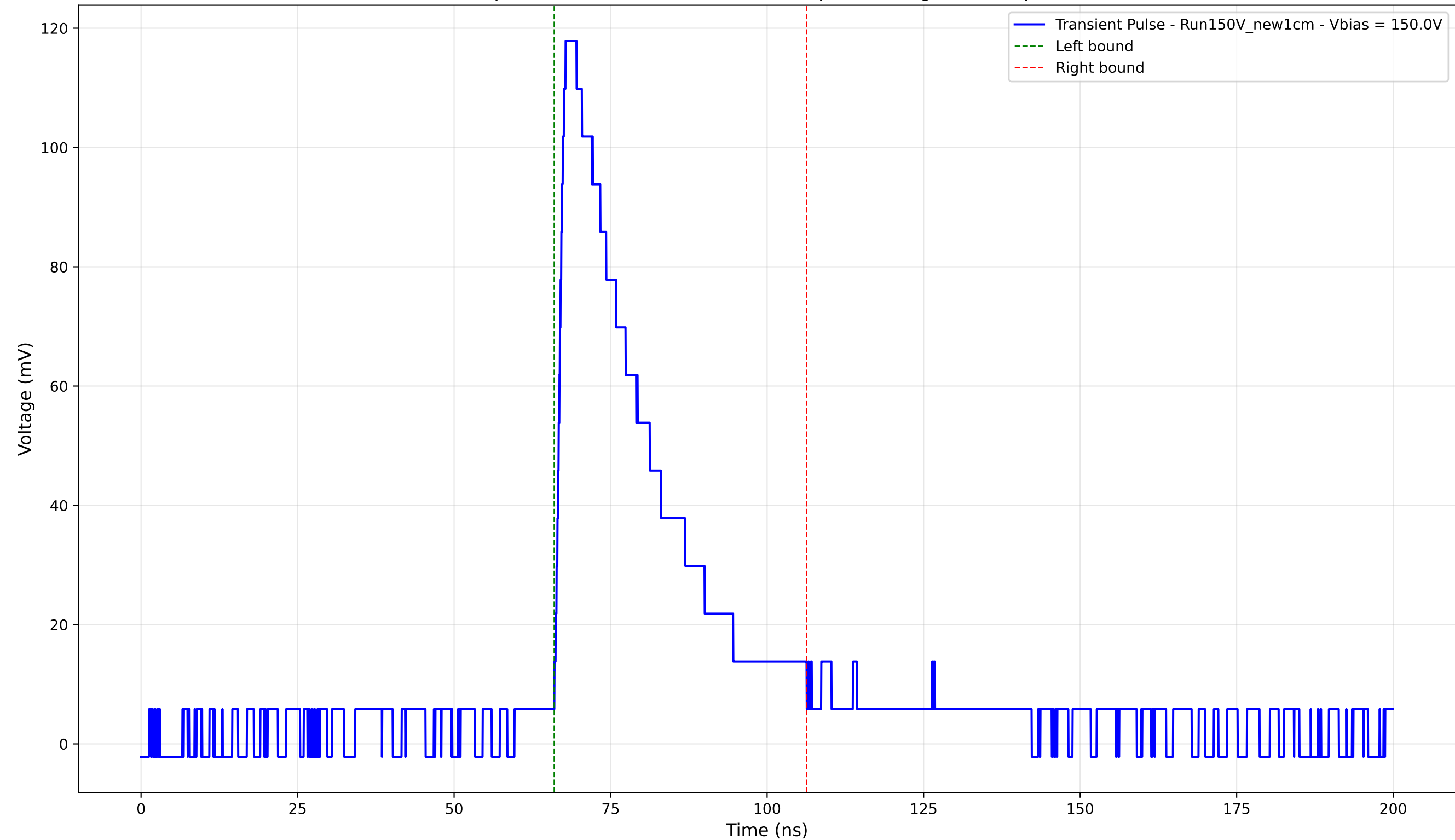
Transient Pulse - Sample: New1cm - Position: 3645.0 \mu\text{m} - Charge: 36.43 pC - Rise Time: 1.53 ns
