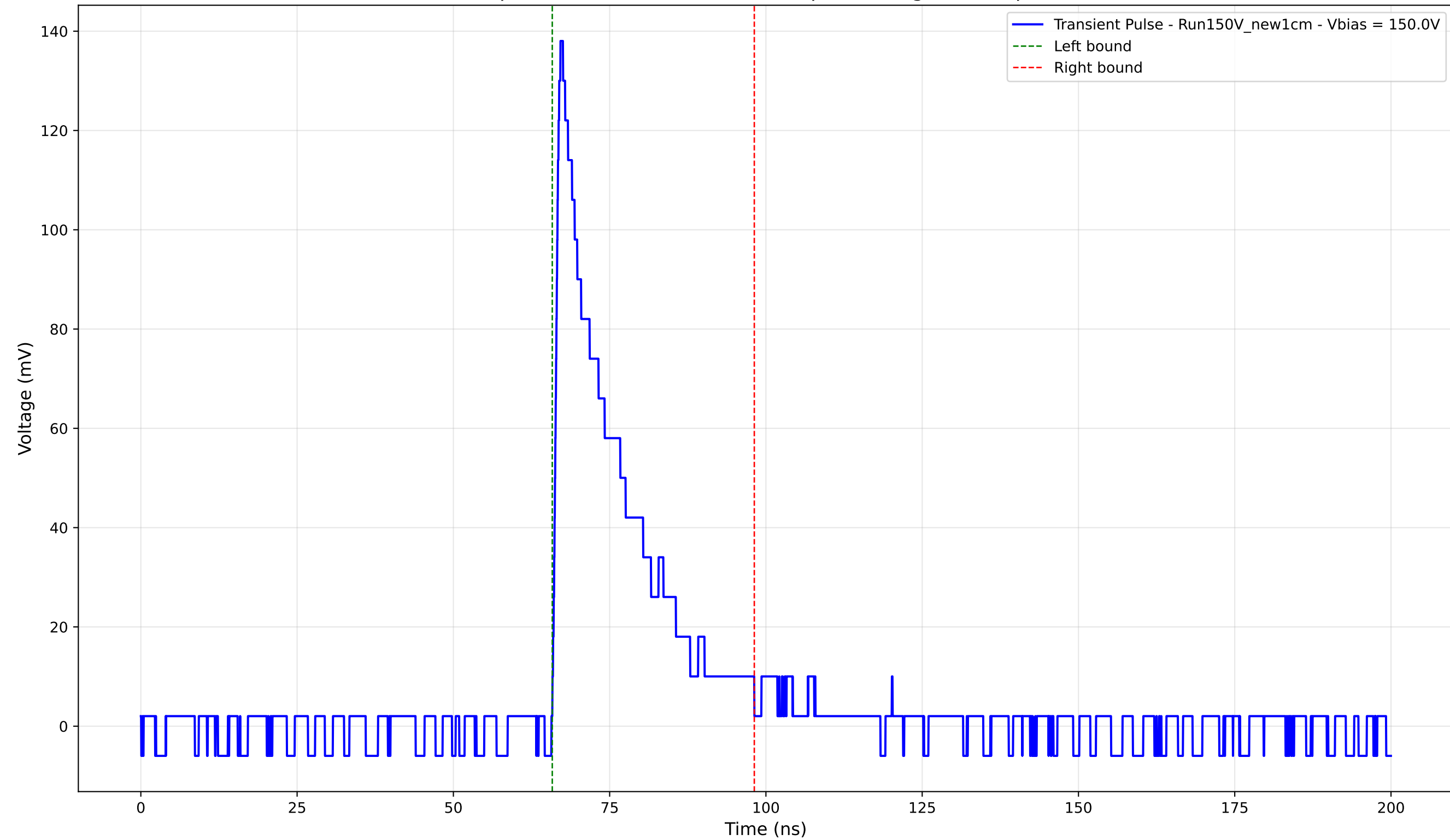
Transient Pulse - Sample: New1cm - Position: 250.0 \mu\text{m} - Charge: 27.23 pC - Rise Time: 0.99 ns
