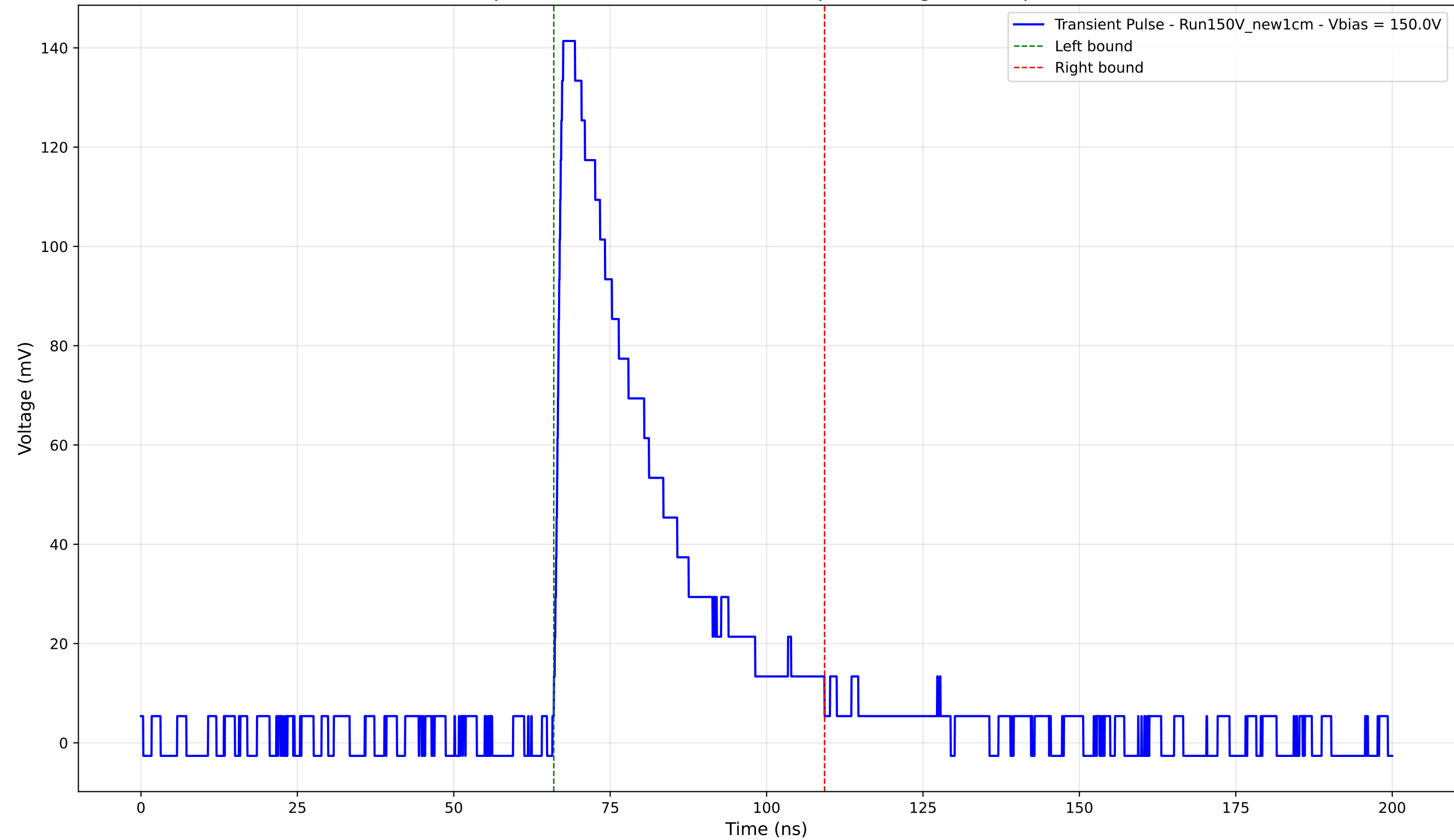
Transient Pulse - Sample: New1cm - Position: 3430.0 \mu\text{m} - Charge: 43.97 pC - Rise Time: 1.18 ns
