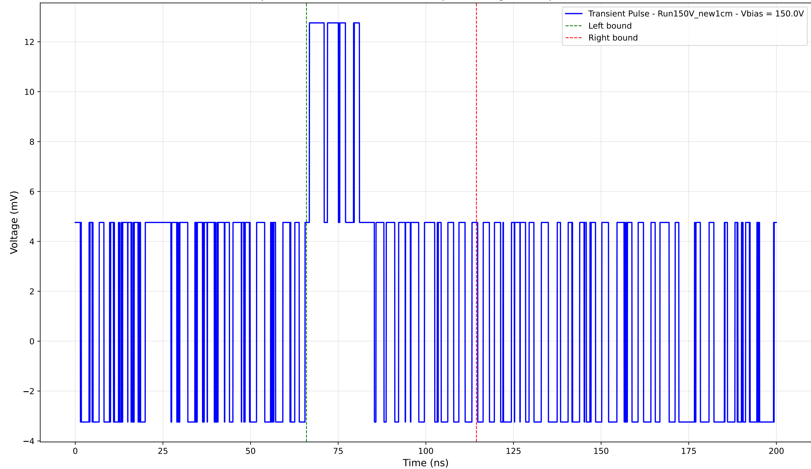
Transient Pulse - Sample: New1cm - Position: 1545.0 \mu\text{m} - Charge: 4.68 pC - Rise Time: 0.00 ns (N/A)
