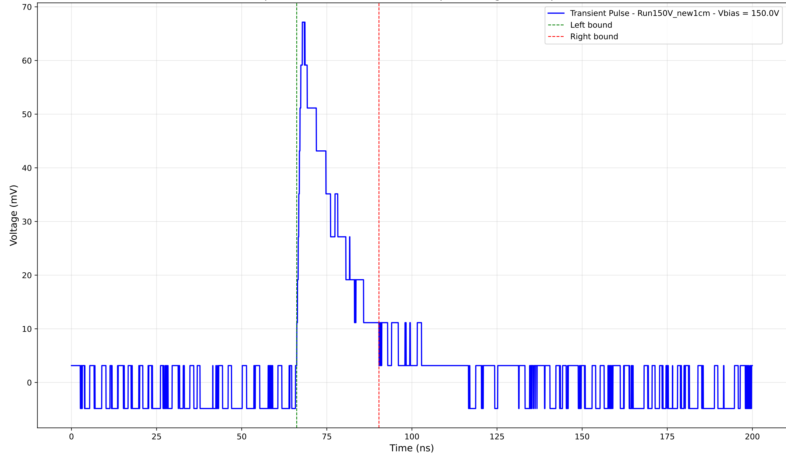
Transient Pulse - Sample: New1cm - Position: 4115.0 \mu\text{m} - Charge: 14.77 pC - Rise Time: 1.63 ns
