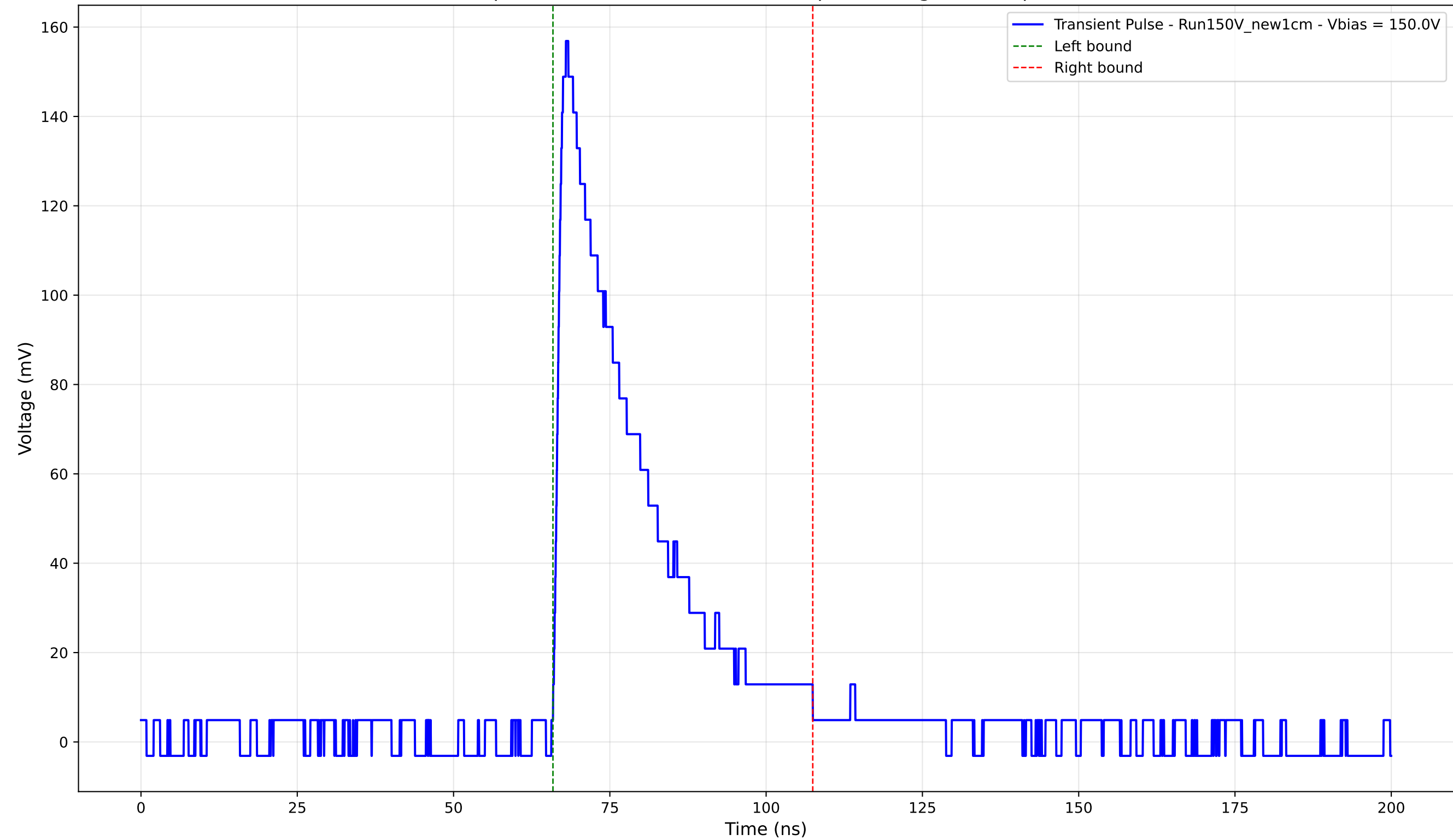
Transient Pulse - Sample: New1cm - Position: 4245.0 \mu\text{m} - Charge: 42.40 pC - Rise Time: 1.45 ns
