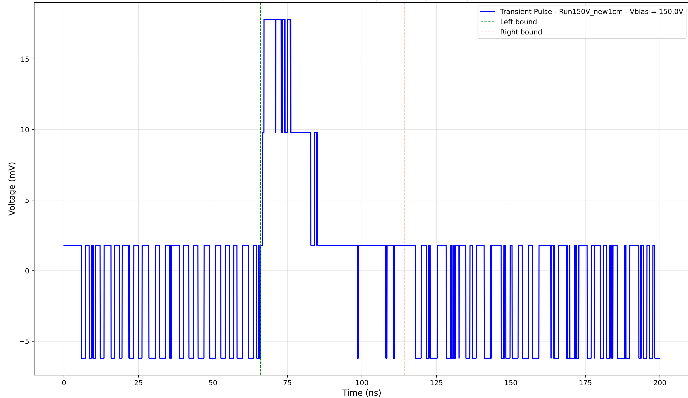
Transient Pulse - Sample: New1cm - Position: 3570.0 \mu\text{m} - Charge: 5.51 pC - Rise Time: 0.00 ns (N/A)
