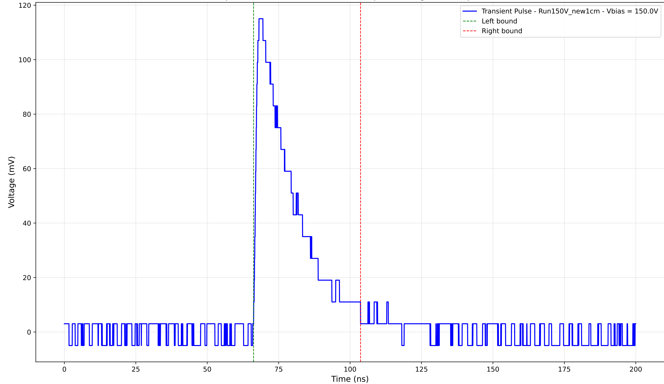
Transient Pulse - Sample: New1cm - Position: 1275.0 \mu\text{m} - Charge: 32.83 pC - Rise Time: 1.32 ns
