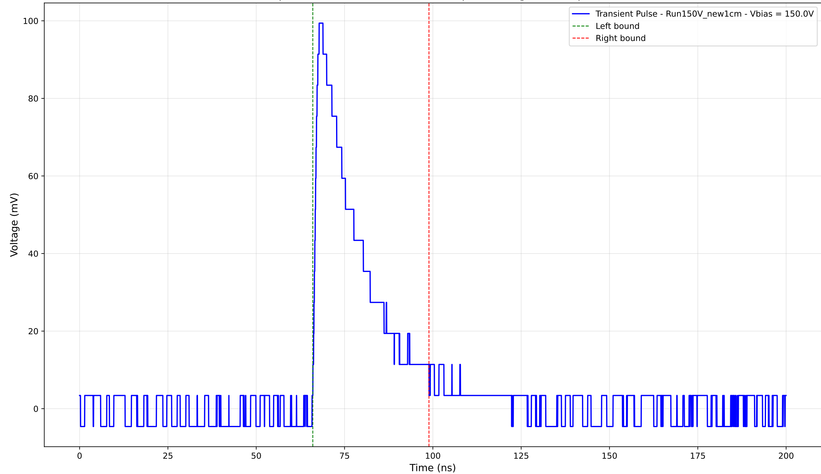
Transient Pulse - Sample: New1cm - Position: 4150.0 \mu\text{m} - Charge: 25.82 pC - Rise Time: 1.40 ns
