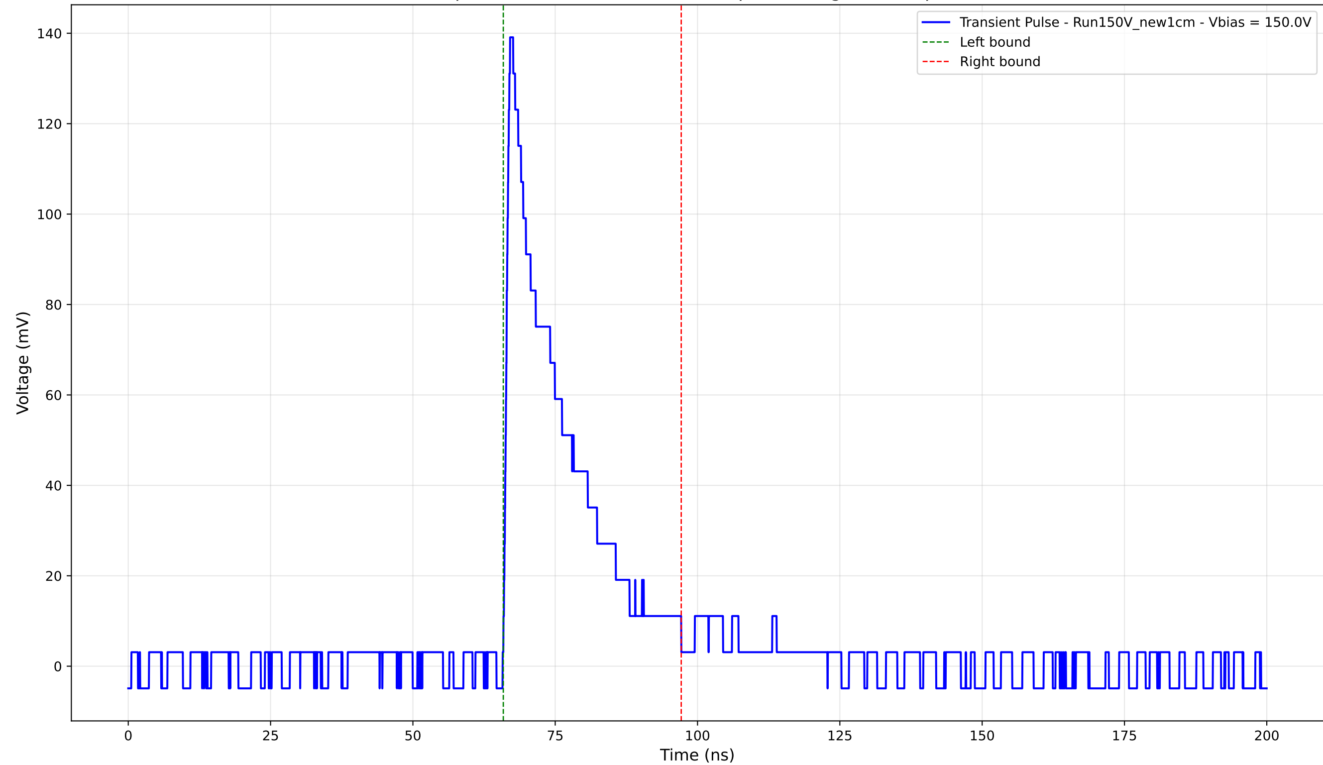
Transient Pulse - Sample: New1cm - Position: 270.0 \mu\text{m} - Charge: 27.90 pC - Rise Time: 0.95 ns
