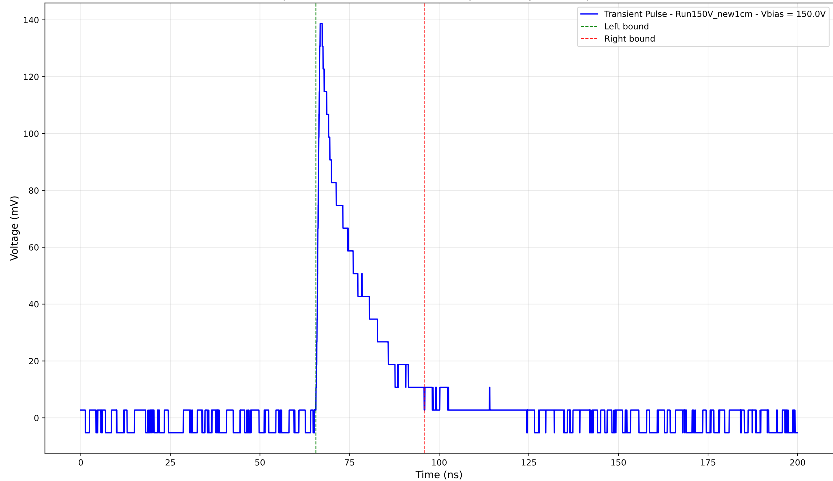
Transient Pulse - Sample: New1cm - Position: 4795.0 \mu\text{m} - Charge: 27.60 pC - Rise Time: 0.93 ns
