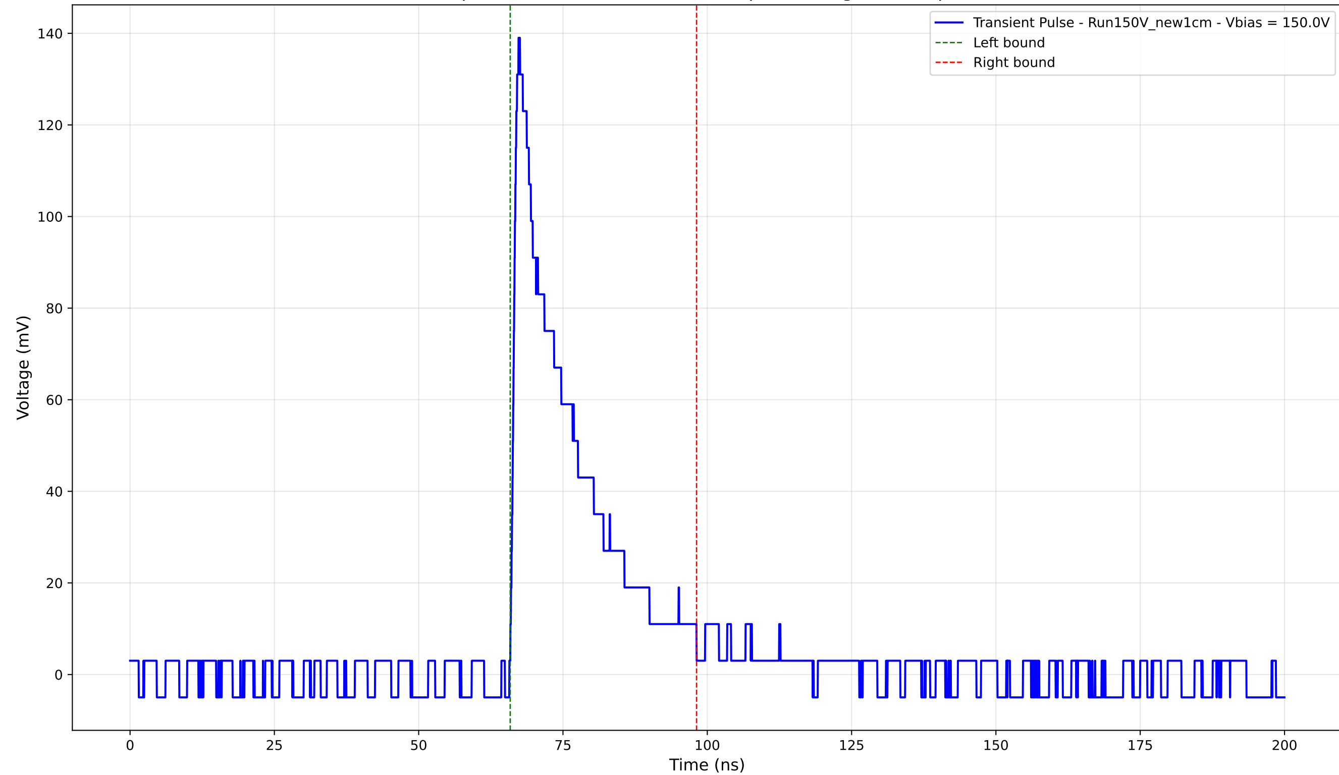
Transient Pulse - Sample: New1cm - Position: 295.0 \mu\text{m} - Charge: 28.09 pC - Rise Time: 1.07 ns
