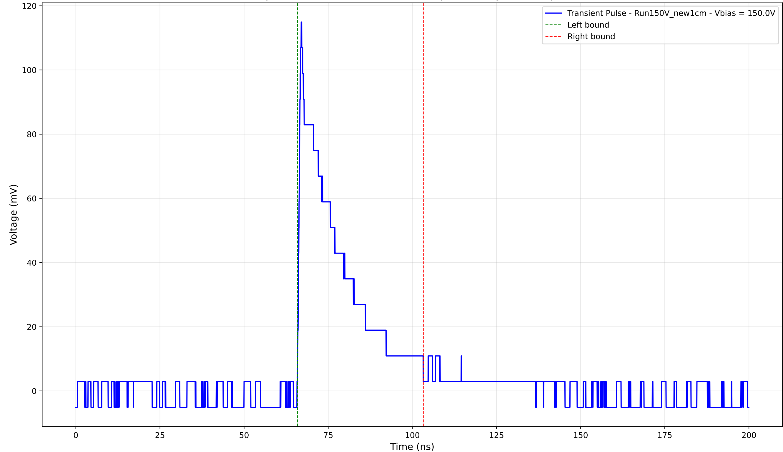
Transient Pulse - Sample: New1cm - Position: 2135.0 \mu\text{m} - Charge: 26.69 pC - Rise Time: 0.84 ns
