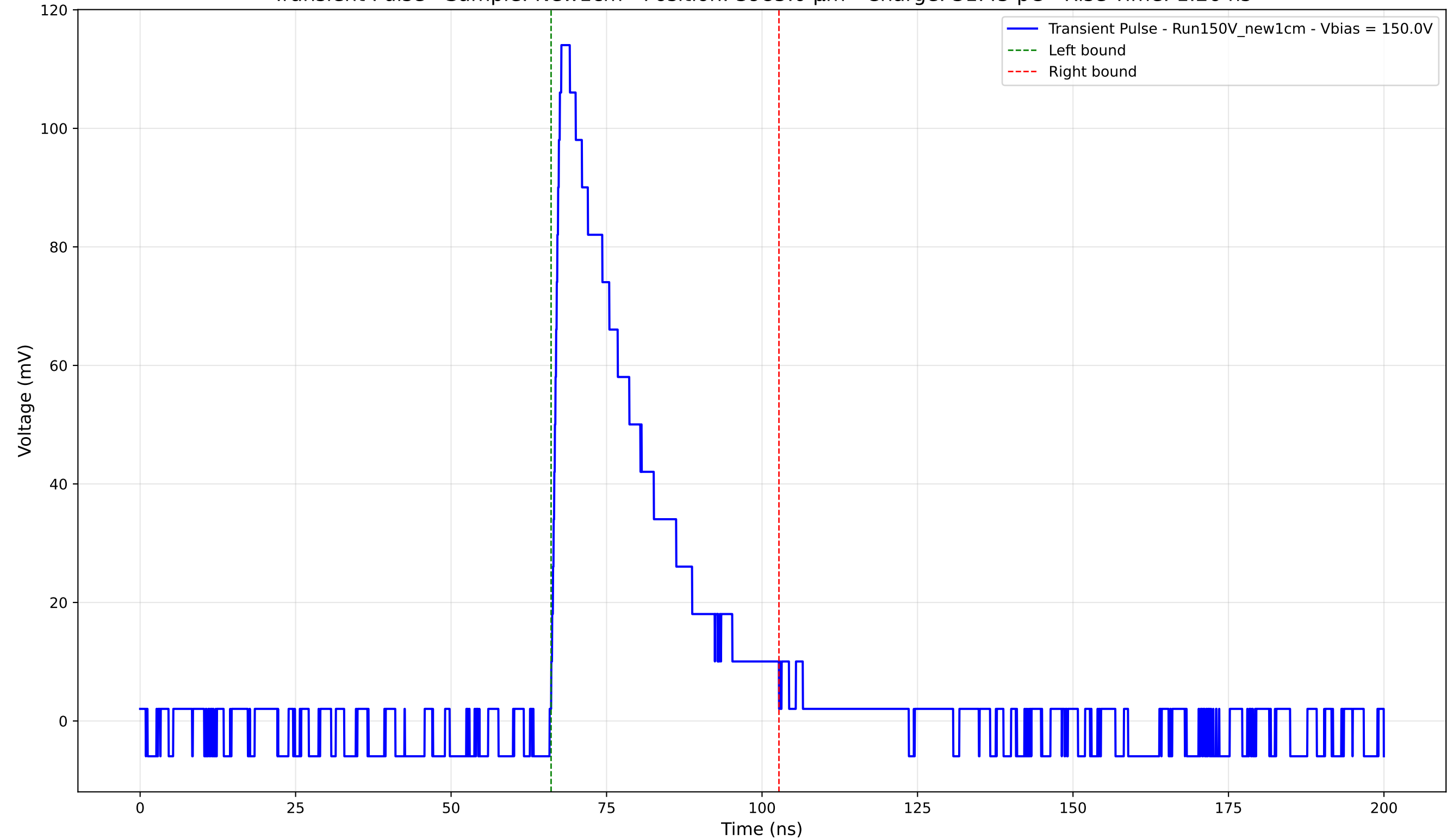
Transient Pulse - Sample: New1cm - Position: 3985.0 \mu\text{m} - Charge: 31.45 pC - Rise Time: 1.26 ns
