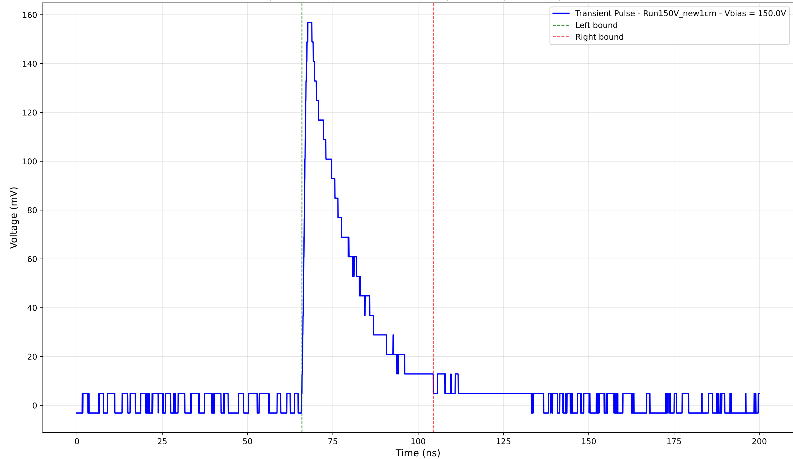
Transient Pulse - Sample: New1cm - Position: 4270.0 \mu\text{m} - Charge: 41.96 pC - Rise Time: 1.33 ns
