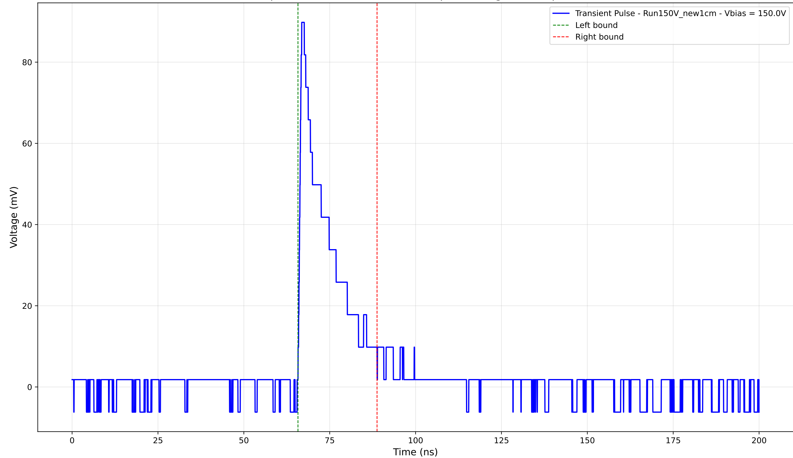
Transient Pulse - Sample: New1cm - Position: 105.0 \mu\text{m} - Charge: 15.50 pC - Rise Time: 0.90 ns
