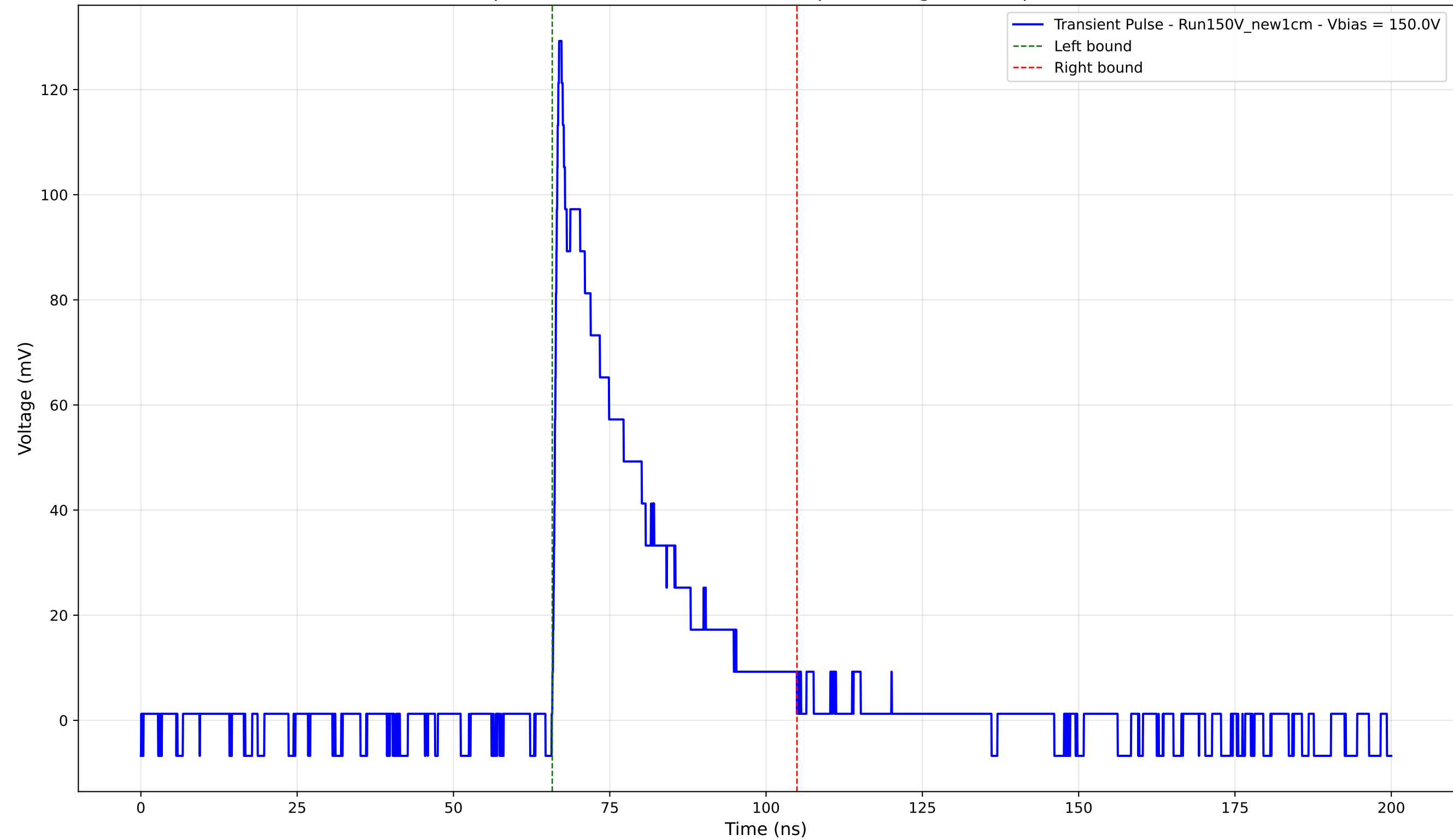
Transient Pulse - Sample: New1cm - Position: 2980.0 \mu\text{m} - Charge: 30.04 pC - Rise Time: 0.85 ns
