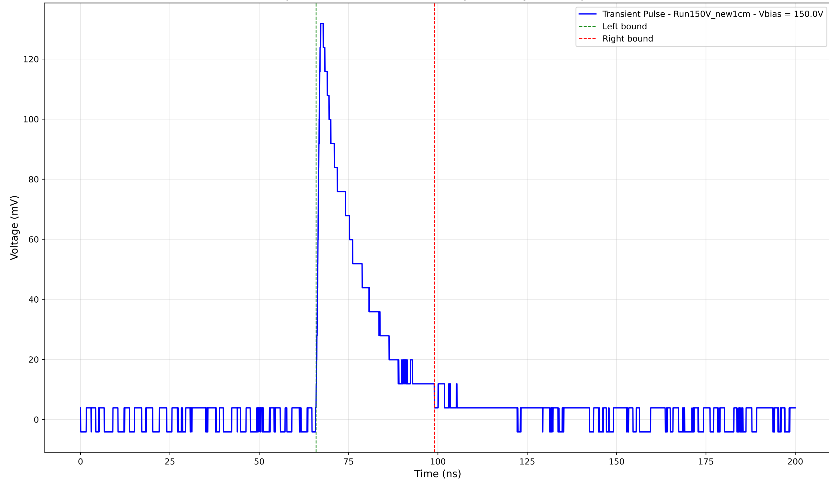
Transient Pulse - Sample: New1cm - Position: 360.0 \mu\text{m} - Charge: 29.45 pC - Rise Time: 1.00 ns
