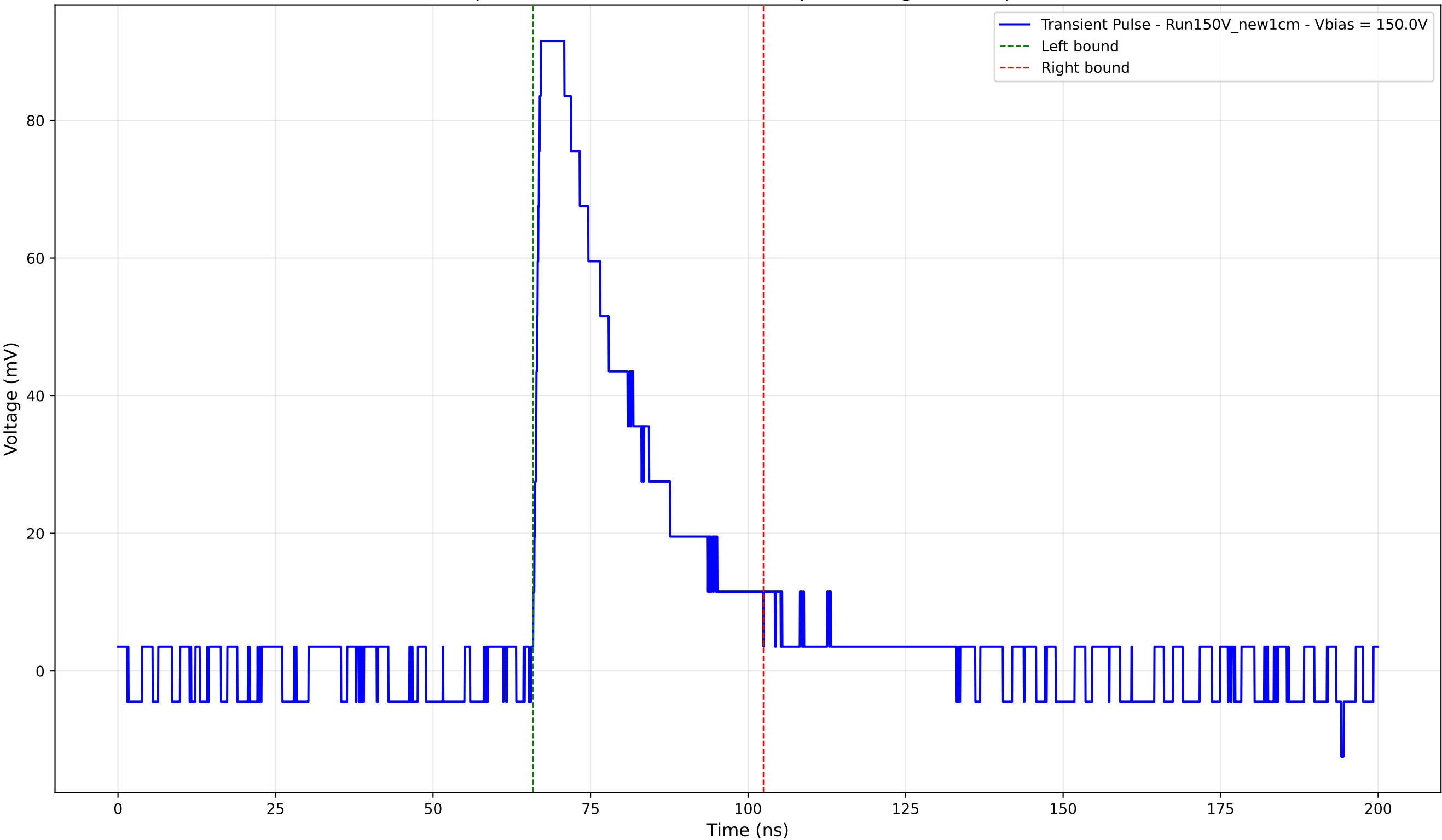
Transient Pulse - Sample: New1cm - Position: 1865.0 \mu\text{m} - Charge: 28.80 pC - Rise Time: 1.03 ns
