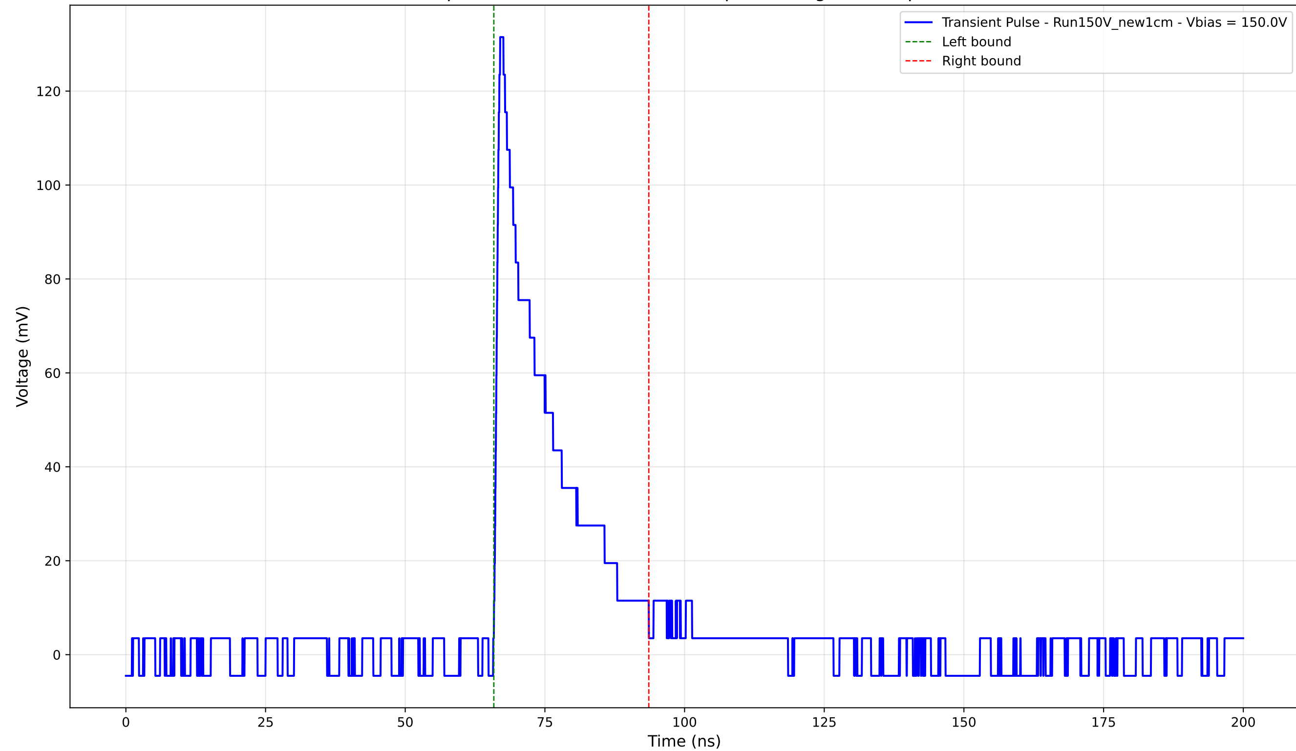
Transient Pulse - Sample: New1cm - Position: 185.0 \mu\text{m} - Charge: 24.71 pC - Rise Time: 0.88 ns
