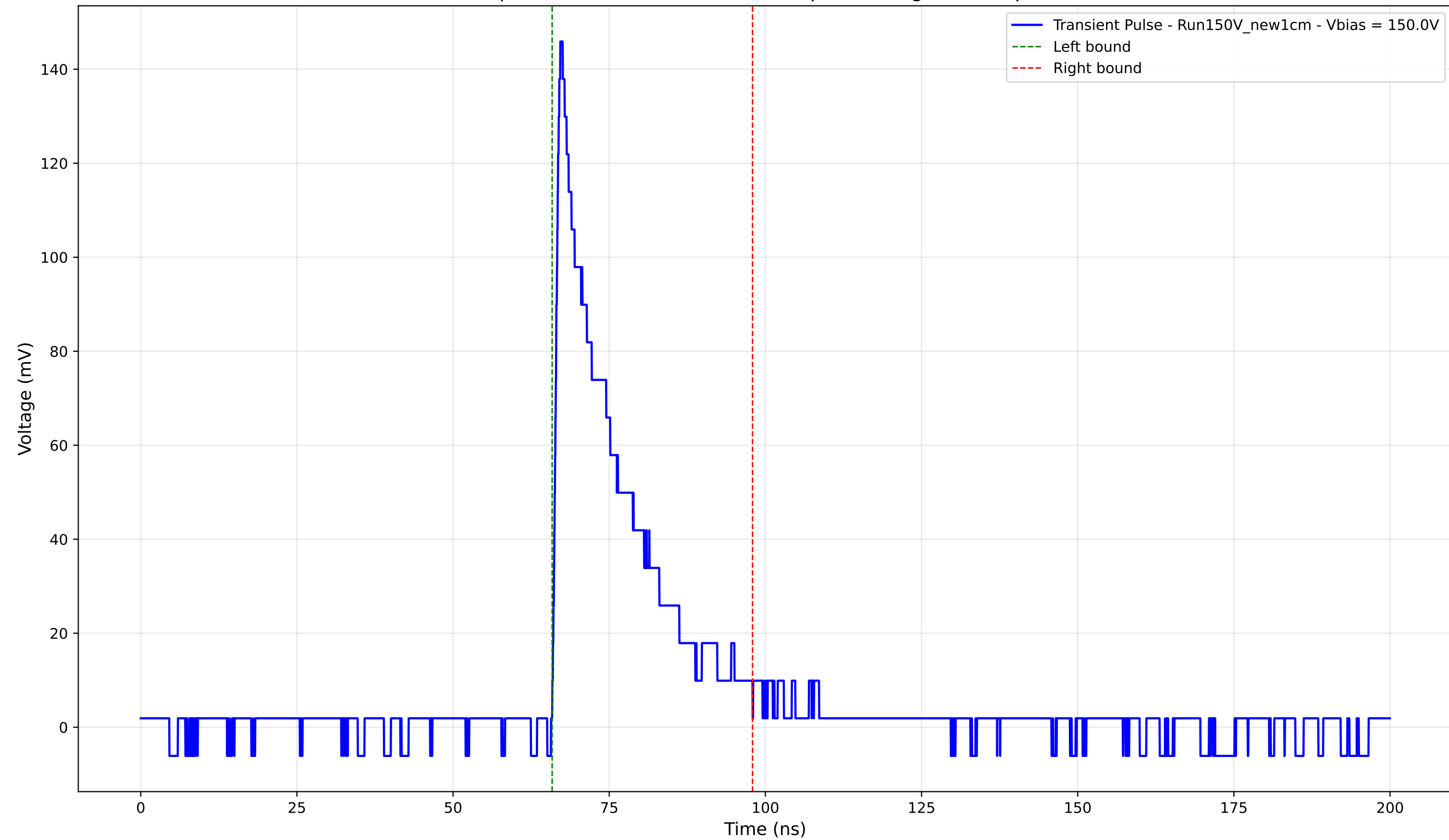
Transient Pulse - Sample: New1cm - Position: 280.0 \mu\text{m} - Charge: 28.85 pC - Rise Time: 1.03 ns
