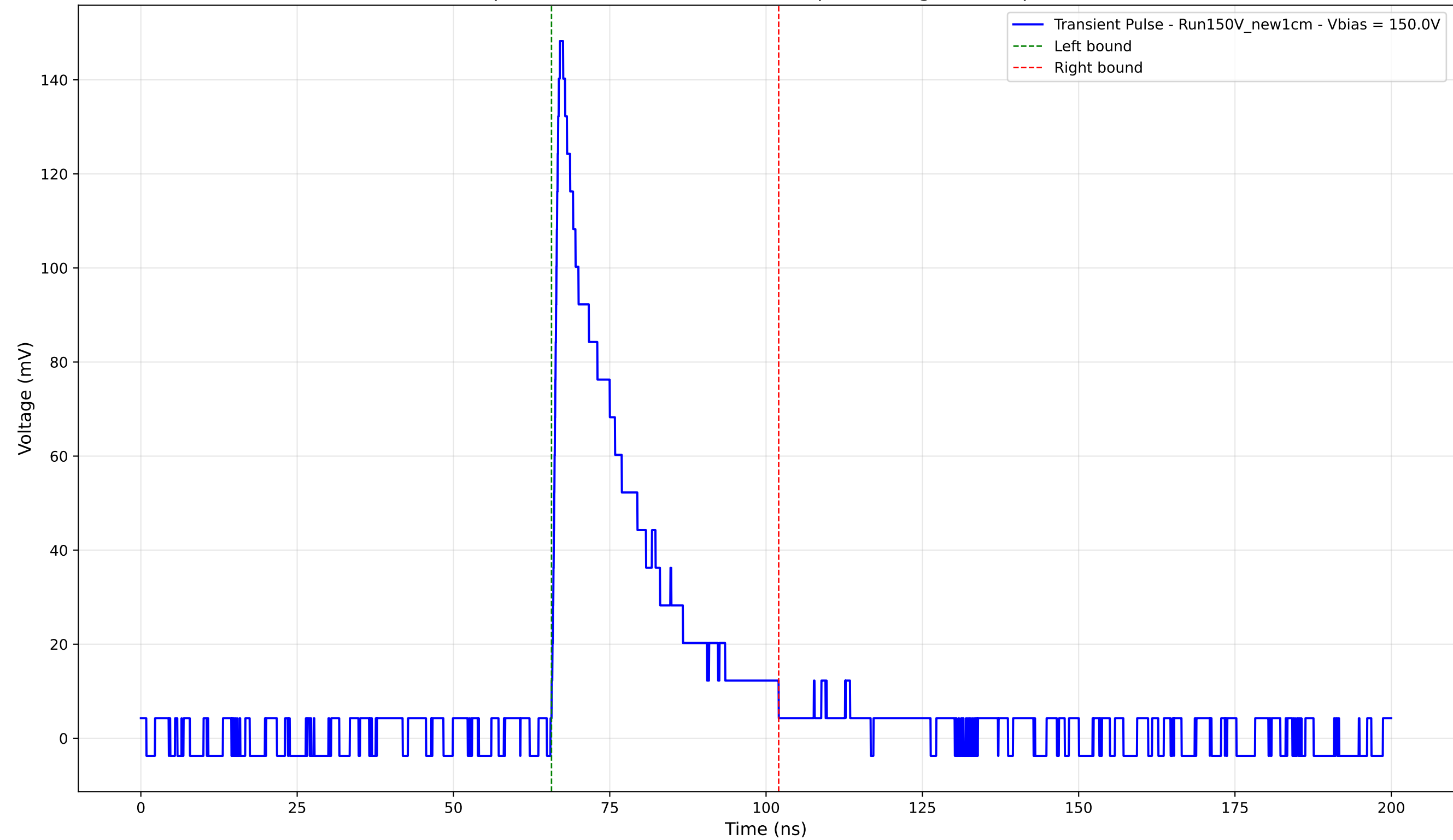
Transient Pulse - Sample: New1cm - Position: 4715.0 \mu\text{m} - Charge: 32.74 pC - Rise Time: 1.03 ns
