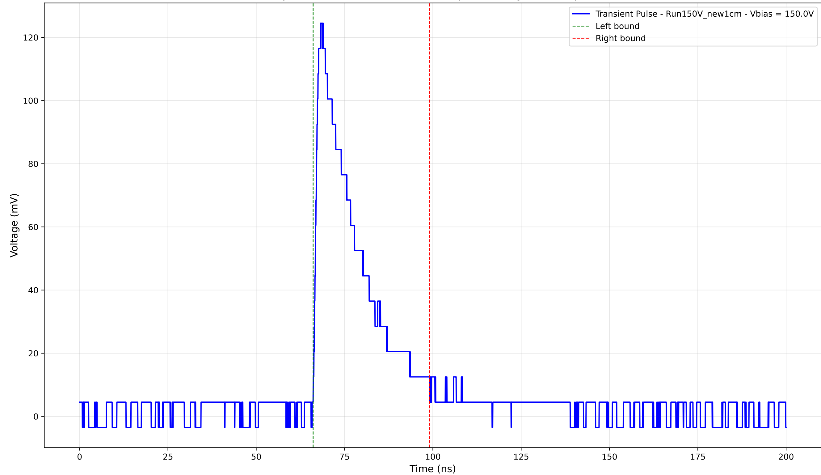
Transient Pulse - Sample: New1cm - Position: 805.0 \mu\text{m} - Charge: 31.52 pC - Rise Time: 1.56 ns
