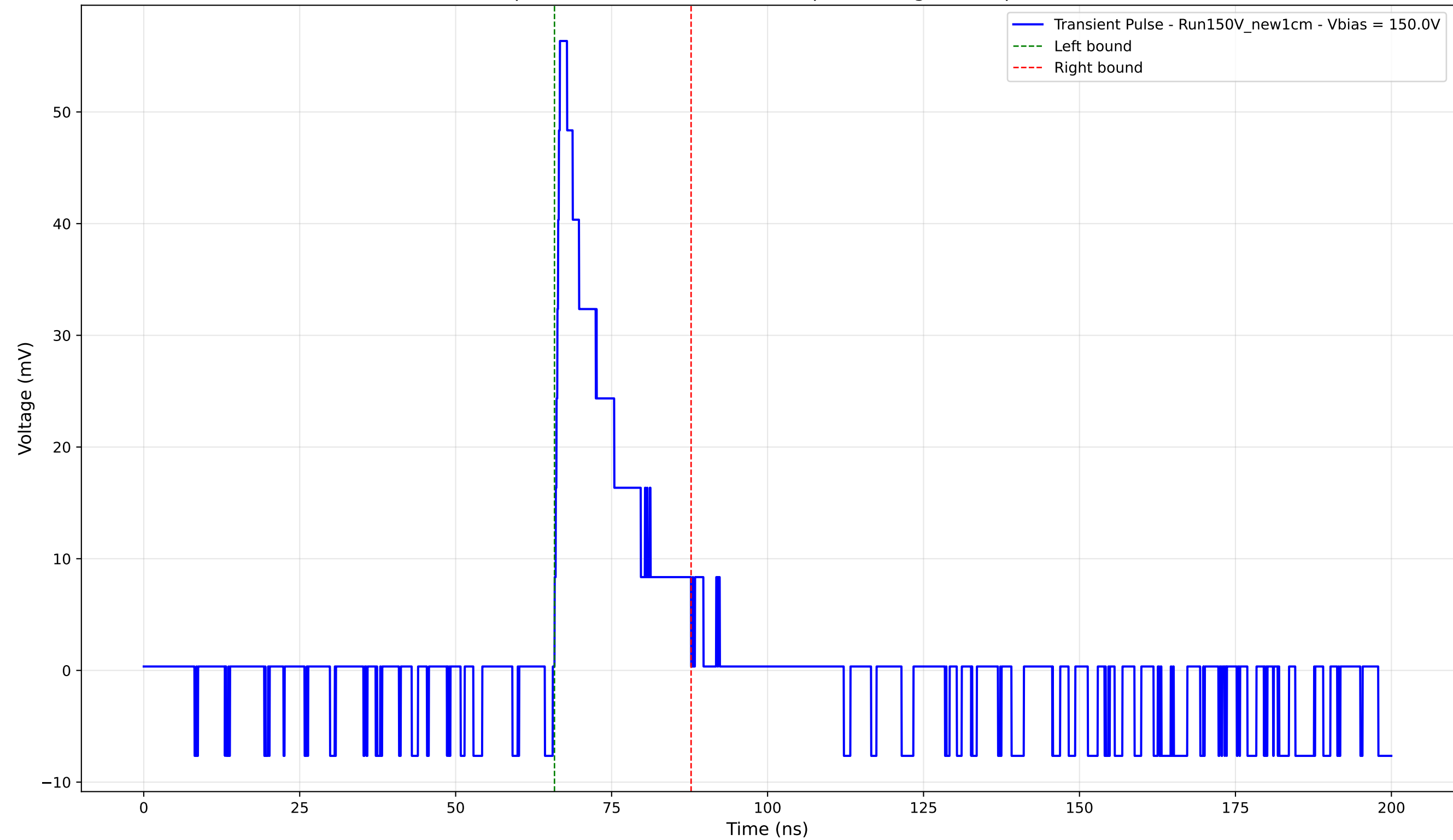
Transient Pulse - Sample: New1cm - Position: 80.0 \mu\text{m} - Charge: 9.44 pC - Rise Time: 0.85 ns
