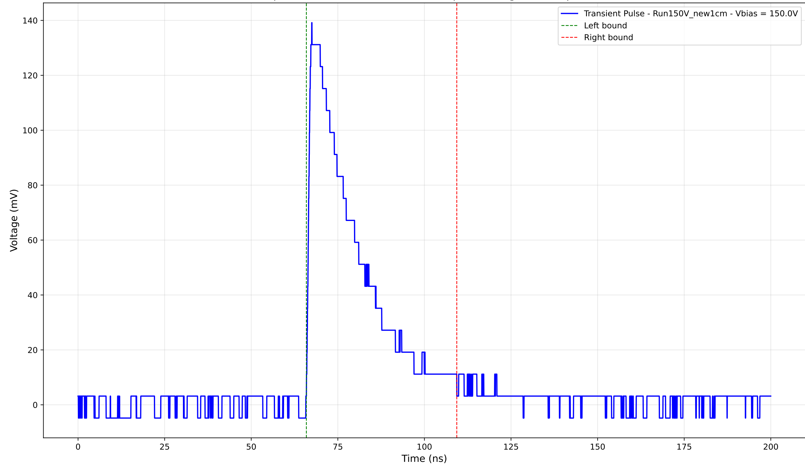
Transient Pulse - Sample: New1cm - Position: 3285.0 \mu\text{m} - Charge: 41.16 pC - Rise Time: 1.15 ns
