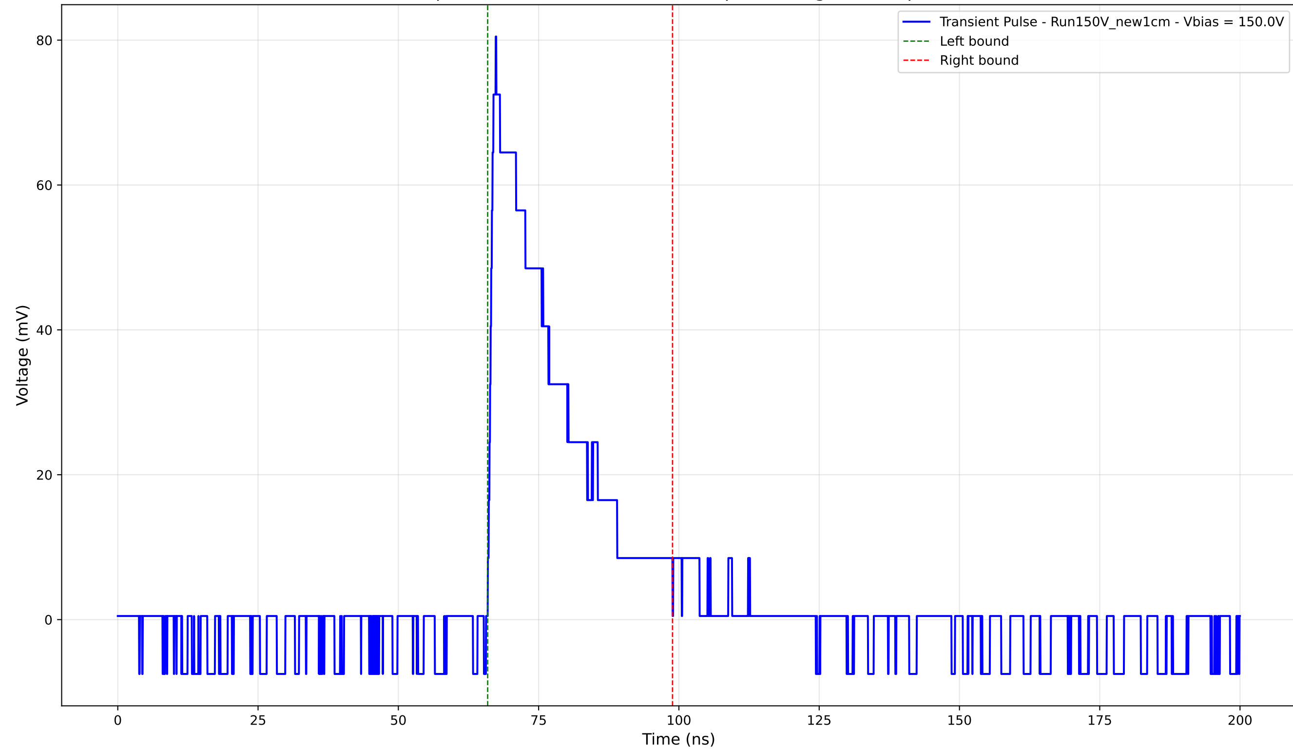
Transient Pulse - Sample: New1cm - Position: 3115.0 \mu\text{m} - Charge: 19.37 pC - Rise Time: 1.00 ns
