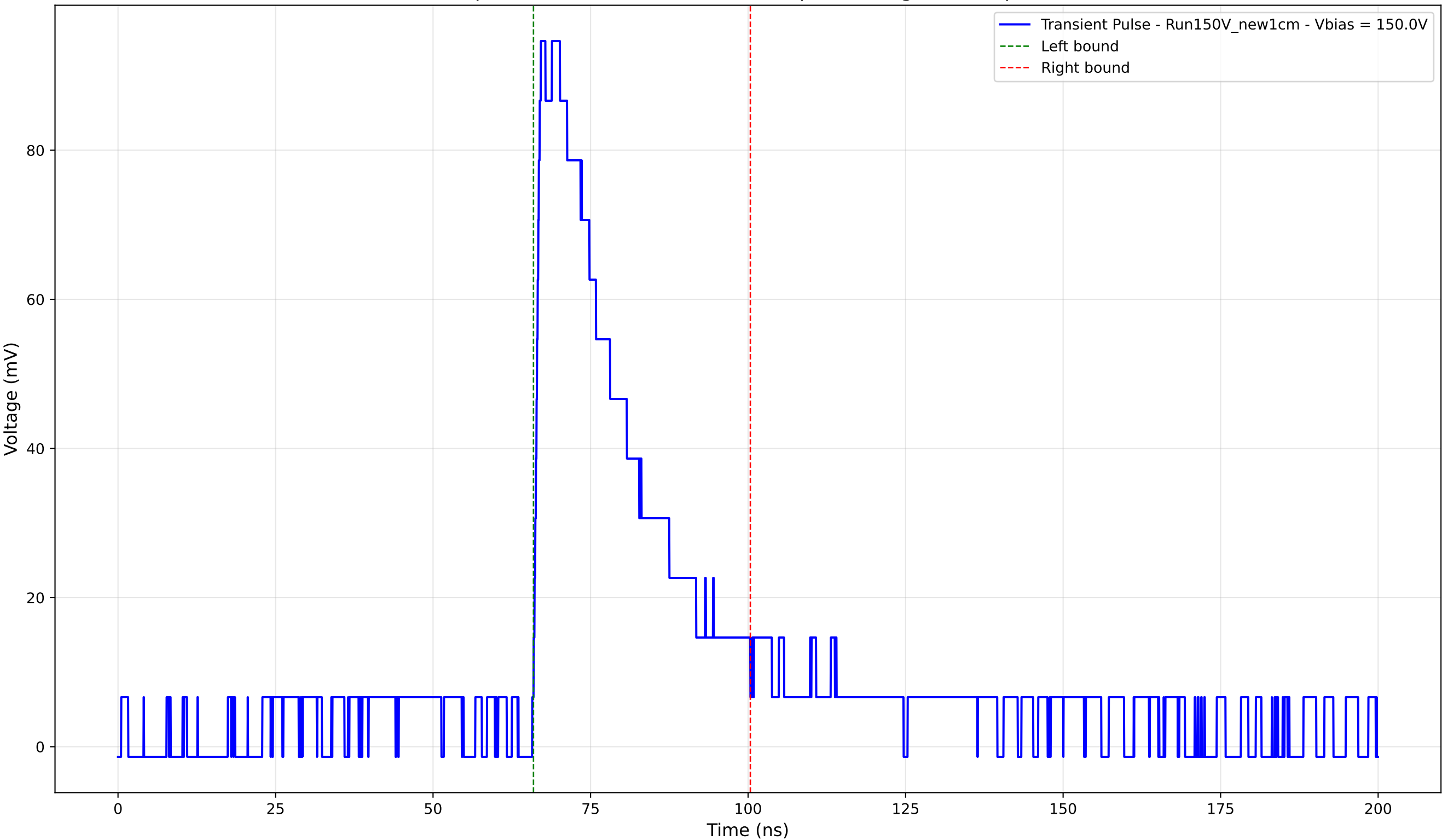
Transient Pulse - Sample: New1cm - Position: 1875.0 \mu\text{m} - Charge: 29.29 pC - Rise Time: 0.97 ns
