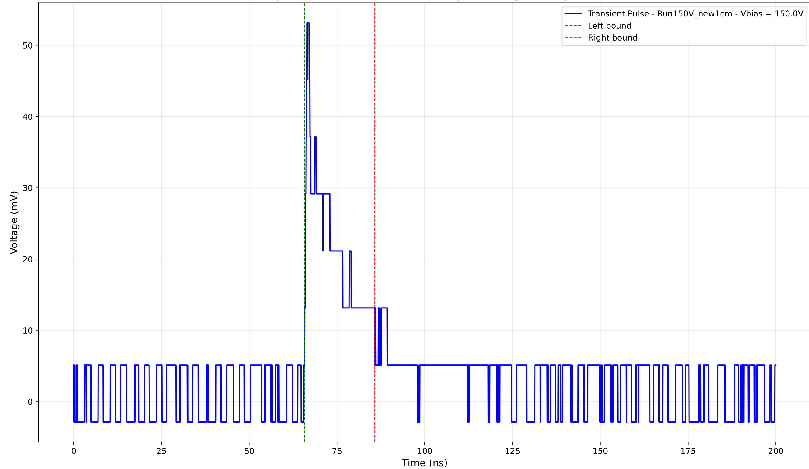
Transient Pulse - Sample: New1cm - Position: 2580.0 \mu\text{m} - Charge: 8.68 pC - Rise Time: 0.72 ns
