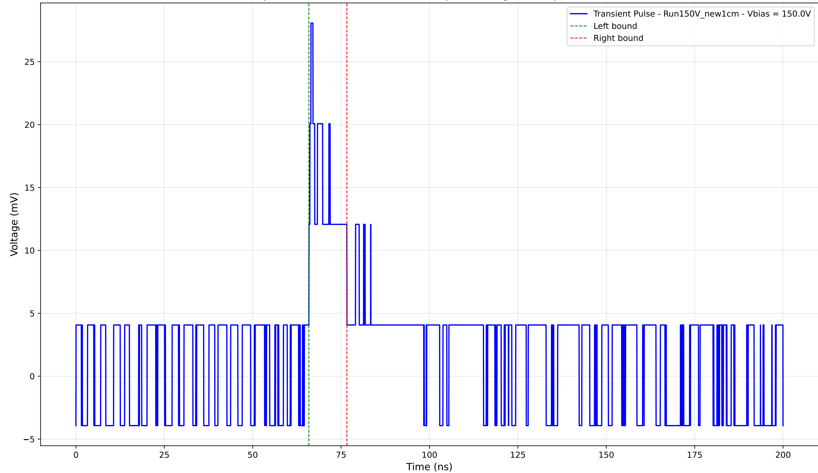
Transient Pulse - Sample: New1cm - Position: 2545.0 \mu\text{m} - Charge: 3.20 pC - Rise Time: 0.00 ns (N/A)
