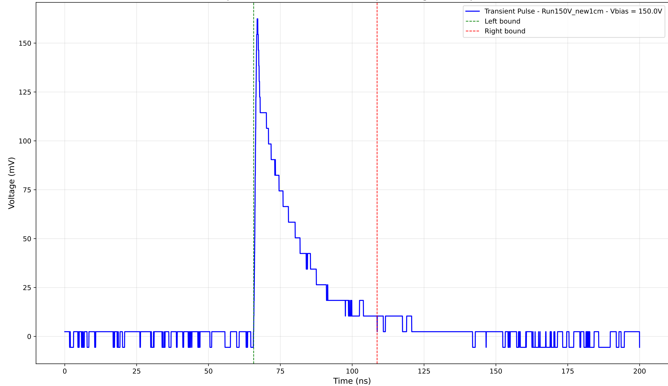
Transient Pulse - Sample: New1cm - Position: 2925.0 \mu\text{m} - Charge: 38.67 pC - Rise Time: 0.87 ns
