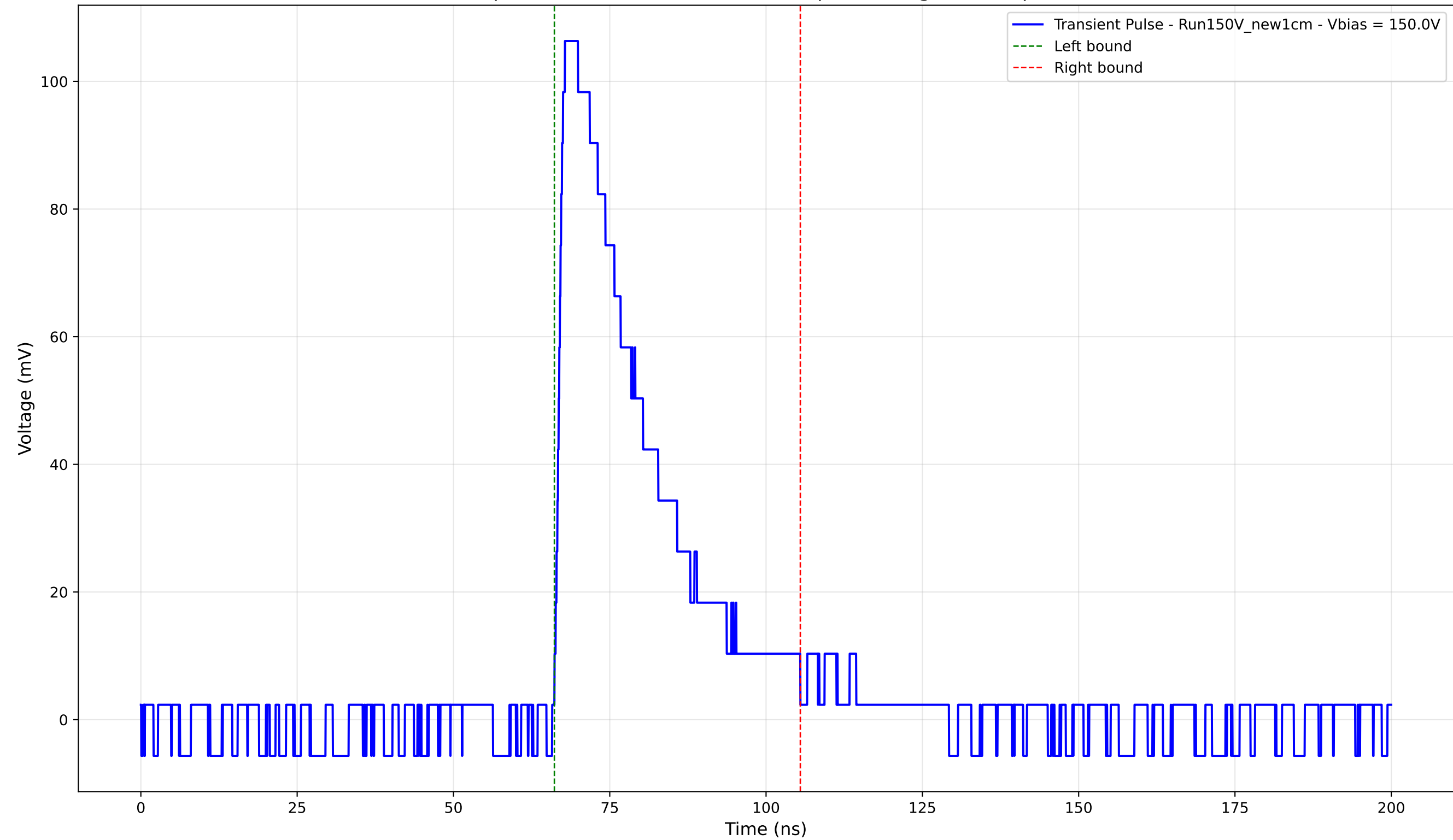
Transient Pulse - Sample: New1cm - Position: 1395.0 \mu\text{m} - Charge: 31.70 pC - Rise Time: 1.20 ns
