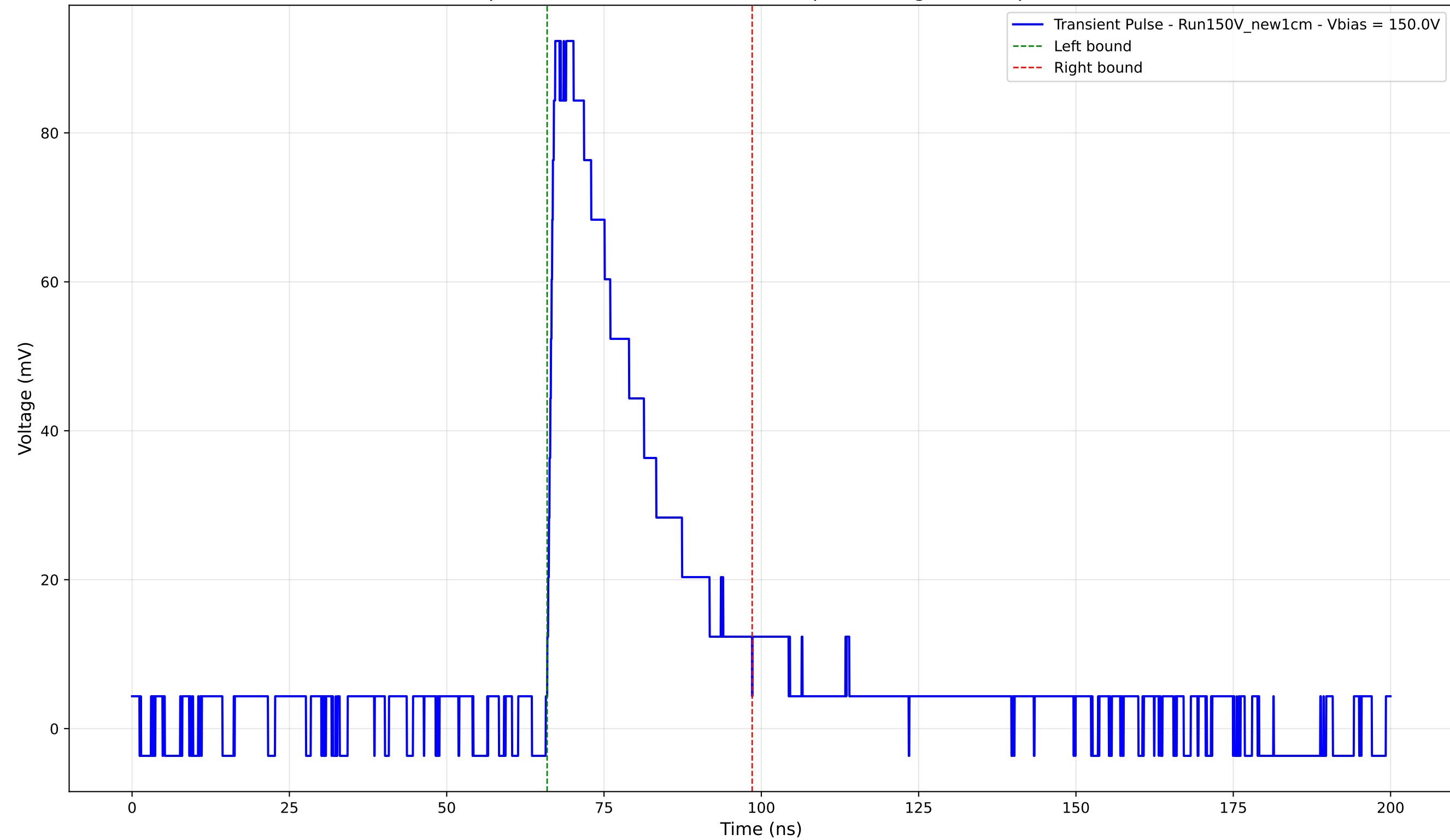
Transient Pulse - Sample: New1cm - Position: 1800.0 \mu\text{m} - Charge: 27.55 pC - Rise Time: 1.05 ns
