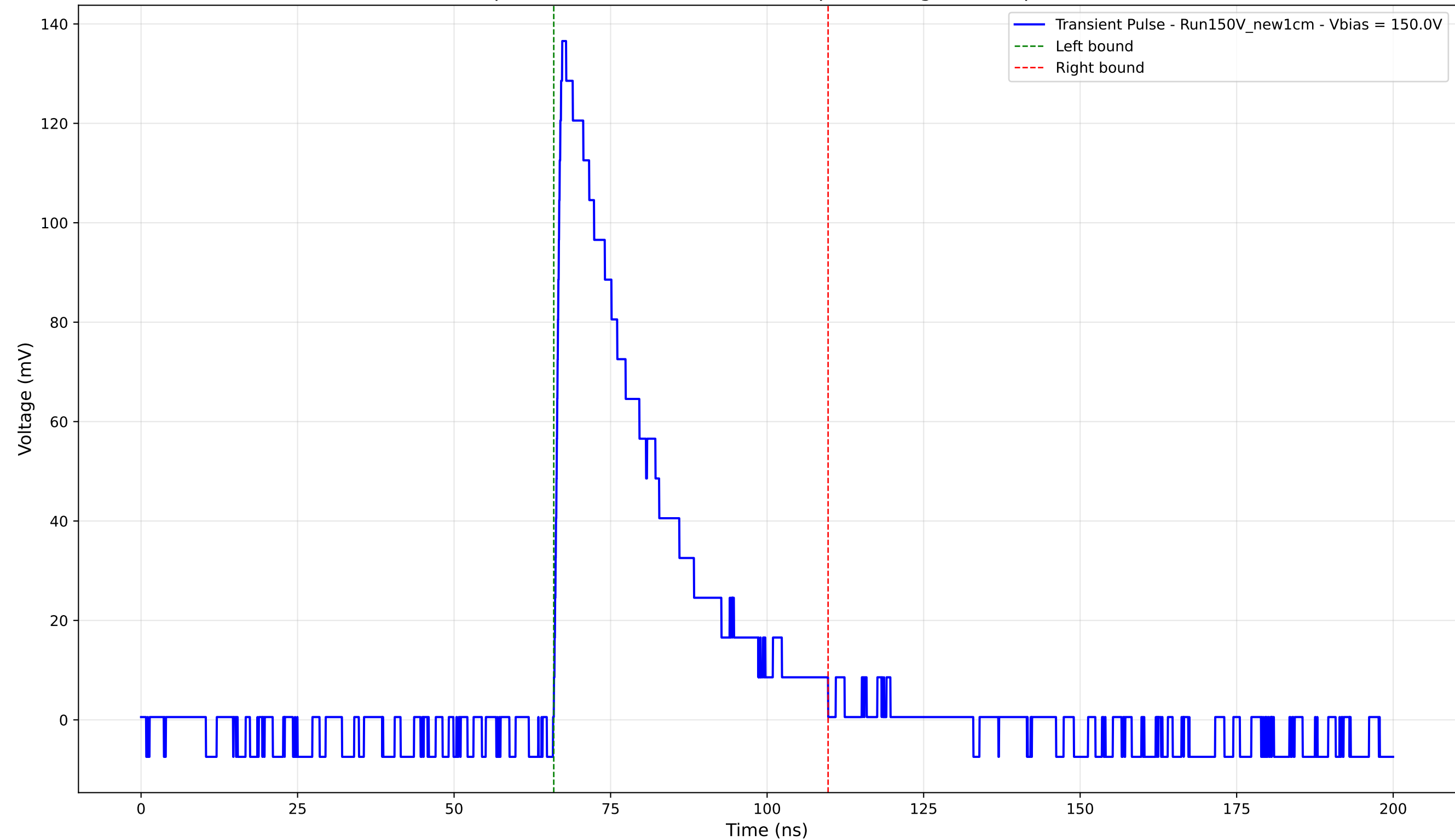
Transient Pulse - Sample: New1cm - Position: 3250.0 \mu\text{m} - Charge: 39.68 pC - Rise Time: 1.05 ns
