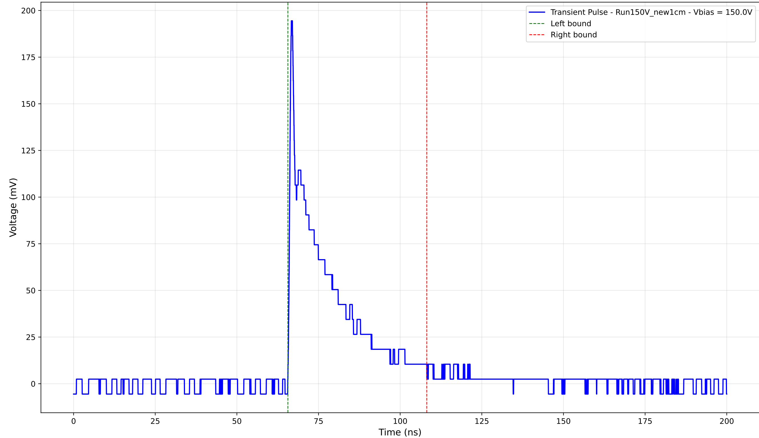
Transient Pulse - Sample: New1cm - Position: 2725.0 \mu\text{m} - Charge: 37.83 pC - Rise Time: 0.74 ns
