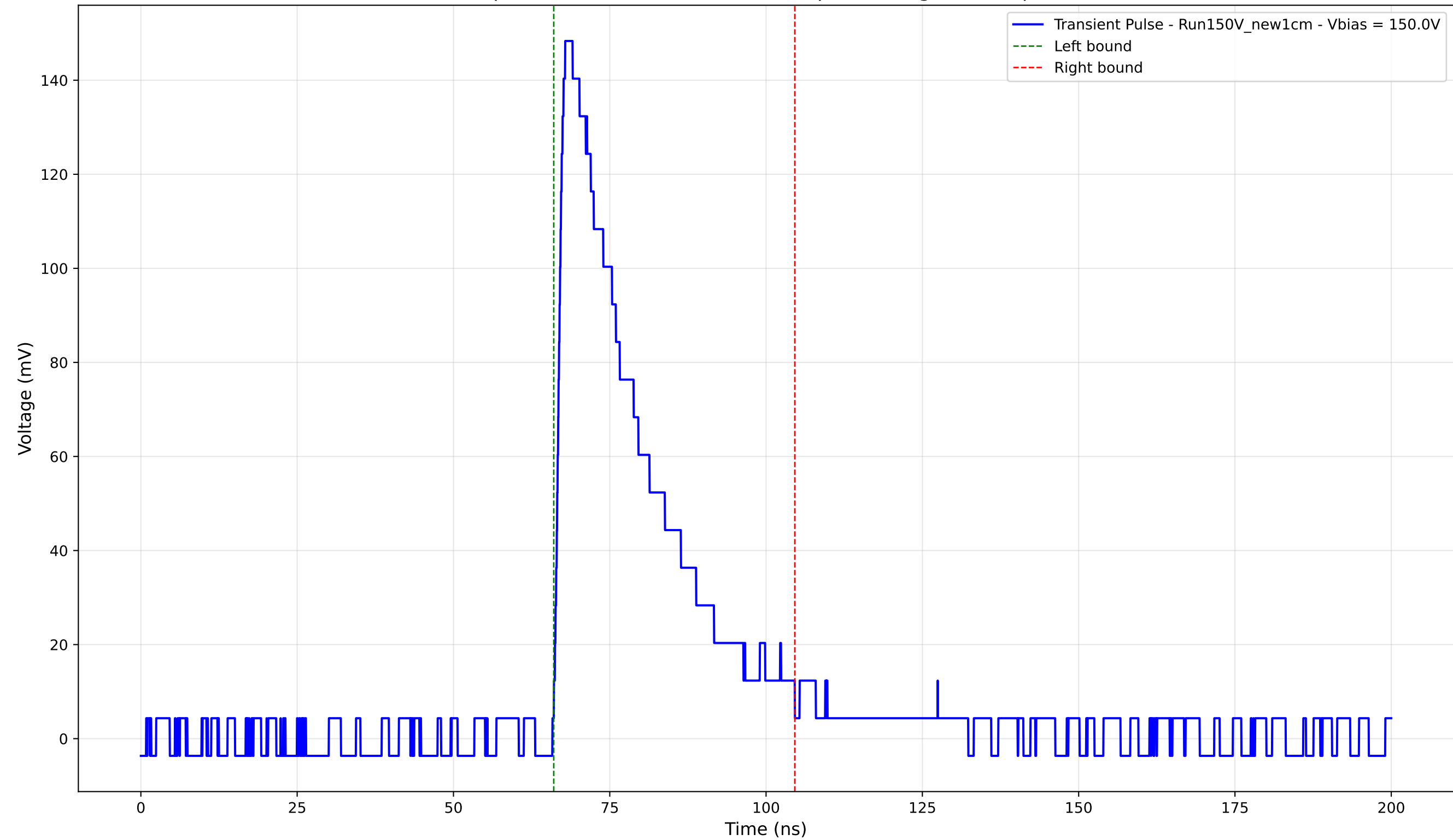
Transient Pulse - Sample: New1cm - Position: 3825.0 \mu\text{m} - Charge: 42.66 pC - Rise Time: 1.39 ns
