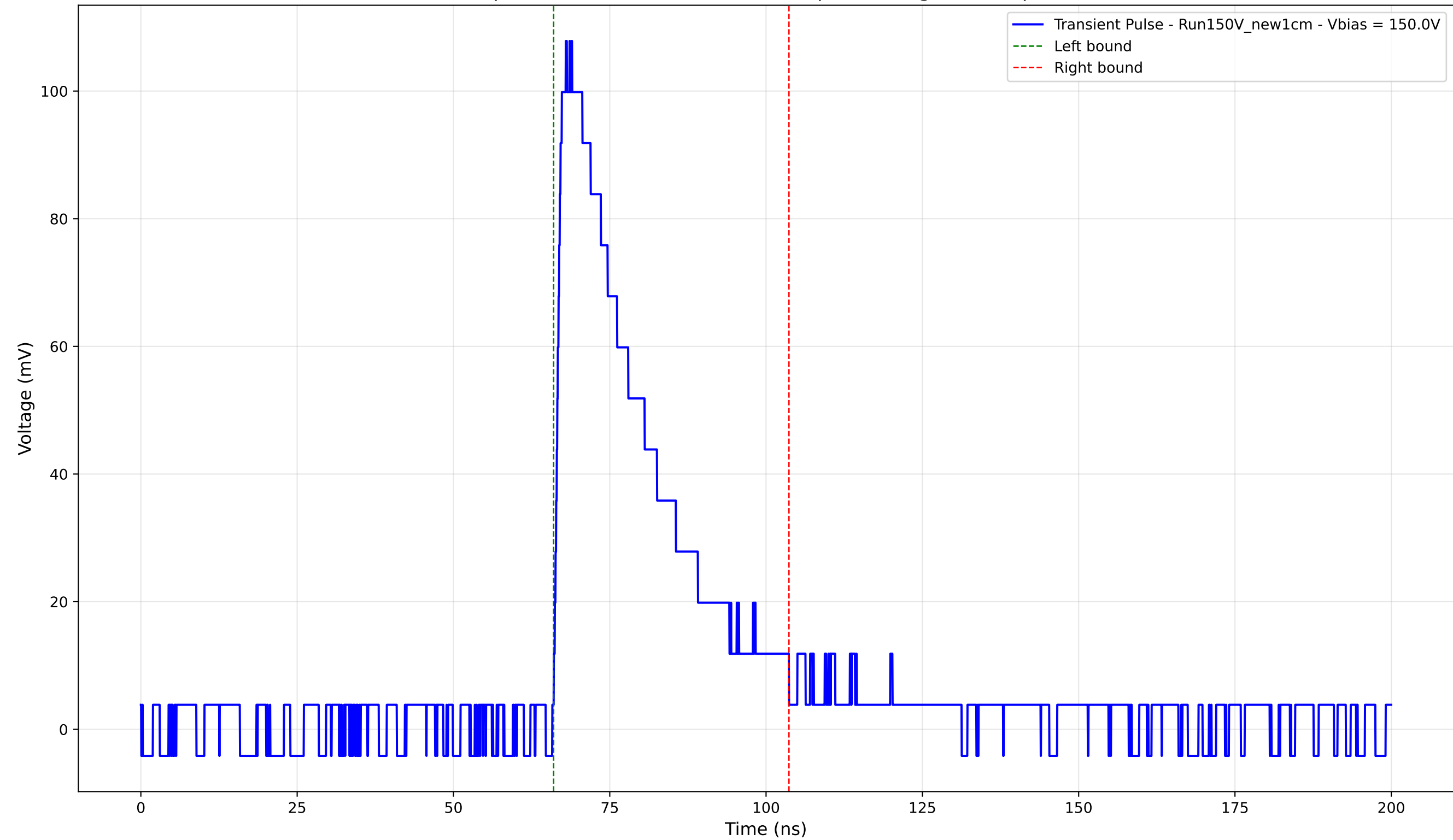
Transient Pulse - Sample: New1cm - Position: 1705.0 \mu\text{m} - Charge: 31.95 pC - Rise Time: 1.28 ns
