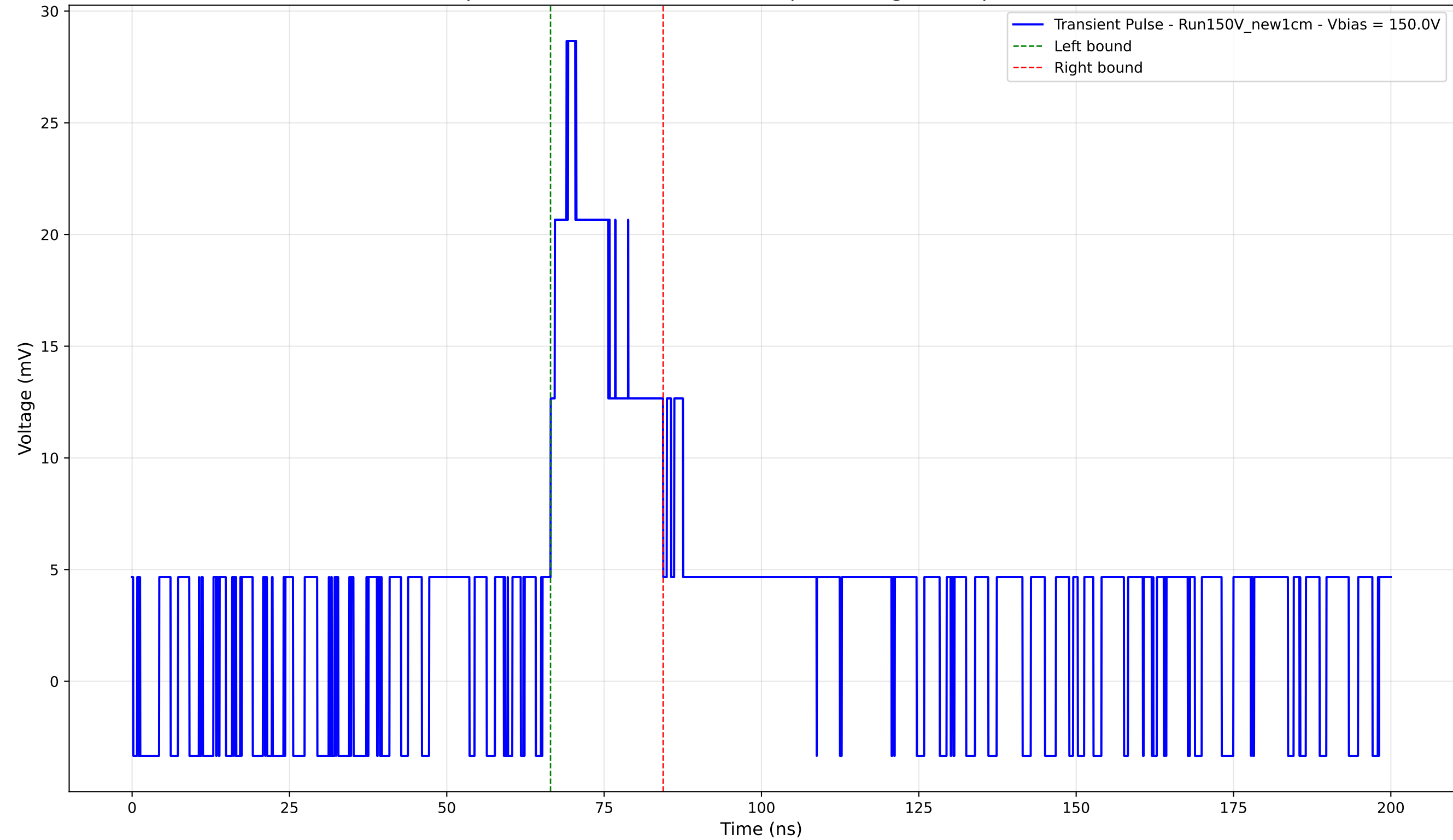
Transient Pulse - Sample: New1cm - Position: 1015.0 \mu\text{m} - Charge: 6.14 pC - Rise Time: 0.00 ns (N/A)
