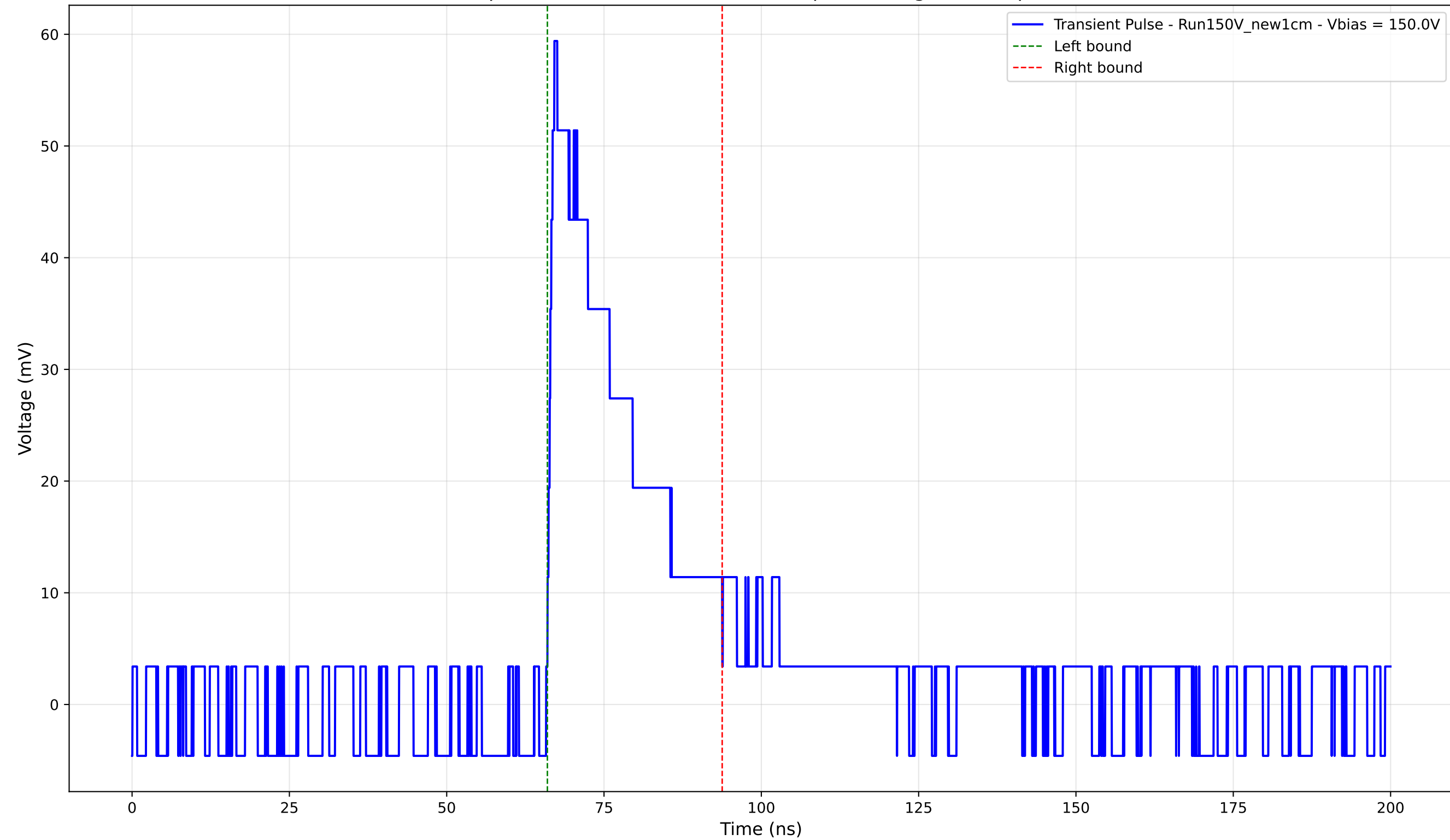
Transient Pulse - Sample: New1cm - Position: 1985.0 \mu\text{m} - Charge: 14.54 pC - Rise Time: 1.09 ns
