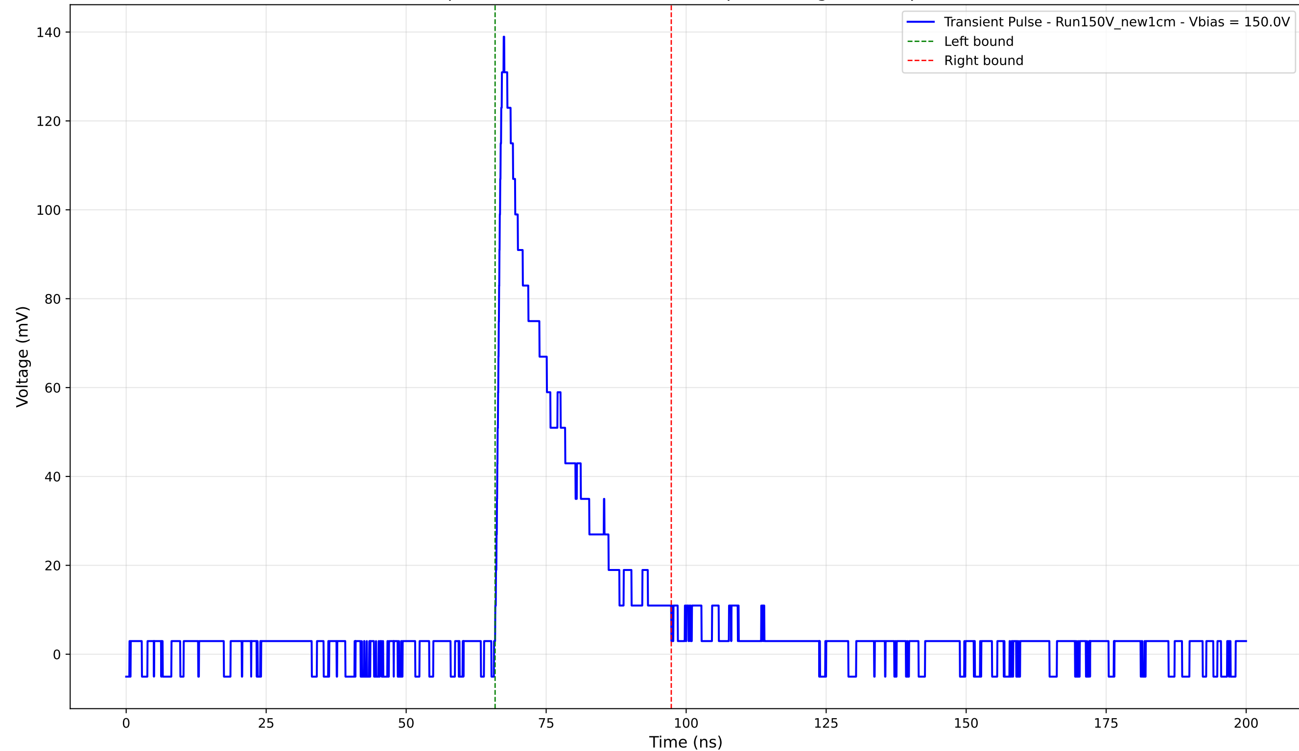
Transient Pulse - Sample: New1cm - Position: 315.0 \mu\text{m} - Charge: 28.34 pC - Rise Time: 1.07 ns
