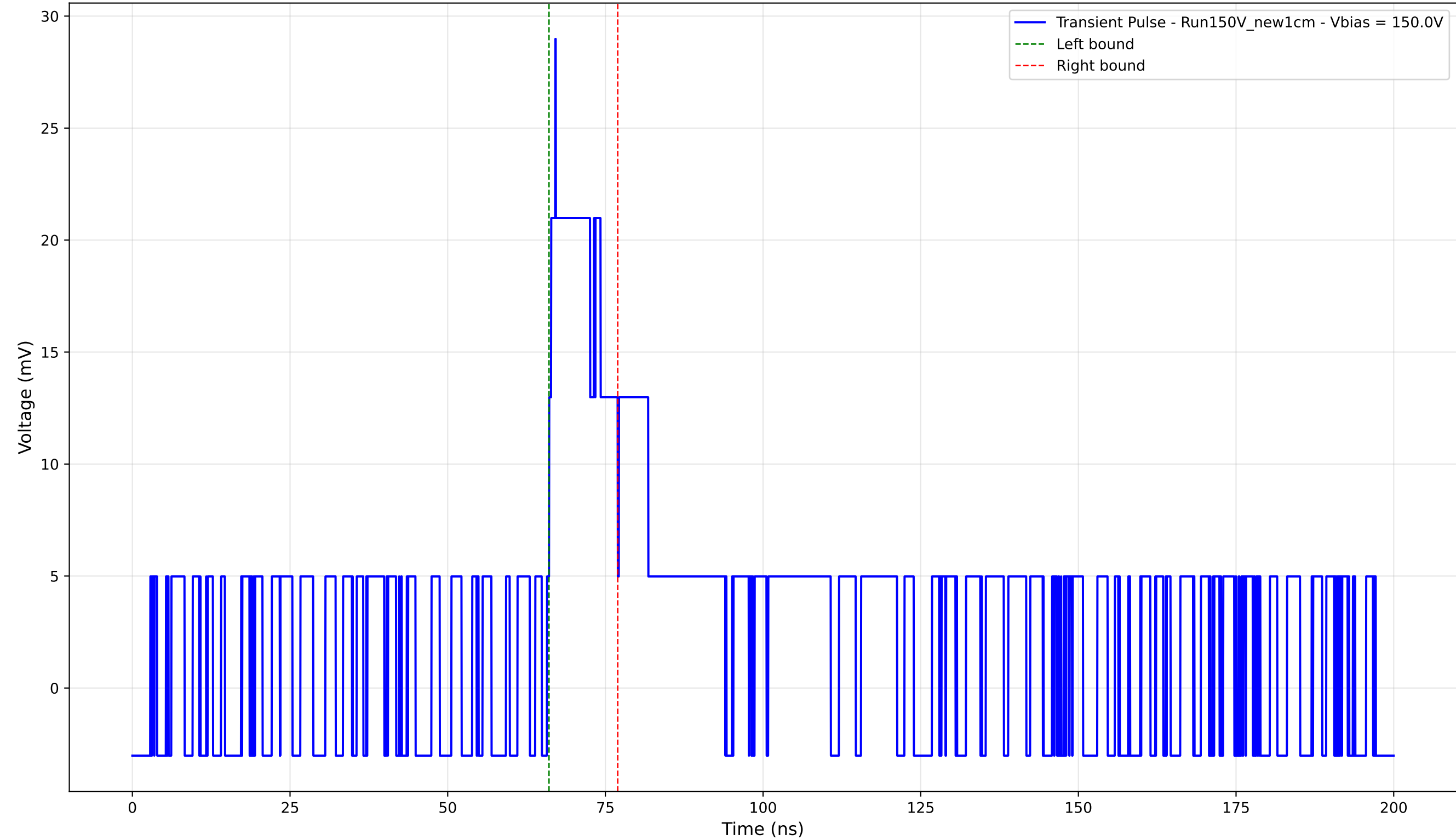
Transient Pulse - Sample: New1cm - Position: 2055.0 \mu\text{m} - Charge: 3.99 pC - Rise Time: 0.00 ns (N/A)
