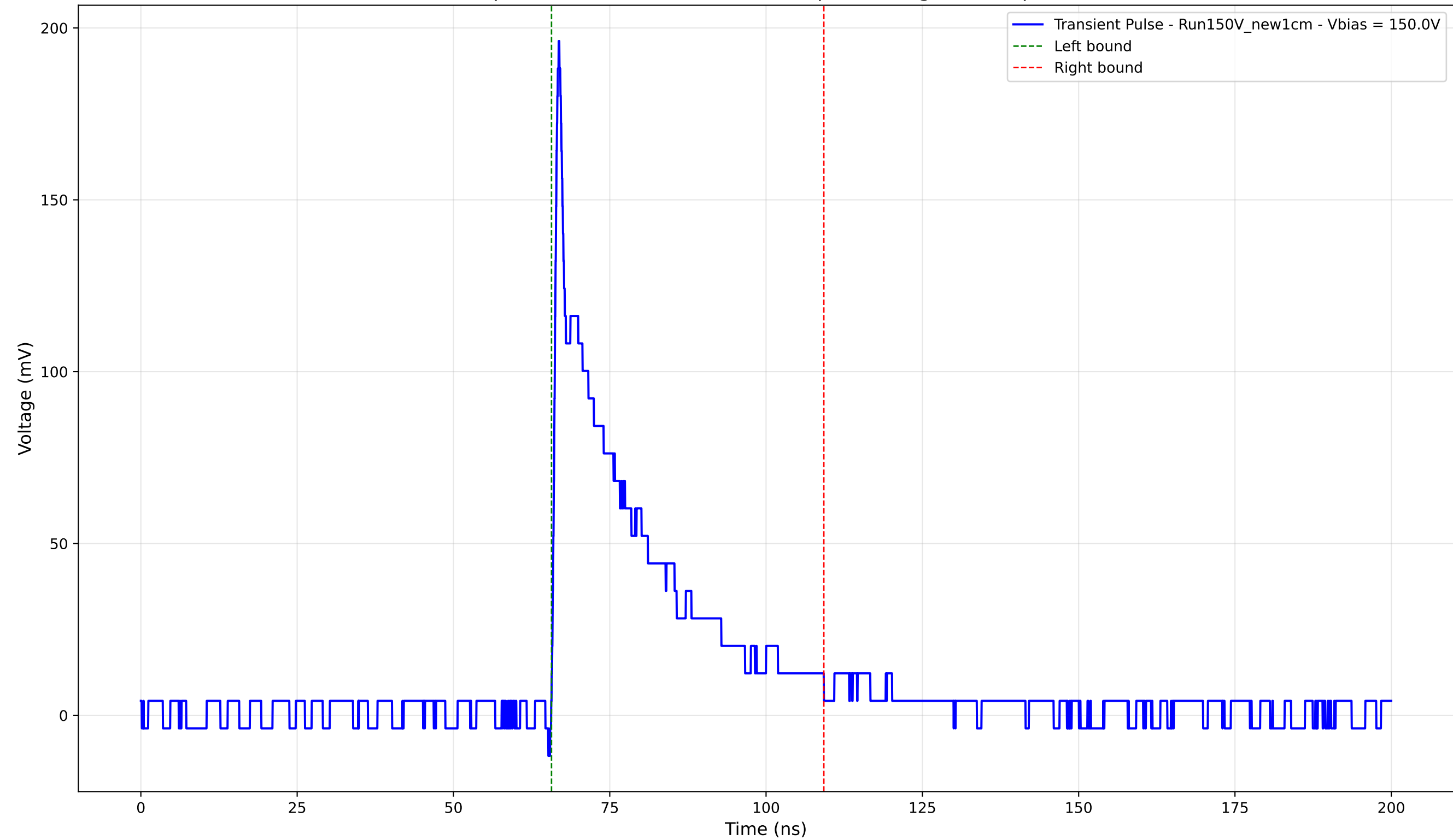
Transient Pulse - Sample: New1cm - Position: 2775.0 \mu\text{m} - Charge: 40.26 pC - Rise Time: 0.82 ns
