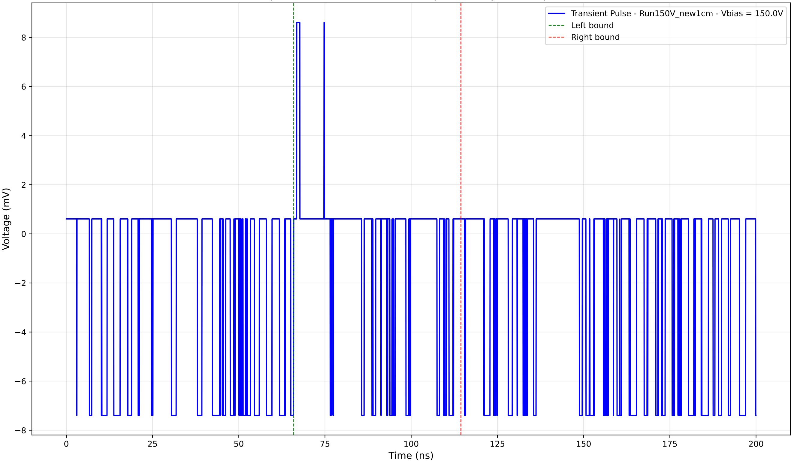
Transient Pulse - Sample: New1cm - Position:15.0 \mu\text{m} - Charge: -0.38 pC - Rise Time: 0.02 ns
