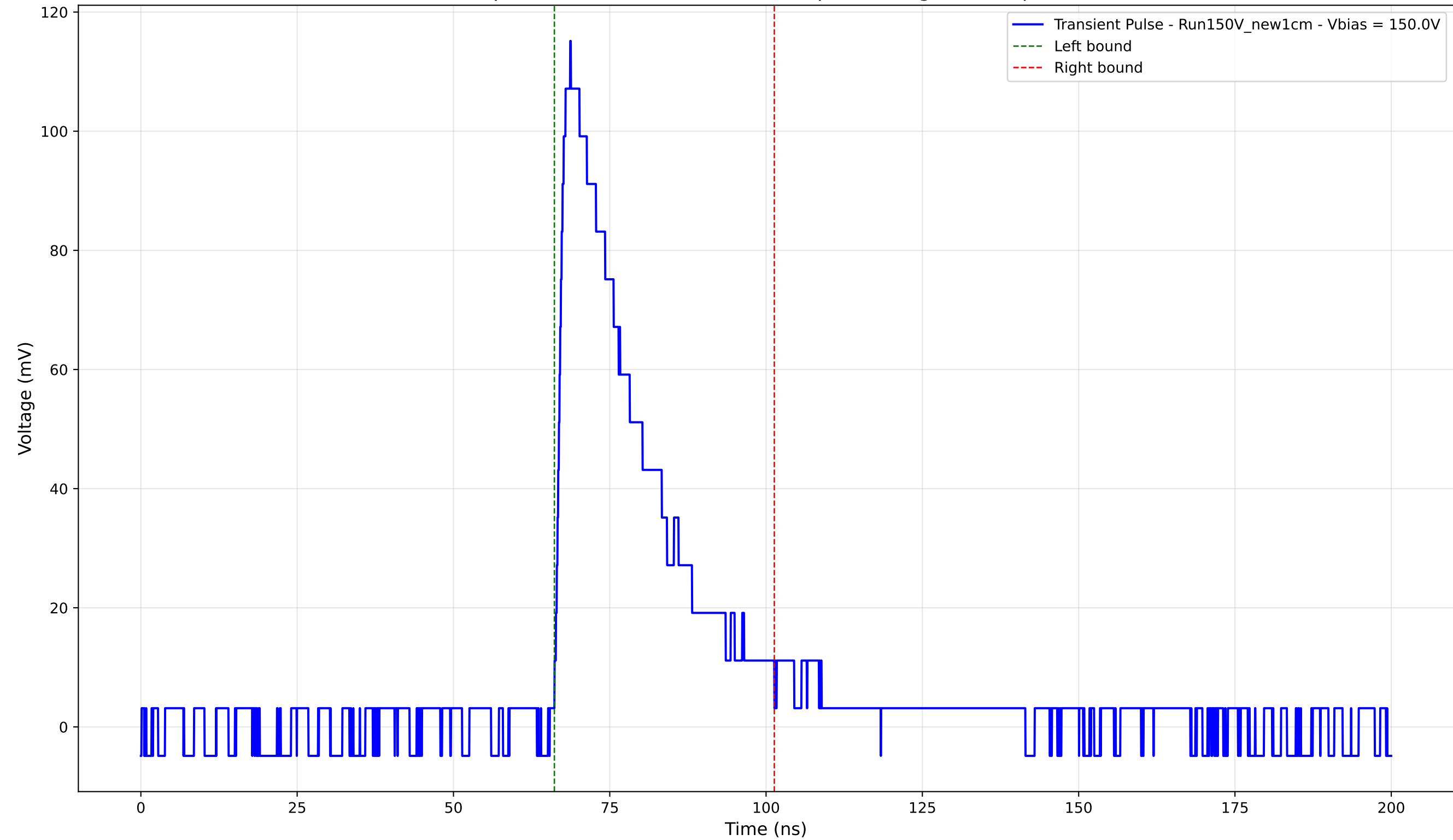
Transient Pulse - Sample: New1cm - Position: 1170.0 \mu\text{m} - Charge: 31.12 pC - Rise Time: 1.56 ns
