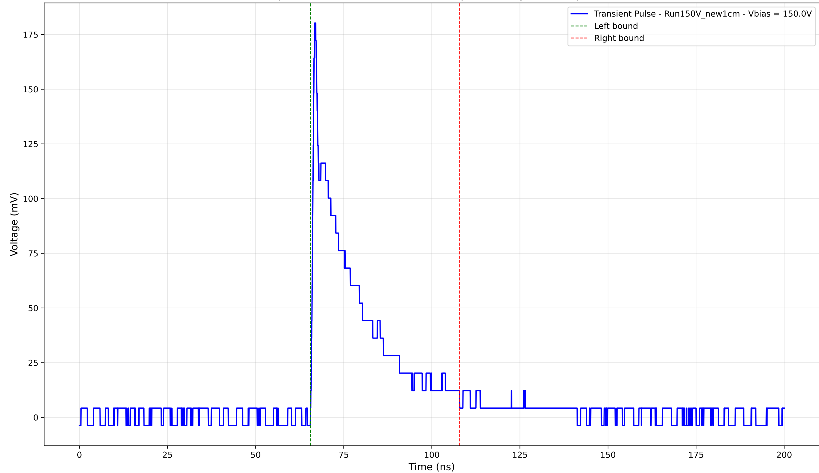
Transient Pulse - Sample: New1cm - Position: 2815.0 \mu\text{m} - Charge: 38.79 pC - Rise Time: 0.83 ns
