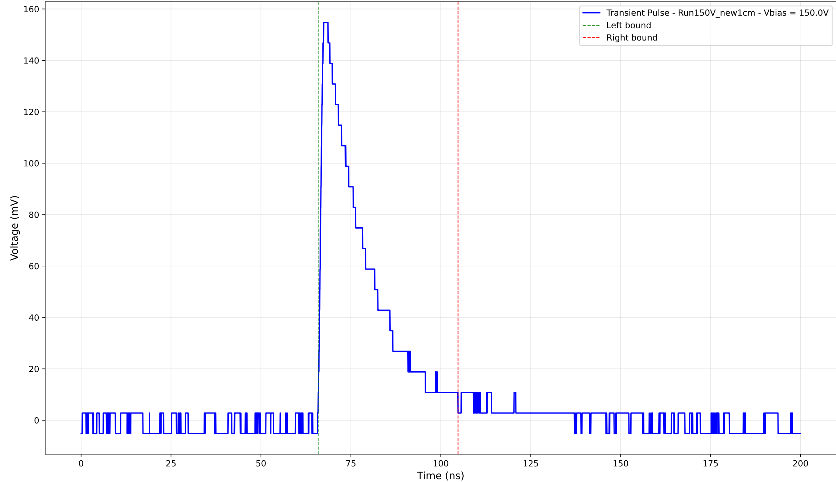
Transient Pulse - Sample: New1cm - Position: 4340.0 \mu\text{m} - Charge: 41.01 pC - Rise Time: 1.23 ns
