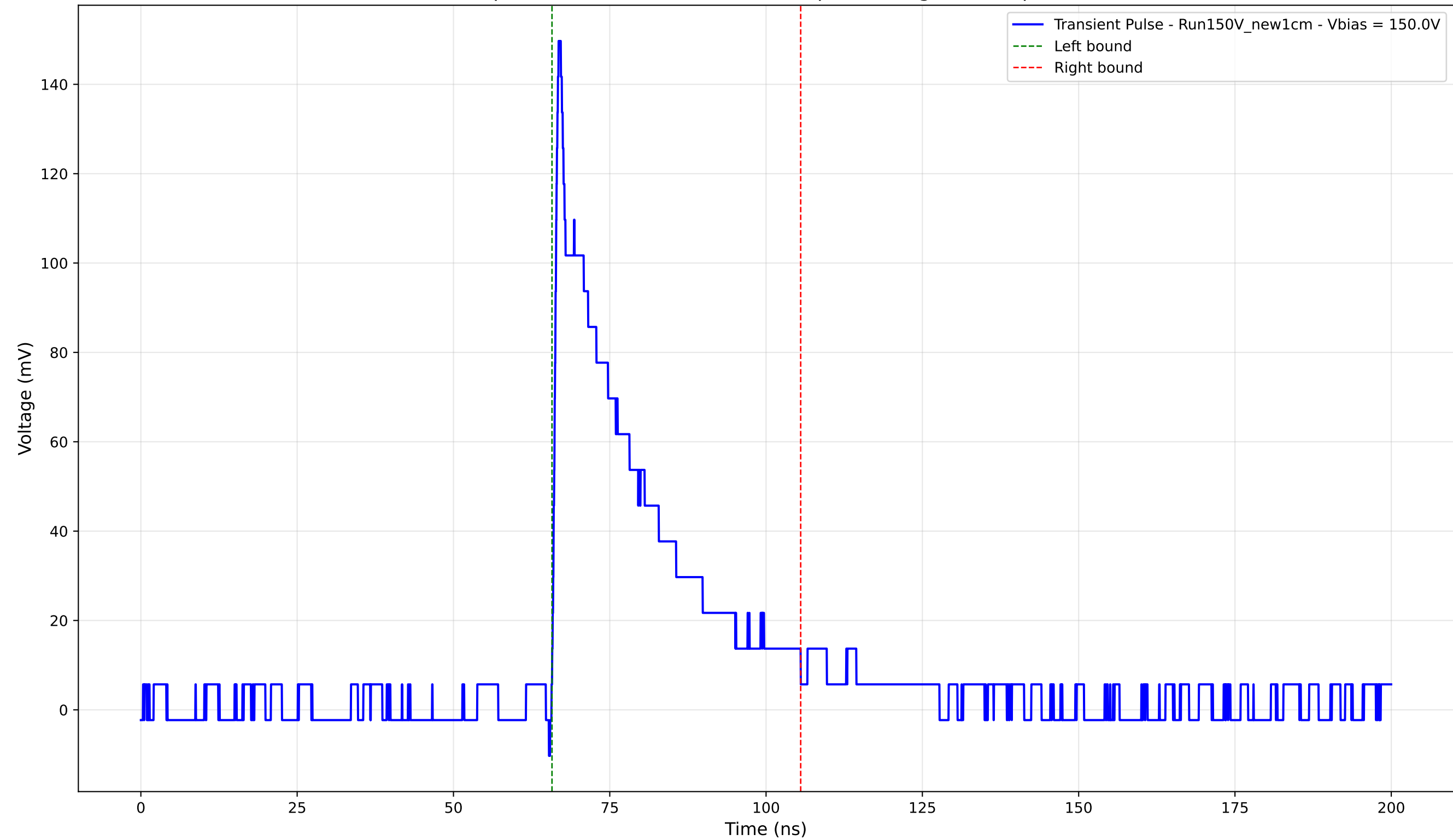
Transient Pulse - Sample: New1cm - Position: 2200.0 \mu\text{m} - Charge: 36.02 pC - Rise Time: 0.86 ns
