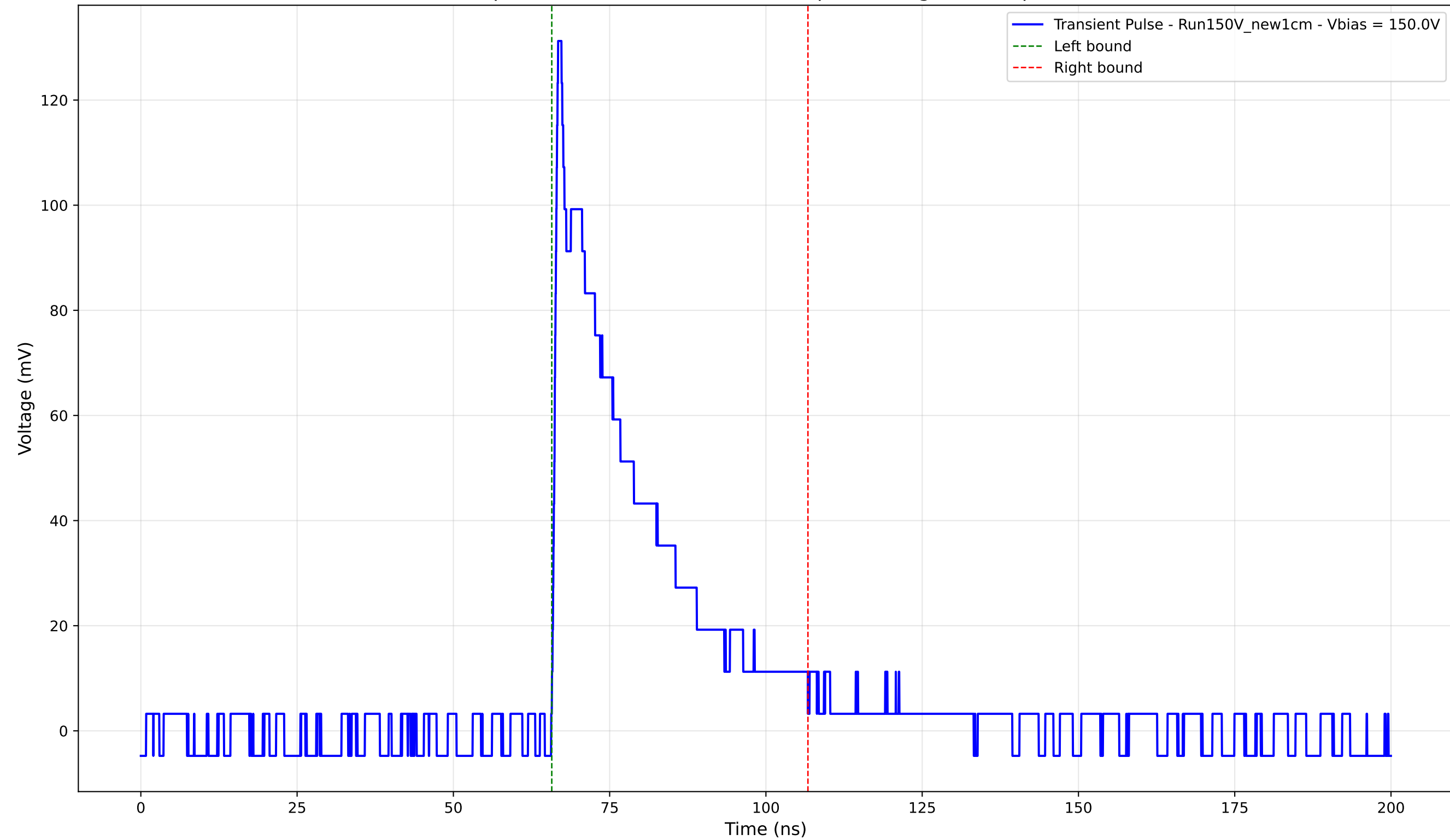
Transient Pulse - Sample: New1cm - Position: 2175.0 \mu\text{m} - Charge: 32.69 pC - Rise Time: 0.82 ns
