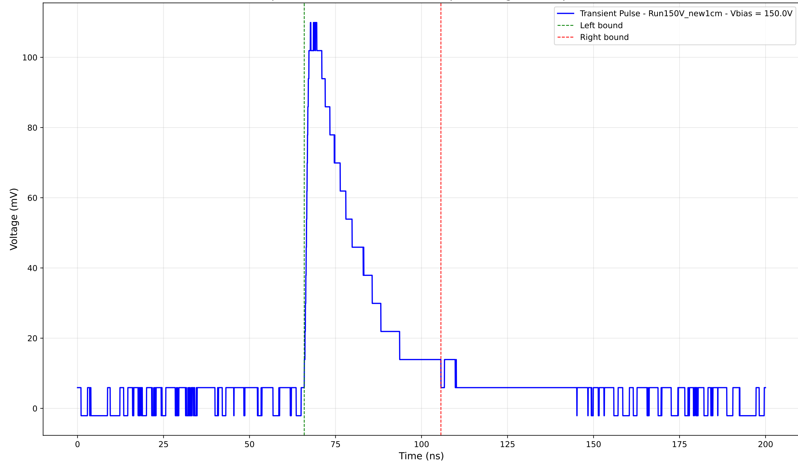
Transient Pulse - Sample: New1cm - Position: 1745.0 \mu\text{m} - Charge: 34.02 pC - Rise Time: 1.35 ns
