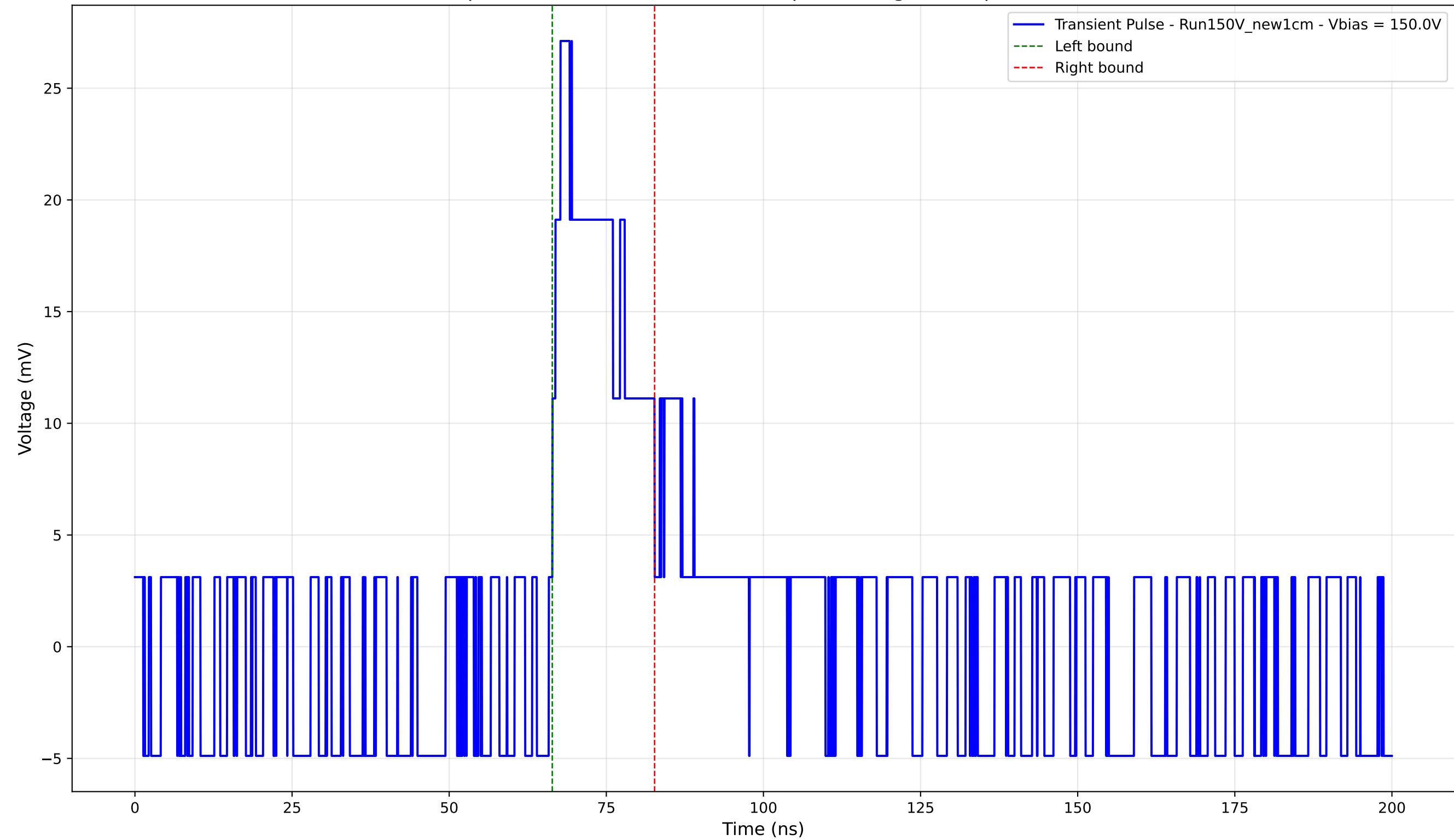
Transient Pulse - Sample: New1cm - Position: 3545.0 \mu\text{m} - Charge: 5.44 pC - Rise Time: 0.00 ns (N/A)
