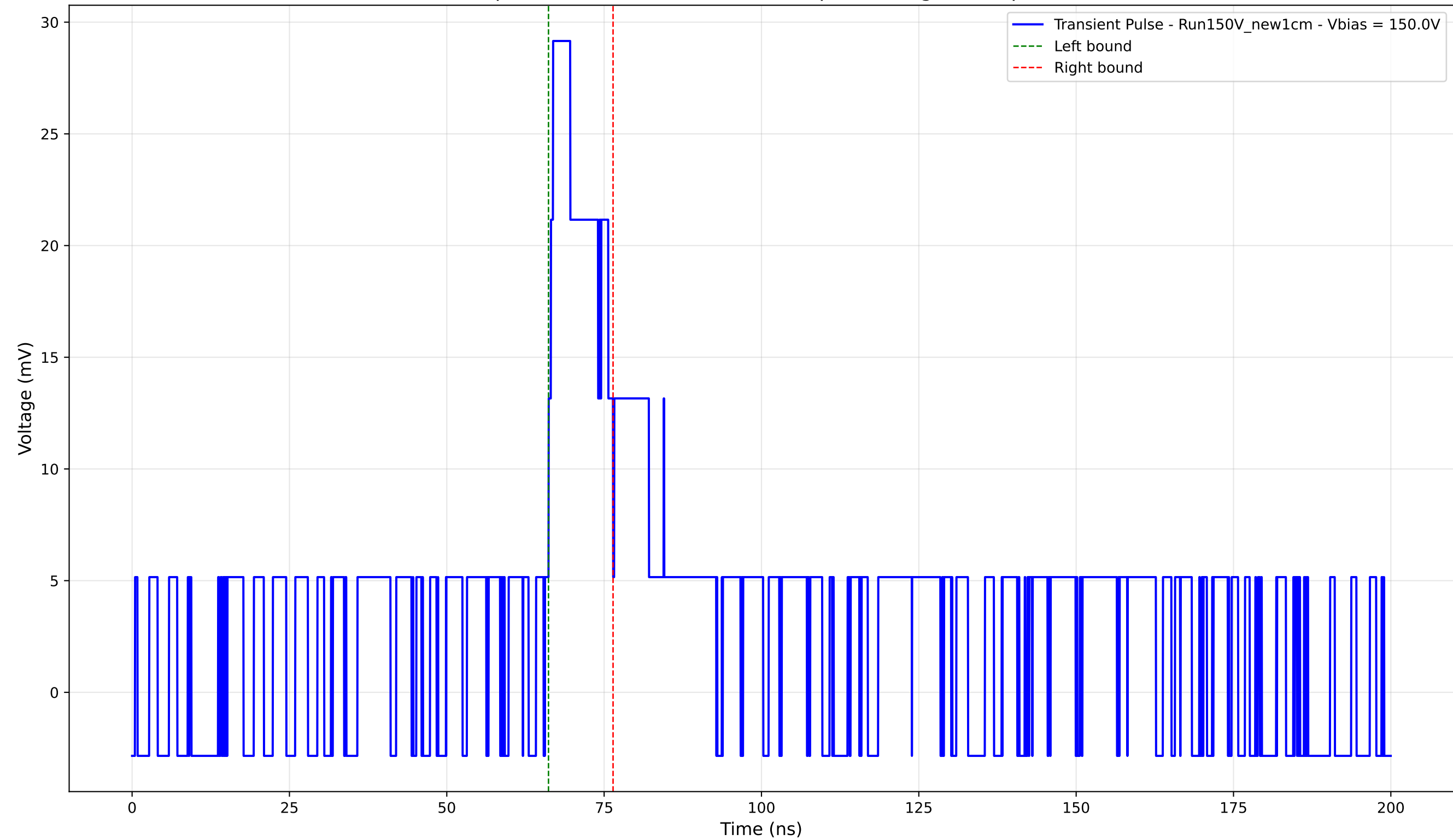
Transient Pulse - Sample: New1cm - Position: 4555.0 \mu\text{m} - Charge: 4.53 pC - Rise Time: 1.32 ns
