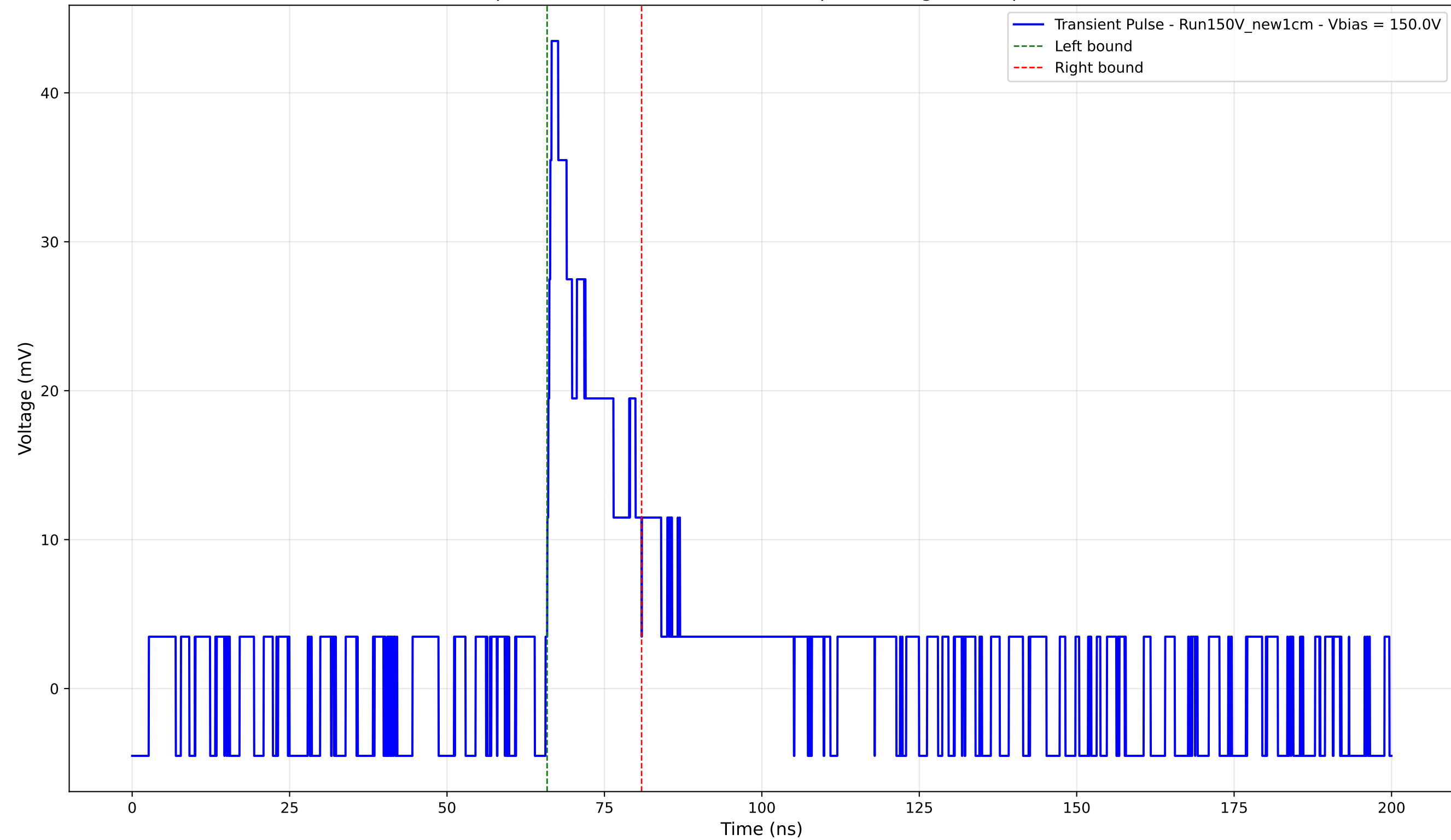
Transient Pulse - Sample: New1cm - Position: 4870.0 \mu\text{m} - Charge: 6.62 pC - Rise Time: 0.70 ns
