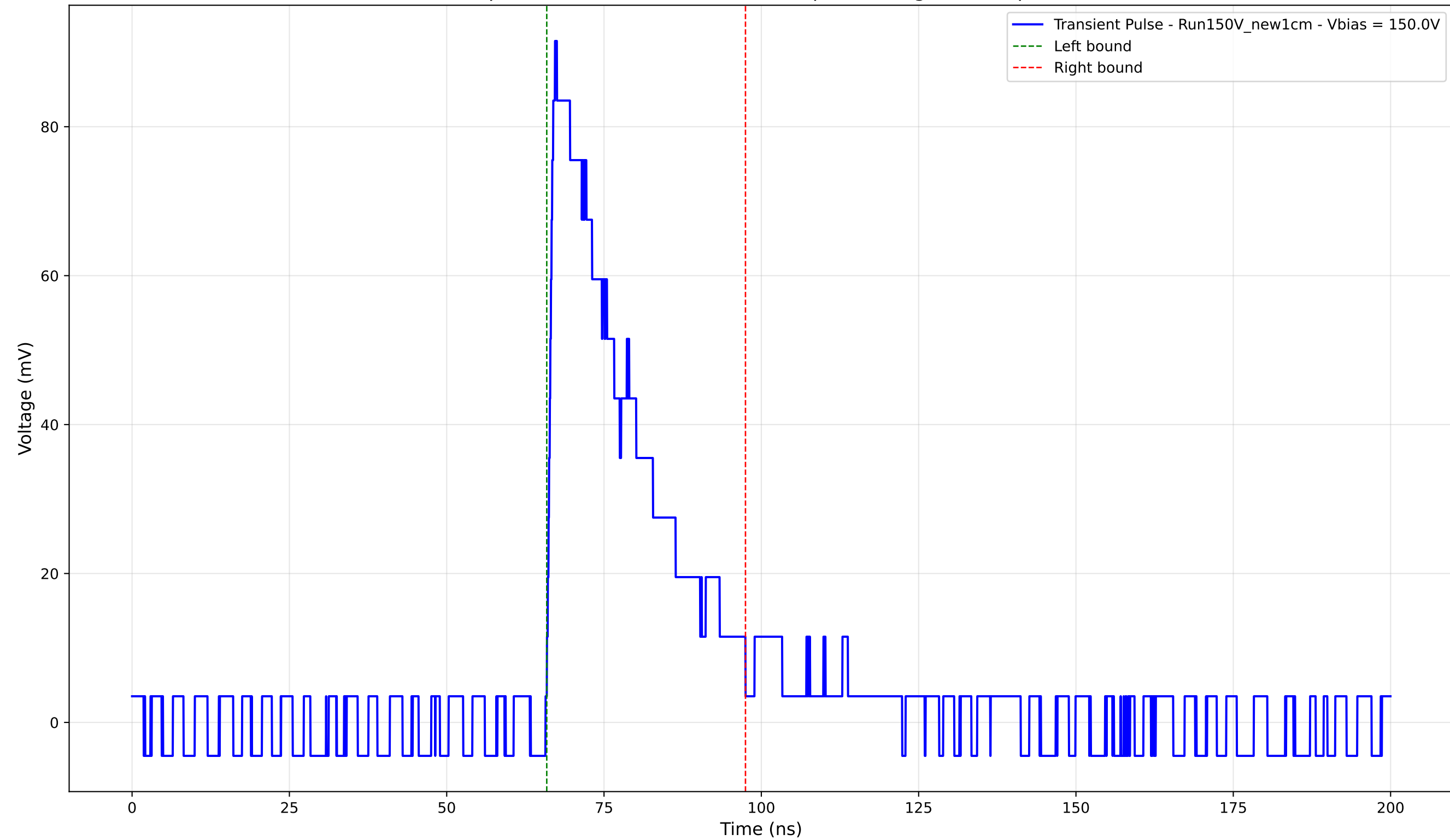
Transient Pulse - Sample: New1cm - Position: 1955.0 \mu\text{m} - Charge: 24.95 pC - Rise Time: 1.01 ns
