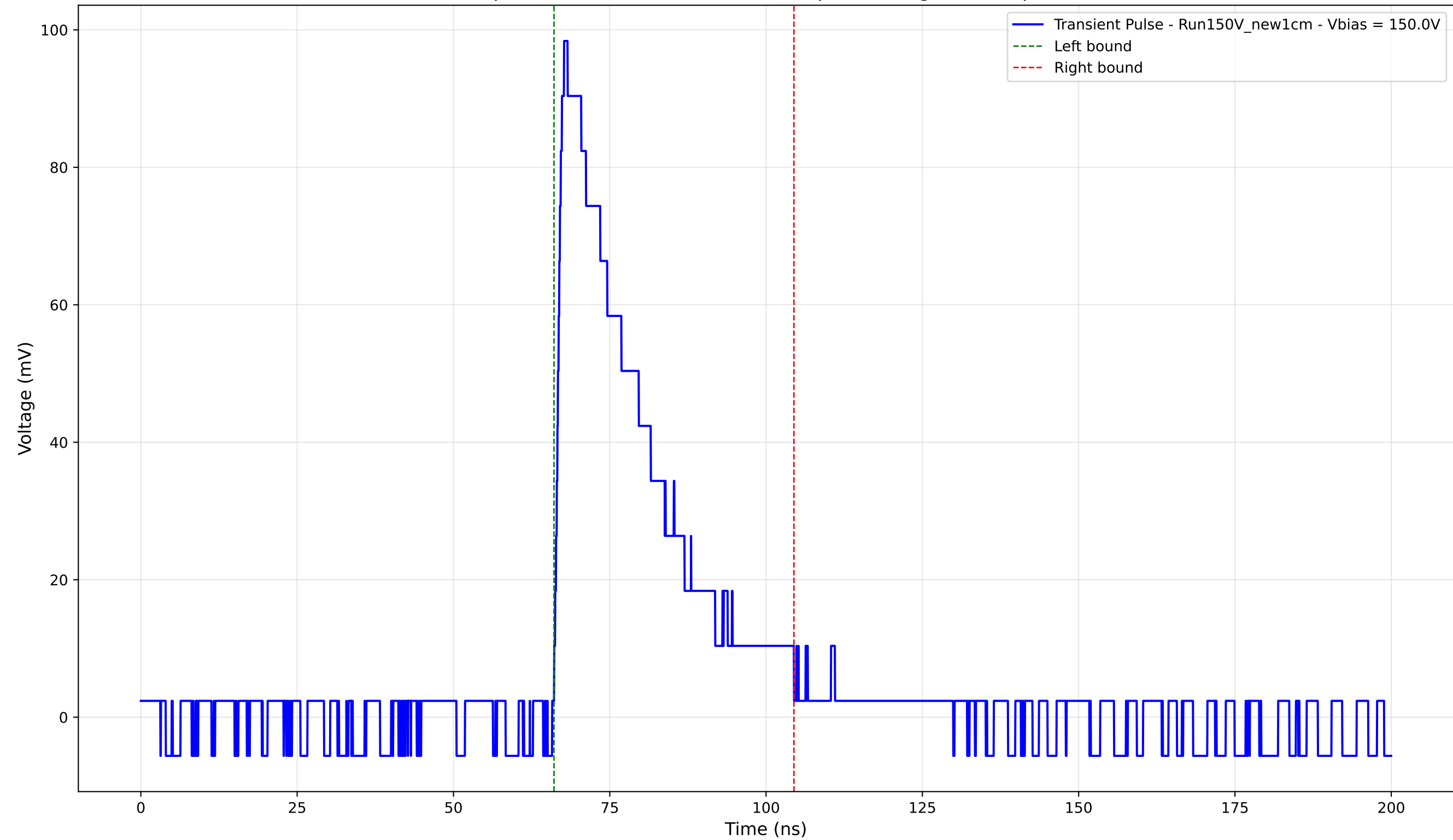
Transient Pulse - Sample: New1cm - Position: 3495.0 \mu\text{m} - Charge: 27.85 pC - Rise Time: 1.24 ns
