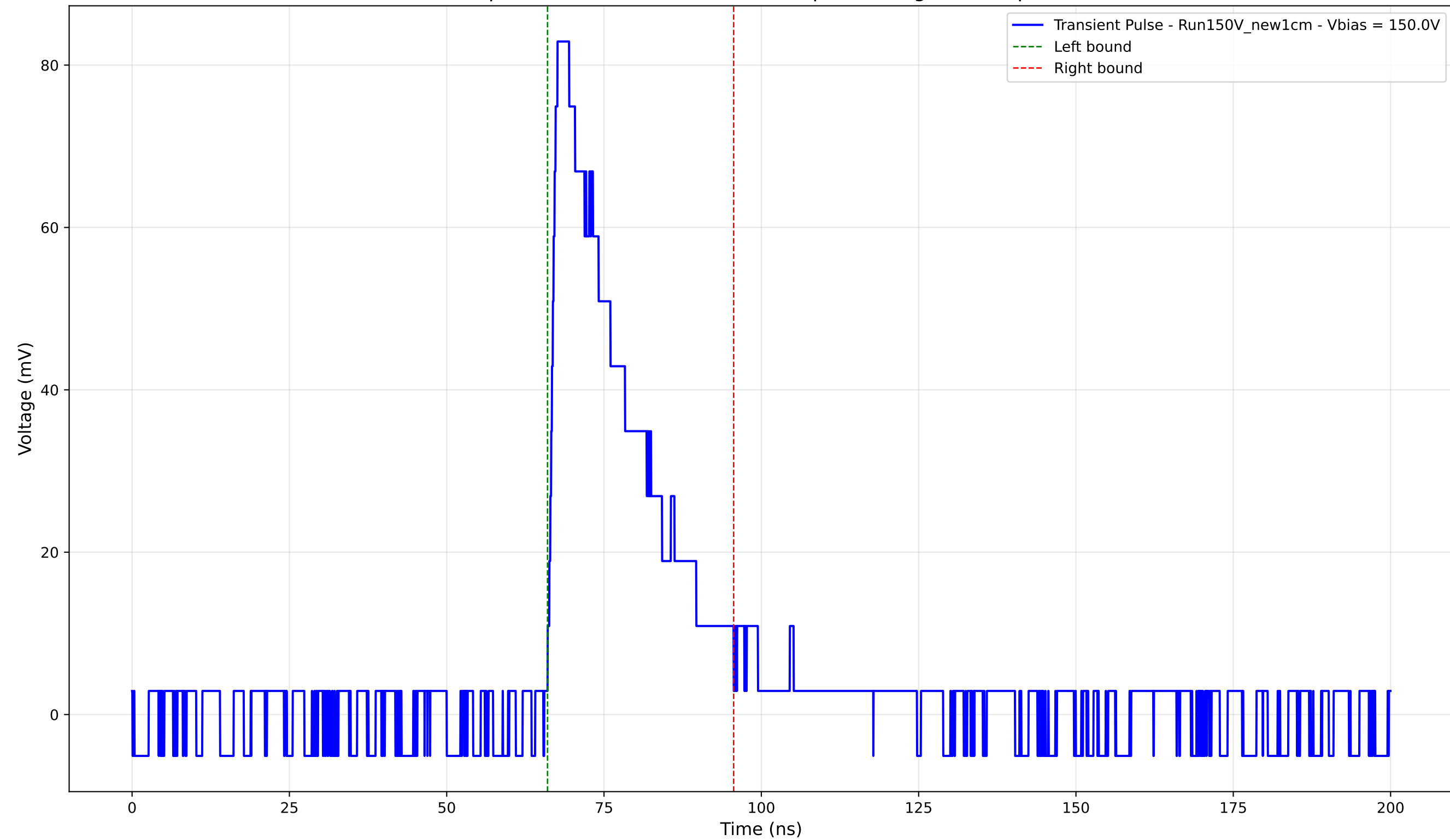
Transient Pulse - Sample: New1cm - Position: 4140.0 \mu\text{m} - Charge: 21.70 pC - Rise Time: 1.27 ns
