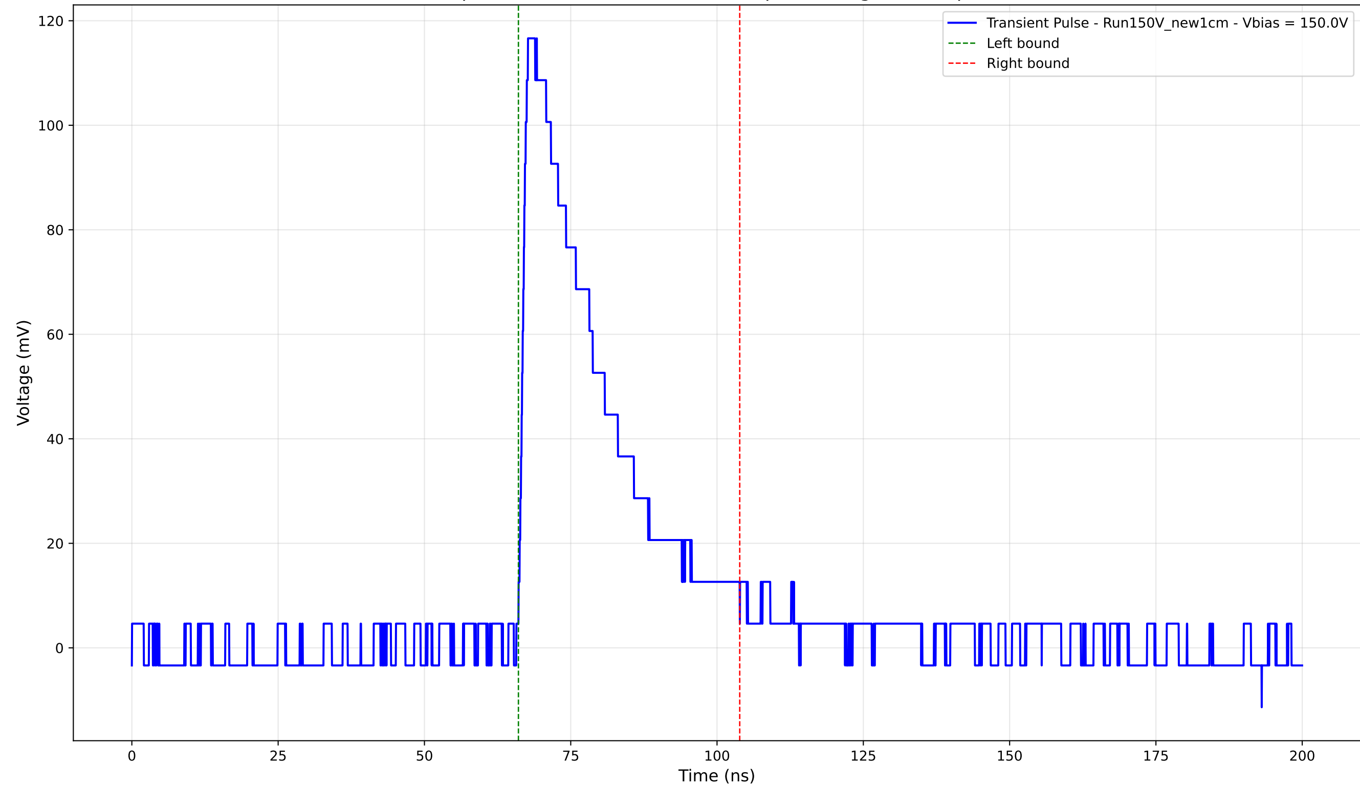
Transient Pulse - Sample: New1cm - Position: 3650.0 \mu\text{m} - Charge: 34.31 pC - Rise Time: 1.40 ns
