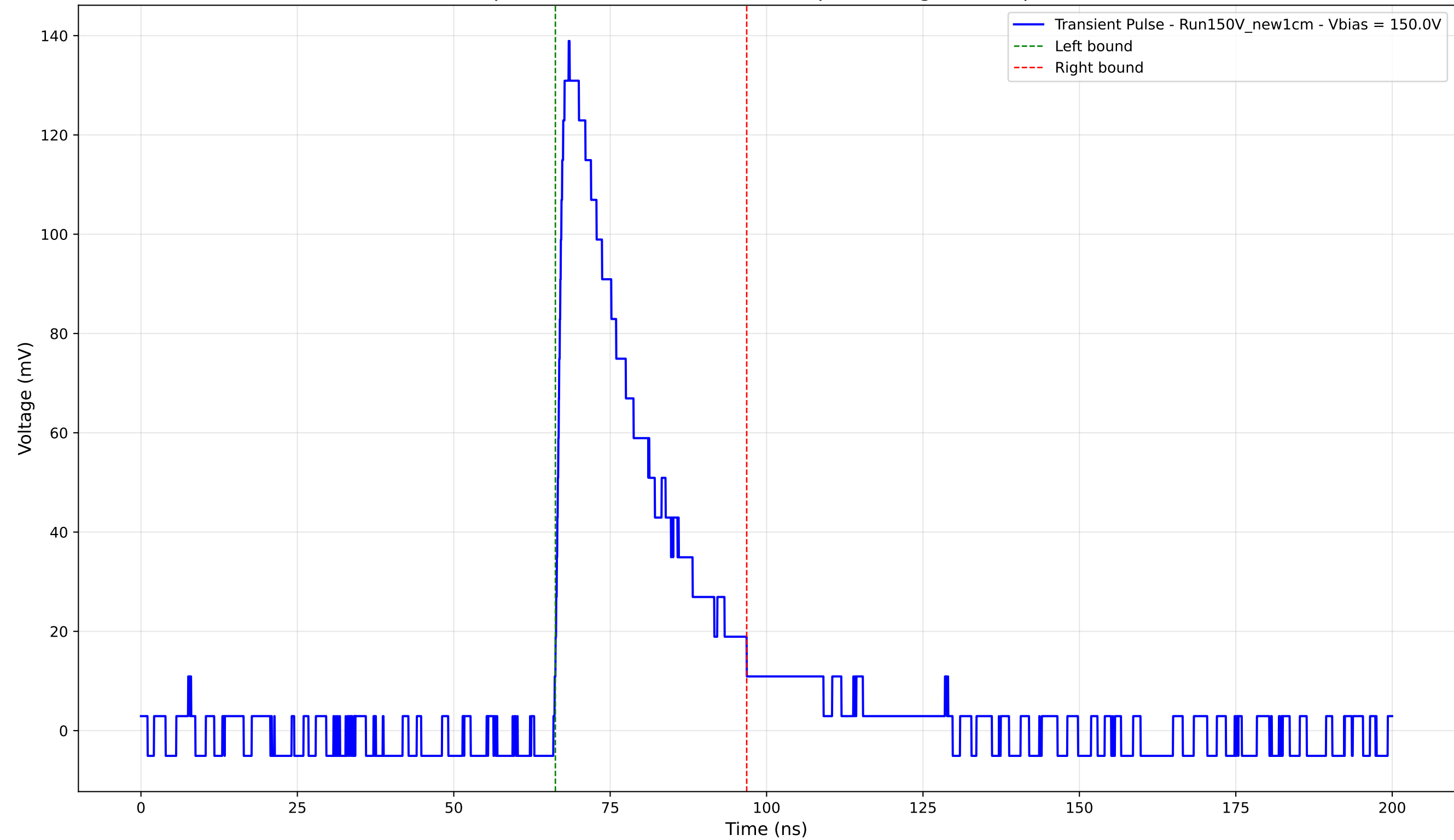
Transient Pulse - Sample: New1cm - Position: 3690.0 \mu\text{m} - Charge: 37.29 pC - Rise Time: 1.45 ns
