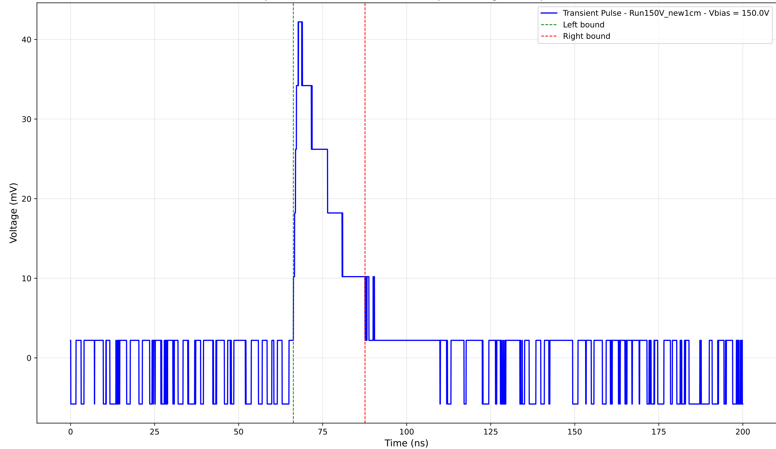
Transient Pulse - Sample: New1cm - Position: 1580.0 \mu\text{m} - Charge: 9.05 pC - Rise Time: 1.43 ns
