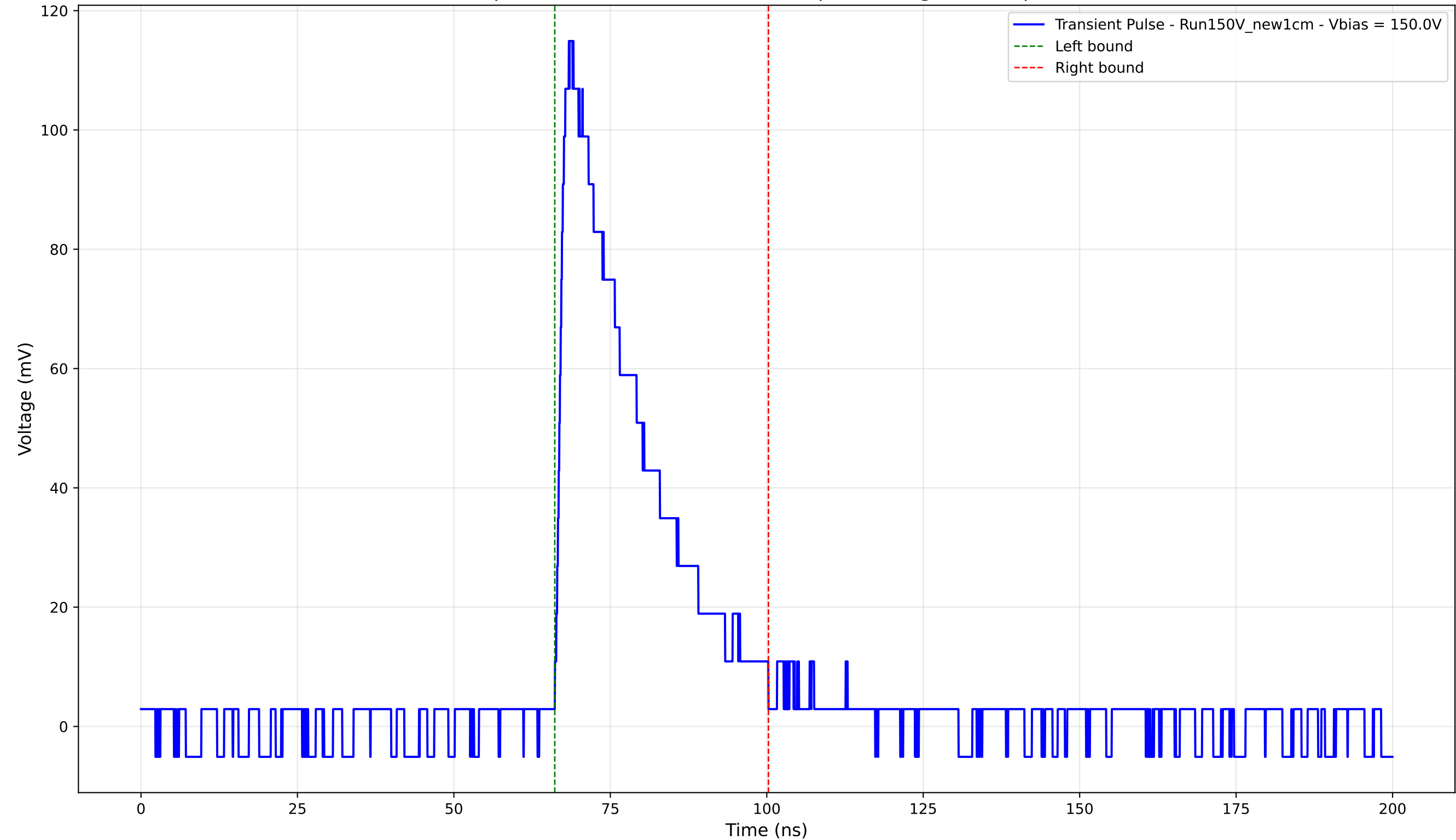
Transient Pulse - Sample: New1cm - Position: 1185.0 \mu\text{m} - Charge: 31.14 pC - Rise Time: 1.46 ns
