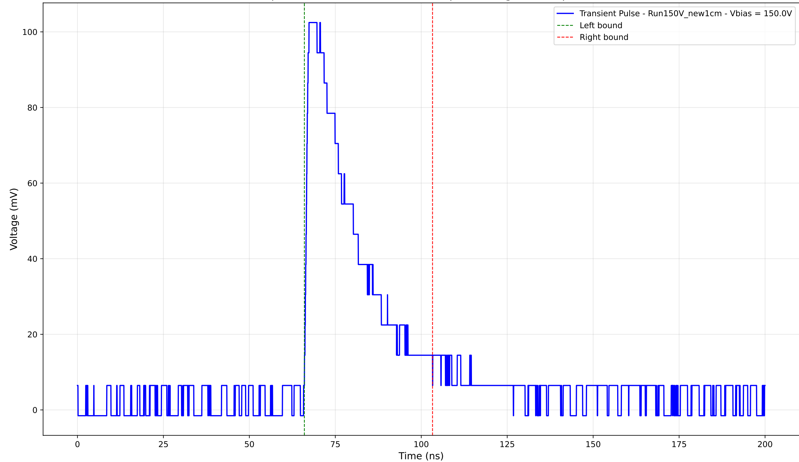
Transient Pulse - Sample: New1cm - Position: 1750.0 \mu\text{m} - Charge: 33.05 pC - Rise Time: 1.07 ns
