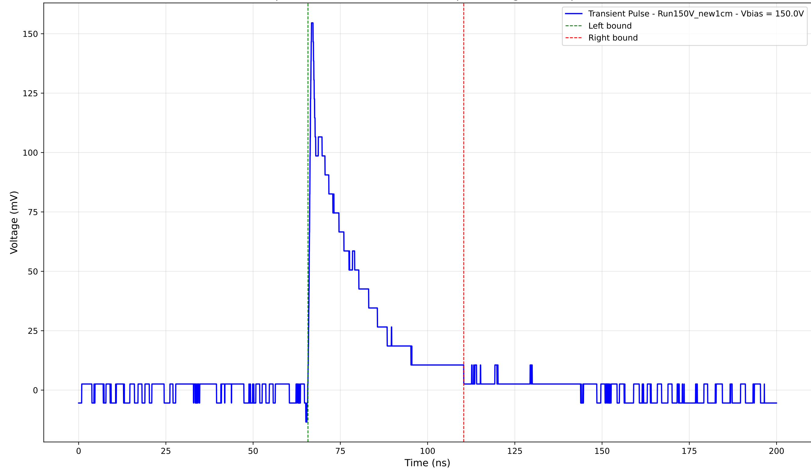
Transient Pulse - Sample: New1cm - Position: 2255.0 \mu\text{m} - Charge: 34.70 pC - Rise Time: 0.83 ns
