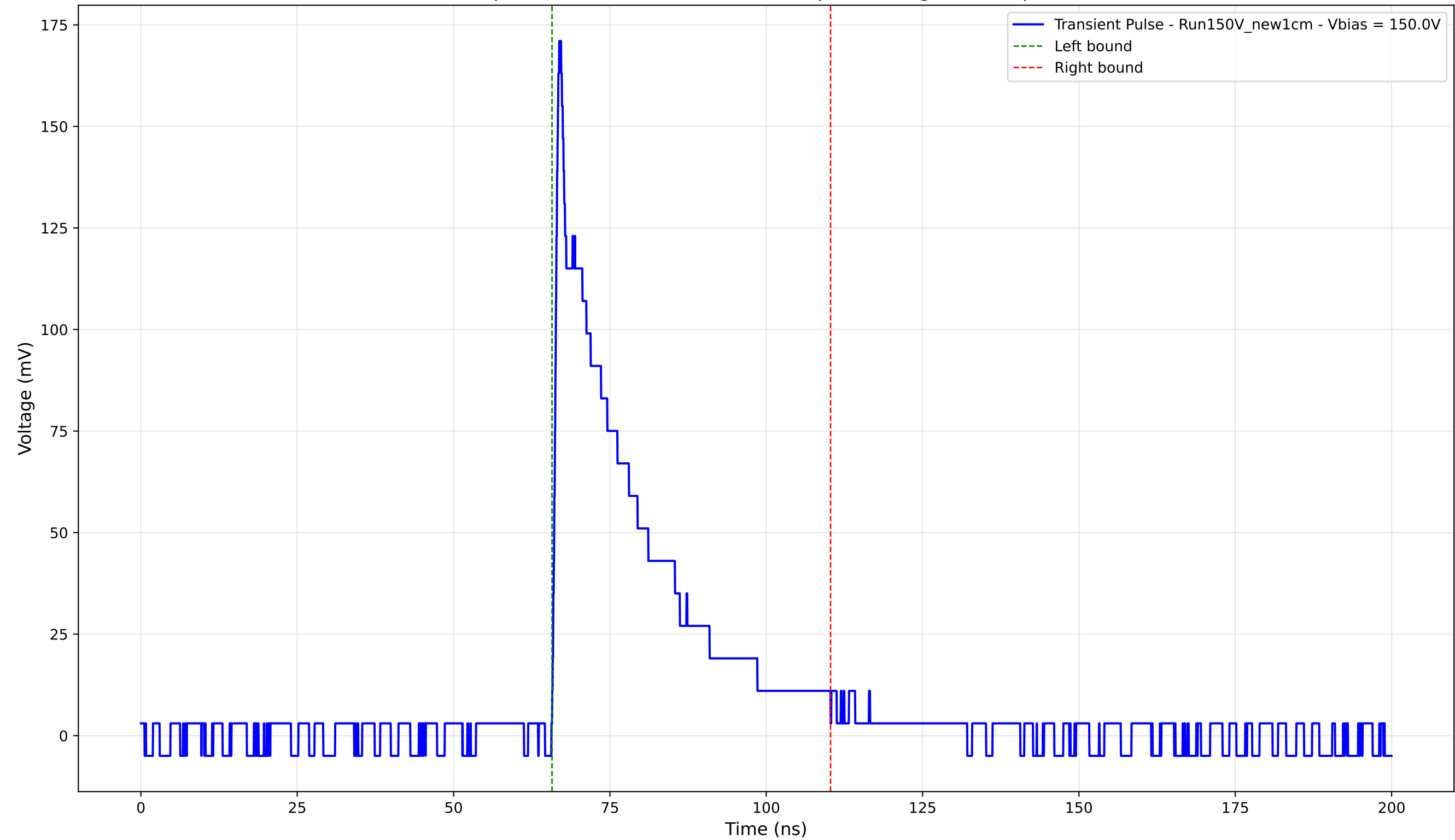
Transient Pulse - Sample: New1cm - Position: 2910.0 \mu\text{m} - Charge: 39.39 pC - Rise Time: 0.84 ns
