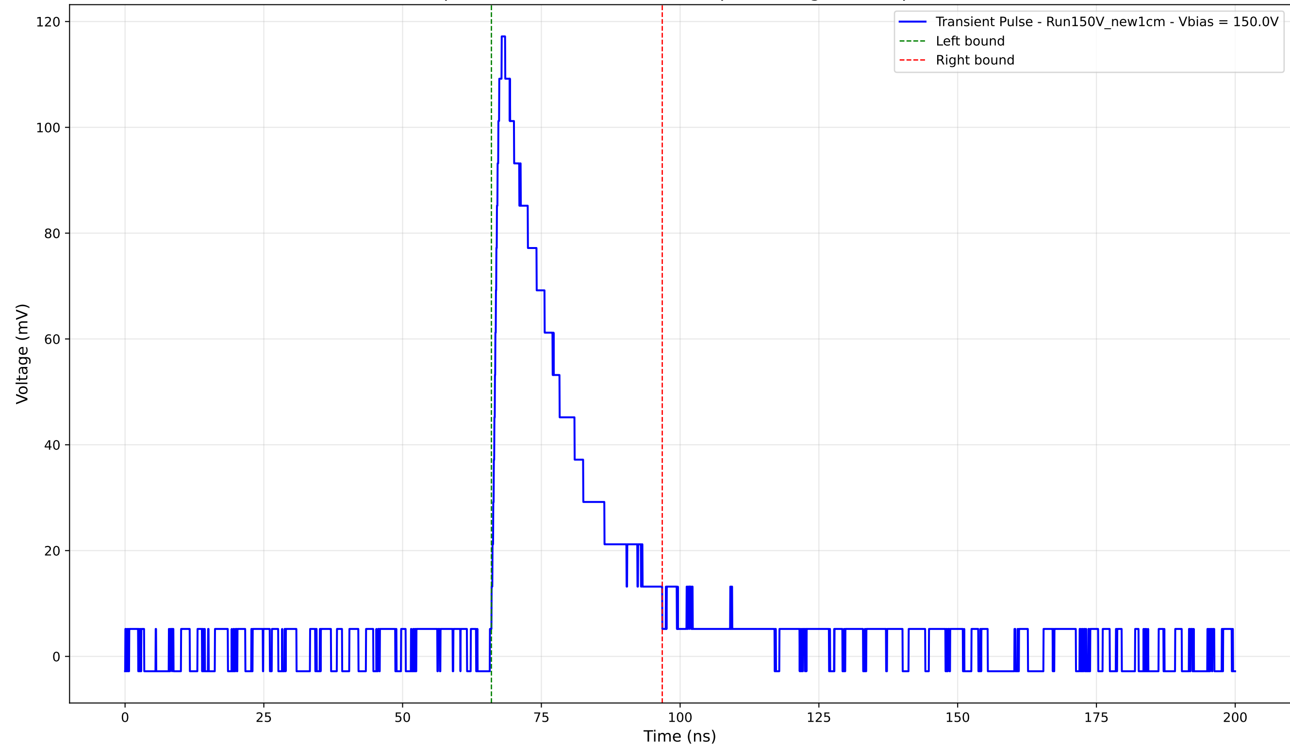
Transient Pulse - Sample: New1cm - Position: 640.0 \mu\text{m} - Charge: 28.98 pC - Rise Time: 1.38 ns
