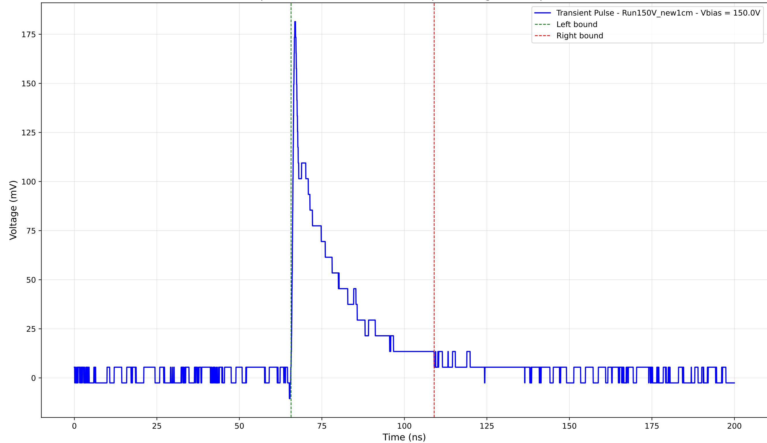
Transient Pulse - Sample: New1cm - Position: 2315.0 \mu\text{m} - Charge: 37.93 pC - Rise Time: 0.83 ns
