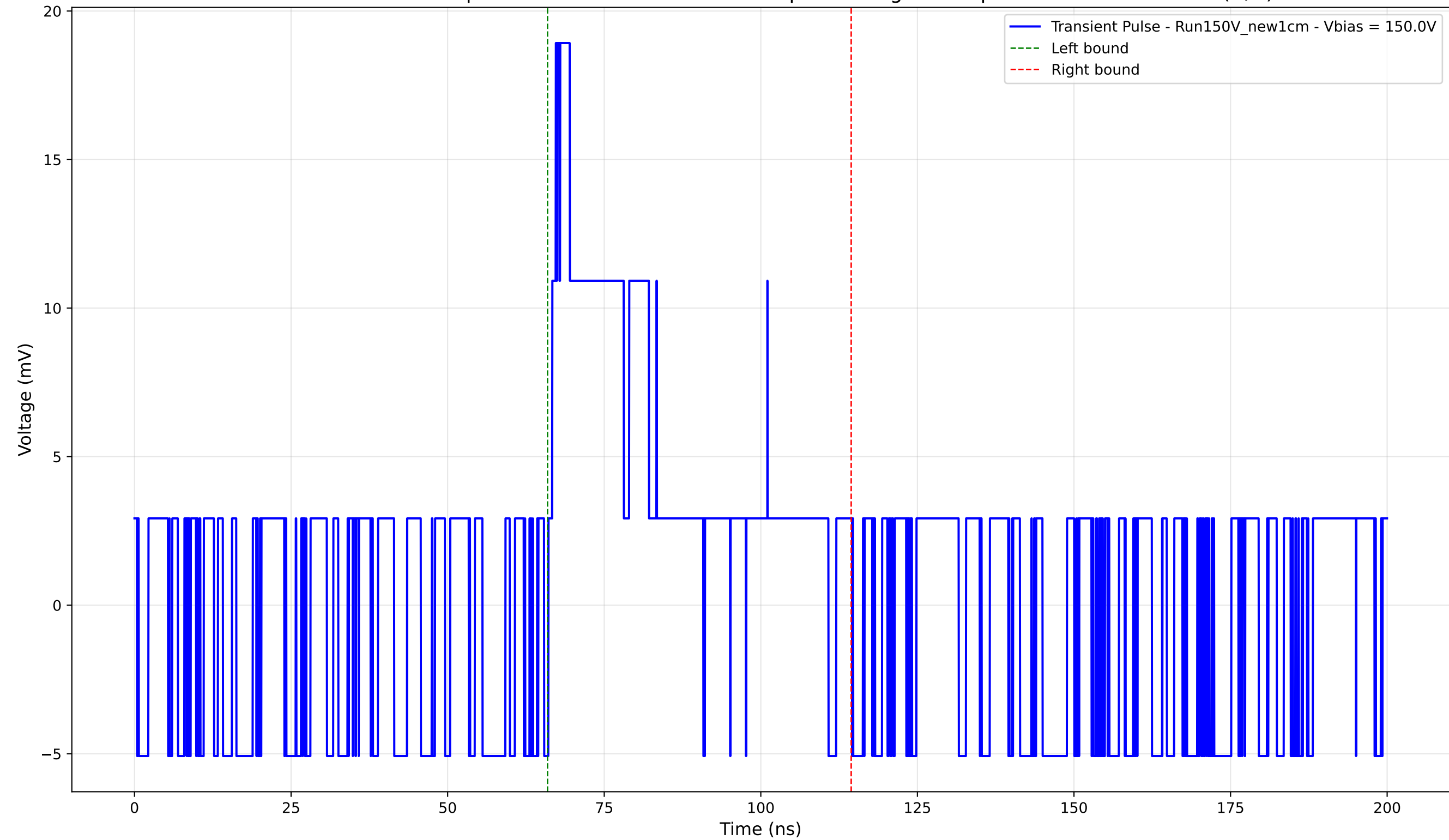
Transient Pulse - Sample: New1cm - Position: 2030.0 \mu\text{m} - Charge: 5.25 pC - Rise Time: 0.00 ns (N/A)
