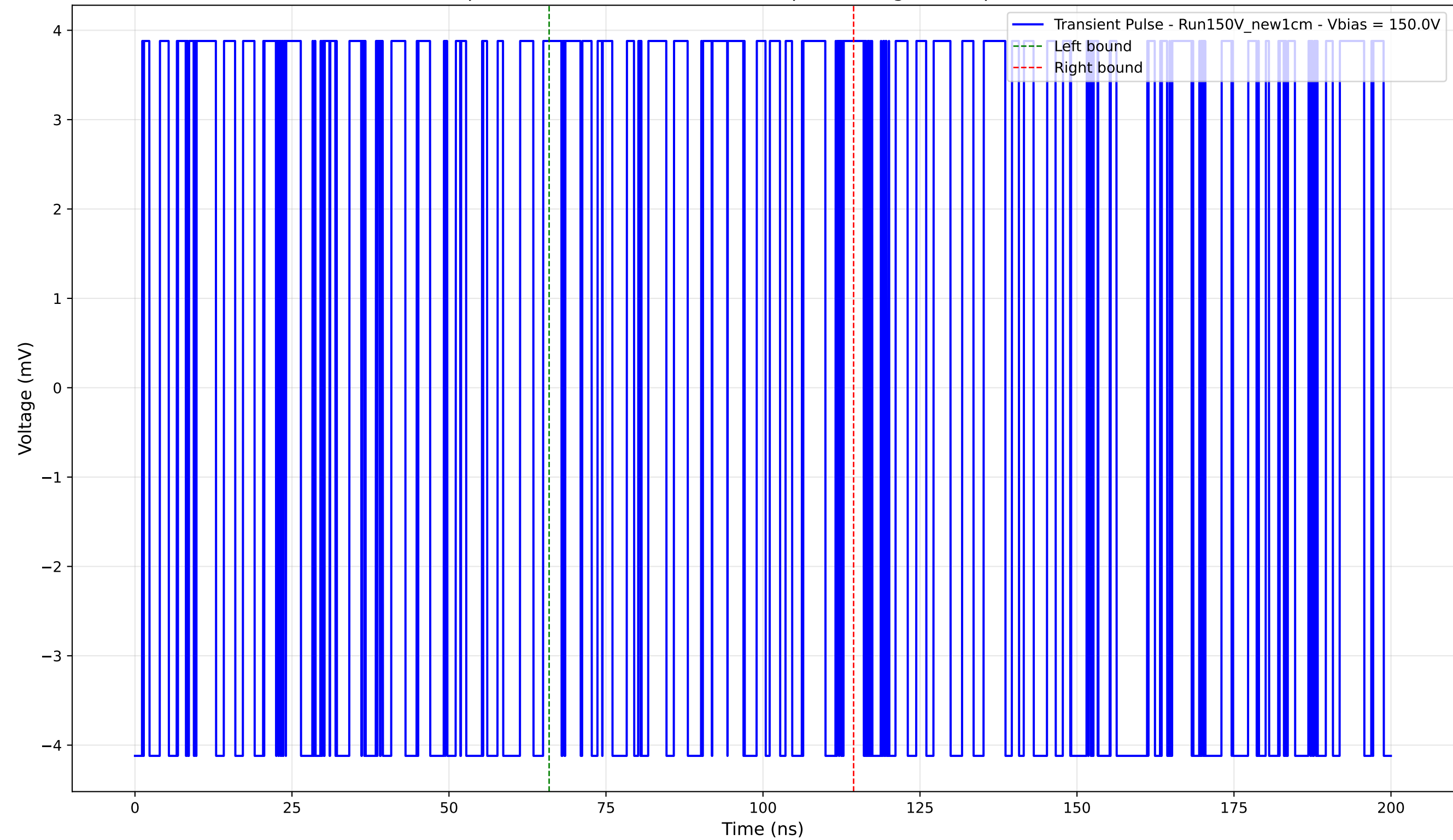
Transient Pulse - Sample: New1cm - Position: 4965.0 \mu\text{m} - Charge: 1.08 pC - Rise Time: 0.00 ns (N/A)
