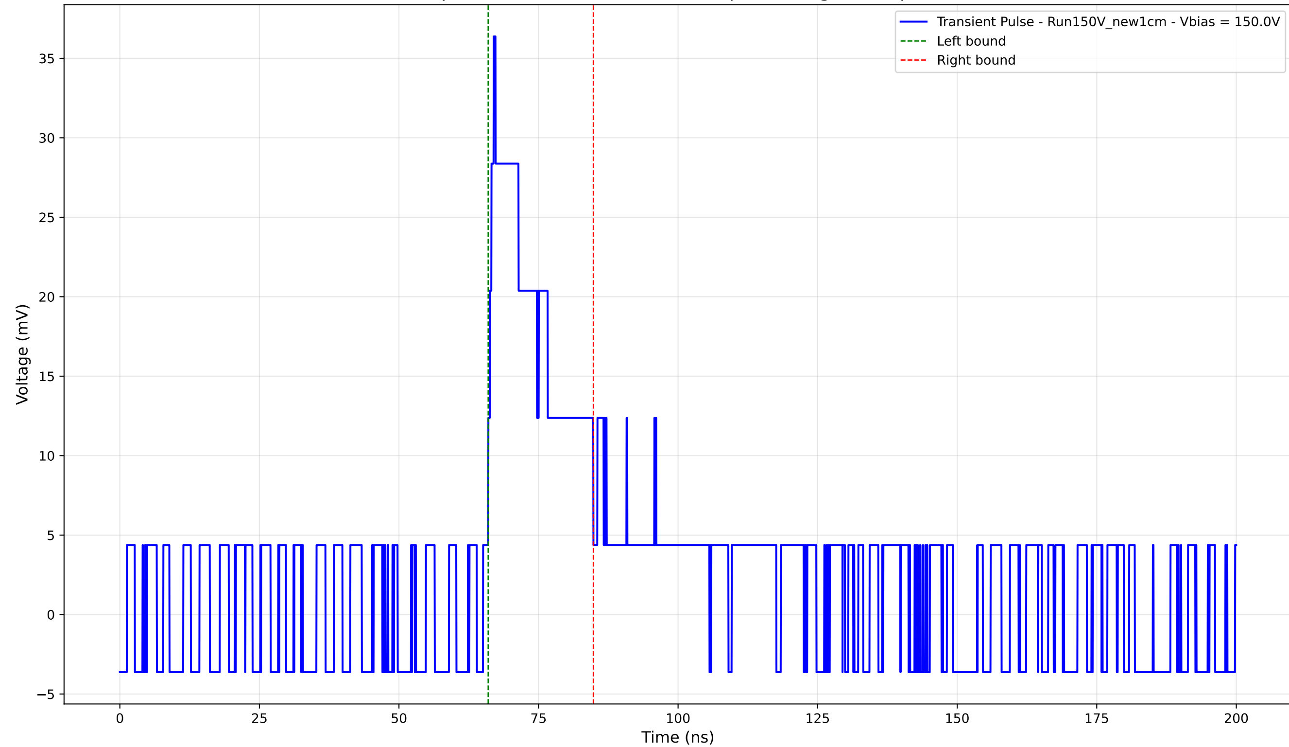
Transient Pulse - Sample: New1cm - Position: 2010.0 \mu\text{m} - Charge: 7.11 pC - Rise Time: 1.92 ns
