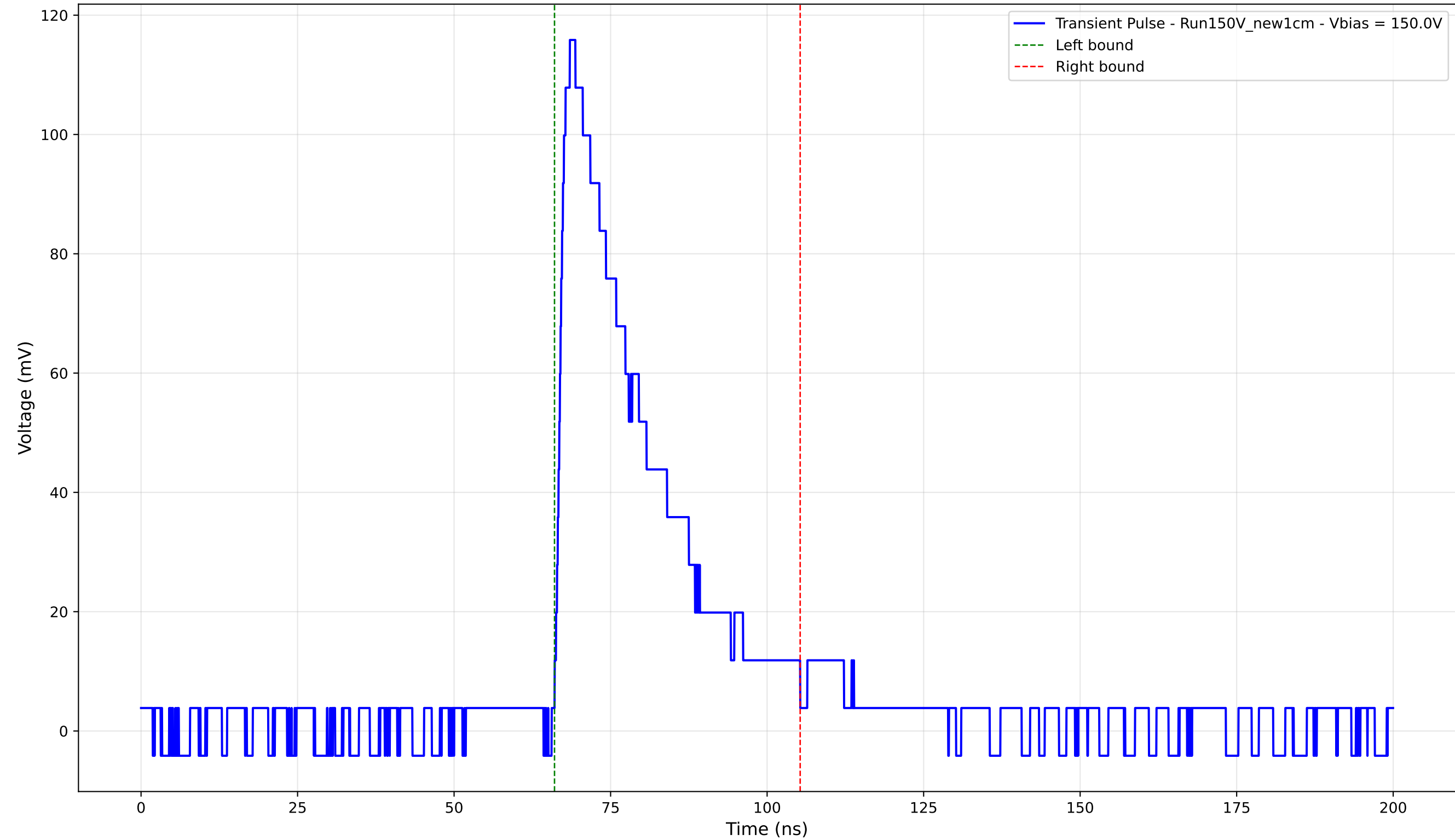
Transient Pulse - Sample: New1cm - Position: 1265.0 \mu\text{m} - Charge: 34.24 pC - Rise Time: 1.74 ns
