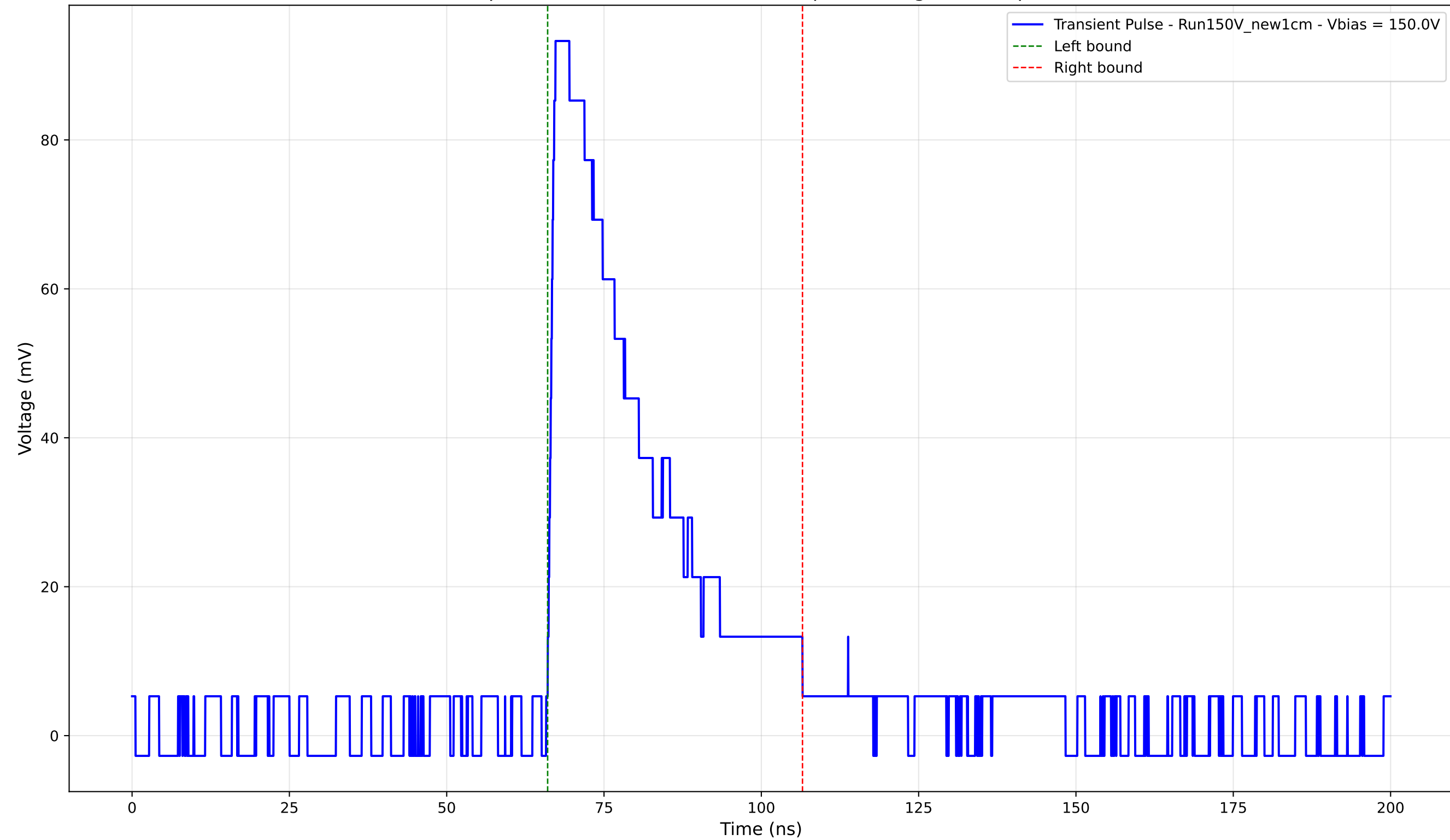
Transient Pulse - Sample: New1cm - Position: 1810.0 \mu\text{m} - Charge: 30.49 pC - Rise Time: 1.03 ns
