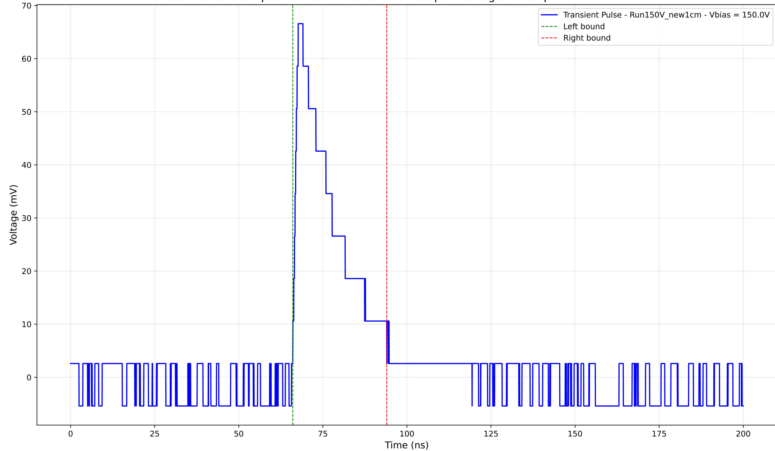
Transient Pulse - Sample: New1cm - Position: 4120.0 \mu\text{m} - Charge: 16.62 pC - Rise Time: 1.59 ns
