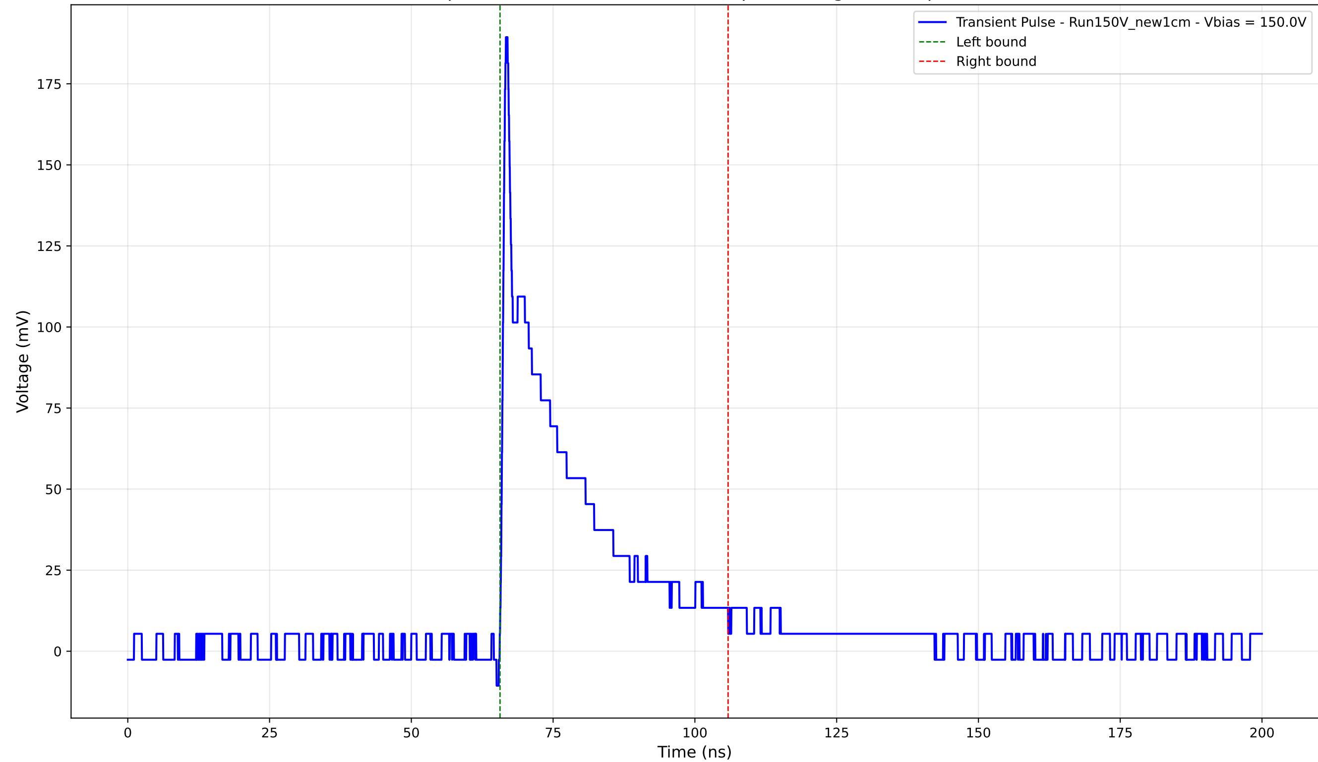
Transient Pulse - Sample: New1cm - Position: 2385.0 \mu\text{m} - Charge: 37.20 pC - Rise Time: 0.79 ns
