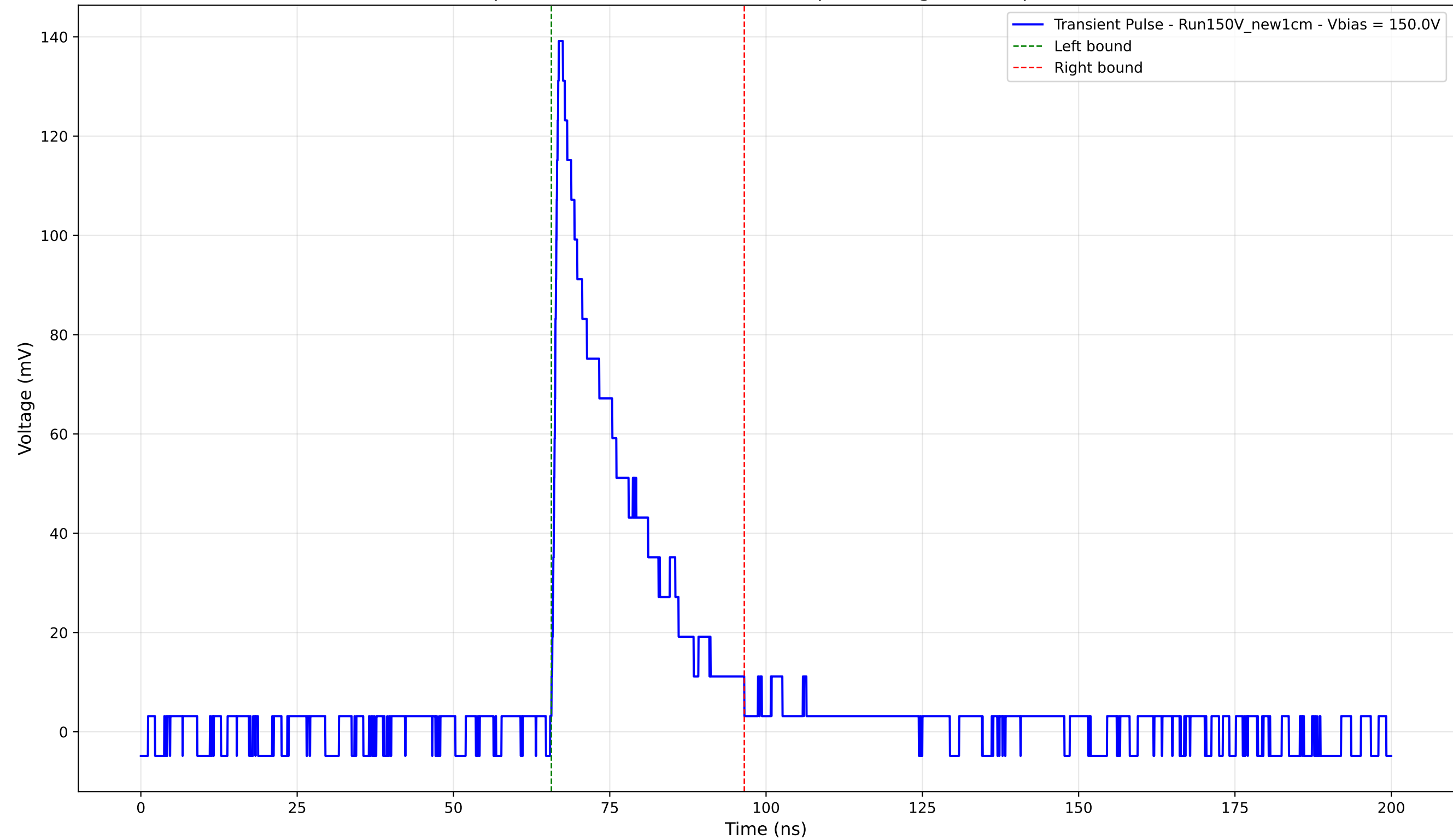
Transient Pulse - Sample: New1cm - Position: 4760.0 \mu\text{m} - Charge: 28.79 pC - Rise Time: 0.95 ns
