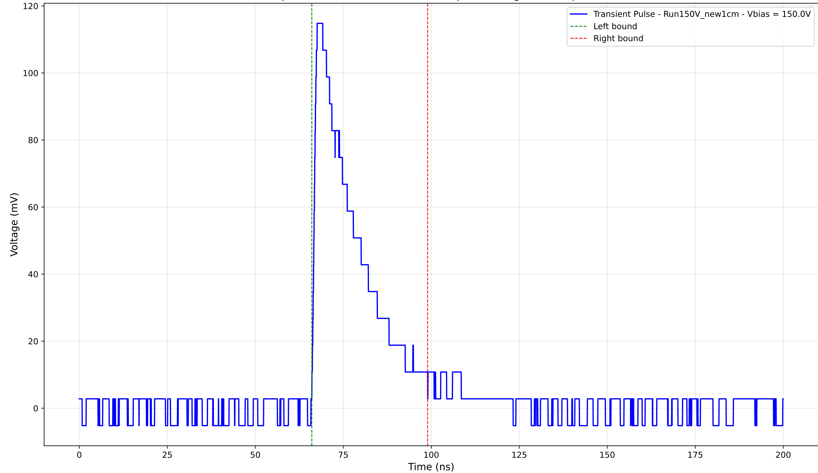
Transient Pulse - Sample: New1cm - Position: 690.0 \mu\text{m} - Charge: 30.09 pC - Rise Time: 1.14 ns
