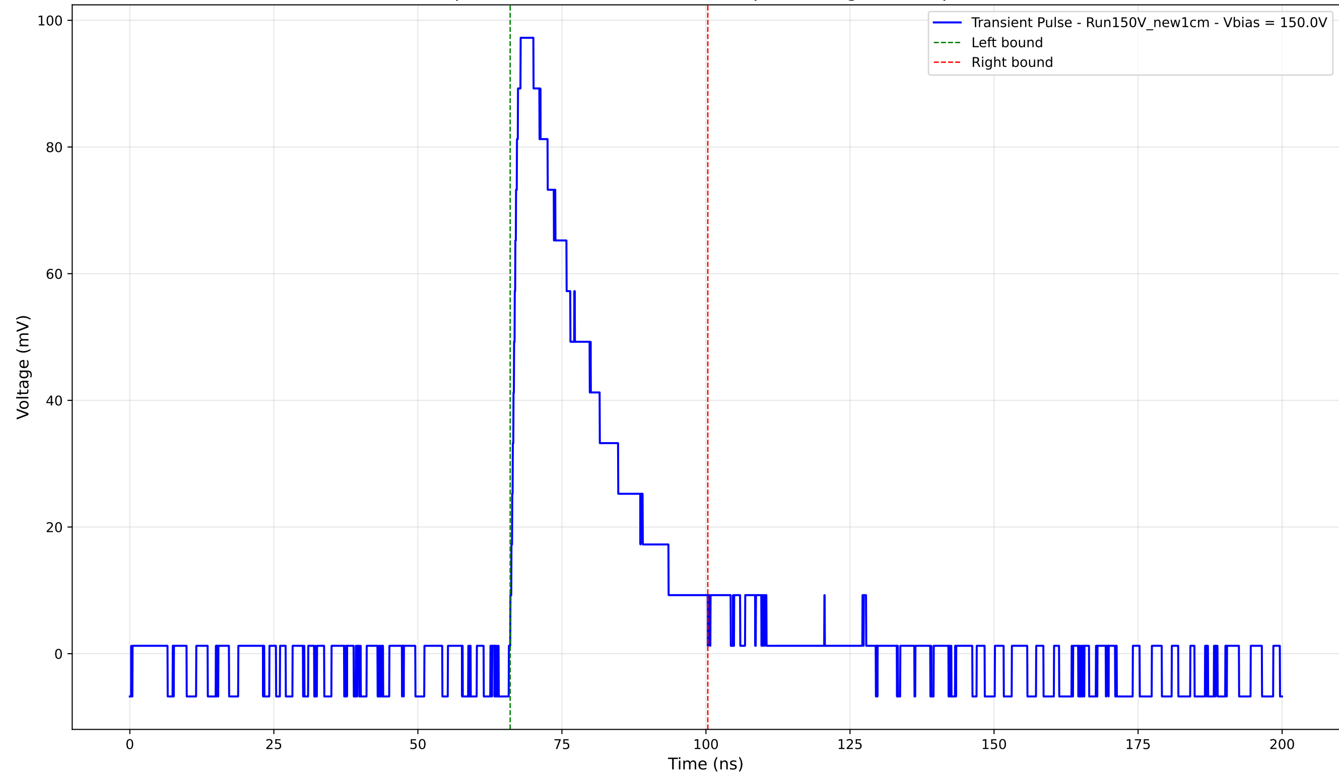
Transient Pulse - Sample: New1cm - Position: 1645.0 \mu\text{m} - Charge: 27.64 pC - Rise Time: 1.16 ns
