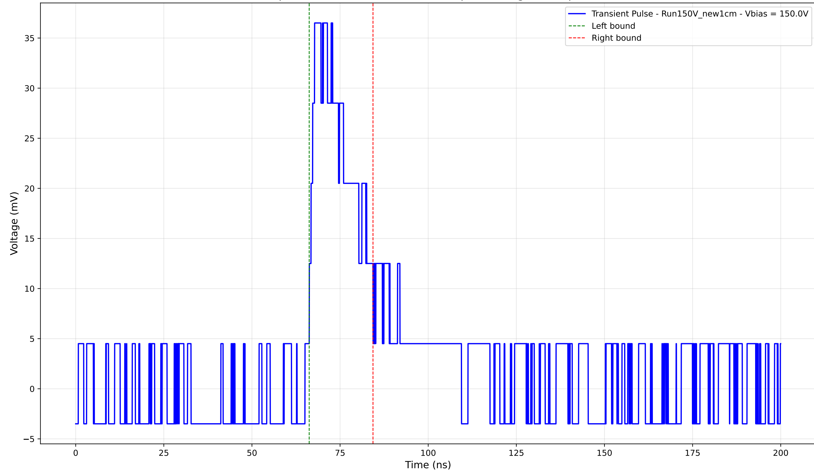
Transient Pulse - Sample: New1cm - Position: 3590.0 \mu\text{m} - Charge: 8.77 pC - Rise Time: 2.74 ns
