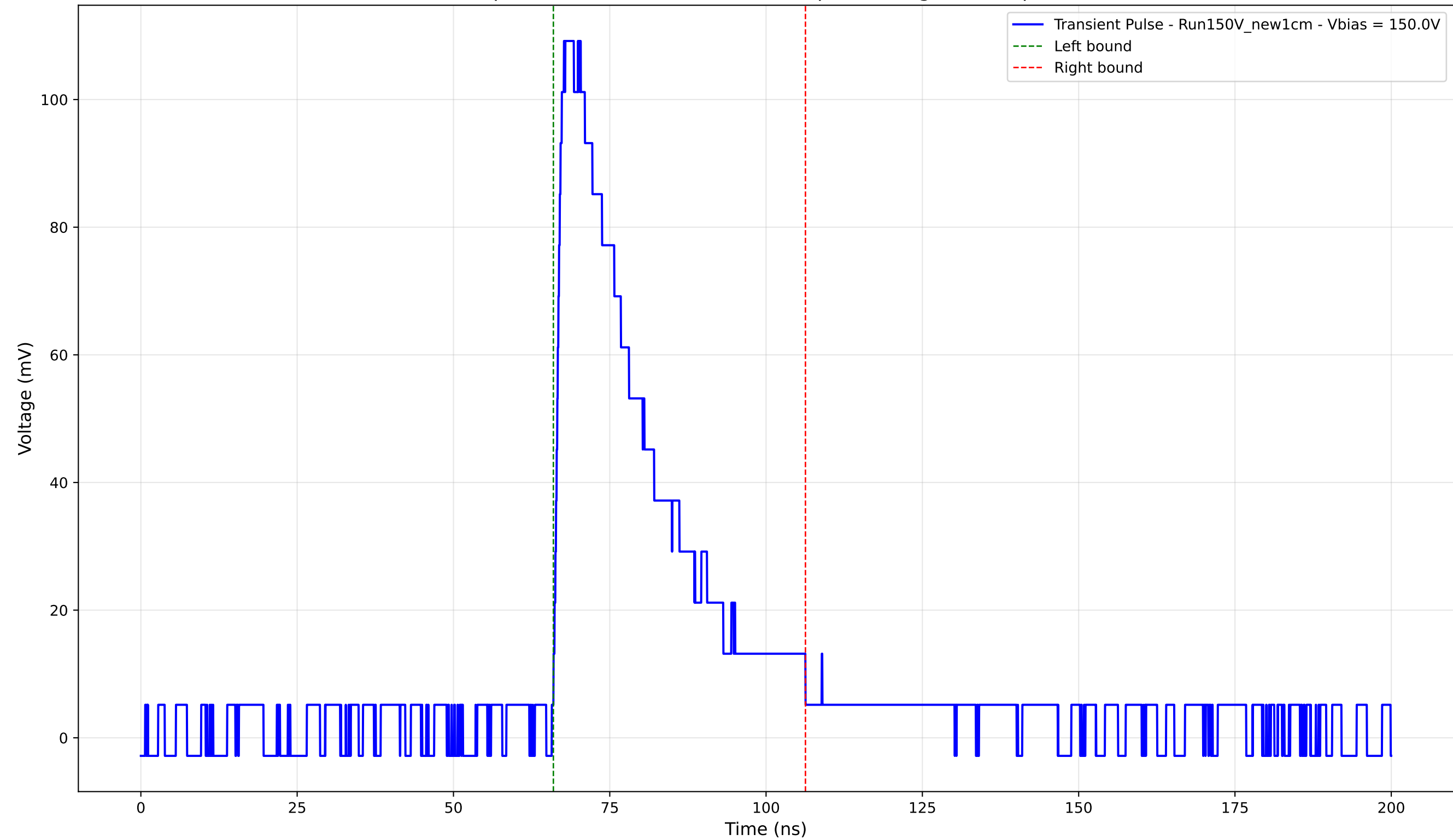
Transient Pulse - Sample: New1cm - Position: 1675.0 \mu\text{m} - Charge: 34.22 pC - Rise Time: 1.33 ns
