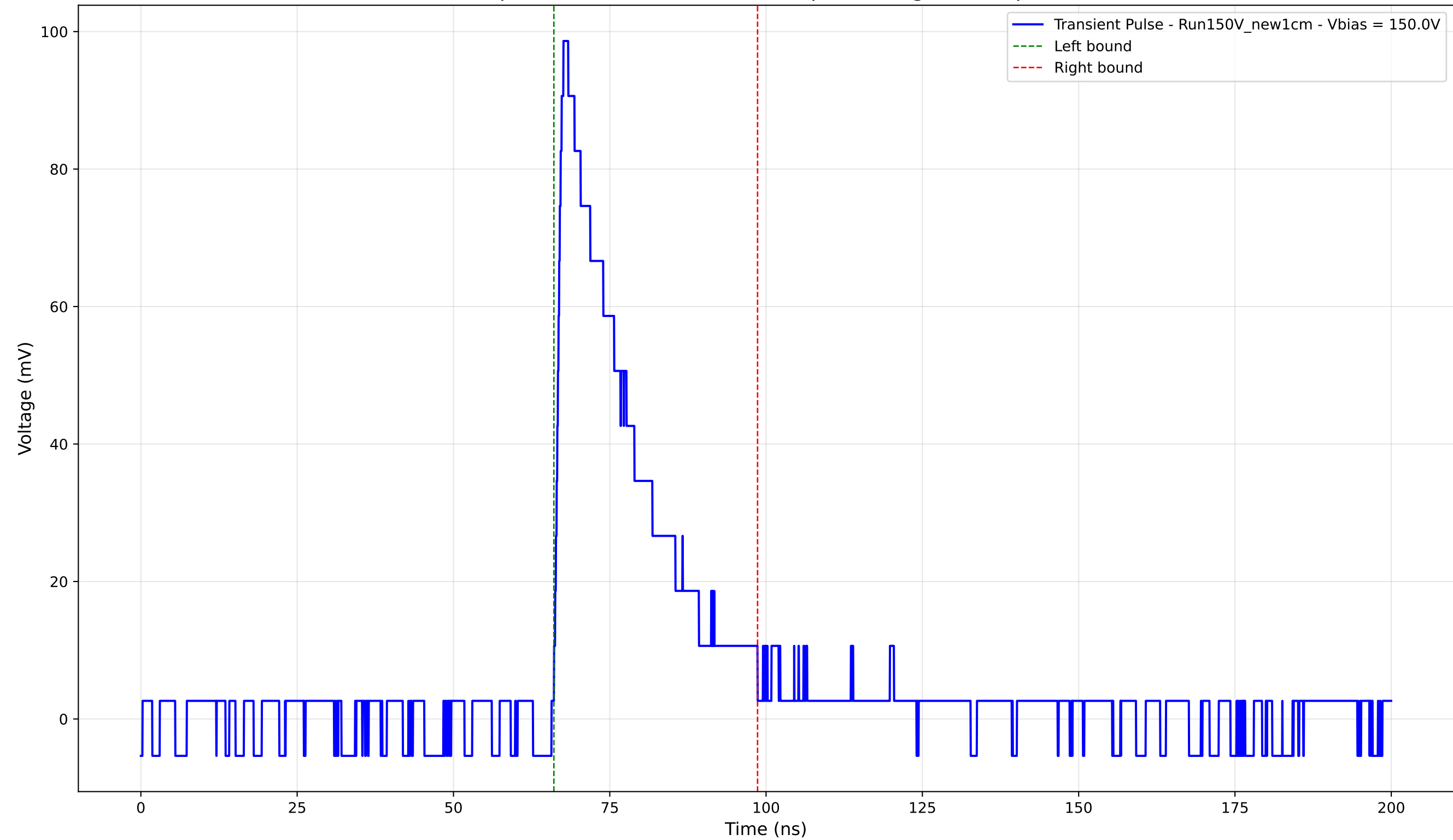
Transient Pulse - Sample: New1cm - Position: 620.0 \mu\text{m} - Charge: 24.17 pC - Rise Time: 1.22 ns
