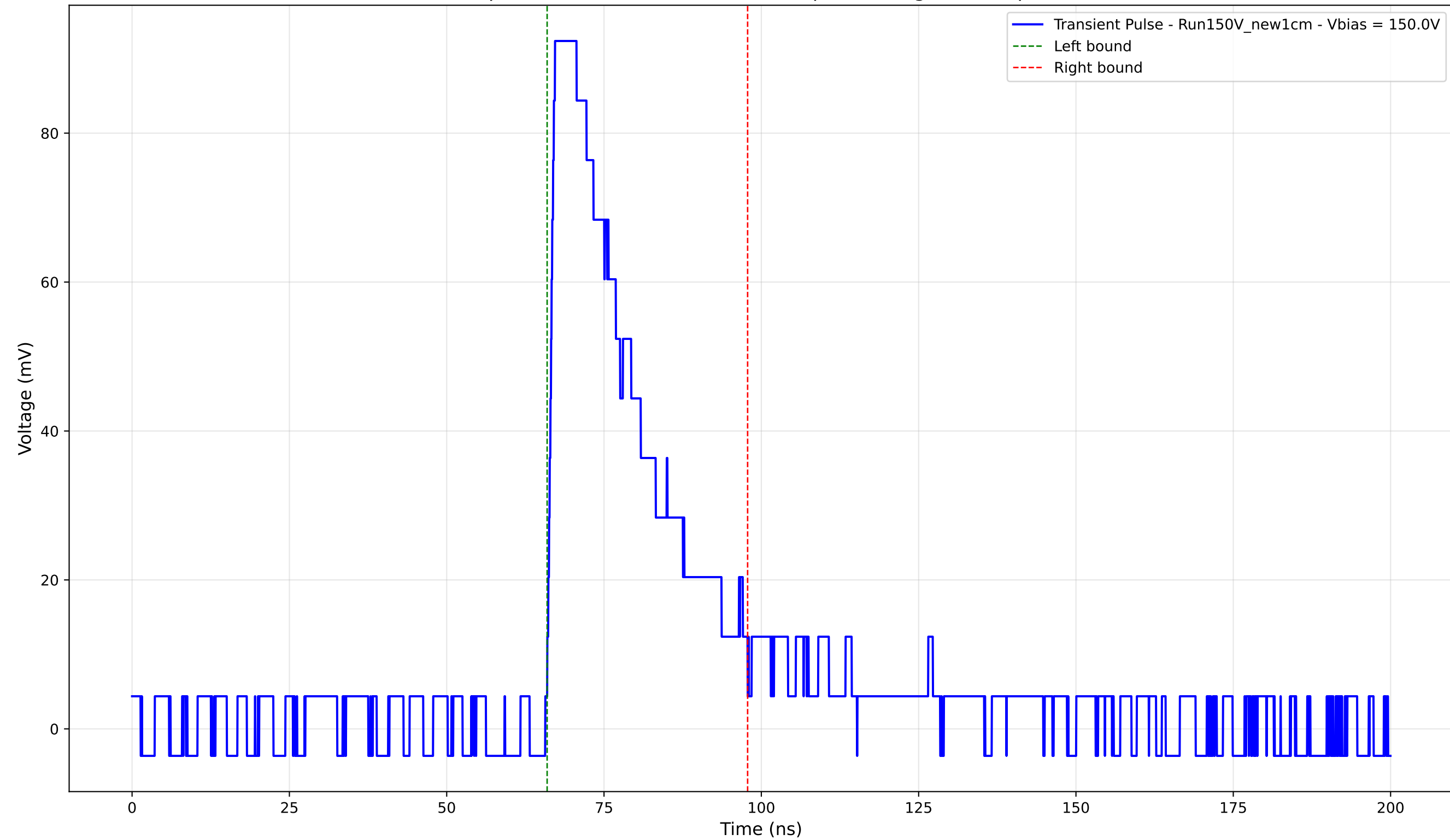
Transient Pulse - Sample: New1cm - Position: 1795.0 \mu\text{m} - Charge: 28.24 pC - Rise Time: 1.05 ns
