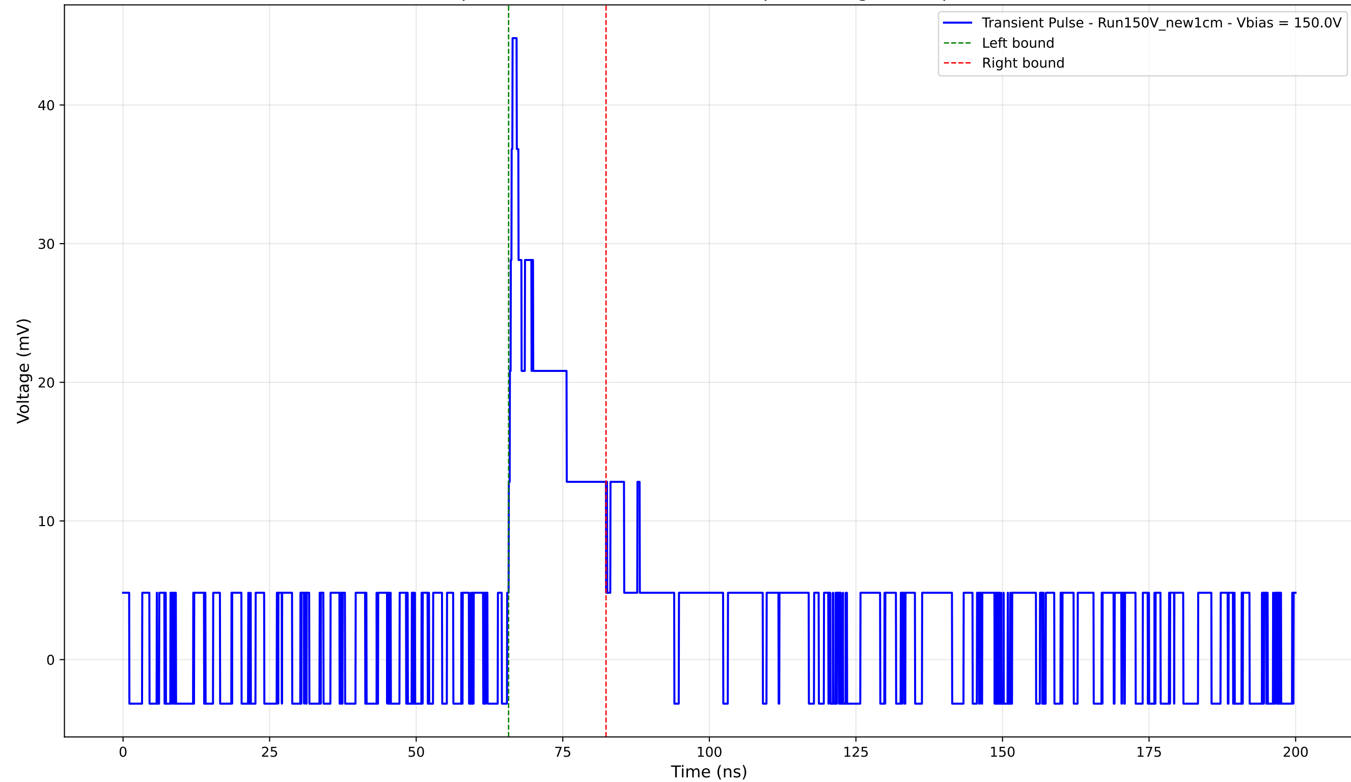
Transient Pulse - Sample: New1cm - Position: 2575.0 \mu\text{m} - Charge: 6.62 pC - Rise Time: 0.92 ns
