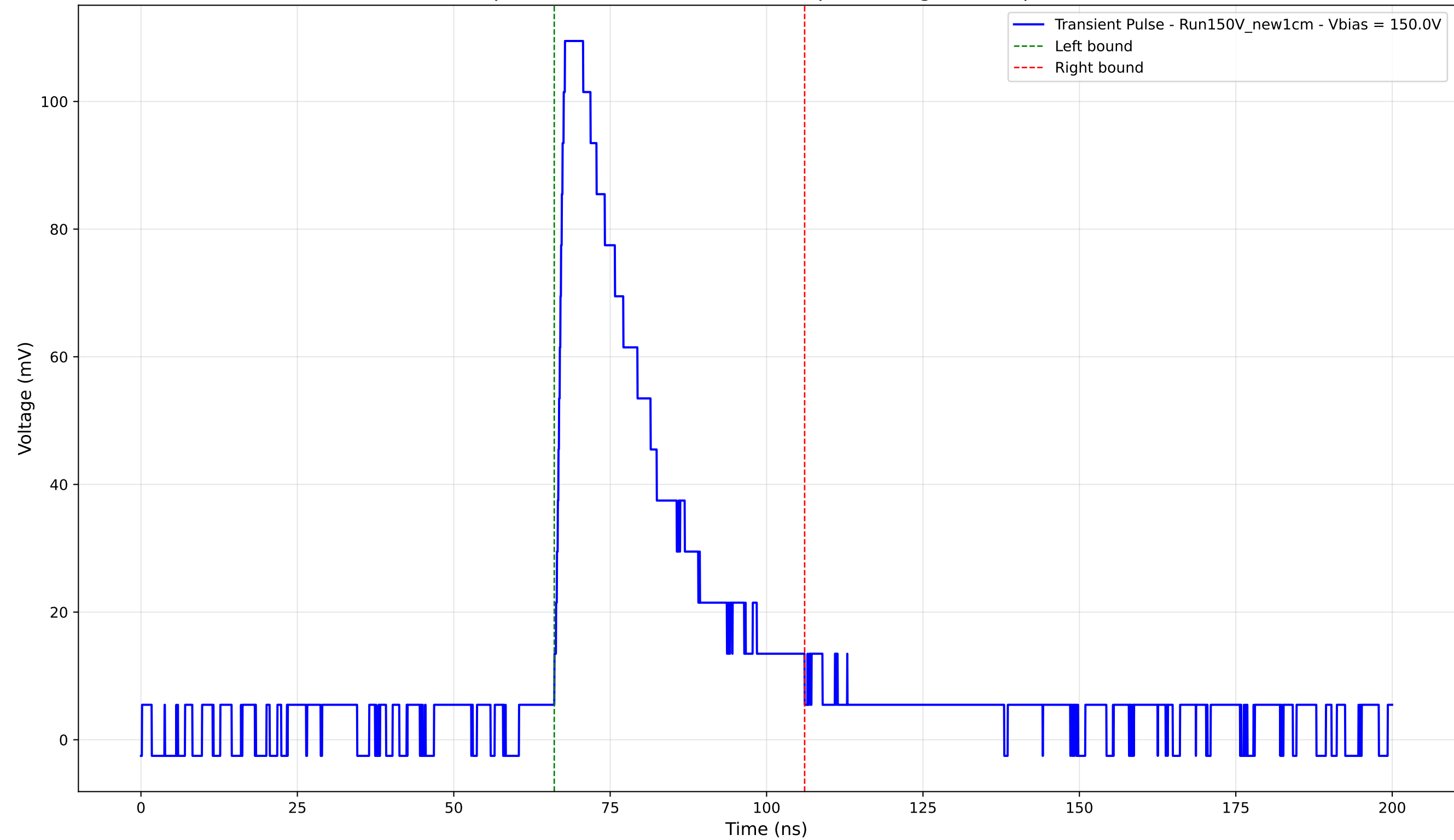
Transient Pulse - Sample: New1cm - Position: 1385.0 \mu\text{m} - Charge: 35.42 pC - Rise Time: 1.49 ns
