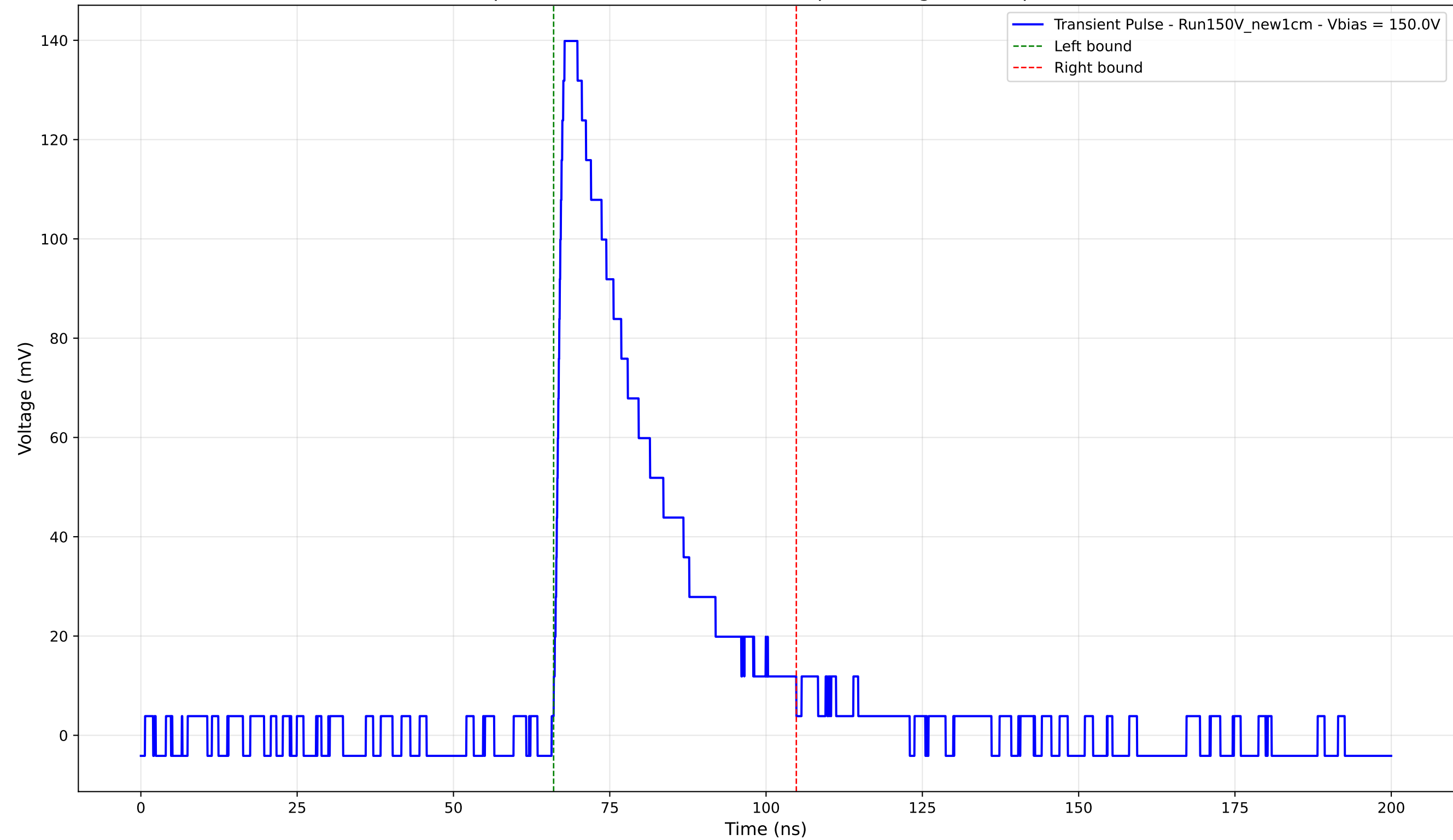
Transient Pulse - Sample: New1cm - Position: 3705.0 \mu\text{m} - Charge: 41.29 pC - Rise Time: 1.37 ns
