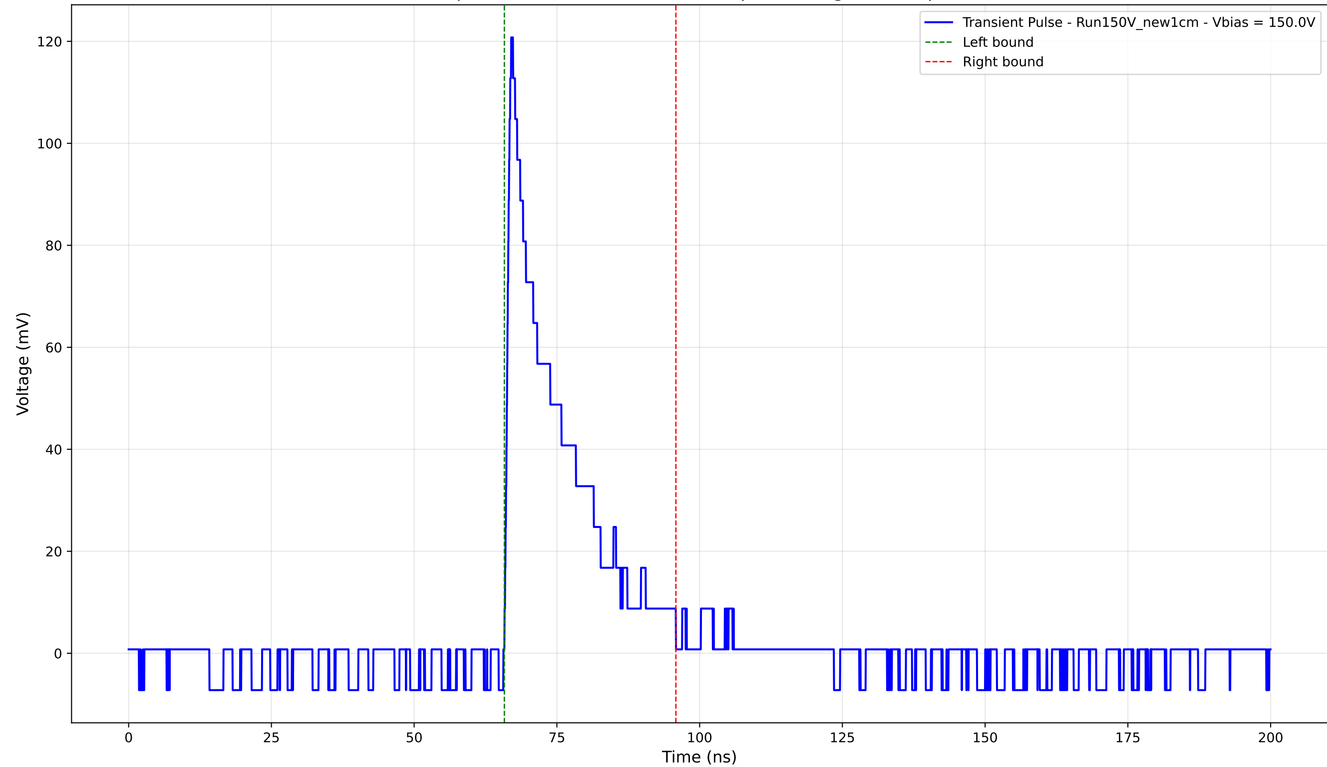
Transient Pulse - Sample: New1cm - Position: 140.0 \mu\text{m} - Charge: 21.84 pC - Rise Time: 0.91 ns
