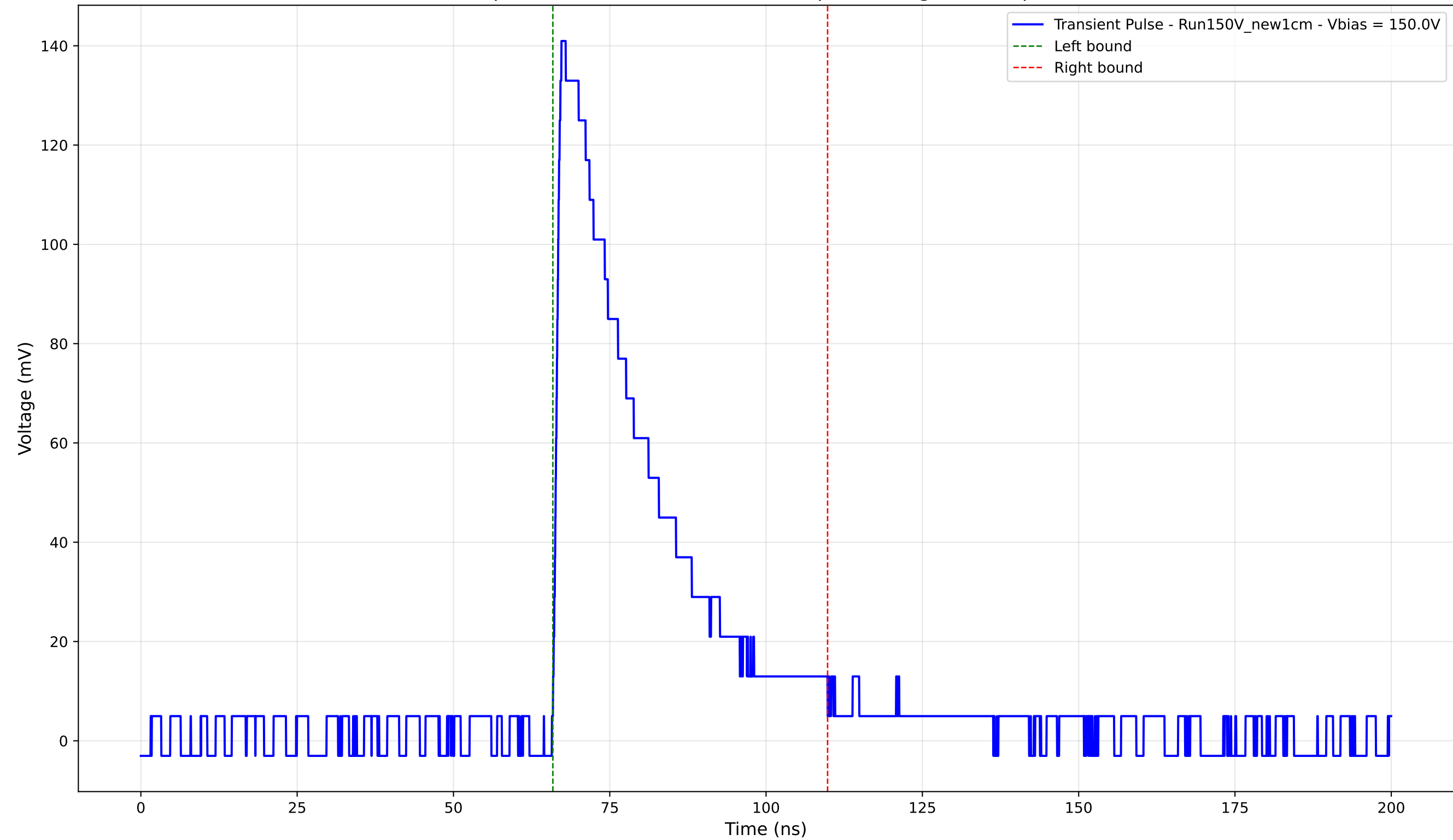
Transient Pulse - Sample: New1cm - Position: 3265.0 \mu\text{m} - Charge: 42.85 pC - Rise Time: 1.10 ns
