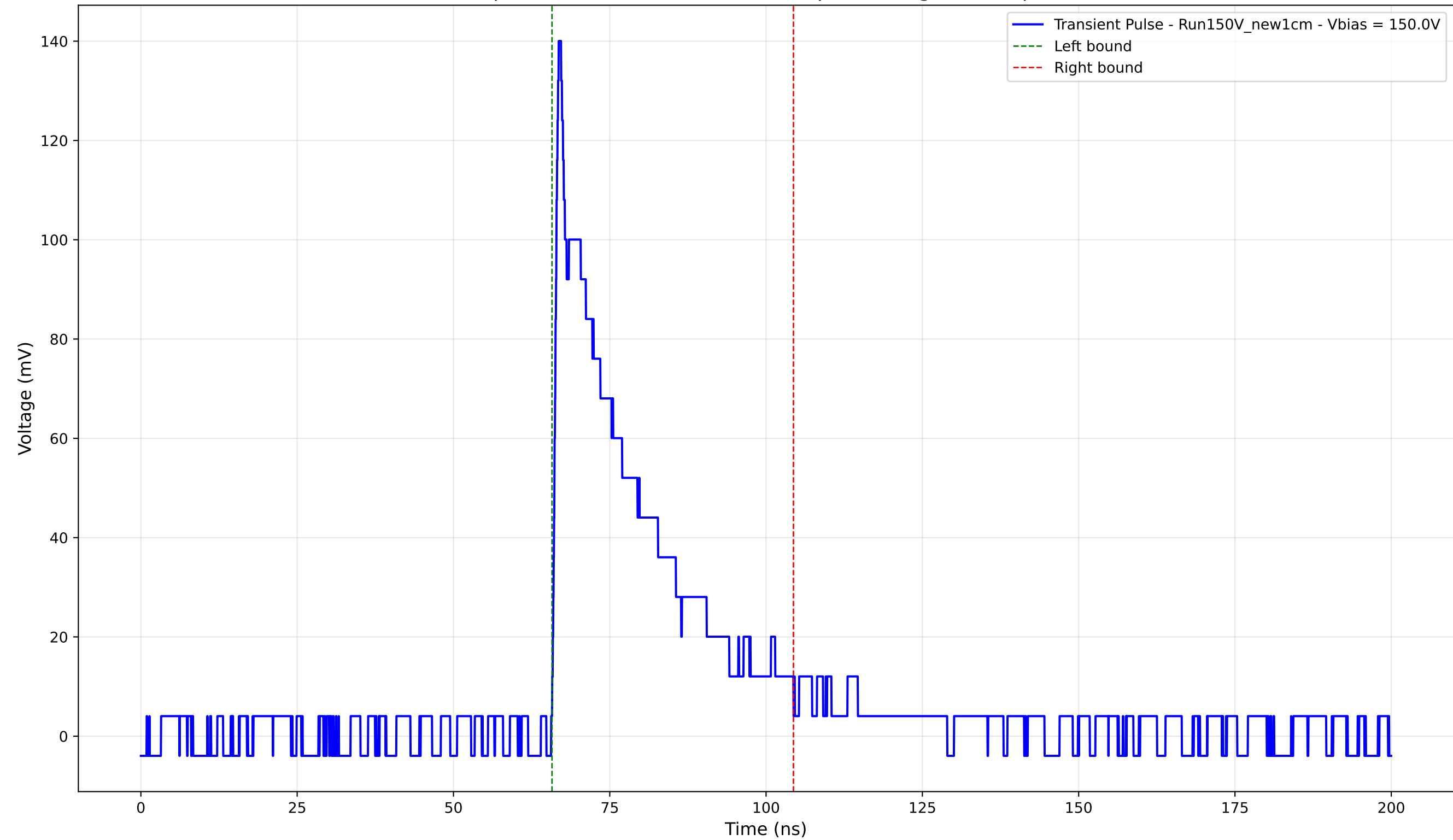
Transient Pulse - Sample: New1cm - Position: 2195.0 \mu\text{m} - Charge: 33.29 pC - Rise Time: 0.86 ns
