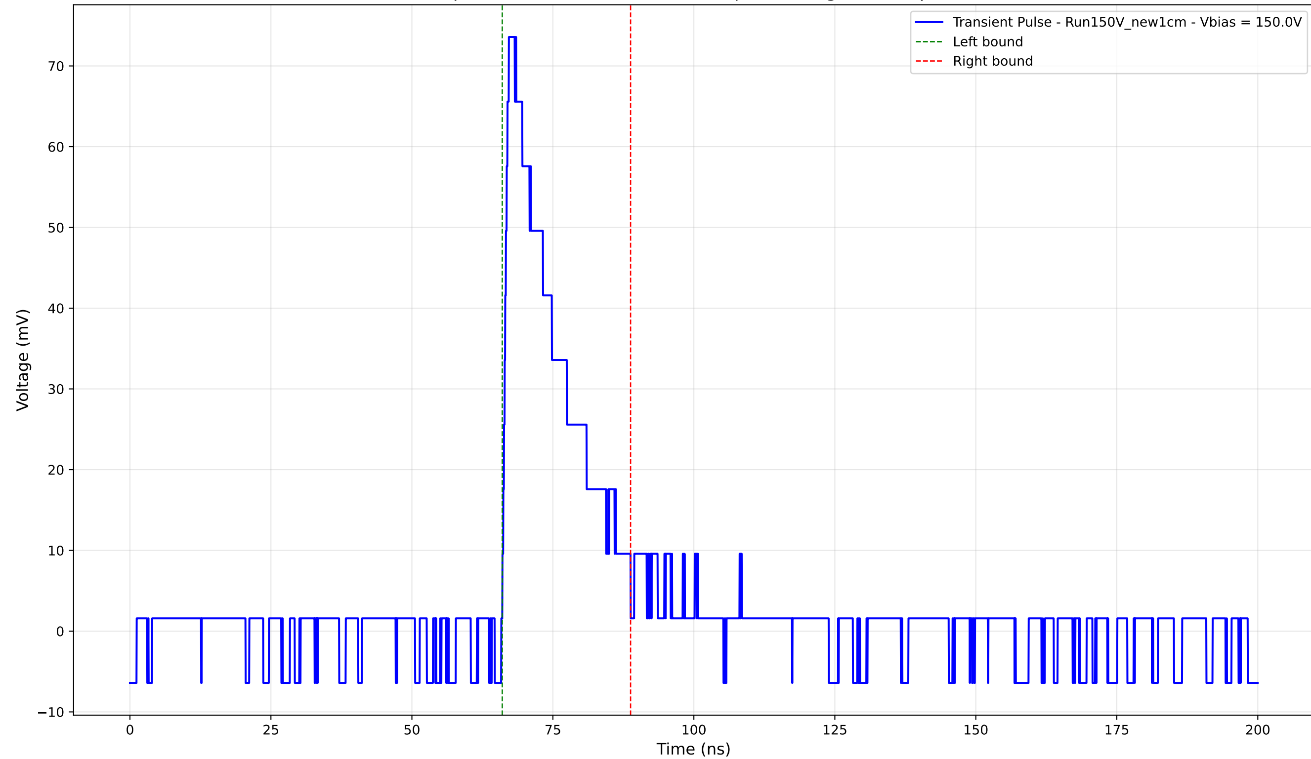
Transient Pulse - Sample: New1cm - Position: 465.0 \mu\text{m} - Charge: 15.23 pC - Rise Time: 1.15 ns
