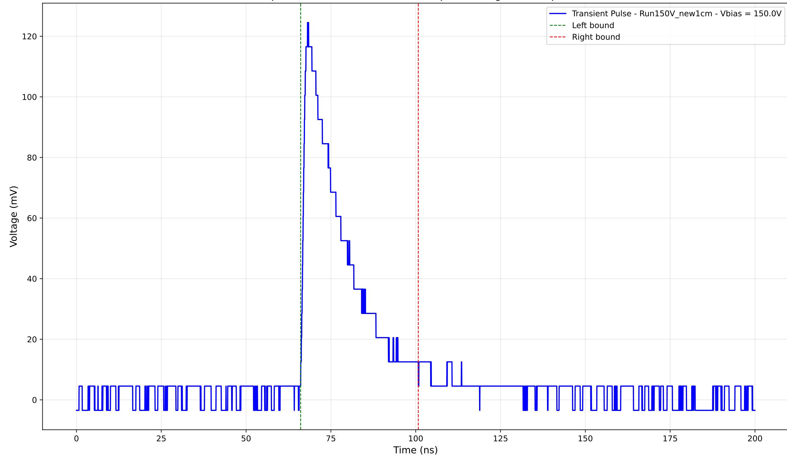
Transient Pulse - Sample: New1cm - Position: 765.0 \mu\text{m} - Charge: 31.88 pC - Rise Time: 1.54 ns
