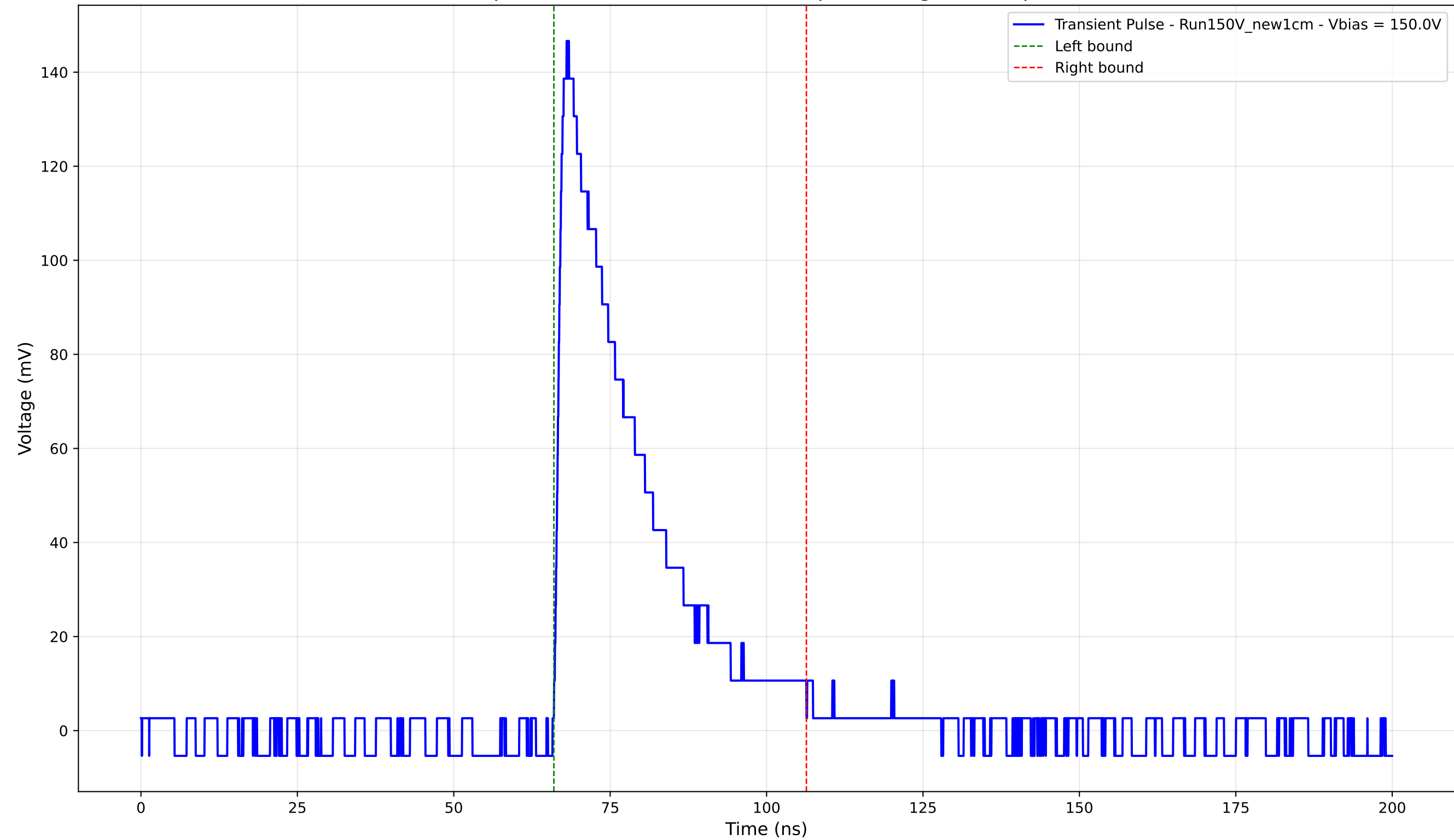
Transient Pulse - Sample: New1cm - Position: 4225.0 \mu\text{m} - Charge: 37.88 pC - Rise Time: 1.41 ns
