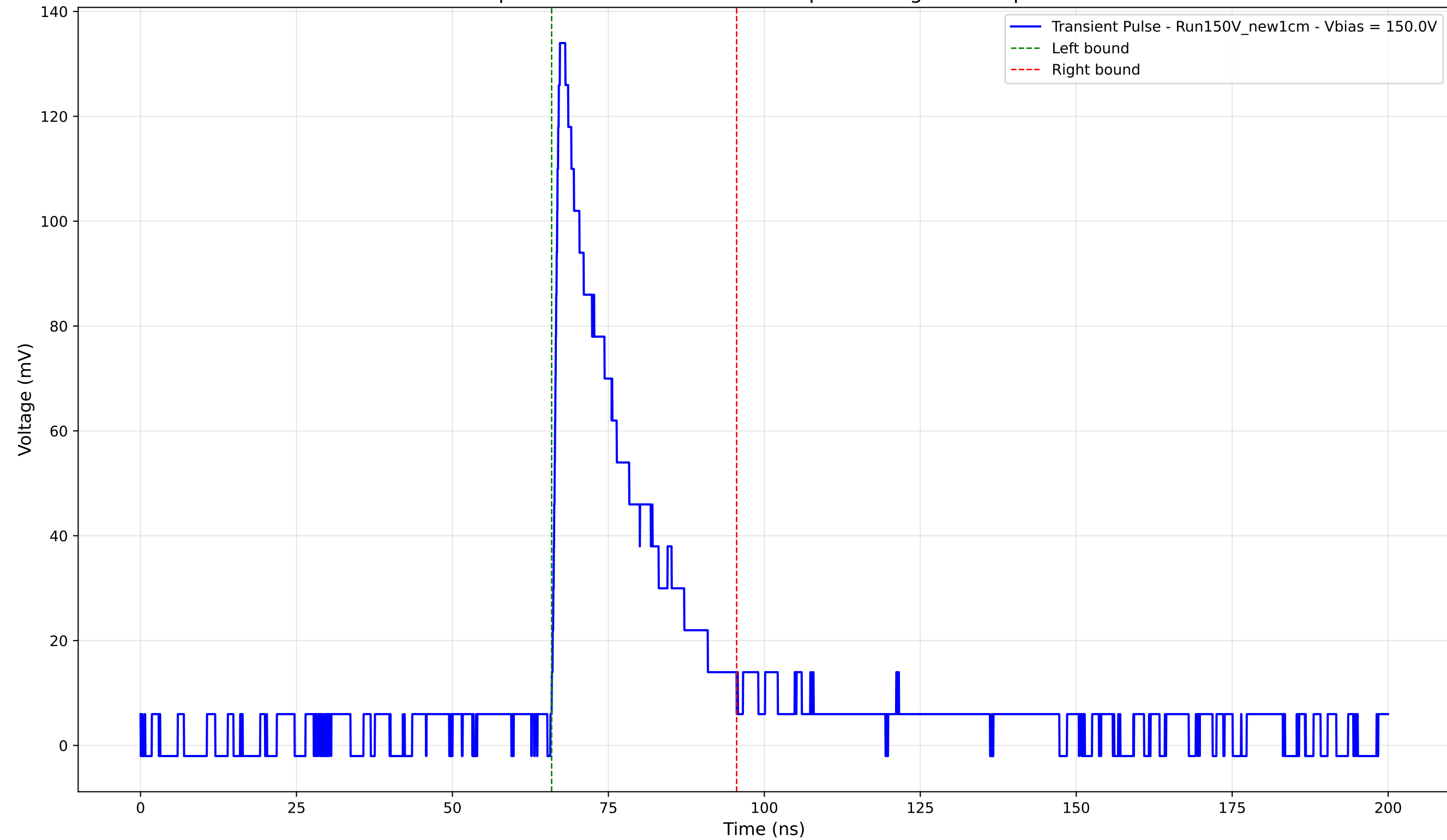
Transient Pulse - Sample: New1cm - Position: 380.0 \mu\text{m} - Charge: 30.45 pC - Rise Time: 1.12 ns
