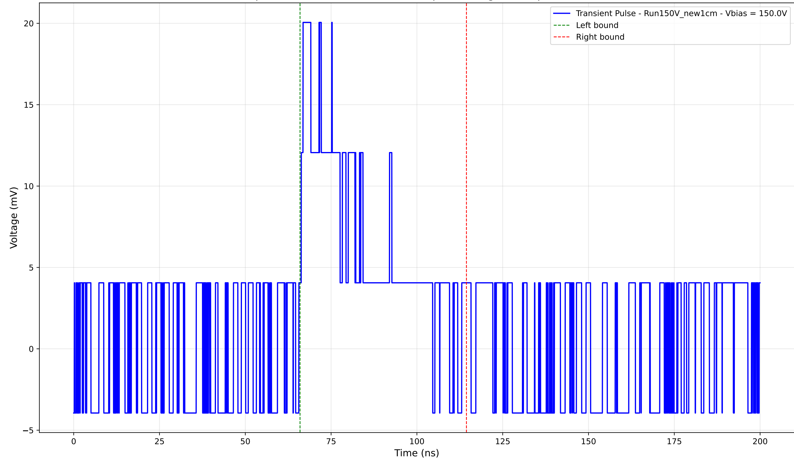
Transient Pulse - Sample: New1cm - Position: 3060.0 \mu\text{m} - Charge: 6.49 pC - Rise Time: 0.00 ns (N/A)
