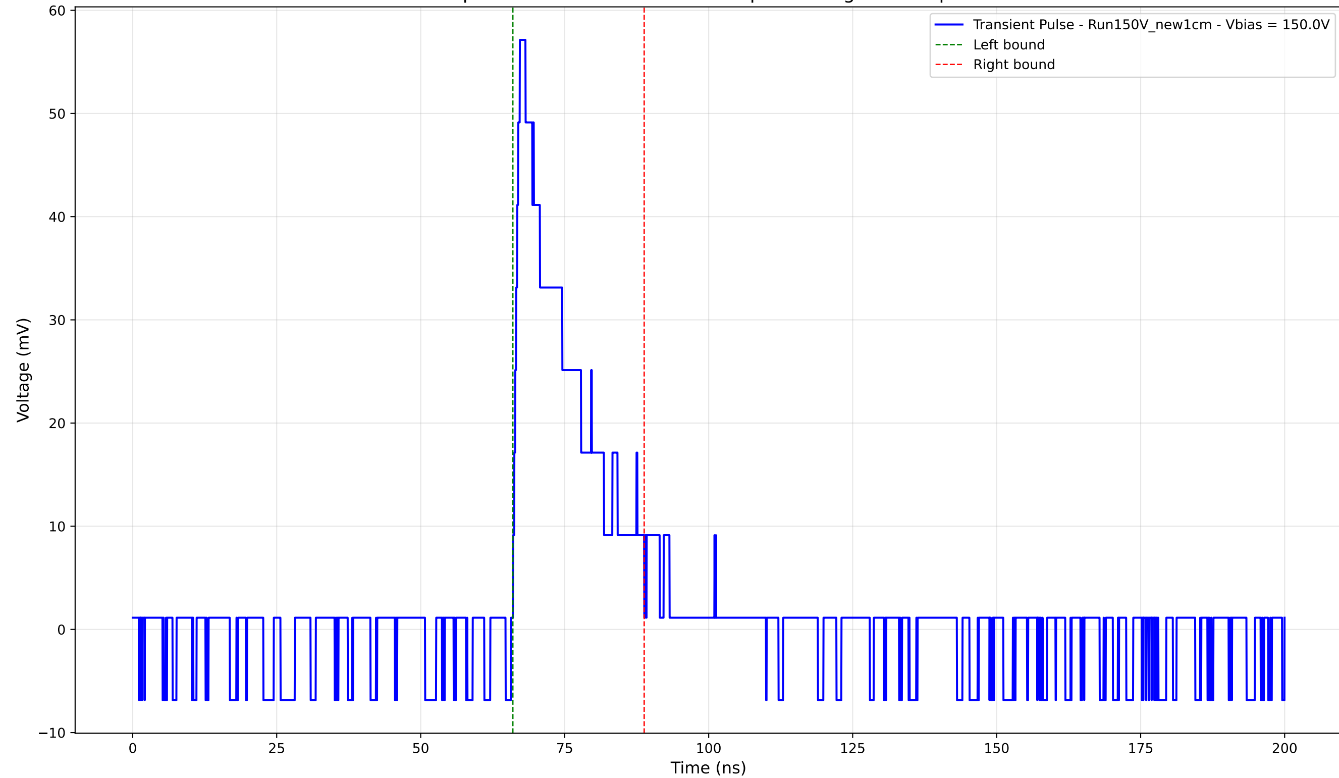
Transient Pulse - Sample: New1cm - Position: 480.0 \mu\text{m} - Charge: 11.16 pC - Rise Time: 1.19 ns
