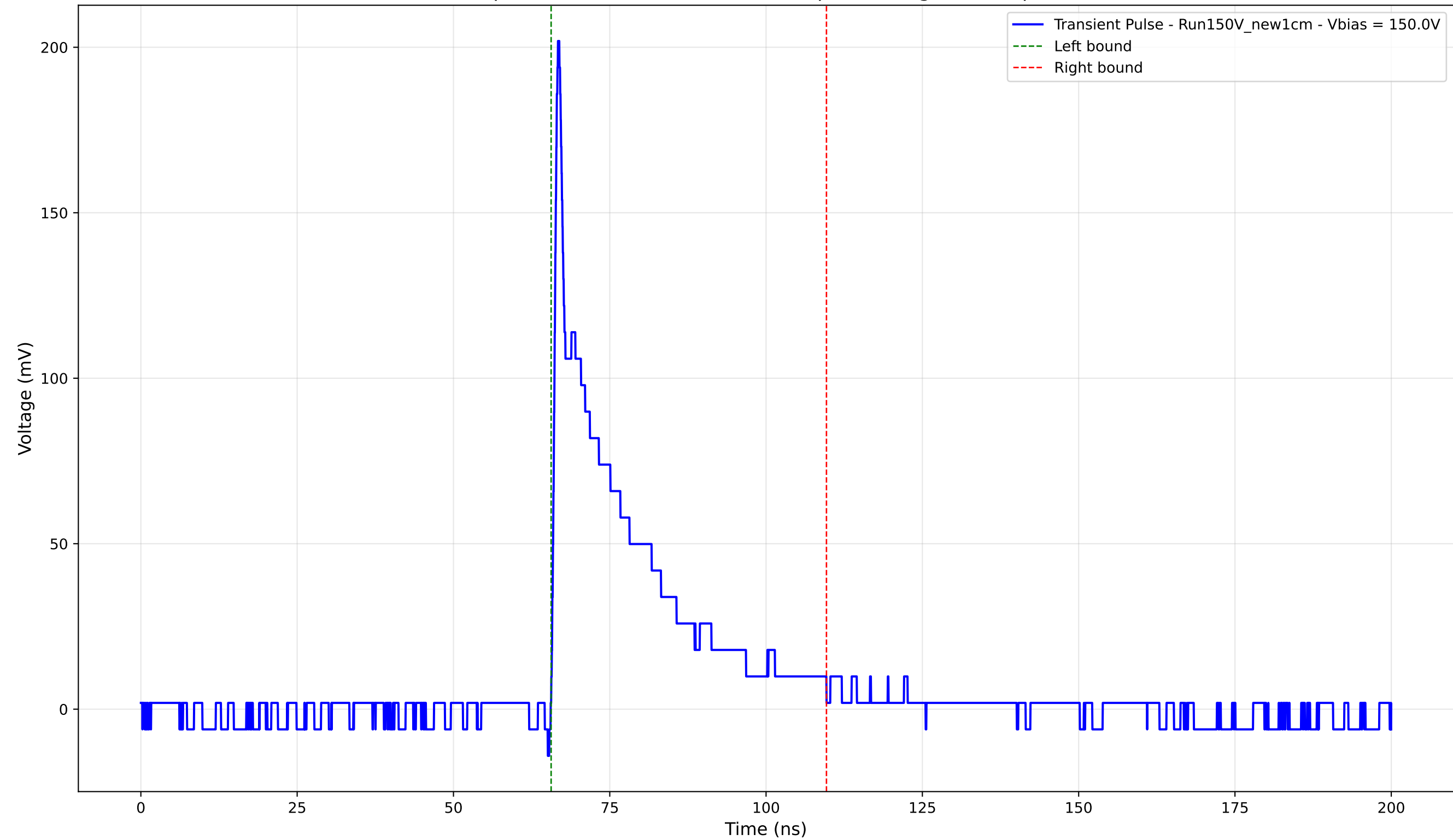
Transient Pulse - Sample: New1cm - Position: 2705.0 \mu\text{m} - Charge: 36.92 pC - Rise Time: 0.77 ns
