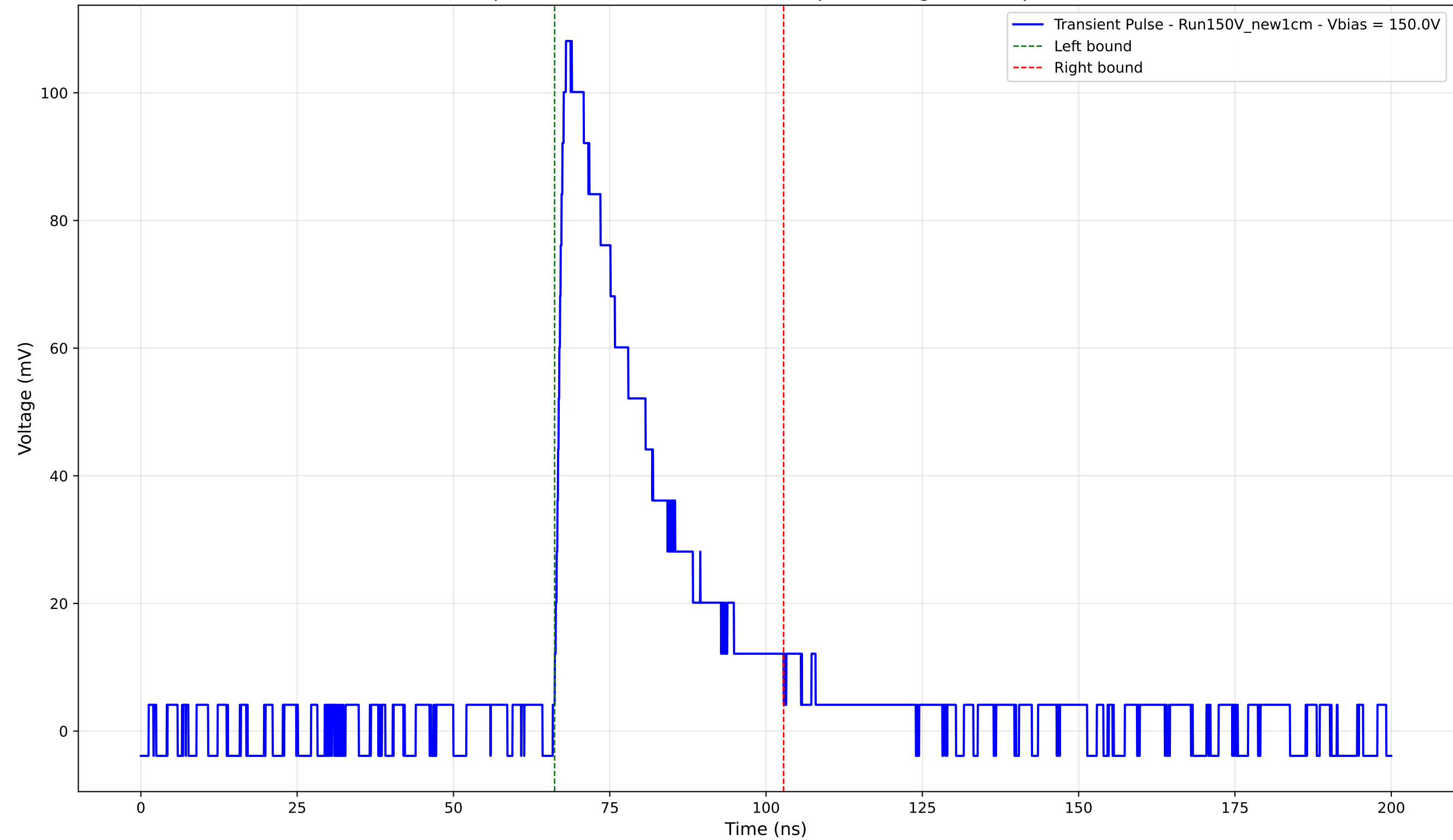
Transient Pulse - Sample: New1cm - Position: 1435.0 \mu\text{m} - Charge: 31.22 pC - Rise Time: 1.42 ns
