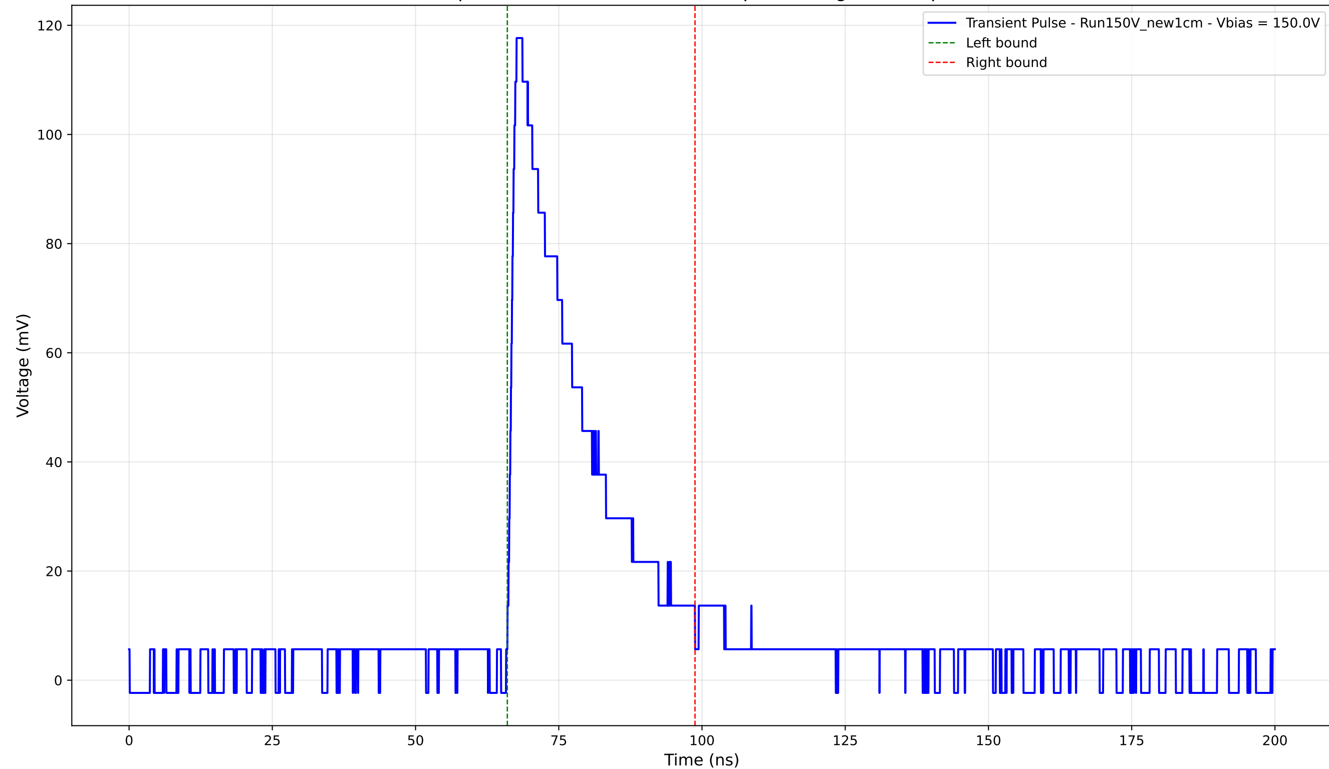
Transient Pulse - Sample: New1cm - Position: 670.0 \mu\text{m} - Charge: 30.61 pC - Rise Time: 1.36 ns
