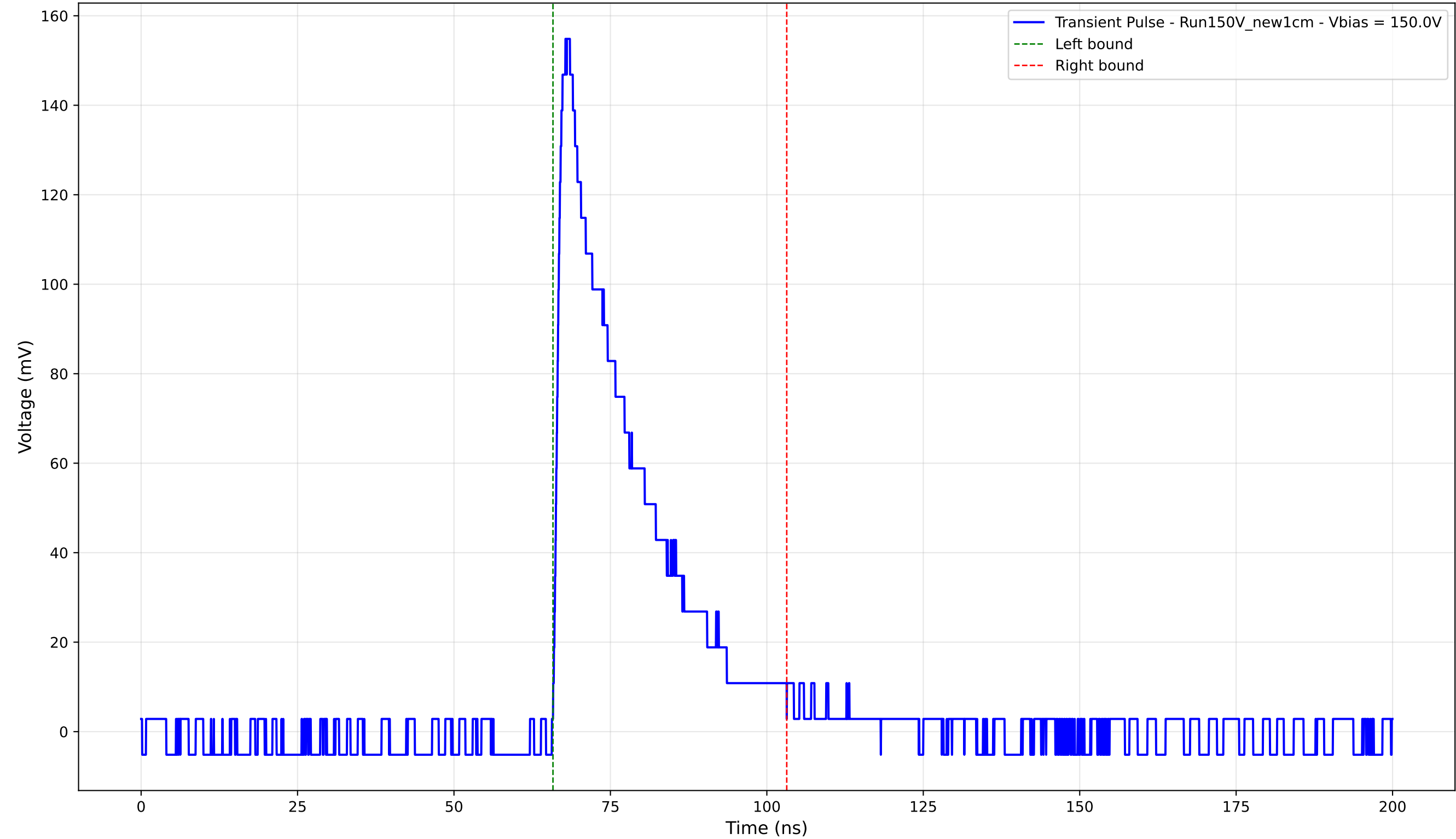
Transient Pulse - Sample: New1cm - Position: 4415.0 \mu\text{m} - Charge: 38.21 pC - Rise Time: 1.39 ns
