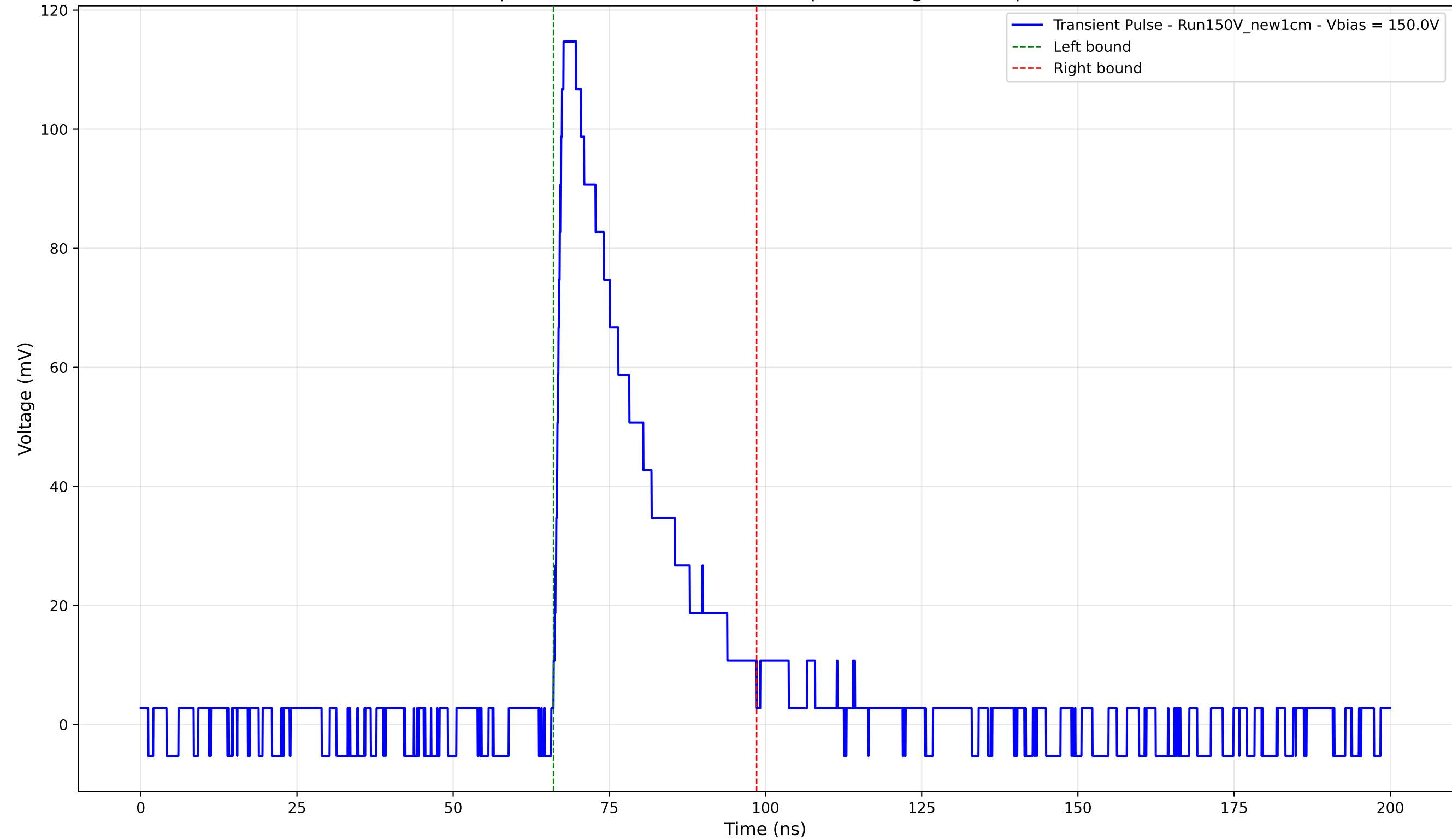
Transient Pulse - Sample: New1cm - Position: 785.0 \mu\text{m} - Charge: 30.60 pC - Rise Time: 1.18 ns
