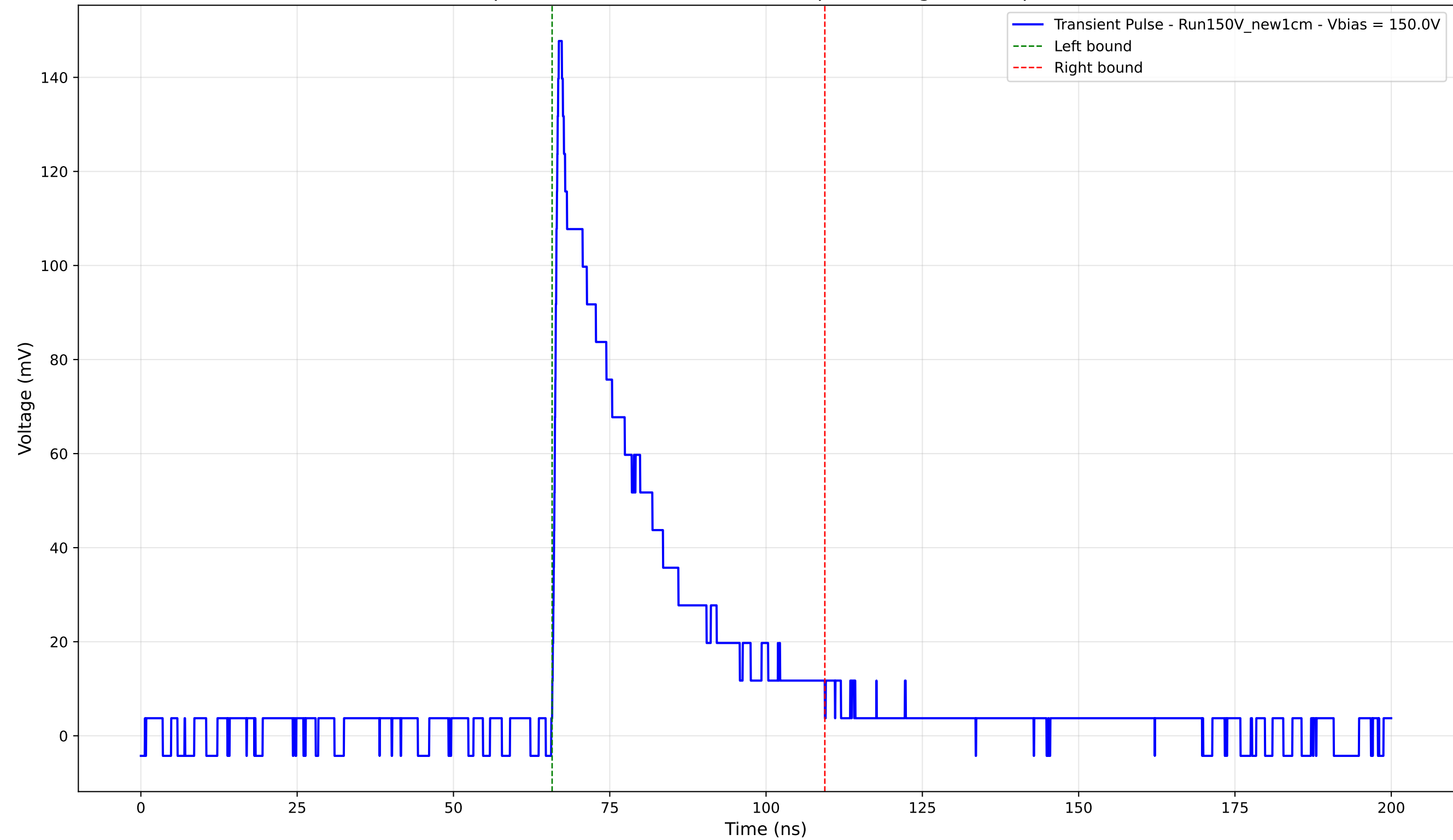
Transient Pulse - Sample: New1cm - Position: 2965.0 \mu\text{m} - Charge: 37.93 pC - Rise Time: 0.87 ns
