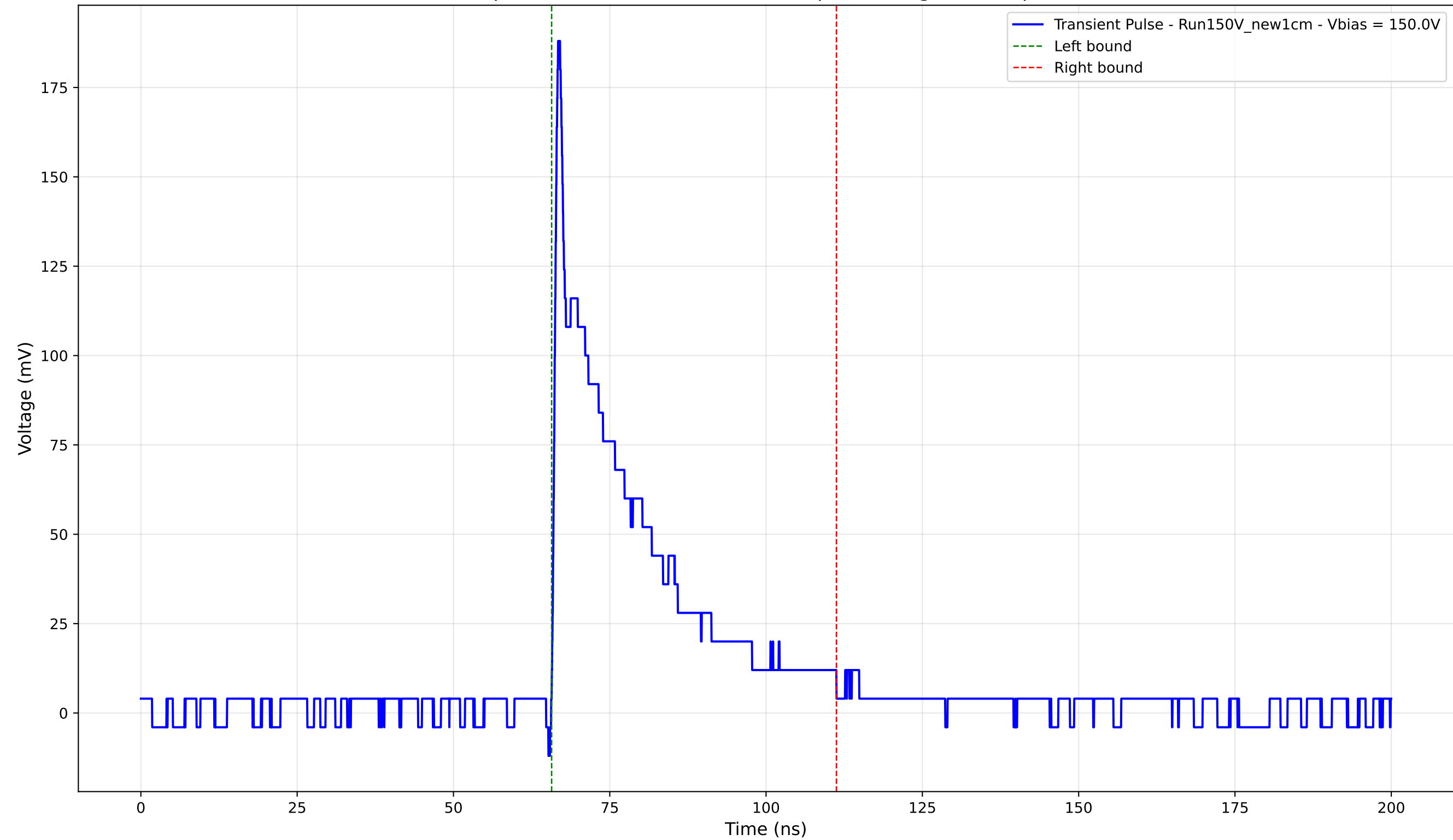
Transient Pulse - Sample: New1cm - Position: 2785.0 \mu\text{m} - Charge: 40.21 pC - Rise Time: 0.80 ns
