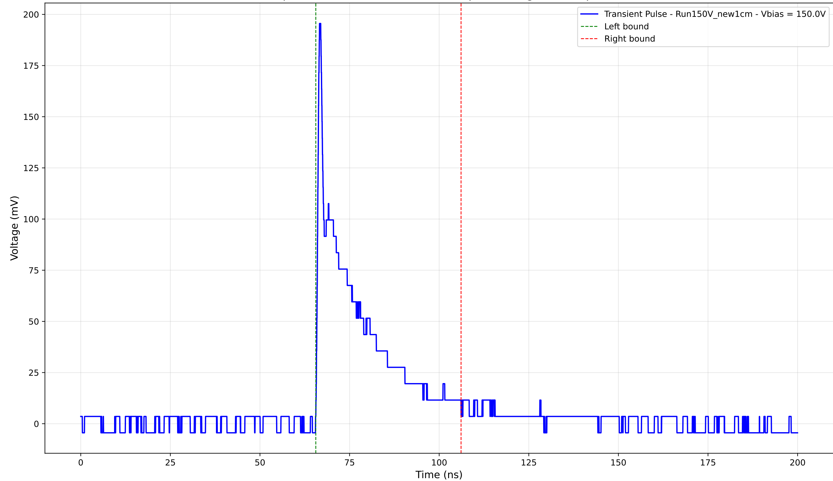
Transient Pulse - Sample: New1cm - Position: 2445.0 \mu\text{m} - Charge: 35.49 pC - Rise Time: 0.80 ns
