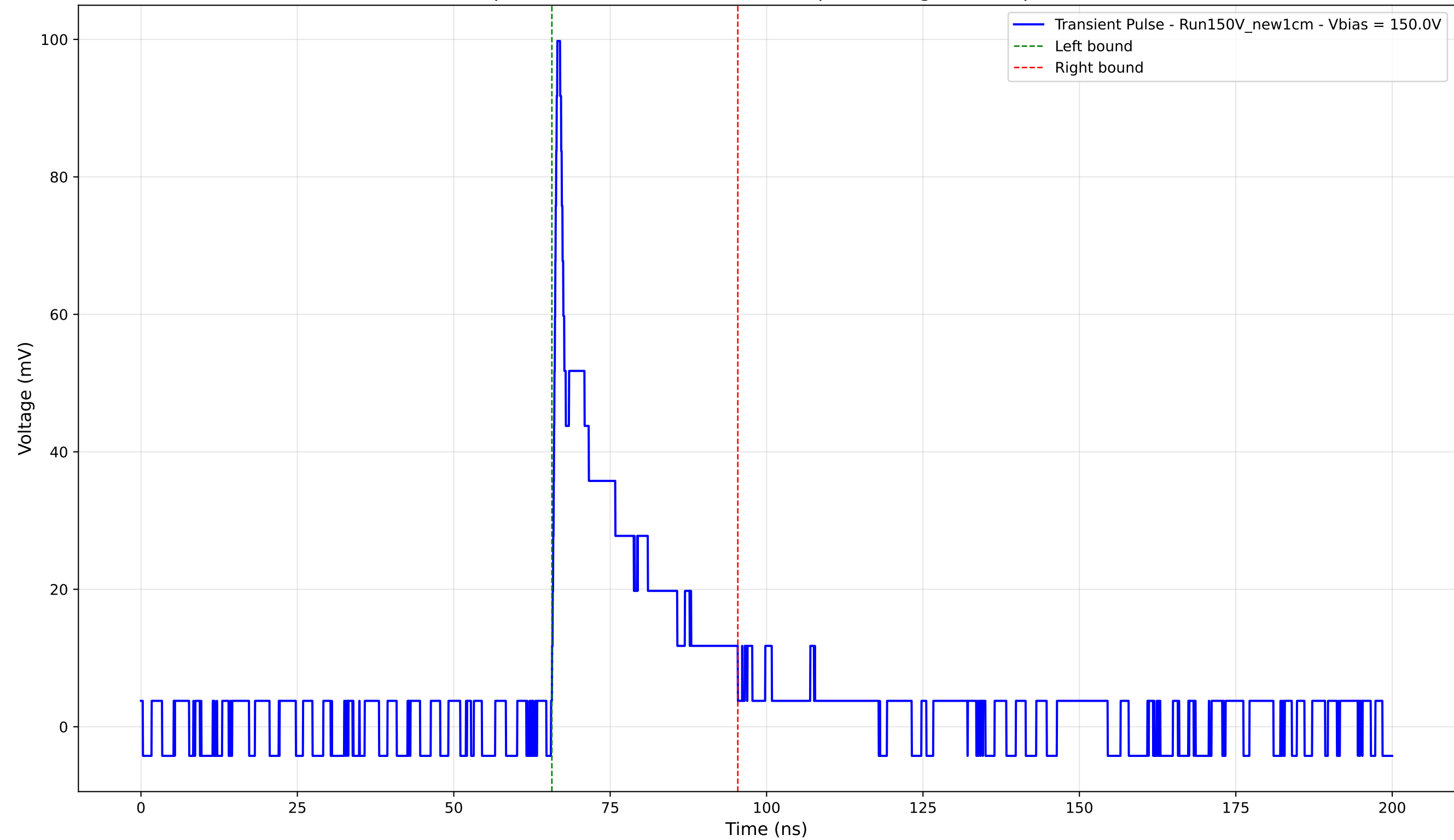
Transient Pulse - Sample: New1cm - Position: 2500.0 \mu\text{m} - Charge: 16.77 pC - Rise Time: 0.74 ns
