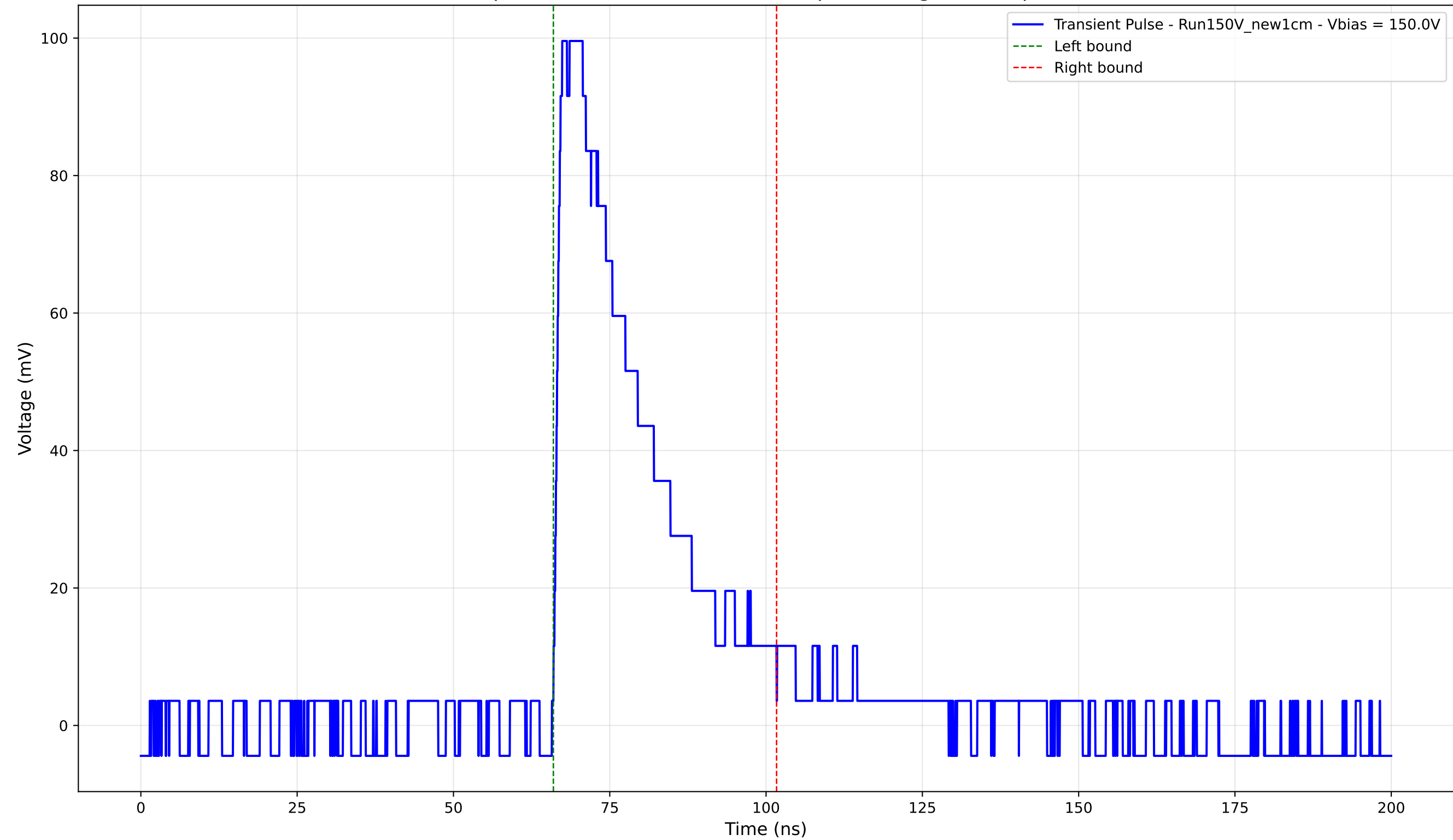
Transient Pulse - Sample: New1cm - Position: 1765.0 \mu\text{m} - Charge: 30.04 pC - Rise Time: 1.12 ns
