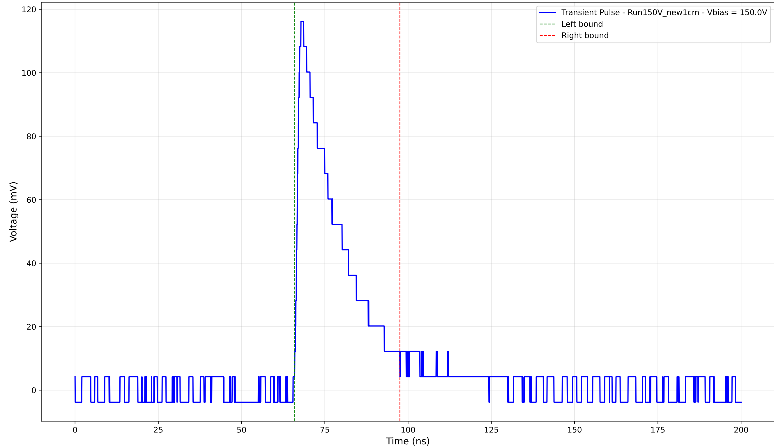
Transient Pulse - Sample: New1cm - Position: 4175.0 \mu\text{m} - Charge: 30.05 pC - Rise Time: 1.48 ns
