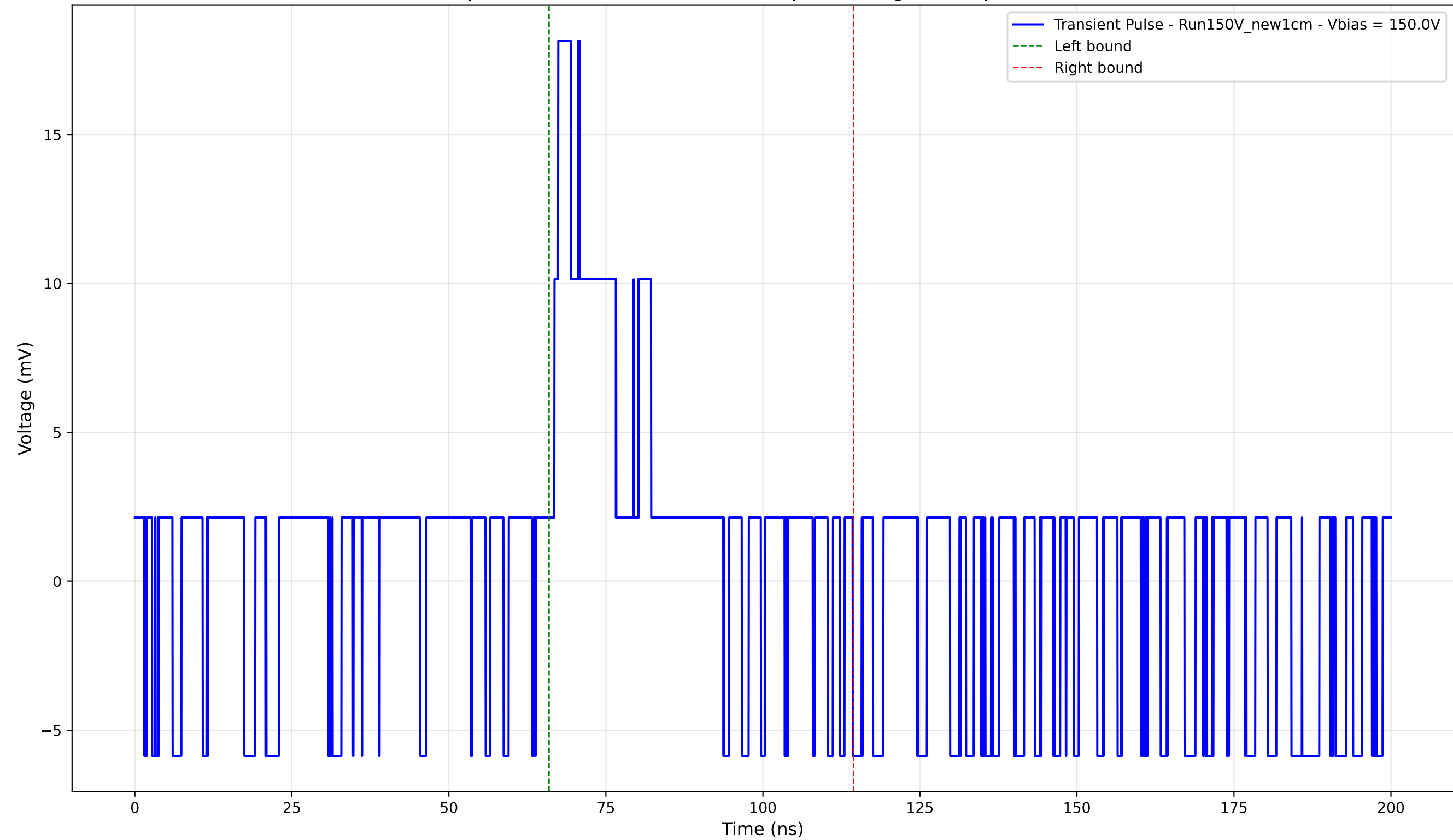
Transient Pulse - Sample: New1cm - Position: 1530.0 \mu\text{m} - Charge: 3.55 pC - Rise Time: 0.00 ns (N/A)
