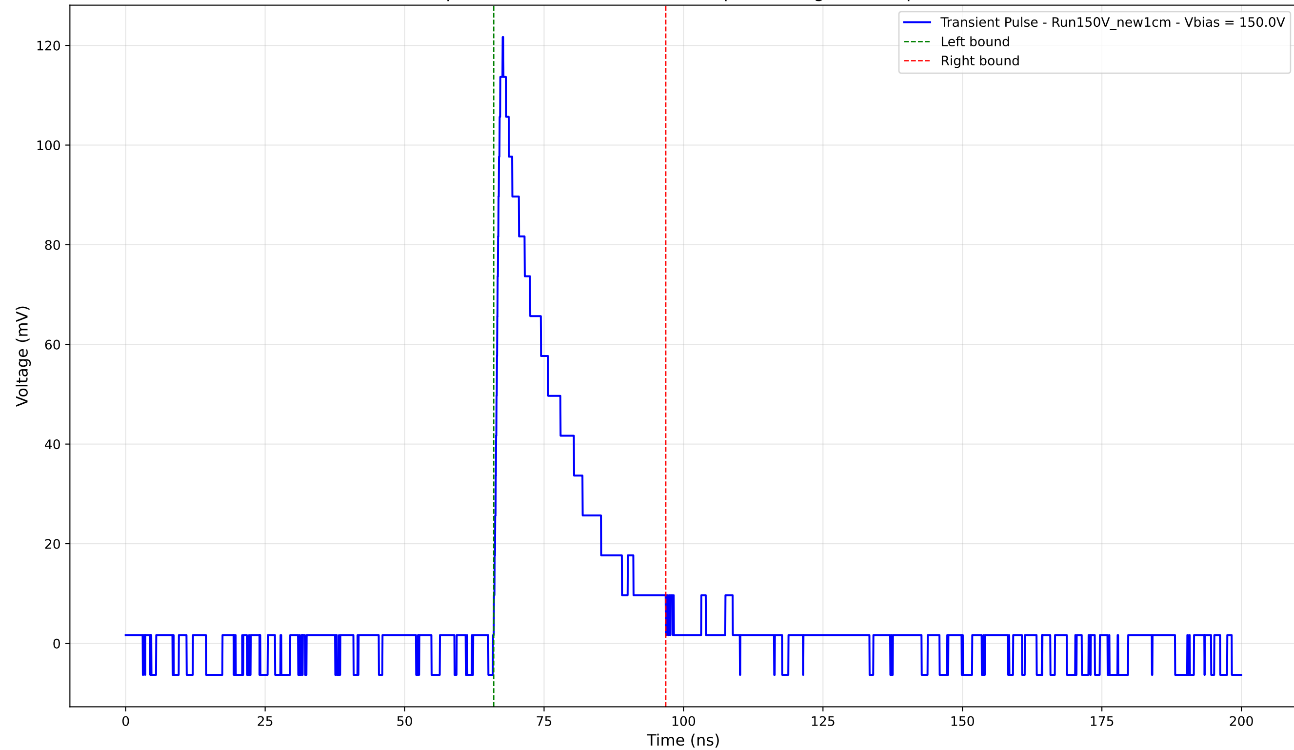
Transient Pulse - Sample: New1cm - Position: 420.0 \mu\text{m} - Charge: 25.24 pC - Rise Time: 1.03 ns
