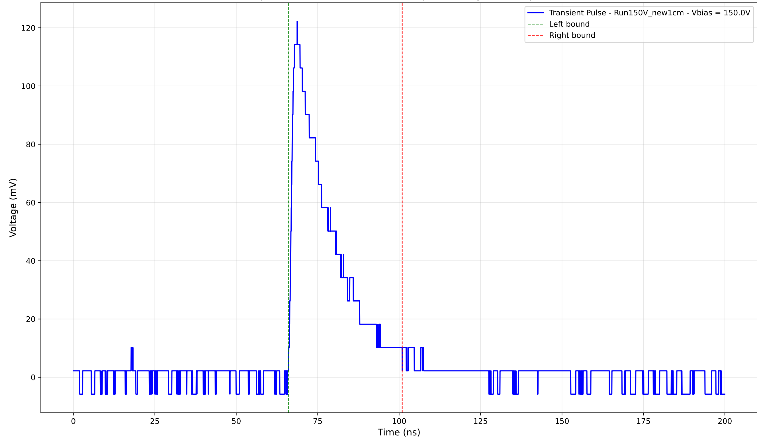
Transient Pulse - Sample: New1cm - Position: 900.0 \mu\text{m} - Charge: 30.44 pC - Rise Time: 1.55 ns
