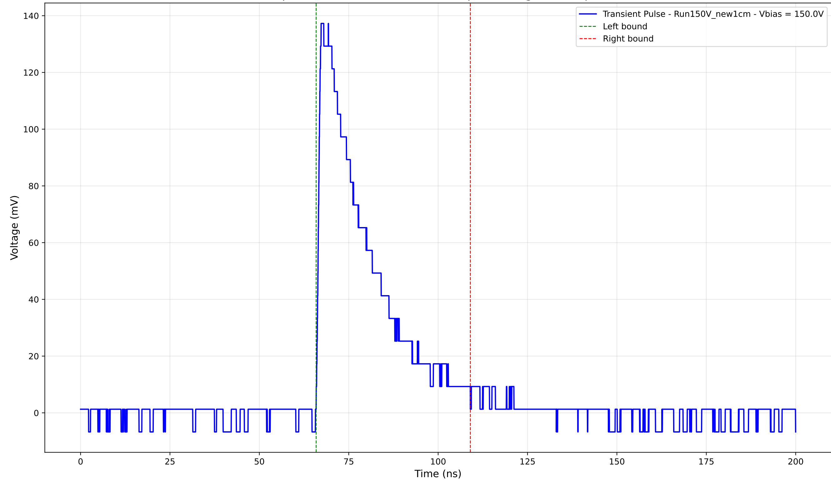
Transient Pulse - Sample: New1cm - Position: 3270.0 \mu\text{m} - Charge: 41.09 pC - Rise Time: 1.09 ns
