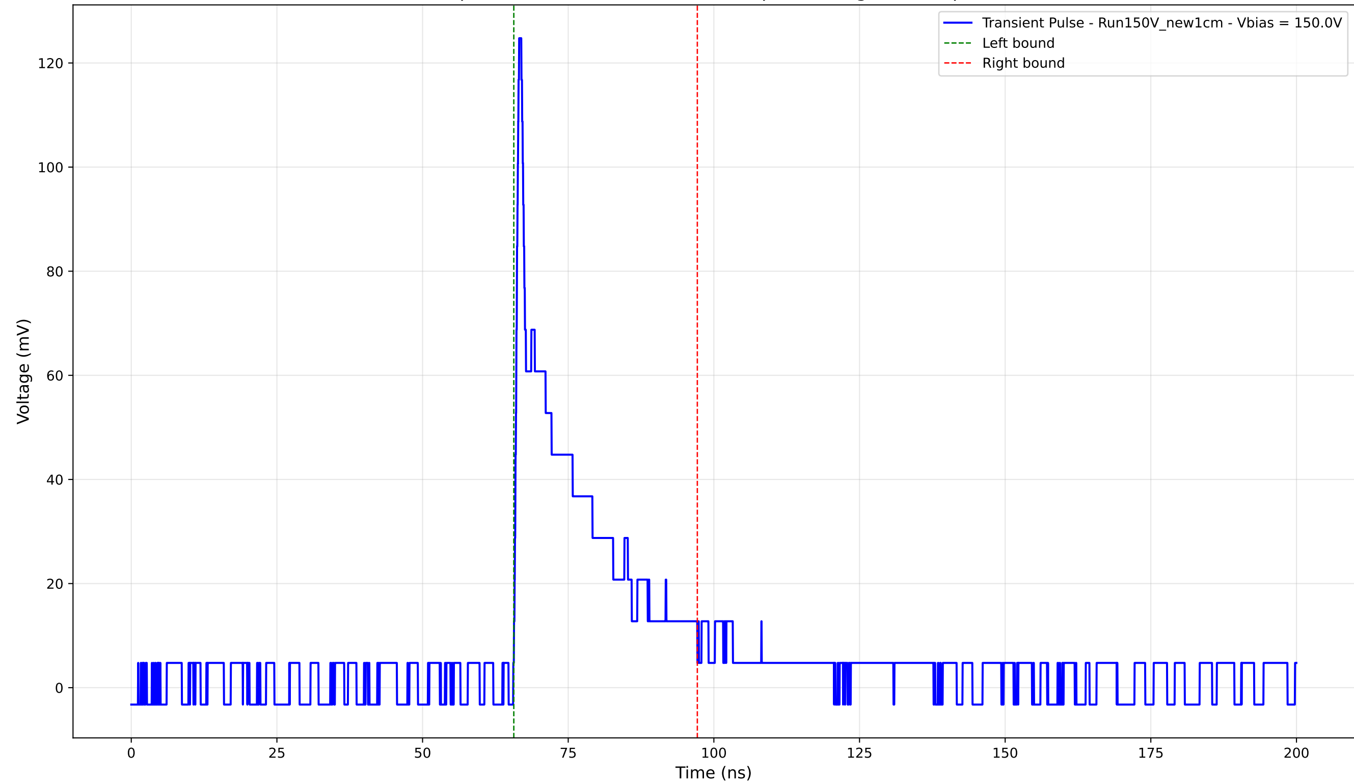
Transient Pulse - Sample: New1cm - Position: 2490.0 \mu\text{m} - Charge: 21.23 pC - Rise Time: 0.78 ns
