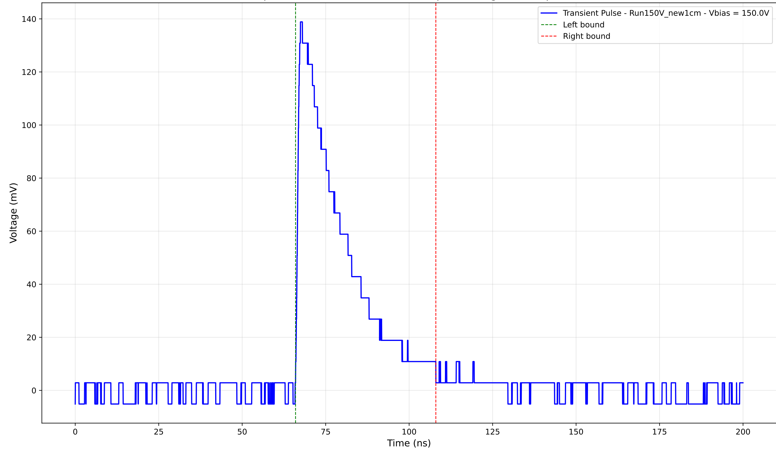
Transient Pulse - Sample: New1cm - Position: 3350.0 \mu\text{m} - Charge: 40.40 pC - Rise Time: 1.11 ns
