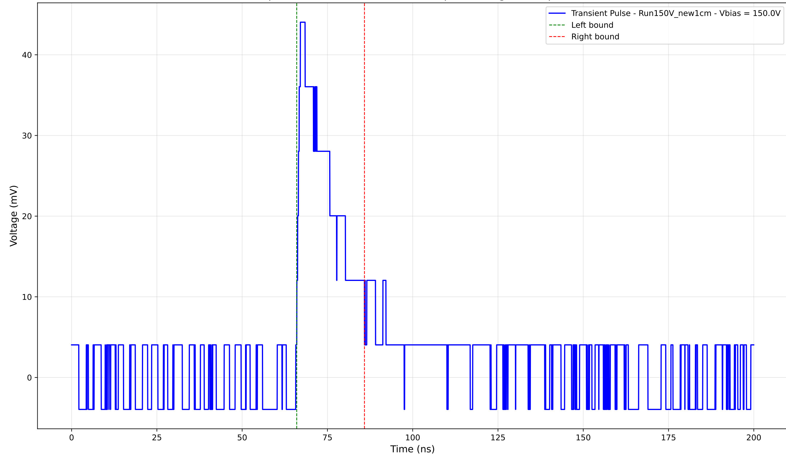
Transient Pulse - Sample: New1cm - Position: 4540.0 \mu\text{m} - Charge: 9.45 pC - Rise Time: 1.06 ns
