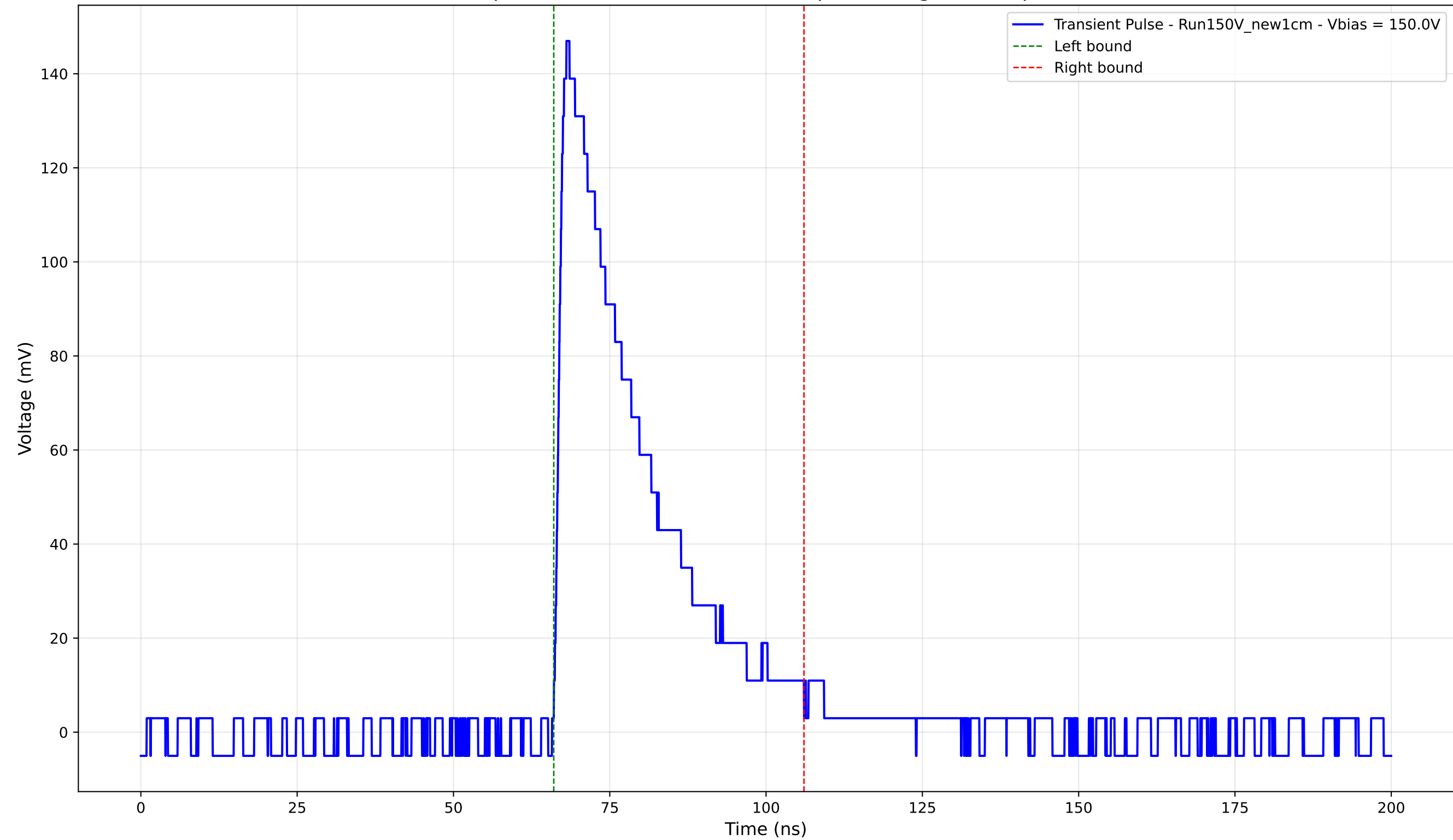
Transient Pulse - Sample: New1cm - Position: 3740.0 \mu\text{m} - Charge: 41.12 pC - Rise Time: 1.47 ns
