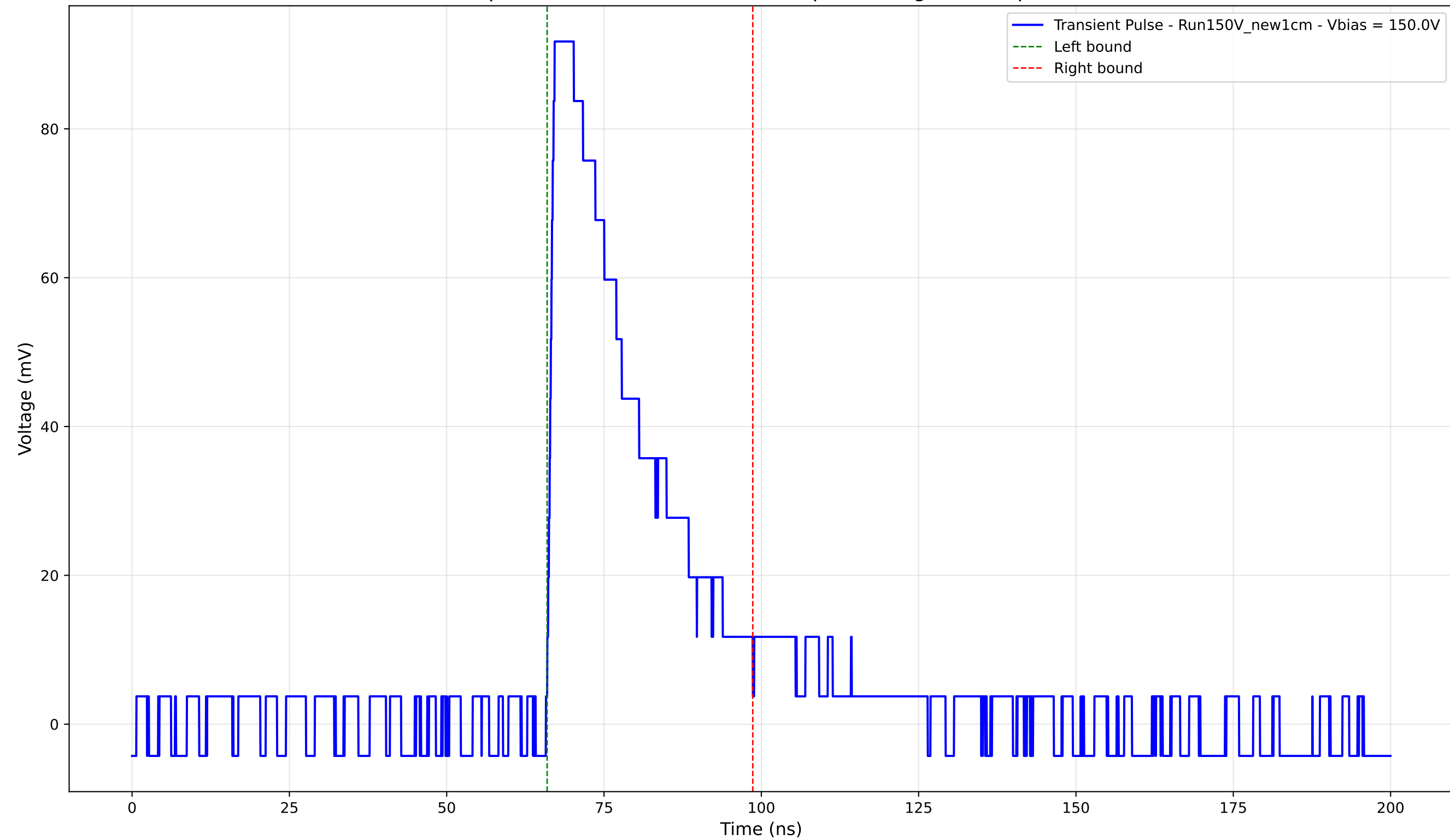
Transient Pulse - Sample: New1cm - Position: 1830.0 \mu\text{m} - Charge: 27.93 pC - Rise Time: 1.01 ns
