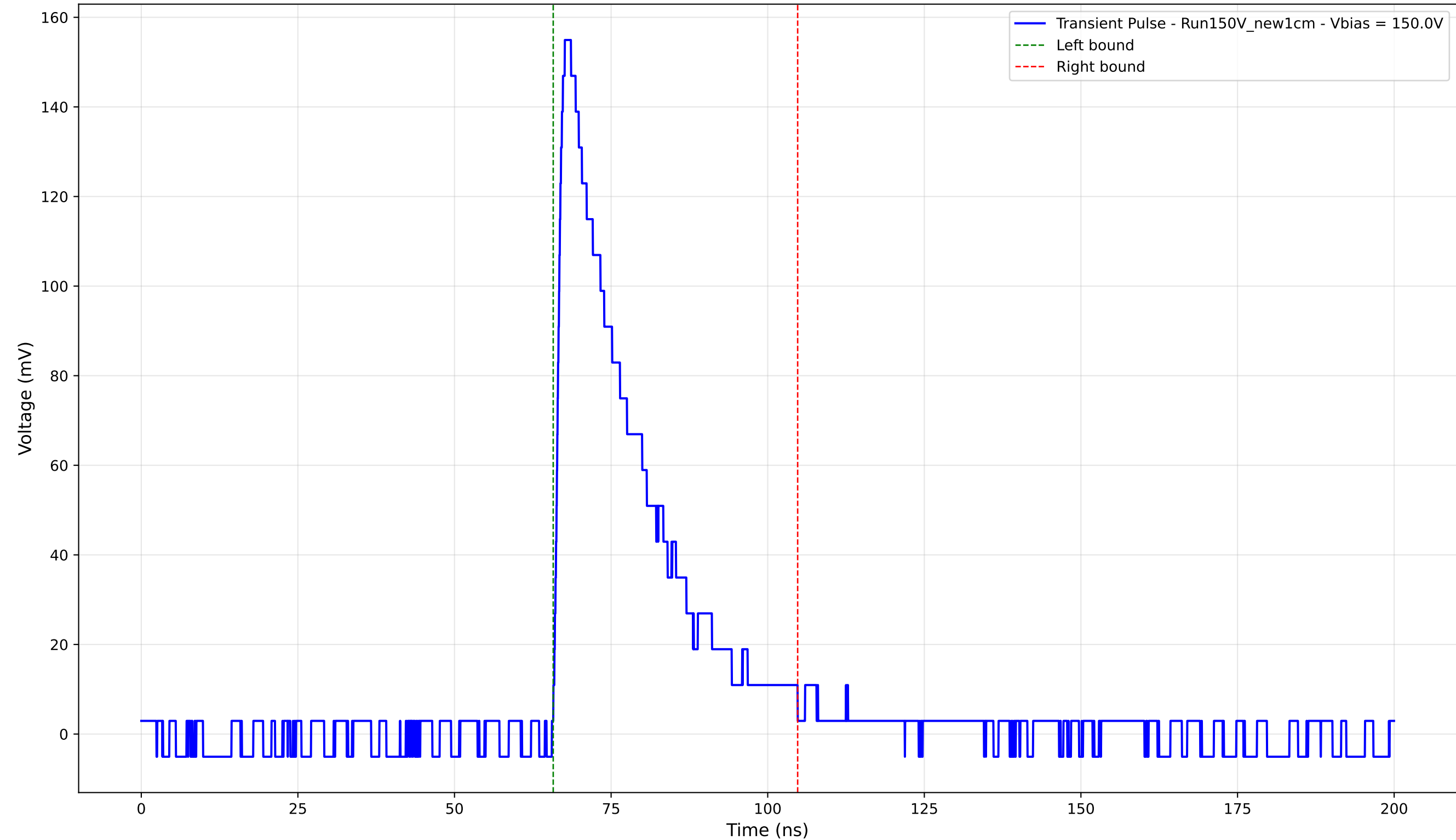
Transient Pulse - Sample: New1cm - Position: 4390.0 \mu\text{m} - Charge: 40.46 pC - Rise Time: 1.37 ns
