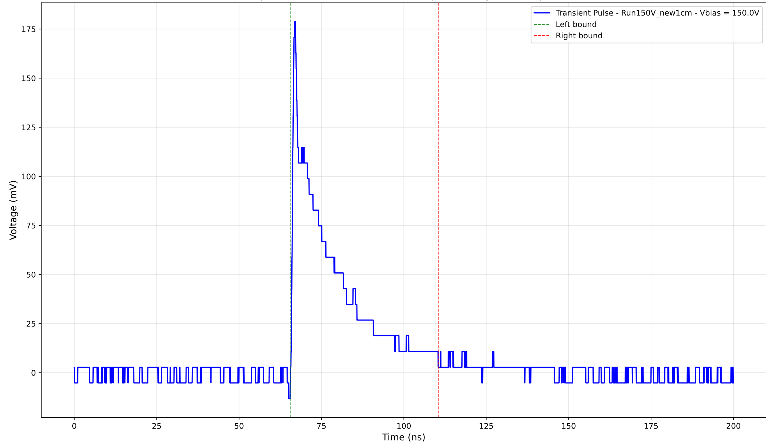
Transient Pulse - Sample: New1cm - Position: 2810.0 \mu\text{m} - Charge: 37.80 pC - Rise Time: 0.78 ns
