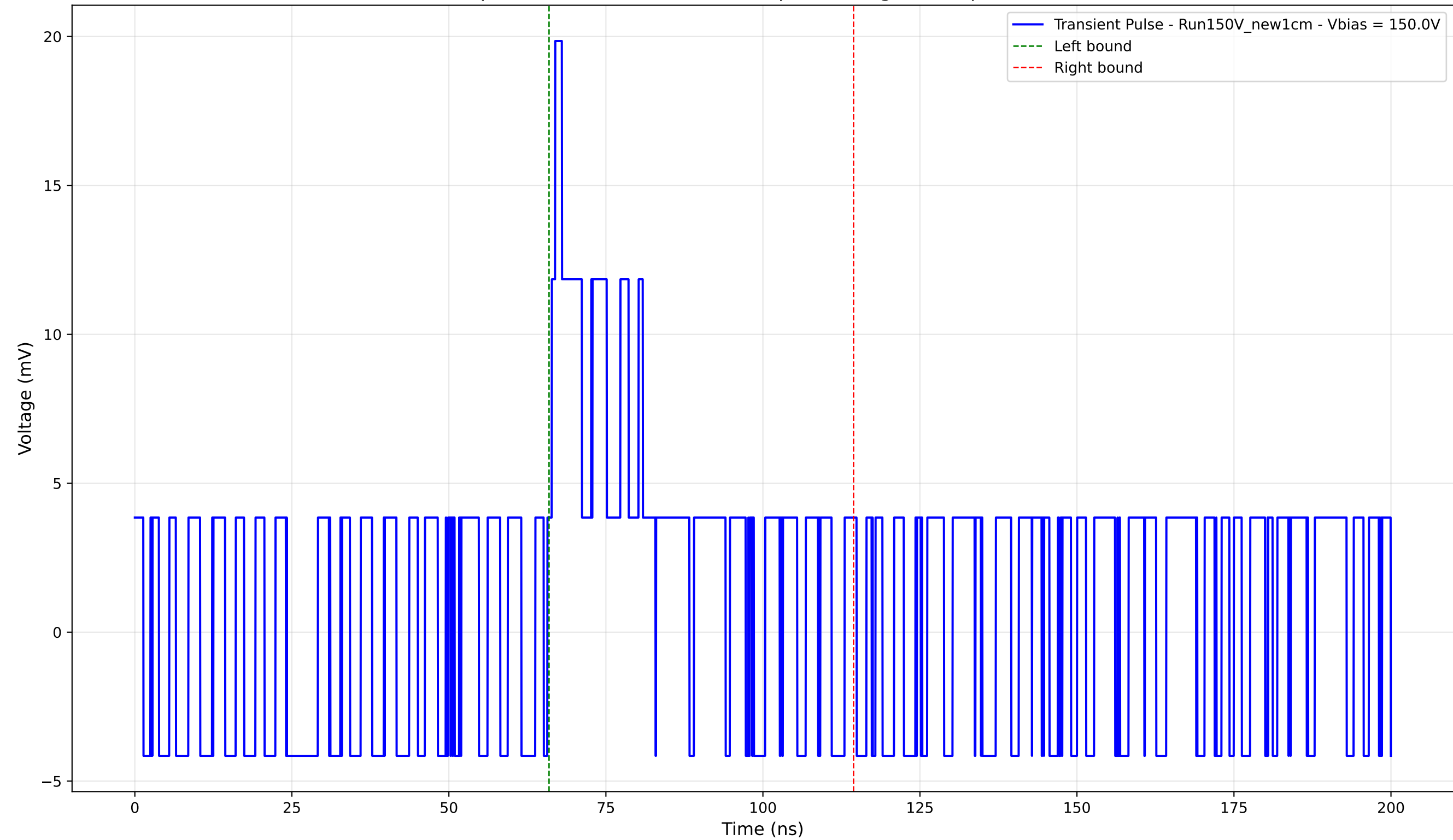
Transient Pulse - Sample: New1cm - Position: 40.0 \mu\text{m} - Charge: 4.11 pC - Rise Time: 0.00 ns (N/A)
