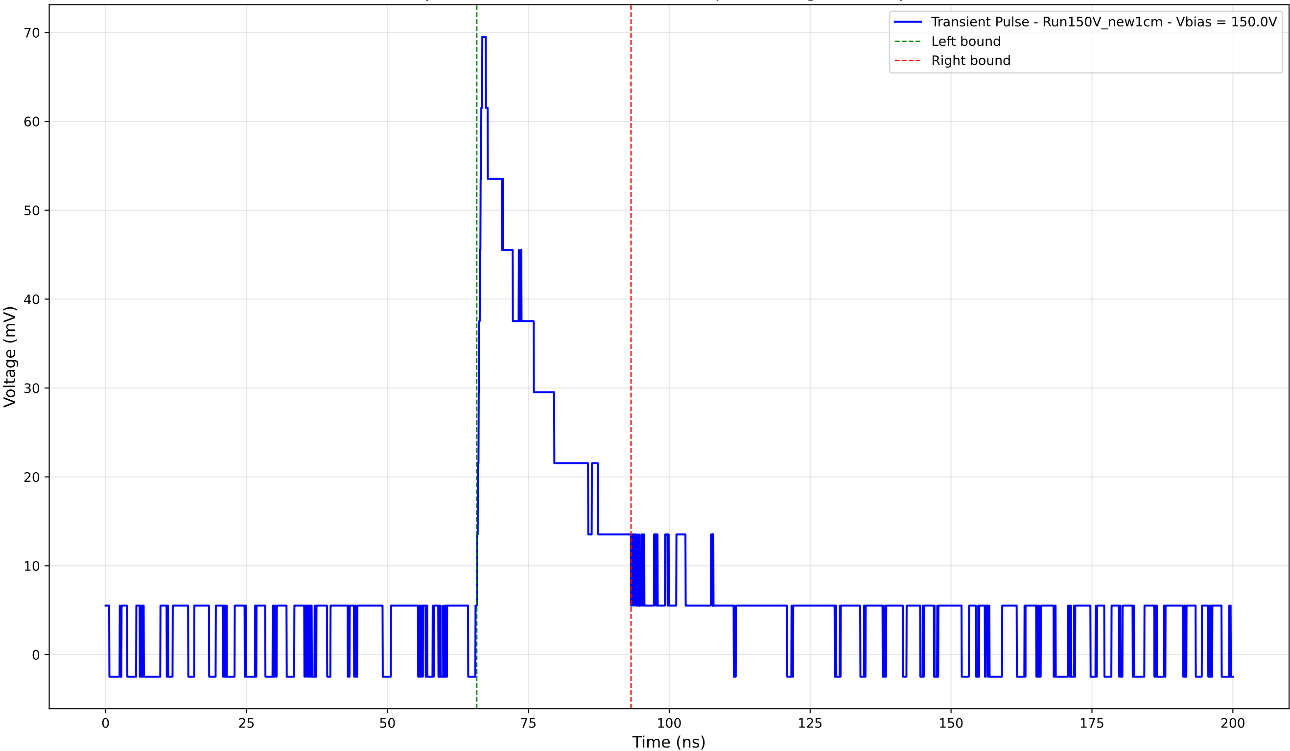
Transient Pulse - Sample: New1cm - Position: 3015.0 \mu\text{m} - Charge: 16.29 pC - Rise Time: 0.96 ns
