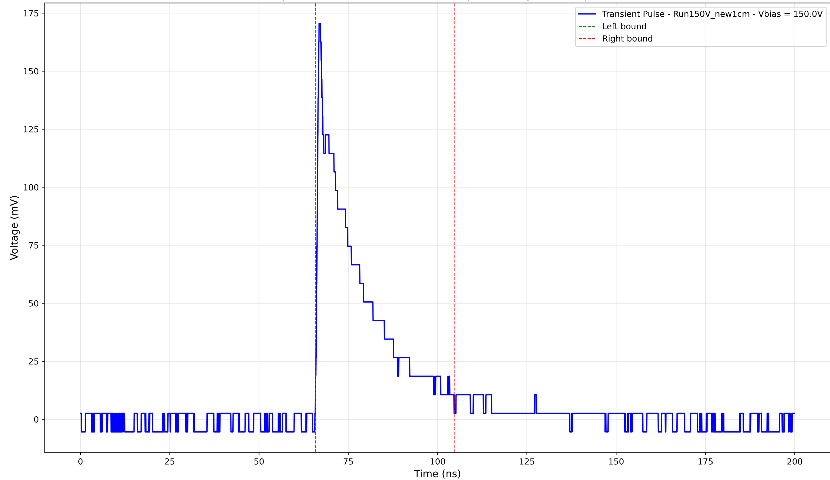
Transient Pulse - Sample: New1cm - Position: 2920.0 \mu\text{m} - Charge: 38.95 pC - Rise Time: 0.82 ns
