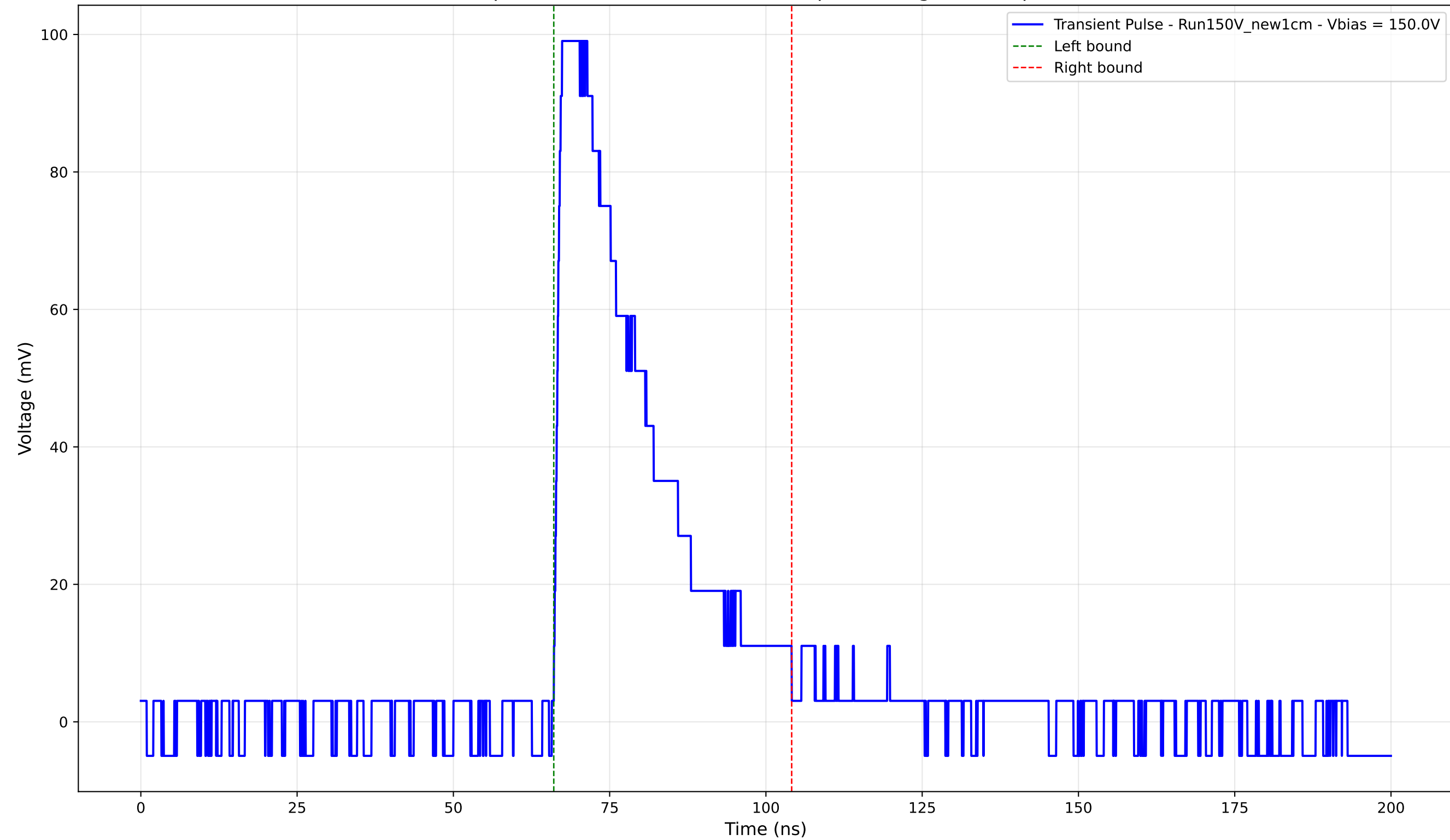
Transient Pulse - Sample: New1cm - Position: 1720.0 \mu\text{m} - Charge: 31.47 pC - Rise Time: 1.08 ns
