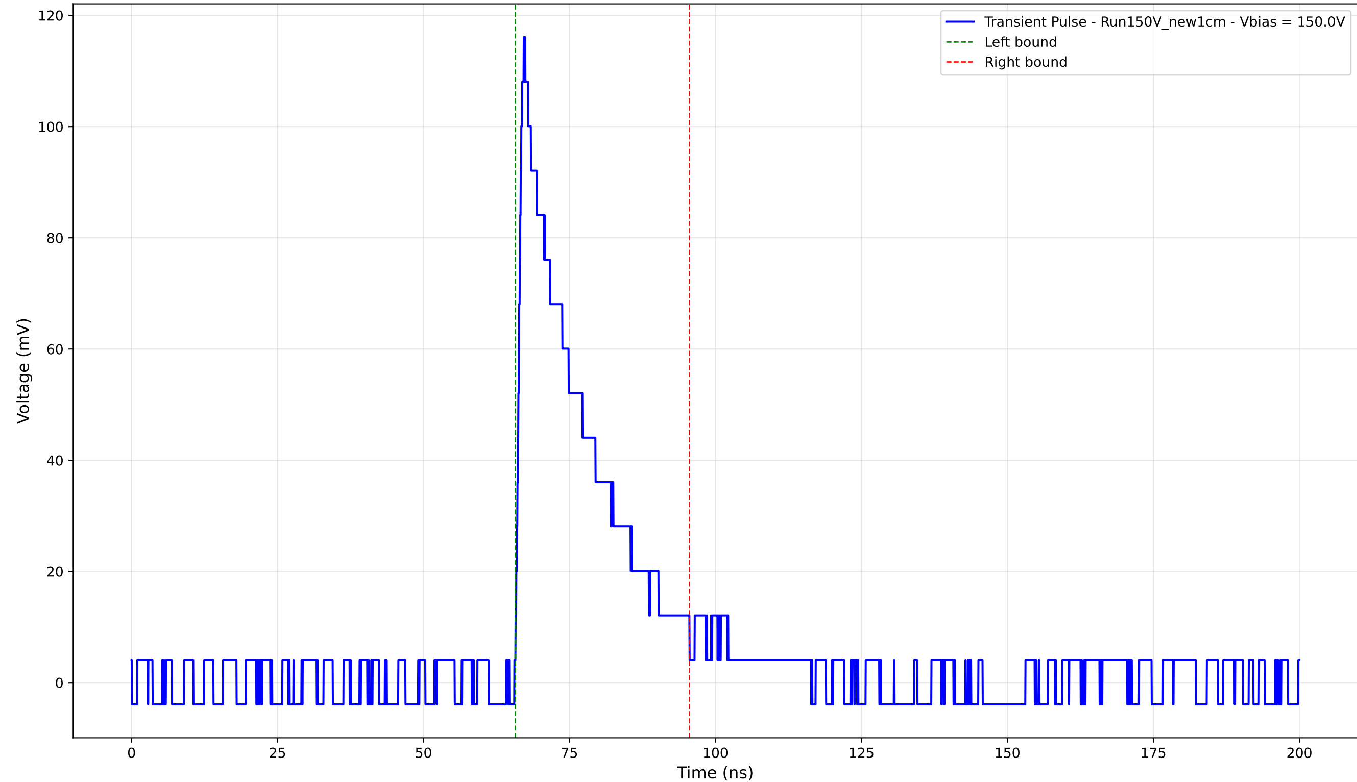
Transient Pulse - Sample: New1cm - Position: 4650.0 \mu\text{m} - Charge: 25.63 pC - Rise Time: 1.14 ns
