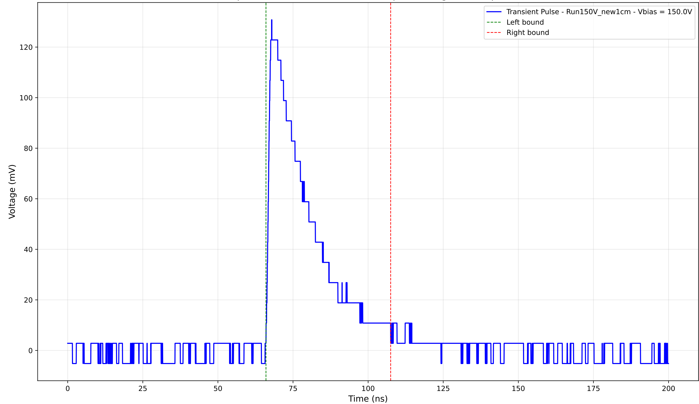
Transient Pulse - Sample: New1cm - Position: 3670.0 \mu\text{m} - Charge: 37.49 pC - Rise Time: 1.37 ns
