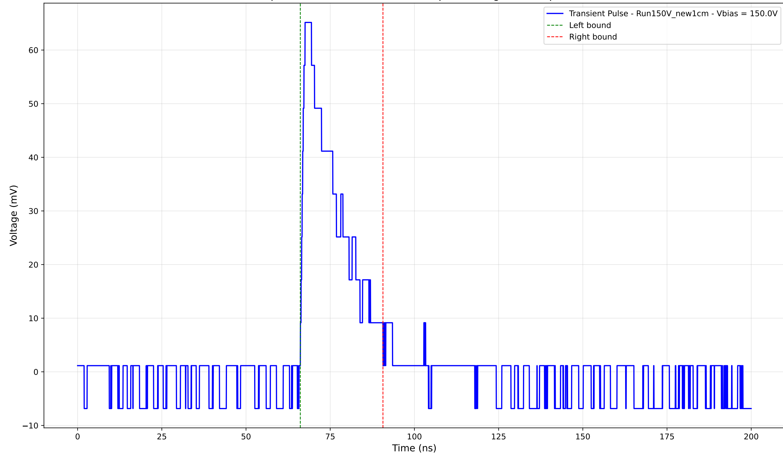
Transient Pulse - Sample: New1cm - Position: 590.0 \mu\text{m} - Charge: 14.89 pC - Rise Time: 1.39 ns
