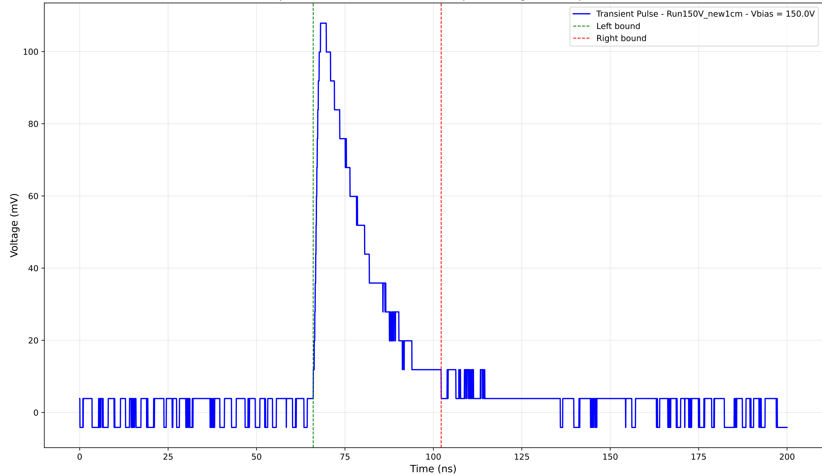
Transient Pulse - Sample: New1cm - Position: 1420.0 \mu\text{m} - Charge: 31.56 pC - Rise Time: 1.66 ns
