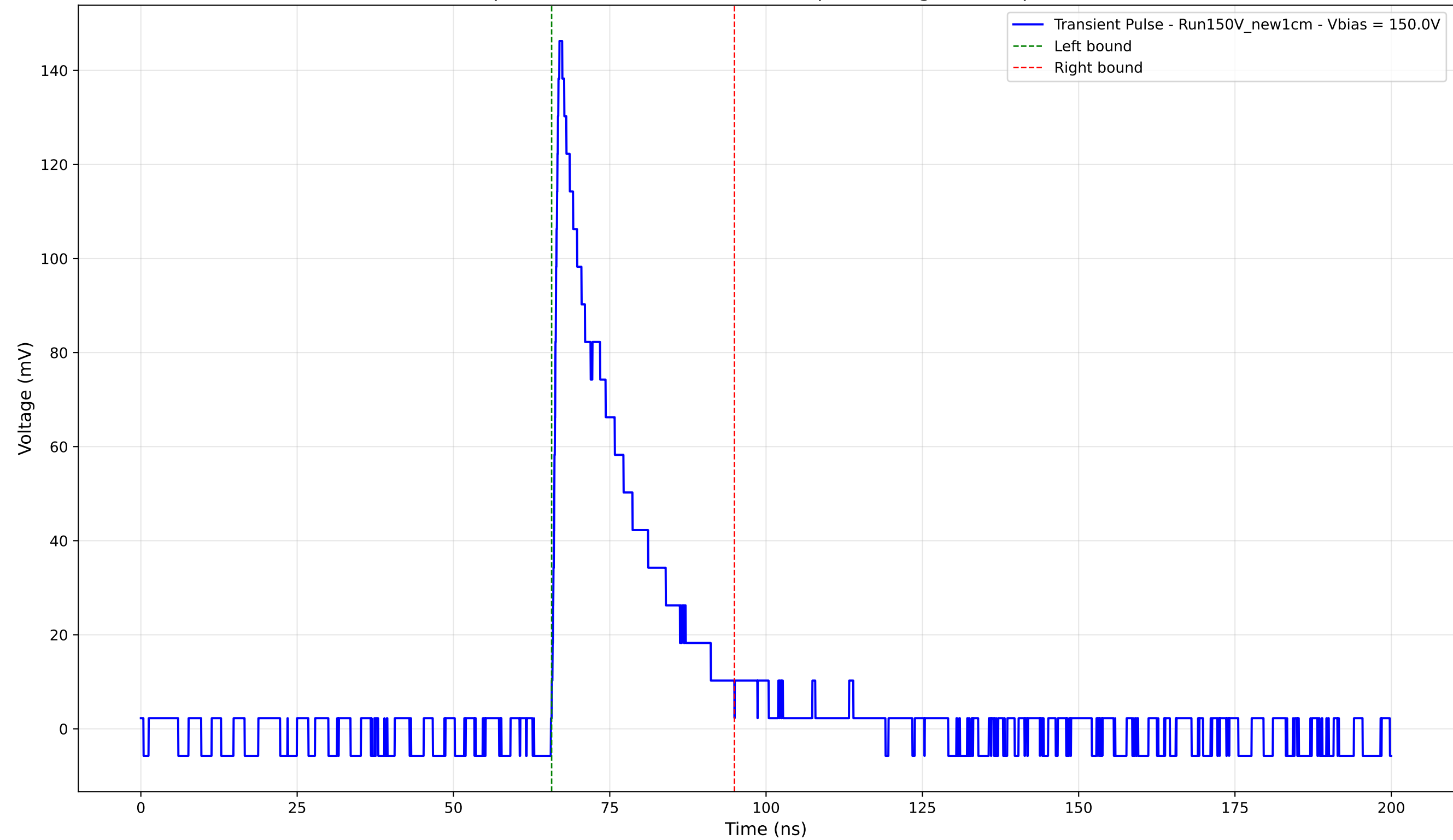
Transient Pulse - Sample: New1cm - Position: 4735.0 \mu\text{m} - Charge: 29.47 pC - Rise Time: 0.95 ns
