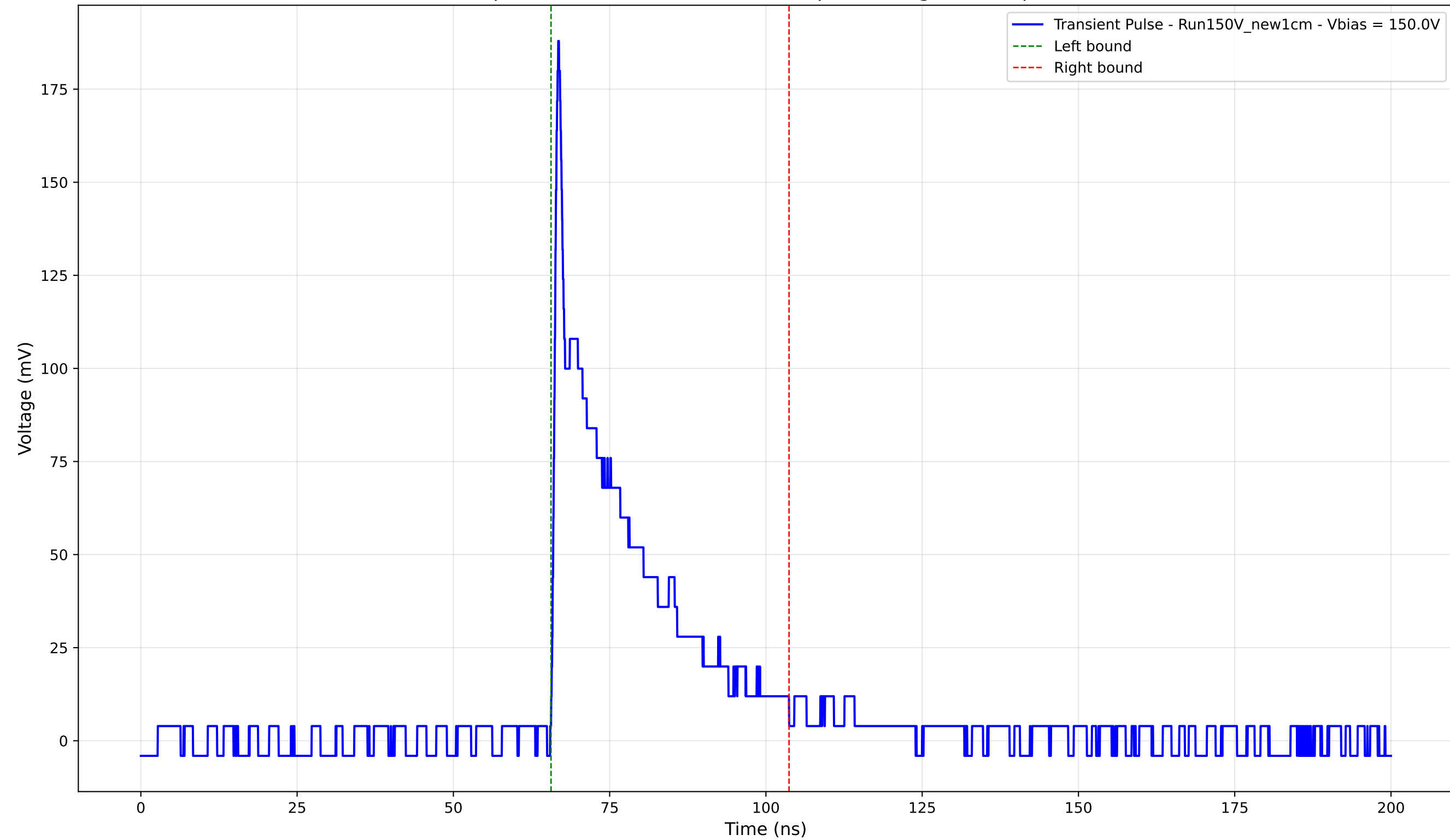
Transient Pulse - Sample: New1cm - Position: 2360.0 \mu\text{m} - Charge: 35.56 pC - Rise Time: 0.86 ns
