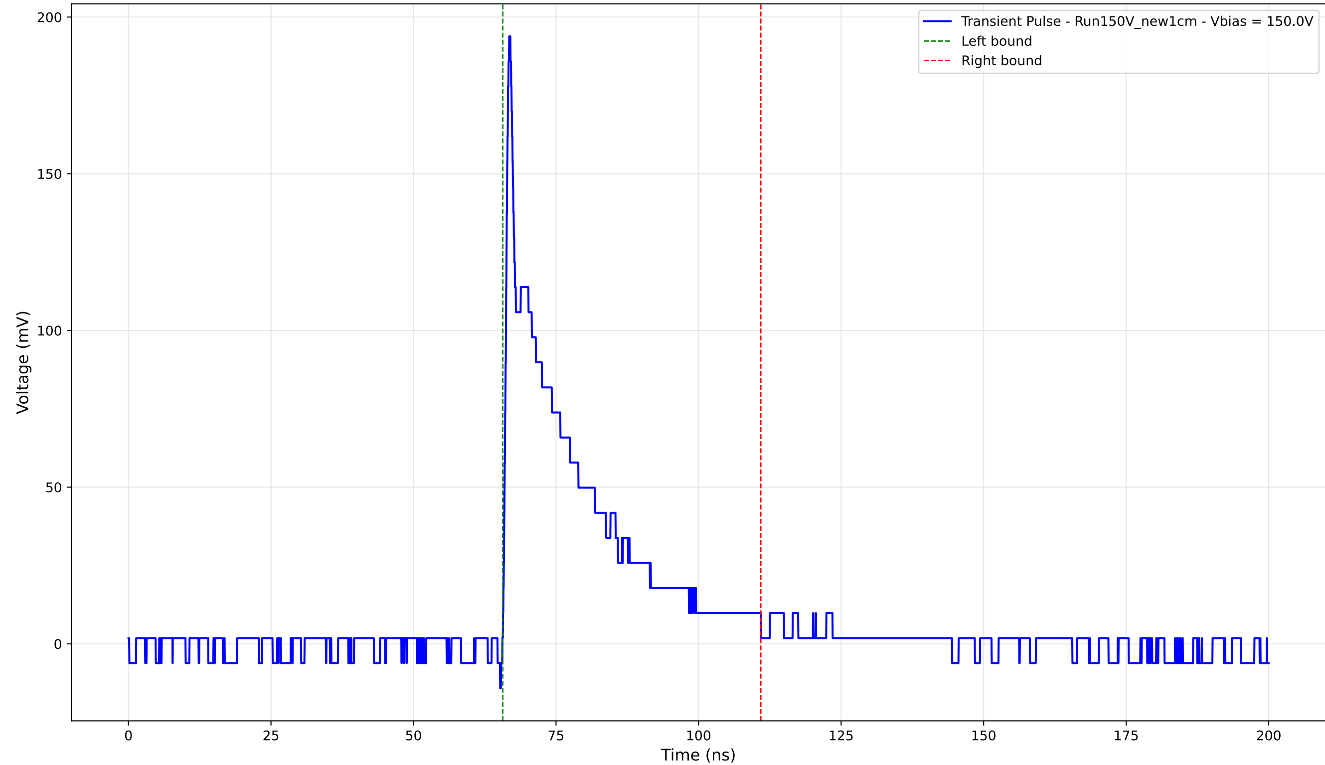
Transient Pulse - Sample: New1cm - Position: 2765.0 \mu\text{m} - Charge: 38.52 pC - Rise Time: 0.78 ns
