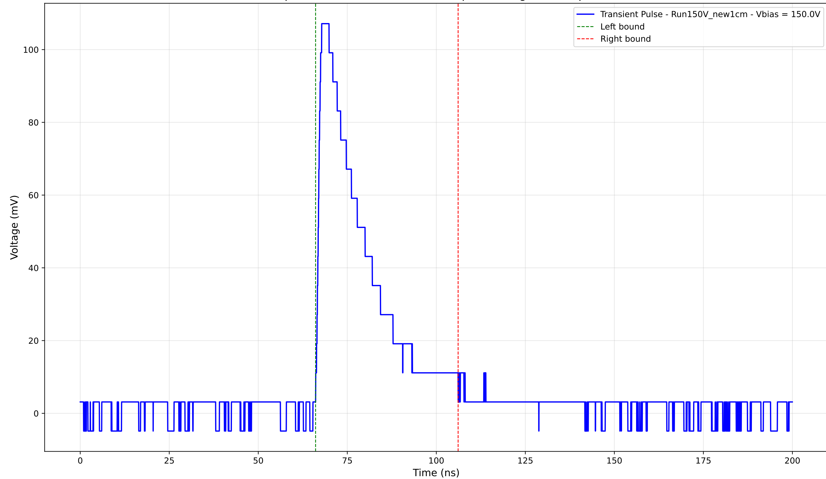
Transient Pulse - Sample: New1cm - Position: 920.0 \mu\text{m} - Charge: 31.02 pC - Rise Time: 1.38 ns
