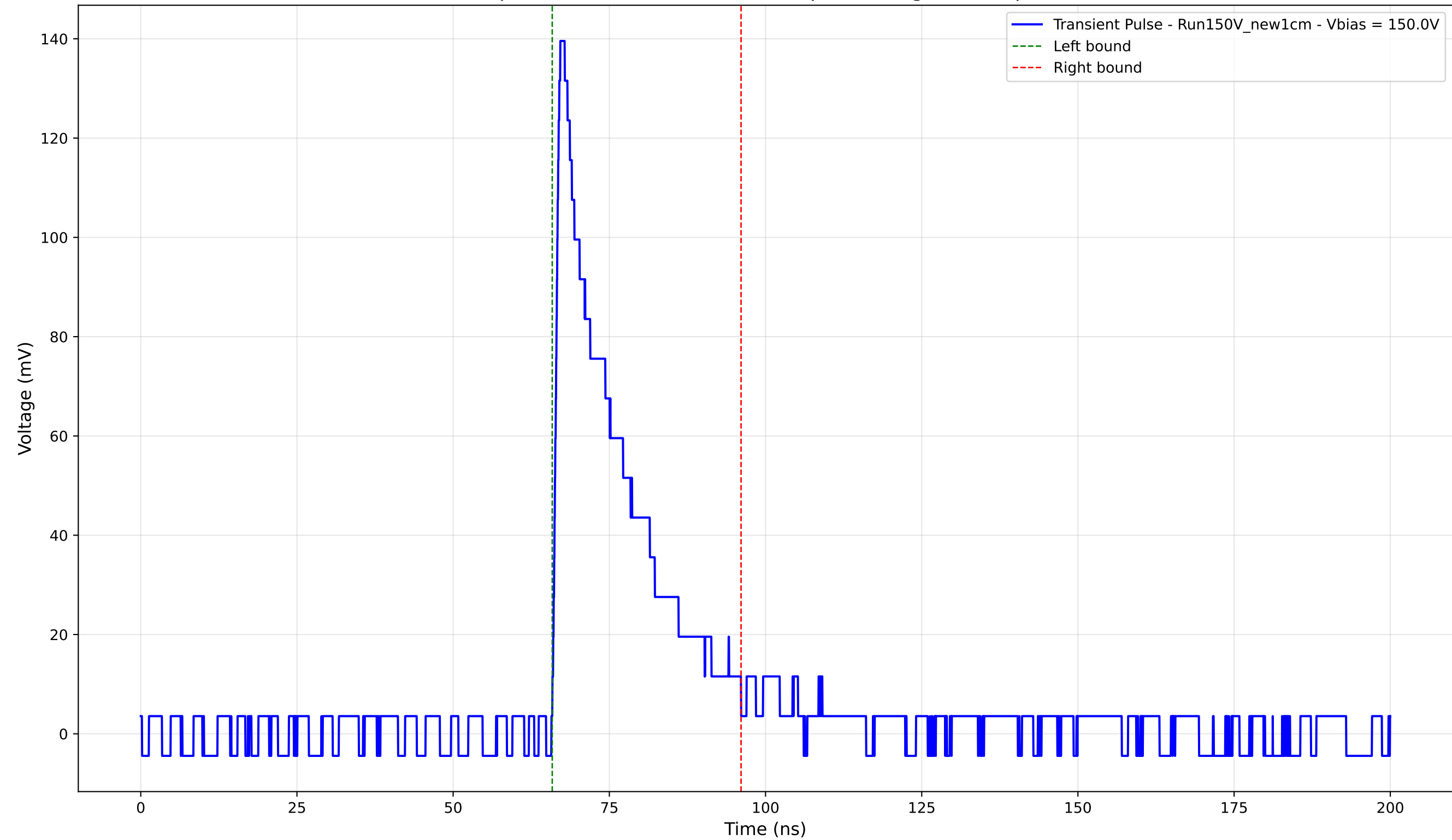
Transient Pulse - Sample: New1cm - Position: 300.0 \mu\text{m} - Charge: 29.17 pC - Rise Time: 0.99 ns
