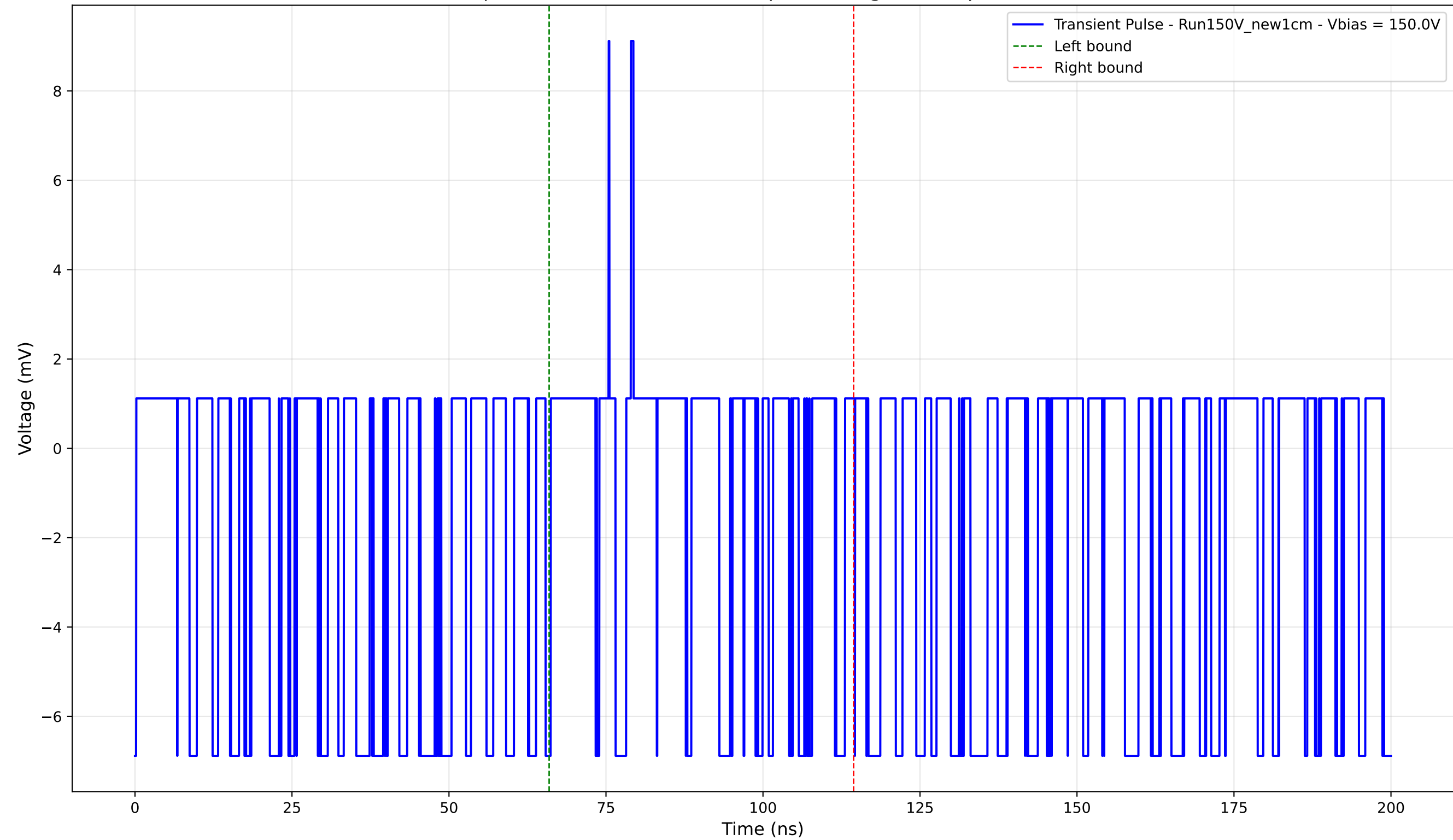
Transient Pulse - Sample: New1cm - Position: 0.0 \mu\text{m} - Charge: -0.59 pC - Rise Time: 0.00 ns (N/A)
