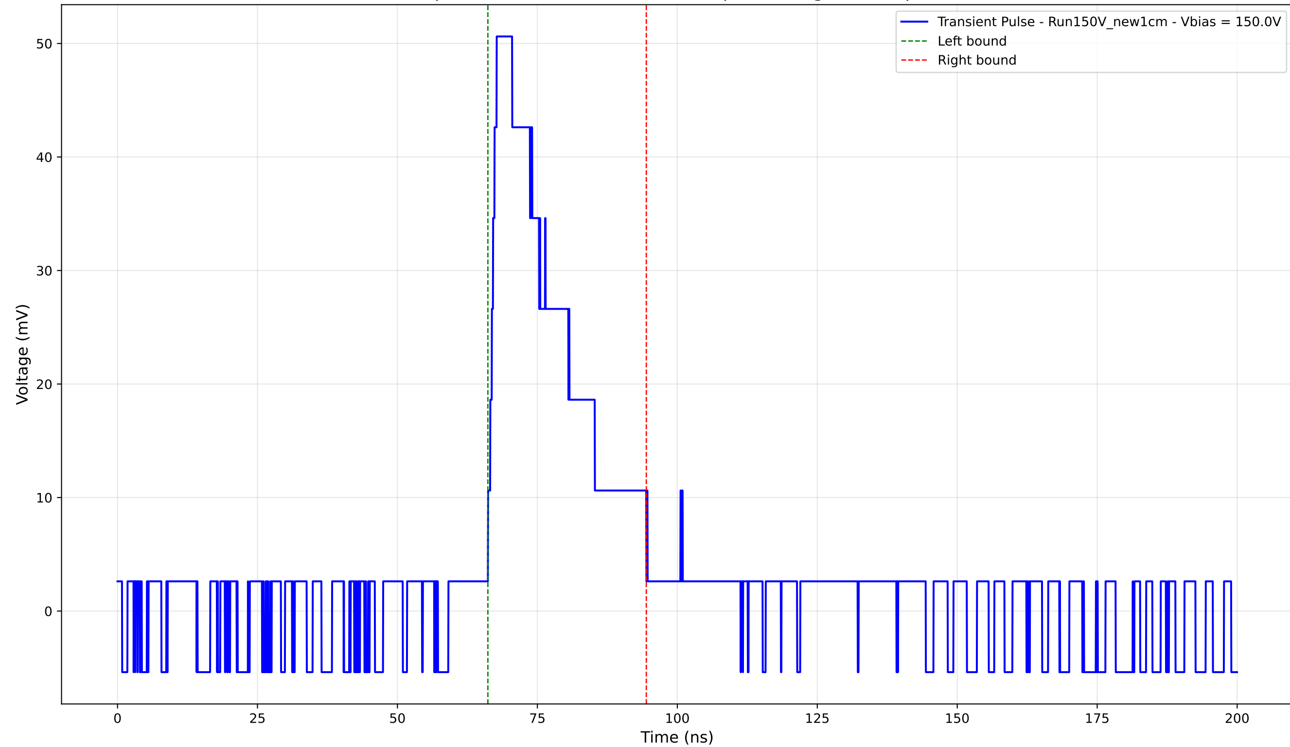
Transient Pulse - Sample: New1cm - Position: 1085.0 \mu\text{m} - Charge: 14.04 pC - Rise Time: 1.55 ns
