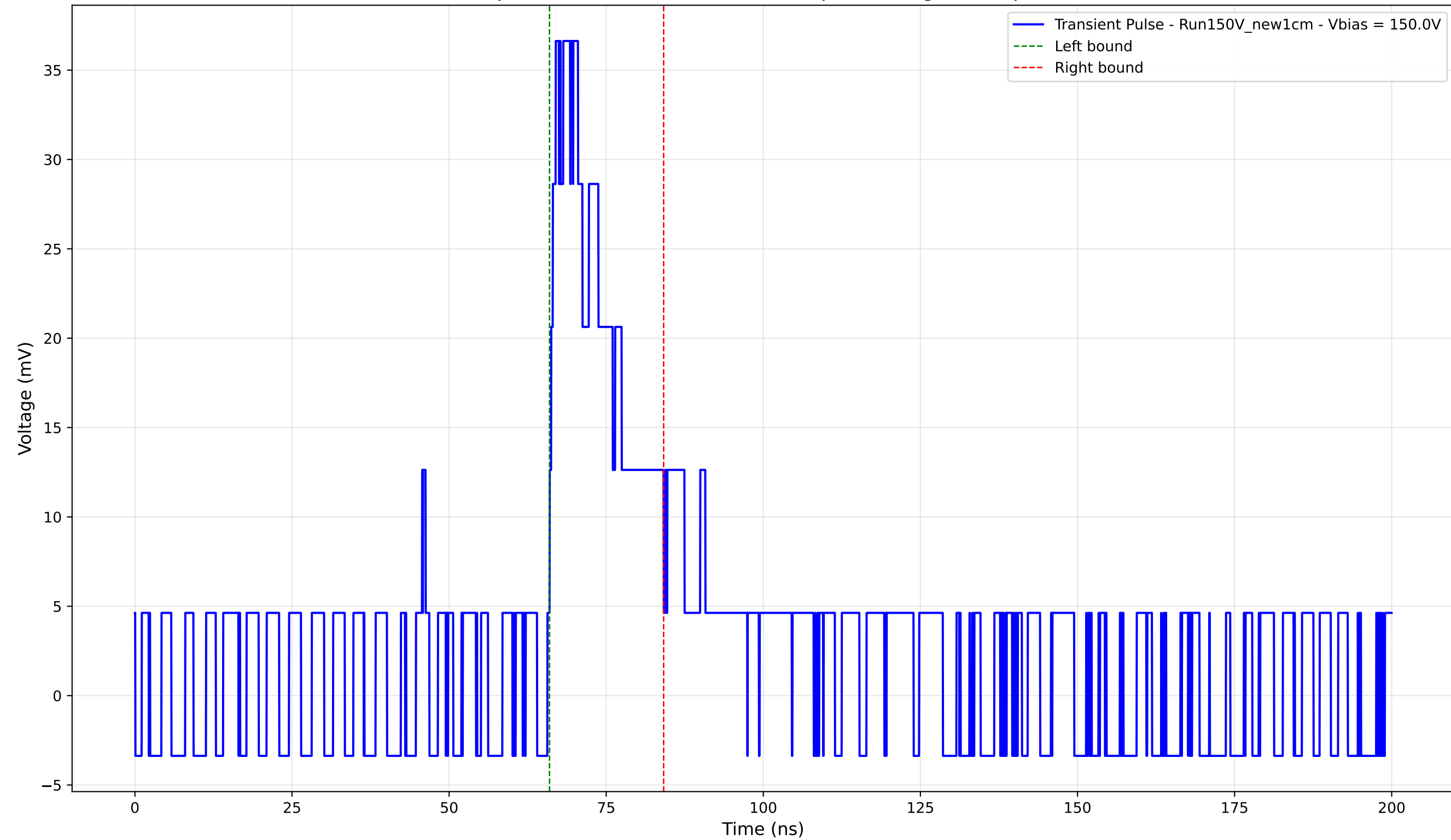
Transient Pulse - Sample: New1cm - Position: 4545.0 \mu\text{m} - Charge: 7.76 pC - Rise Time: 1.34 ns
