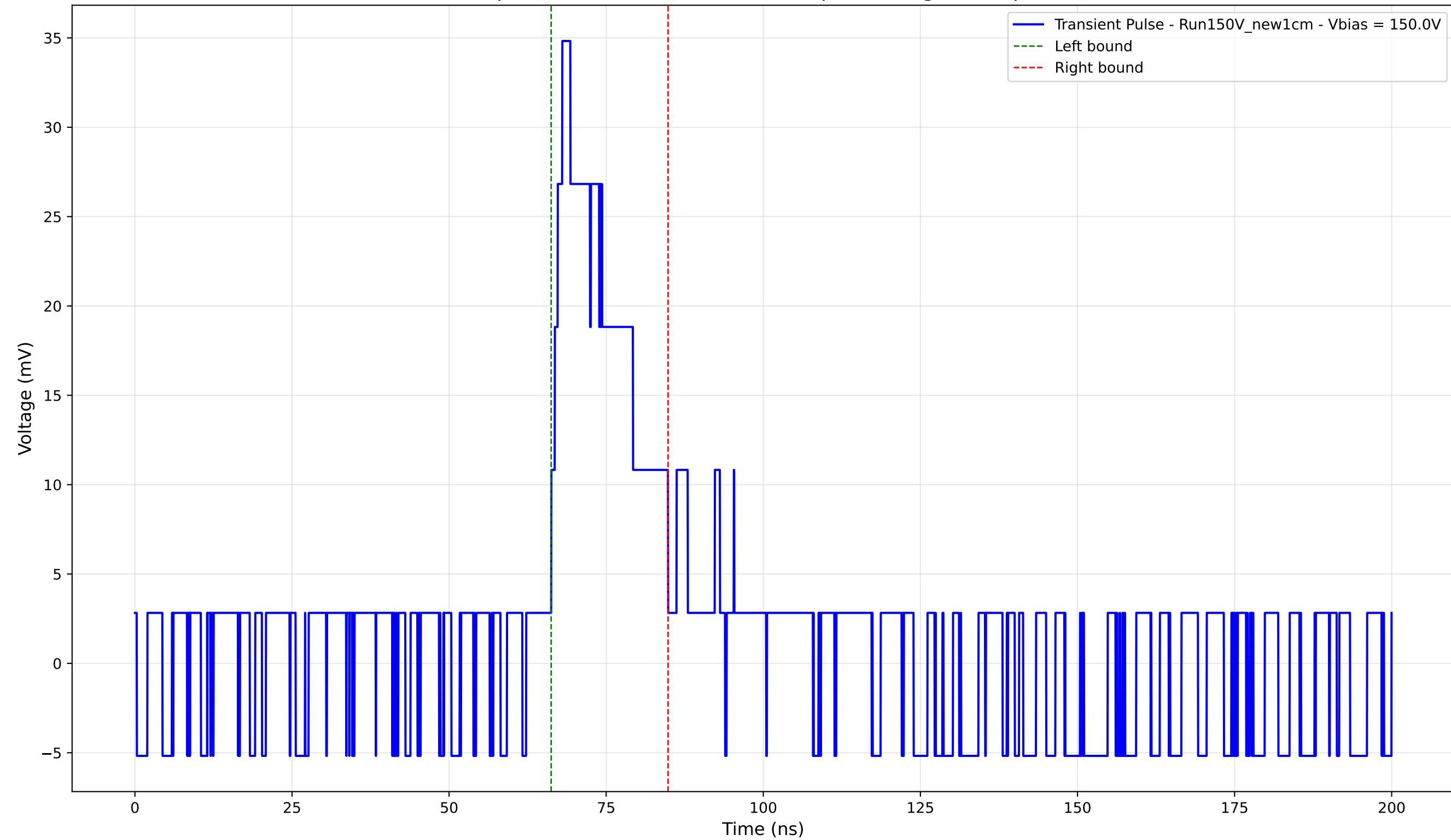
Transient Pulse - Sample: New1cm - Position: 1570.0 \mu\text{m} - Charge: 7.28 pC - Rise Time: 1.76 ns
