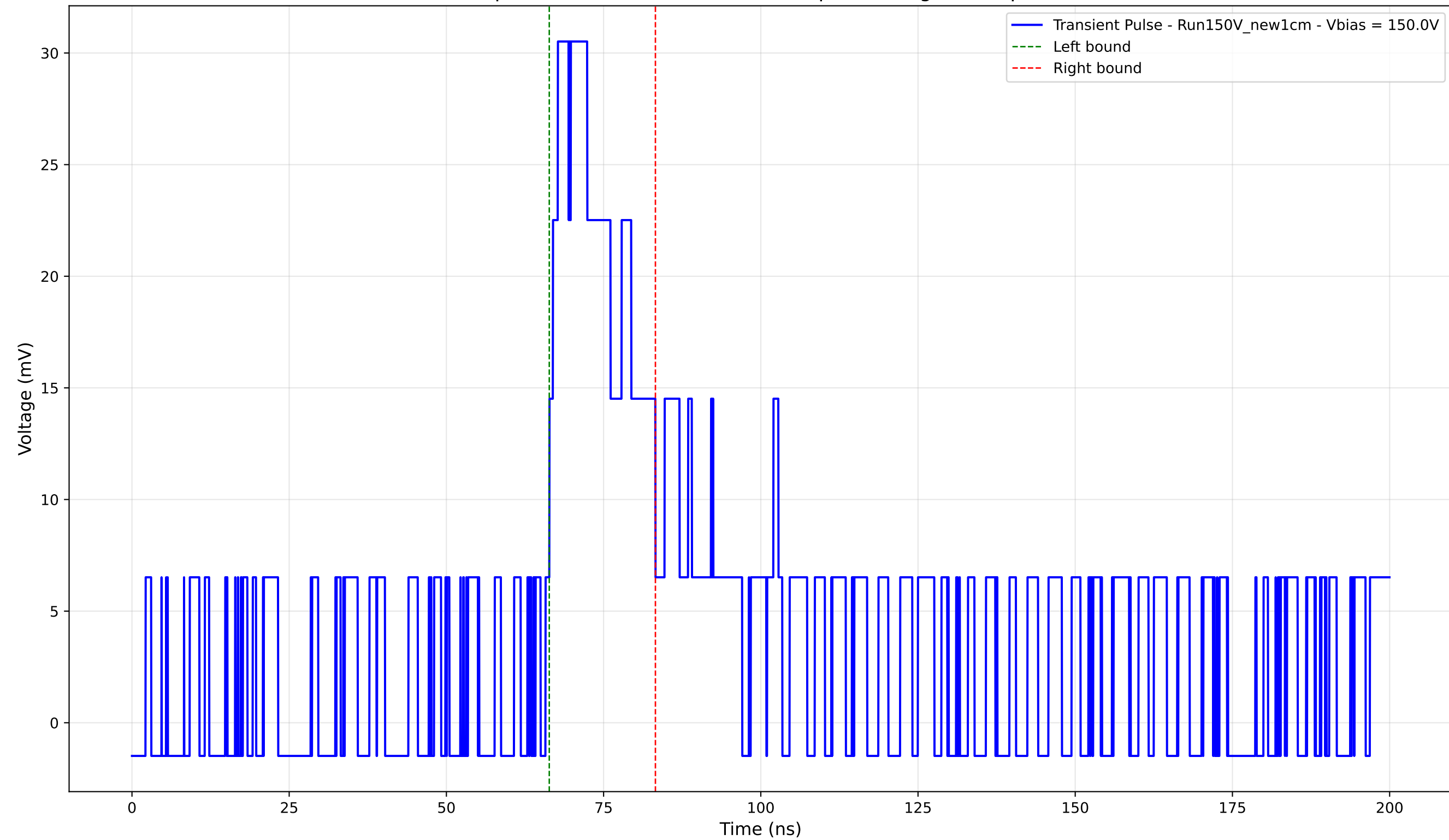
Transient Pulse - Sample: New1cm - Position: 3540.0 \mu\text{m} - Charge: 7.33 pC - Rise Time: 1.97 ns
