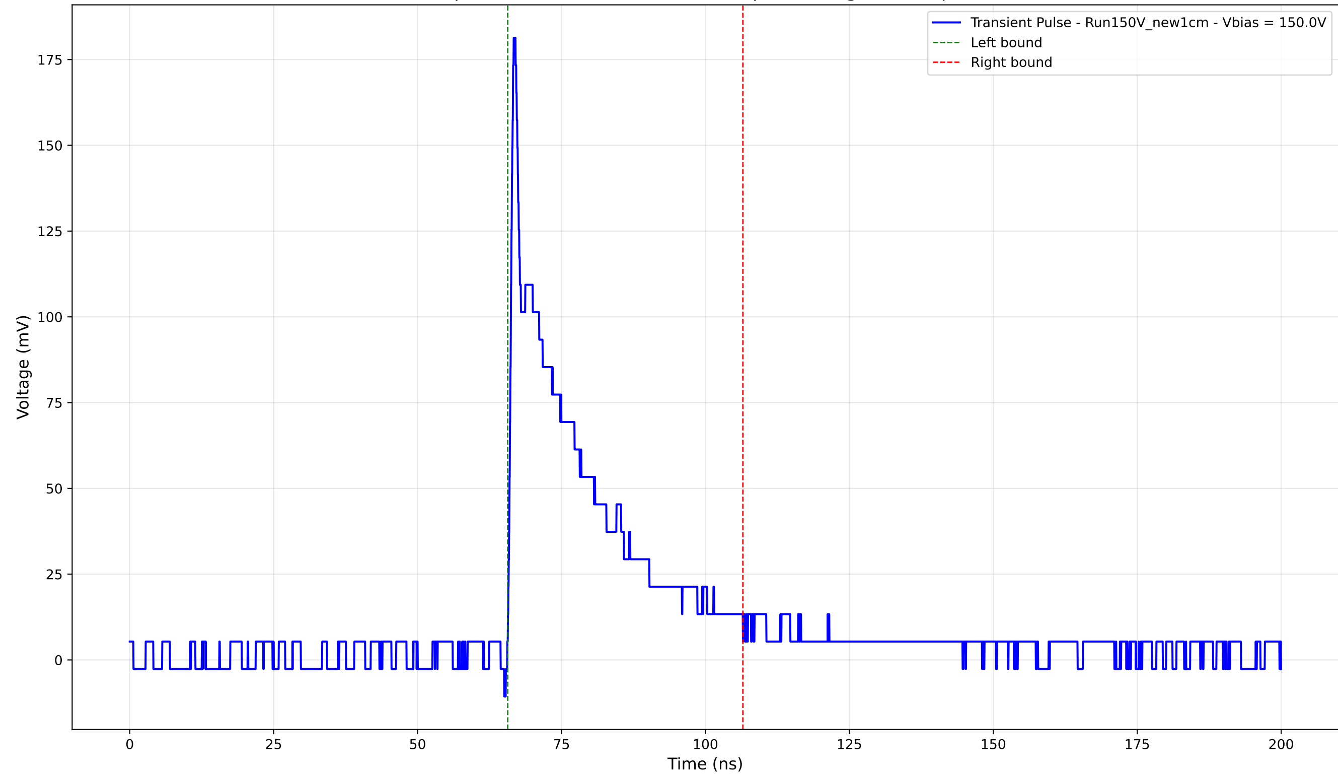
Transient Pulse - Sample: New1cm - Position: 2335.0 \mu\text{m} - Charge: 38.43 pC - Rise Time: 0.81 ns
