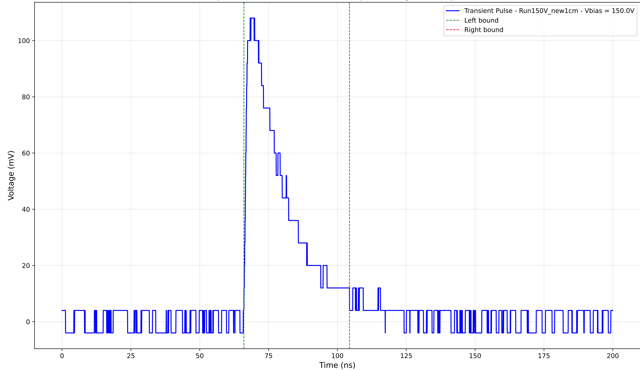
Transient Pulse - Sample: New1cm - Position: 1700.0 \mu\text{m} - Charge: 32.88 pC - Rise Time: 1.30 ns
