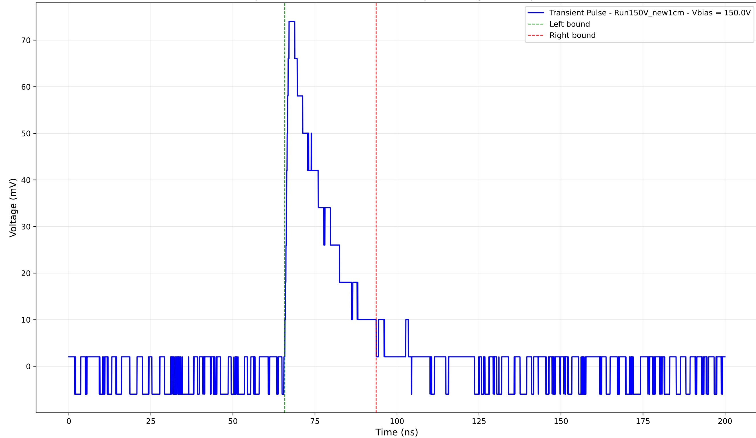
Transient Pulse - Sample: New1cm - Position: 4520.0 \mu\text{m} - Charge: 17.81 pC - Rise Time: 1.27 ns
