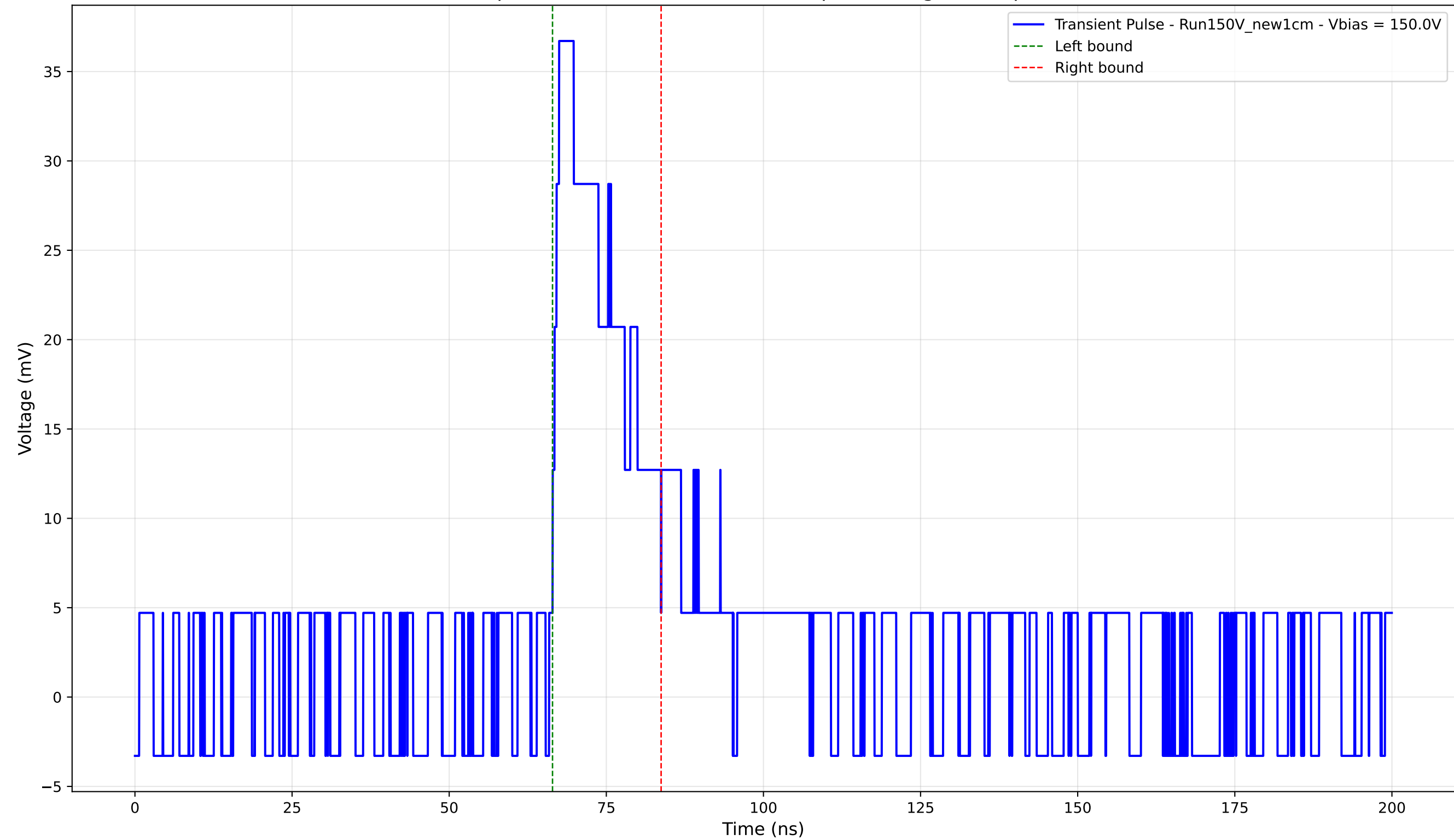
Transient Pulse - Sample: New1cm - Position: 4040.0 \mu\text{m} - Charge: 7.86 pC - Rise Time: 1.59 ns
