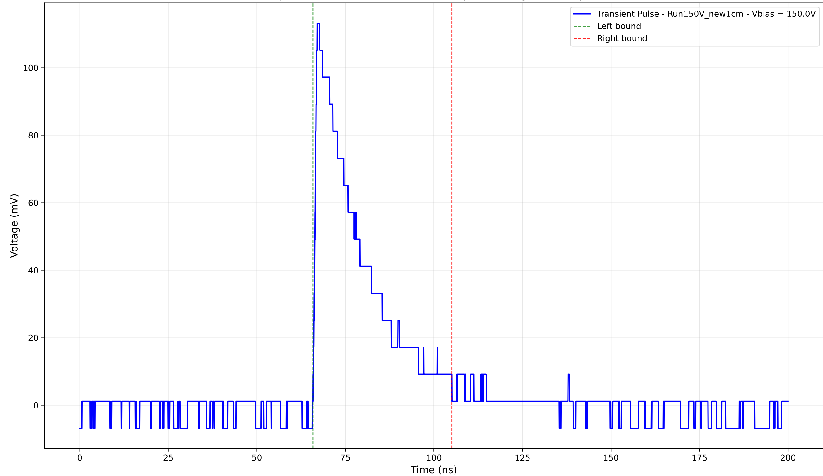
Transient Pulse - Sample: New1cm - Position: 3140.0 \mu\text{m} - Charge: 30.60 pC - Rise Time: 0.93 ns
