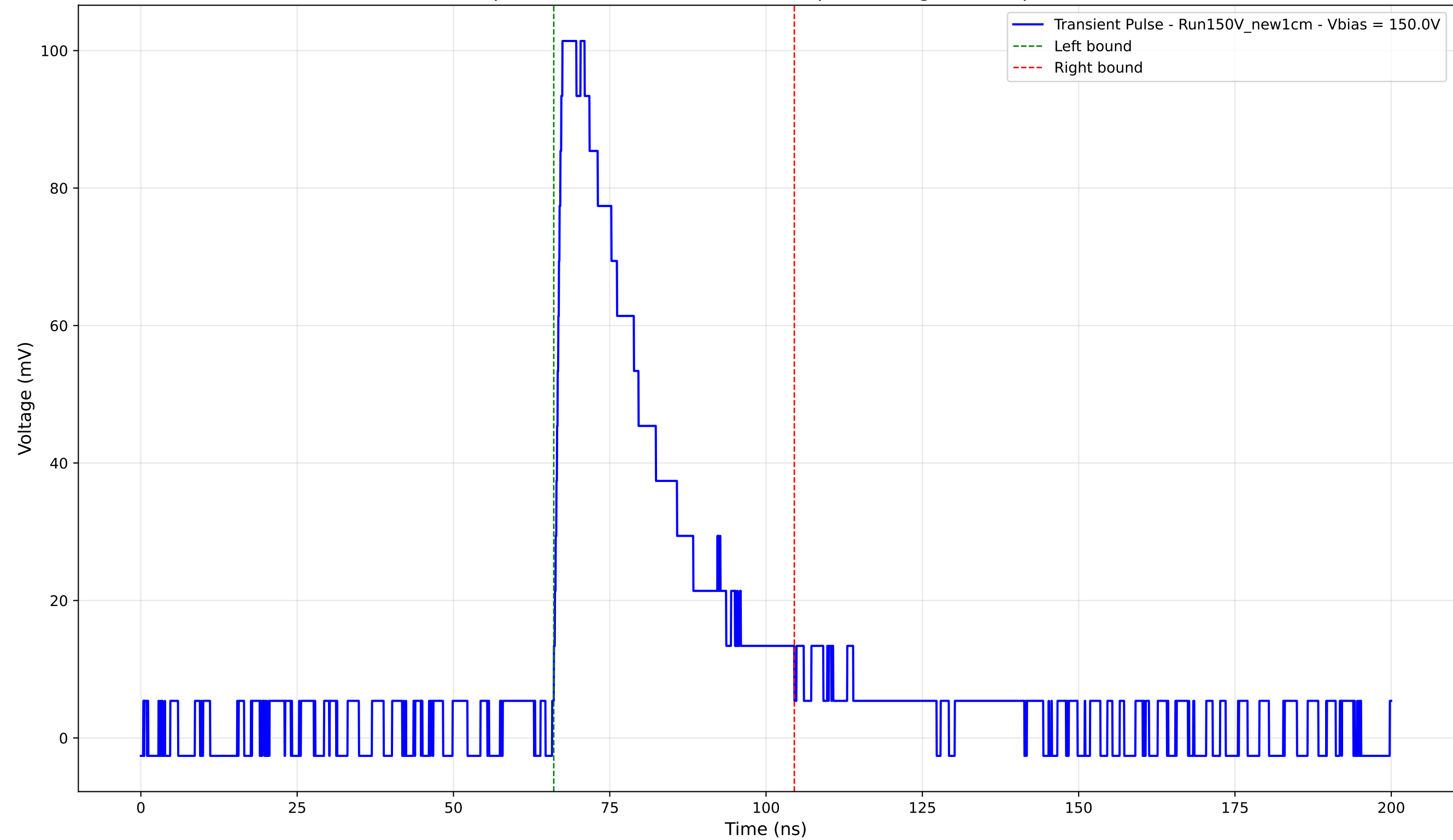
Transient Pulse - Sample: New1cm - Position: 1655.0 \mu\text{m} - Charge: 32.99 pC - Rise Time: 1.19 ns
