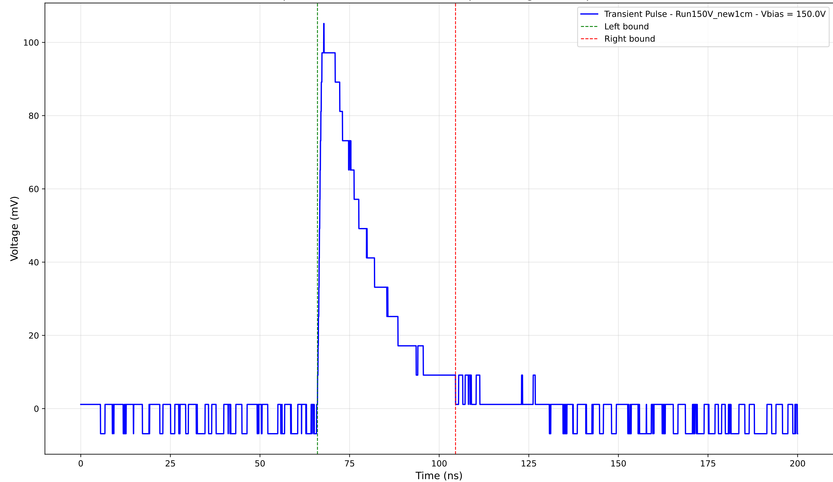
Transient Pulse - Sample: New1cm - Position: 1740.0 \mu\text{m} - Charge: 29.88 pC - Rise Time: 1.10 ns
