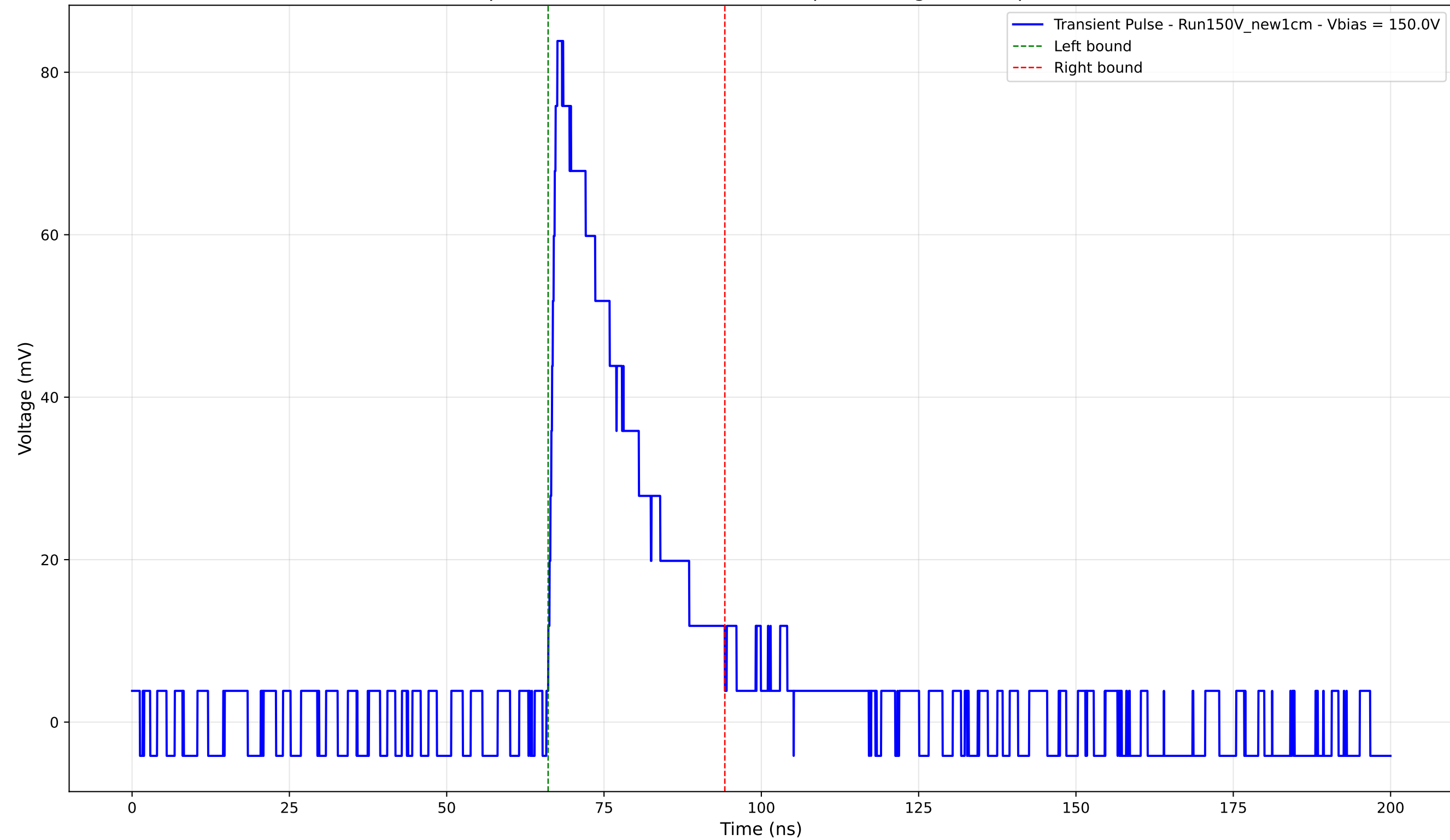
Transient Pulse - Sample: New1cm - Position: 4130.0 \mu\text{m} - Charge: 20.79 pC - Rise Time: 1.17 ns
