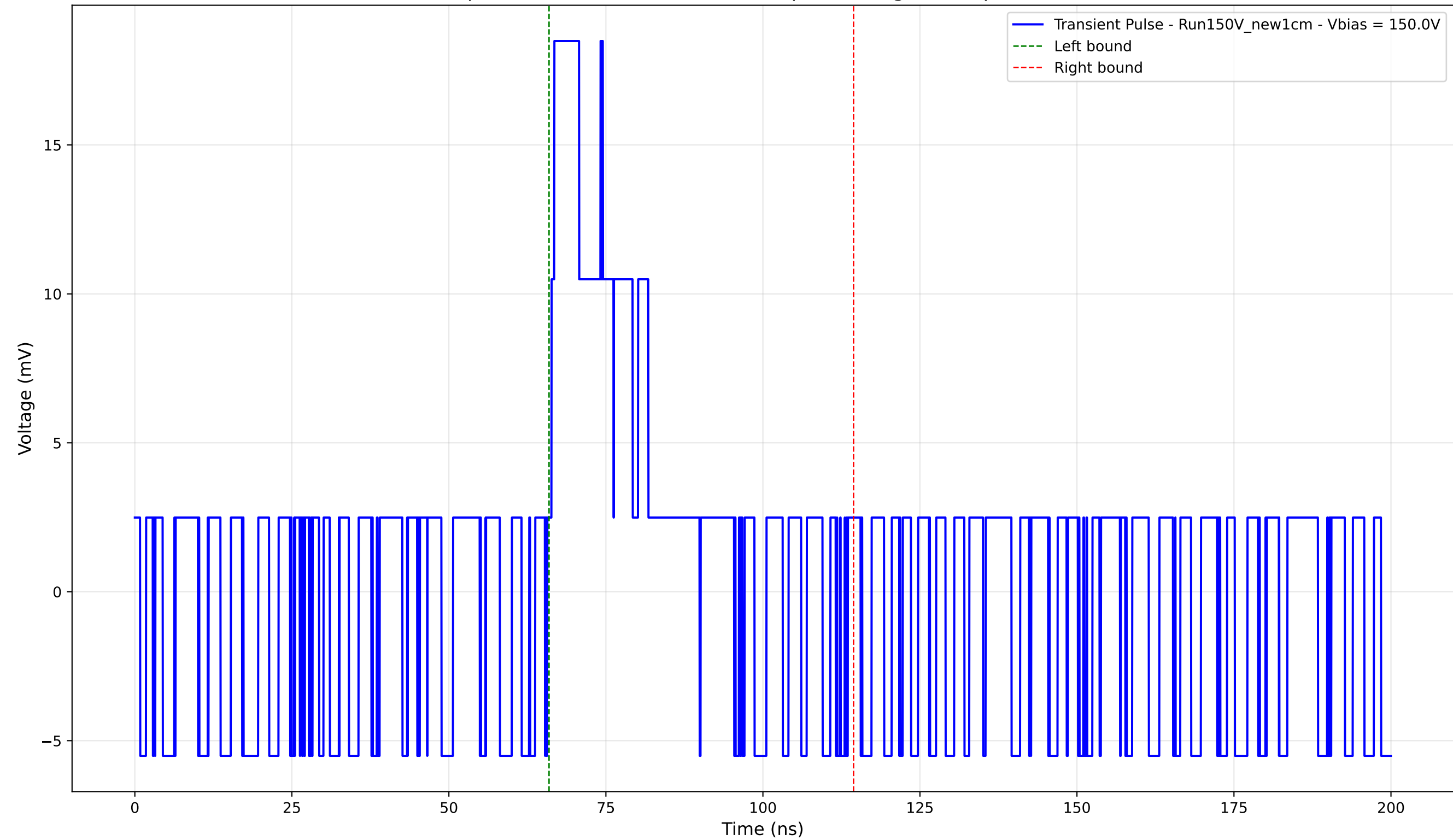
Transient Pulse - Sample: New1cm - Position: 4570.0 \mu\text{m} - Charge: 4.14 pC - Rise Time: 0.00 ns (N/A)
