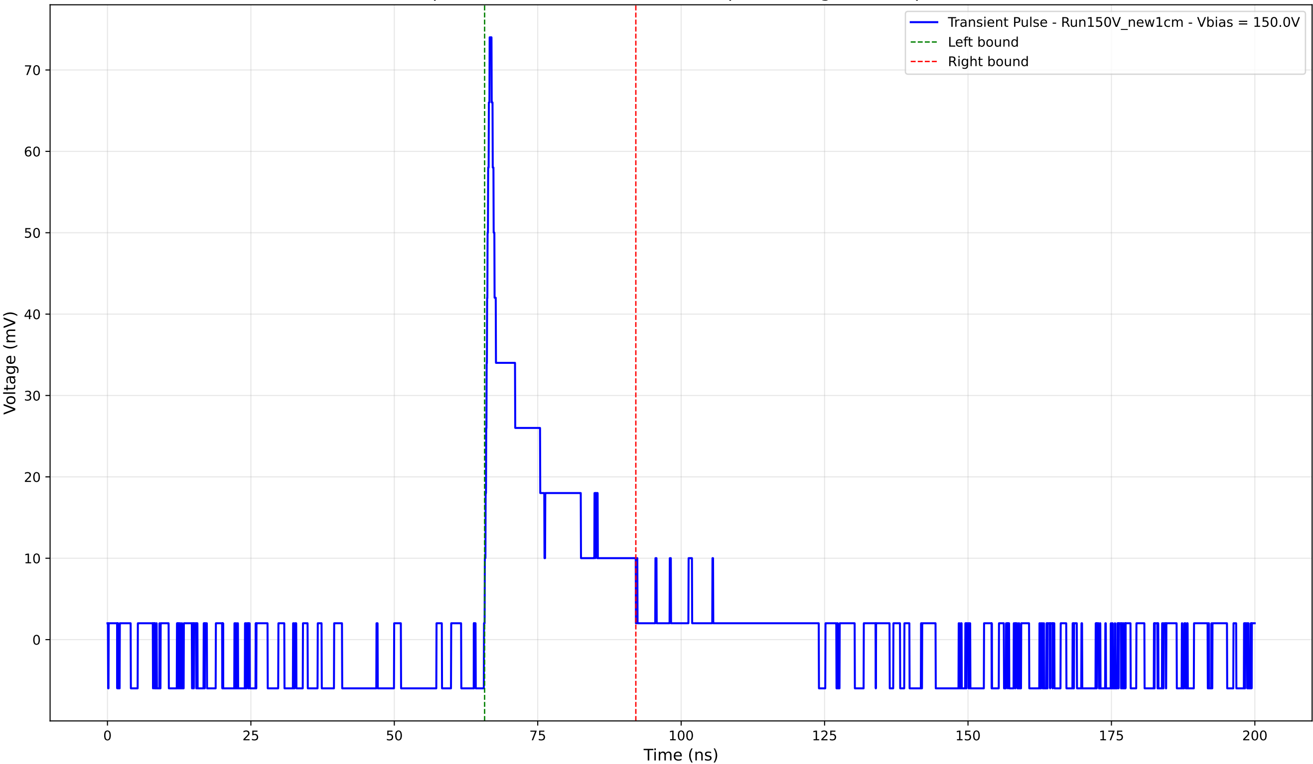
Transient Pulse - Sample: New1cm - Position: 2590.0 \mu\text{m} - Charge: 11.06 pC - Rise Time: 0.85 ns
