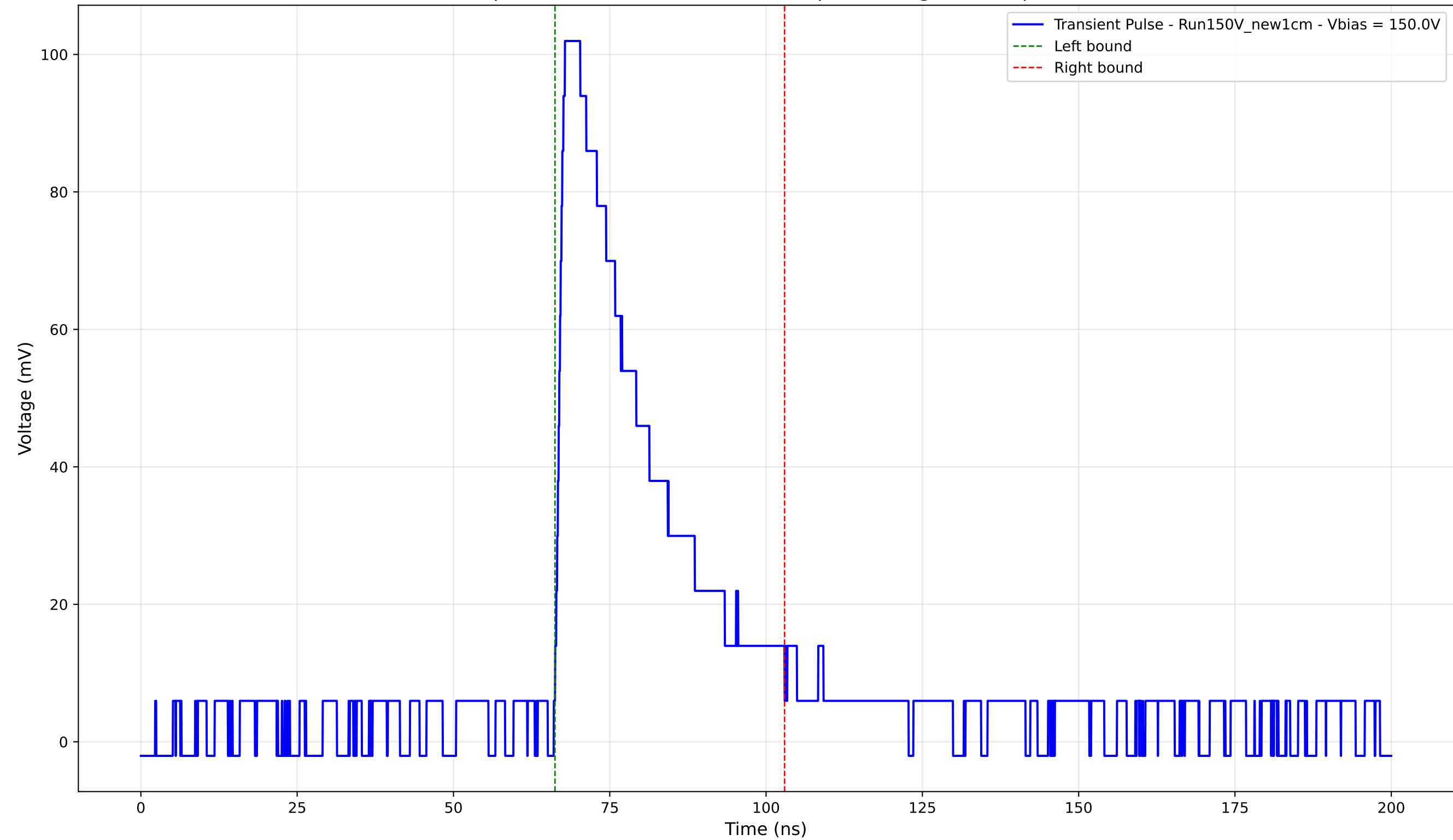
Transient Pulse - Sample: New1cm - Position: 1150.0 \mu\text{m} - Charge: 31.20 pC - Rise Time: 1.33 ns
