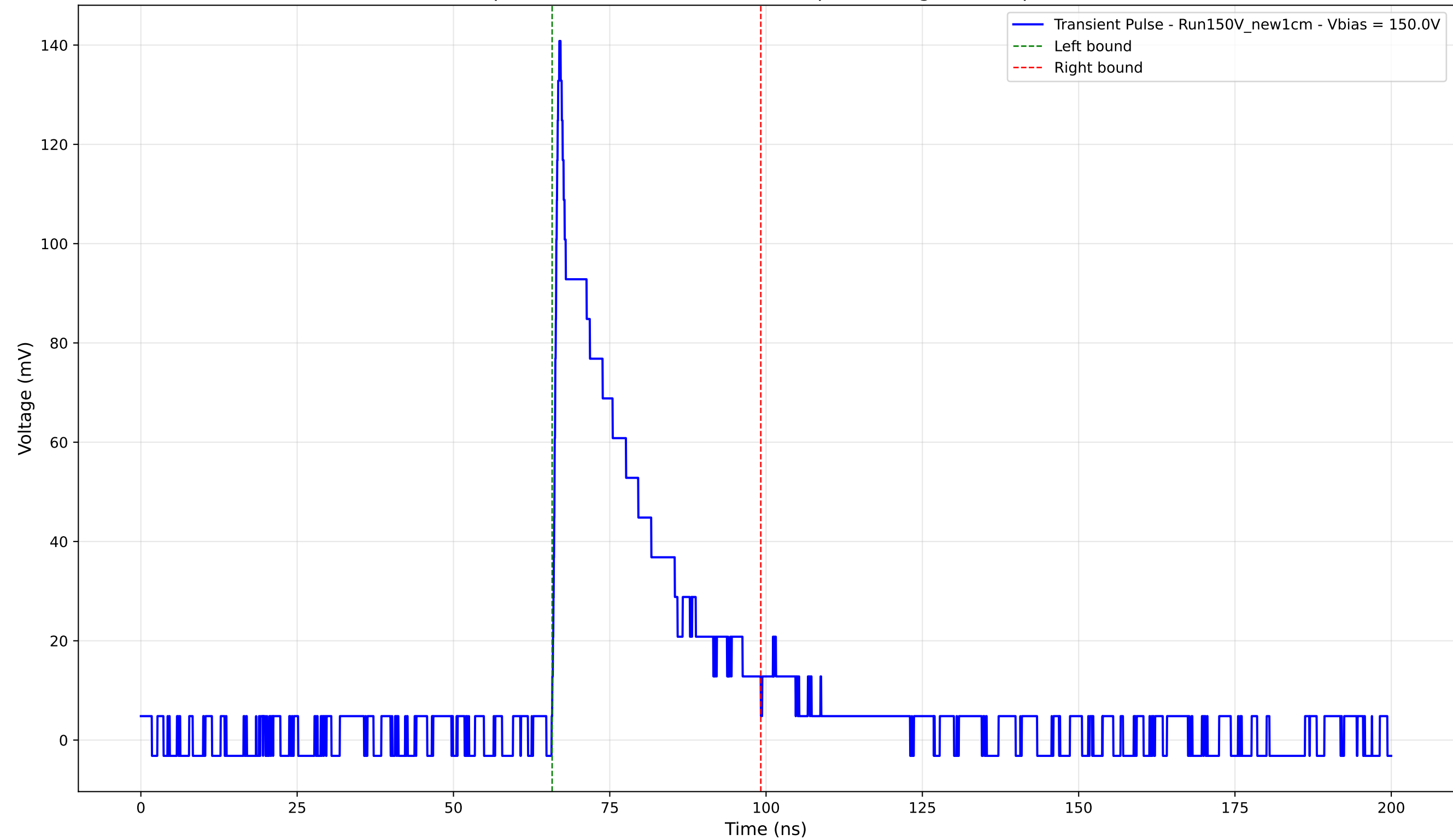
Transient Pulse - Sample: New1cm - Position: 2190.0 \mu\text{m} - Charge: 31.49 pC - Rise Time: 0.86 ns
