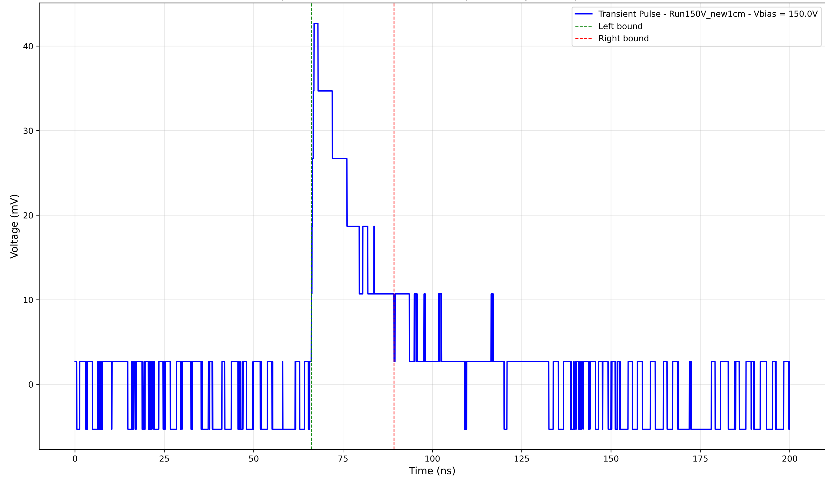
Transient Pulse - Sample: New1cm - Position: 1995.0 \mu\text{m} - Charge: 9.89 pC - Rise Time: 0.78 ns
