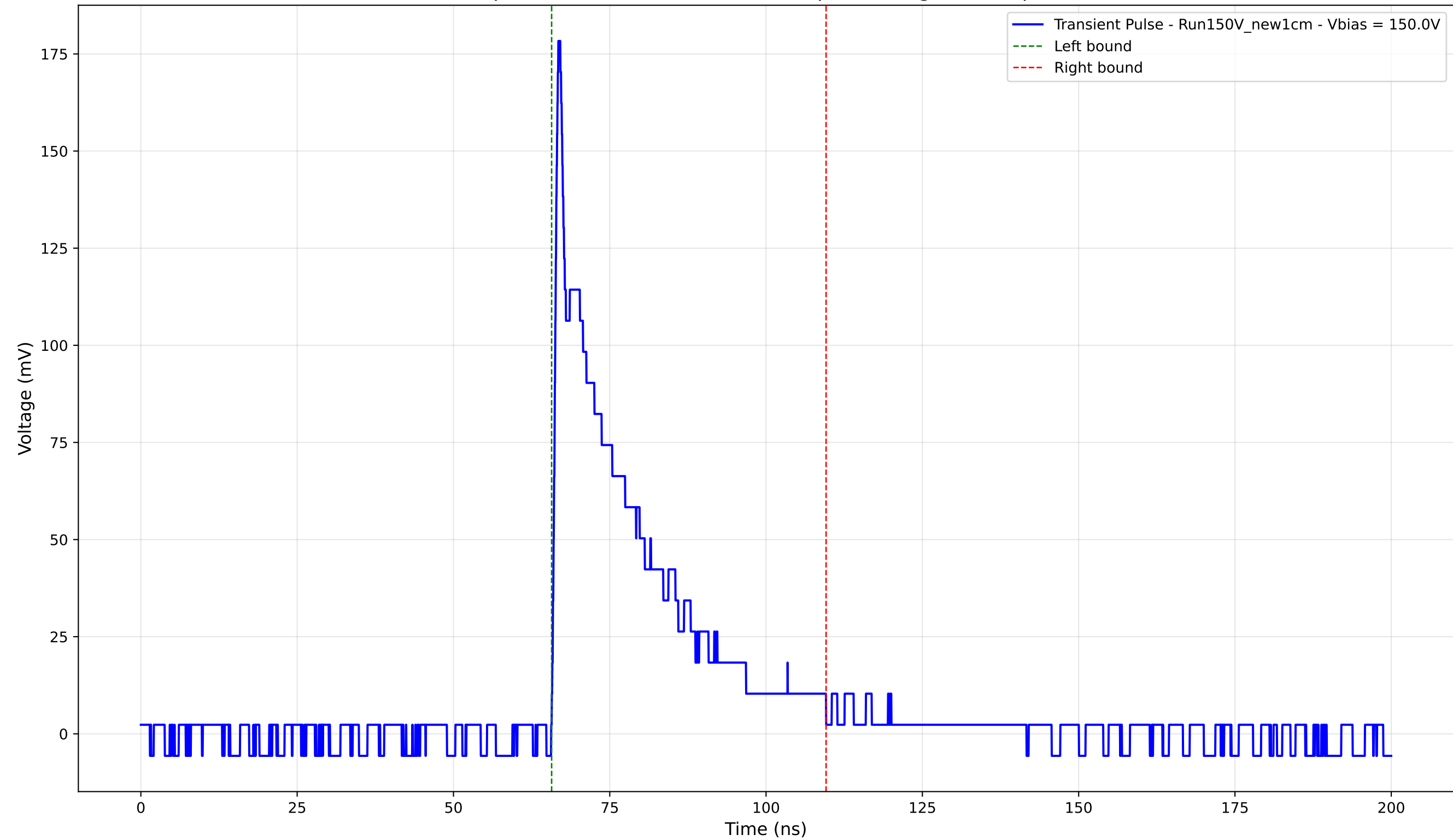
Transient Pulse - Sample: New1cm - Position: 2825.0 \mu\text{m} - Charge: 37.58 pC - Rise Time: 0.82 ns
