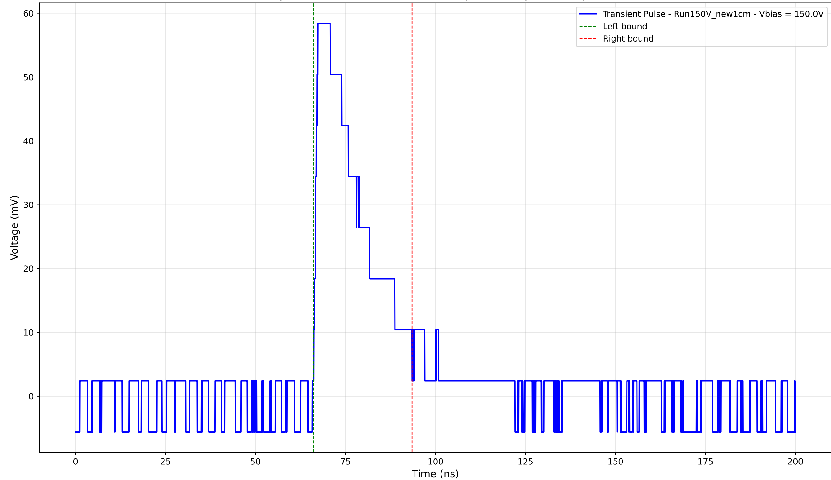
Transient Pulse - Sample: New1cm - Position: 3610.0 \mu\text{m} - Charge: 16.69 pC - Rise Time: 1.15 ns
