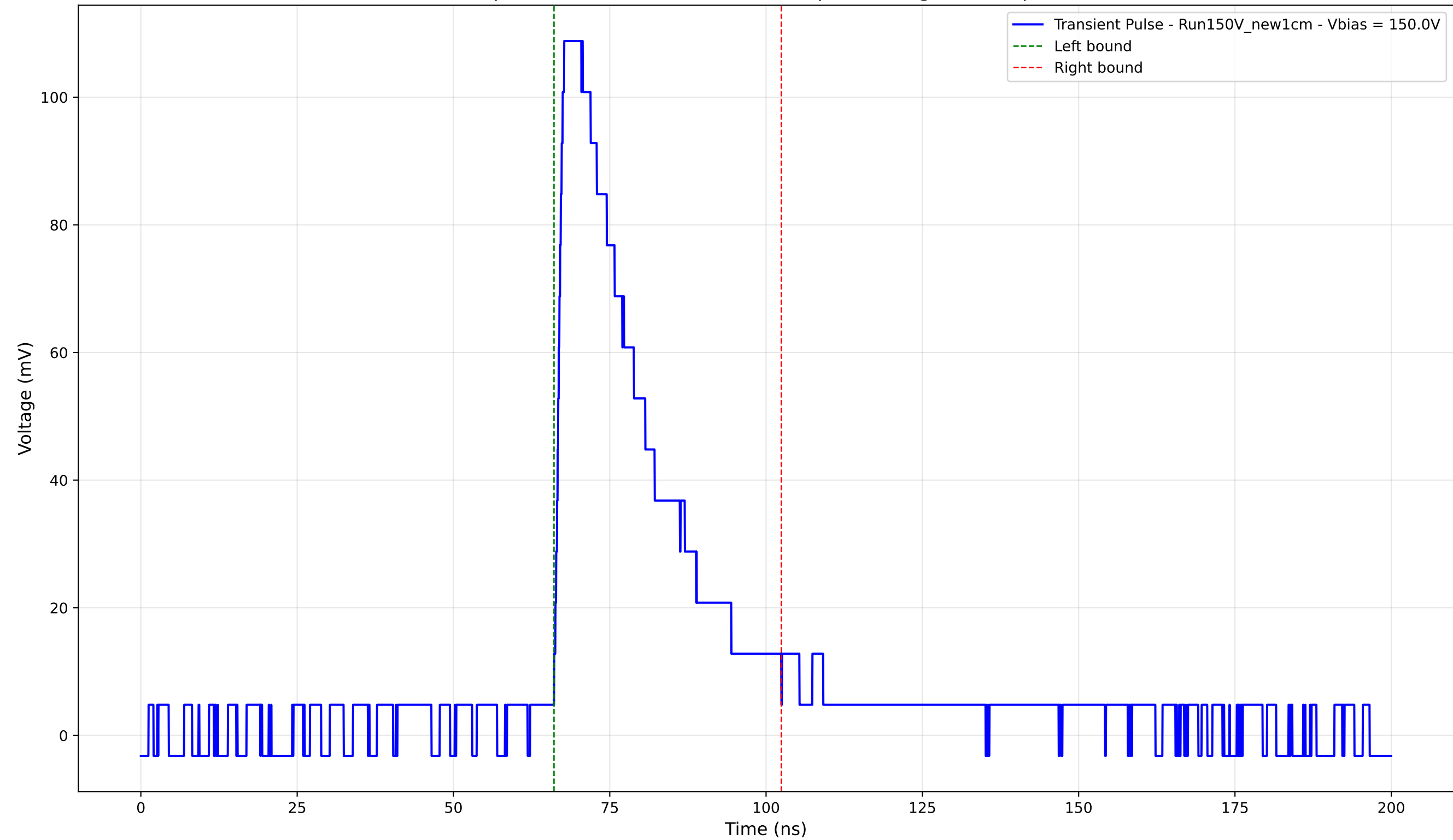
Transient Pulse - Sample: New1cm - Position: 1405.0 \mu\text{m} - Charge: 33.59 pC - Rise Time: 1.36 ns
