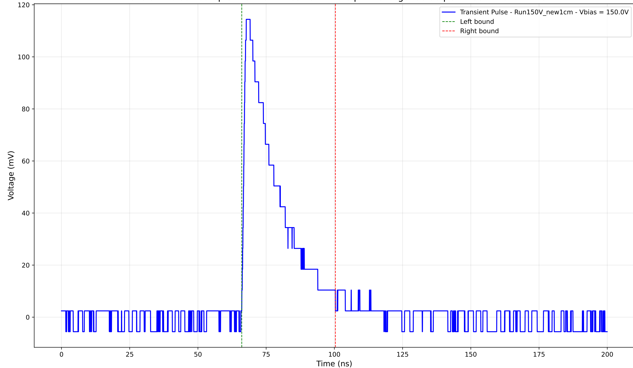
Transient Pulse - Sample: New1cm - Position: 725.0 \mu\text{m} - Charge: 30.30 pC - Rise Time: 1.22 ns
