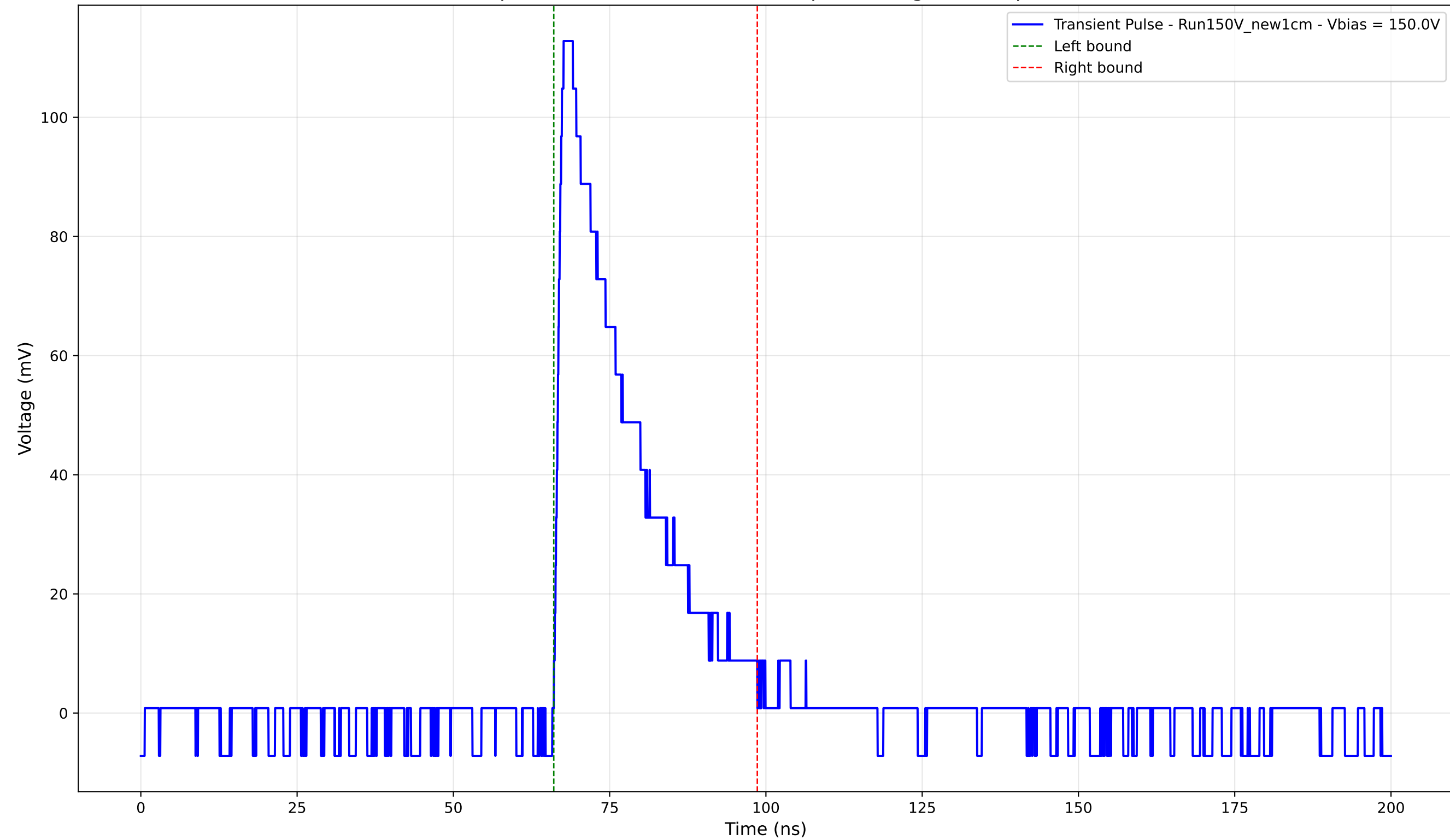
Transient Pulse - Sample: New1cm - Position: 680.0 \mu\text{m} - Charge: 27.72 pC - Rise Time: 1.15 ns
