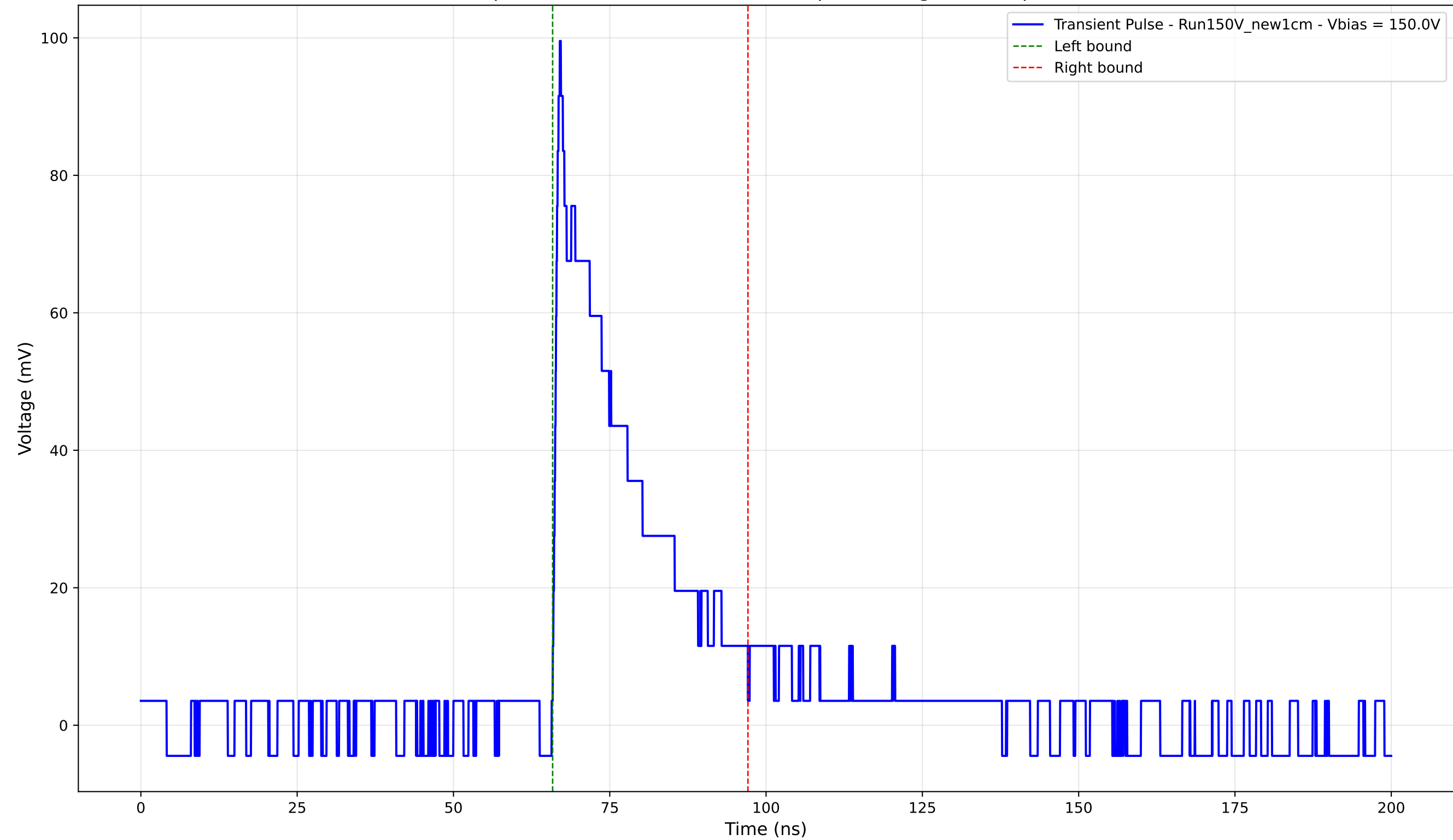
Transient Pulse - Sample: New1cm - Position: 2115.0 \mu\text{m} - Charge: 22.52 pC - Rise Time: 0.92 ns
