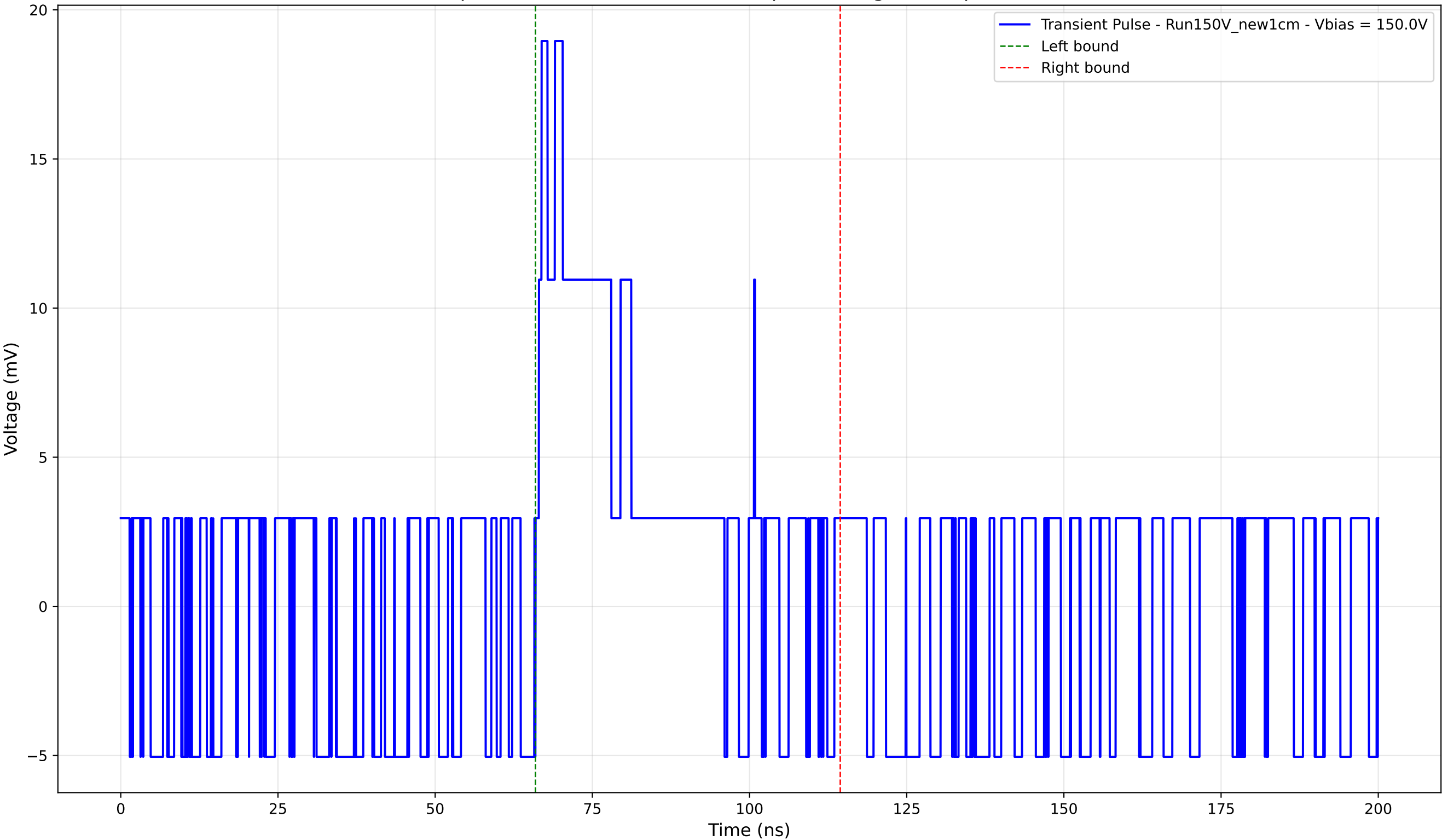
Transient Pulse - Sample: New1cm - Position: 520.0 \mu\text{m} - Charge: 4.43 pC - Rise Time: 0.00 ns (N/A)
