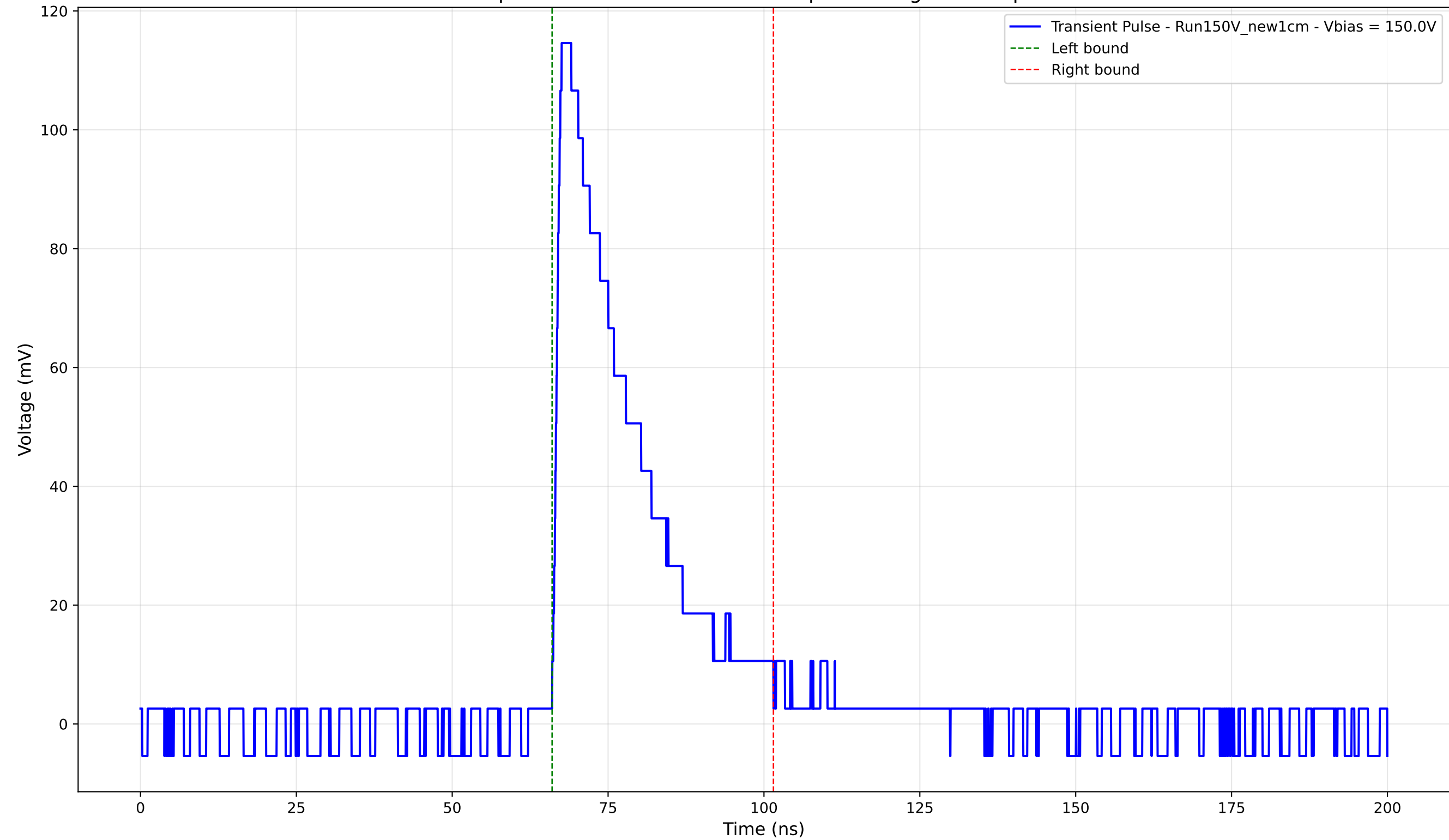
Transient Pulse - Sample: New1cm - Position: 735.0 \mu\text{m} - Charge: 30.31 pC - Rise Time: 1.14 ns
