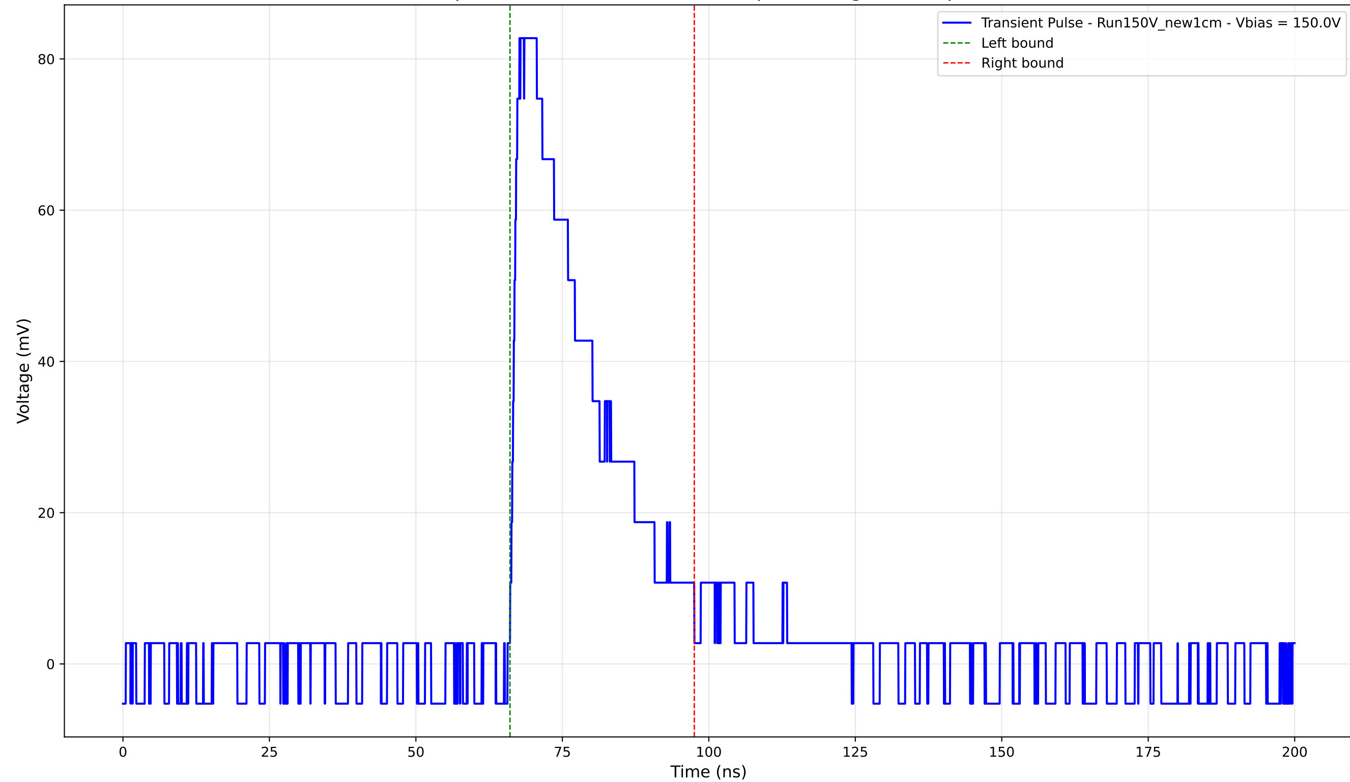
Transient Pulse - Sample: New1cm - Position: 1620.0 \mu\text{m} - Charge: 23.97 pC - Rise Time: 1.23 ns
