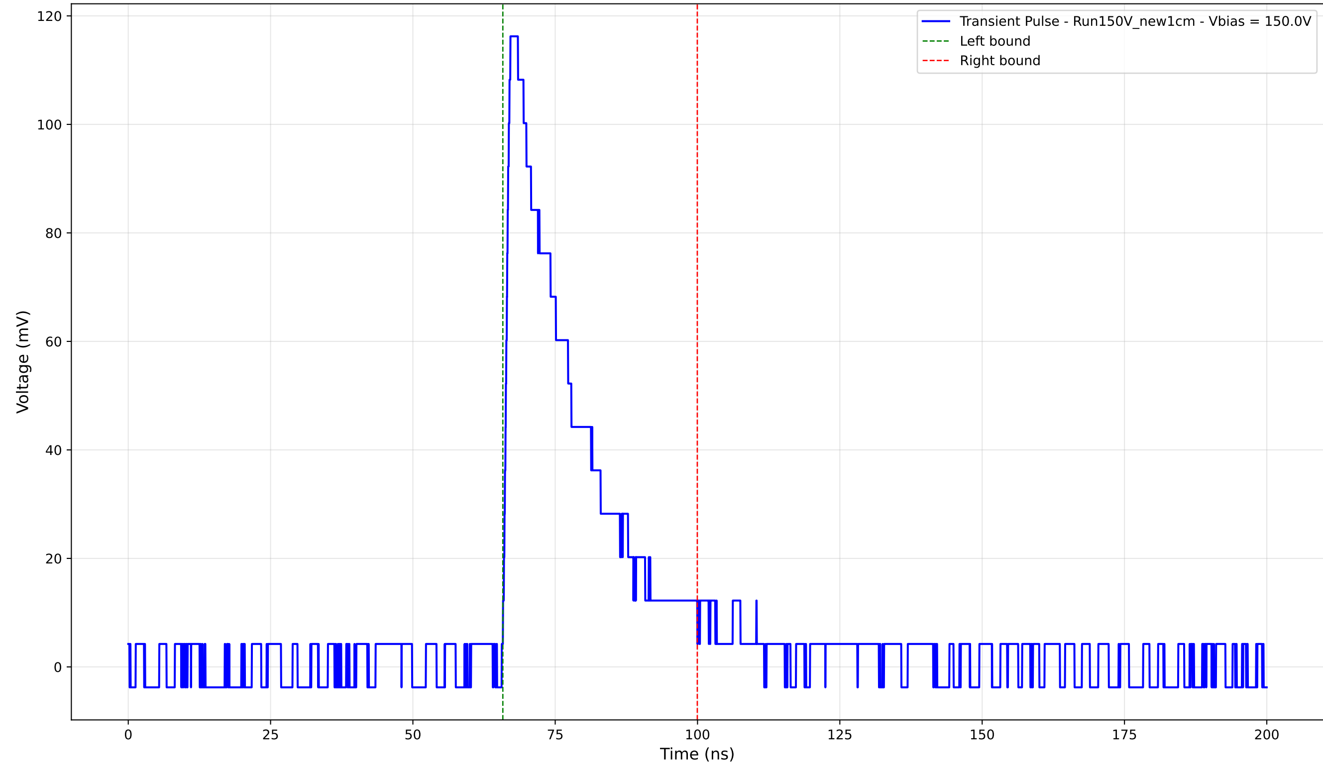
Transient Pulse - Sample: New1cm - Position: 4495.0 \mu\text{m} - Charge: 29.66 pC - Rise Time: 1.14 ns
