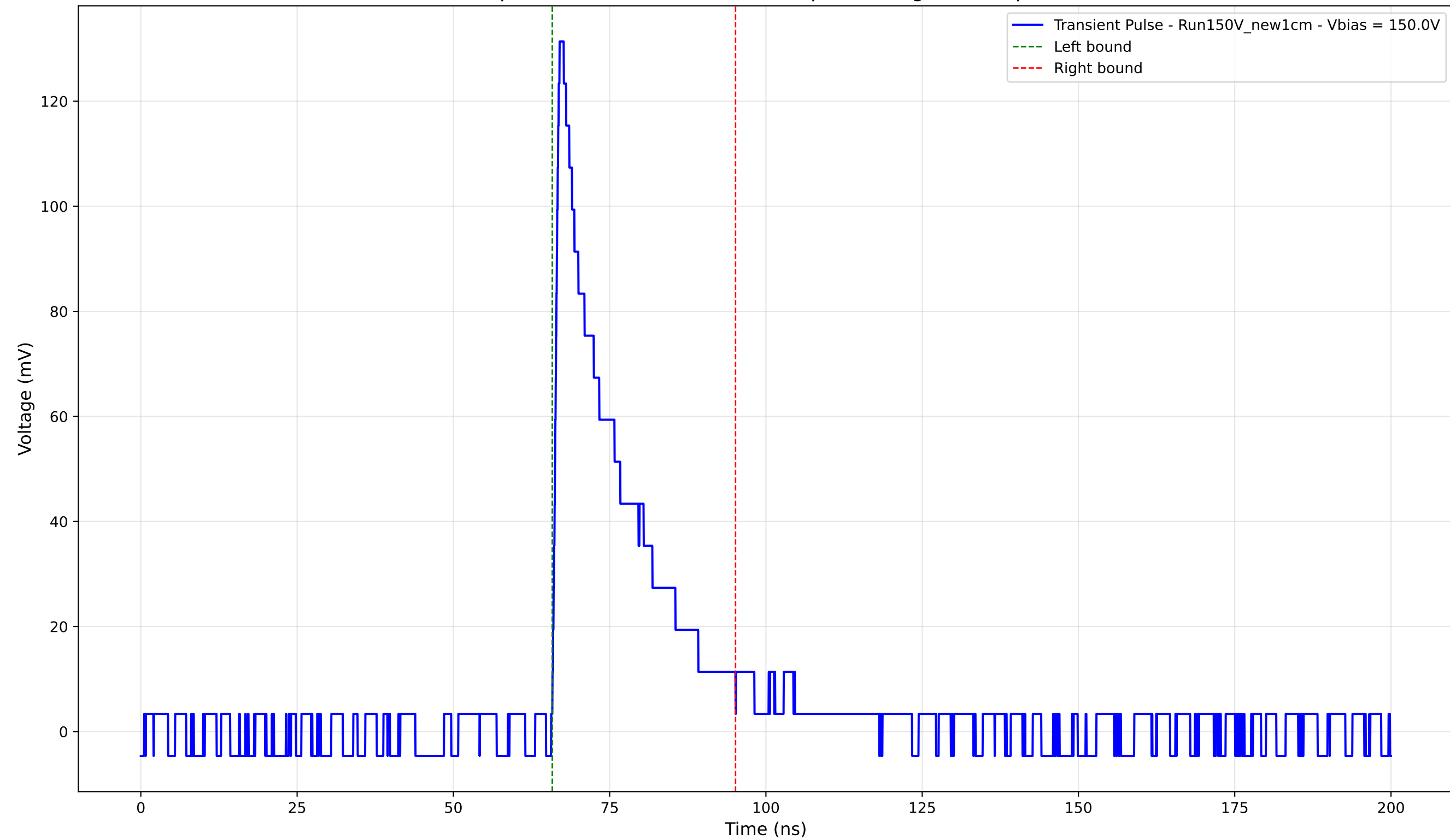
Transient Pulse - Sample: New1cm - Position: 210.0 \mu\text{m} - Charge: 26.22 pC - Rise Time: 0.92 ns
