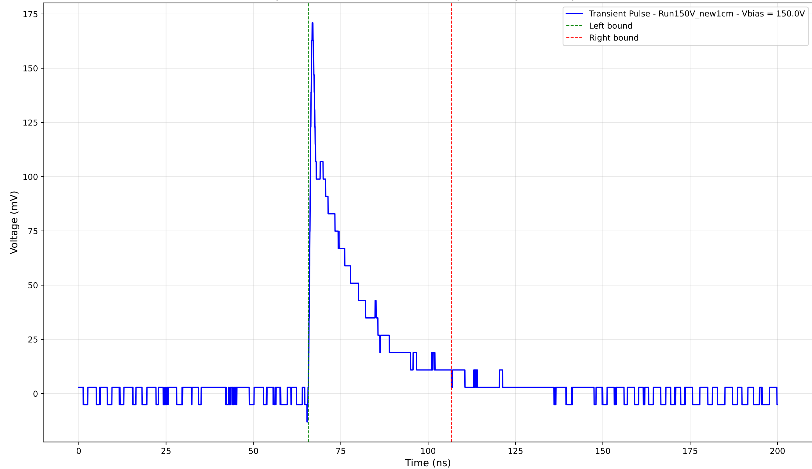
Transient Pulse - Sample: New1cm - Position: 2285.0 \mu\text{m} - Charge: 34.49 pC - Rise Time: 0.80 ns
