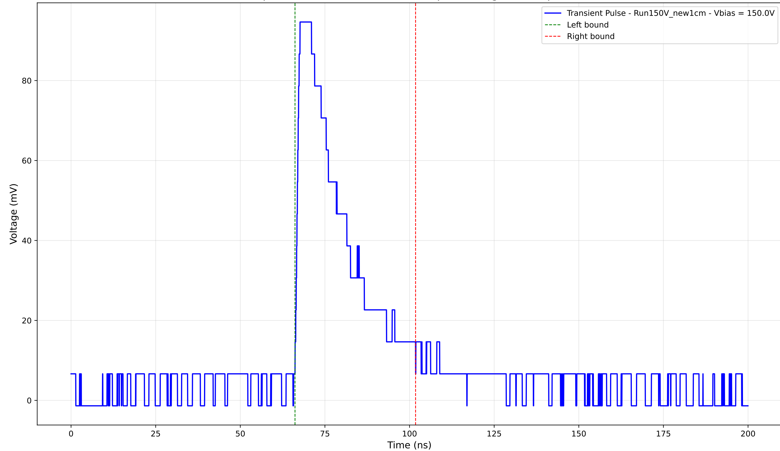
Transient Pulse - Sample: New1cm - Position: 1455.0 \mu\text{m} - Charge: 30.02 pC - Rise Time: 1.21 ns
