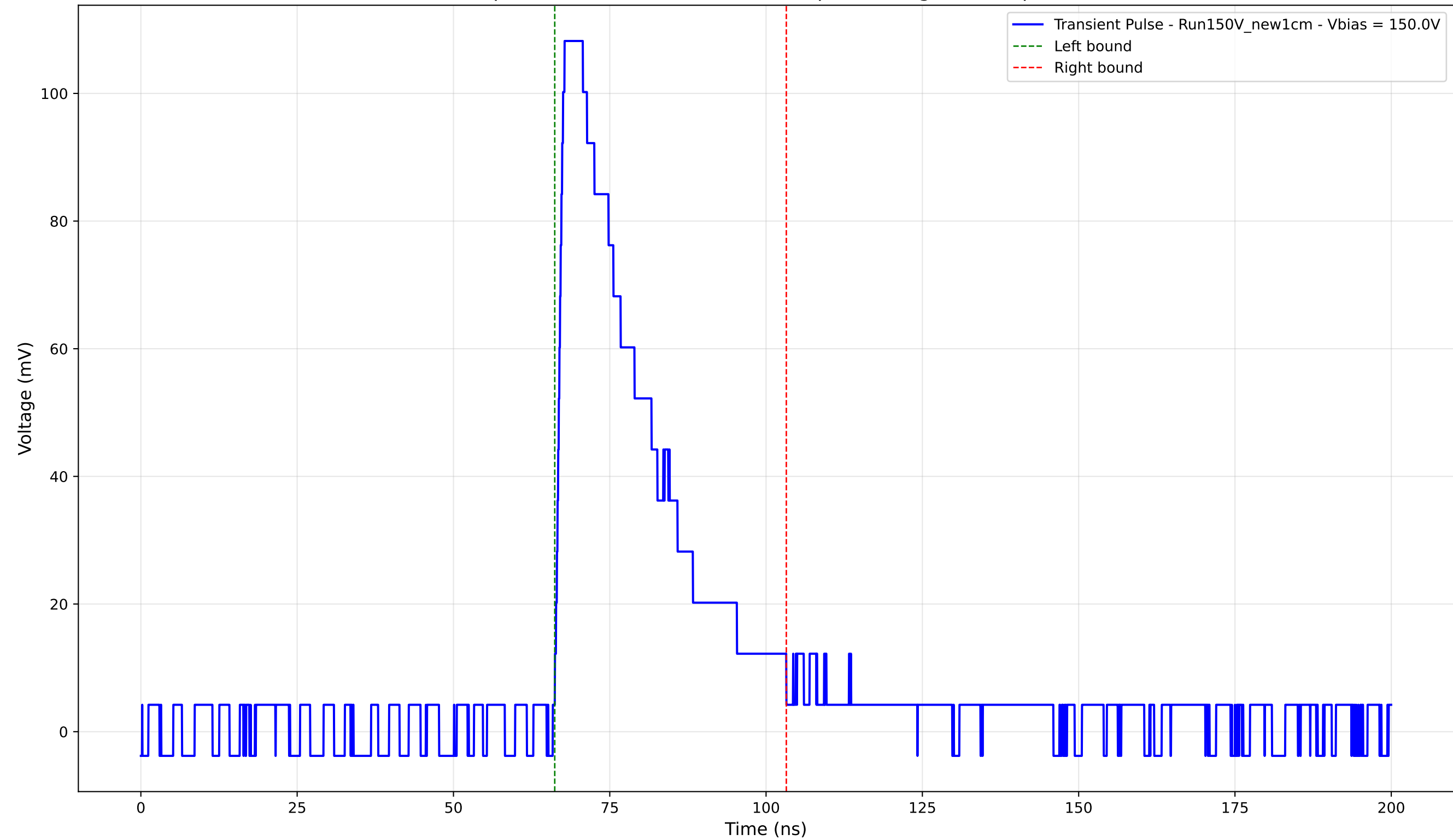
Transient Pulse - Sample: New1cm - Position: 1240.0 \mu\text{m} - Charge: 33.21 pC - Rise Time: 1.30 ns
