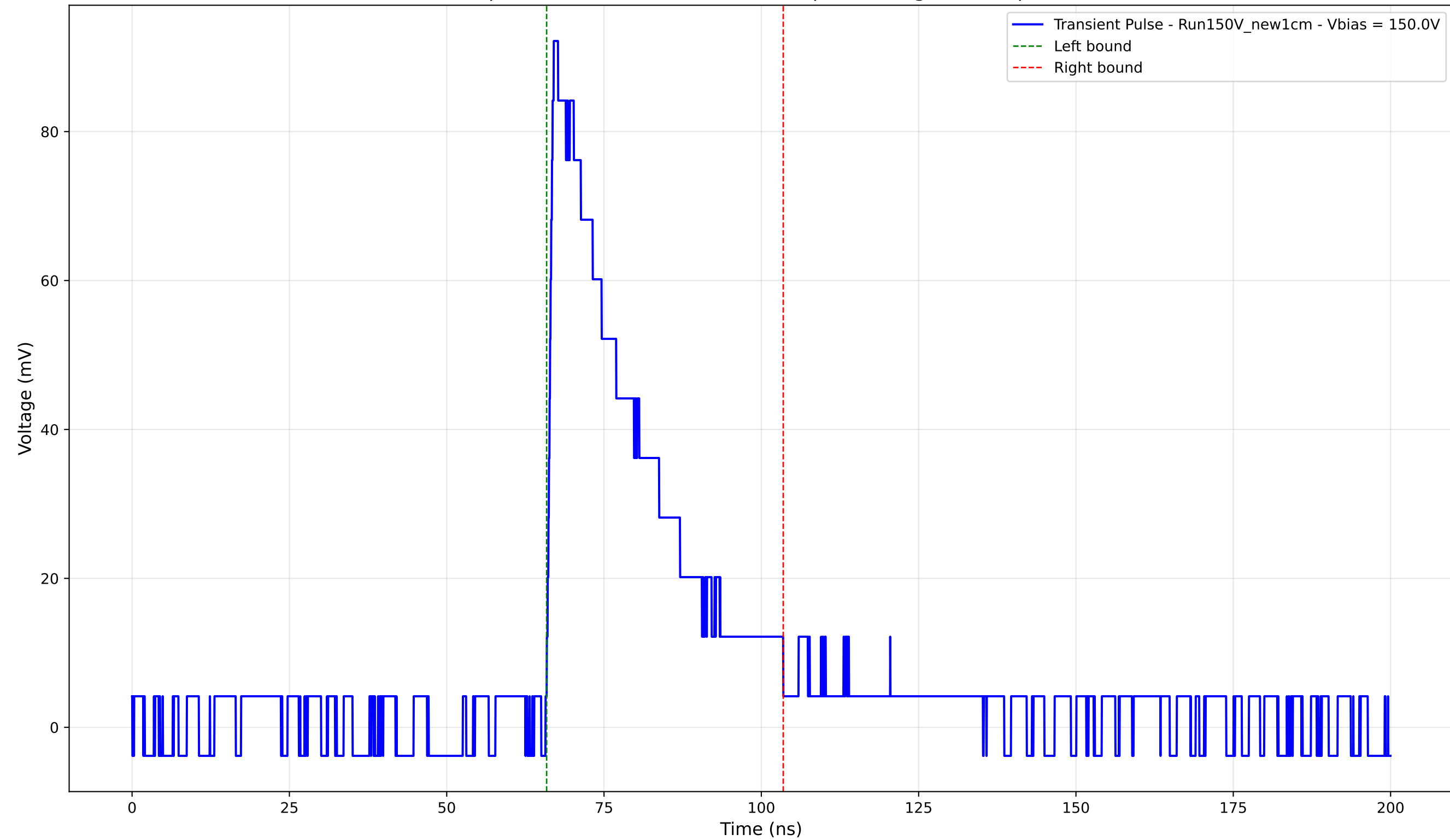
Transient Pulse - Sample: New1cm - Position: 3125.0 \mu\text{m} - Charge: 27.09 pC - Rise Time: 0.93 ns
