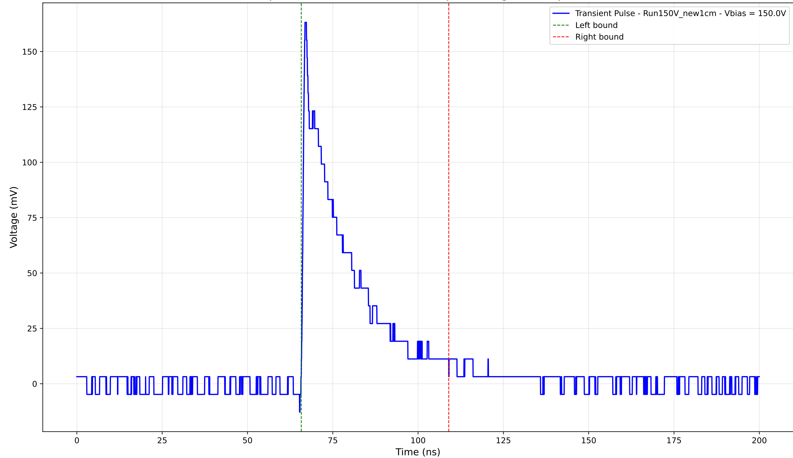
Transient Pulse - Sample: New1cm - Position: 2940.0 \mu\text{m} - Charge: 39.99 pC - Rise Time: 0.83 ns
