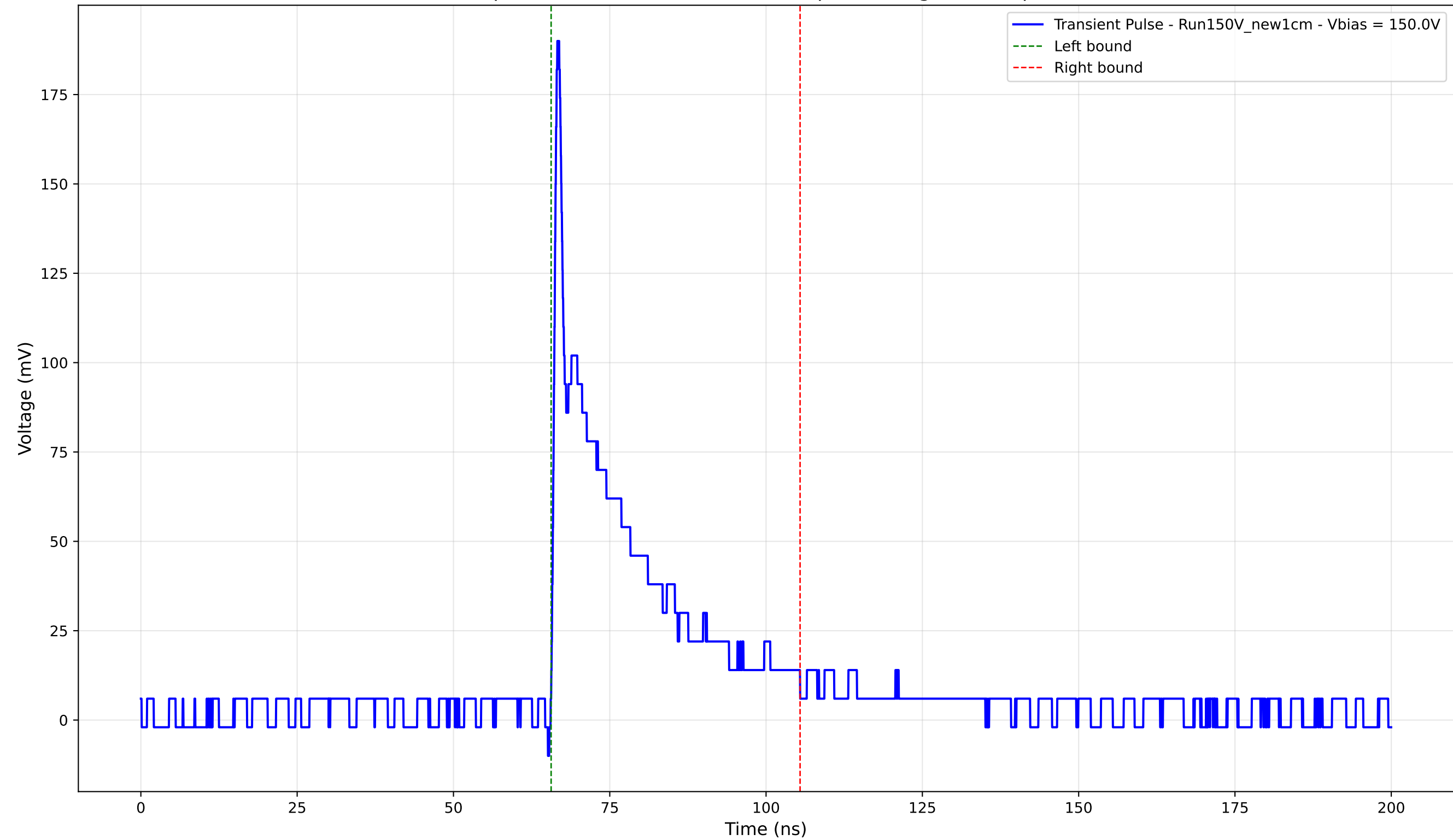
Transient Pulse - Sample: New1cm - Position: 2455.0 \mu\text{m} - Charge: 34.67 pC - Rise Time: 0.79 ns
