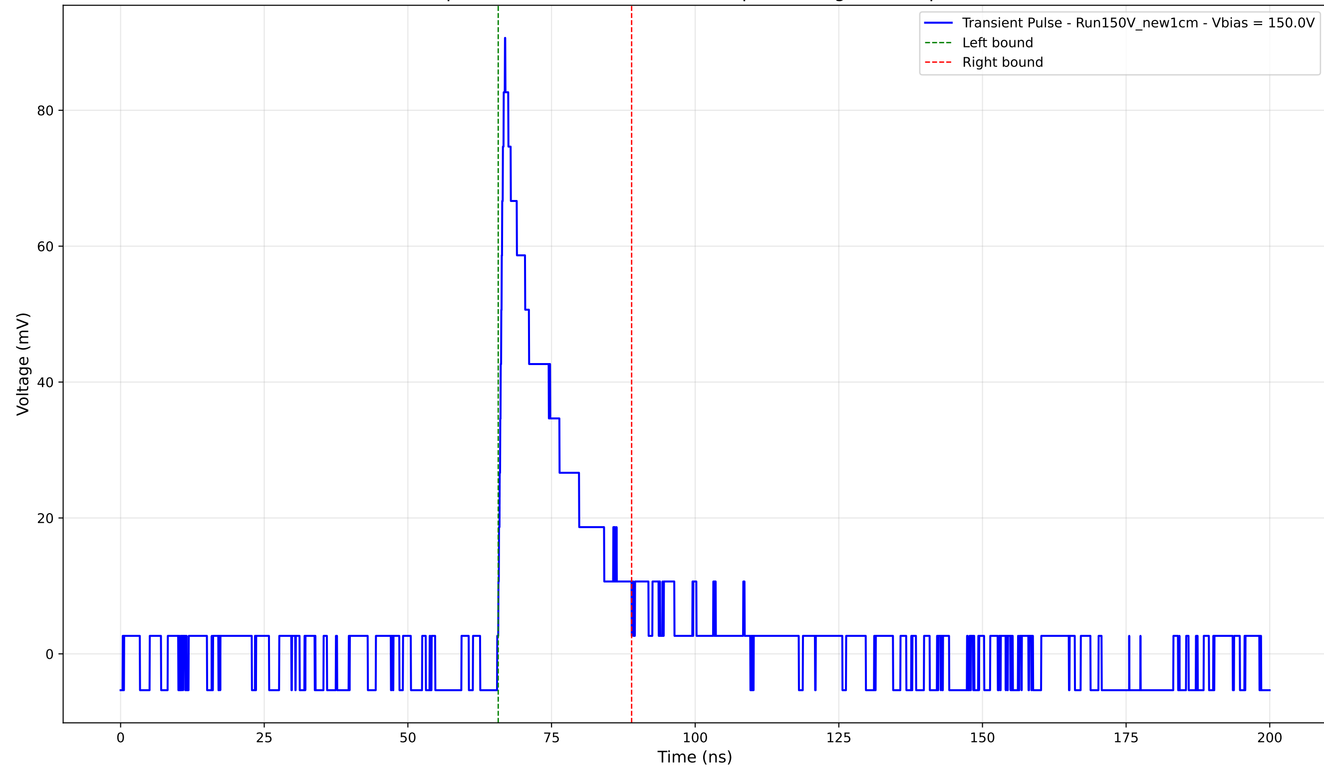
Transient Pulse - Sample: New1cm - Position: 4845.0 \mu\text{m} - Charge: 15.35 pC - Rise Time: 0.92 ns
