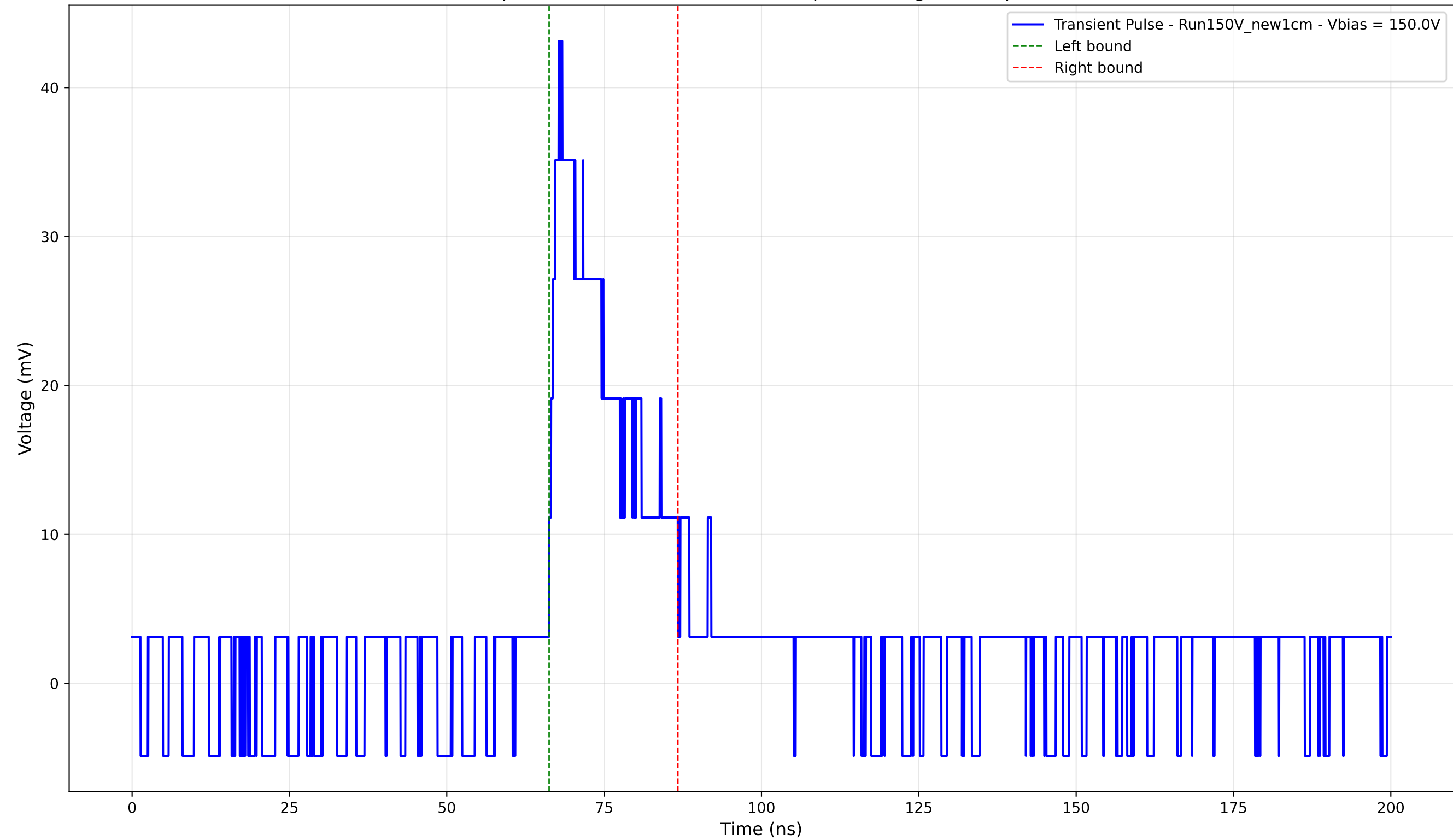
Transient Pulse - Sample: New1cm - Position: 565.0 \mu\text{m} - Charge: 8.60 pC - Rise Time: 1.52 ns
