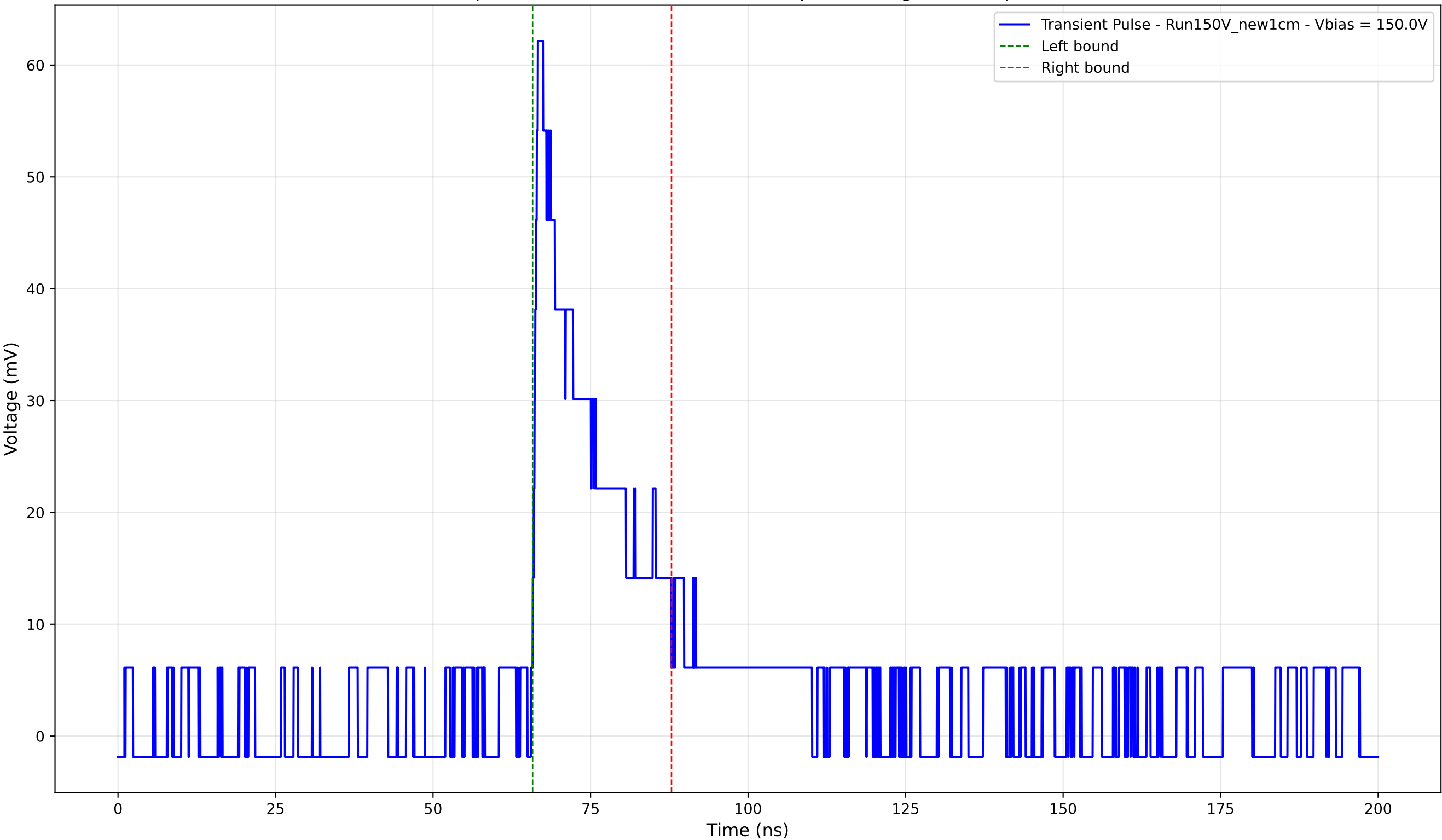
Transient Pulse - Sample: New1cm - Position: 4860.0 \mu\text{m} - Charge: 12.07 pC - Rise Time: 0.82 ns
