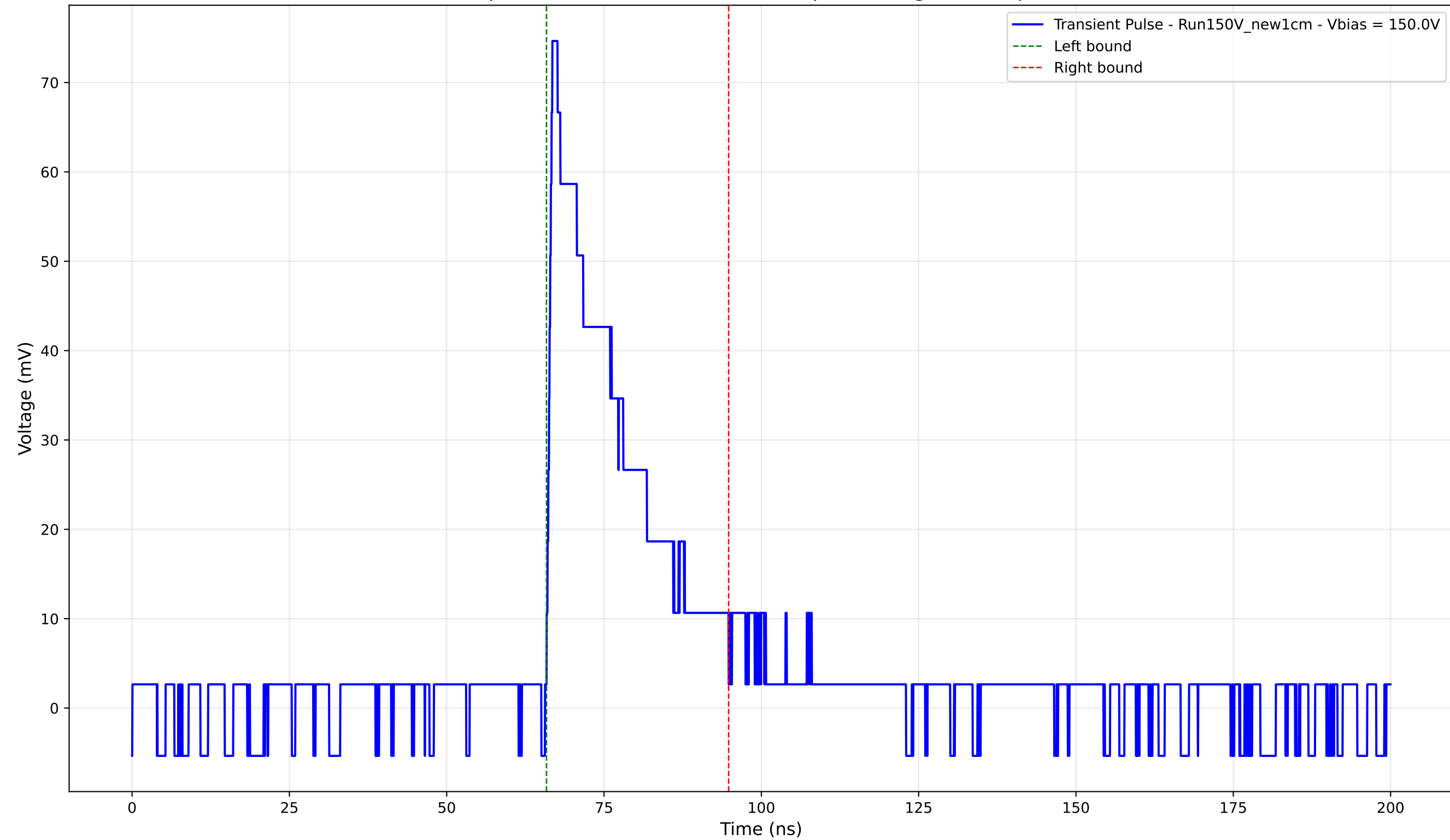
Transient Pulse - Sample: New1cm - Position: 3010.0 \mu\text{m} - Charge: 17.31 pC - Rise Time: 0.91 ns
