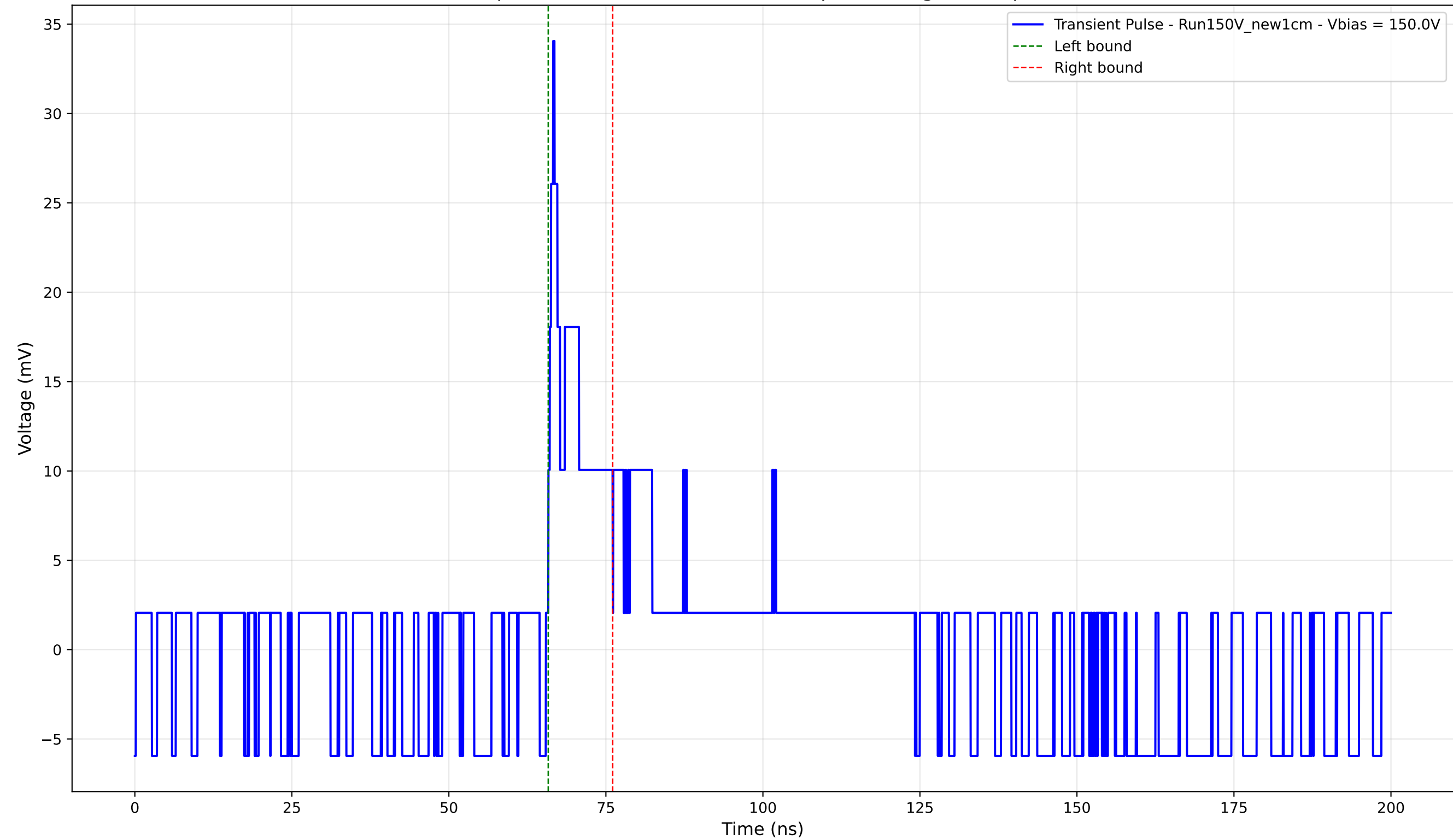
Transient Pulse - Sample: New1cm - Position: 2565.0 \mu\text{m} - Charge: 2.88 pC - Rise Time: 0.78 ns
