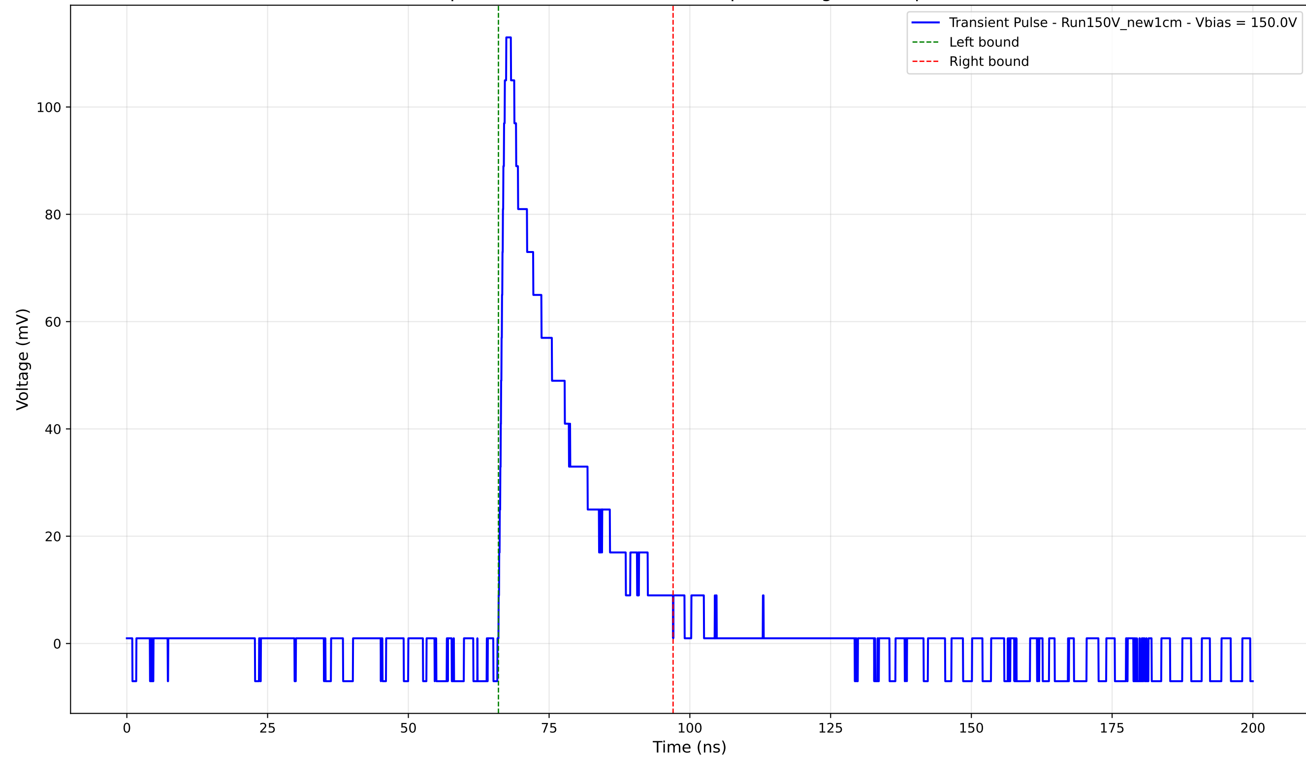
Transient Pulse - Sample: New1cm - Position: 425.0 \mu\text{m} - Charge: 24.23 pC - Rise Time: 1.01 ns
