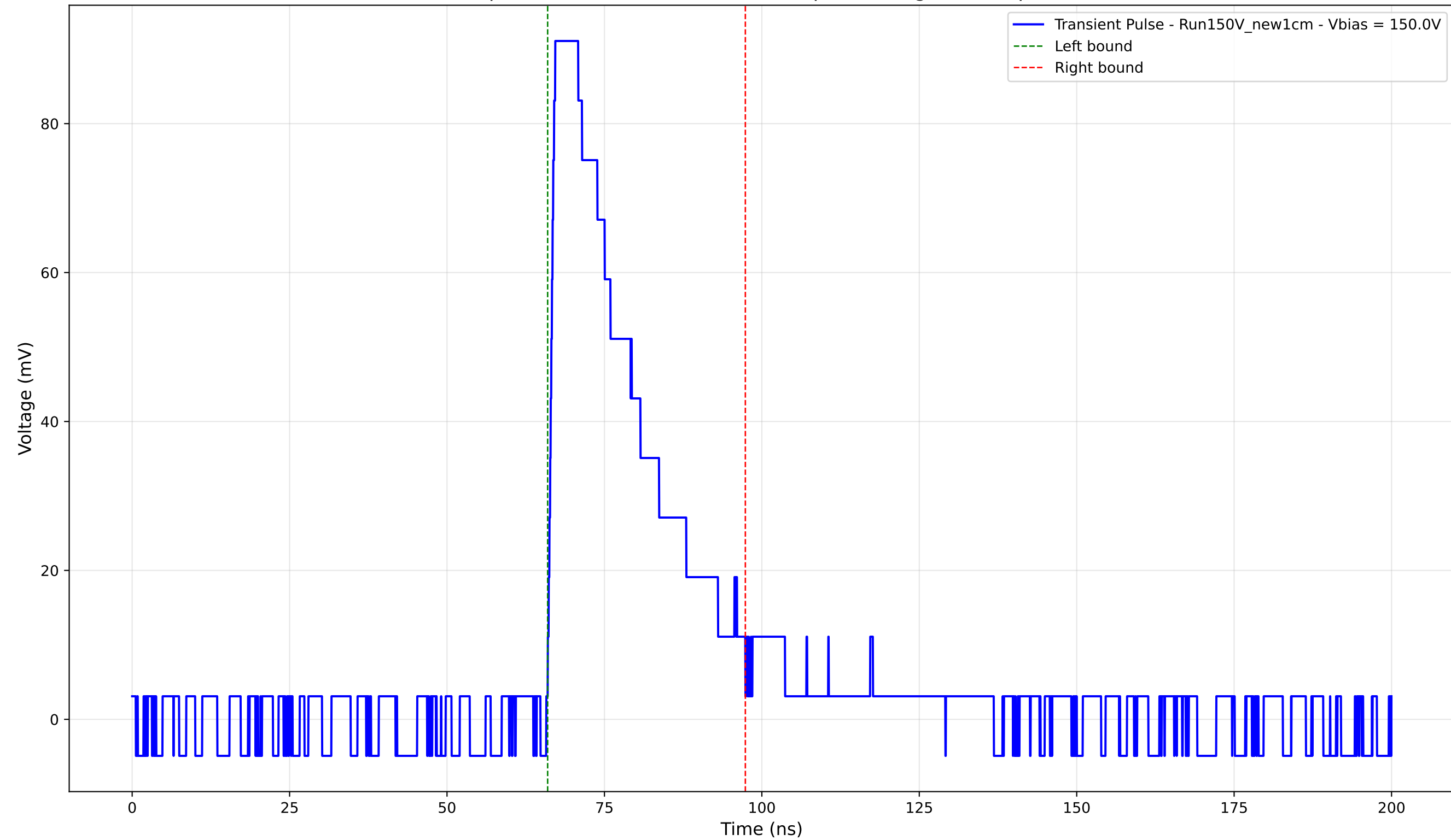
Transient Pulse - Sample: New1cm - Position: 1815.0 \mu\text{m} - Charge: 27.13 pC - Rise Time: 1.00 ns
