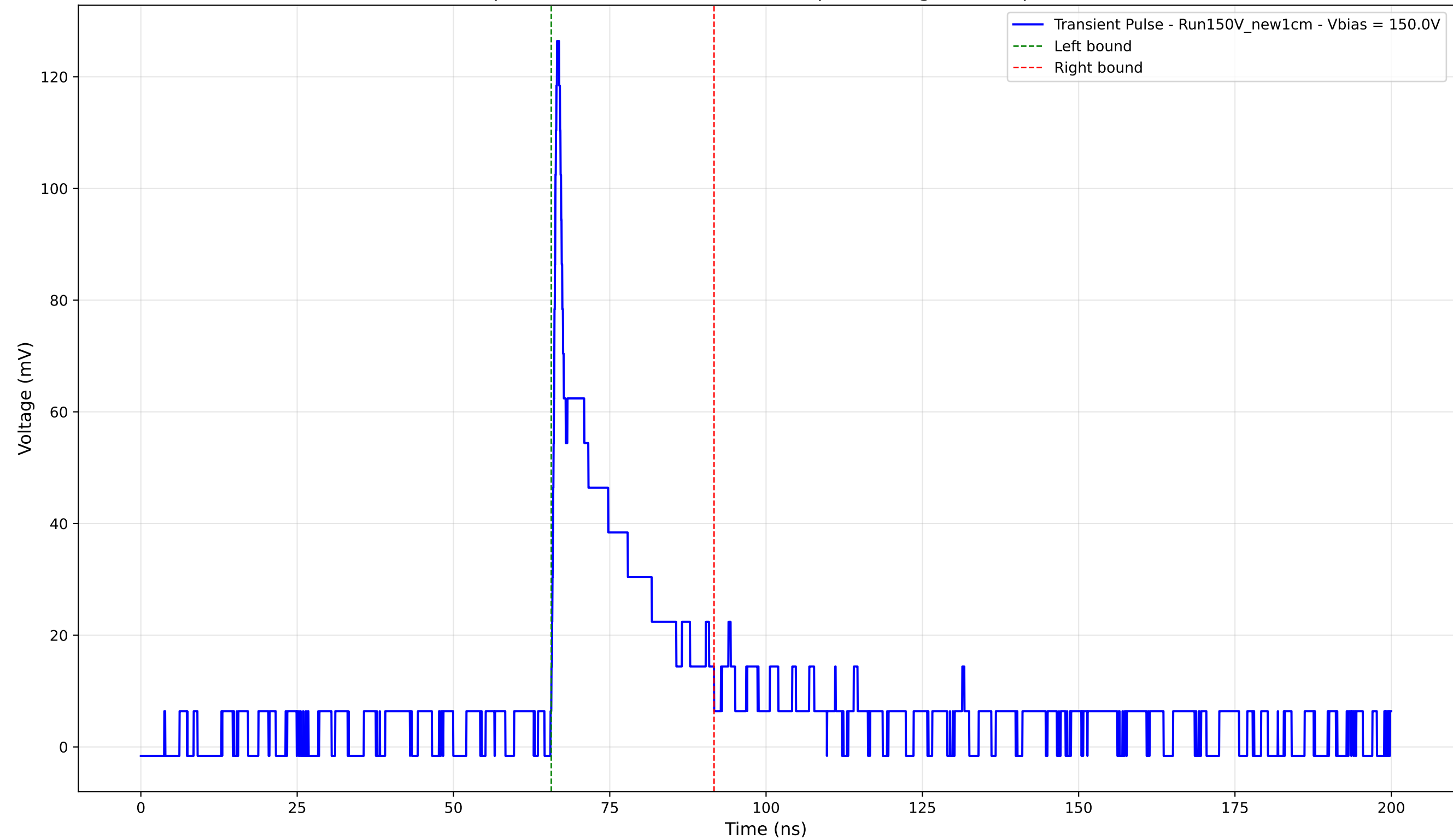
Transient Pulse - Sample: New1cm - Position: 2610.0 \mu\text{m} - Charge: 19.70 pC - Rise Time: 0.80 ns
