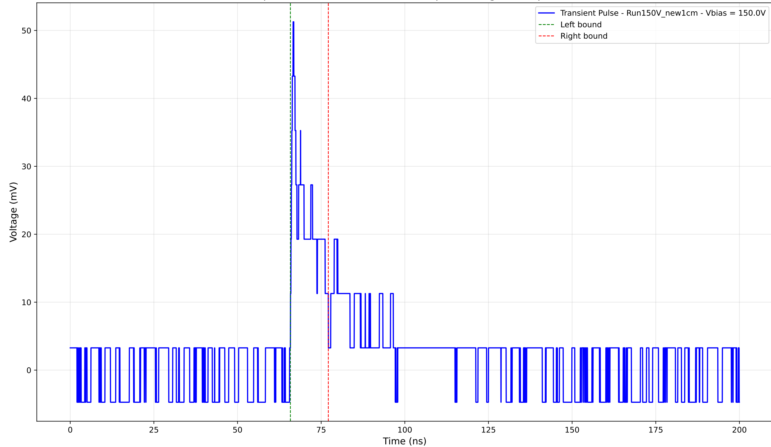
Transient Pulse - Sample: New1cm - Position: 2525.0 \mu\text{m} - Charge: 5.14 pC - Rise Time: 0.80 ns
