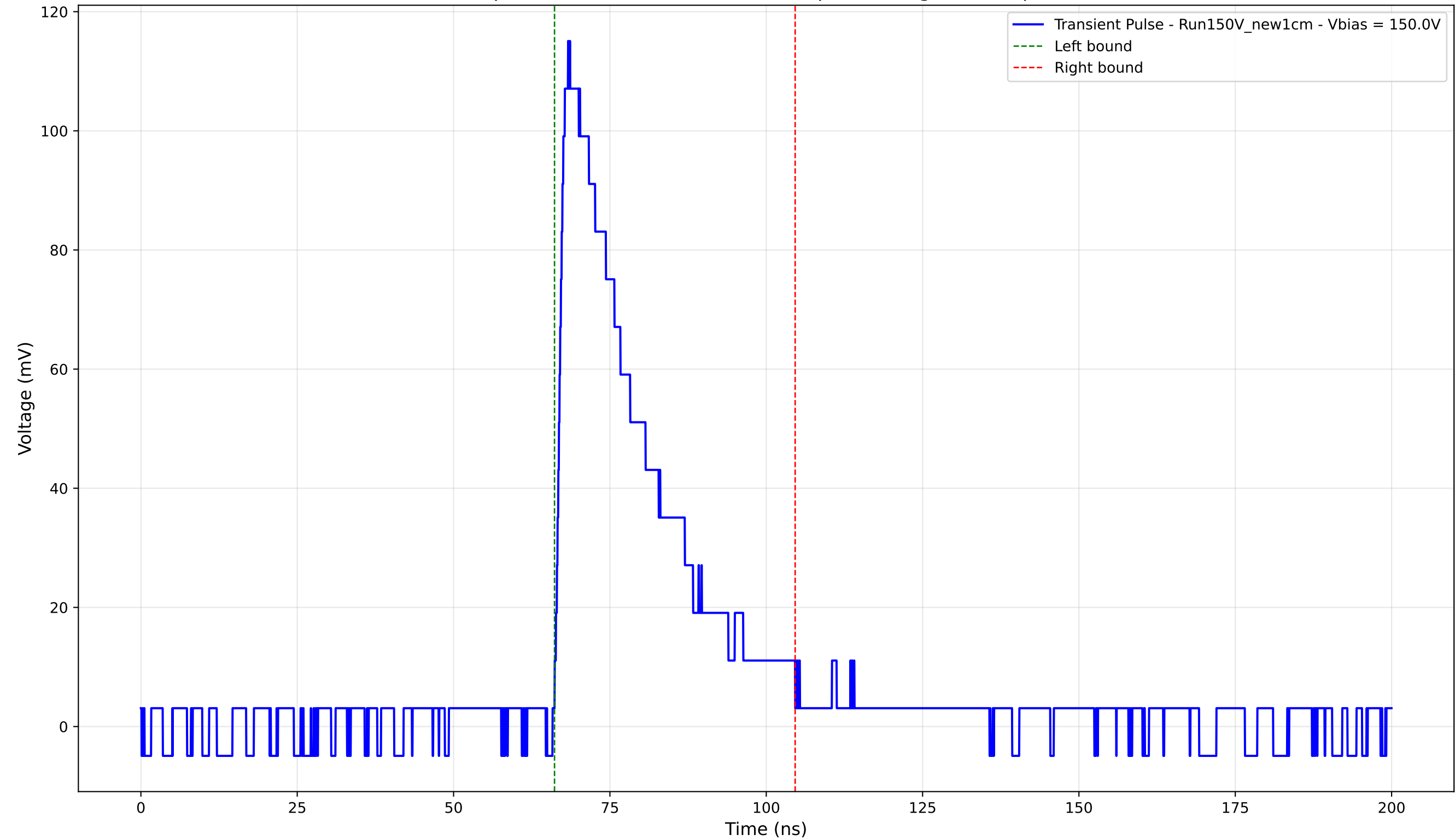
Transient Pulse - Sample: New1cm - Position: 1195.0 \mu\text{m} - Charge: 32.48 pC - Rise Time: 1.44 ns
