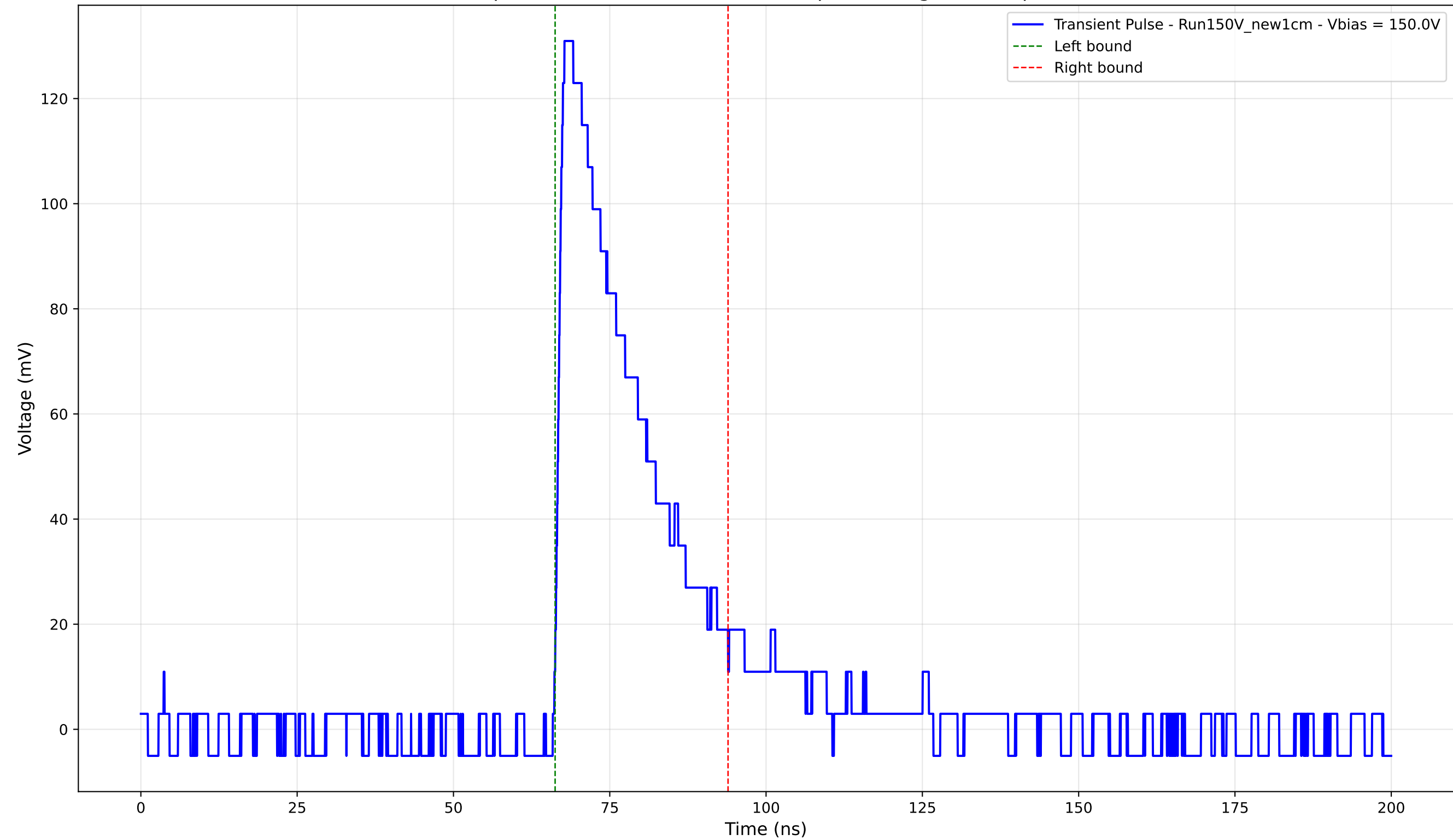
Transient Pulse - Sample: New1cm - Position: 3685.0 \mu\text{m} - Charge: 35.13 pC - Rise Time: 1.23 ns
