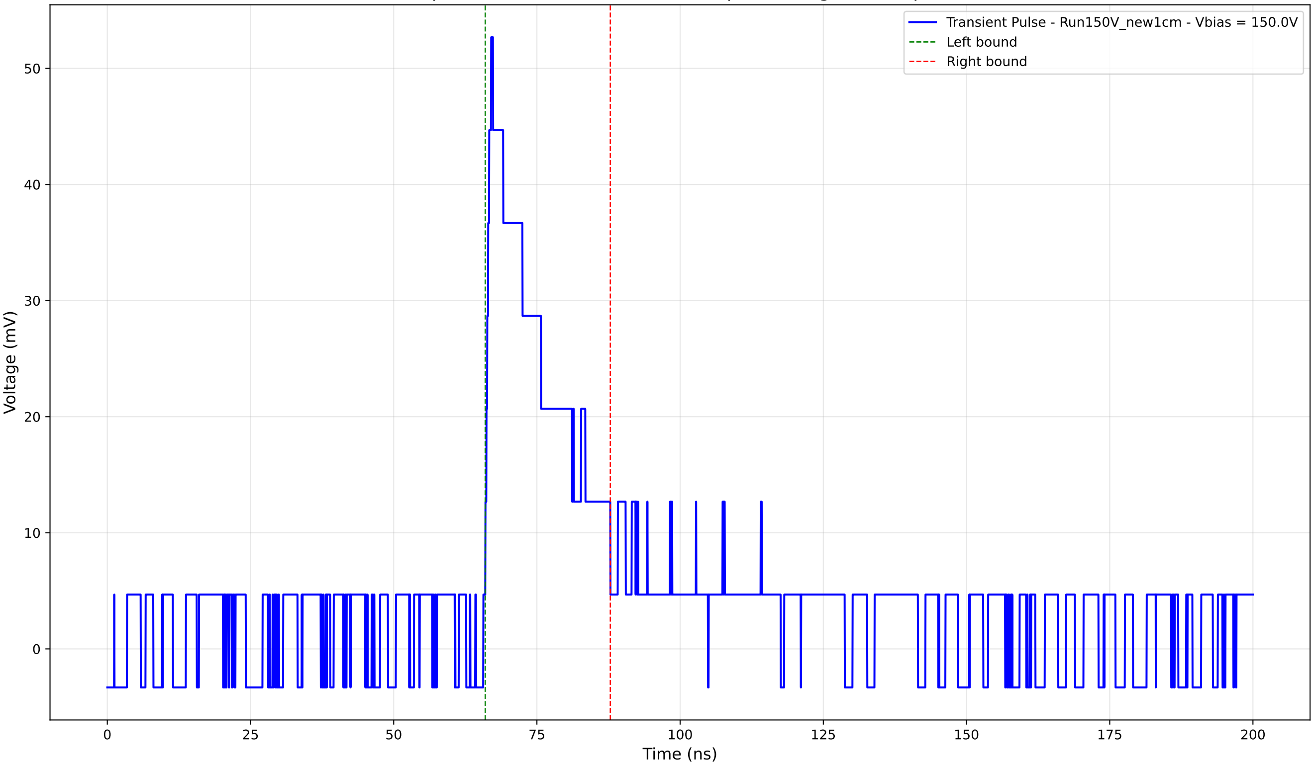
Transient Pulse - Sample: New1cm - Position: 3025.0 \mu\text{m} - Charge: 10.98 pC - Rise Time: 1.02 ns
