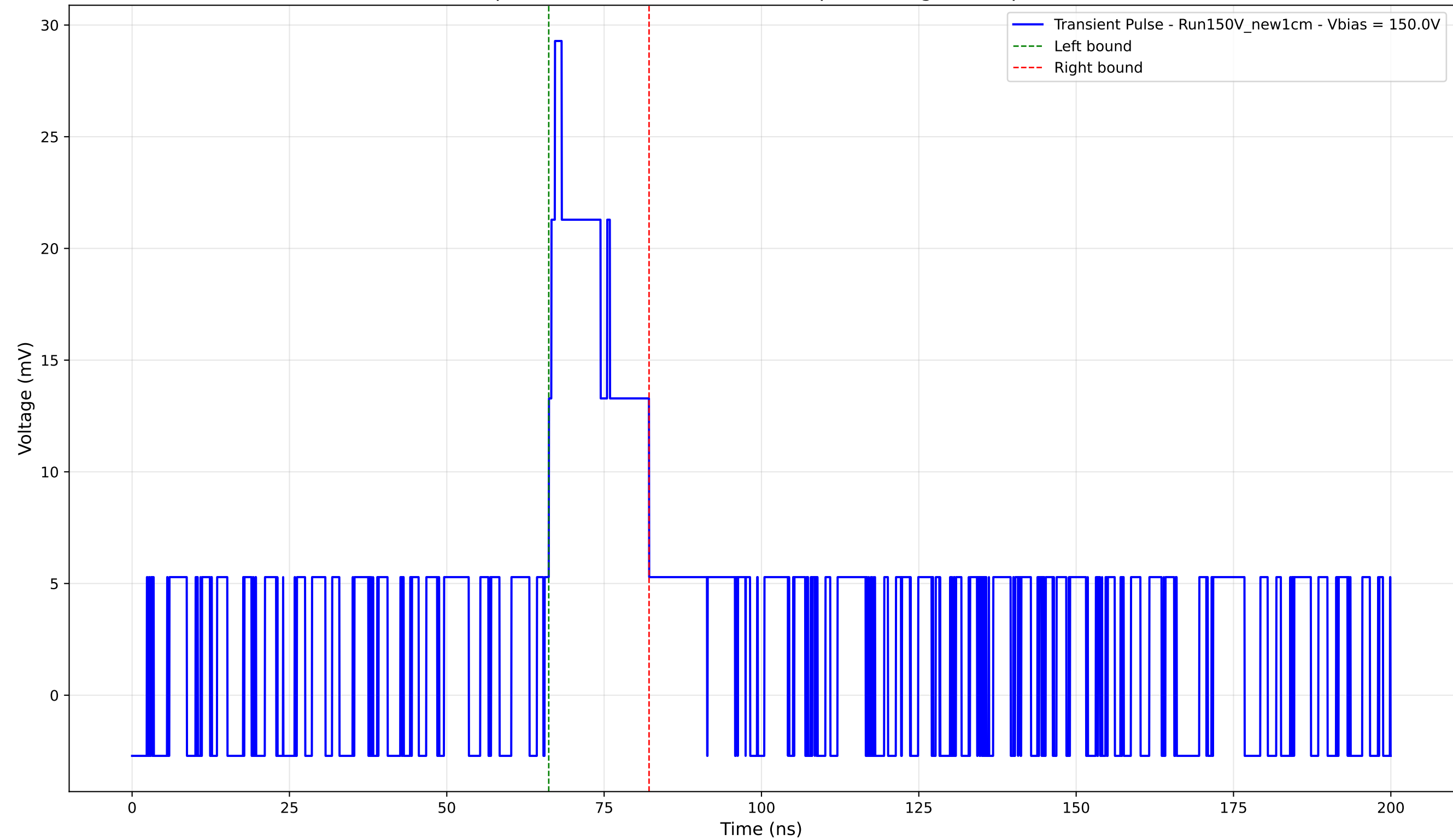
Transient Pulse - Sample: New1cm - Position: 4585.0 \mu\text{m} - Charge: 5.73 pC - Rise Time: 1.66 ns
