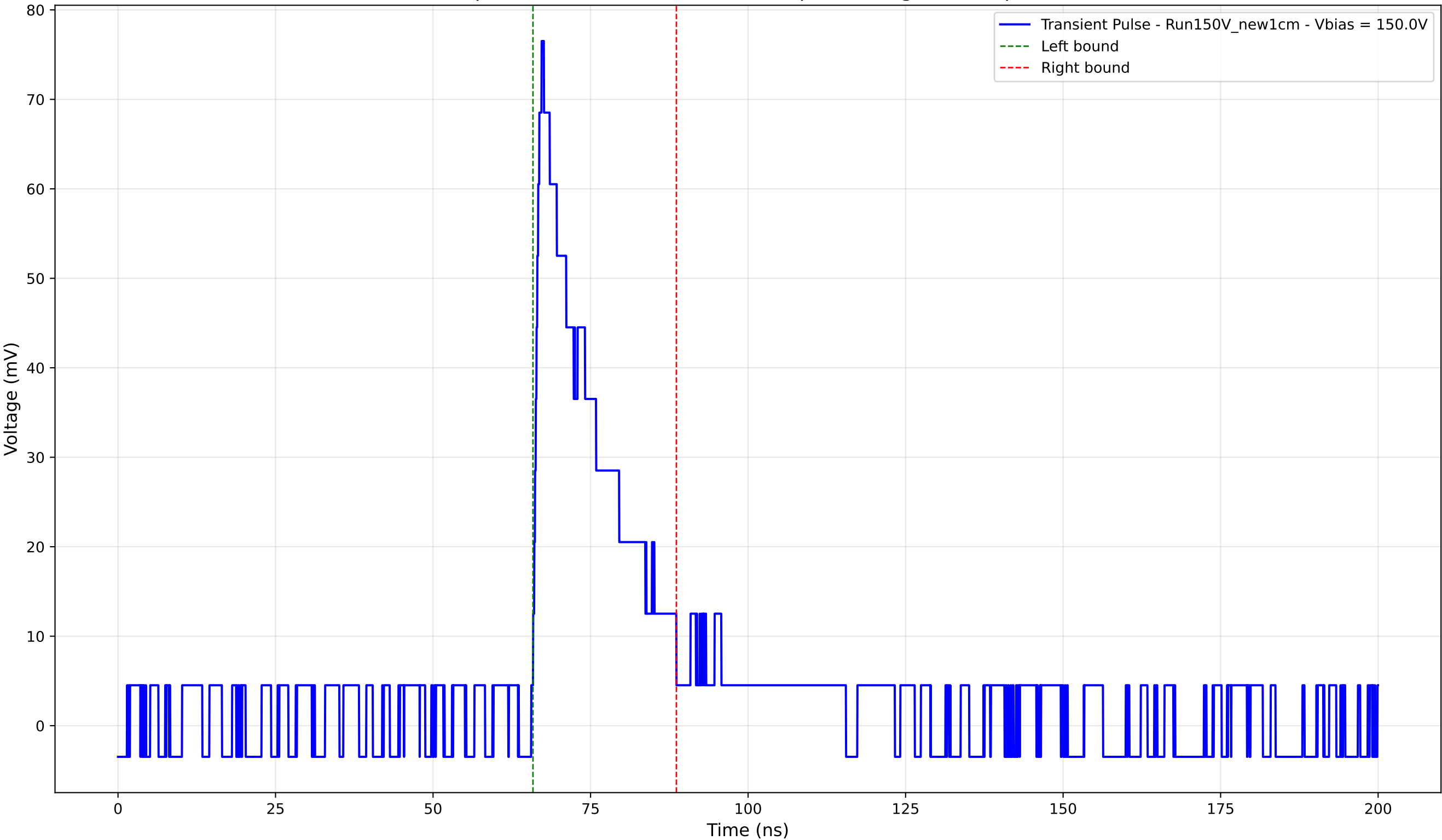
Transient Pulse - Sample: New1cm - Position: 4620.0 \mu\text{m} - Charge: 14.91 pC - Rise Time: 1.35 ns
