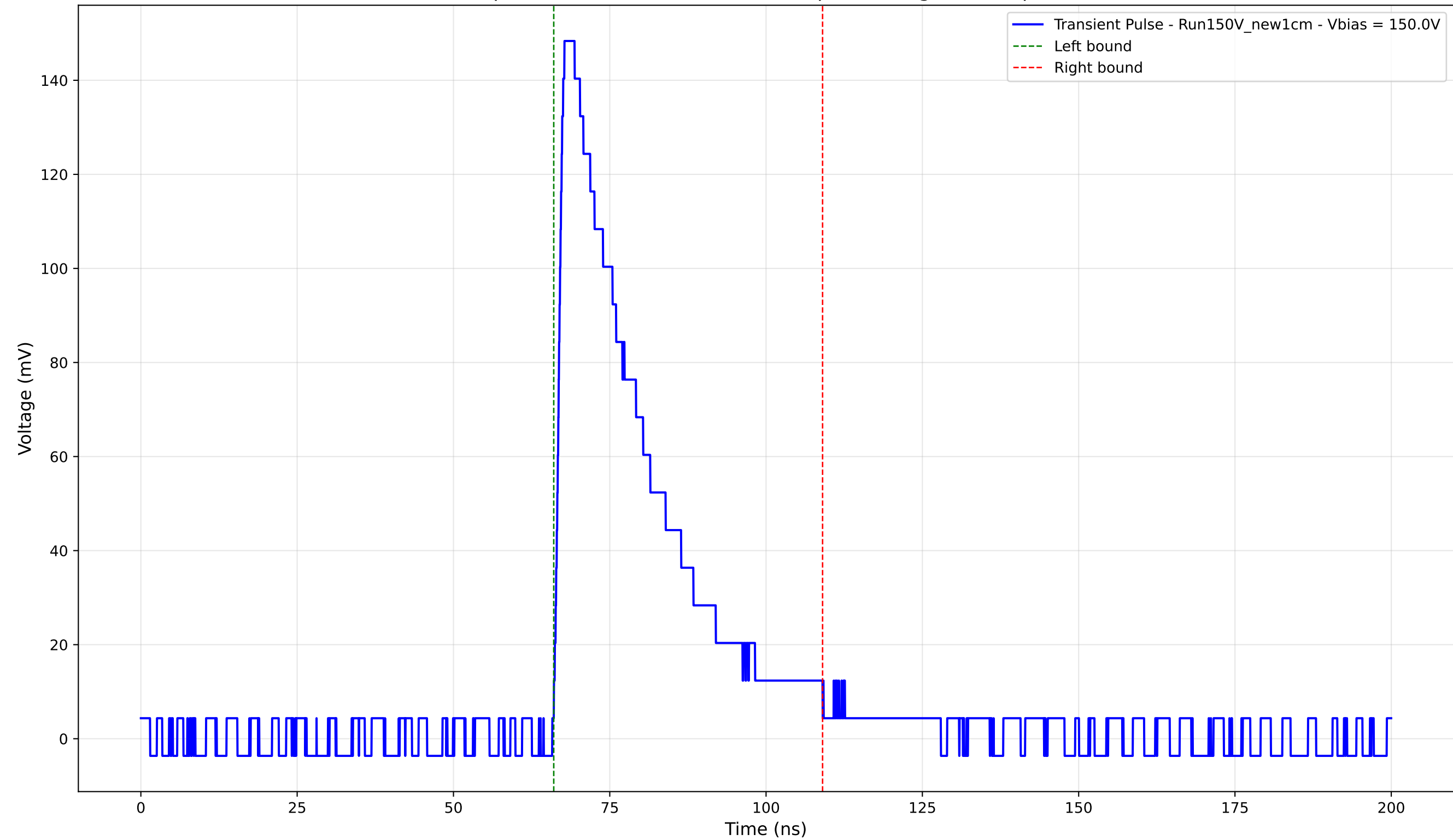
Transient Pulse - Sample: New1cm - Position: 3875.0 \mu\text{m} - Charge: 44.15 pC - Rise Time: 1.35 ns
