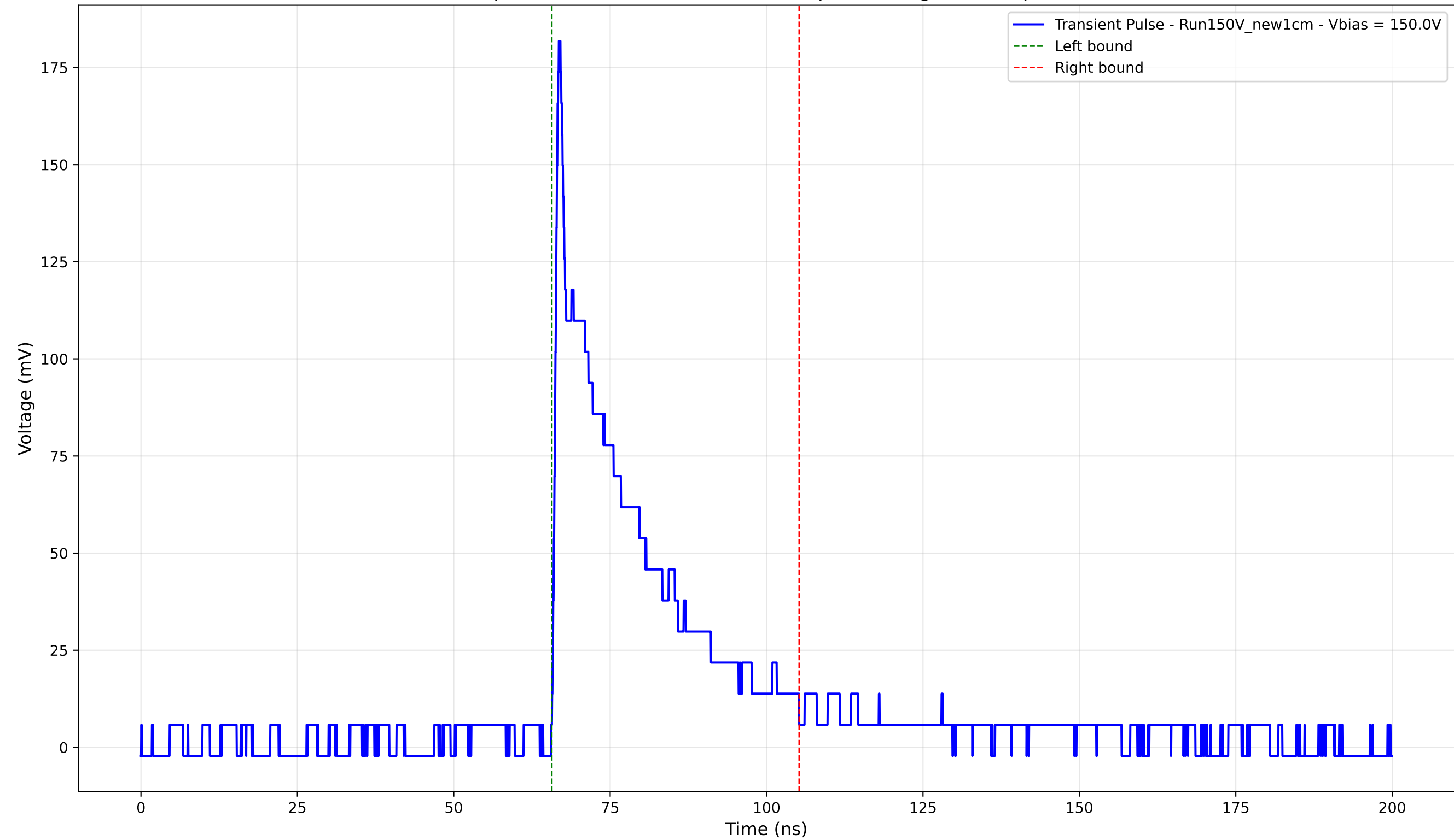
Transient Pulse - Sample: New1cm - Position: 2830.0 \mu\text{m} - Charge: 39.23 pC - Rise Time: 0.83 ns
