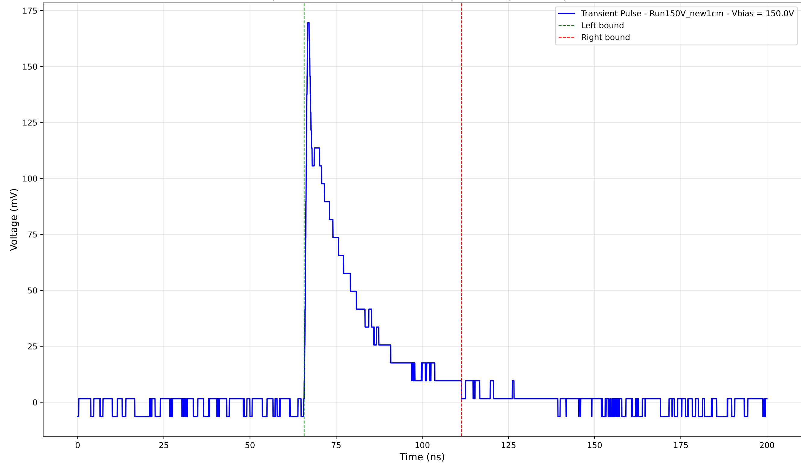
Transient Pulse - Sample: New1cm - Position: 2855.0 \mu\text{m} - Charge: 37.77 pC - Rise Time: 0.80 ns
