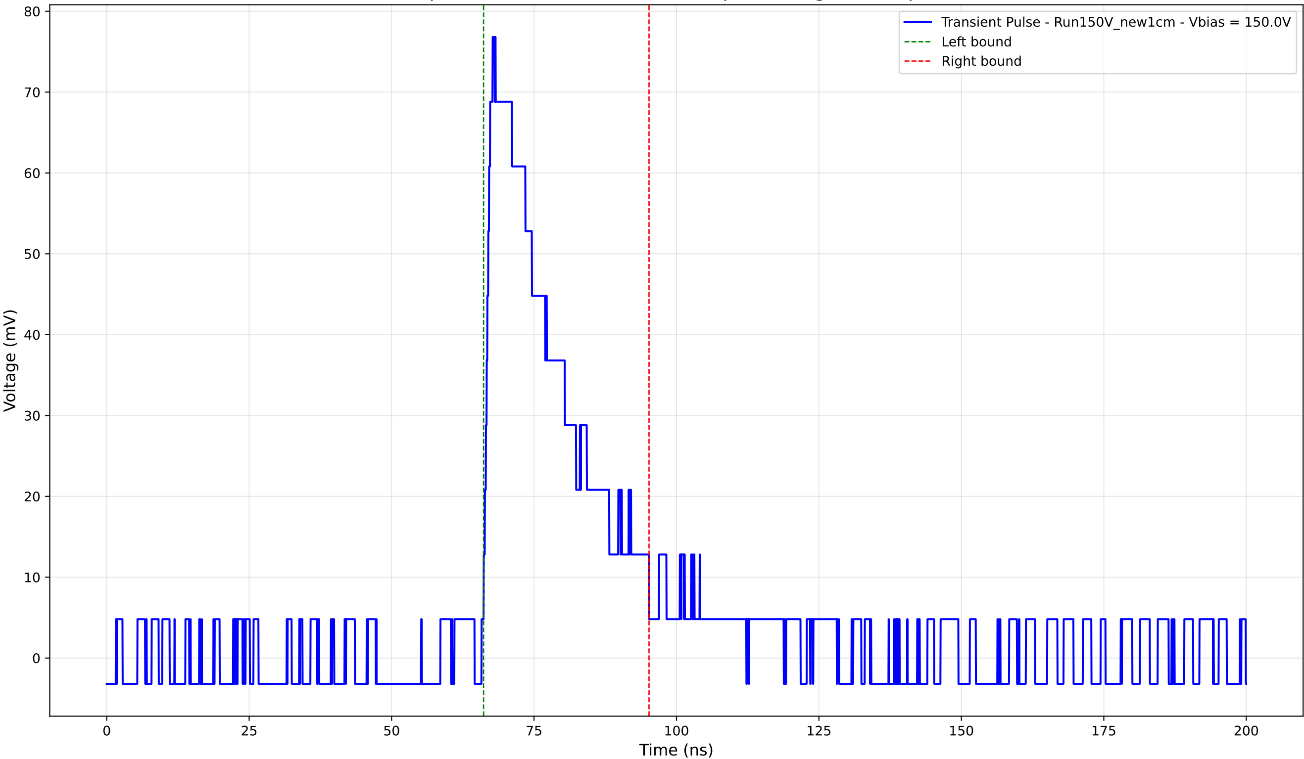
Transient Pulse - Sample: New1cm - Position: 3615.0 \mu\text{m} - Charge: 20.56 pC - Rise Time: 1.57 ns
