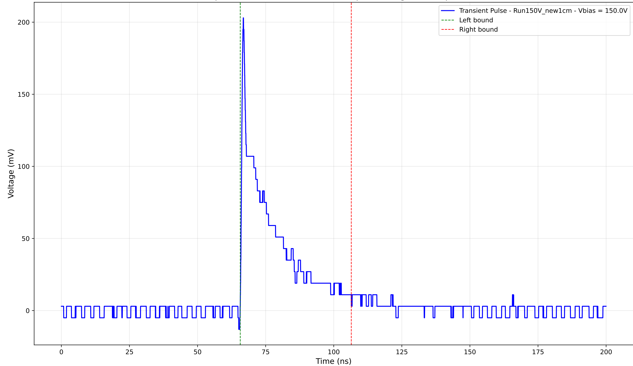
Transient Pulse - Sample: New1cm - Position: 2715.0 \mu\text{m} - Charge: 37.62 pC - Rise Time: 0.78 ns
