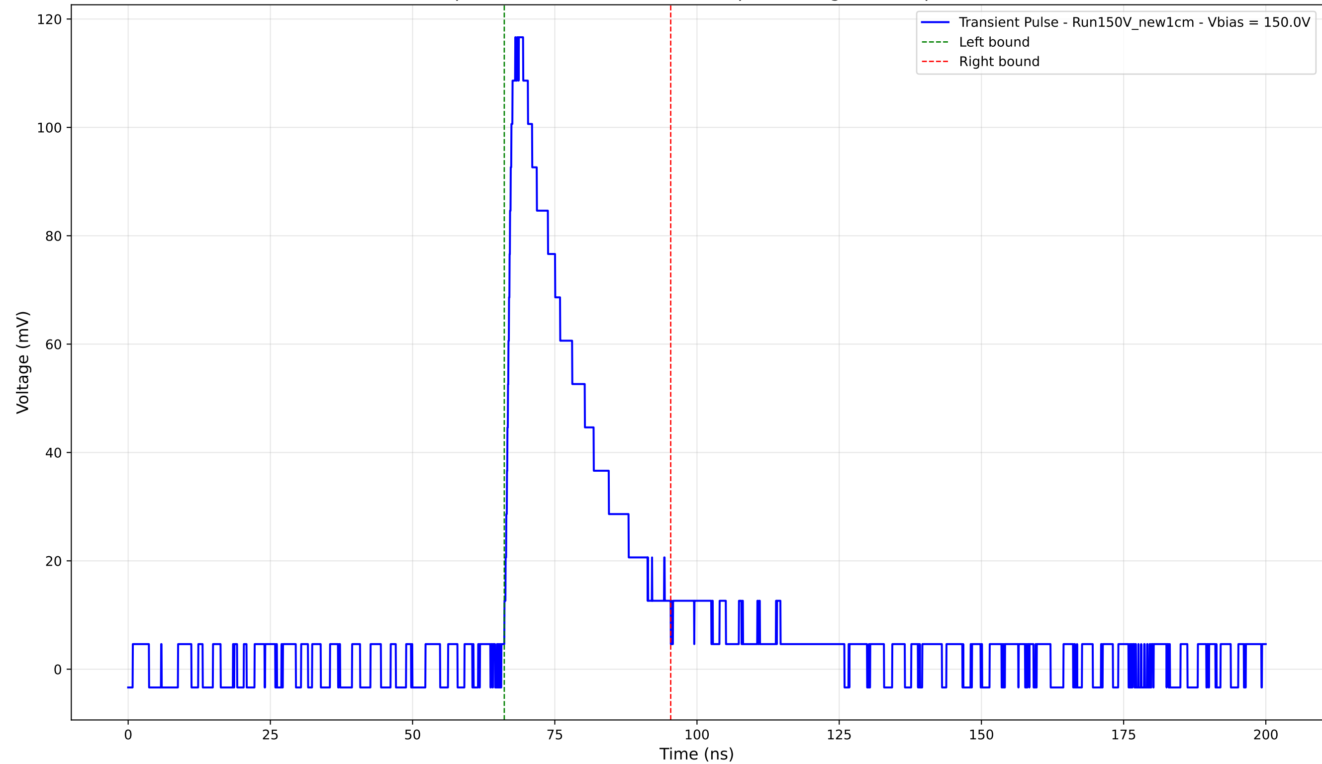
Transient Pulse - Sample: New1cm - Position: 905.0 \mu\text{m} - Charge: 29.84 pC - Rise Time: 1.42 ns
