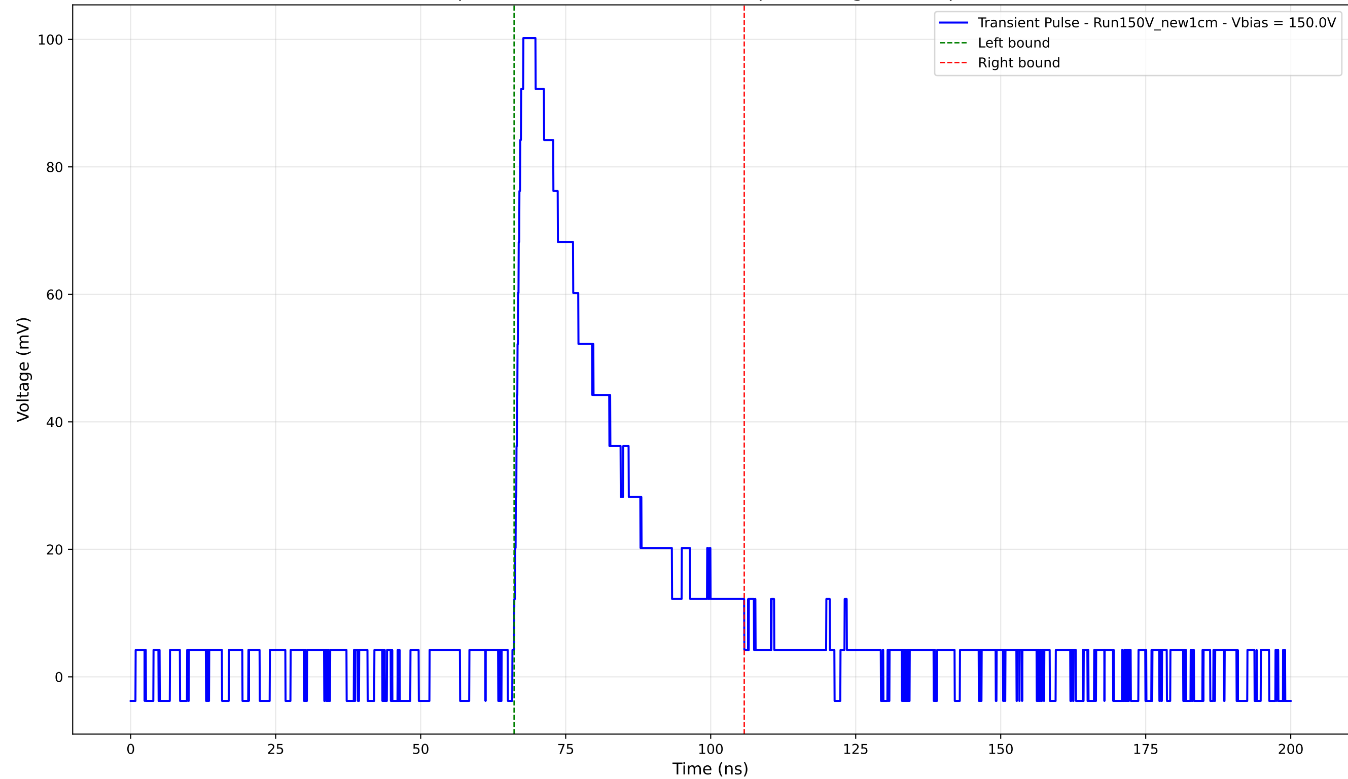
Transient Pulse - Sample: New1cm - Position: 1650.0 \mu\text{m} - Charge: 31.56 pC - Rise Time: 1.19 ns
