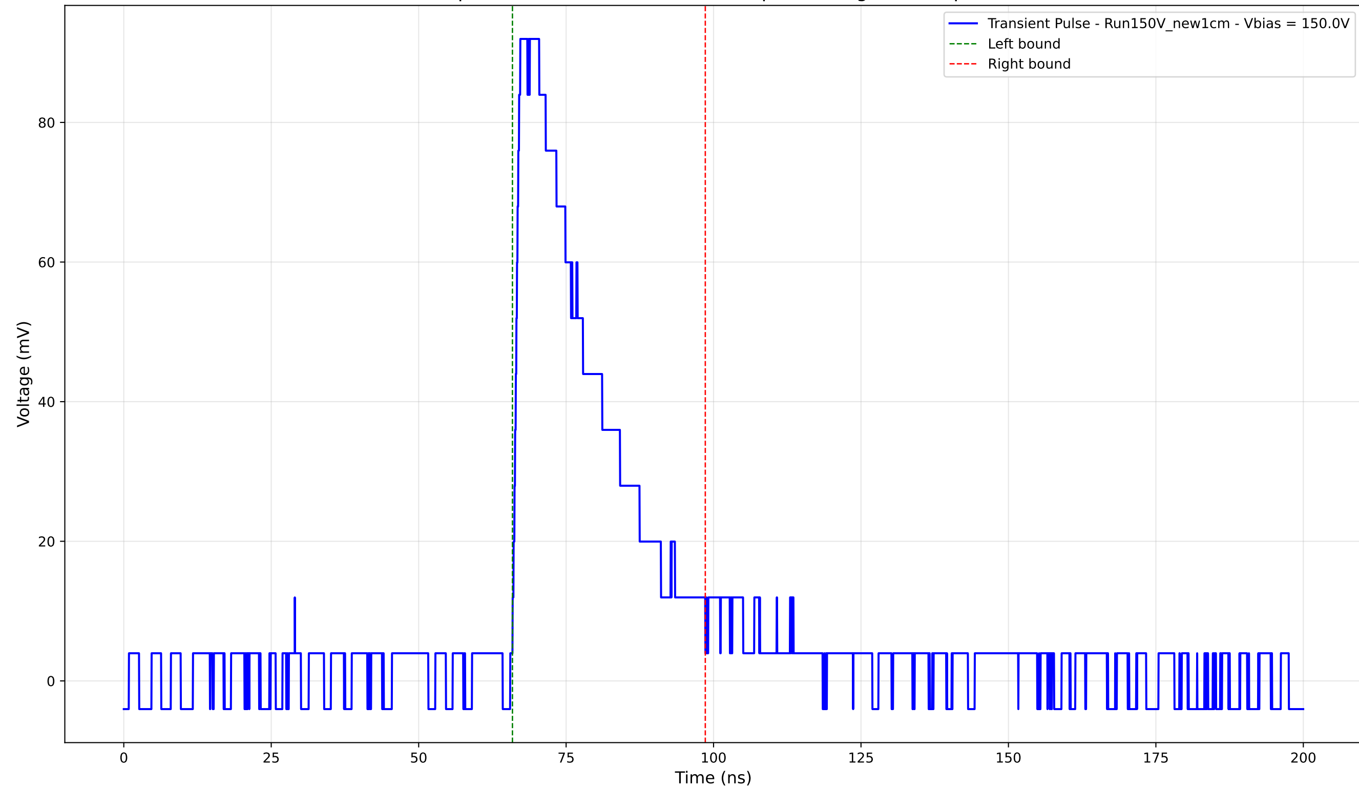
Transient Pulse - Sample: New1cm - Position: 1790.0 \mu\text{m} - Charge: 27.38 pC - Rise Time: 1.11 ns
