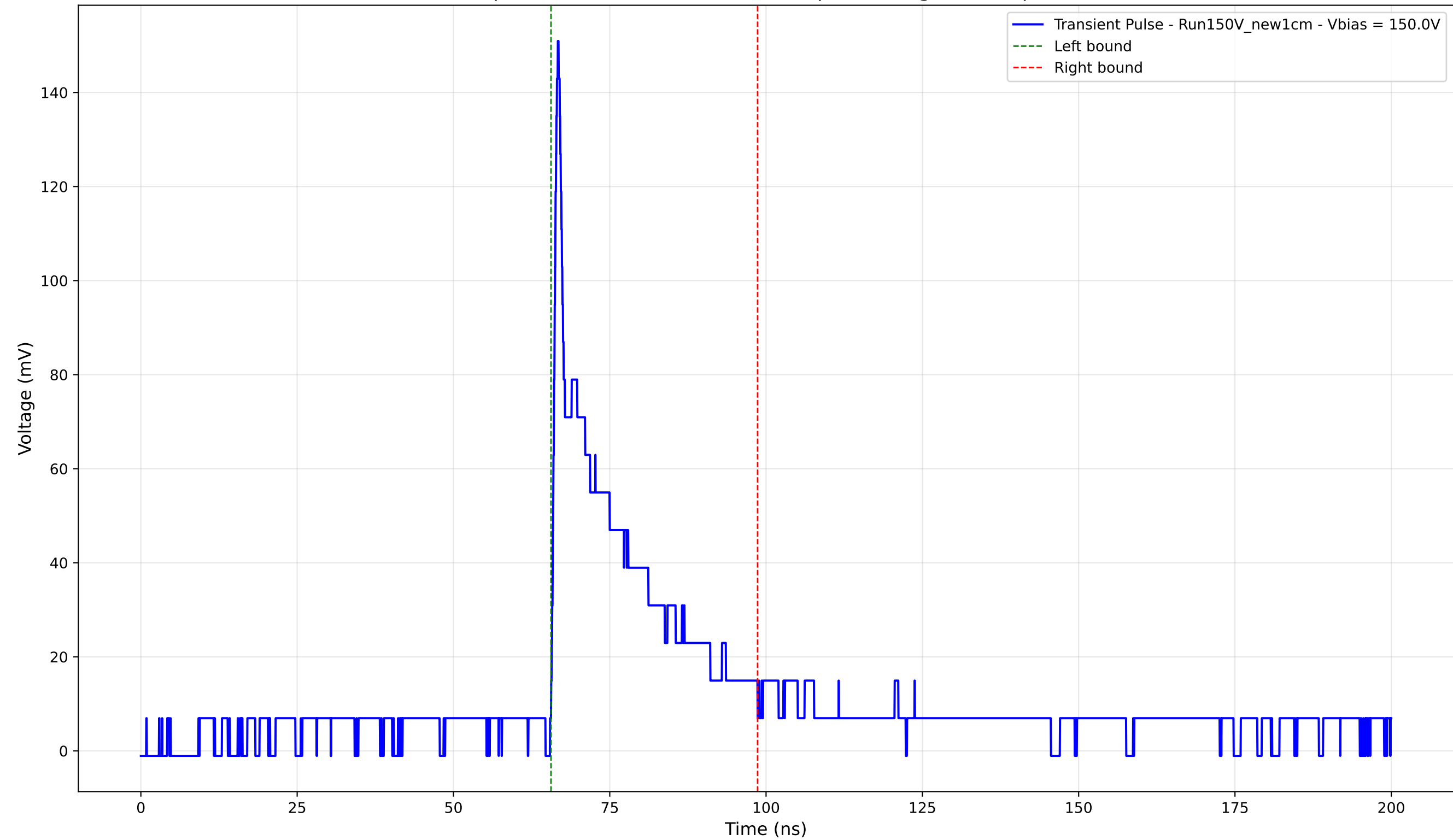
Transient Pulse - Sample: New1cm - Position: 2620.0 \mu\text{m} - Charge: 26.41 pC - Rise Time: 0.86 ns
