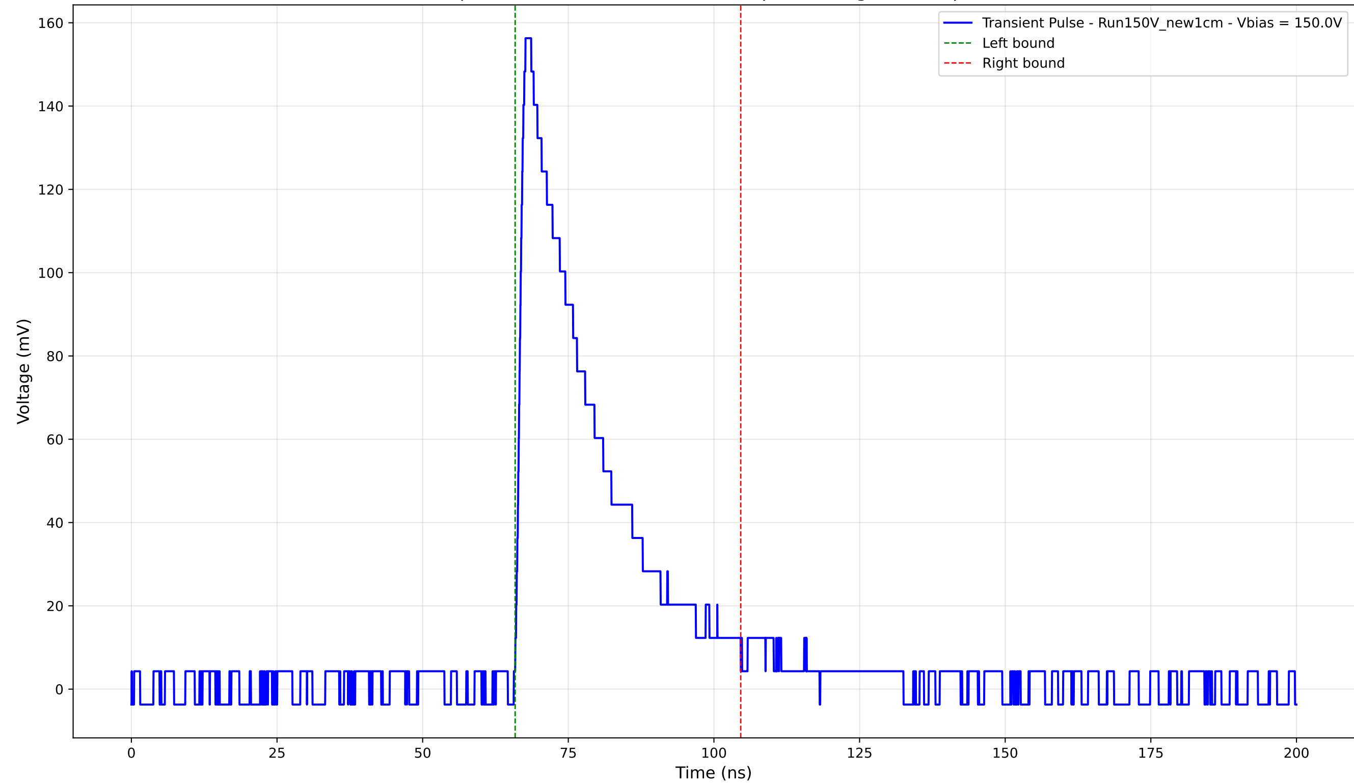
Transient Pulse - Sample: New1cm - Position: 4265.0 \mu\text{m} - Charge: 42.05 pC - Rise Time: 1.41 ns
