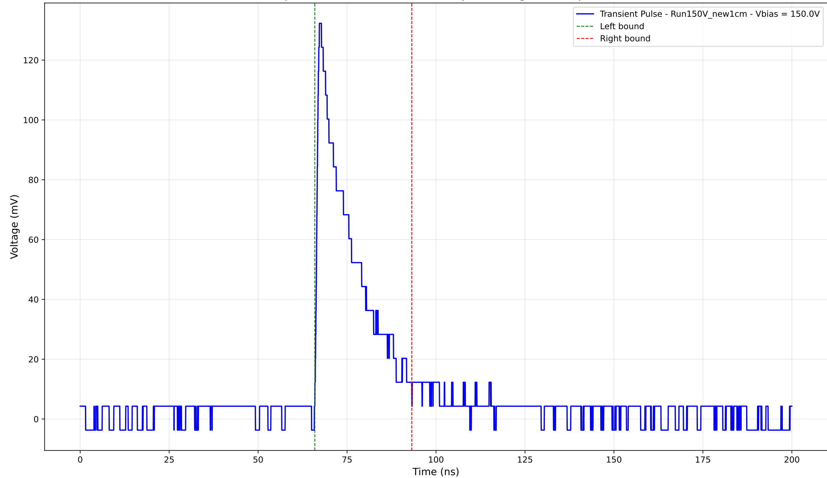
Transient Pulse - Sample: New1cm - Position: 390.0 \mu\text{m} - Charge: 28.23 pC - Rise Time: 0.98 ns
