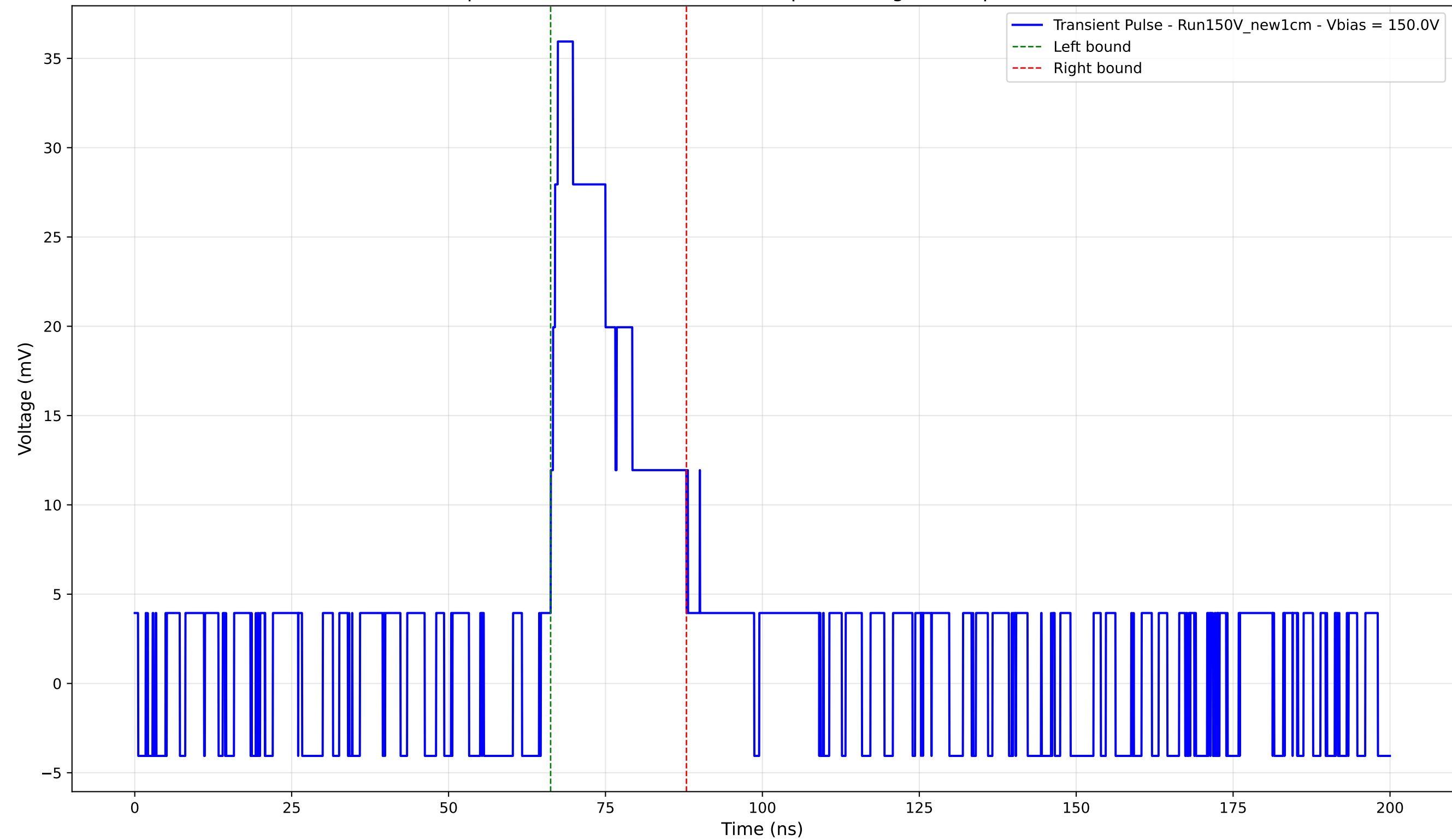
Transient Pulse - Sample: New1cm - Position: 4095.0 \mu\text{m} - Charge: 8.83 pC - Rise Time: 0.00 ns (N/A)
