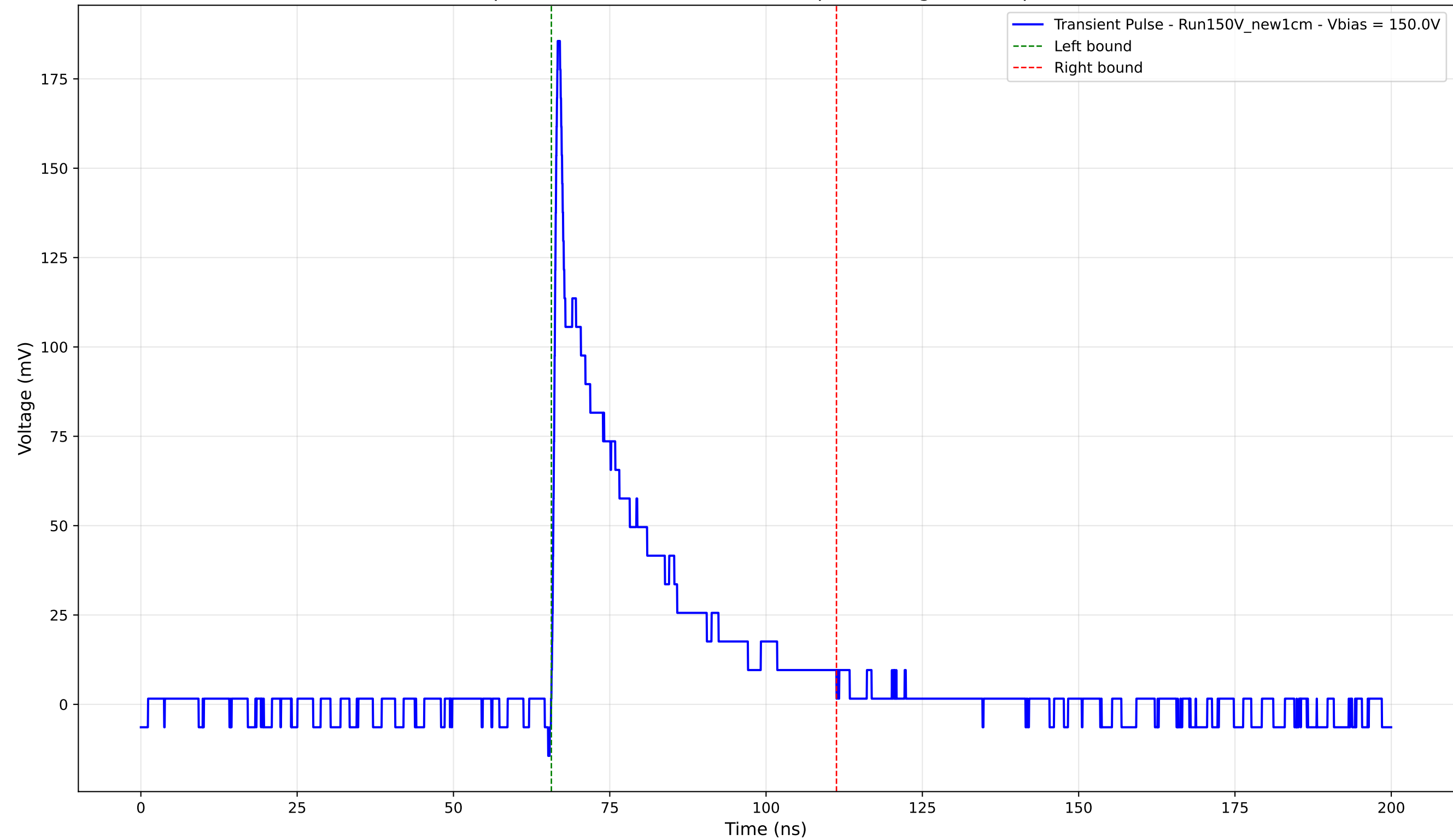
Transient Pulse - Sample: New1cm - Position: 2750.0 \mu\text{m} - Charge: 37.44 pC - Rise Time: 0.74 ns
