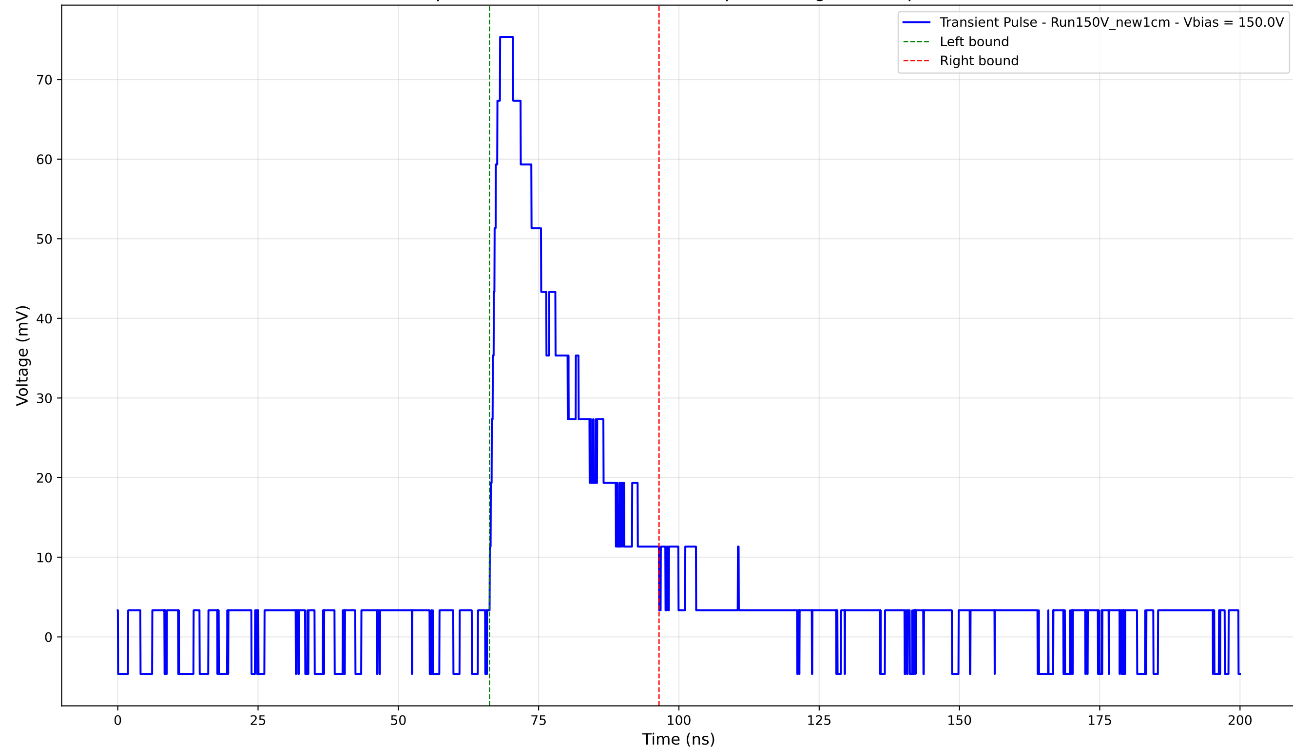
Transient Pulse - Sample: New1cm - Position: 1475.0 \mu\text{m} - Charge: 21.00 pC - Rise Time: 1.85 ns
