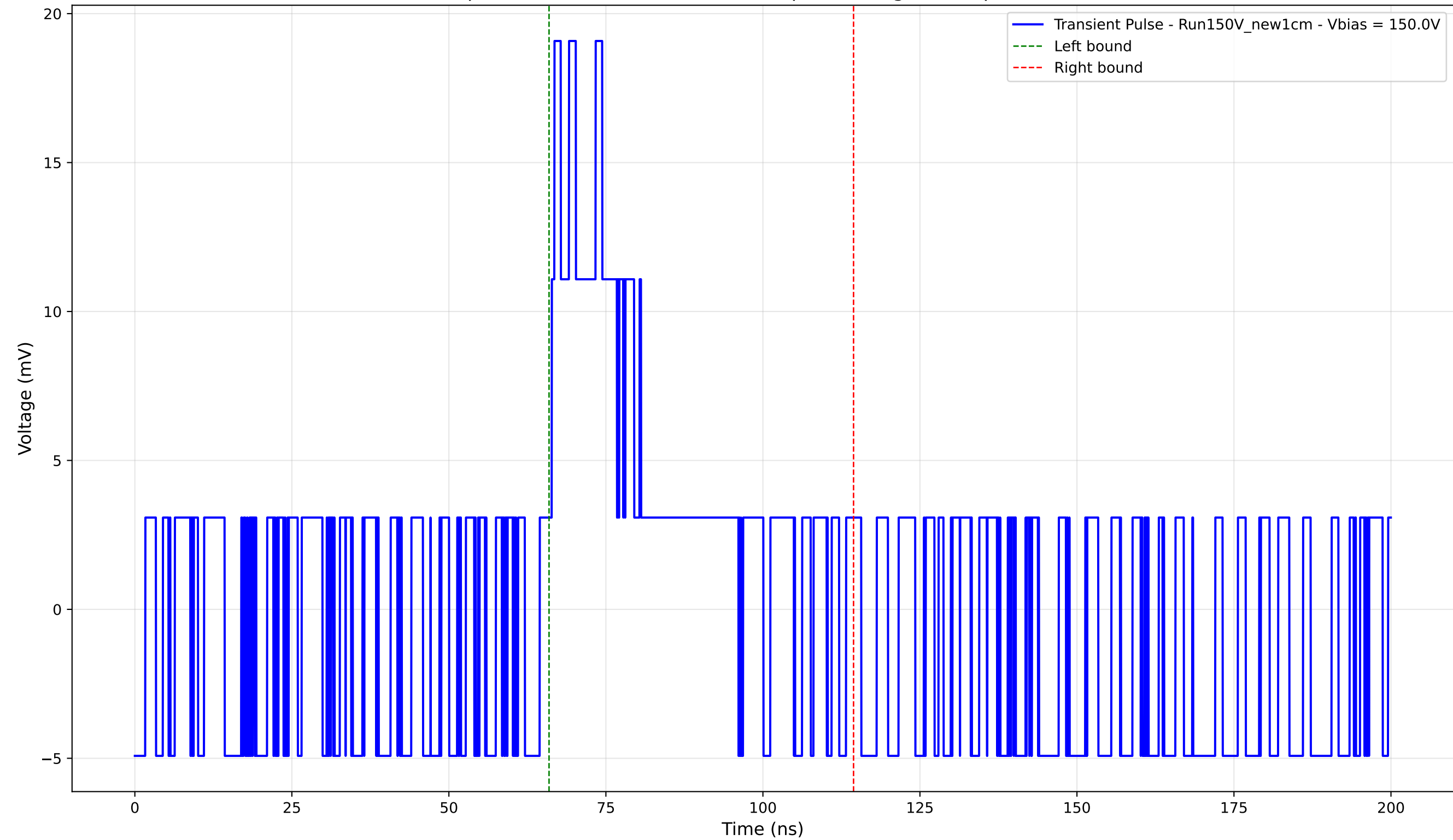
Transient Pulse - Sample: New1cm - Position: 2025.0 \mu\text{m} - Charge: 4.78 pC - Rise Time: 0.00 ns (N/A)
