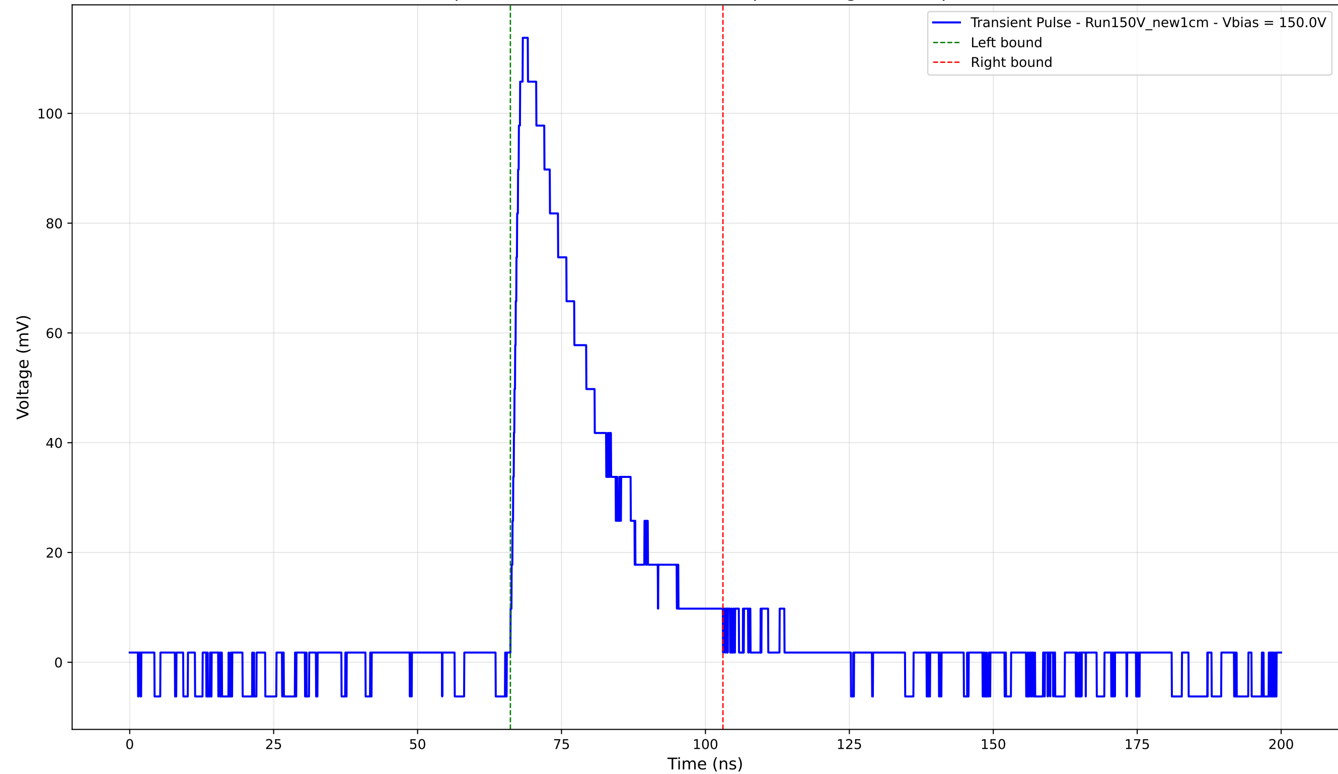
Transient Pulse - Sample: New1cm - Position: 1300.0 \mu\text{m} - Charge: 31.65 pC - Rise Time: 1.50 ns
