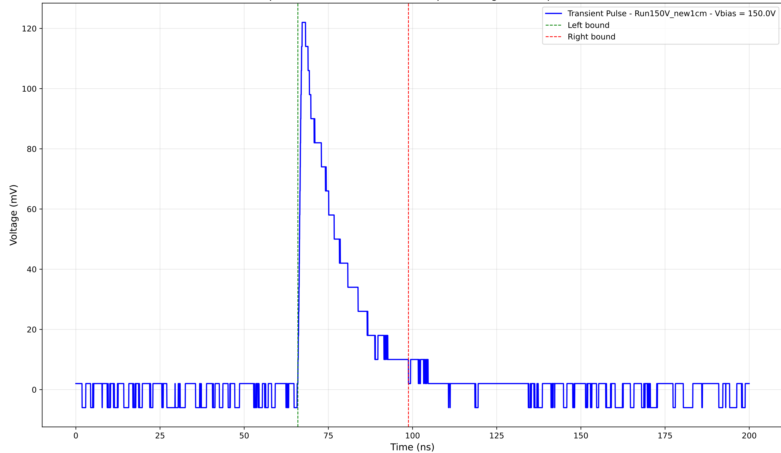
Transient Pulse - Sample: New1cm - Position: 400.0 \mu\text{m} - Charge: 28.13 pC - Rise Time: 0.99 ns
