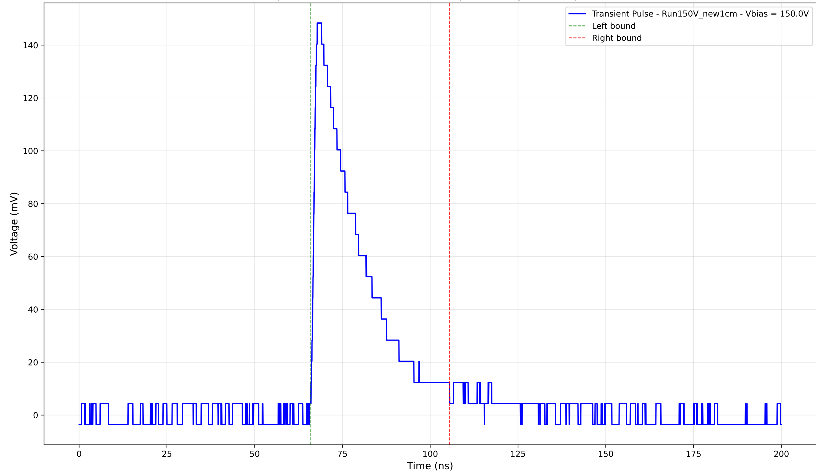
Transient Pulse - Sample: New1cm - Position: 3905.0 \mu\text{m} - Charge: 41.72 pC - Rise Time: 1.39 ns
