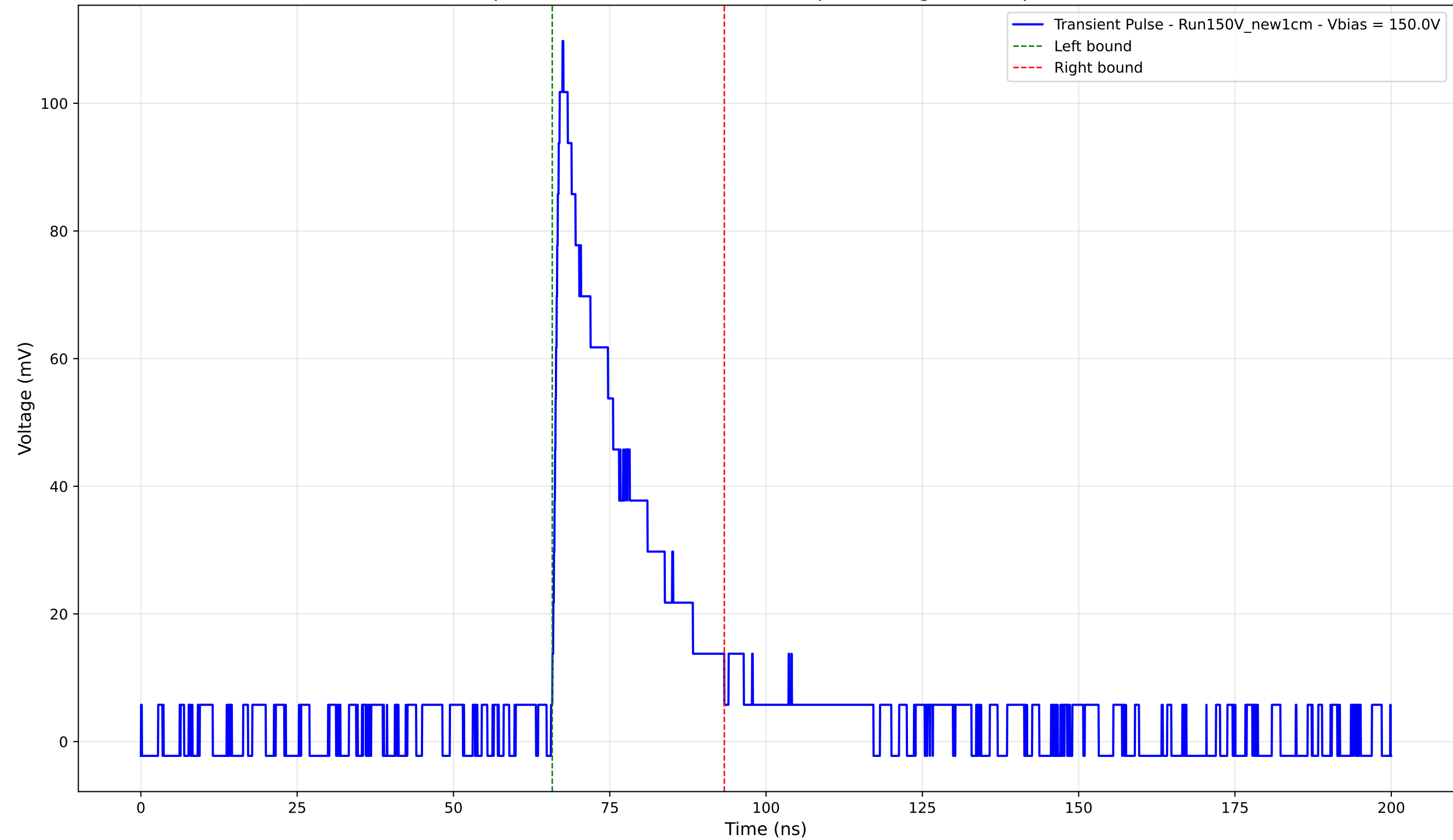
Transient Pulse - Sample: New1cm - Position: 4640.0 \mu\text{m} - Charge: 23.46 pC - Rise Time: 1.17 ns
