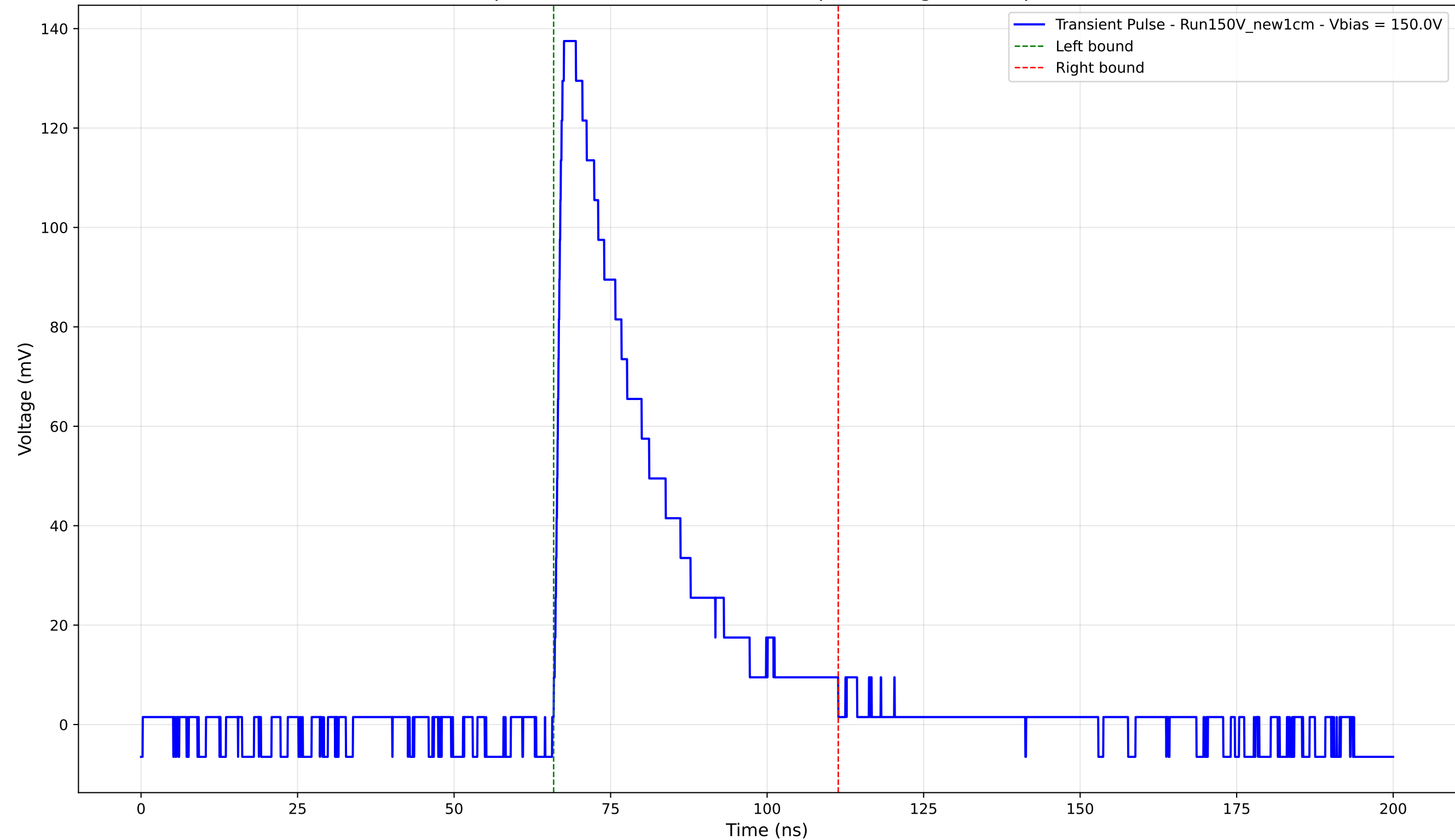
Transient Pulse - Sample: New1cm - Position: 3385.0 \mu\text{m} - Charge: 41.20 pC - Rise Time: 1.23 ns
