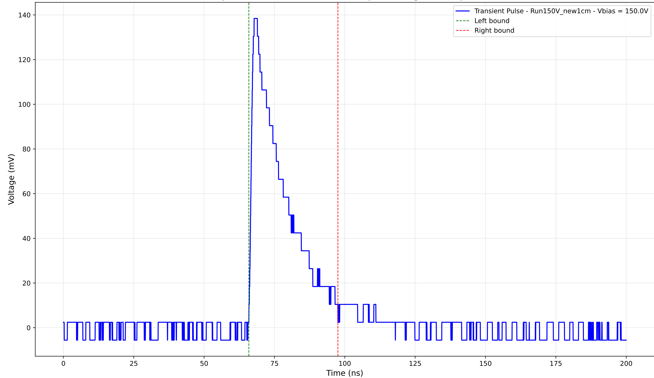
Transient Pulse - Sample: New1cm - Position: 4220.0 \mu\text{m} - Charge: 35.14 pC - Rise Time: 1.41 ns
