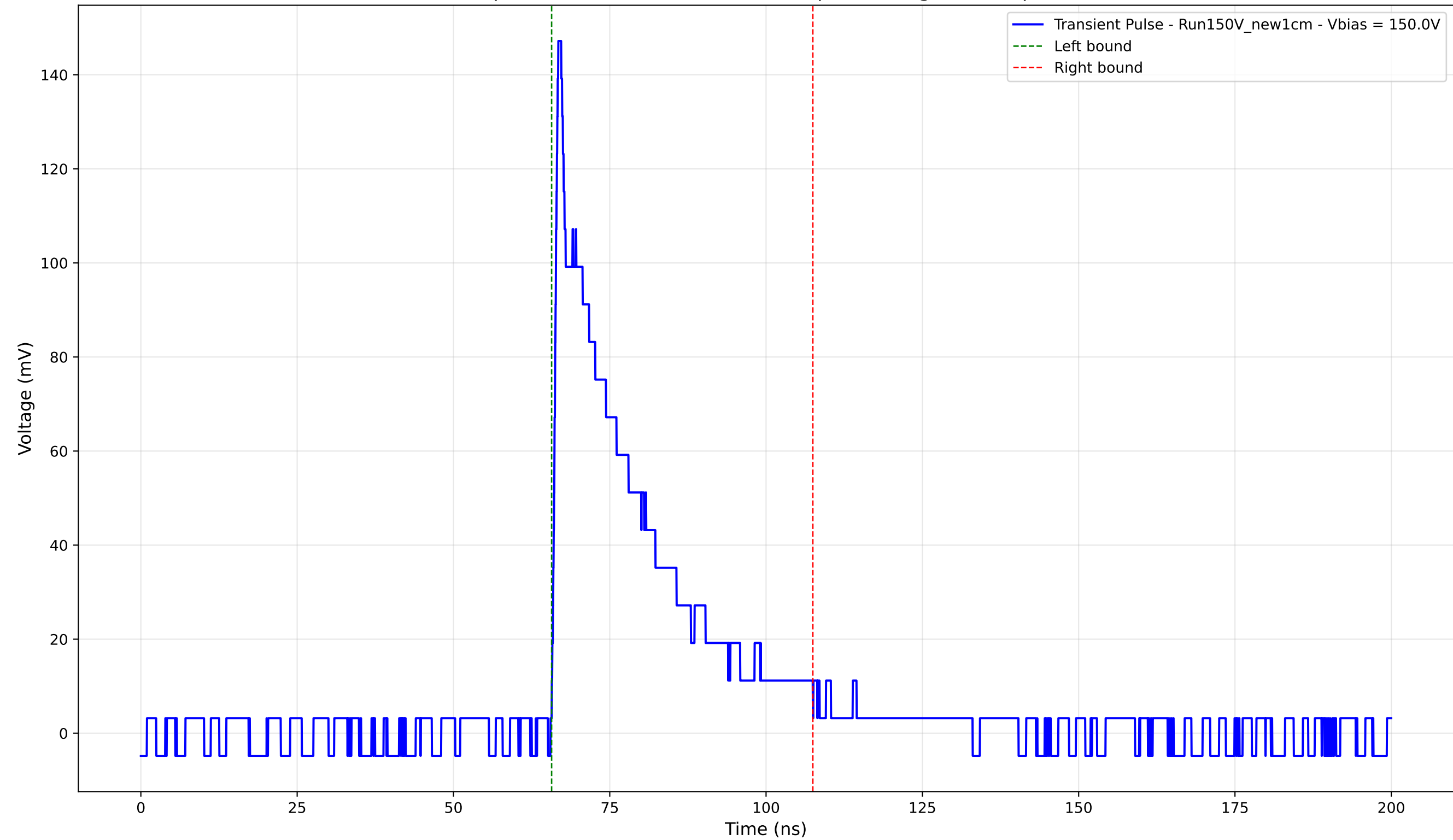
Transient Pulse - Sample: New1cm - Position: 2220.0 \mu\text{m} - Charge: 34.51 pC - Rise Time: 0.87 ns
