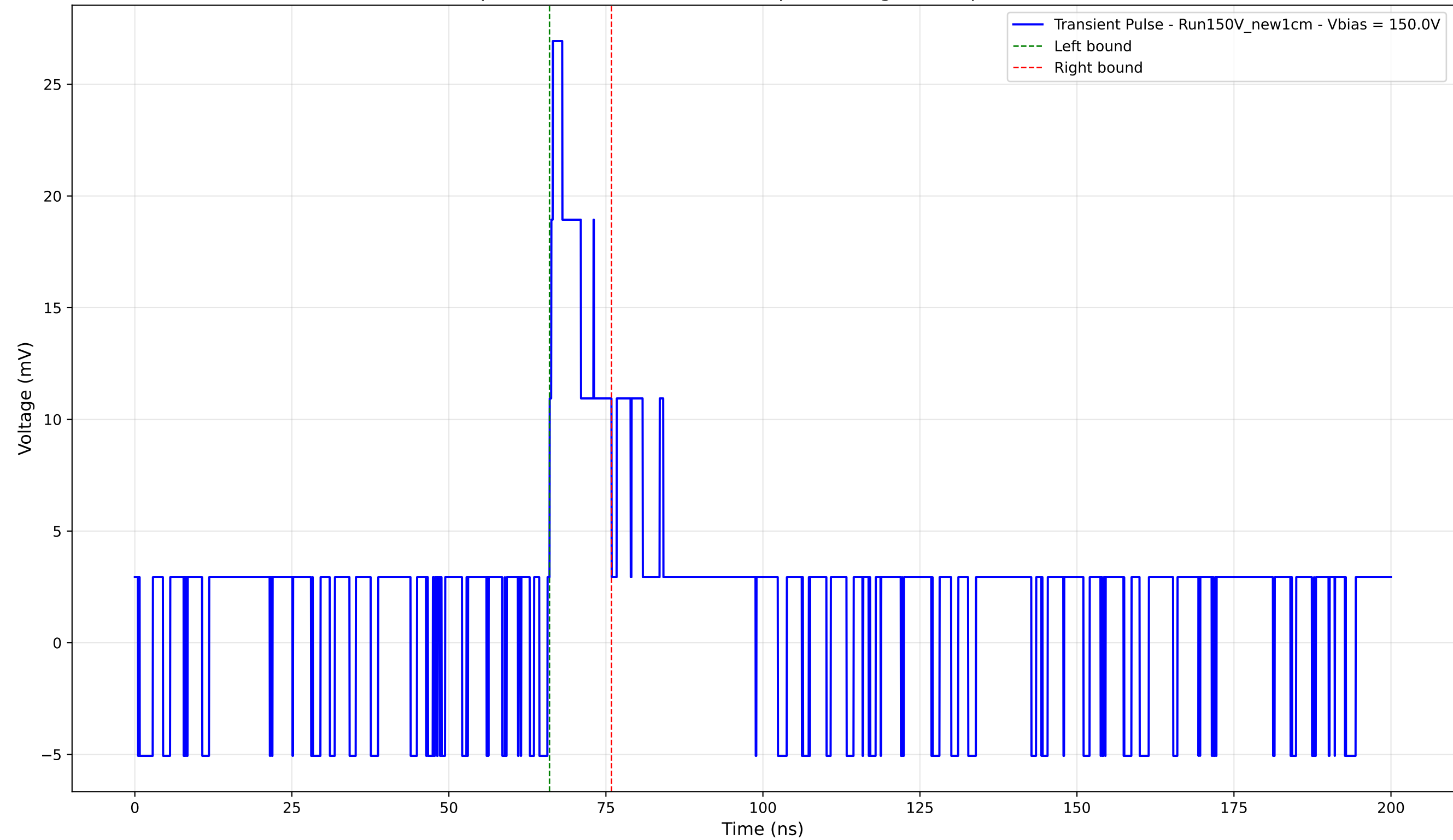
Transient Pulse - Sample: New1cm - Position: 50.0 \mu\text{m} - Charge: 3.17 pC - Rise Time: 0.00 ns (N/A)
