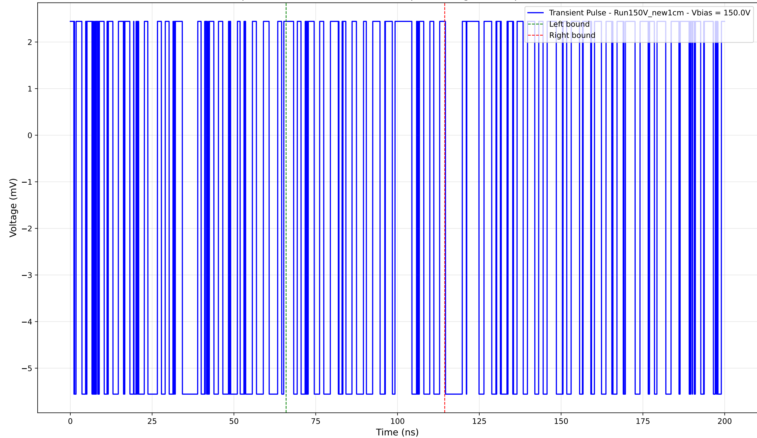
Transient Pulse - Sample: New1cm - Position: 5000.0 \mu\text{m} - Charge: -1.08 pC - Rise Time: 0.00 ns (N/A)
