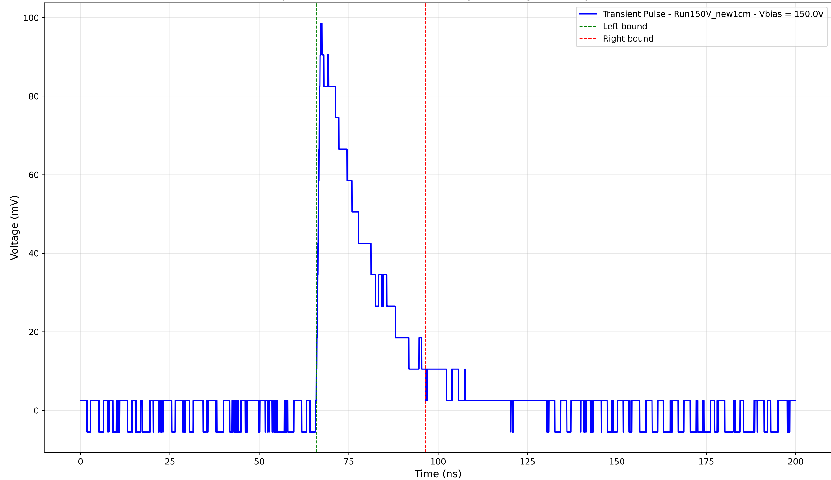
Transient Pulse - Sample: New1cm - Position: 1925.0 \mu\text{m} - Charge: 25.87 pC - Rise Time: 1.02 ns
