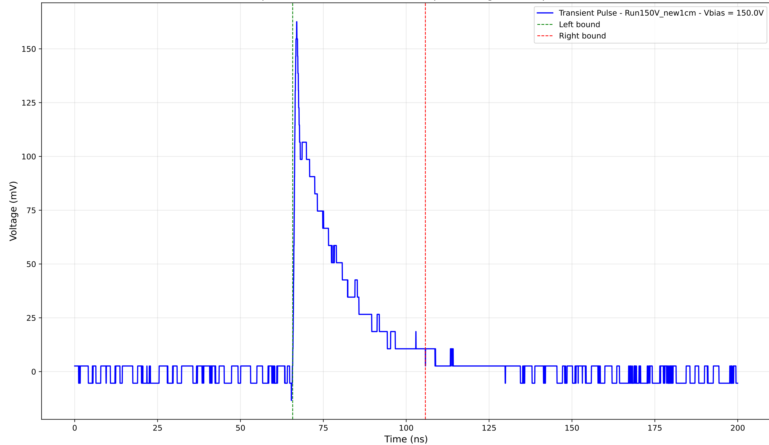
Transient Pulse - Sample: New1cm - Position: 2235.0 \mu\text{m} - Charge: 34.57 pC - Rise Time: 0.81 ns
