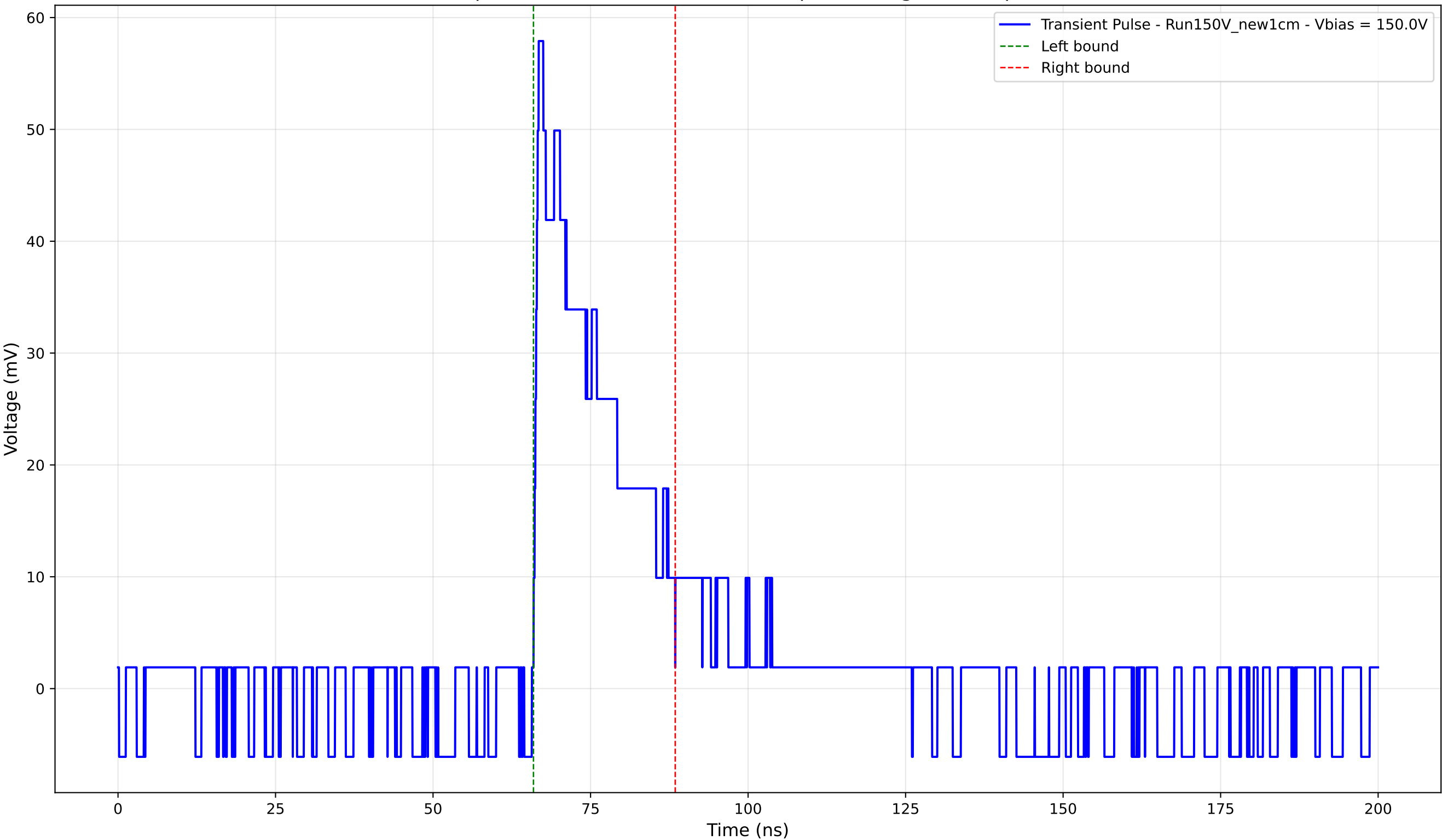
Transient Pulse - Sample: New1cm - Position: 3020.0 \mu\text{m} - Charge: 12.34 pC - Rise Time: 0.81 ns
