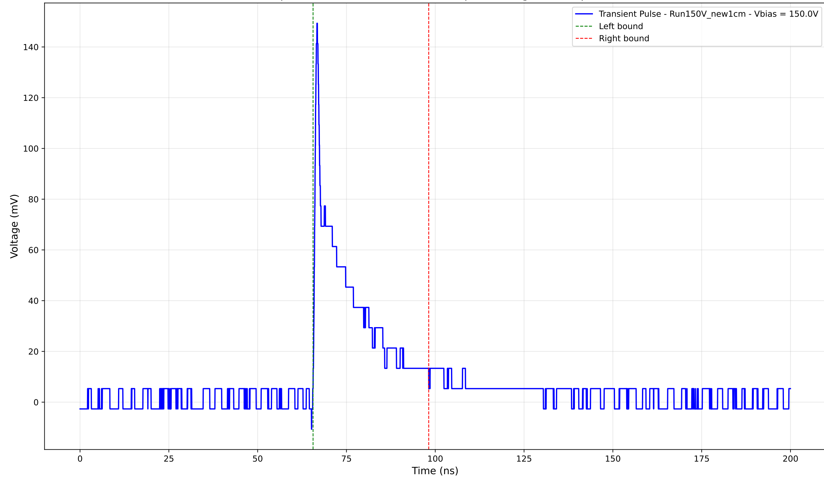
Transient Pulse - Sample: New1cm - Position: 2480.0 \mu\text{m} - Charge: 24.47 pC - Rise Time: 0.82 ns
