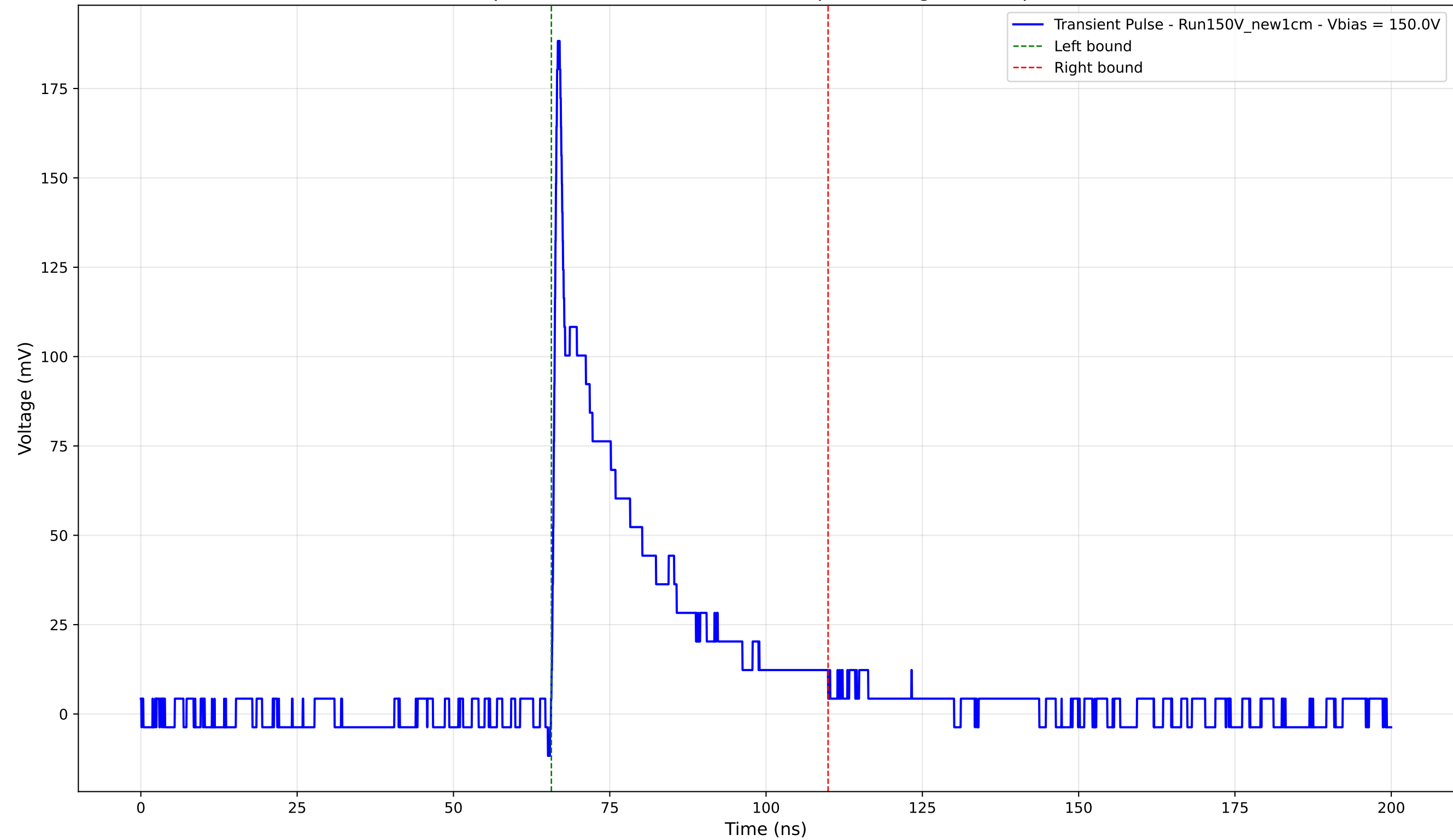
Transient Pulse - Sample: New1cm - Position: 2380.0 \mu\text{m} - Charge: 37.66 pC - Rise Time: 0.78 ns
