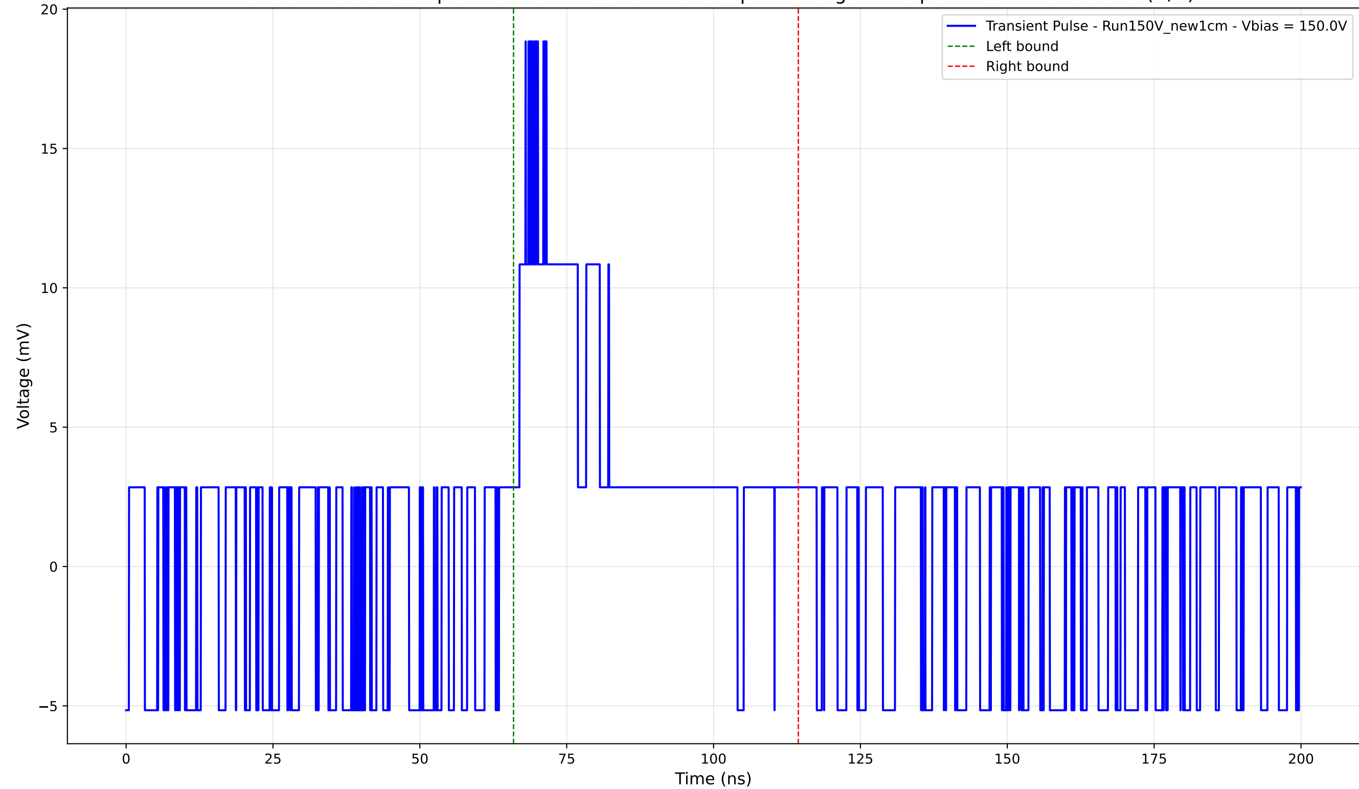
Transient Pulse - Sample: New1cm - Position: 1045.0 \mu\text{m} - Charge: 4.78 pC - Rise Time: 0.00 ns (N/A)
