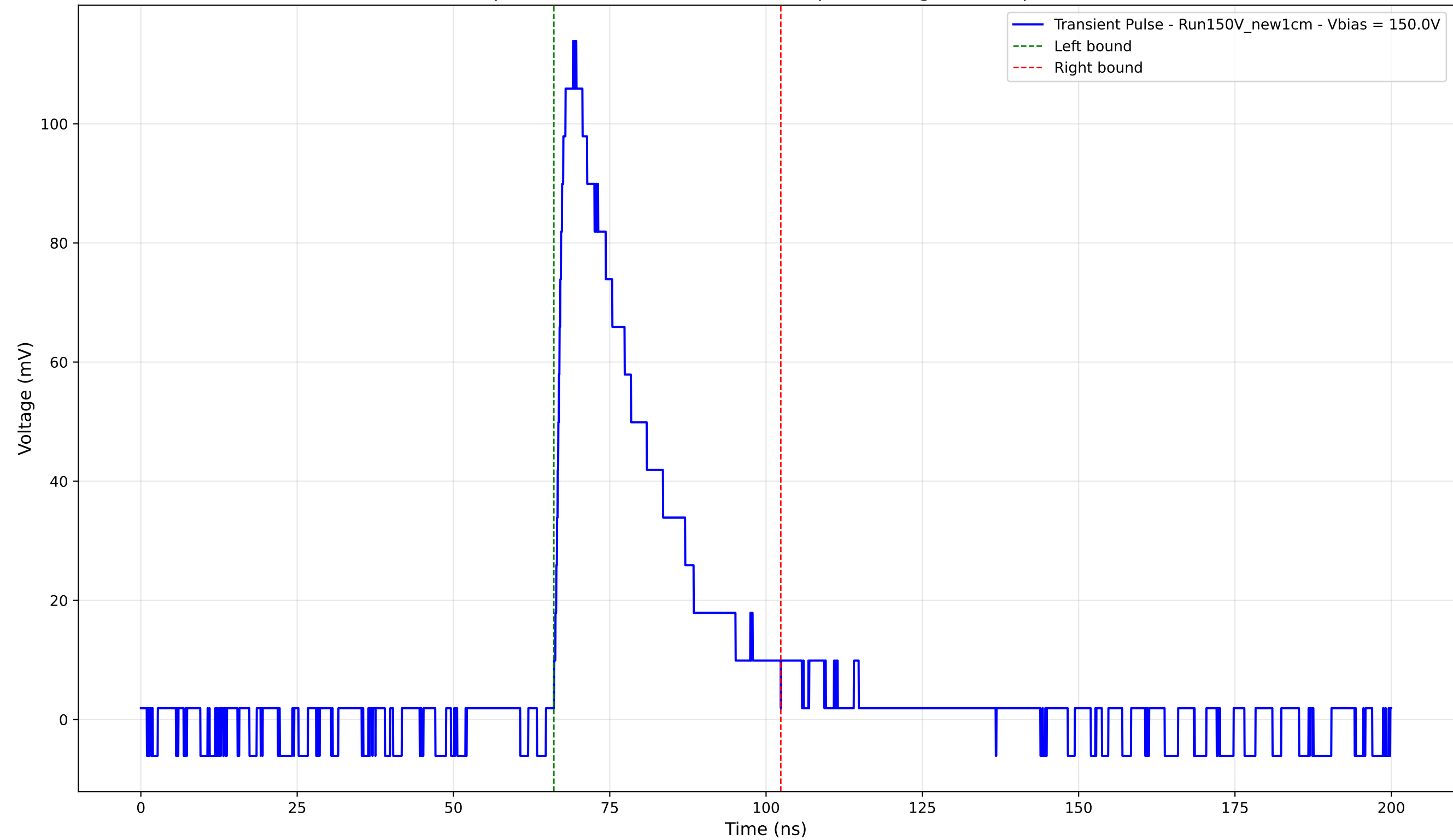
Transient Pulse - Sample: New1cm - Position: 1370.0 \mu\text{m} - Charge: 31.54 pC - Rise Time: 1.64 ns
