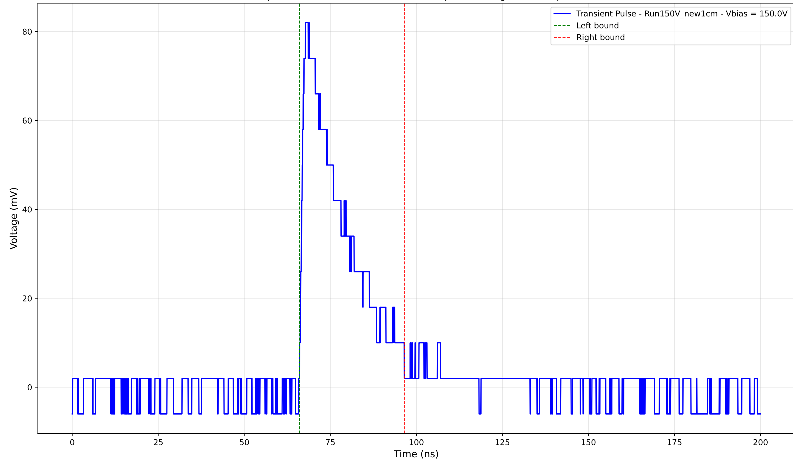
Transient Pulse - Sample: New1cm - Position: 3505.0 \mu\text{m} - Charge: 21.42 pC - Rise Time: 1.28 ns
