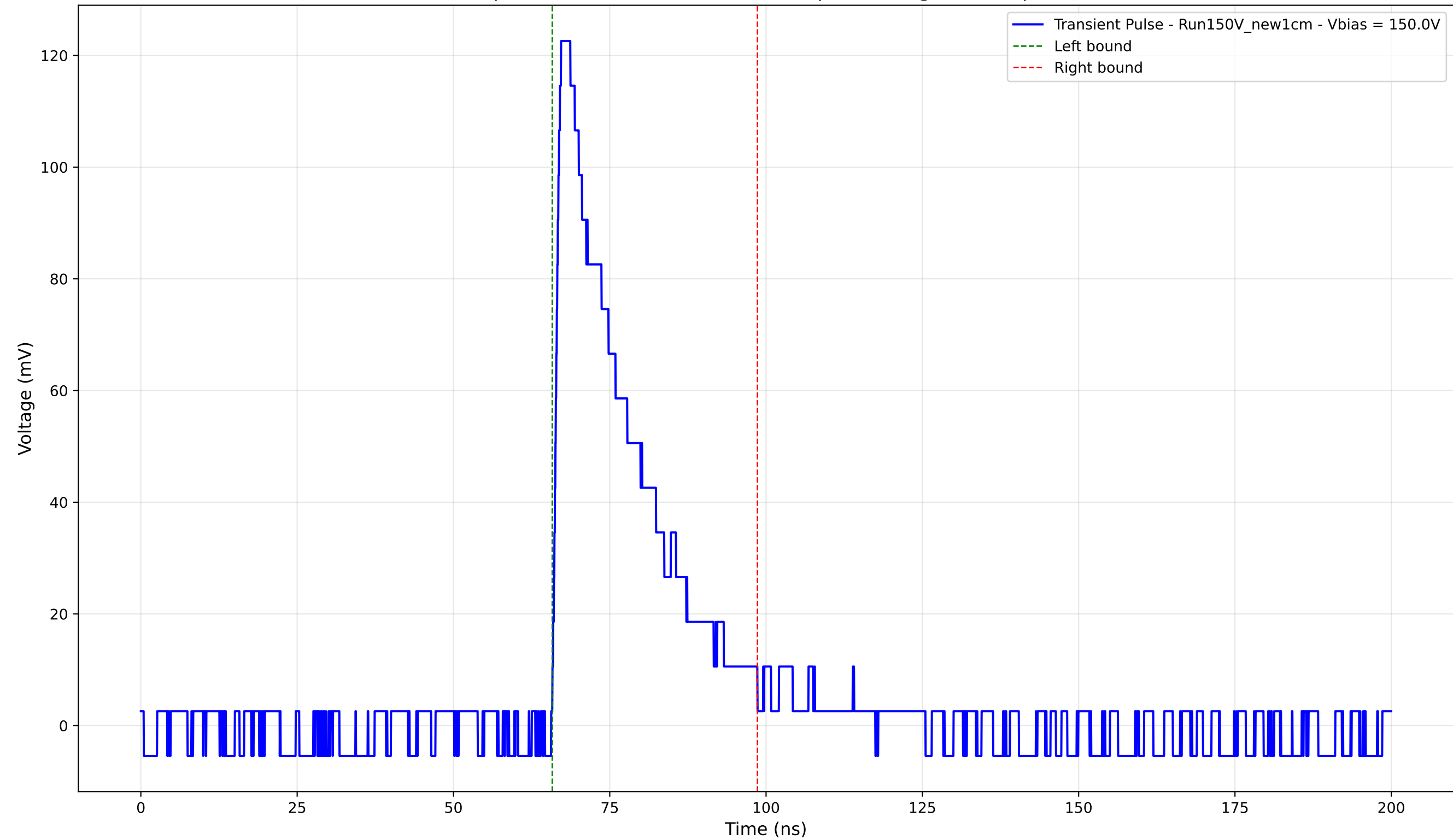
Transient Pulse - Sample: New1cm - Position: 4490.0 \mu\text{m} - Charge: 30.65 pC - Rise Time: 1.10 ns
