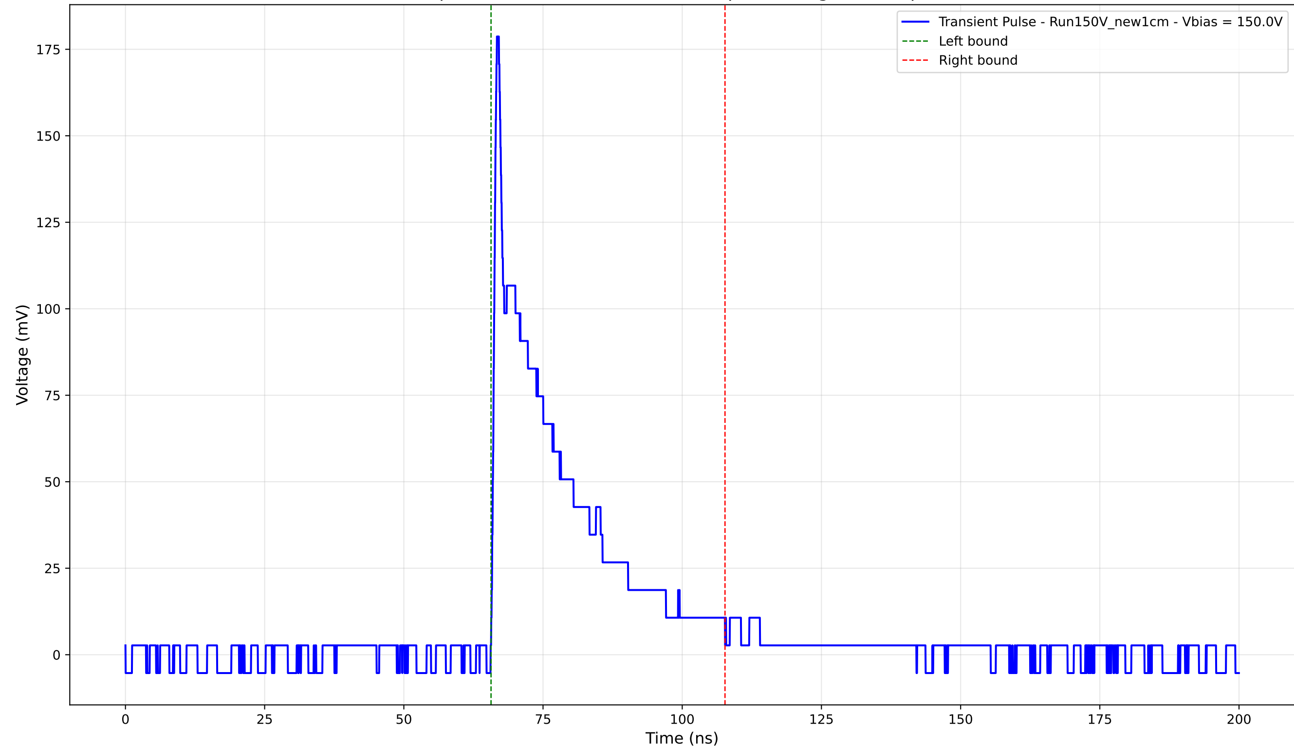
Transient Pulse - Sample: New1cm - Position: 2325.0 \mu\text{m} - Charge: 36.25 pC - Rise Time: 0.80 ns
