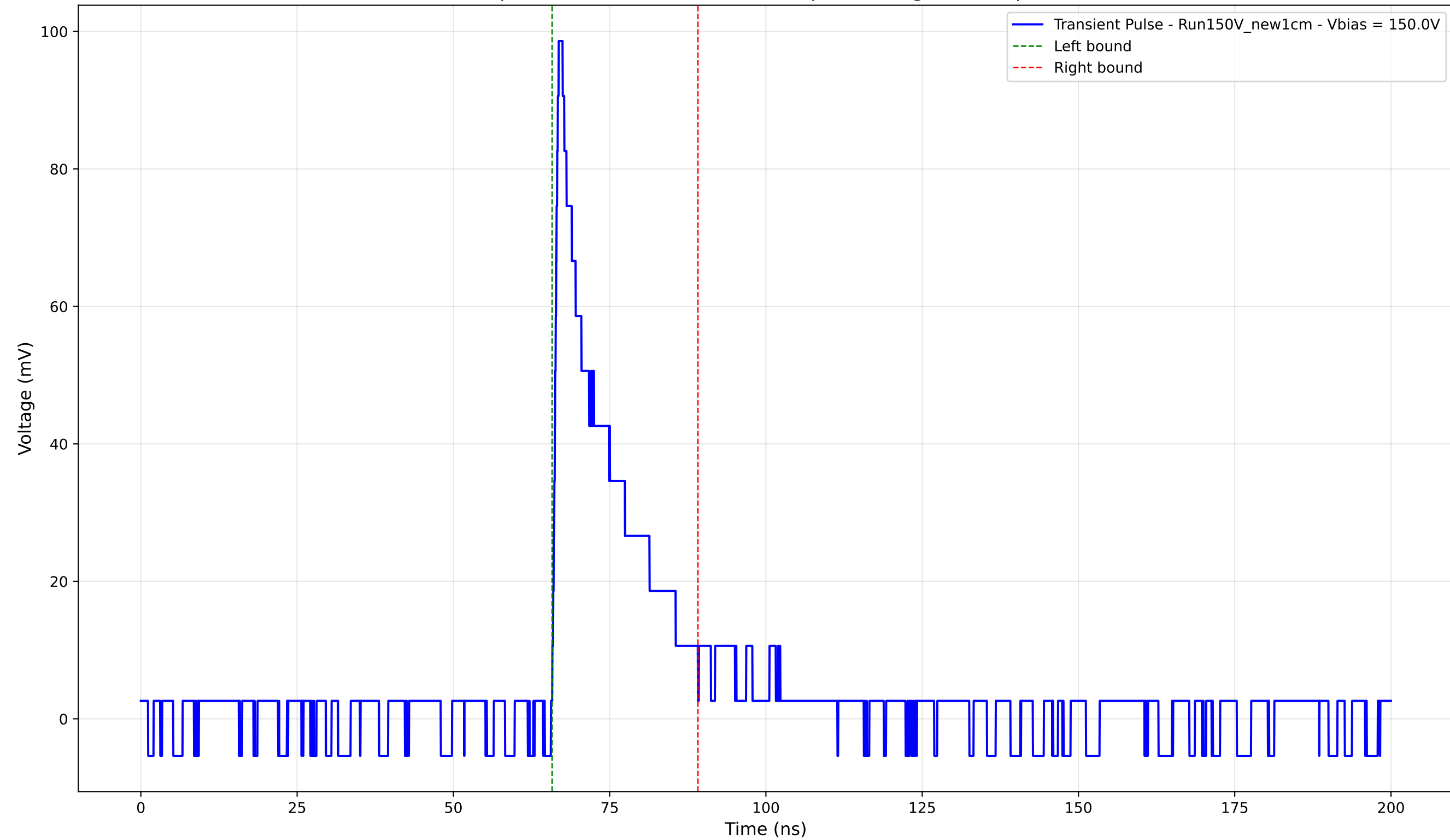
Transient Pulse - Sample: New1cm - Position: 110.0 \mu\text{m} - Charge: 16.73 pC - Rise Time: 0.88 ns
