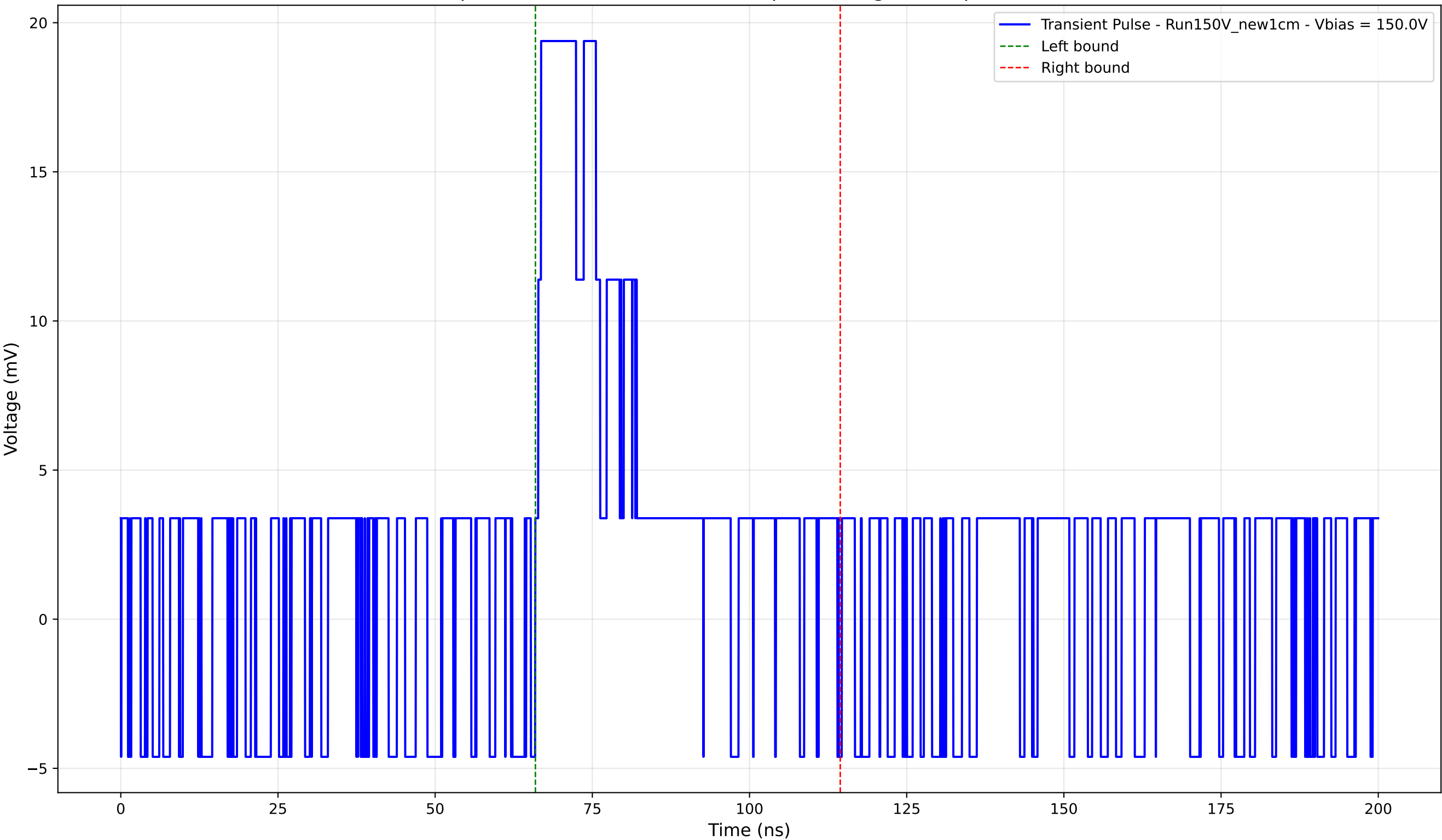
Transient Pulse - Sample: New1cm - Position: 545.0 \mu\text{m} - Charge: 6.29 pC - Rise Time: 0.00 ns (N/A)
