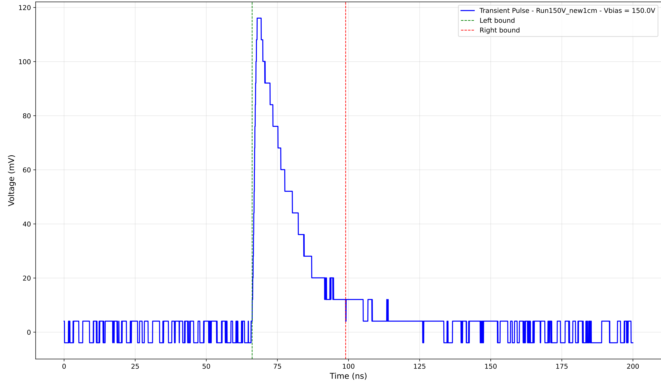
Transient Pulse - Sample: New1cm - Position: 850.0 \mu\text{m} - Charge: 30.39 pC - Rise Time: 1.48 ns
