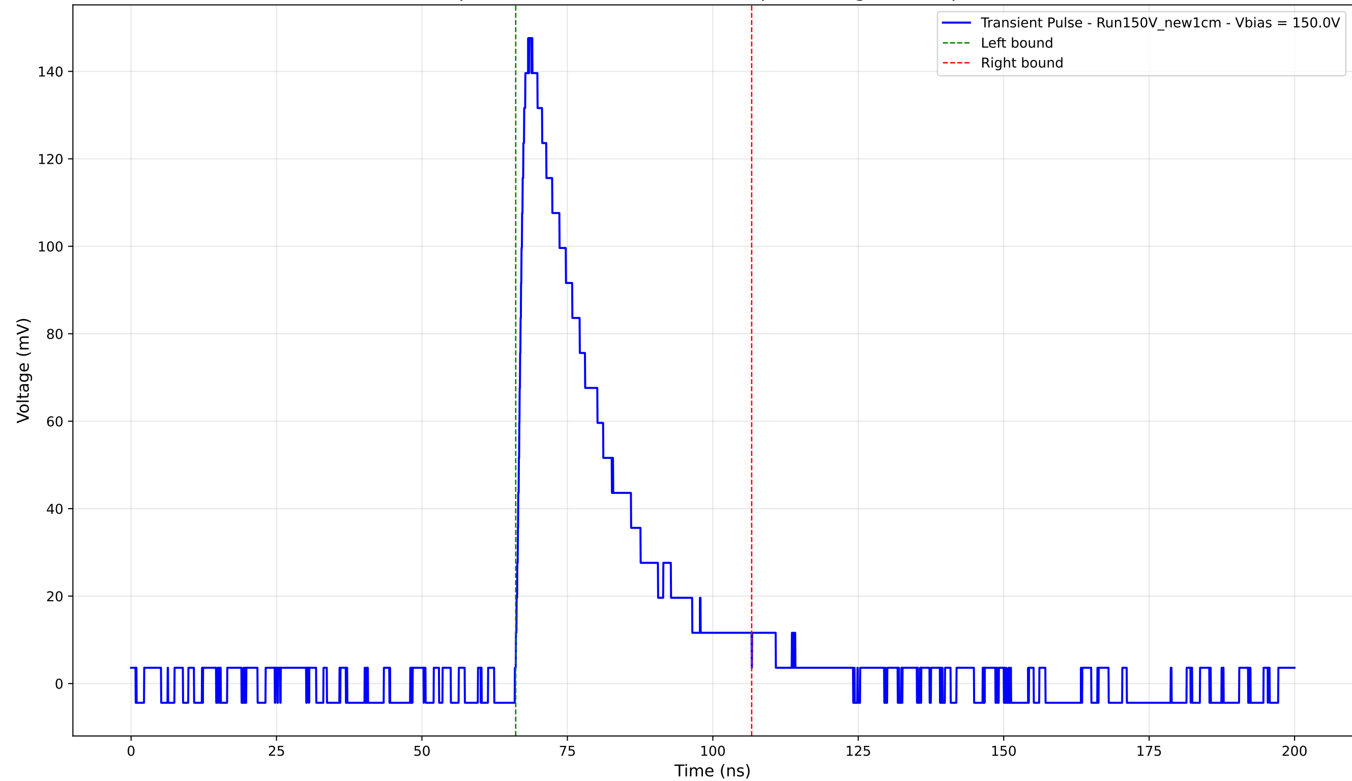
Transient Pulse - Sample: New1cm - Position: 3865.0 \mu\text{m} - Charge: 41.29 pC - Rise Time: 1.51 ns
