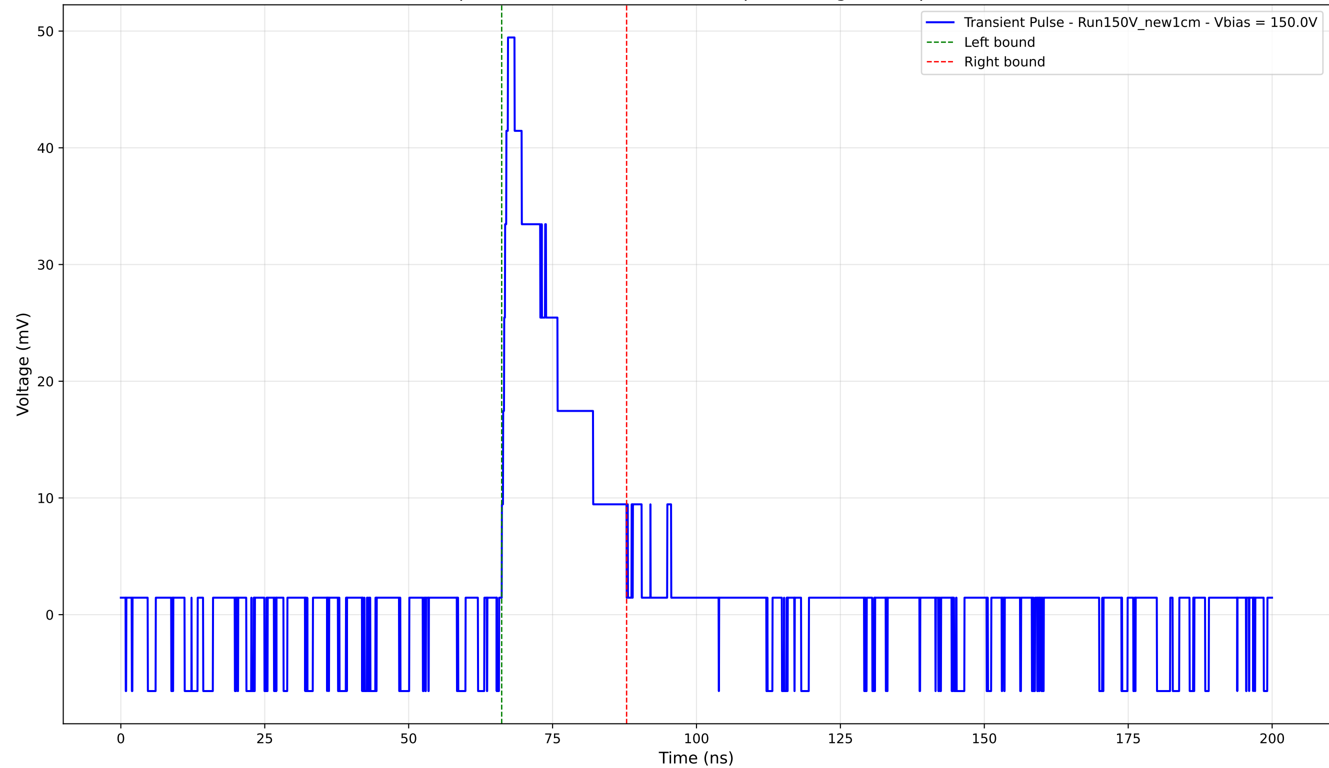
Transient Pulse - Sample: New1cm - Position: 485.0 \mu\text{m} - Charge: 9.72 pC - Rise Time: 1.07 ns
