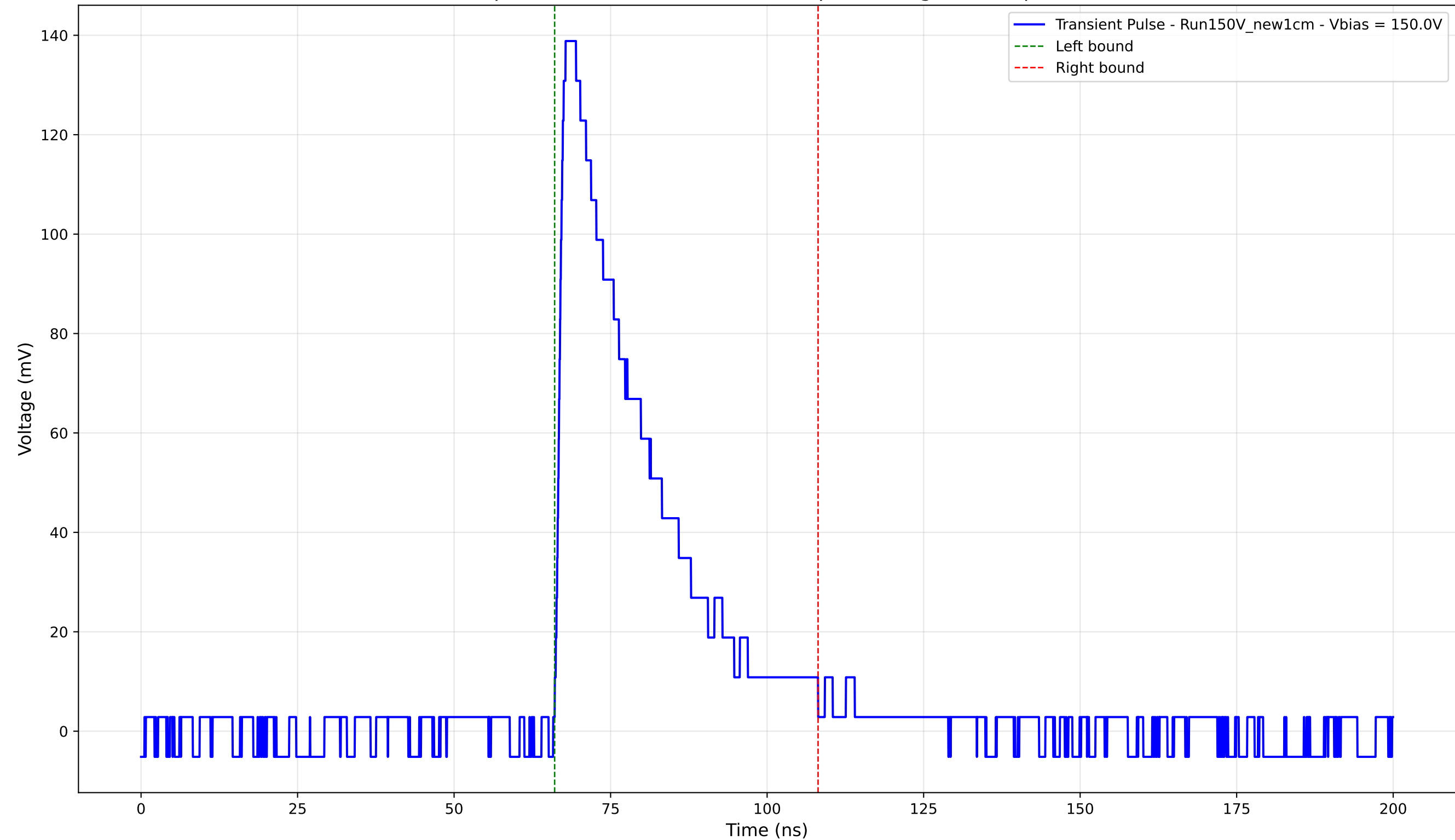
Transient Pulse - Sample: New1cm - Position: 3695.0 \mu\text{m} - Charge: 40.12 pC - Rise Time: 1.27 ns
