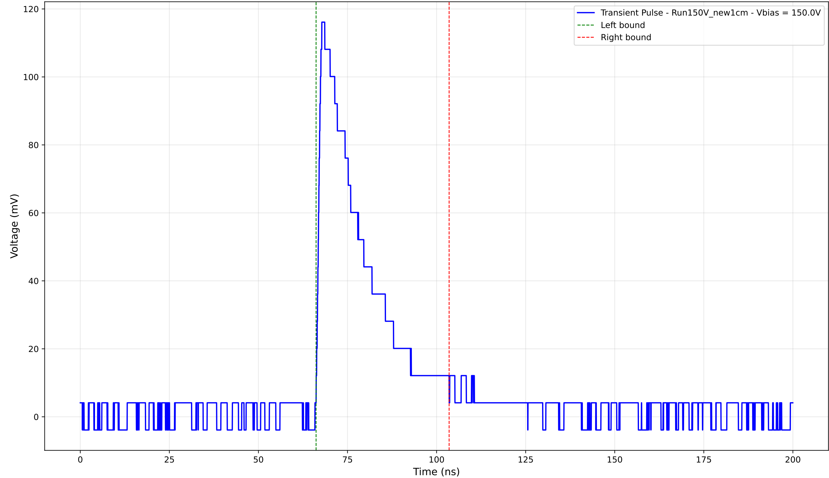
Transient Pulse - Sample: New1cm - Position: 890.0 \mu\text{m} - Charge: 31.87 pC - Rise Time: 1.34 ns
