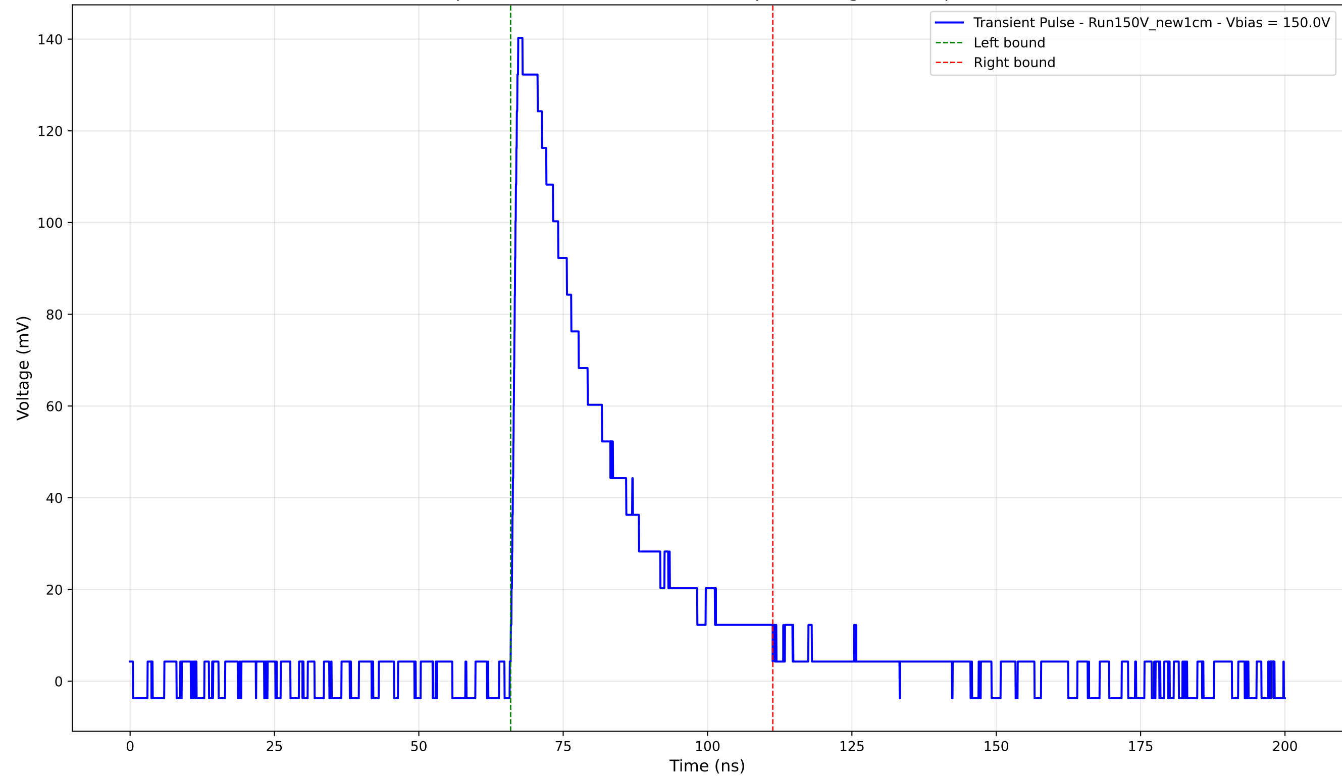
Transient Pulse - Sample: New1cm - Position: 3280.0 \mu\text{m} - Charge: 43.90 pC - Rise Time: 1.04 ns
