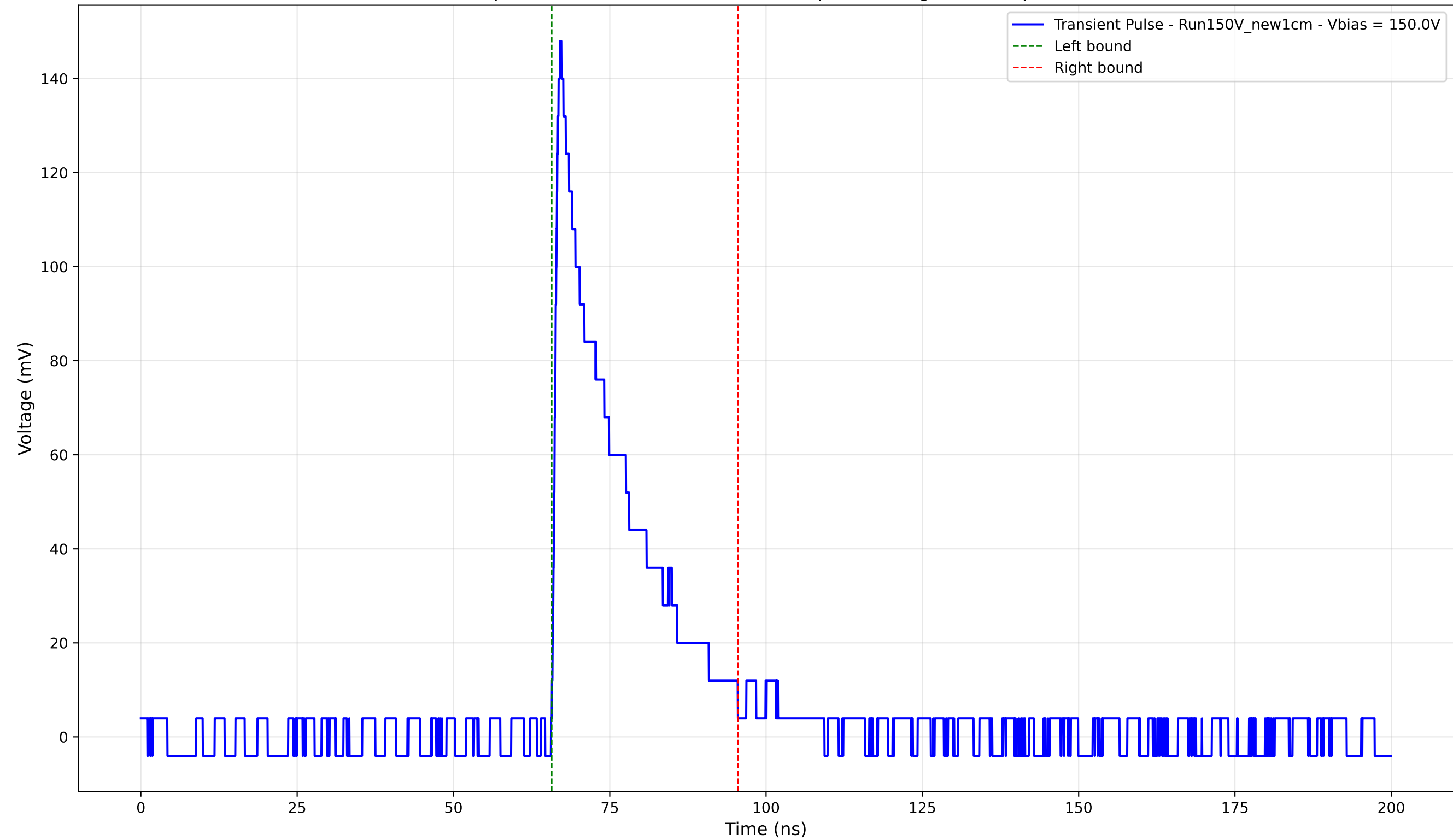
Transient Pulse - Sample: New1cm - Position: 4750.0 \mu\text{m} - Charge: 29.89 pC - Rise Time: 0.97 ns
