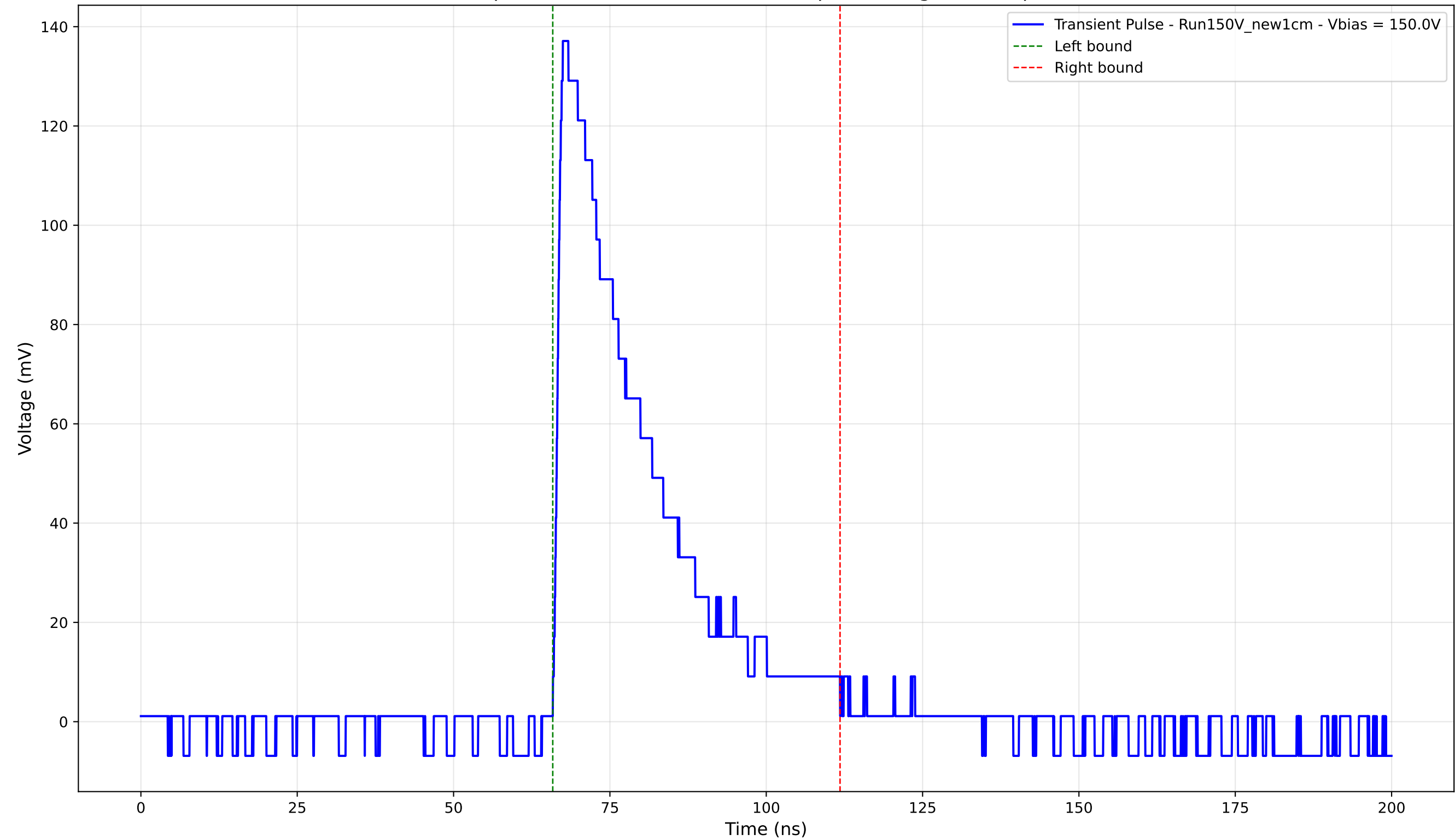
Transient Pulse - Sample: New1cm - Position: 3365.0 \mu\text{m} - Charge: 40.43 pC - Rise Time: 1.25 ns
