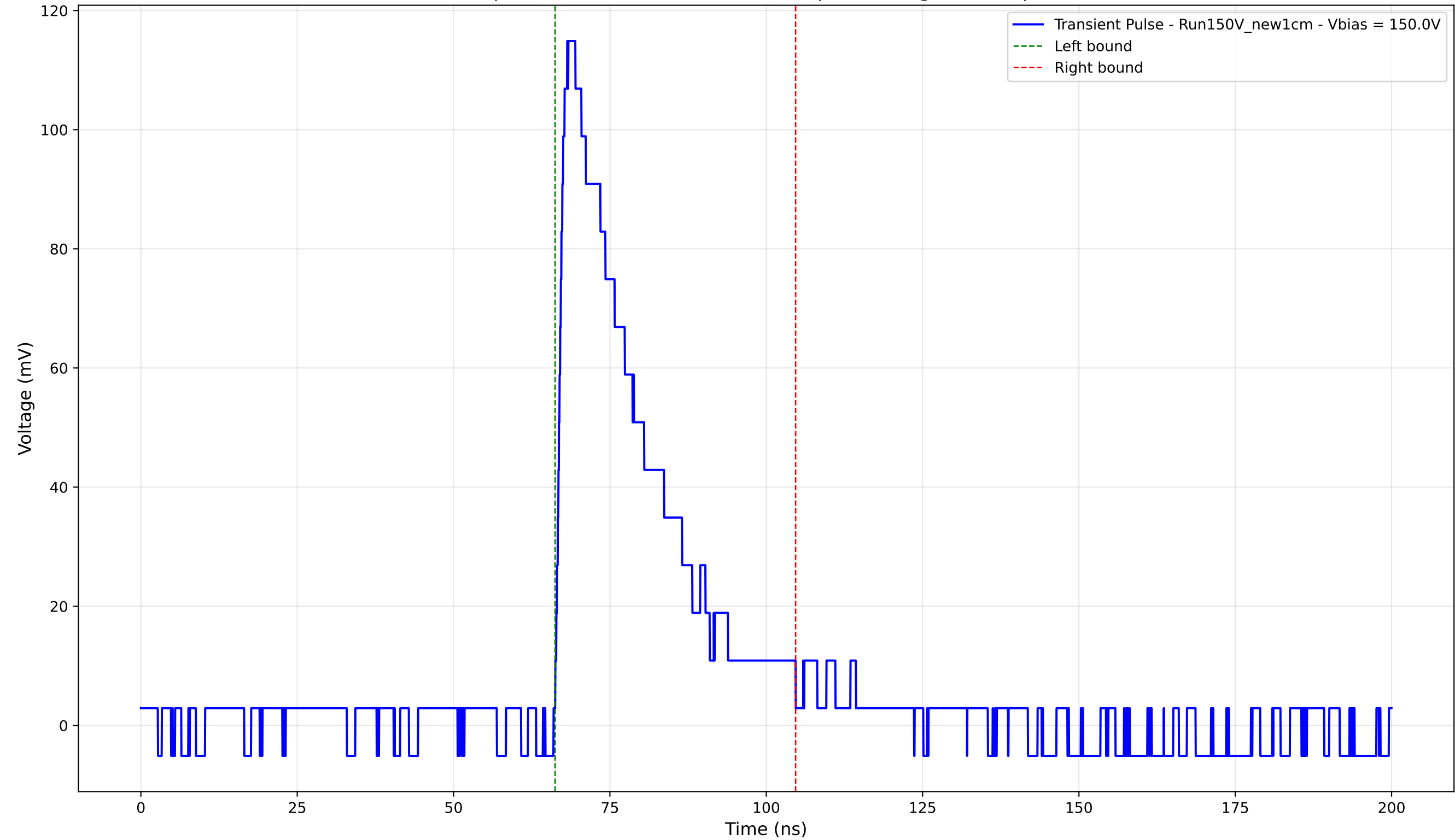
Transient Pulse - Sample: New1cm - Position: 1235.0 \mu\text{m} - Charge: 32.54 pC - Rise Time: 1.34 ns
