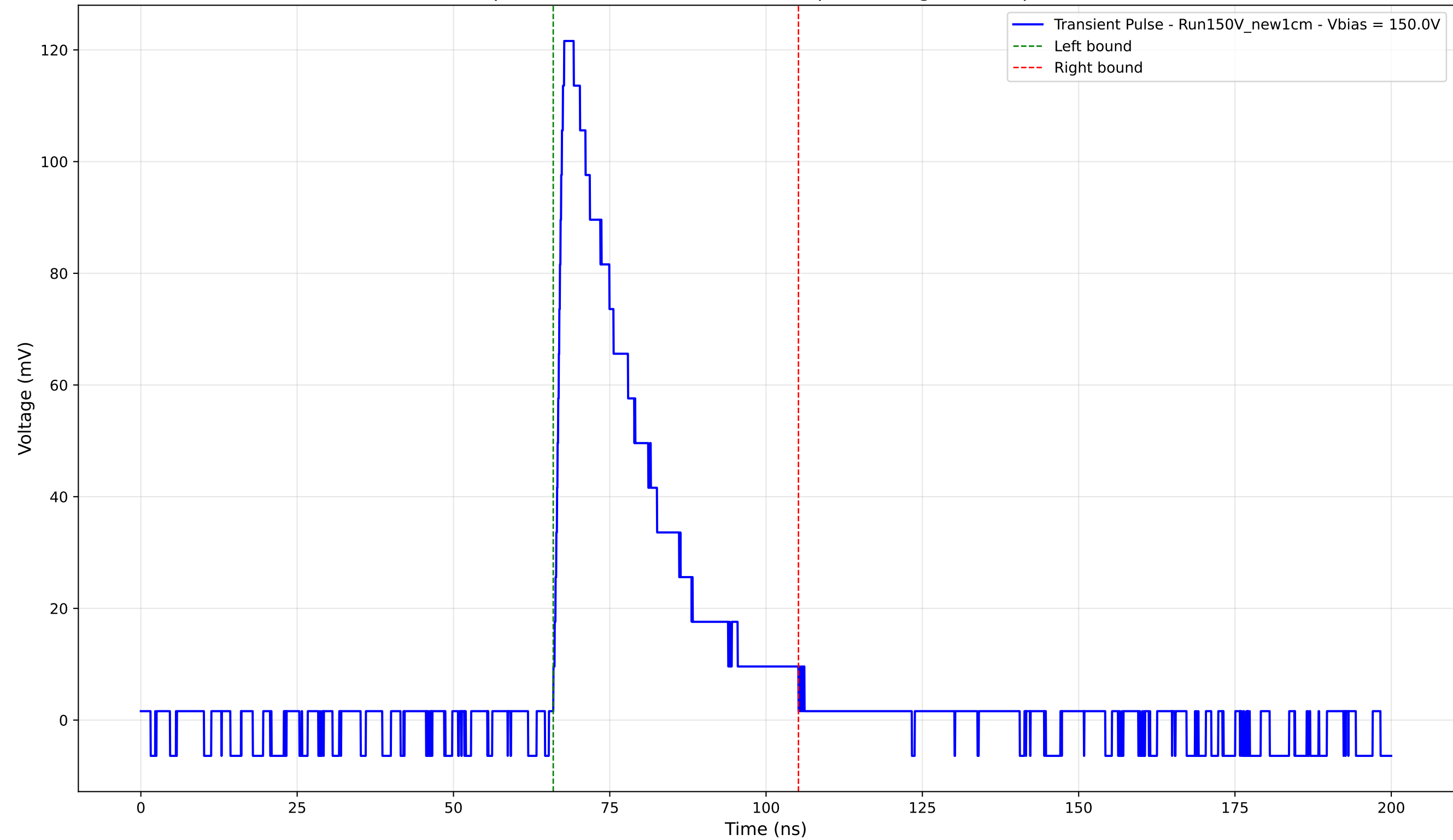
Transient Pulse - Sample: New1cm - Position: 3980.0 \mu\text{m} - Charge: 33.15 pC - Rise Time: 1.33 ns
