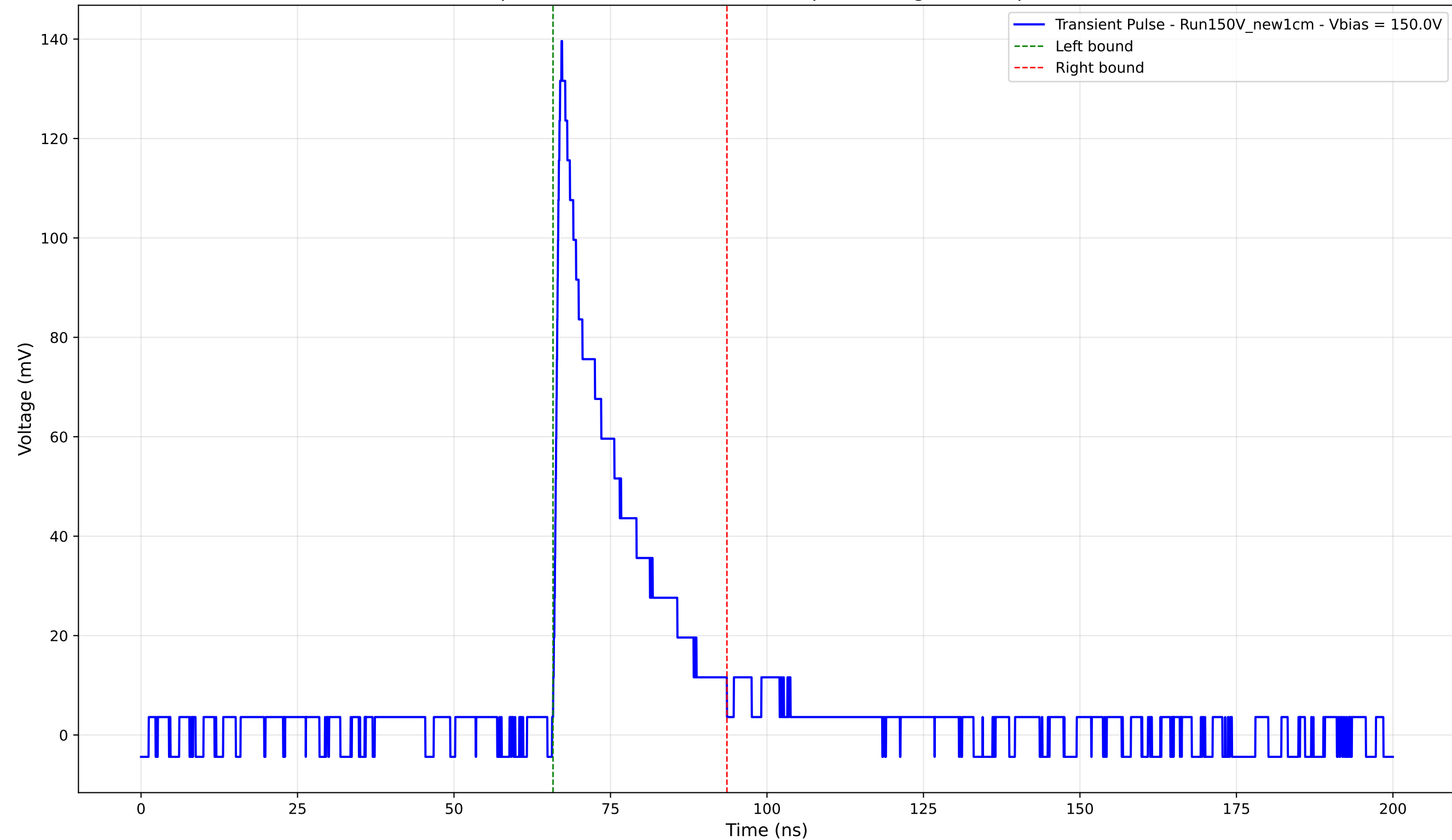
Transient Pulse - Sample: New1cm - Position: 215.0 \mu\text{m} - Charge: 25.70 pC - Rise Time: 1.01 ns
