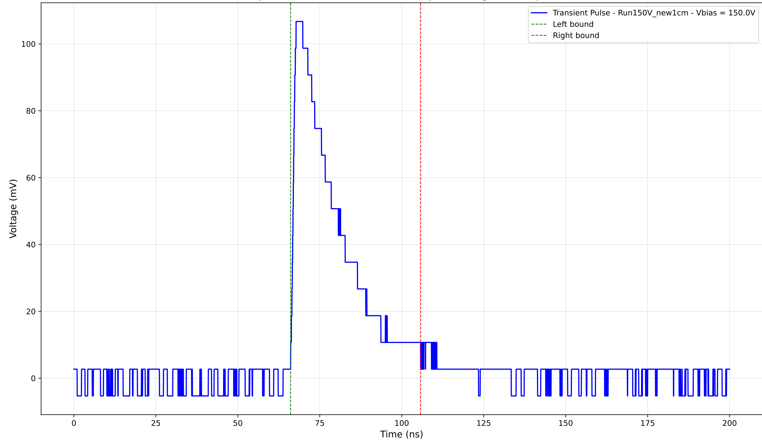
Transient Pulse - Sample: New1cm - Position: 1415.0 \mu\text{m} - Charge: 32.02 pC - Rise Time: 1.42 ns
