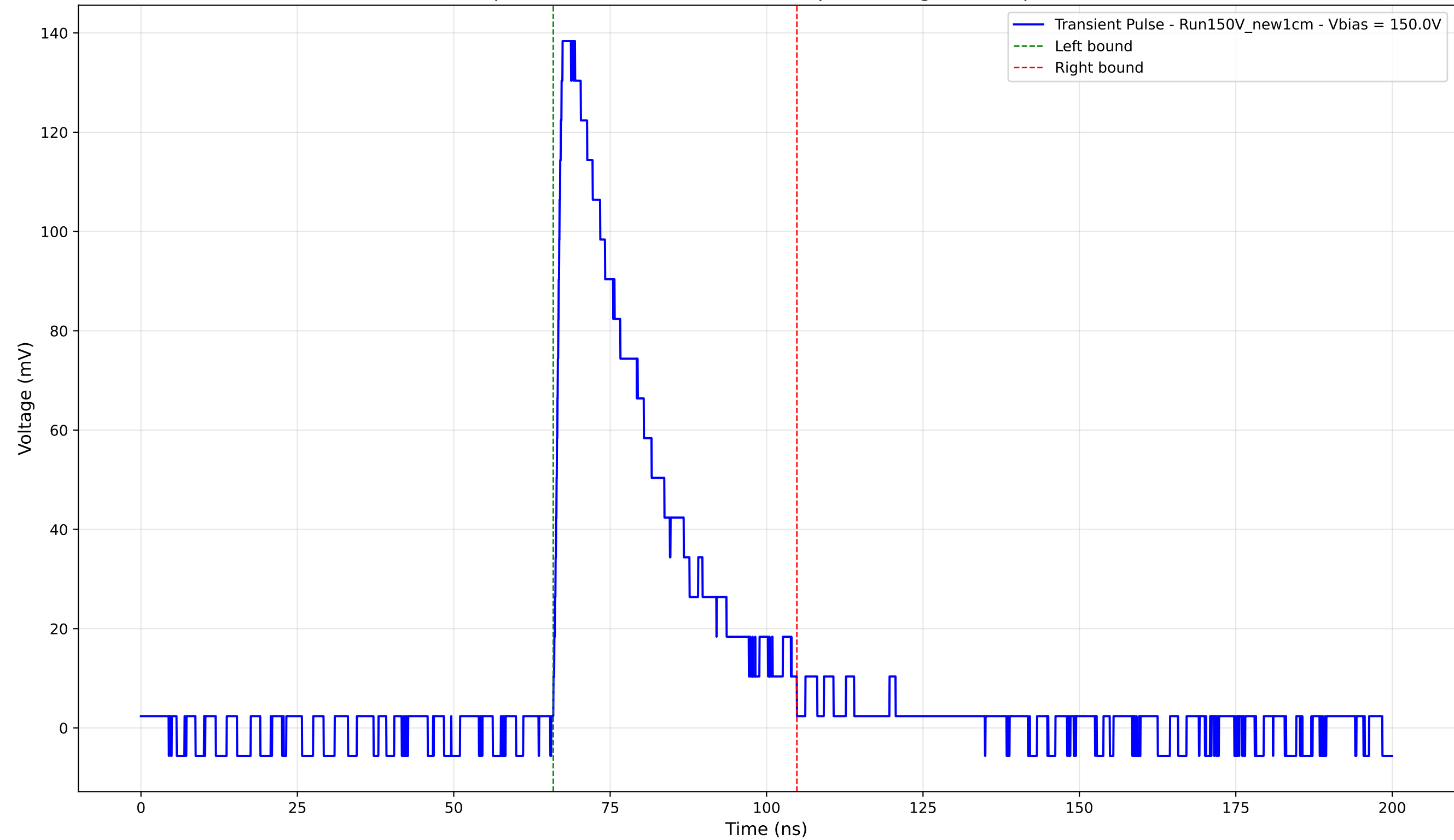
Transient Pulse - Sample: New1cm - Position: 3360.0 \mu\text{m} - Charge: 41.66 pC - Rise Time: 1.17 ns
