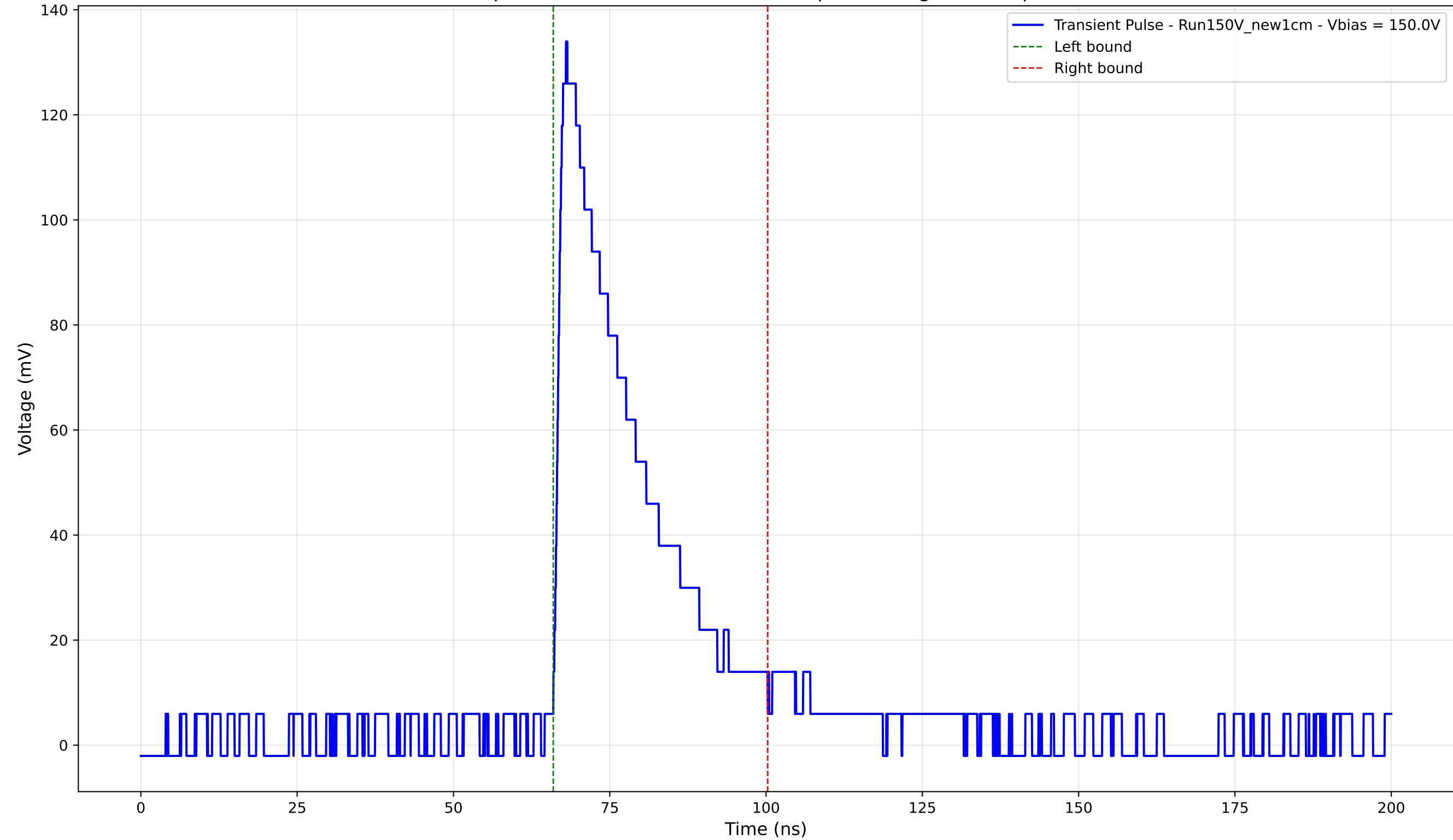
Transient Pulse - Sample: New1cm - Position: 4195.0 \mu\text{m} - Charge: 35.38 pC - Rise Time: 1.54 ns
