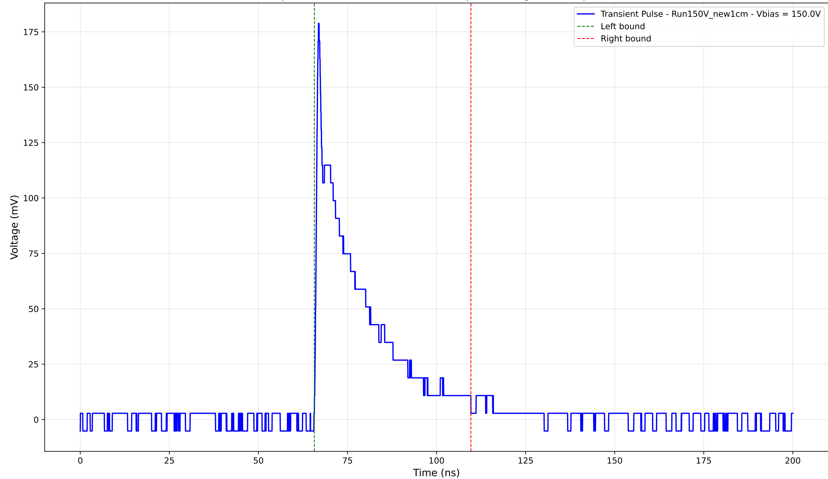
Transient Pulse - Sample: New1cm - Position: 2850.0 \mu\text{m} - Charge: 38.91 pC - Rise Time: 0.84 ns
