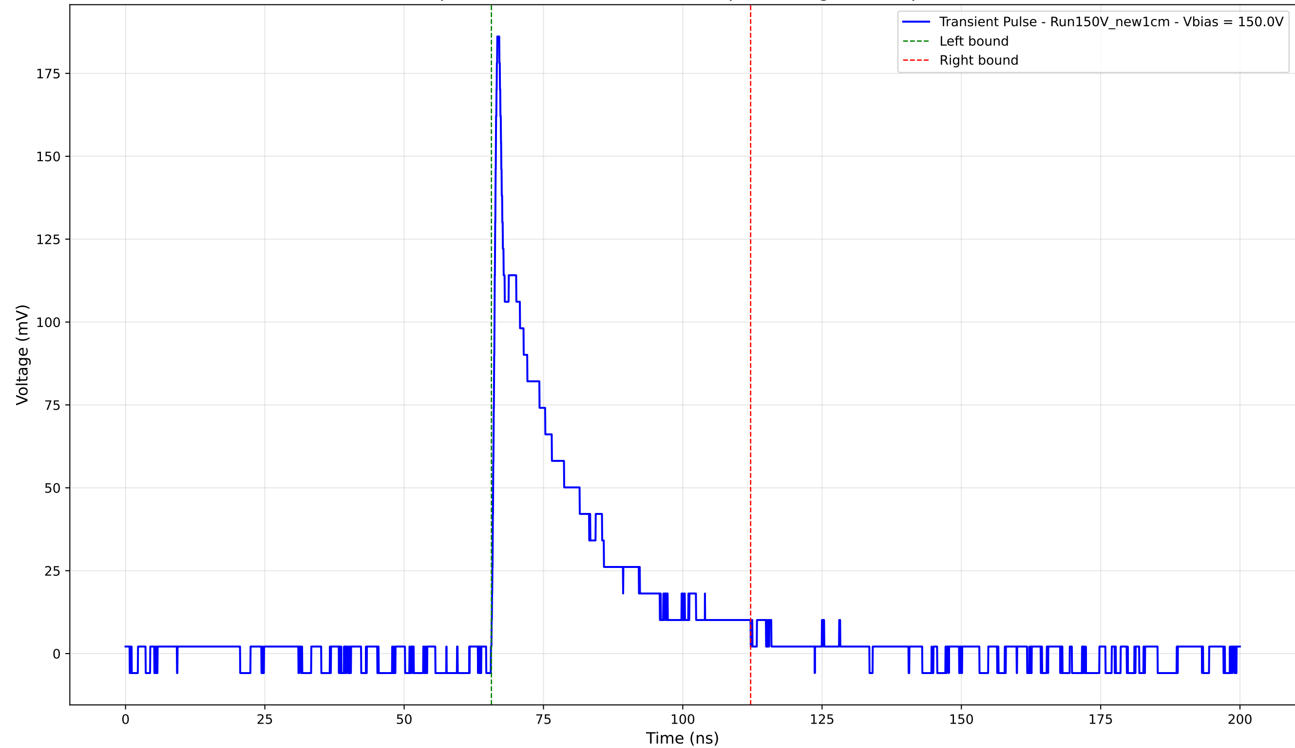
Transient Pulse - Sample: New1cm - Position: 2770.0 \mu\text{m} - Charge: 38.34 pC - Rise Time: 0.76 ns
