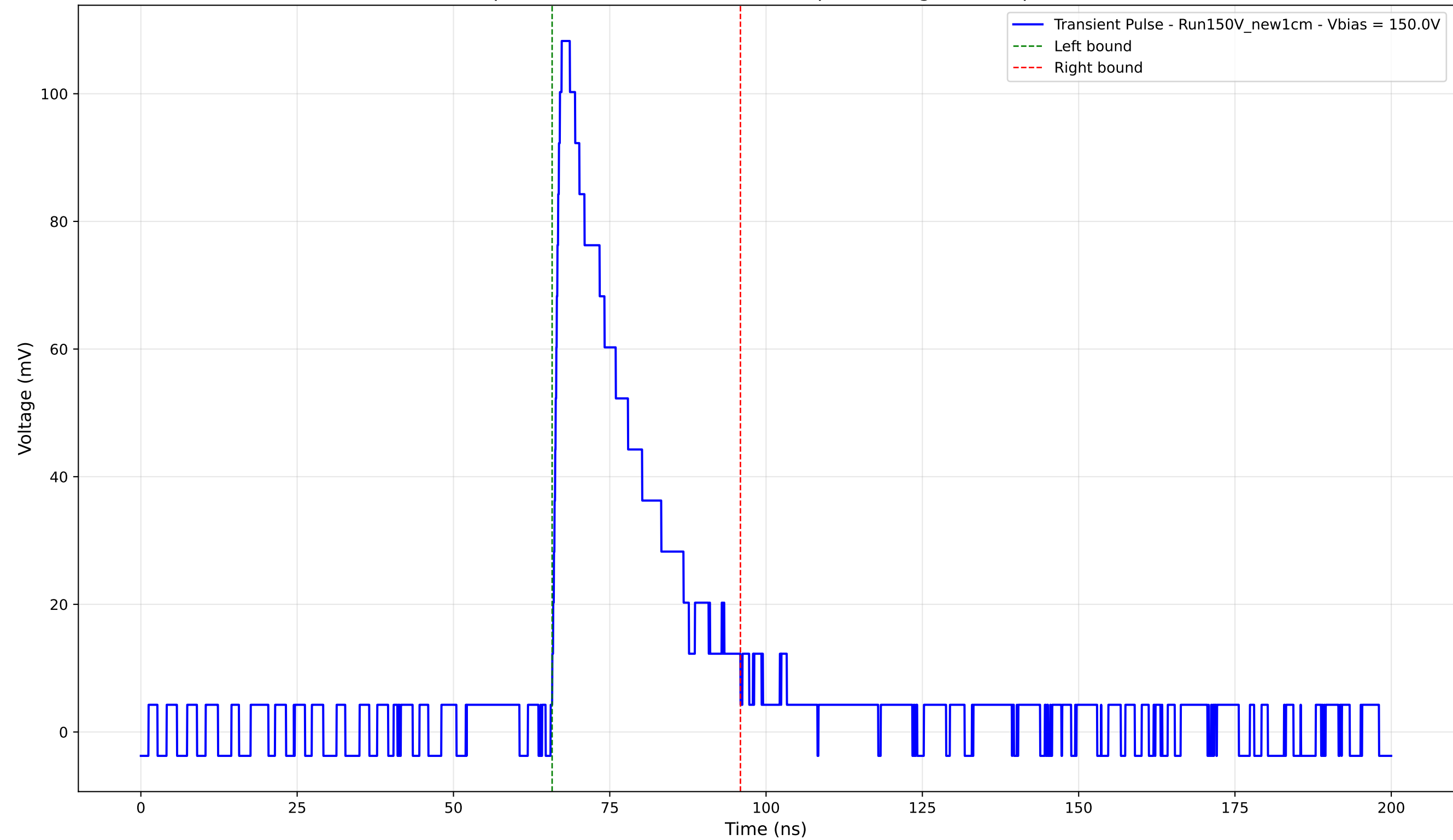
Transient Pulse - Sample: New1cm - Position: 4500.0 \mu\text{m} - Charge: 27.04 pC - Rise Time: 1.22 ns
