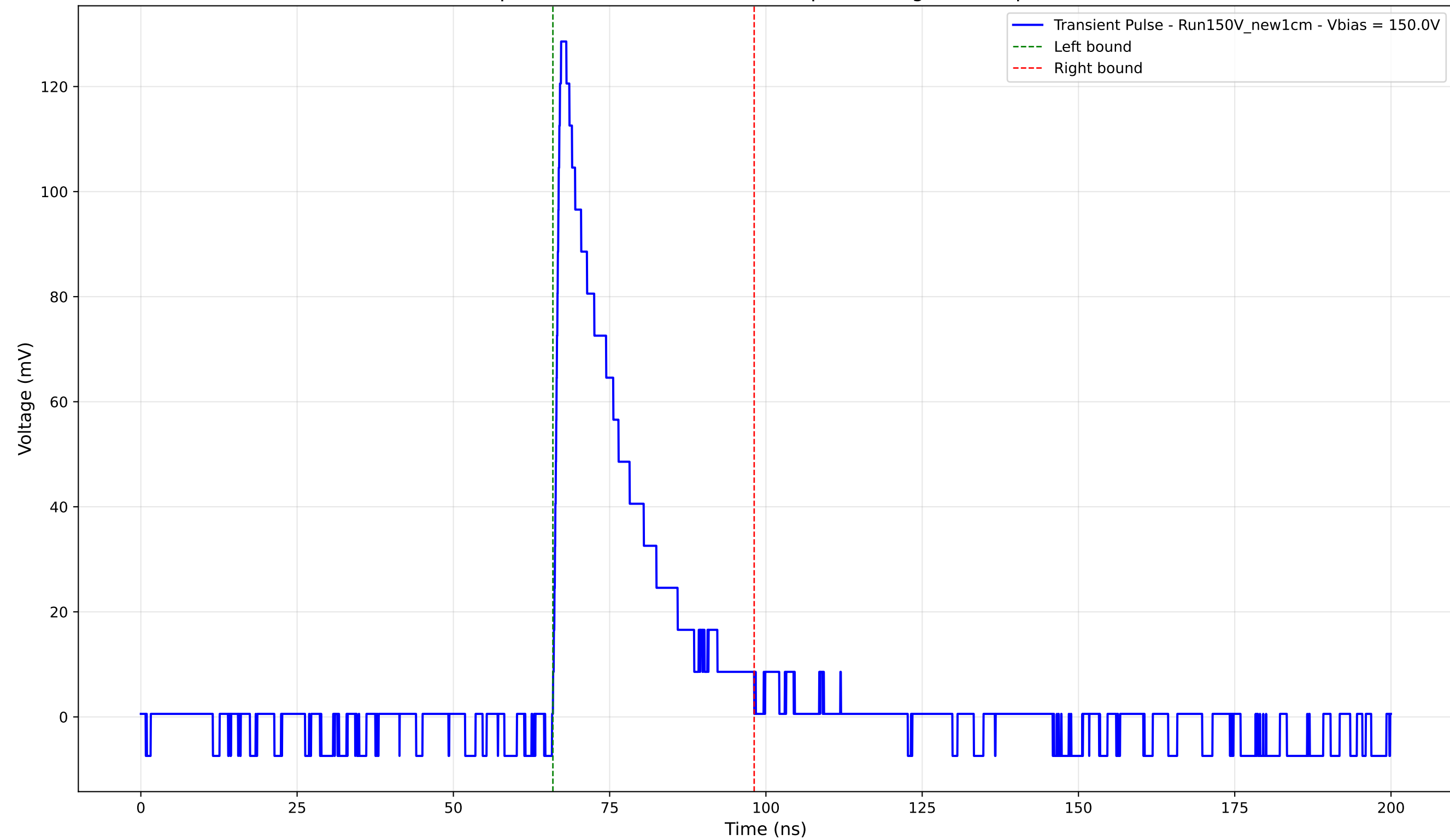
Transient Pulse - Sample: New1cm - Position: 375.0 \mu\text{m} - Charge: 27.10 pC - Rise Time: 0.99 ns
