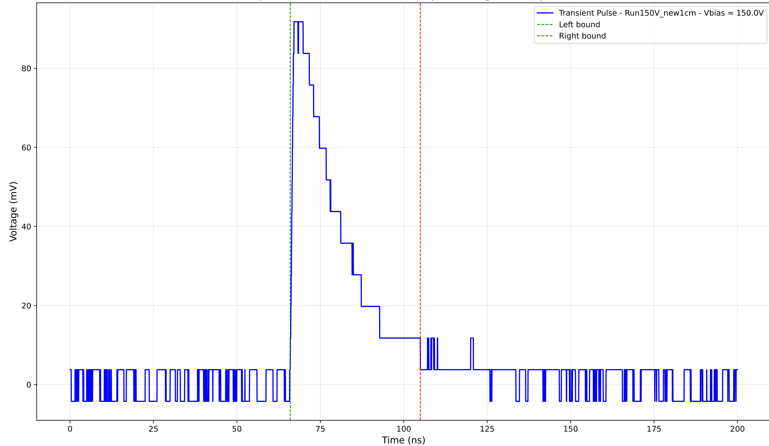
Transient Pulse - Sample: New1cm - Position: 1840.0 \mu\text{m} - Charge: 28.99 pC - Rise Time: 0.93 ns
