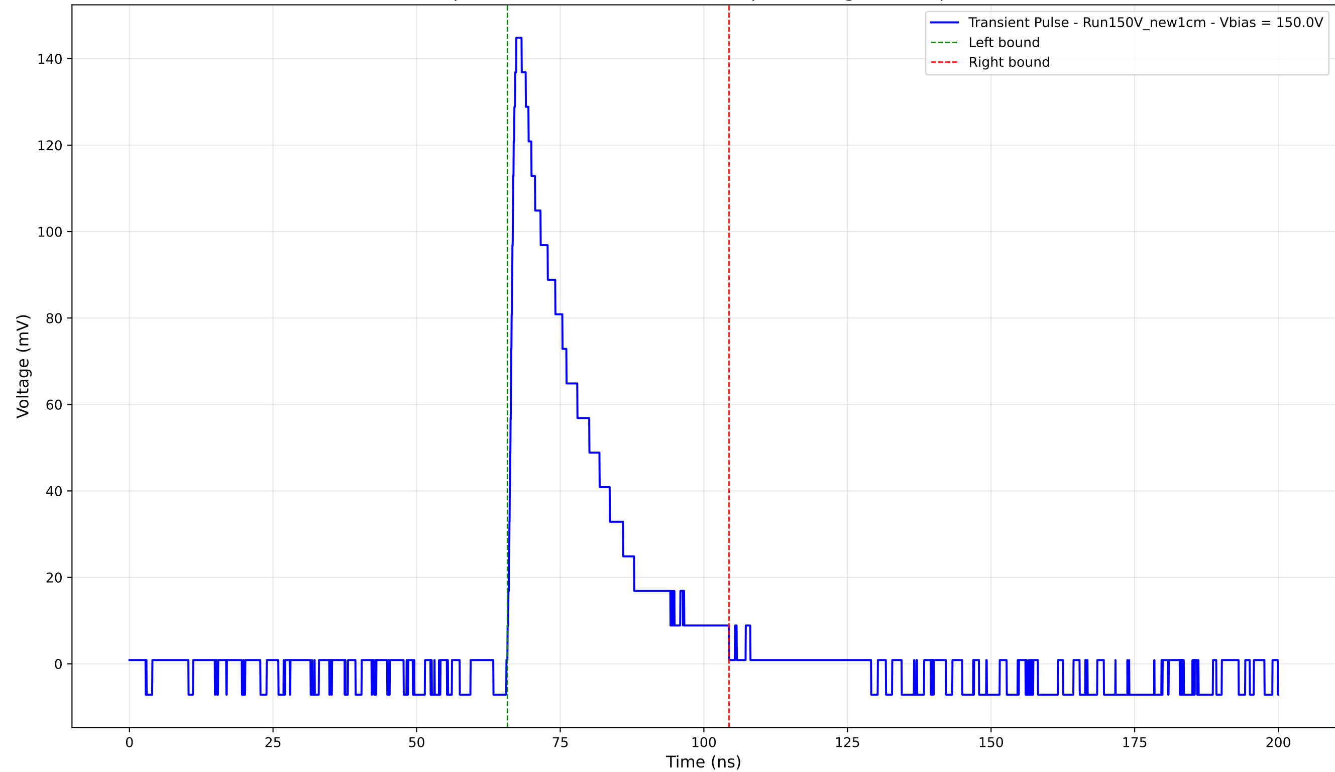
Transient Pulse - Sample: New1cm - Position: 4460.0 \mu\text{m} - Charge: 35.34 pC - Rise Time: 1.19 ns
