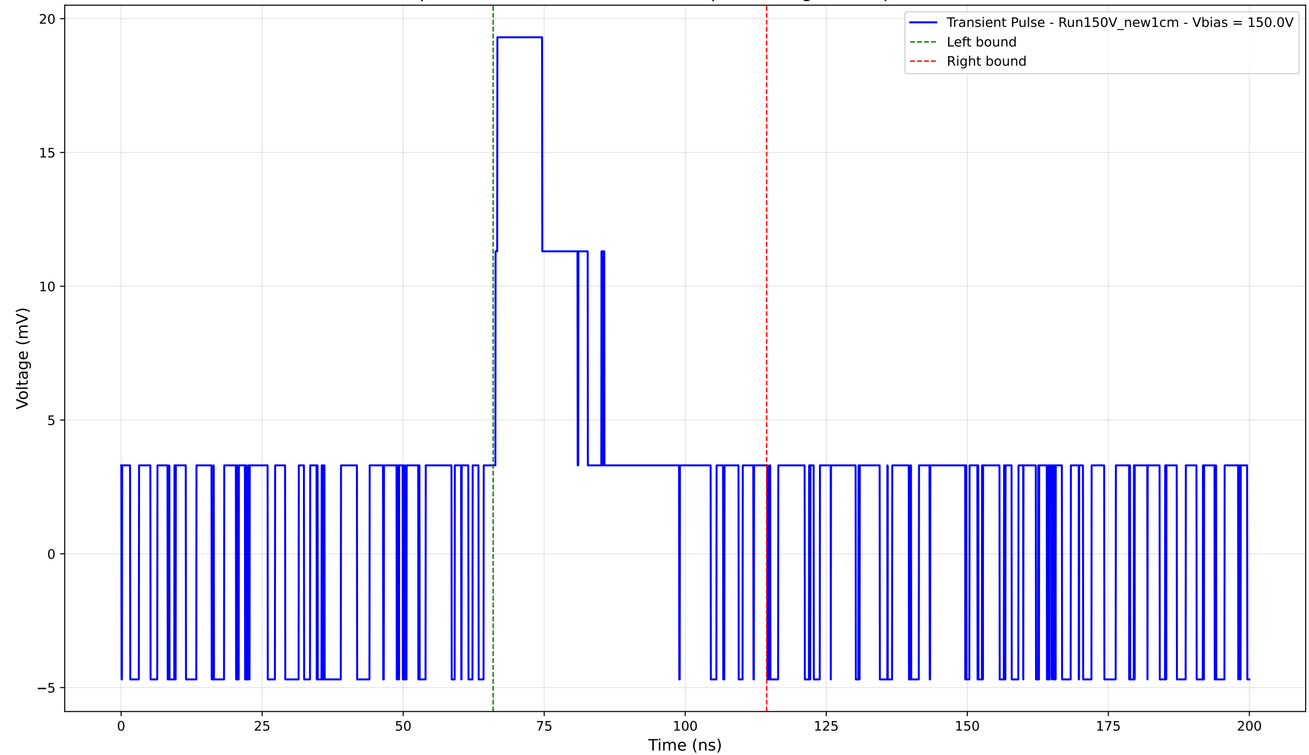
Transient Pulse - Sample: New1cm - Position: 3075.0 \mu\text{m} - Charge: 6.79 pC - Rise Time: 0.00 ns (N/A)
