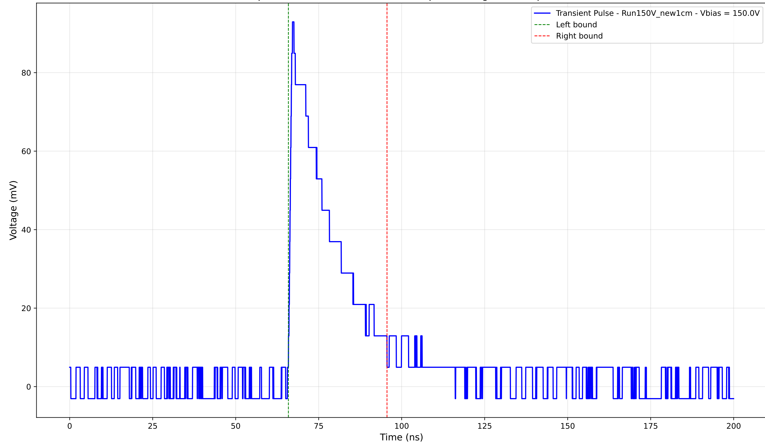
Transient Pulse - Sample: New1cm - Position: 1960.0 \mu\text{m} - Charge: 23.65 pC - Rise Time: 0.97 ns
