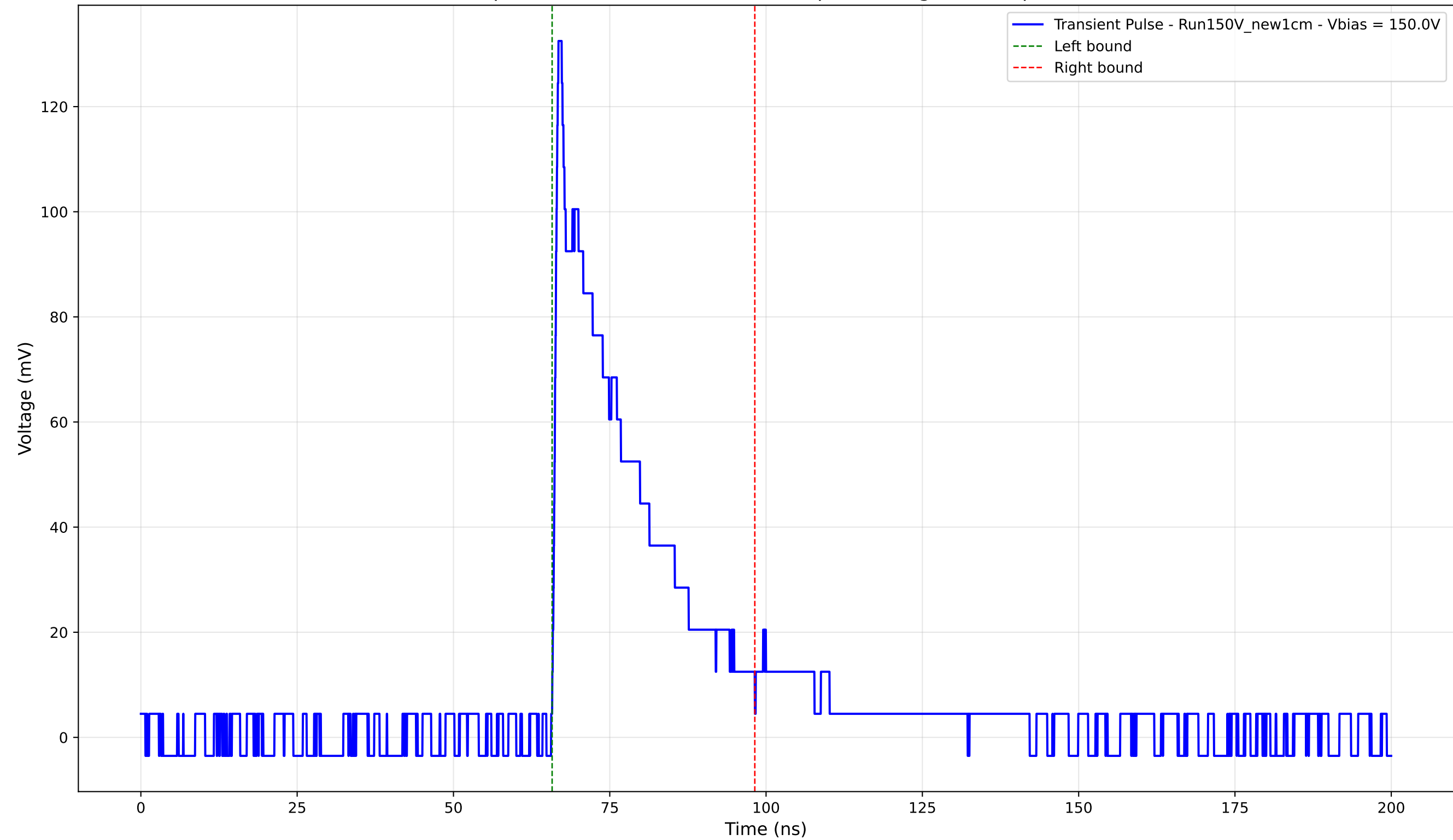
Transient Pulse - Sample: New1cm - Position: 2180.0 \mu\text{m} - Charge: 30.85 pC - Rise Time: 0.82 ns
