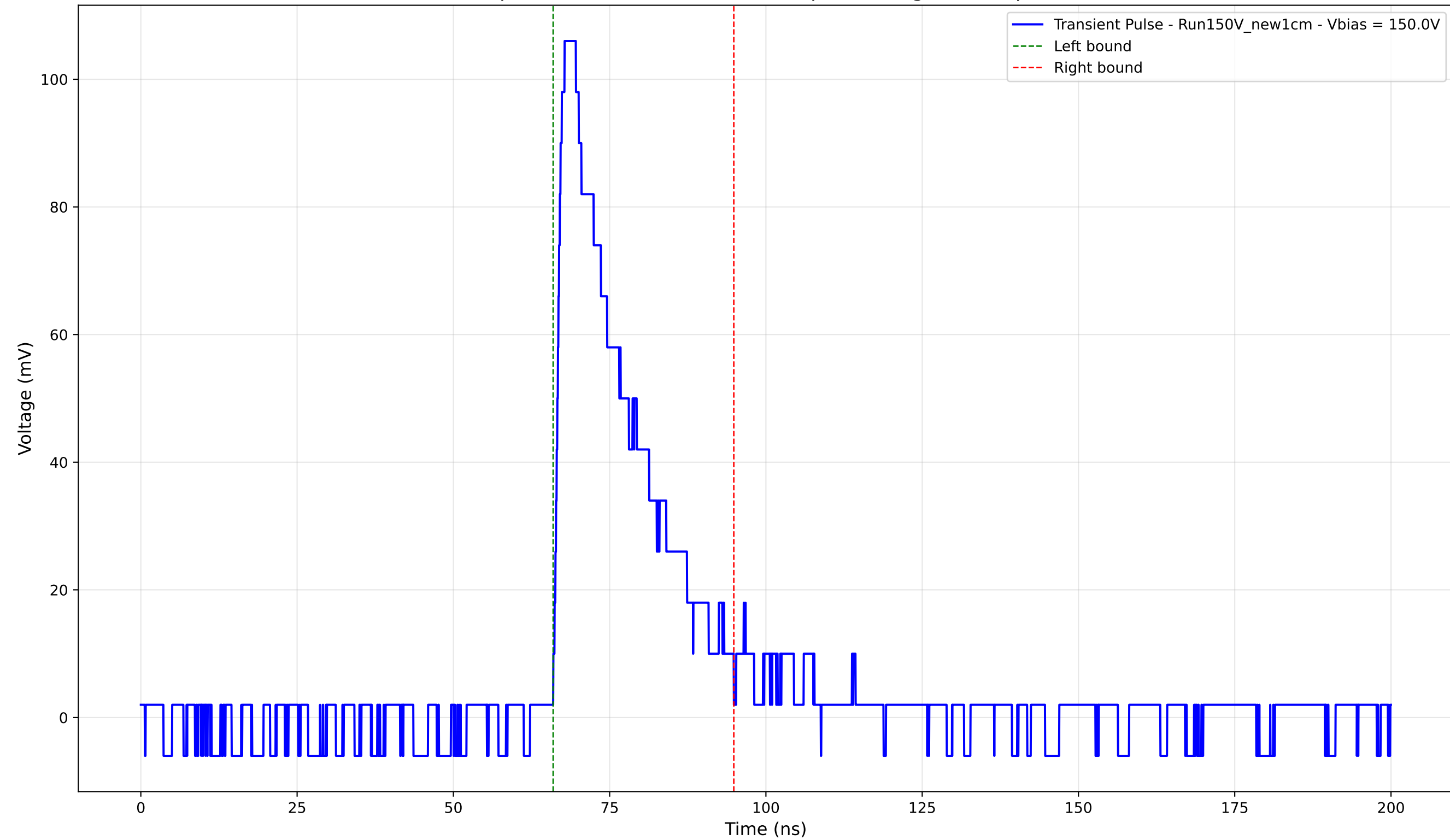
Transient Pulse - Sample: New1cm - Position: 645.0 \mu\text{m} - Charge: 26.31 pC - Rise Time: 1.18 ns
