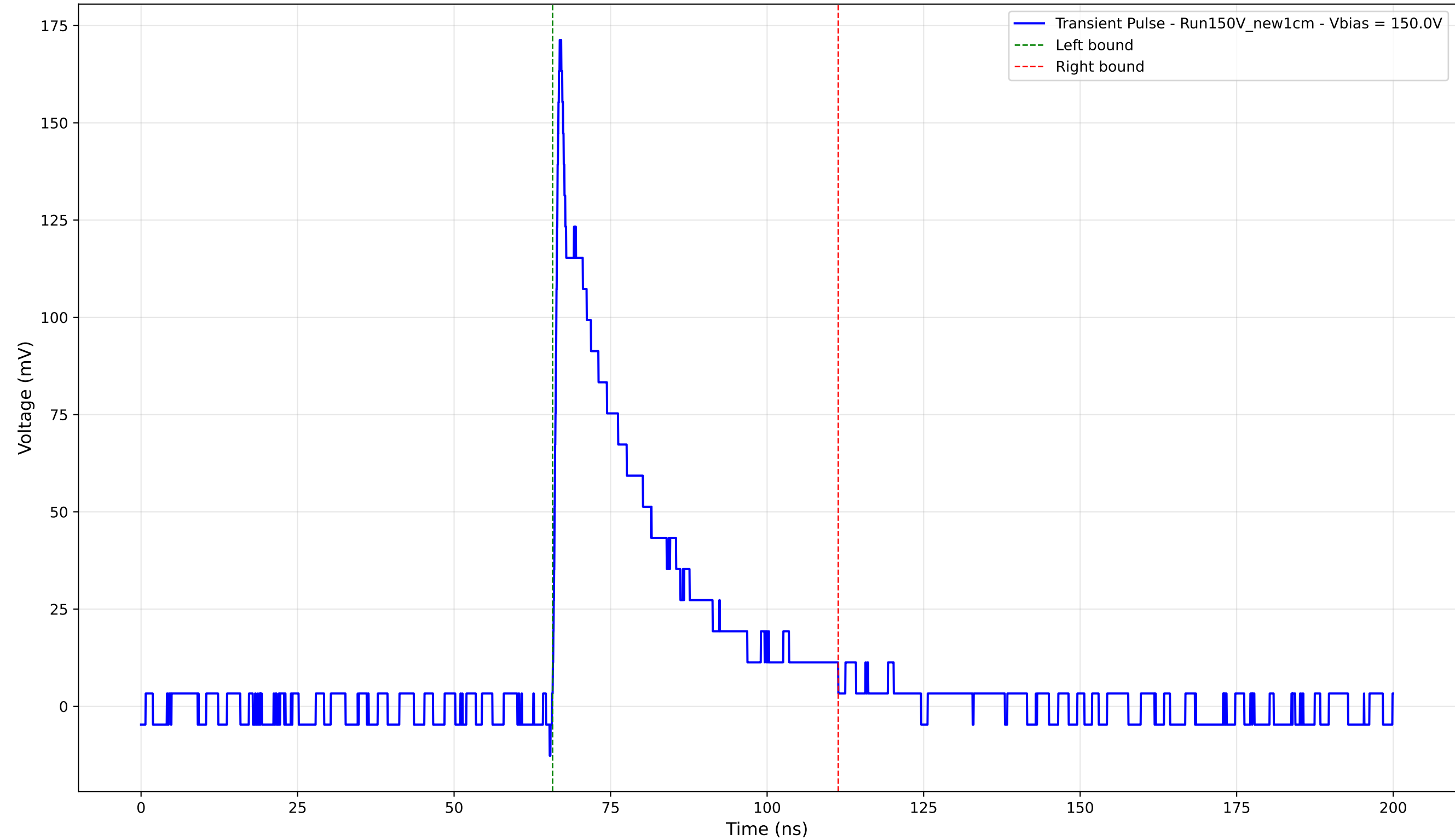
Transient Pulse - Sample: New1cm - Position: 2900.0 \mu\text{m} - Charge: 39.99 pC - Rise Time: 0.83 ns
