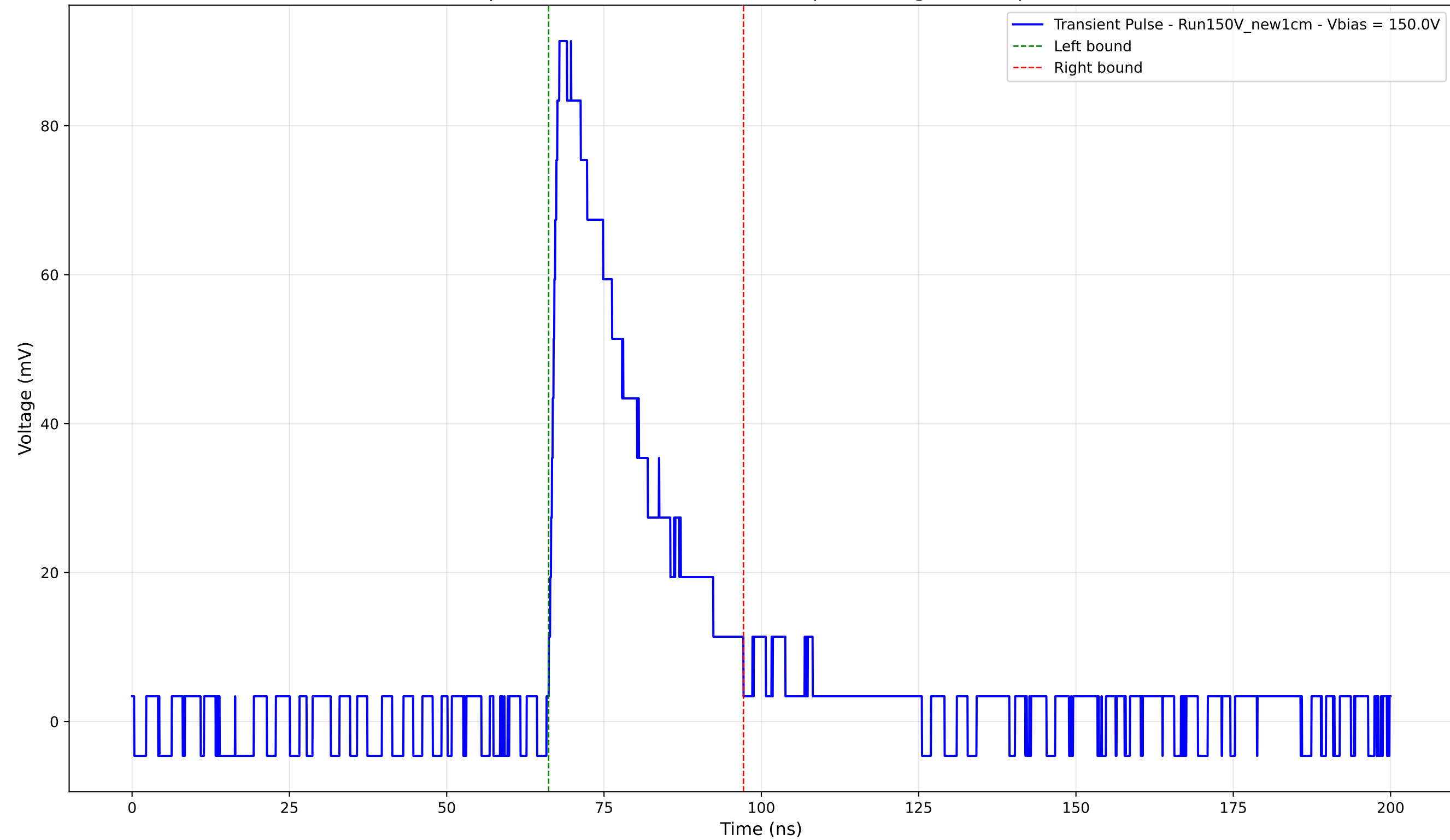
Transient Pulse - Sample: New1cm - Position: 1125.0 \mu\text{m} - Charge: 25.03 pC - Rise Time: 1.37 ns
