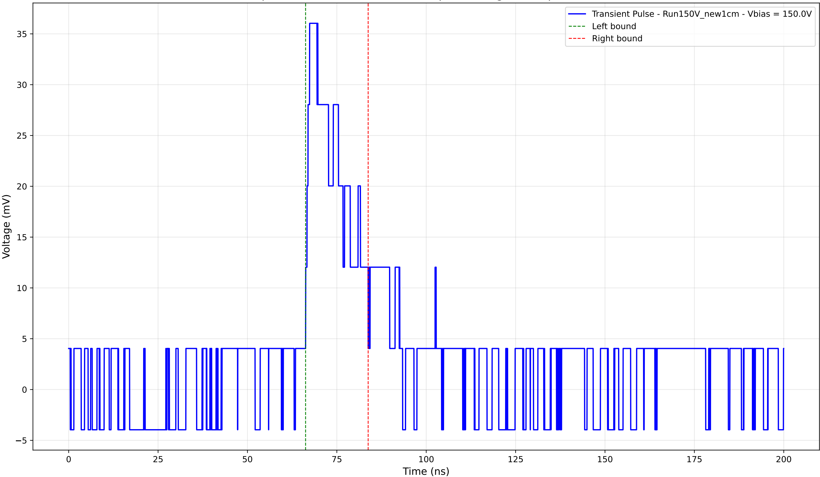
Transient Pulse - Sample: New1cm - Position: 560.0 \mu\text{m} - Charge: 7.69 pC - Rise Time: 0.00 ns (N/A)
