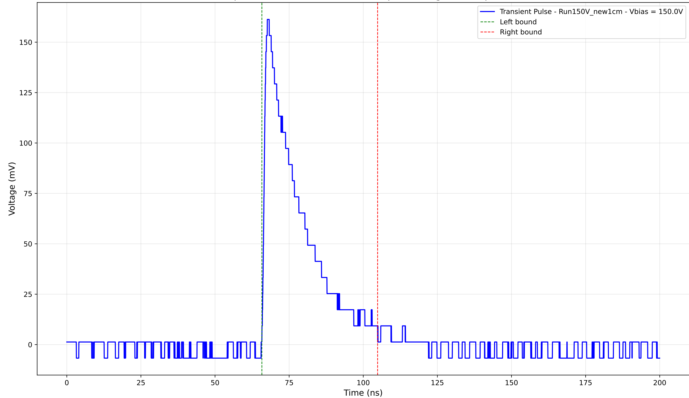
Transient Pulse - Sample: New1cm - Position: 4380.0 \mu\text{m} - Charge: 41.59 pC - Rise Time: 1.18 ns
