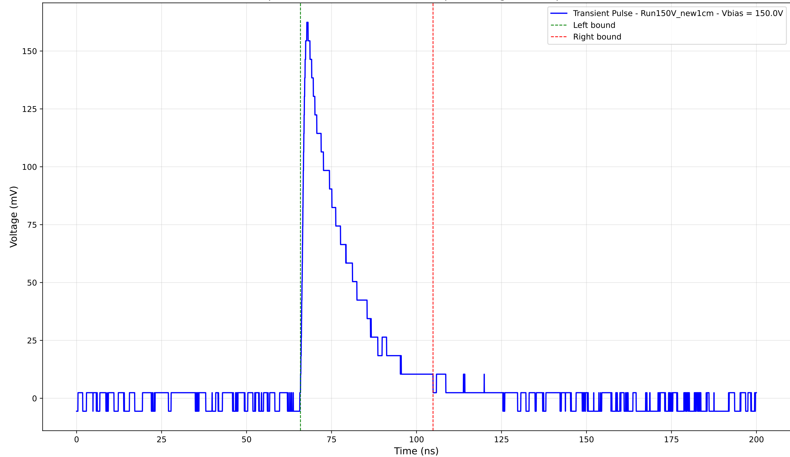
Transient Pulse - Sample: New1cm - Position: 4420.0 \mu\text{m} - Charge: 39.76 pC - Rise Time: 1.25 ns
