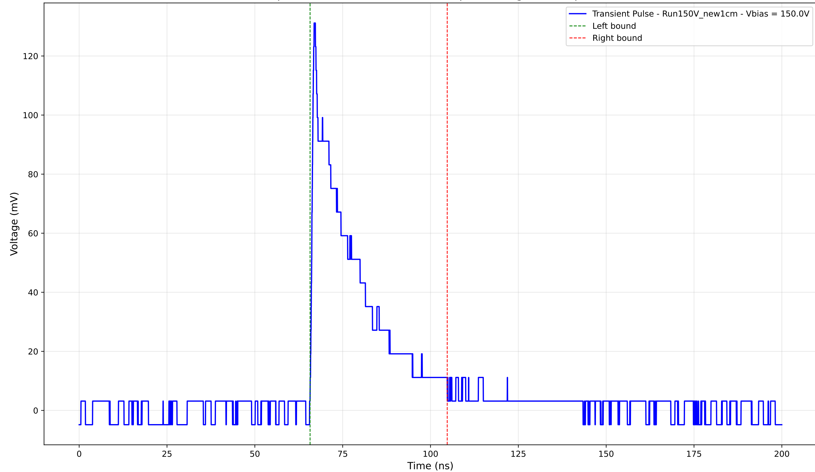
Transient Pulse - Sample: New1cm - Position: 2165.0 \mu\text{m} - Charge: 31.03 pC - Rise Time: 0.90 ns
