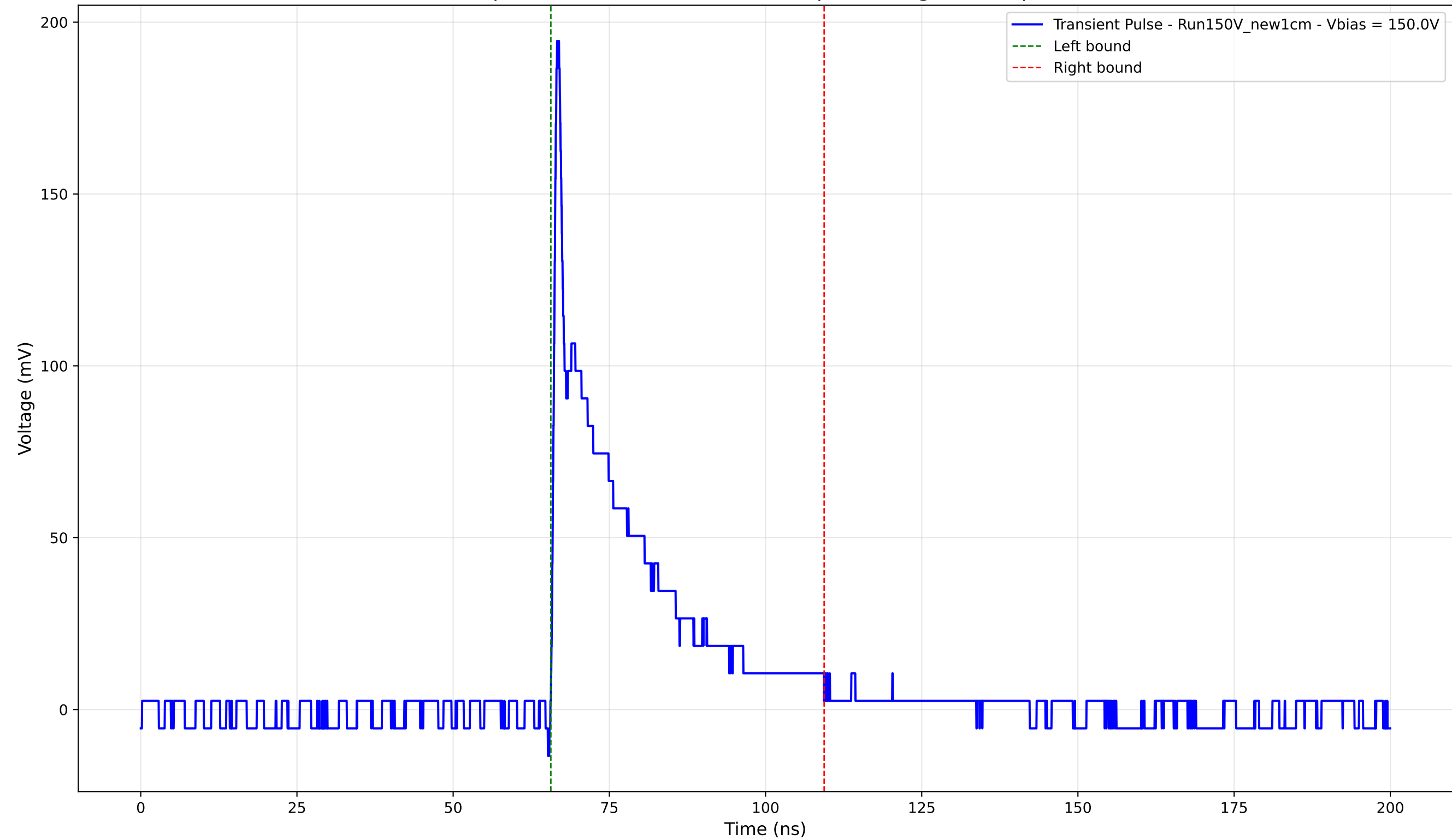
Transient Pulse - Sample: New1cm - Position: 2670.0 \mu\text{m} - Charge: 35.43 pC - Rise Time: 0.74 ns
