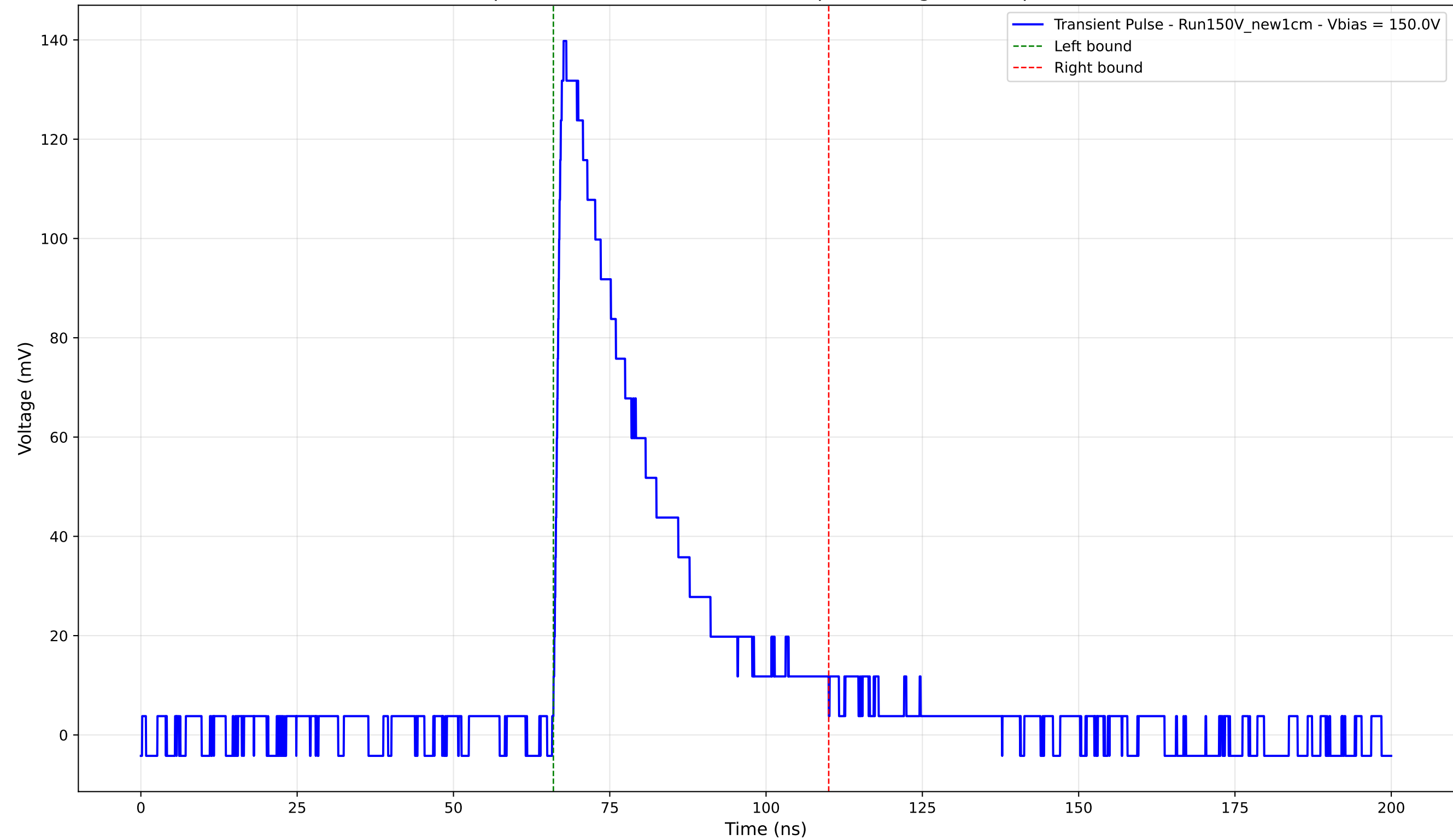
Transient Pulse - Sample: New1cm - Position: 3345.0 \mu\text{m} - Charge: 41.16 pC - Rise Time: 1.21 ns
