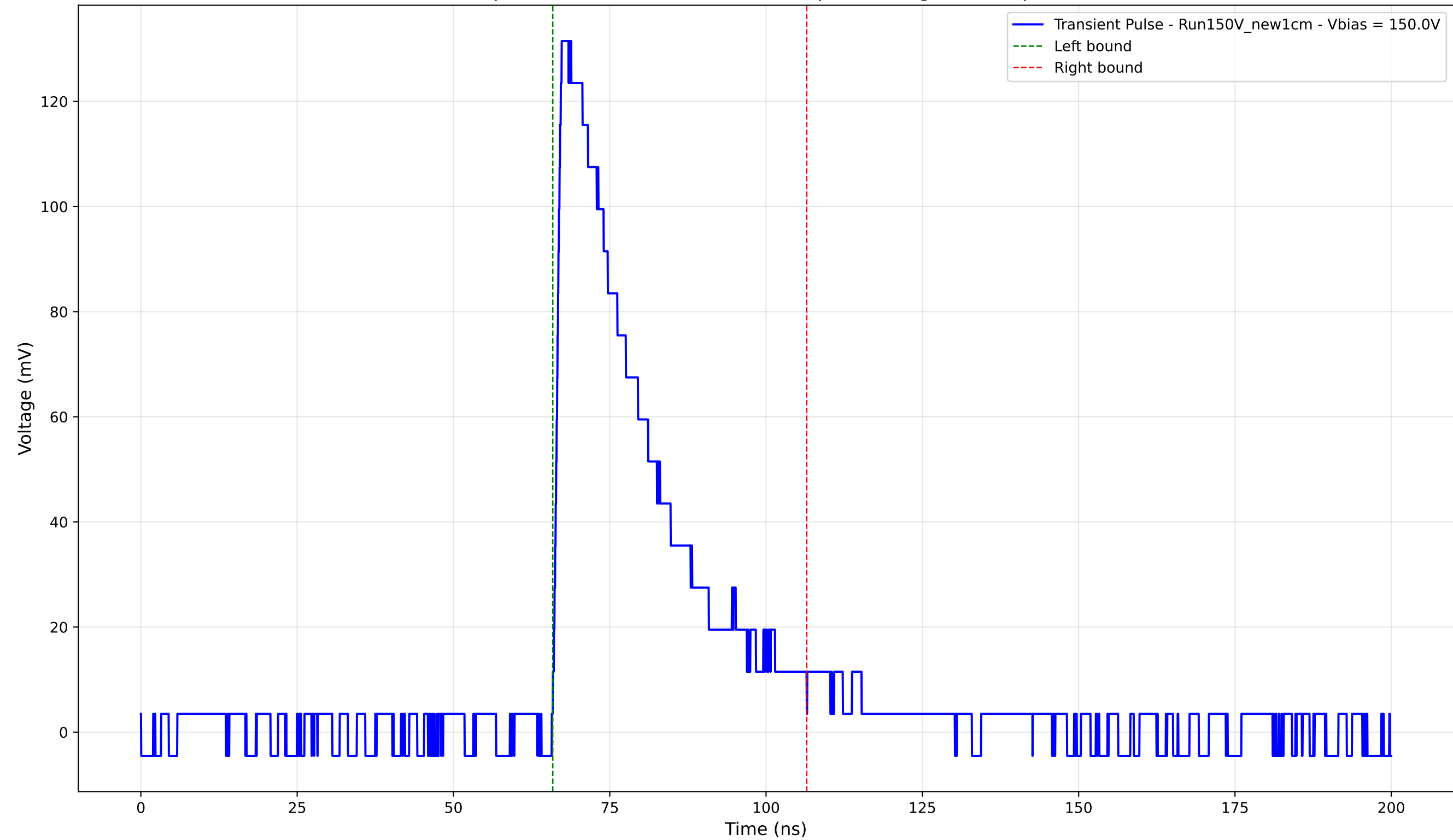
Transient Pulse - Sample: New1cm - Position: 3355.0 \mu\text{m} - Charge: 40.34 pC - Rise Time: 1.12 ns
