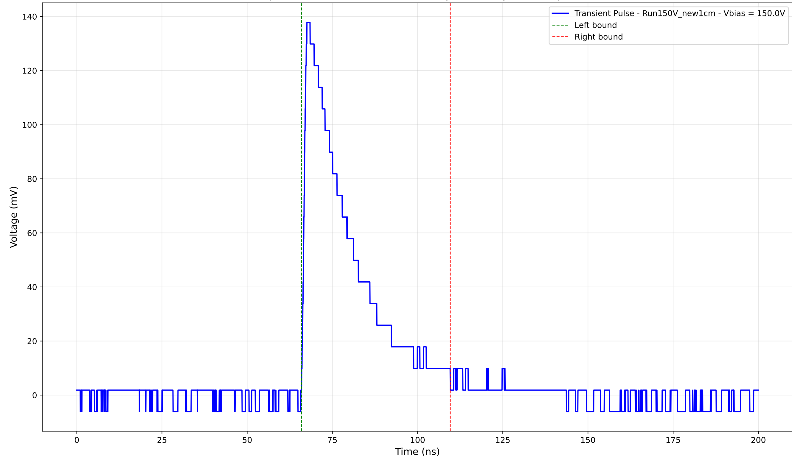
Transient Pulse - Sample: New1cm - Position: 3455.0 \mu\text{m} - Charge: 40.44 pC - Rise Time: 1.23 ns
