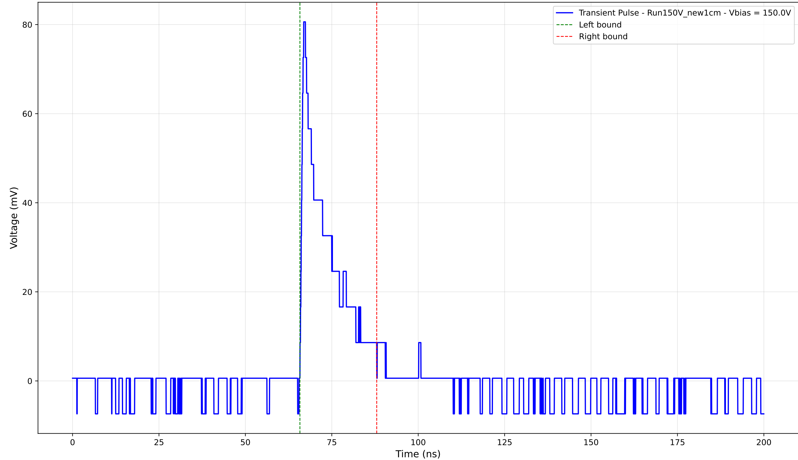
Transient Pulse - Sample: New1cm - Position: 90.0 \mu\text{m} - Charge: 12.26 pC - Rise Time: 0.88 ns
