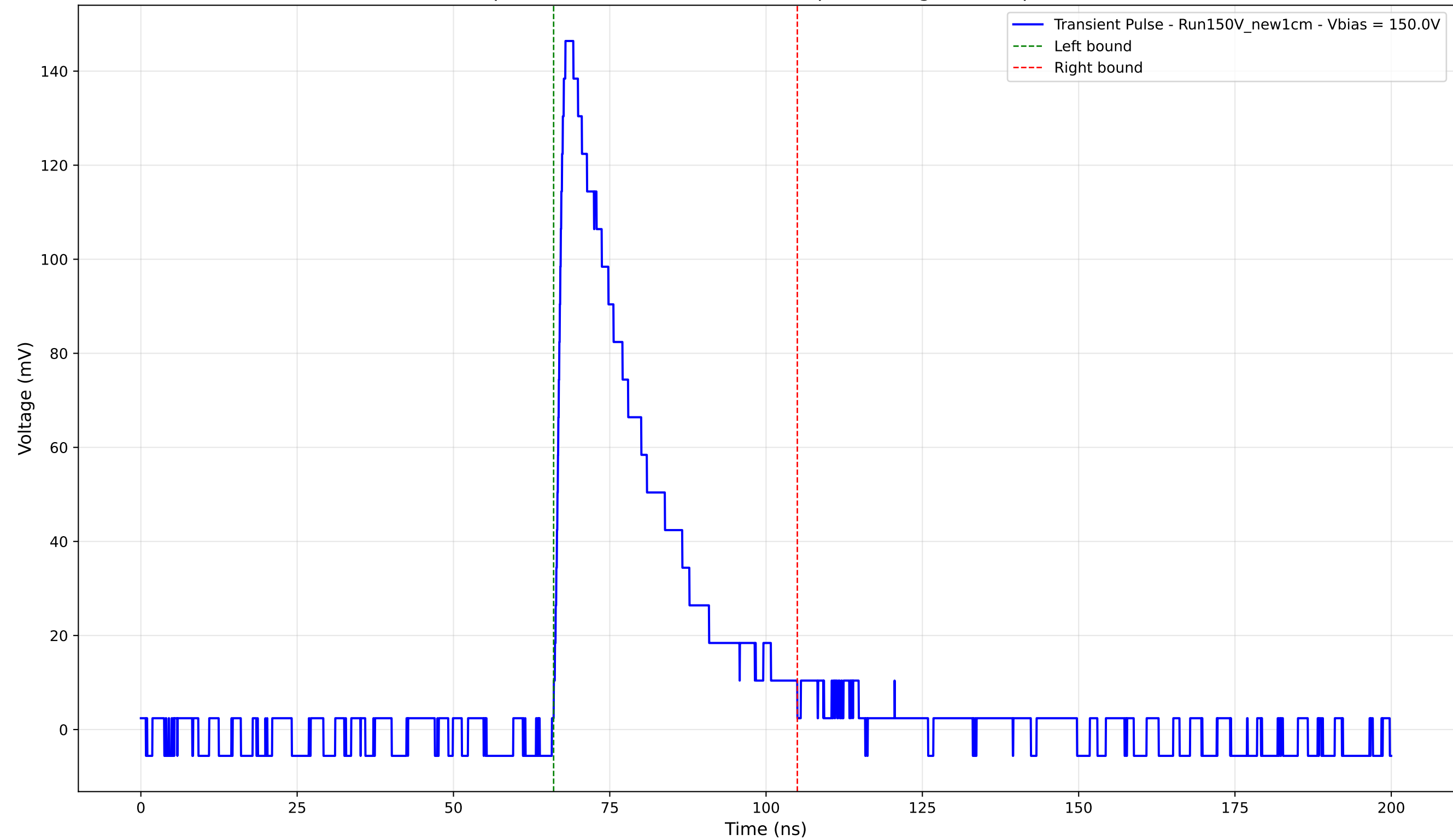
Transient Pulse - Sample: New1cm - Position: 3855.0 \mu\text{m} - Charge: 40.78 pC - Rise Time: 1.43 ns
