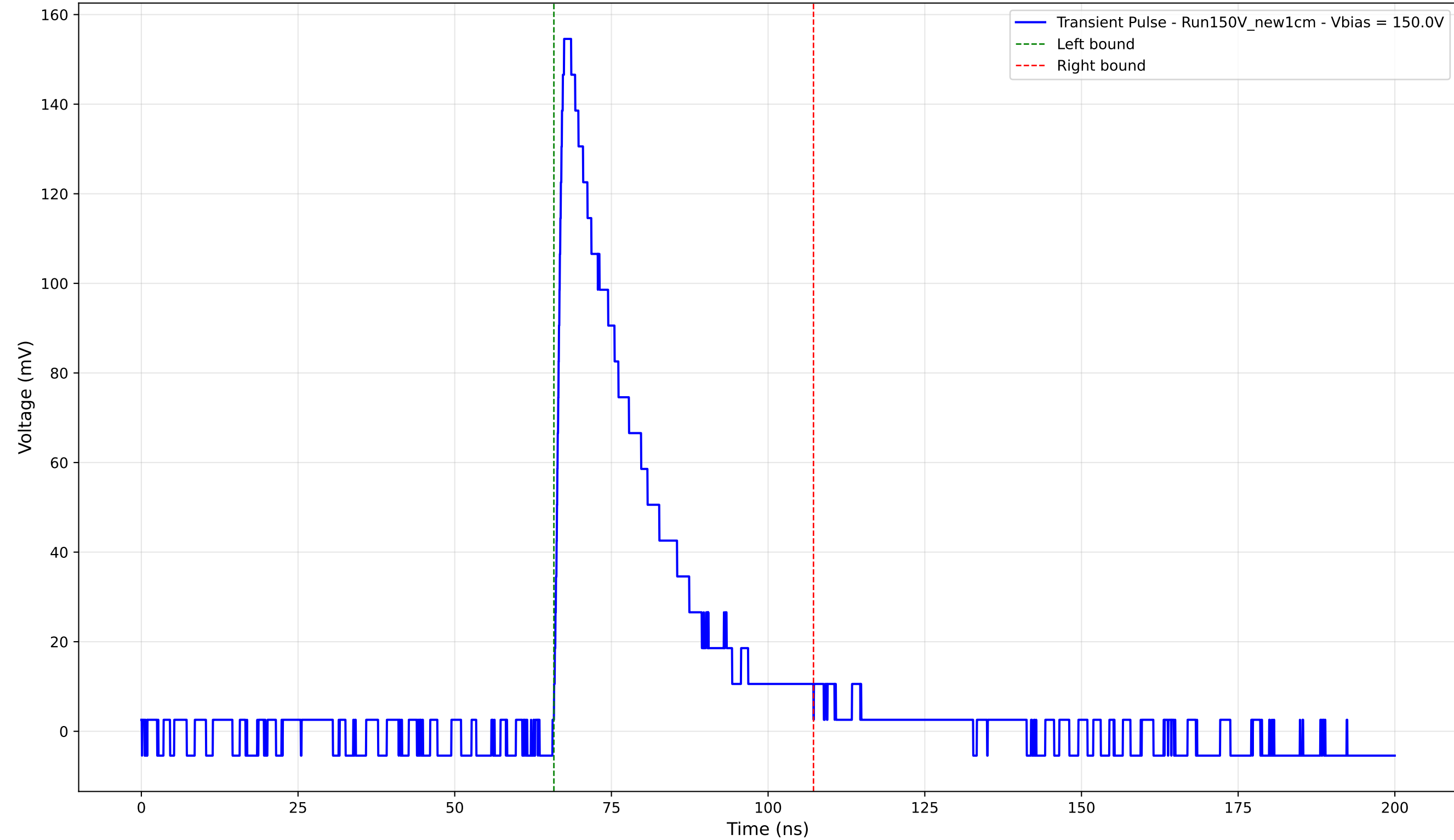
Transient Pulse - Sample: New1cm - Position: 4375.0 \mu\text{m} - Charge: 40.79 pC - Rise Time: 1.29 ns
