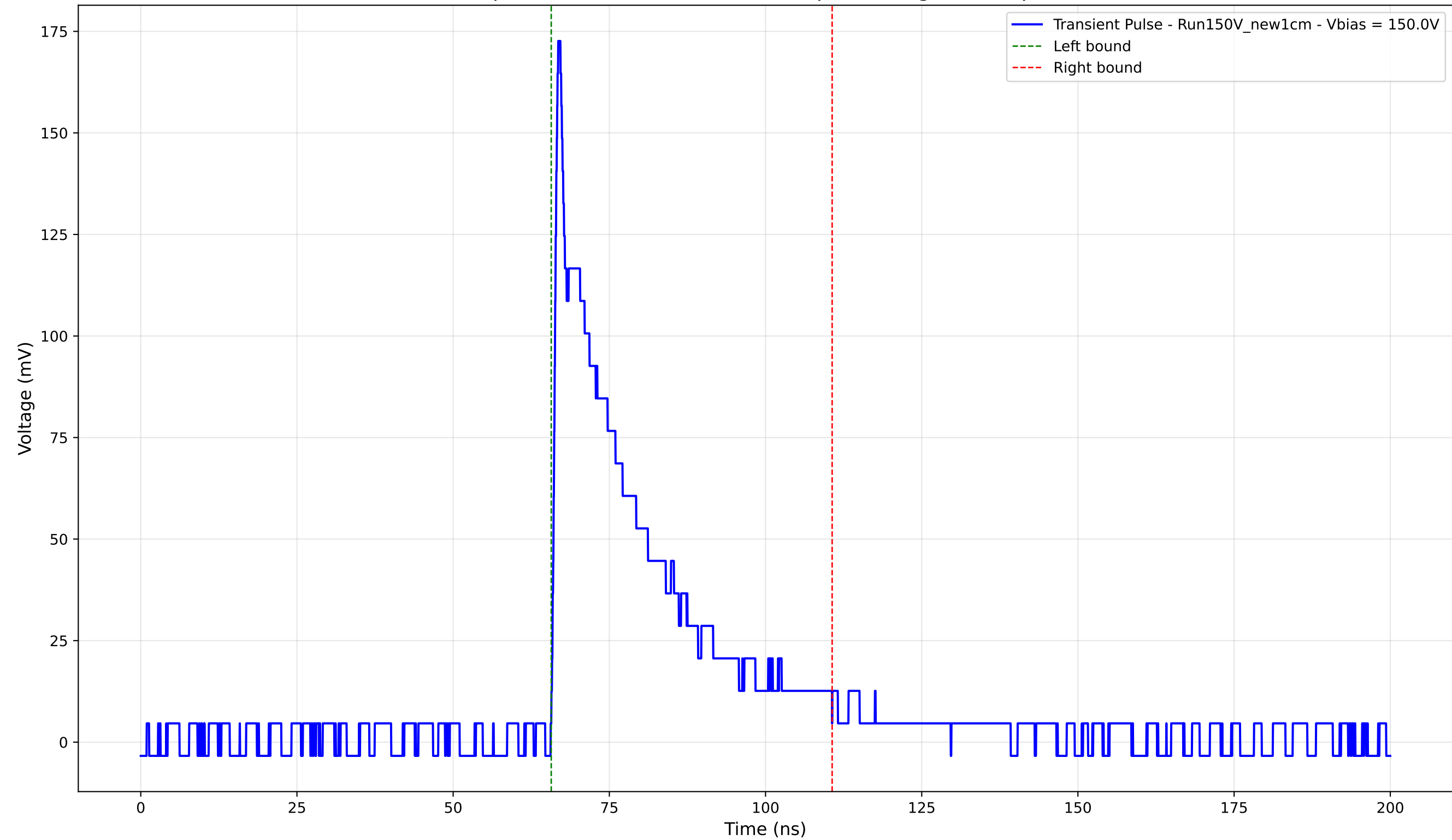
Transient Pulse - Sample: New1cm - Position: 2880.0 \mu\text{m} - Charge: 40.52 pC - Rise Time: 0.83 ns
