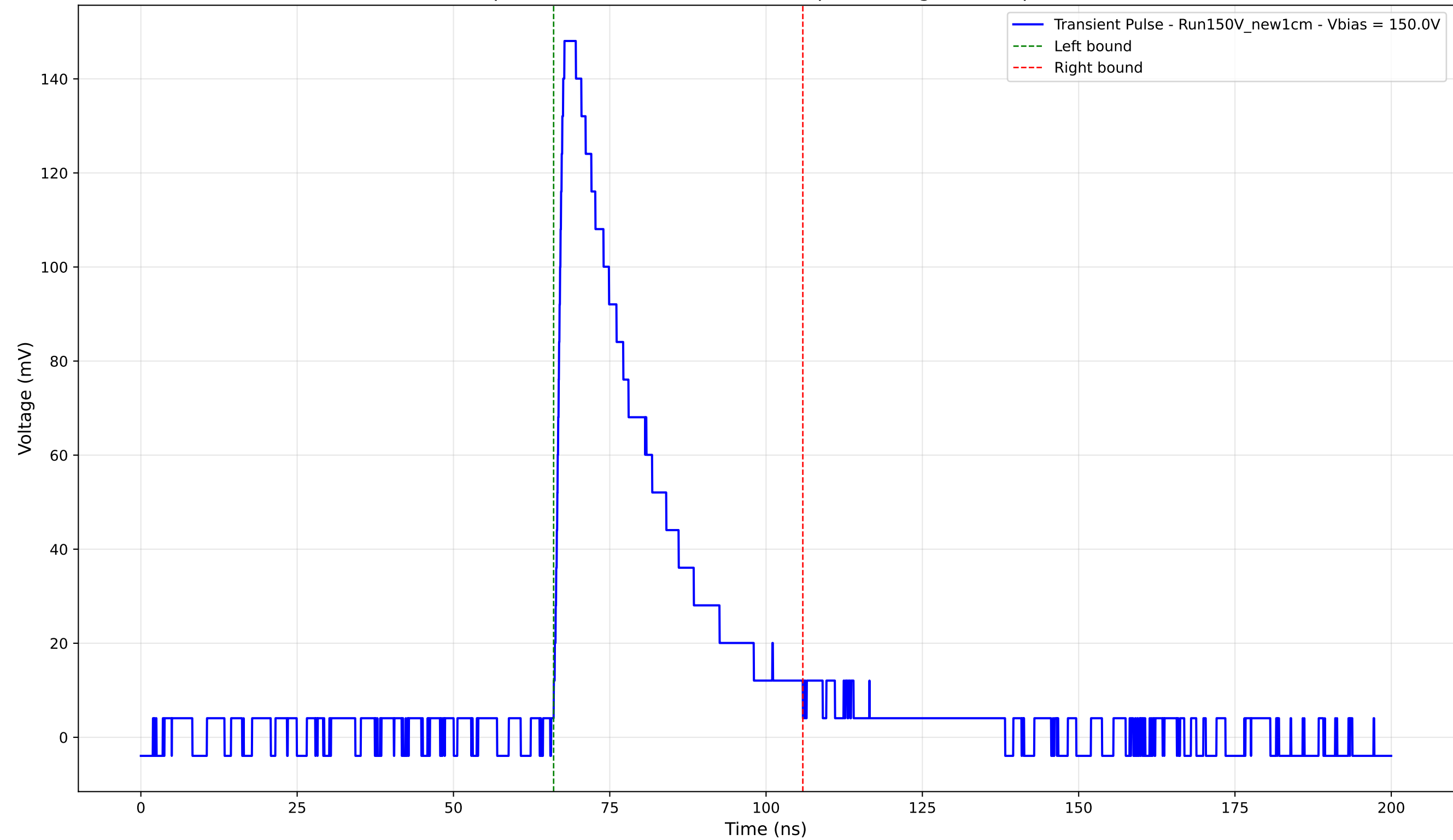
Transient Pulse - Sample: New1cm - Position: 3800.0 \mu\text{m} - Charge: 43.27 pC - Rise Time: 1.35 ns
