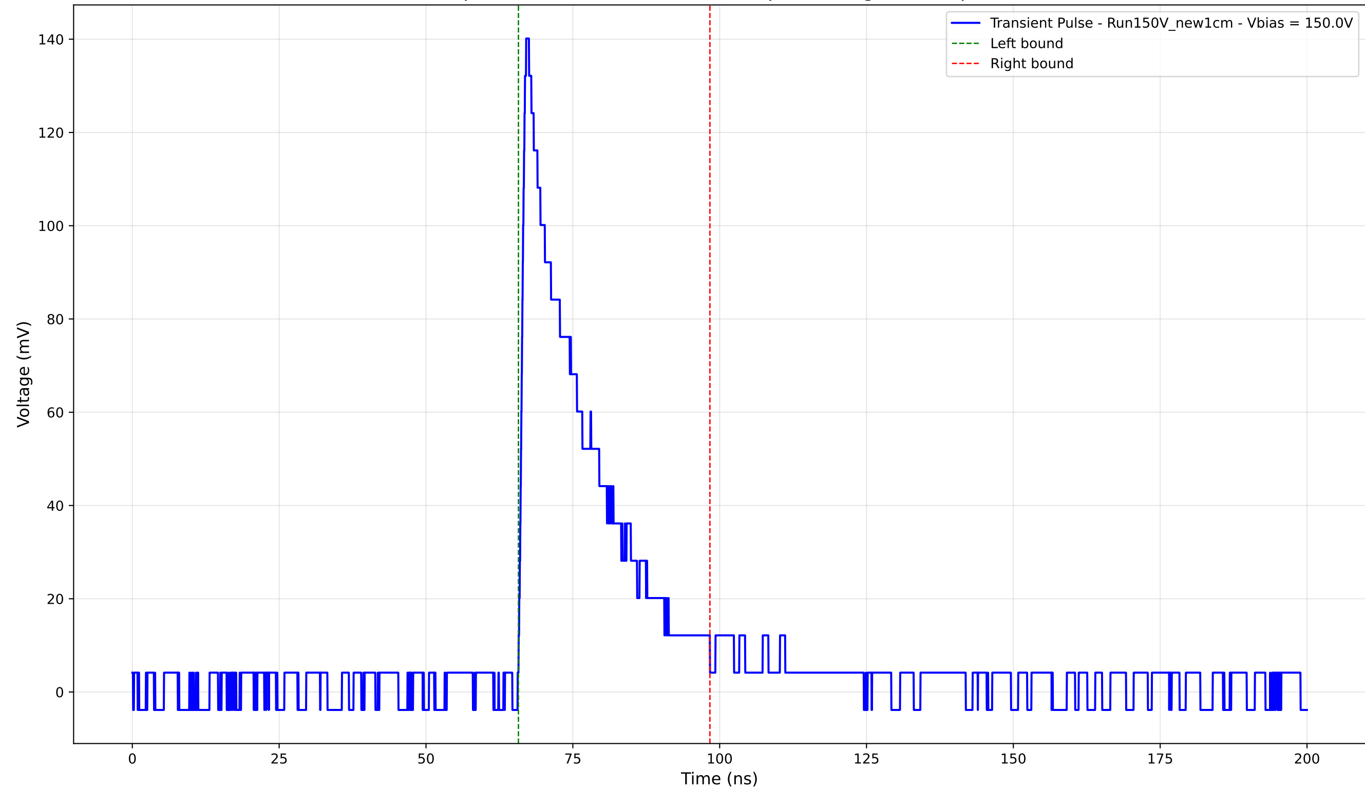
Transient Pulse - Sample: New1cm - Position: 4675.0 \mu\text{m} - Charge: 31.06 pC - Rise Time: 1.00 ns
