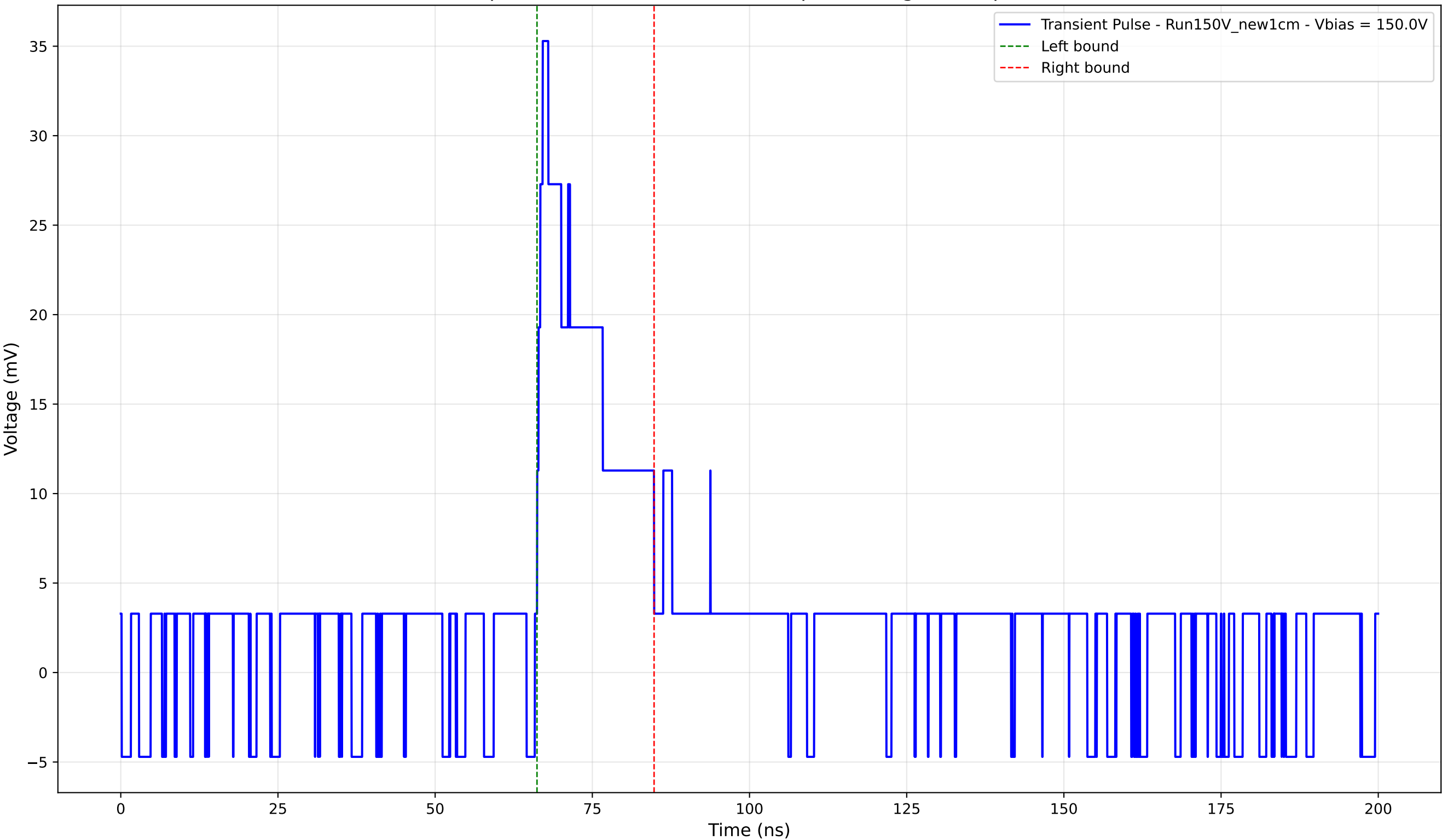
Transient Pulse - Sample: New1cm - Position: 500.0 \mu\text{m} - Charge: 6.54 pC - Rise Time: 0.90 ns
