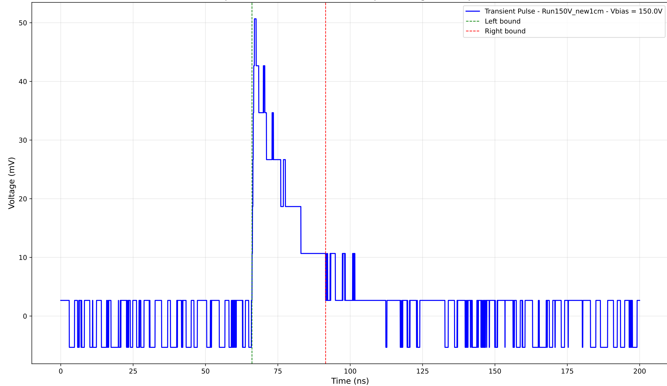
Transient Pulse - Sample: New1cm - Position: 2080.0 \mu\text{m} - Charge: 10.98 pC - Rise Time: 0.83 ns
