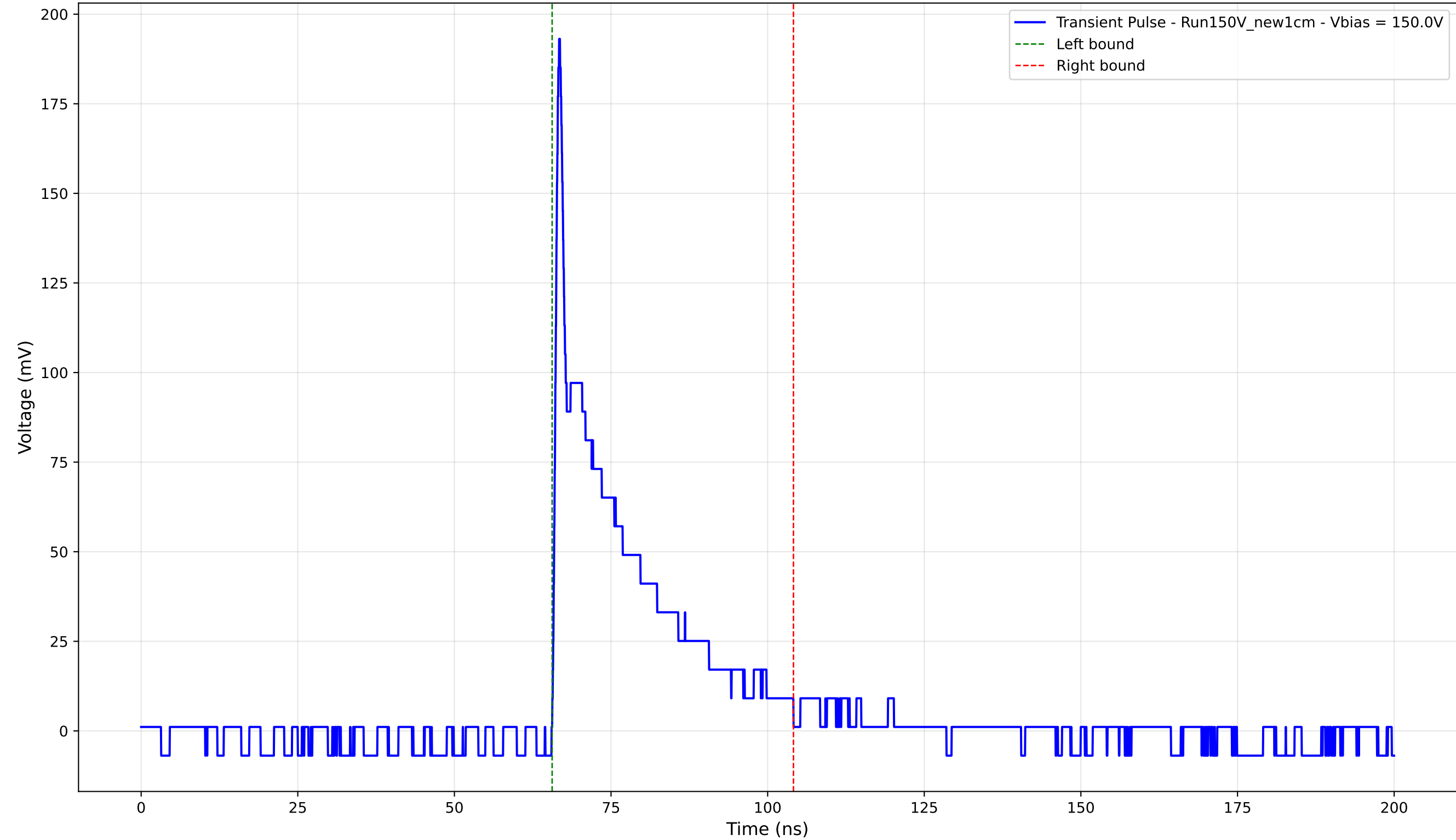
Transient Pulse - Sample: New1cm - Position: 2425.0 \mu\text{m} - Charge: 32.80 pC - Rise Time: 0.77 ns
