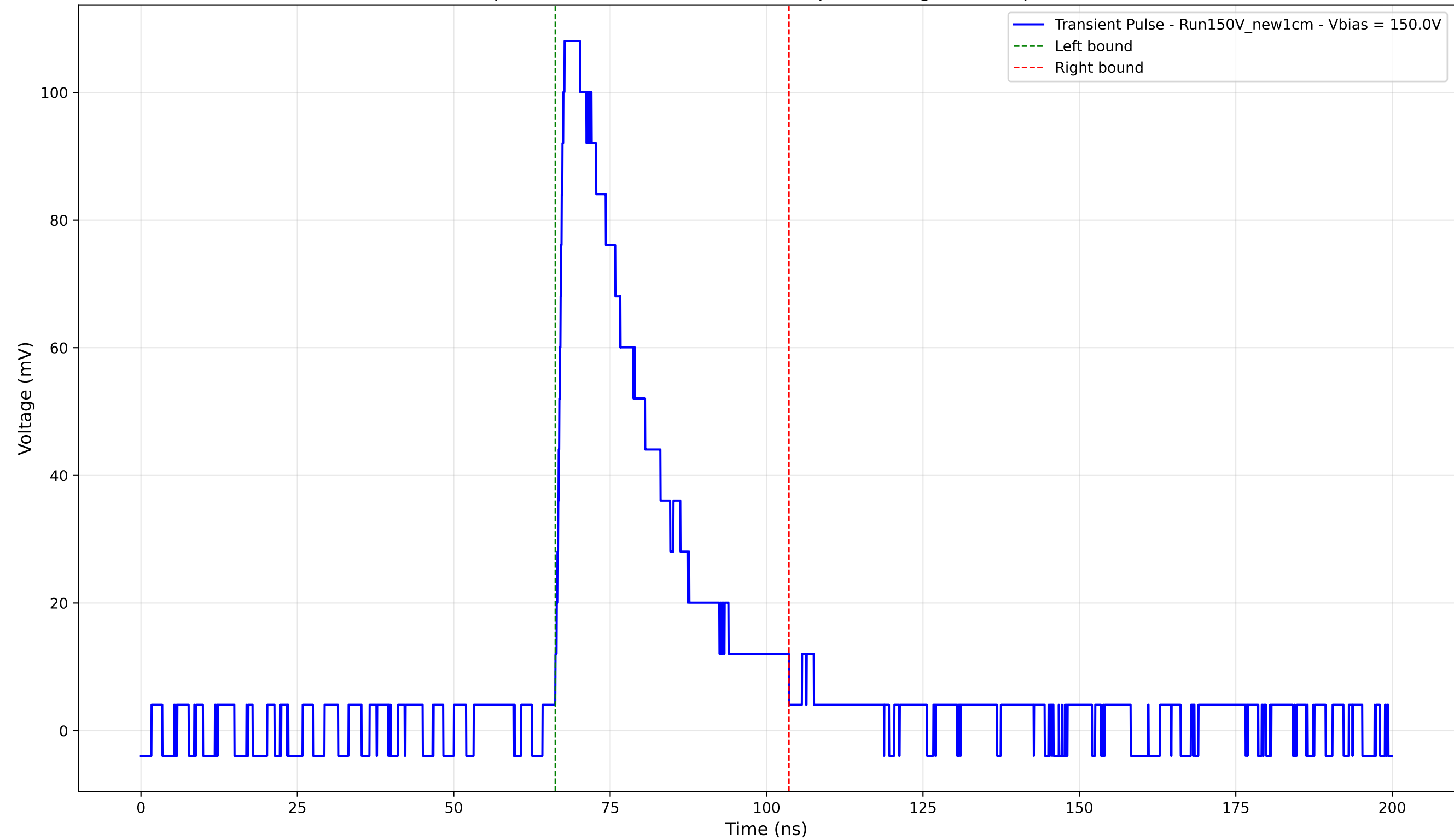
Transient Pulse - Sample: New1cm - Position: 1225.0 \mu\text{m} - Charge: 32.43 pC - Rise Time: 1.26 ns
