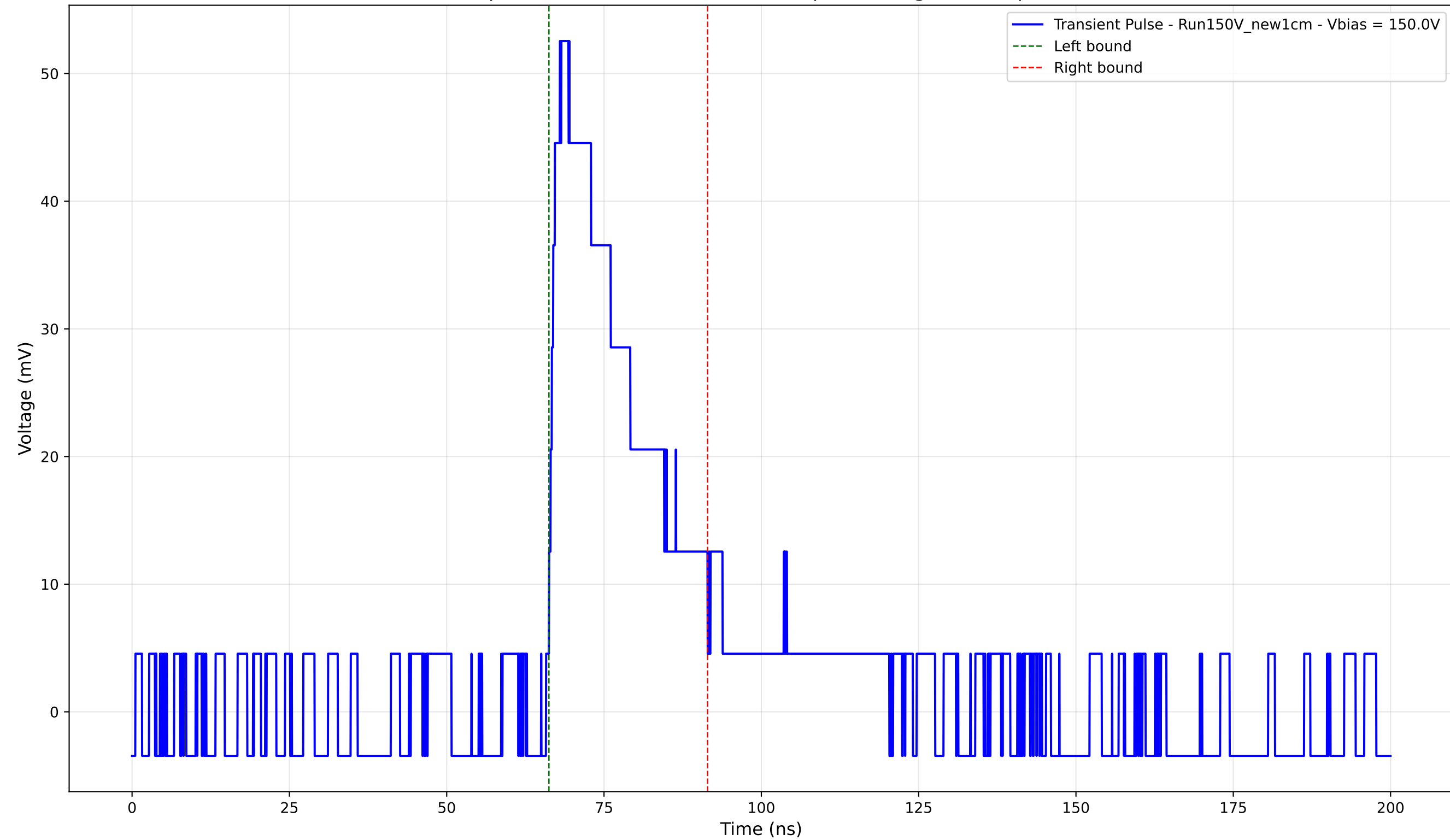
Transient Pulse - Sample: New1cm - Position: 3600.0 \mu\text{m} - Charge: 13.83 pC - Rise Time: 1.74 ns
