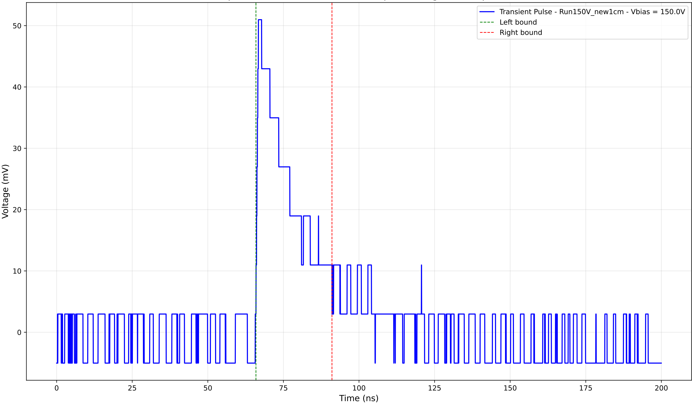
Transient Pulse - Sample: New1cm - Position: 2085.0 \mu\text{m} - Charge: 11.94 pC - Rise Time: 0.79 ns
