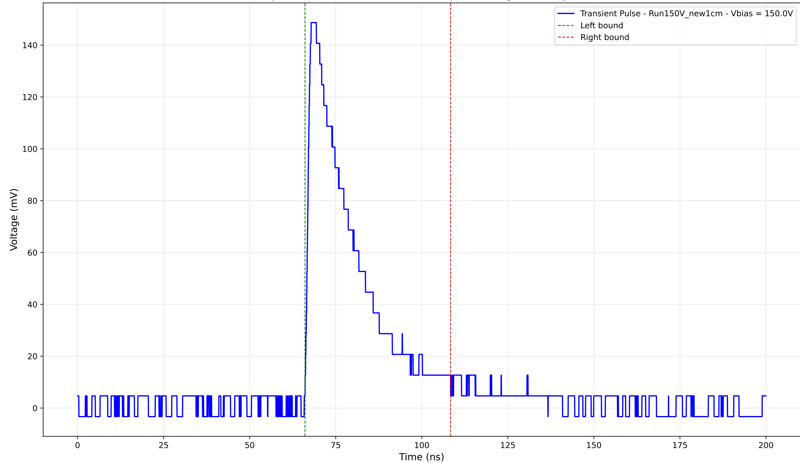
Transient Pulse - Sample: New1cm - Position: 3805.0 \mu\text{m} - Charge: 43.67 pC - Rise Time: 1.39 ns
