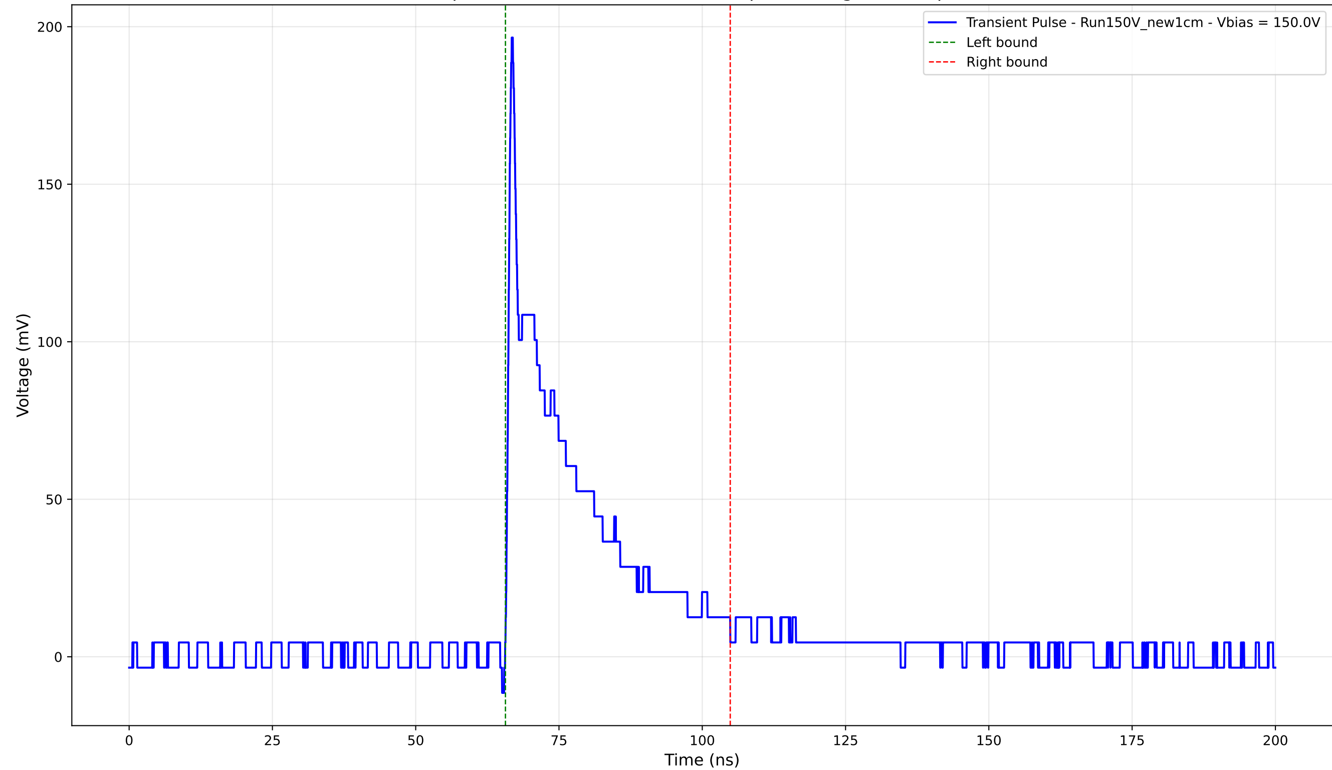
Transient Pulse - Sample: New1cm - Position: 2745.0 \mu\text{m} - Charge: 37.22 pC - Rise Time: 0.82 ns
