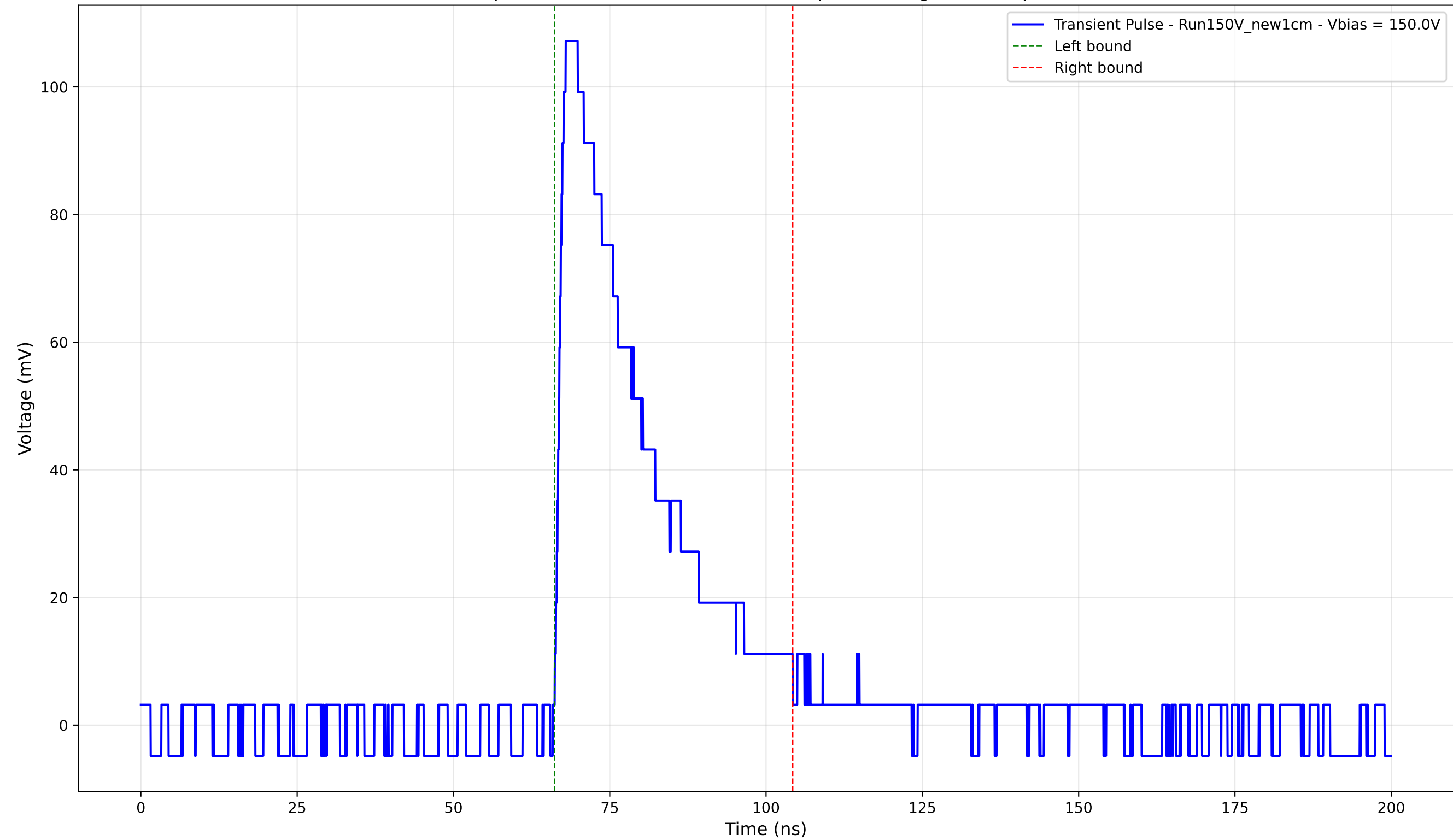
Transient Pulse - Sample: New1cm - Position: 1440.0 \mu\text{m} - Charge: 32.08 pC - Rise Time: 1.42 ns
