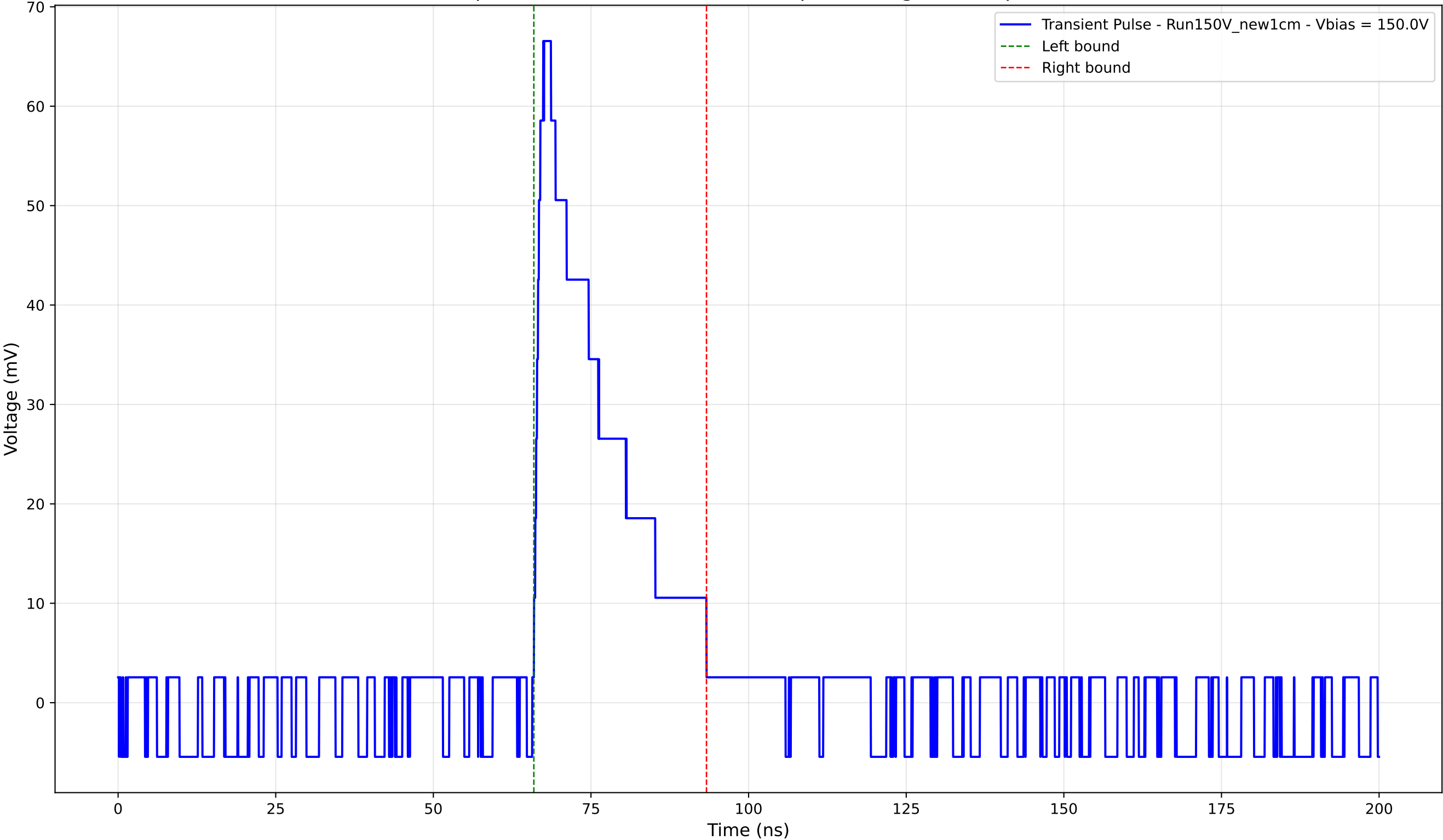
Transient Pulse - Sample: New1cm - Position: 4525.0 \mu\text{m} - Charge: 15.23 pC - Rise Time: 1.47 ns
