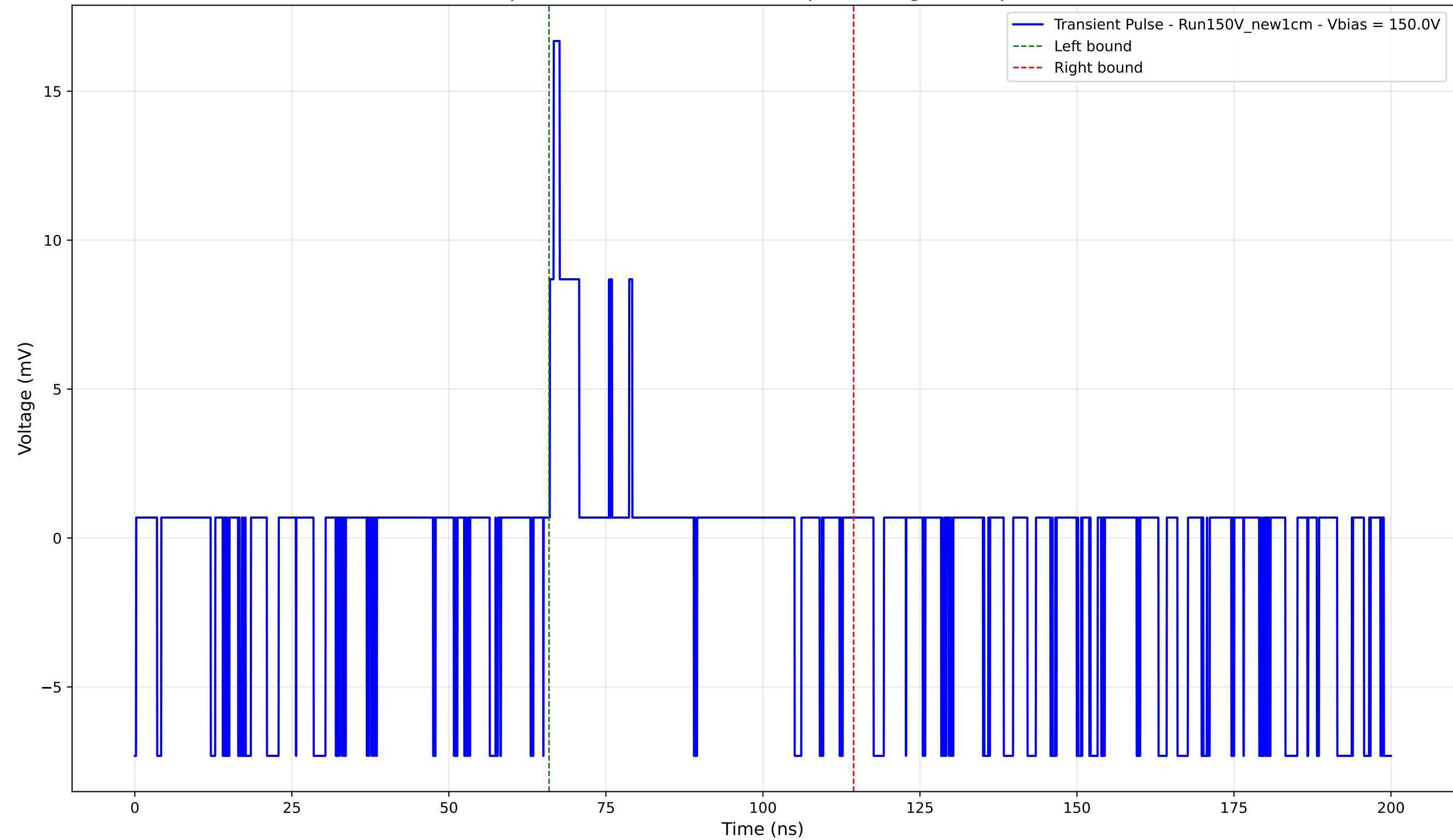
Transient Pulse - Sample: New1cm - Position: 30.0 \mu\text{m} - Charge: 1.33 pC - Rise Time: 0.62 ns
