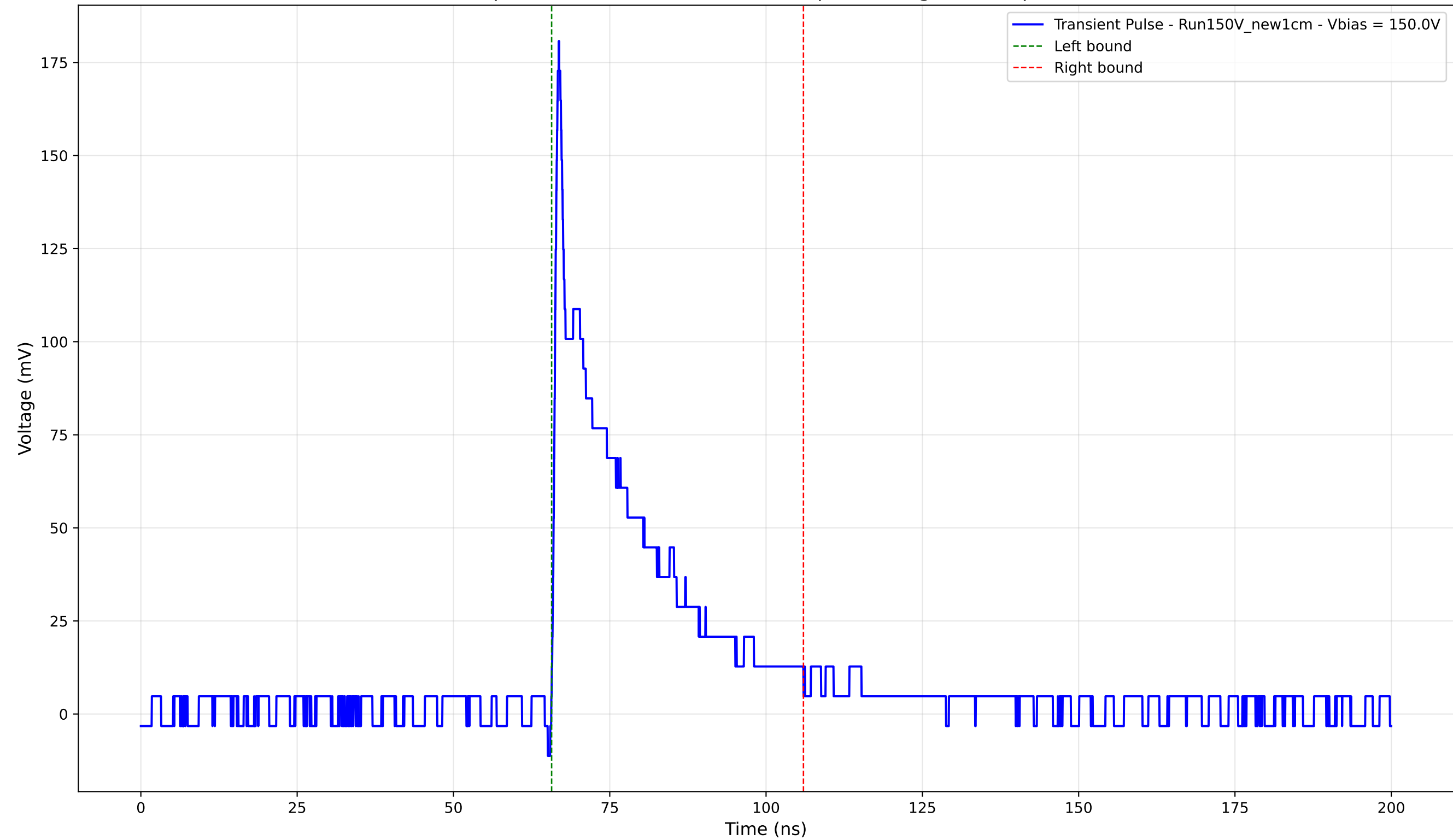
Transient Pulse - Sample: New1cm - Position: 2320.0 \mu\text{m} - Charge: 36.25 pC - Rise Time: 0.83 ns
