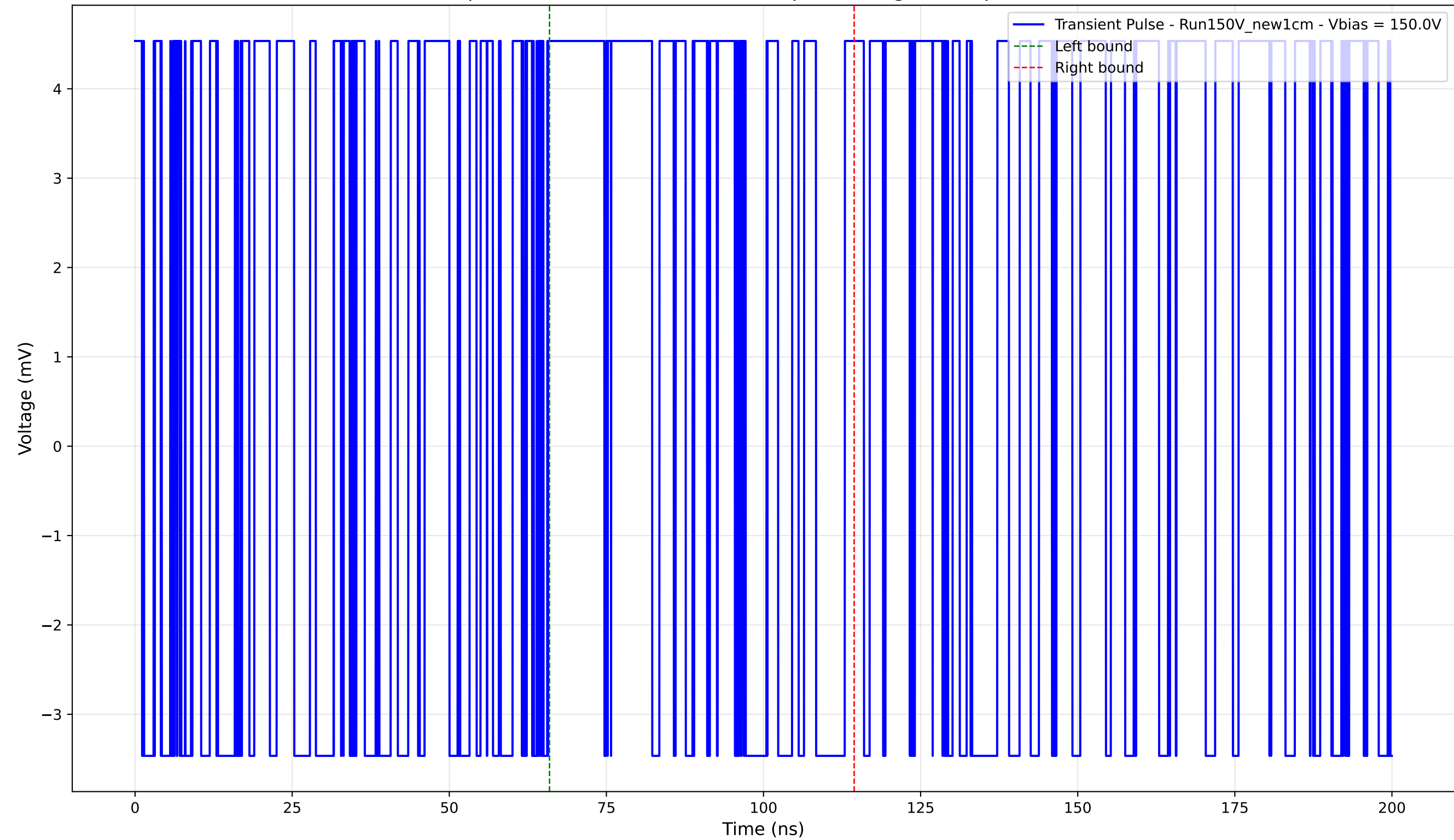
Transient Pulse - Sample: New1cm - Position: 4930.0 \mu\text{m} - Charge: 1.96 pC - Rise Time: 0.00 ns (N/A)
