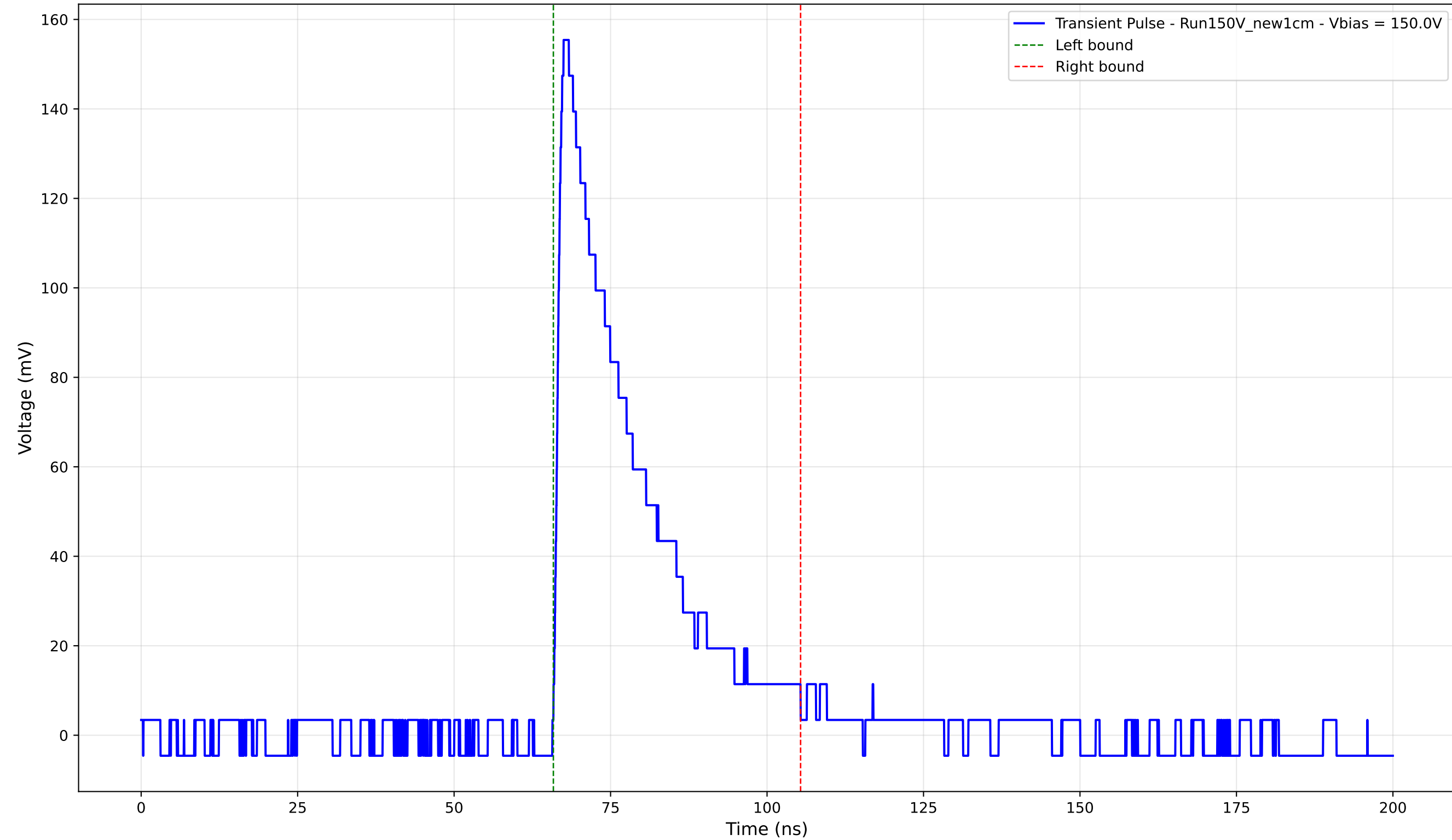
Transient Pulse - Sample: New1cm - Position: 4395.0 \mu\text{m} - Charge: 40.12 pC - Rise Time: 1.27 ns
