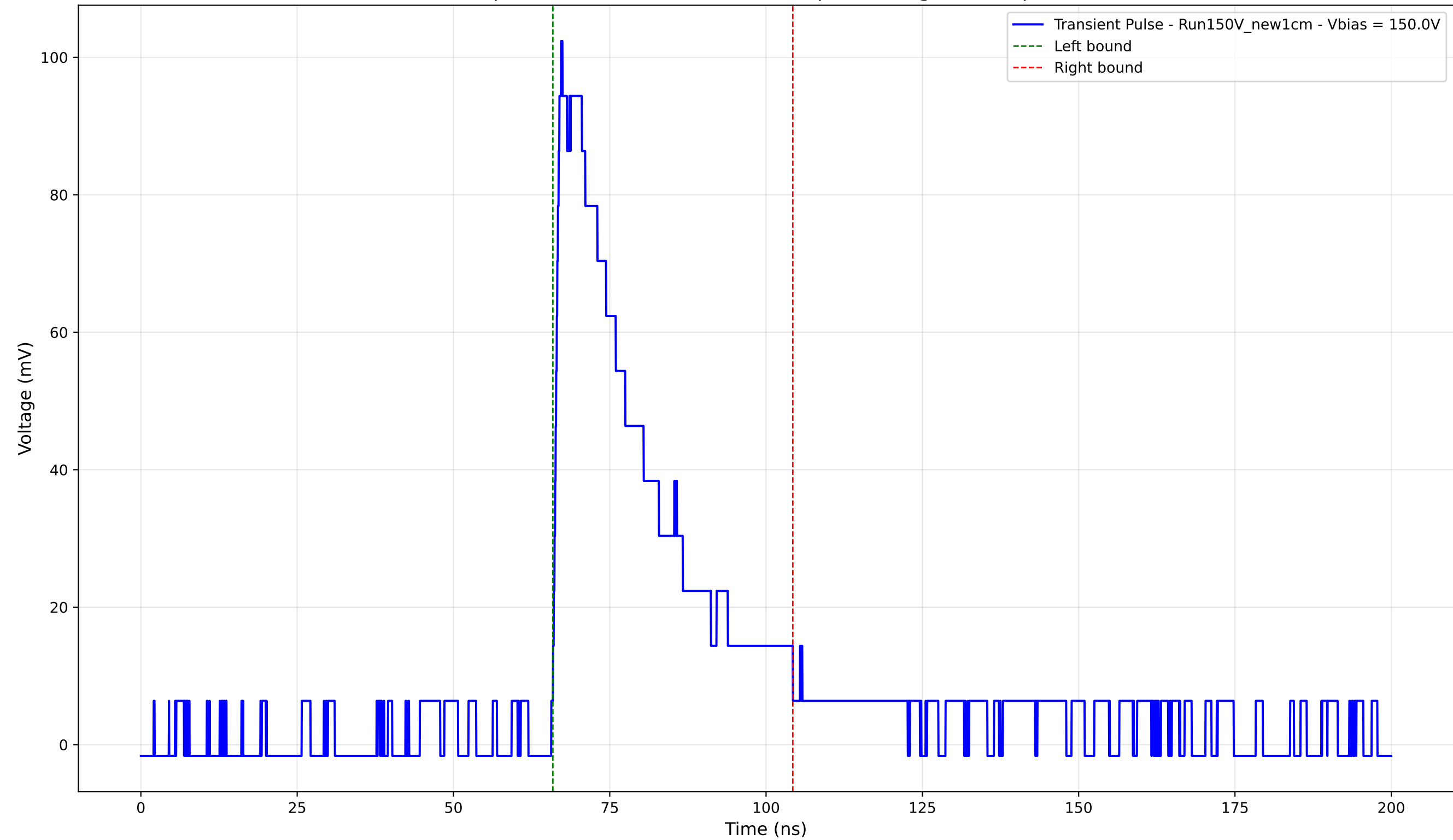
Transient Pulse - Sample: New1cm - Position: 1920.0 \mu\text{m} - Charge: 30.34 pC - Rise Time: 1.03 ns
