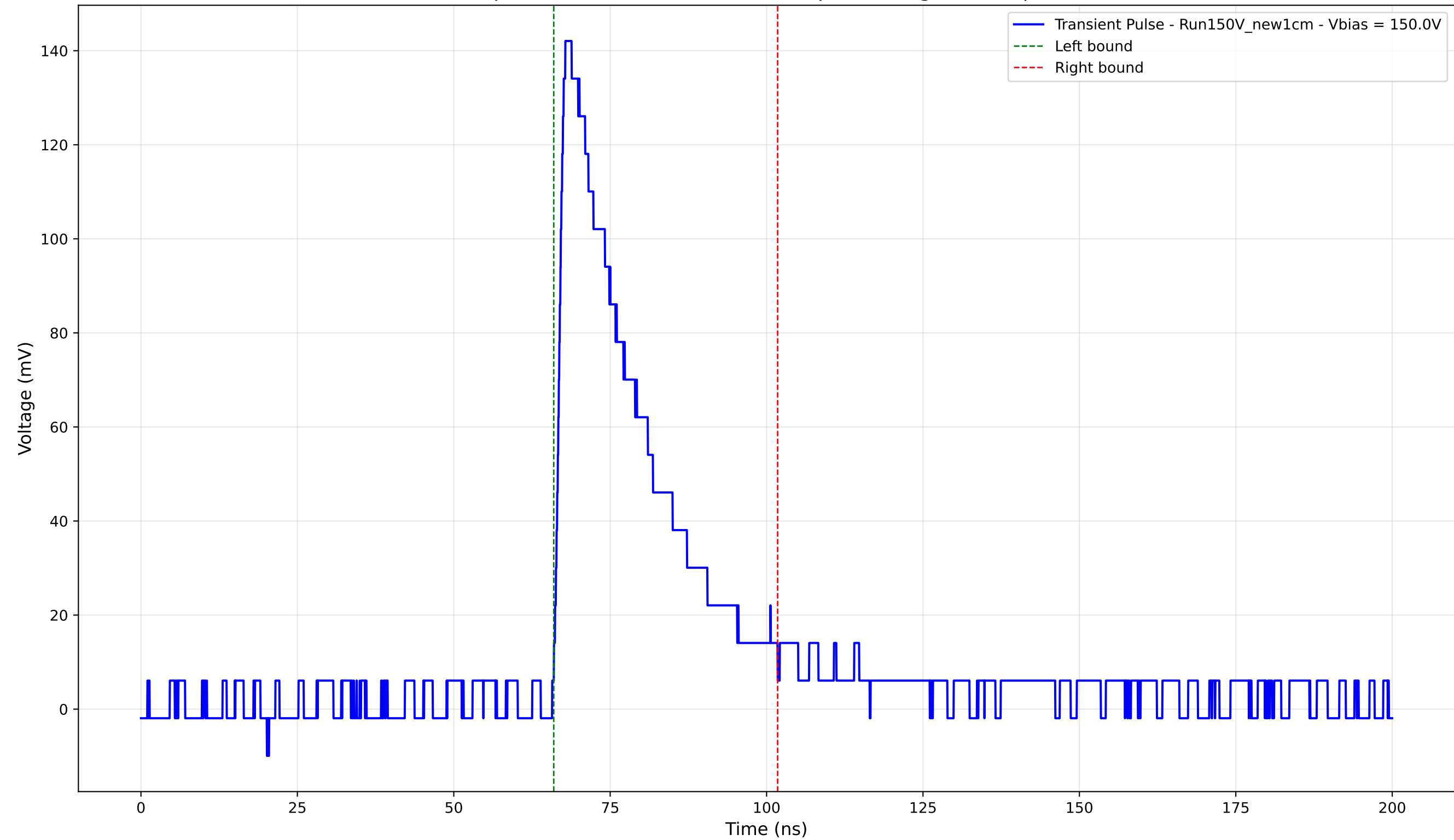
Transient Pulse - Sample: New1cm - Position: 3960.0 \mu\text{m} - Charge: 39.72 pC - Rise Time: 1.40 ns
