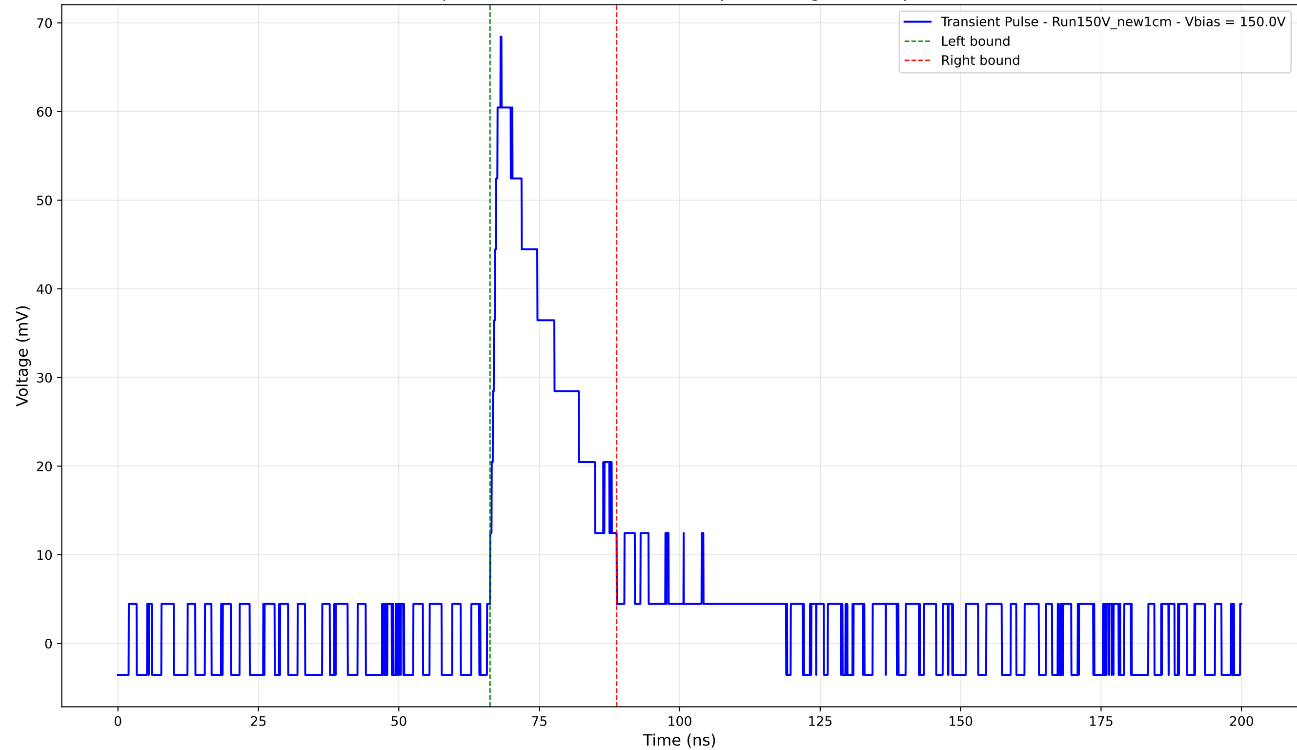
Transient Pulse - Sample: New1cm - Position: 980.0 \mu\text{m} - Charge: 15.27 pC - Rise Time: 1.85 ns
