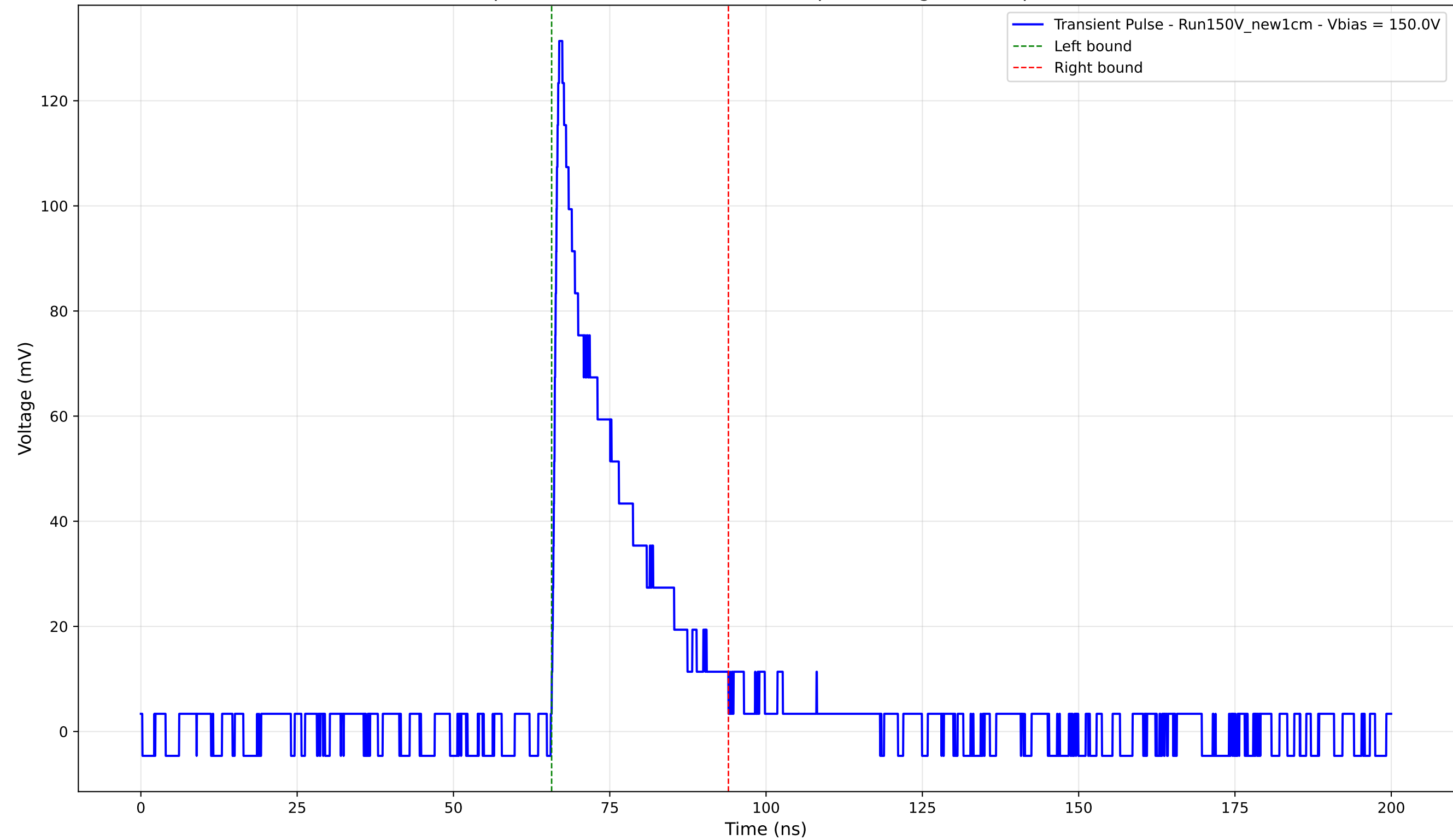
Transient Pulse - Sample: New1cm - Position: 4815.0 \mu\text{m} - Charge: 24.88 pC - Rise Time: 0.94 ns
