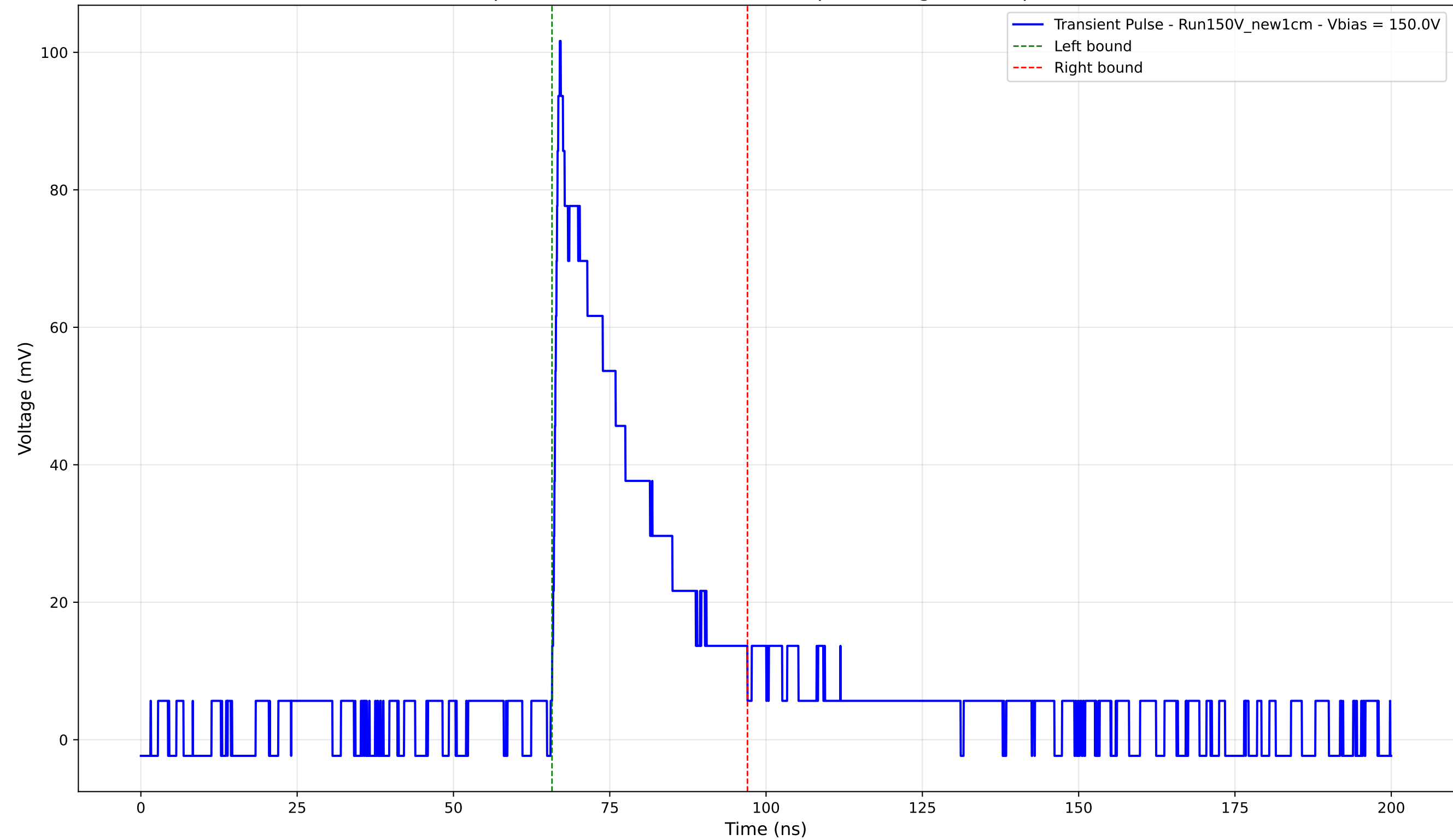
Transient Pulse - Sample: New1cm - Position: 2120.0 \mu\text{m} - Charge: 24.00 pC - Rise Time: 0.99 ns
