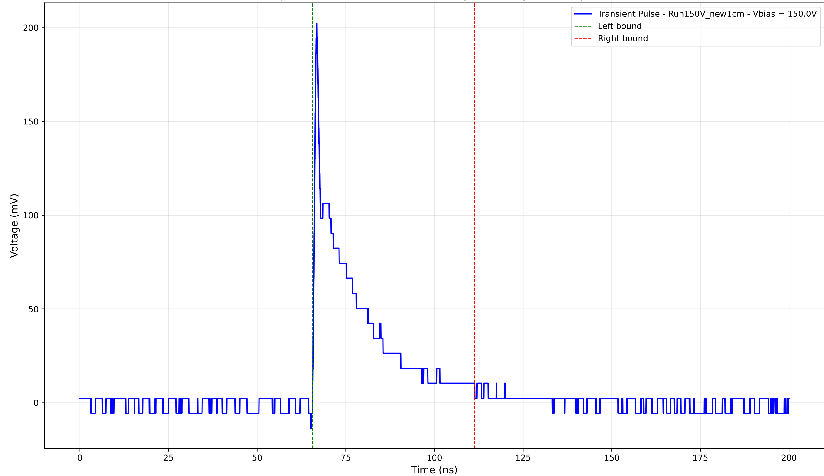
Transient Pulse - Sample: New1cm - Position: 2690.0 \mu\text{m} - Charge: 37.25 pC - Rise Time: 0.78 ns
