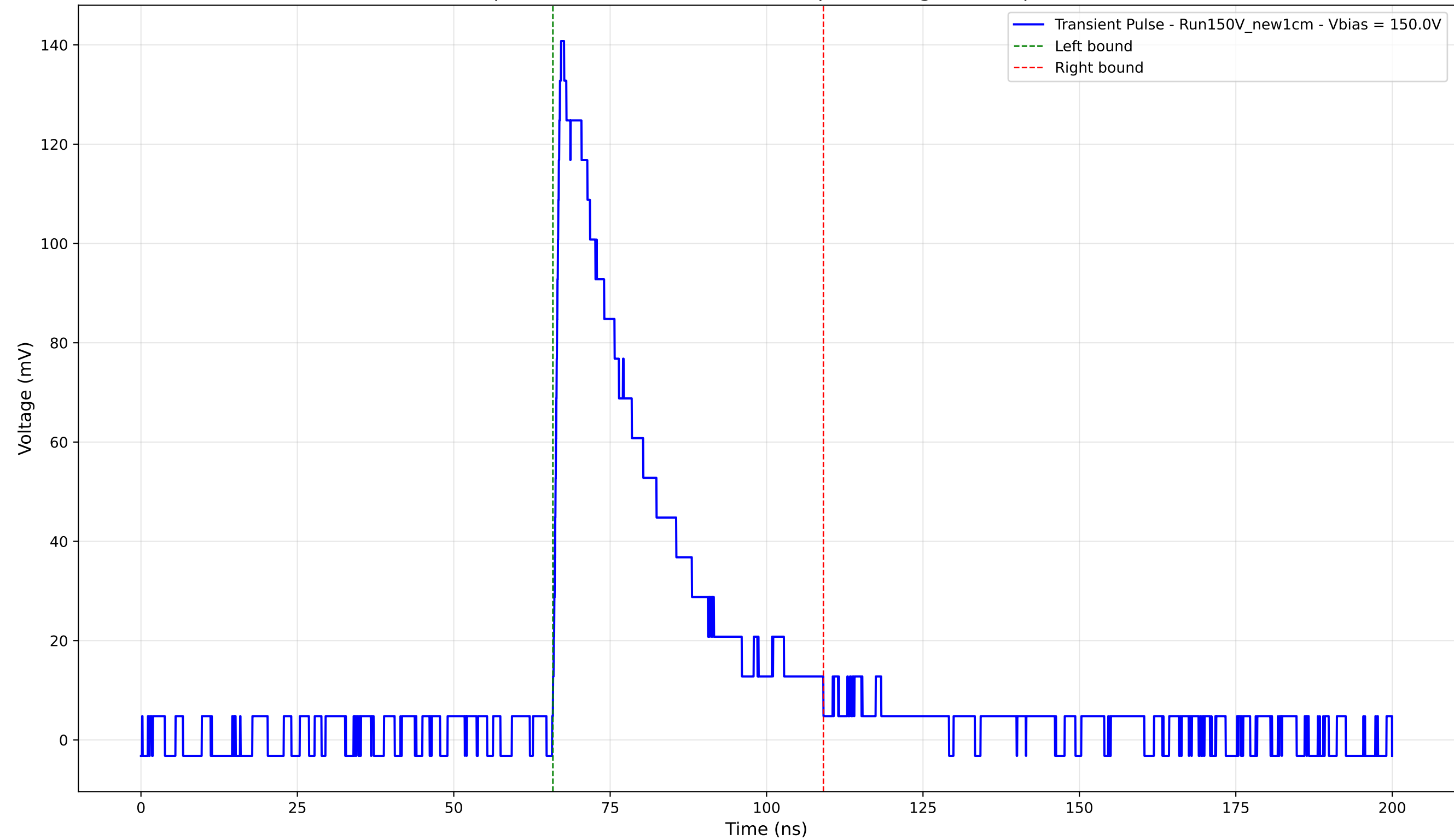
Transient Pulse - Sample: New1cm - Position: 3170.0 \mu\text{m} - Charge: 41.29 pC - Rise Time: 1.02 ns
