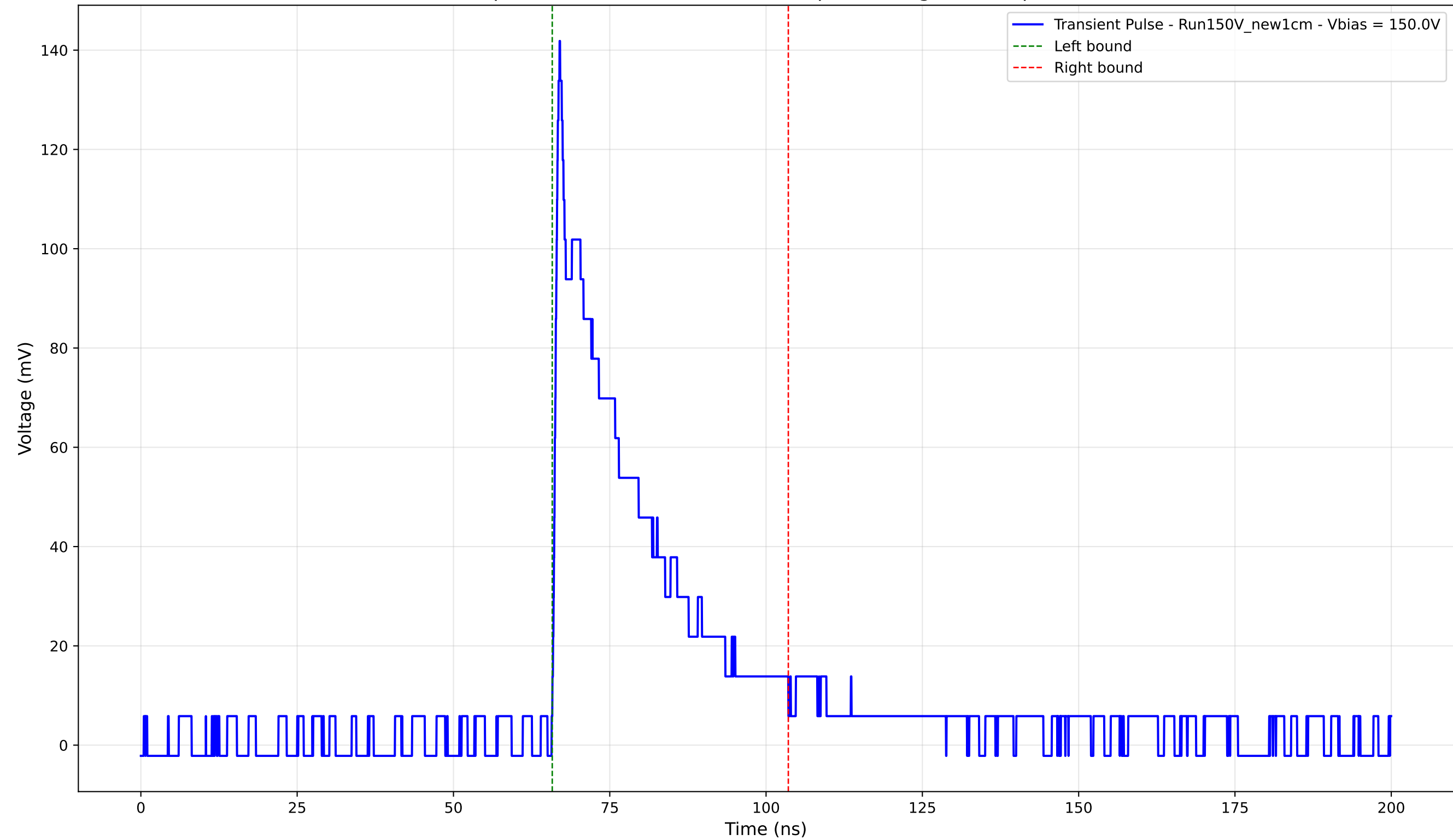
Transient Pulse - Sample: New1cm - Position: 2170.0 \mu\text{m} - Charge: 33.11 pC - Rise Time: 0.90 ns
