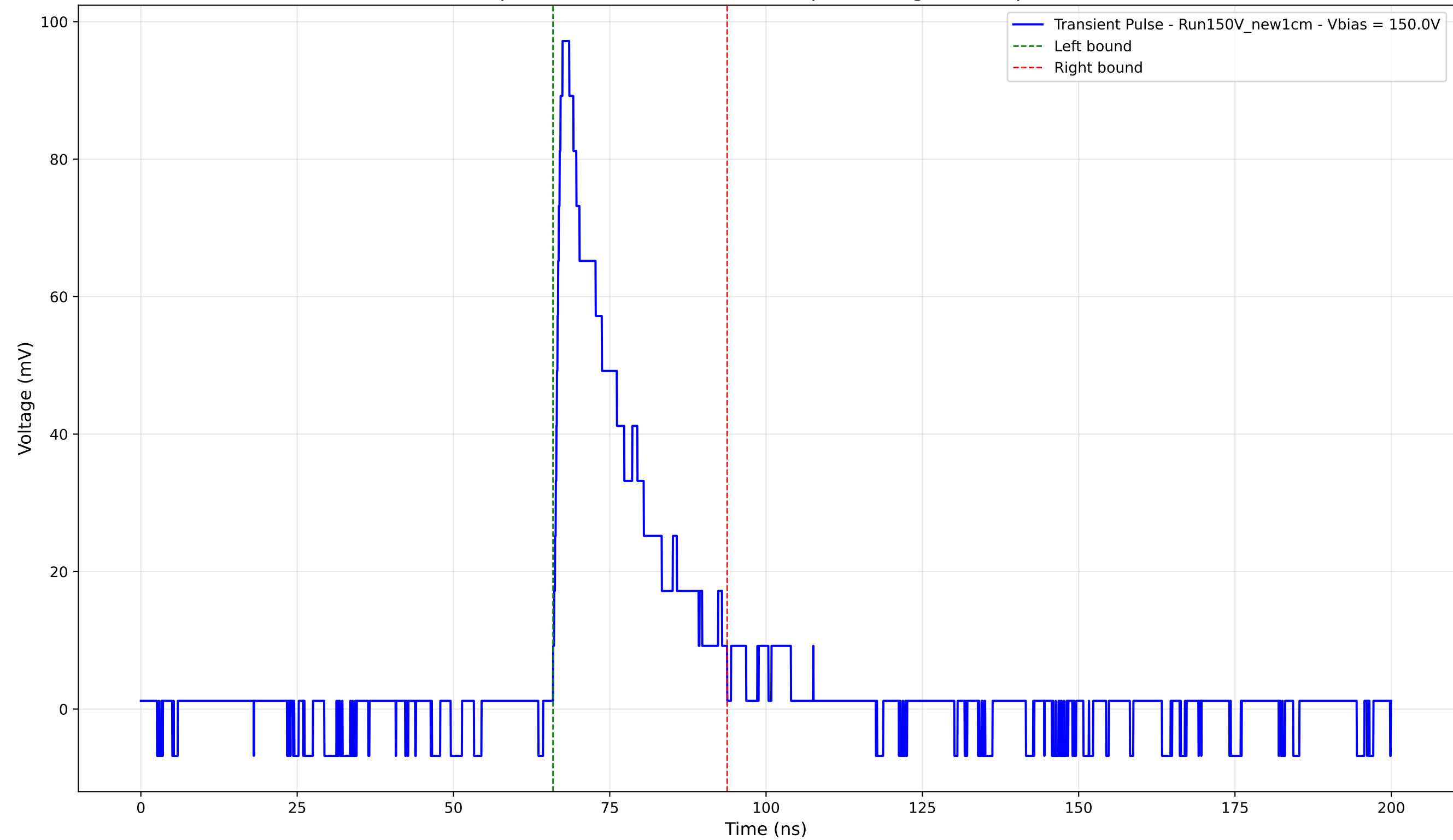
Transient Pulse - Sample: New1cm - Position: 450.0 \mu\text{m} - Charge: 21.04 pC - Rise Time: 1.04 ns
