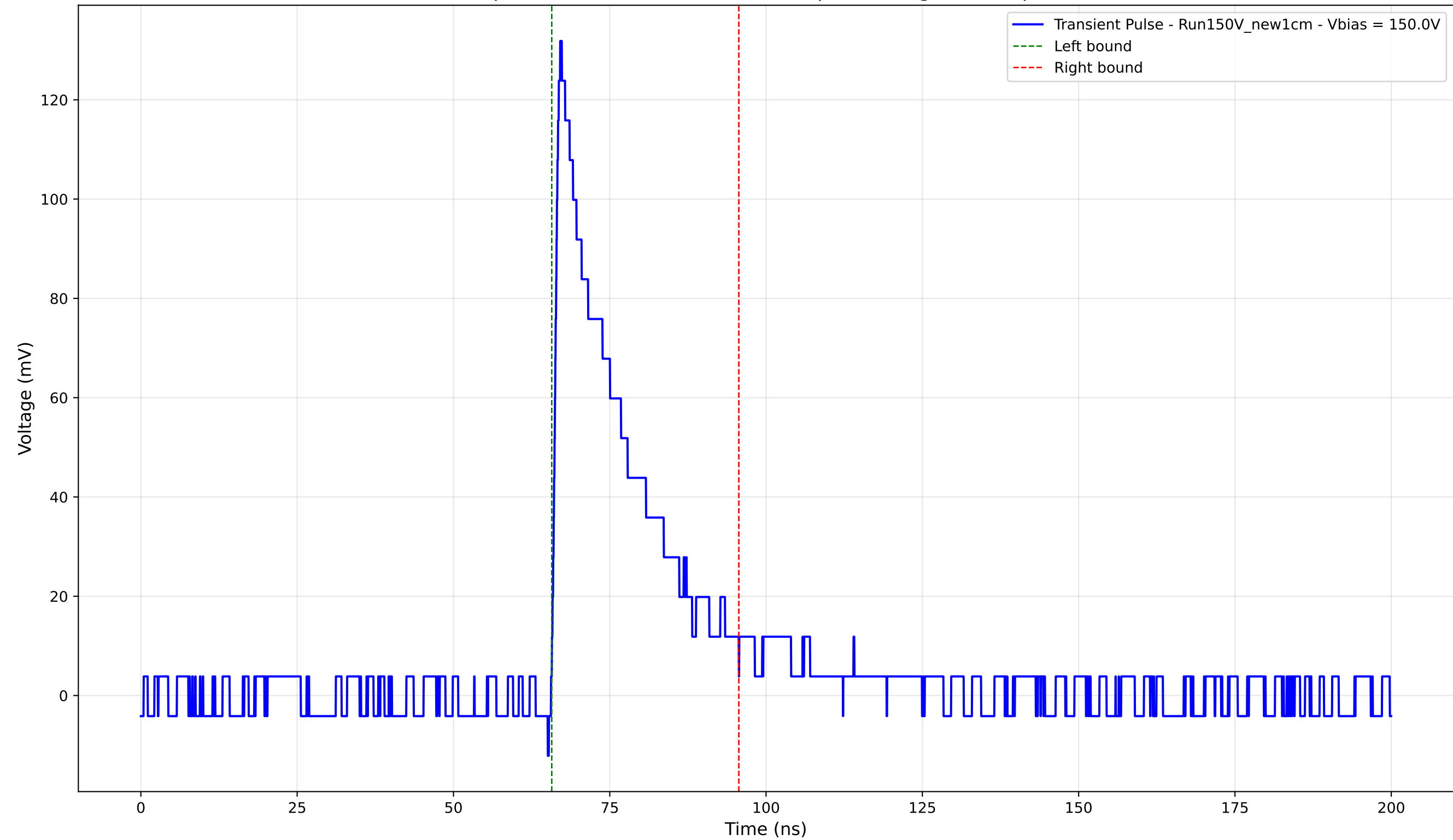
Transient Pulse - Sample: New1cm - Position: 4670.0 \mu\text{m} - Charge: 28.60 pC - Rise Time: 1.02 ns
