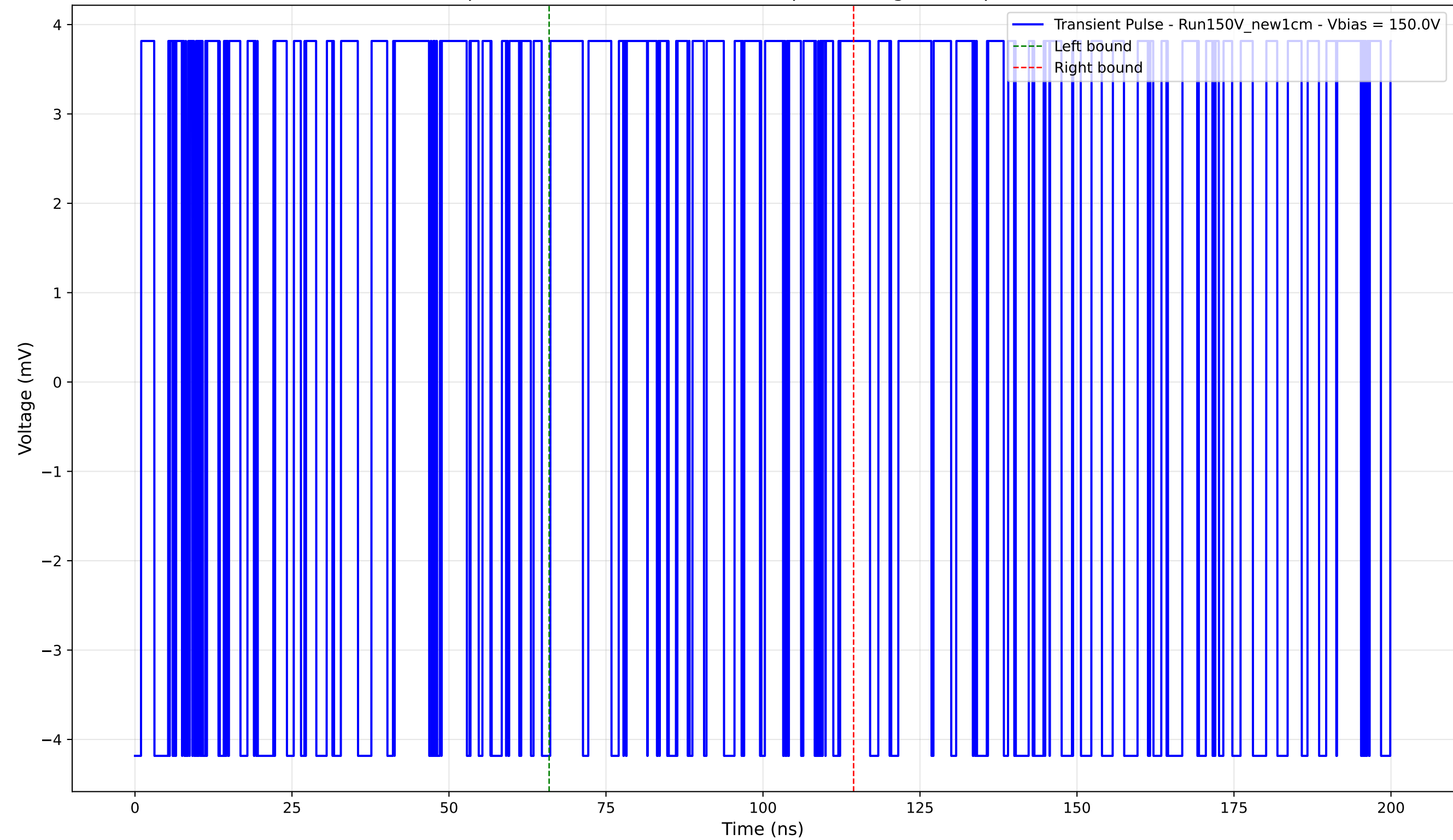
Transient Pulse - Sample: New1cm - Position: 4955.0 \mu\text{m} - Charge: 1.95 pC - Rise Time: 0.00 ns (N/A)
