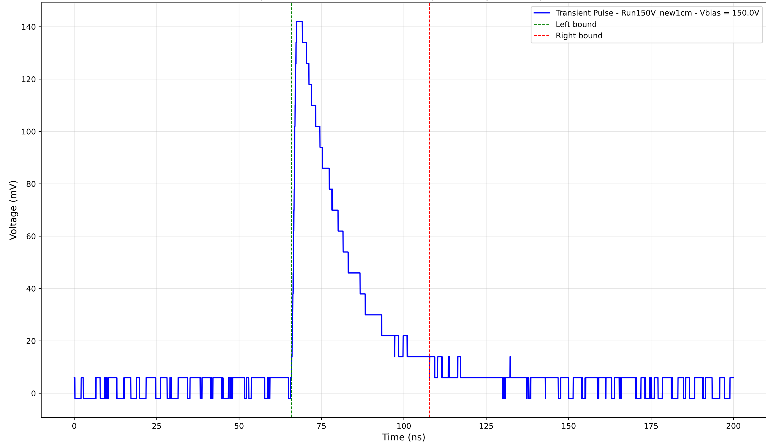
Transient Pulse - Sample: New1cm - Position: 3440.0 \mu\text{m} - Charge: 44.68 pC - Rise Time: 1.20 ns
