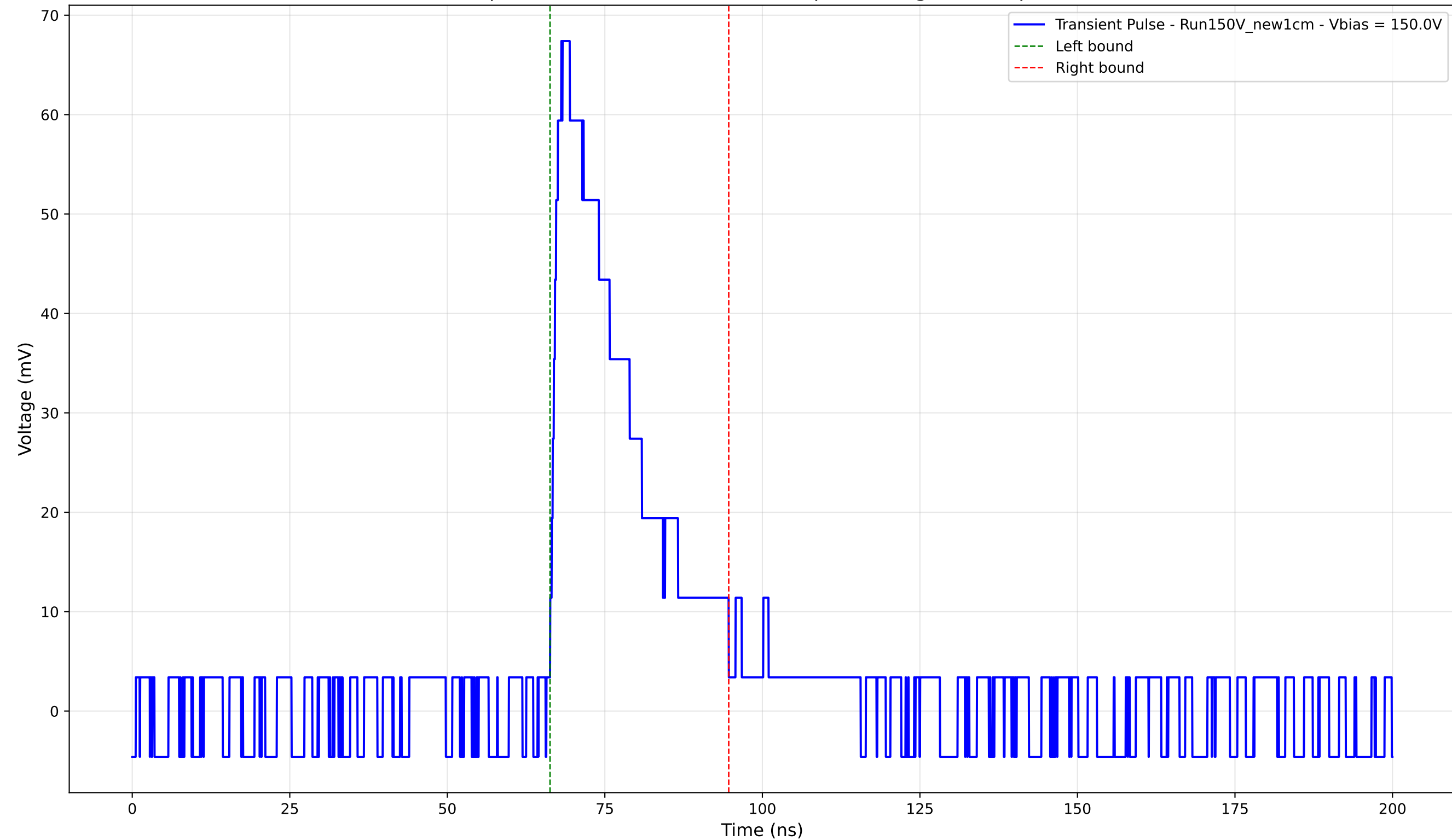
Transient Pulse - Sample: New1cm - Position: 1095.0 \mu\text{m} - Charge: 17.15 pC - Rise Time: 1.77 ns
