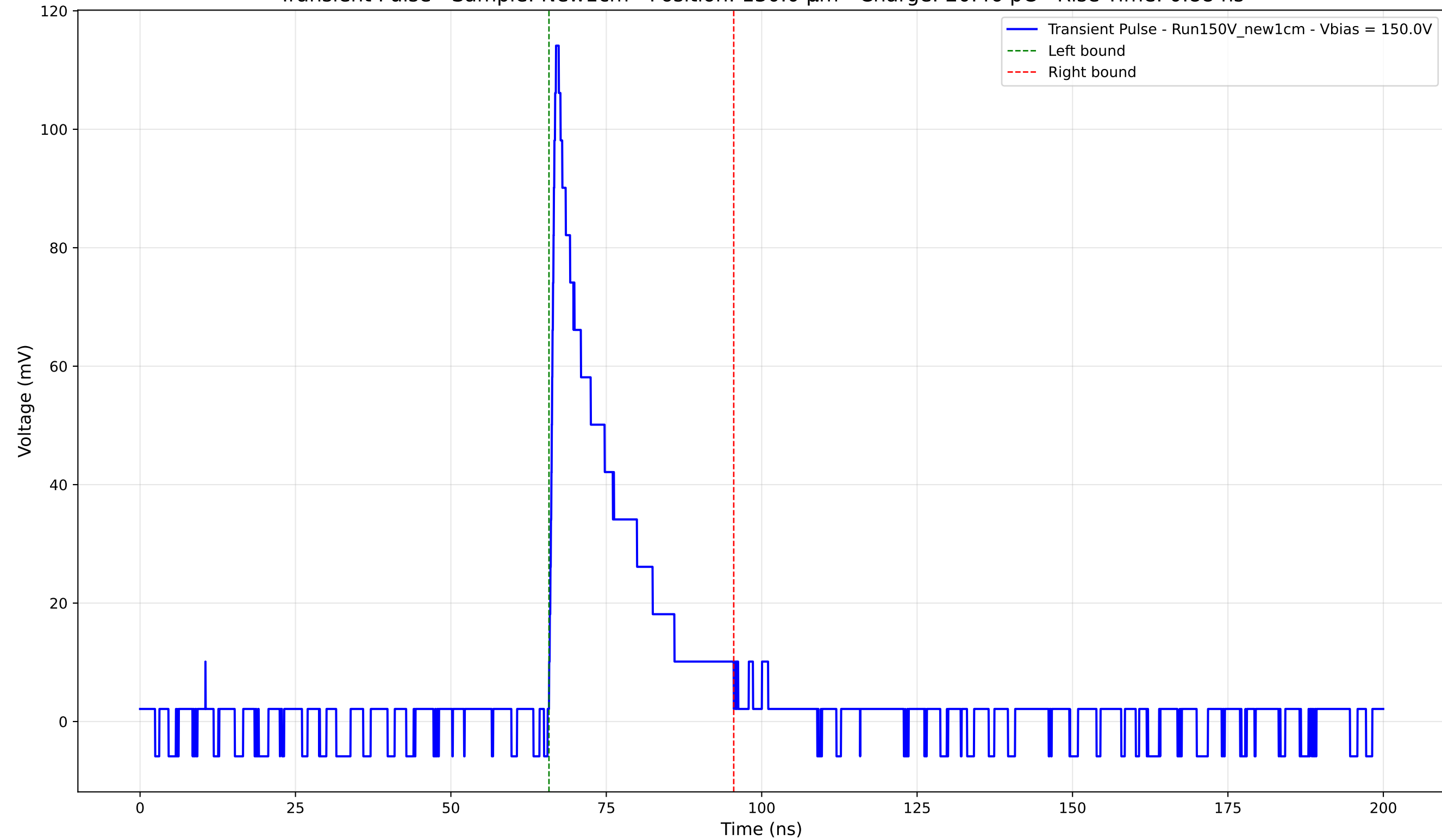
Transient Pulse - Sample: New1cm - Position: 130.0 \mu\text{m} - Charge: 20.46 pC - Rise Time: 0.88 ns
