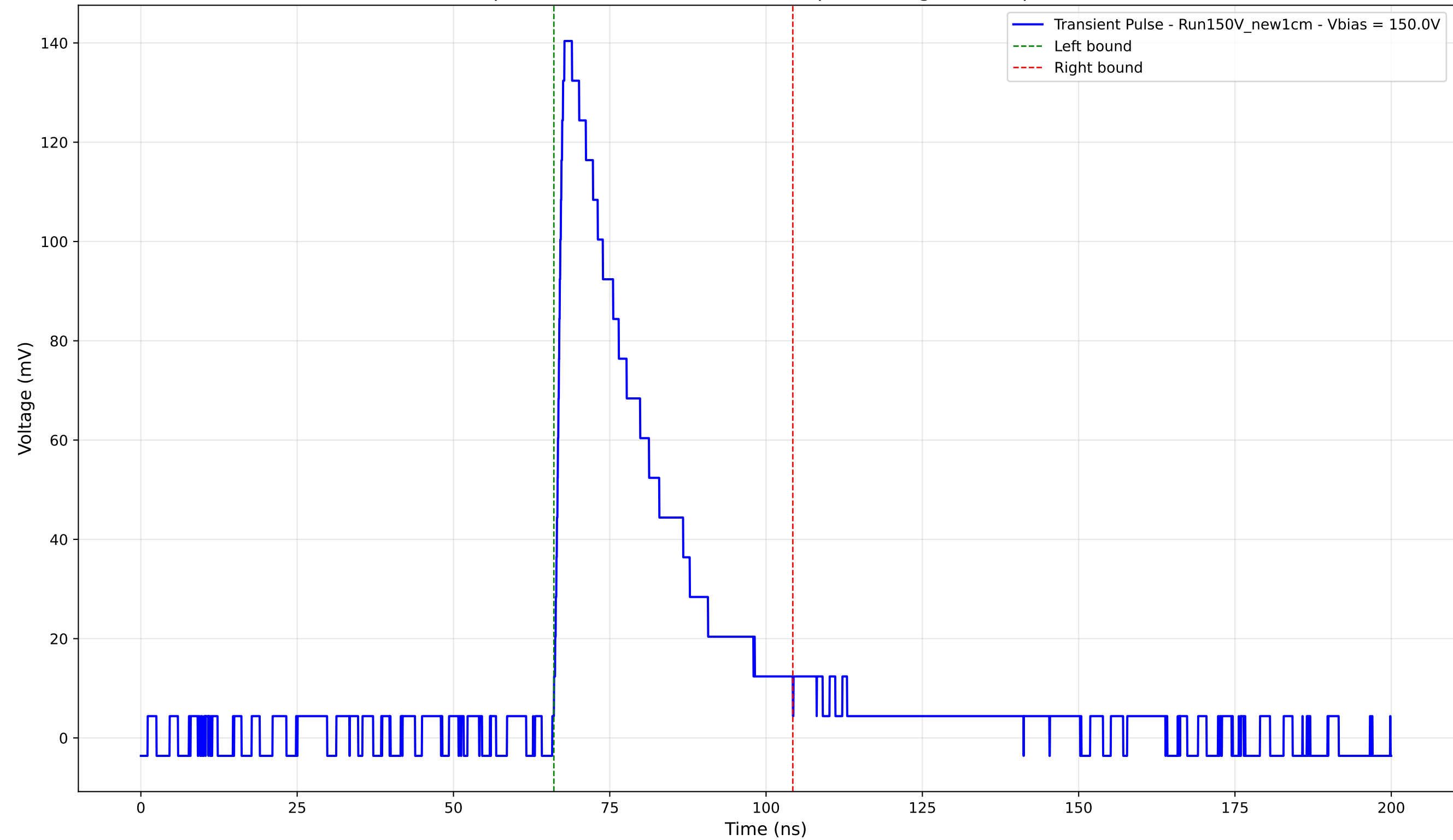
Transient Pulse - Sample: New1cm - Position: 3720.0 \mu\text{m} - Charge: 40.82 pC - Rise Time: 1.28 ns
