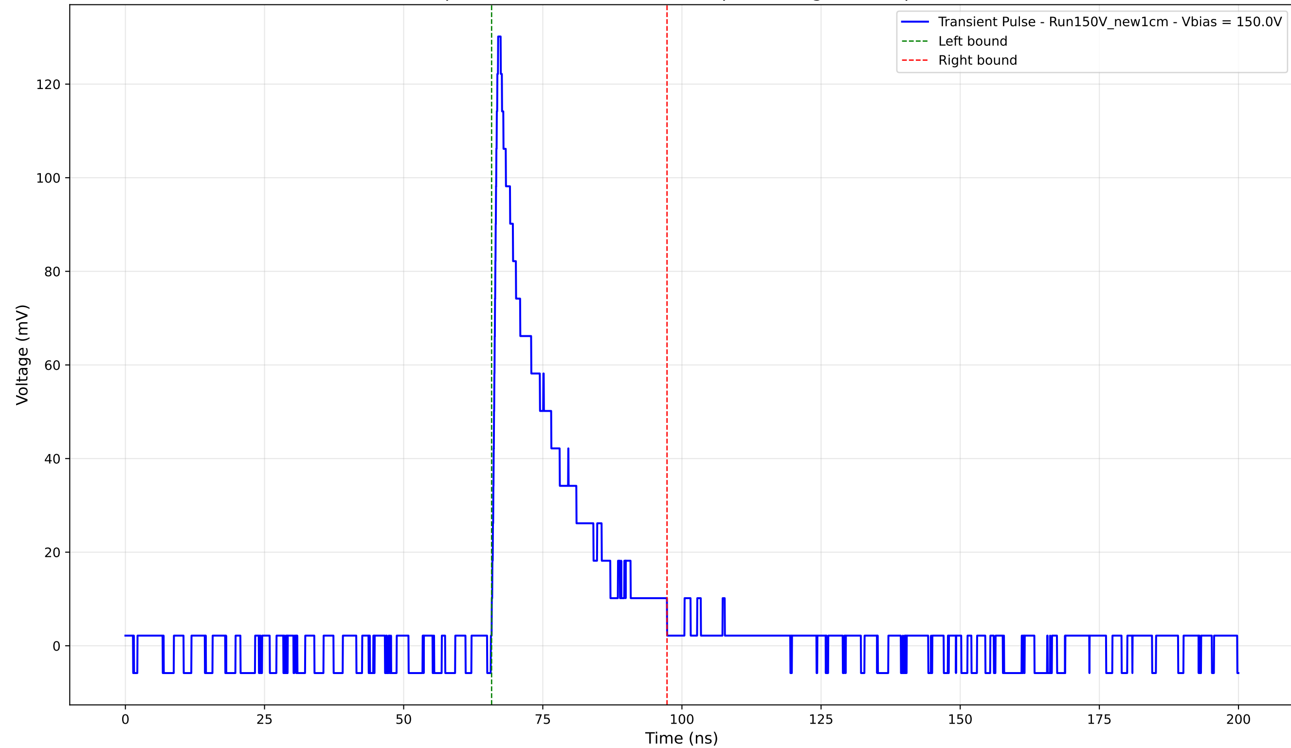
Transient Pulse - Sample: New1cm - Position: 170.0 \mu\text{m} - Charge: 24.31 pC - Rise Time: 0.91 ns
