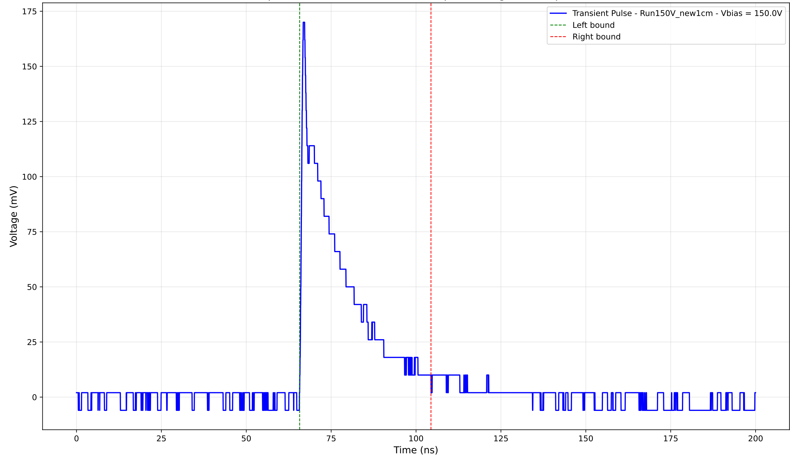
Transient Pulse - Sample: New1cm - Position: 2875.0 \mu\text{m} - Charge: 36.93 pC - Rise Time: 0.80 ns
