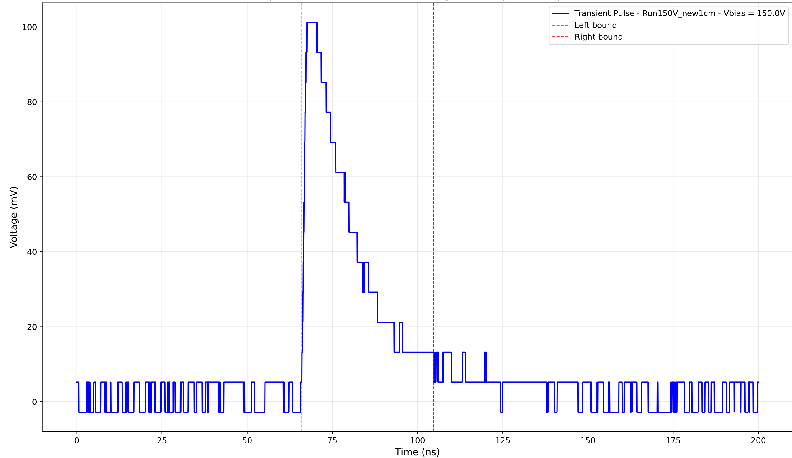
Transient Pulse - Sample: New1cm - Position: 1660.0 \mu\text{m} - Charge: 32.47 pC - Rise Time: 1.21 ns
