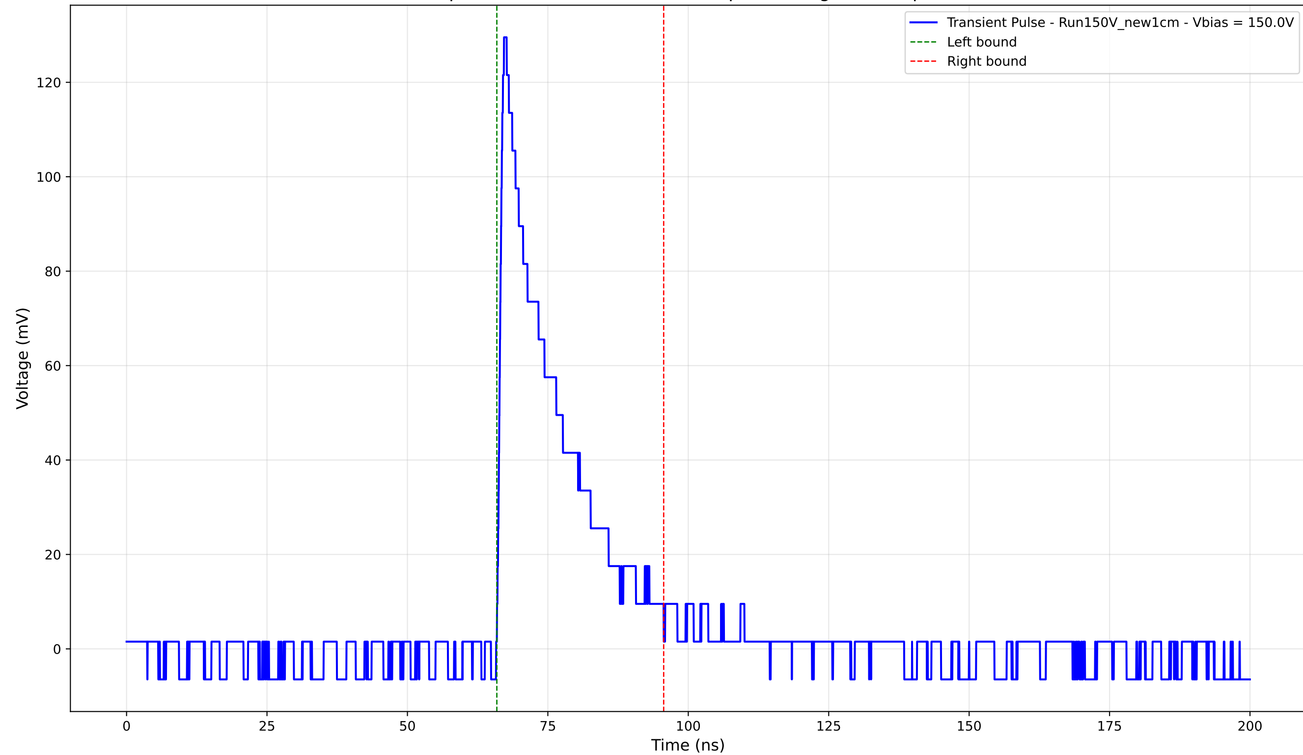
Transient Pulse - Sample: New1cm - Position: 310.0 \mu\text{m} - Charge: 26.29 pC - Rise Time: 0.97 ns
