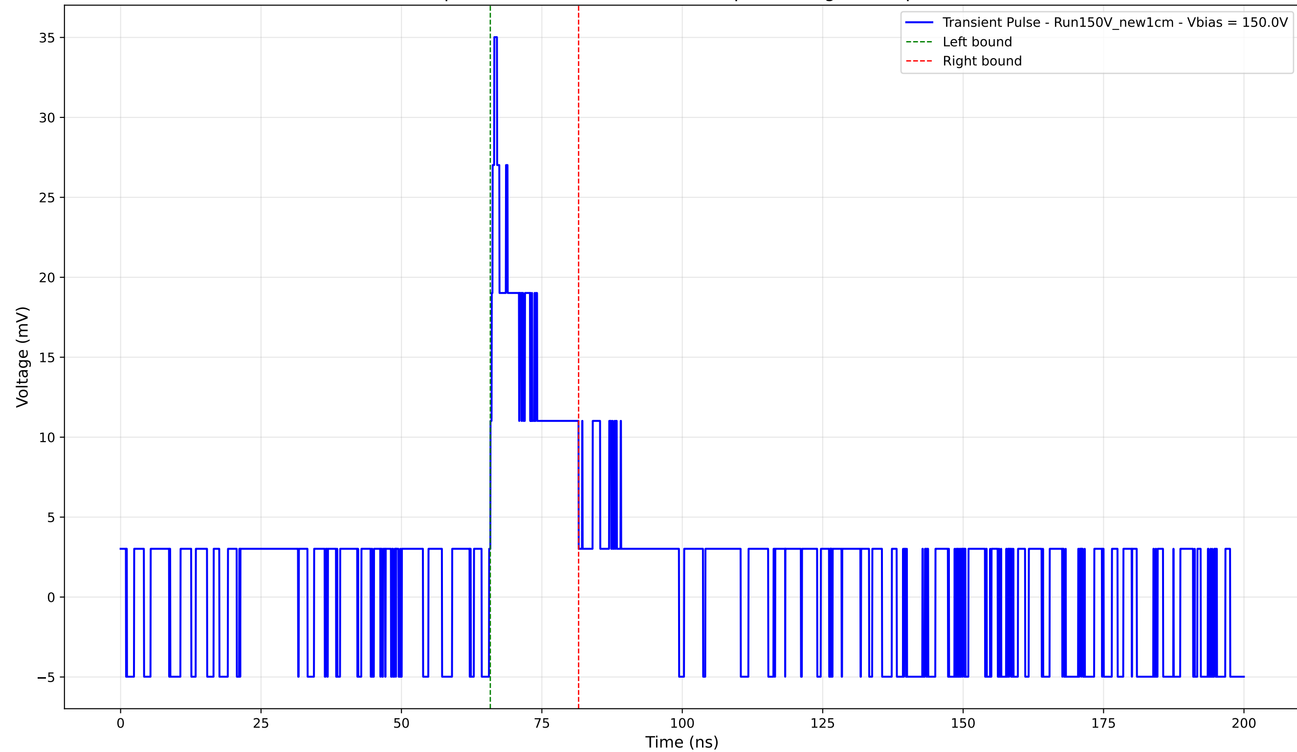
Transient Pulse - Sample: New1cm - Position: 2535.0 \mu\text{m} - Charge: 4.87 pC - Rise Time: 0.70 ns
