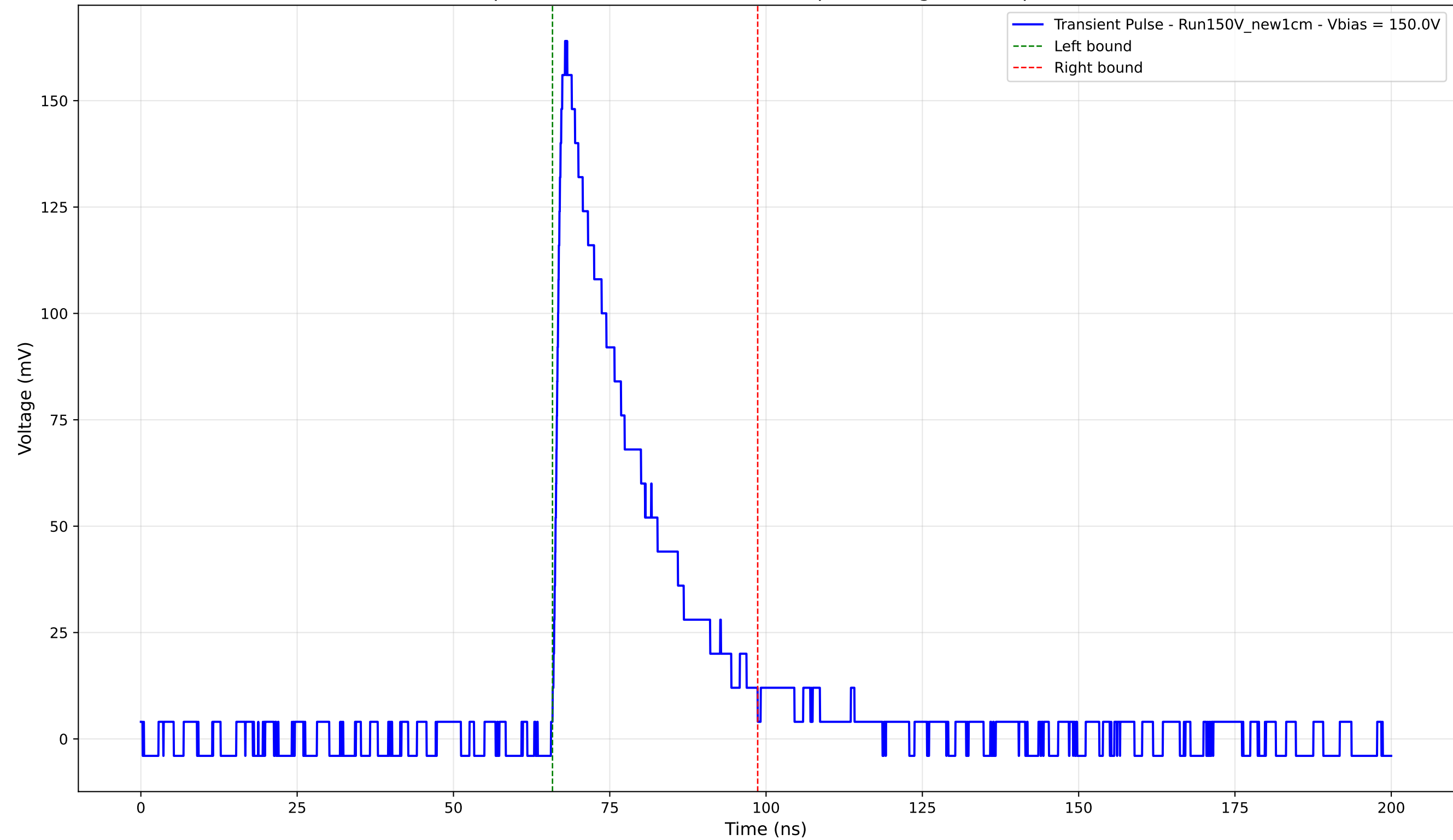
Transient Pulse - Sample: New1cm - Position: 4345.0 \mu\text{m} - Charge: 40.64 pC - Rise Time: 1.25 ns
