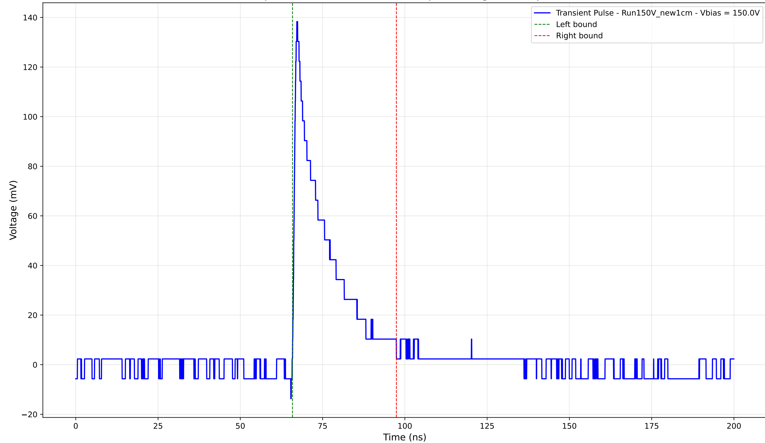
Transient Pulse - Sample: New1cm - Position: 240.0 \mu\text{m} - Charge: 26.03 pC - Rise Time: 1.01 ns
