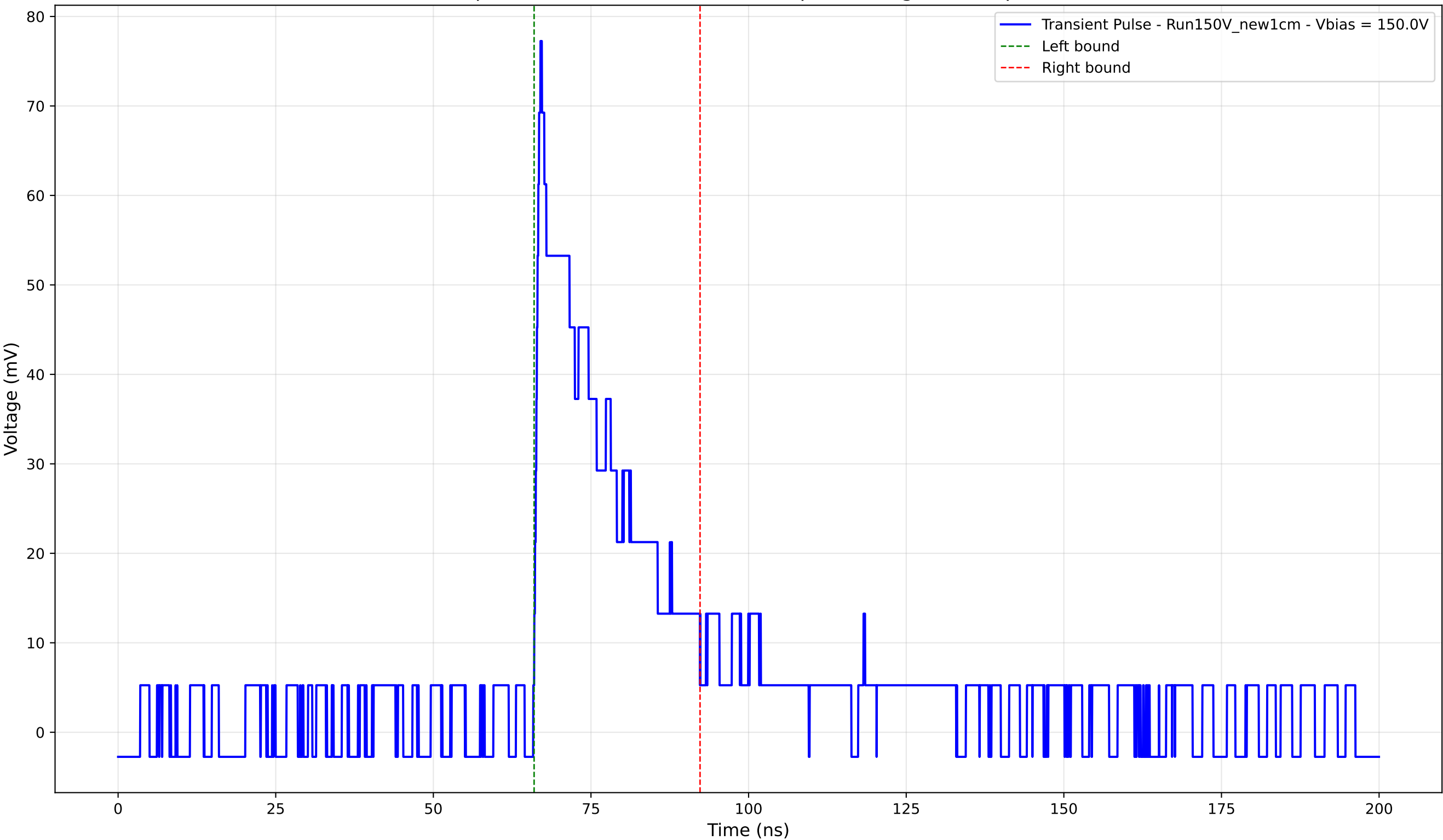
Transient Pulse - Sample: New1cm - Position: 2095.0 \mu\text{m} - Charge: 16.42 pC - Rise Time: 0.99 ns
