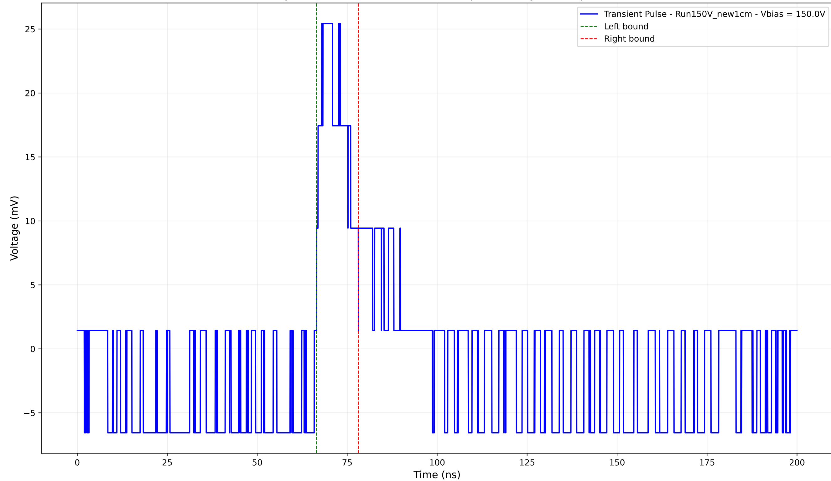
Transient Pulse - Sample: New1cm - Position: 4085.0 \mu\text{m} - Charge: 4.14 pC - Rise Time: 1.46 ns
