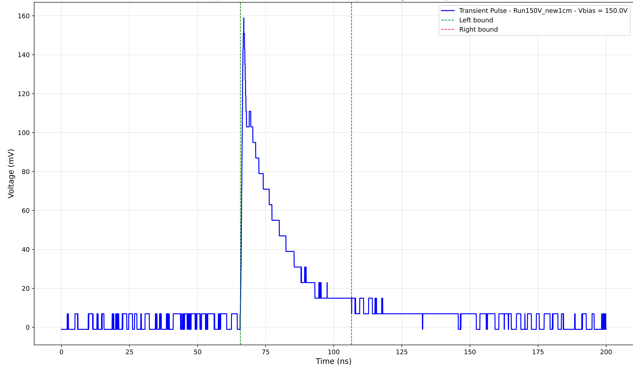
Transient Pulse - Sample: New1cm - Position: 2230.0 \mu\text{m} - Charge: 36.39 pC - Rise Time: 0.96 ns
