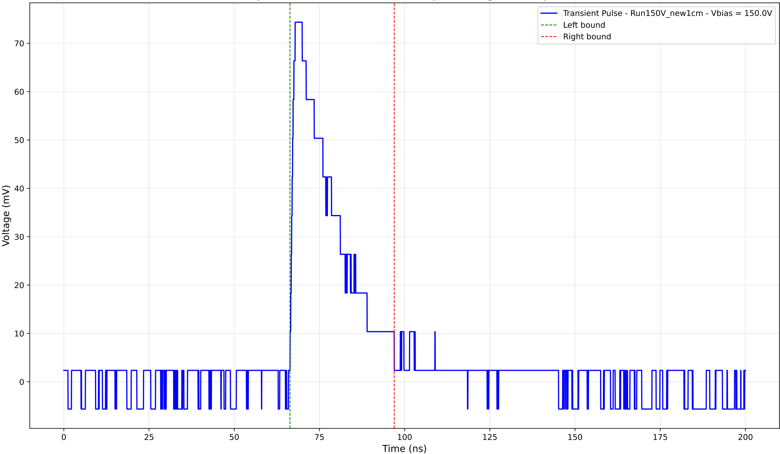
Transient Pulse - Sample: New1cm - Position: 1105.0 \mu\text{m} - Charge: 20.08 pC - Rise Time: 1.49 ns
