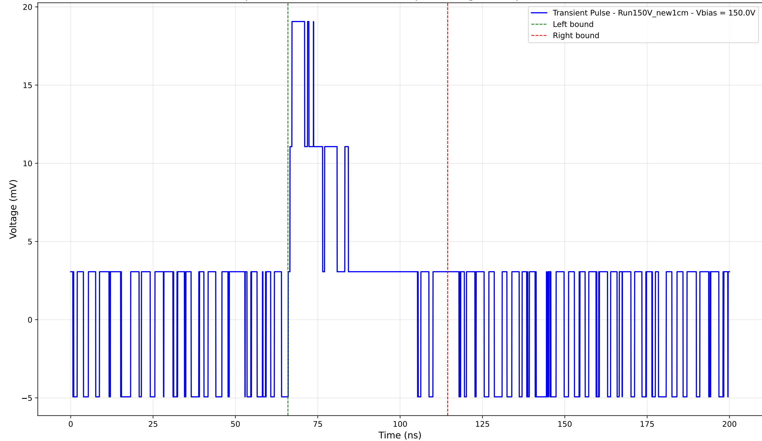
Transient Pulse - Sample: New1cm - Position: 3560.0 \mu\text{m} - Charge: 5.69 pC - Rise Time: 0.00 ns (N/A)
