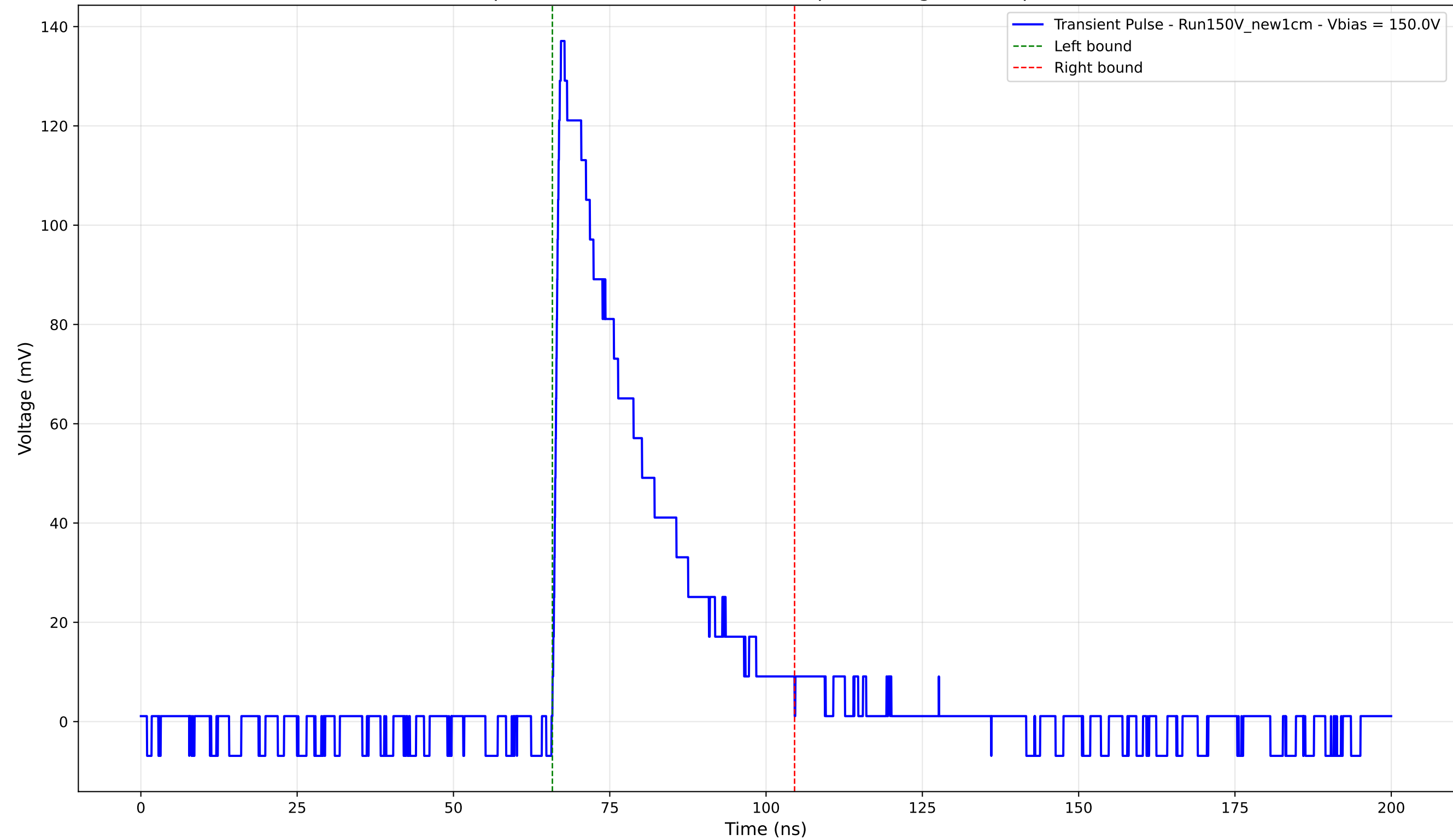
Transient Pulse - Sample: New1cm - Position: 3180.0 \mu\text{m} - Charge: 37.10 pC - Rise Time: 1.05 ns
