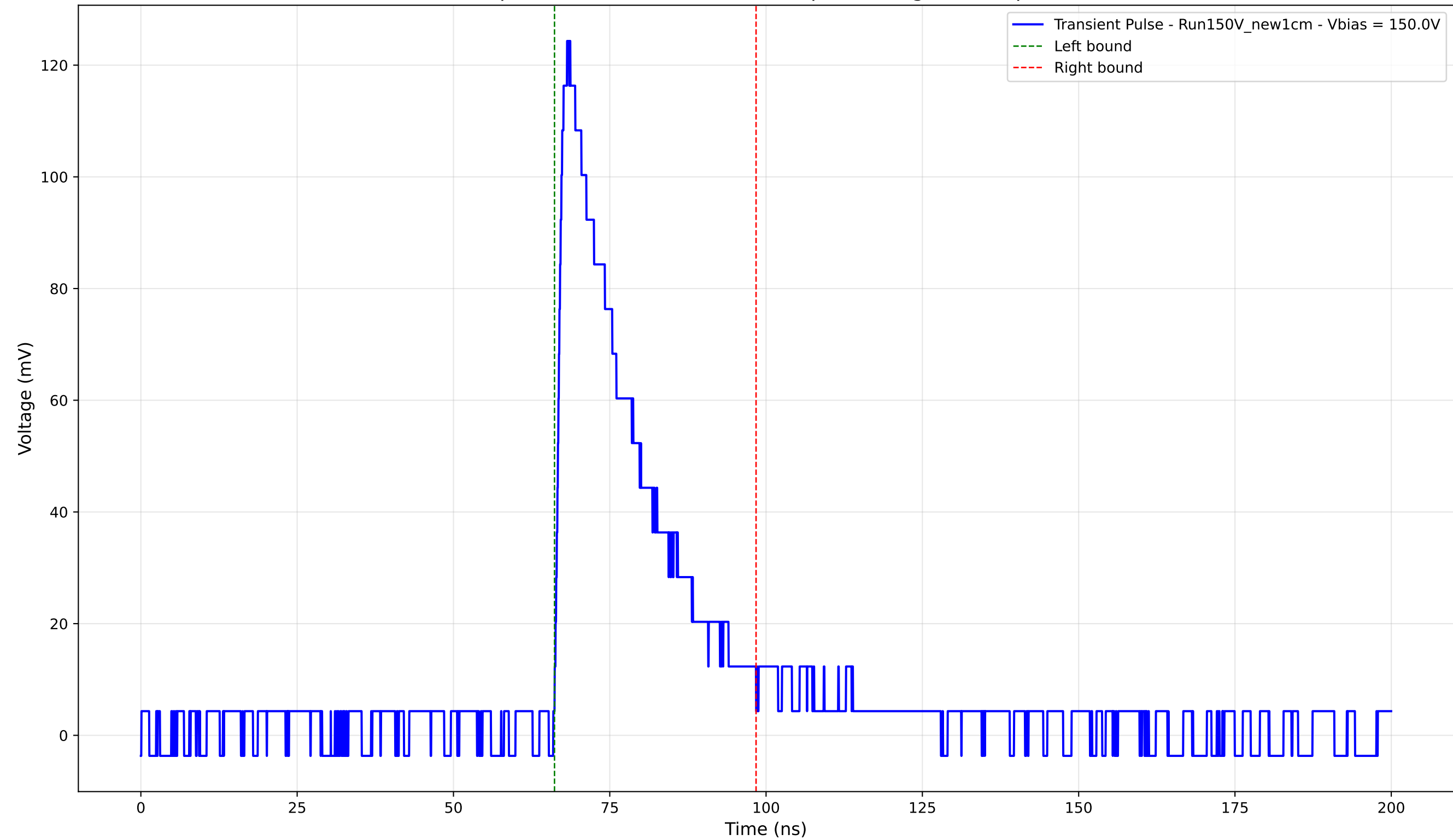
Transient Pulse - Sample: New1cm - Position: 750.0 \mu\text{m} - Charge: 31.67 pC - Rise Time: 1.30 ns
