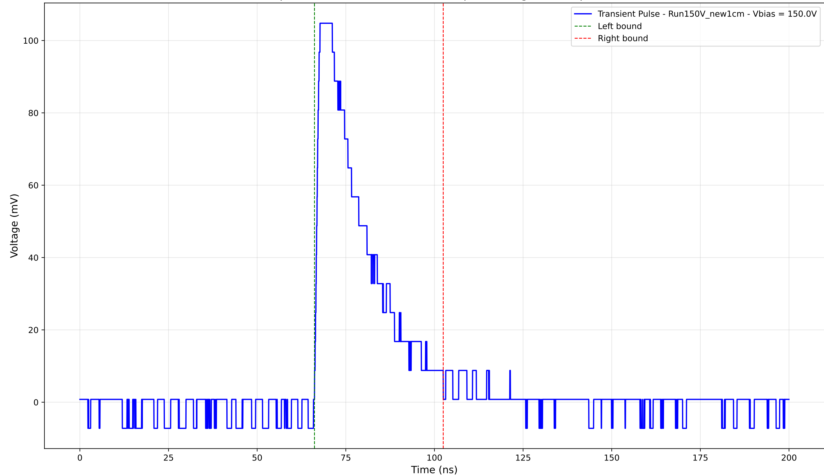
Transient Pulse - Sample: New1cm - Position: 1355.0 \mu\text{m} - Charge: 31.04 pC - Rise Time: 1.14 ns
