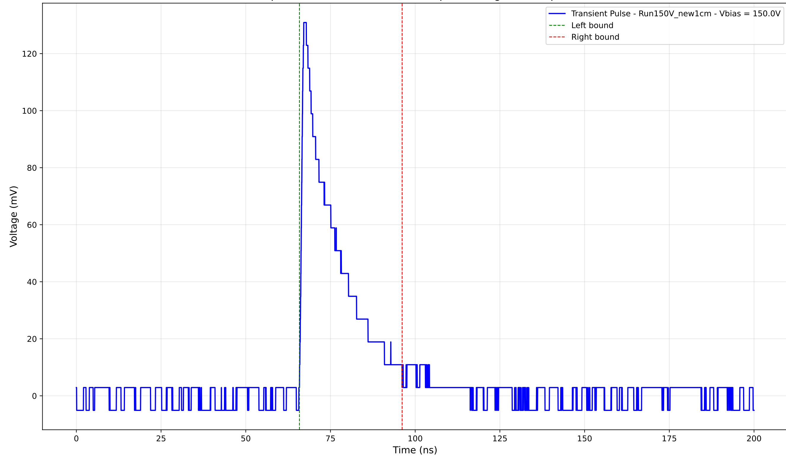
Transient Pulse - Sample: New1cm - Position: 320.0 \mu\text{m} - Charge: 27.66 pC - Rise Time: 1.01 ns
