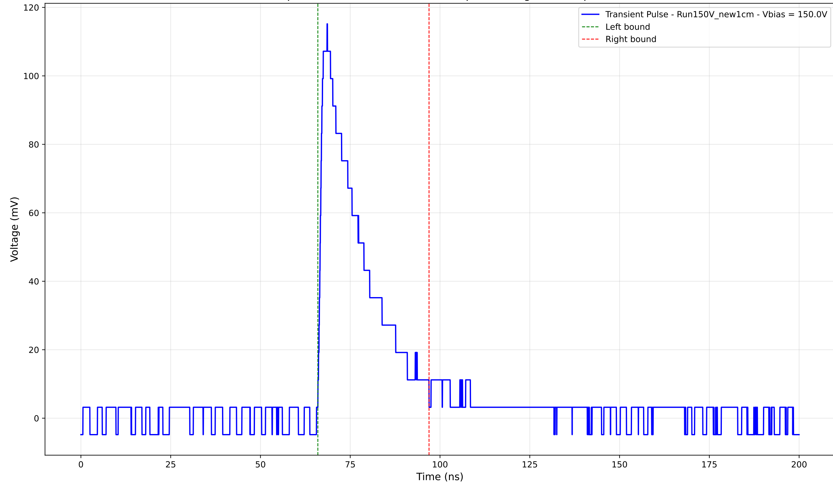
Transient Pulse - Sample: New1cm - Position: 655.0 \mu\text{m} - Charge: 27.96 pC - Rise Time: 1.34 ns
