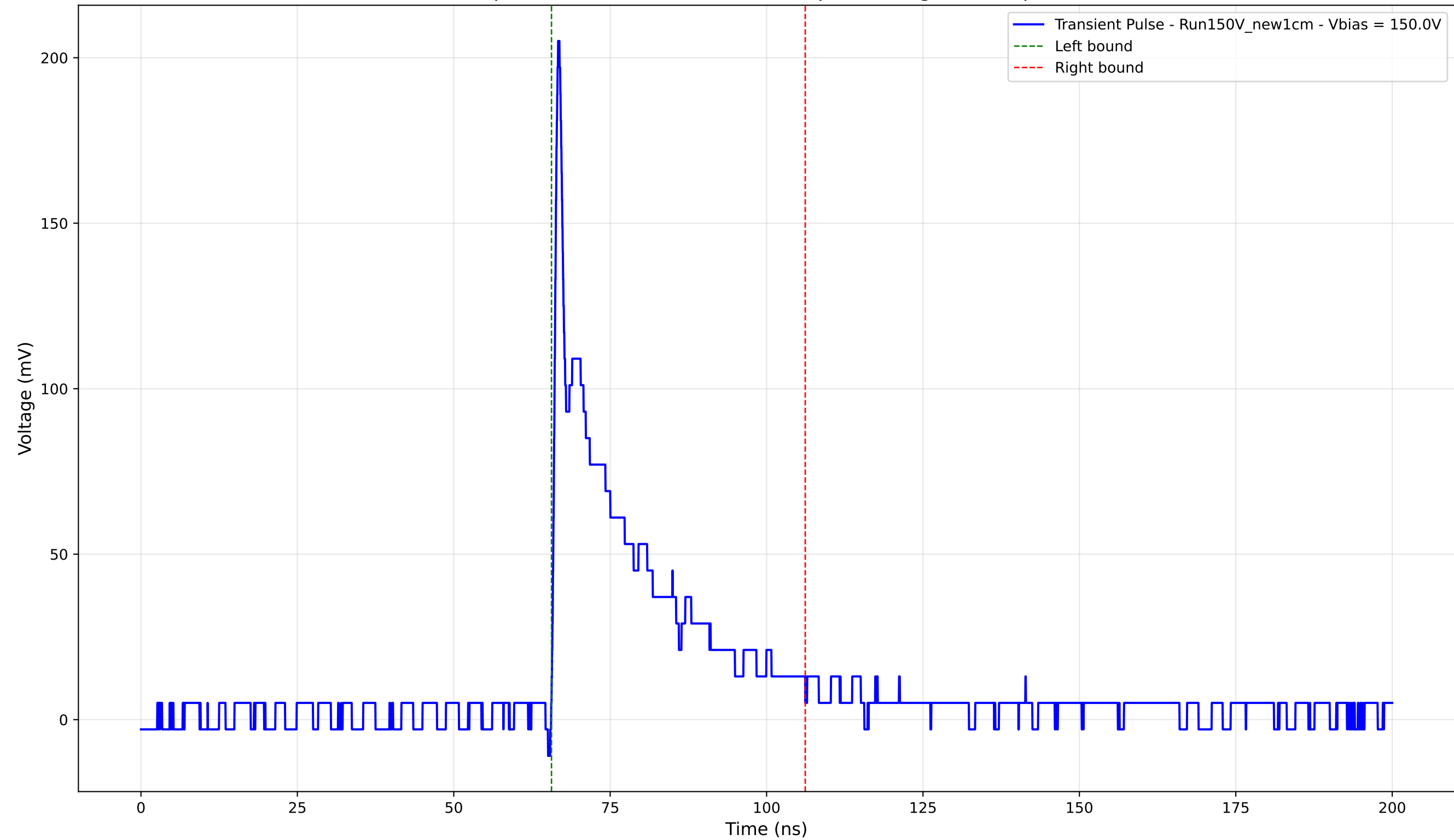
Transient Pulse - Sample: New1cm - Position: 2435.0 \mu\text{m} - Charge: 37.07 pC - Rise Time: 0.82 ns
