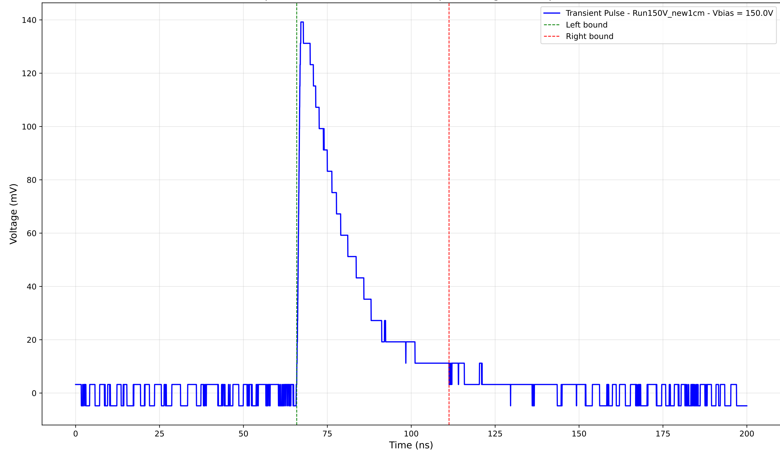
Transient Pulse - Sample: New1cm - Position: 3215.0 \mu\text{m} - Charge: 42.42 pC - Rise Time: 0.97 ns
