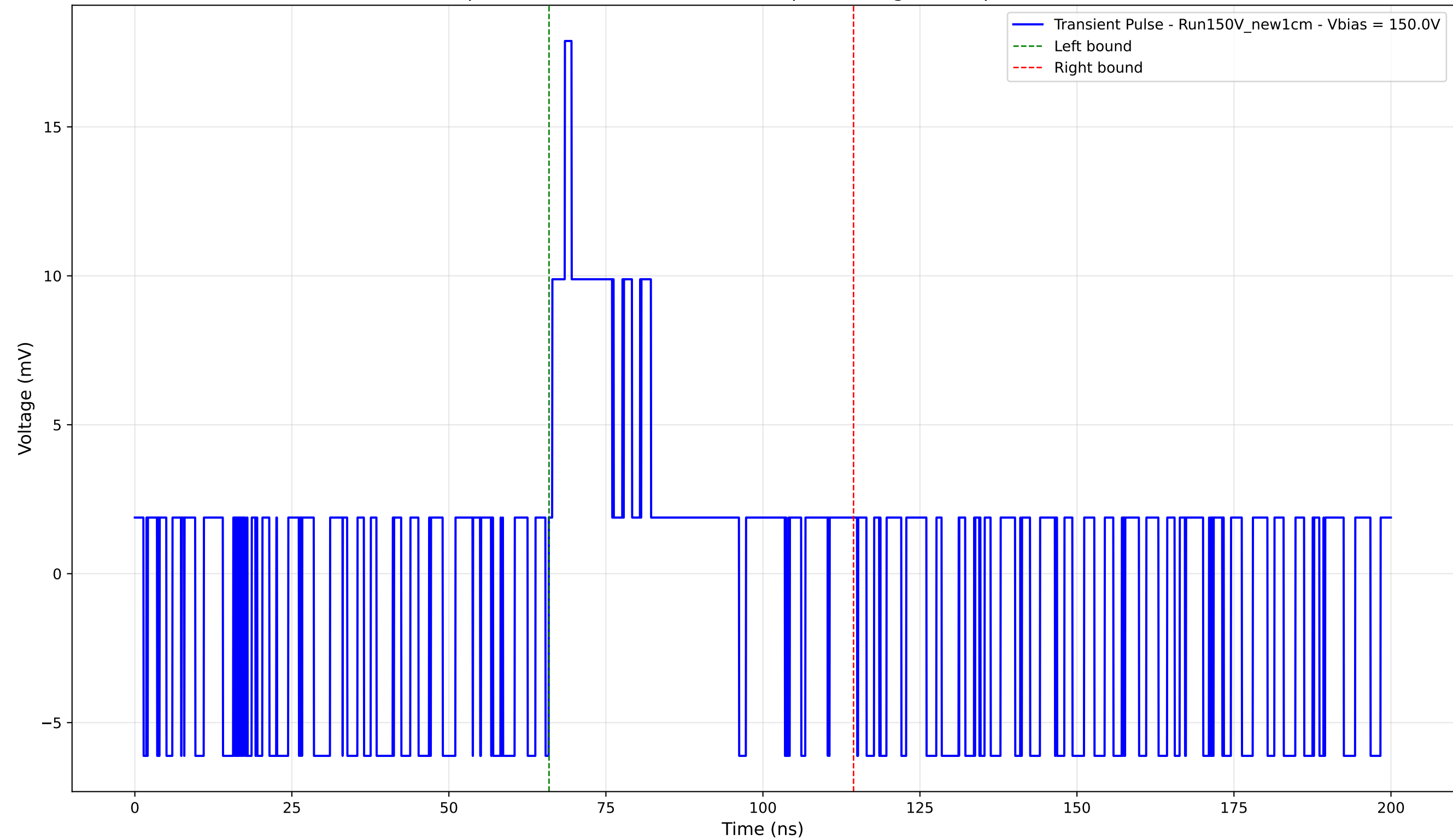
Transient Pulse - Sample: New1cm - Position: 2035.0 \mu\text{m} - Charge: 3.64 pC - Rise Time: 0.00 ns (N/A)
