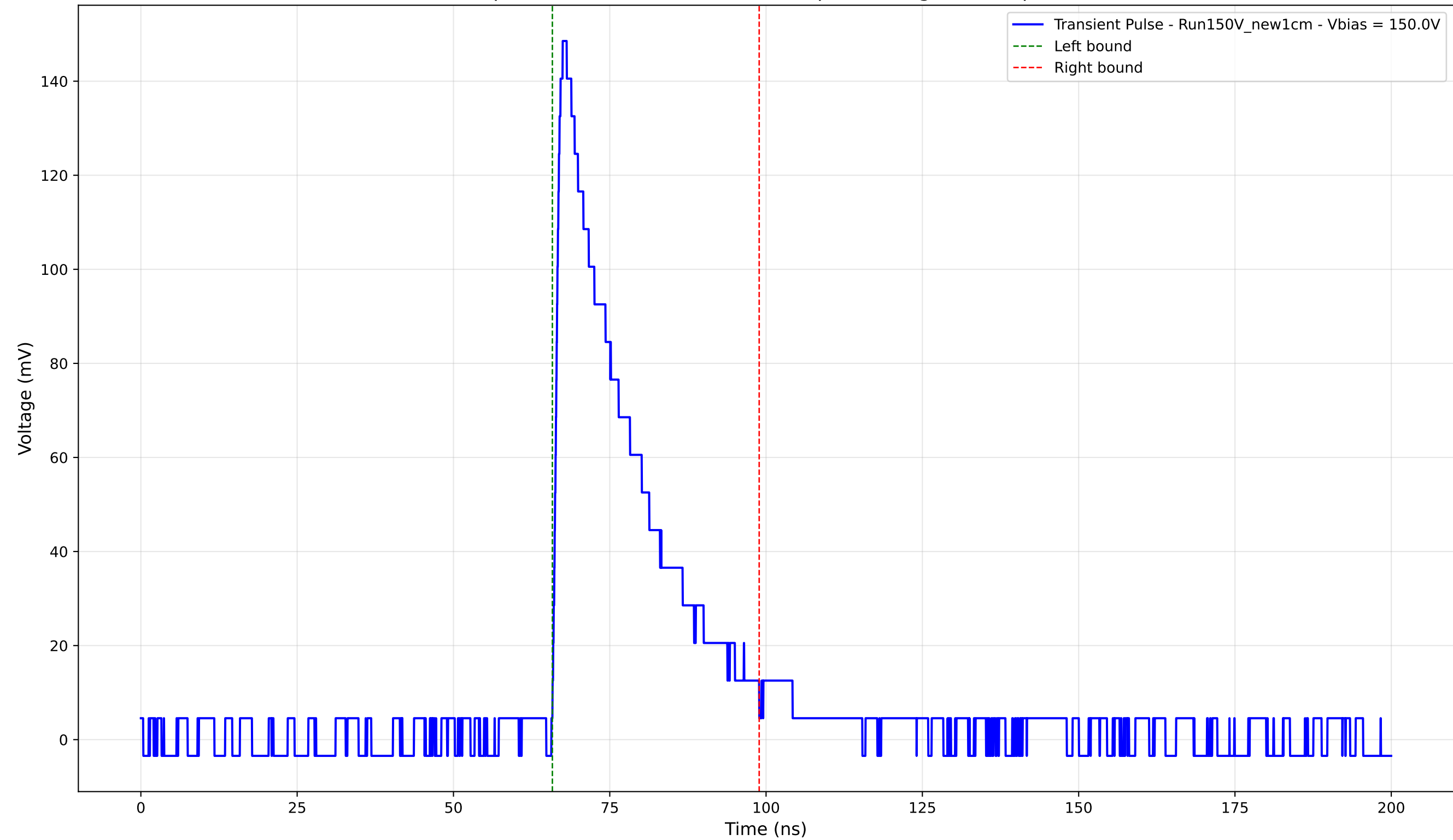
Transient Pulse - Sample: New1cm - Position: 4470.0 \mu\text{m} - Charge: 37.11 pC - Rise Time: 1.19 ns
