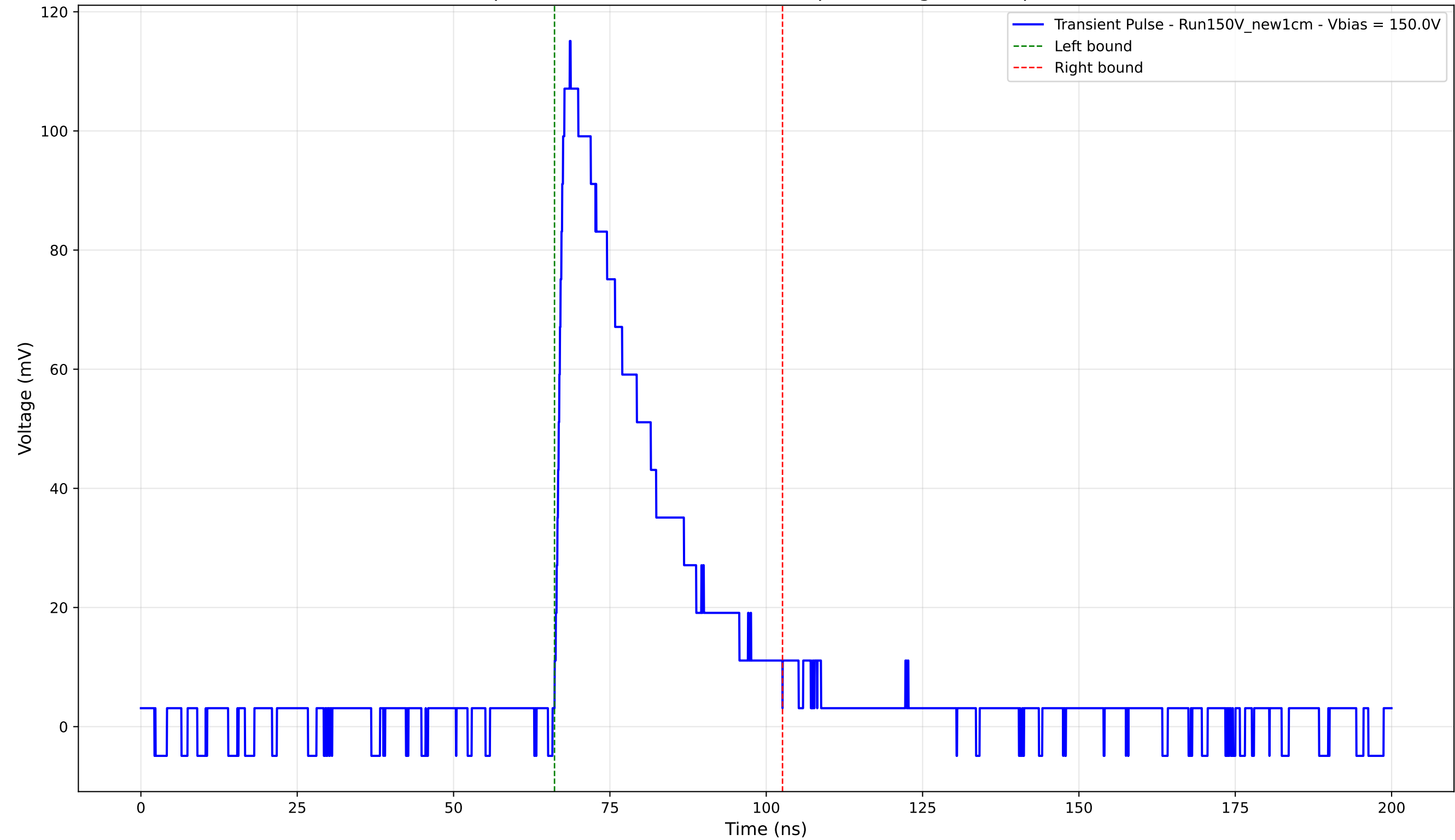
Transient Pulse - Sample: New1cm - Position: 1360.0 \mu\text{m} - Charge: 32.63 pC - Rise Time: 1.40 ns
