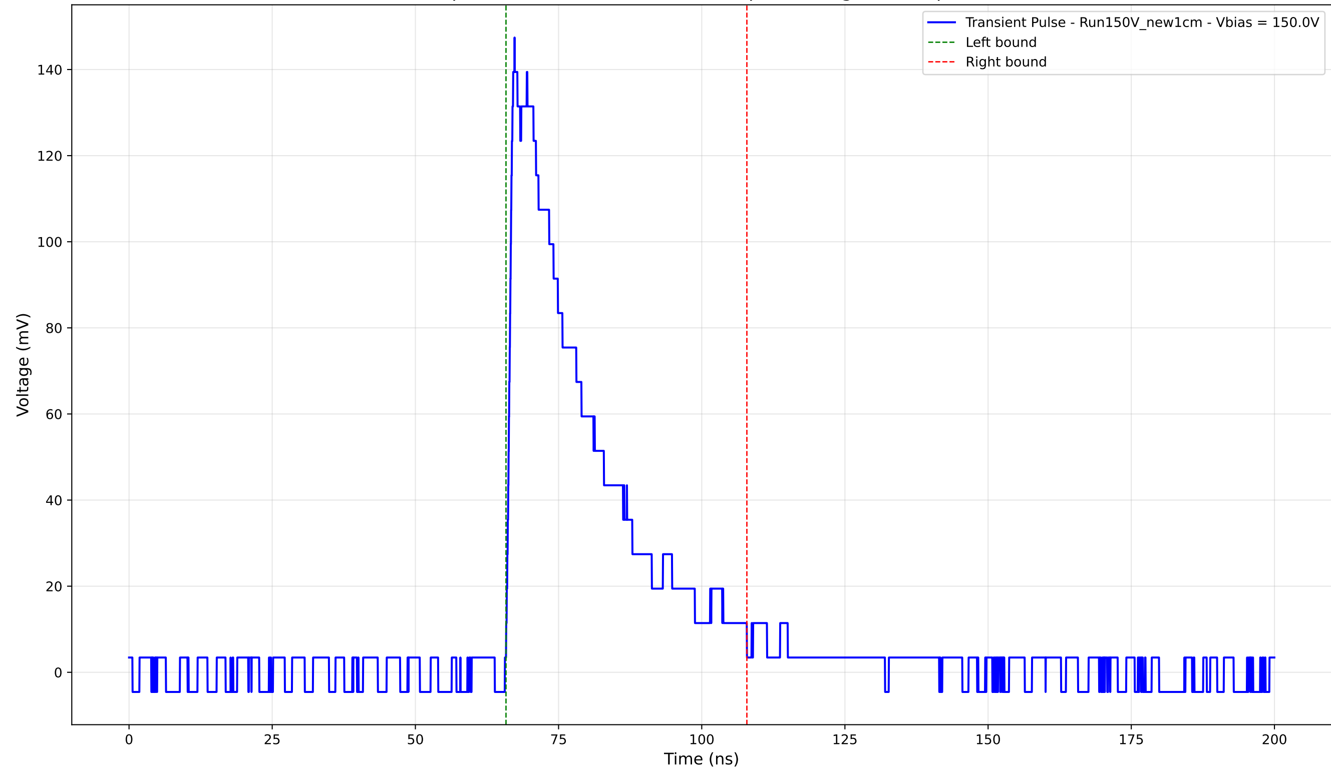
Transient Pulse - Sample: New1cm - Position: 3220.0 \mu\text{m} - Charge: 42.36 pC - Rise Time: 1.13 ns
