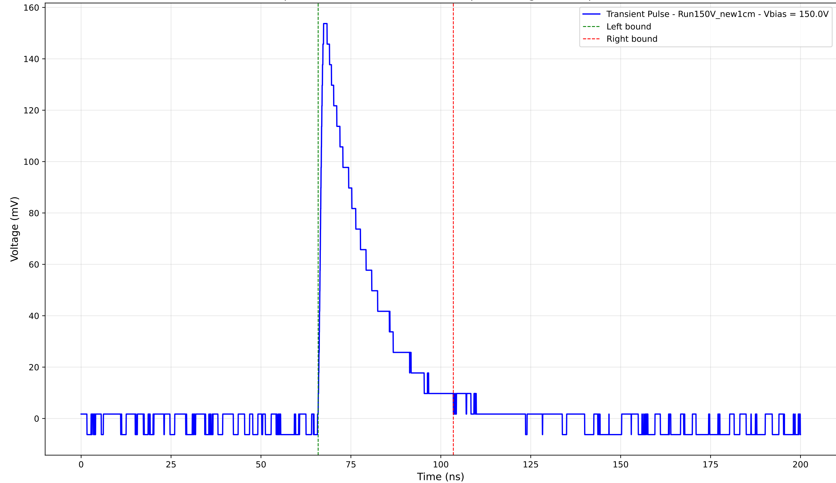
Transient Pulse - Sample: New1cm - Position: 4385.0 \mu\text{m} - Charge: 39.24 pC - Rise Time: 1.21 ns
