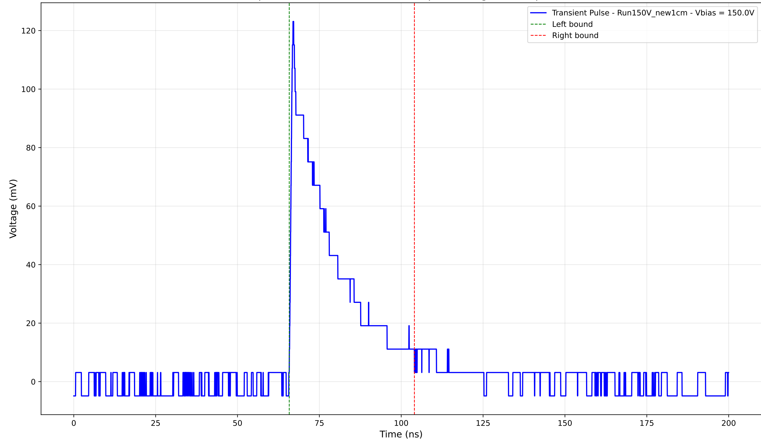
Transient Pulse - Sample: New1cm - Position: 2150.0 \mu\text{m} - Charge: 30.11 pC - Rise Time: 0.86 ns
