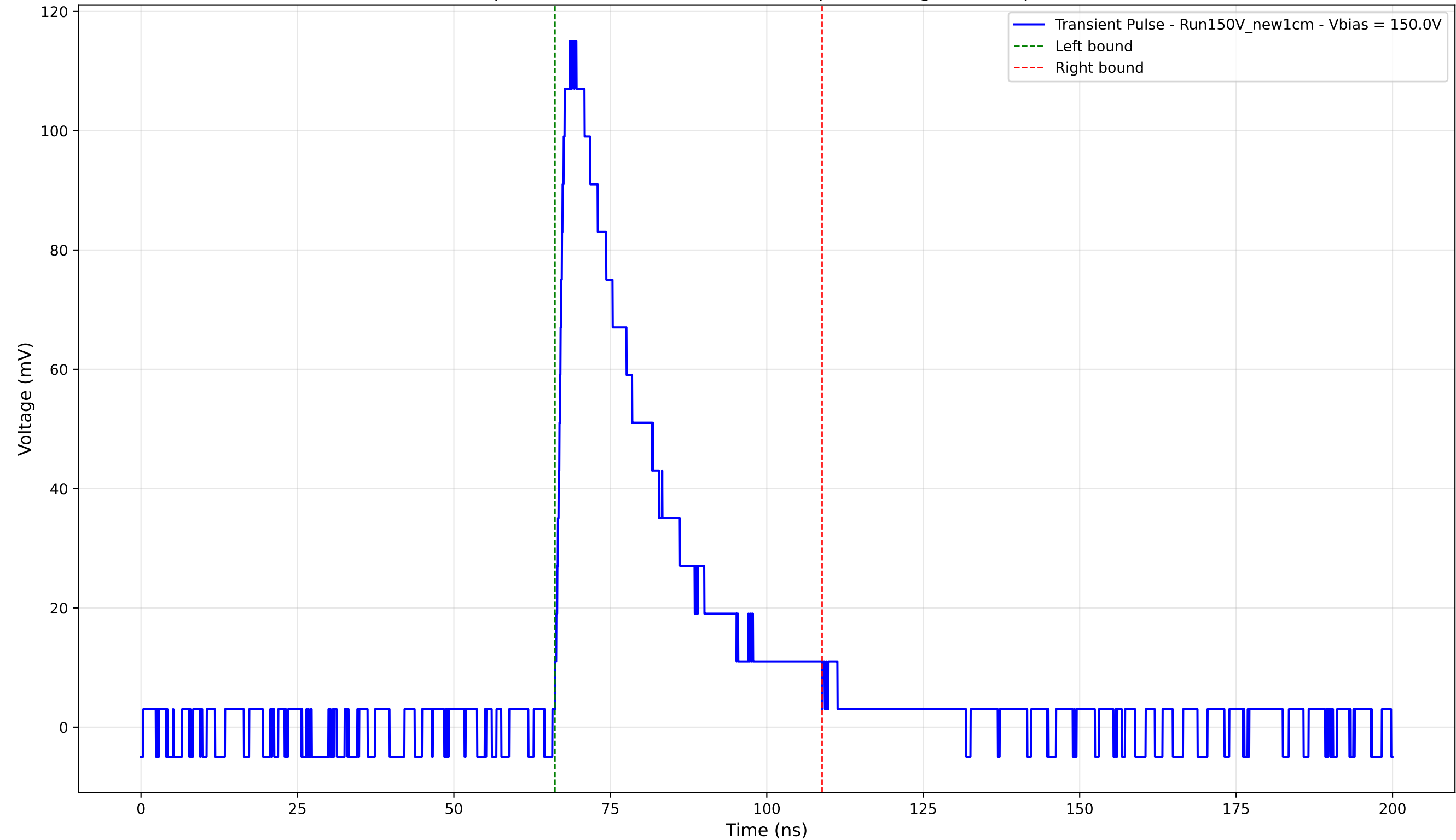
Transient Pulse - Sample: New1cm - Position: 1230.0 \mu\text{m} - Charge: 34.11 pC - Rise Time: 1.36 ns
