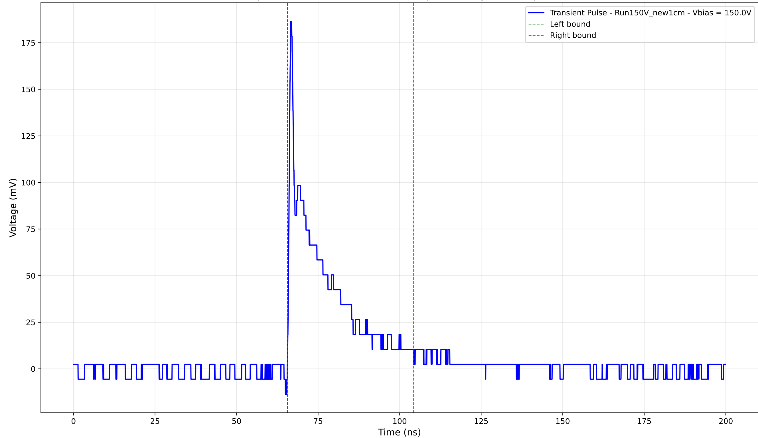
Transient Pulse - Sample: New1cm - Position: 2645.0 \mu\text{m} - Charge: 31.63 pC - Rise Time: 0.74 ns
