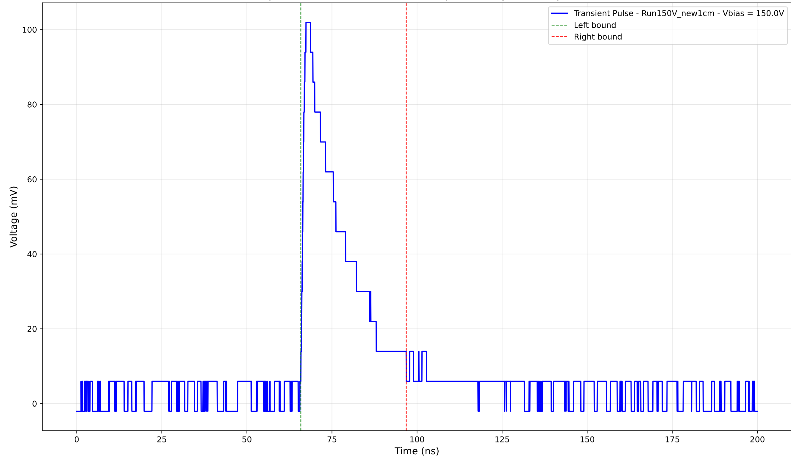
Transient Pulse - Sample: New1cm - Position: 4505.0 \mu\text{m} - Charge: 25.83 pC - Rise Time: 1.19 ns
