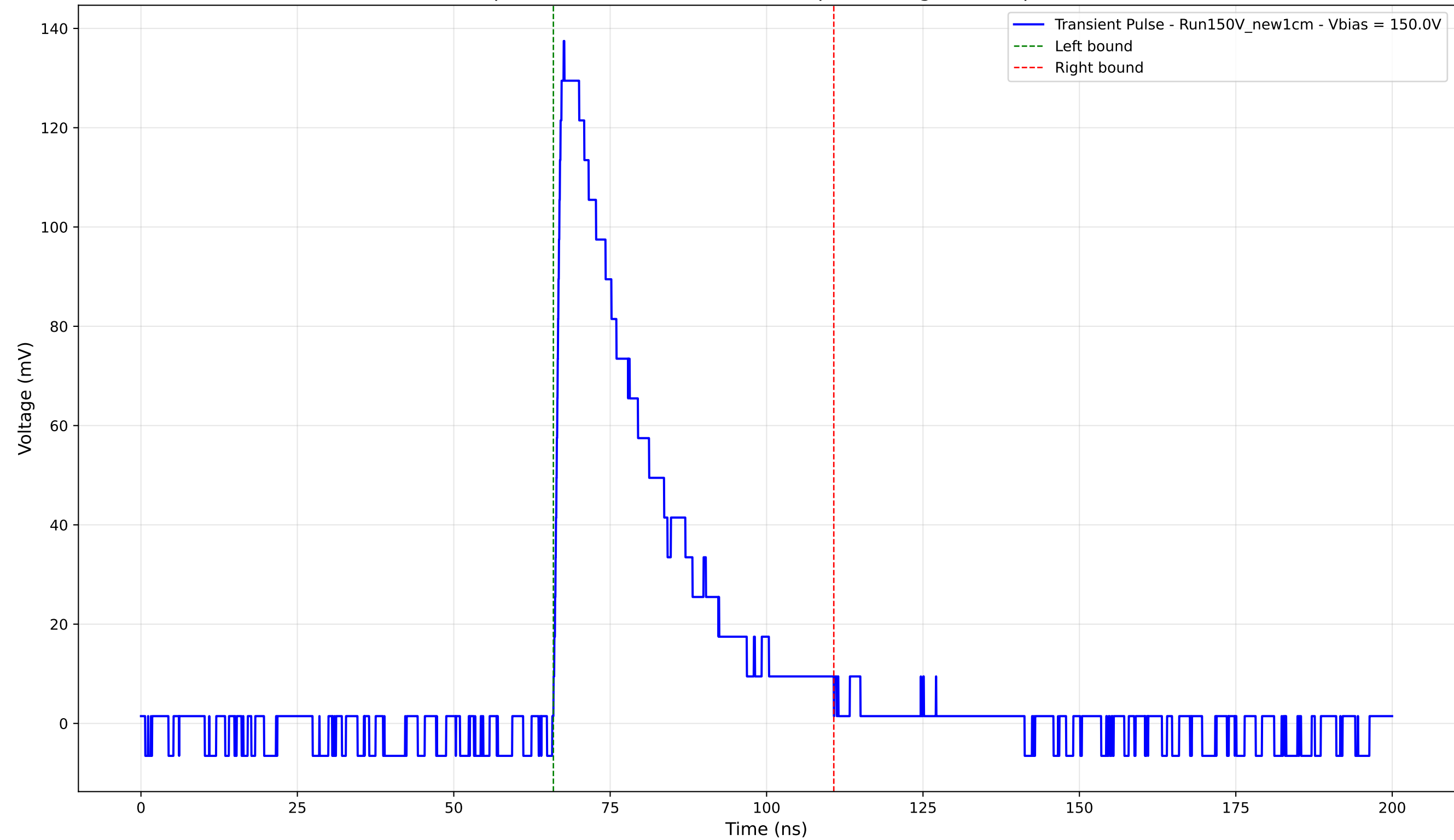
Transient Pulse - Sample: New1cm - Position: 3310.0 \mu\text{m} - Charge: 40.42 pC - Rise Time: 1.17 ns
