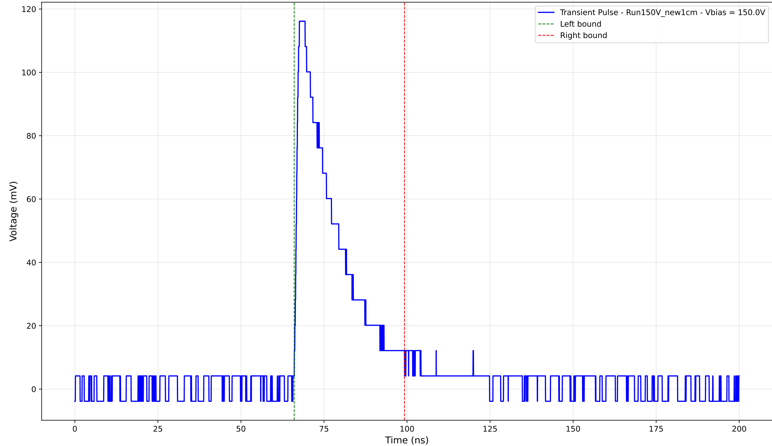
Transient Pulse - Sample: New1cm - Position: 665.0 \mu\text{m} - Charge: 30.11 pC - Rise Time: 1.28 ns
