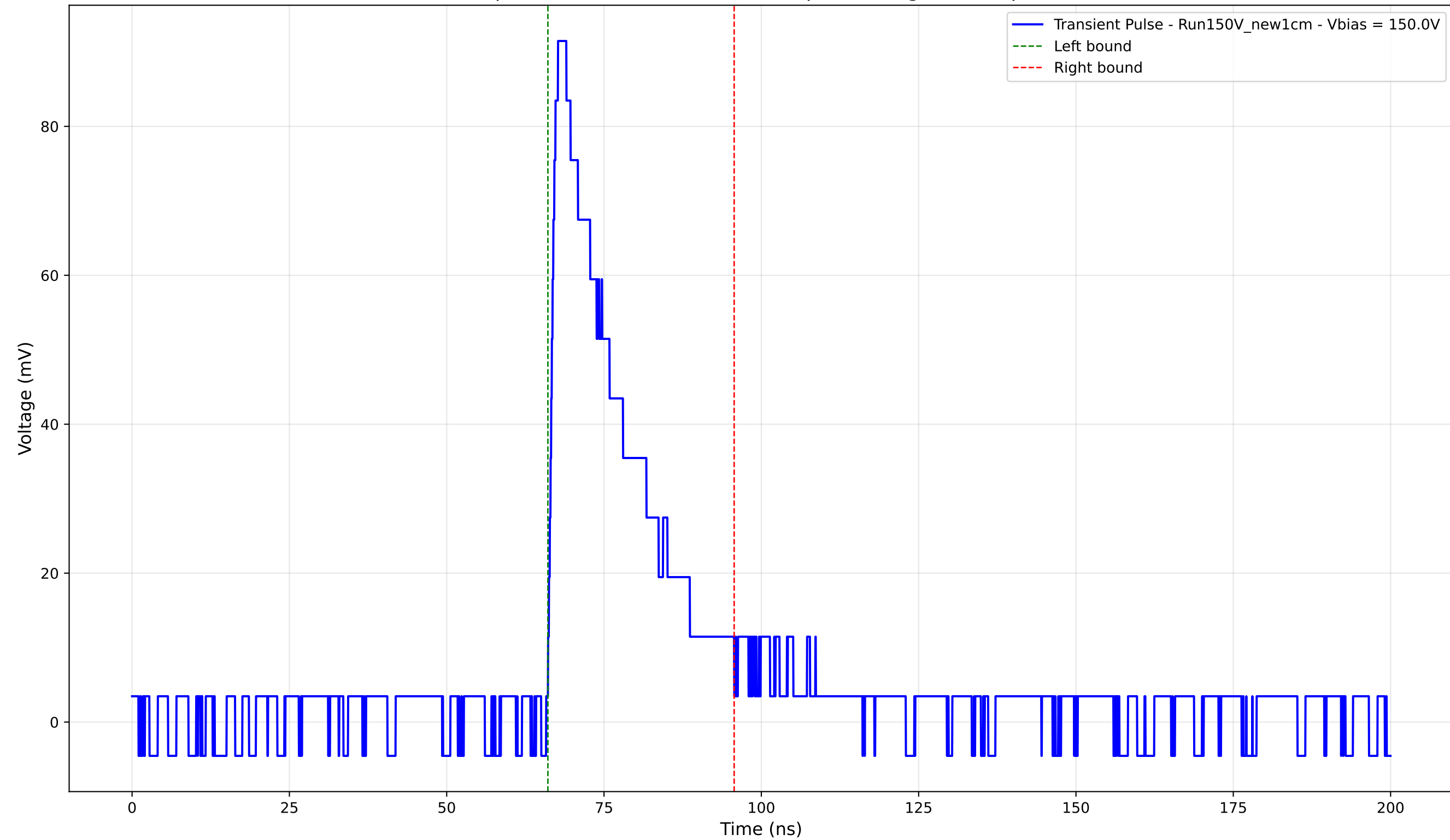
Transient Pulse - Sample: New1cm - Position: 610.0 \mu\text{m} - Charge: 22.30 pC - Rise Time: 1.19 ns
