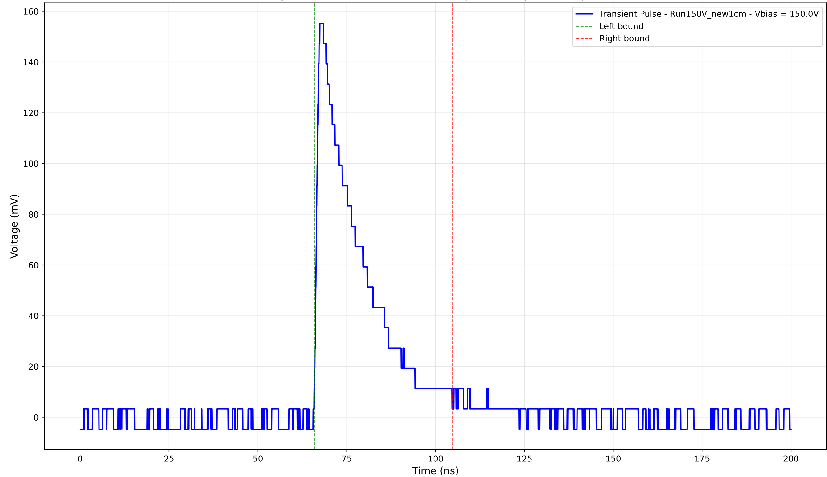
Transient Pulse - Sample: New1cm - Position: 4405.0 \mu\text{m} - Charge: 40.13 pC - Rise Time: 1.27 ns
