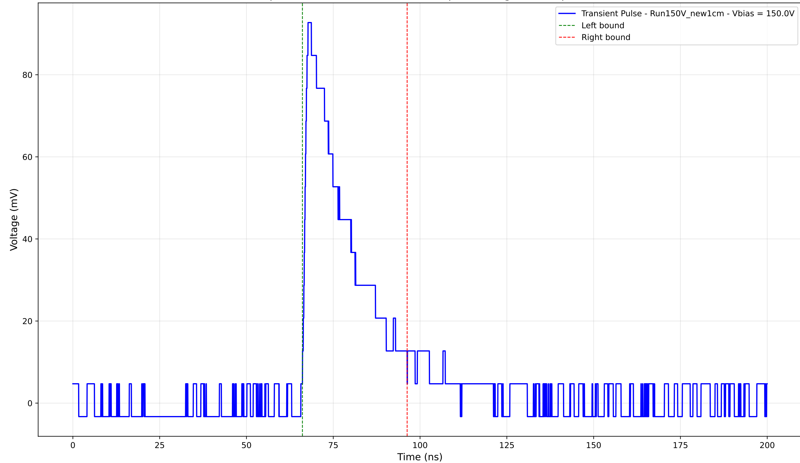
Transient Pulse - Sample: New1cm - Position: 4005.0 \mu\text{m} - Charge: 24.67 pC - Rise Time: 1.31 ns
