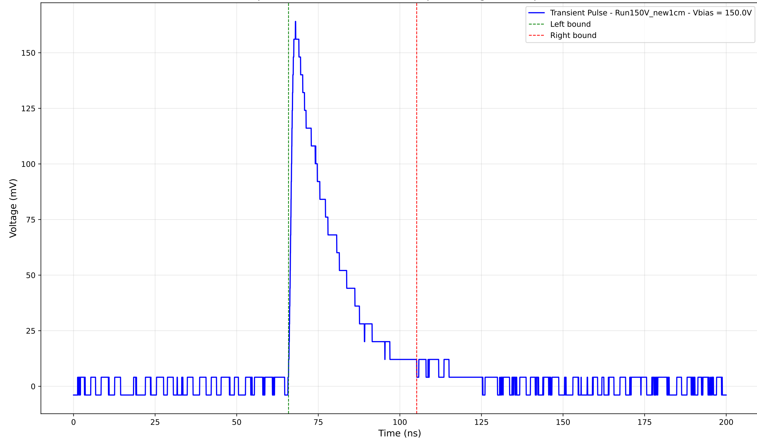
Transient Pulse - Sample: New1cm - Position: 4300.0 \mu\text{m} - Charge: 43.18 pC - Rise Time: 1.31 ns
