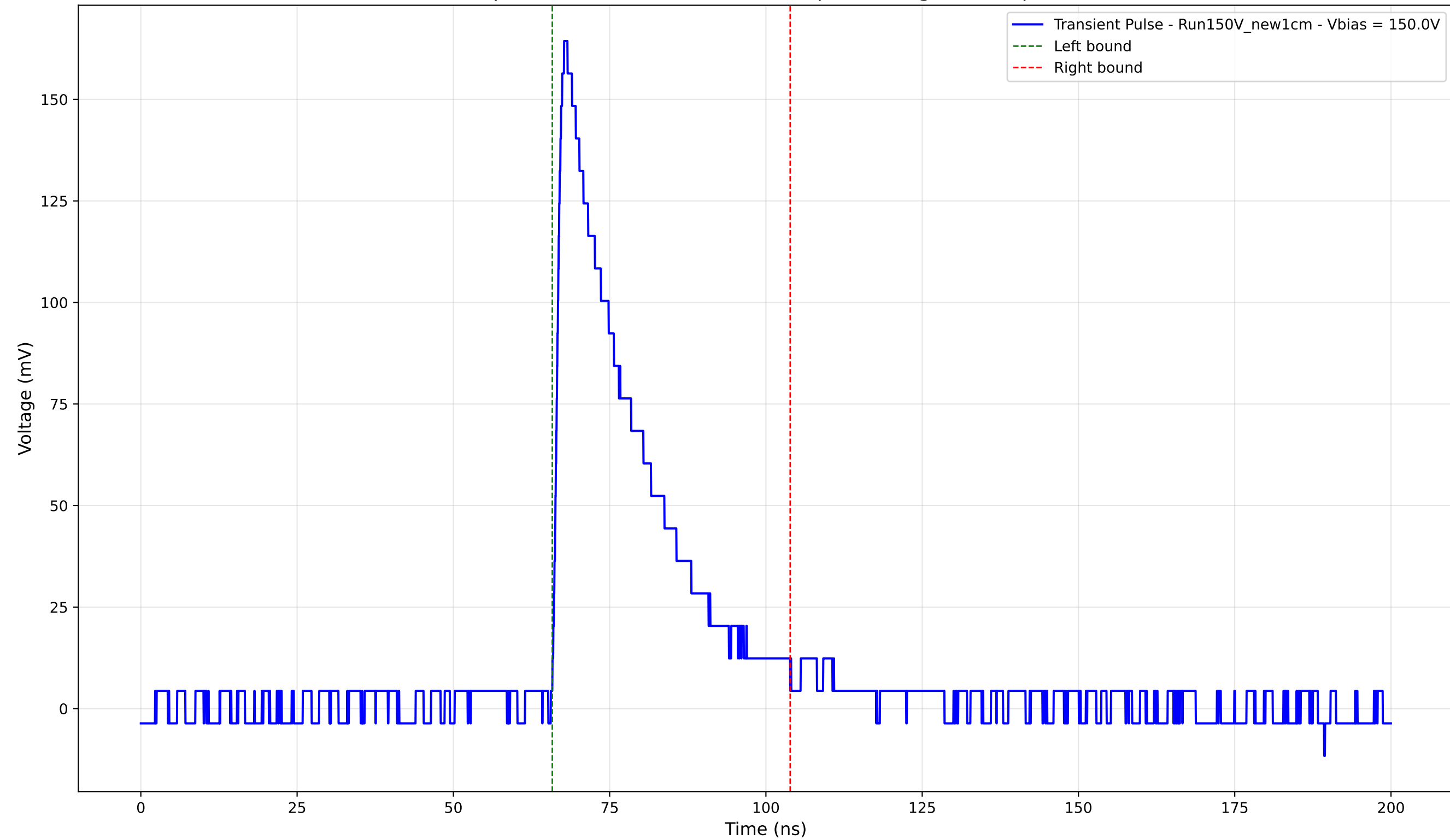
Transient Pulse - Sample: New1cm - Position: 4325.0 \mu\text{m} - Charge: 43.10 pC - Rise Time: 1.25 ns
