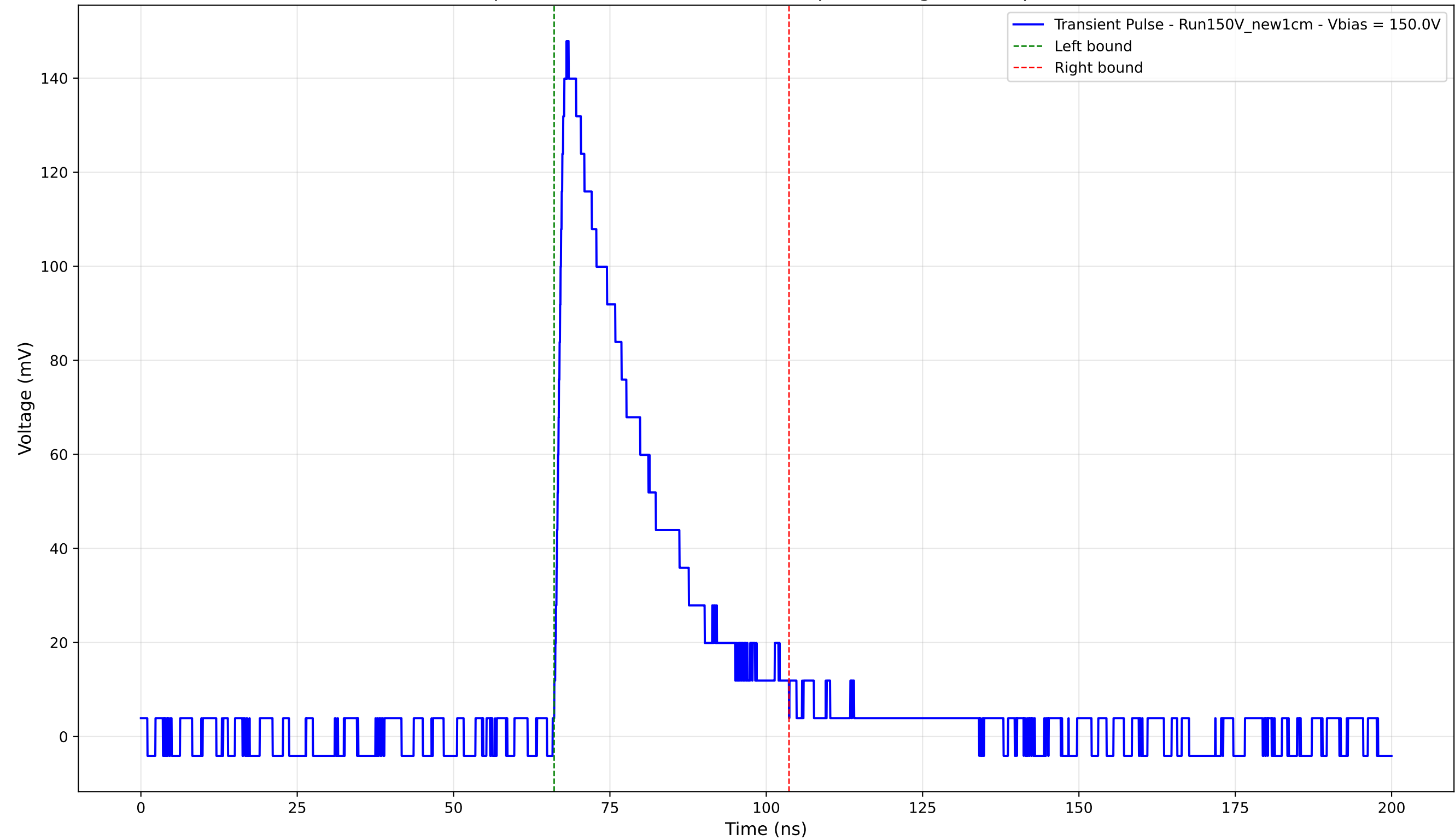
Transient Pulse - Sample: New1cm - Position: 3950.0 \mu\text{m} - Charge: 40.17 pC - Rise Time: 1.45 ns
