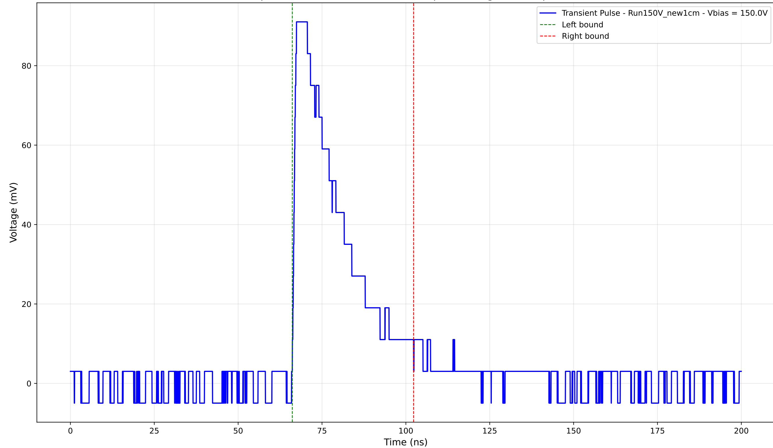
Transient Pulse - Sample: New1cm - Position: 1635.0 \mu\text{m} - Charge: 28.14 pC - Rise Time: 1.04 ns
