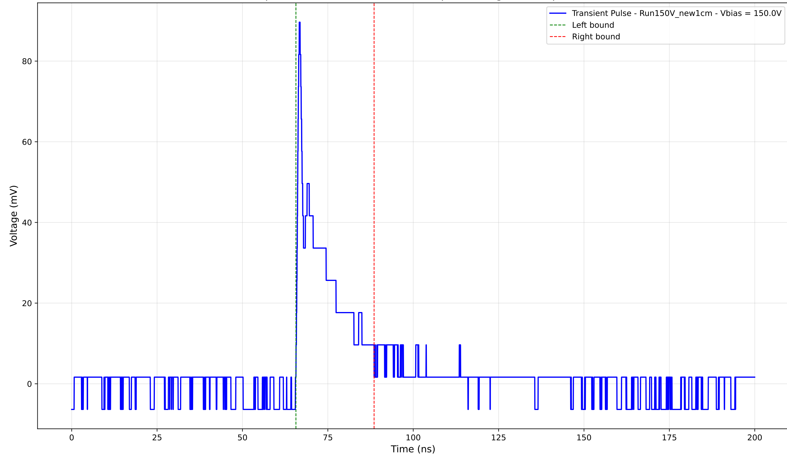
Transient Pulse - Sample: New1cm - Position: 2595.0 \mu\text{m} - Charge: 12.10 pC - Rise Time: 0.78 ns
