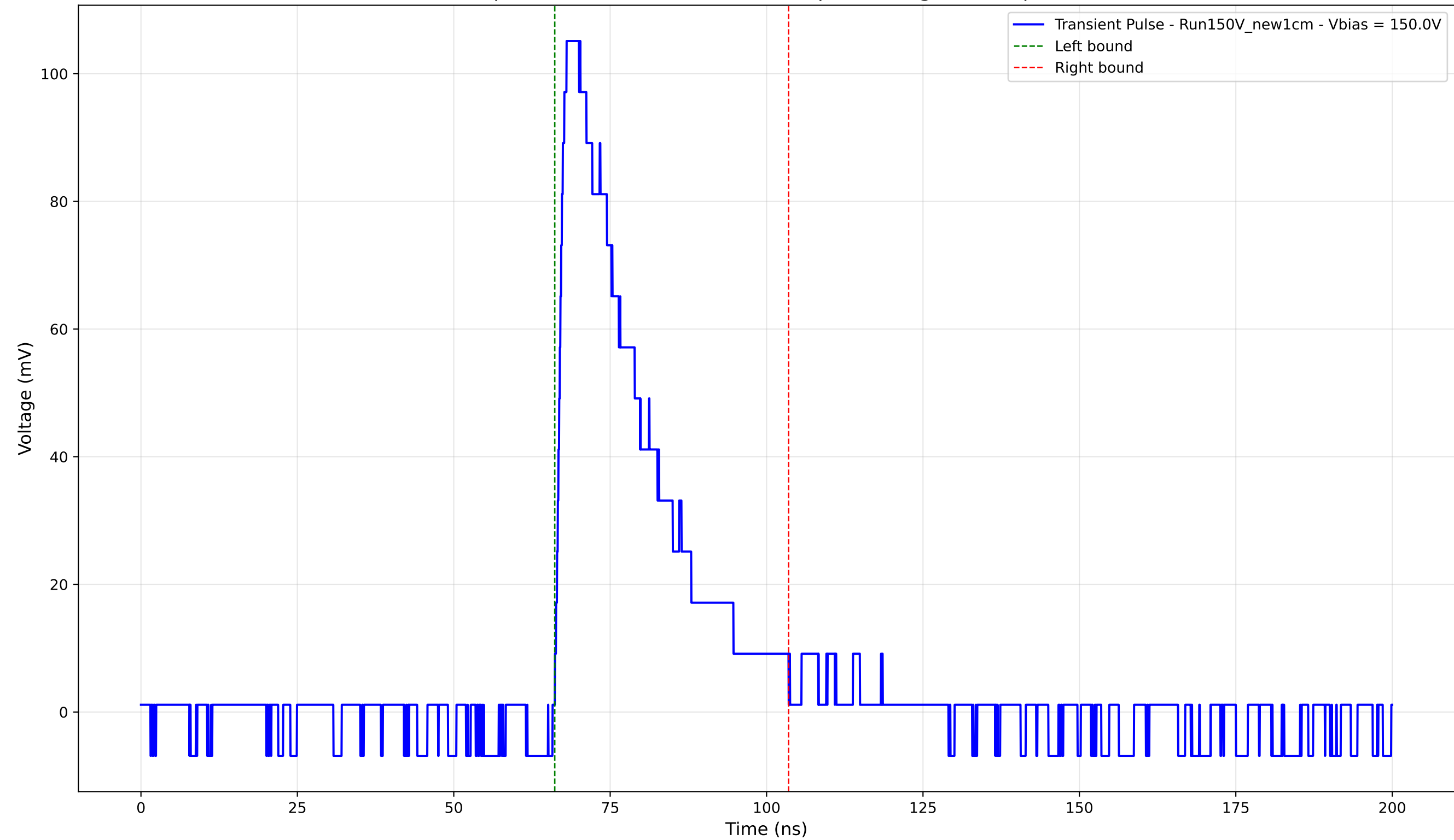
Transient Pulse - Sample: New1cm - Position: 1305.0 \mu\text{m} - Charge: 29.99 pC - Rise Time: 1.34 ns
