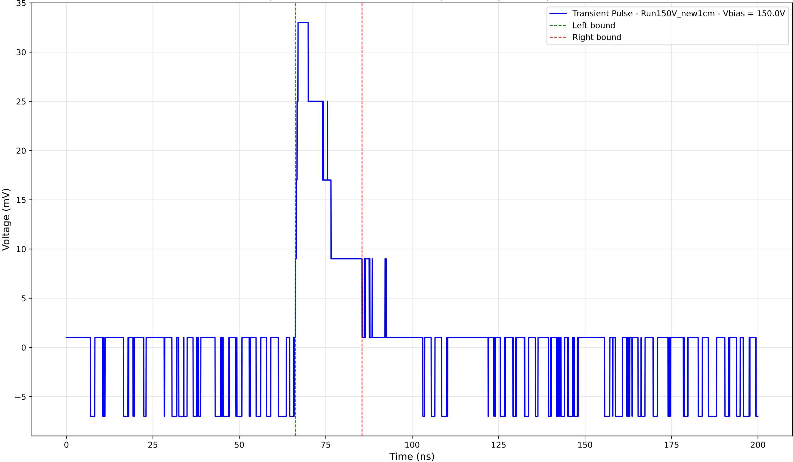
Transient Pulse - Sample: New1cm - Position: 495.0 \mu\text{m} - Charge: 6.77 pC - Rise Time: 0.77 ns
