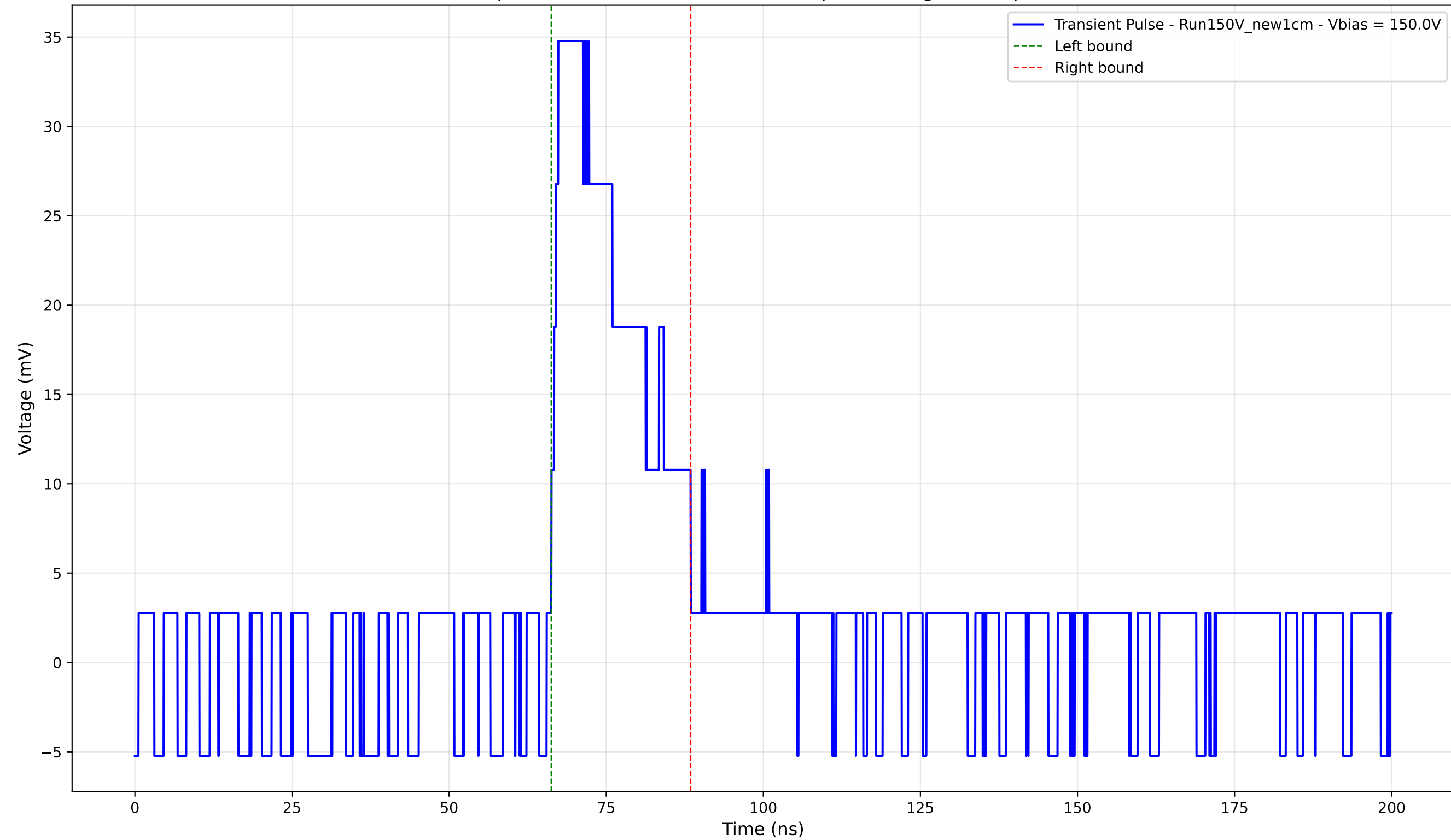
Transient Pulse - Sample: New1cm - Position: 1070.0 \mu\text{m} - Charge: 9.37 pC - Rise Time: 1.10 ns
