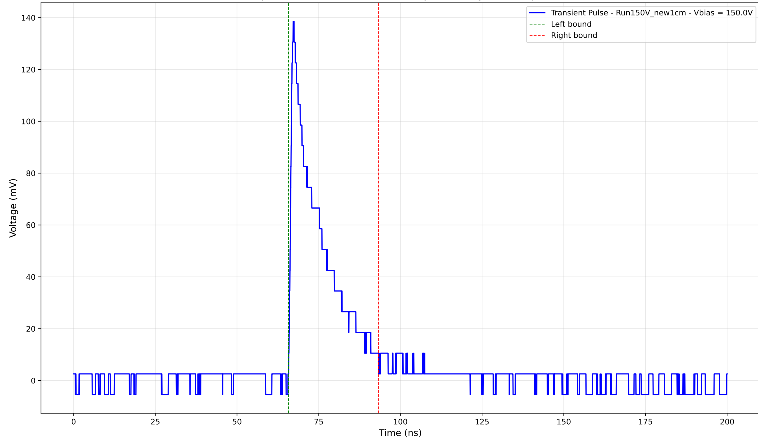
Transient Pulse - Sample: New1cm - Position: 245.0 \mu\text{m} - Charge: 26.59 pC - Rise Time: 1.05 ns
