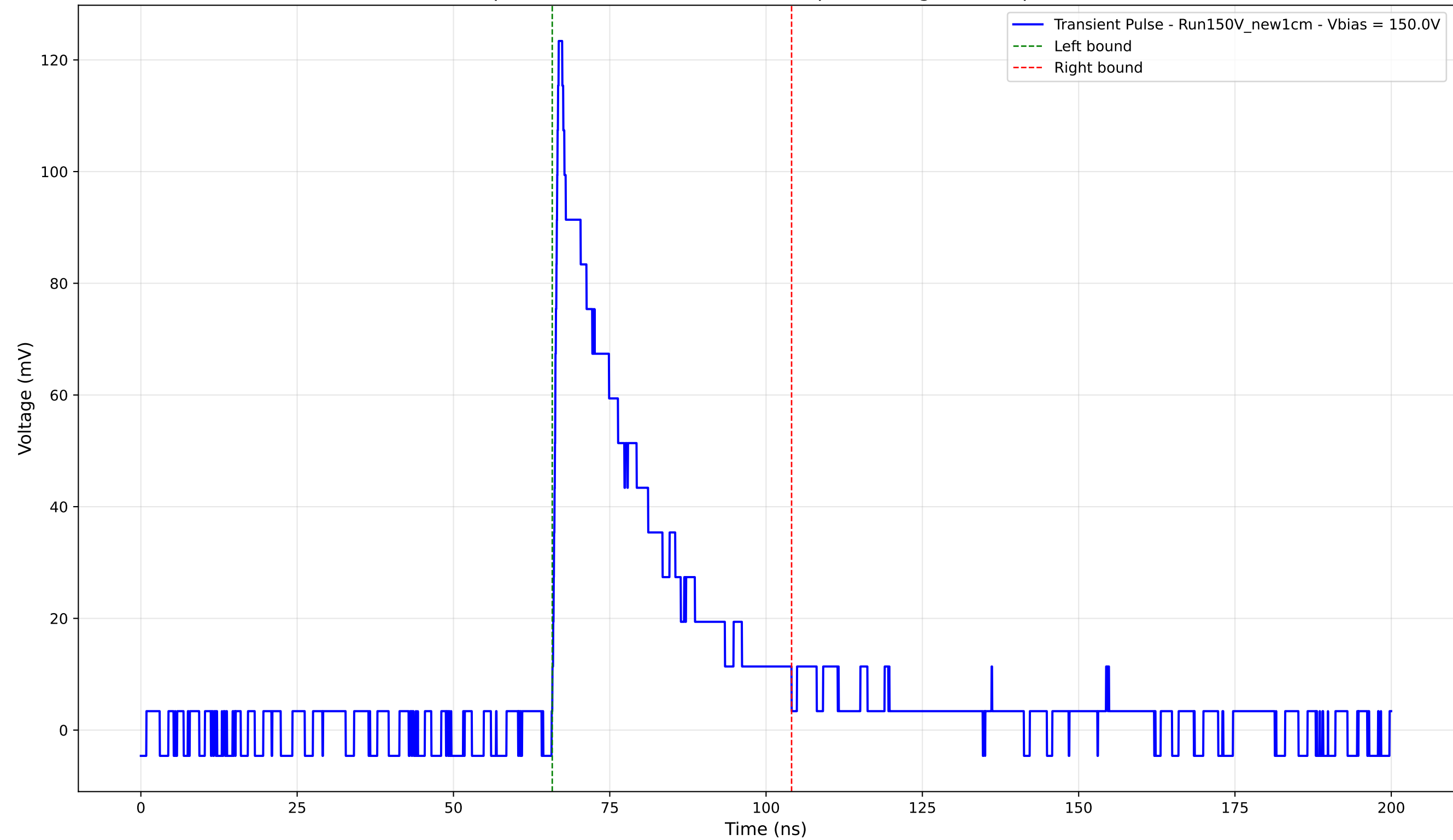
Transient Pulse - Sample: New1cm - Position: 2985.0 \mu\text{m} - Charge: 30.14 pC - Rise Time: 0.80 ns
