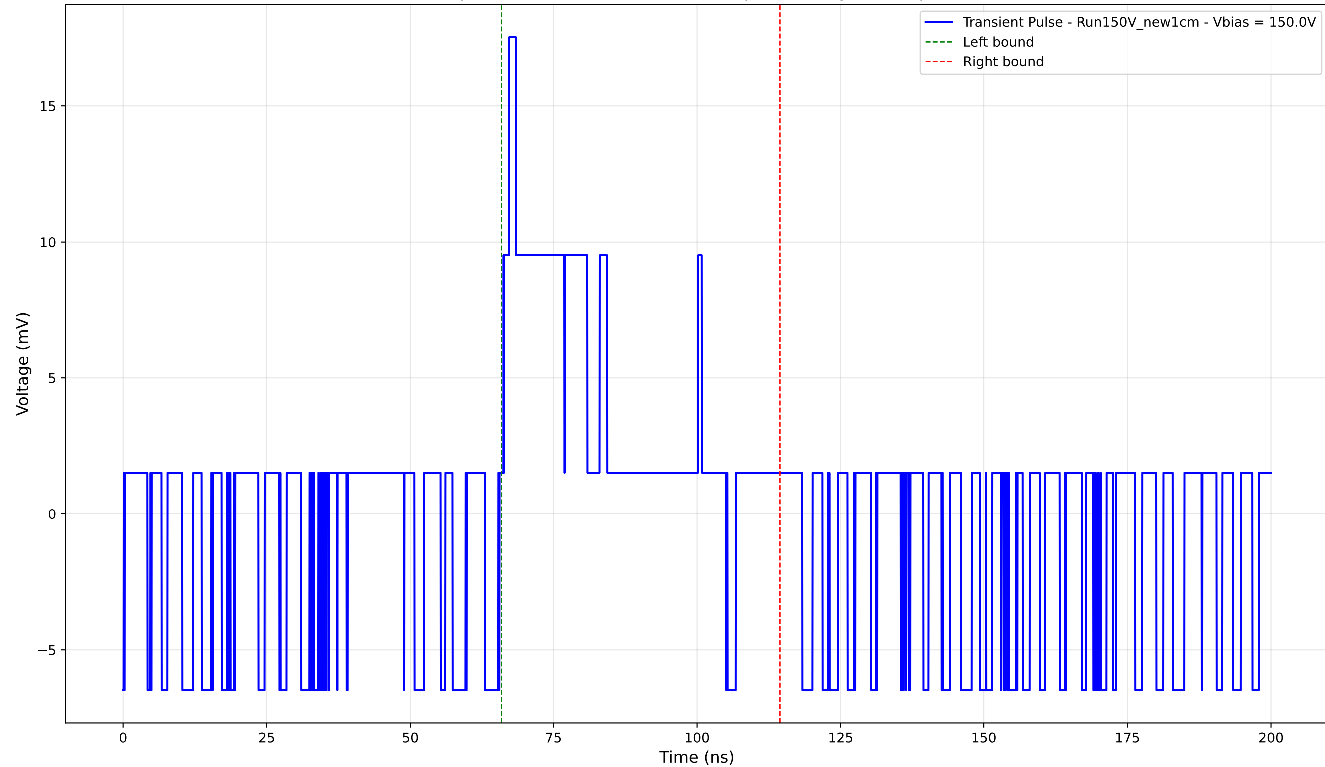
Transient Pulse - Sample: New1cm - Position: 535.0 \mu\text{m} - Charge: 4.04 pC - Rise Time: 0.88 ns
