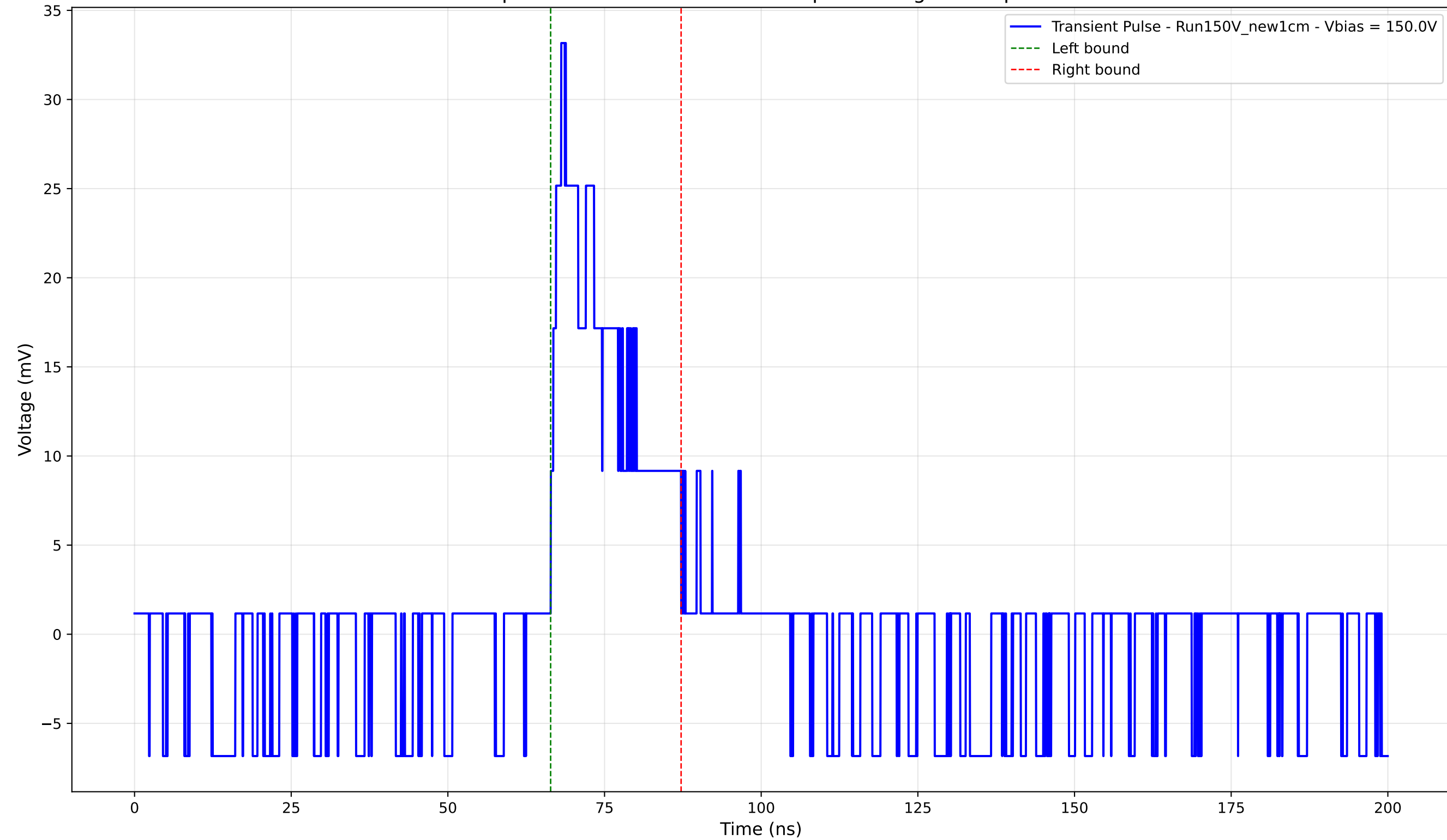
Transient Pulse - Sample: New1cm - Position: 555.0 \mu\text{m} - Charge: 6.56 pC - Rise Time: 1.67 ns
