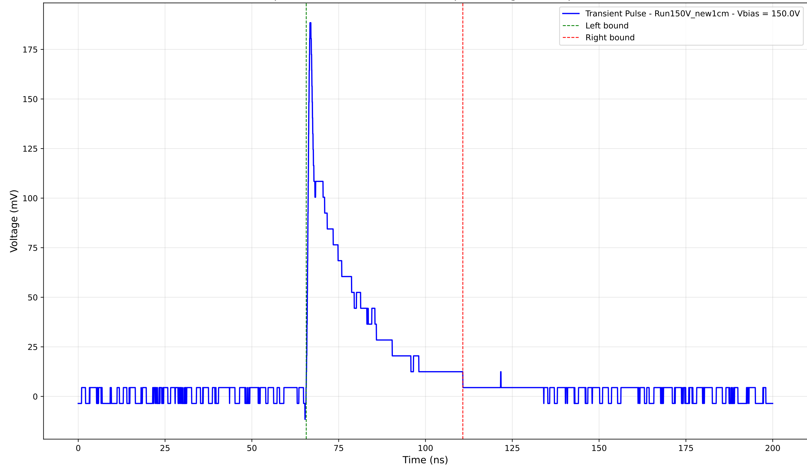
Transient Pulse - Sample: New1cm - Position: 2350.0 \mu\text{m} - Charge: 38.65 pC - Rise Time: 0.82 ns
