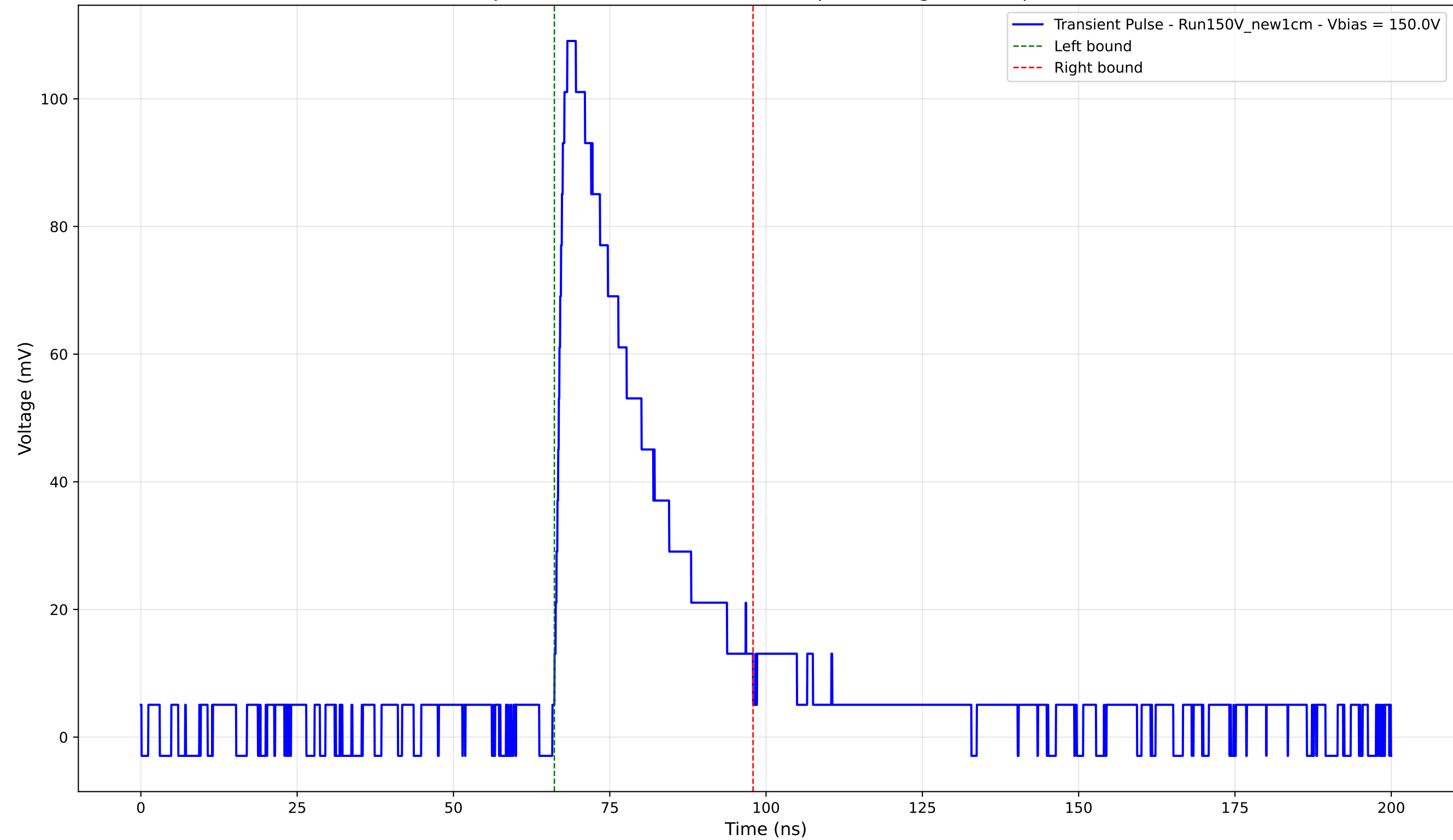
Transient Pulse - Sample: New1cm - Position: 1160.0 \mu\text{m} - Charge: 30.44 pC - Rise Time: 1.59 ns
