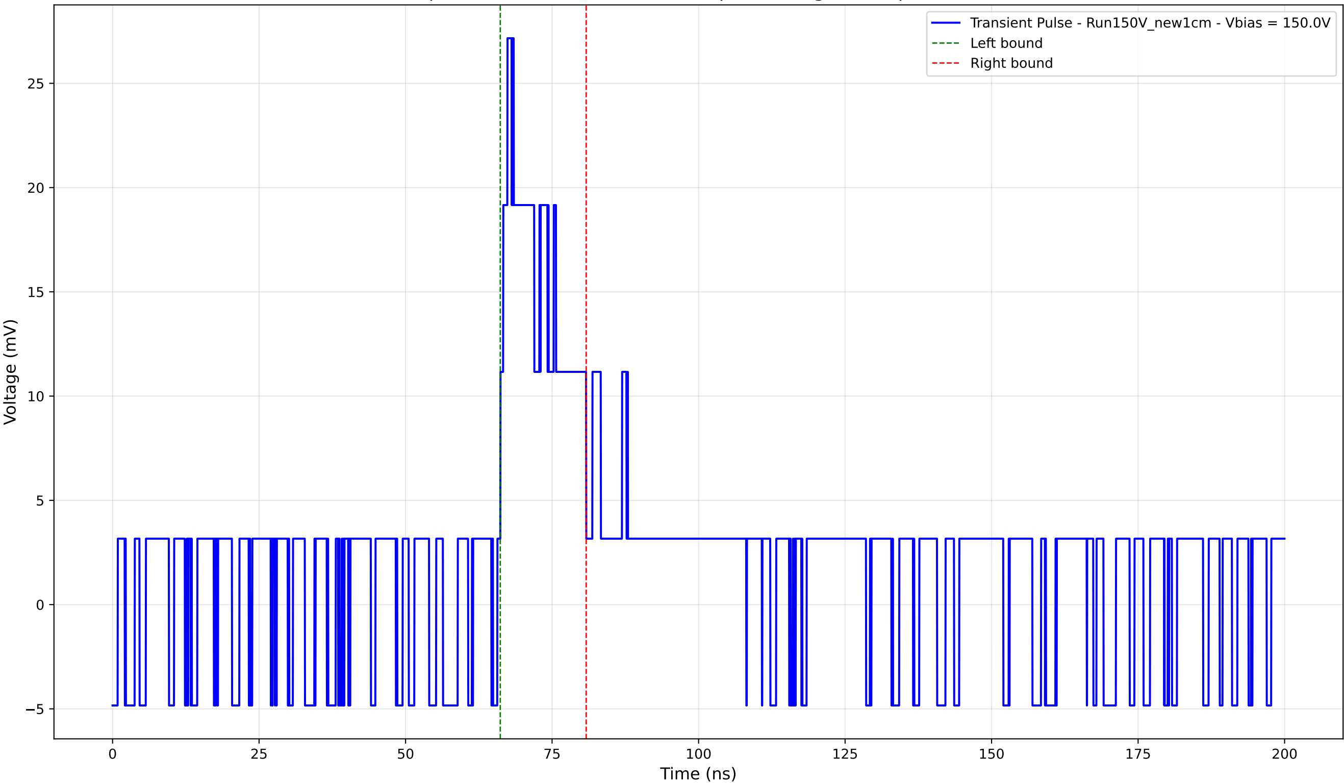
Transient Pulse - Sample: New1cm - Position: 510.0 \mu\text{m} - Charge: 4.54 pC - Rise Time: 0.00 ns (N/A)
