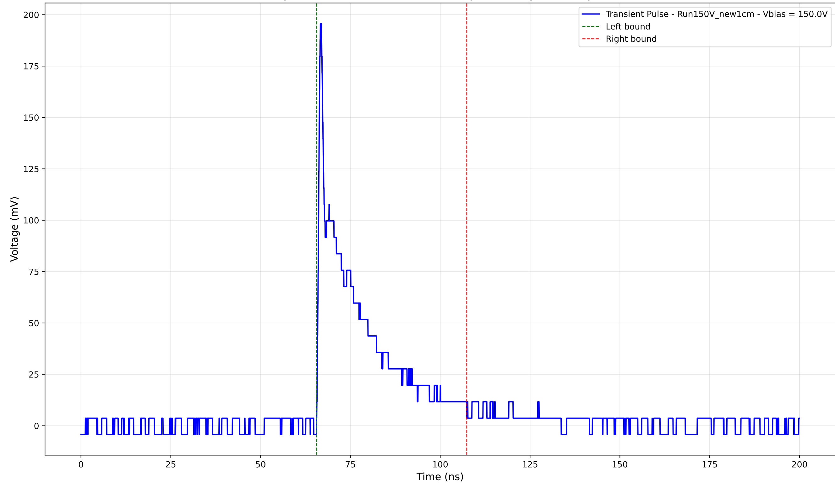
Transient Pulse - Sample: New1cm - Position: 2660.0 \mu\text{m} - Charge: 35.96 pC - Rise Time: 0.78 ns
