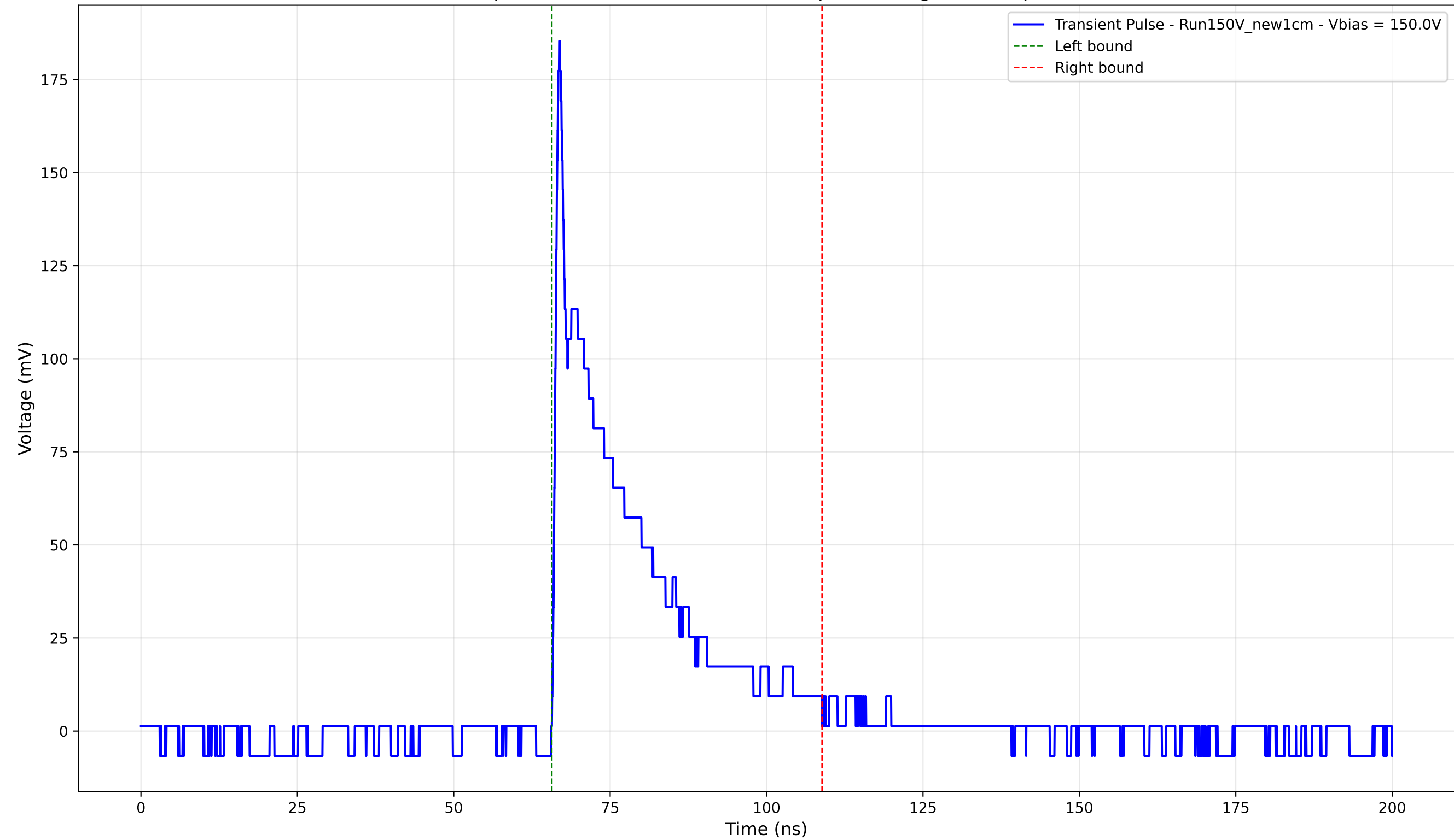
Transient Pulse - Sample: New1cm - Position: 2805.0 \mu\text{m} - Charge: 37.35 pC - Rise Time: 0.82 ns
