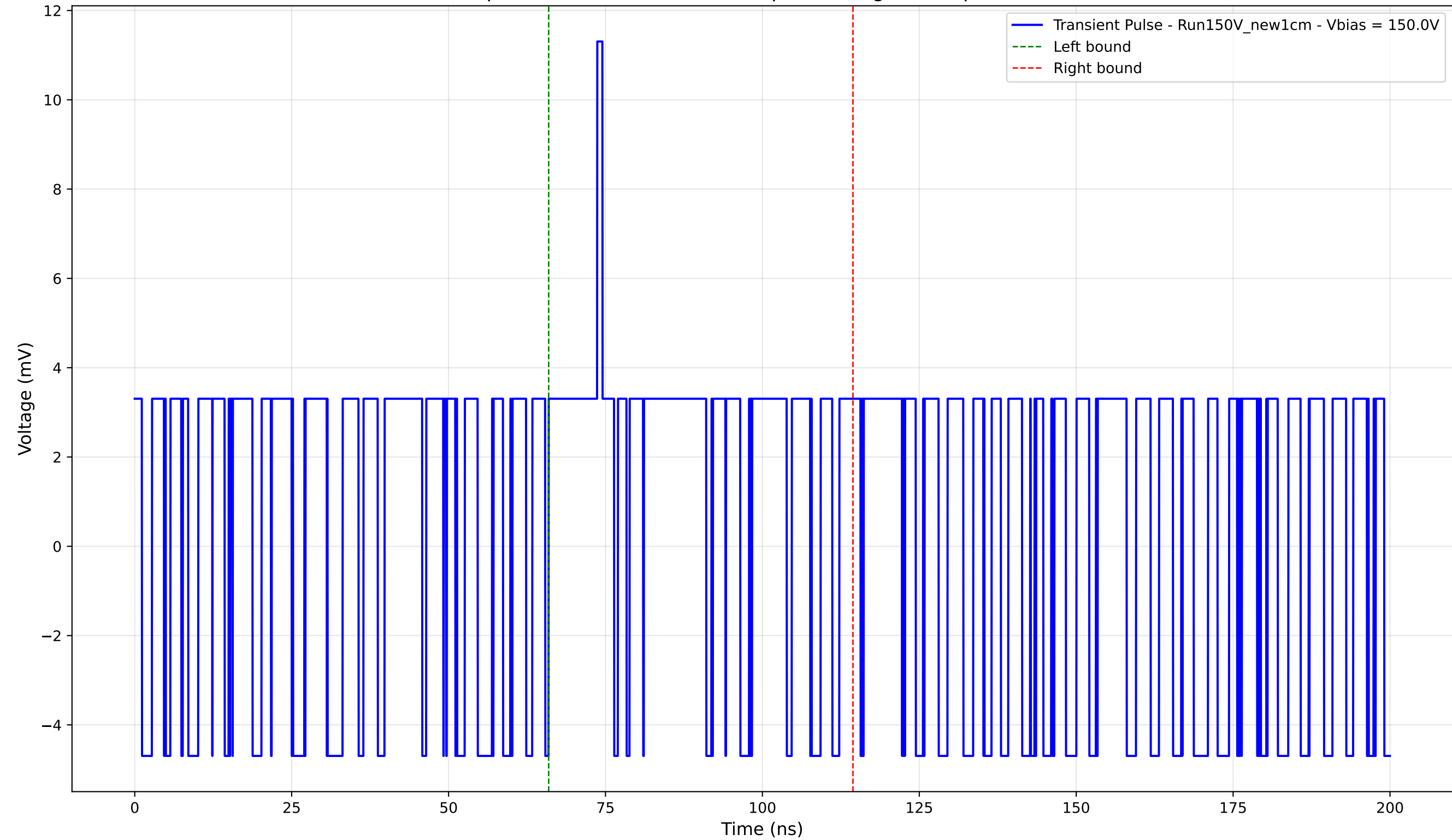
Transient Pulse - Sample: New1cm - Position: 5.0 \mu\text{m} - Charge: 2.15 pC - Rise Time: 0.00 ns (N/A)
