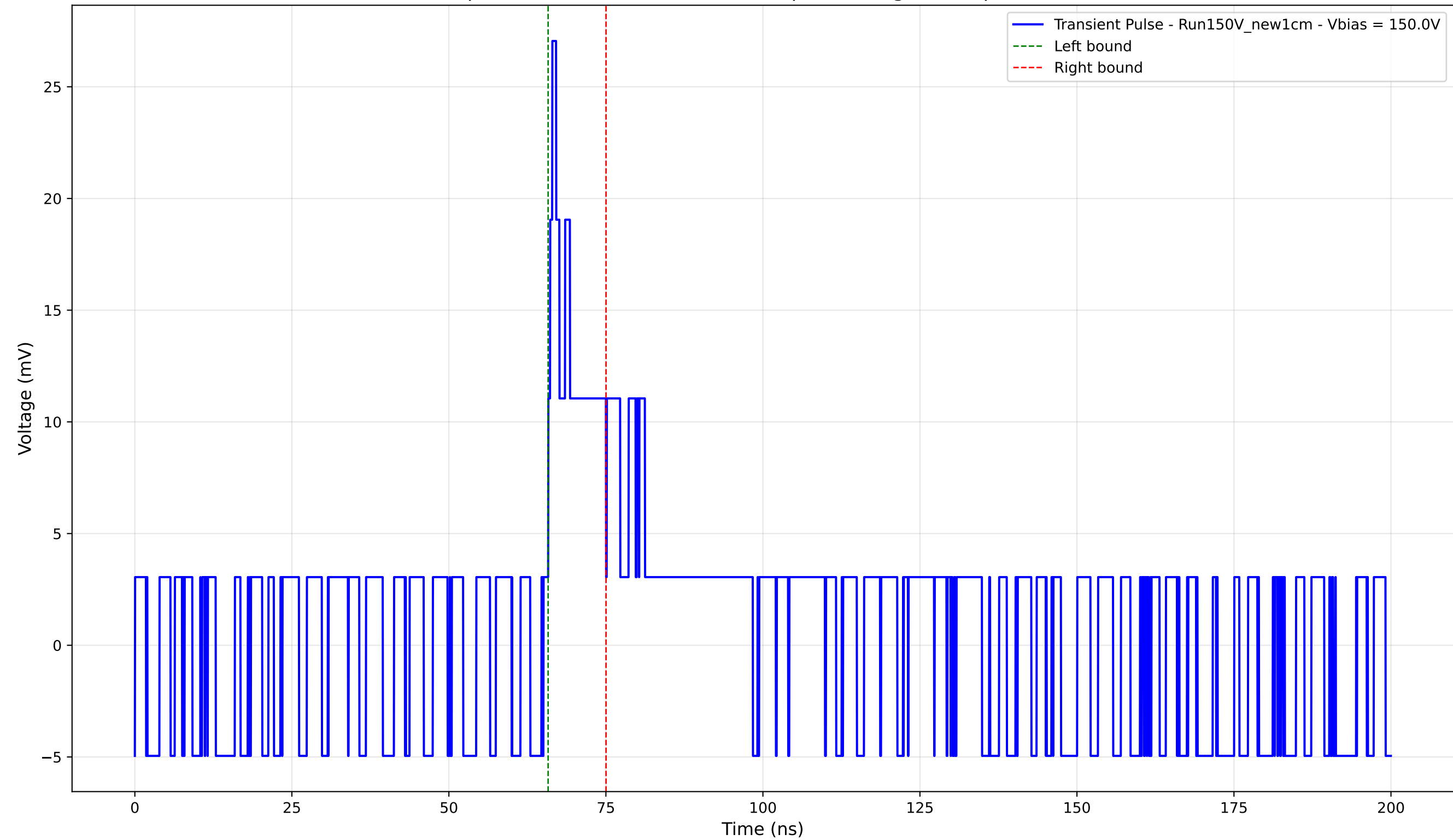
Transient Pulse - Sample: New1cm - Position: 2550.0 \mu\text{m} - Charge: 2.50 pC - Rise Time: 0.00 ns (N/A)
