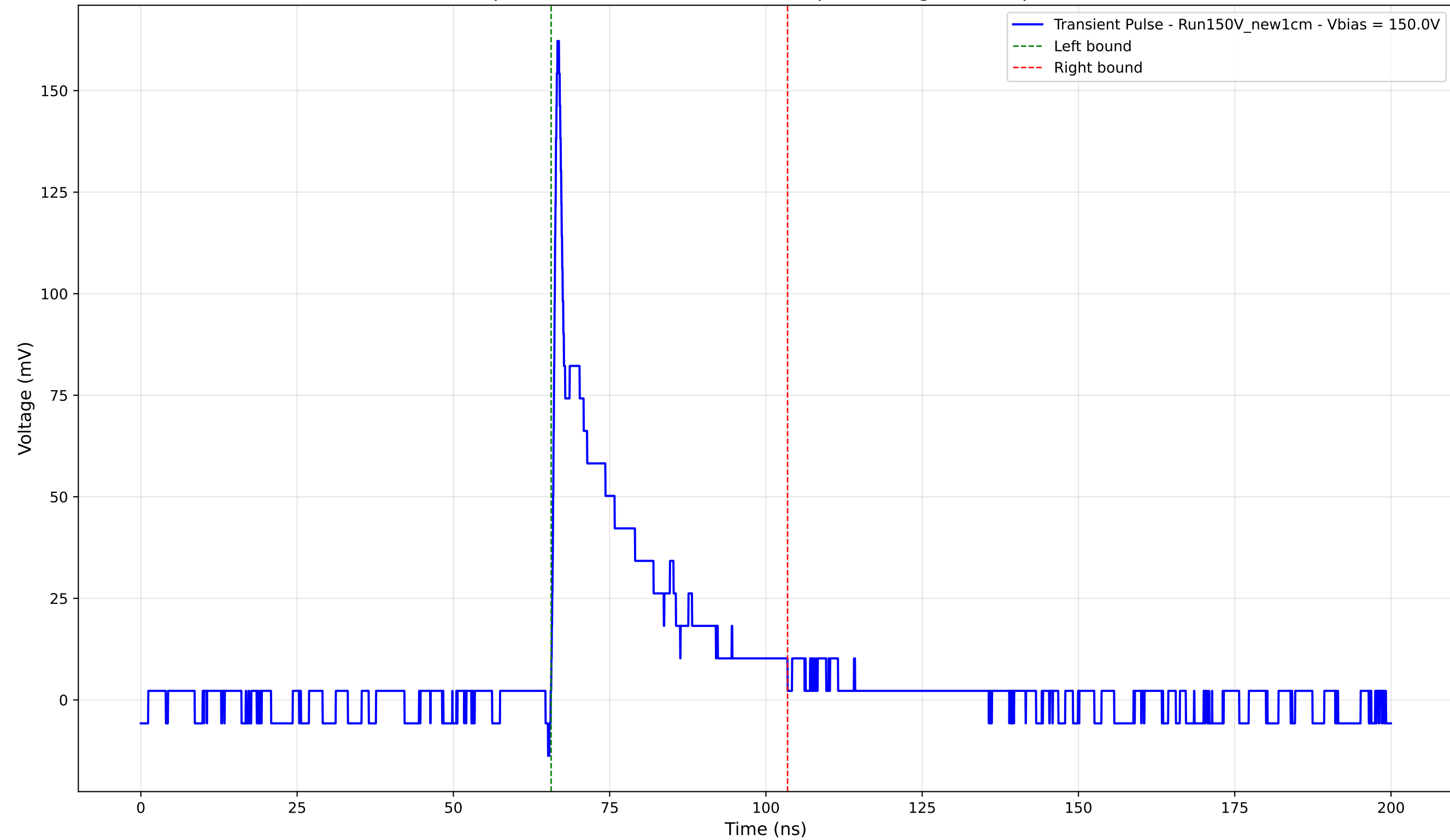
Transient Pulse - Sample: New1cm - Position: 2475.0 \mu\text{m} - Charge: 26.55 pC - Rise Time: 0.74 ns
