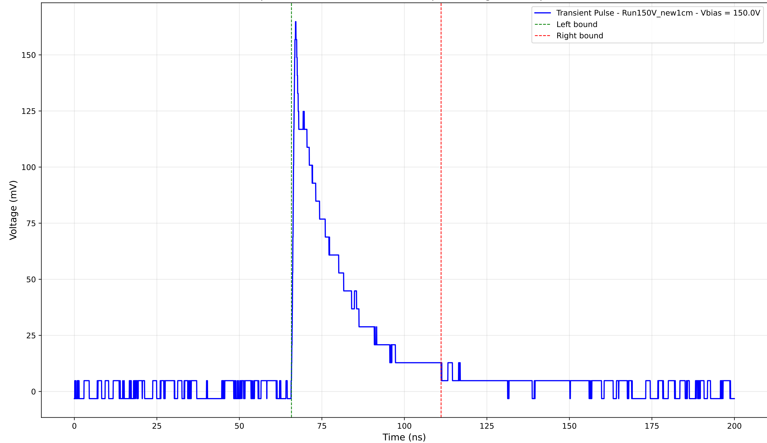
Transient Pulse - Sample: New1cm - Position: 2950.0 \mu\text{m} - Charge: 40.32 pC - Rise Time: 0.87 ns
