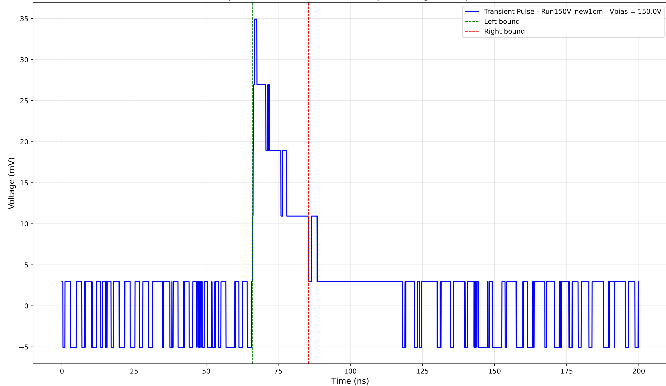
Transient Pulse - Sample: New1cm - Position: 2065.0 \mu\text{m} - Charge: 6.91 pC - Rise Time: 0.74 ns
