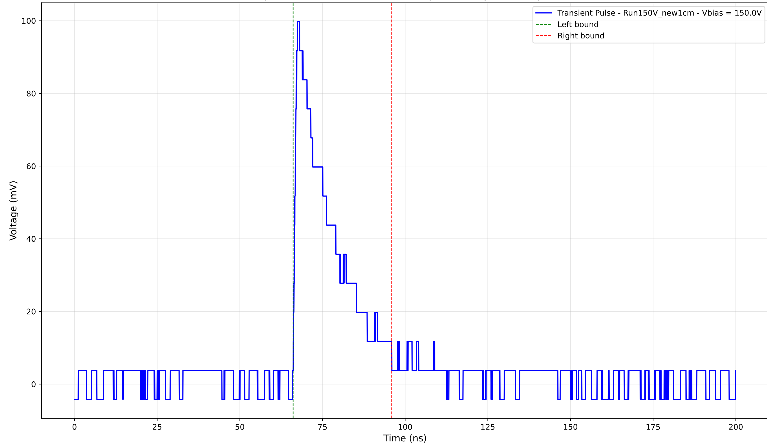
Transient Pulse - Sample: New1cm - Position: 615.0 \mu\text{m} - Charge: 23.39 pC - Rise Time: 1.08 ns
