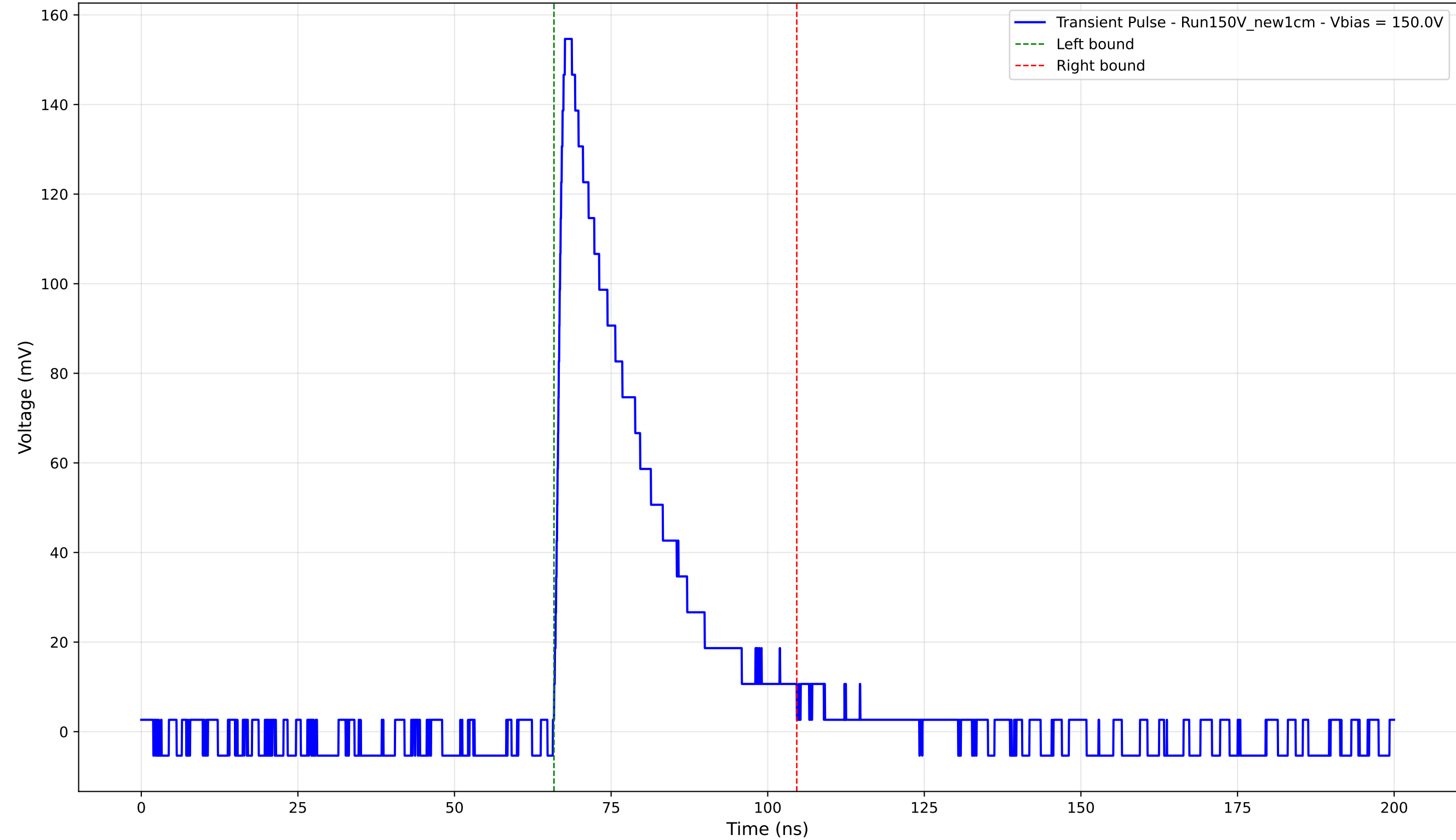
Transient Pulse - Sample: New1cm - Position: 4275.0 \mu\text{m} - Charge: 40.78 pC - Rise Time: 1.39 ns
