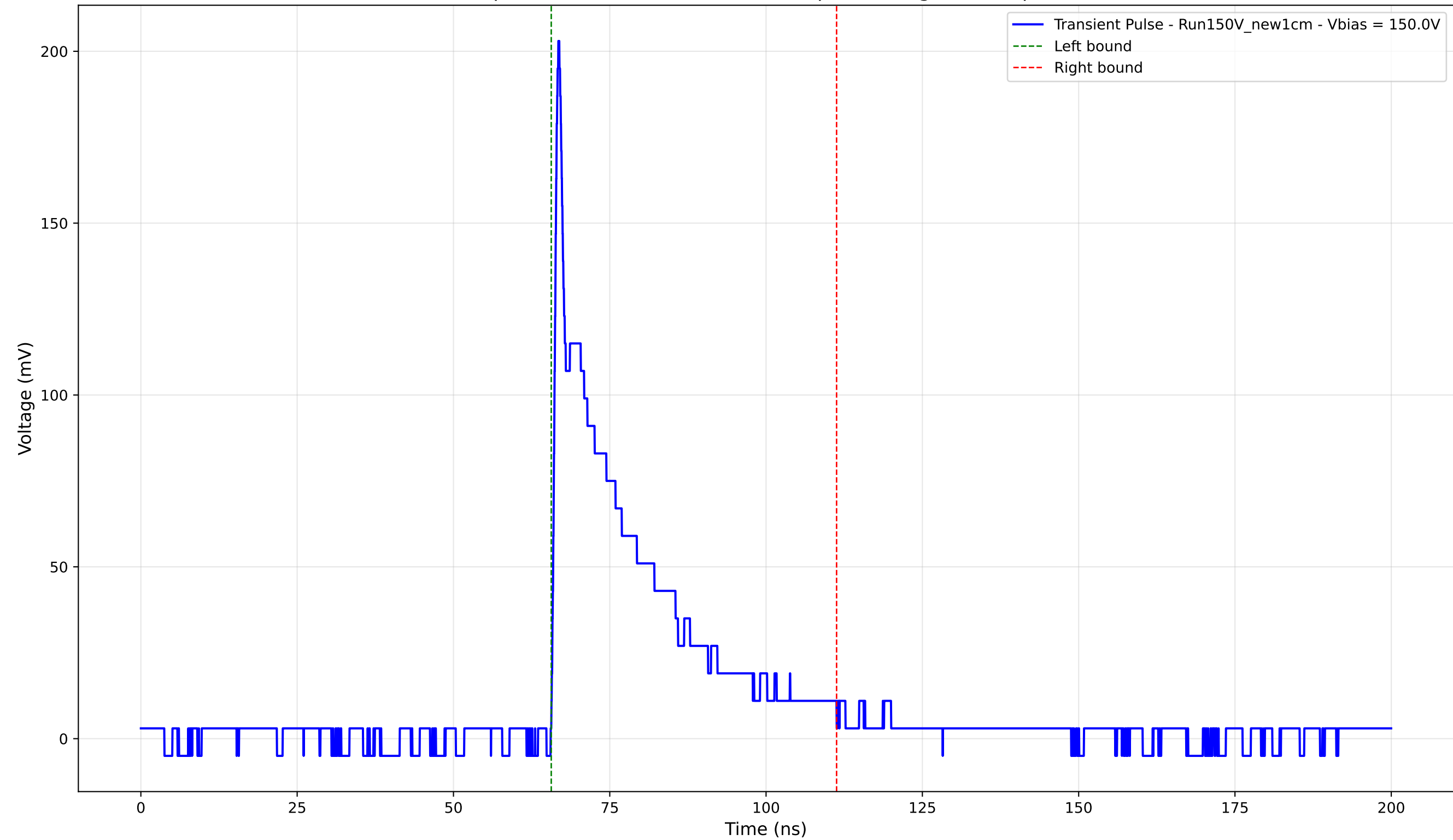
Transient Pulse - Sample: New1cm - Position: 2740.0 \mu\text{m} - Charge: 40.29 pC - Rise Time: 0.80 ns
