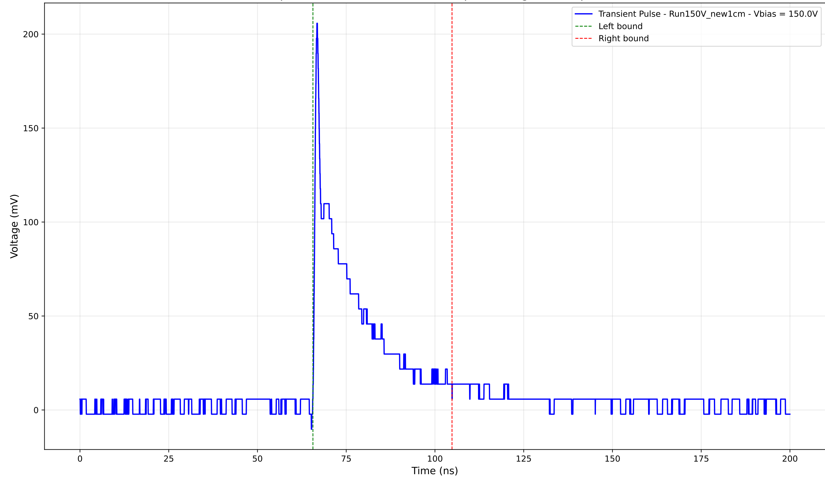
Transient Pulse - Sample: New1cm - Position: 2410.0 \mu\text{m} - Charge: 38.07 pC - Rise Time: 0.82 ns
