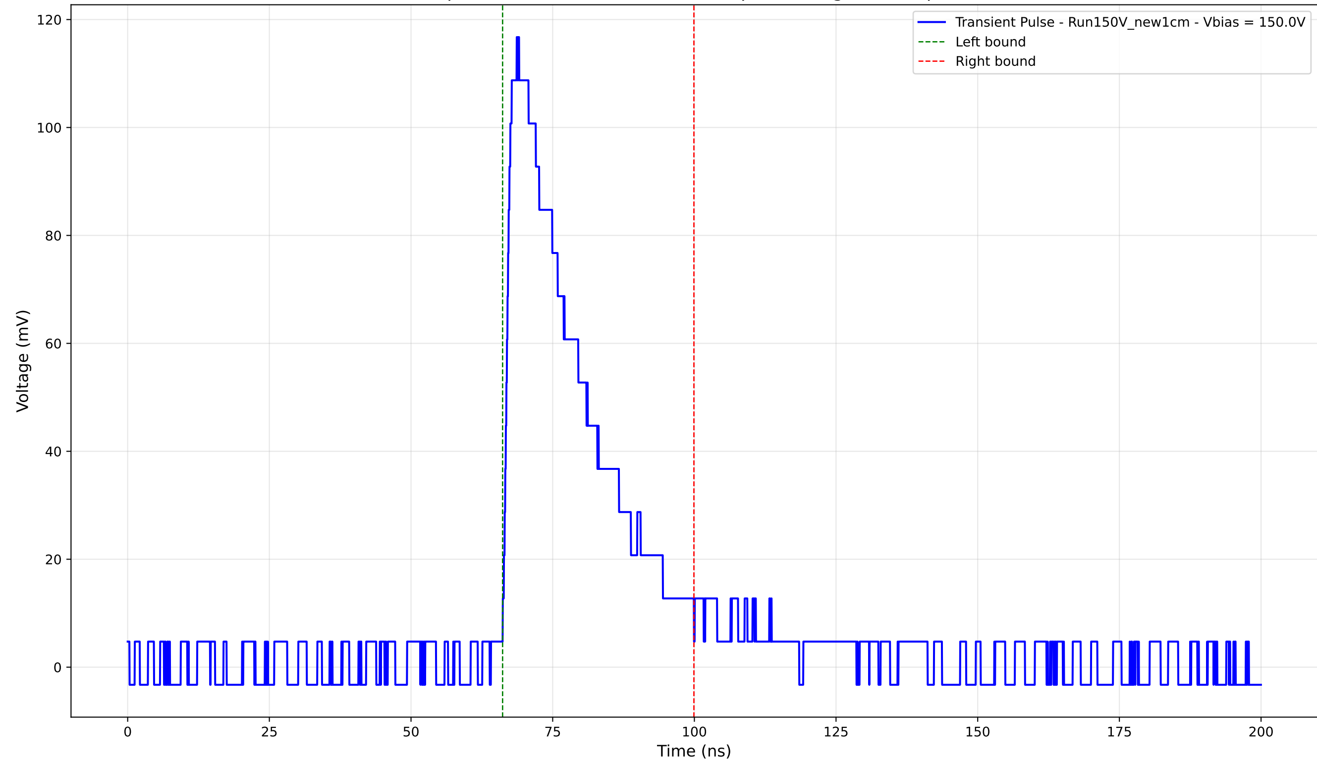
Transient Pulse - Sample: New1cm - Position: 1345.0 \mu\text{m} - Charge: 33.17 pC - Rise Time: 1.58 ns
