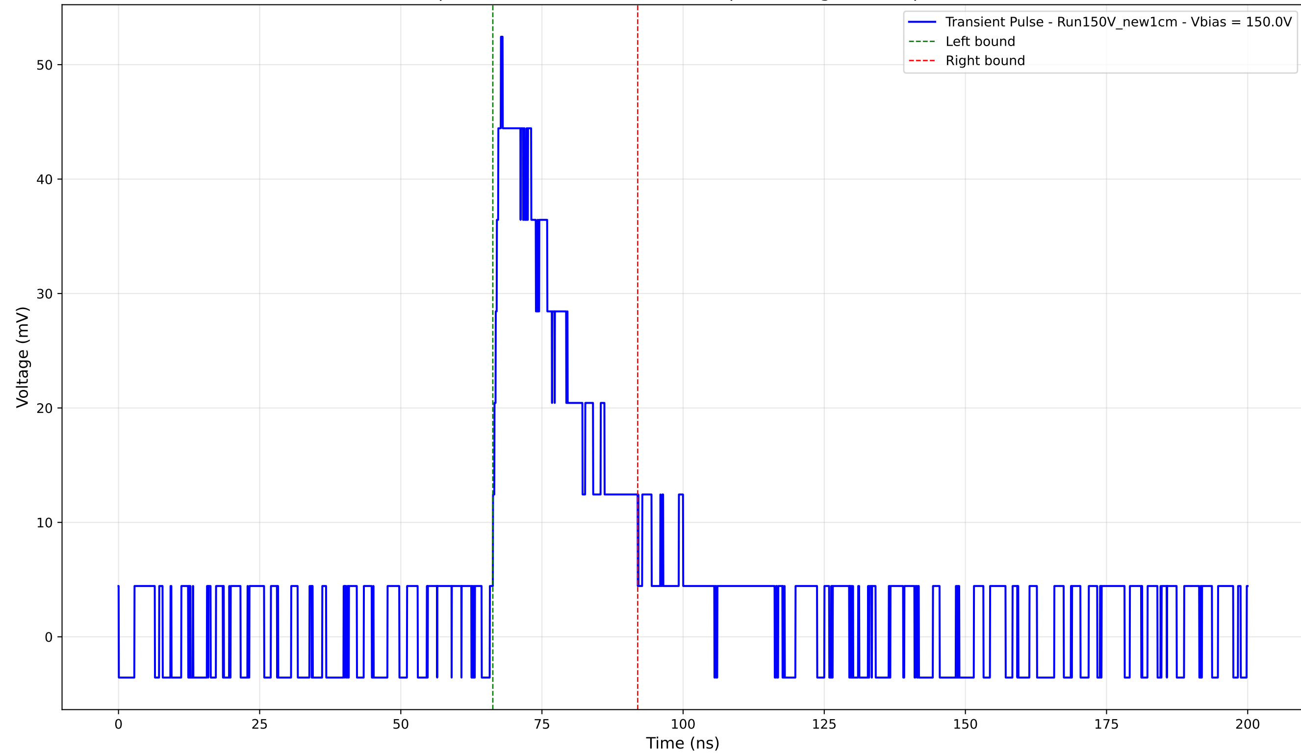
Transient Pulse - Sample: New1cm - Position: 1495.0 \mu\text{m} - Charge: 13.44 pC - Rise Time: 1.42 ns
