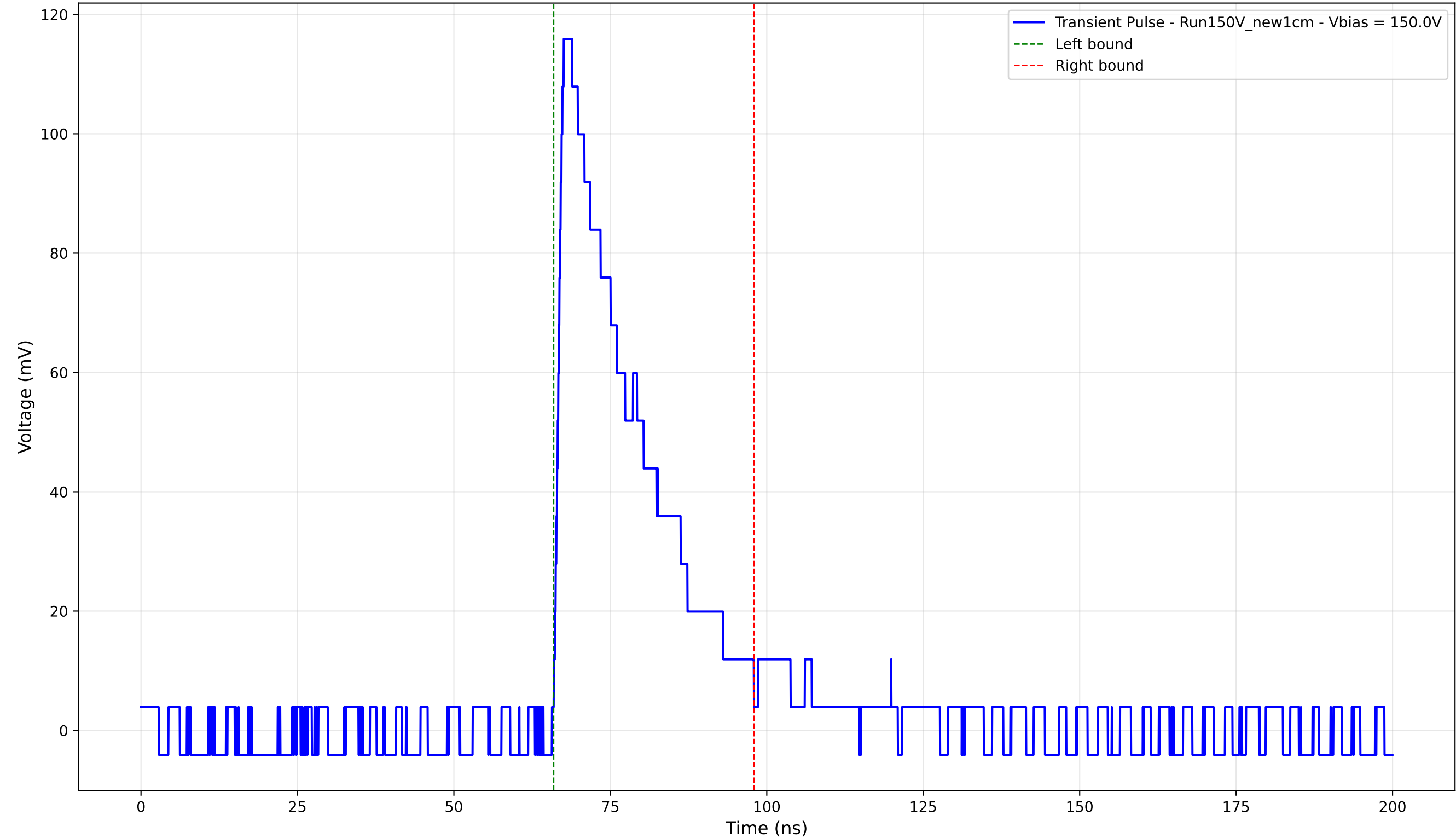
Transient Pulse - Sample: New1cm - Position: 4180.0 \mu\text{m} - Charge: 30.81 pC - Rise Time: 1.38 ns
