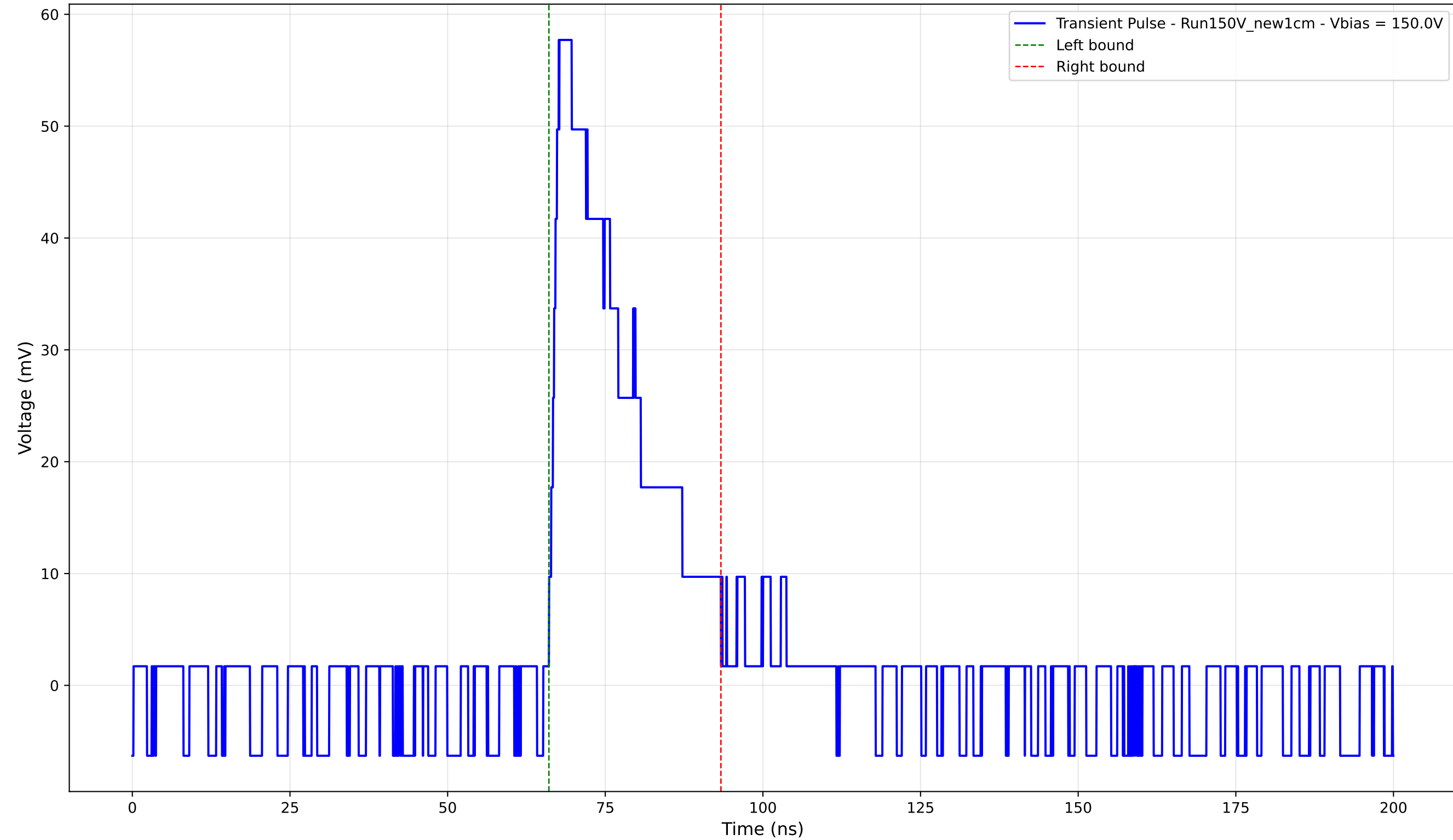
Transient Pulse - Sample: New1cm - Position: 1485.0 \mu\text{m} - Charge: 14.97 pC - Rise Time: 1.55 ns
