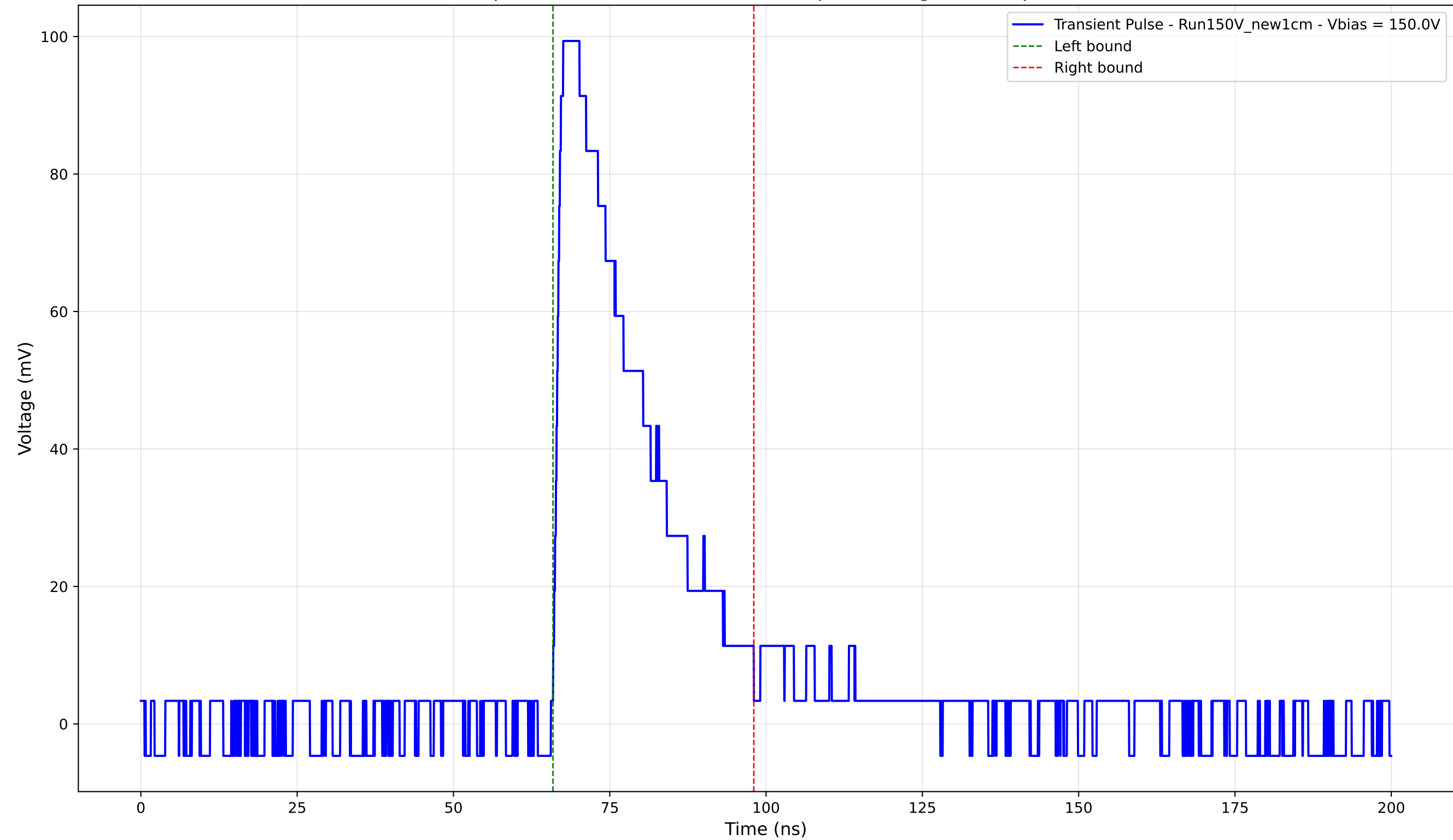
Transient Pulse - Sample: New1cm - Position: 1760.0 \mu\text{m} - Charge: 28.93 pC - Rise Time: 1.24 ns
