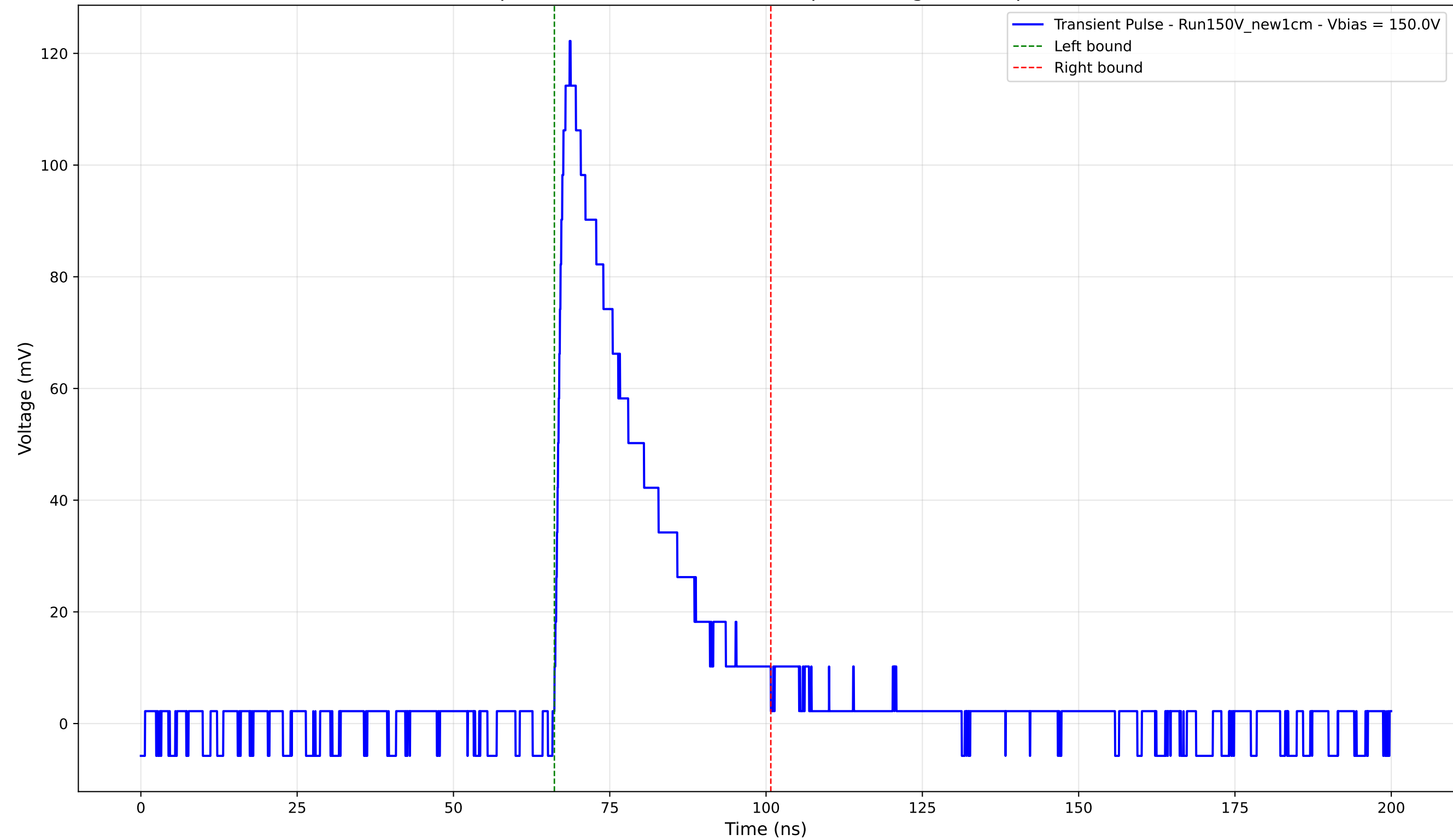
Transient Pulse - Sample: New1cm - Position: 880.0 \mu\text{m} - Charge: 30.80 pC - Rise Time: 1.63 ns
