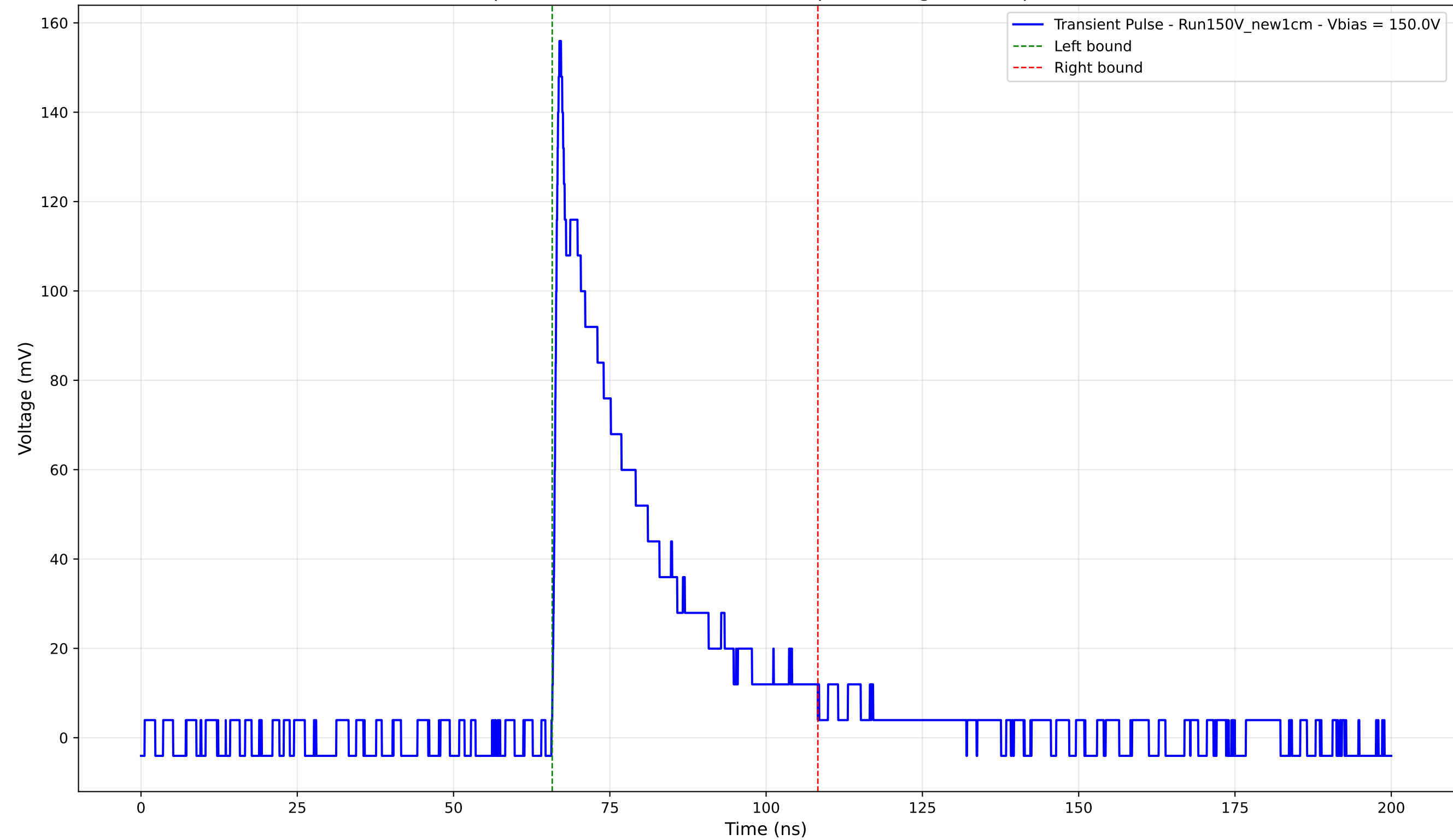
Transient Pulse - Sample: New1cm - Position: 2960.0 \mu\text{m} - Charge: 37.51 pC - Rise Time: 0.93 ns
