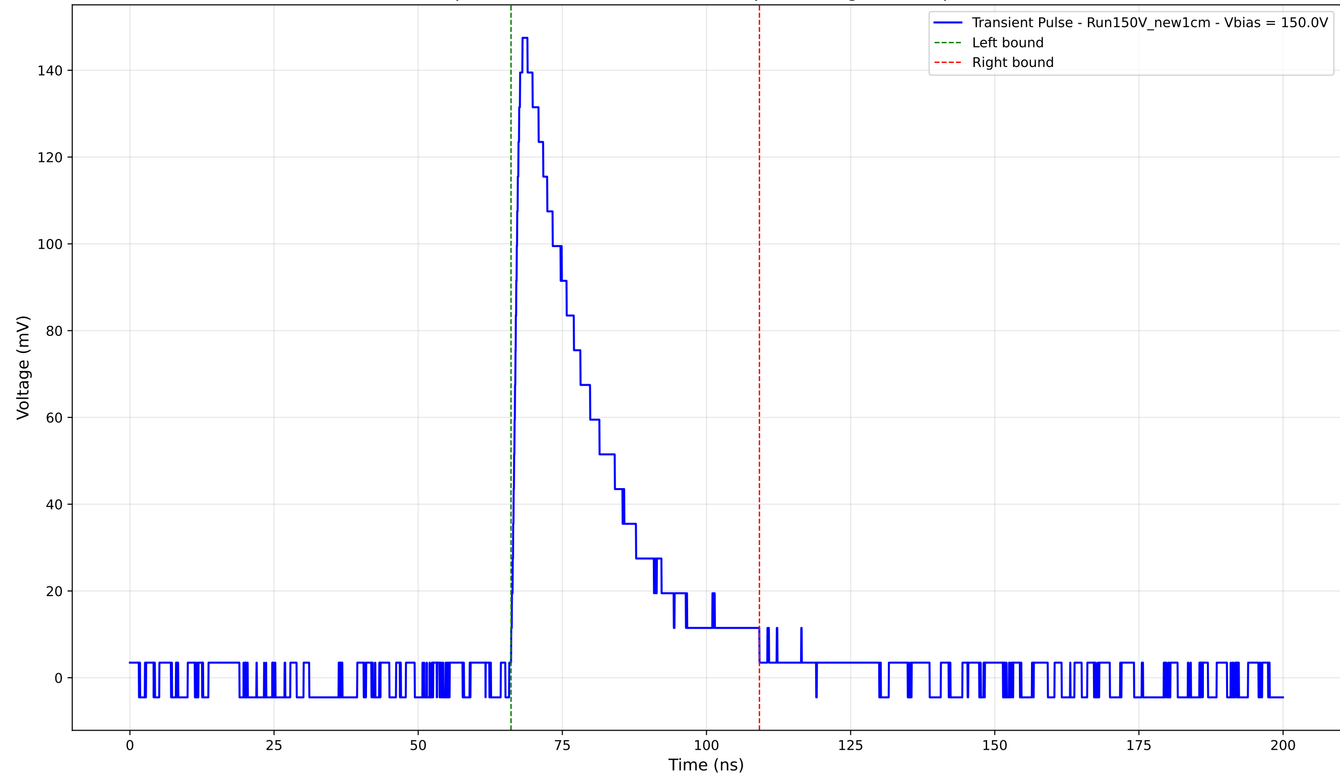
Transient Pulse - Sample: New1cm - Position: 3915.0 \mu\text{m} - Charge: 42.12 pC - Rise Time: 1.43 ns
