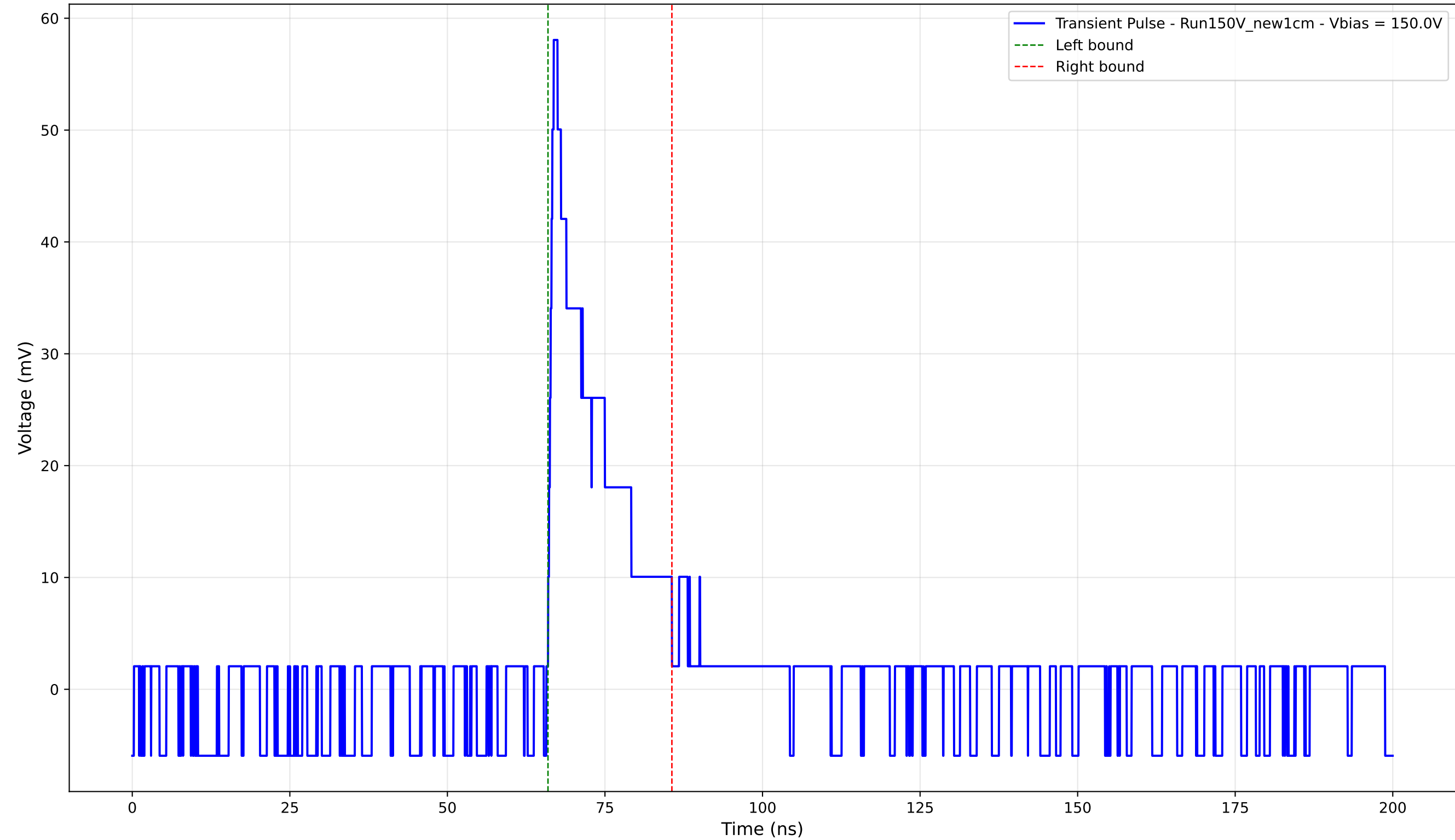
Transient Pulse - Sample: New1cm - Position: 75.0 \mu\text{m} - Charge: 8.91 pC - Rise Time: 0.89 ns
