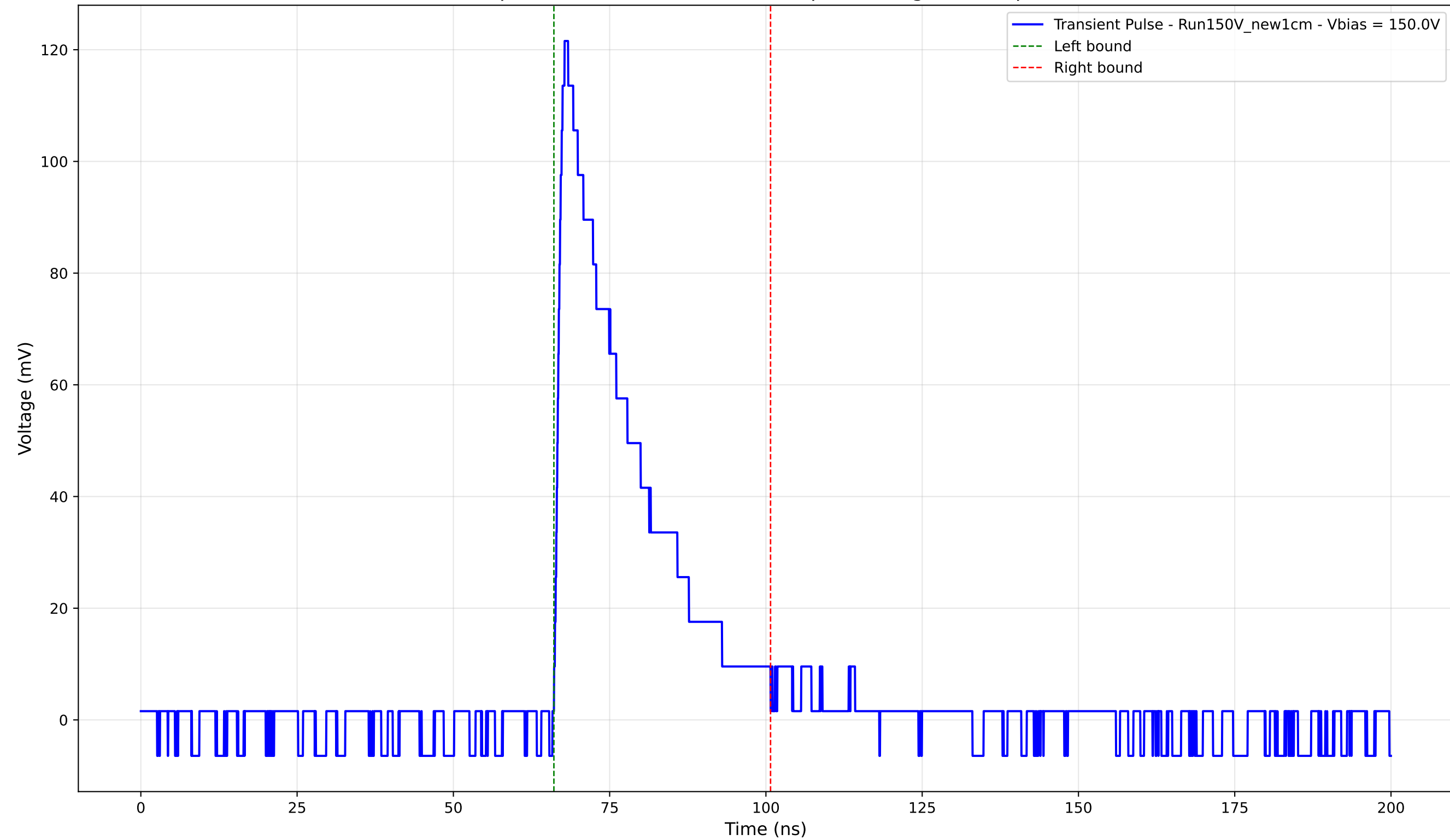
Transient Pulse - Sample: New1cm - Position: 695.0 \mu\text{m} - Charge: 29.66 pC - Rise Time: 1.23 ns
