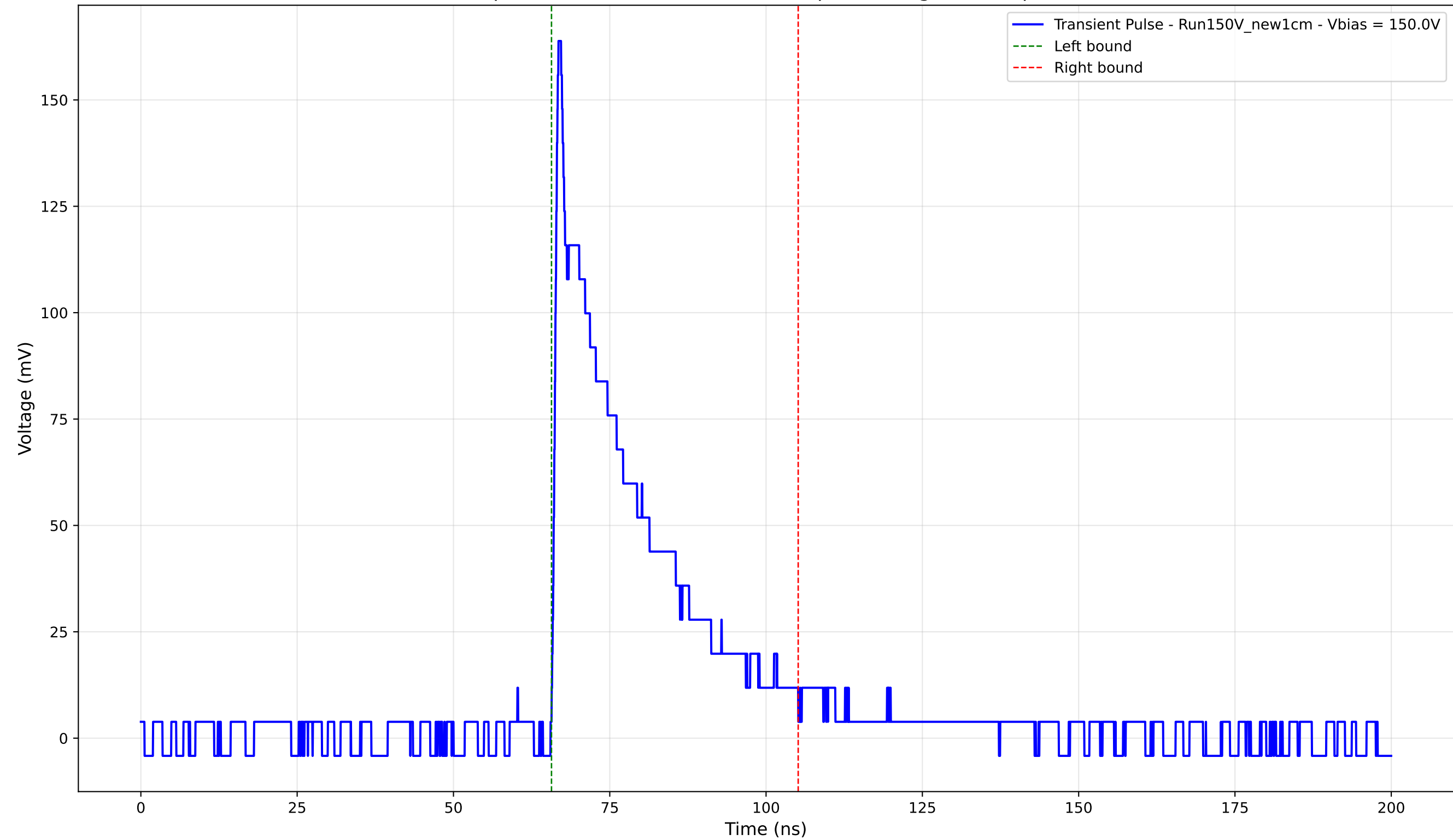
Transient Pulse - Sample: New1cm - Position: 2895.0 \mu\text{m} - Charge: 38.67 pC - Rise Time: 0.85 ns
