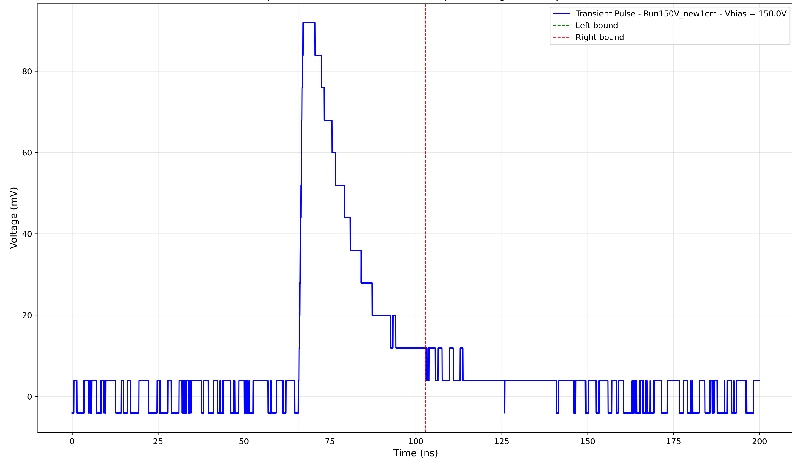
Transient Pulse - Sample: New1cm - Position: 1825.0 \mu\text{m} - Charge: 29.20 pC - Rise Time: 1.01 ns
