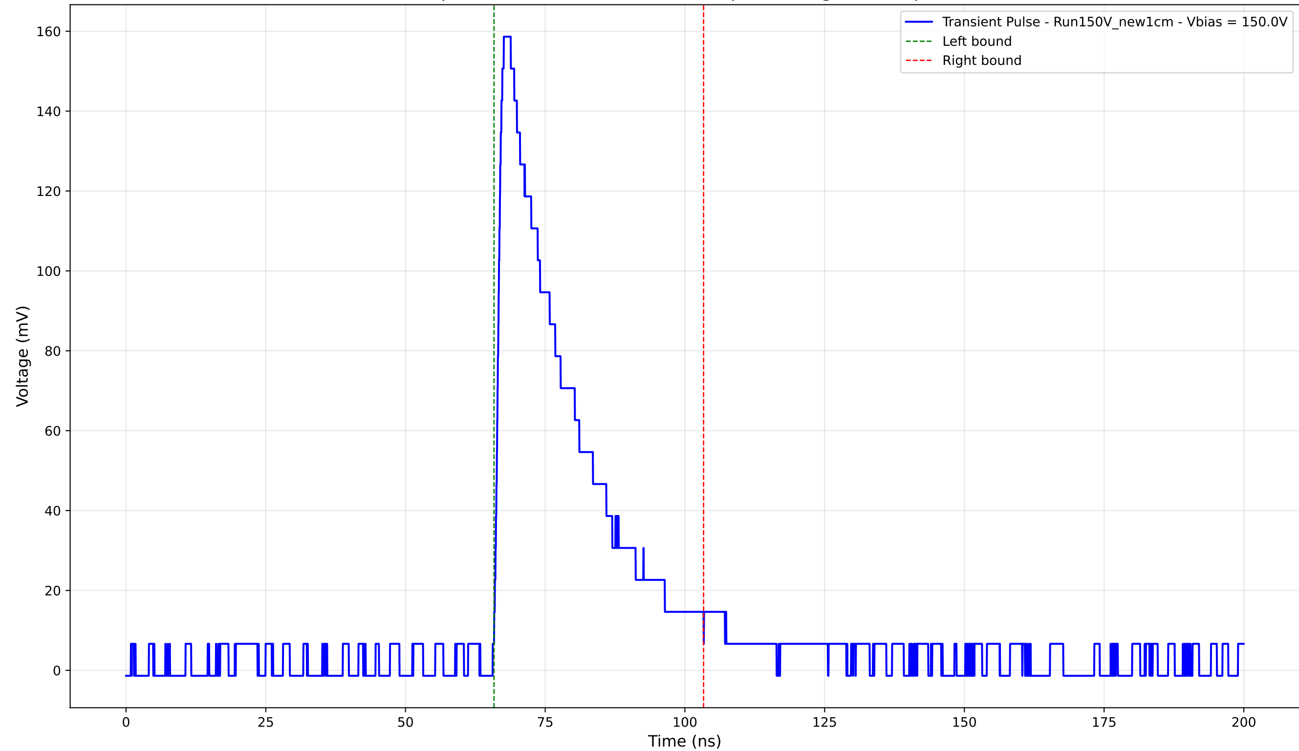
Transient Pulse - Sample: New1cm - Position: 4335.0 \mu\text{m} - Charge: 44.03 pC - Rise Time: 1.36 ns
