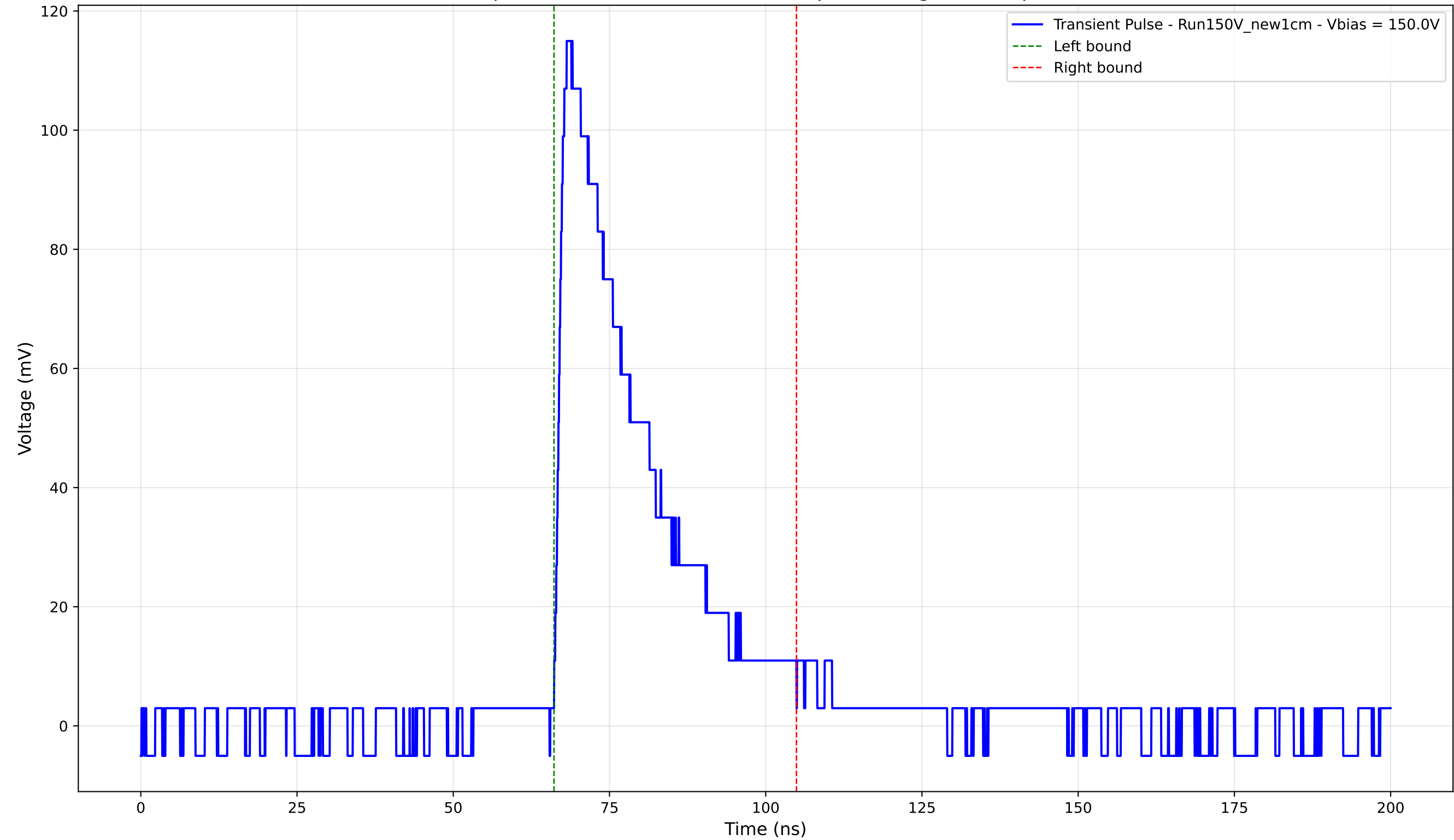
Transient Pulse - Sample: New1cm - Position: 1295.0 \mu\text{m} - Charge: 32.68 pC - Rise Time: 1.46 ns
