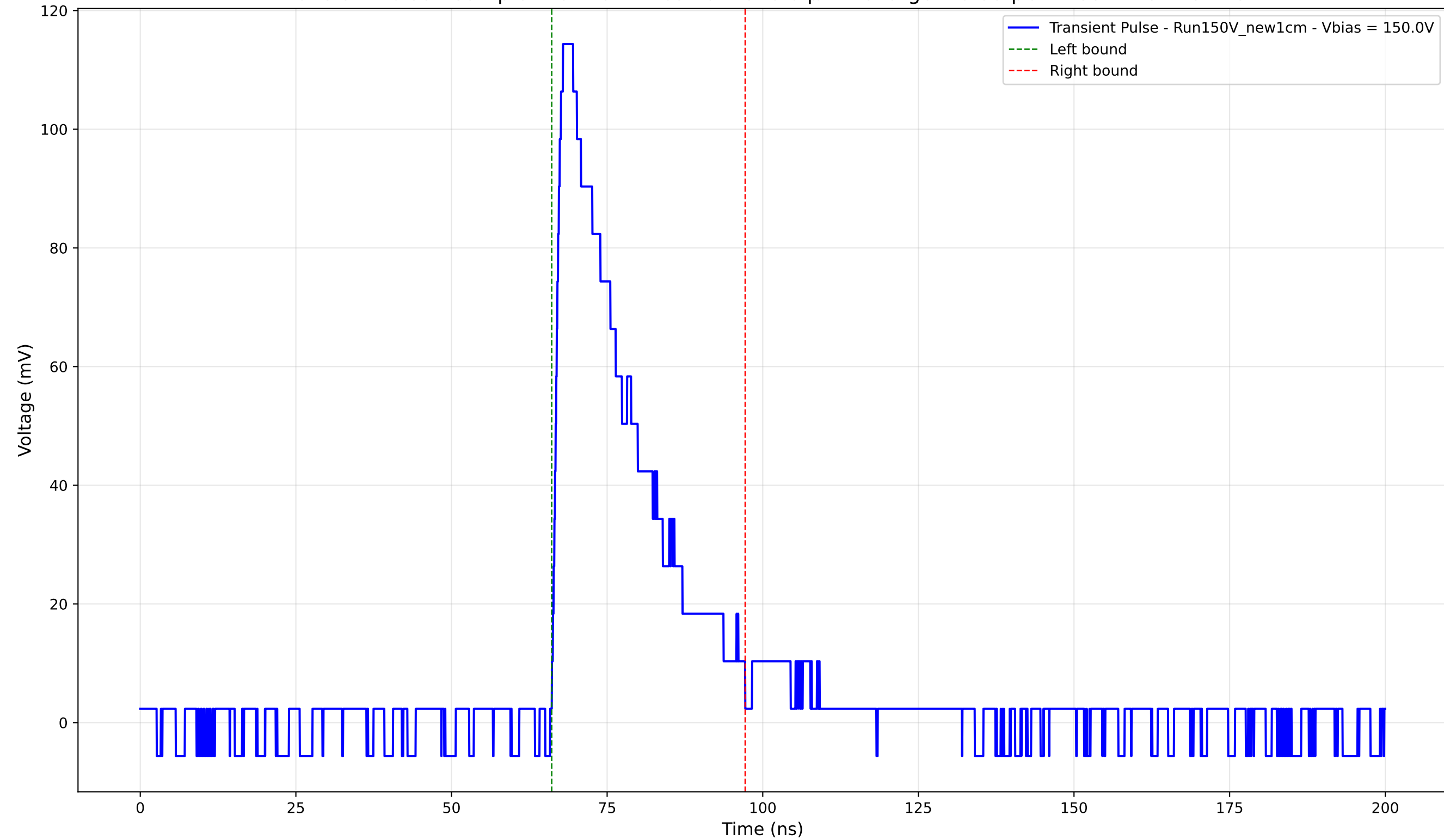
Transient Pulse - Sample: New1cm - Position: 840.0 \mu\text{m} - Charge: 29.55 pC - Rise Time: 1.32 ns
