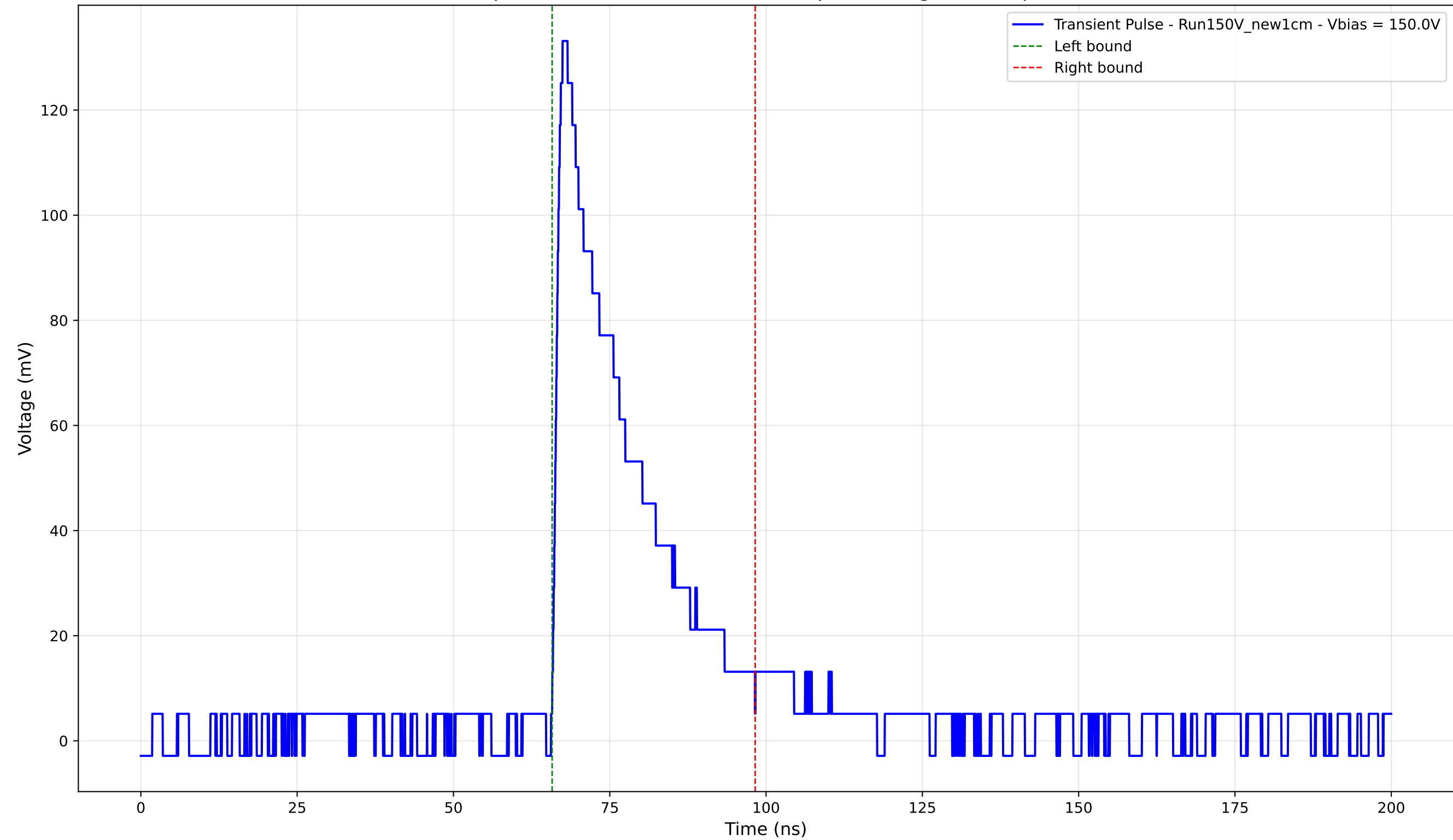
Transient Pulse - Sample: New1cm - Position: 4485.0 \mu\text{m} - Charge: 33.13 pC - Rise Time: 1.26 ns
