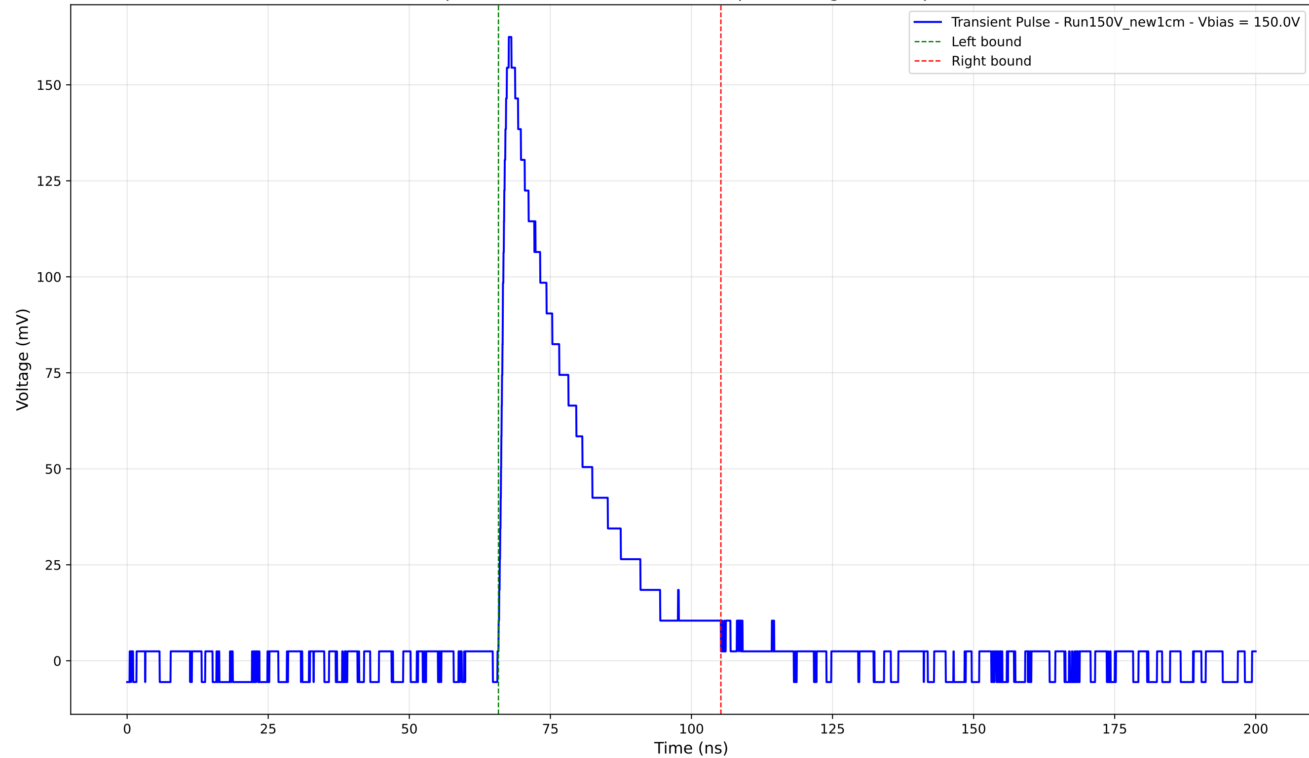
Transient Pulse - Sample: New1cm - Position: 4410.0 \mu\text{m} - Charge: 40.71 pC - Rise Time: 1.23 ns
