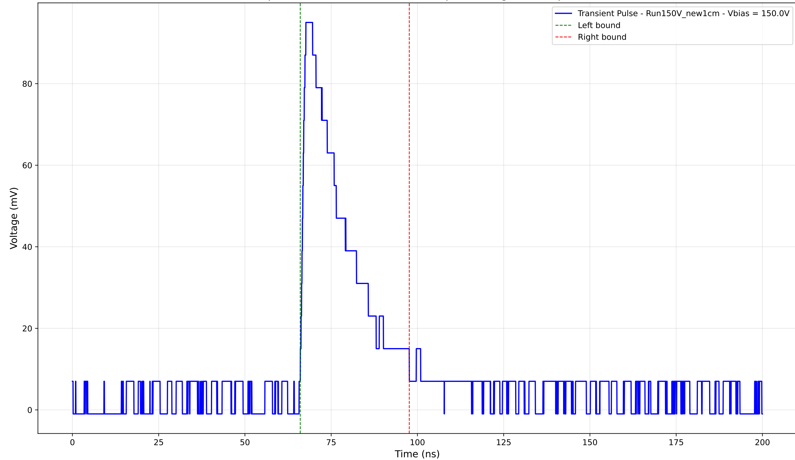
Transient Pulse - Sample: New1cm - Position: 4145.0 \mu\text{m} - Charge: 26.51 pC - Rise Time: 1.35 ns
