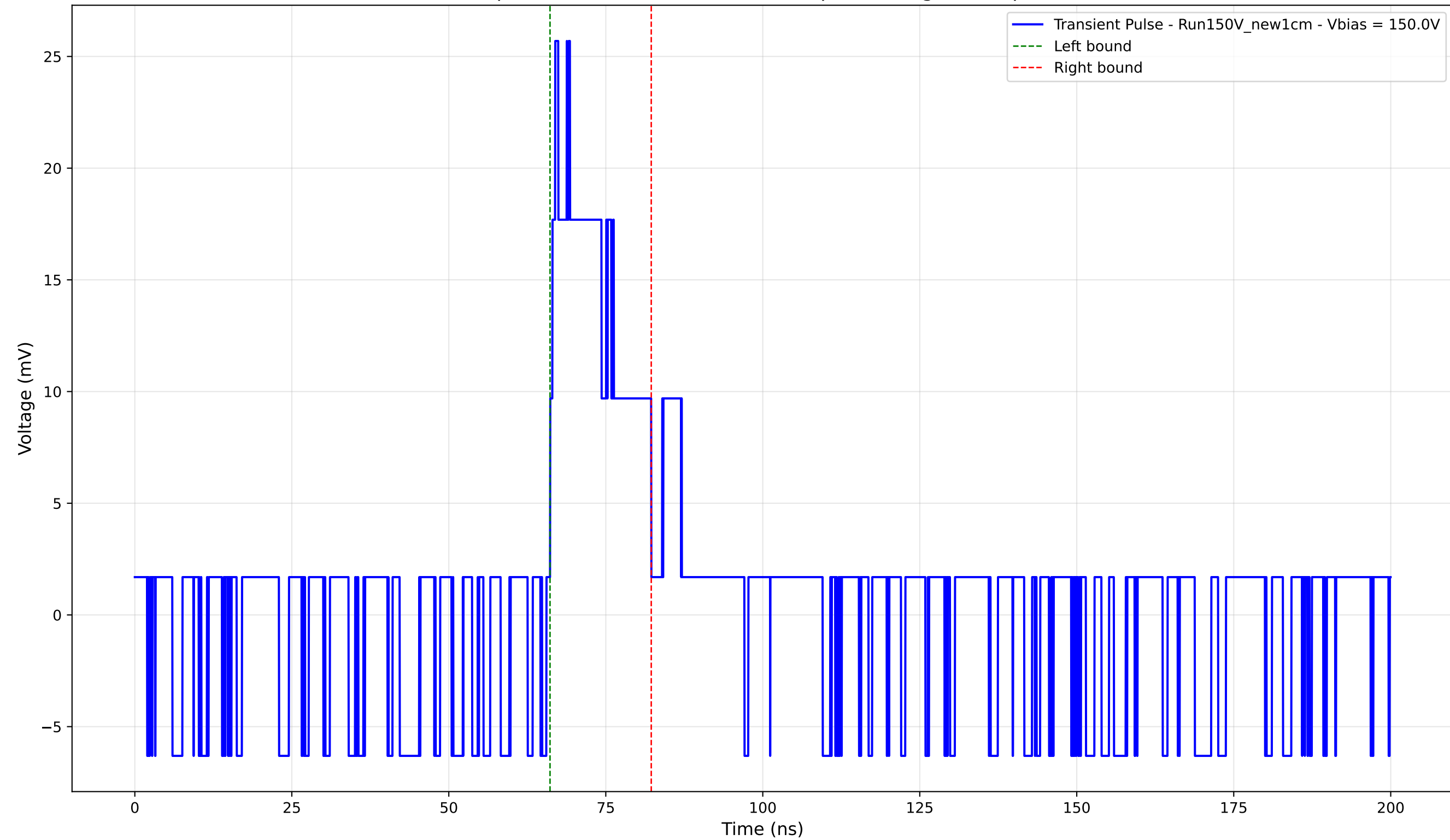
Transient Pulse - Sample: New1cm - Position: 3045.0 \mu\text{m} - Charge: 4.64 pC - Rise Time: 0.82 ns
