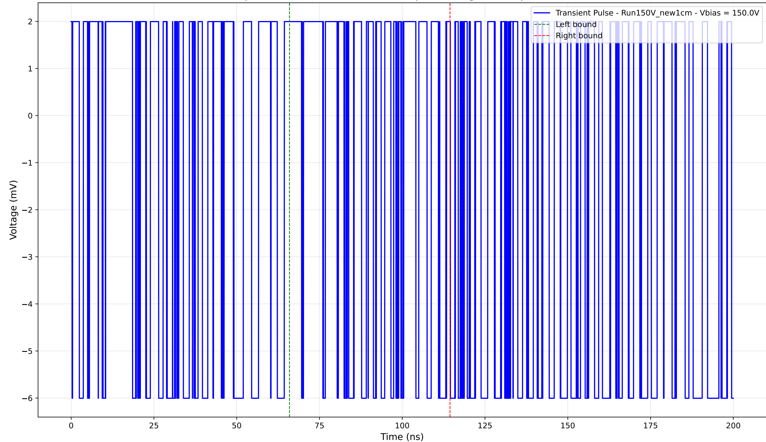
Transient Pulse - Sample: New1cm - Position: 4970.0 \mu\text{m} - Charge: -0.27 pC - Rise Time: 0.00 ns (N/A)
