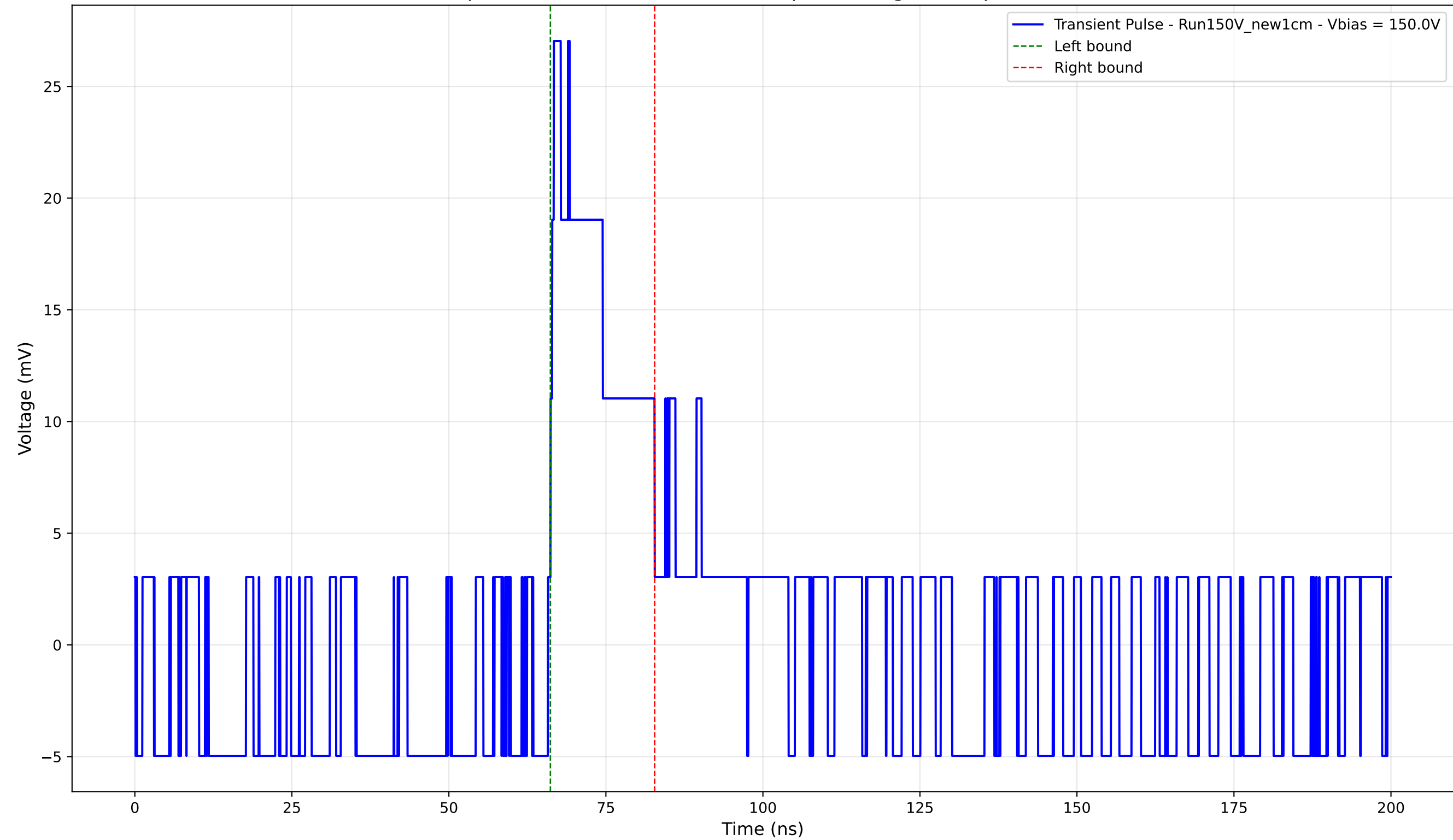
Transient Pulse - Sample: New1cm - Position: 2060.0 \mu\text{m} - Charge: 5.15 pC - Rise Time: 0.00 ns (N/A)
