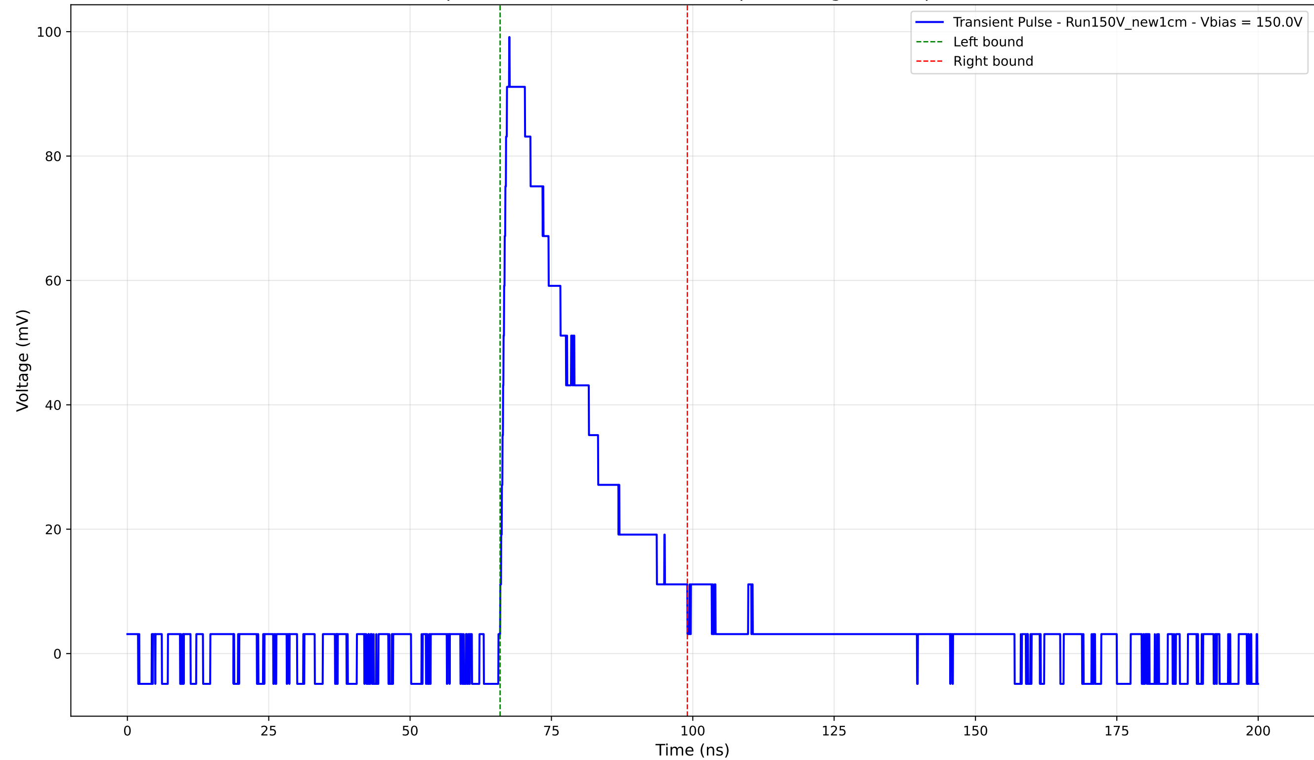
Transient Pulse - Sample: New1cm - Position: 1855.0 \mu\text{m} - Charge: 27.23 pC - Rise Time: 1.18 ns
