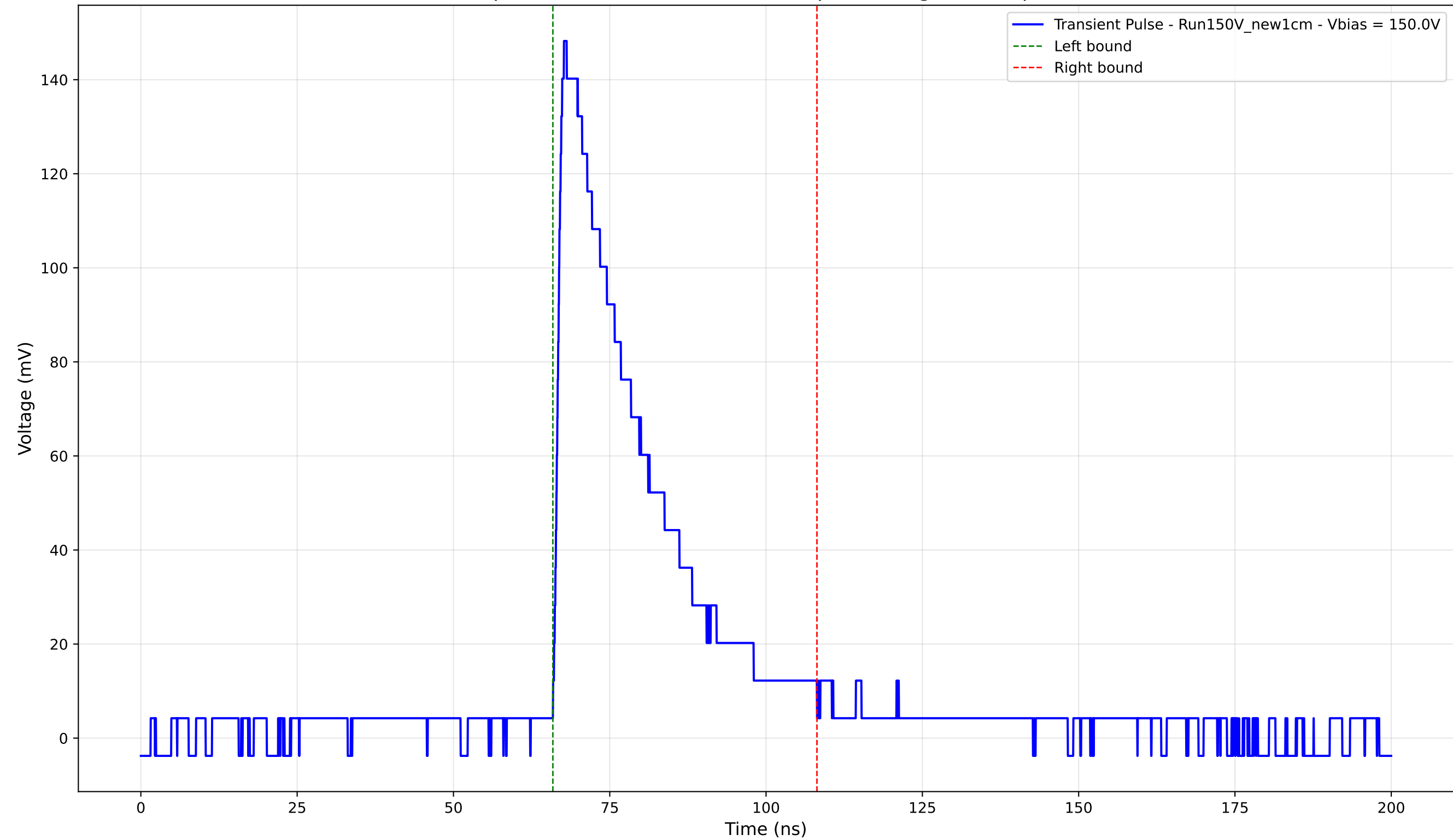
Transient Pulse - Sample: New1cm - Position: 3420.0 \mu\text{m} - Charge: 43.10 pC - Rise Time: 1.31 ns
