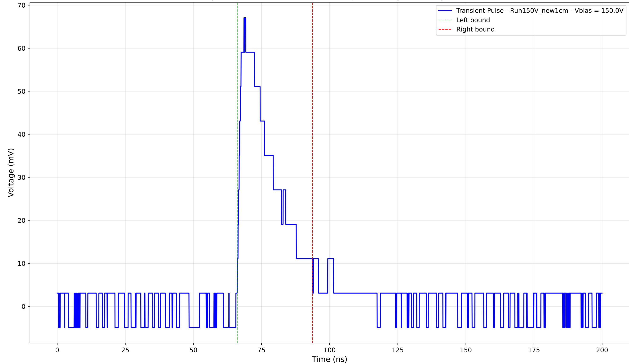
Transient Pulse - Sample: New1cm - Position: 1480.0 \mu\text{m} - Charge: 17.71 pC - Rise Time: 2.47 ns
