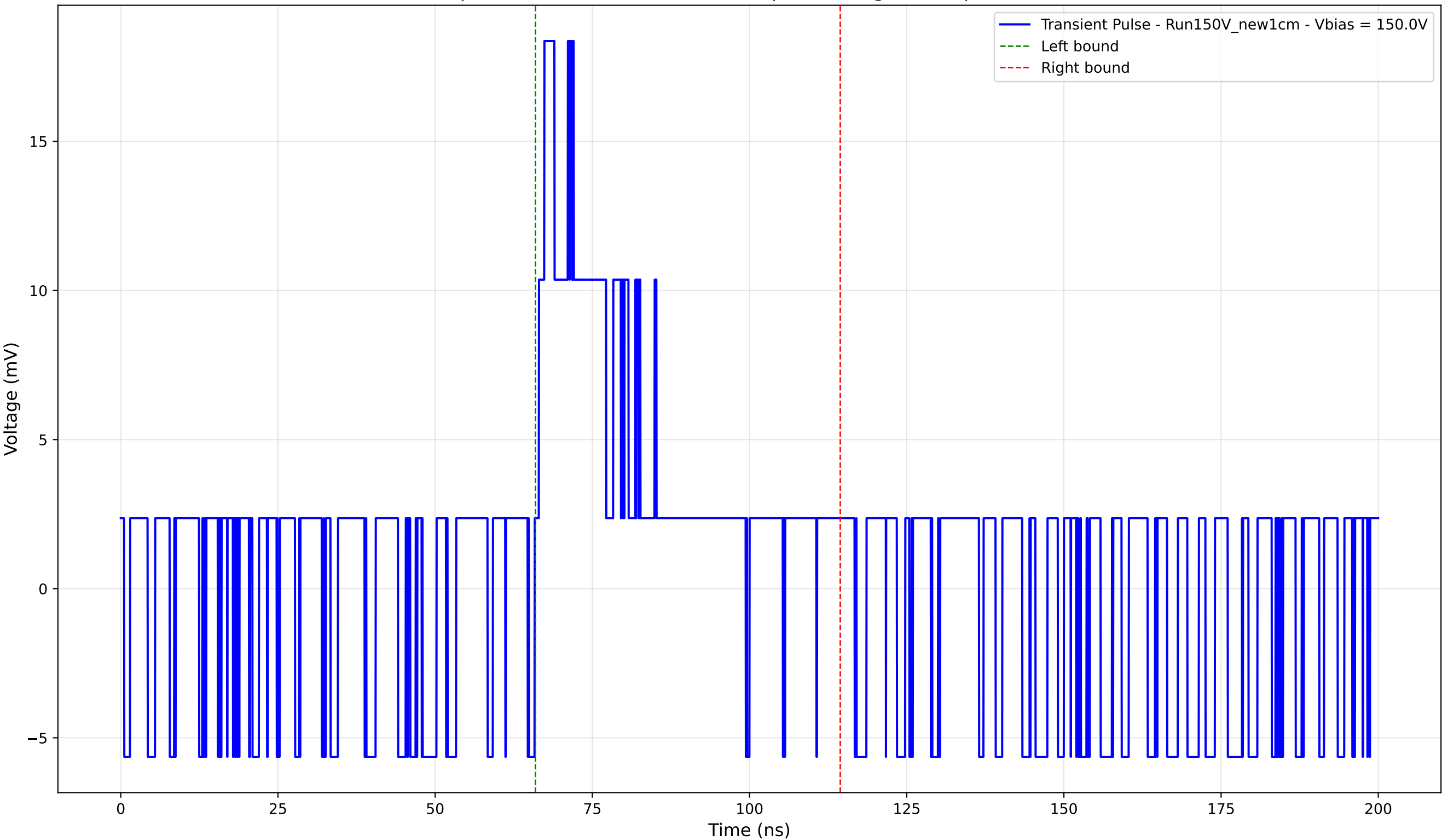
Transient Pulse - Sample: New1cm - Position: 525.0 \mu\text{m} - Charge: 4.71 pC - Rise Time: 0.00 ns (N/A)
