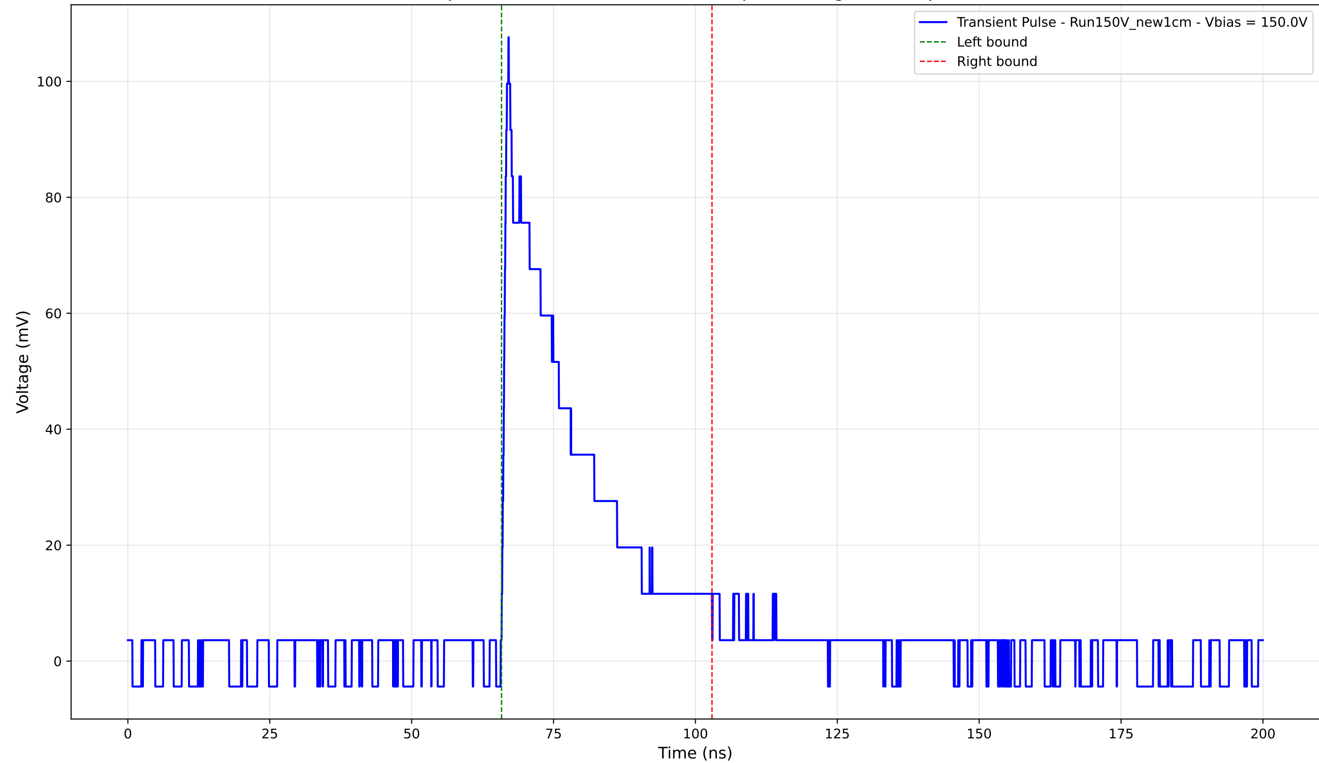
Transient Pulse - Sample: New1cm - Position: 2125.0 \mu\text{m} - Charge: 25.35 pC - Rise Time: 0.92 ns
