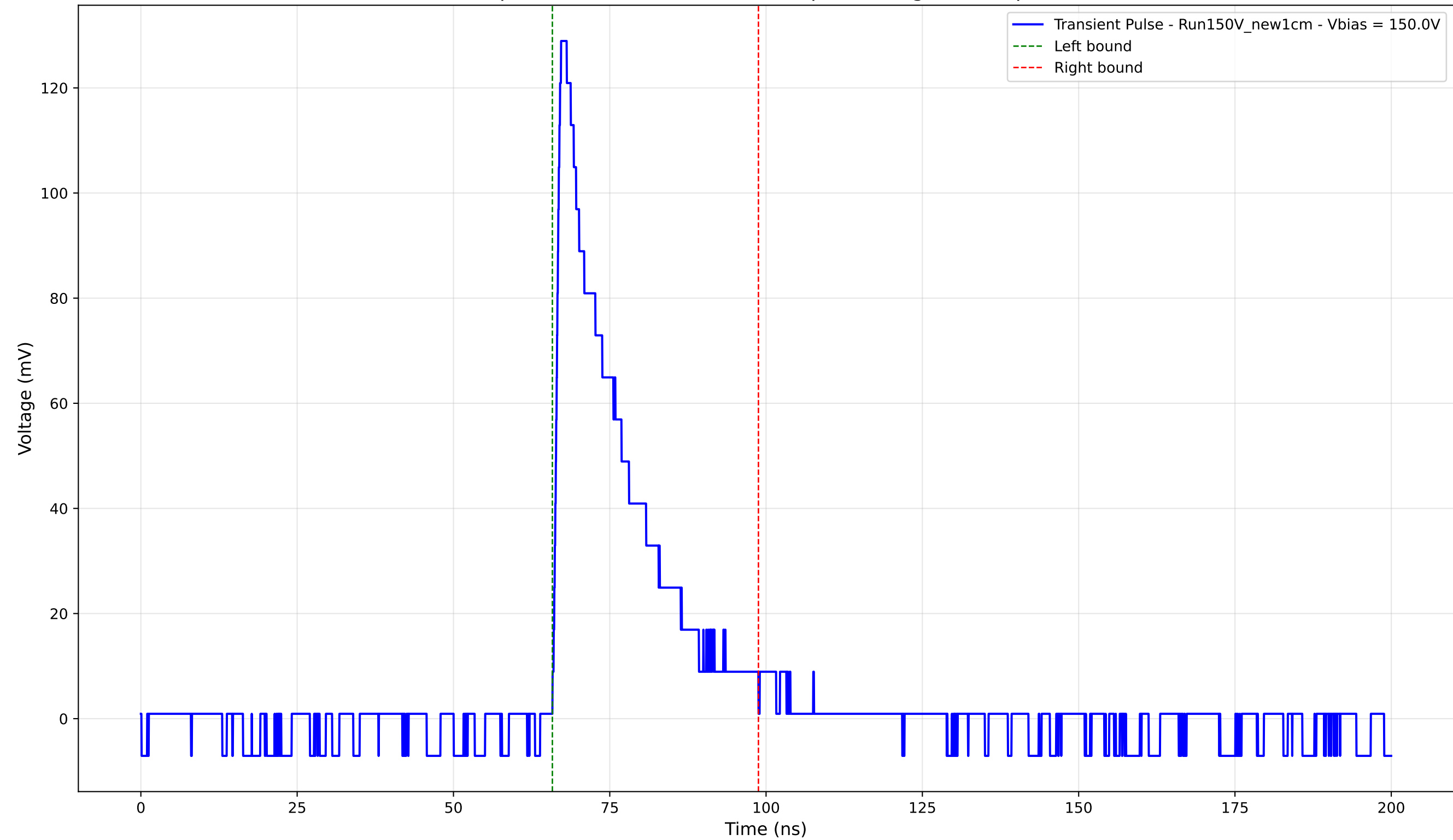
Transient Pulse - Sample: New1cm - Position: 370.0 \mu\text{m} - Charge: 27.58 pC - Rise Time: 1.03 ns
