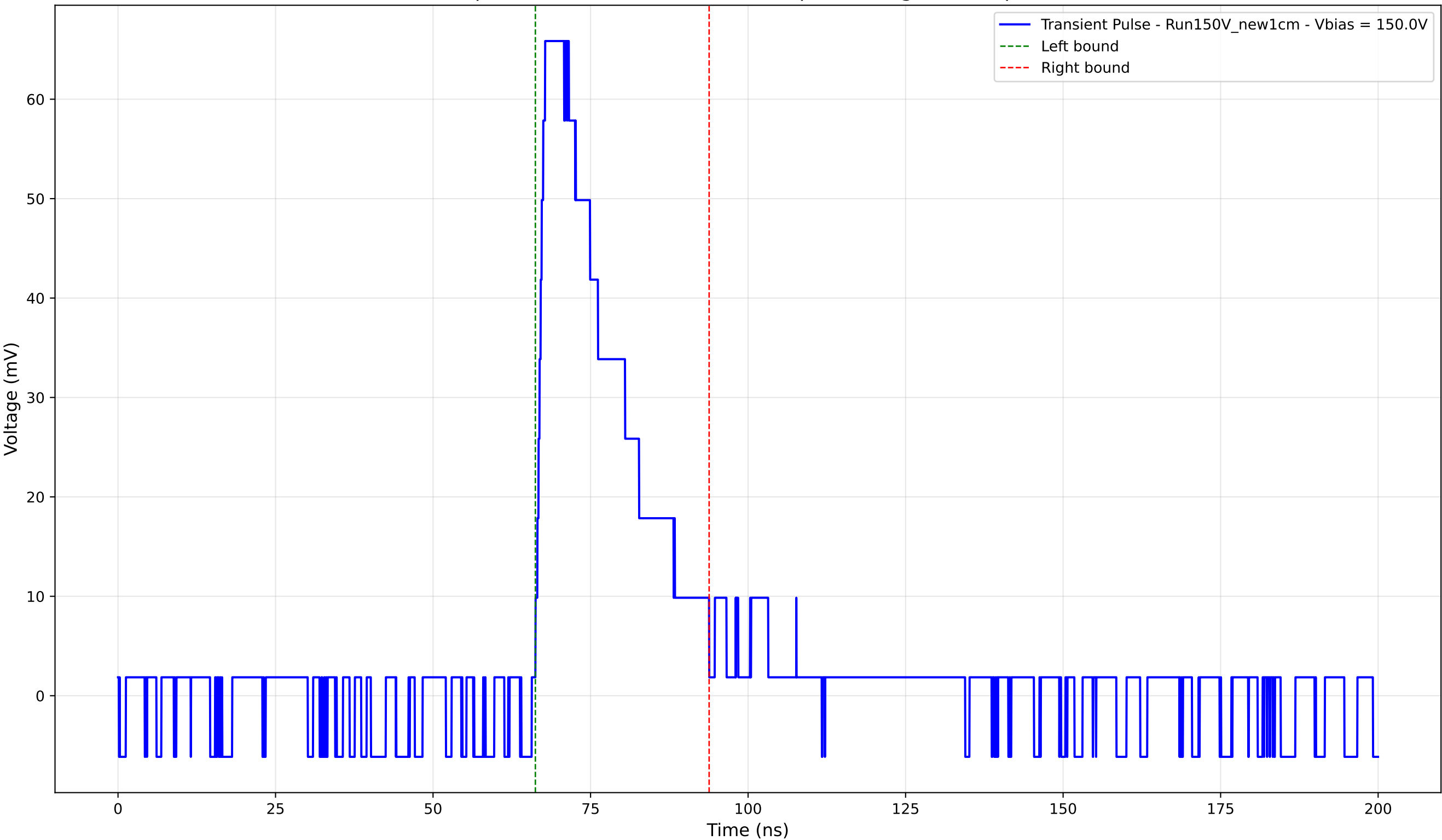
Transient Pulse - Sample: New1cm - Position: 1100.0 \mu\text{m} - Charge: 17.72 pC - Rise Time: 1.53 ns
