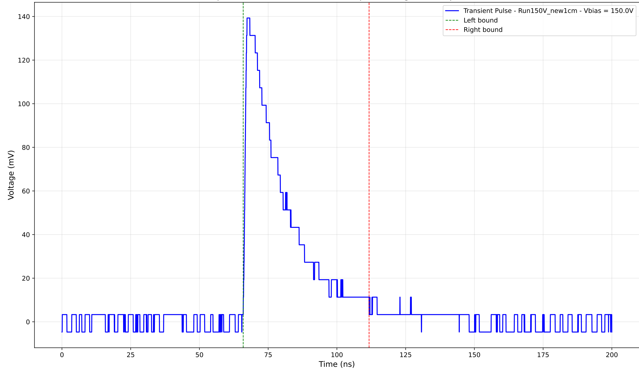
Transient Pulse - Sample: New1cm - Position: 3305.0 \mu\text{m} - Charge: 42.82 pC - Rise Time: 1.09 ns
