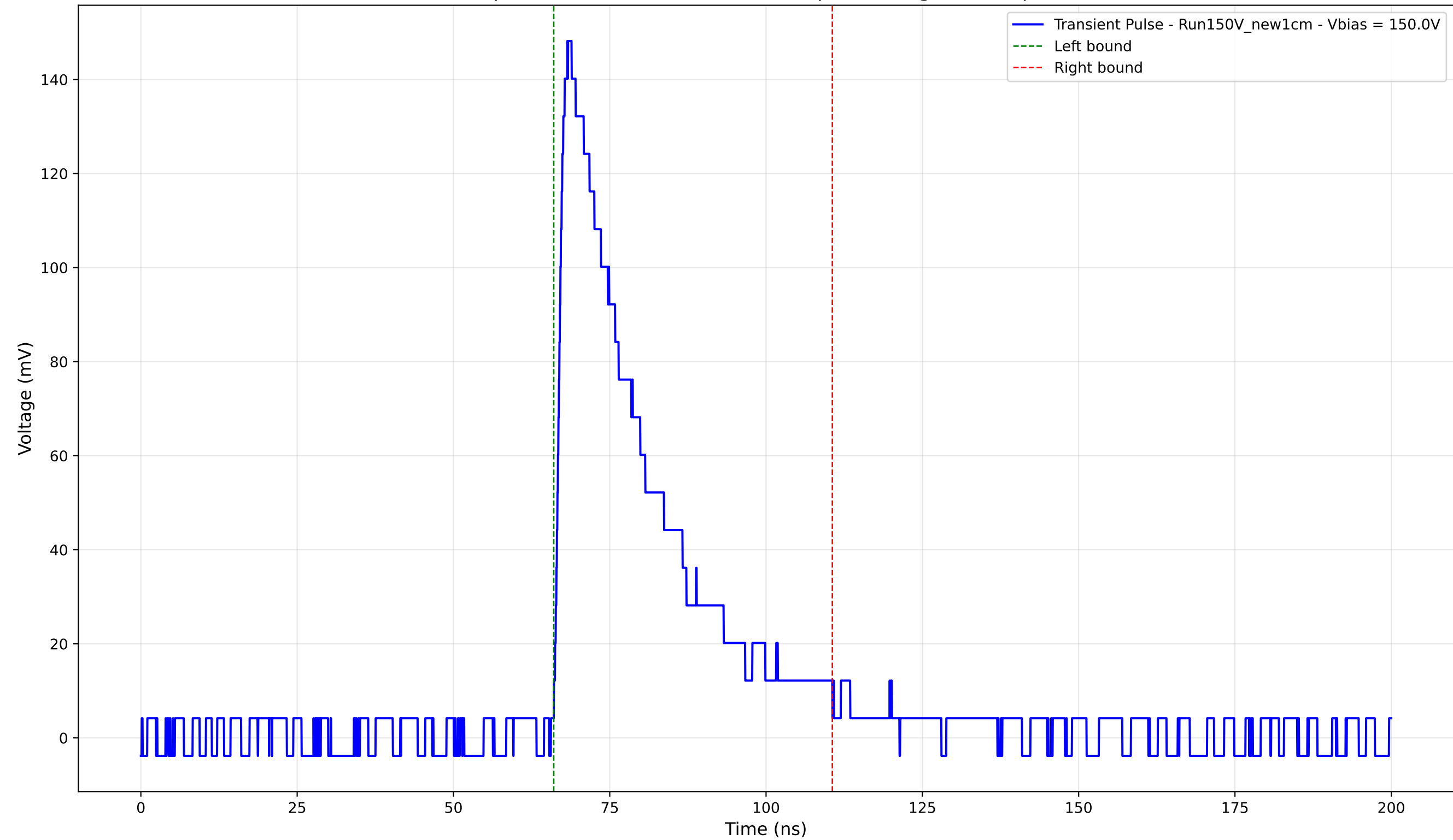
Transient Pulse - Sample: New1cm - Position: 3745.0 \mu\text{m} - Charge: 43.51 pC - Rise Time: 1.55 ns
