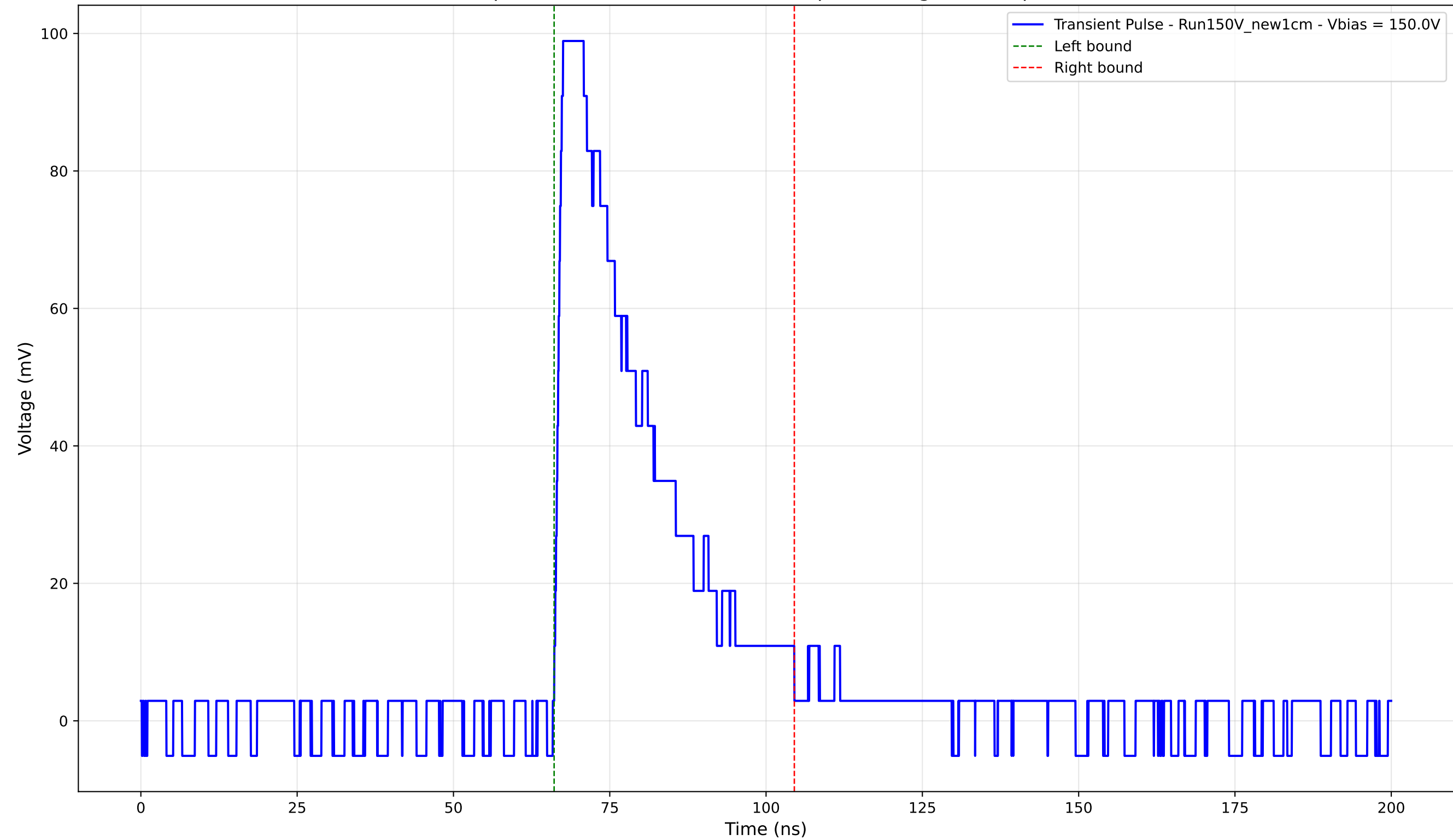
Transient Pulse - Sample: New1cm - Position: 3635.0 \mu\text{m} - Charge: 30.64 pC - Rise Time: 1.20 ns
