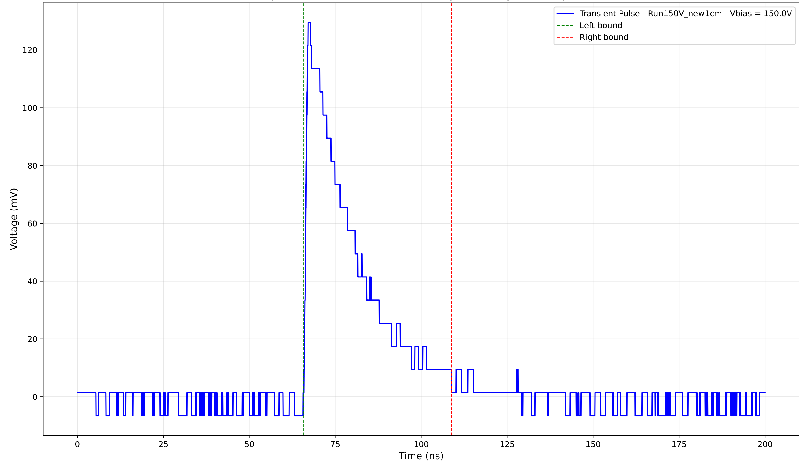
Transient Pulse - Sample: New1cm - Position: 3175.0 \mu\text{m} - Charge: 37.47 pC - Rise Time: 0.97 ns
