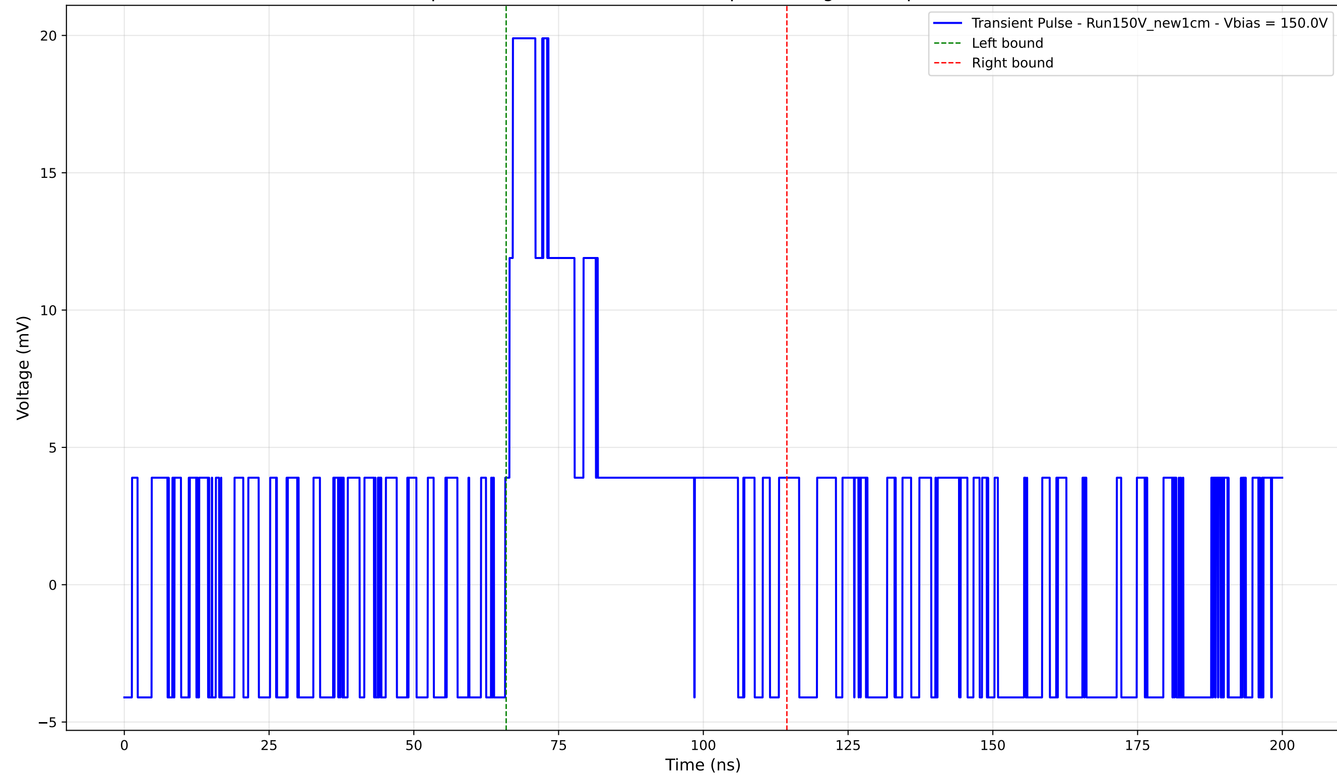
Transient Pulse - Sample: New1cm - Position: 4065.0 \mu\text{m} - Charge: 6.08 pC - Rise Time: 0.00 ns (N/A)
