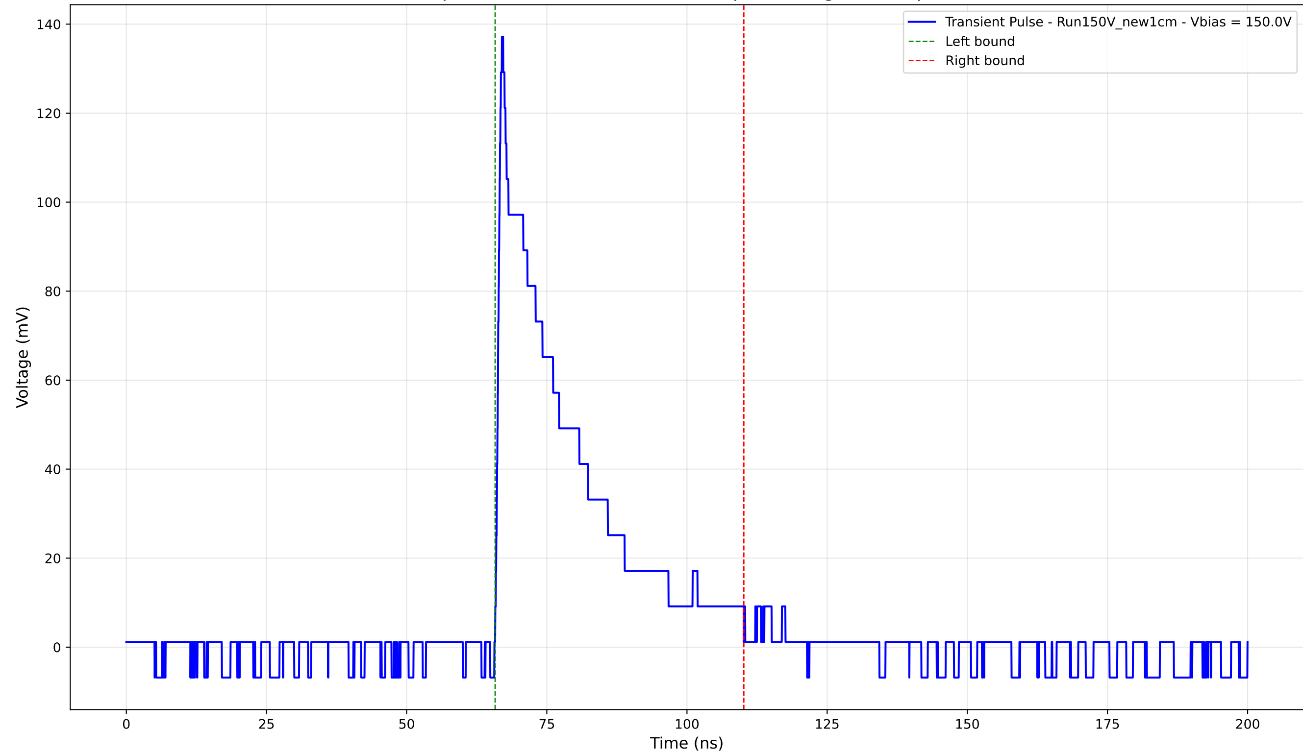
Transient Pulse - Sample: New1cm - Position: 2975.0 \mu\text{m} - Charge: 32.84 pC - Rise Time: 0.91 ns
