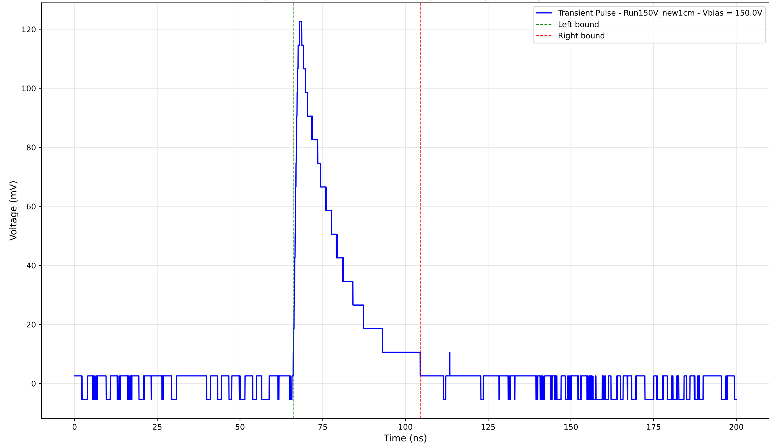
Transient Pulse - Sample: New1cm - Position: 685.0 \mu\text{m} - Charge: 30.42 pC - Rise Time: 1.36 ns
