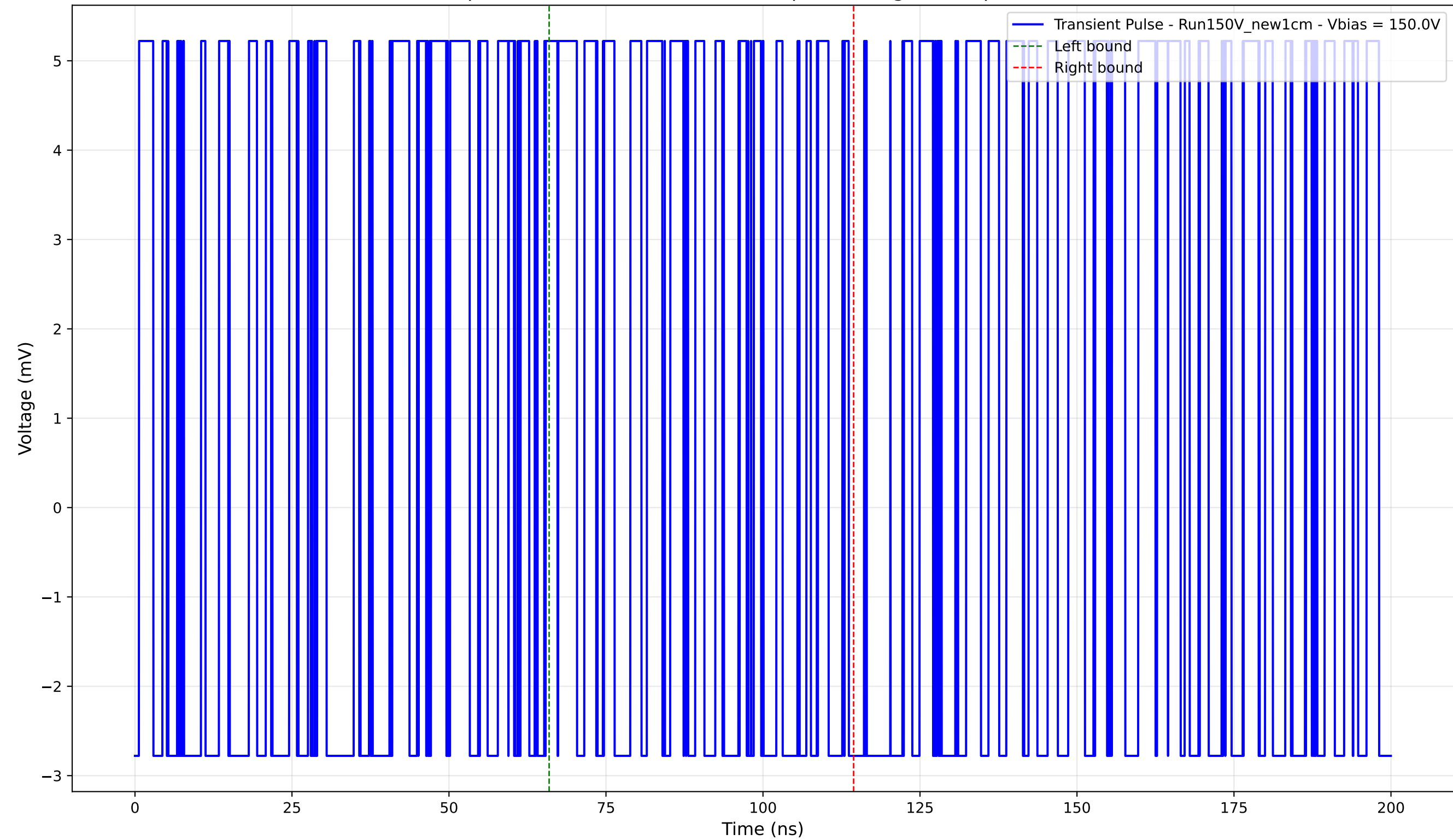
Transient Pulse - Sample: New1cm - Position: 4985.0 \mu\text{m} - Charge: 1.28 pC - Rise Time: 0.00 ns (N/A)
