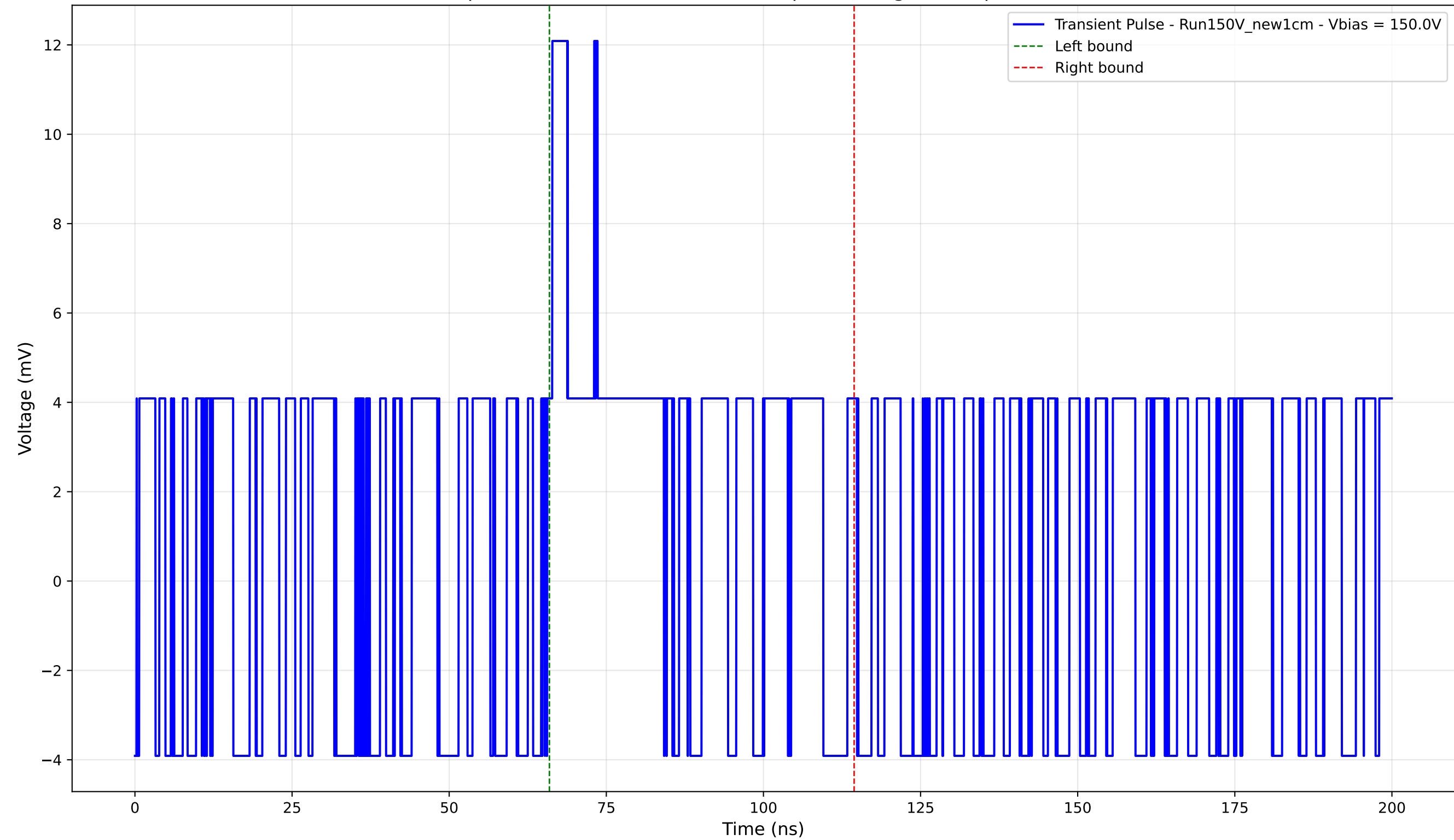
Transient Pulse - Sample: New1cm - Position: 4905.0 \mu\text{m} - Charge: 2.77 pC - Rise Time: 0.00 ns (N/A)
