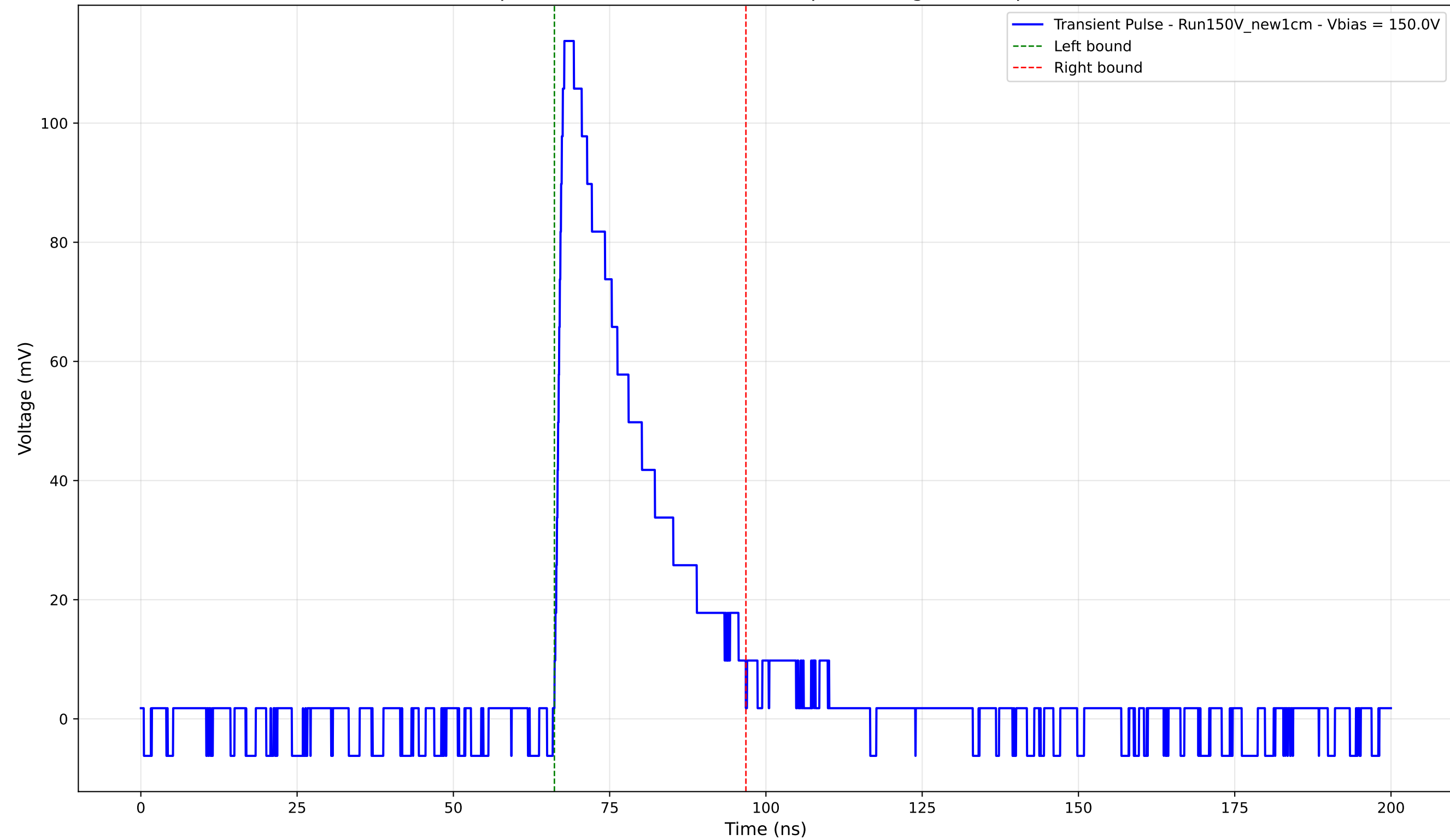
Transient Pulse - Sample: New1cm - Position: 855.0 \mu\text{m} - Charge: 29.73 pC - Rise Time: 1.20 ns
