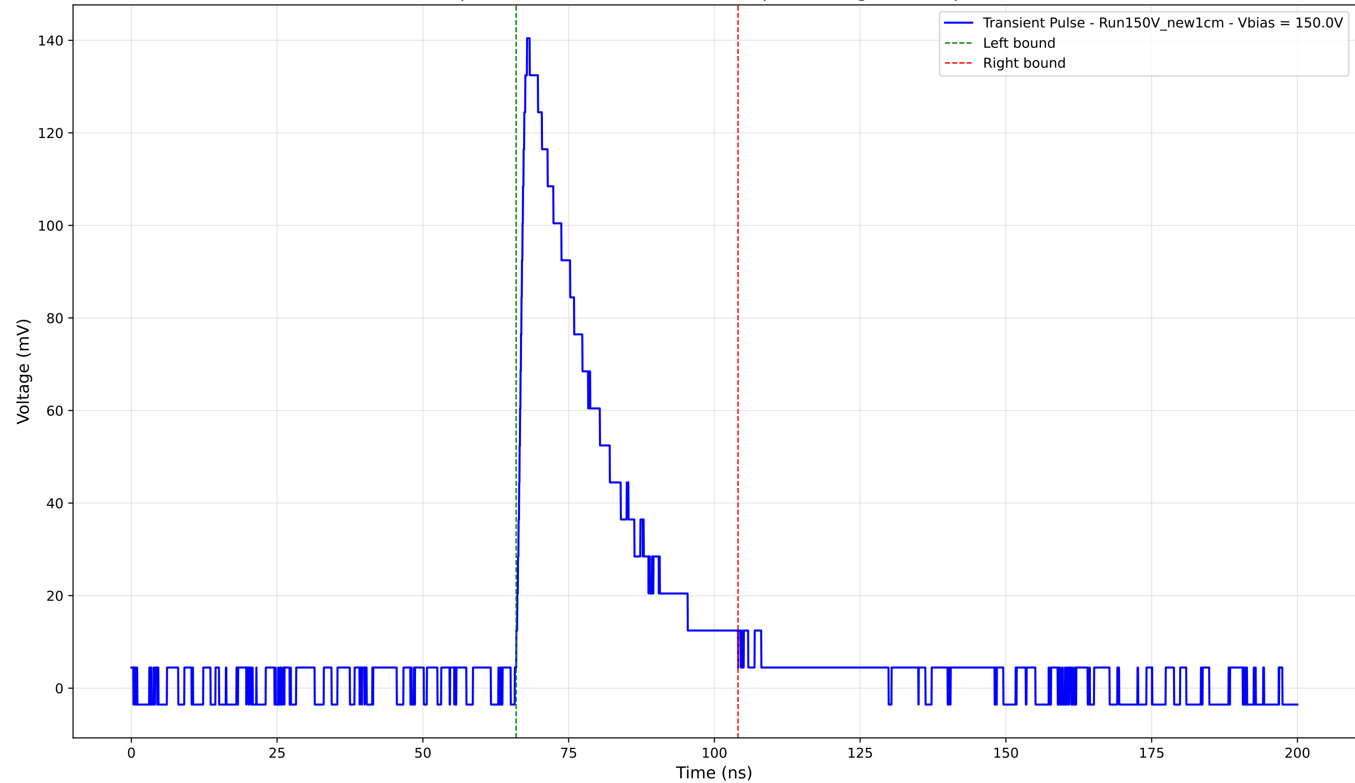
Transient Pulse - Sample: New1cm - Position: 3965.0 \mu\text{m} - Charge: 38.56 pC - Rise Time: 1.40 ns
