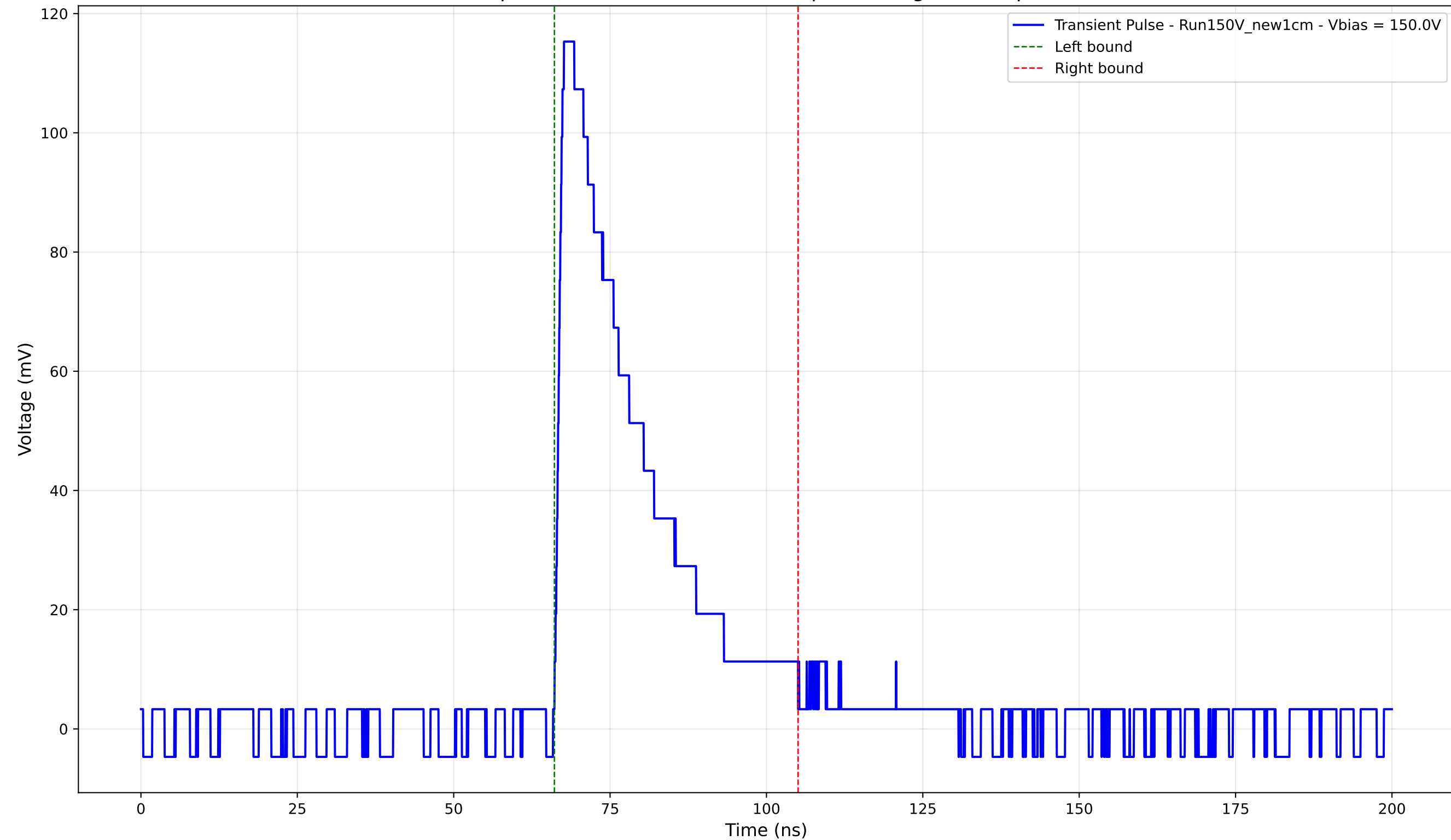
Transient Pulse - Sample: New1cm - Position: 775.0 \mu\text{m} - Charge: 32.48 pC - Rise Time: 1.12 ns
