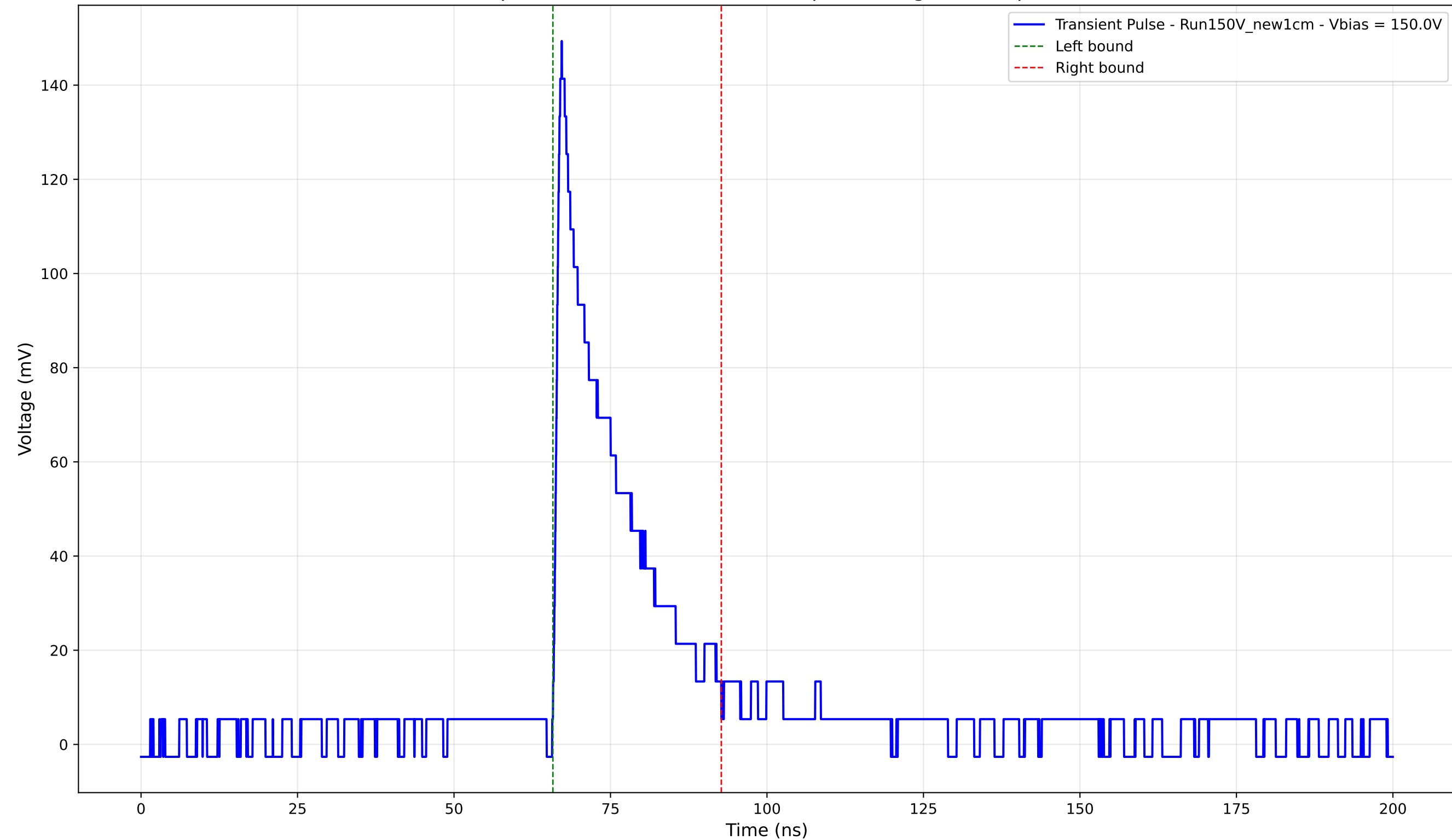
Transient Pulse - Sample: New1cm - Position: 230.0 \mu\text{m} - Charge: 28.17 pC - Rise Time: 1.04 ns
