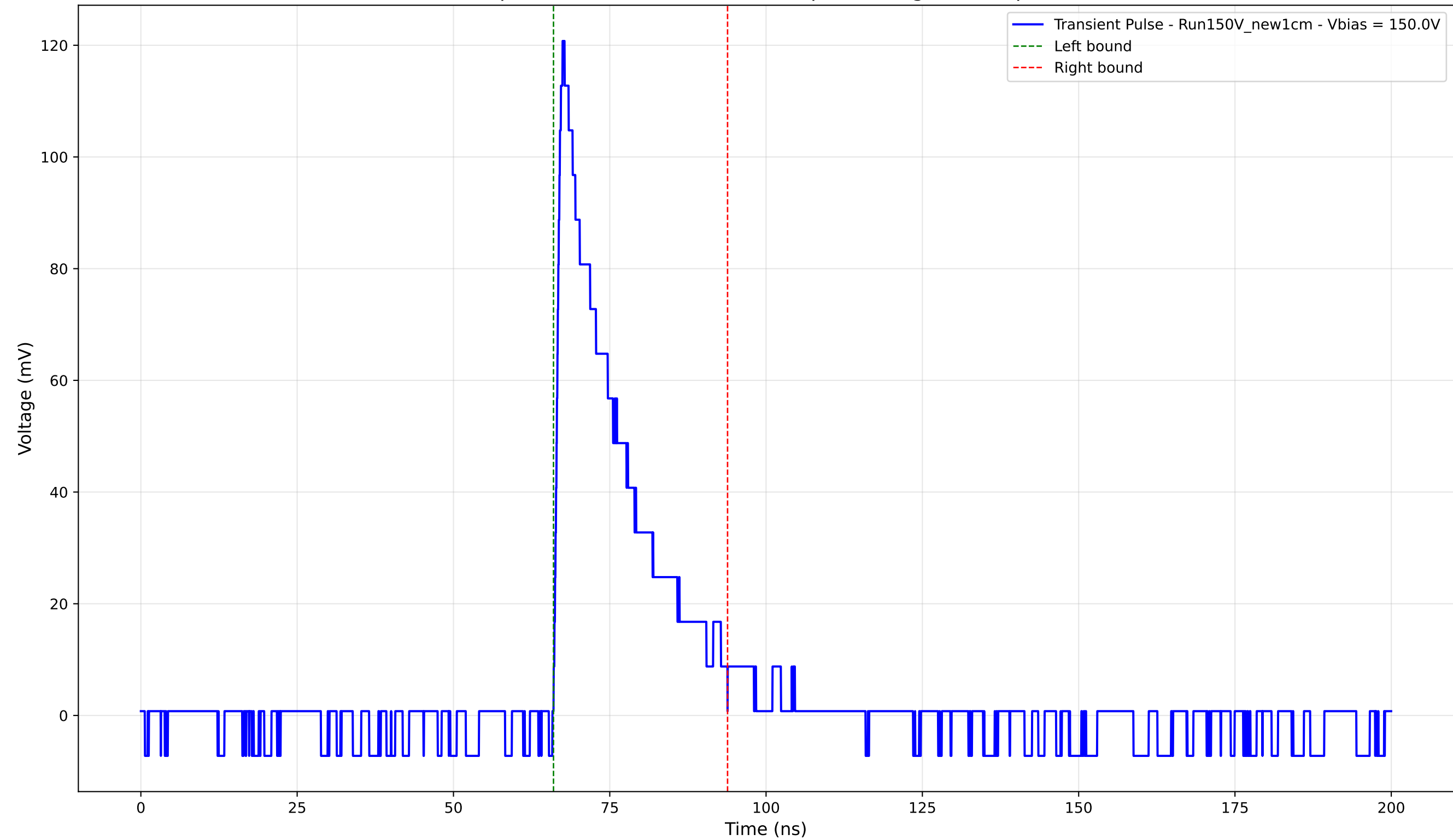
Transient Pulse - Sample: New1cm - Position: 415.0 \mu\text{m} - Charge: 24.53 pC - Rise Time: 1.05 ns
