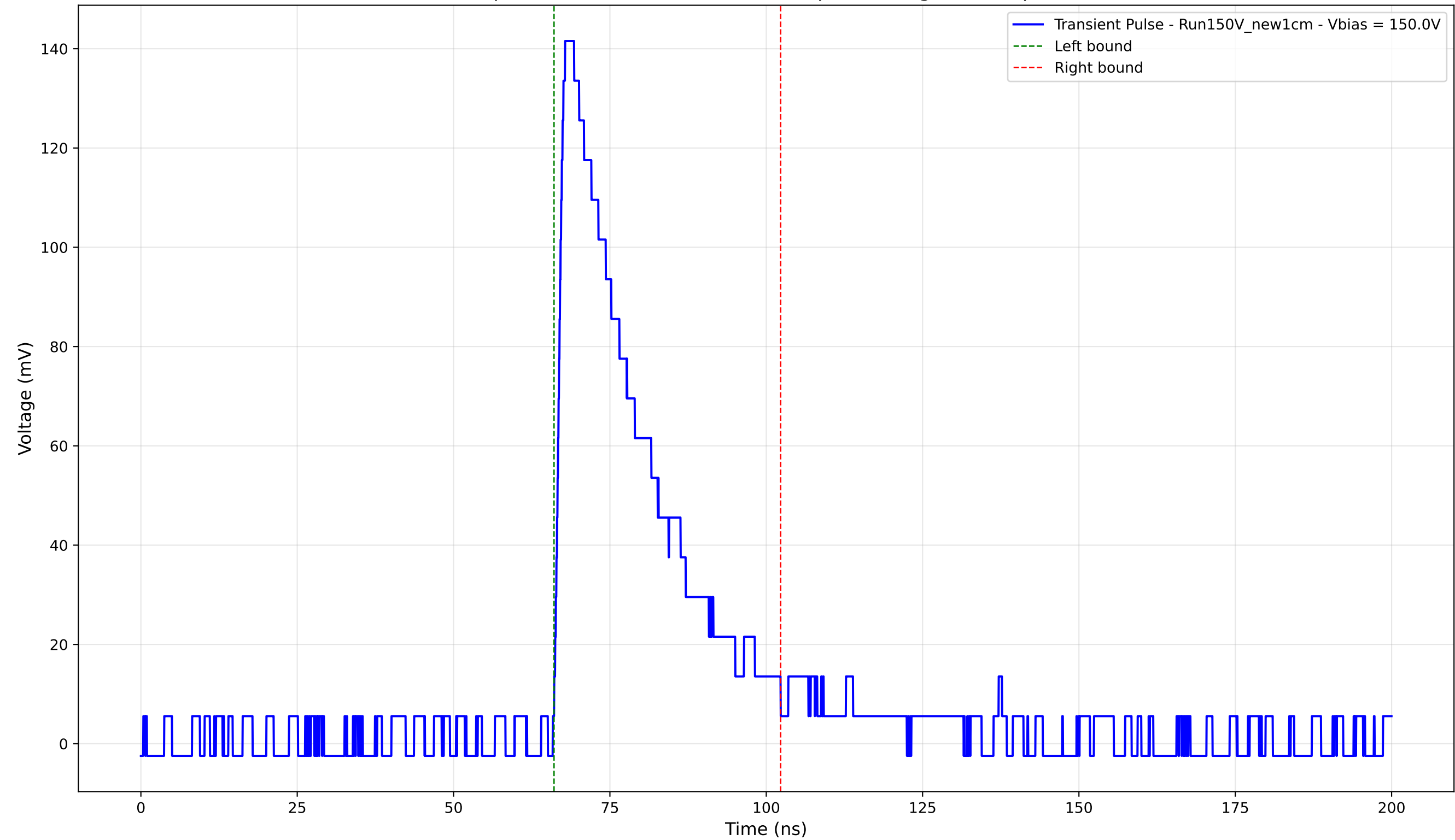
Transient Pulse - Sample: New1cm - Position: 3920.0 \mu\text{m} - Charge: 40.69 pC - Rise Time: 1.34 ns
