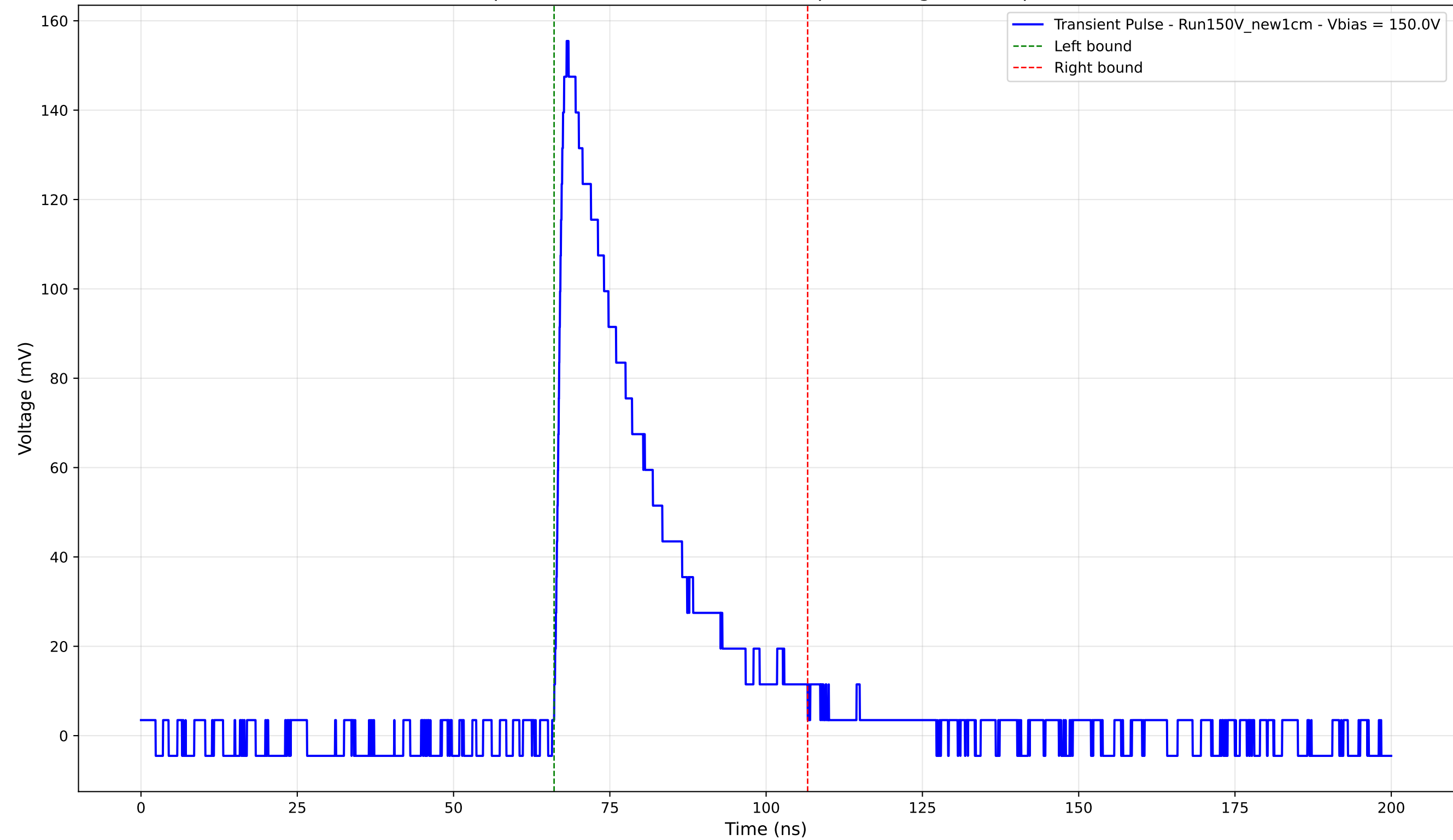
Transient Pulse - Sample: New1cm - Position: 3900.0 \mu\text{m} - Charge: 43.13 pC - Rise Time: 1.45 ns
