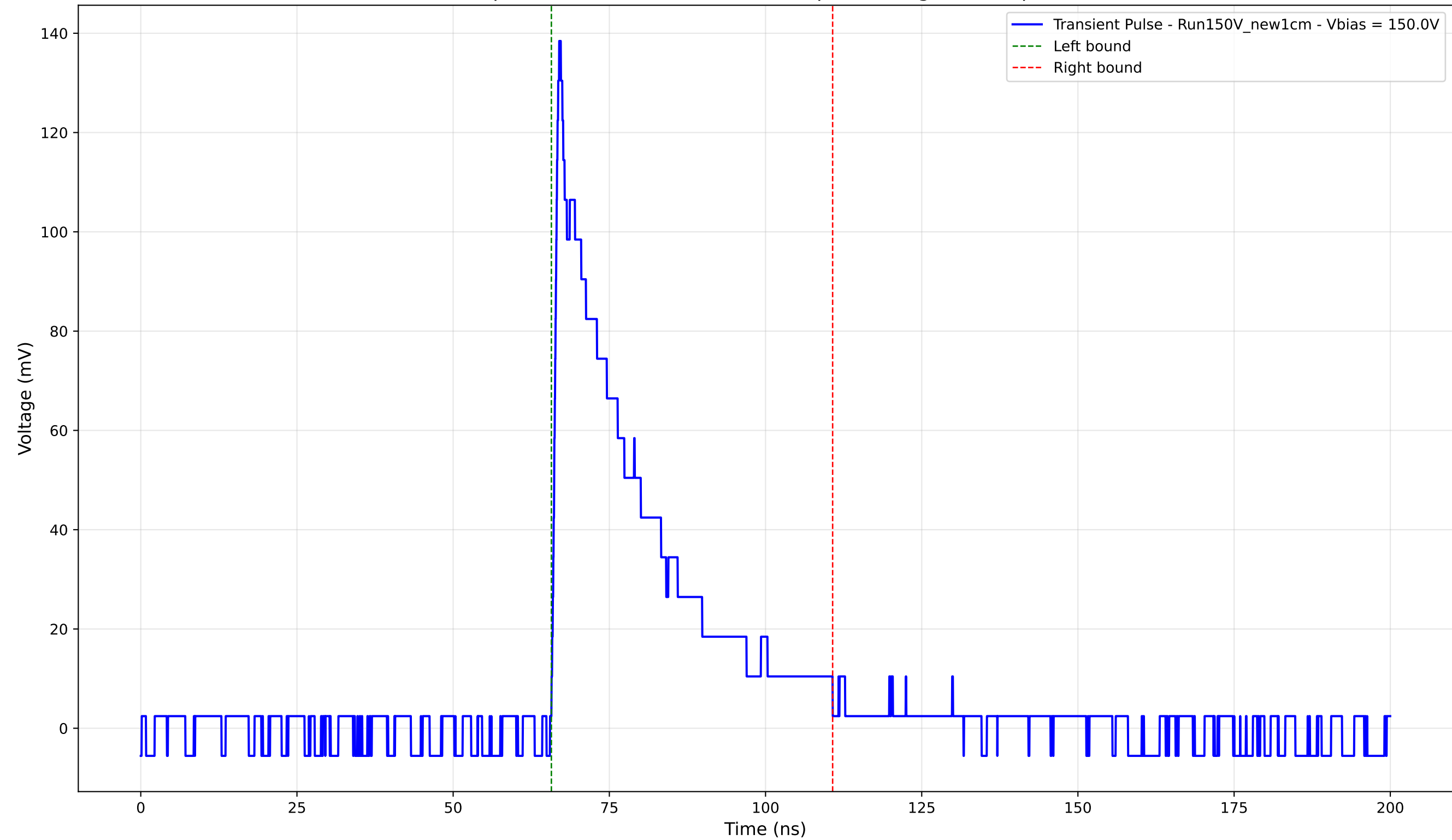
Transient Pulse - Sample: New1cm - Position: 2970.0 \mu\text{m} - Charge: 34.59 pC - Rise Time: 0.97 ns
