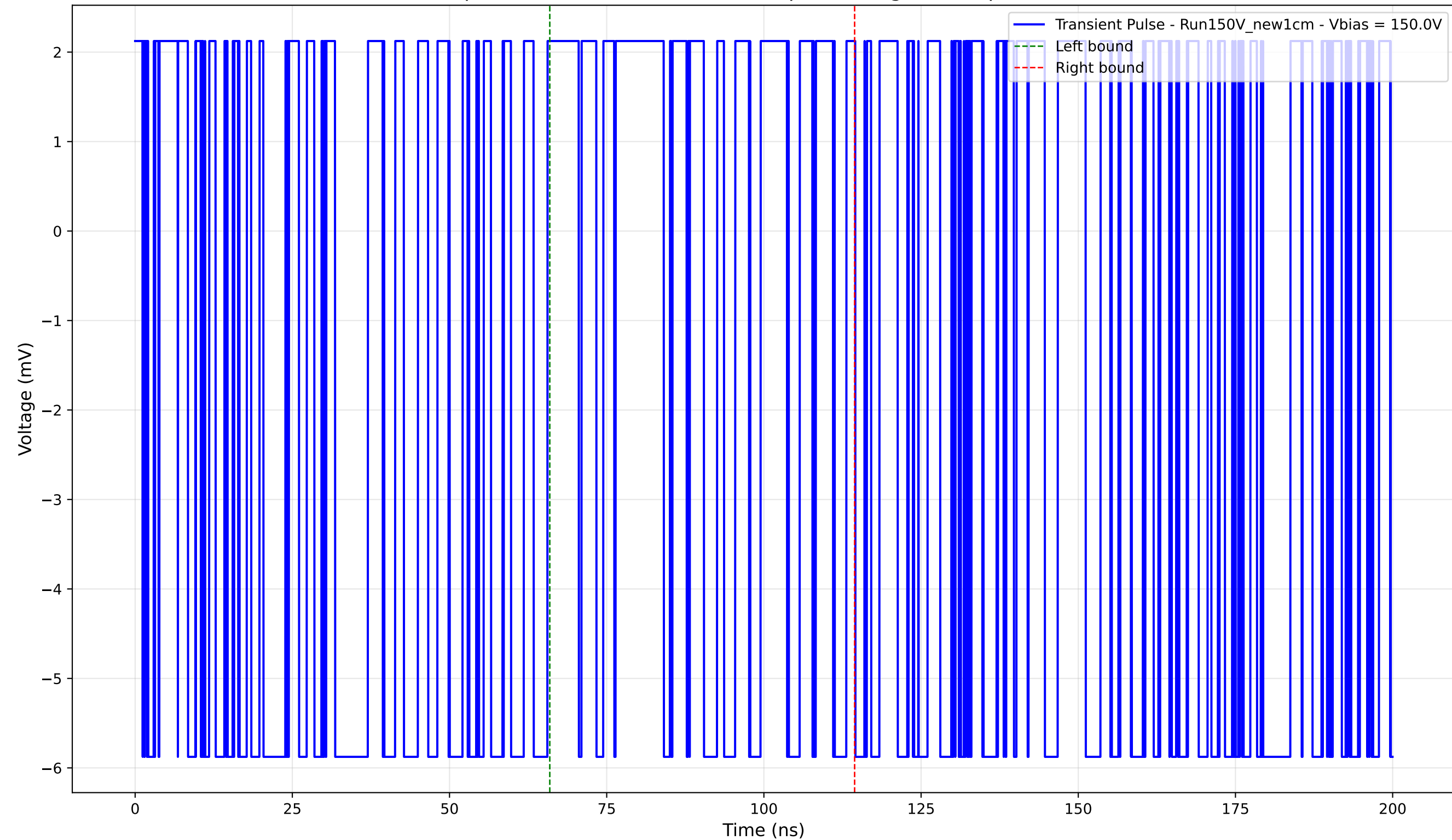
Transient Pulse - Sample: New1cm - Position: 4920.0 \mu\text{m} - Charge: -0.05 pC - Rise Time: 0.00 ns (N/A)
