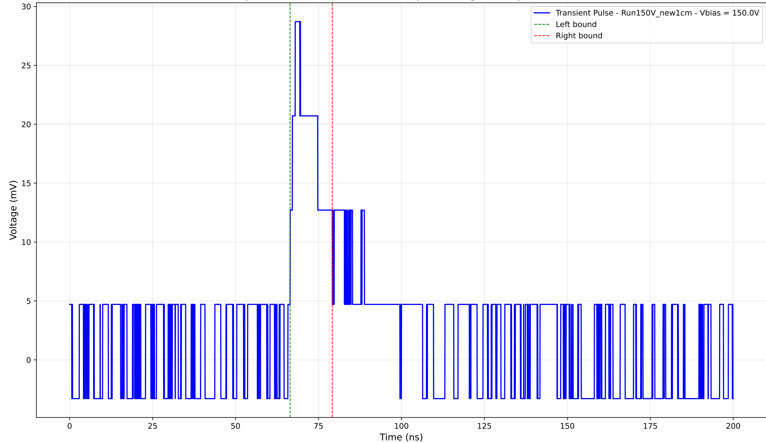
Transient Pulse - Sample: New1cm - Position: 4080.0 \mu\text{m} - Charge: 4.70 pC - Rise Time: 0.00 ns (N/A)
