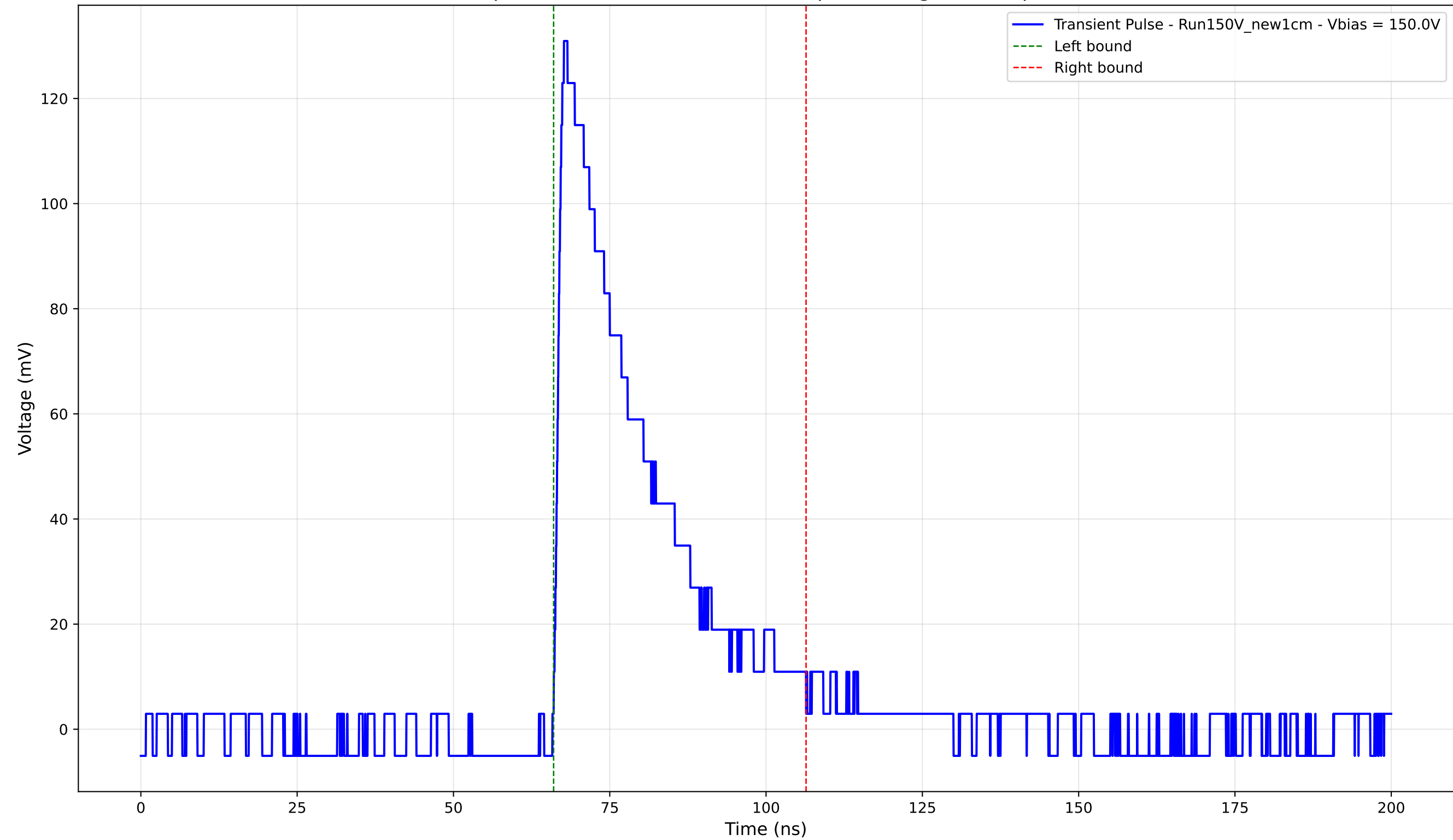
Transient Pulse - Sample: New1cm - Position: 3470.0 \mu\text{m} - Charge: 37.53 pC - Rise Time: 1.23 ns
