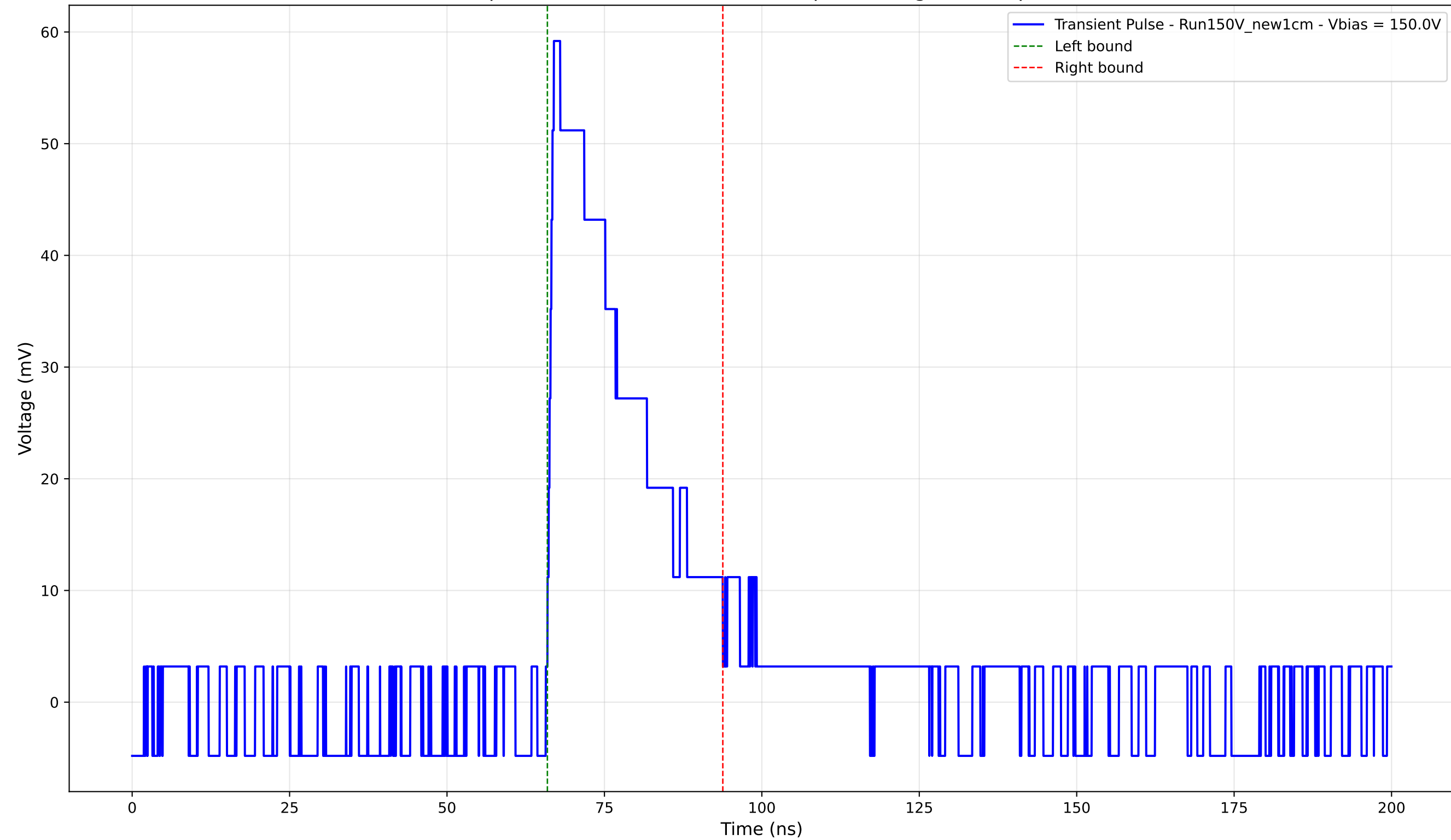
Transient Pulse - Sample: New1cm - Position: 1980.0 \mu\text{m} - Charge: 16.06 pC - Rise Time: 1.01 ns
