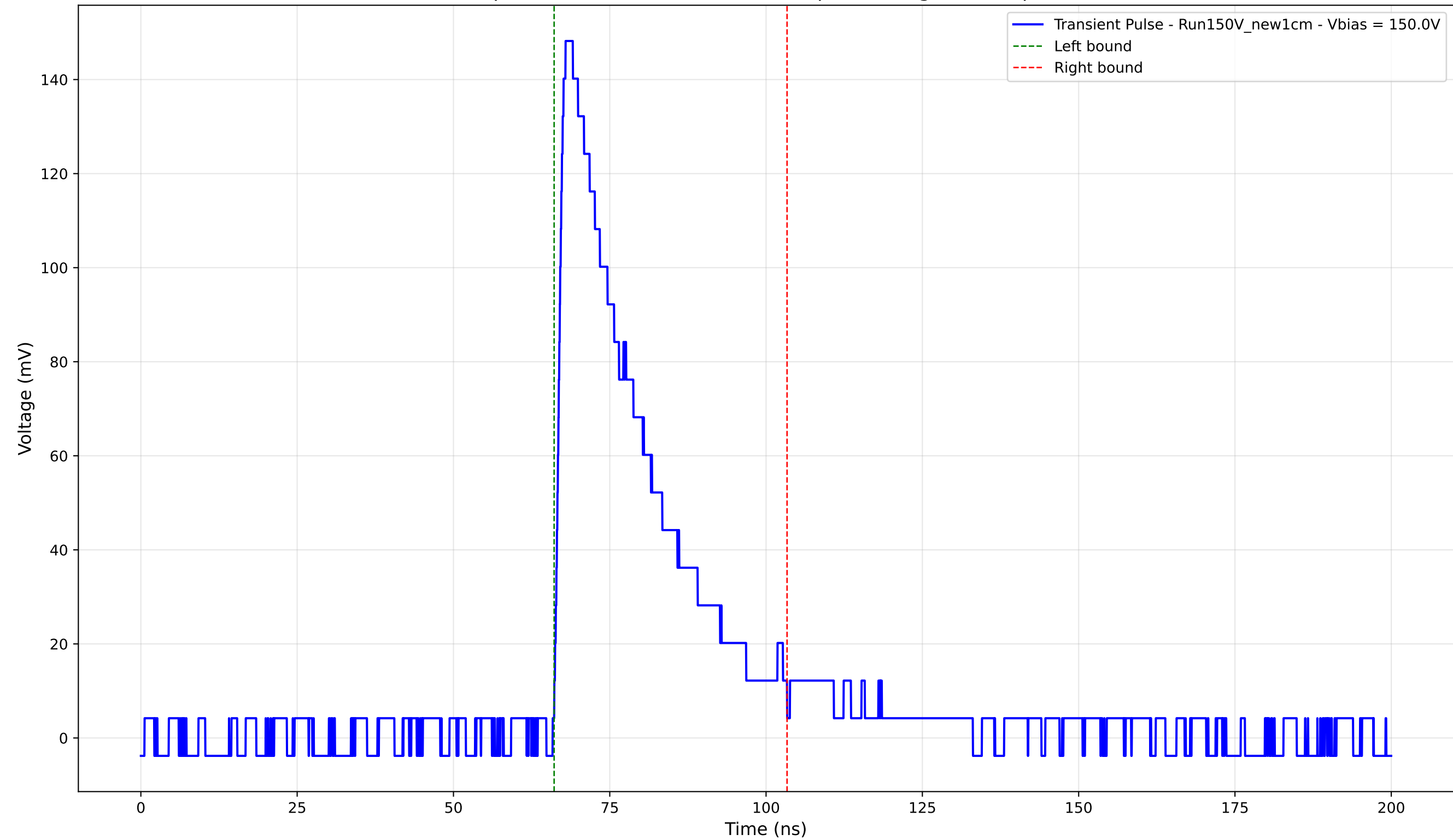
Transient Pulse - Sample: New1cm - Position: 3840.0 \mu\text{m} - Charge: 42.09 pC - Rise Time: 1.37 ns
