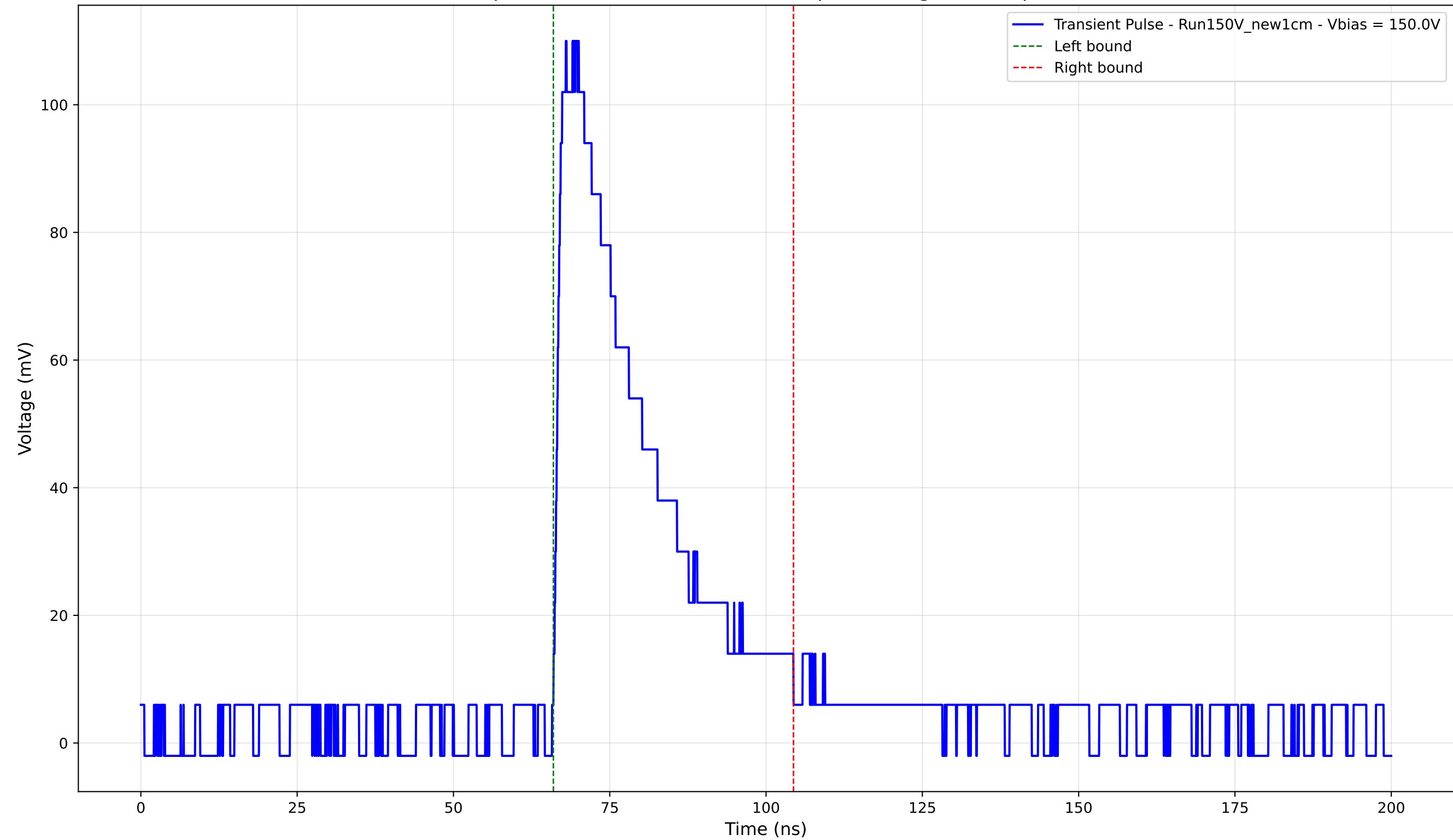
Transient Pulse - Sample: New1cm - Position: 1695.0 \mu\text{m} - Charge: 33.73 pC - Rise Time: 1.39 ns
