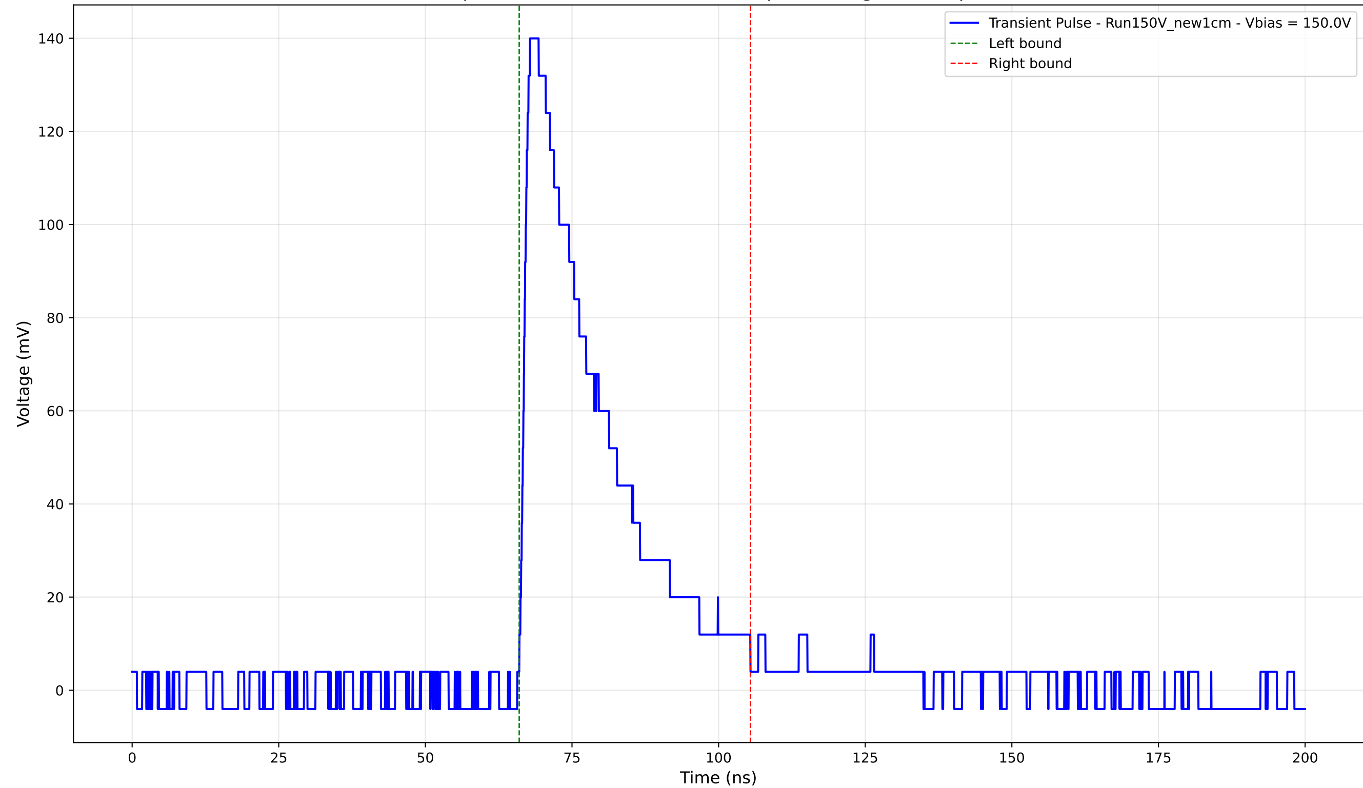
Transient Pulse - Sample: New1cm - Position: 3945.0 \mu\text{m} - Charge: 40.24 pC - Rise Time: 1.39 ns
