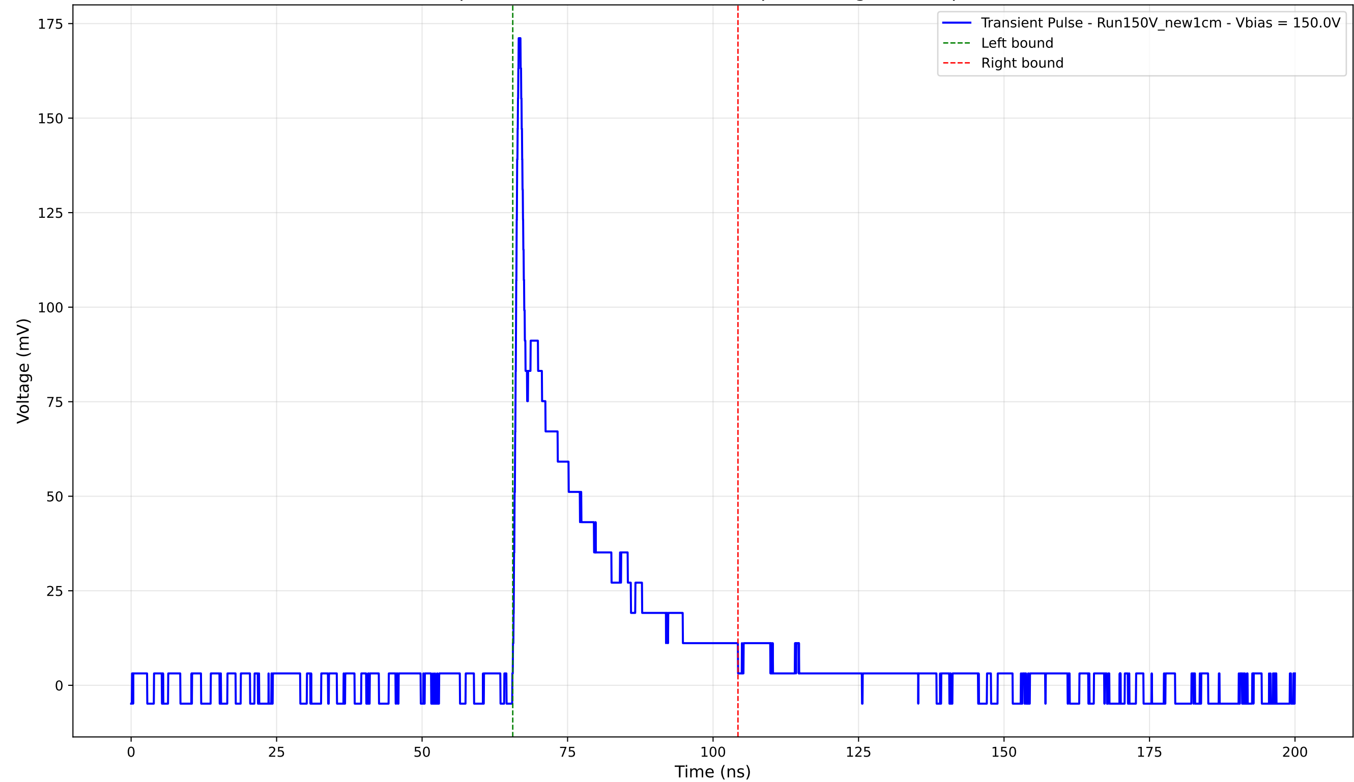
Transient Pulse - Sample: New1cm - Position: 2640.0 \mu\text{m} - Charge: 29.71 pC - Rise Time: 0.77 ns
