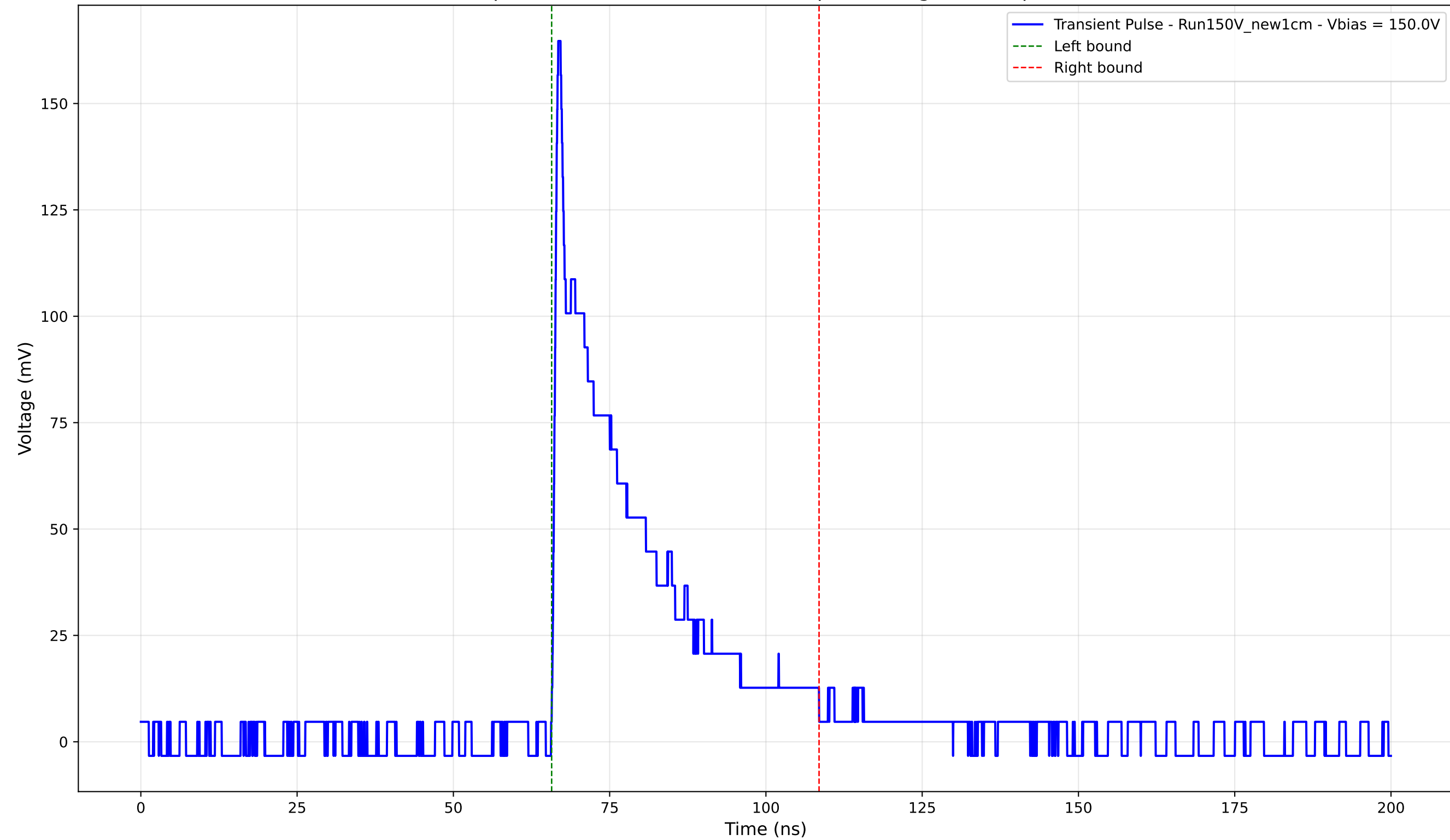
Transient Pulse - Sample: New1cm - Position: 2270.0 \mu\text{m} - Charge: 36.66 pC - Rise Time: 0.77 ns
