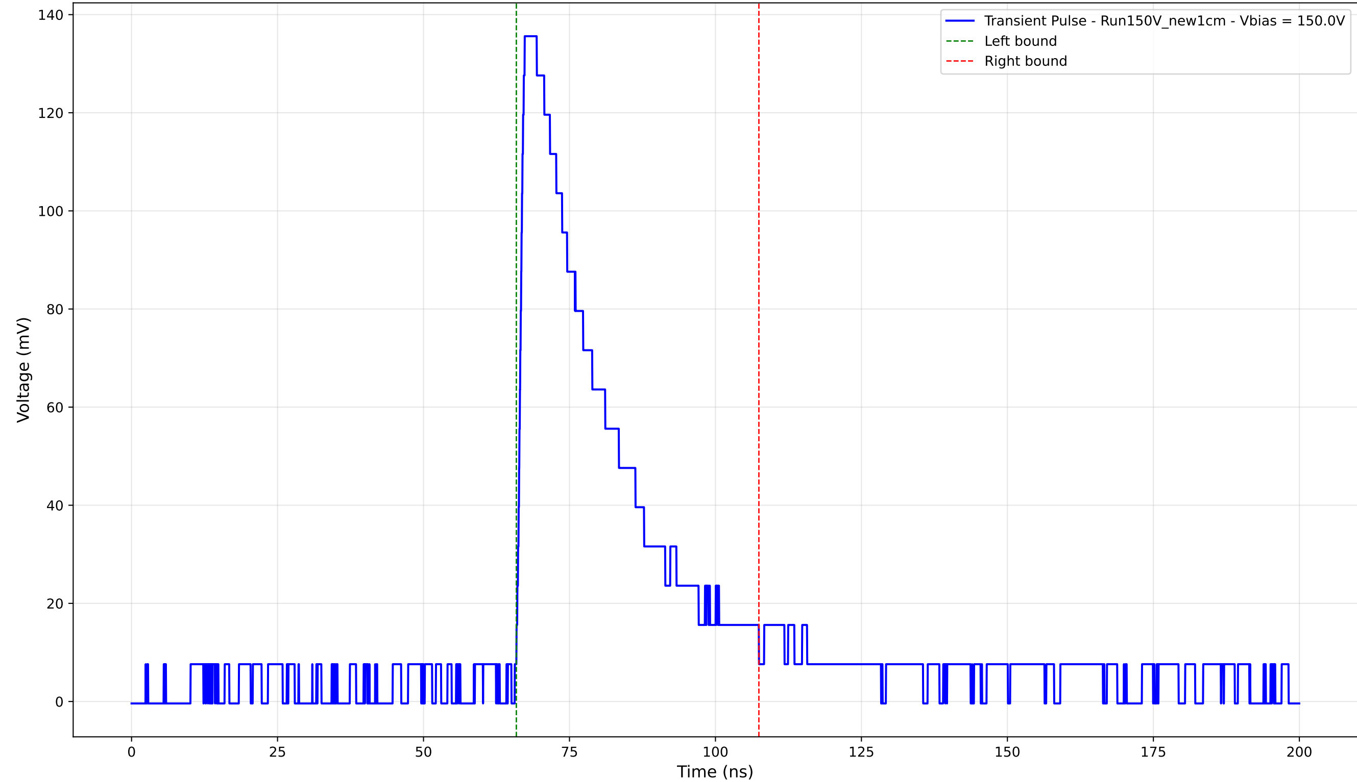
Transient Pulse - Sample: New1cm - Position: 3335.0 \mu\text{m} - Charge: 44.08 pC - Rise Time: 1.25 ns
