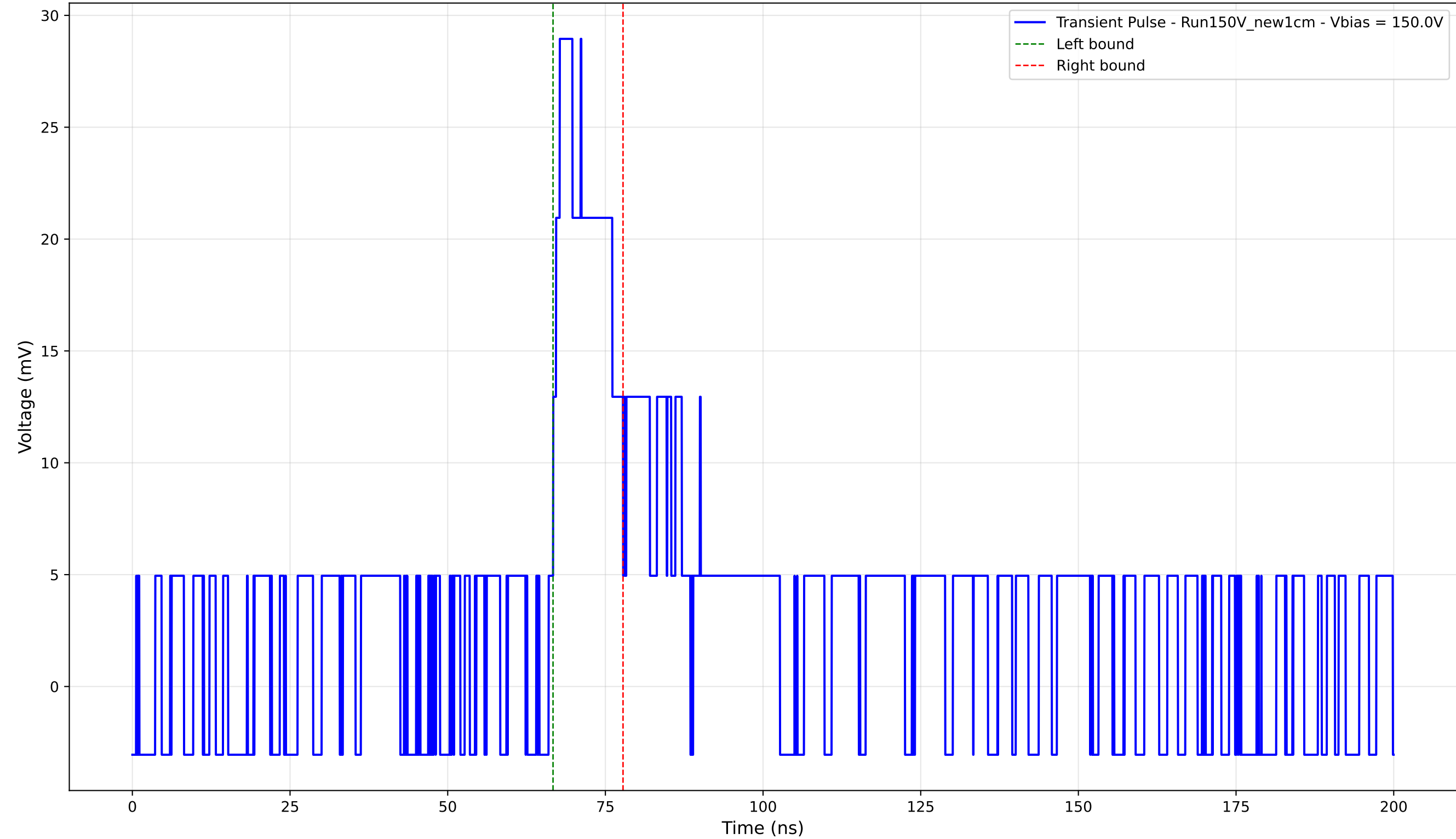
Transient Pulse - Sample: New1cm - Position: 1010.0 \mu\text{m} - Charge: 4.64 pC - Rise Time: 0.00 ns (N/A)
