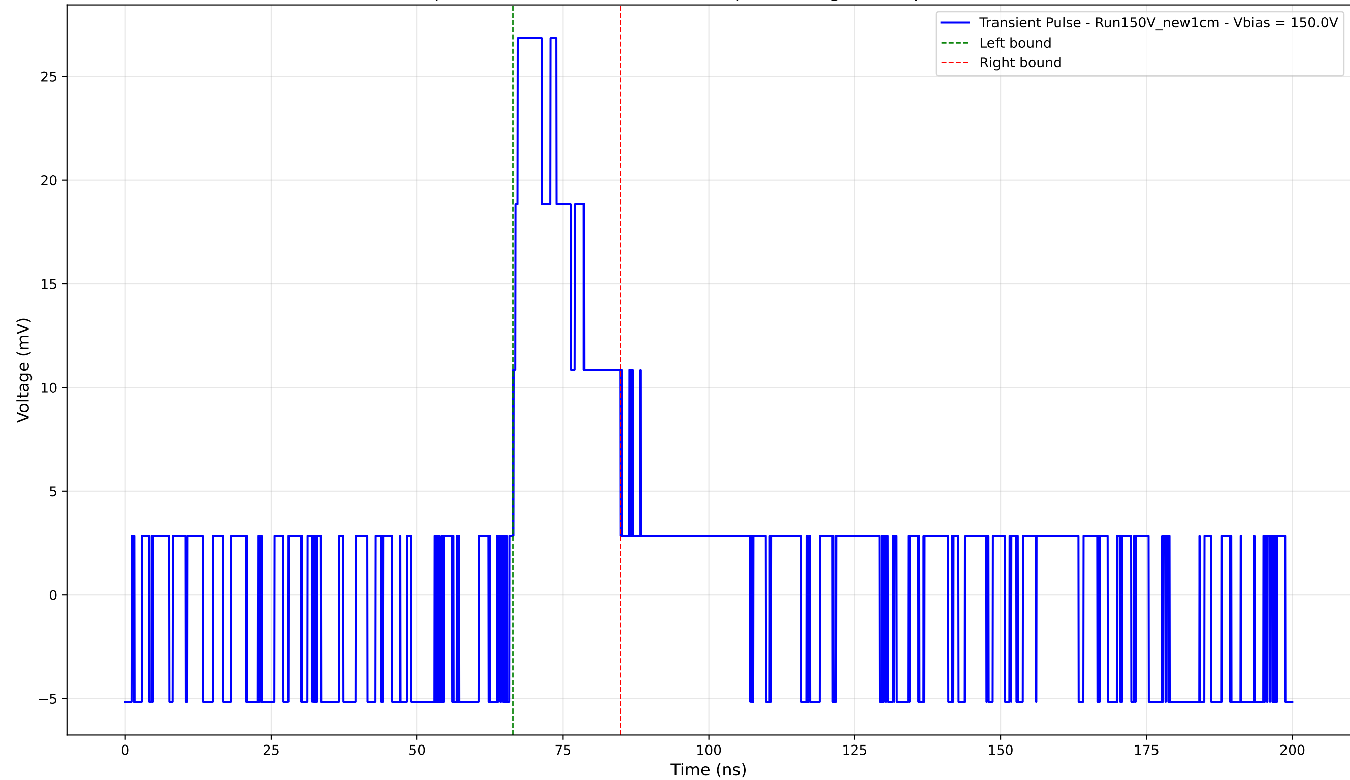
Transient Pulse - Sample: New1cm - Position: 4045.0 \mu\text{m} - Charge: 6.60 pC - Rise Time: 0.00 ns (N/A)
