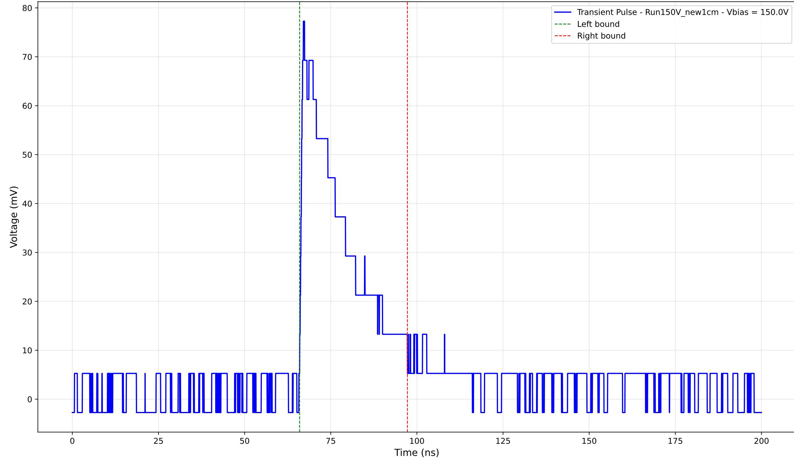
Transient Pulse - Sample: New1cm - Position: 1975.0 \mu\text{m} - Charge: 20.66 pC - Rise Time: 1.07 ns
