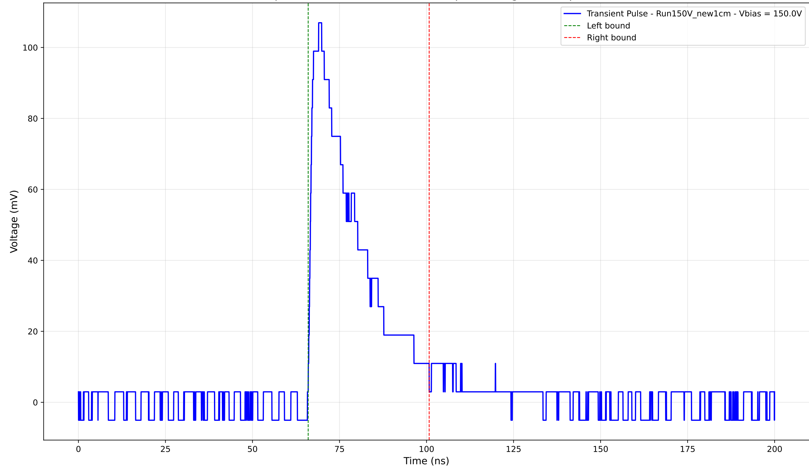
Transient Pulse - Sample: New1cm - Position: 1685.0 \mu\text{m} - Charge: 30.80 pC - Rise Time: 1.50 ns
