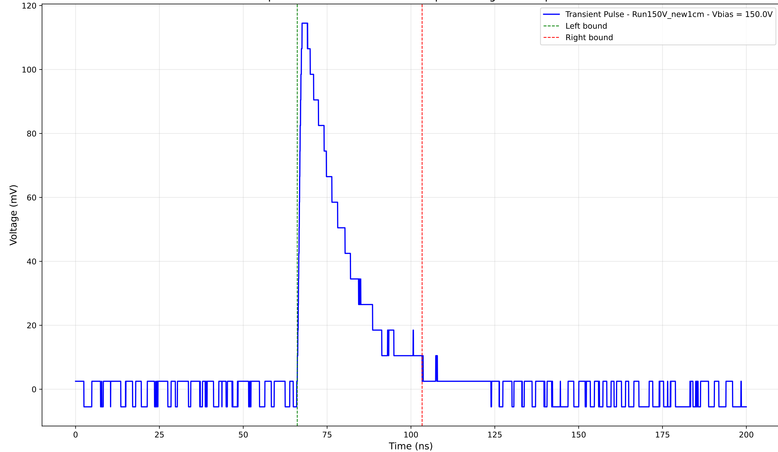
Transient Pulse - Sample: New1cm - Position: 705.0 \mu\text{m} - Charge: 31.13 pC - Rise Time: 1.08 ns
