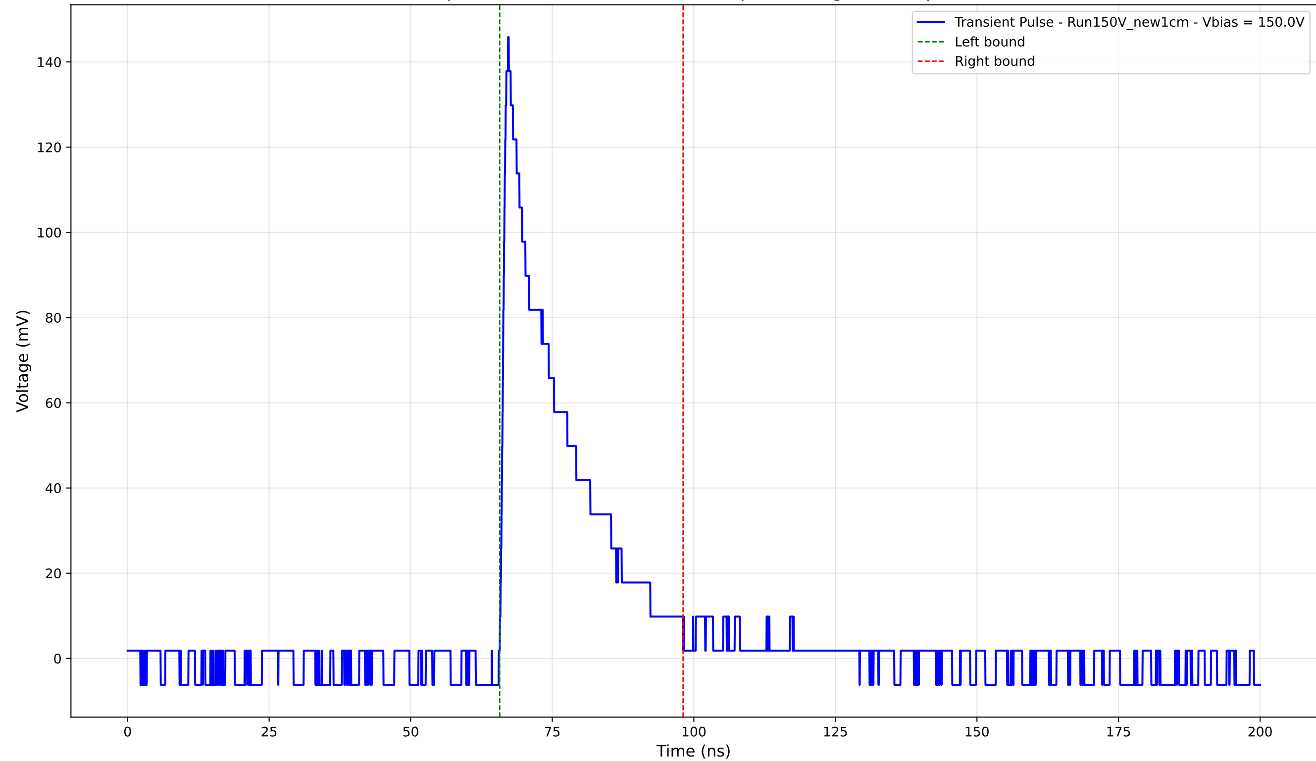
Transient Pulse - Sample: New1cm - Position: 4695.0 \mu\text{m} - Charge: 30.26 pC - Rise Time: 1.03 ns
