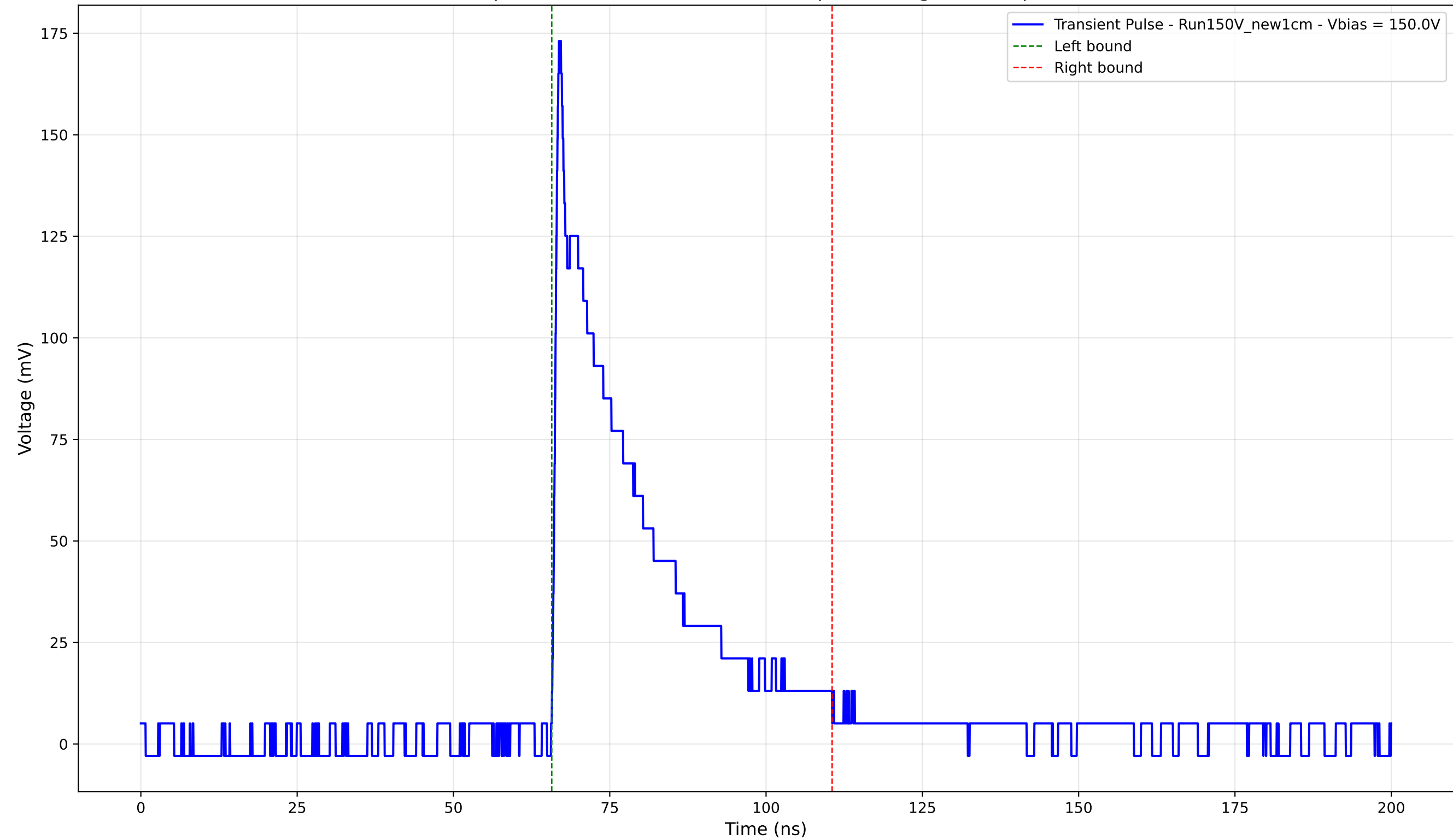
Transient Pulse - Sample: New1cm - Position: 2915.0 \mu\text{m} - Charge: 42.93 pC - Rise Time: 0.87 ns
