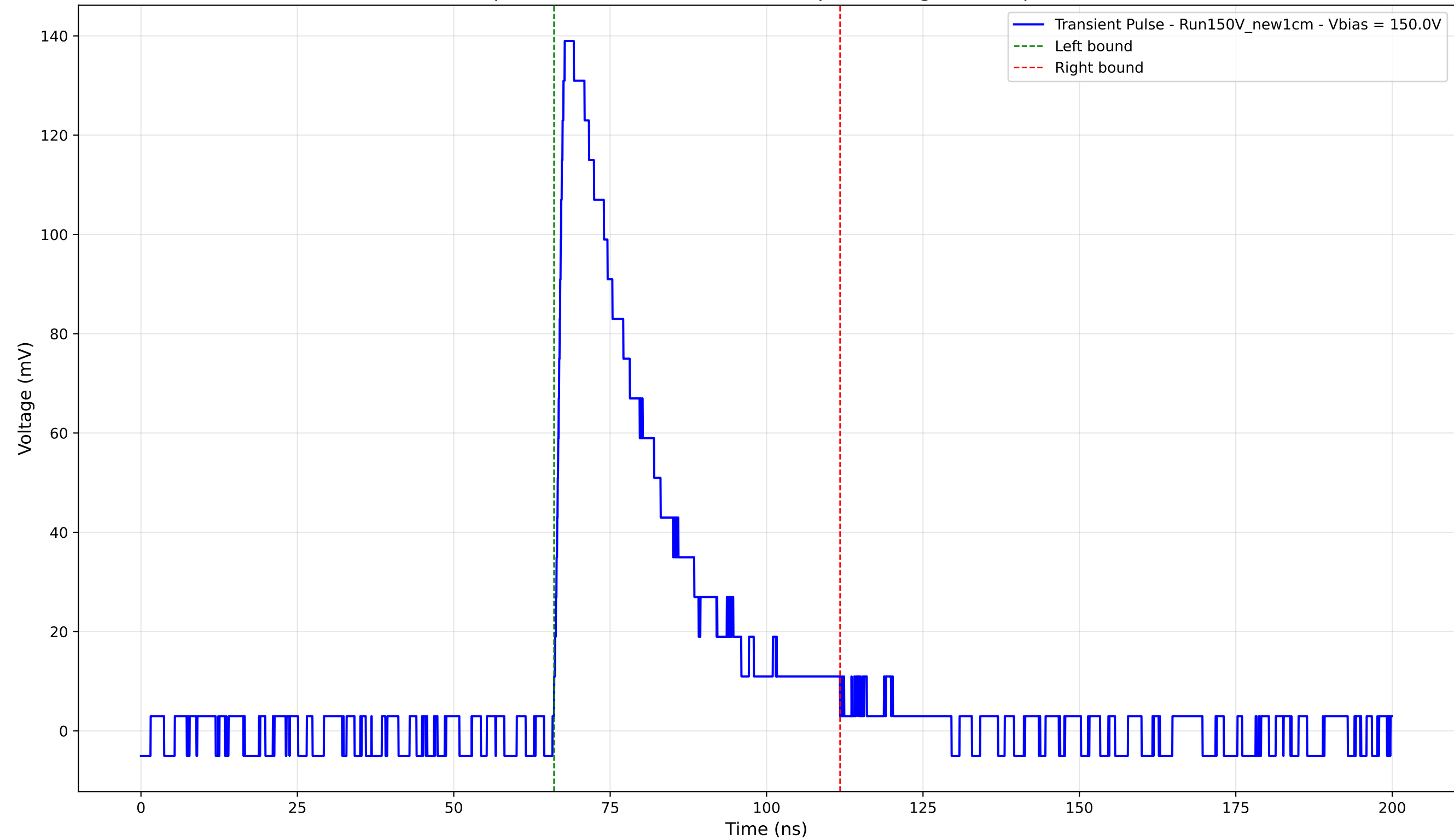
Transient Pulse - Sample: New1cm - Position: 3755.0 \mu\text{m} - Charge: 42.29 pC - Rise Time: 1.35 ns
