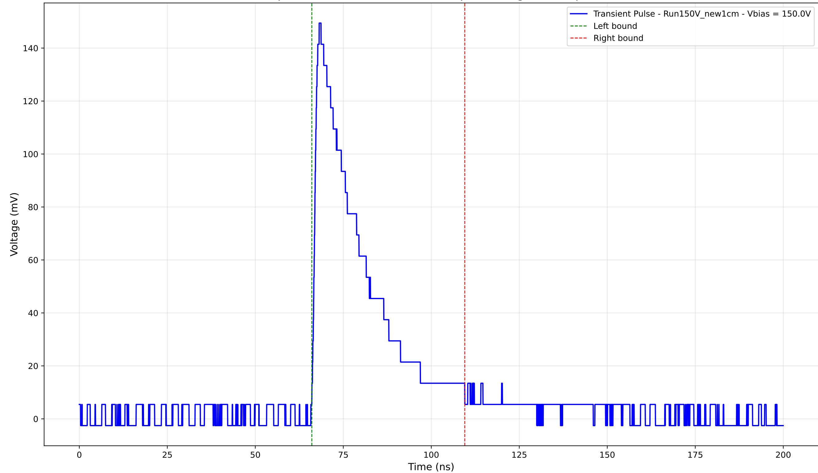
Transient Pulse - Sample: New1cm - Position: 3810.0 \mu\text{m} - Charge: 43.23 pC - Rise Time: 1.52 ns
