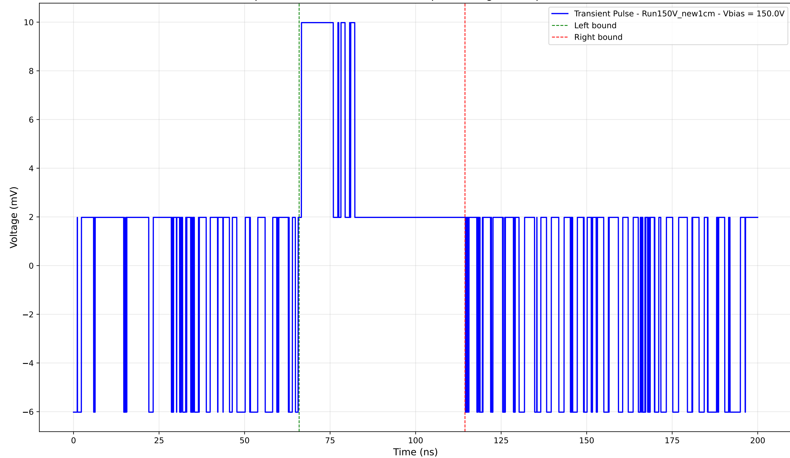
Transient Pulse - Sample: New1cm - Position: 1035.0 \mu\text{m} - Charge: 3.83 pC - Rise Time: 0.00 ns (N/A)
