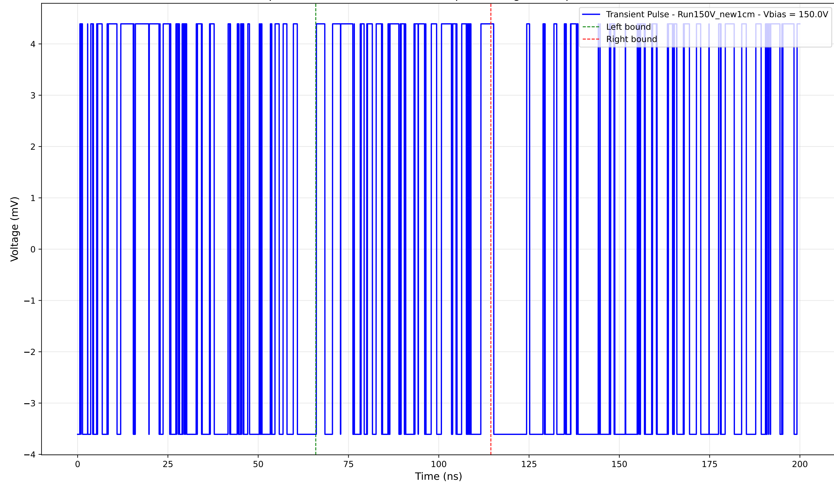
Transient Pulse - Sample: New1cm - Position: 4980.0 \mu\text{m} - Charge: 1.18 pC - Rise Time: 0.00 ns (N/A)
