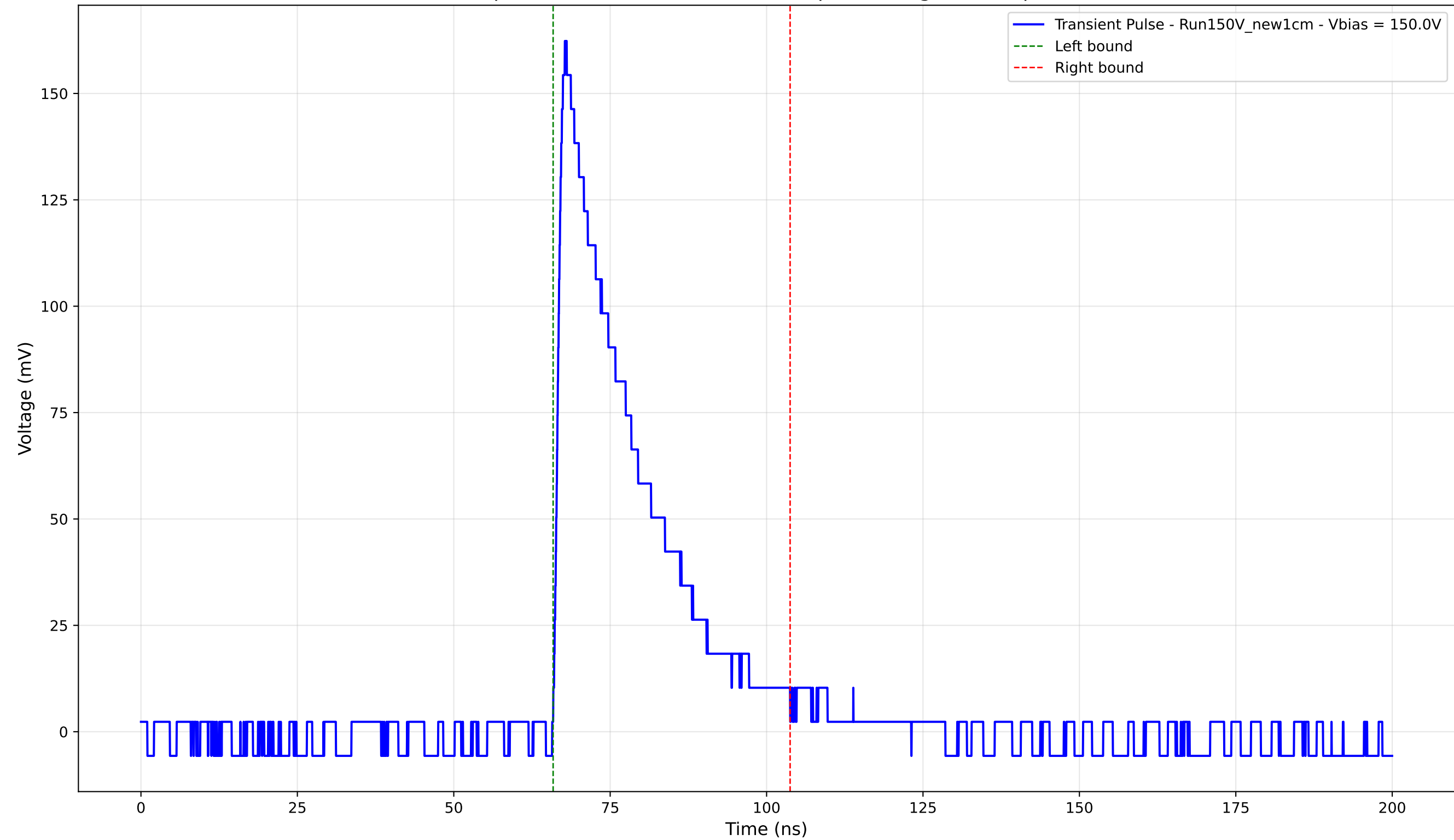
Transient Pulse - Sample: New1cm - Position: 4305.0 \mu\text{m} - Charge: 41.36 pC - Rise Time: 1.25 ns
