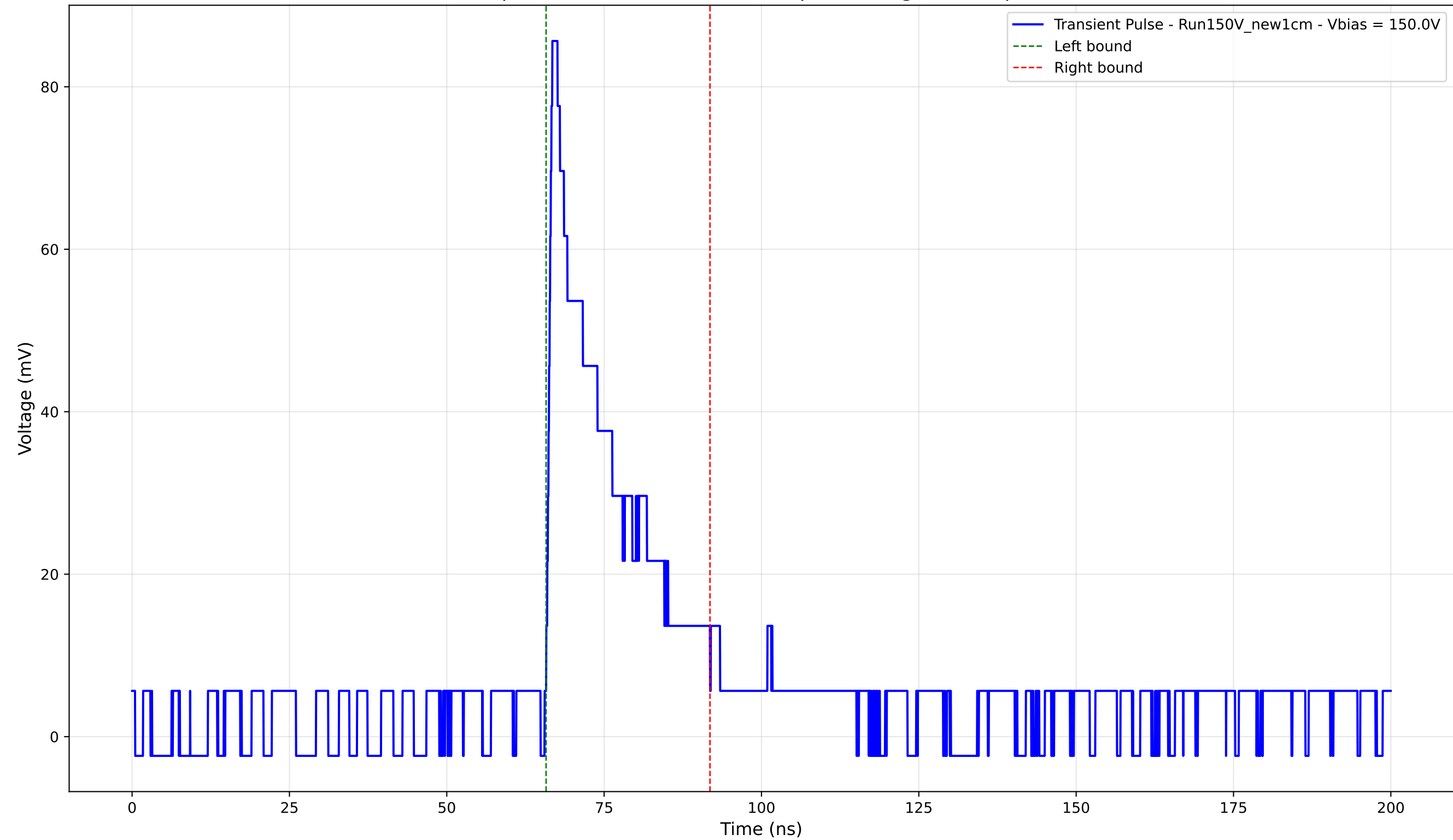
Transient Pulse - Sample: New1cm - Position: 95.0 \mu\text{m} - Charge: 17.30 pC - Rise Time: 0.83 ns
