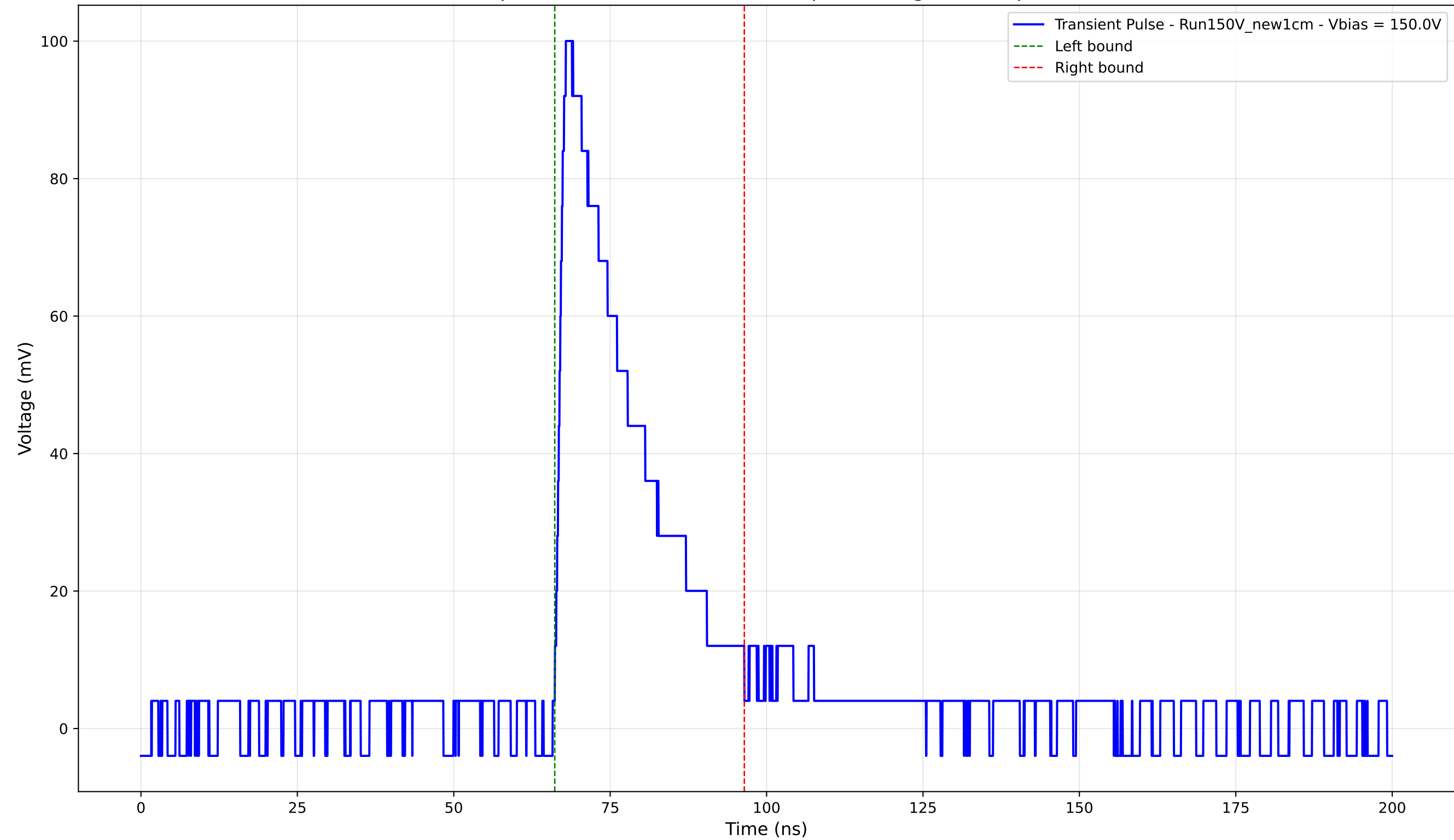
Transient Pulse - Sample: New1cm - Position: 945.0 \mu\text{m} - Charge: 25.81 pC - Rise Time: 1.47 ns
