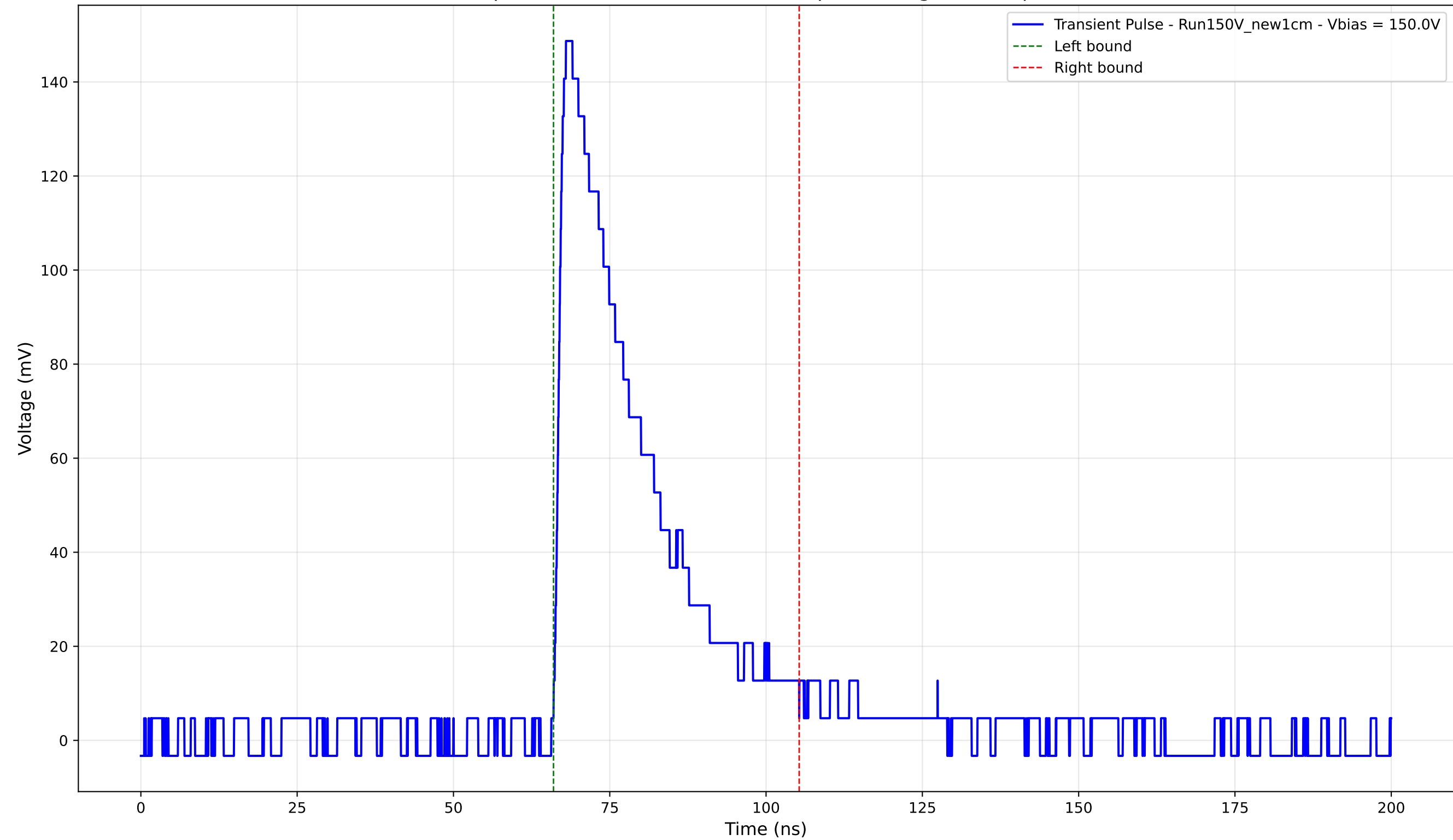
Transient Pulse - Sample: New1cm - Position: 3820.0 \mu\text{m} - Charge: 42.55 pC - Rise Time: 1.47 ns
