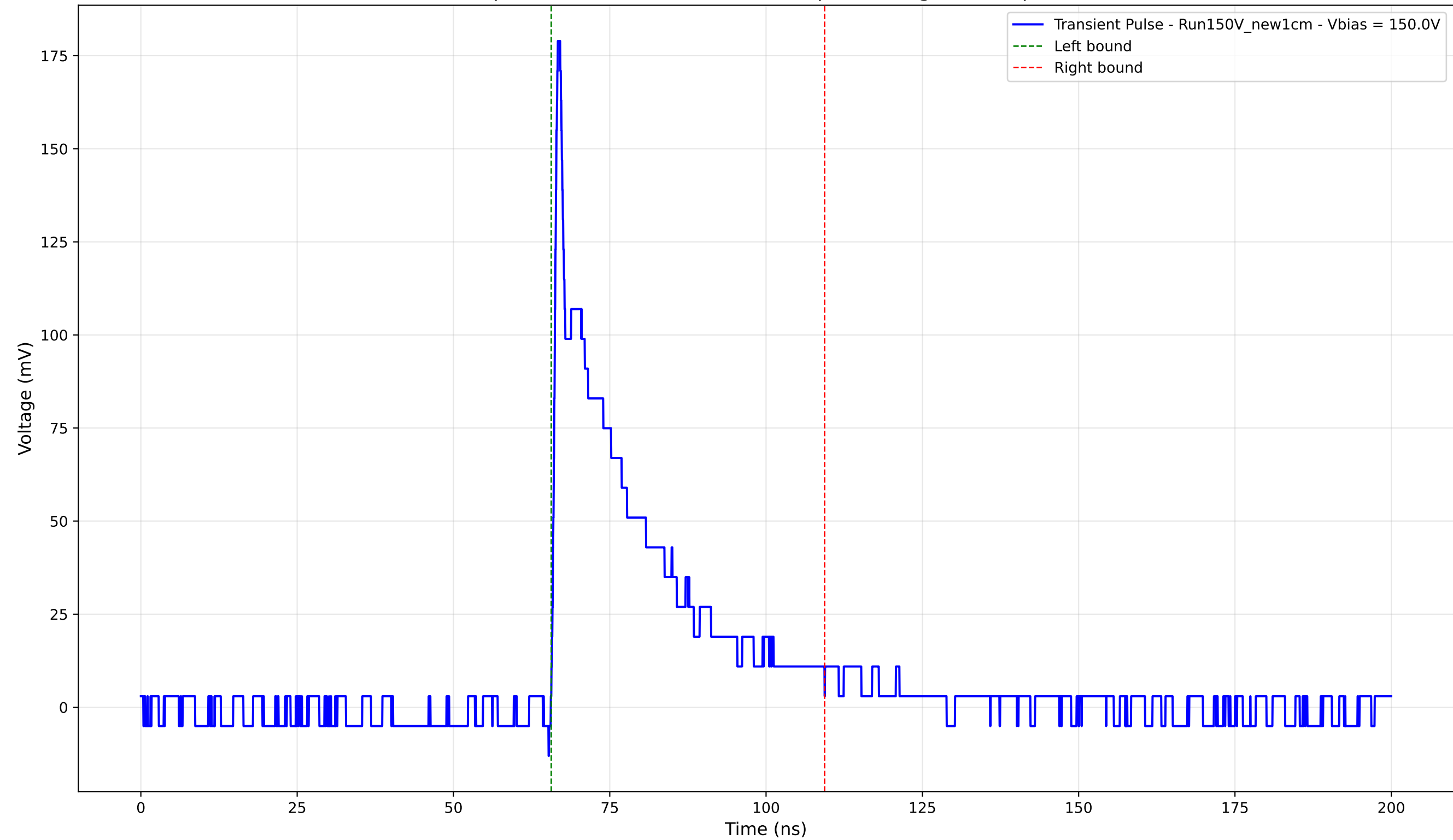
Transient Pulse - Sample: New1cm - Position: 2330.0 \mu\text{m} - Charge: 37.10 pC - Rise Time: 0.80 ns
