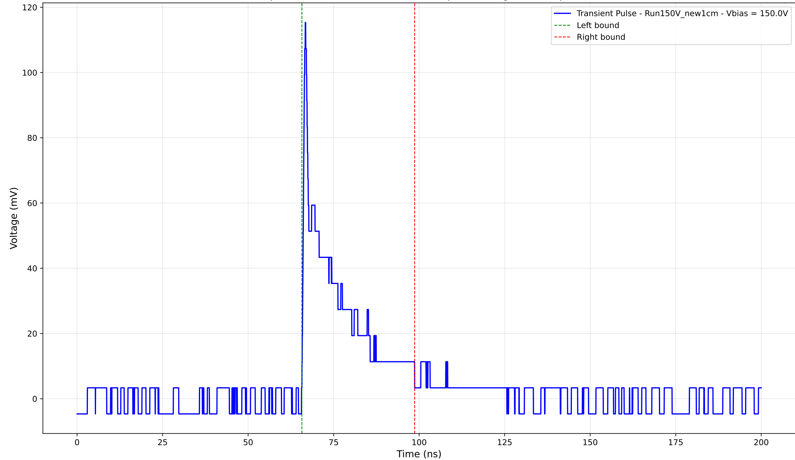
Transient Pulse - Sample: New1cm - Position: 2495.0 \mu\text{m} - Charge: 18.41 pC - Rise Time: 0.74 ns
