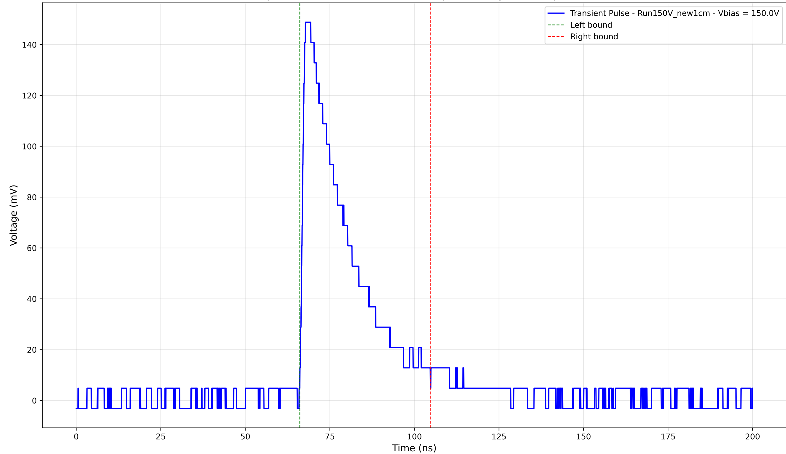
Transient Pulse - Sample: New1cm - Position: 3790.0 \mu\text{m} - Charge: 43.57 pC - Rise Time: 1.29 ns
