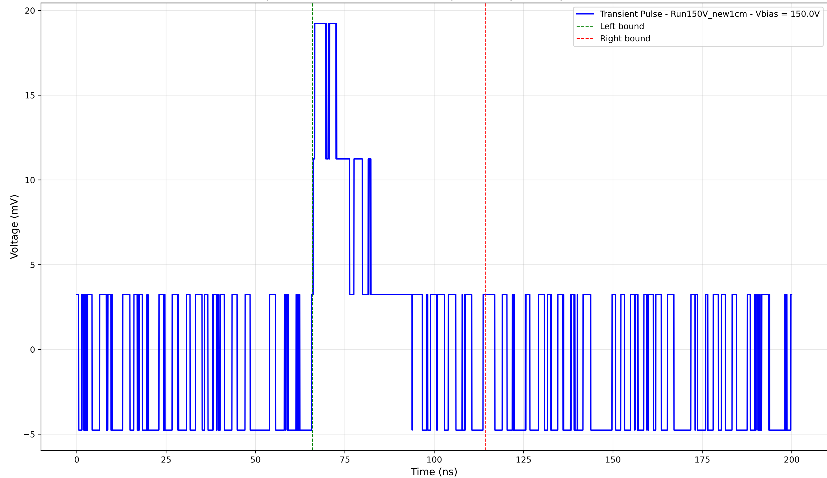
Transient Pulse - Sample: New1cm - Position: 4580.0 \mu\text{m} - Charge: 4.71 pC - Rise Time: 0.00 ns (N/A)
