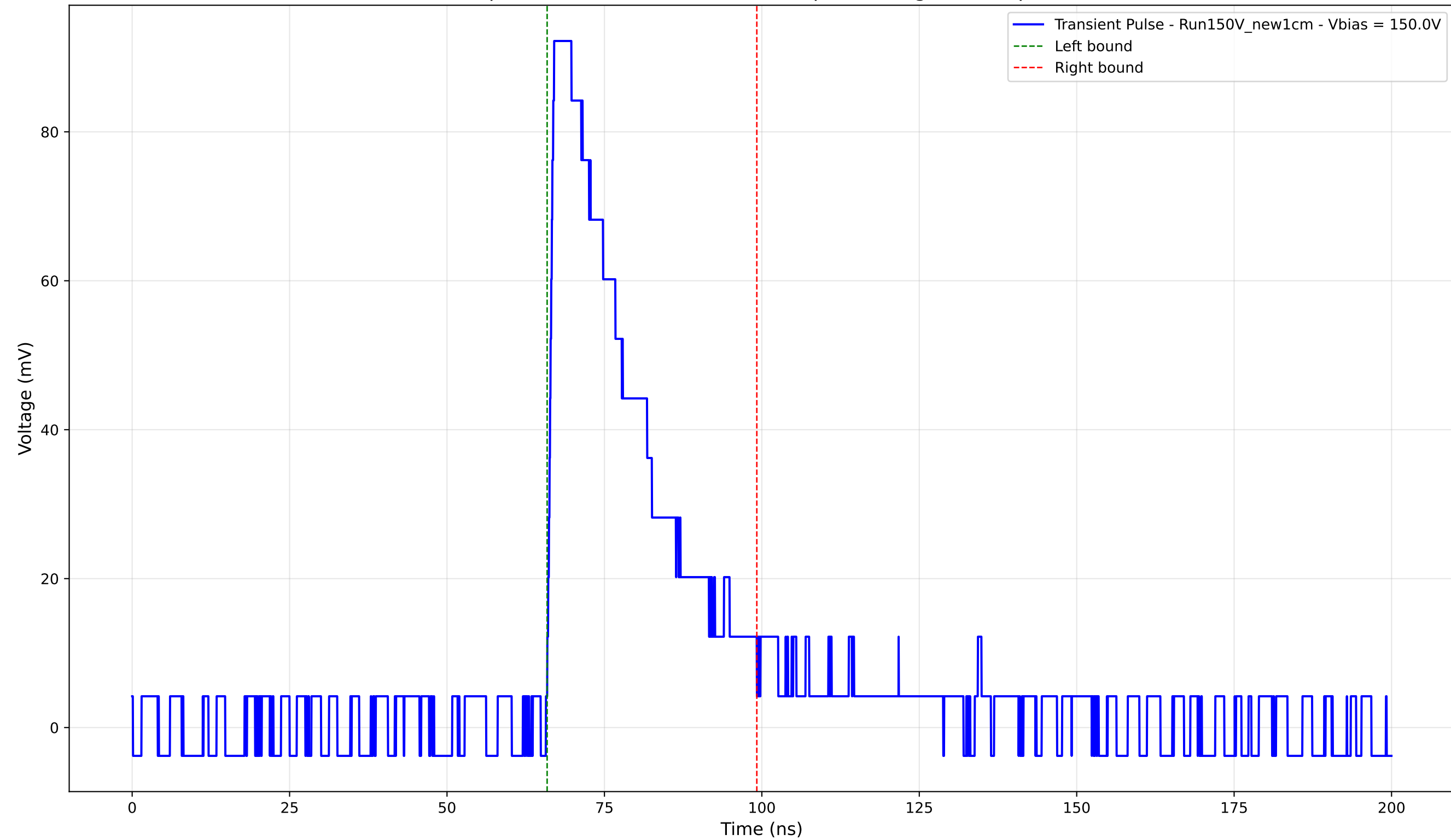
Transient Pulse - Sample: New1cm - Position: 1905.0 \mu\text{m} - Charge: 27.66 pC - Rise Time: 0.95 ns
