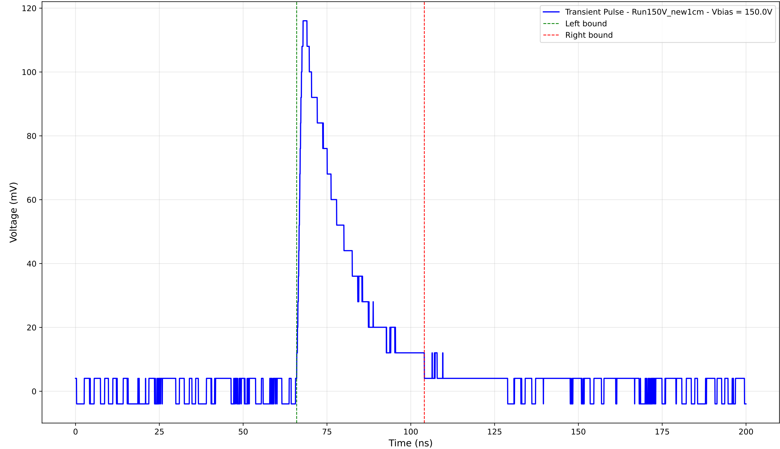
Transient Pulse - Sample: New1cm - Position: 3990.0 \mu\text{m} - Charge: 32.18 pC - Rise Time: 1.56 ns
