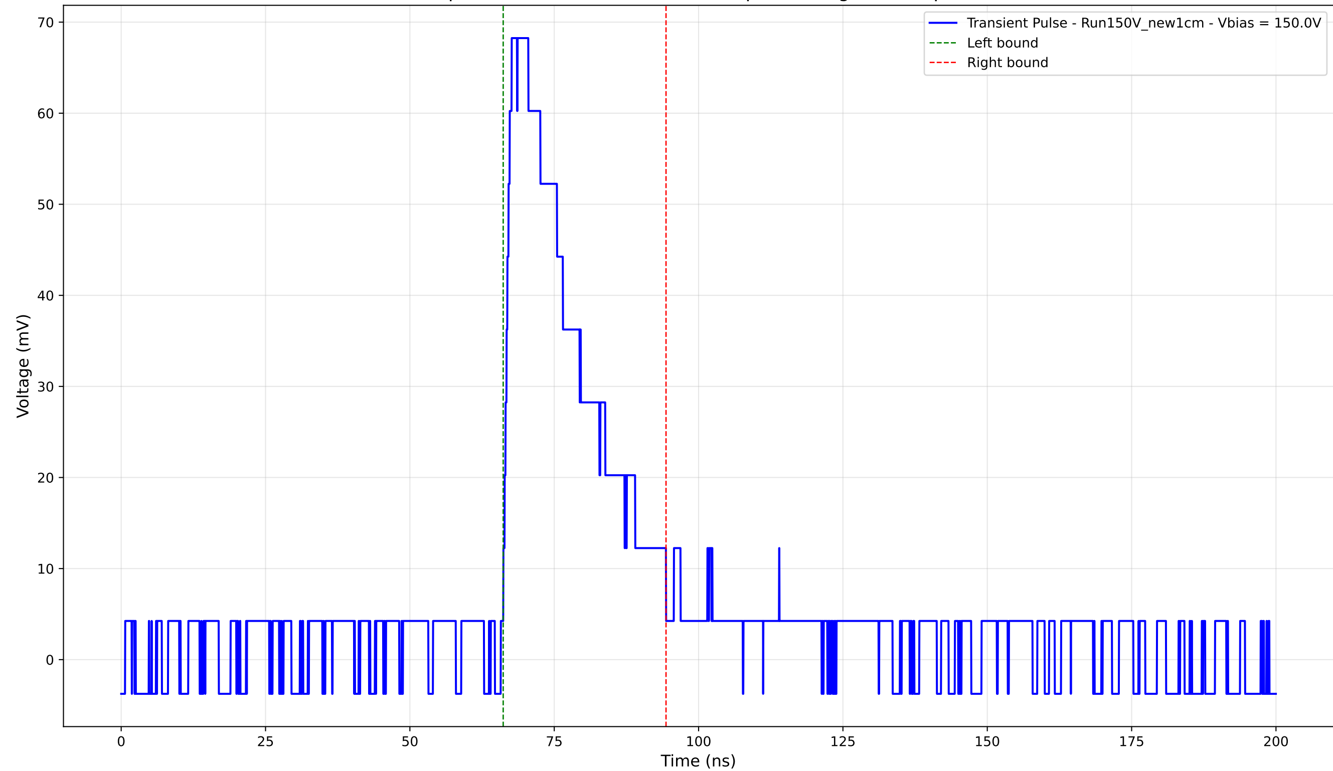
Transient Pulse - Sample: New1cm - Position: 1605.0 \mu\text{m} - Charge: 19.46 pC - Rise Time: 1.45 ns
