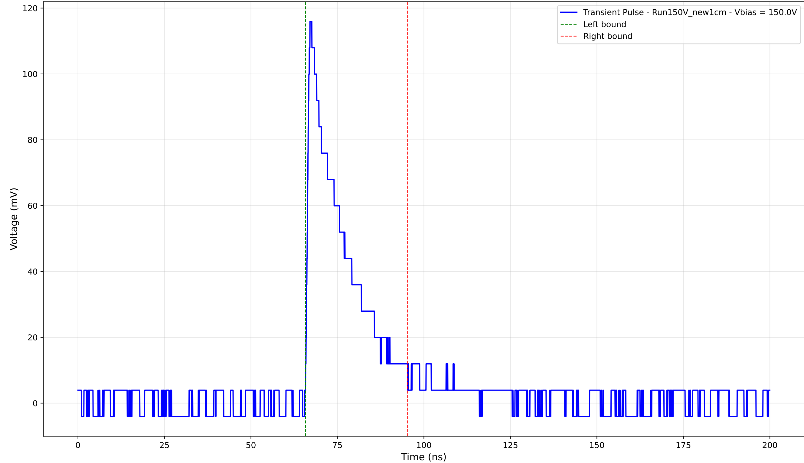
Transient Pulse - Sample: New1cm - Position: 4655.0 \mu\text{m} - Charge: 25.70 pC - Rise Time: 1.06 ns
