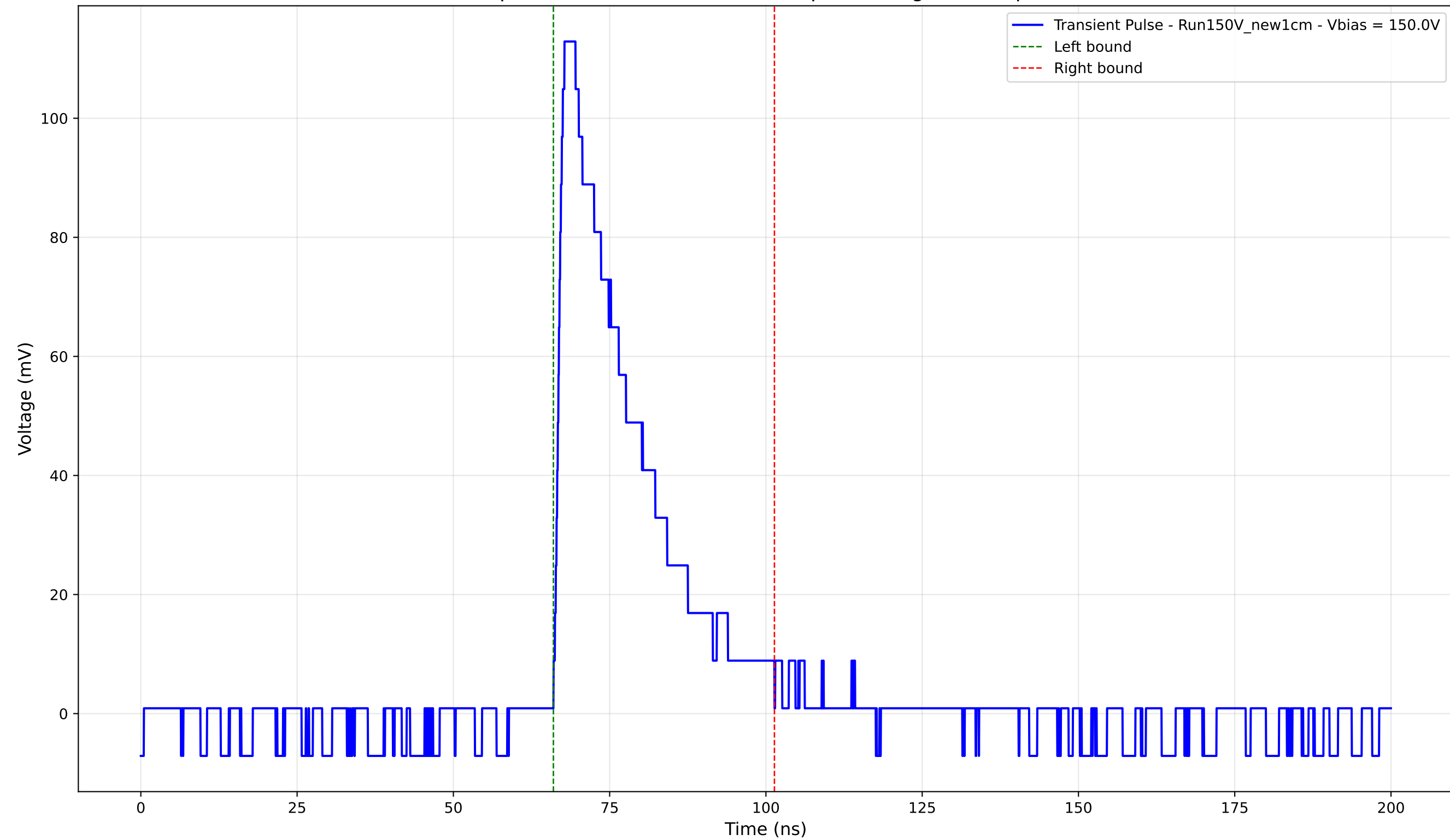
Transient Pulse - Sample: New1cm - Position: 755.0 \mu\text{m} - Charge: 29.17 pC - Rise Time: 1.27 ns
