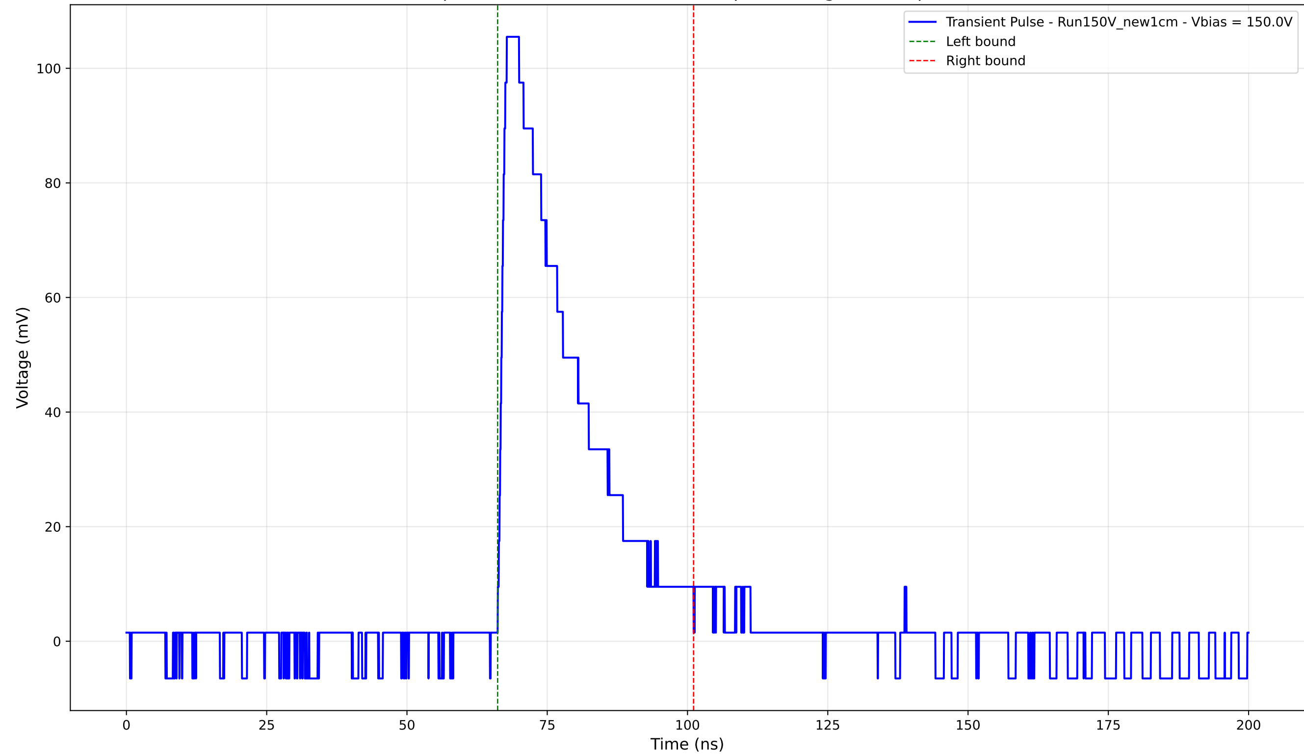
Transient Pulse - Sample: New1cm - Position: 1380.0 \mu\text{m} - Charge: 29.59 pC - Rise Time: 1.18 ns
