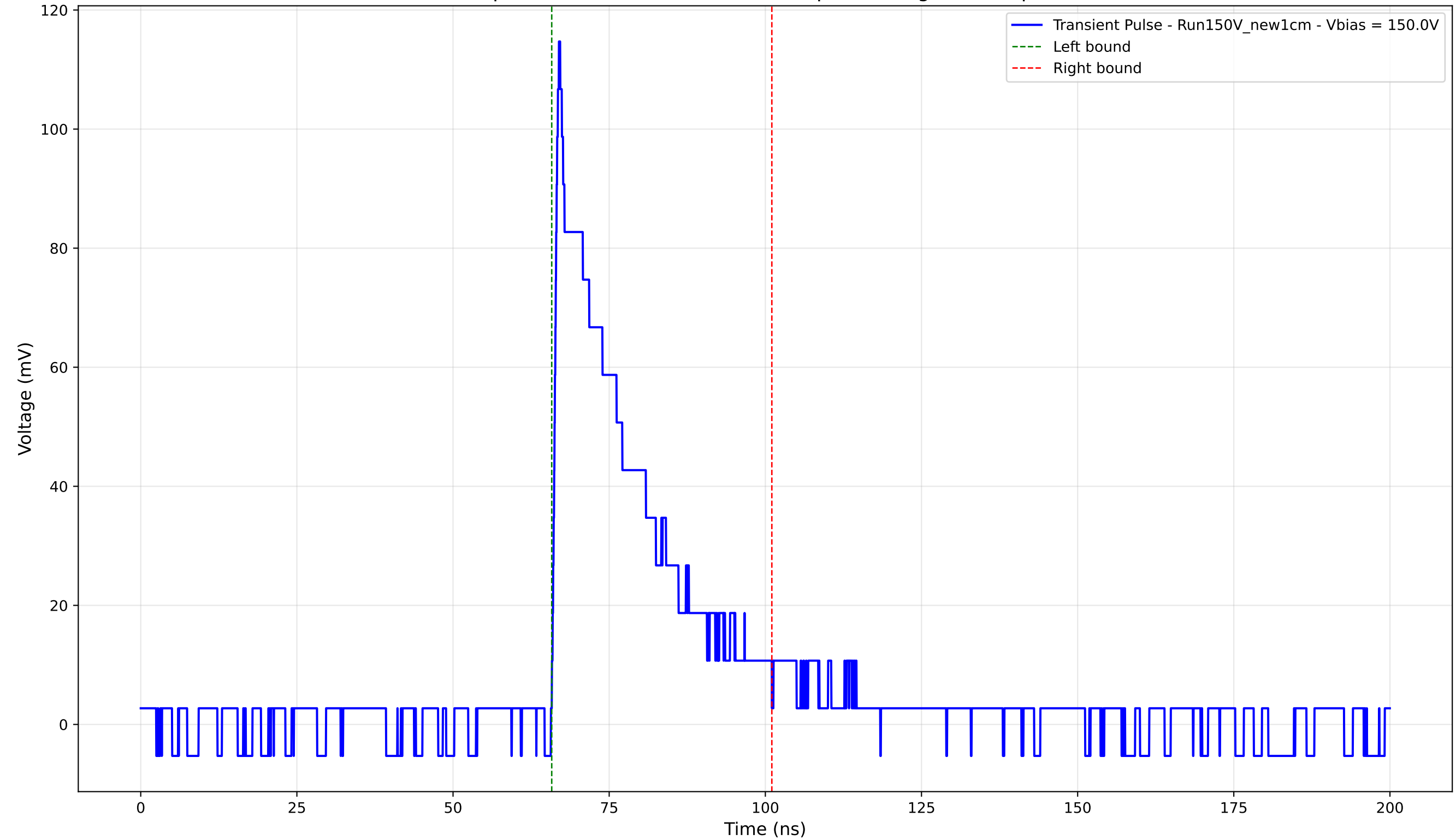
Transient Pulse - Sample: New1cm - Position: 2140.0 \mu\text{m} - Charge: 26.89 pC - Rise Time: 0.86 ns
