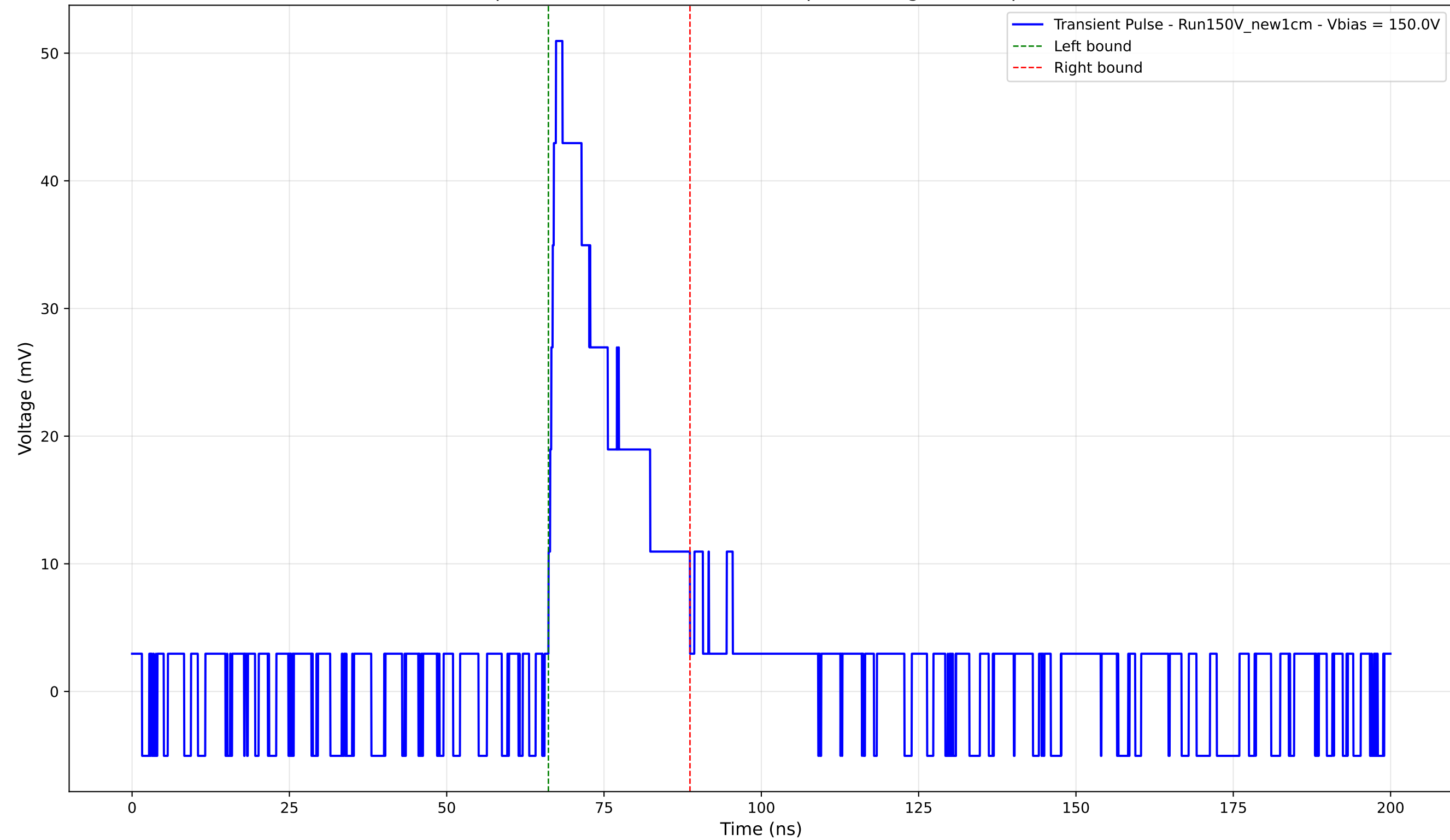
Transient Pulse - Sample: New1cm - Position: 575.0 \mu\text{m} - Charge: 10.74 pC - Rise Time: 1.19 ns
