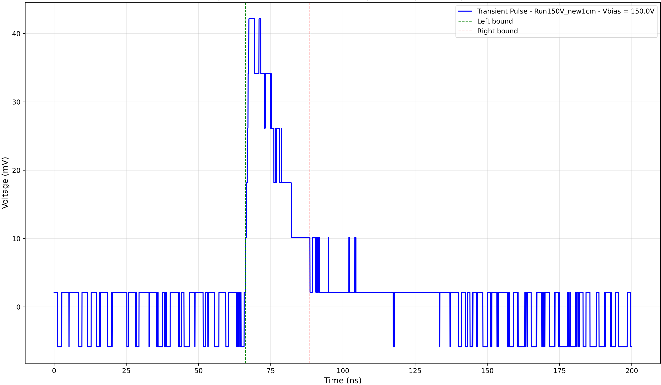
Transient Pulse - Sample: New1cm - Position: 3595.0 \mu\text{m} - Charge: 10.29 pC - Rise Time: 1.17 ns
