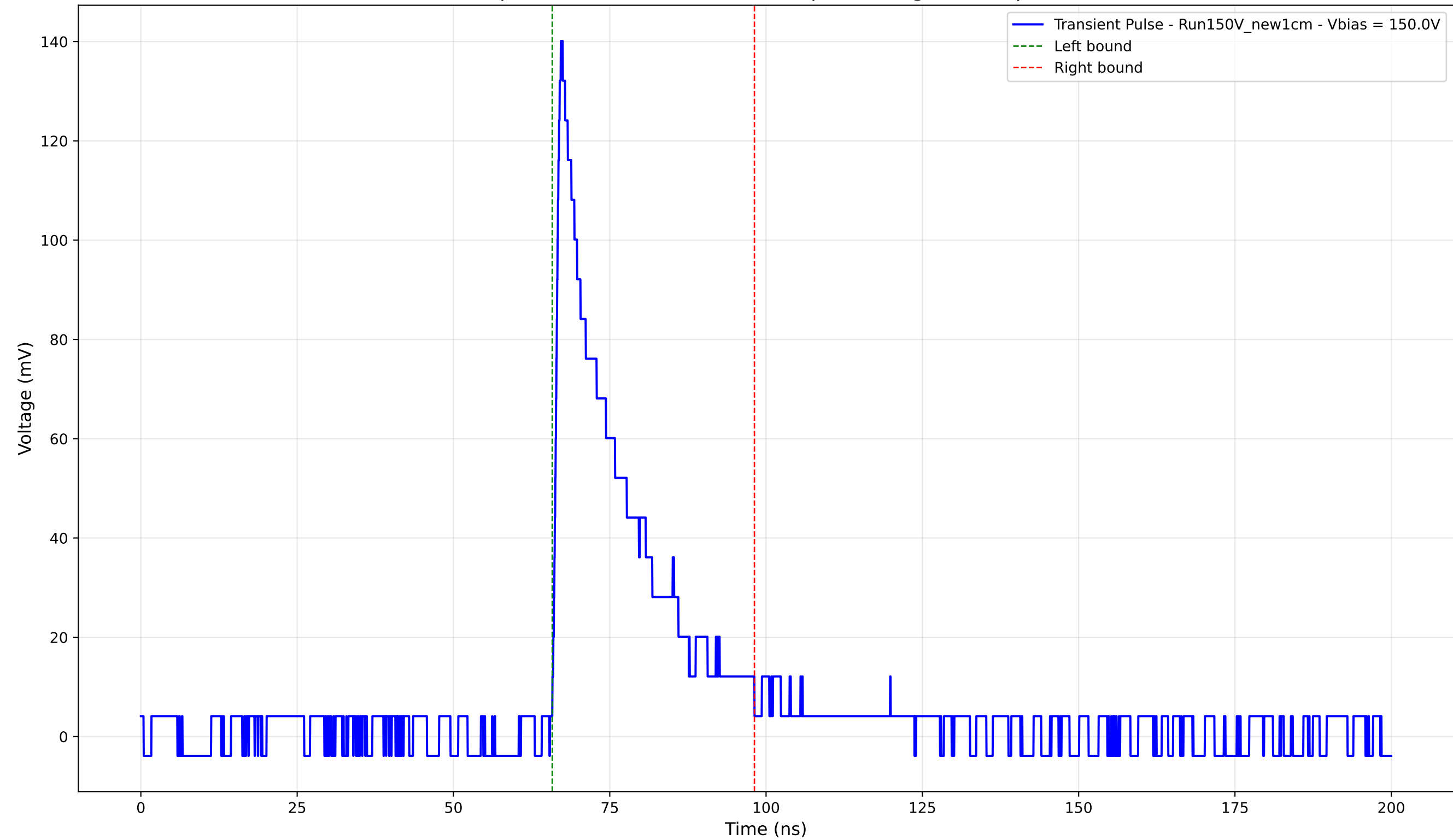
Transient Pulse - Sample: New1cm - Position: 255.0 \mu\text{m} - Charge: 28.40 pC - Rise Time: 1.04 ns
