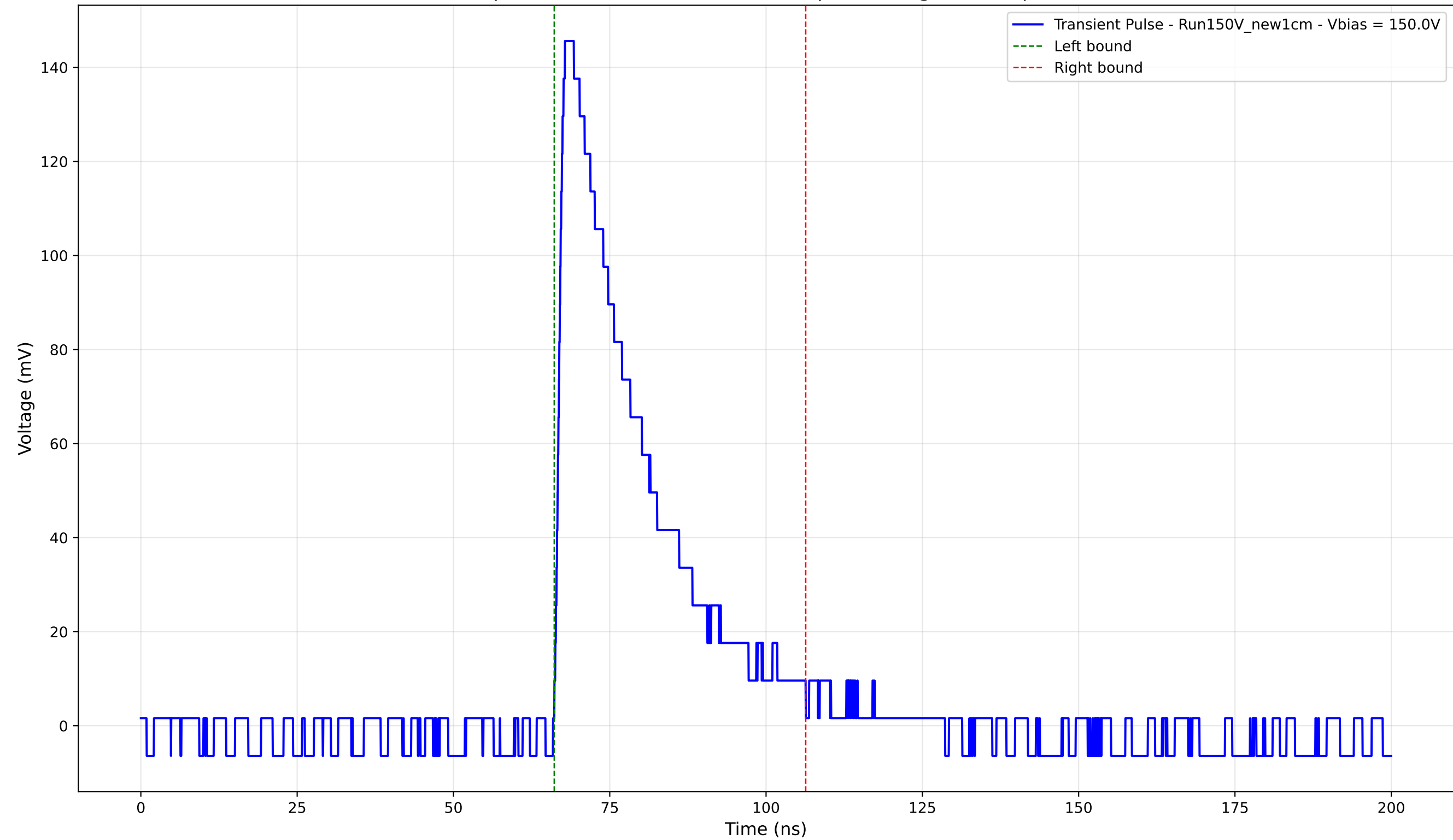
Transient Pulse - Sample: New1cm - Position: 3780.0 \mu\text{m} - Charge: 40.63 pC - Rise Time: 1.33 ns
