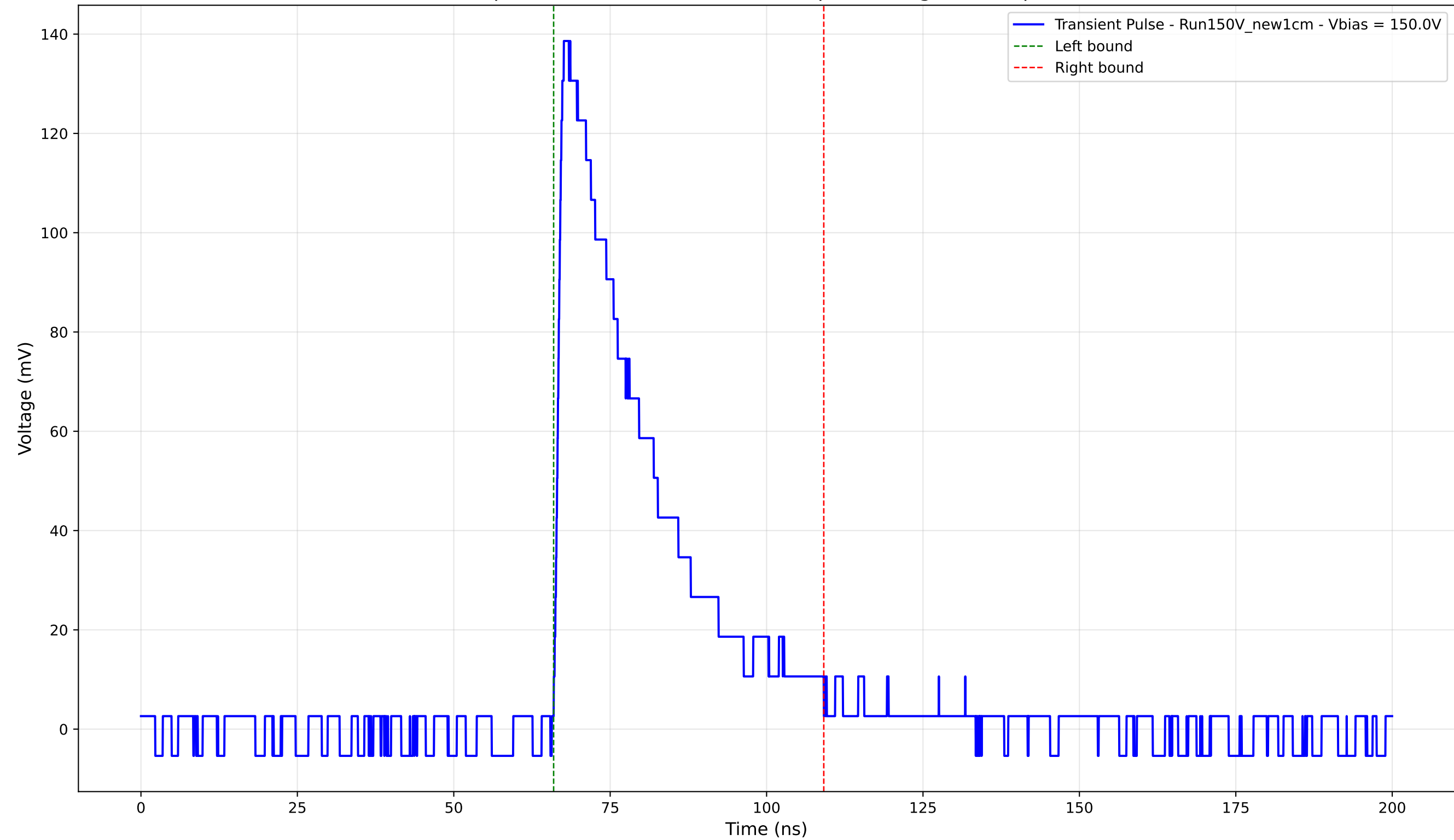
Transient Pulse - Sample: New1cm - Position: 3435.0 \mu\text{m} - Charge: 41.08 pC - Rise Time: 1.23 ns
