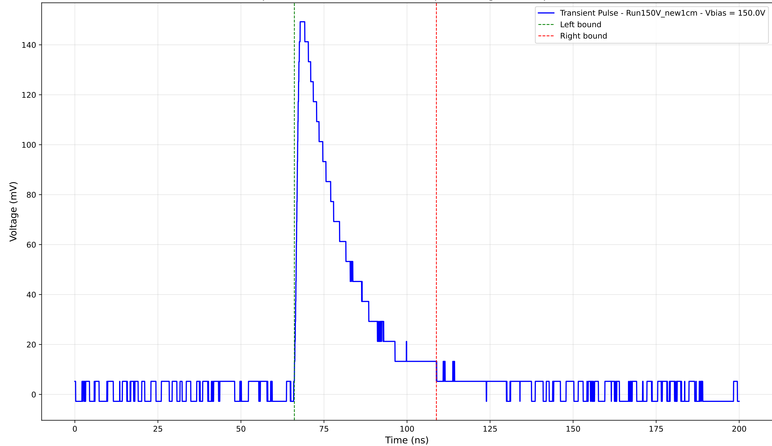
Transient Pulse - Sample: New1cm - Position: 3835.0 \mu\text{m} - Charge: 43.95 pC - Rise Time: 1.36 ns
