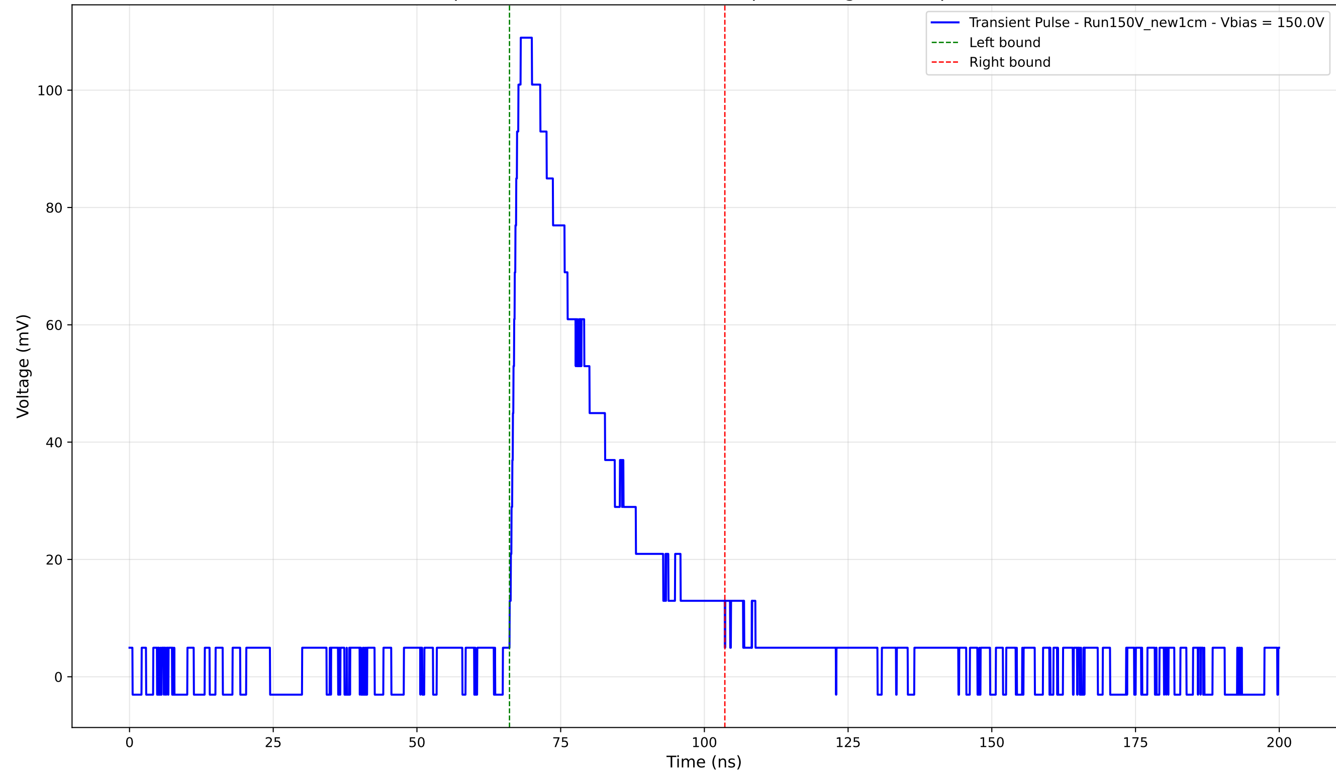
Transient Pulse - Sample: New1cm - Position: 1425.0 \mu\text{m} - Charge: 32.76 pC - Rise Time: 1.53 ns
