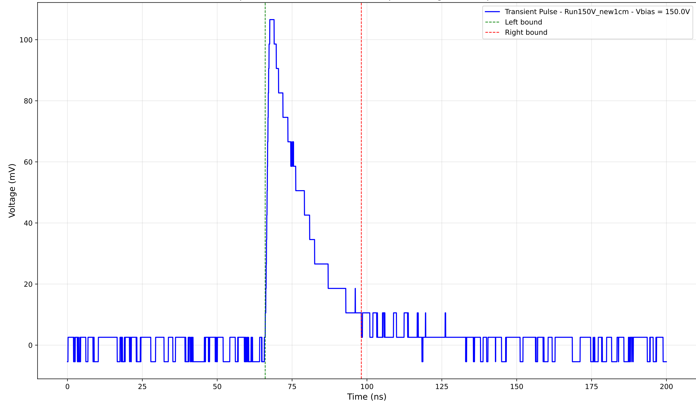
Transient Pulse - Sample: New1cm - Position: 635.0 \mu\text{m} - Charge: 27.05 pC - Rise Time: 1.10 ns
