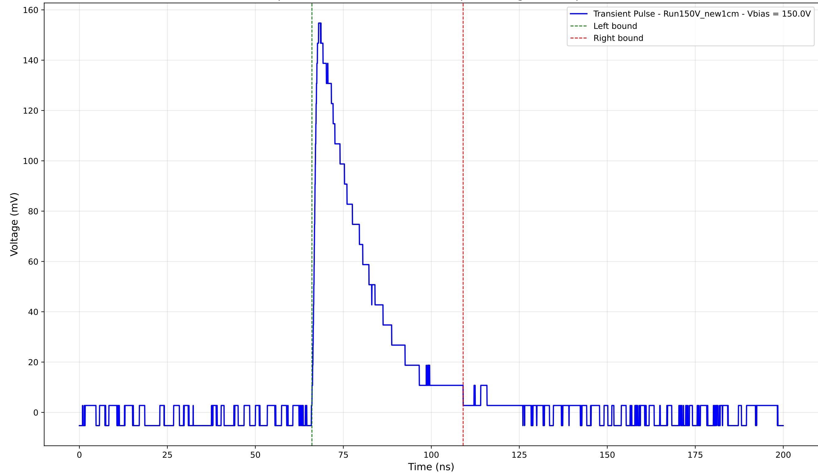
Transient Pulse - Sample: New1cm - Position: 3870.0 \mu\text{m} - Charge: 43.31 pC - Rise Time: 1.39 ns
