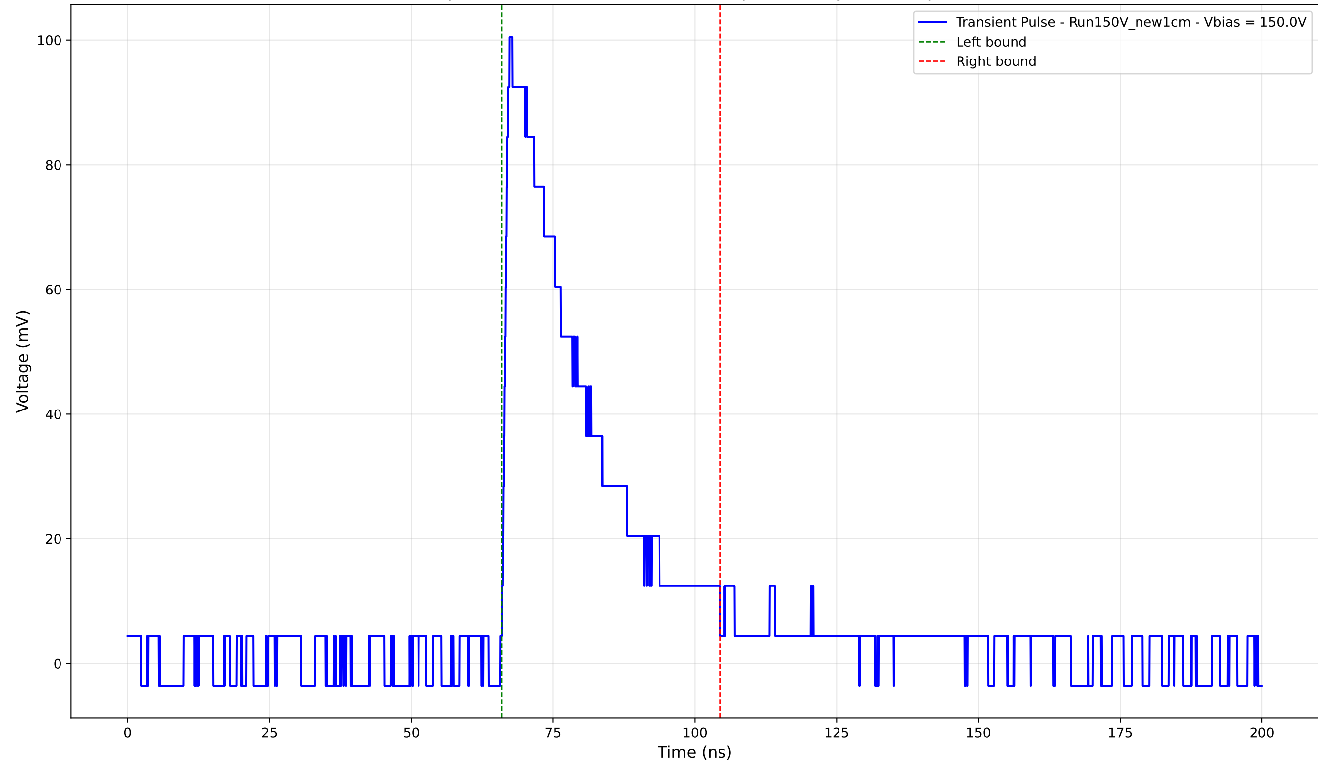
Transient Pulse - Sample: New1cm - Position: 1835.0 \mu\text{m} - Charge: 29.90 pC - Rise Time: 1.09 ns
