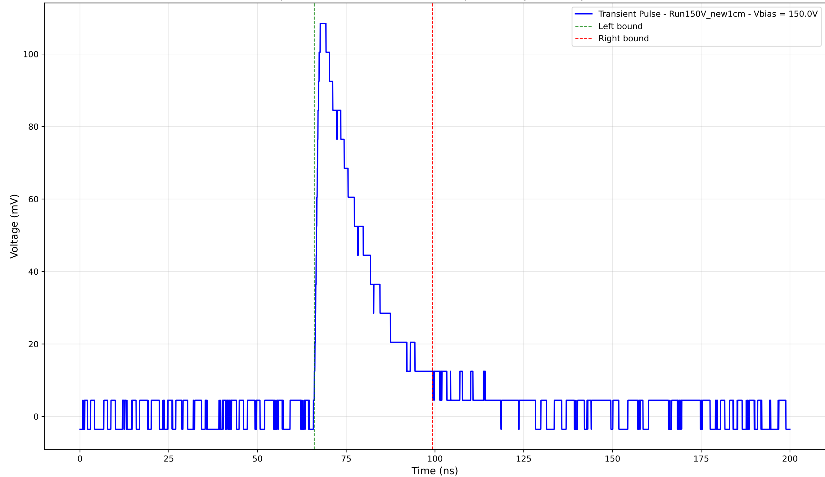
Transient Pulse - Sample: New1cm - Position: 4165.0 \mu\text{m} - Charge: 30.14 pC - Rise Time: 1.36 ns
