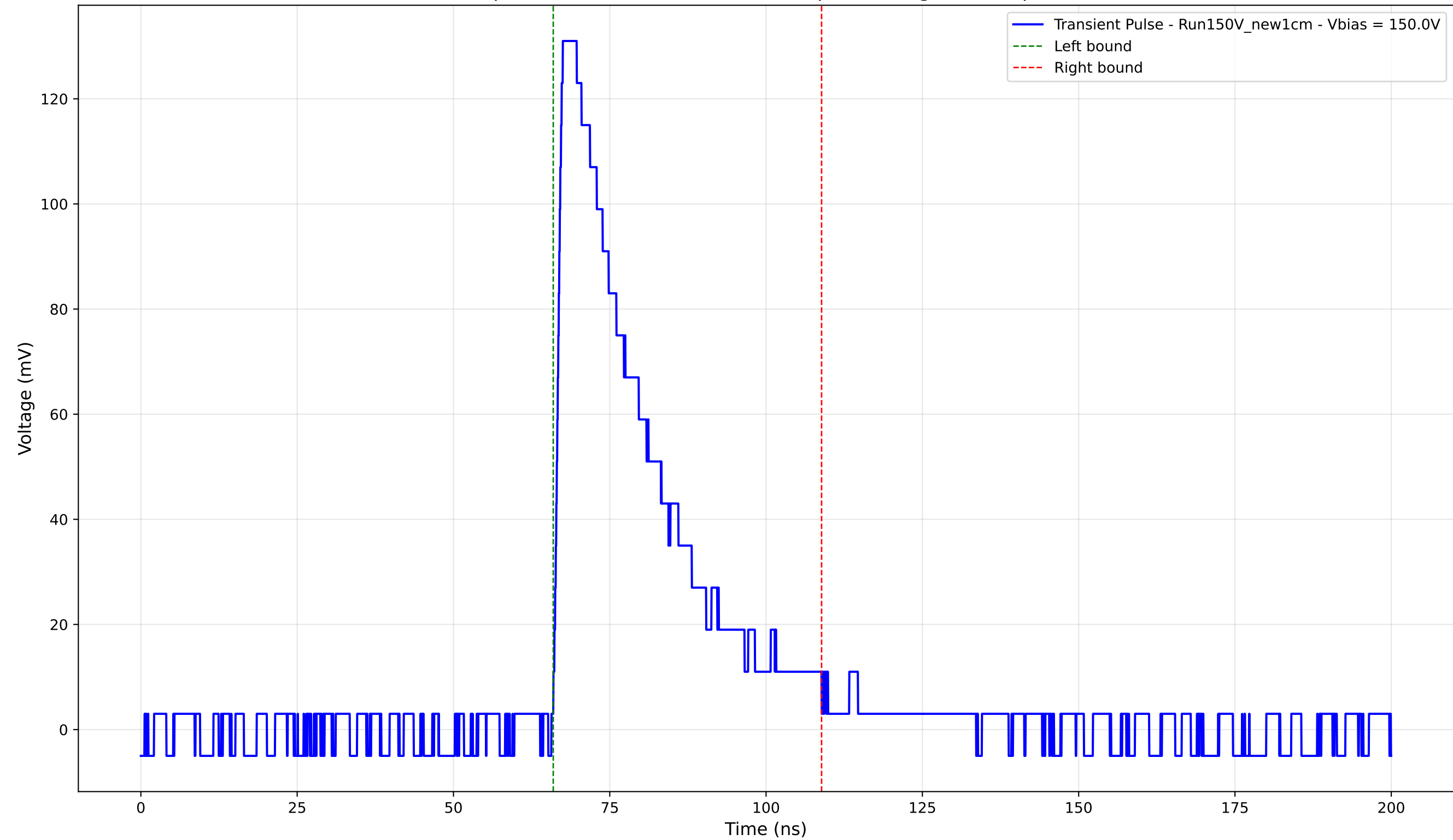
Transient Pulse - Sample: New1cm - Position: 3460.0 \mu\text{m} - Charge: 40.37 pC - Rise Time: 1.17 ns
