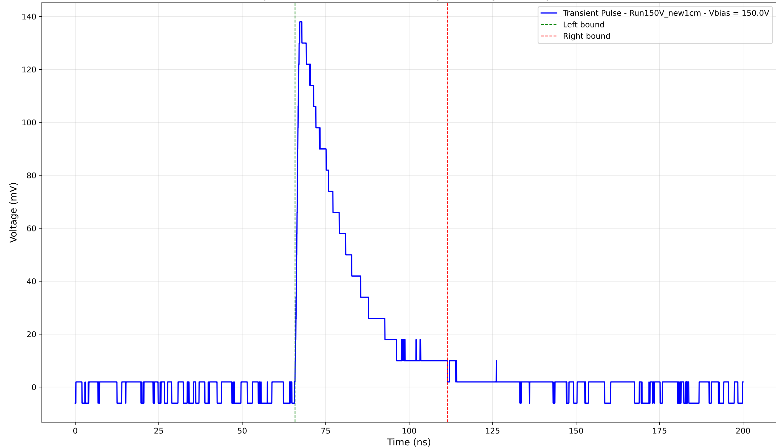
Transient Pulse - Sample: New1cm - Position: 3190.0 \mu\text{m} - Charge: 40.13 pC - Rise Time: 1.07 ns
