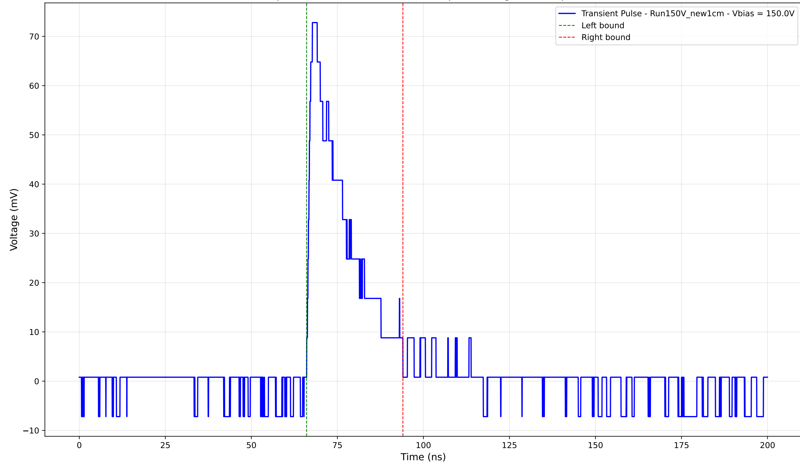
Transient Pulse - Sample: New1cm - Position: 595.0 \mu\text{m} - Charge: 16.78 pC - Rise Time: 1.64 ns
