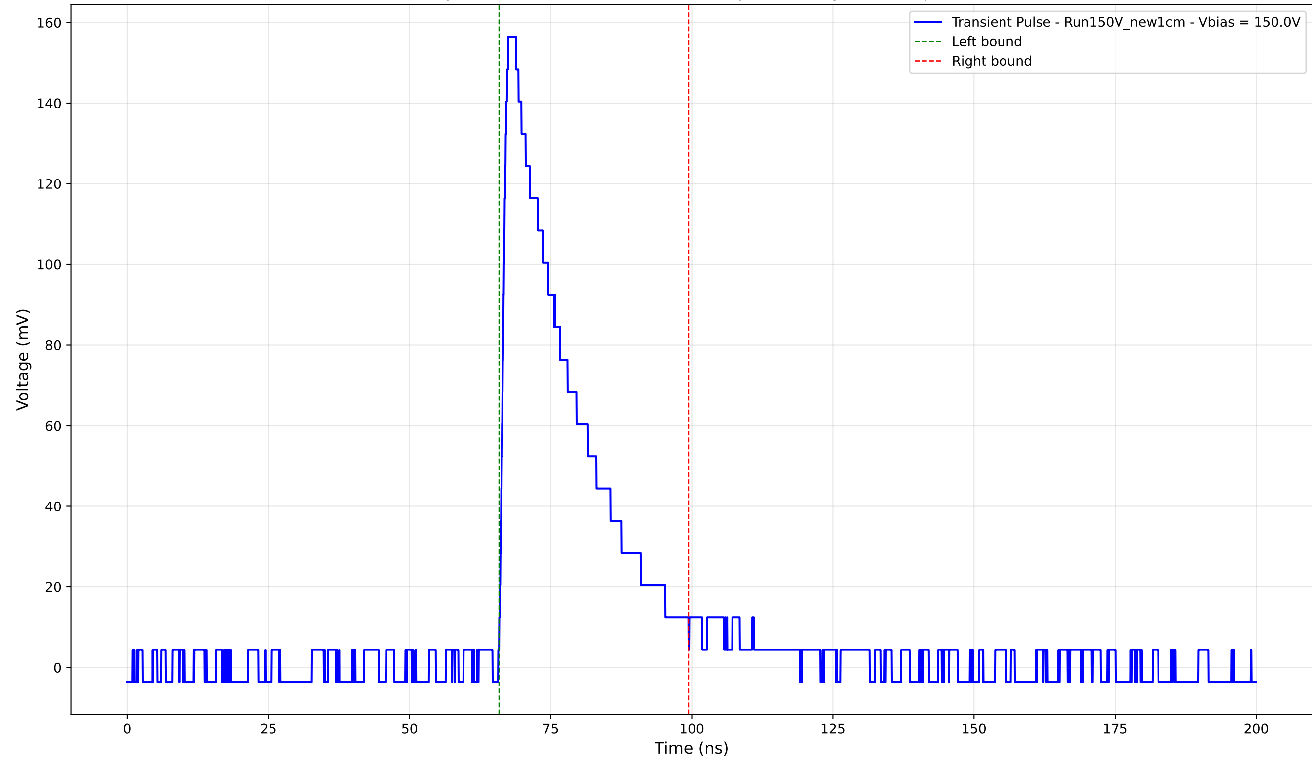
Transient Pulse - Sample: New1cm - Position: 4365.0 \mu\text{m} - Charge: 41.17 pC - Rise Time: 1.27 ns
