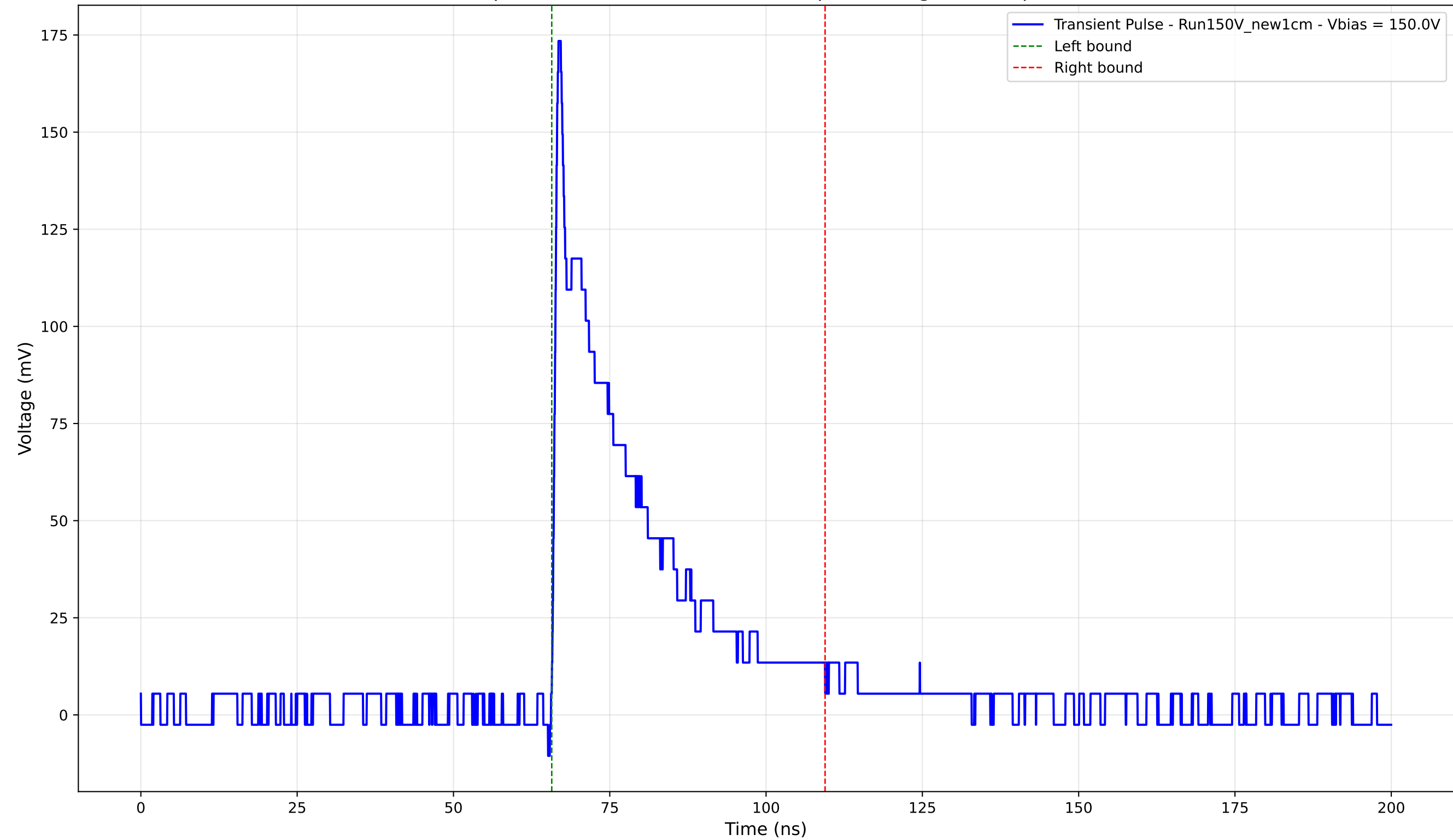
Transient Pulse - Sample: New1cm - Position: 2860.0 \mu\text{m} - Charge: 40.61 pC - Rise Time: 0.79 ns
