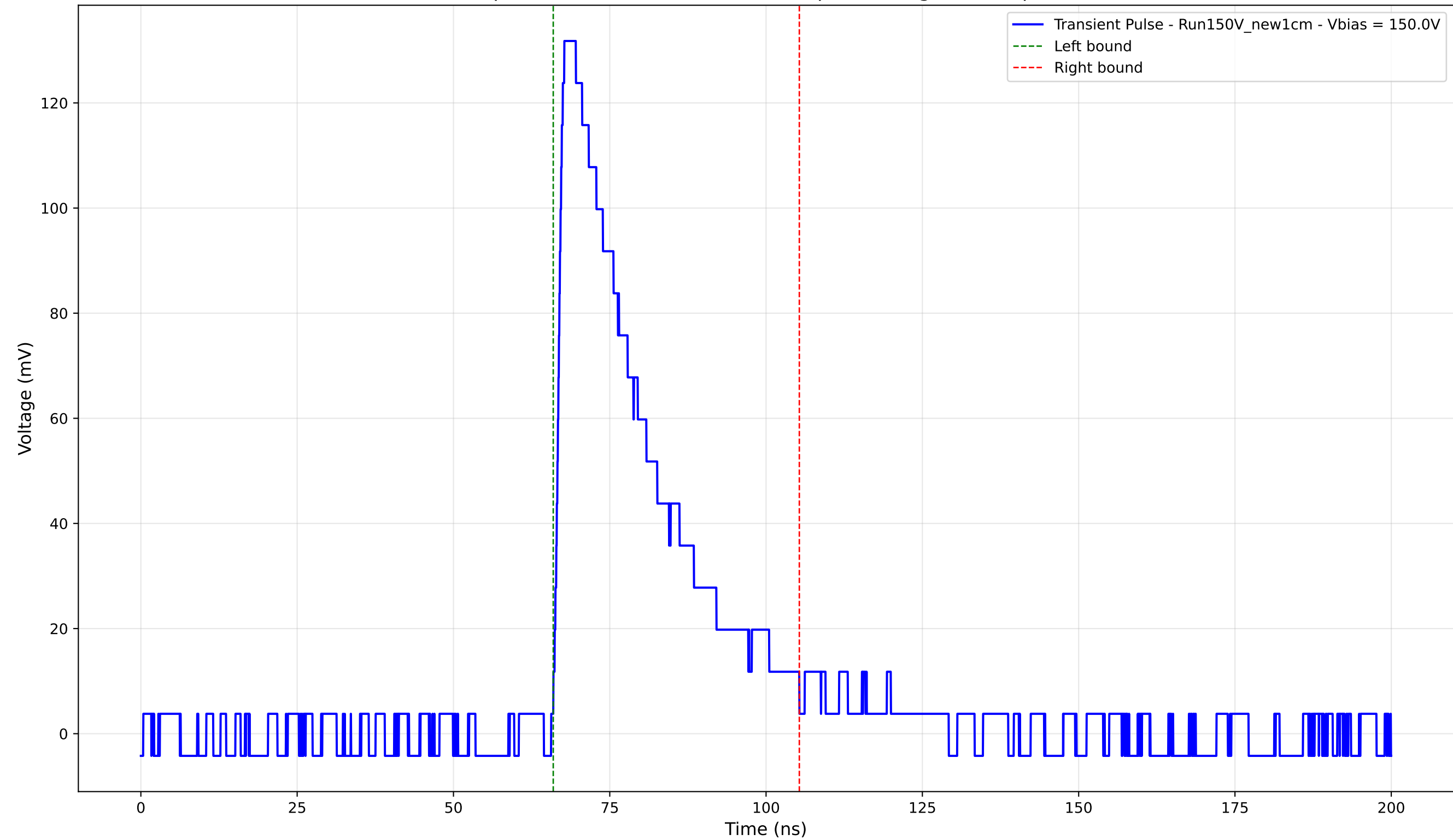
Transient Pulse - Sample: New1cm - Position: 3675.0 \mu\text{m} - Charge: 40.40 pC - Rise Time: 1.32 ns
