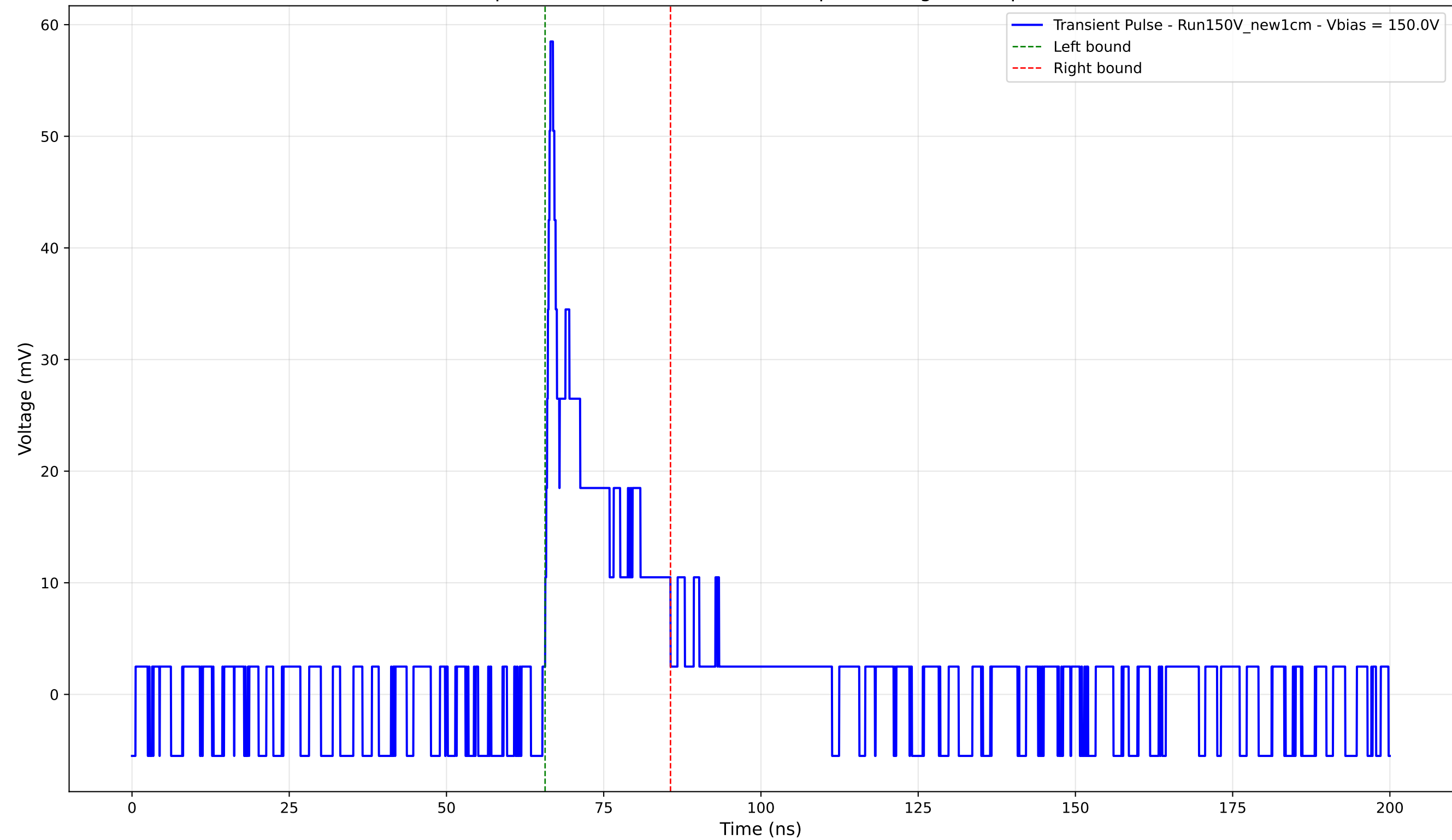
Transient Pulse - Sample: New1cm - Position: 2520.0 \mu\text{m} - Charge: 7.73 pC - Rise Time: 0.83 ns
