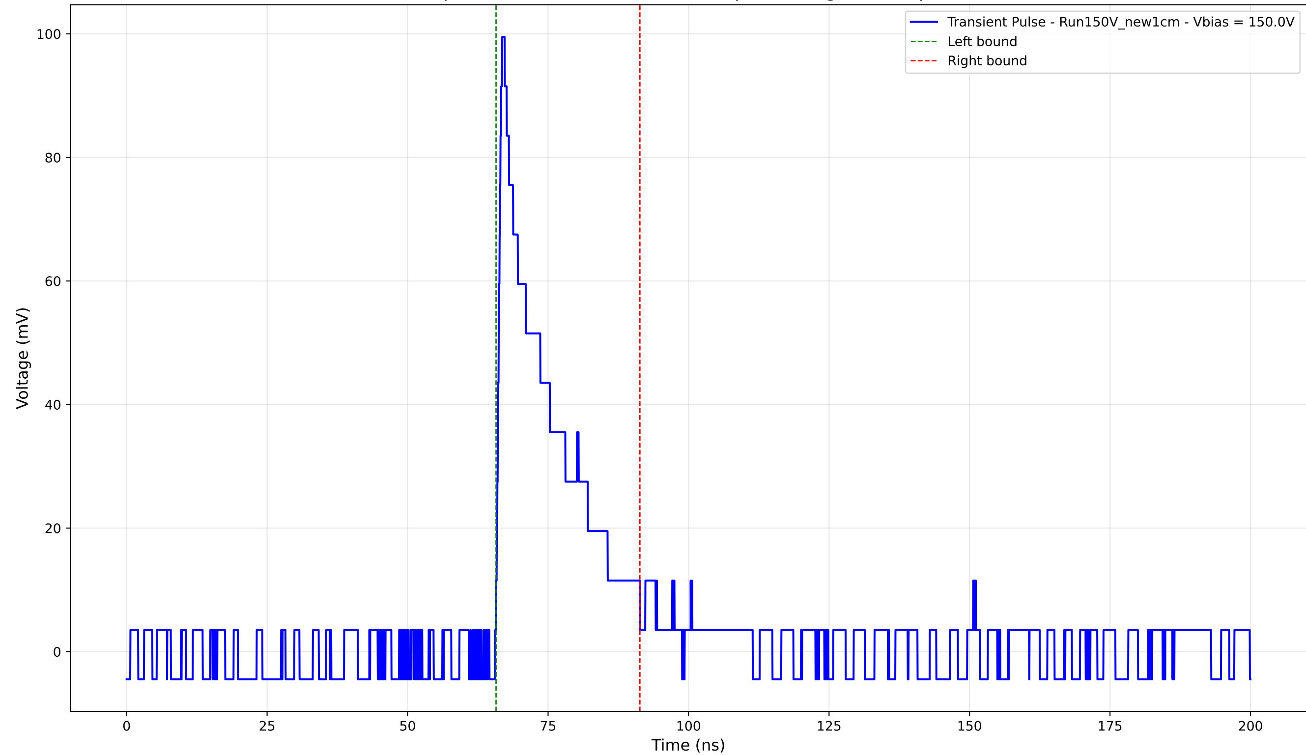
Transient Pulse - Sample: New1cm - Position: 4840.0 \mu\text{m} - Charge: 18.40 pC - Rise Time: 0.88 ns
