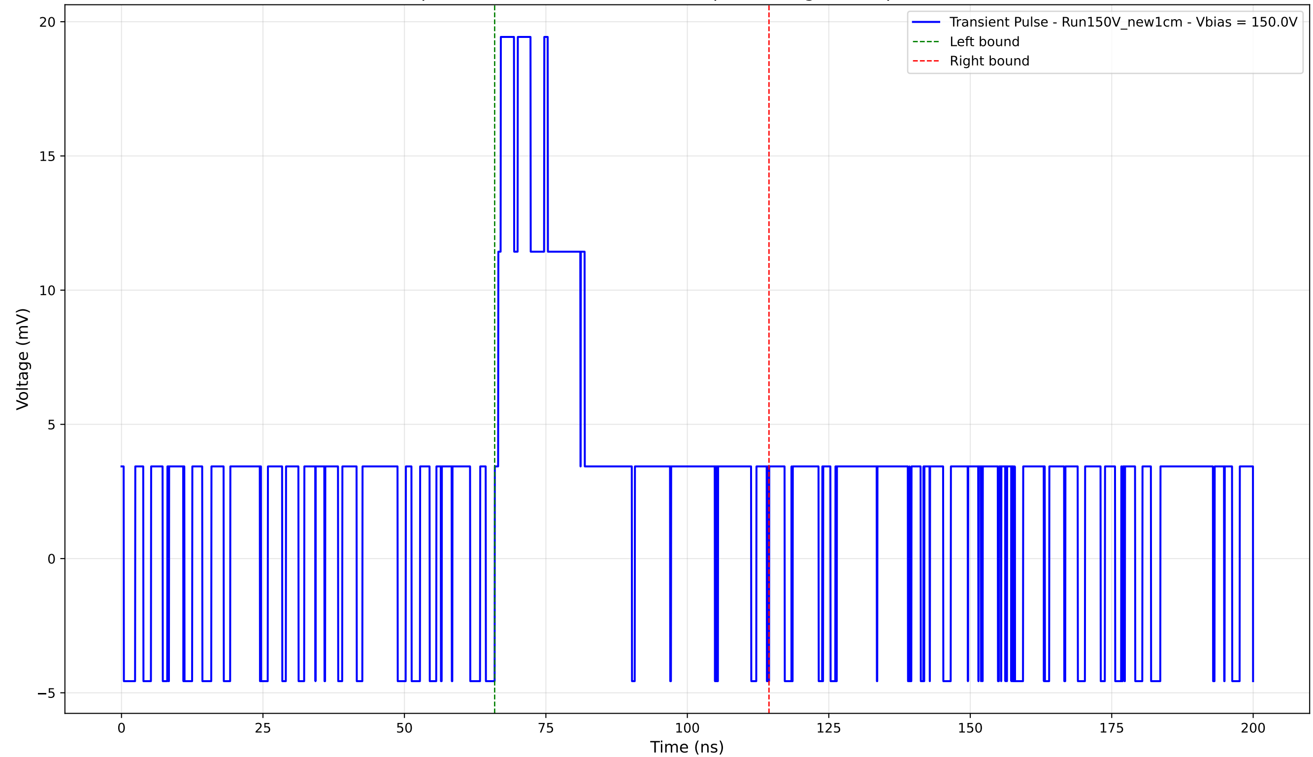
Transient Pulse - Sample: New1cm - Position: 1555.0 \mu\text{m} - Charge: 6.25 pC - Rise Time: 0.00 ns (N/A)
