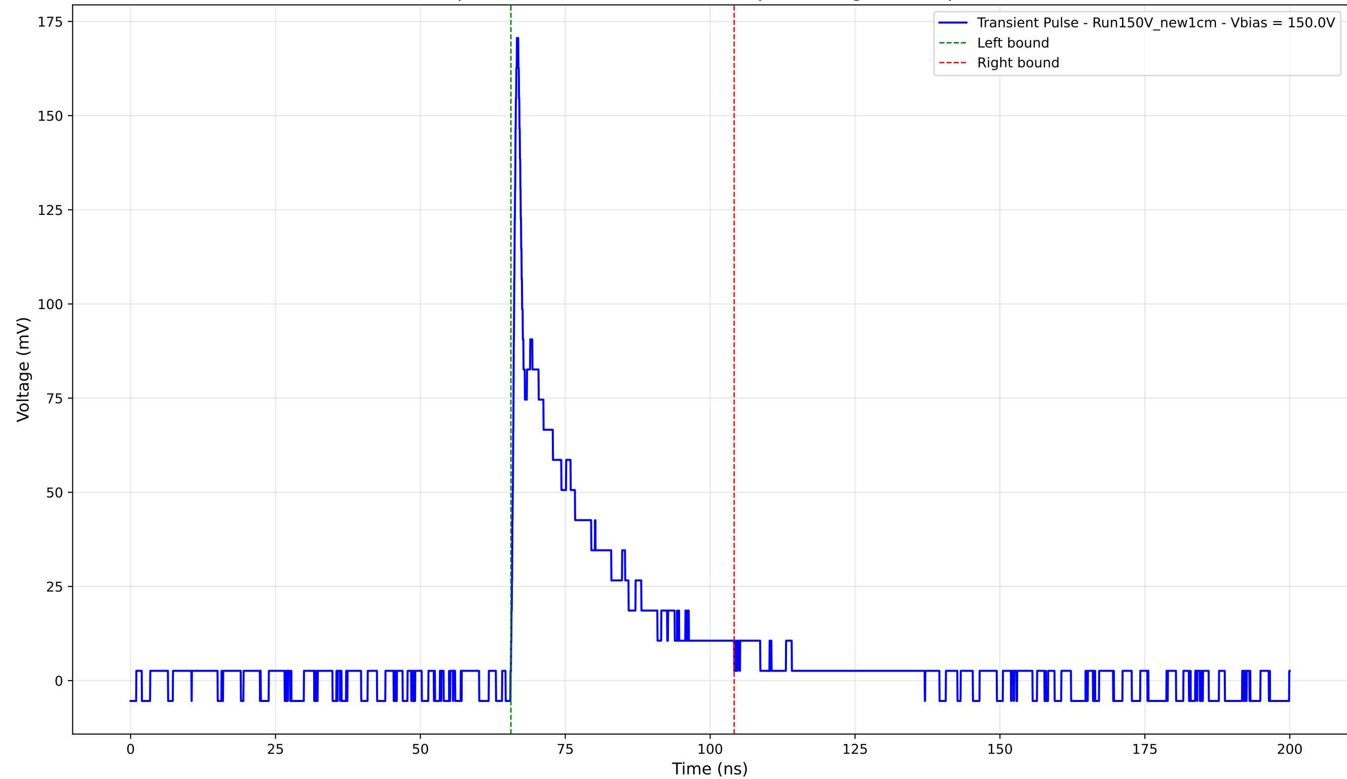
Transient Pulse - Sample: New1cm - Position: 2470.0 \mu\text{m} - Charge: 28.52 pC - Rise Time: 0.76 ns
