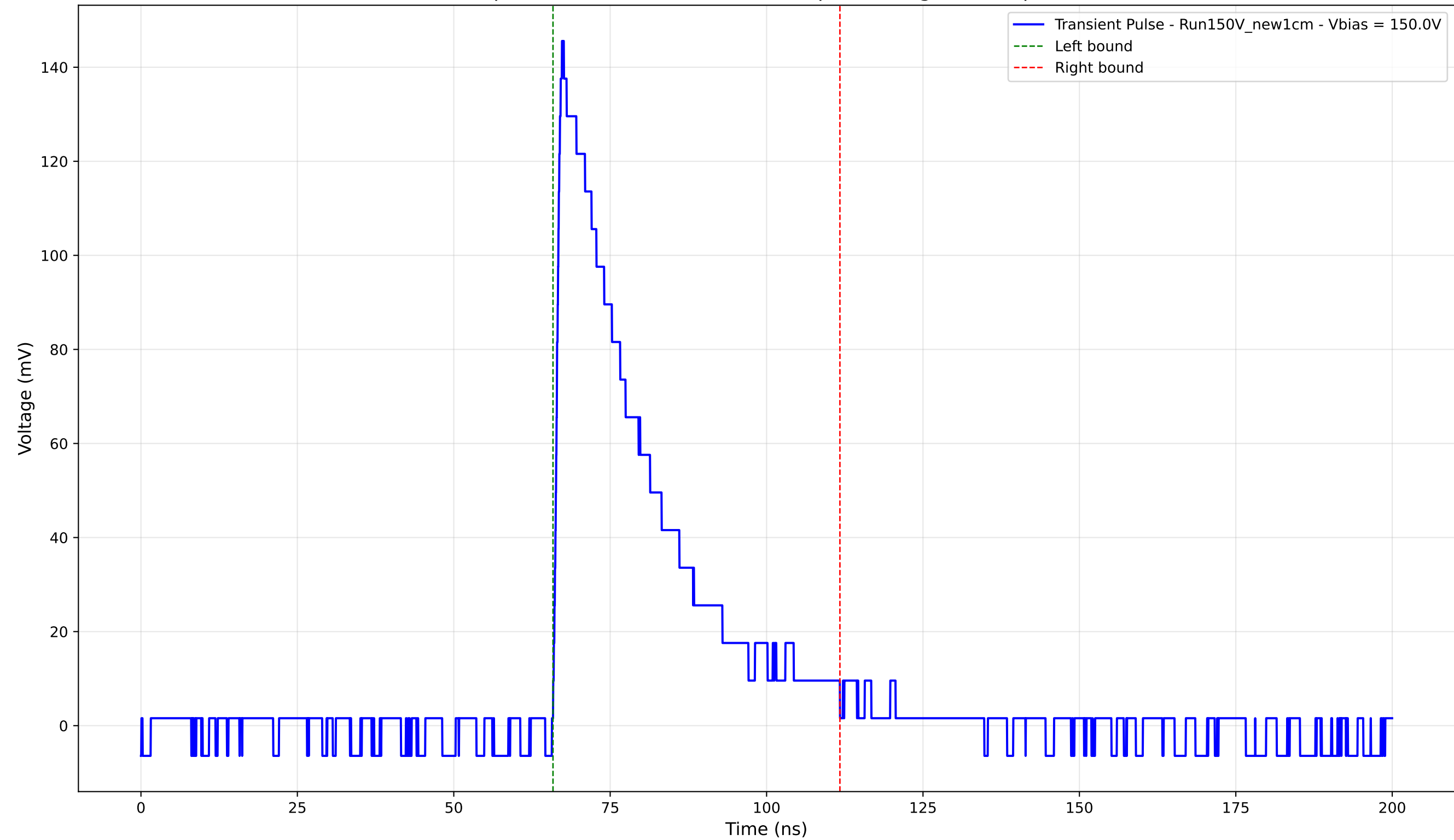
Transient Pulse - Sample: New1cm - Position: 3205.0 \mu\text{m} - Charge: 41.67 pC - Rise Time: 1.11 ns
