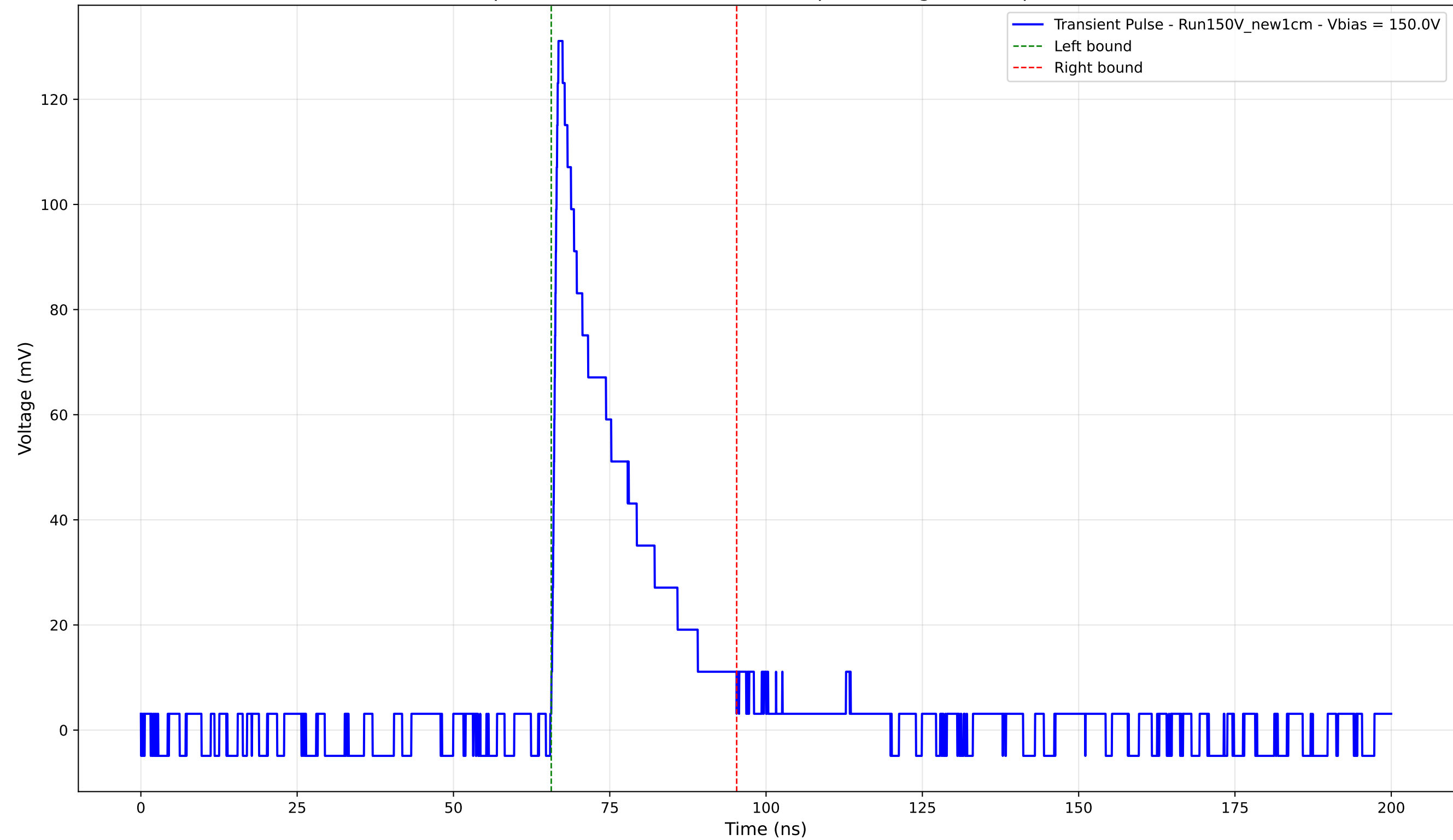
Transient Pulse - Sample: New1cm - Position: 4810.0 \mu\text{m} - Charge: 26.38 pC - Rise Time: 0.89 ns
