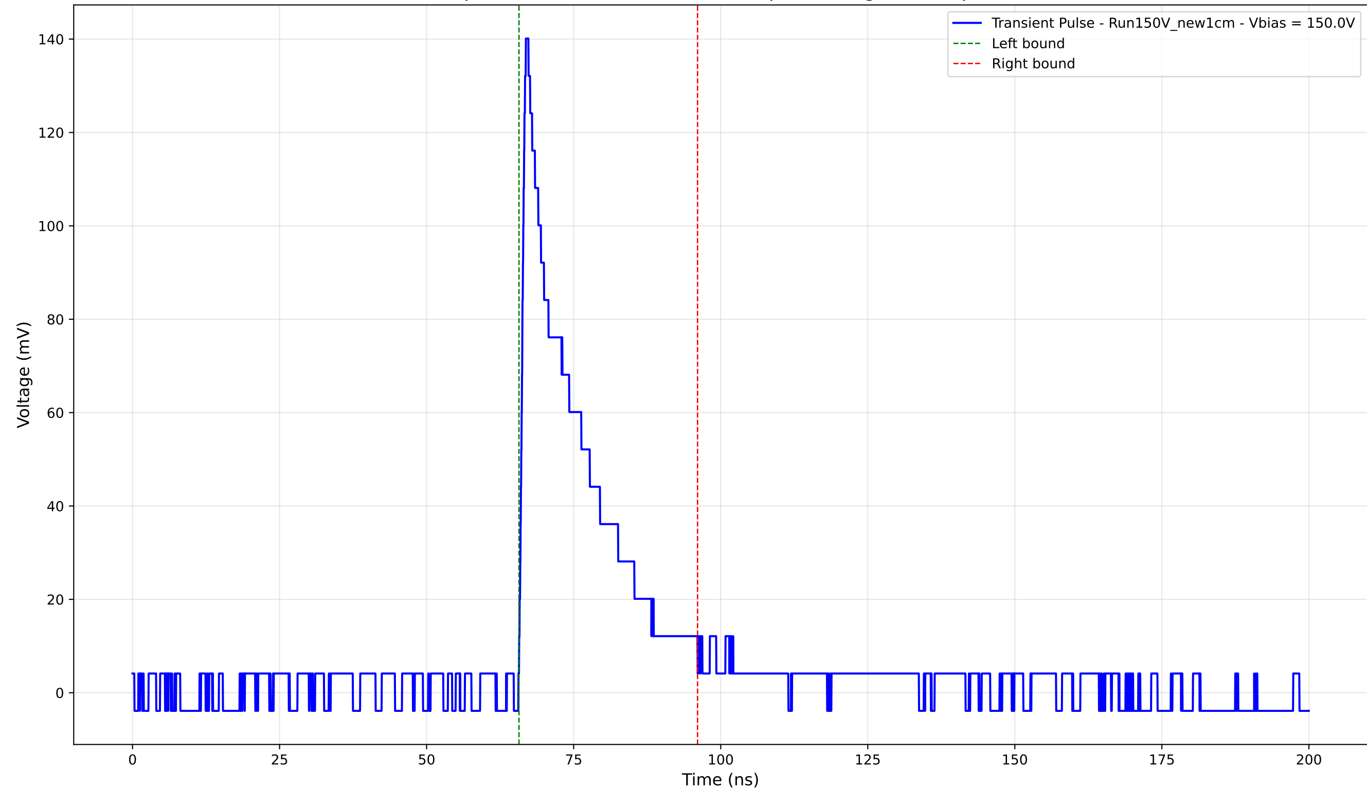
Transient Pulse - Sample: New1cm - Position: 4785.0 \mu\text{m} - Charge: 27.65 pC - Rise Time: 0.94 ns
