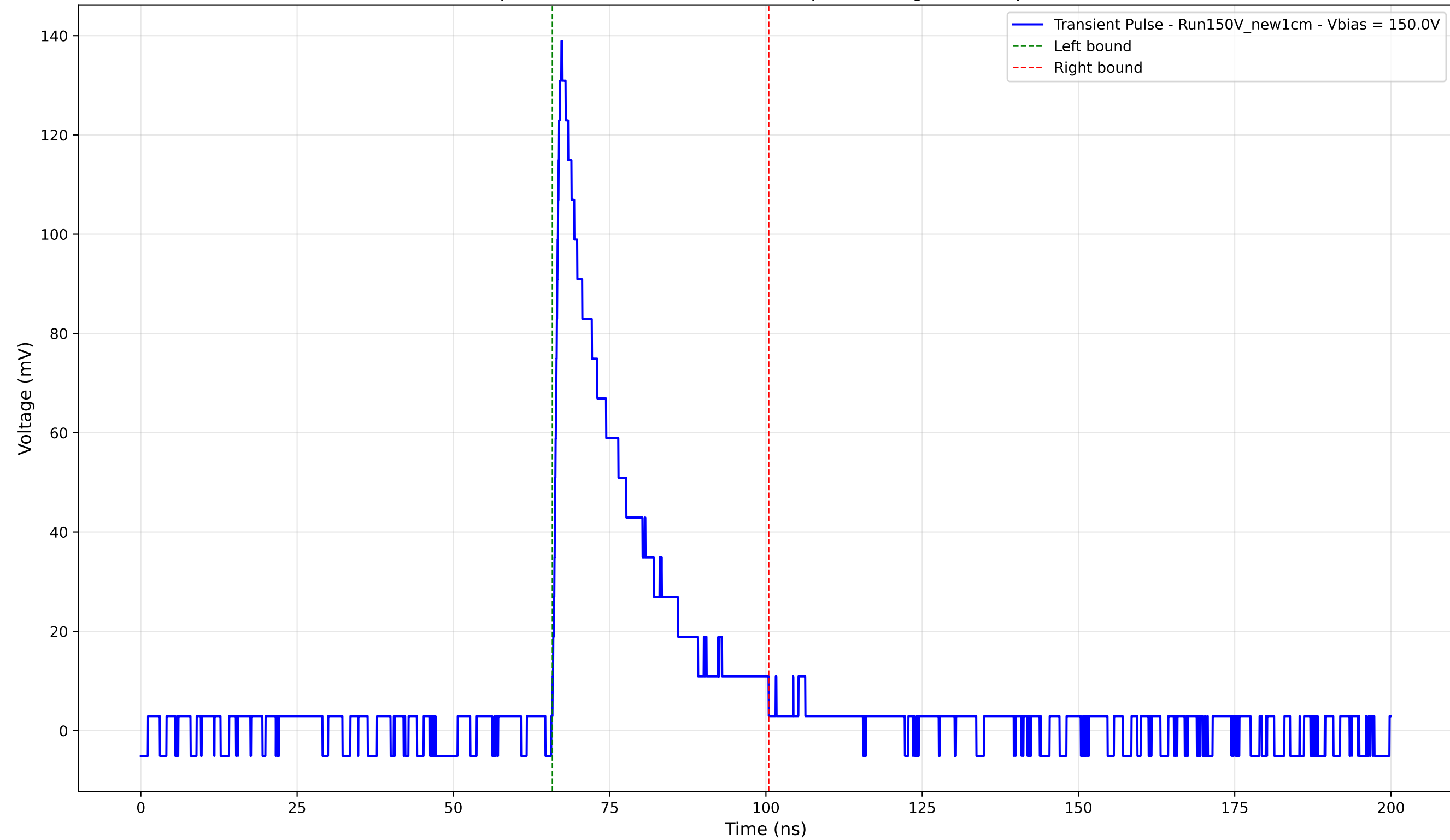
Transient Pulse - Sample: New1cm - Position: 275.0 \mu\text{m} - Charge: 28.37 pC - Rise Time: 1.09 ns
