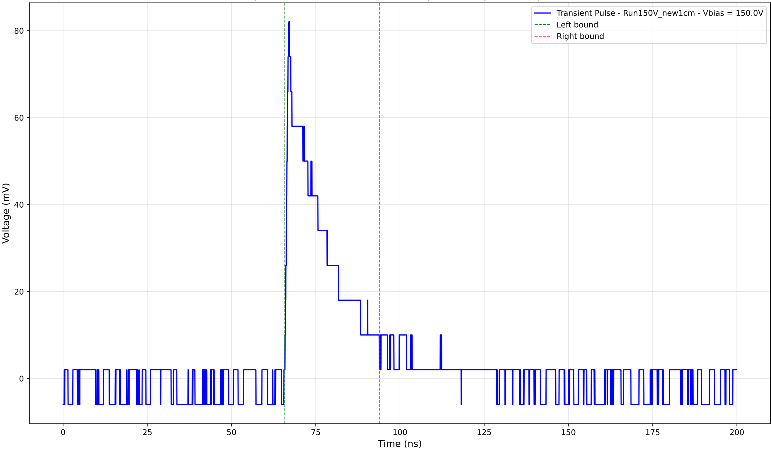
Transient Pulse - Sample: New1cm - Position: 2105.0 \mu\text{m} - Charge: 17.31 pC - Rise Time: 0.90 ns
