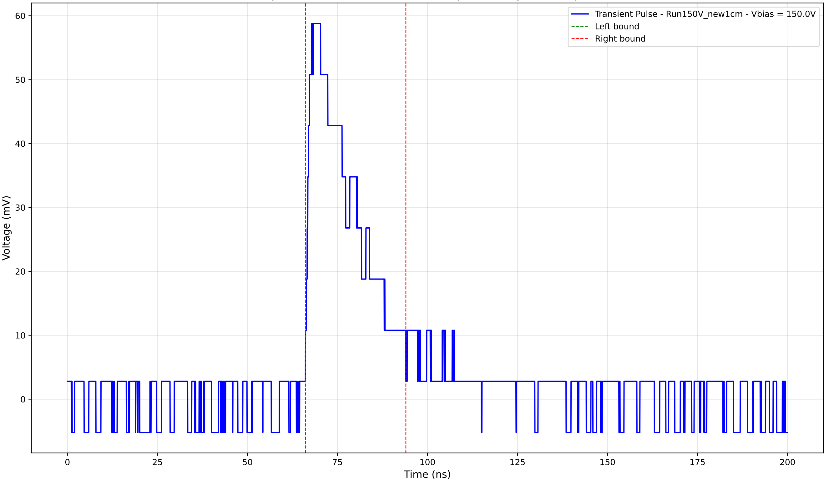
Transient Pulse - Sample: New1cm - Position: 1595.0 \mu\text{m} - Charge: 16.75 pC - Rise Time: 1.73 ns
