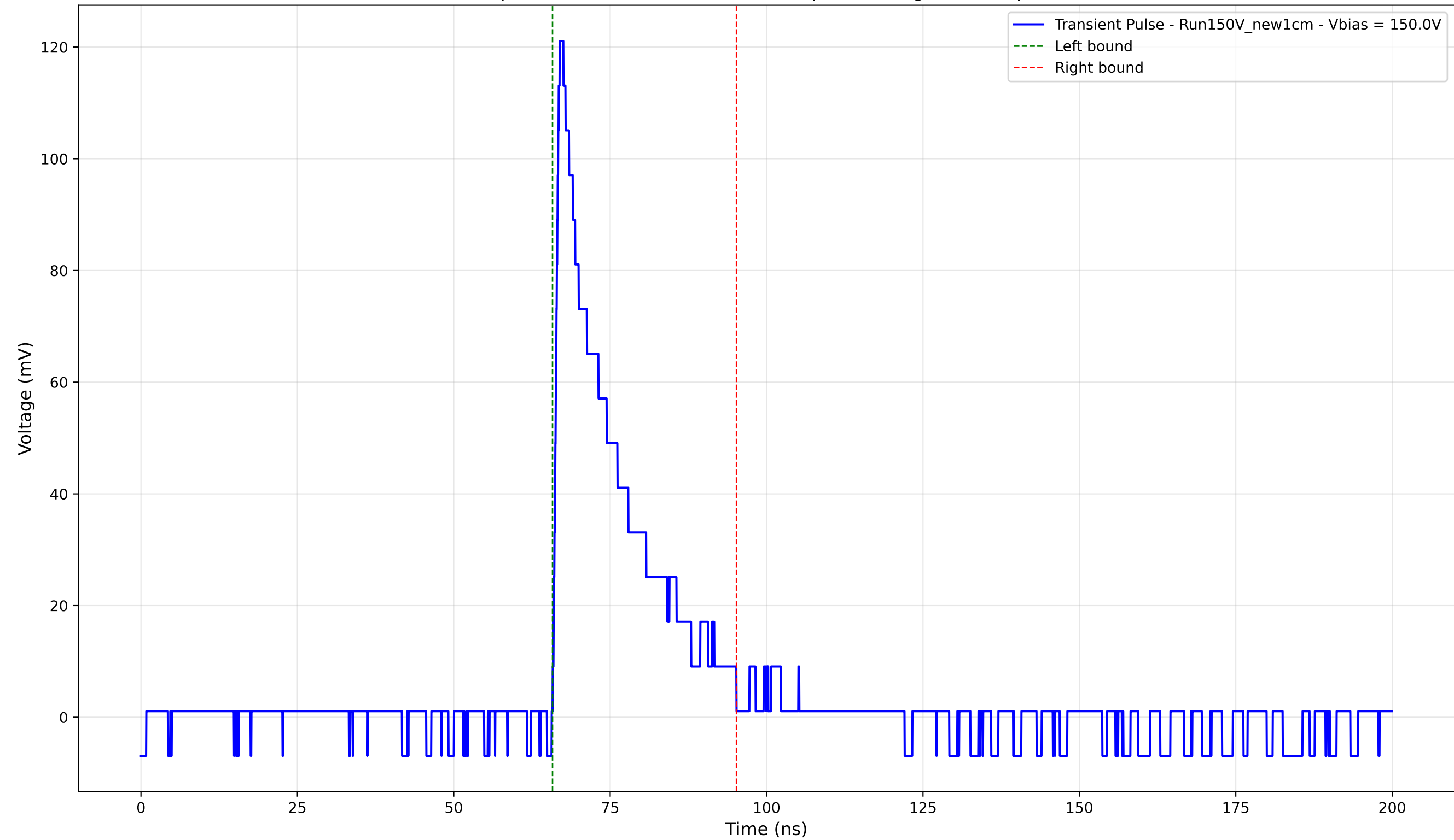
Transient Pulse - Sample: New1cm - Position: 180.0 \mu\text{m} - Charge: 23.14 pC - Rise Time: 0.83 ns
