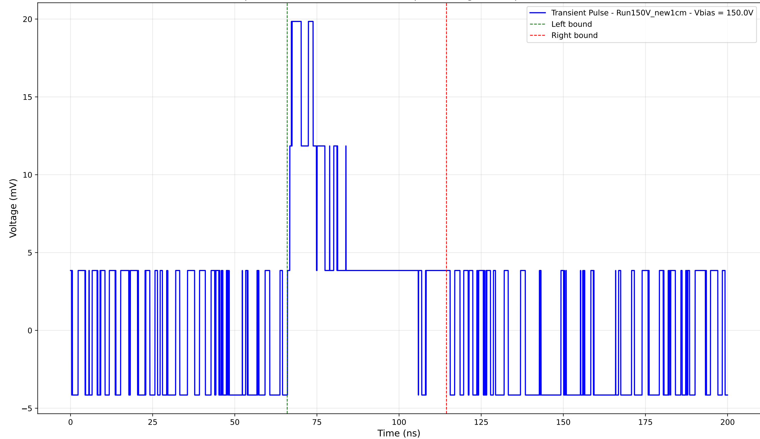
Transient Pulse - Sample: New1cm - Position: 4060.0 \mu\text{m} - Charge: 6.08 pC - Rise Time: 0.00 ns (N/A)
