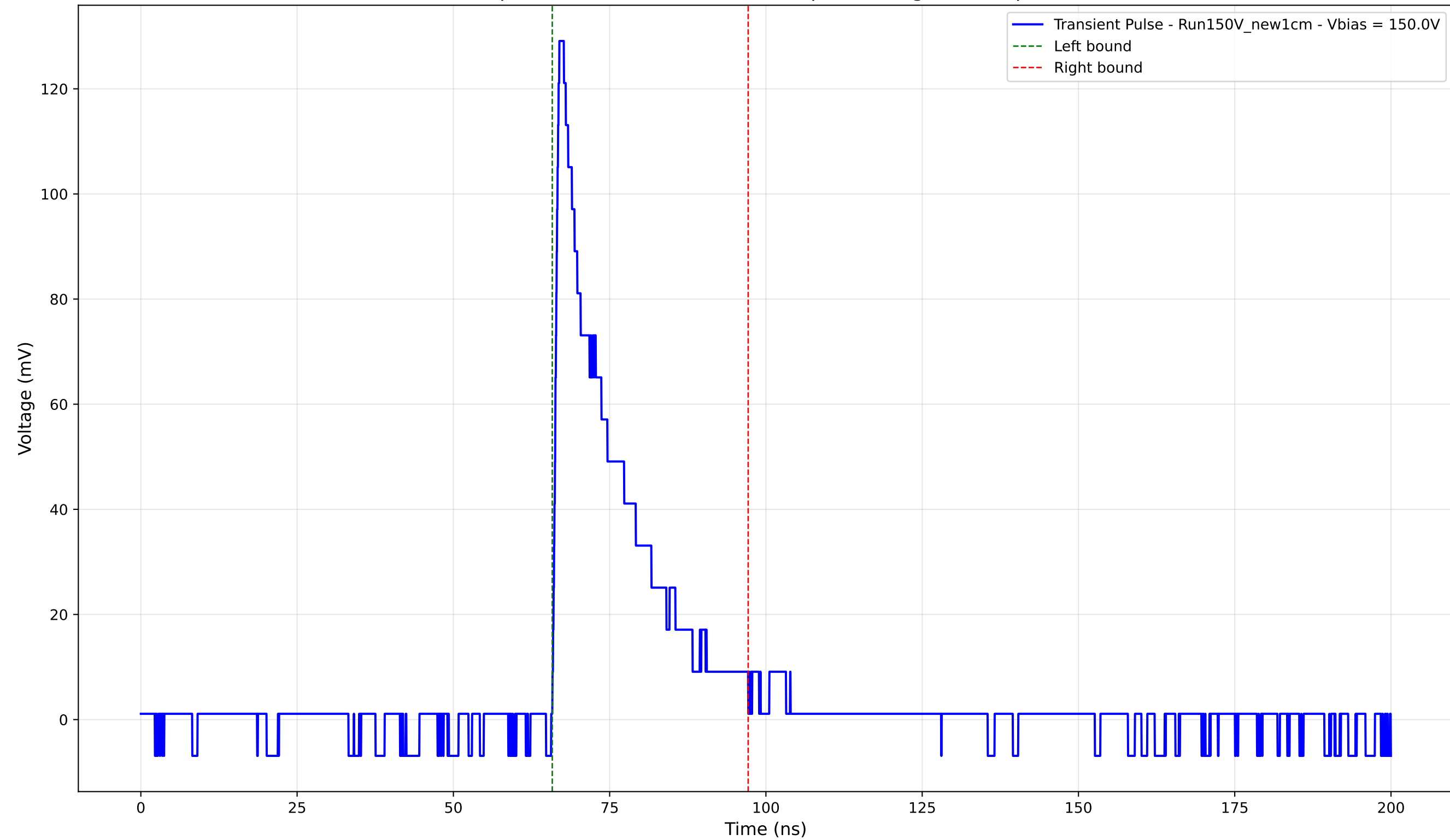
Transient Pulse - Sample: New1cm - Position: 195.0 \mu\text{m} - Charge: 24.79 pC - Rise Time: 0.89 ns
