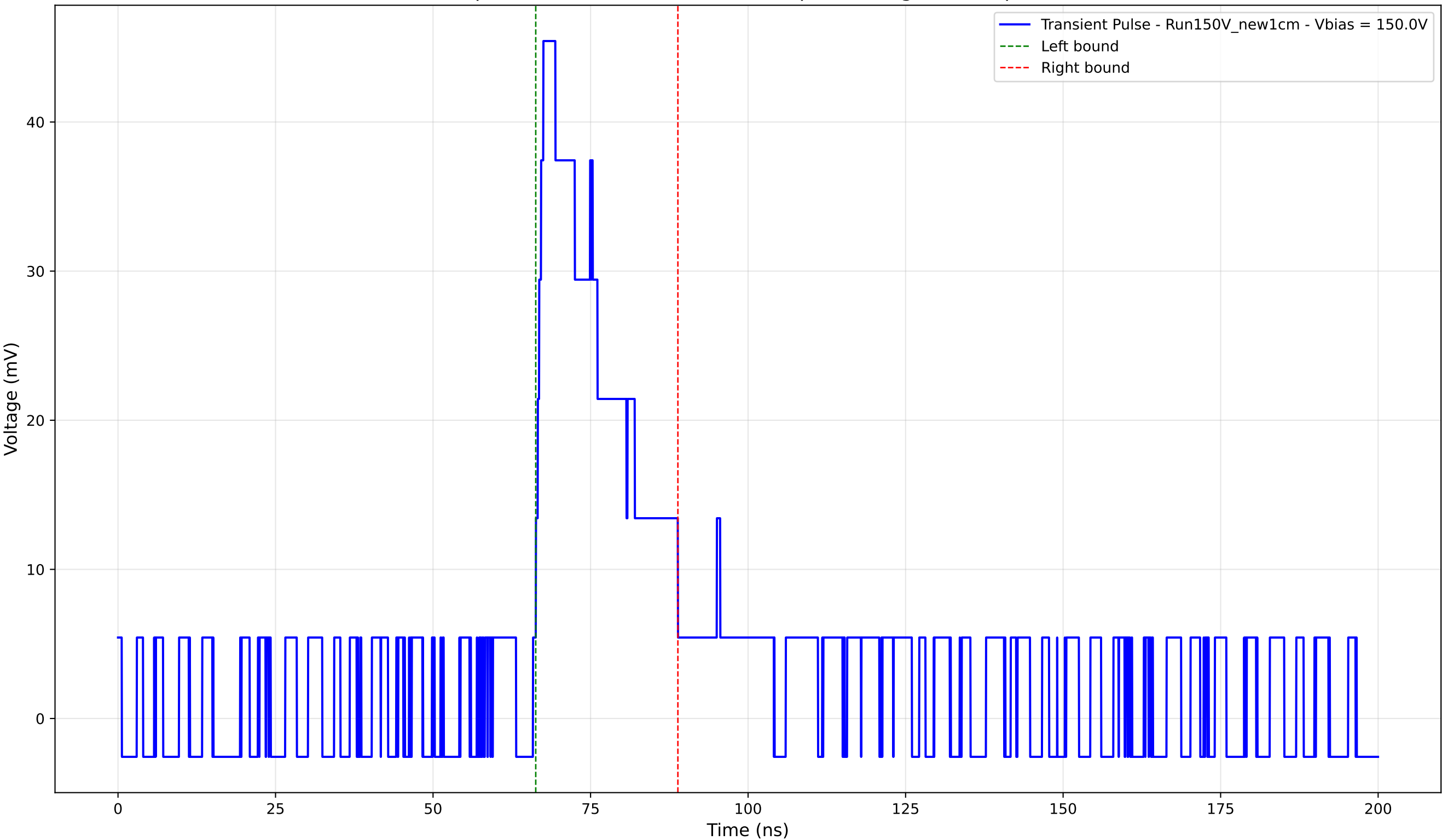
Transient Pulse - Sample: New1cm - Position: 4100.0 \mu\text{m} - Charge: 11.20 pC - Rise Time: 1.65 ns
