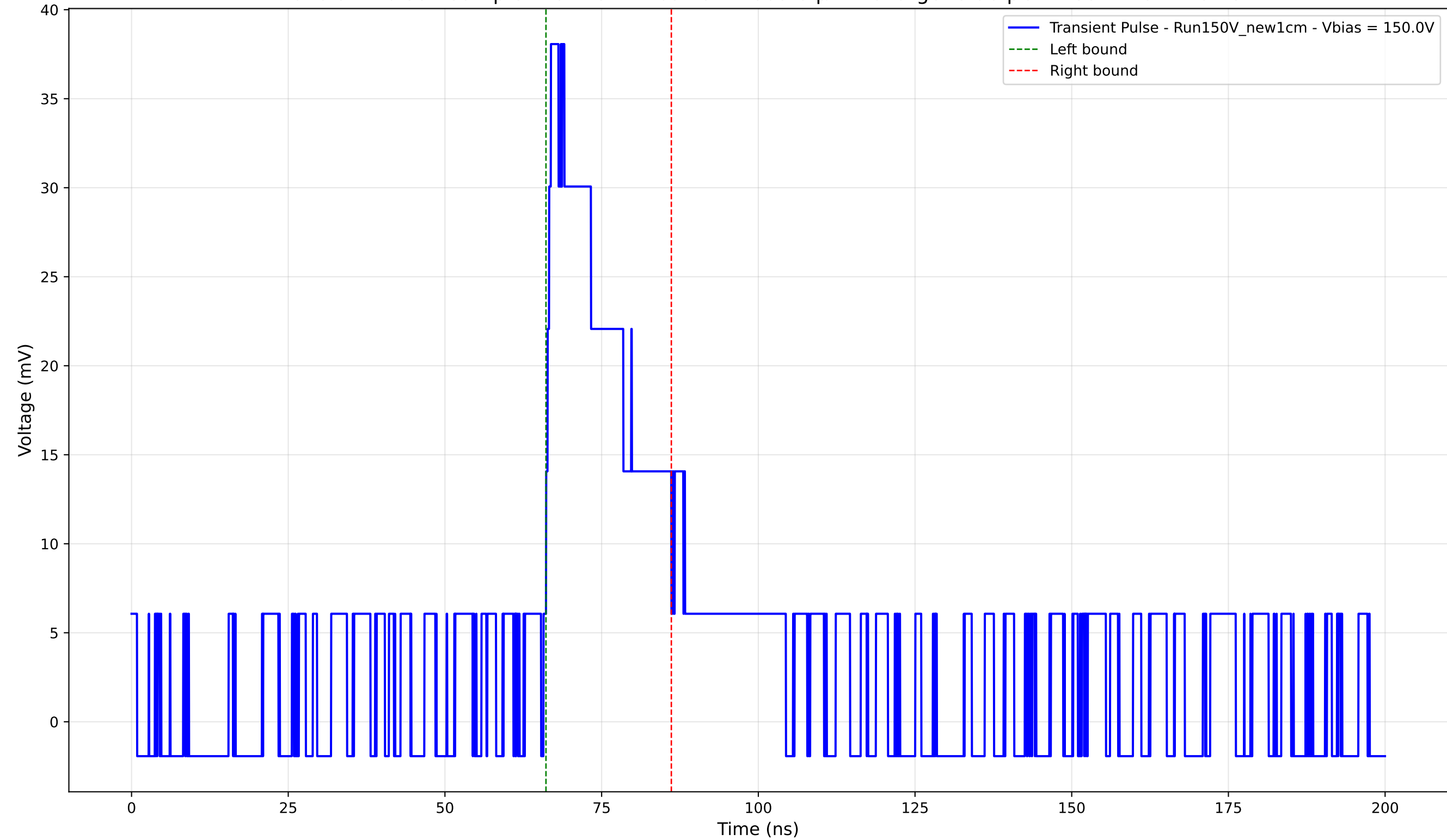
Transient Pulse - Sample: New1cm - Position: 2005.0 \mu\text{m} - Charge: 8.90 pC - Rise Time: 1.19 ns
