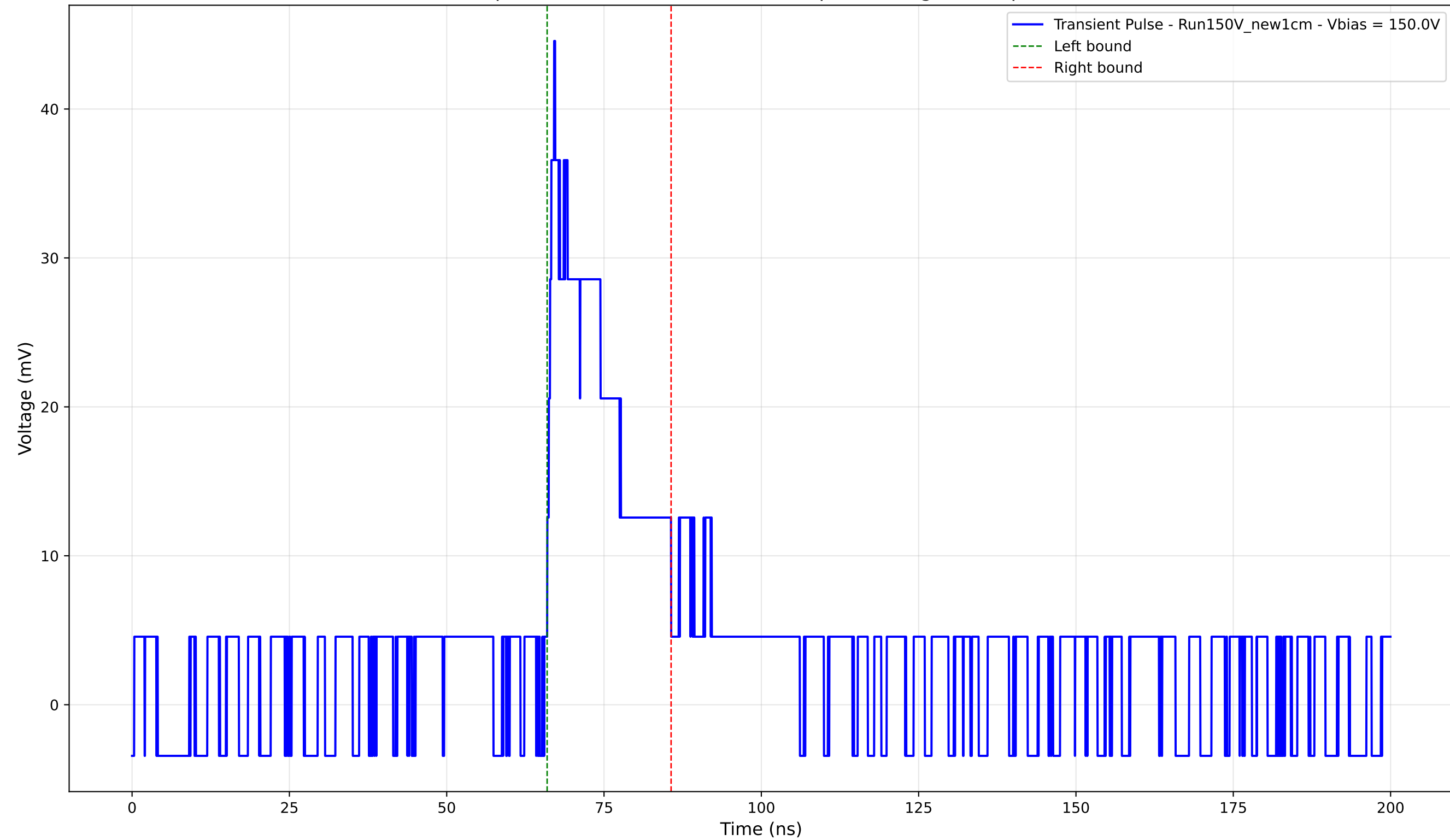
Transient Pulse - Sample: New1cm - Position: 3035.0 \mu\text{m} - Charge: 8.33 pC - Rise Time: 1.56 ns
