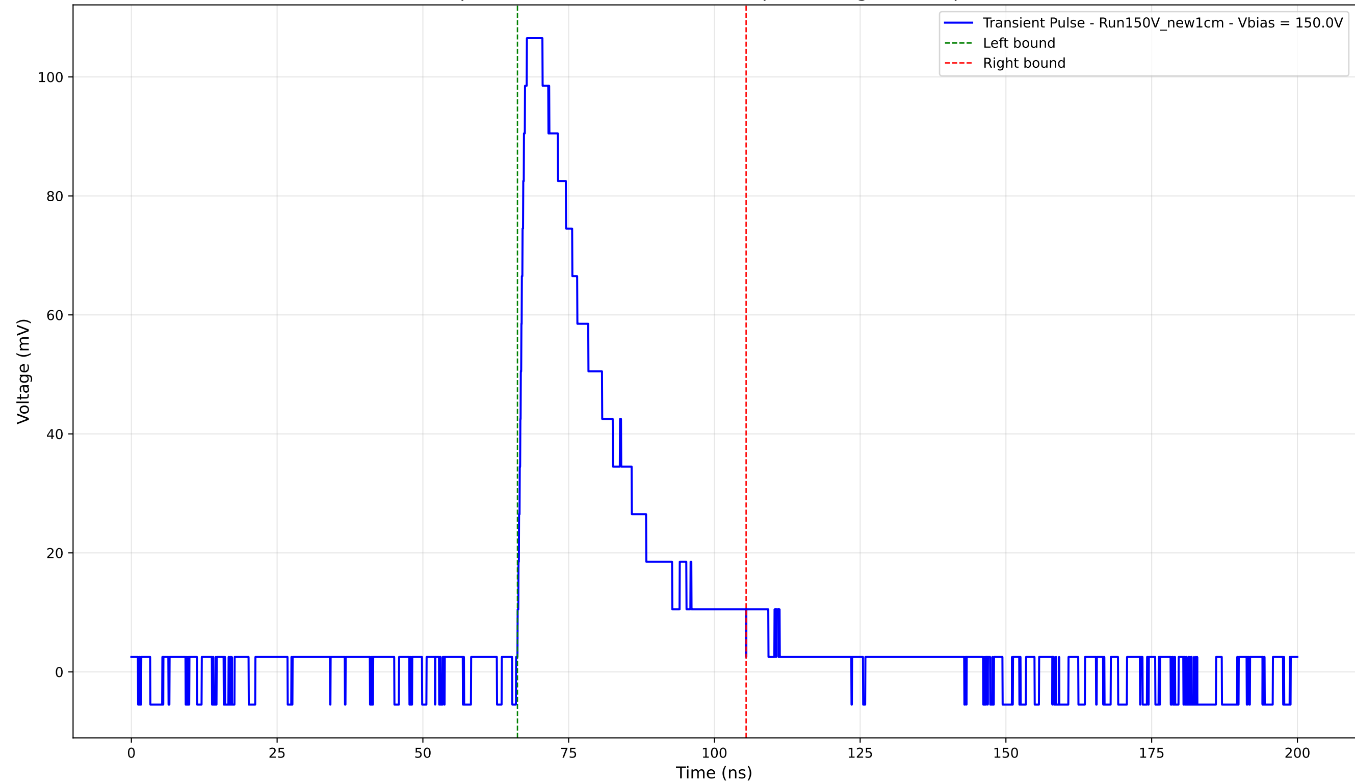
Transient Pulse - Sample: New1cm - Position: 1375.0 \mu\text{m} - Charge: 31.97 pC - Rise Time: 1.14 ns
