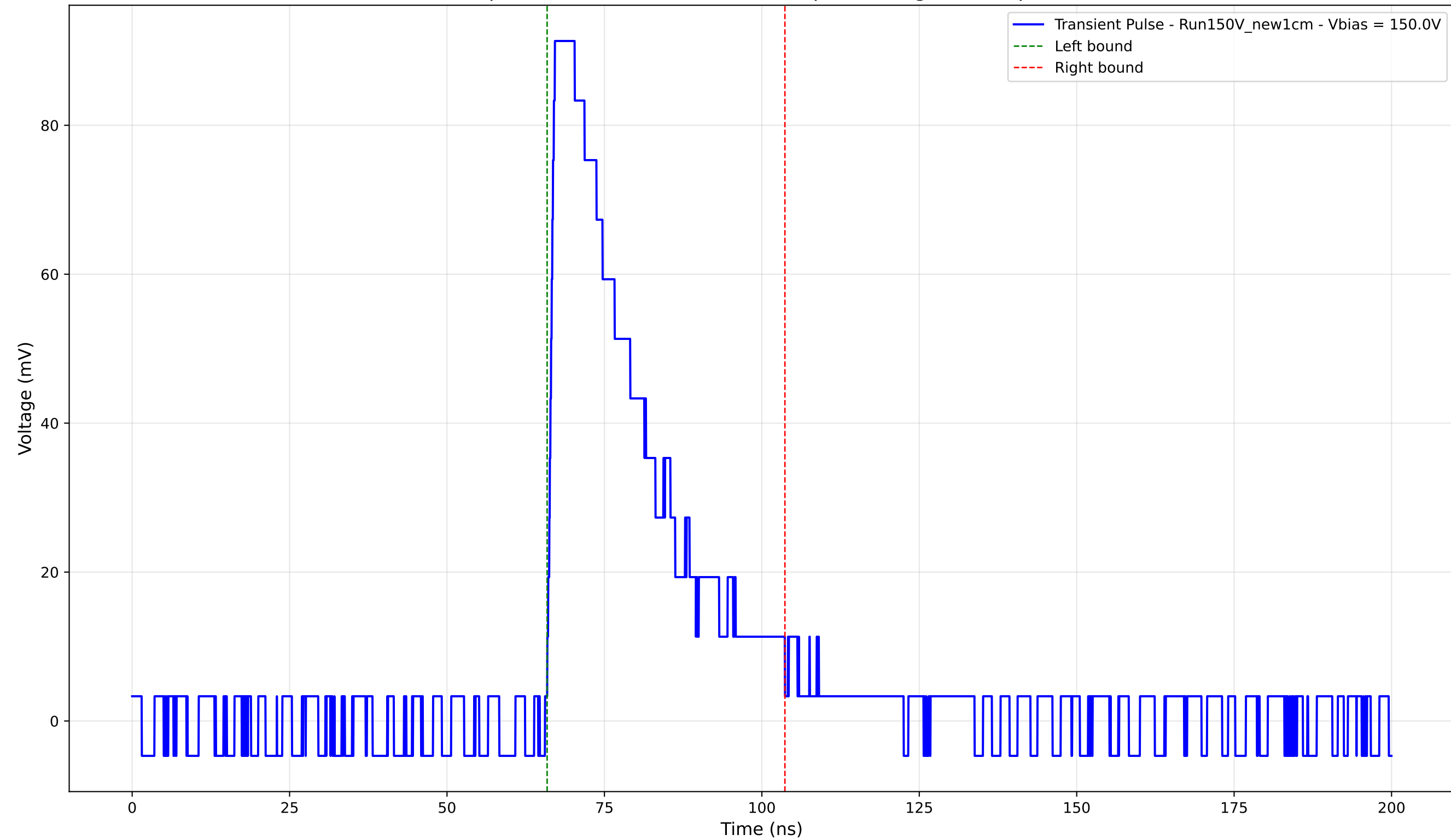
Transient Pulse - Sample: New1cm - Position: 1820.0 \mu\text{m} - Charge: 28.88 pC - Rise Time: 1.05 ns
