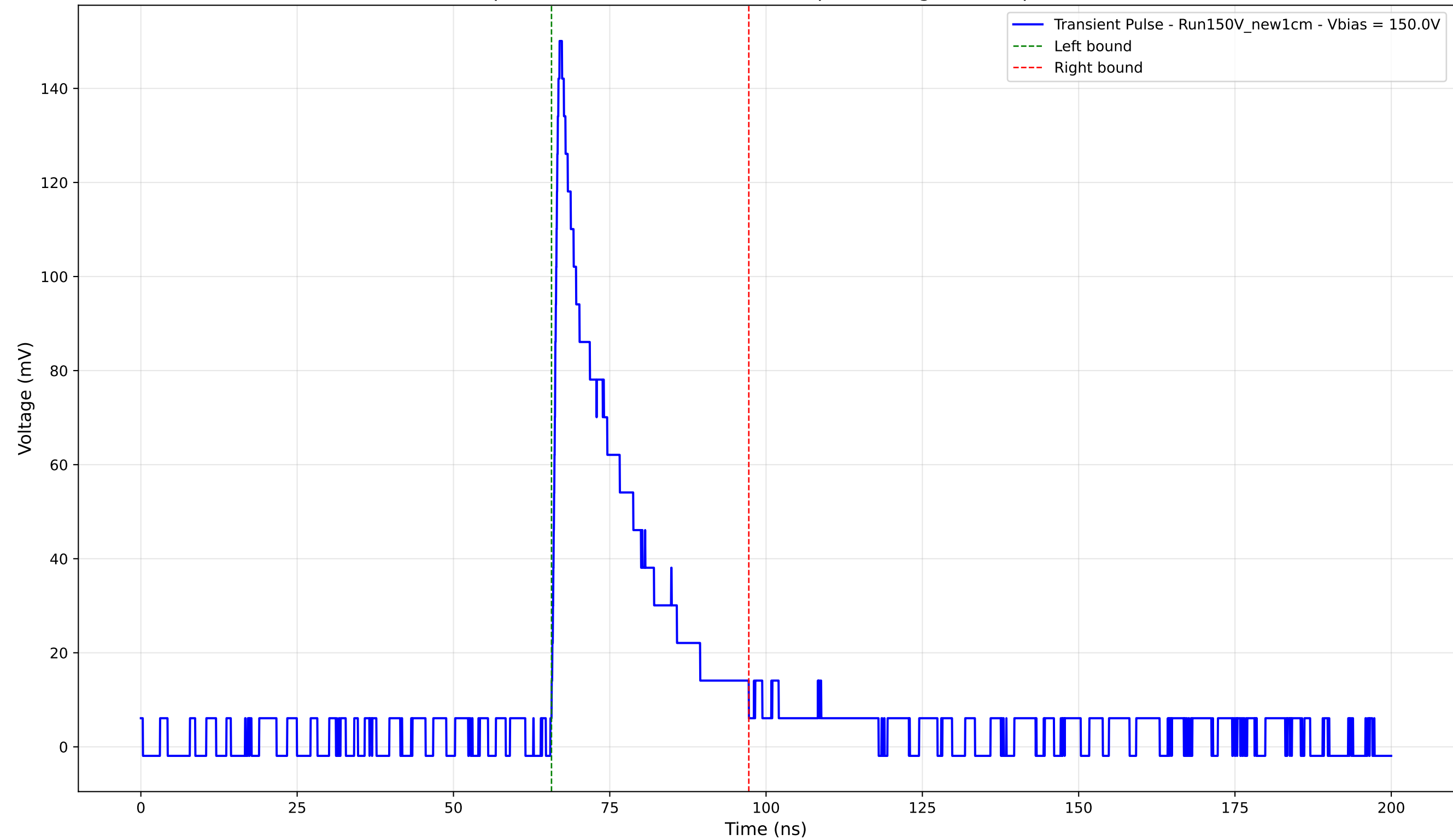
Transient Pulse - Sample: New1cm - Position: 4790.0 \mu\text{m} - Charge: 30.45 pC - Rise Time: 1.00 ns
