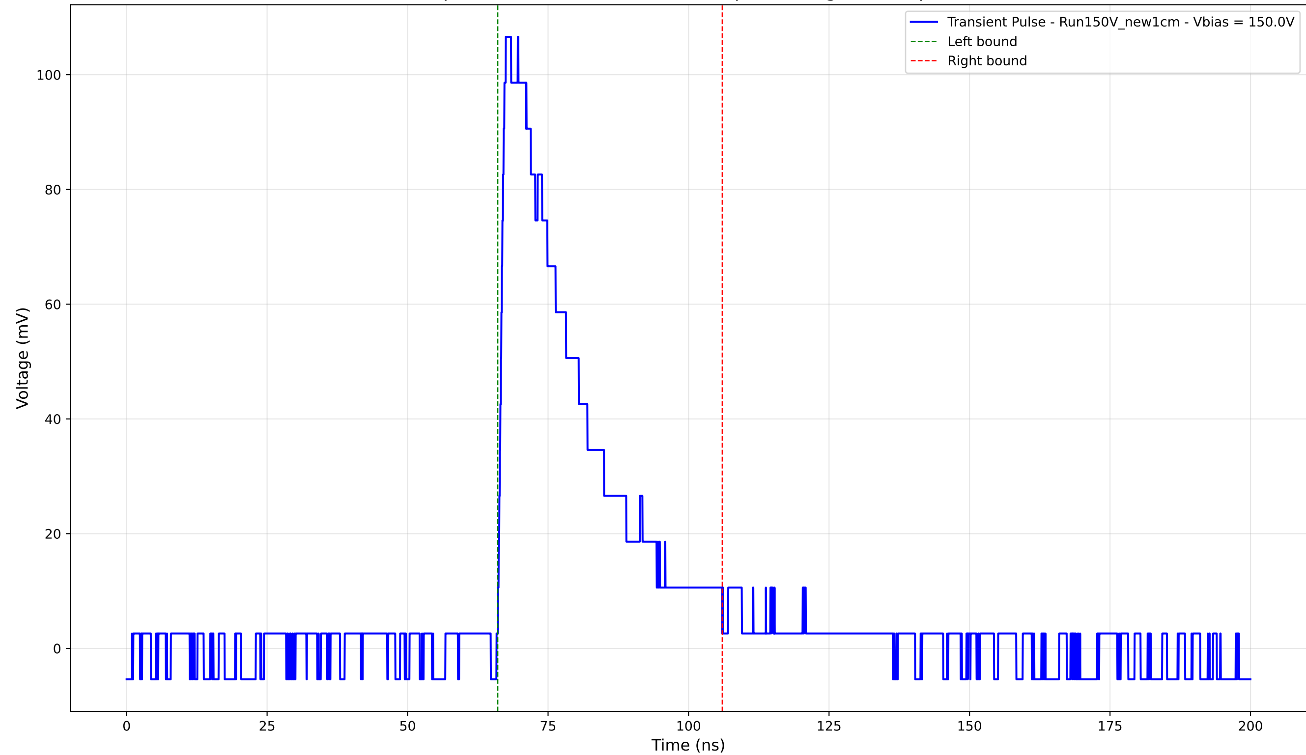
Transient Pulse - Sample: New1cm - Position: 1725.0 \mu\text{m} - Charge: 31.66 pC - Rise Time: 1.04 ns
