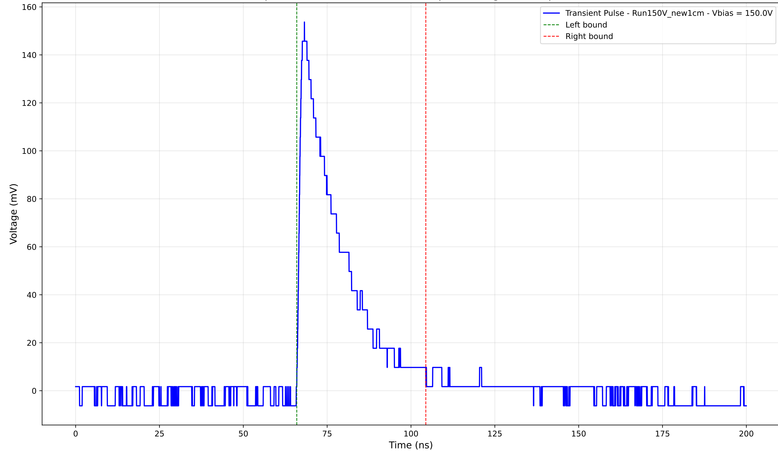
Transient Pulse - Sample: New1cm - Position: 4250.0 \mu\text{m} - Charge: 38.13 pC - Rise Time: 1.51 ns
