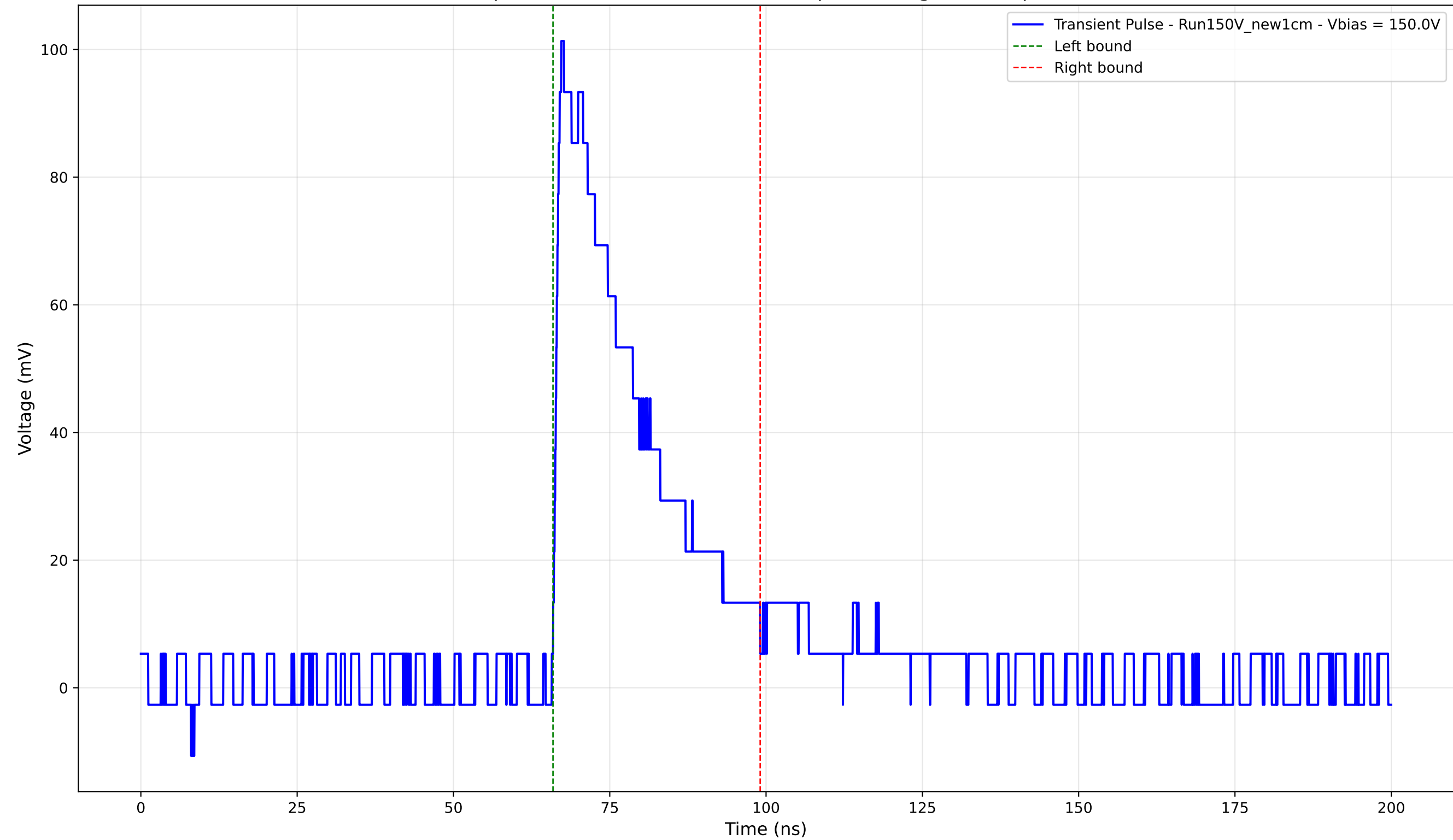
Transient Pulse - Sample: New1cm - Position: 1930.0 \mu\text{m} - Charge: 28.37 pC - Rise Time: 1.05 ns
