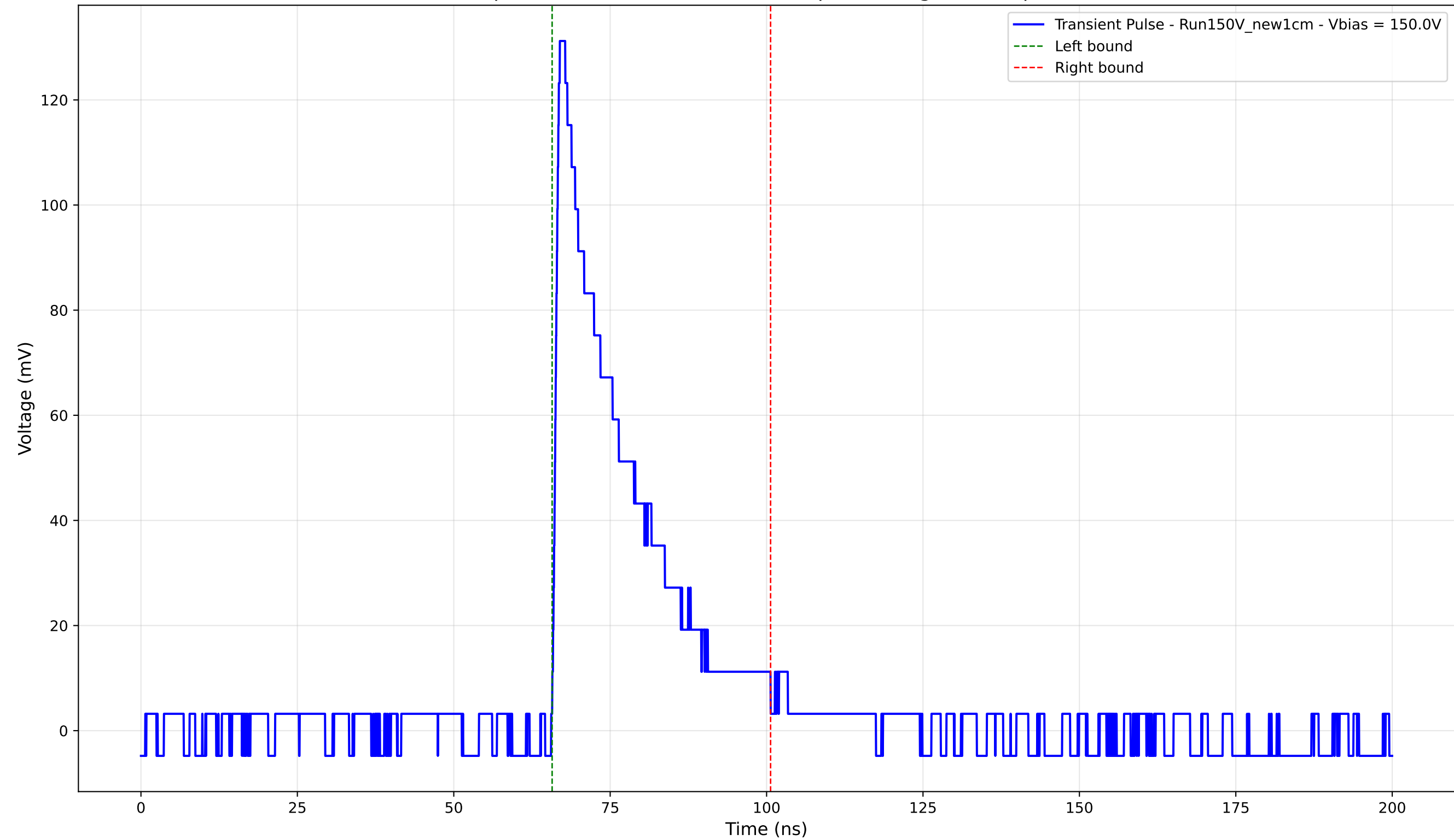
Transient Pulse - Sample: New1cm - Position: 4680.0 \mu\text{m} - Charge: 29.91 pC - Rise Time: 0.94 ns
