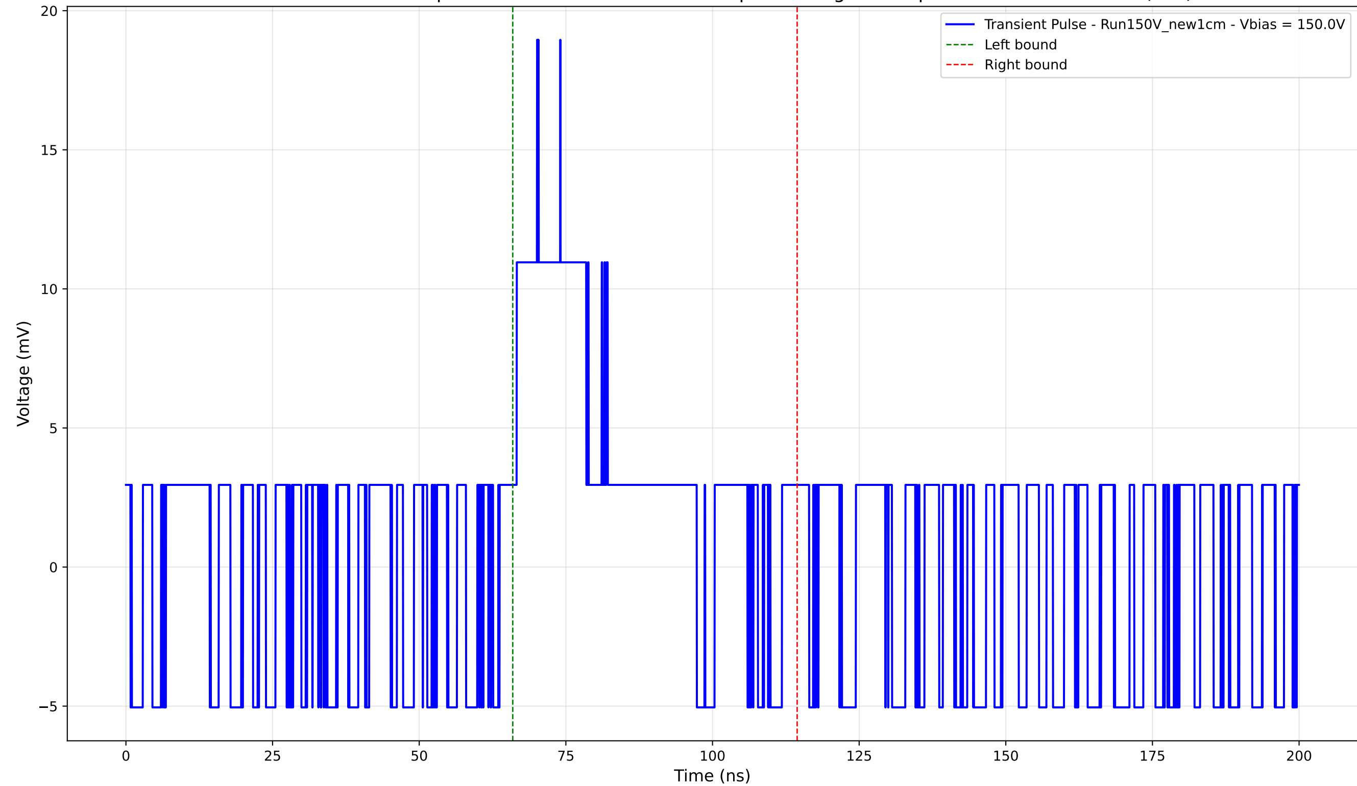
Transient Pulse - Sample: New1cm - Position: 1040.0 \mu\text{m} - Charge: 3.83 pC - Rise Time: 0.00 ns (N/A)
