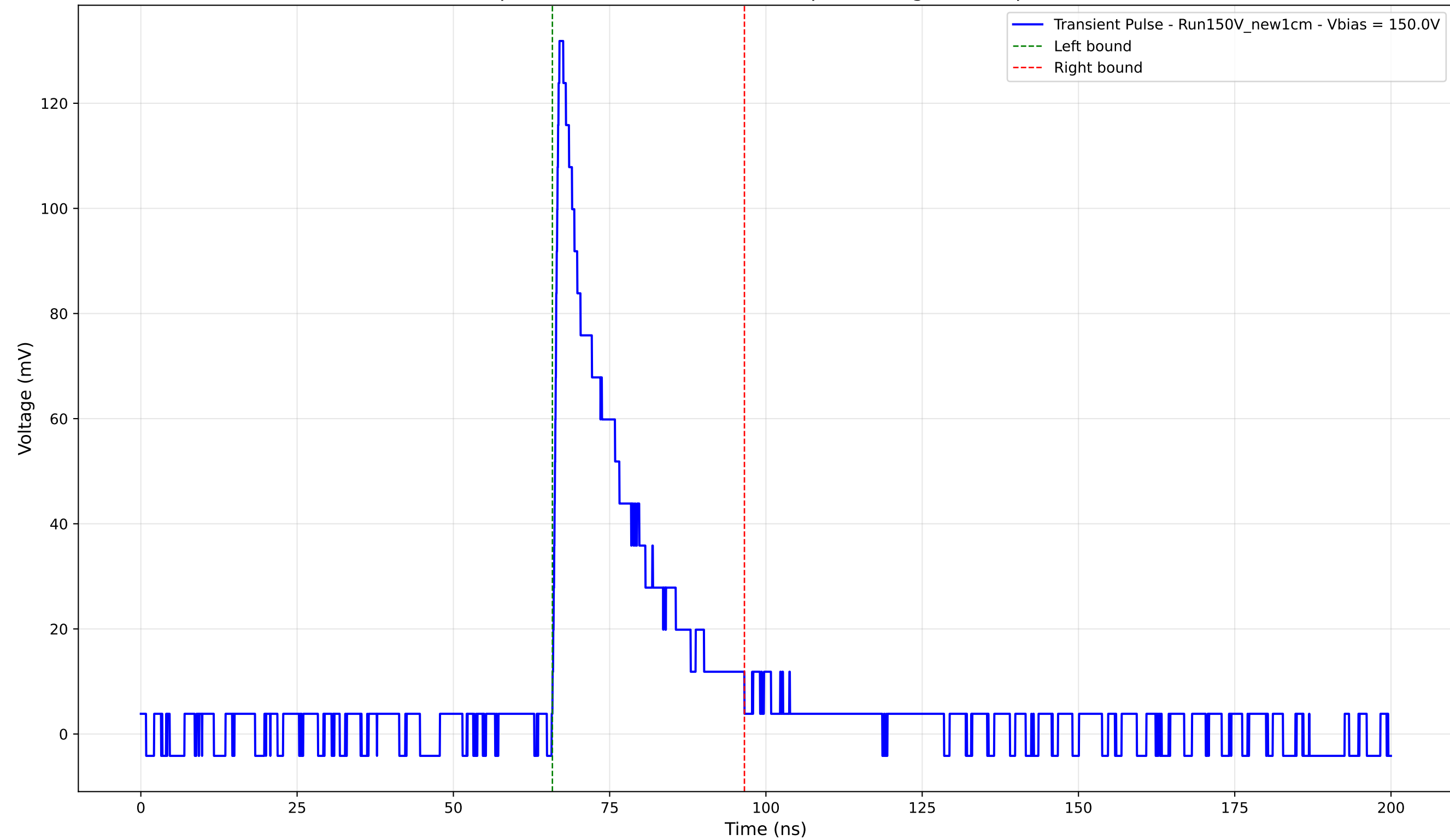
Transient Pulse - Sample: New1cm - Position: 200.0 \mu\text{m} - Charge: 26.38 pC - Rise Time: 0.88 ns
