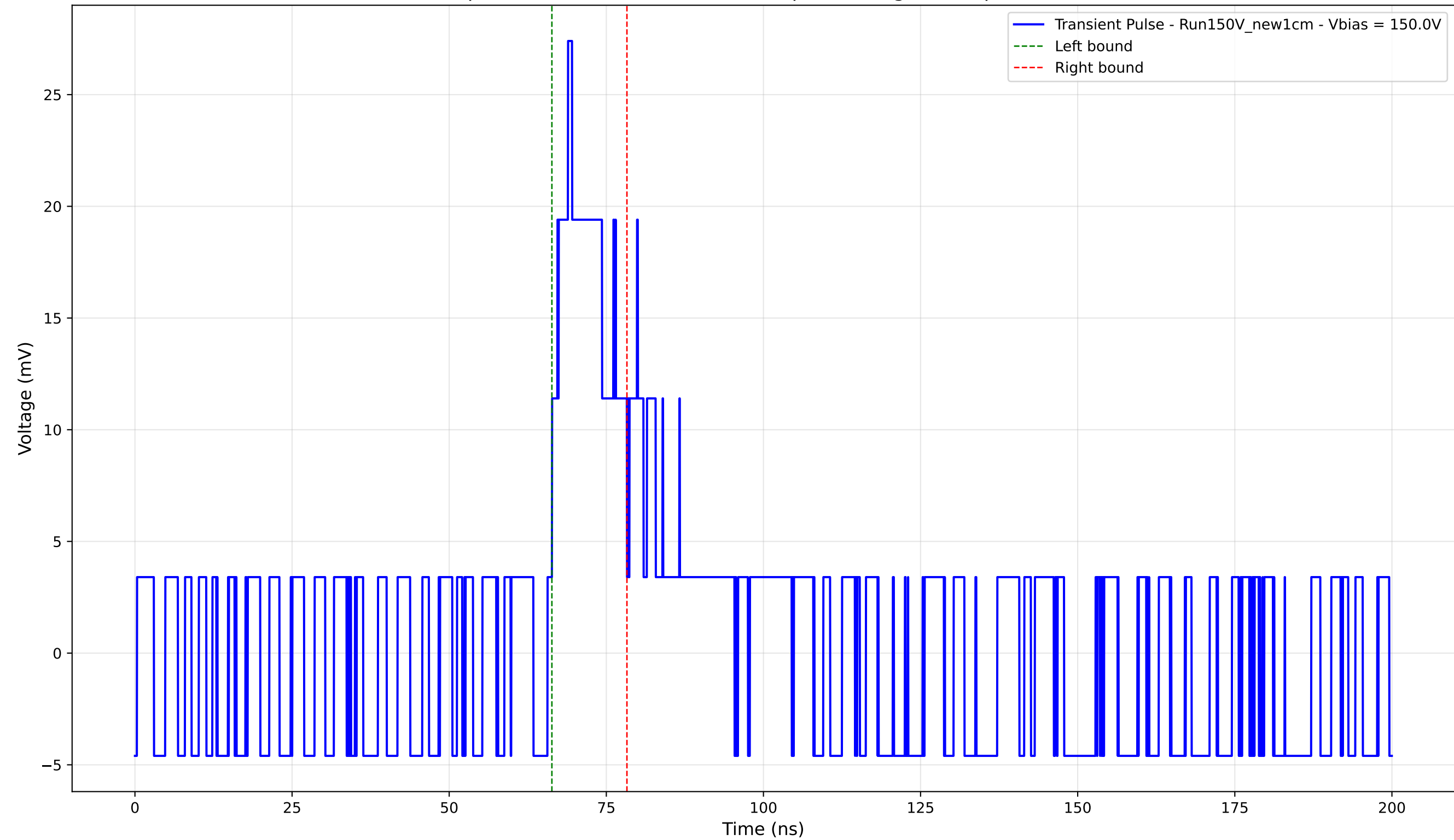
Transient Pulse - Sample: New1cm - Position: 3550.0 \mu\text{m} - Charge: 3.98 pC - Rise Time: 0.00 ns (N/A)
