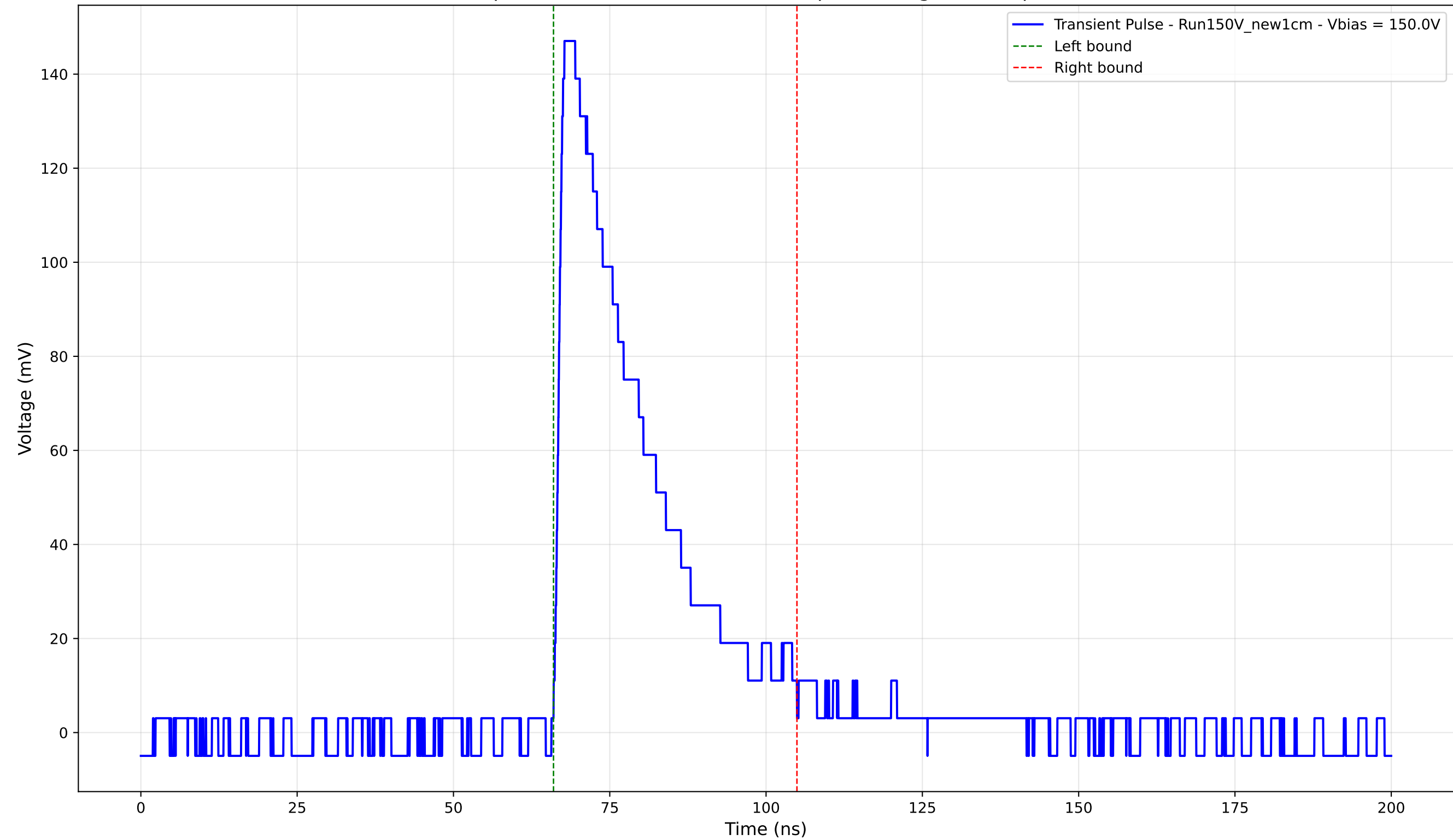
Transient Pulse - Sample: New1cm - Position: 3775.0 \mu\text{m} - Charge: 43.03 pC - Rise Time: 1.33 ns
