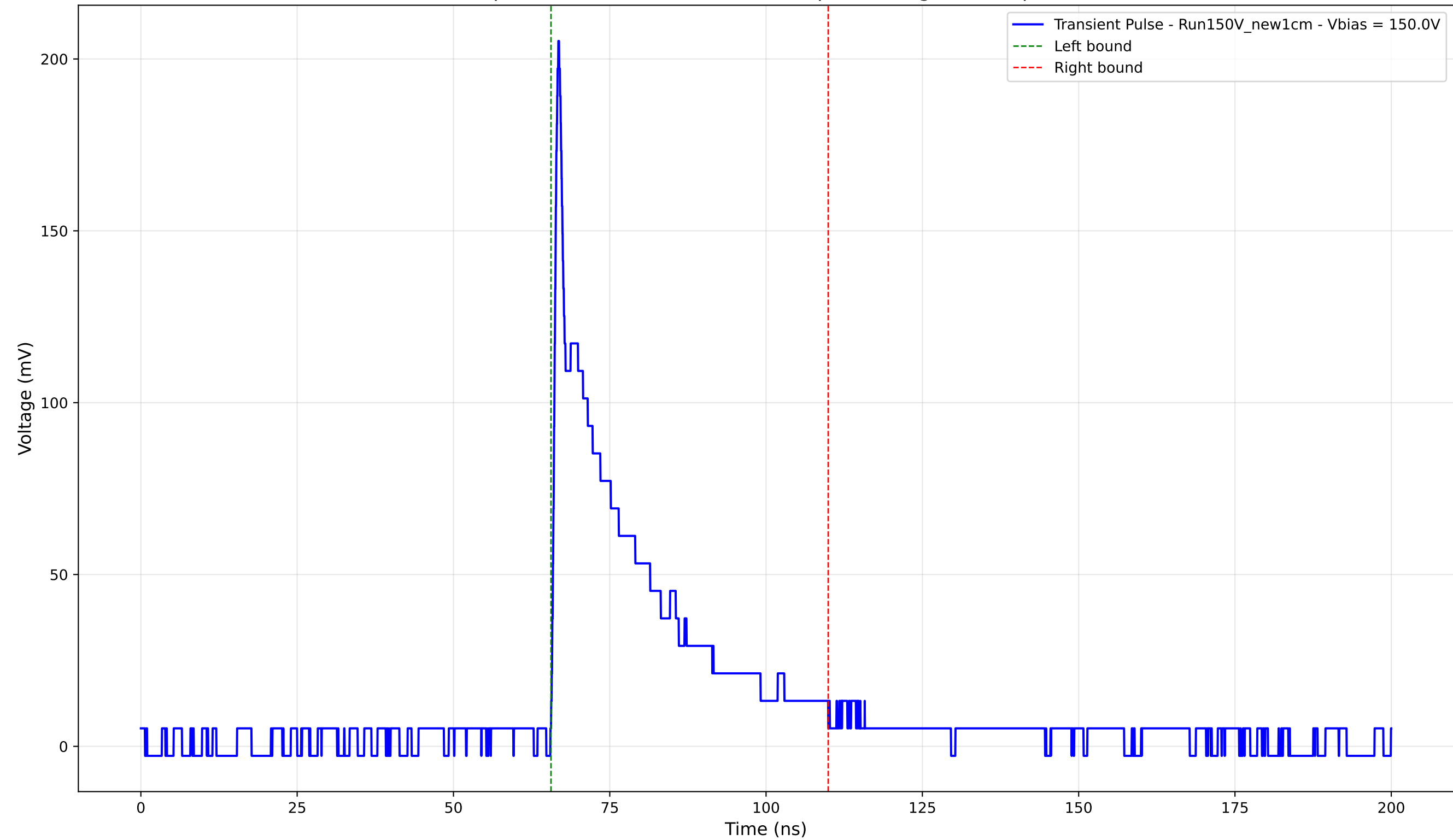
Transient Pulse - Sample: New1cm - Position: 2730.0 \mu\text{m} - Charge: 41.09 pC - Rise Time: 0.88 ns
