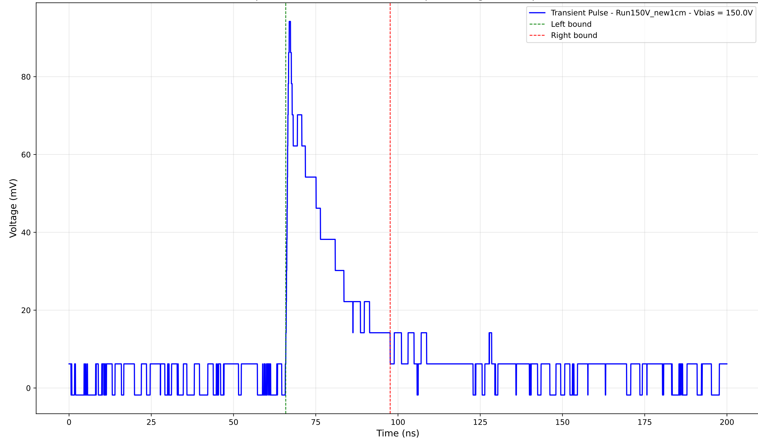
Transient Pulse - Sample: New1cm - Position: 2110.0 \mu\text{m} - Charge: 22.76 pC - Rise Time: 0.85 ns
