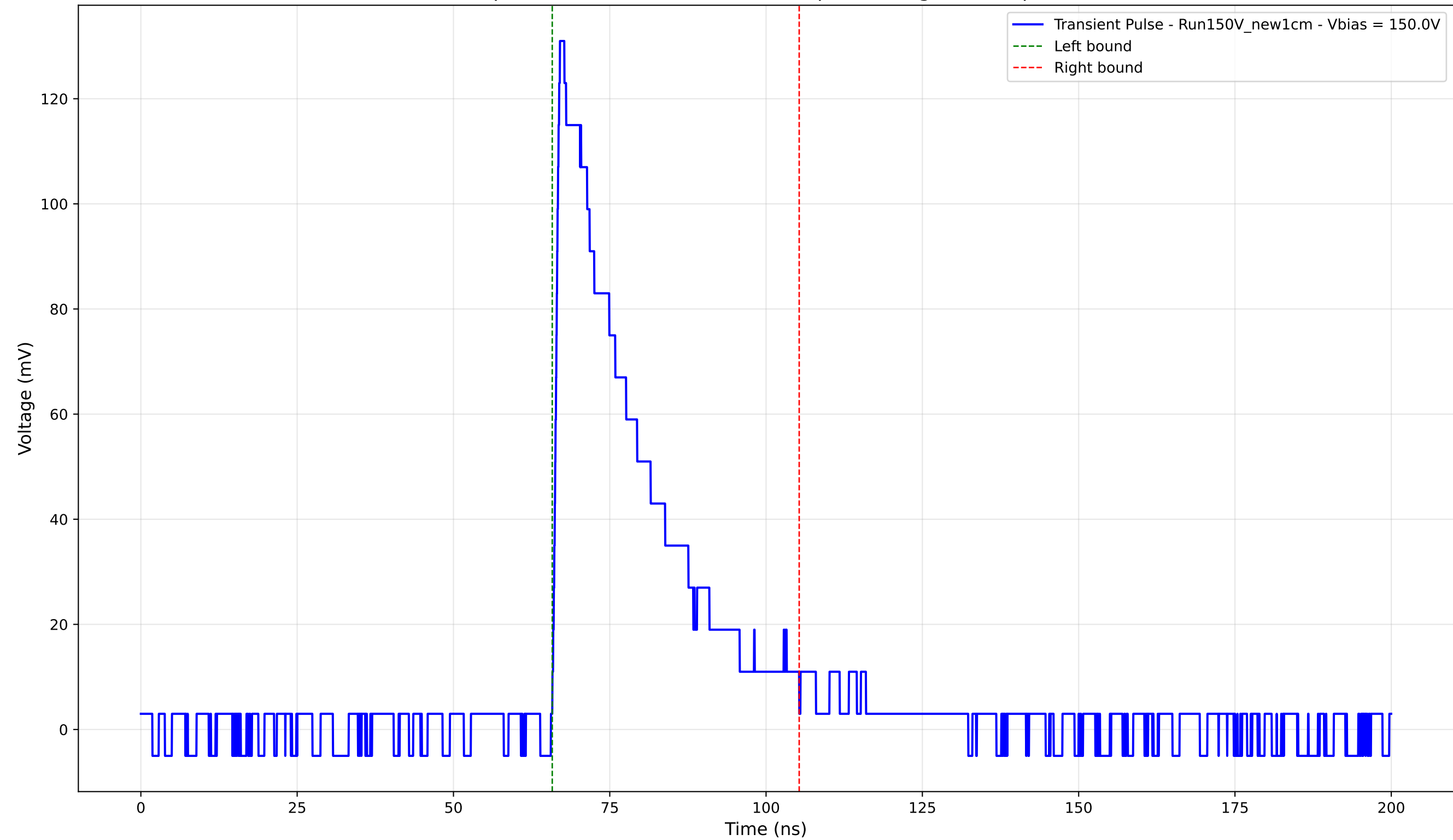
Transient Pulse - Sample: New1cm - Position: 3160.0 \mu\text{m} - Charge: 36.24 pC - Rise Time: 0.97 ns
