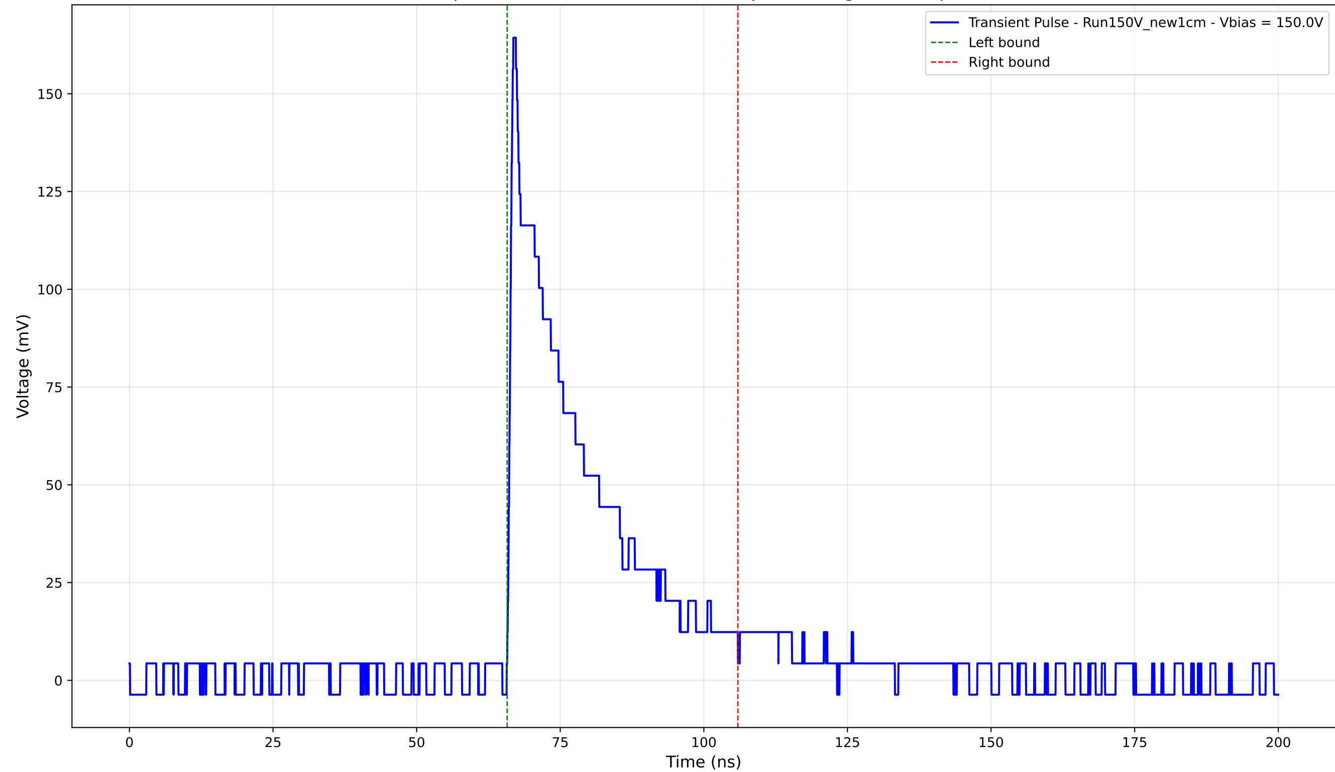
Transient Pulse - Sample: New1cm - Position: 2930.0 \mu\text{m} - Charge: 39.49 pC - Rise Time: 0.81 ns
