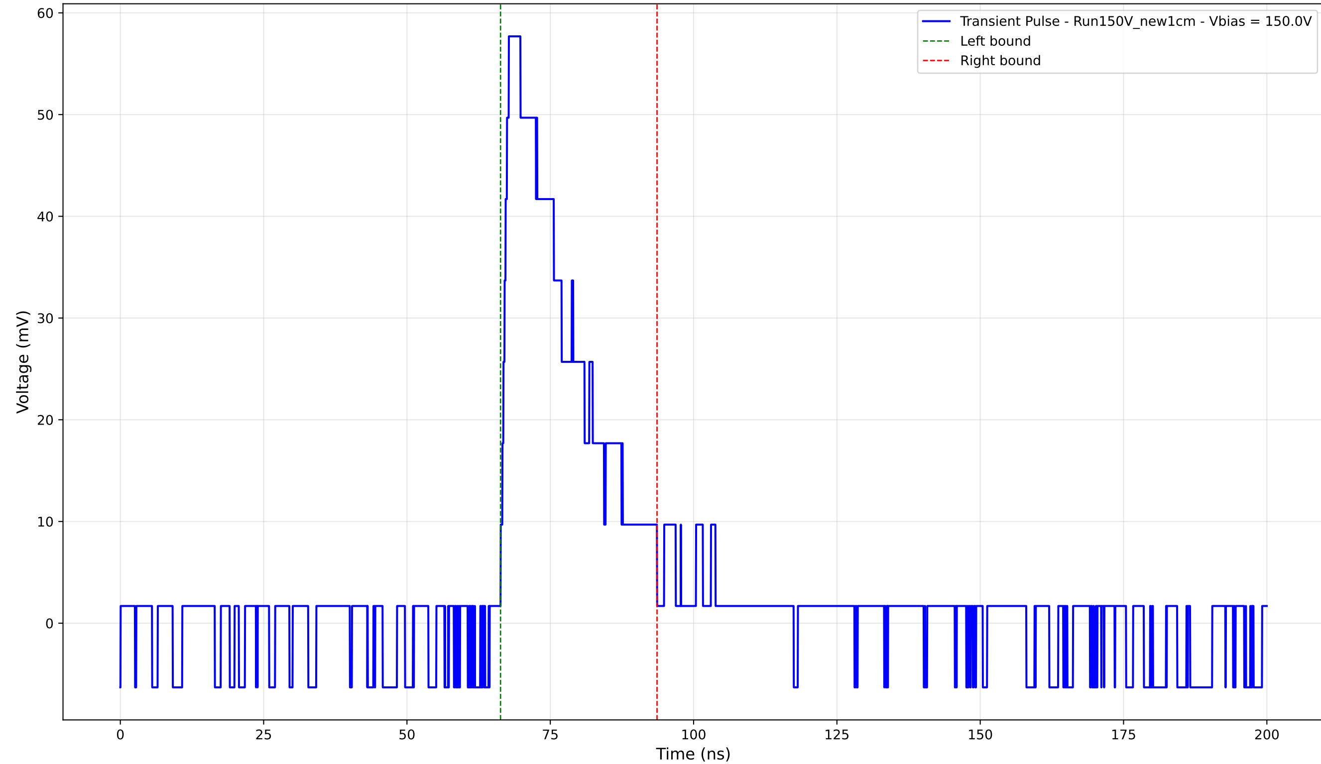
Transient Pulse - Sample: New1cm - Position: 1090.0 \mu\text{m} - Charge: 15.08 pC - Rise Time: 1.43 ns
