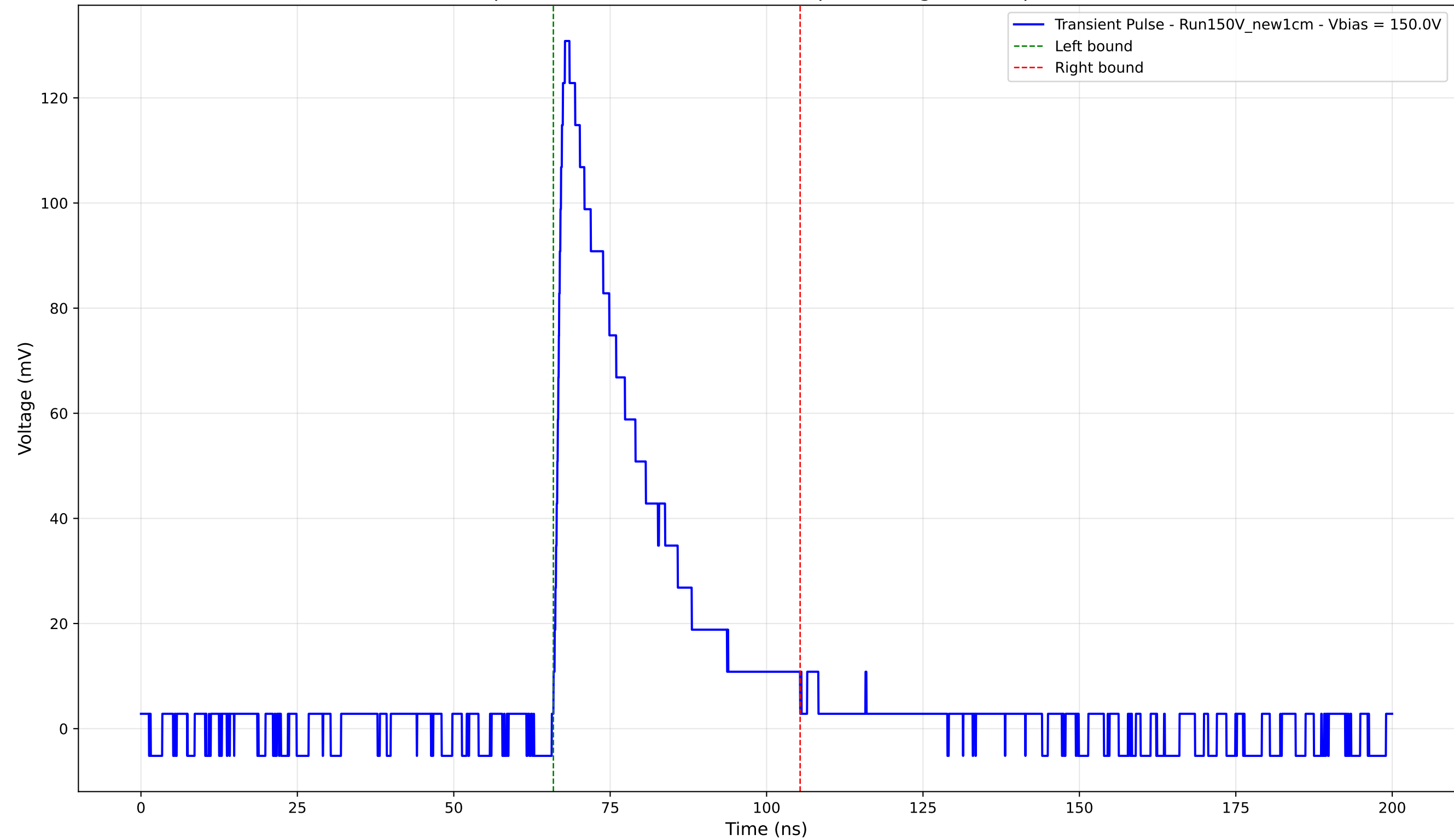
Transient Pulse - Sample: New1cm - Position: 4205.0 \mu\text{m} - Charge: 34.40 pC - Rise Time: 1.33 ns
