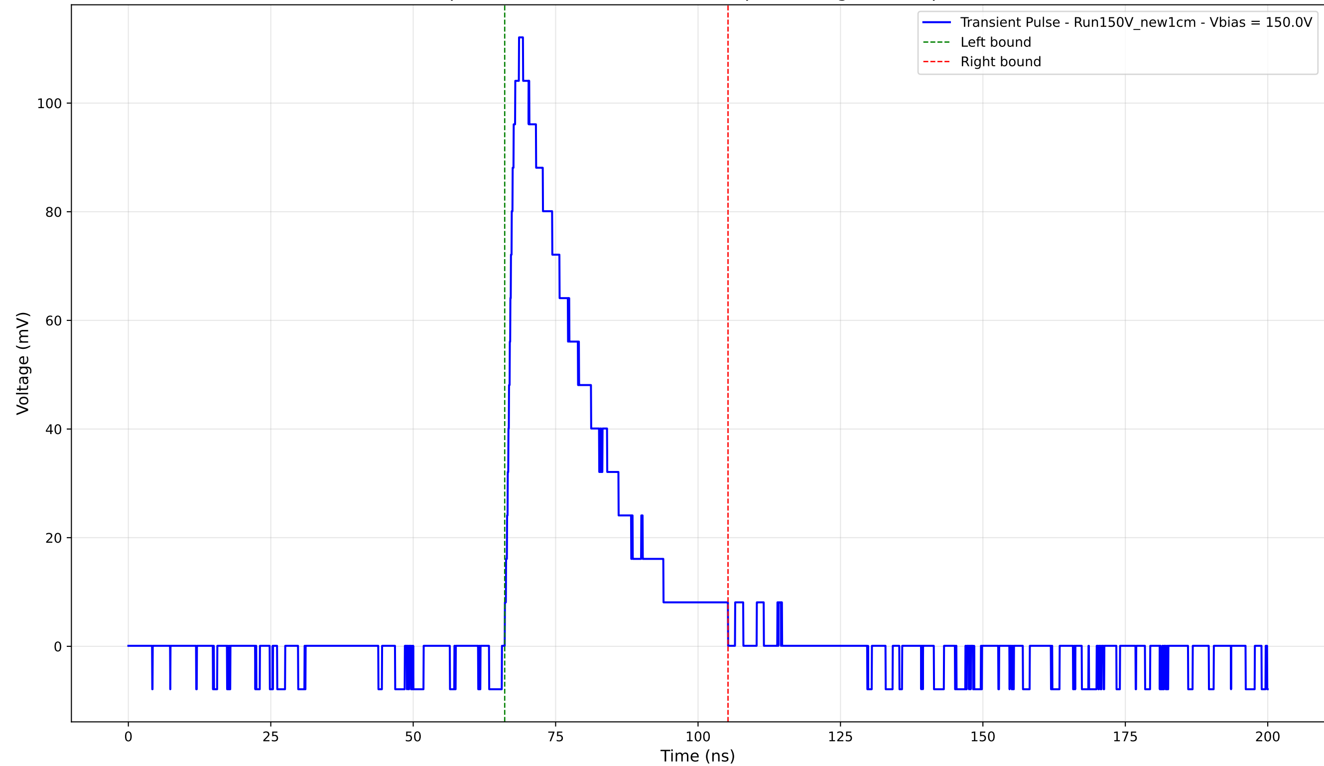
Transient Pulse - Sample: New1cm - Position: 1245.0 \mu\text{m} - Charge: 30.51 pC - Rise Time: 1.63 ns
