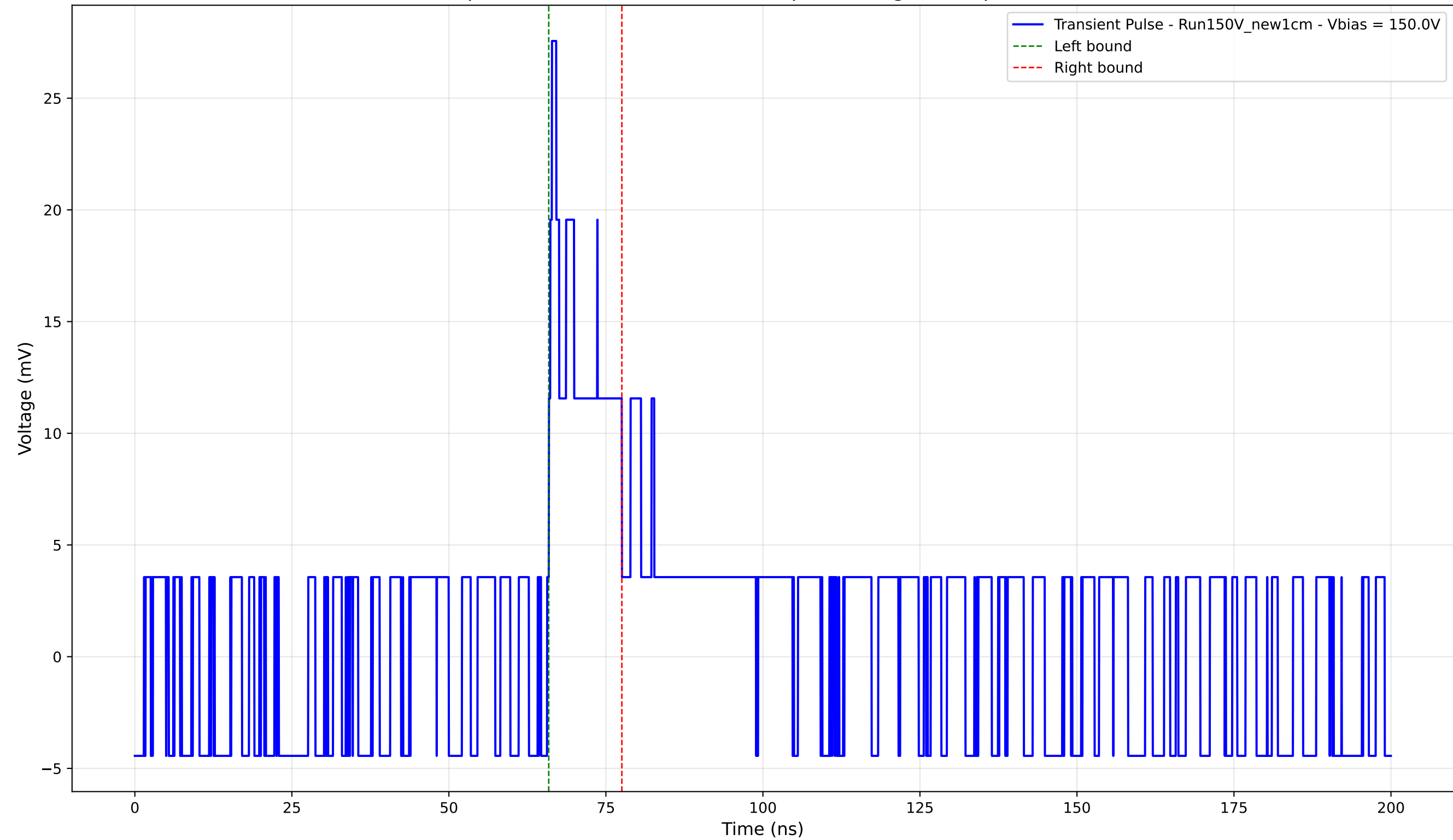
Transient Pulse - Sample: New1cm - Position: 2560.0 \mu\text{m} - Charge: 3.24 pC - Rise Time: 0.00 ns (N/A)
