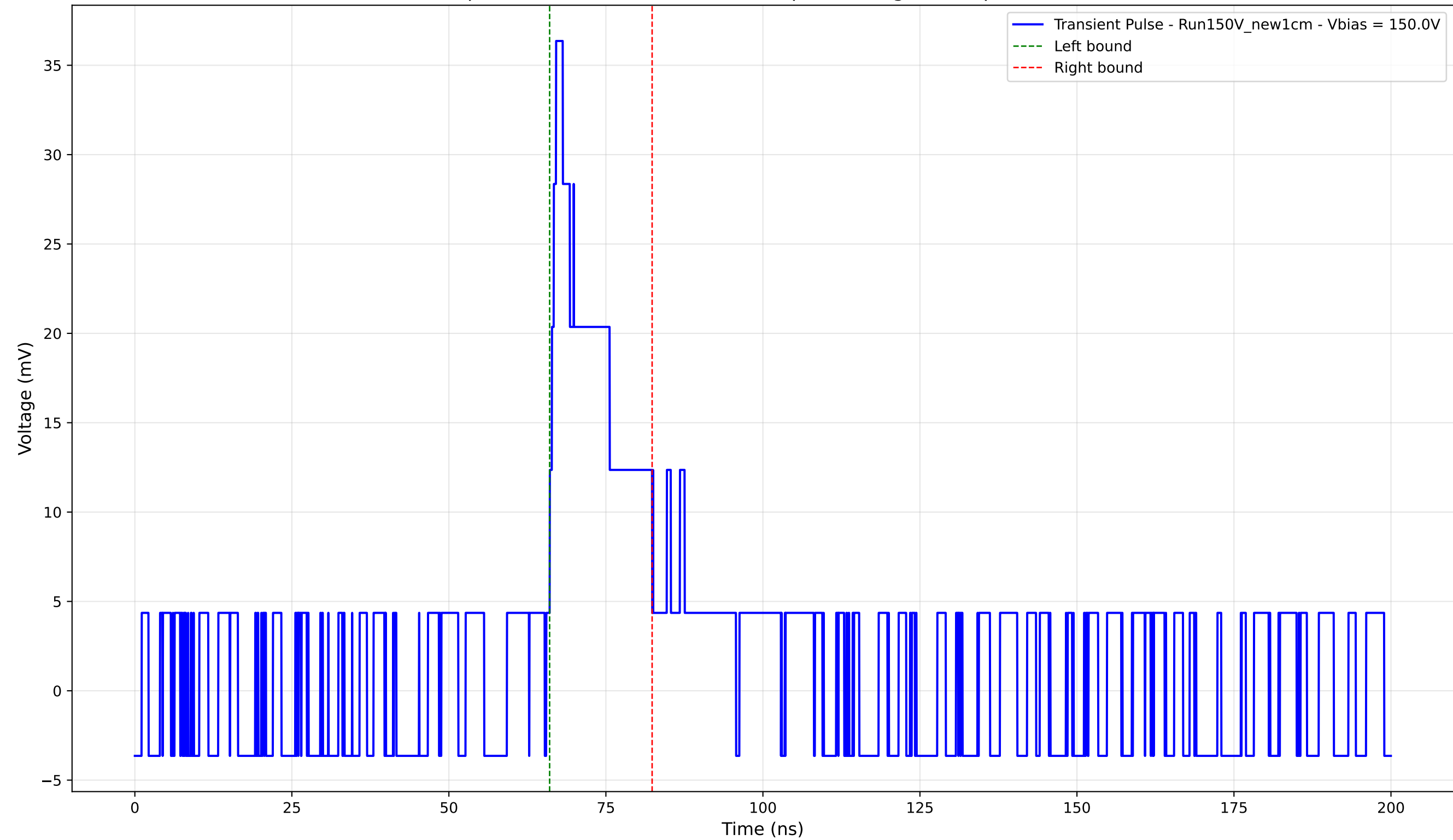
Transient Pulse - Sample: New1cm - Position: 4590.0 \mu\text{m} - Charge: 6.09 pC - Rise Time: 0.00 ns (N/A)
