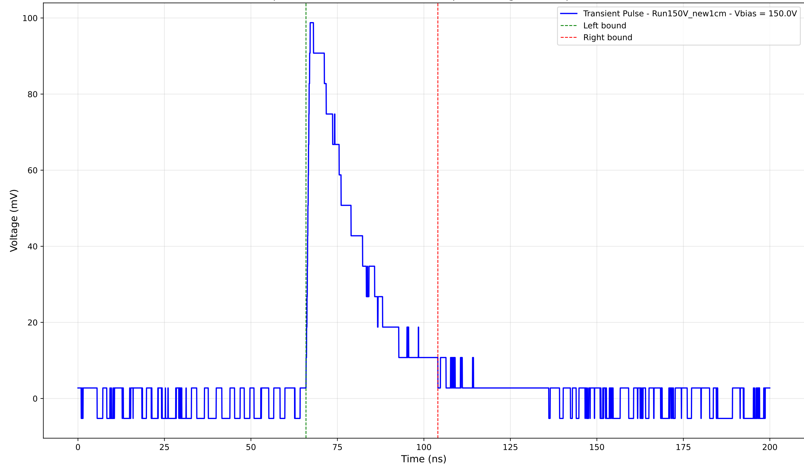
Transient Pulse - Sample: New1cm - Position: 1885.0 \mu\text{m} - Charge: 29.22 pC - Rise Time: 1.02 ns
