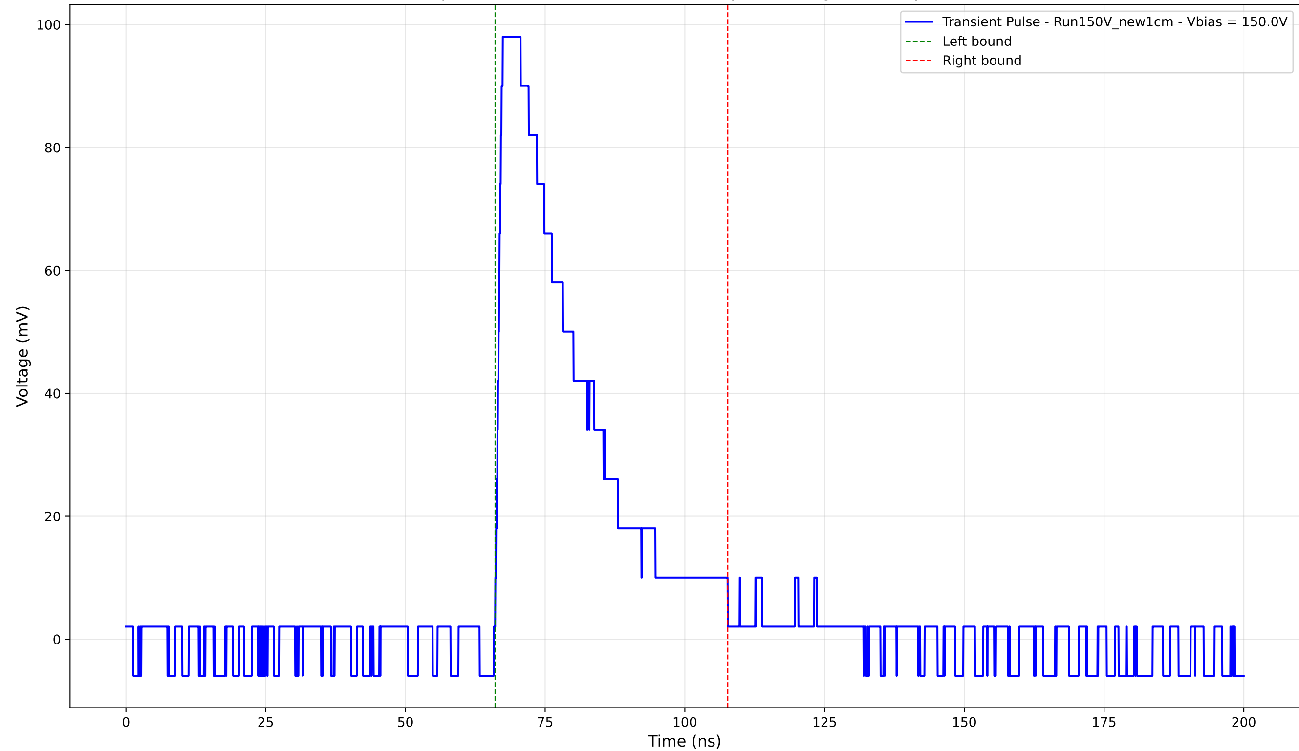
Transient Pulse - Sample: New1cm - Position: 1670.0 \mu\text{m} - Charge: 31.25 pC - Rise Time: 1.12 ns
