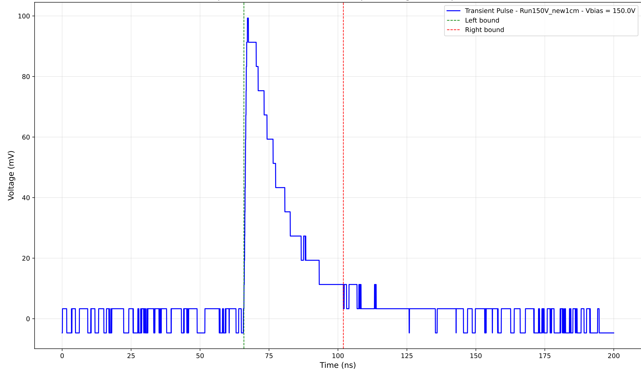
Transient Pulse - Sample: New1cm - Position: 1945.0 \mu\text{m} - Charge: 27.77 pC - Rise Time: 0.98 ns
