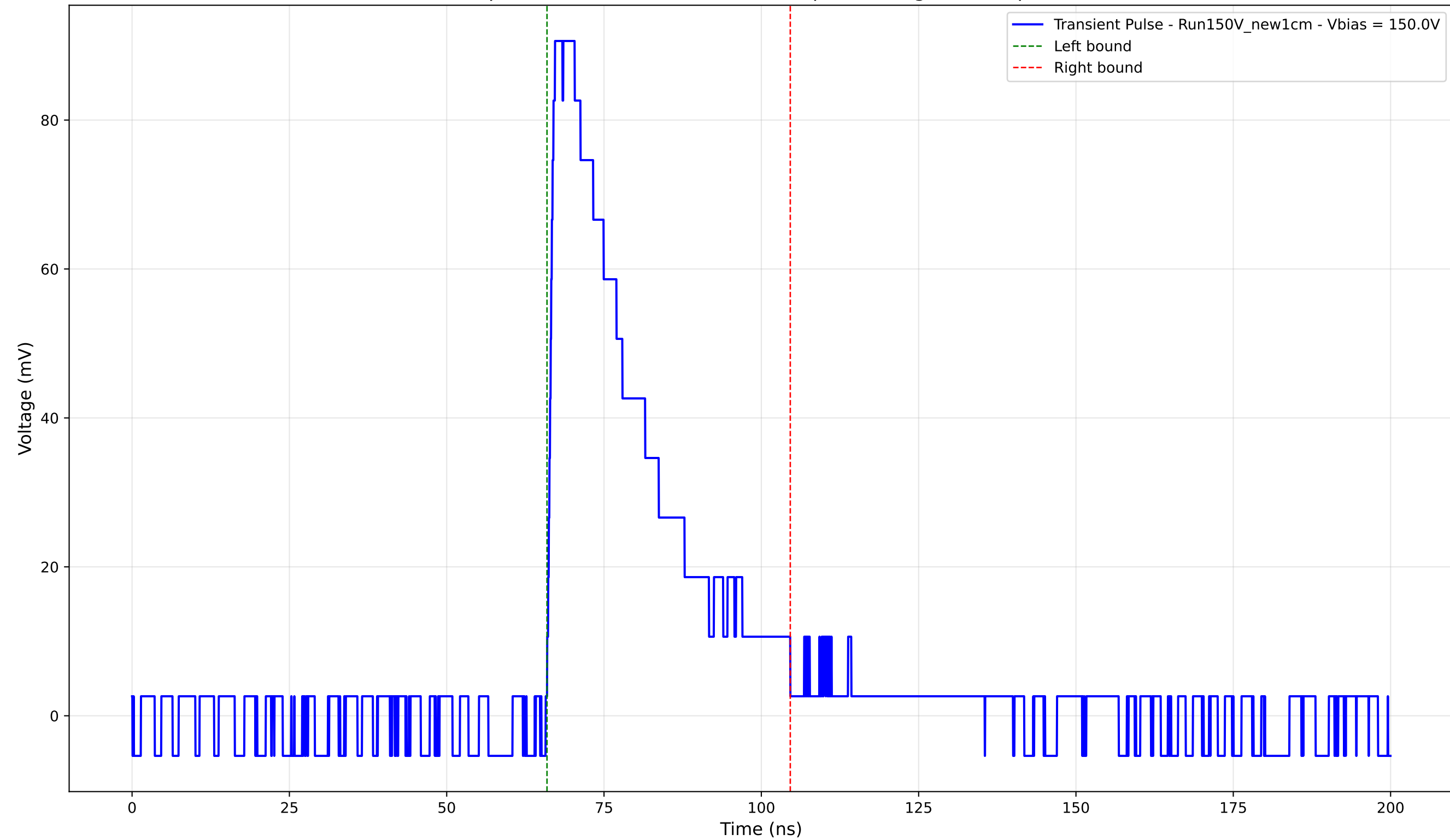
Transient Pulse - Sample: New1cm - Position: 1850.0 \mu\text{m} - Charge: 28.53 pC - Rise Time: 1.00 ns
