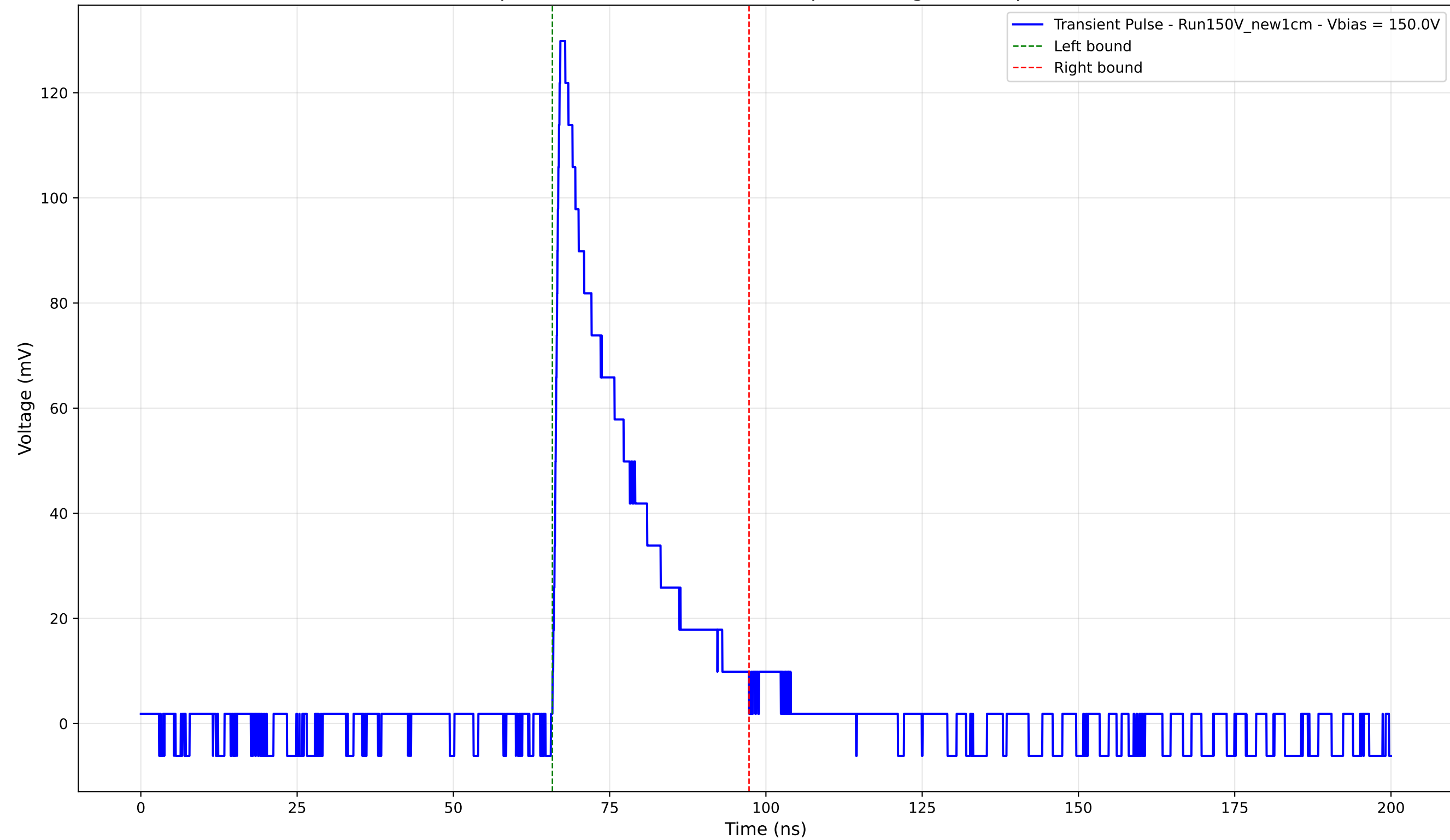
Transient Pulse - Sample: New1cm - Position: 345.0 \mu\text{m} - Charge: 28.40 pC - Rise Time: 1.01 ns
