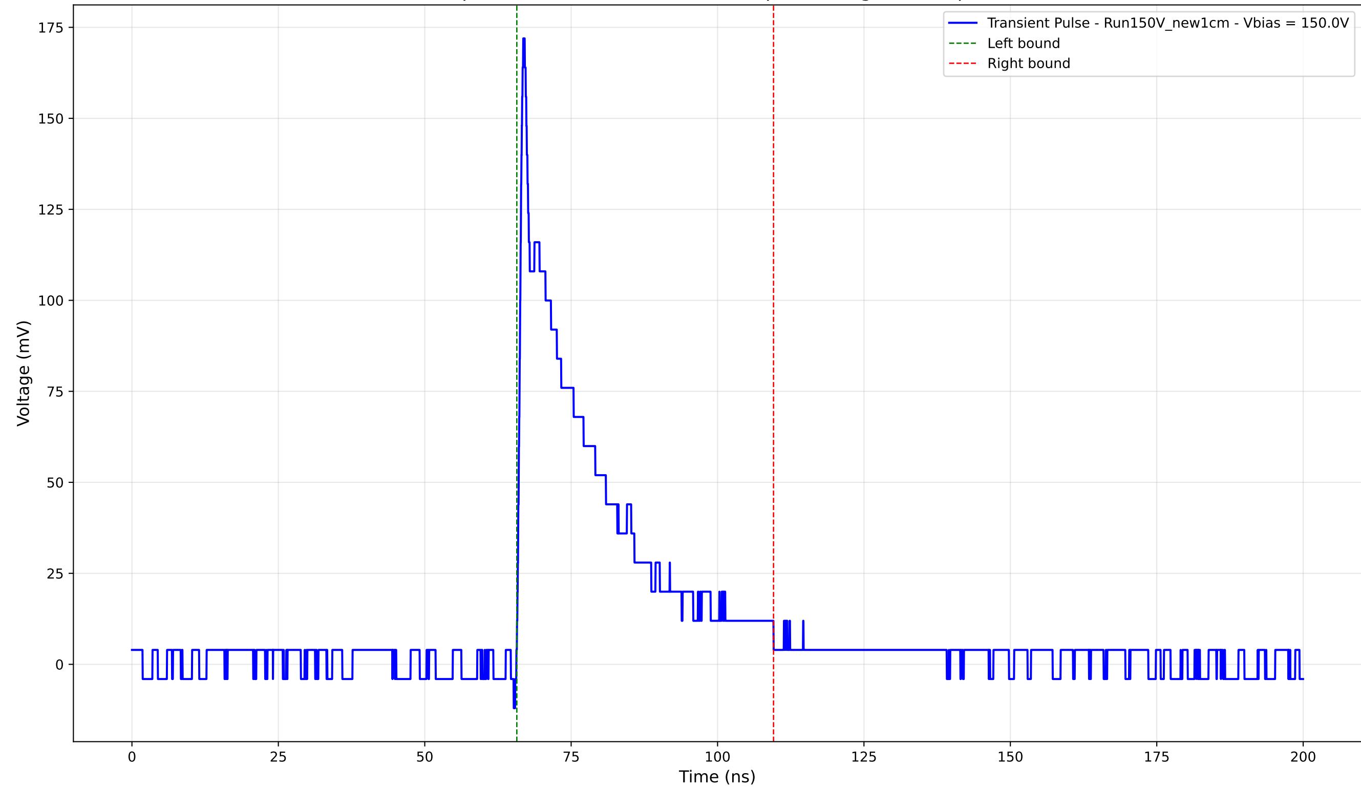
Transient Pulse - Sample: New1cm - Position: 2845.0 \mu\text{m} - Charge: 38.14 pC - Rise Time: 0.81 ns
