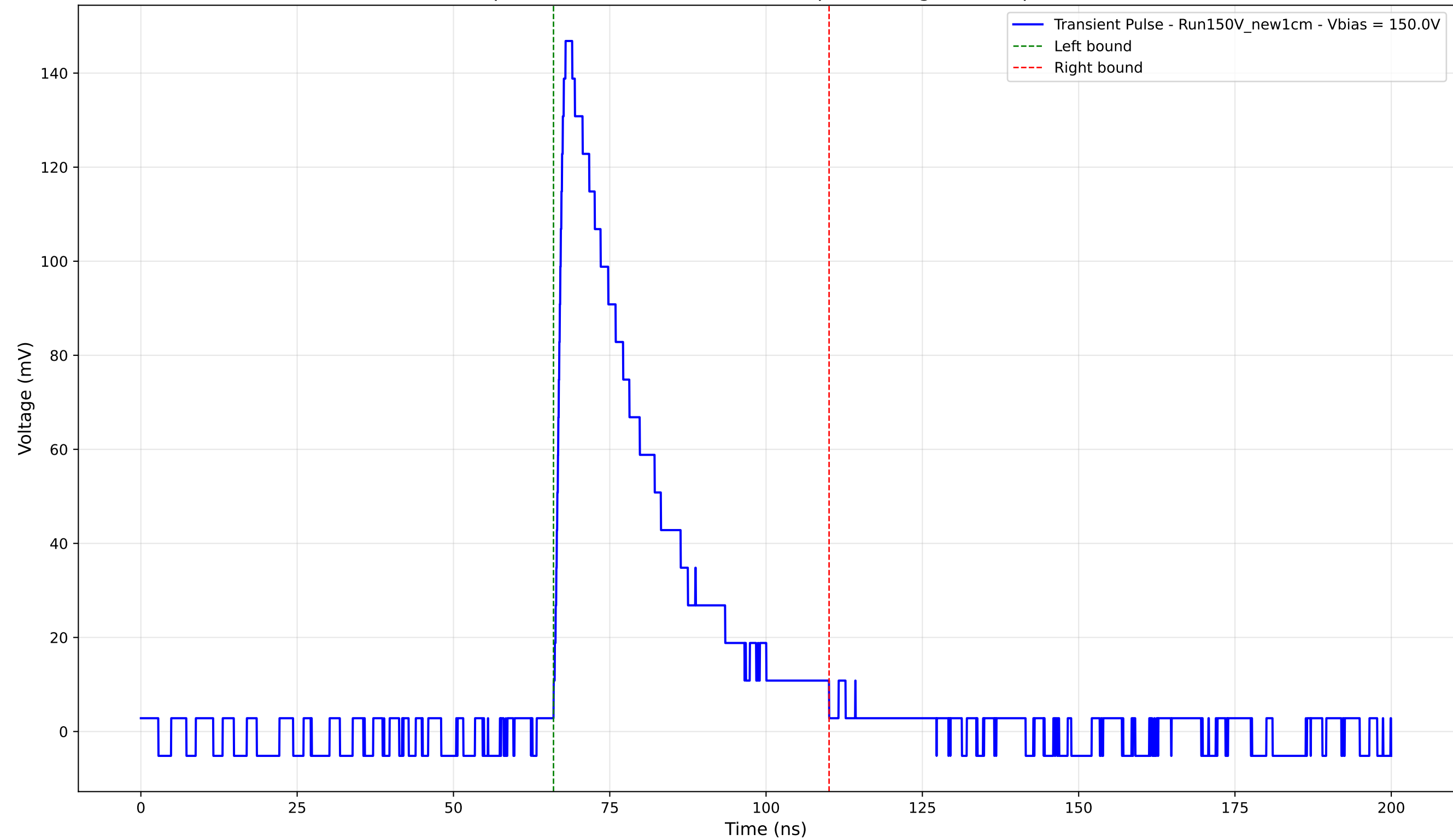
Transient Pulse - Sample: New1cm - Position: 3735.0 \mu\text{m} - Charge: 42.52 pC - Rise Time: 1.45 ns
