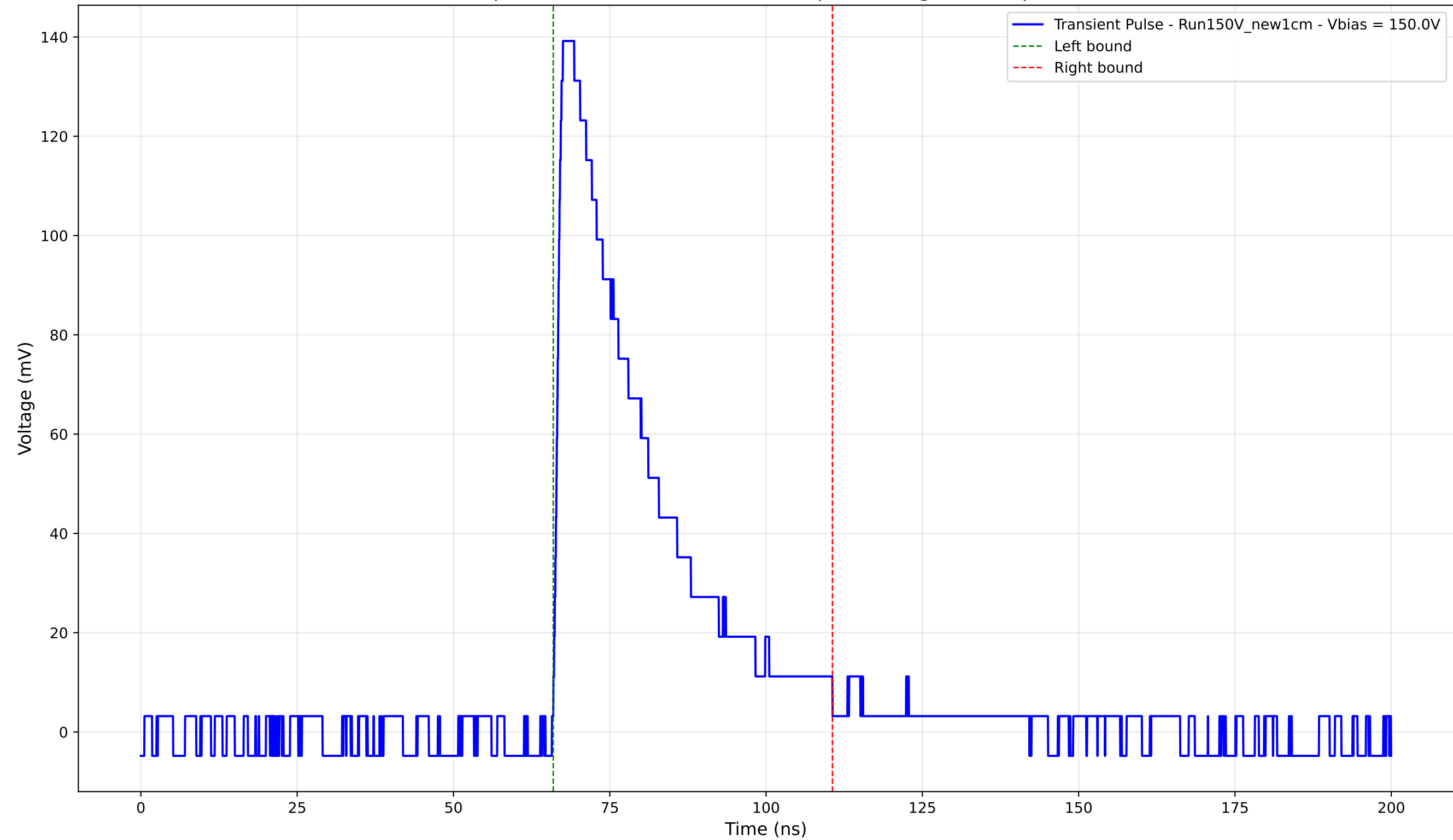
Transient Pulse - Sample: New1cm - Position: 3415.0 \mu\text{m} - Charge: 42.21 pC - Rise Time: 1.19 ns
