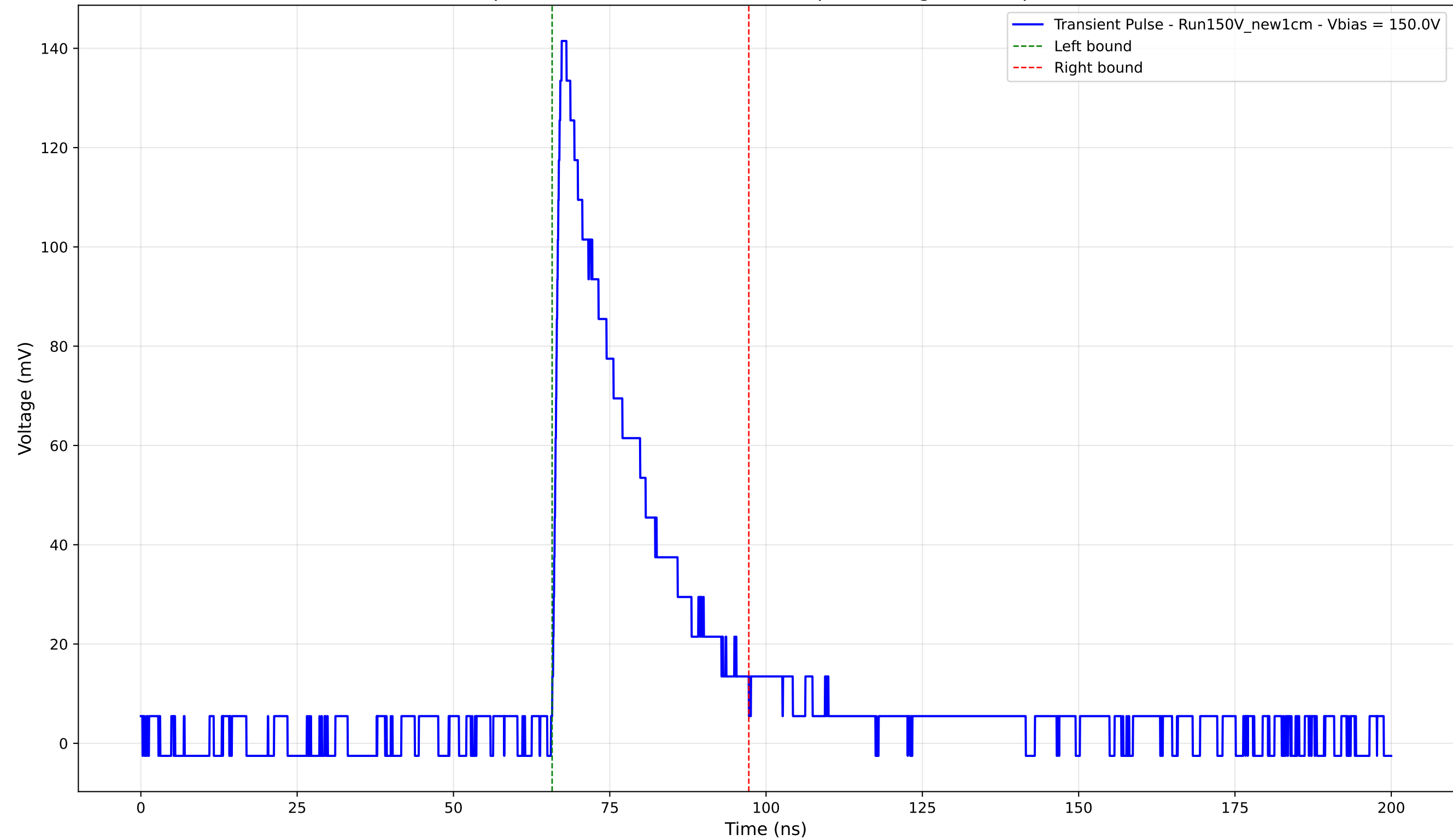
Transient Pulse - Sample: New1cm - Position: 4480.0 \mu\text{m} - Charge: 34.94 pC - Rise Time: 1.16 ns
