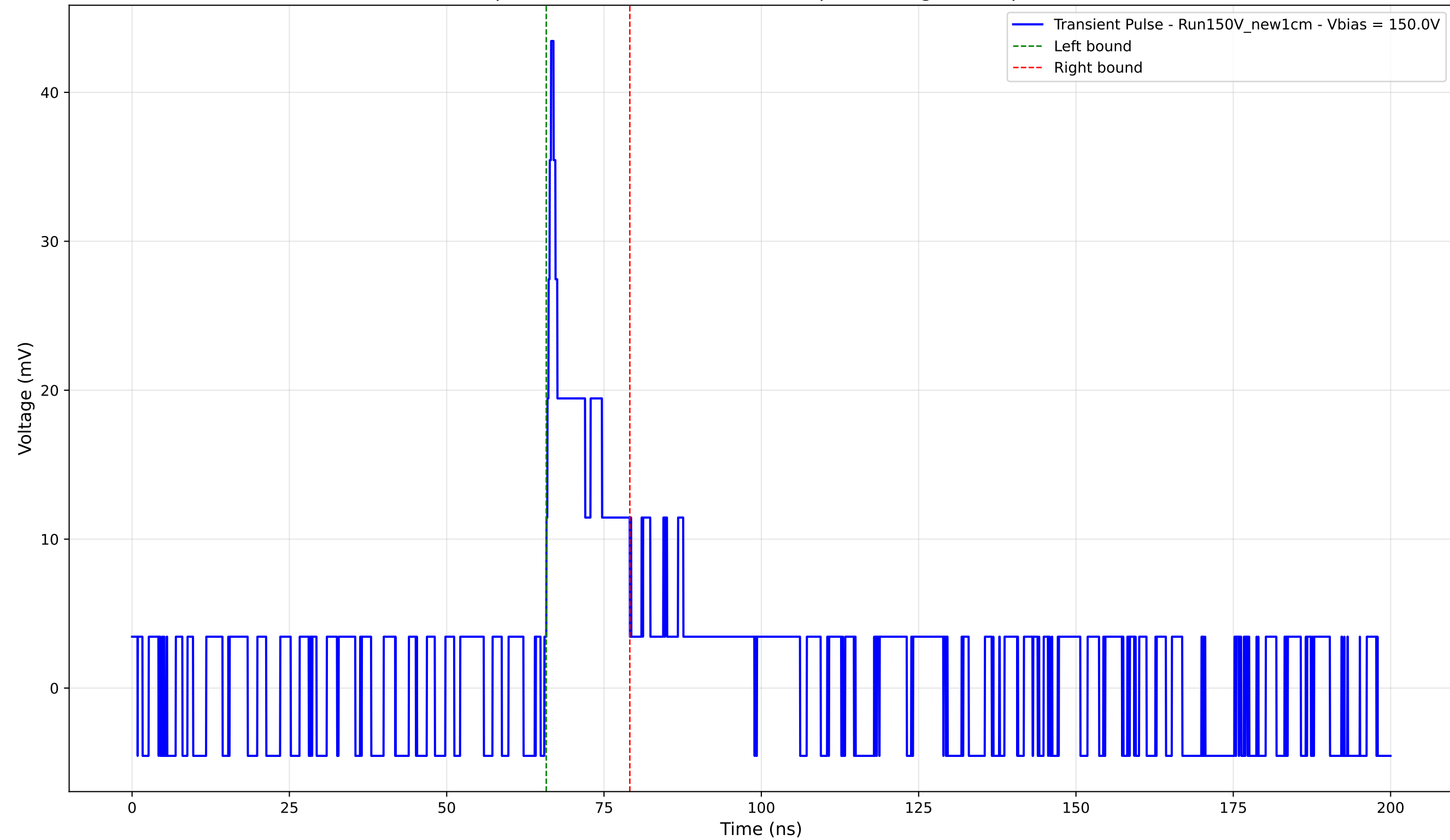
Transient Pulse - Sample: New1cm - Position: 2530.0 \mu\text{m} - Charge: 4.72 pC - Rise Time: 0.76 ns
