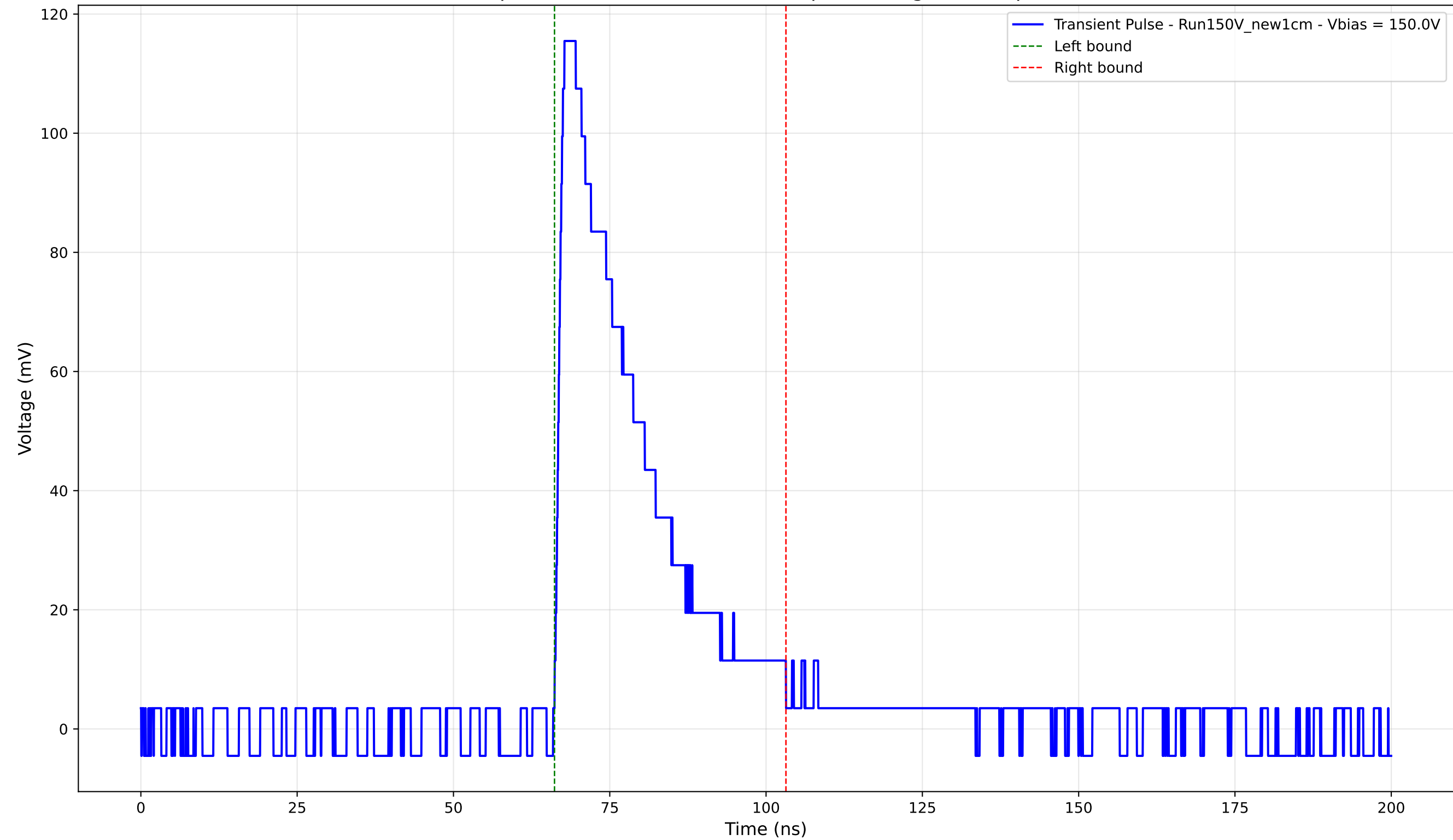
Transient Pulse - Sample: New1cm - Position: 870.0 \mu\text{m} - Charge: 31.99 pC - Rise Time: 1.18 ns
