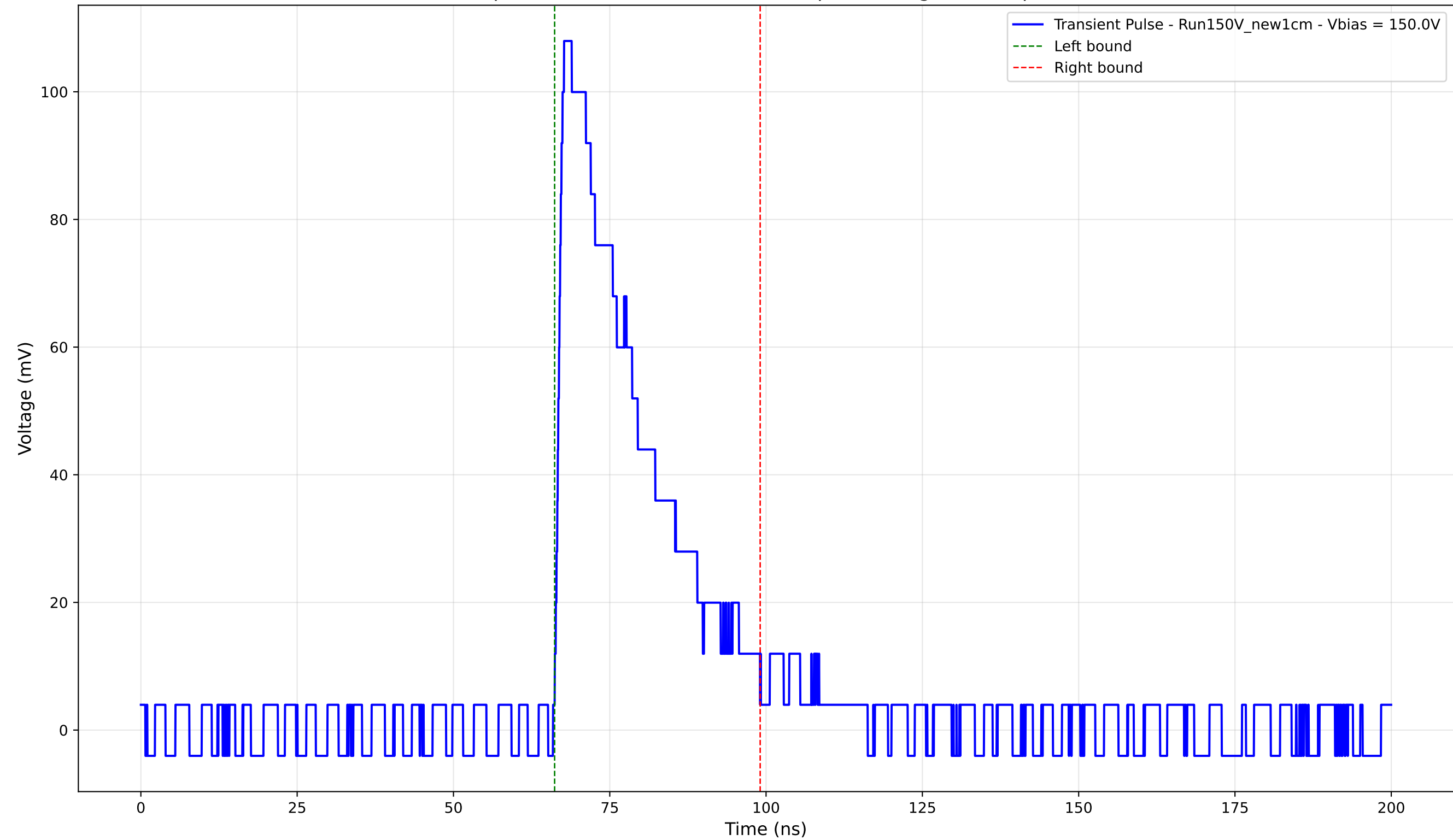
Transient Pulse - Sample: New1cm - Position: 3640.0 \mu\text{m} - Charge: 30.58 pC - Rise Time: 1.24 ns
