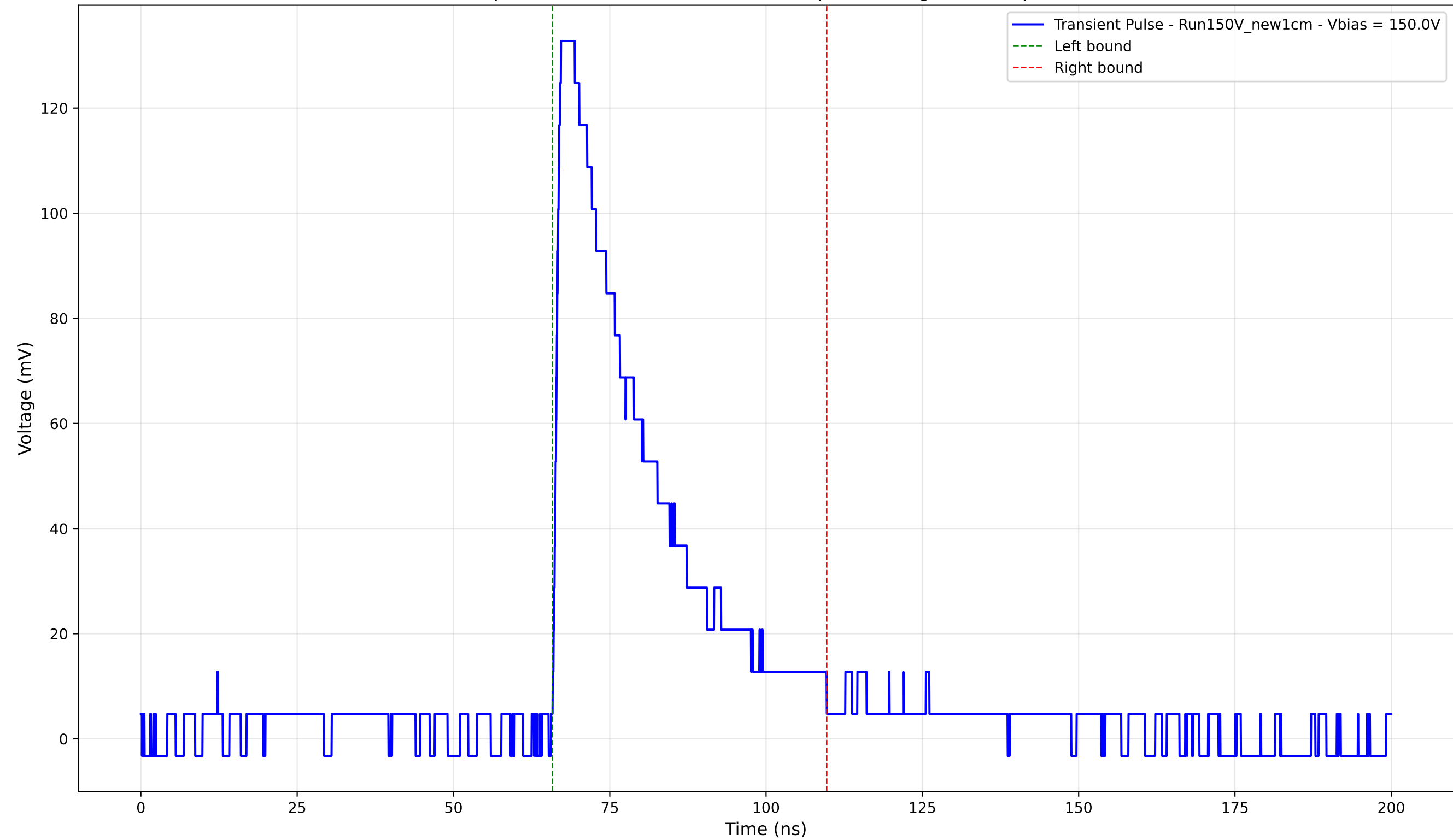
Transient Pulse - Sample: New1cm - Position: 3235.0 \mu\text{m} - Charge: 41.30 pC - Rise Time: 1.04 ns
