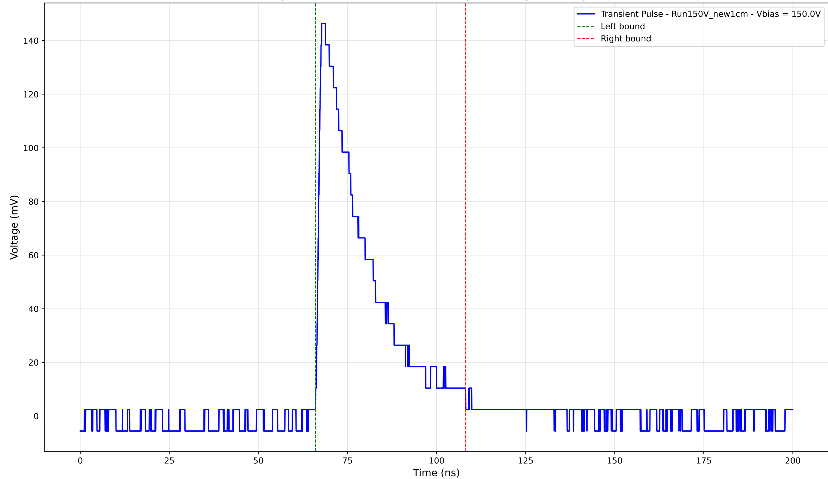
Transient Pulse - Sample: New1cm - Position: 3770.0 \mu\text{m} - Charge: 41.79 pC - Rise Time: 1.33 ns
