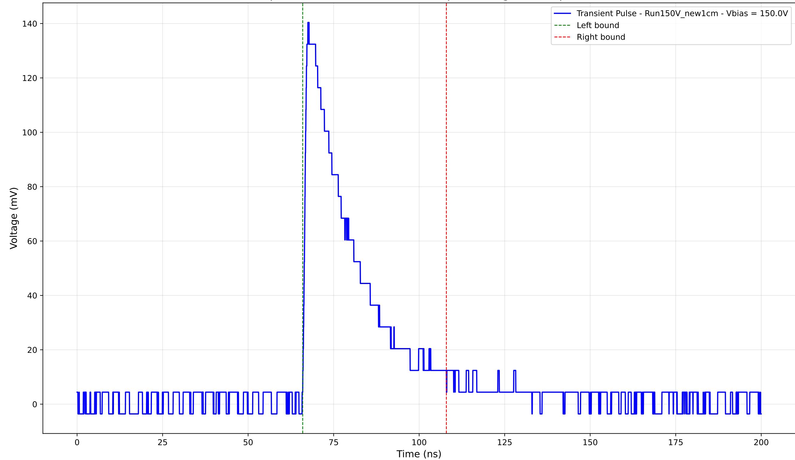
Transient Pulse - Sample: New1cm - Position: 3295.0 \mu\text{m} - Charge: 41.47 pC - Rise Time: 1.12 ns
