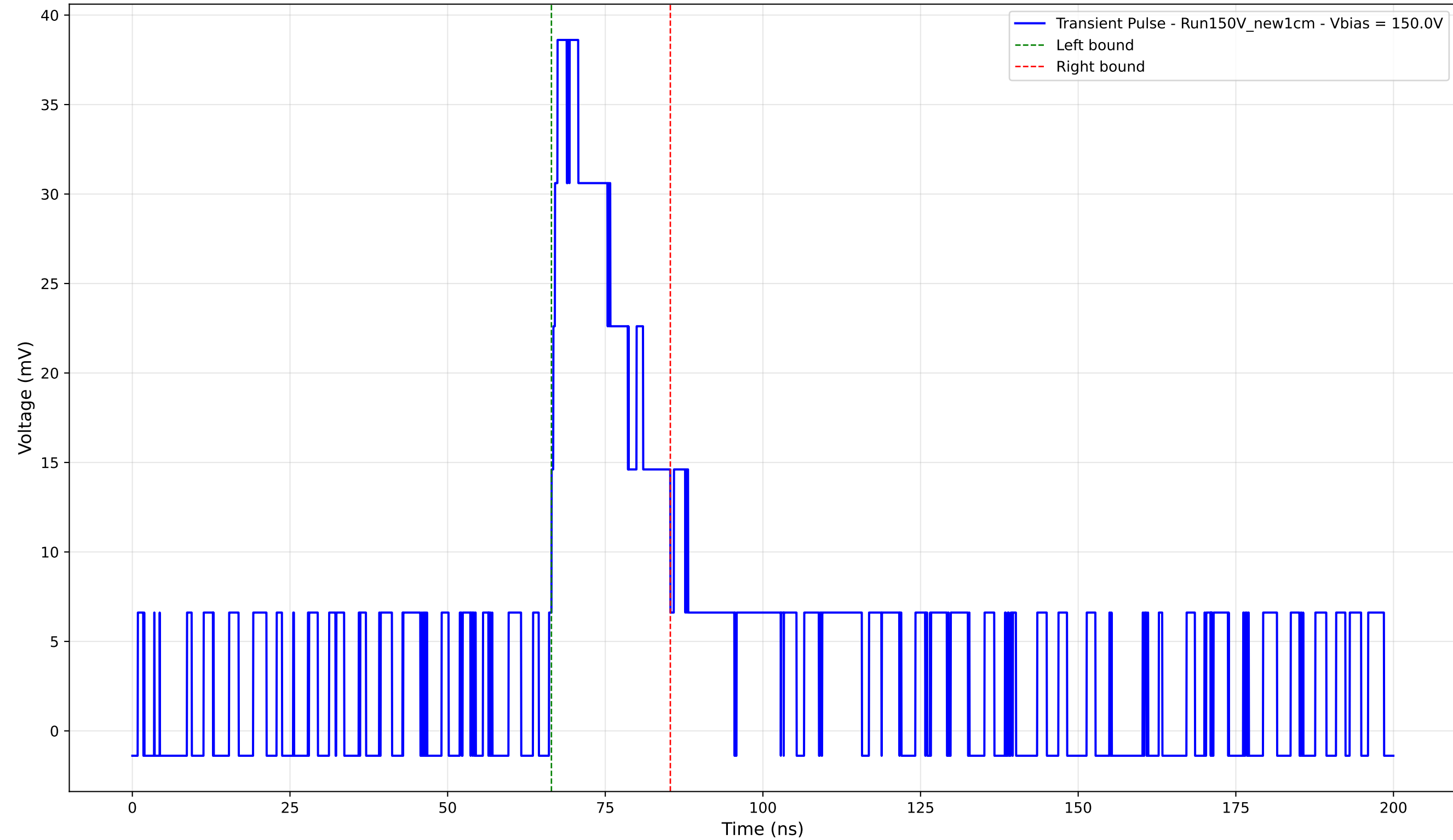
Transient Pulse - Sample: New1cm - Position: 3535.0 \mu\text{m} - Charge: 9.45 pC - Rise Time: 1.35 ns
