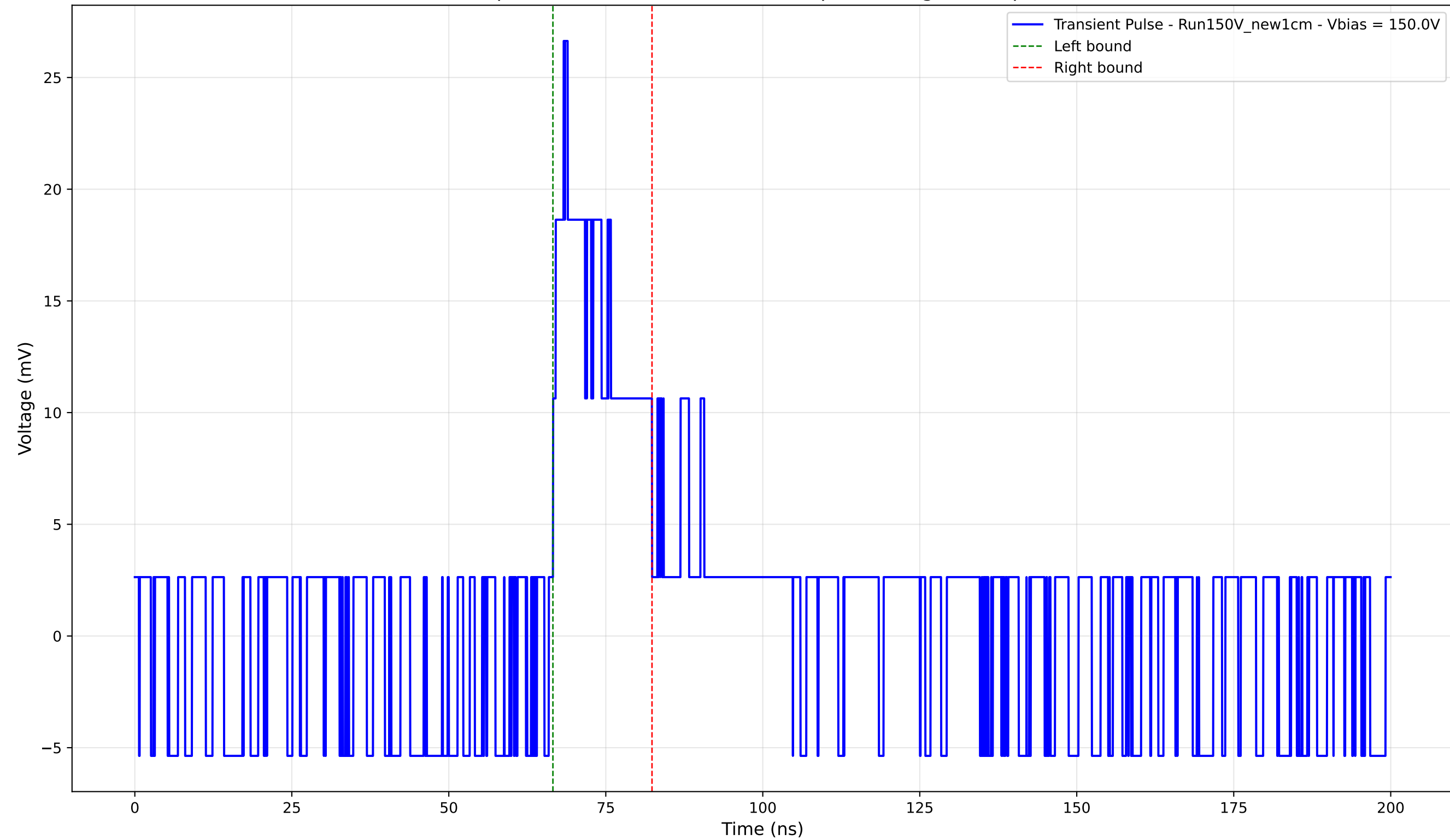
Transient Pulse - Sample: New1cm - Position: 1520.0 \mu\text{m} - Charge: 4.64 pC - Rise Time: 1.70 ns
