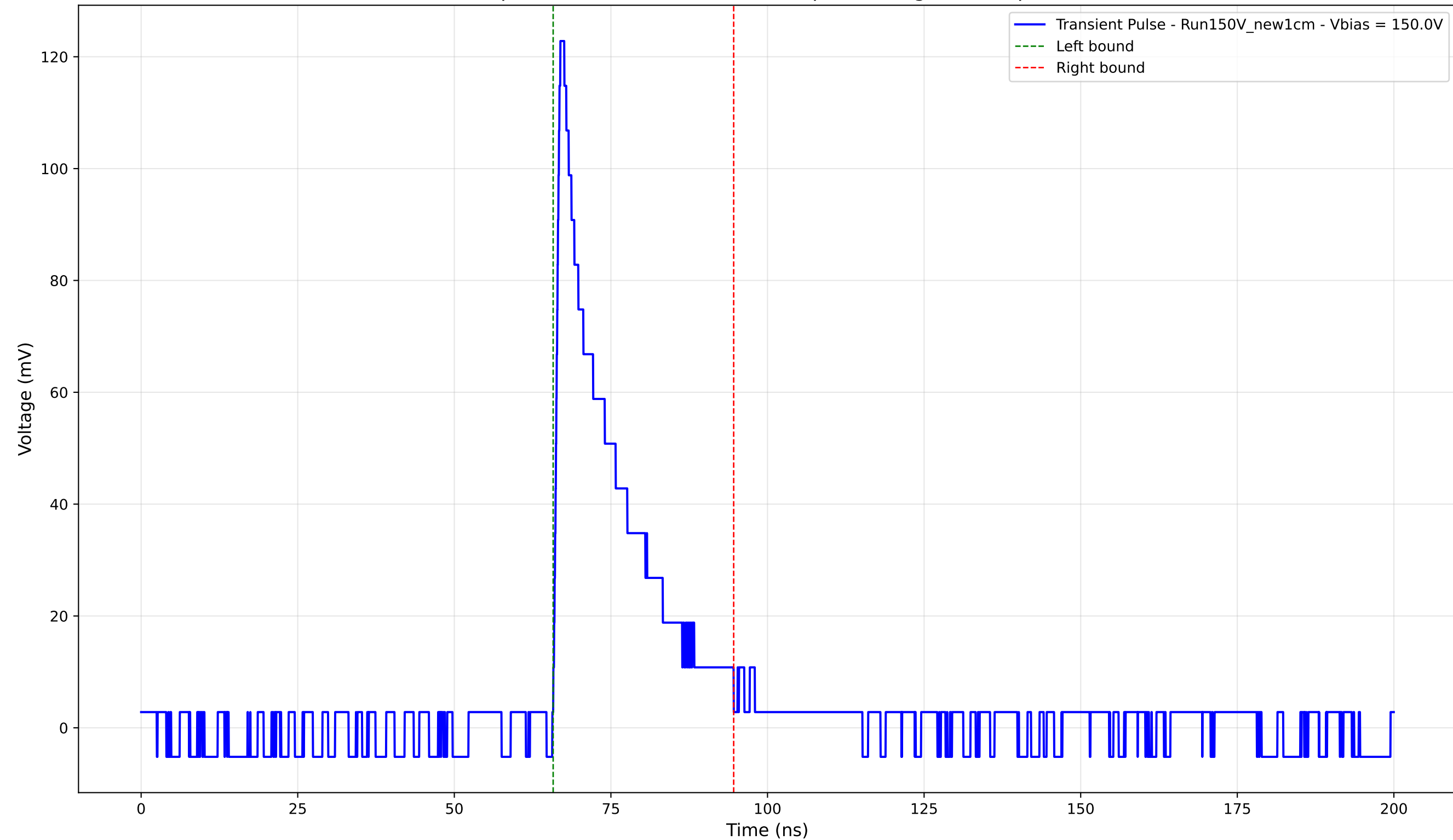
Transient Pulse - Sample: New1cm - Position: 160.0 \mu\text{m} - Charge: 22.77 pC - Rise Time: 0.88 ns
