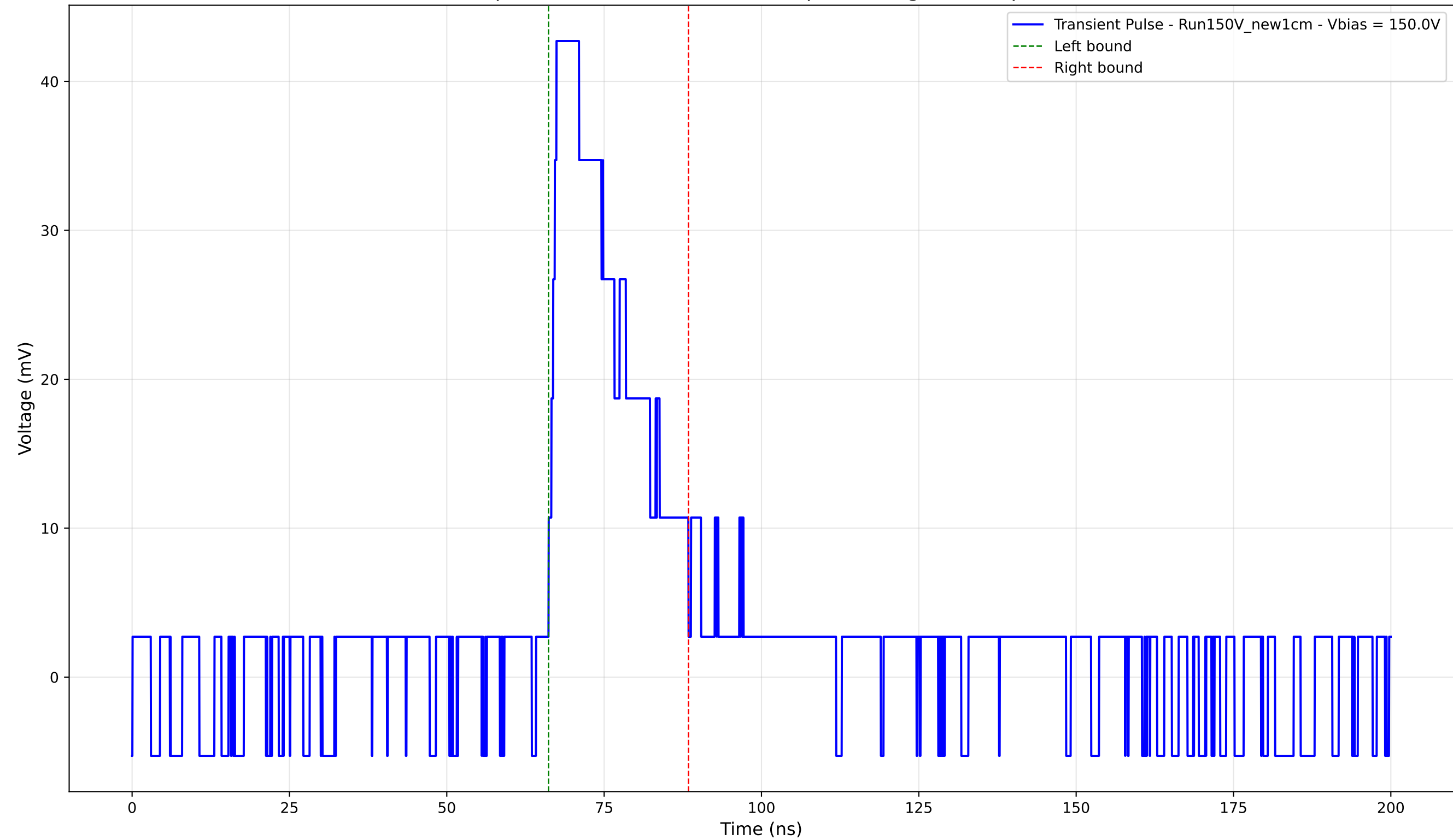
Transient Pulse - Sample: New1cm - Position: 990.0 \mu\text{m} - Charge: 10.85 pC - Rise Time: 1.26 ns
