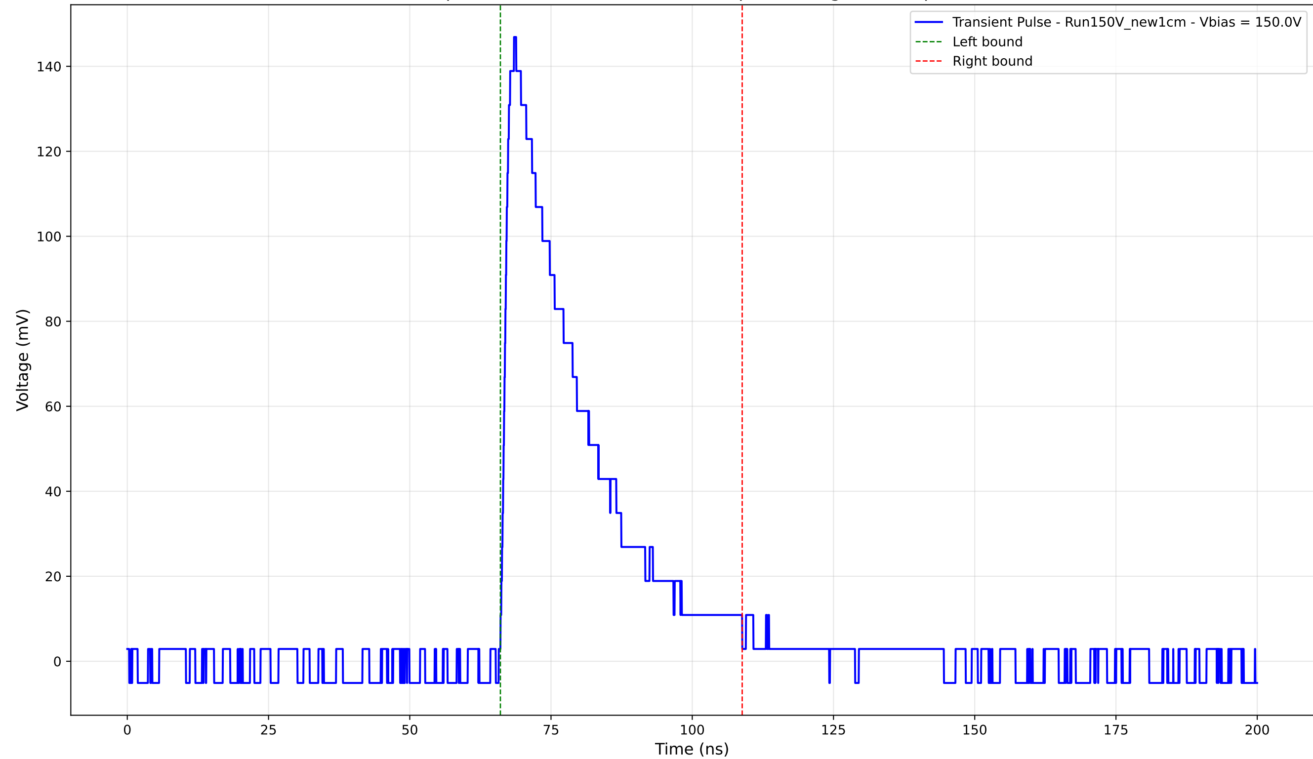
Transient Pulse - Sample: New1cm - Position: 3765.0 \mu\text{m} - Charge: 41.78 pC - Rise Time: 1.57 ns
