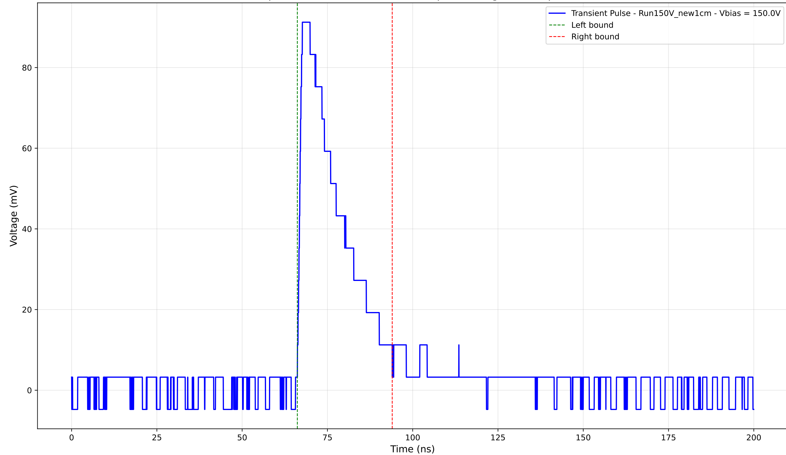
Transient Pulse - Sample: New1cm - Position: 950.0 \mu\text{m} - Charge: 24.22 pC - Rise Time: 1.23 ns
