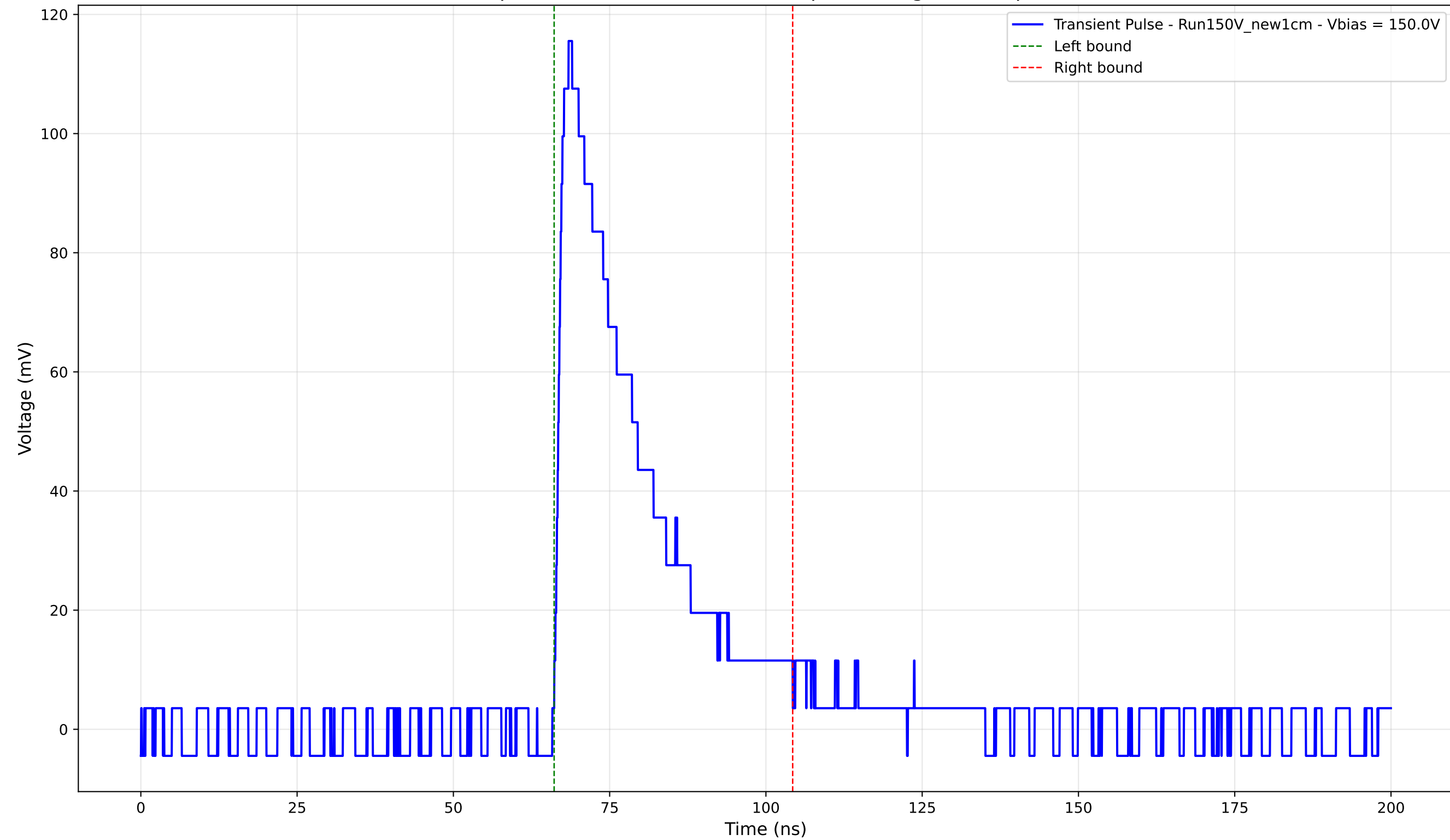
Transient Pulse - Sample: New1cm - Position: 915.0 \mu\text{m} - Charge: 31.41 pC - Rise Time: 1.40 ns
