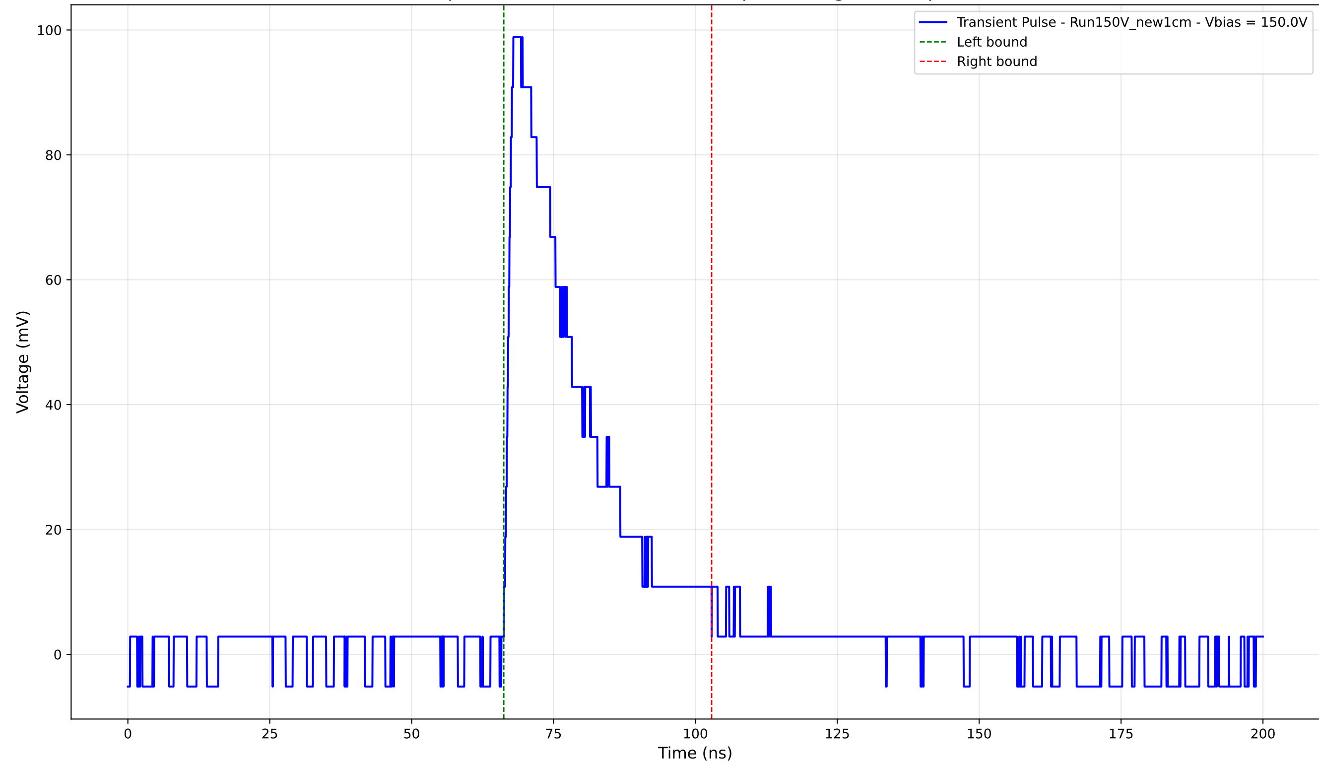
Transient Pulse - Sample: New1cm - Position: 1135.0 \mu\text{m} - Charge: 27.35 pC - Rise Time: 1.40 ns
