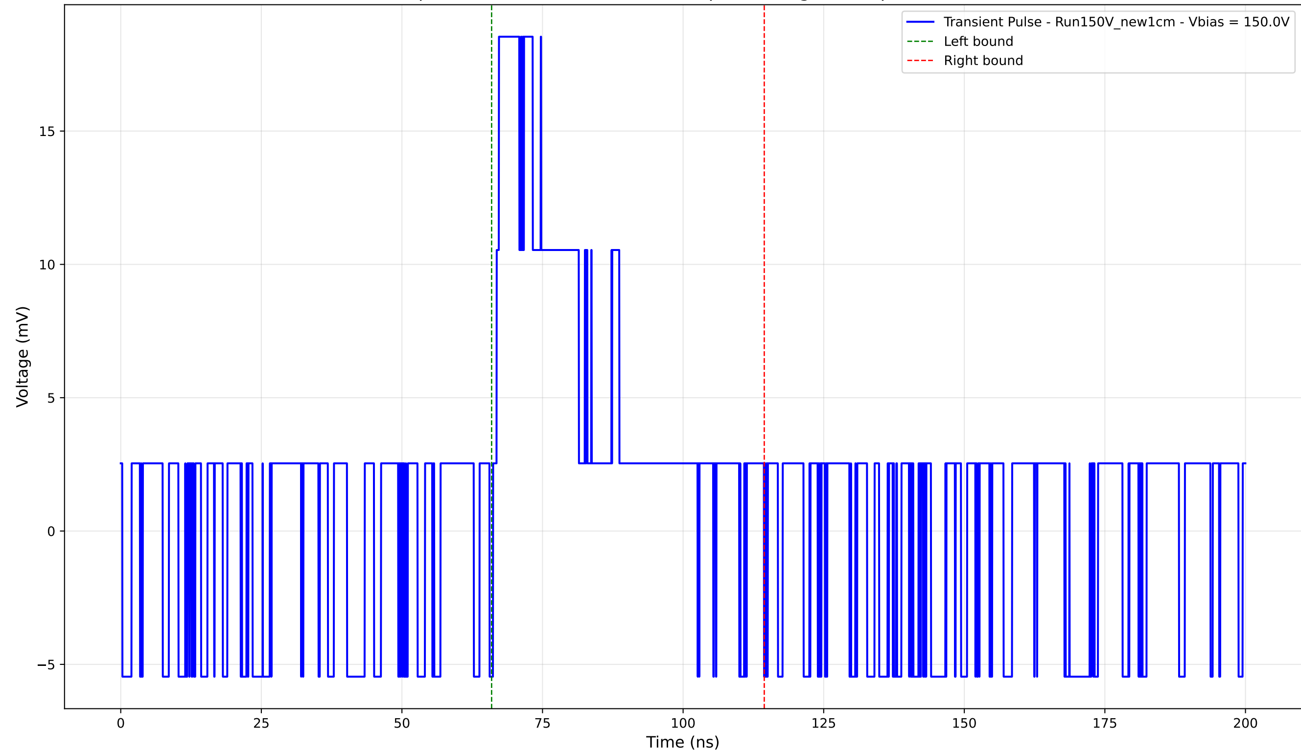
Transient Pulse - Sample: New1cm - Position: 1020.0 \mu\text{m} - Charge: 5.70 pC - Rise Time: 0.00 ns (N/A)
