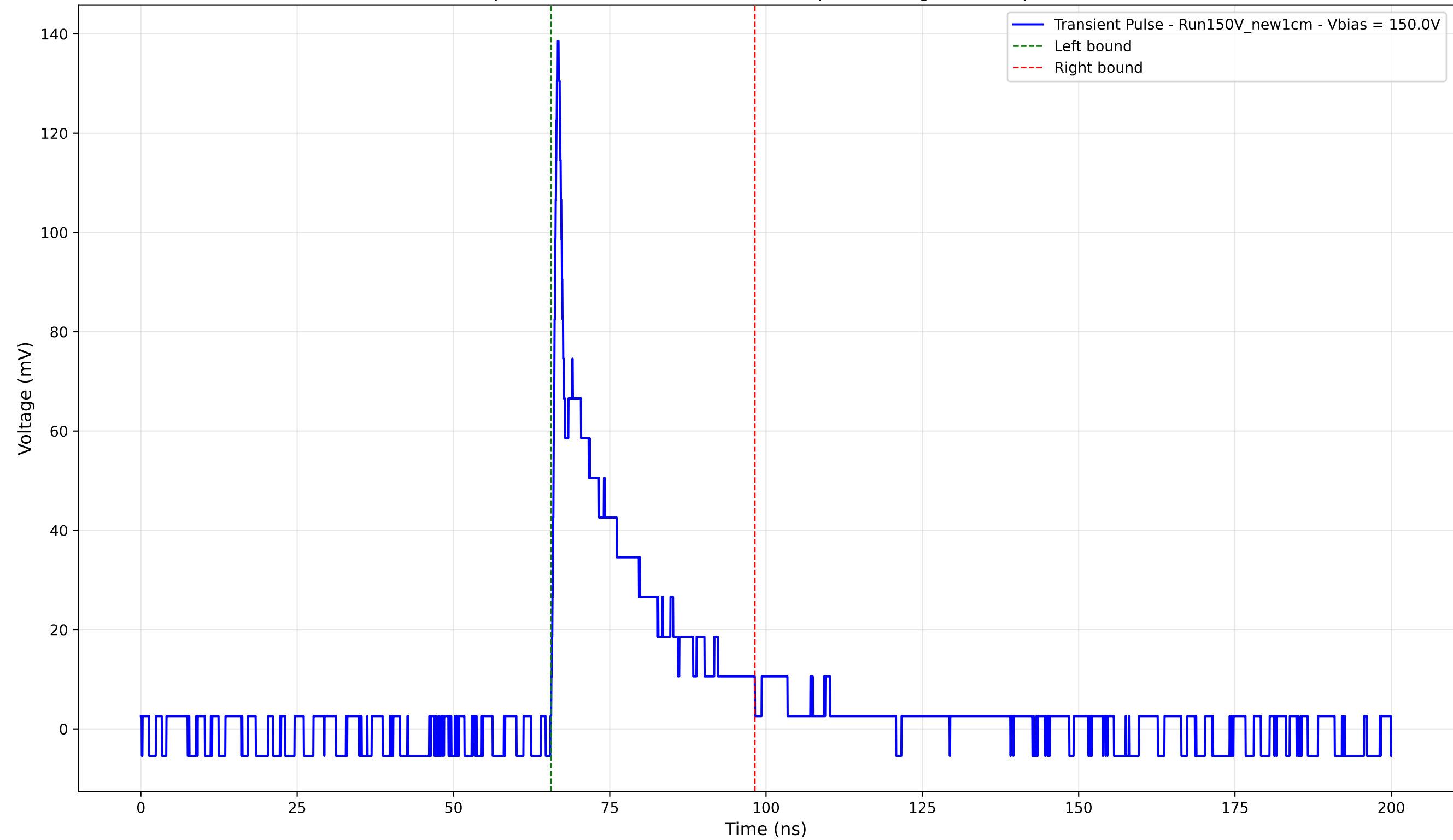
Transient Pulse - Sample: New1cm - Position: 2485.0 \mu\text{m} - Charge: 21.40 pC - Rise Time: 0.81 ns
