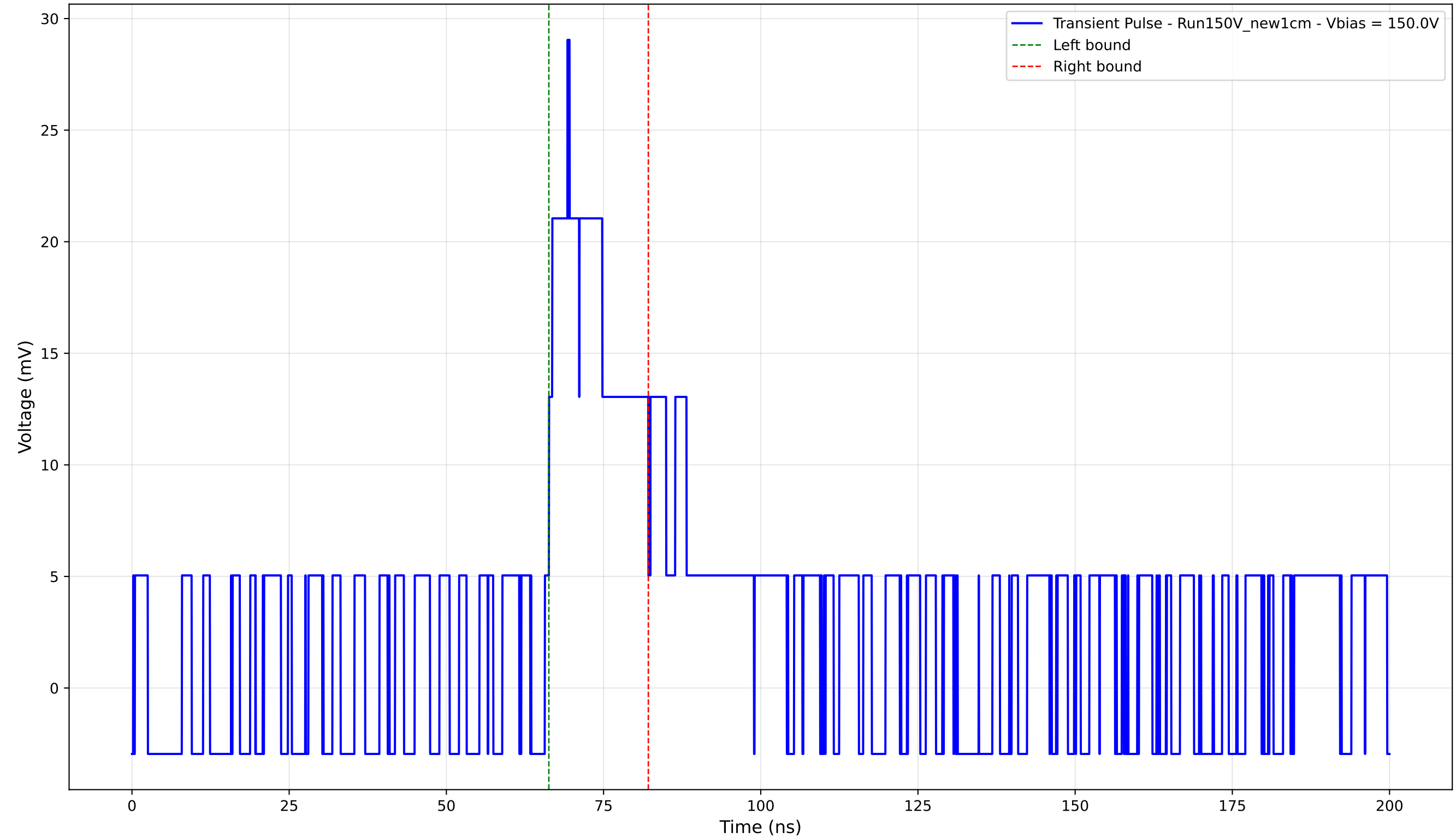
Transient Pulse - Sample: New1cm - Position: 3575.0 \mu\text{m} - Charge: 5.43 pC - Rise Time: 0.00 ns (N/A)
