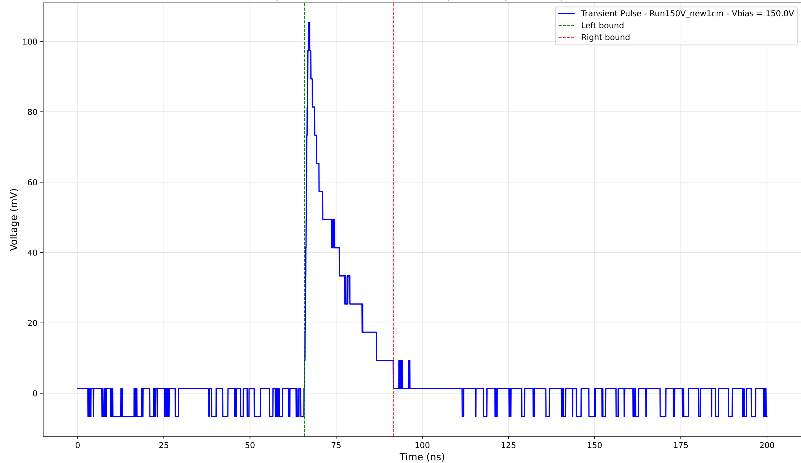
Transient Pulse - Sample: New1cm - Position: 115.0 \mu\text{m} - Charge: 18.12 pC - Rise Time: 0.84 ns
