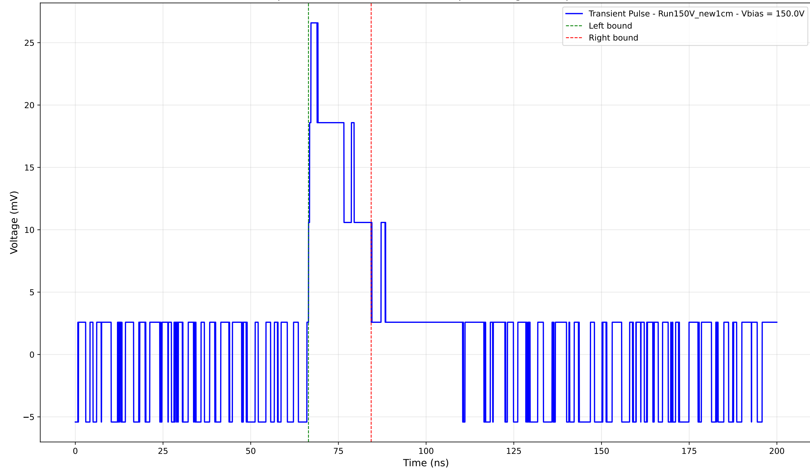
Transient Pulse - Sample: New1cm - Position: 4050.0 \mu\text{m} - Charge: 5.77 pC - Rise Time: 0.70 ns
