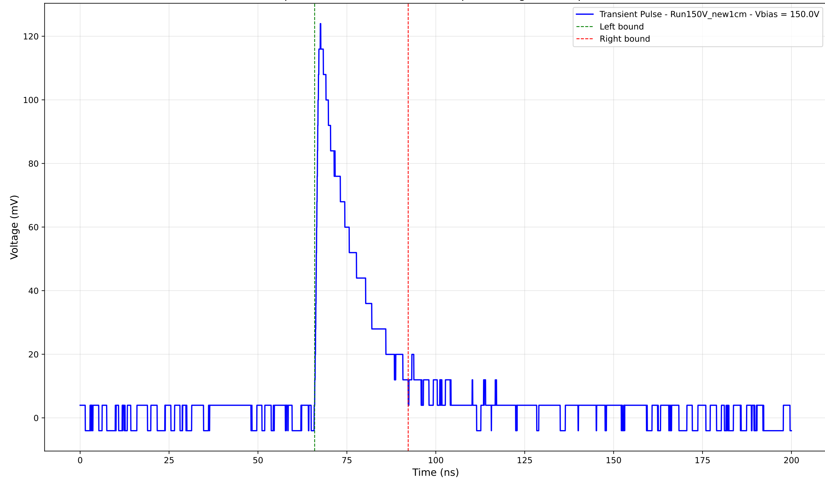
Transient Pulse - Sample: New1cm - Position: 410.0 \mu\text{m} - Charge: 26.04 pC - Rise Time: 1.06 ns
