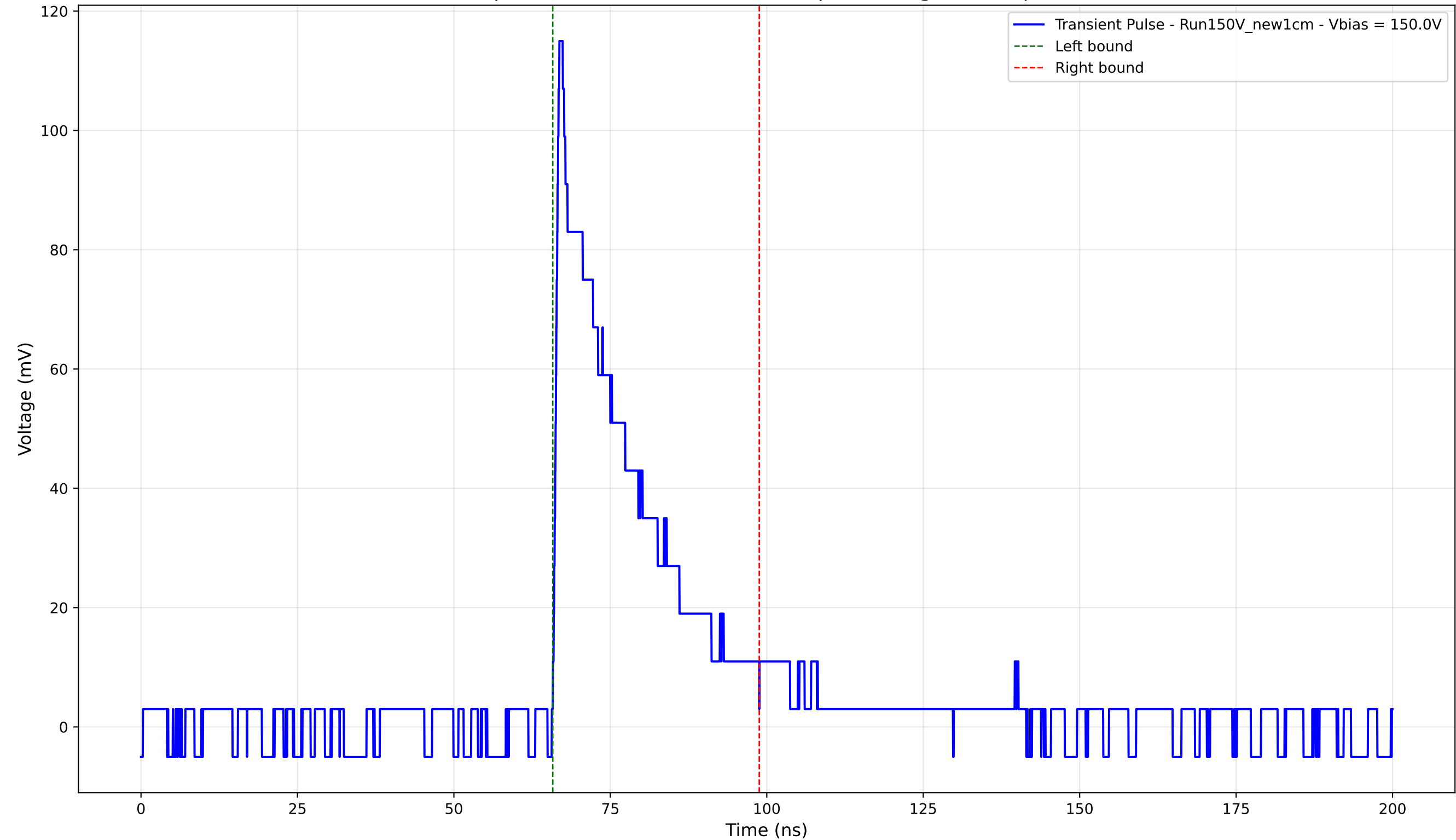
Transient Pulse - Sample: New1cm - Position: 2990.0 \mu\text{m} - Charge: 26.00 pC - Rise Time: 0.80 ns
