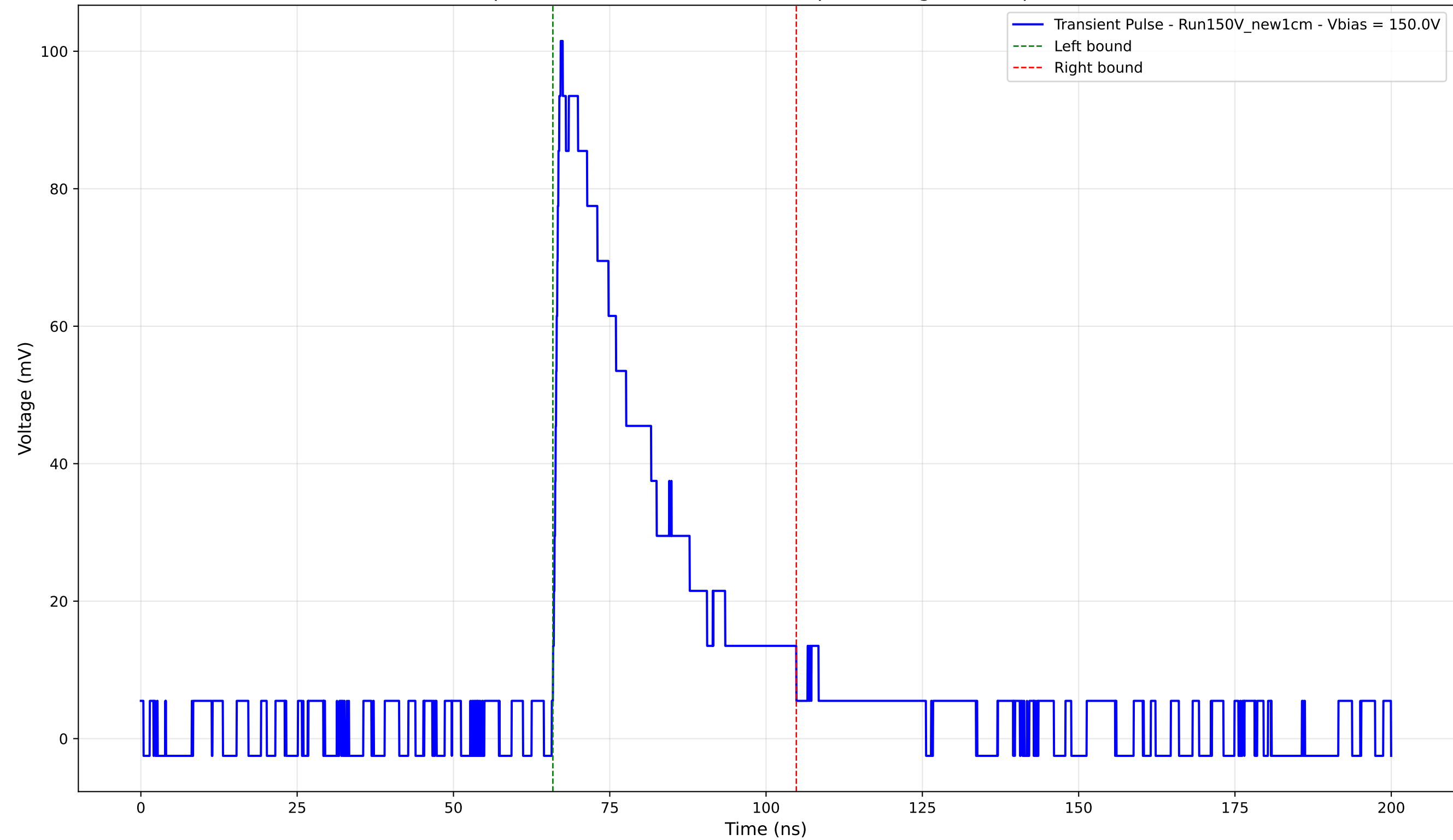
Transient Pulse - Sample: New1cm - Position: 1915.0 \mu\text{m} - Charge: 30.09 pC - Rise Time: 1.01 ns
