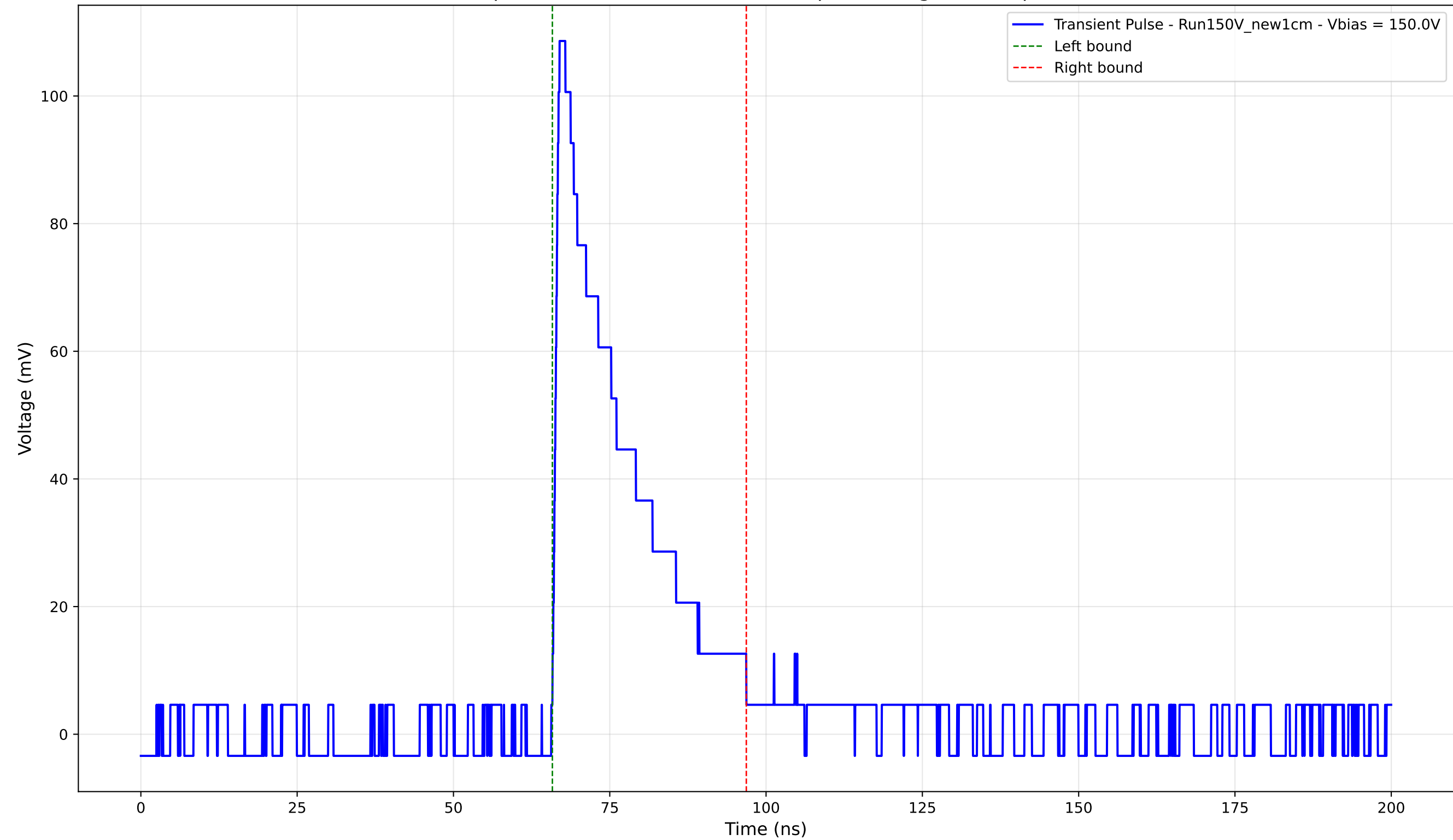
Transient Pulse - Sample: New1cm - Position: 4645.0 \mu\text{m} - Charge: 25.43 pC - Rise Time: 0.96 ns
