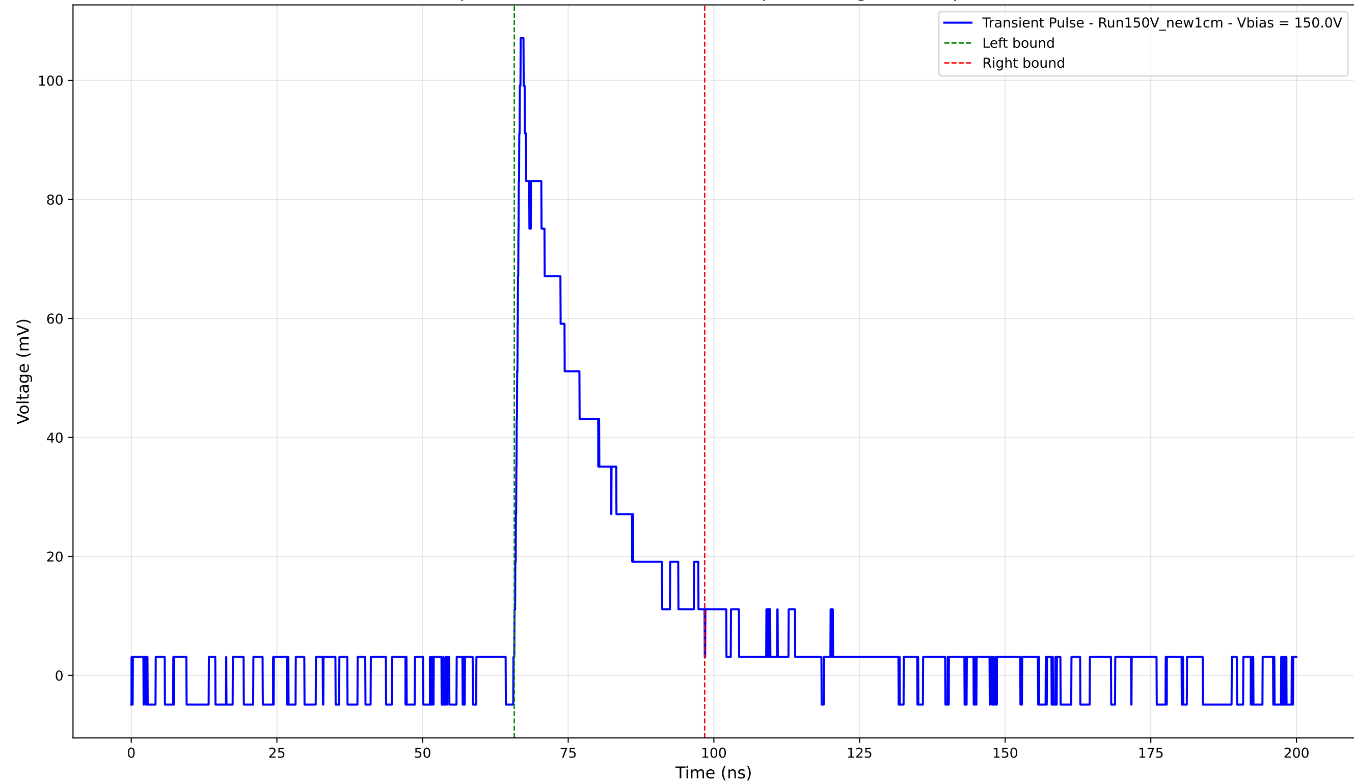
Transient Pulse - Sample: New1cm - Position: 2130.0 \mu\text{m} - Charge: 25.74 pC - Rise Time: 0.92 ns
