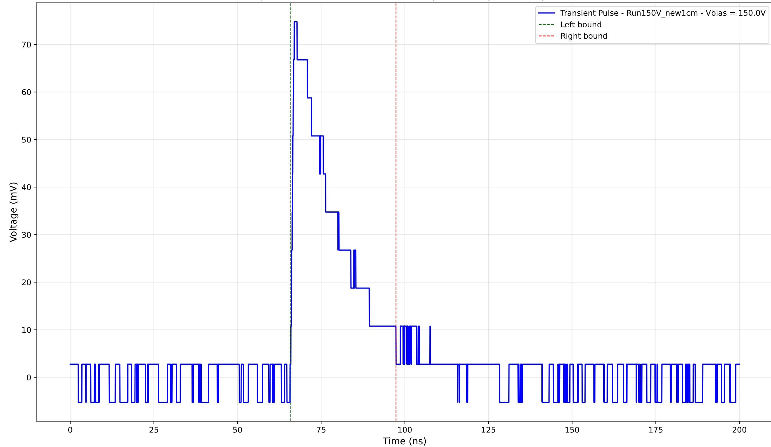
Transient Pulse - Sample: New1cm - Position: 1970.0 \mu\text{m} - Charge: 20.33 pC - Rise Time: 1.01 ns
