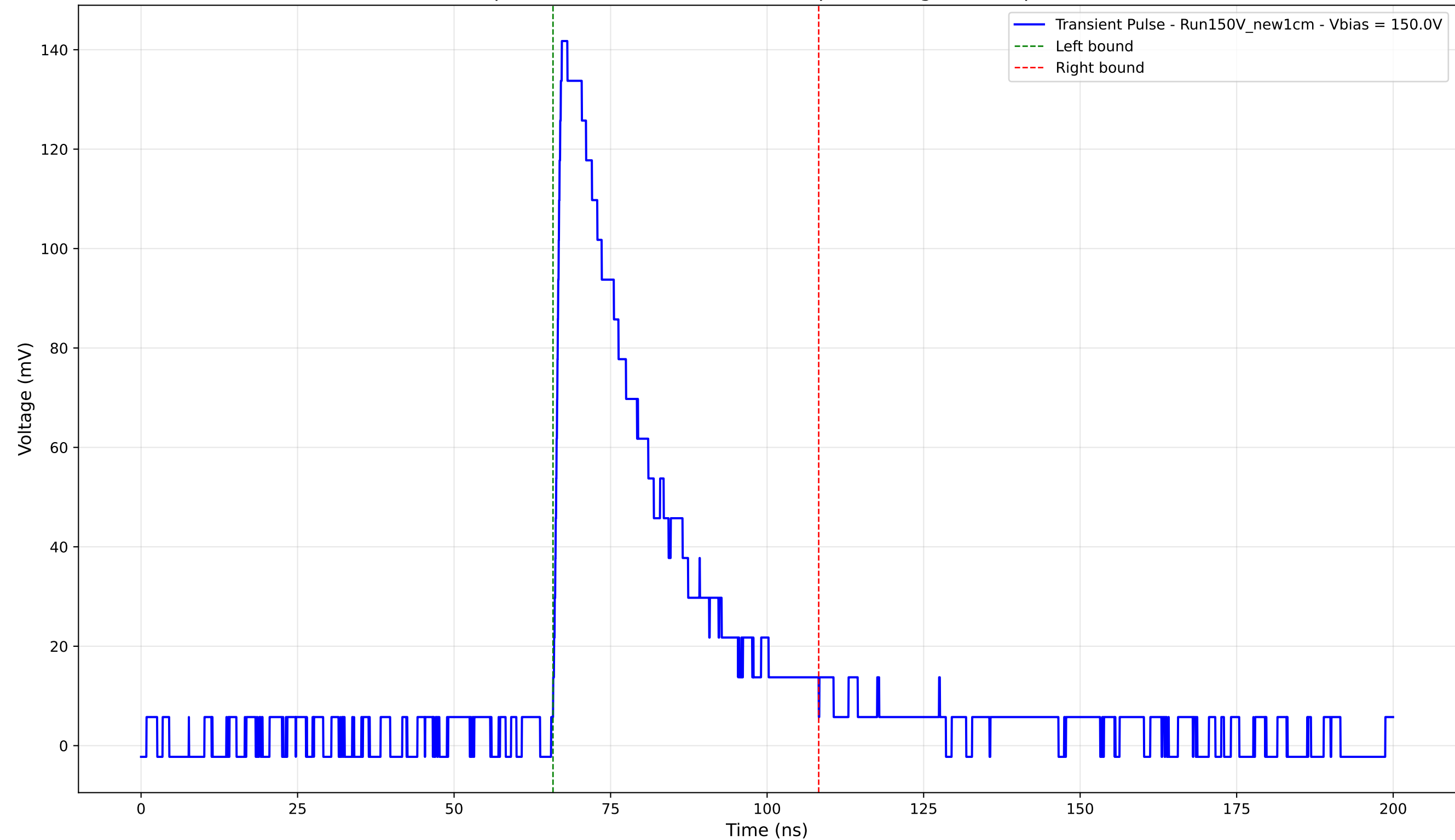
Transient Pulse - Sample: New1cm - Position: 3240.0 \mu\text{m} - Charge: 43.64 pC - Rise Time: 1.10 ns
