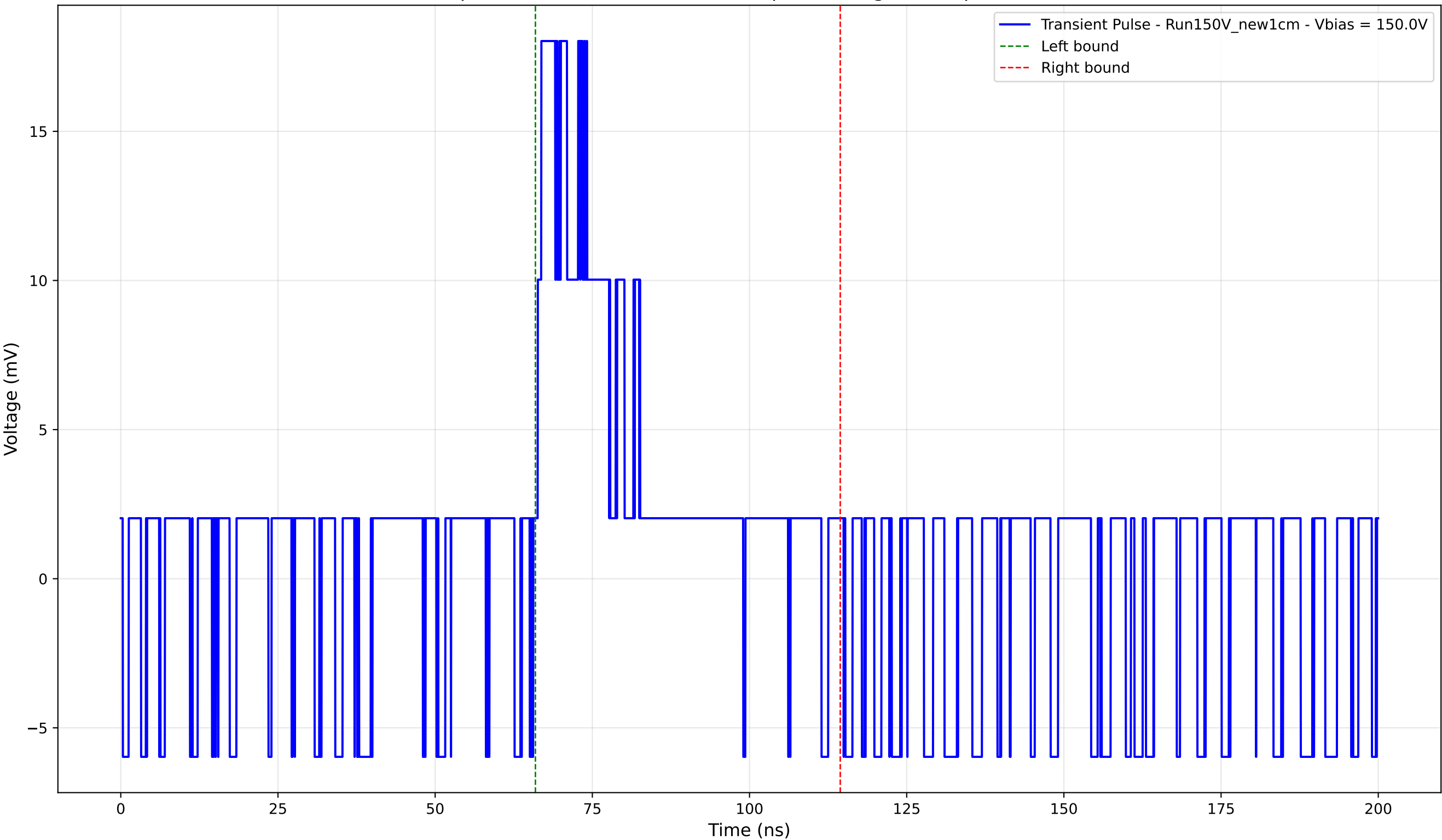
Transient Pulse - Sample: New1cm - Position: 540.0 \mu\text{m} - Charge: 4.64 pC - Rise Time: 0.00 ns (N/A)
