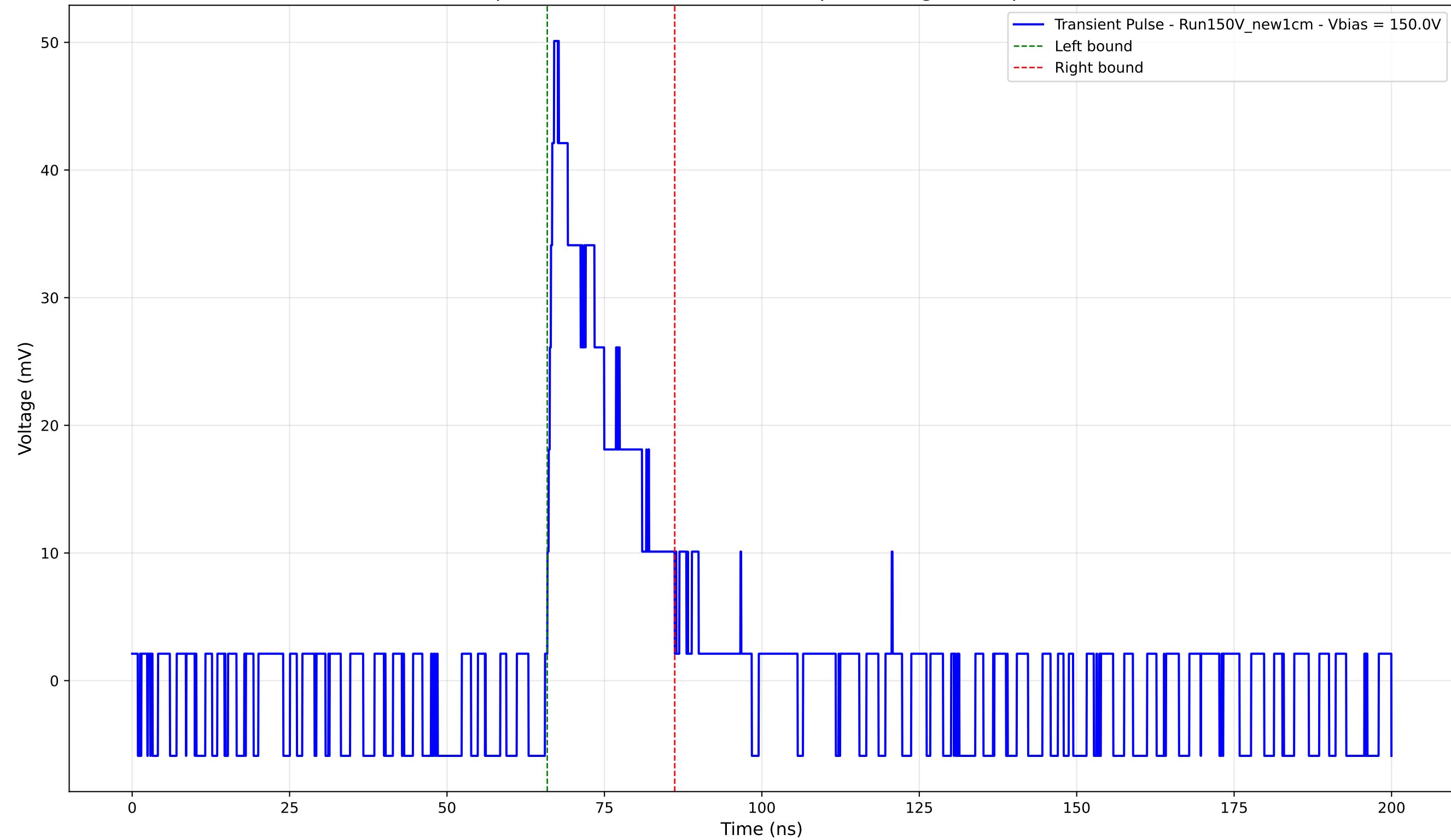
Transient Pulse - Sample: New1cm - Position: 4605.0 \mu\text{m} - Charge: 9.46 pC - Rise Time: 1.07 ns
