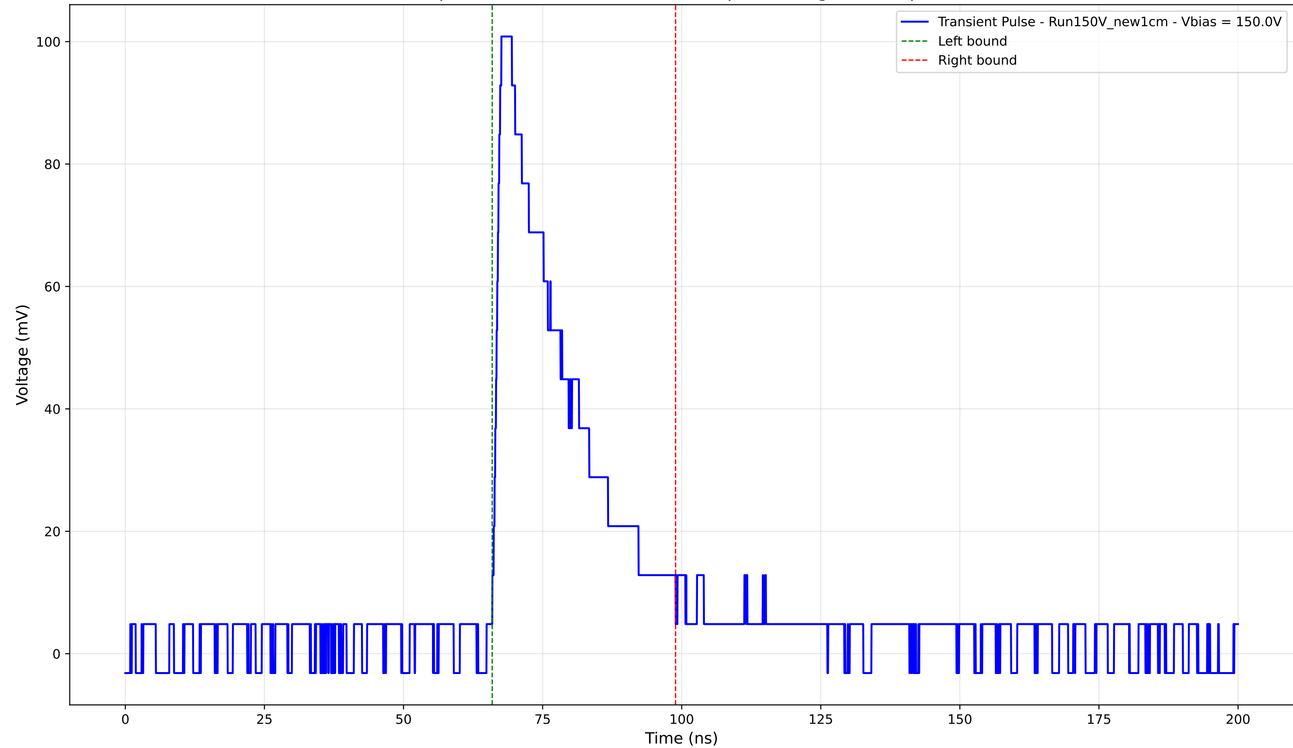
Transient Pulse - Sample: New1cm - Position: 4155.0 \mu\text{m} - Charge: 27.82 pC - Rise Time: 1.41 ns
