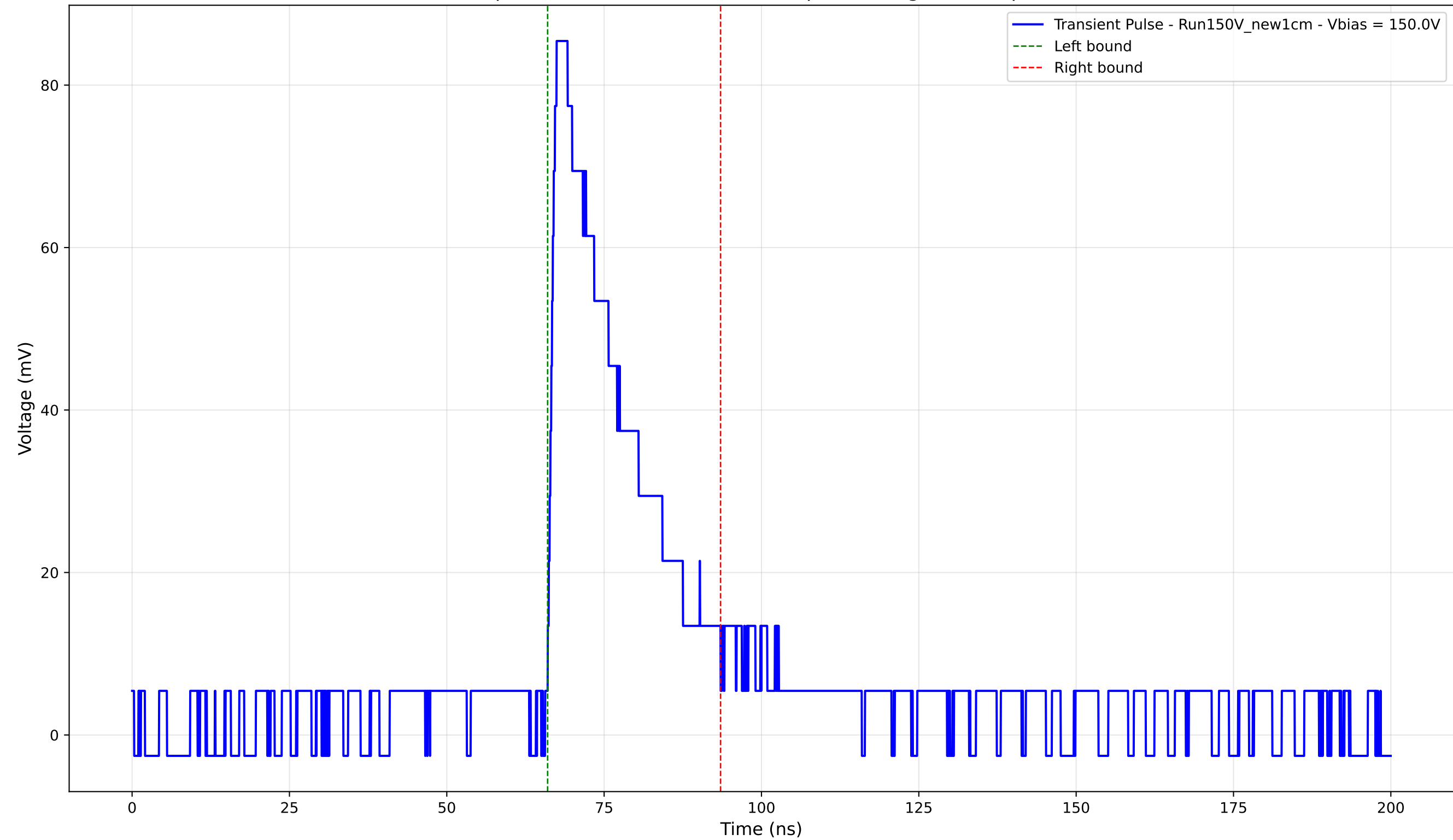
Transient Pulse - Sample: New1cm - Position: 605.0 \mu\text{m} - Charge: 21.61 pC - Rise Time: 1.15 ns
