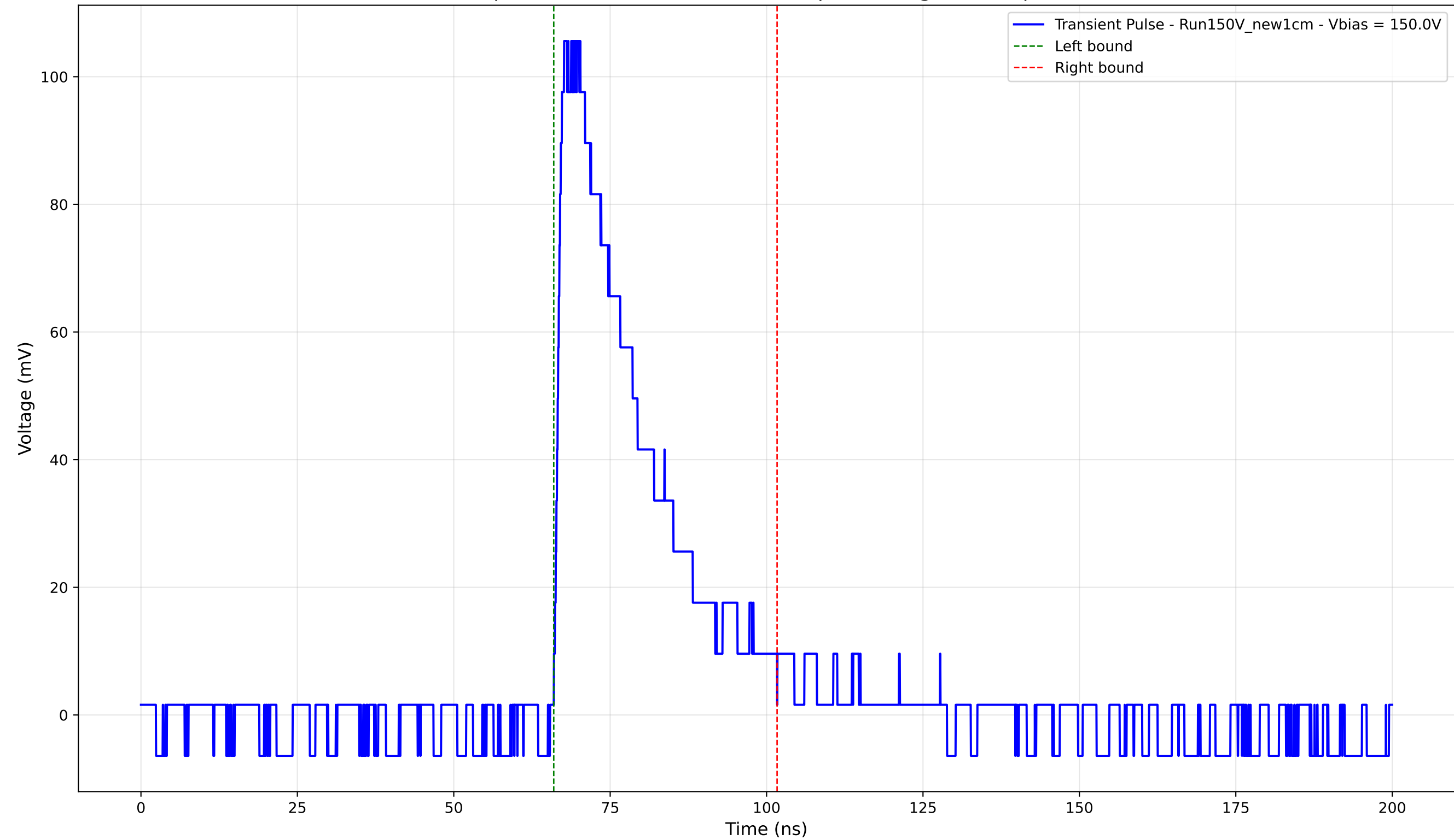
Transient Pulse - Sample: New1cm - Position: 1715.0 \mu\text{m} - Charge: 29.82 pC - Rise Time: 1.14 ns
