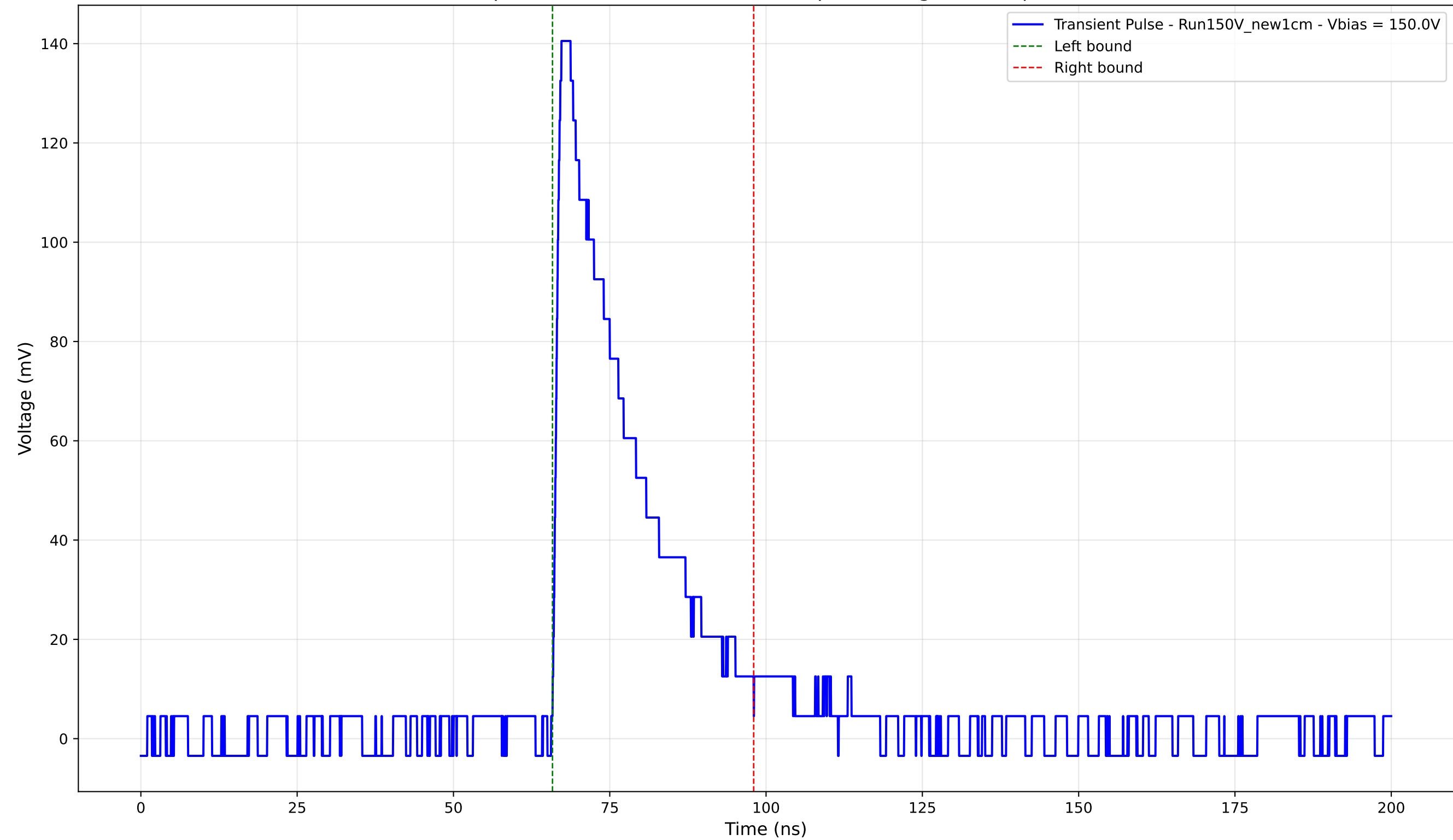
Transient Pulse - Sample: New1cm - Position: 4475.0 \mu\text{m} - Charge: 35.78 pC - Rise Time: 1.14 ns
