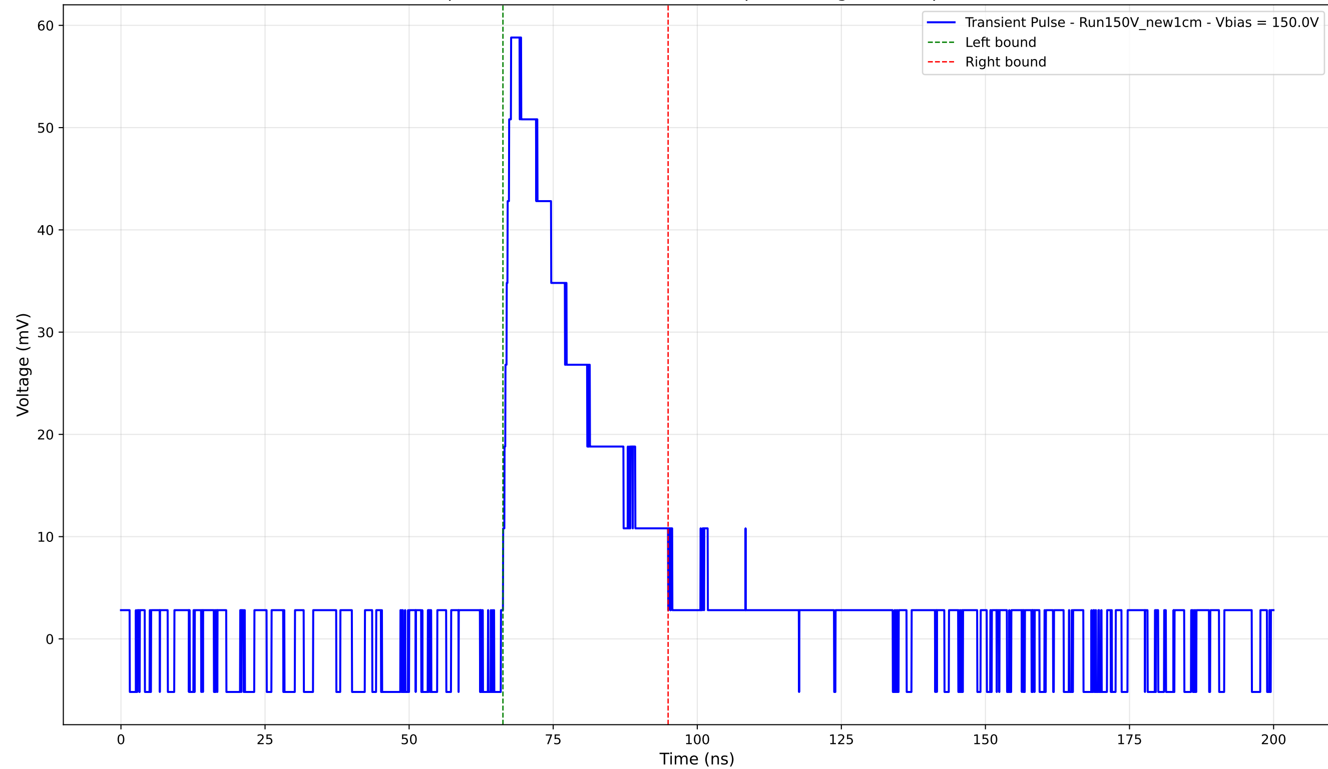
Transient Pulse - Sample: New1cm - Position: 3605.0 \mu\text{m} - Charge: 15.83 pC - Rise Time: 1.39 ns
