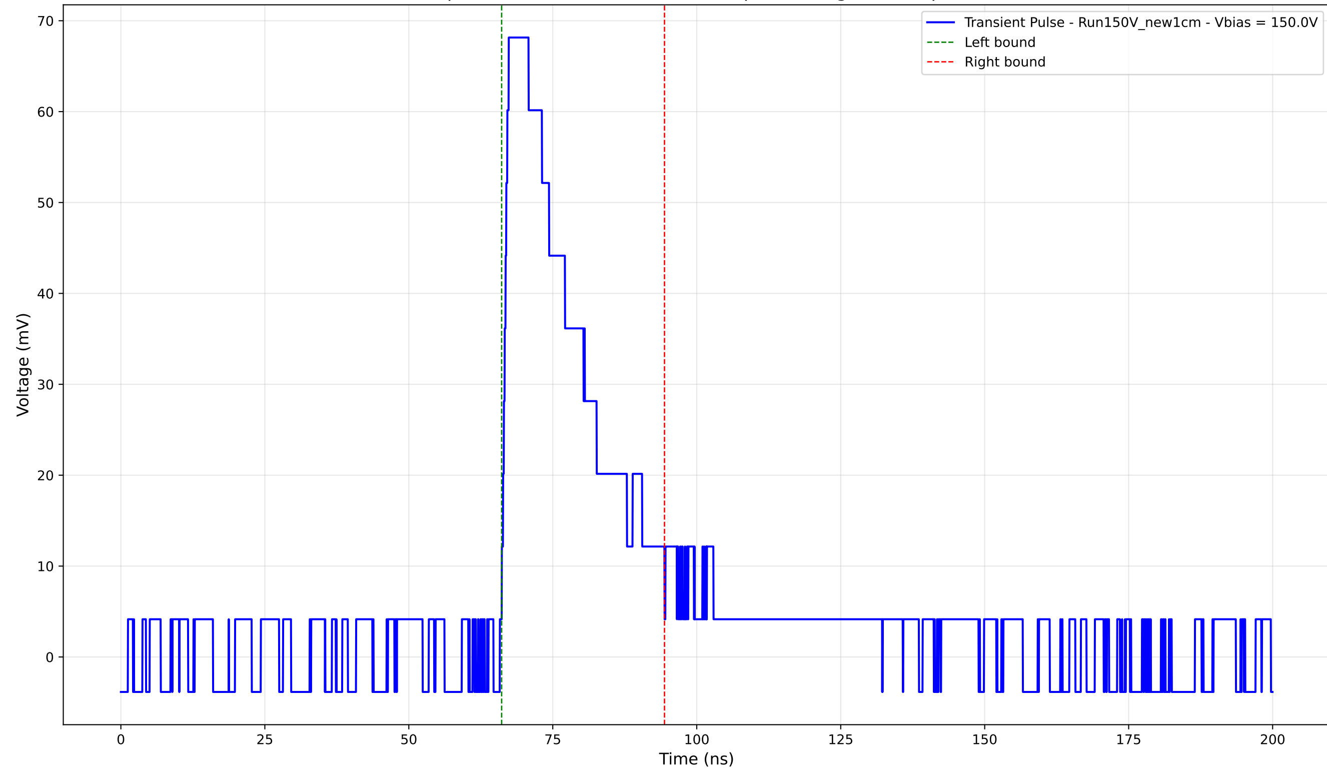
Transient Pulse - Sample: New1cm - Position: 3510.0 \mu\text{m} - Charge: 19.72 pC - Rise Time: 1.21 ns
