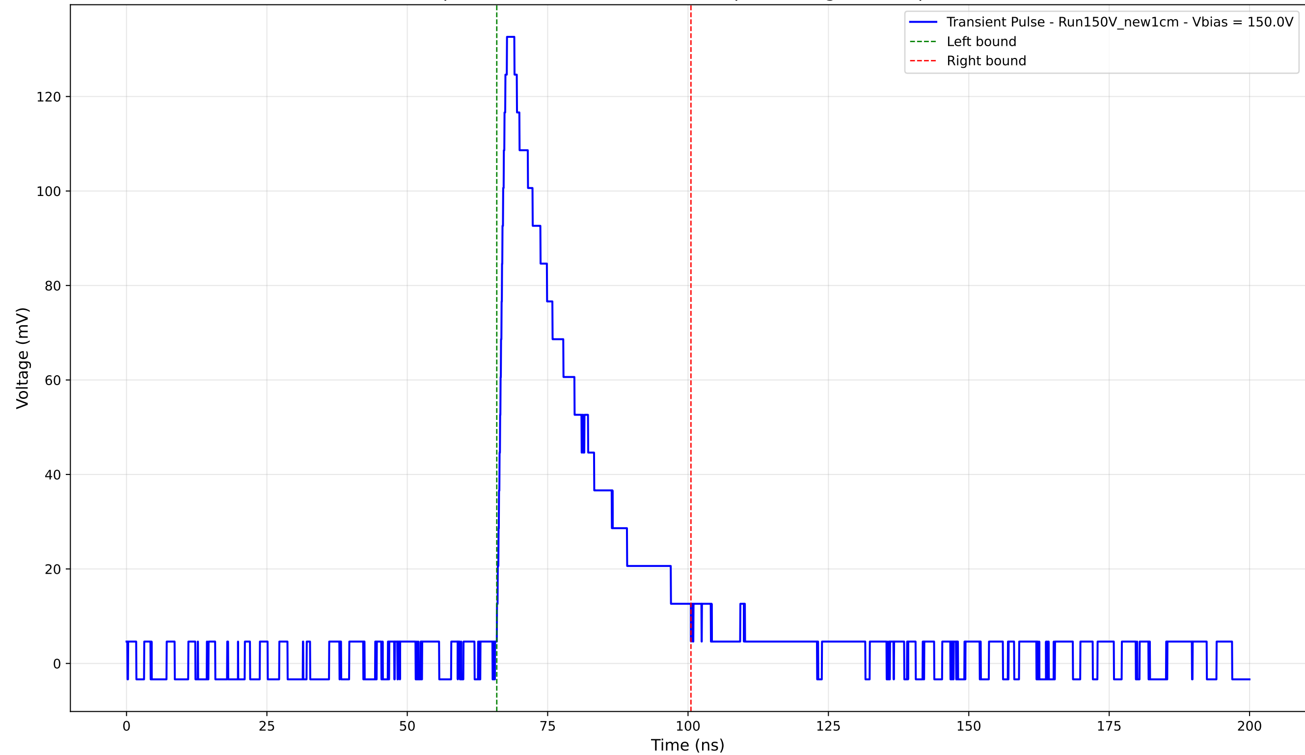
Transient Pulse - Sample: New1cm - Position: 4200.0 \mu\text{m} - Charge: 35.91 pC - Rise Time: 1.38 ns
