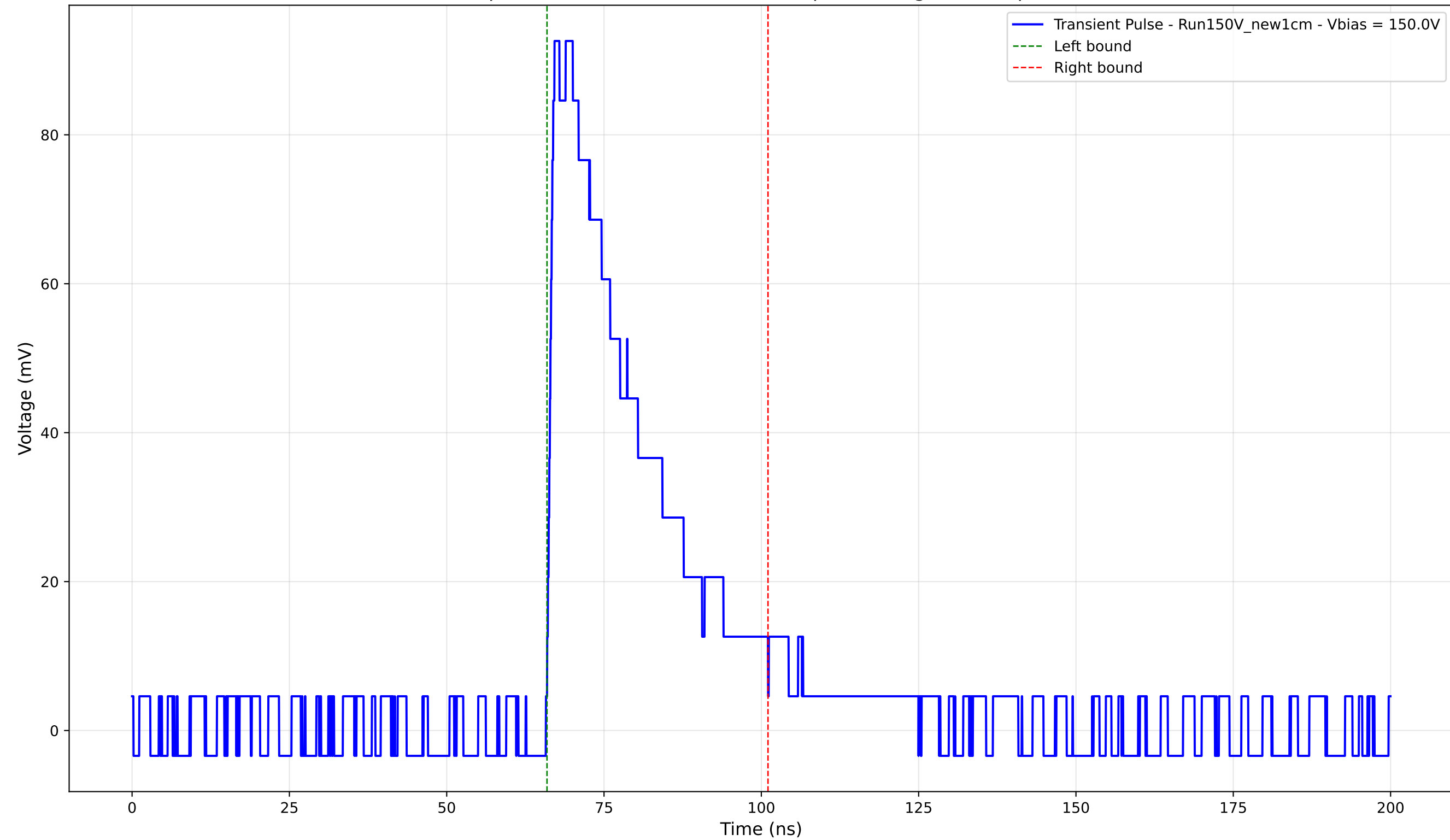
Transient Pulse - Sample: New1cm - Position: 1880.0 \mu\text{m} - Charge: 28.27 pC - Rise Time: 0.97 ns
