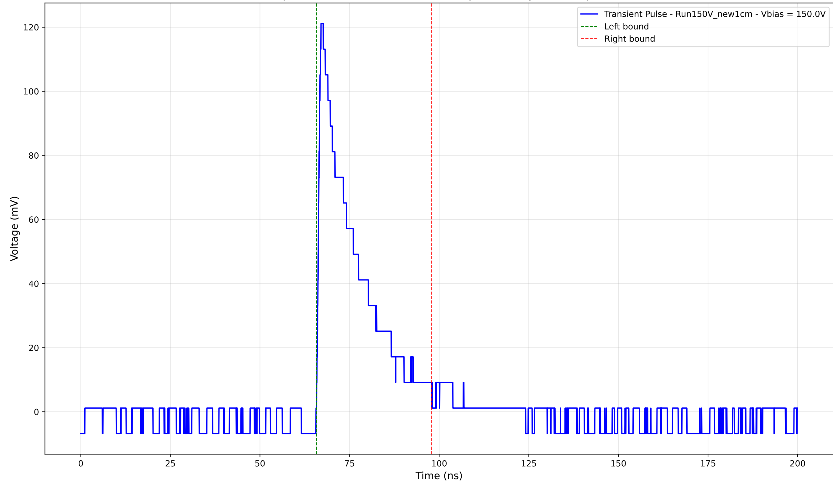
Transient Pulse - Sample: New1cm - Position: 4665.0 \mu\text{m} - Charge: 26.15 pC - Rise Time: 0.97 ns
