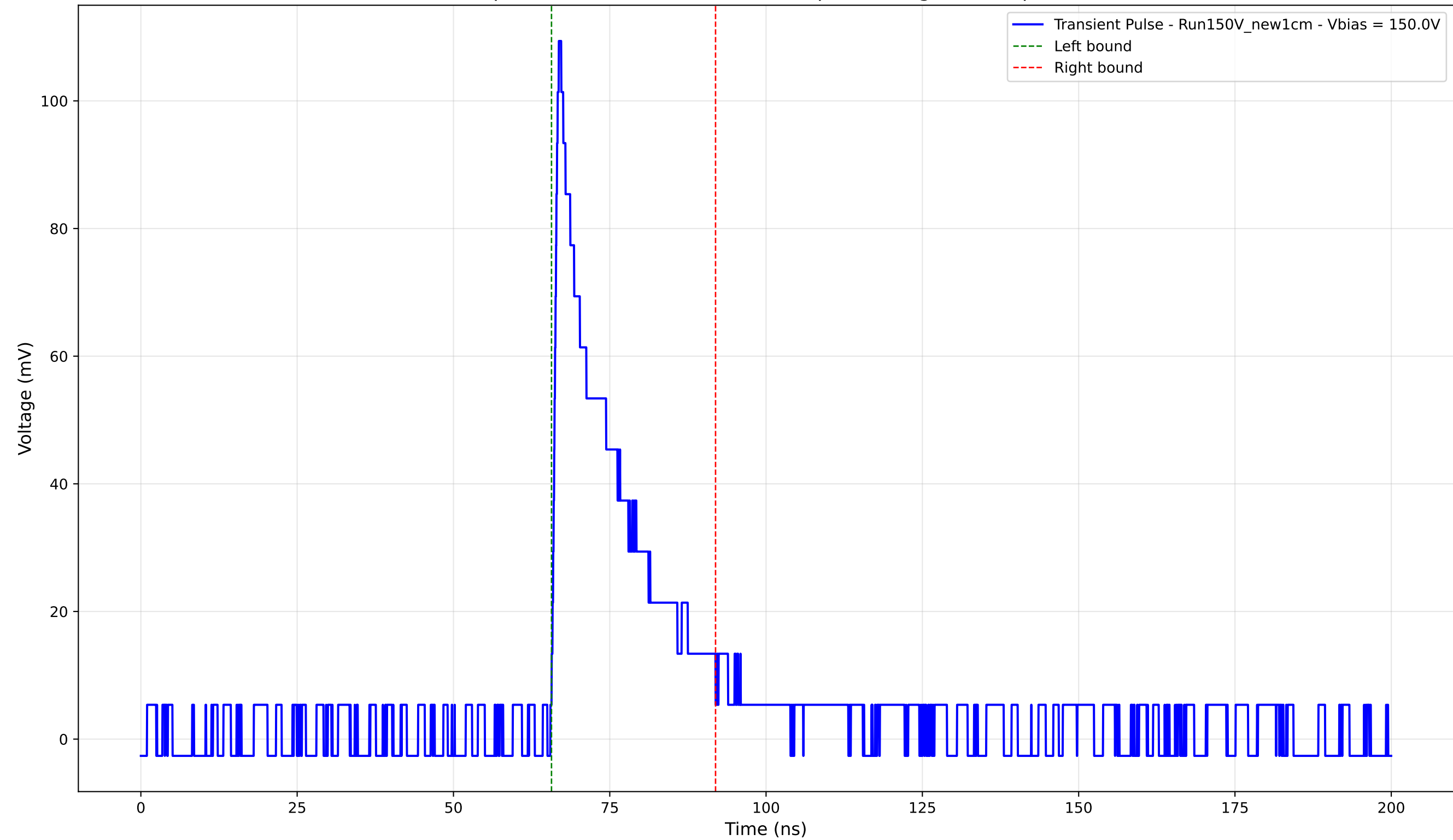
Transient Pulse - Sample: New1cm - Position: 4835.0 \mu\text{m} - Charge: 20.45 pC - Rise Time: 0.97 ns
