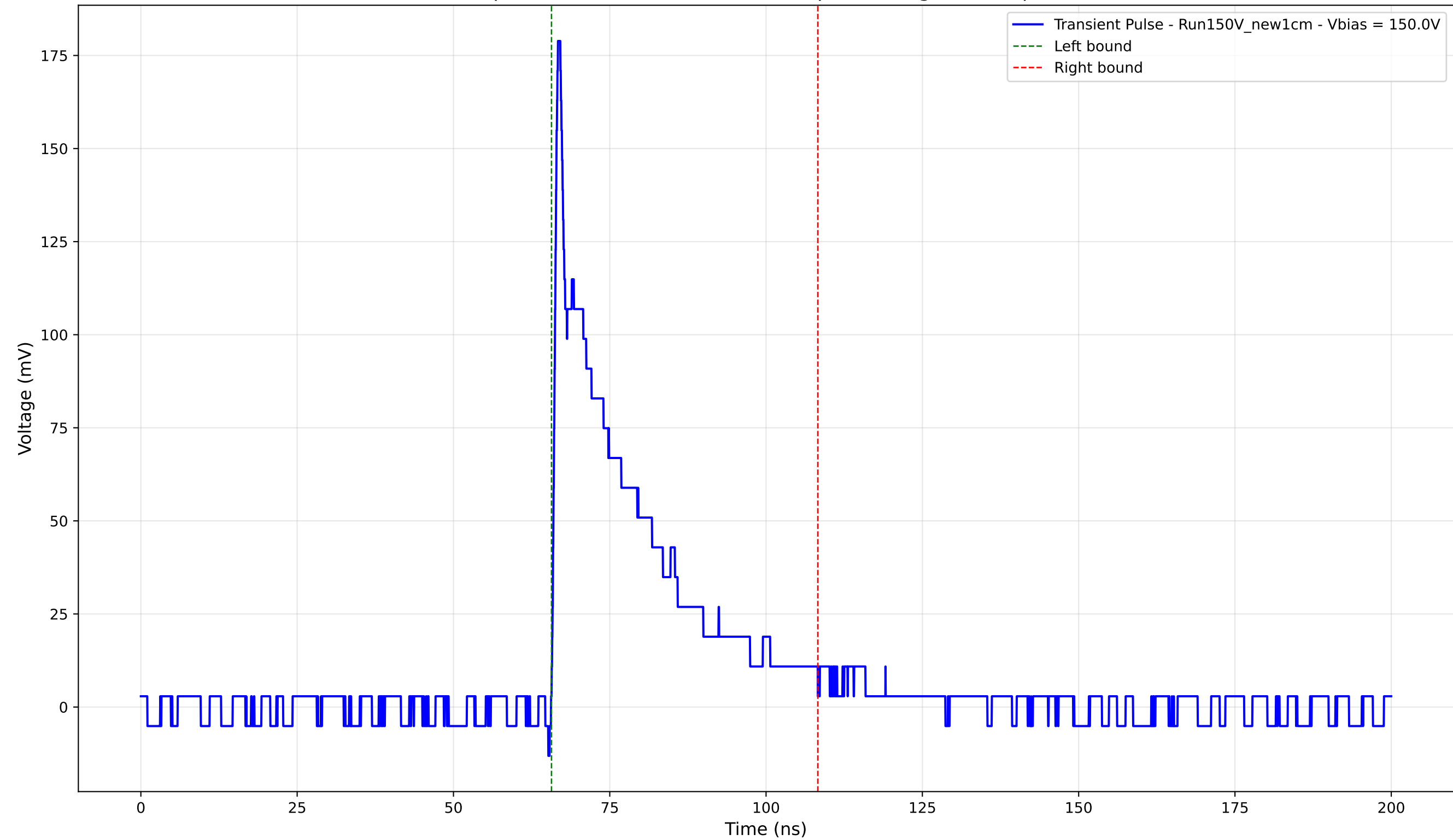
Transient Pulse - Sample: New1cm - Position: 2790.0 \mu\text{m} - Charge: 37.48 pC - Rise Time: 0.78 ns
