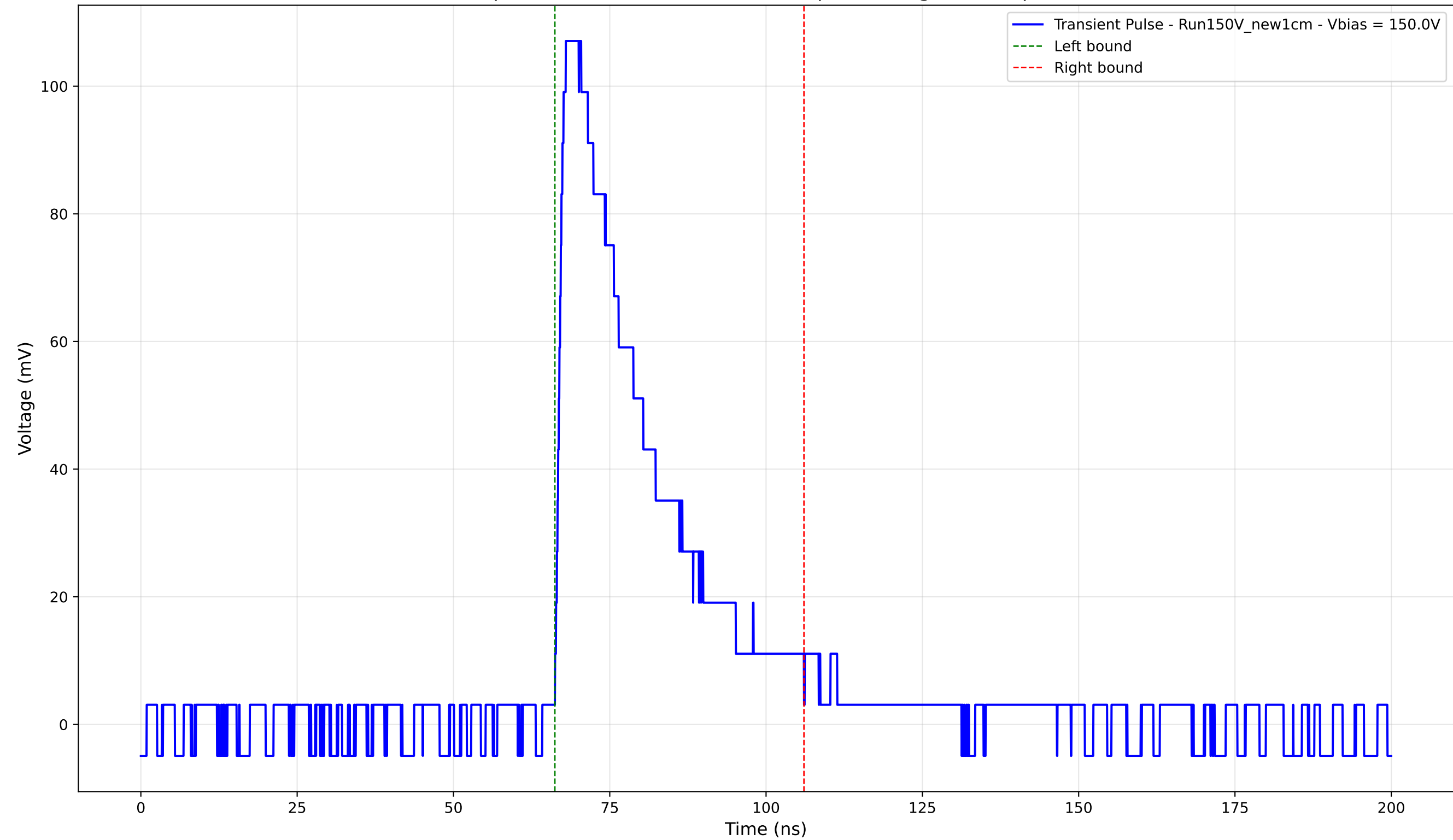
Transient Pulse - Sample: New1cm - Position: 1310.0 \mu\text{m} - Charge: 32.68 pC - Rise Time: 1.36 ns
