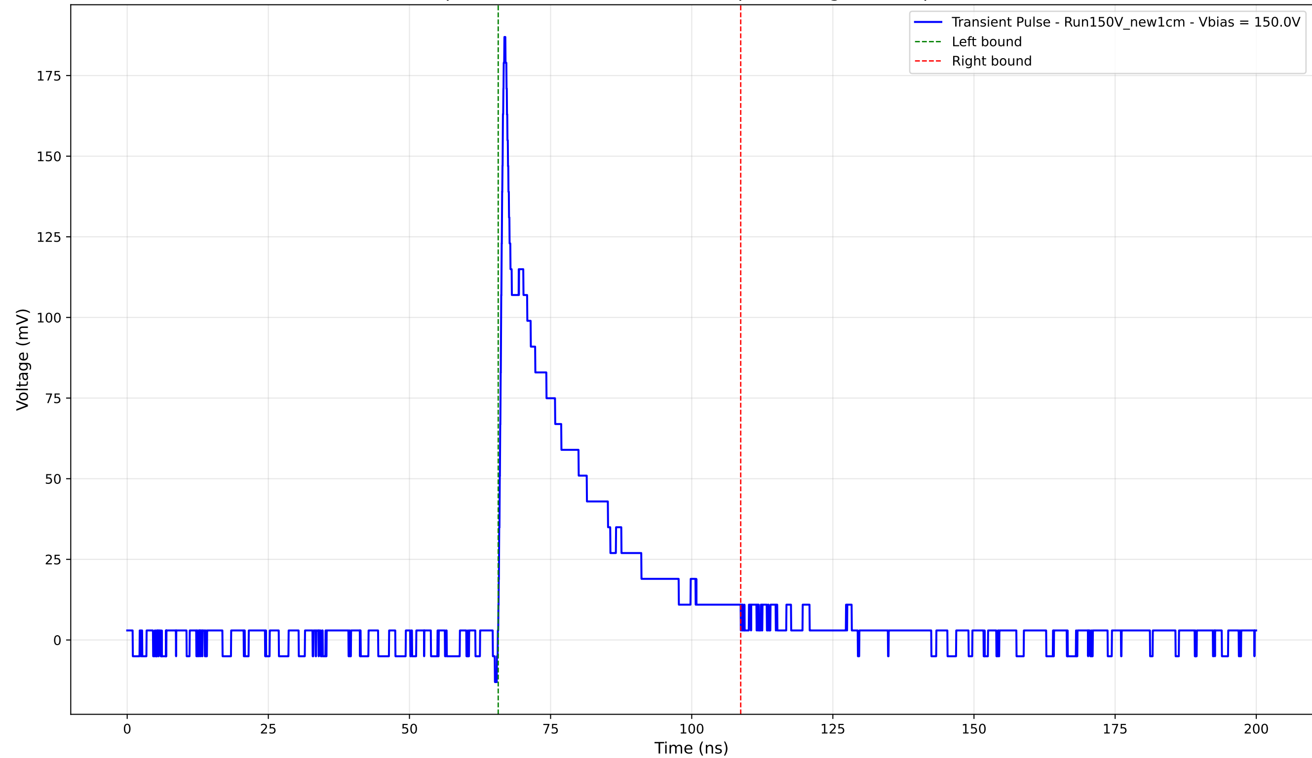
Transient Pulse - Sample: New1cm - Position: 2800.0 \mu\text{m} - Charge: 38.61 pC - Rise Time: 0.82 ns
