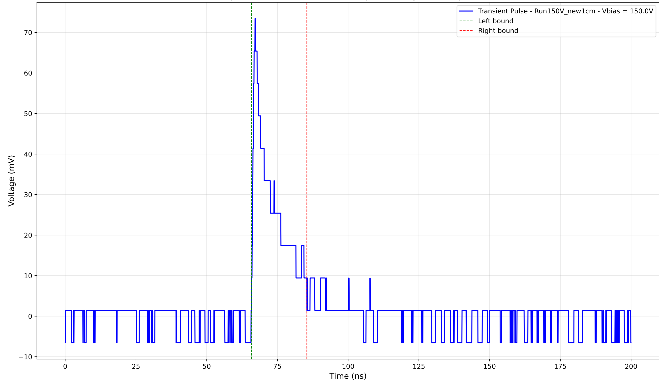
Transient Pulse - Sample: New1cm - Position: 85.0 \mu\text{m} - Charge: 10.45 pC - Rise Time: 1.21 ns
