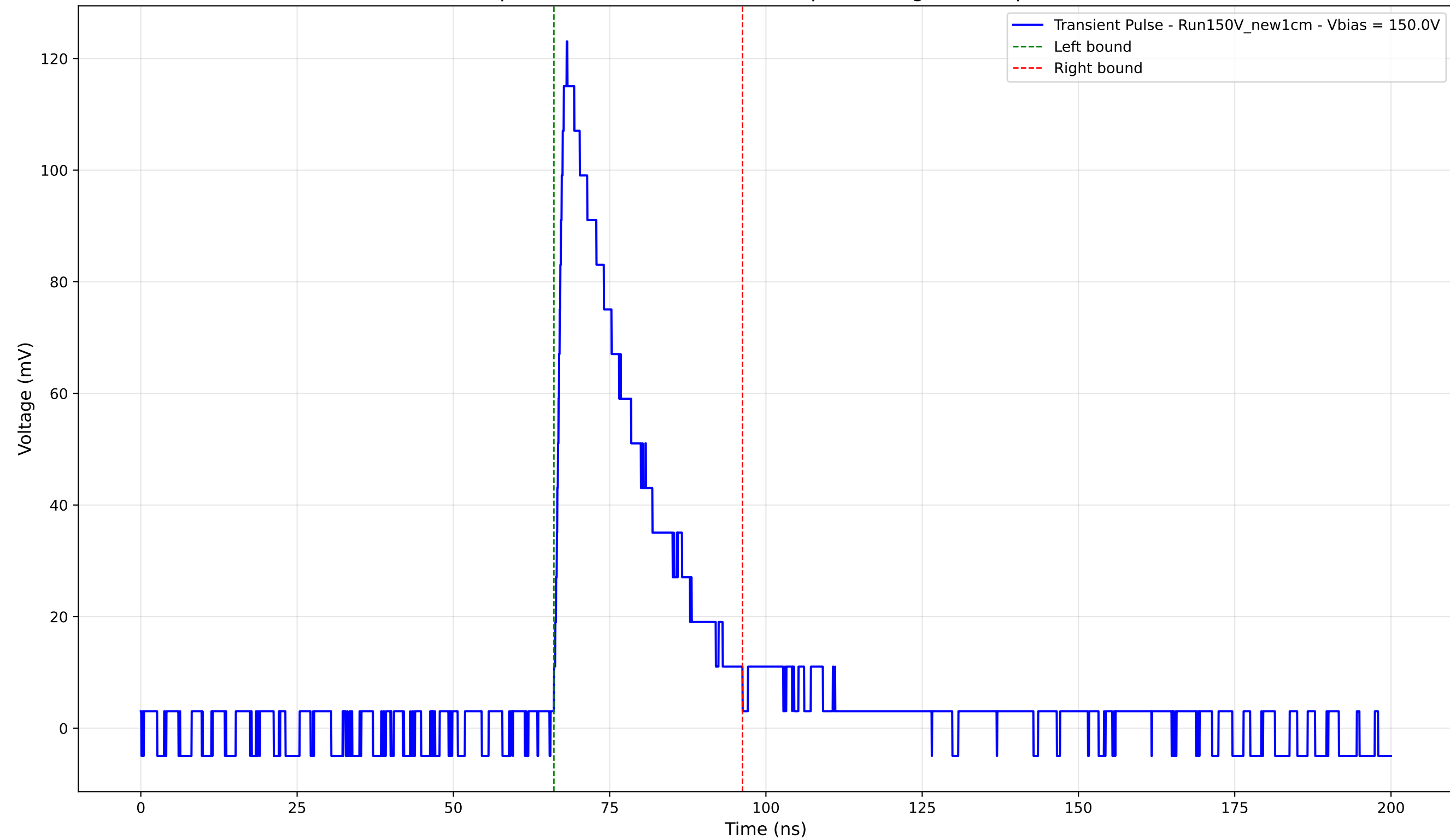
Transient Pulse - Sample: New1cm - Position: 830.0 \mu\text{m} - Charge: 30.16 pC - Rise Time: 1.38 ns
