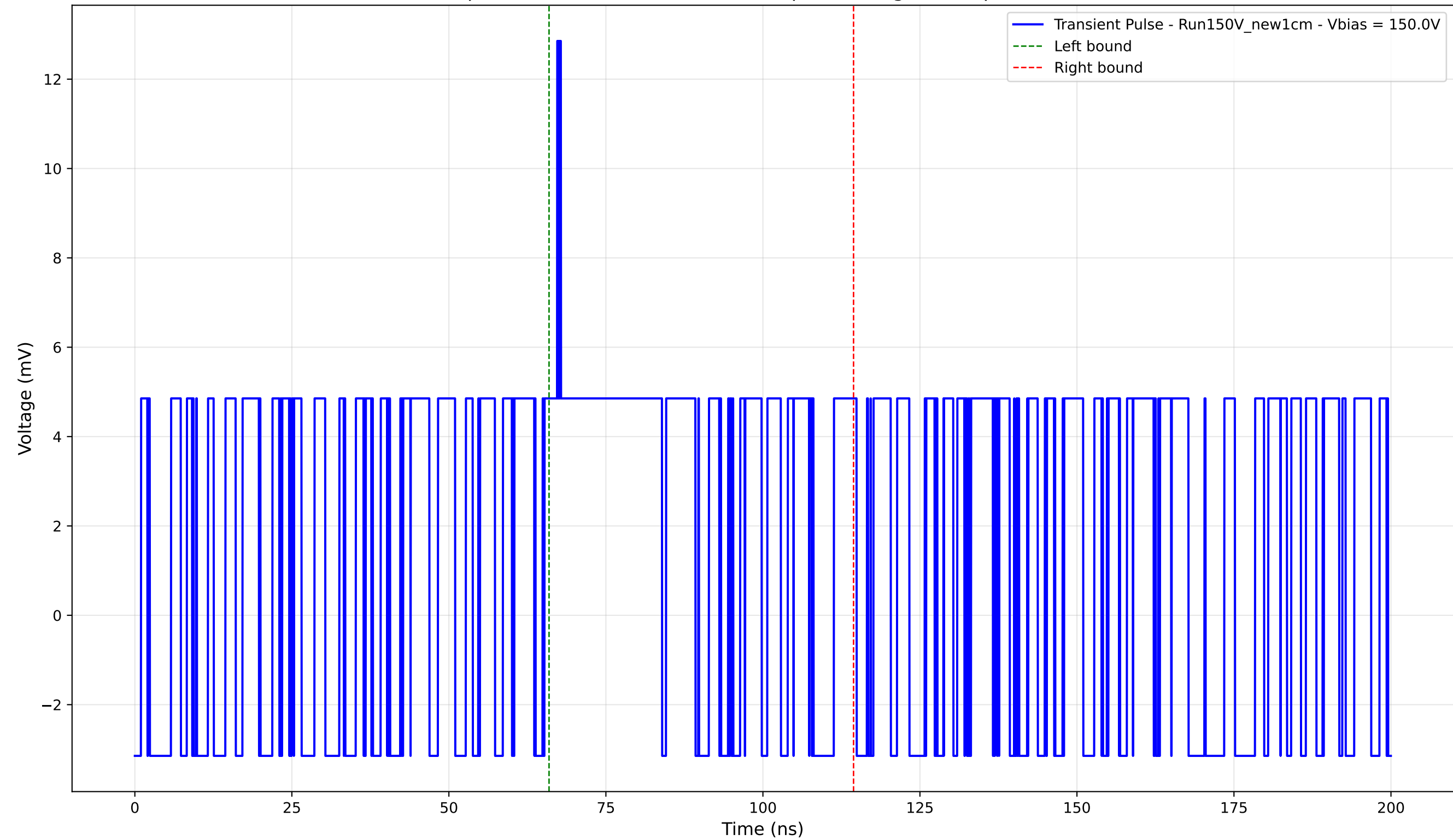
Transient Pulse - Sample: New1cm - Position: 4910.0 \mu\text{m} - Charge: 3.03 pC - Rise Time: 0.00 ns (N/A)
