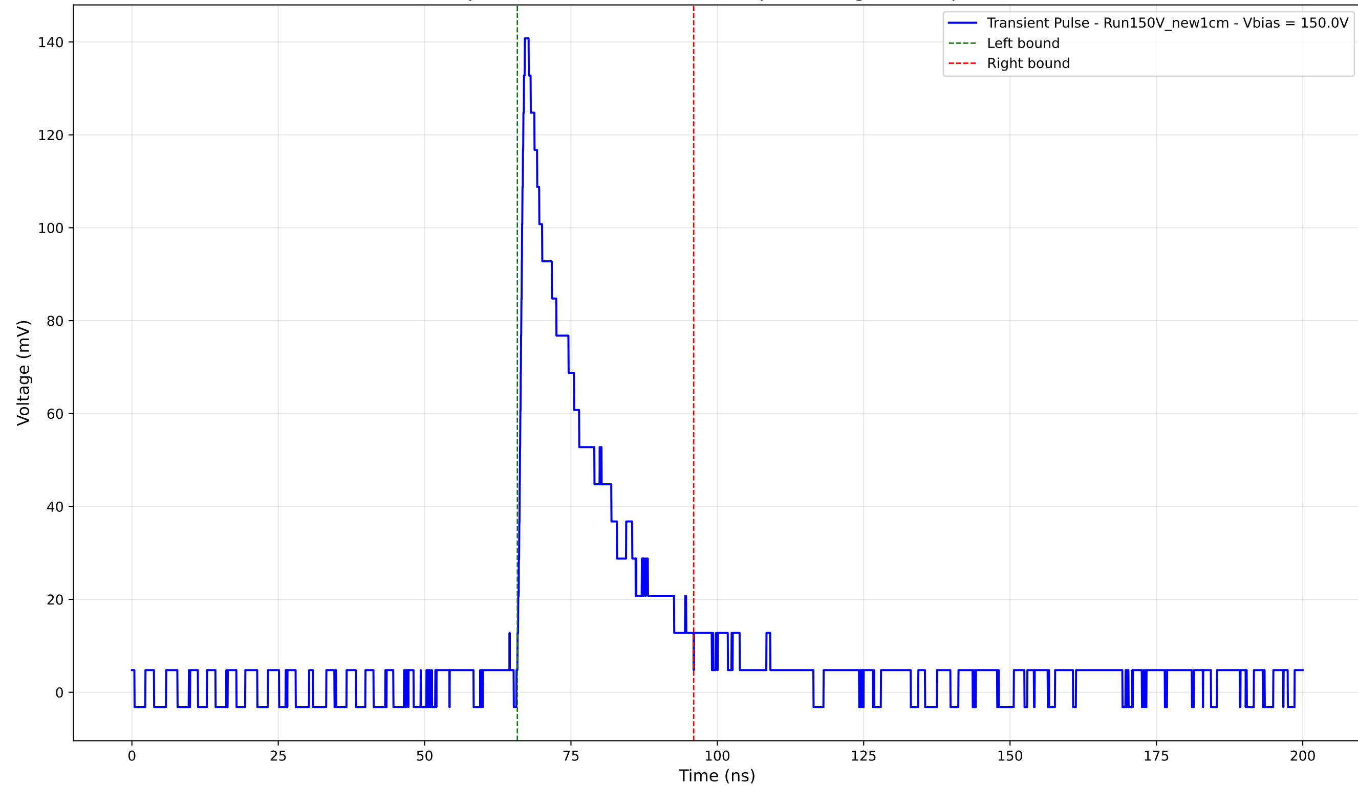
Transient Pulse - Sample: New1cm - Position: 305.0 \mu\text{m} - Charge: 30.88 pC - Rise Time: 1.00 ns
