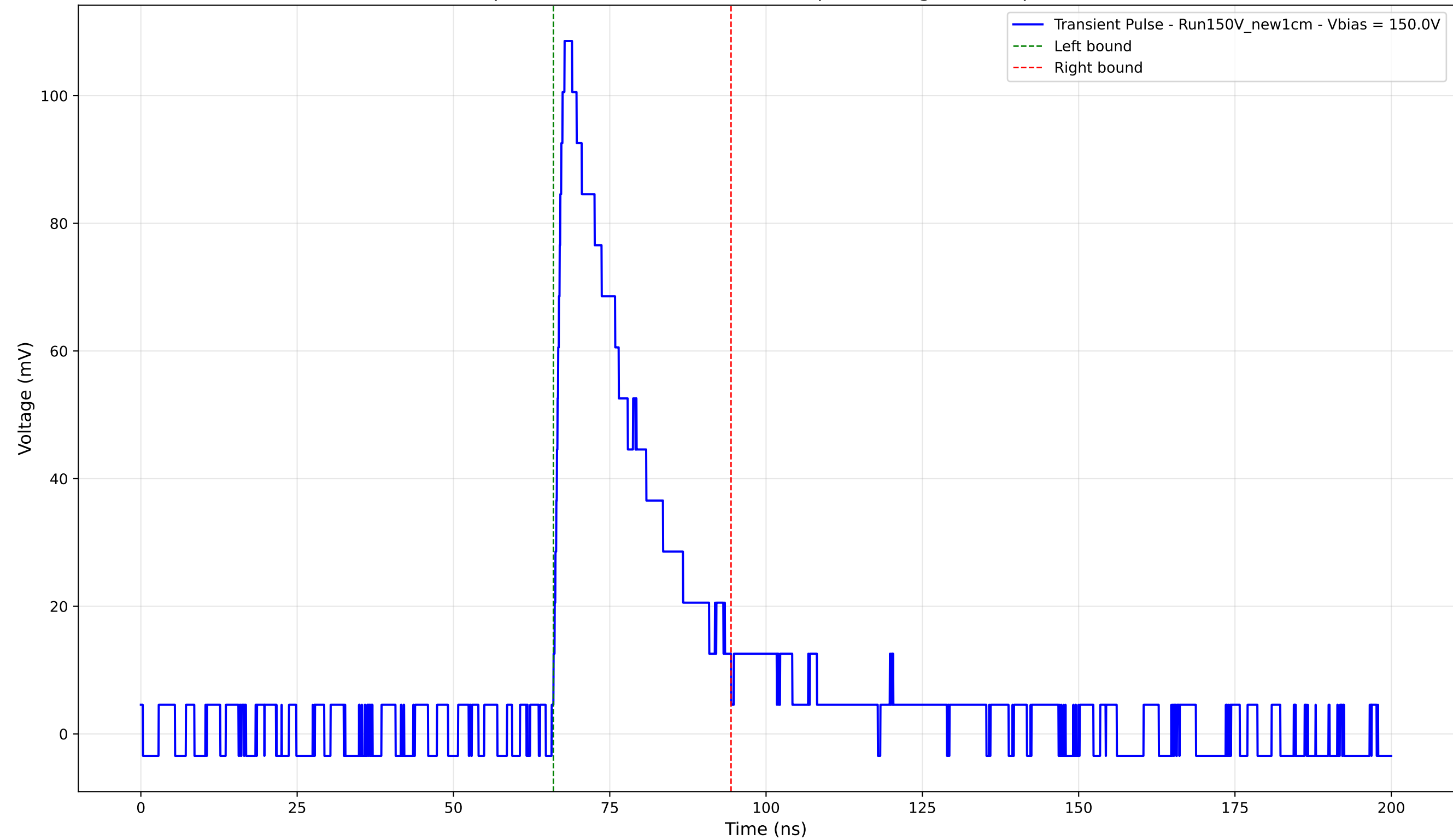
Transient Pulse - Sample: New1cm - Position: 4170.0 \mu\text{m} - Charge: 27.49 pC - Rise Time: 1.44 ns
