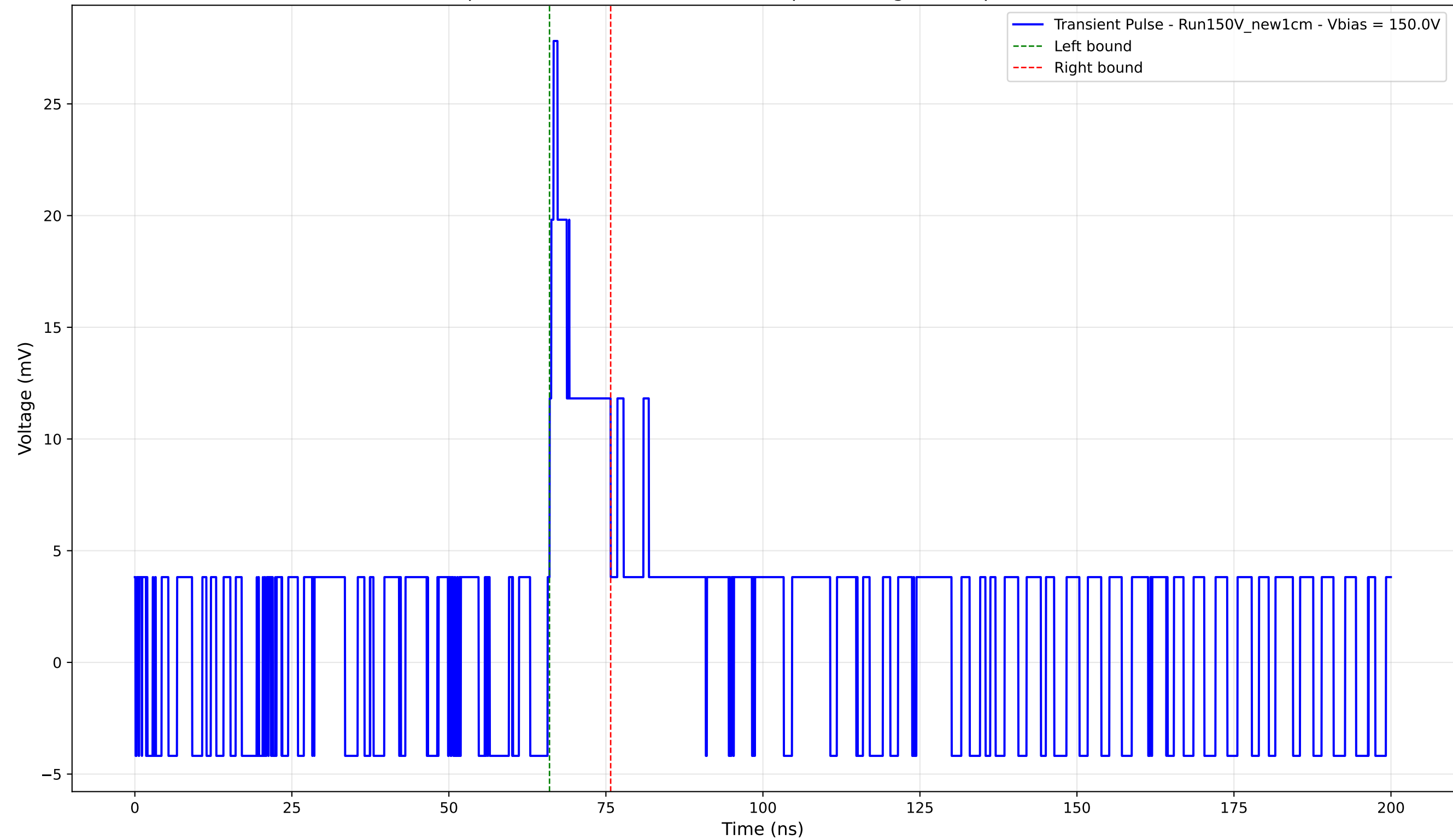
Transient Pulse - Sample: New1cm - Position: 4885.0 \mu\text{m} - Charge: 2.80 pC - Rise Time: 0.00 ns (N/A)
