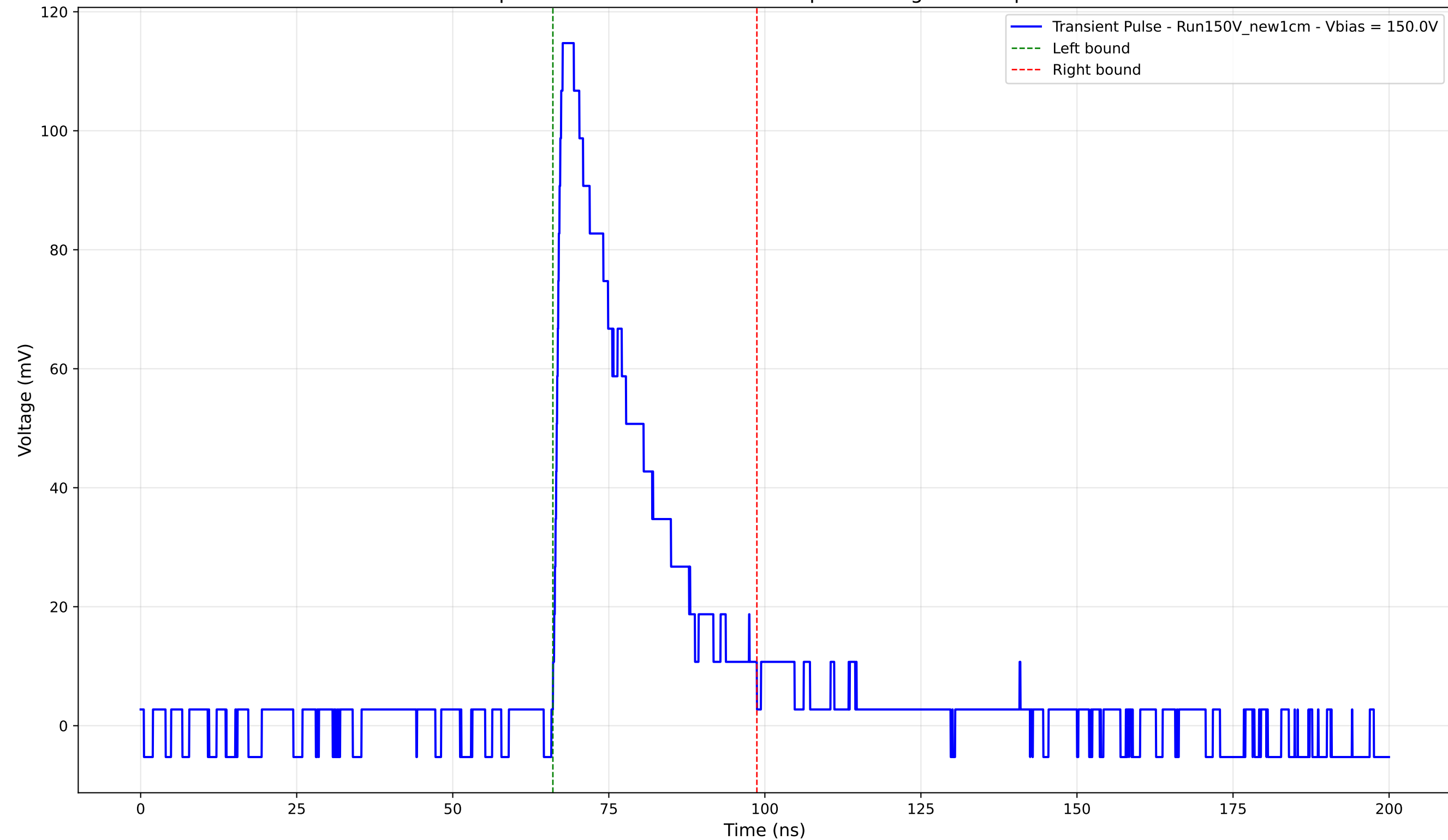
Transient Pulse - Sample: New1cm - Position: 730.0 \mu\text{m} - Charge: 30.10 pC - Rise Time: 1.14 ns
