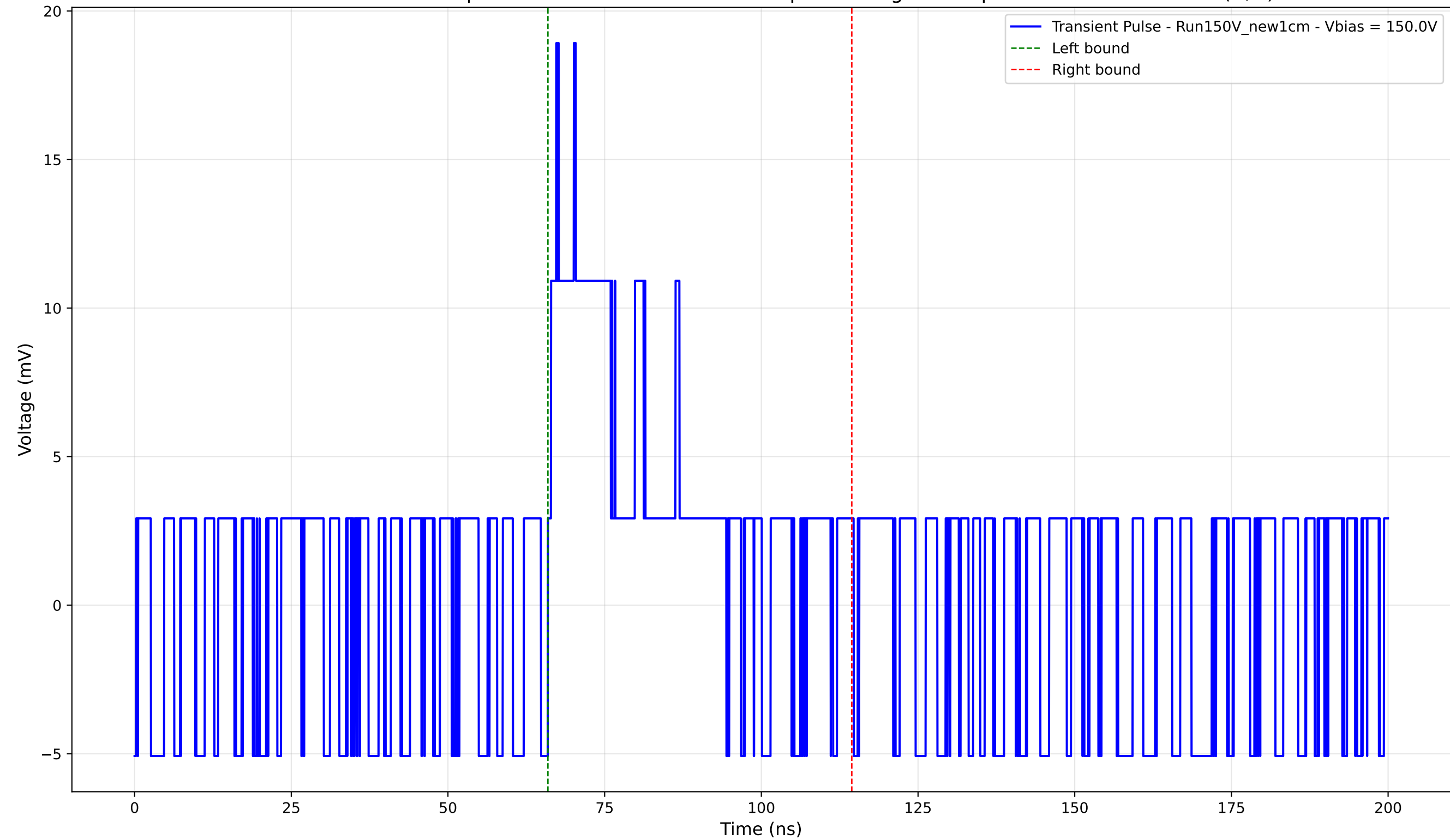
Transient Pulse - Sample: New1cm - Position: 1535.0 \mu\text{m} - Charge: 4.09 pC - Rise Time: 0.00 ns (N/A)
