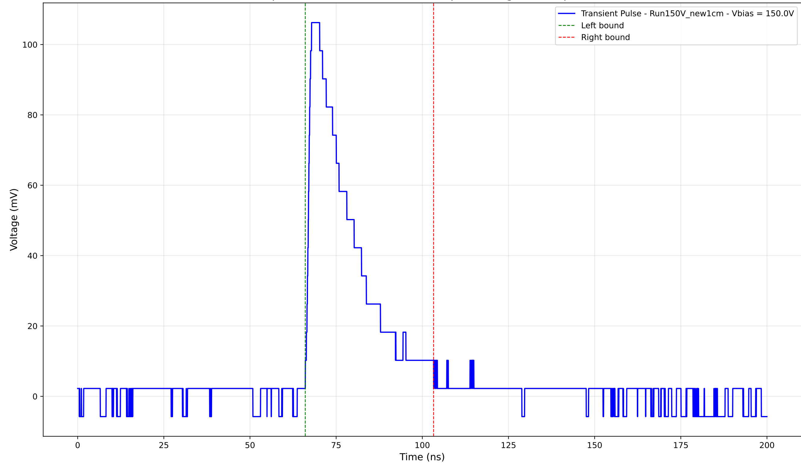
Transient Pulse - Sample: New1cm - Position: 1180.0 \mu\text{m} - Charge: 29.87 pC - Rise Time: 1.24 ns
