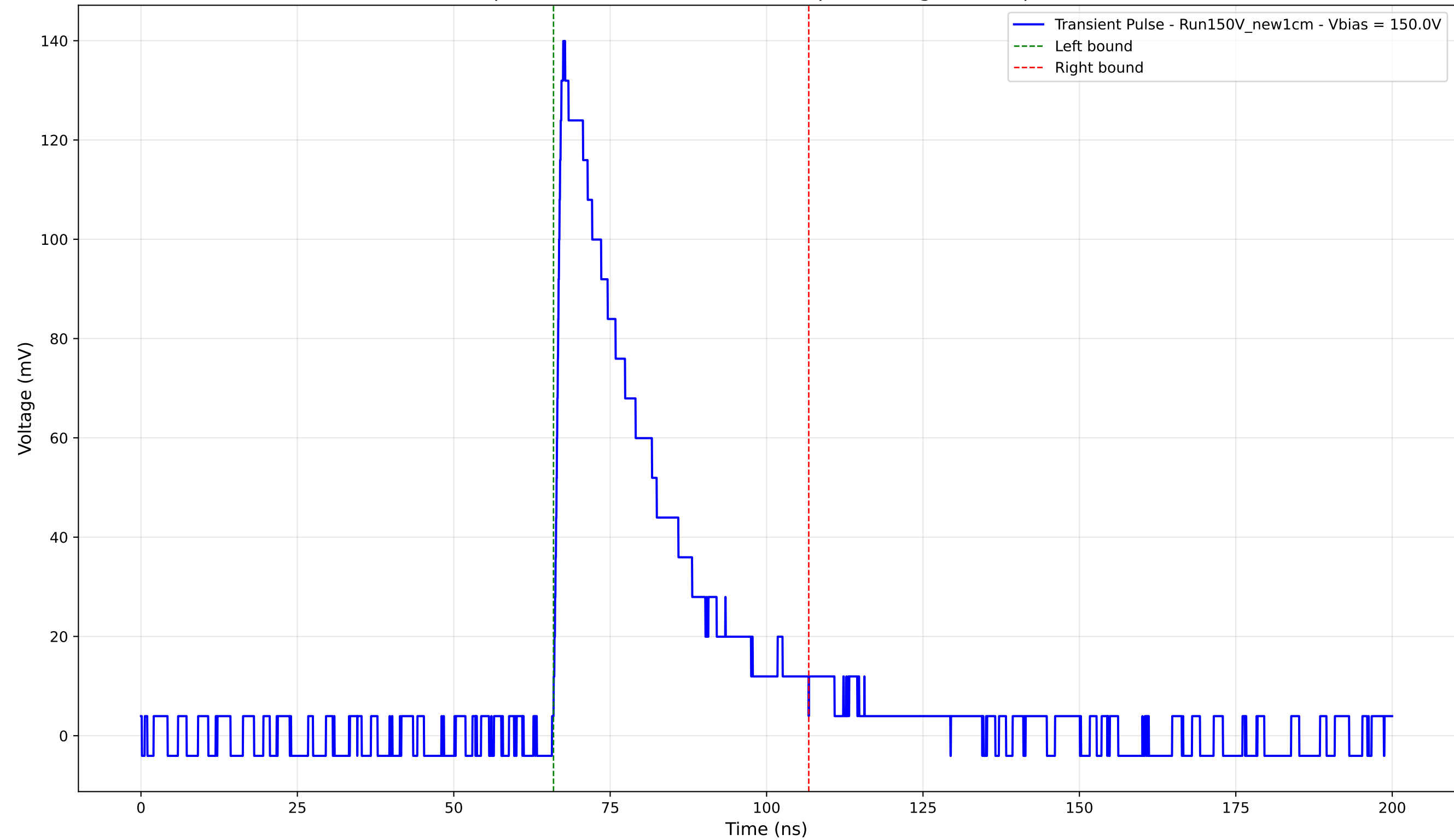
Transient Pulse - Sample: New1cm - Position: 3275.0 \mu\text{m} - Charge: 40.50 pC - Rise Time: 1.13 ns
