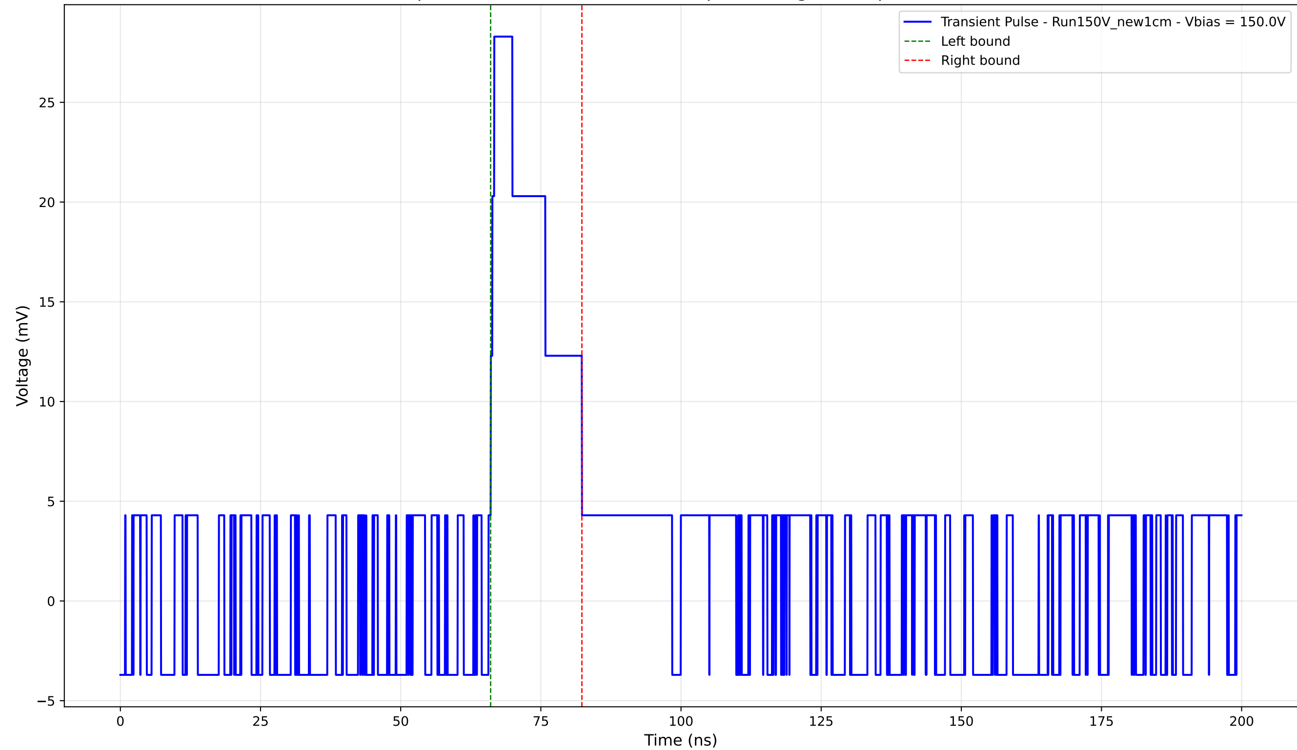
Transient Pulse - Sample: New1cm - Position: 4550.0 \mu\text{m} - Charge: 6.03 pC - Rise Time: 0.00 ns (N/A)
