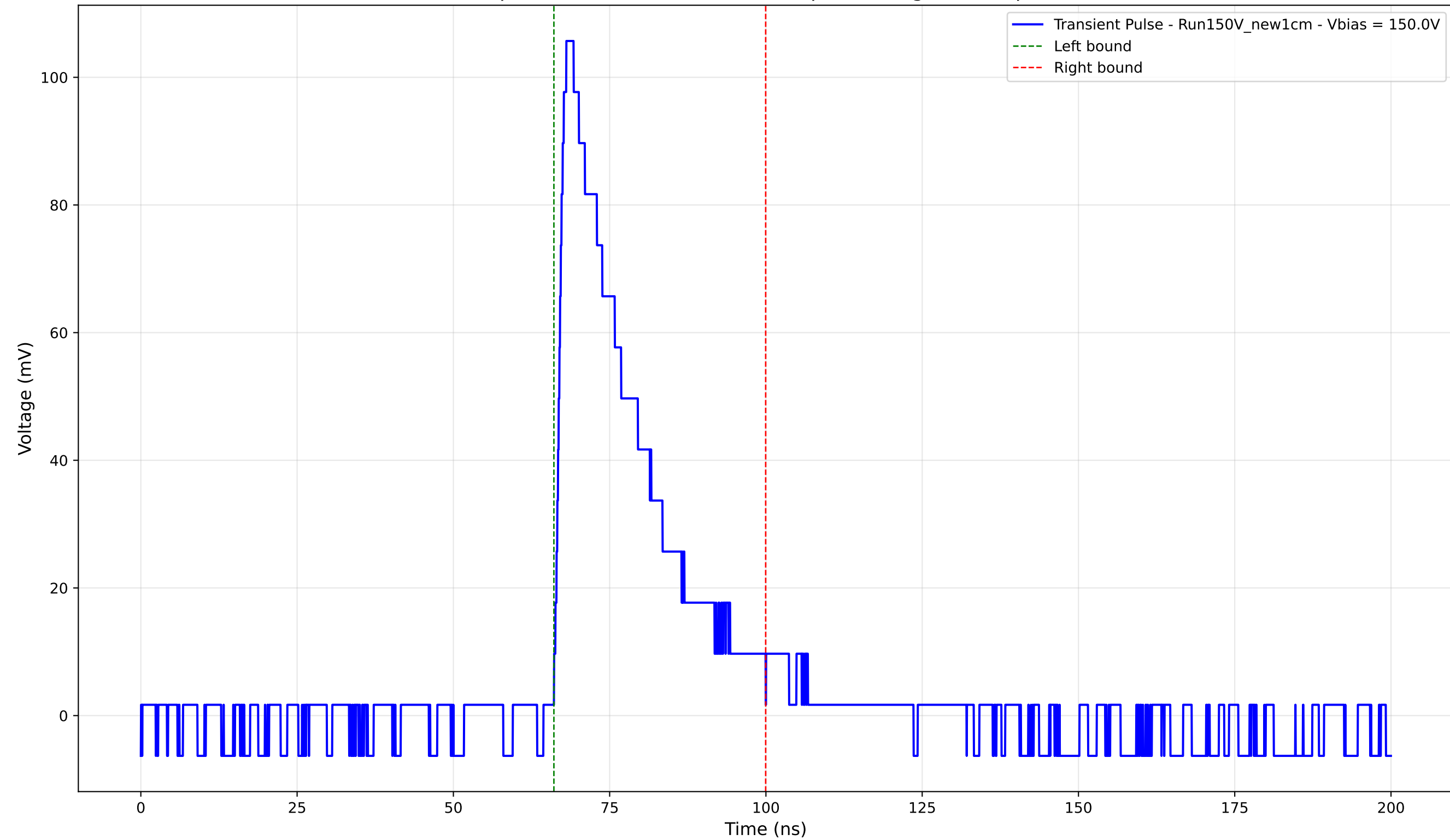
Transient Pulse - Sample: New1cm - Position: 940.0 \mu\text{m} - Charge: 27.28 pC - Rise Time: 1.36 ns
