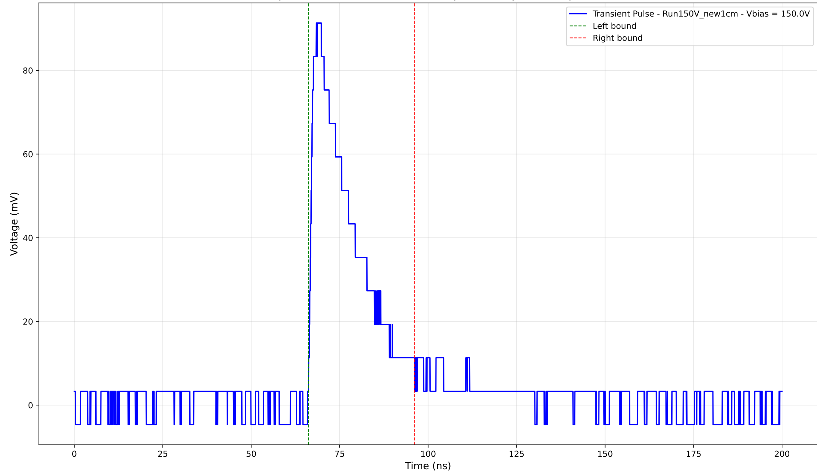
Transient Pulse - Sample: New1cm - Position: 955.0 \mu\text{m} - Charge: 23.58 pC - Rise Time: 1.37 ns
