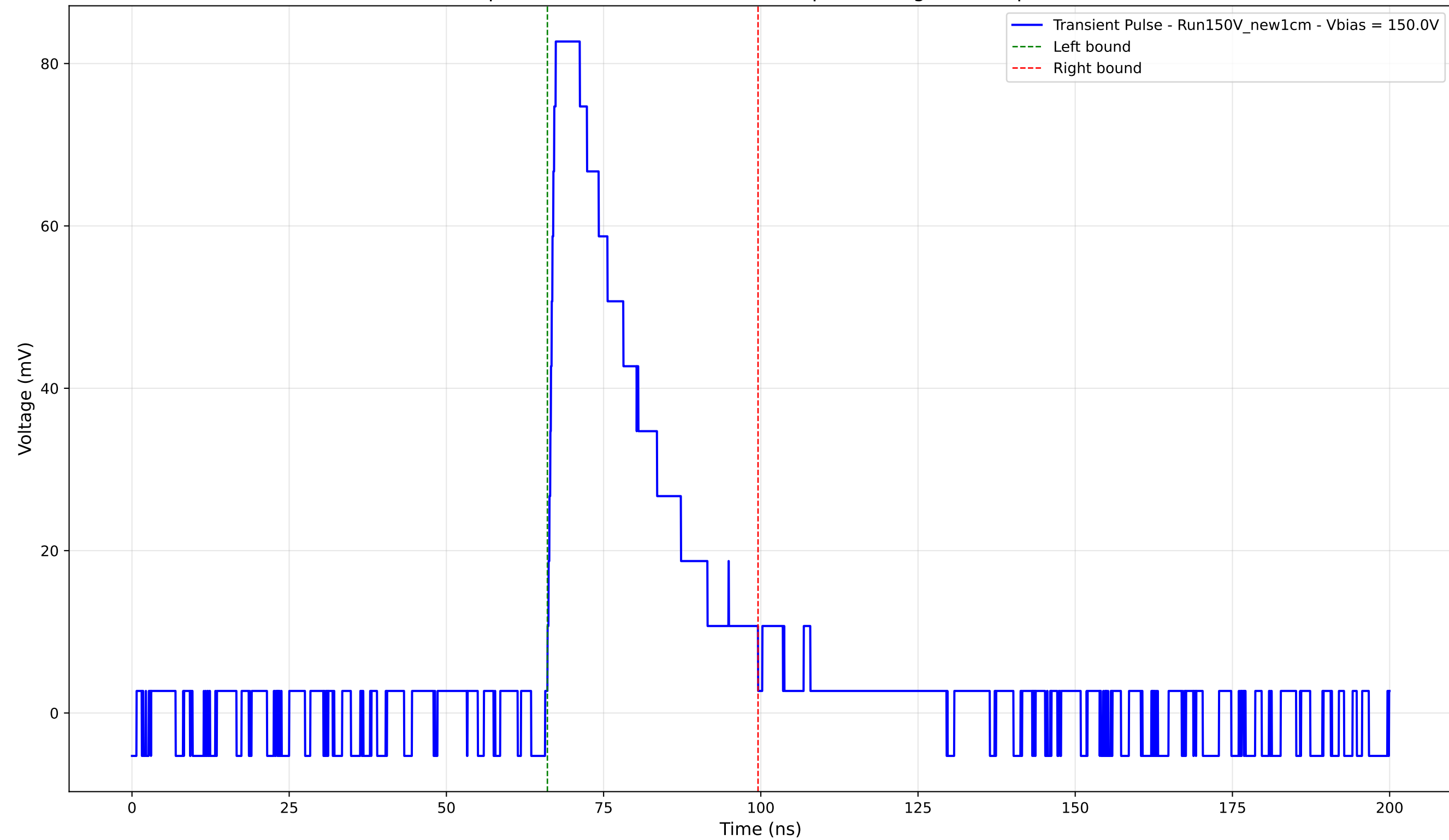
Transient Pulse - Sample: New1cm - Position: 1625.0 \mu\text{m} - Charge: 25.35 pC - Rise Time: 1.07 ns
