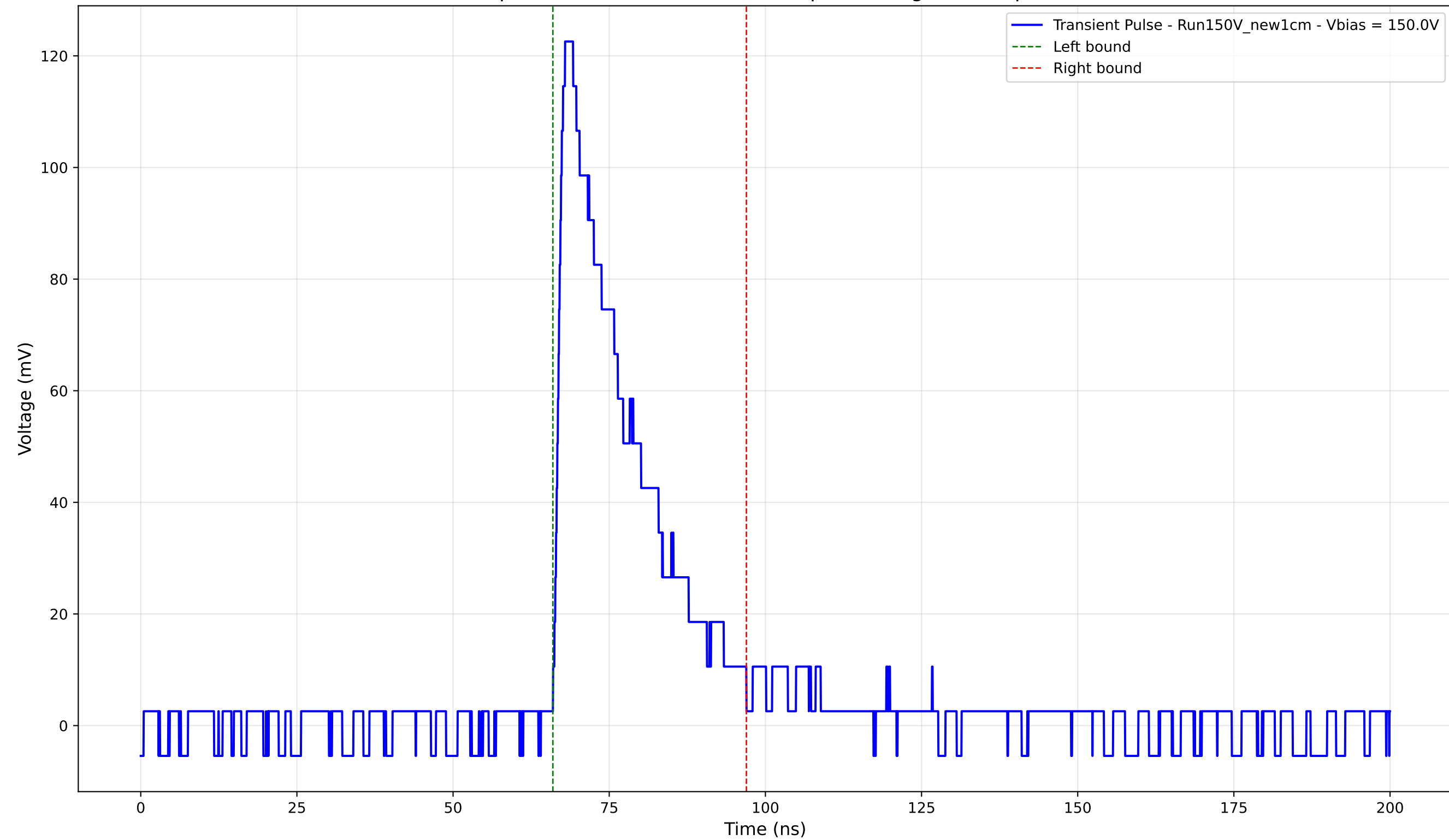
Transient Pulse - Sample: New1cm - Position: 760.0 \mu\text{m} - Charge: 30.06 pC - Rise Time: 1.40 ns
