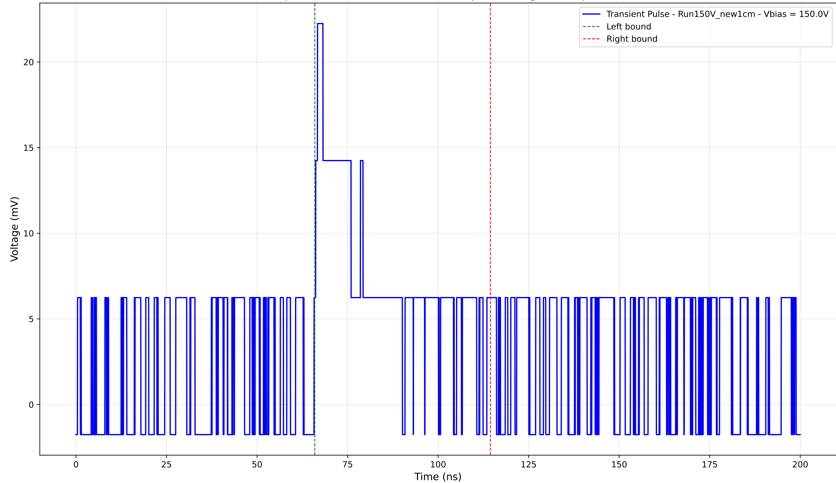
Transient Pulse - Sample: New1cm - Position: 4890.0 \mu\text{m} - Charge: 7.32 pC - Rise Time: 0.96 ns
