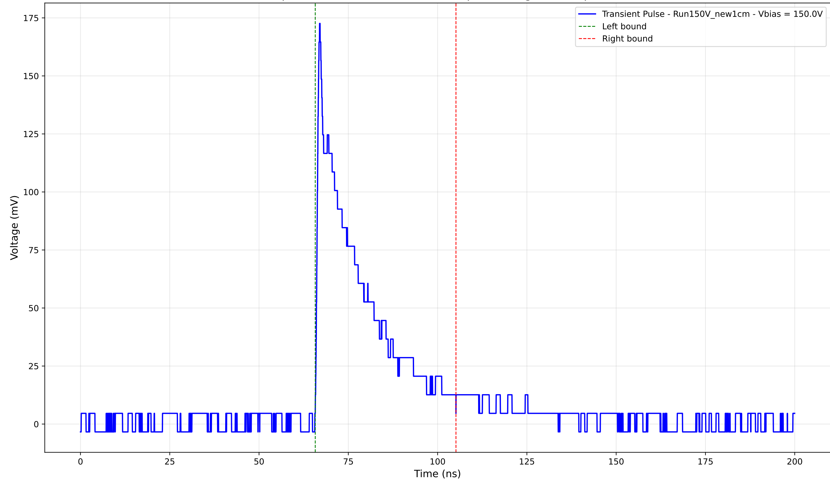
Transient Pulse - Sample: New1cm - Position: 2905.0 \mu\text{m} - Charge: 40.05 pC - Rise Time: 0.85 ns
