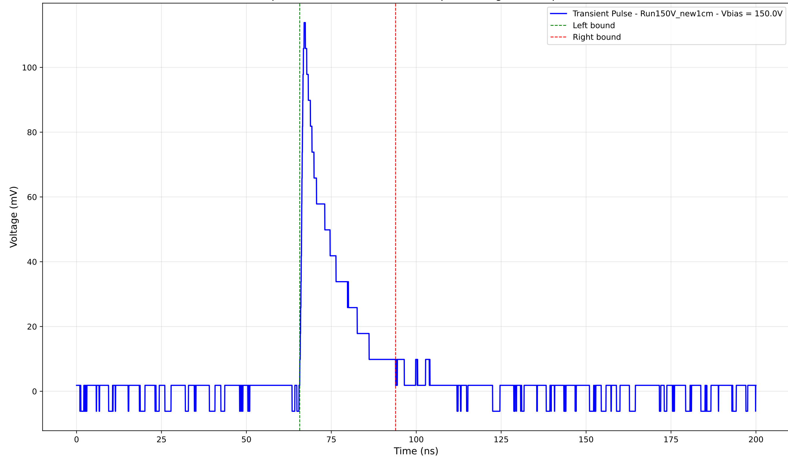
Transient Pulse - Sample: New1cm - Position: 135.0 \mu\text{m} - Charge: 20.28 pC - Rise Time: 0.94 ns
