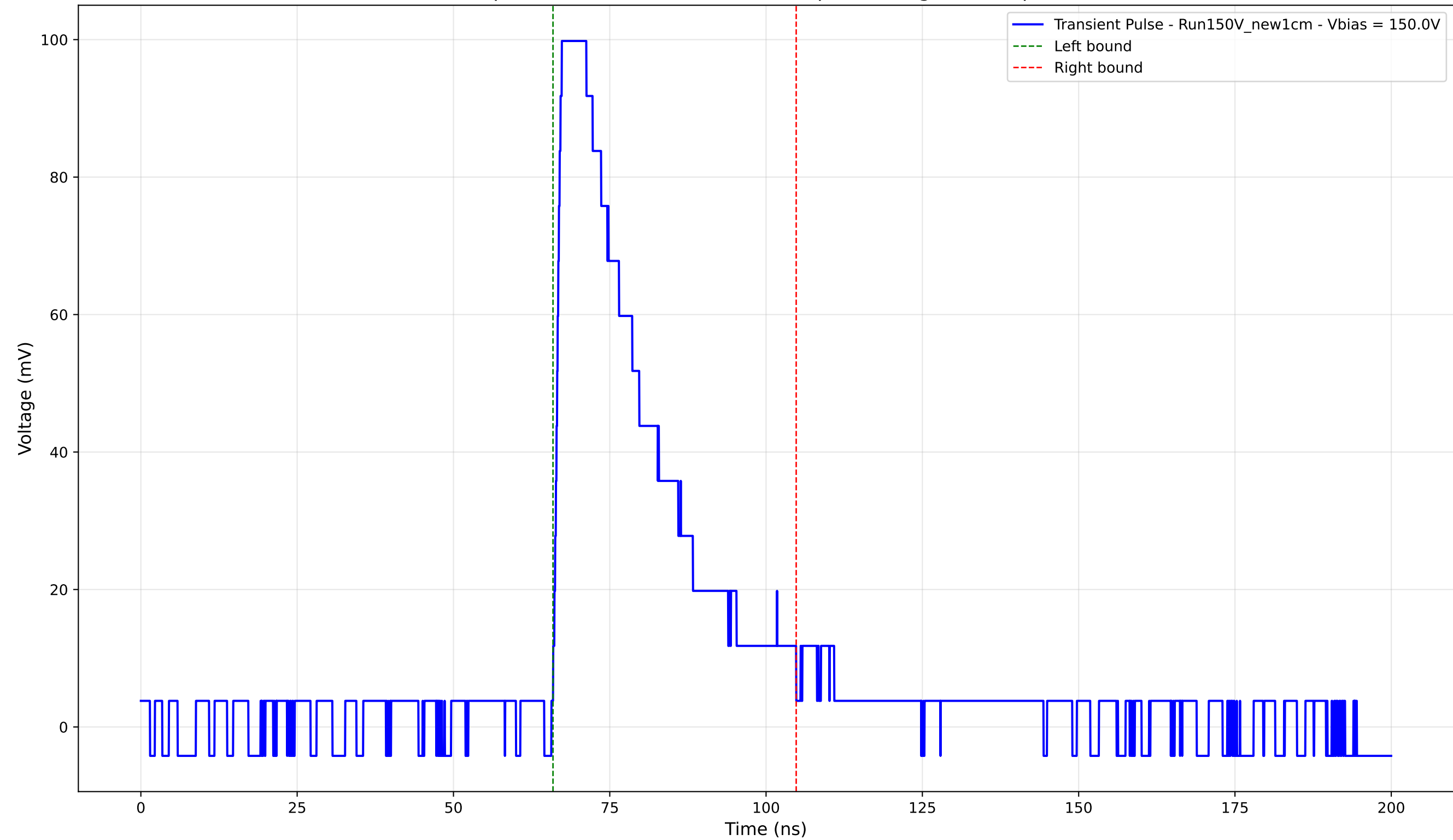
Transient Pulse - Sample: New1cm - Position: 1710.0 \mu\text{m} - Charge: 32.43 pC - Rise Time: 1.18 ns
