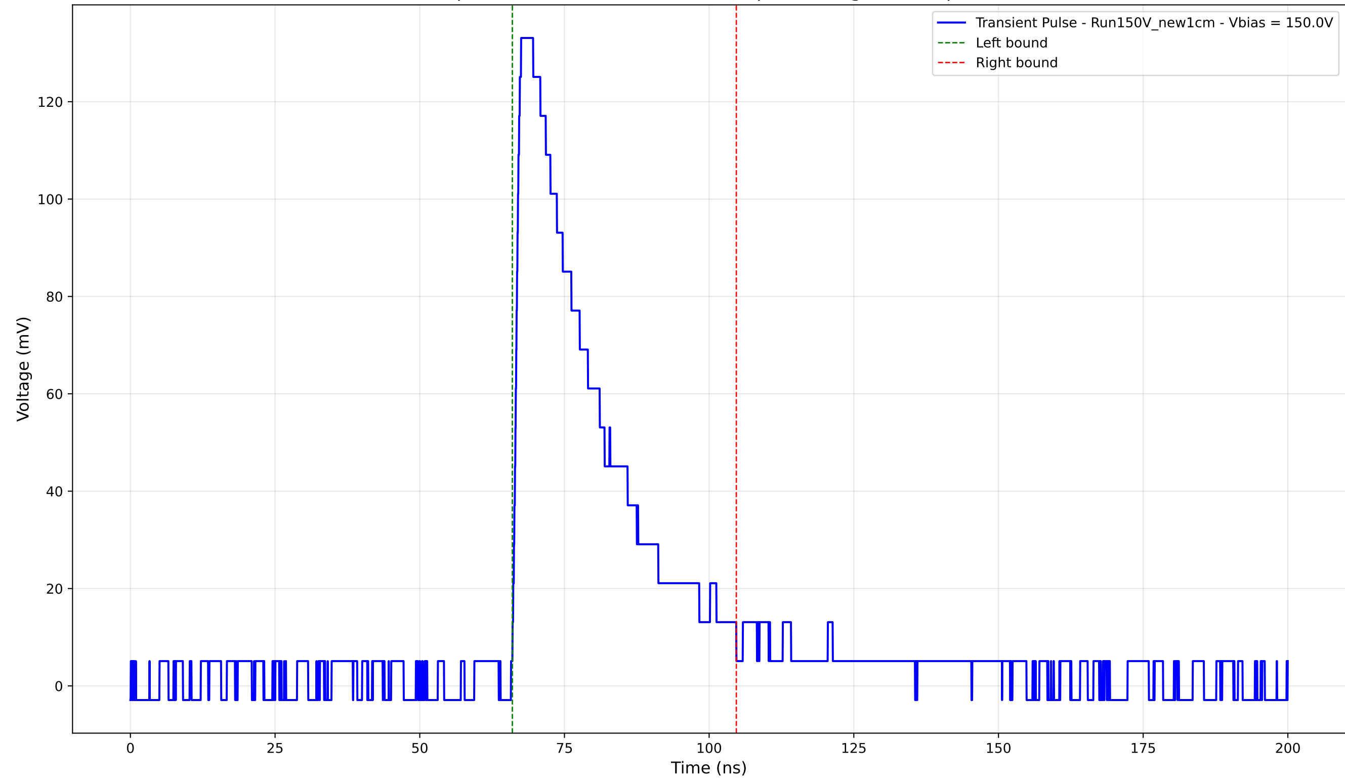
Transient Pulse - Sample: New1cm - Position: 3465.0 \mu\text{m} - Charge: 40.88 pC - Rise Time: 1.16 ns
