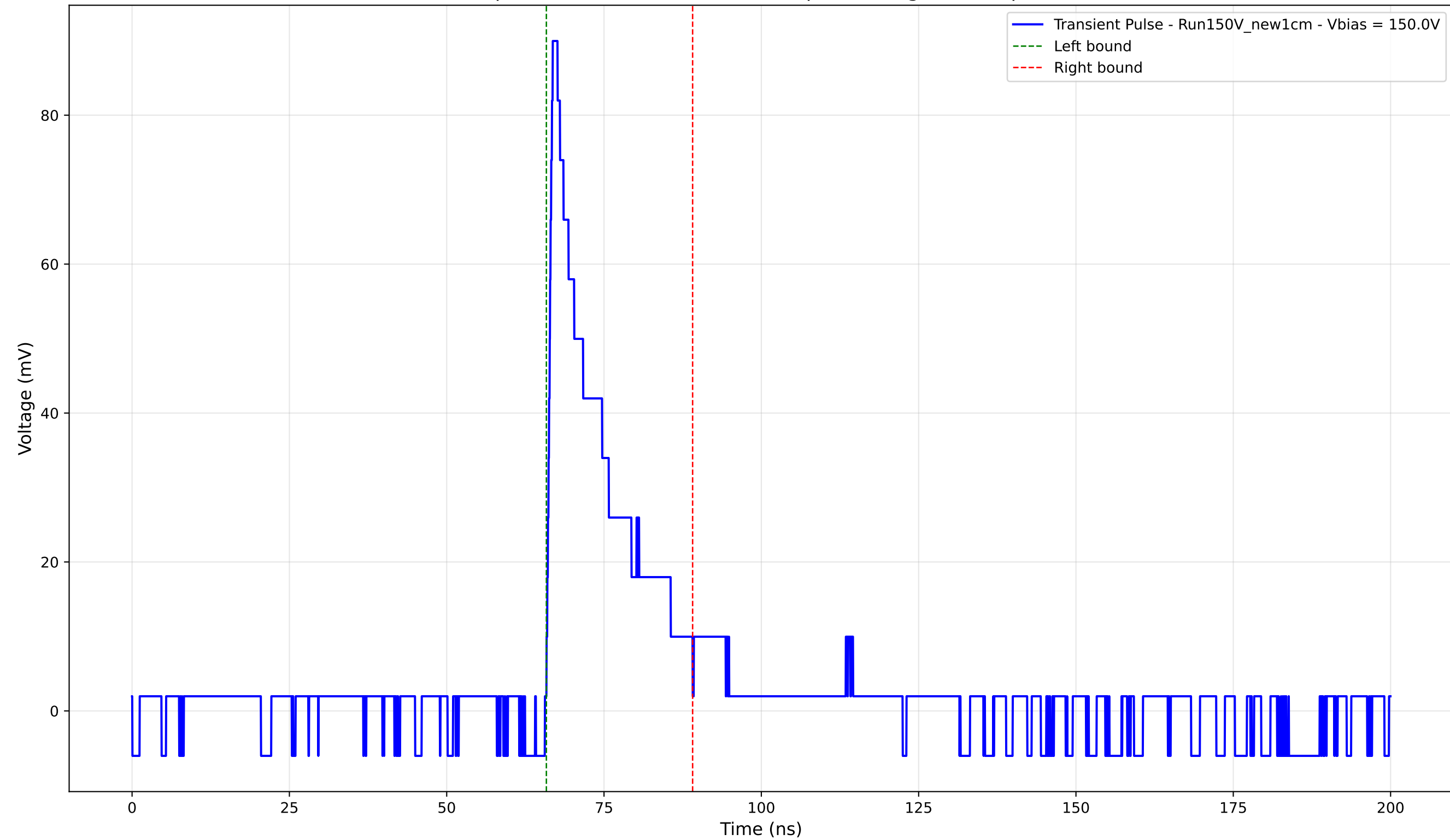
Transient Pulse - Sample: New1cm - Position: 100.0 \mu\text{m} - Charge: 15.39 pC - Rise Time: 0.86 ns
