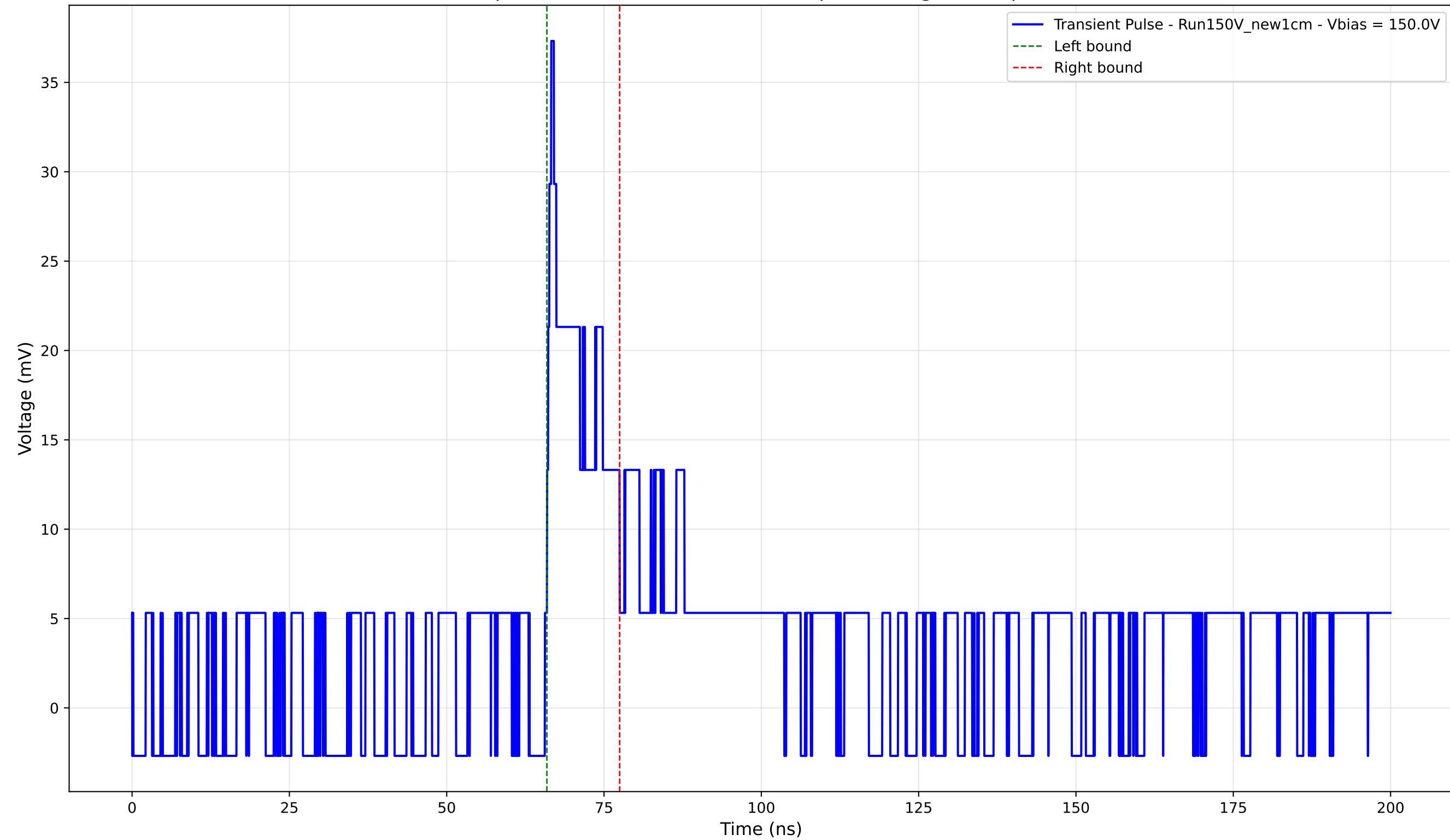
Transient Pulse - Sample: New1cm - Position: 2540.0 \mu\text{m} - Charge: 4.34 pC - Rise Time: 1.01 ns
