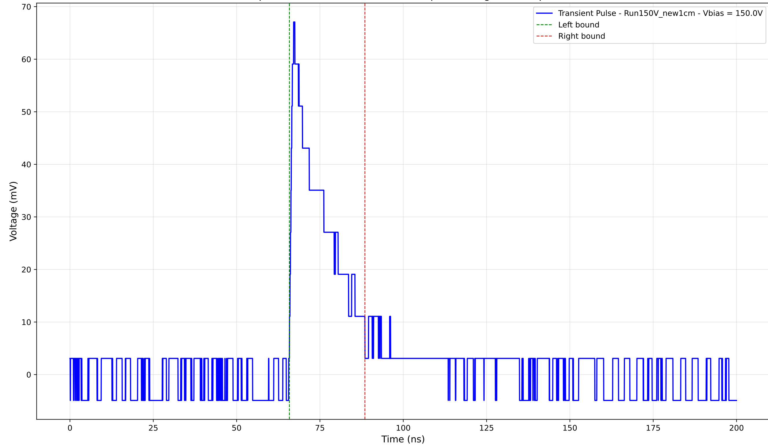
Transient Pulse - Sample: New1cm - Position: 4615.0 \mu\text{m} - Charge: 13.59 pC - Rise Time: 1.25 ns
