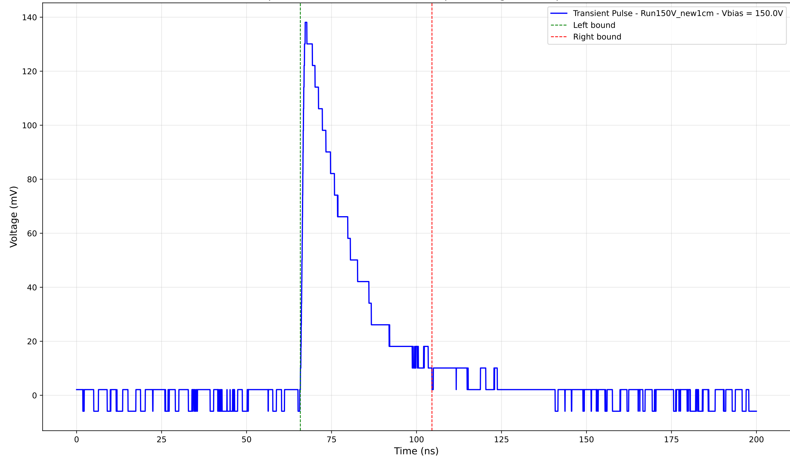
Transient Pulse - Sample: New1cm - Position: 3185.0 \mu\text{m} - Charge: 39.11 pC - Rise Time: 1.07 ns
