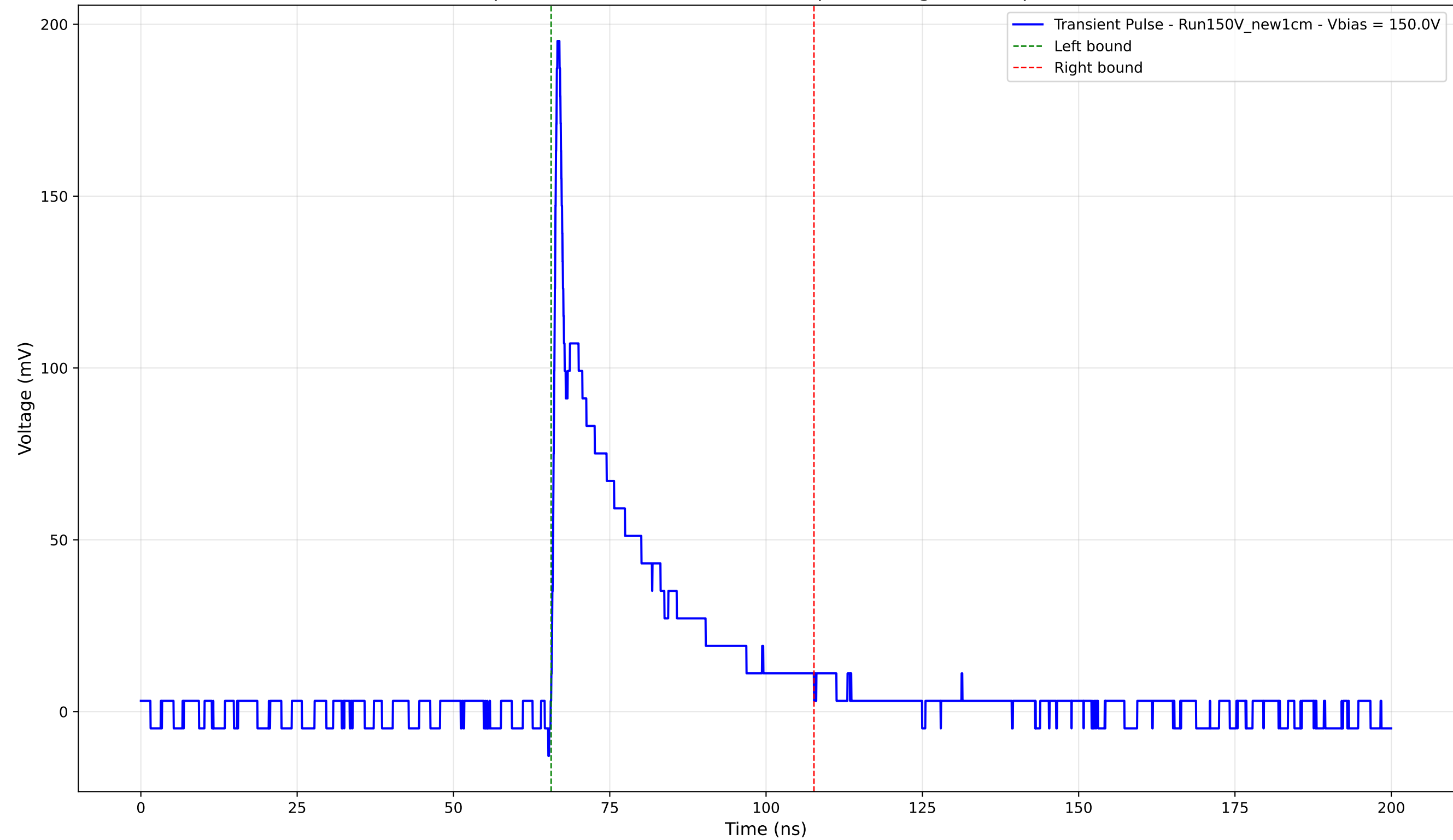
Transient Pulse - Sample: New1cm - Position: 2675.0 \mu\text{m} - Charge: 35.82 pC - Rise Time: 0.74 ns
