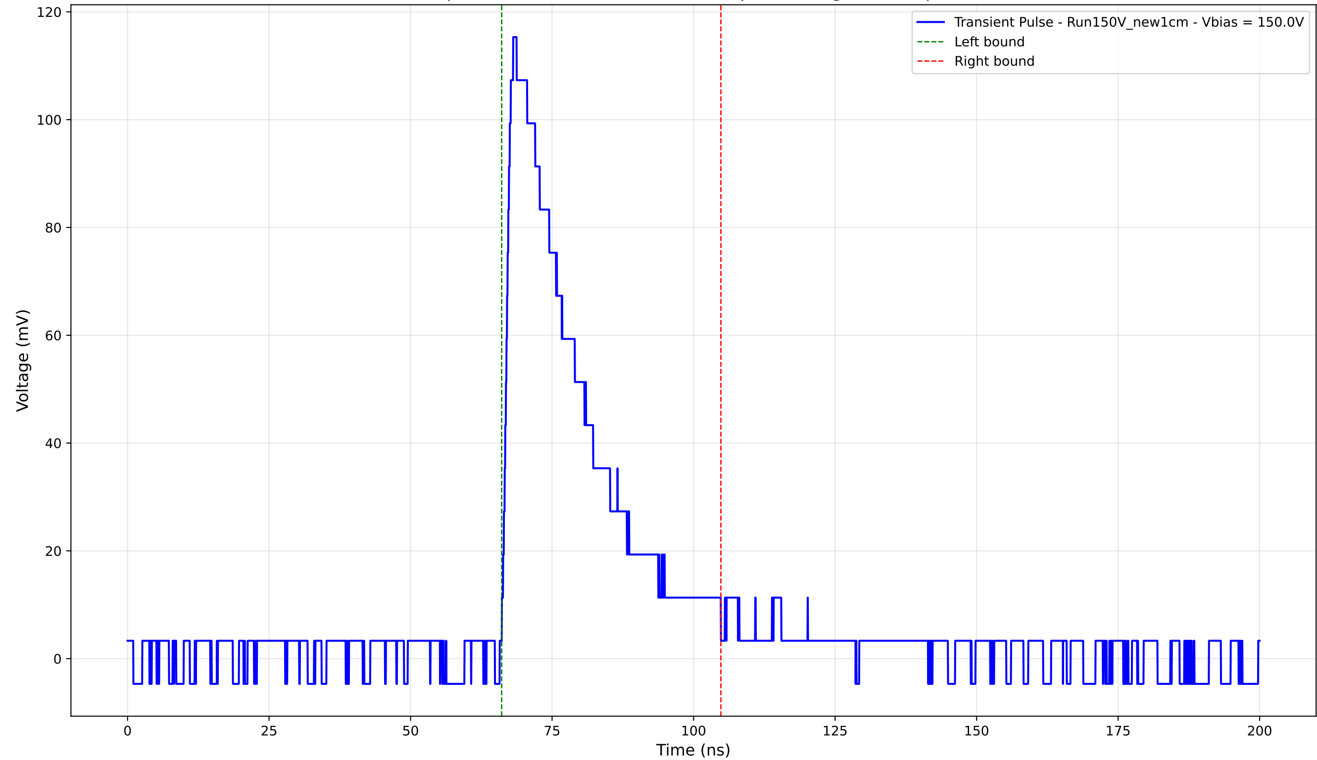
Transient Pulse - Sample: New1cm - Position: 1325.0 \mu\text{m} - Charge: 32.65 pC - Rise Time: 1.38 ns
