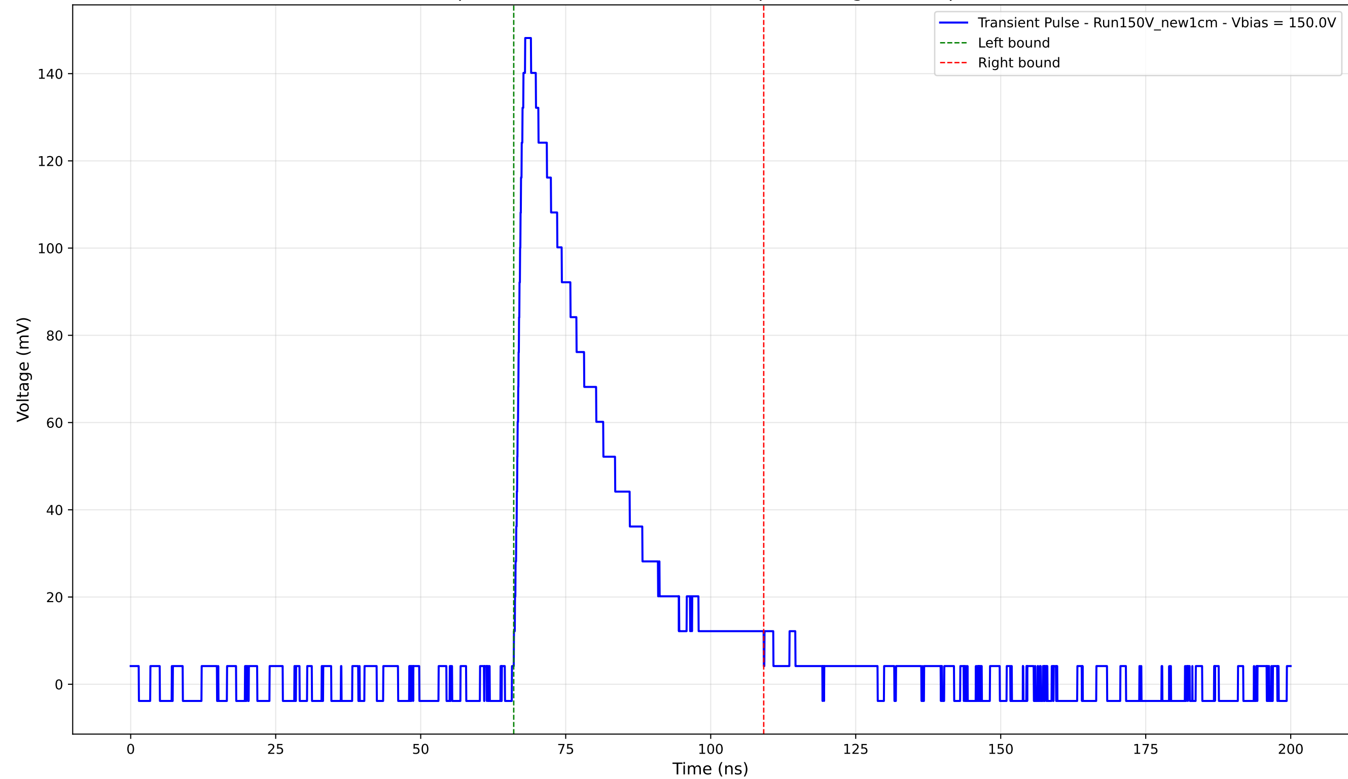
Transient Pulse - Sample: New1cm - Position: 3845.0 \mu\text{m} - Charge: 42.54 pC - Rise Time: 1.47 ns
