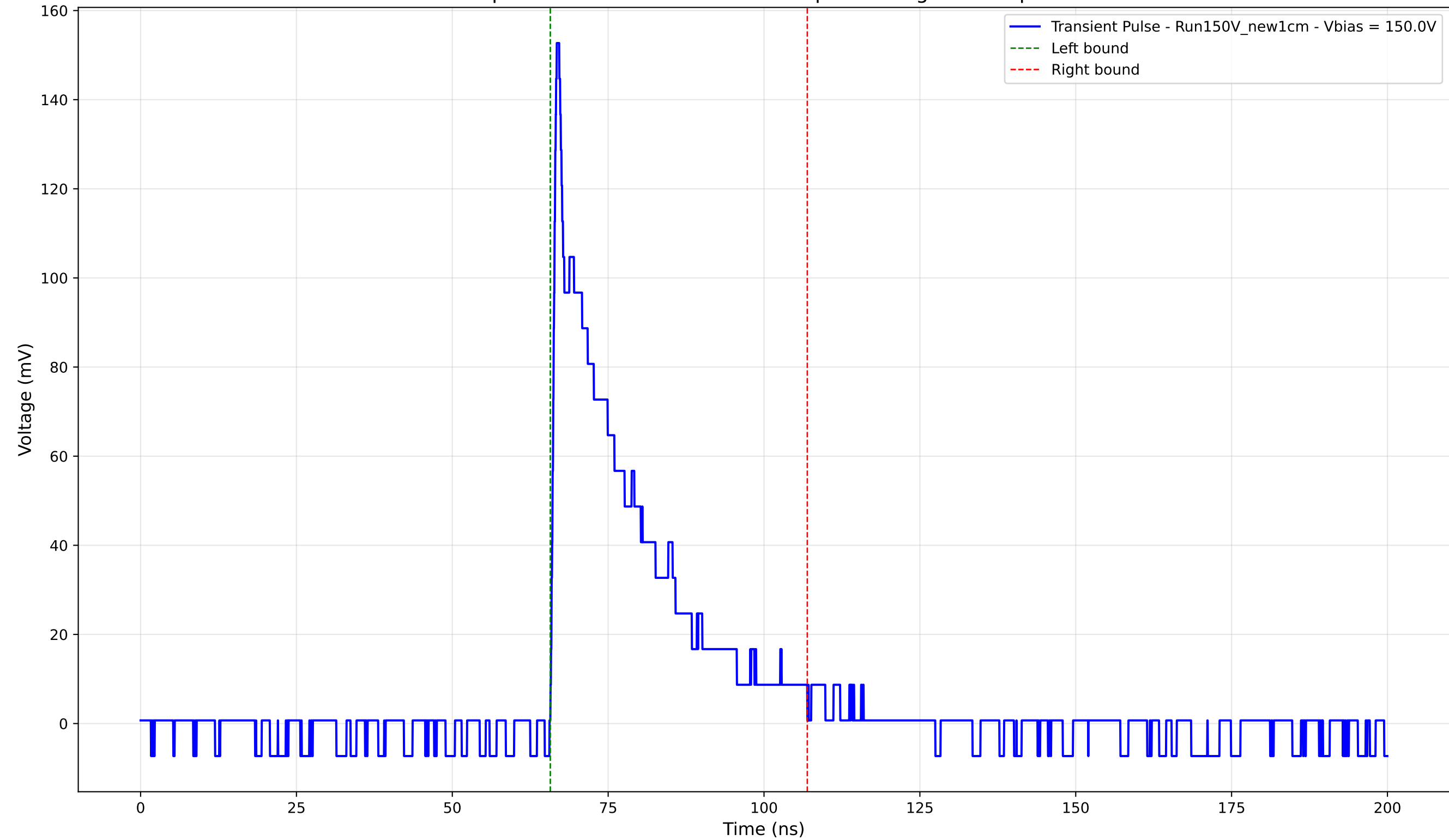
Transient Pulse - Sample: New1cm - Position: 2250.0 \mu\text{m} - Charge: 32.79 pC - Rise Time: 0.82 ns
