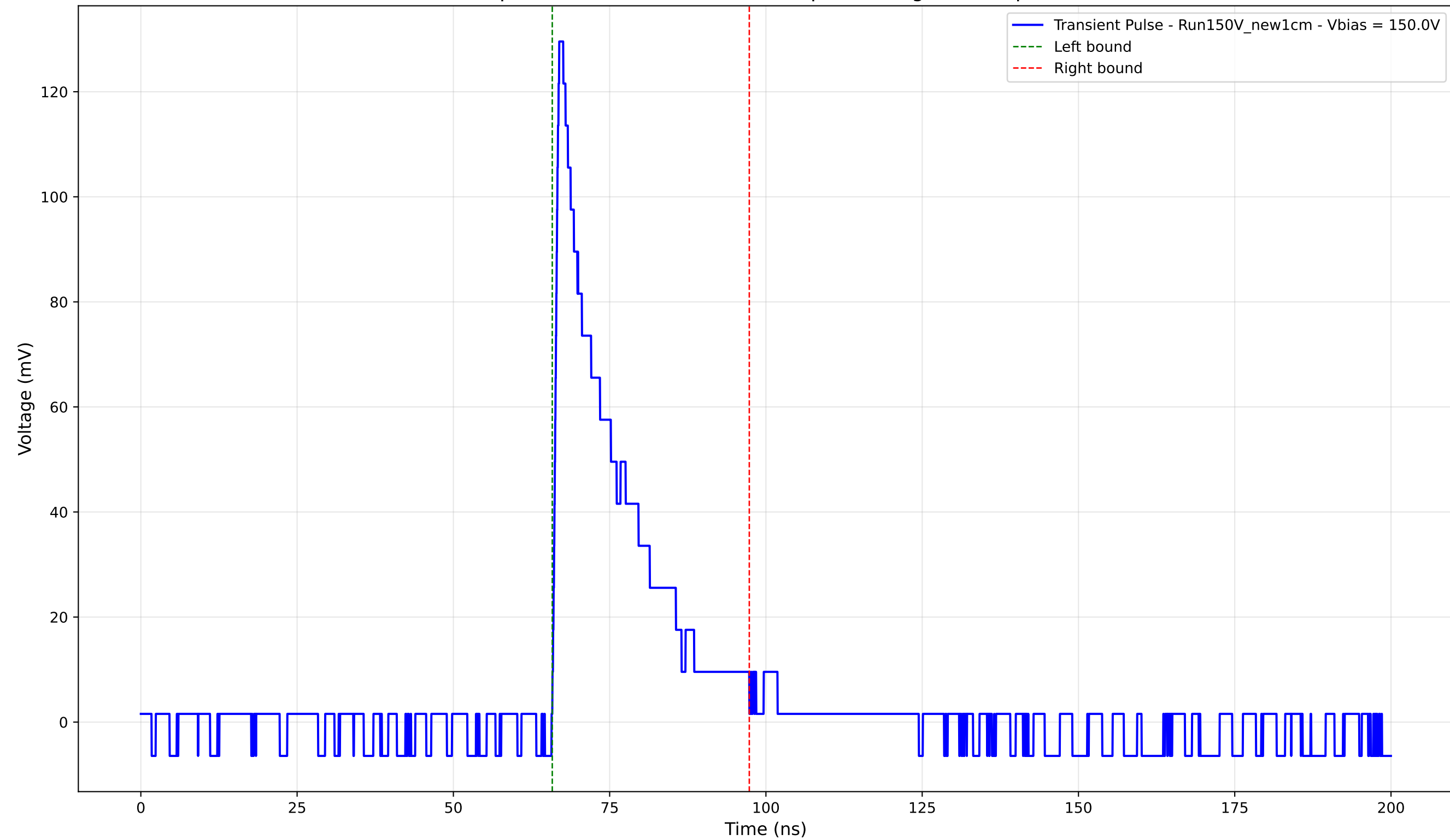
Transient Pulse - Sample: New1cm - Position: 190.0 \mu\text{m} - Charge: 24.96 pC - Rise Time: 0.89 ns
