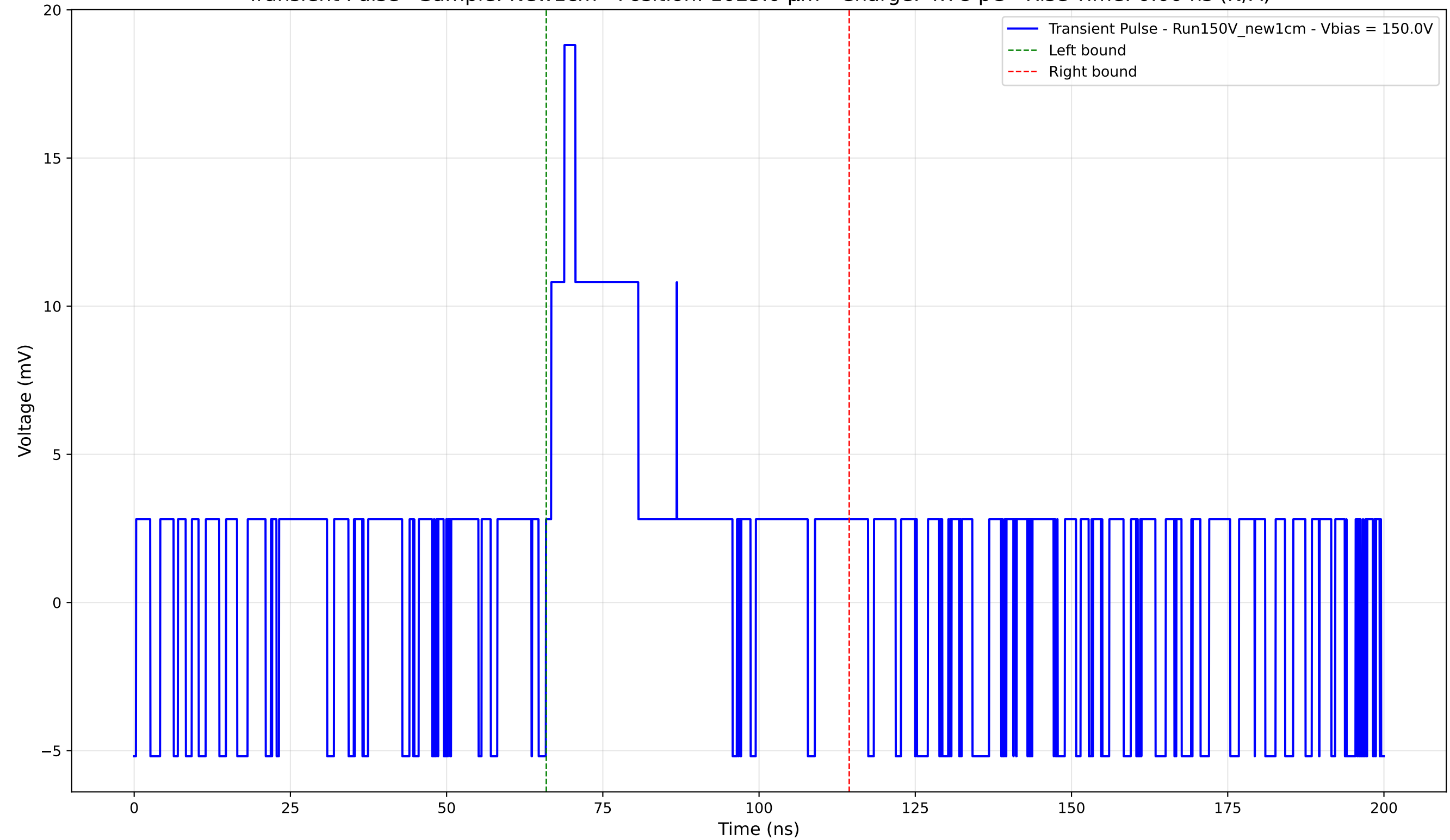
Transient Pulse - Sample: New1cm - Position: 1025.0 \mu\text{m} - Charge: 4.78 pC - Rise Time: 0.00 ns (N/A)
