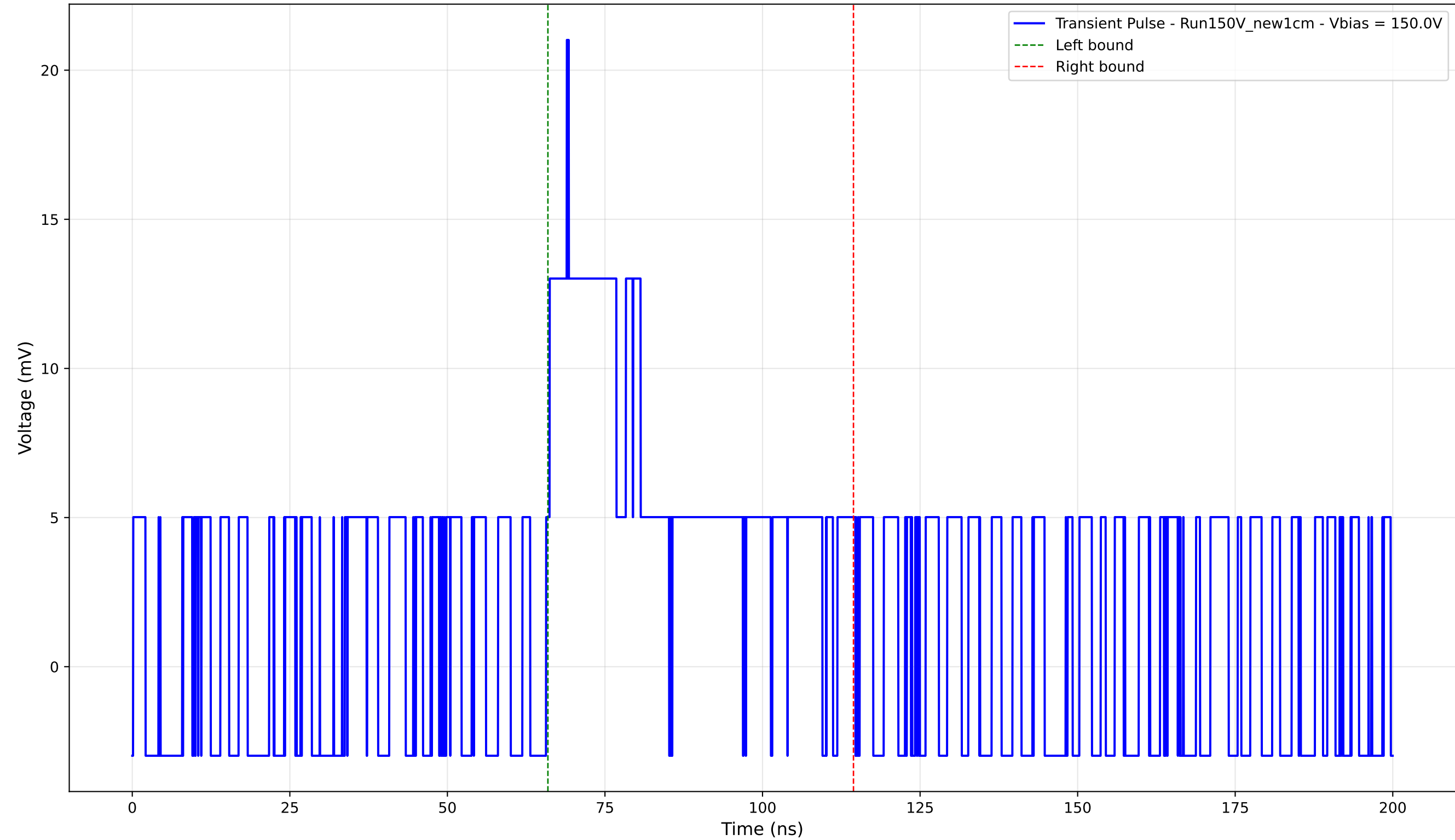
Transient Pulse - Sample: New1cm - Position: 2040.0 \mu\text{m} - Charge: 6.60 pC - Rise Time: 0.00 ns (N/A)
