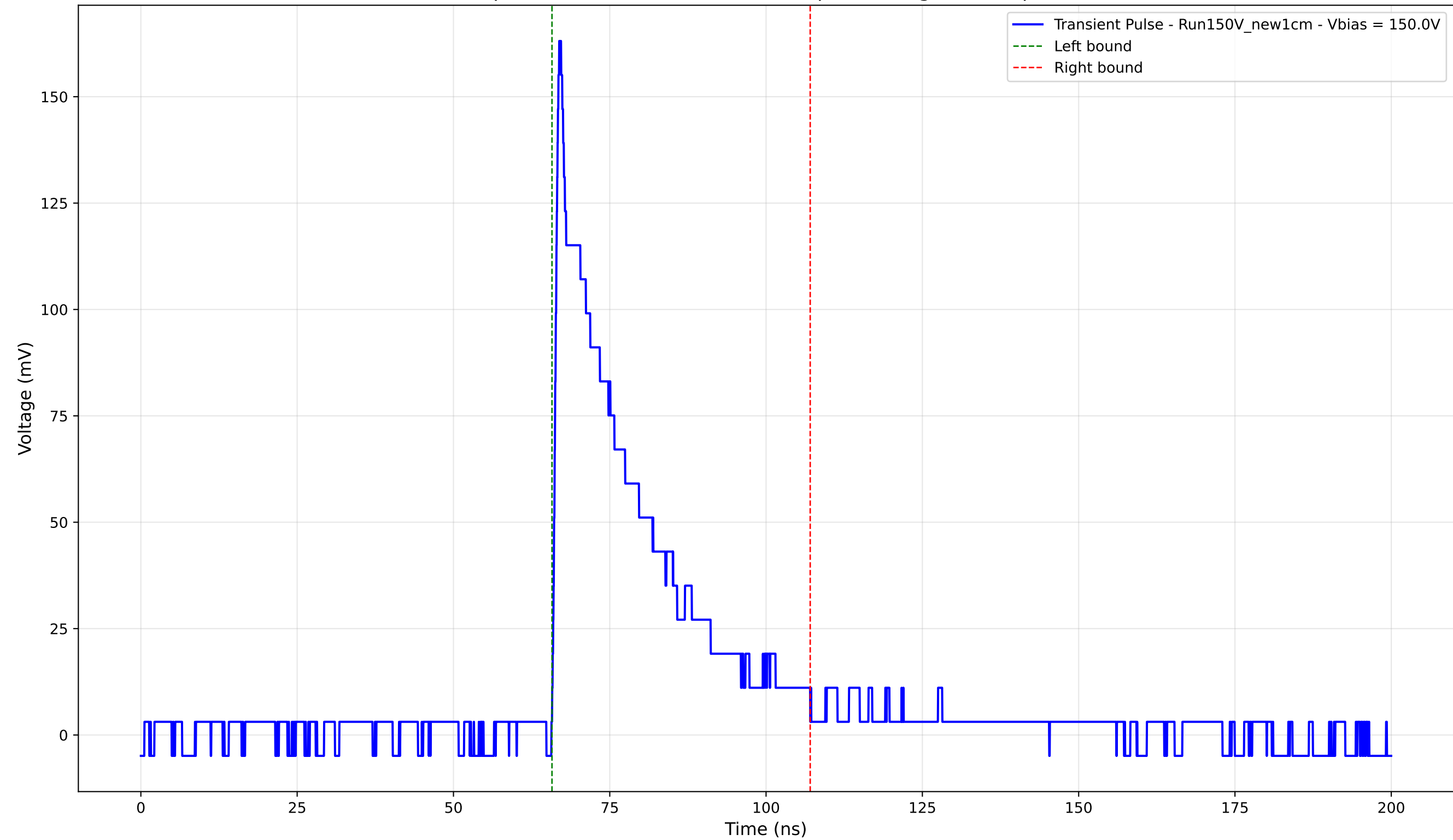
Transient Pulse - Sample: New1cm - Position: 2935.0 \mu\text{m} - Charge: 38.45 pC - Rise Time: 0.85 ns
