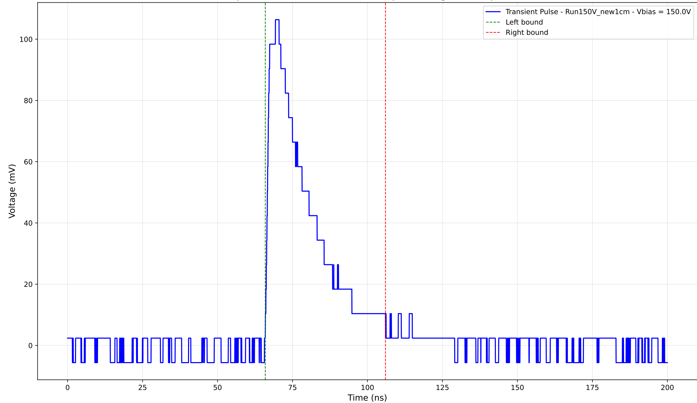
Transient Pulse - Sample: New1cm - Position: 1665.0 \mu\text{m} - Charge: 31.88 pC - Rise Time: 1.28 ns
