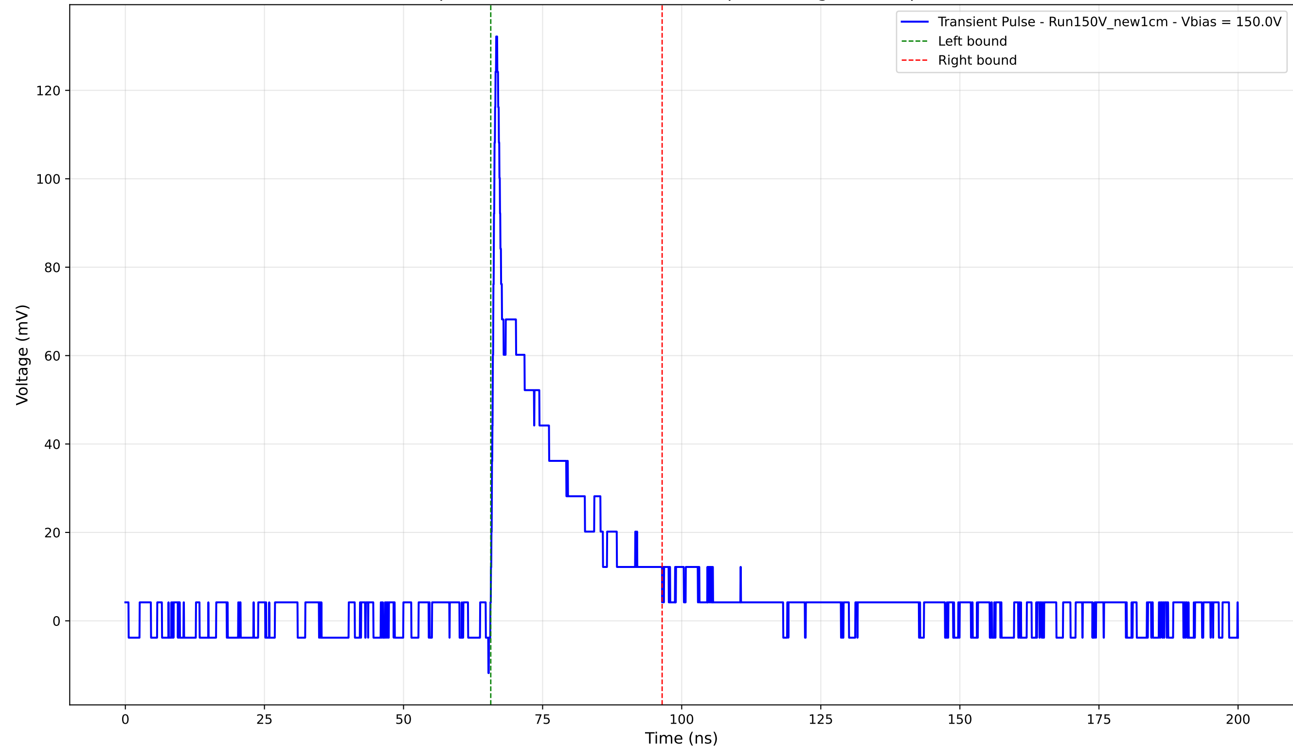
Transient Pulse - Sample: New1cm - Position: 2615.0 \mu\text{m} - Charge: 21.66 pC - Rise Time: 0.76 ns
