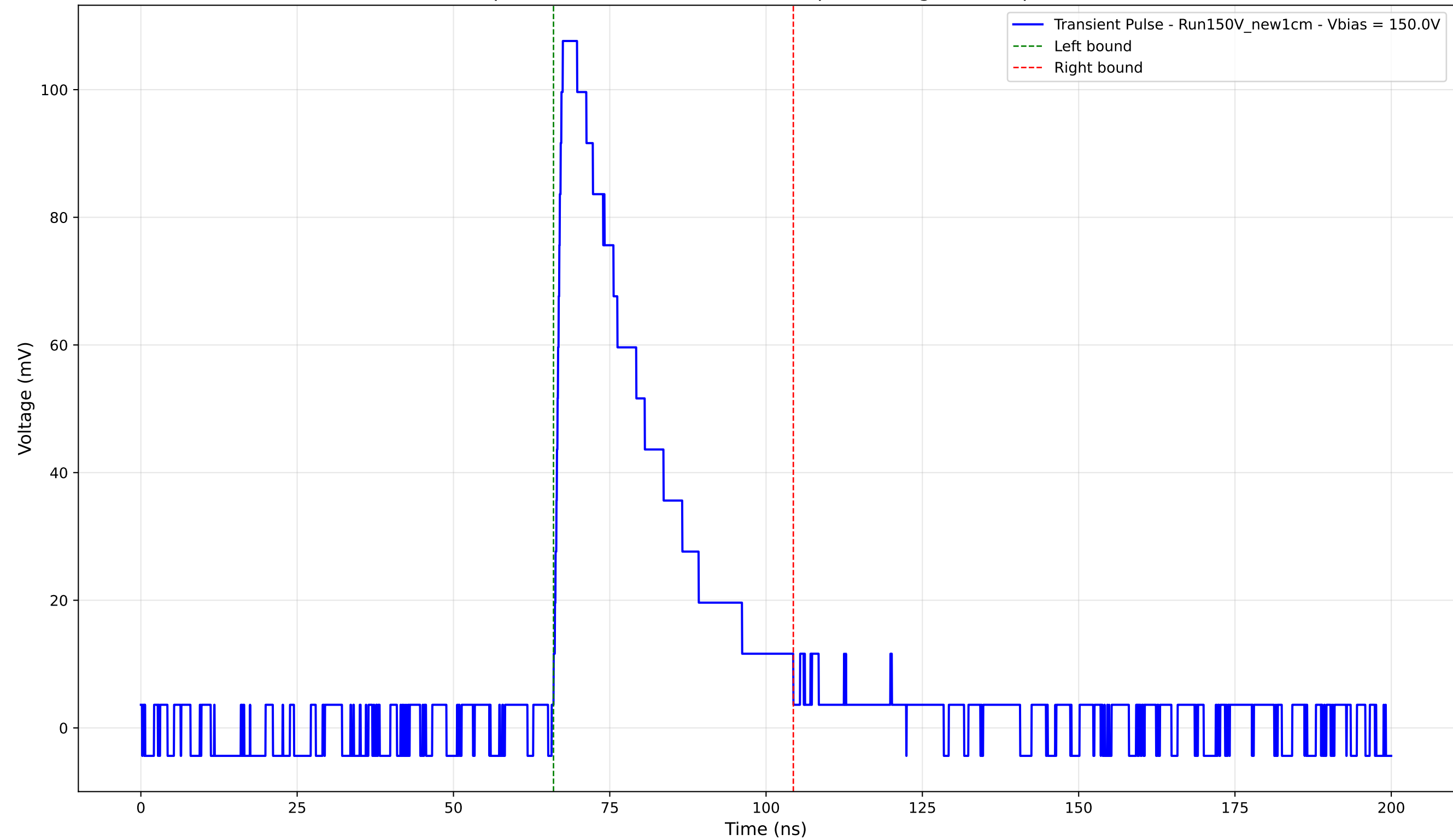
Transient Pulse - Sample: New1cm - Position: 1690.0 \mu\text{m} - Charge: 33.41 pC - Rise Time: 1.24 ns
