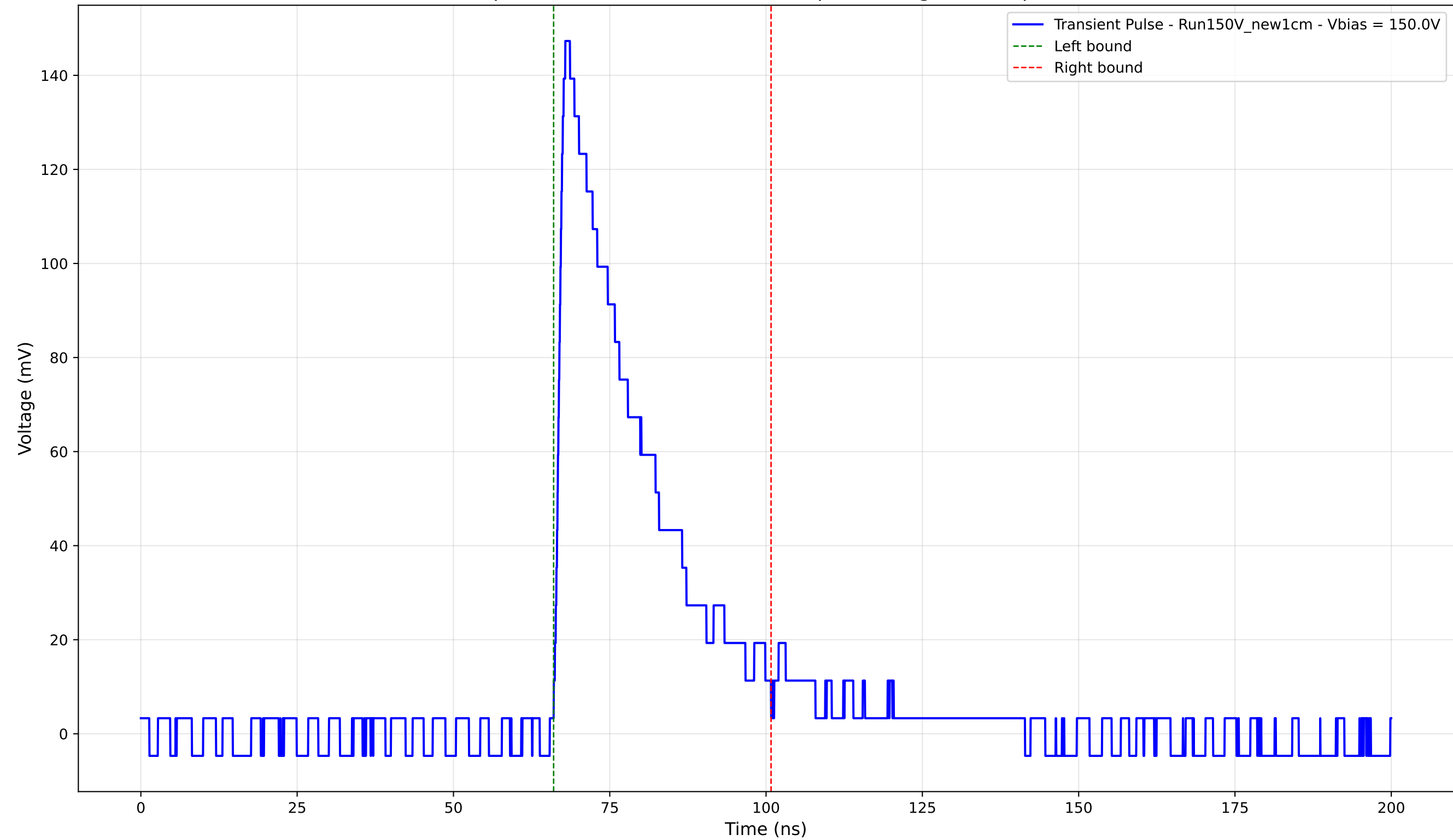
Transient Pulse - Sample: New1cm - Position: 3710.0 \mu\text{m} - Charge: 40.00 pC - Rise Time: 1.41 ns
