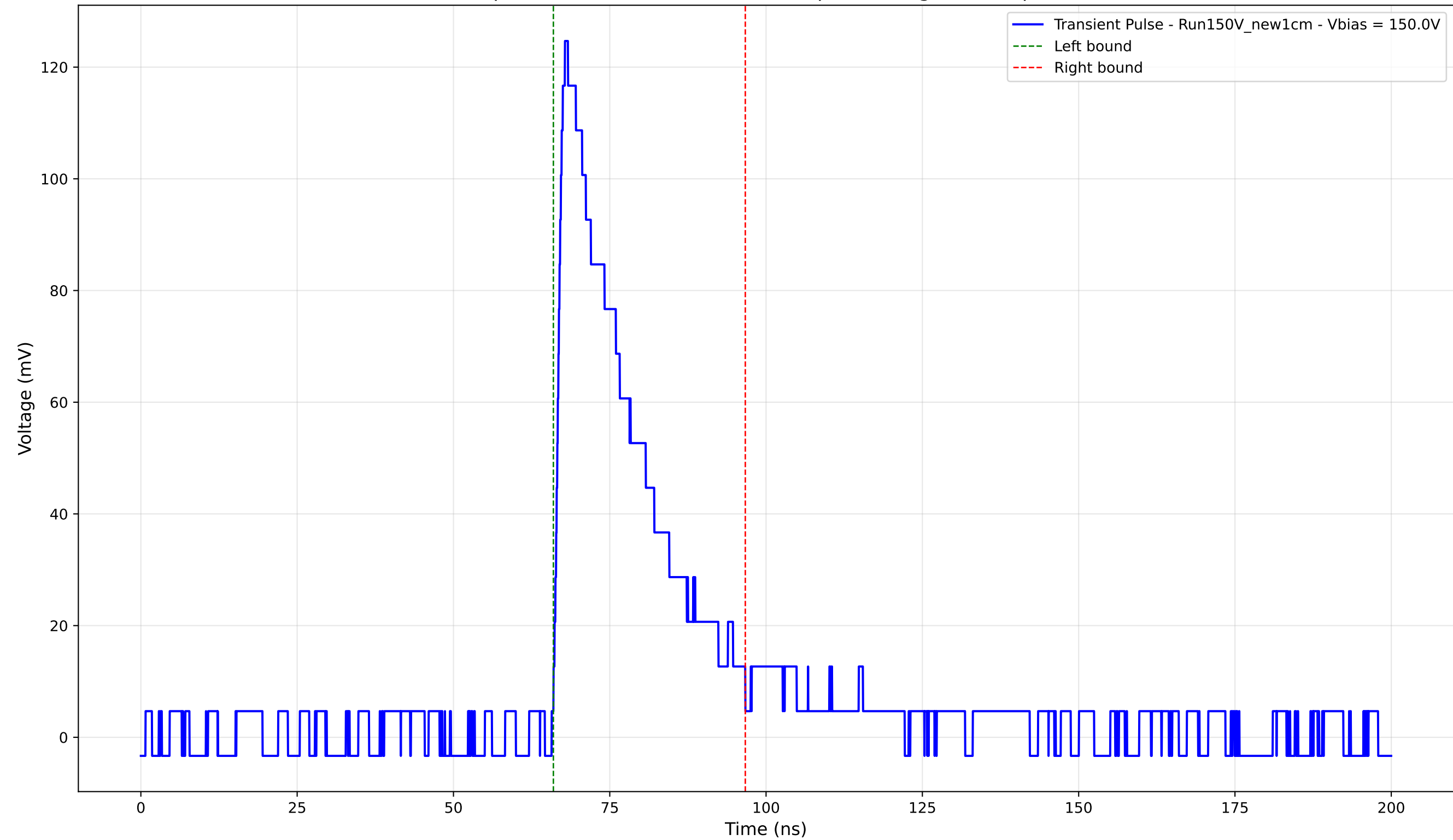
Transient Pulse - Sample: New1cm - Position: 4185.0 \mu\text{m} - Charge: 31.59 pC - Rise Time: 1.48 ns
