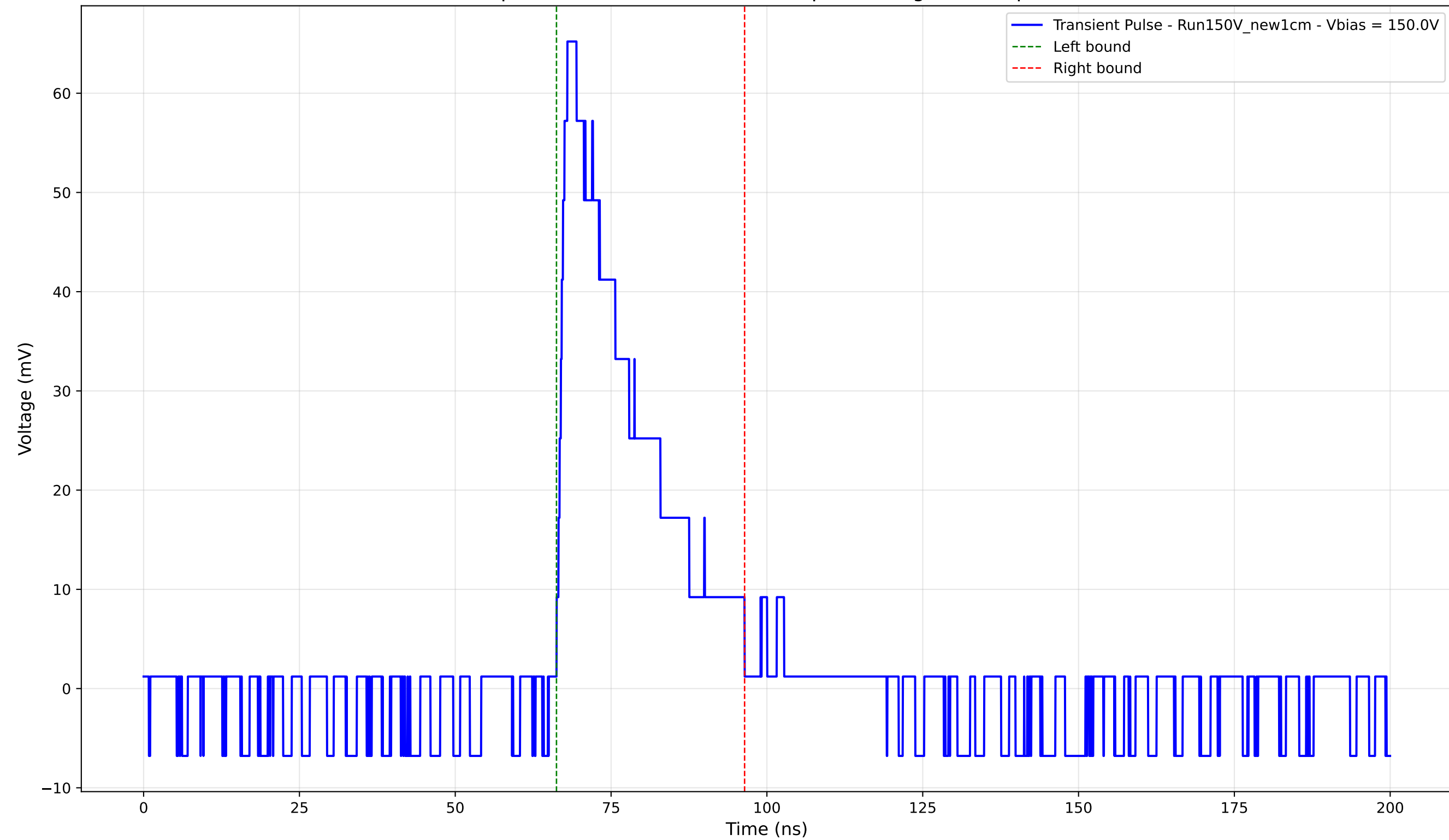
Transient Pulse - Sample: New1cm - Position: 975.0 \mu\text{m} - Charge: 16.37 pC - Rise Time: 1.73 ns
