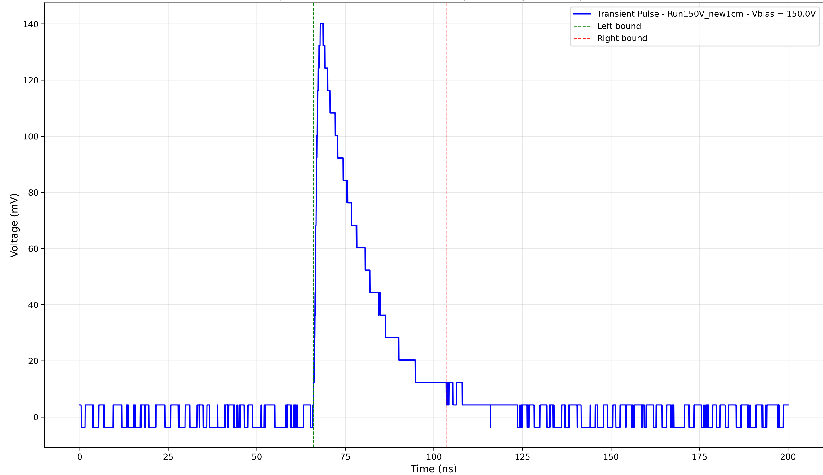
Transient Pulse - Sample: New1cm - Position: 4210.0 \mu\text{m} - Charge: 37.64 pC - Rise Time: 1.42 ns
