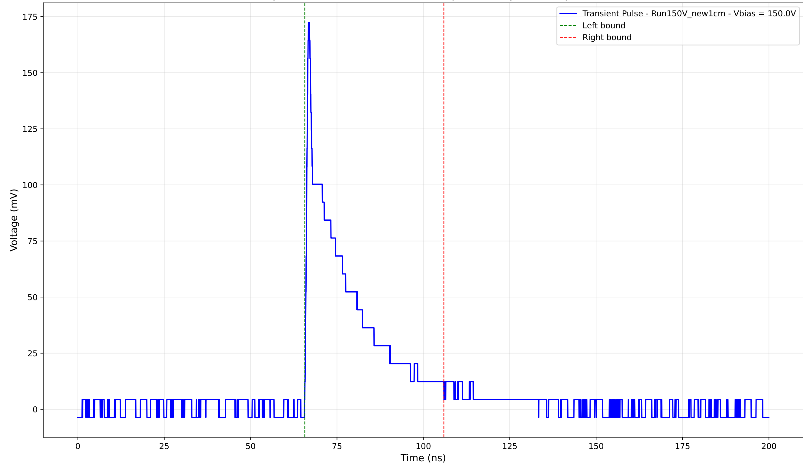
Transient Pulse - Sample: New1cm - Position: 2310.0 \mu\text{m} - Charge: 36.02 pC - Rise Time: 0.79 ns
