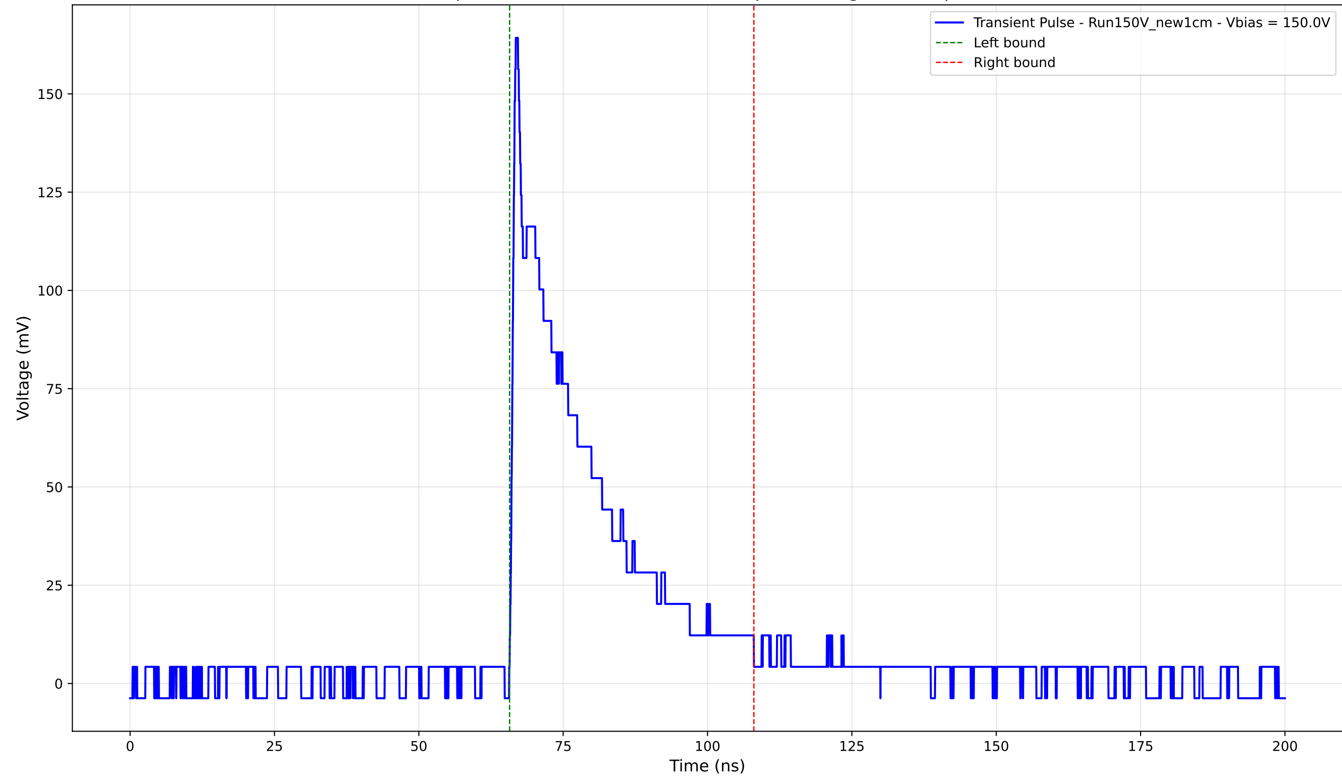
Transient Pulse - Sample: New1cm - Position: 2885.0 \mu\text{m} - Charge: 39.09 pC - Rise Time: 0.79 ns
