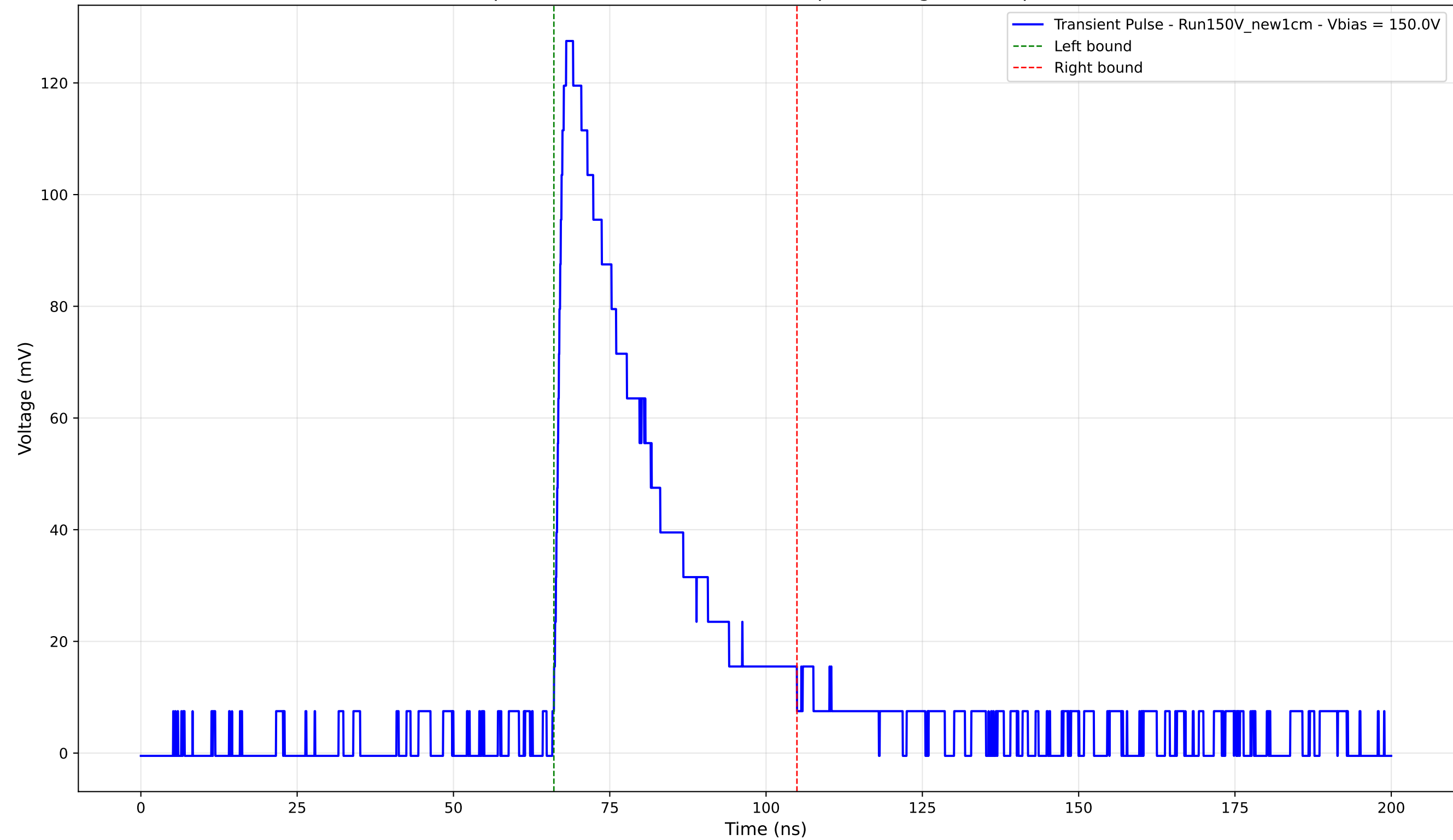
Transient Pulse - Sample: New1cm - Position: 3655.0 \mu\text{m} - Charge: 38.50 pC - Rise Time: 1.57 ns
