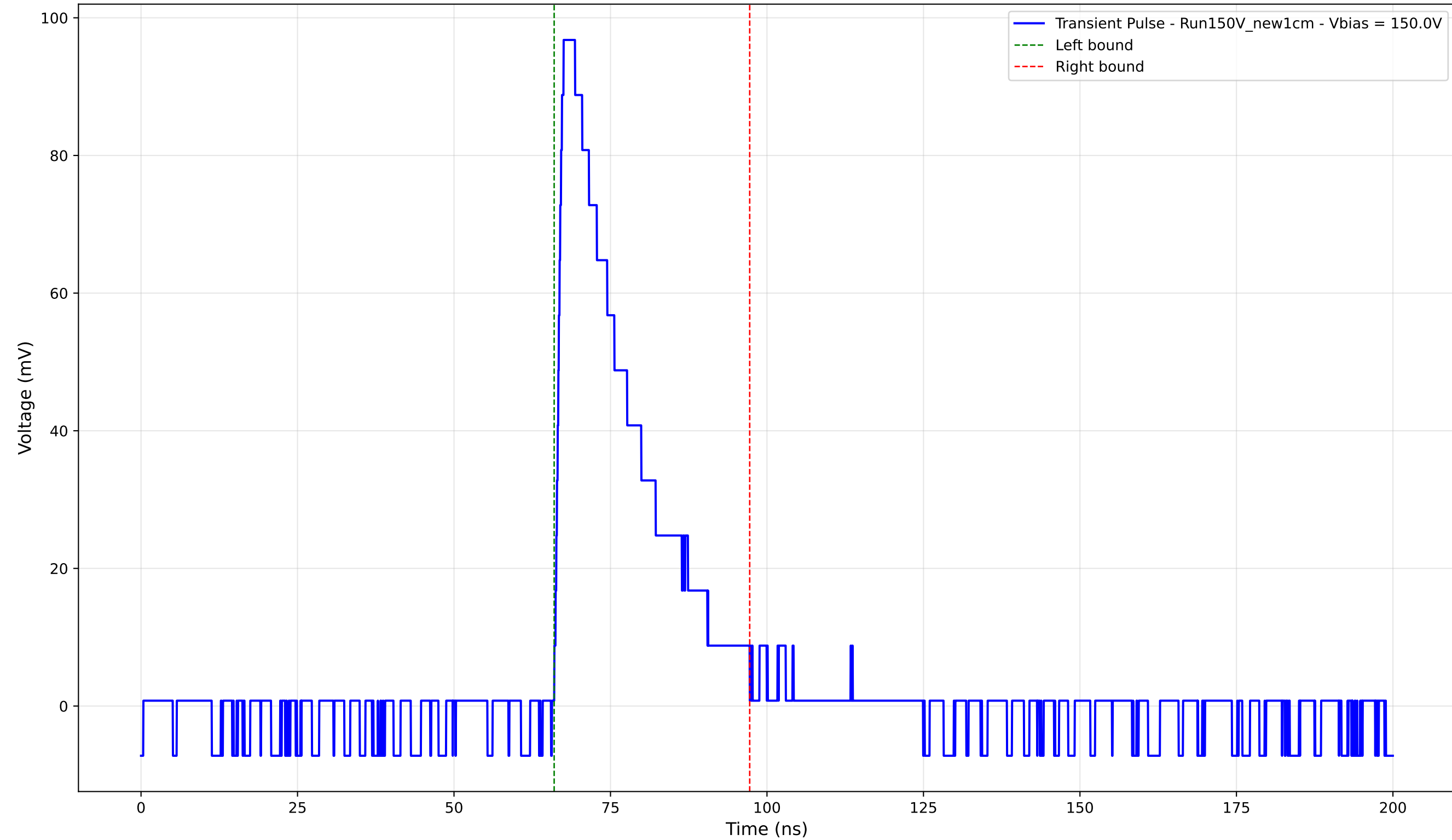
Transient Pulse - Sample: New1cm - Position: 630.0 \mu\text{m} - Charge: 24.21 pC - Rise Time: 1.04 ns
