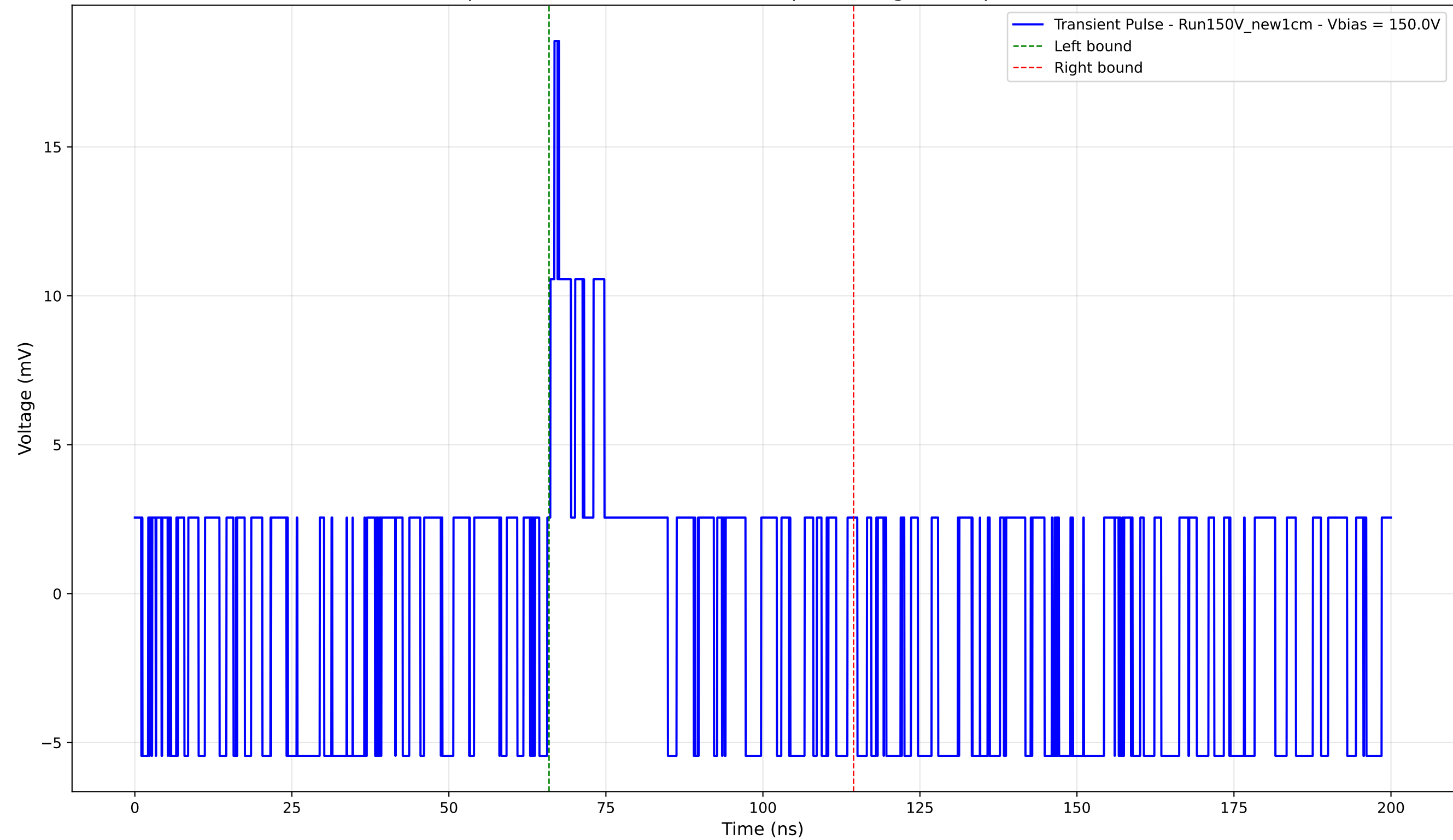
Transient Pulse - Sample: New1cm - Position: 4895.0 \mu\text{m} - Charge: 1.71 pC - Rise Time: 0.00 ns (N/A)
