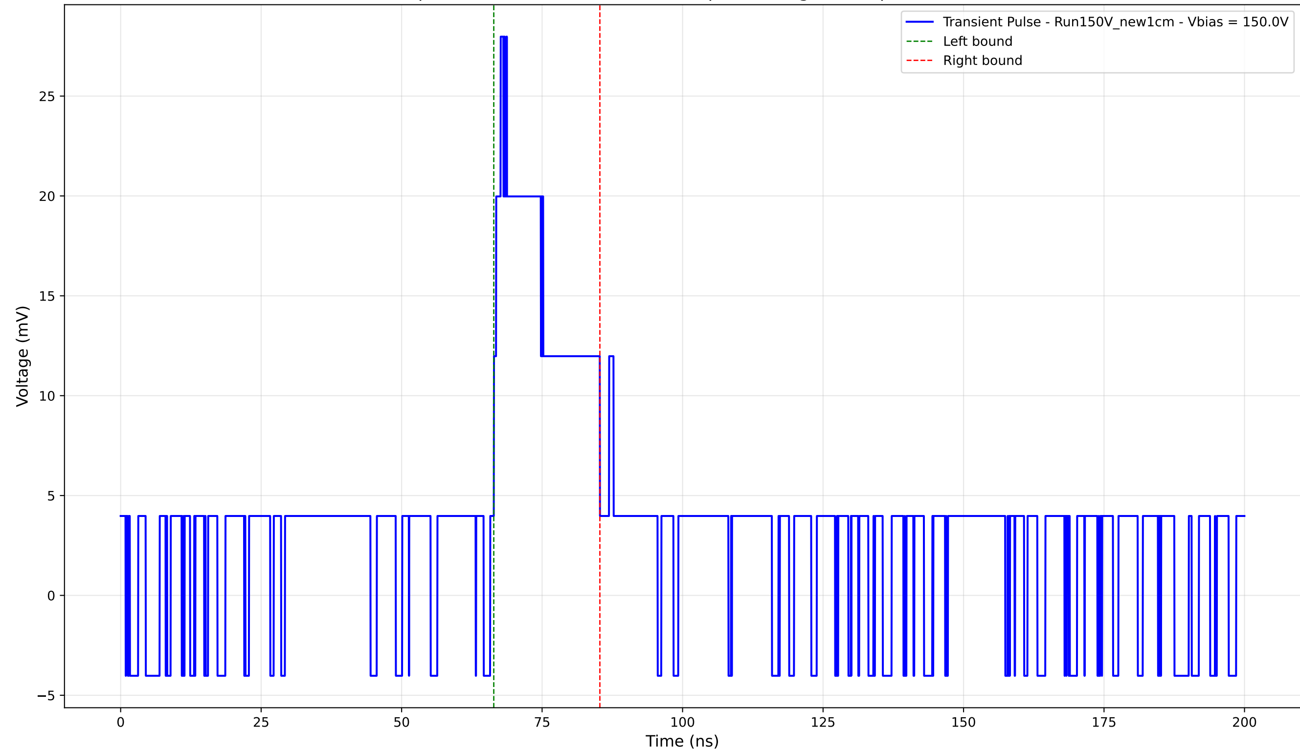
Transient Pulse - Sample: New1cm - Position: 1560.0 \mu\text{m} - Charge: 5.94 pC - Rise Time: 0.00 ns (N/A)
