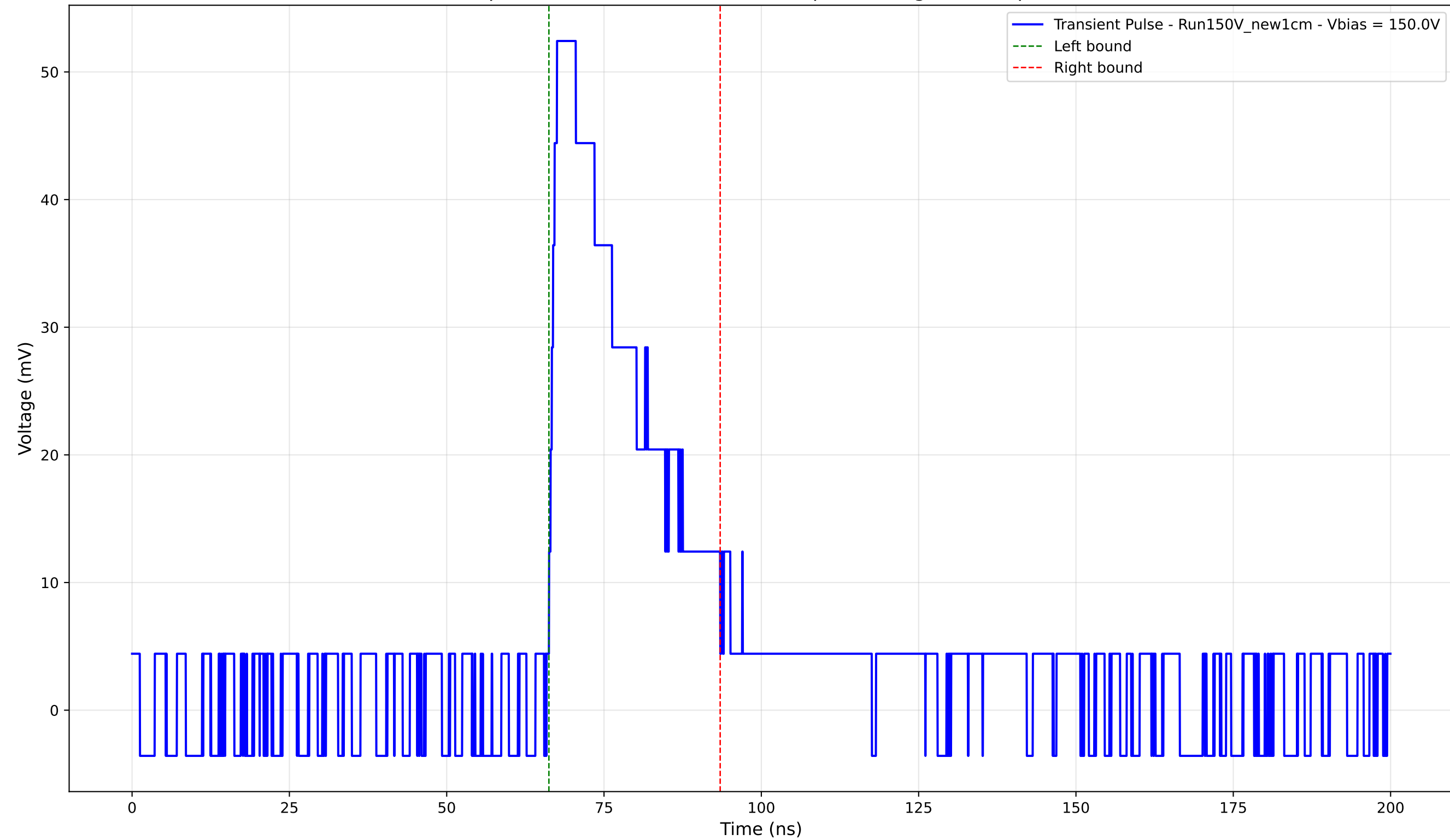
Transient Pulse - Sample: New1cm - Position: 1590.0 \mu\text{m} - Charge: 15.21 pC - Rise Time: 1.28 ns
