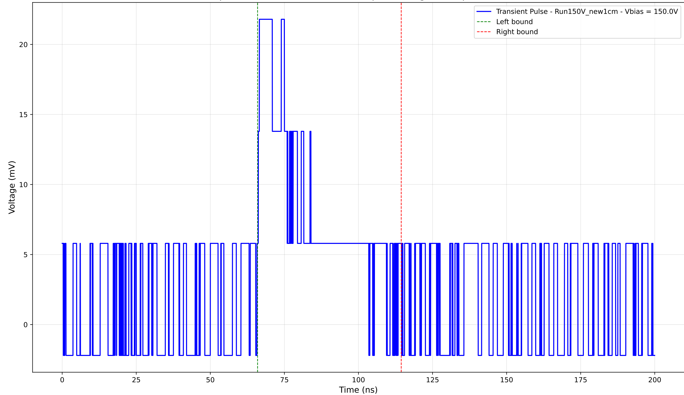
Transient Pulse - Sample: New1cm - Position: 2050.0 \mu\text{m} - Charge: 8.15 pC - Rise Time: 0.00 ns (N/A)
