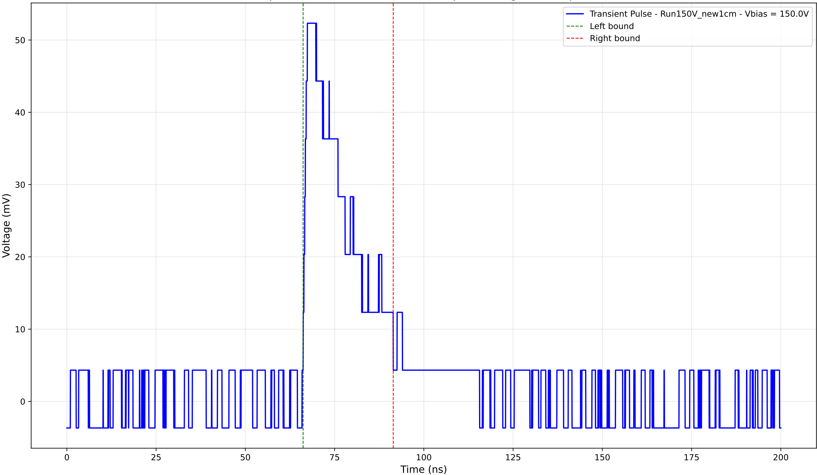
Transient Pulse - Sample: New1cm - Position: 4110.0 \mu\text{m} - Charge: 13.55 pC - Rise Time: 1.18 ns
