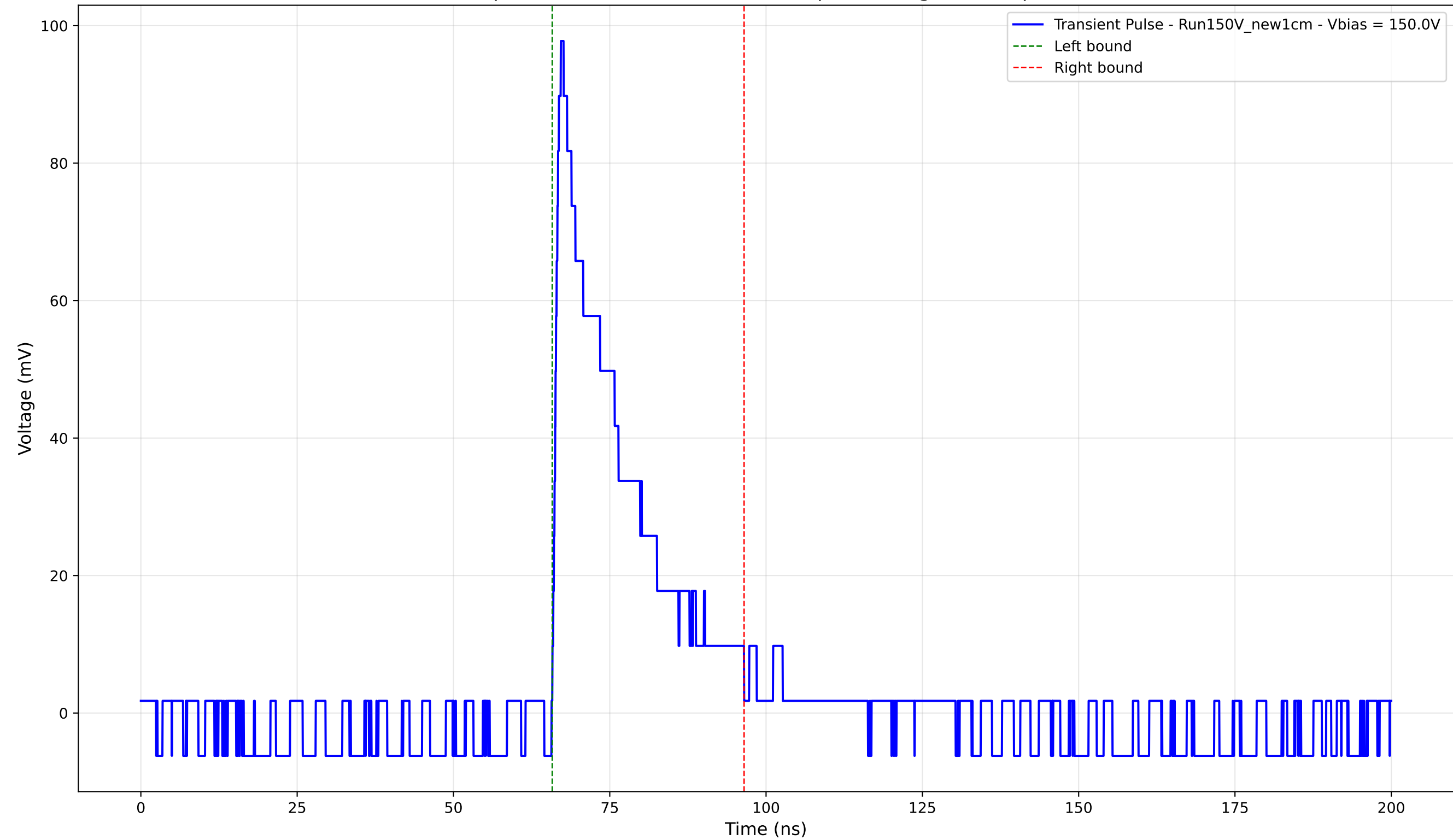
Transient Pulse - Sample: New1cm - Position: 4635.0 \mu\text{m} - Charge: 20.46 pC - Rise Time: 0.92 ns
