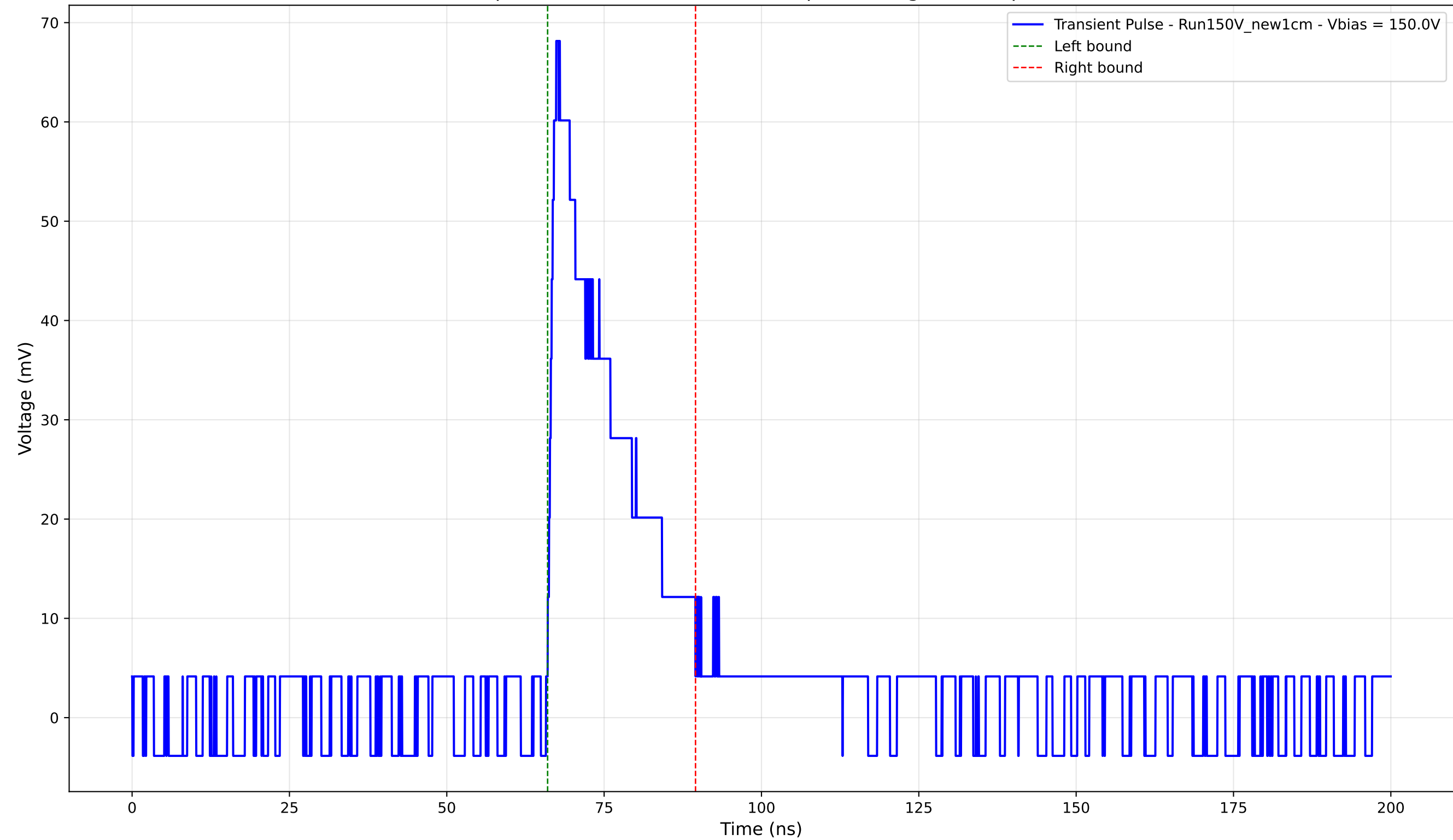
Transient Pulse - Sample: New1cm - Position: 475.0 \mu\text{m} - Charge: 14.26 pC - Rise Time: 1.35 ns
