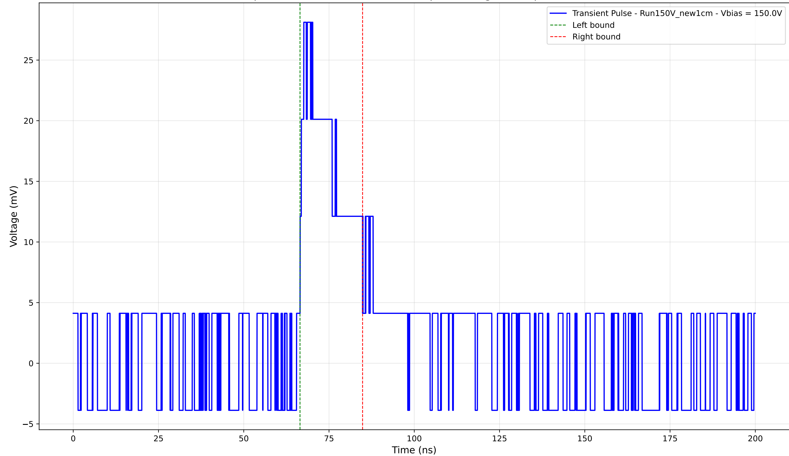
Transient Pulse - Sample: New1cm - Position: 3580.0 \mu\text{m} - Charge: 6.26 pC - Rise Time: 0.00 ns (N/A)
