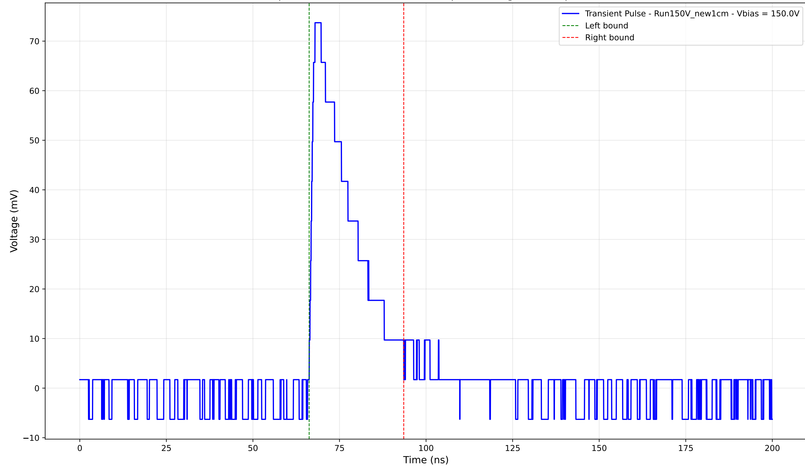
Transient Pulse - Sample: New1cm - Position: 965.0 \mu\text{m} - Charge: 18.43 pC - Rise Time: 1.67 ns
