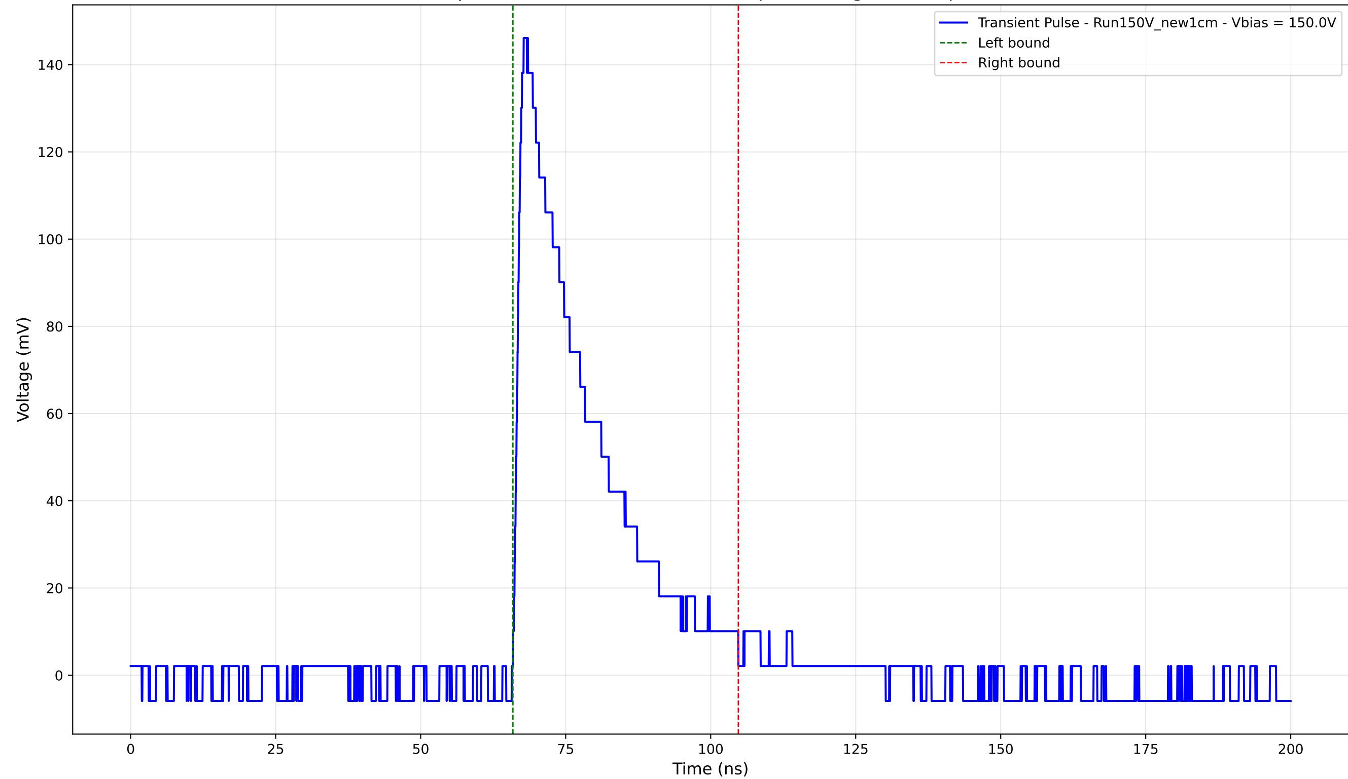
Transient Pulse - Sample: New1cm - Position: 4235.0 \mu\text{m} - Charge: 38.40 pC - Rise Time: 1.41 ns
