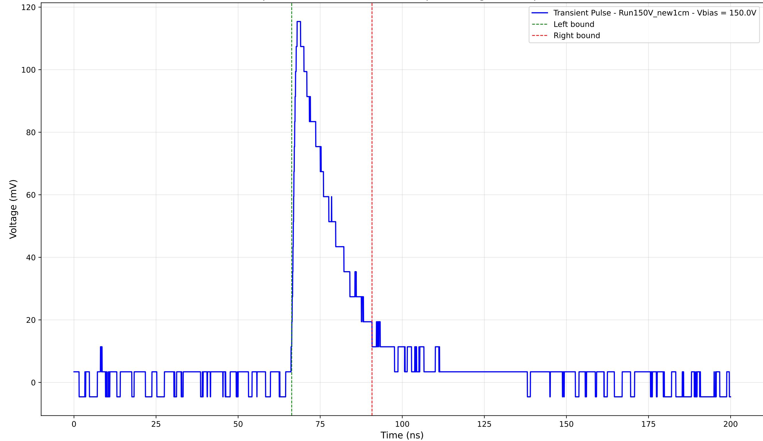
Transient Pulse - Sample: New1cm - Position: 885.0 \mu\text{m} - Charge: 27.62 pC - Rise Time: 1.36 ns
