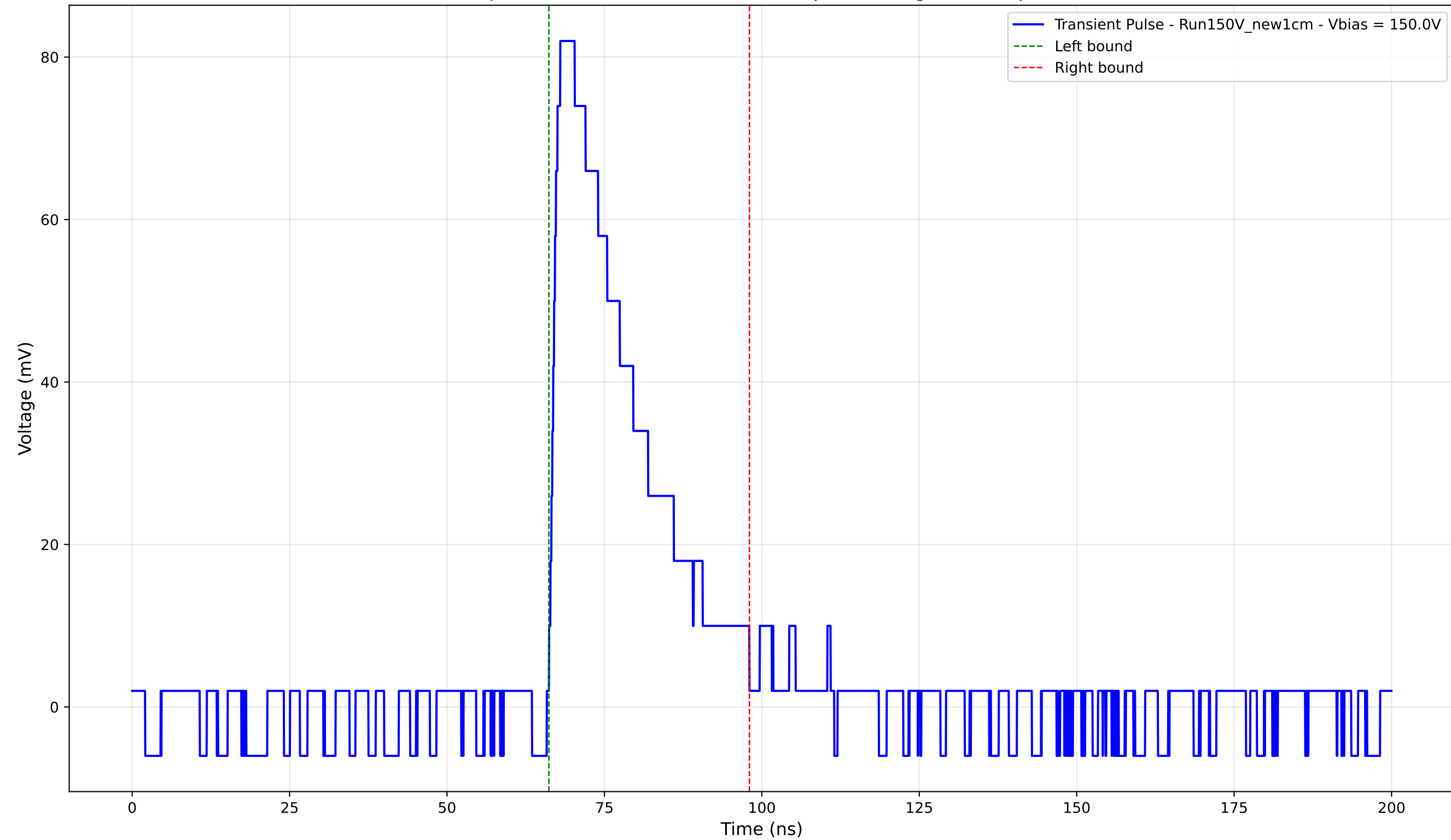
Transient Pulse - Sample: New1cm - Position: 1115.0 \mu\text{m} - Charge: 22.93 pC - Rise Time: 1.34 ns
