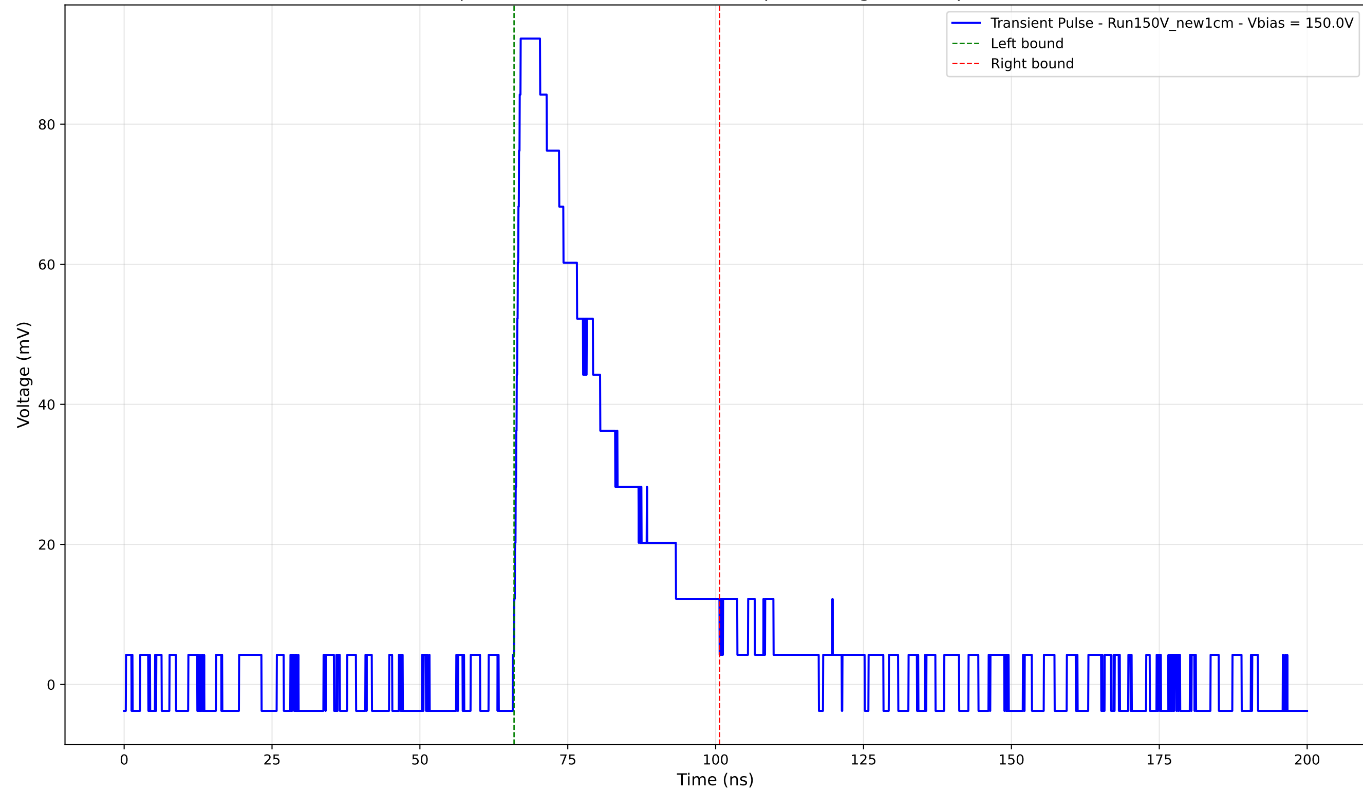
Transient Pulse - Sample: New1cm - Position: 1890.0 \mu\text{m} - Charge: 28.35 pC - Rise Time: 0.93 ns
