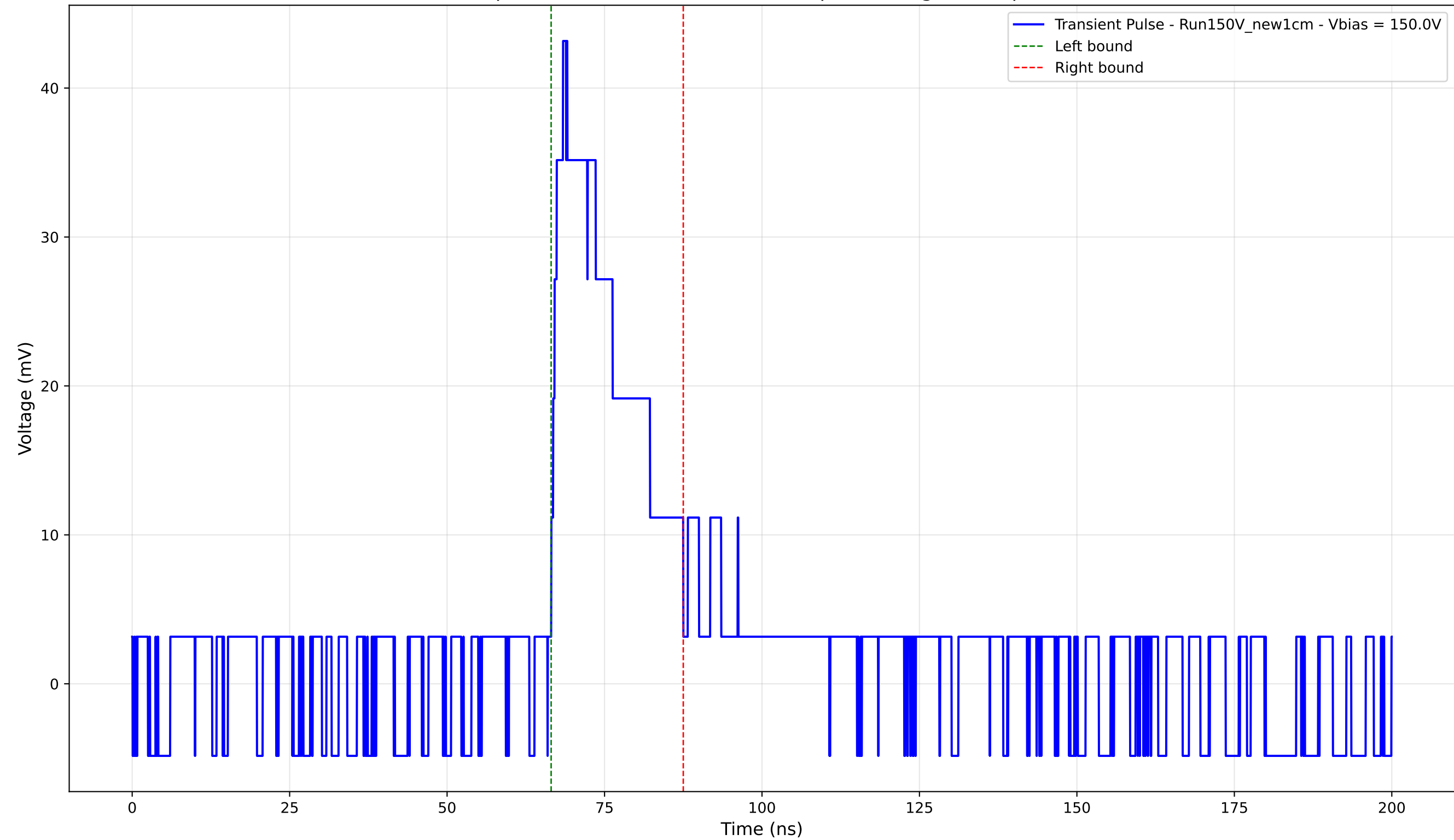
Transient Pulse - Sample: New1cm - Position: 1500.0 \mu\text{m} - Charge: 9.69 pC - Rise Time: 1.88 ns
