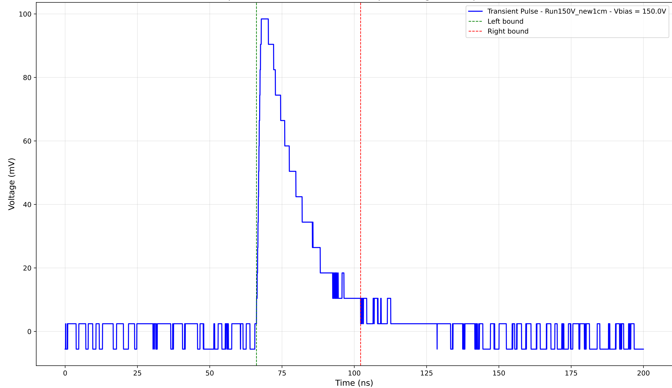
Transient Pulse - Sample: New1cm - Position: 1155.0 \mu\text{m} - Charge: 29.15 pC - Rise Time: 1.38 ns
