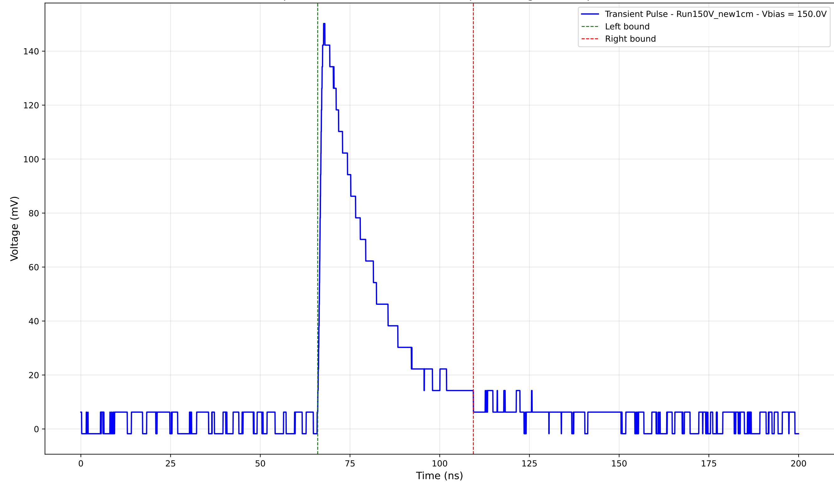
Transient Pulse - Sample: New1cm - Position: 3445.0 \mu\text{m} - Charge: 44.62 pC - Rise Time: 1.24 ns
