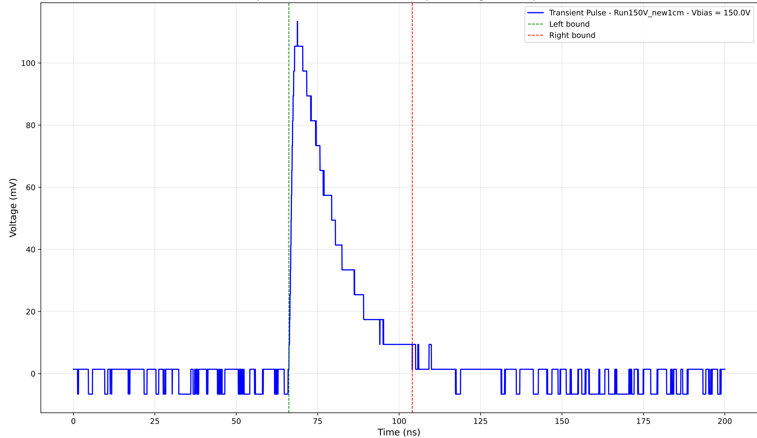
Transient Pulse - Sample: New1cm - Position: 1330.0 \mu\text{m} - Charge: 31.14 pC - Rise Time: 1.56 ns
