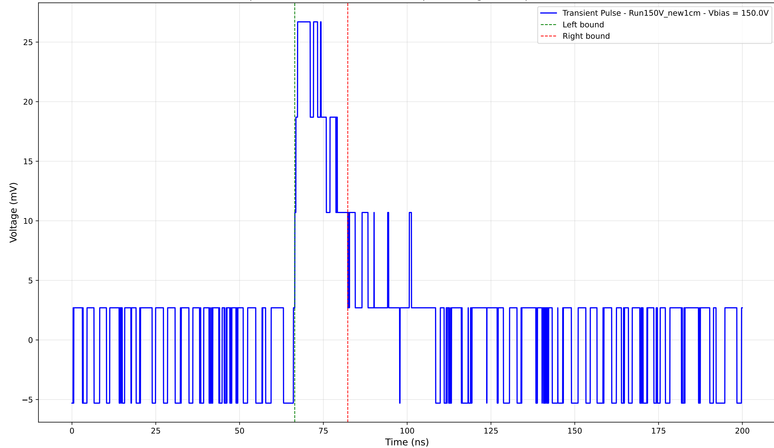
Transient Pulse - Sample: New1cm - Position: 1005.0 \mu\text{m} - Charge: 5.97 pC - Rise Time: 0.00 ns (N/A)
