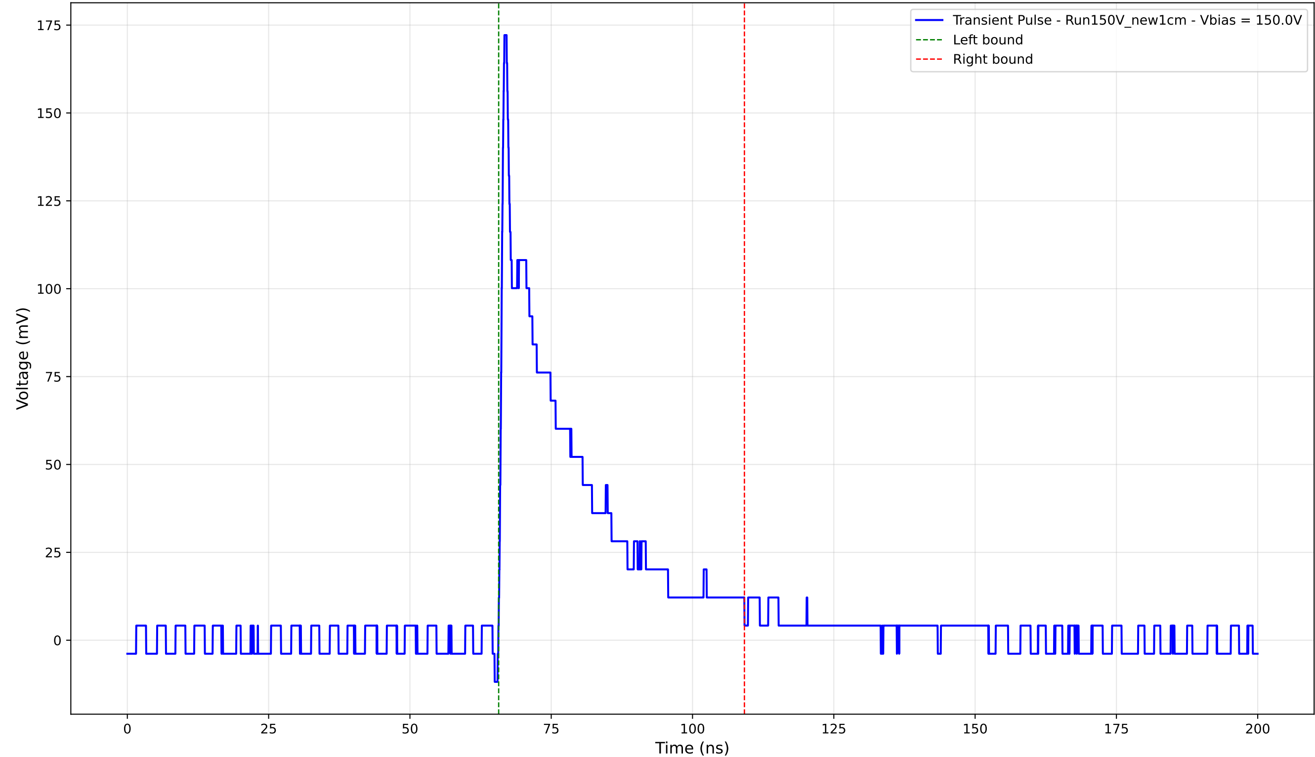
Transient Pulse - Sample: New1cm - Position: 2305.0 \mu\text{m} - Charge: 36.78 pC - Rise Time: 0.77 ns
