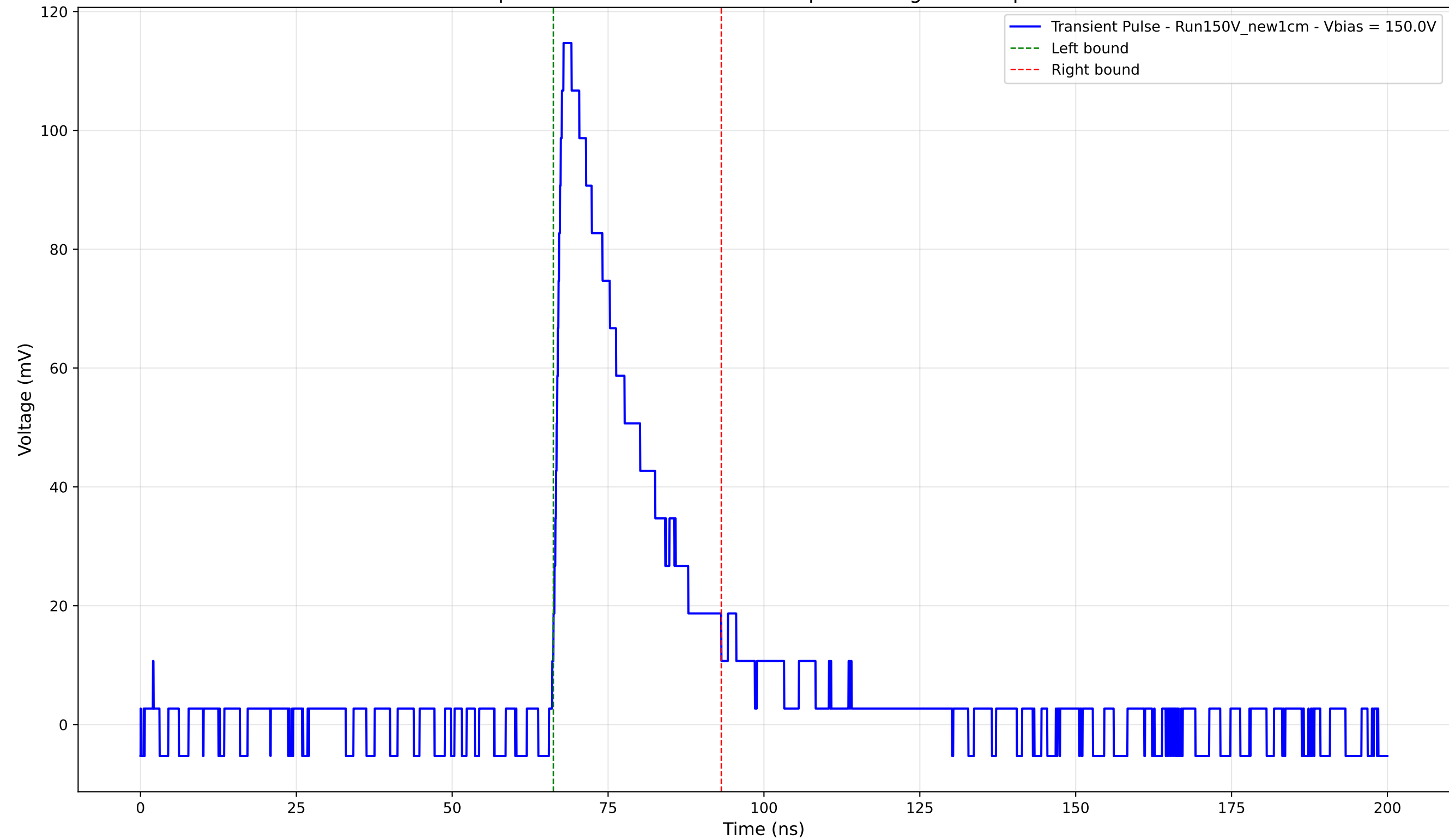
Transient Pulse - Sample: New1cm - Position: 865.0 \mu\text{m} - Charge: 28.94 pC - Rise Time: 1.36 ns
