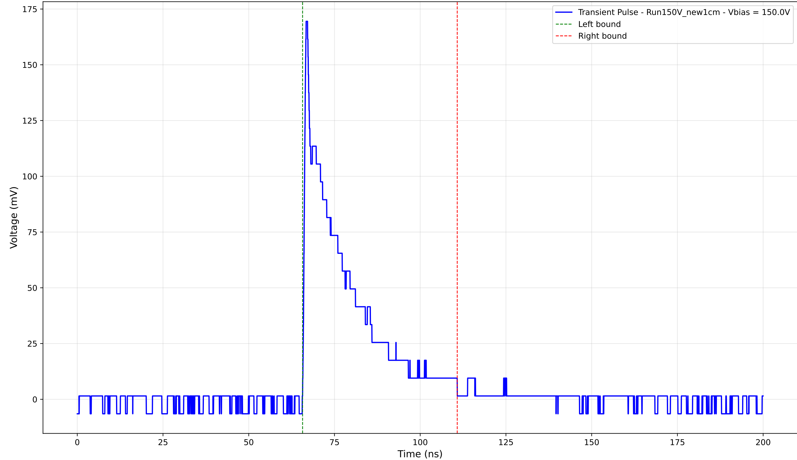
Transient Pulse - Sample: New1cm - Position: 2840.0 \mu\text{m} - Charge: 37.12 pC - Rise Time: 0.78 ns
