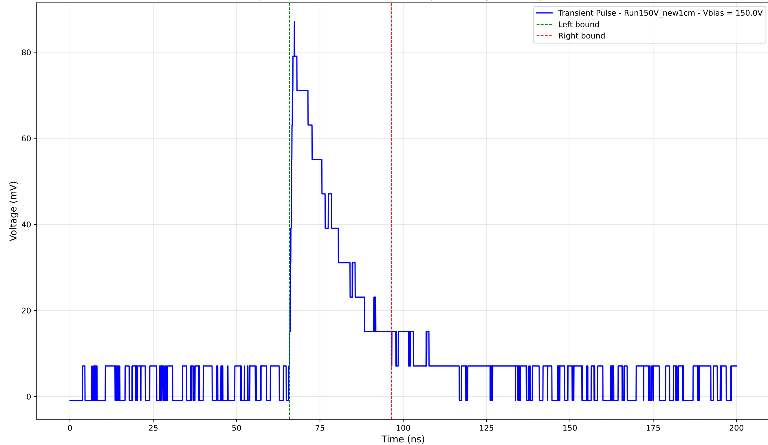
Transient Pulse - Sample: New1cm - Position: 1965.0 \mu\text{m} - Charge: 23.32 pC - Rise Time: 1.00 ns
