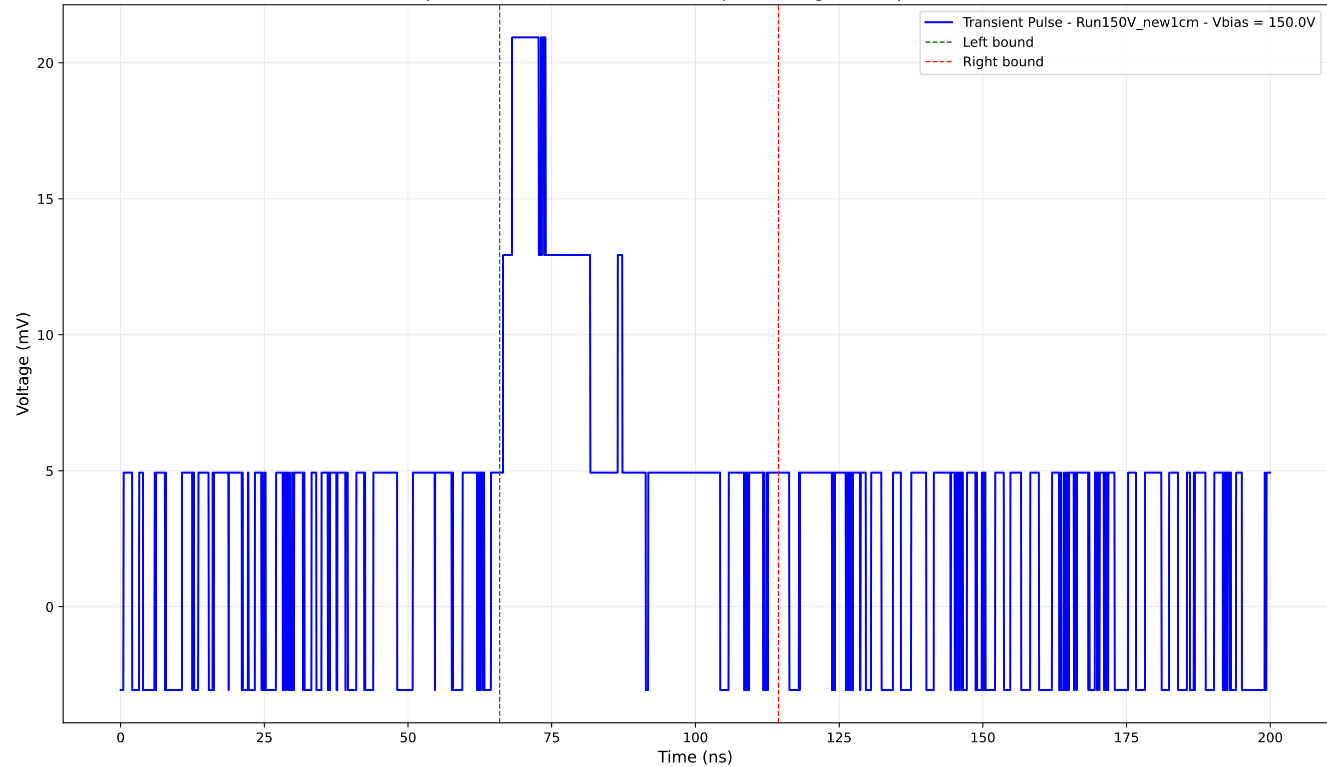
Transient Pulse - Sample: New1cm - Position: 3555.0 \mu\text{m} - Charge: 7.69 pC - Rise Time: 0.00 ns (N/A)
