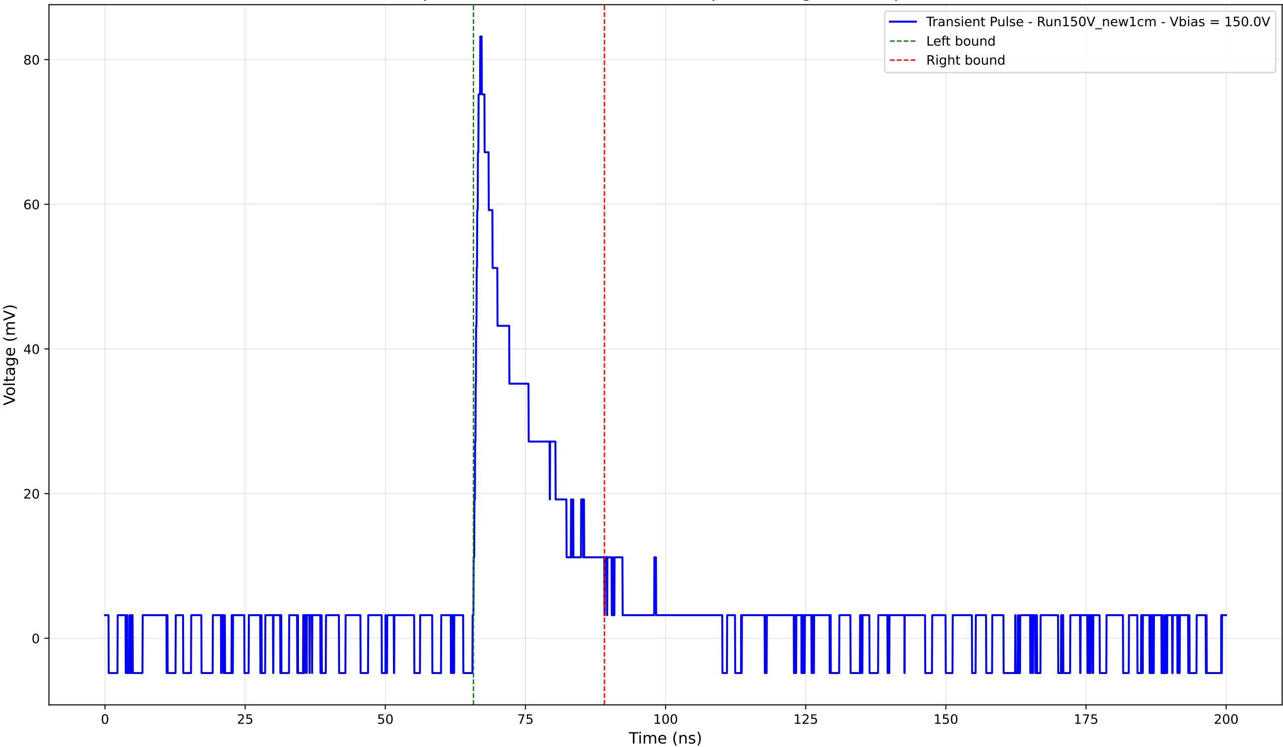
Transient Pulse - Sample: New1cm - Position: 4850.0 \mu\text{m} - Charge: 14.28 pC - Rise Time: 0.89 ns
