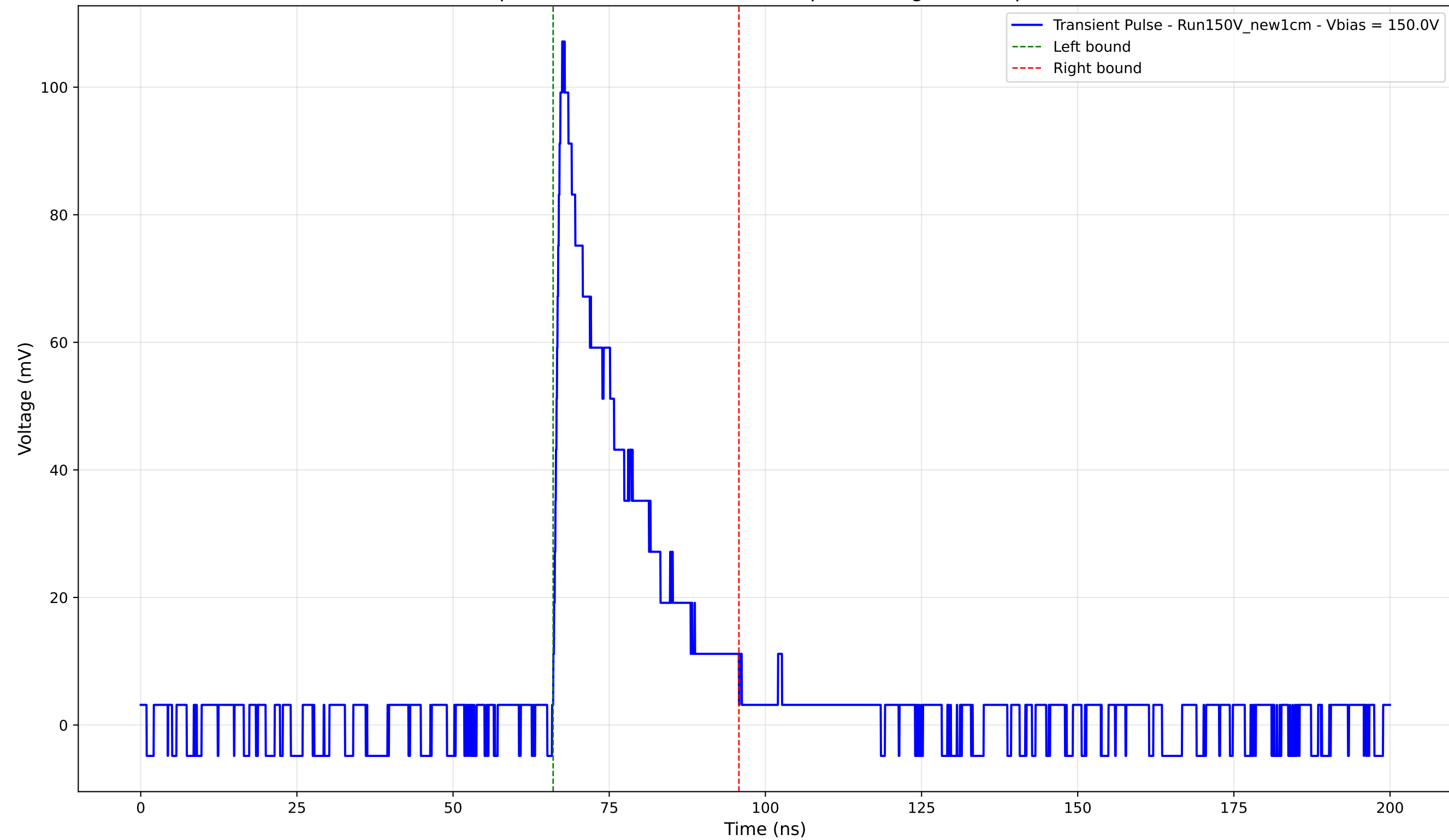
Transient Pulse - Sample: New1cm - Position: 445.0 \mu\text{m} - Charge: 22.42 pC - Rise Time: 1.14 ns
