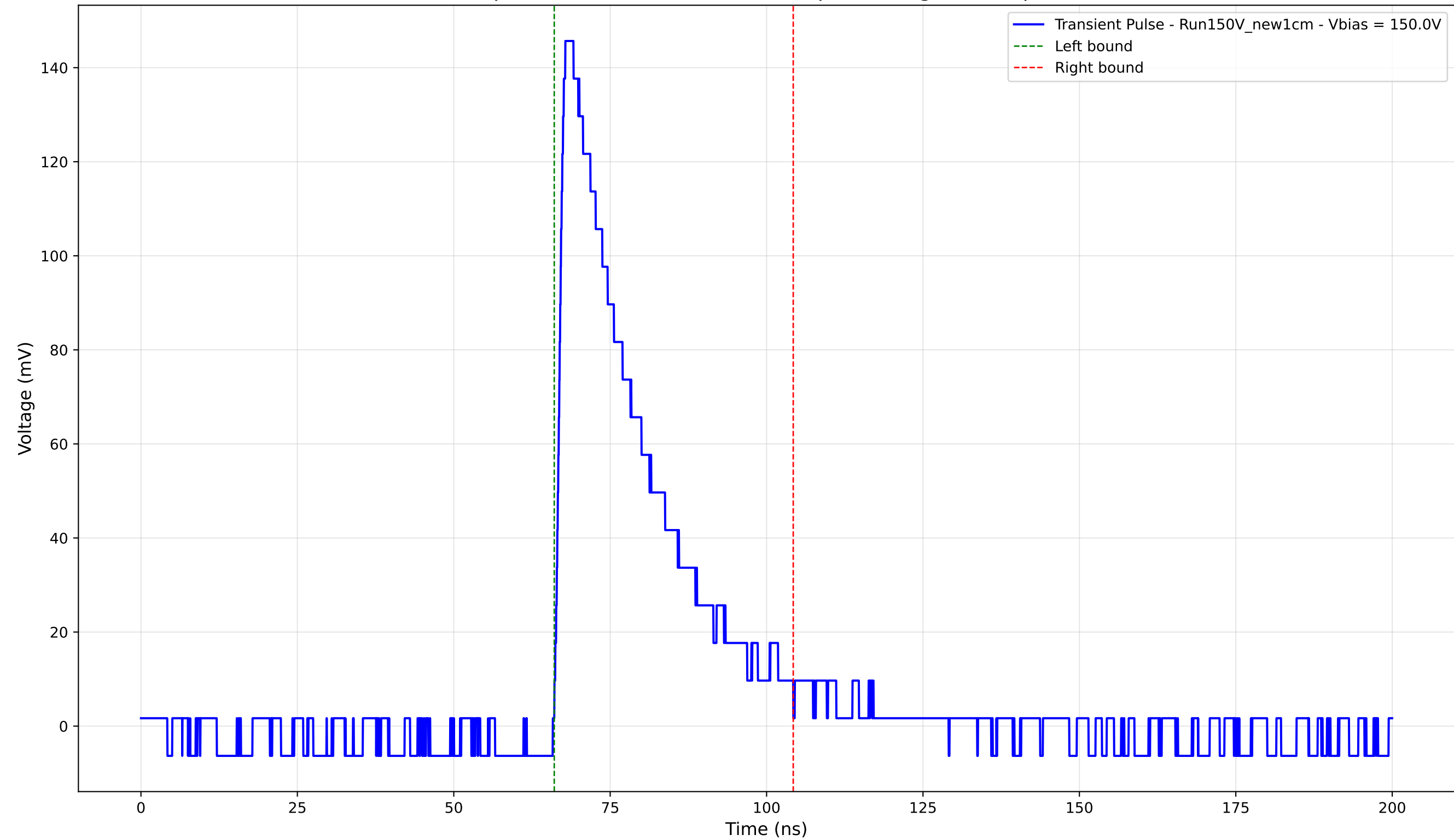
Transient Pulse - Sample: New1cm - Position: 3830.0 \mu\text{m} - Charge: 40.59 pC - Rise Time: 1.37 ns
