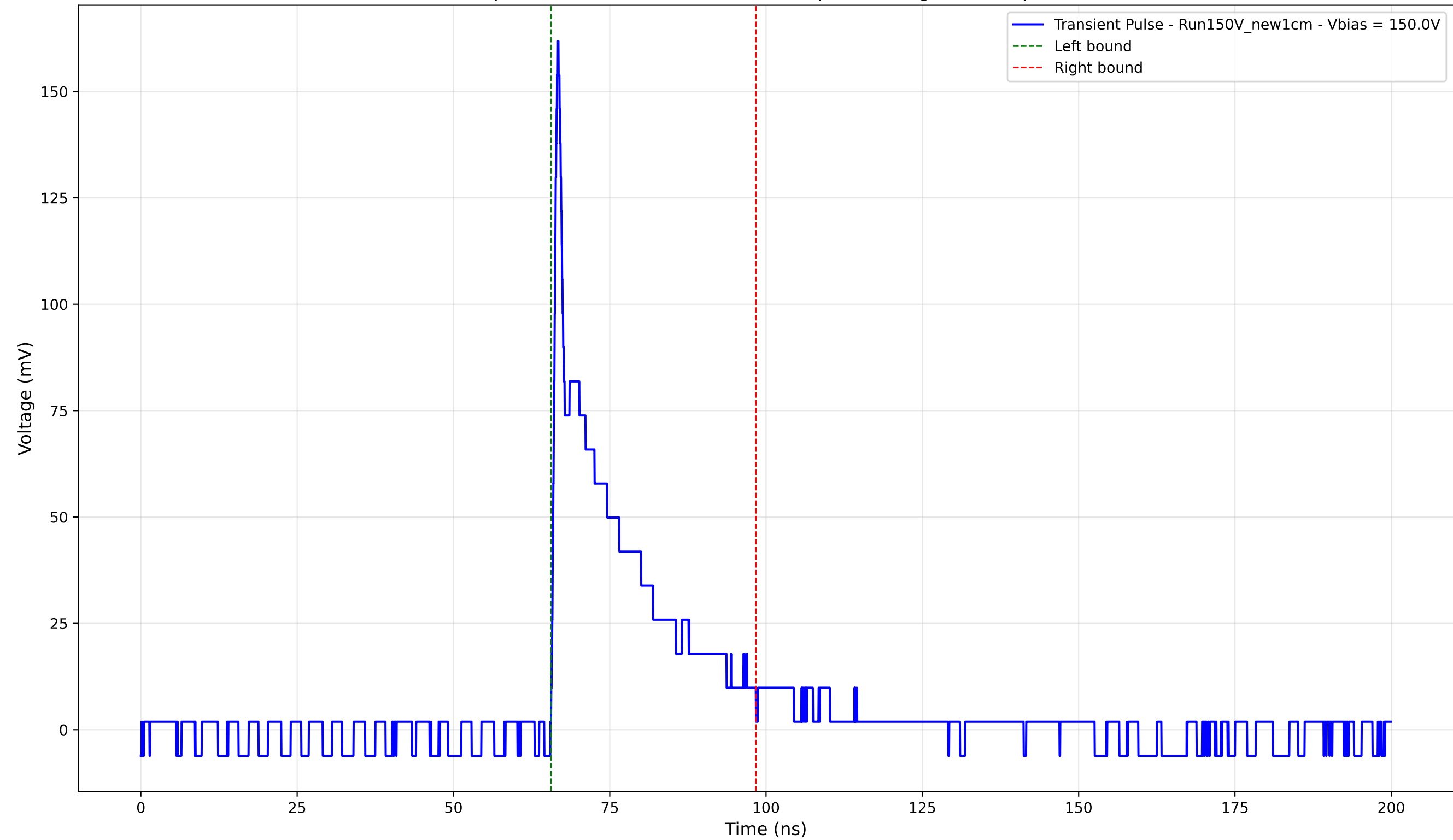
Transient Pulse - Sample: New1cm - Position: 2630.0 \mu\text{m} - Charge: 26.02 pC - Rise Time: 0.78 ns
