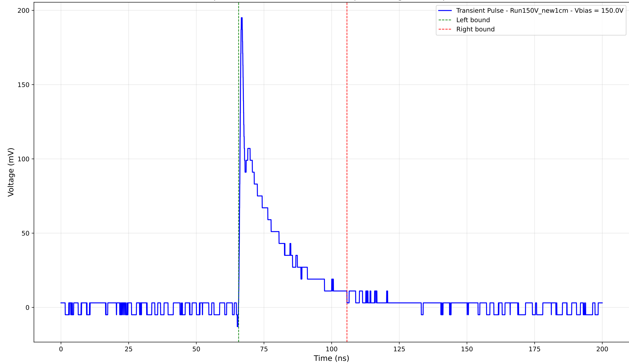
Transient Pulse - Sample: New1cm - Position: 2430.0 \mu\text{m} - Charge: 35.81 pC - Rise Time: 0.74 ns
