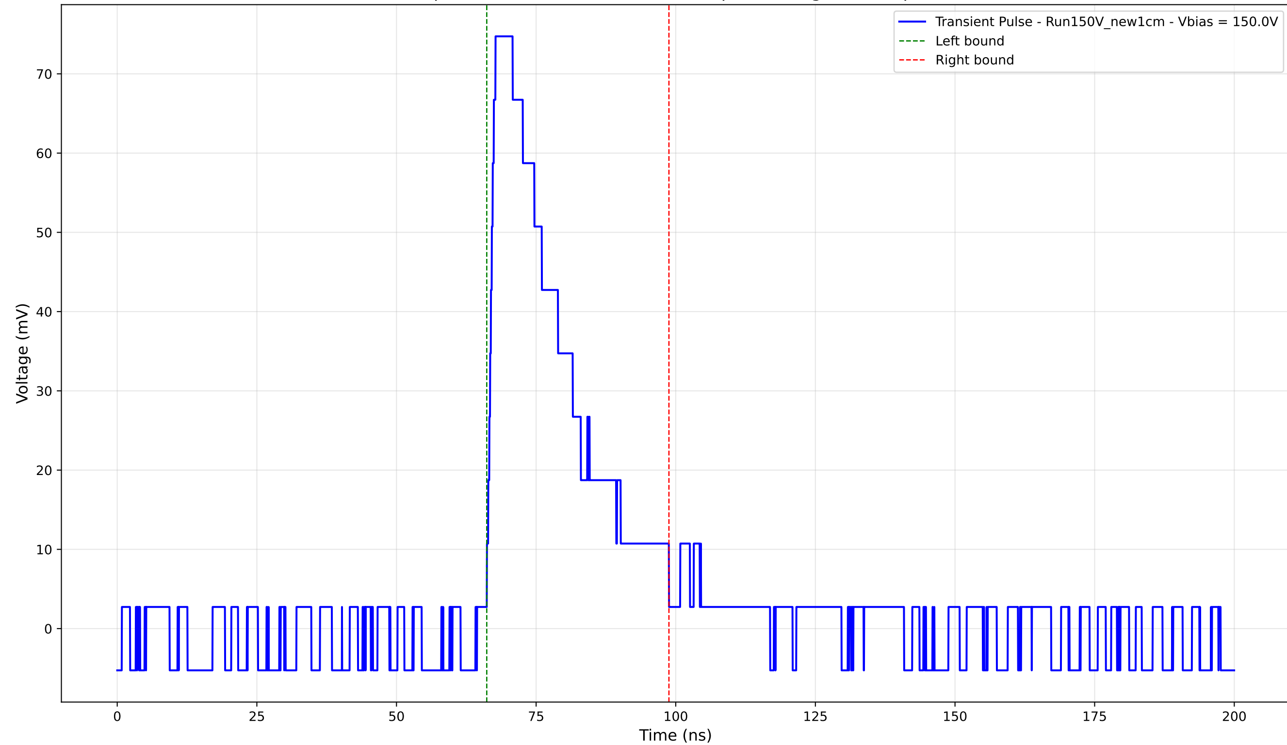
Transient Pulse - Sample: New1cm - Position: 1470.0 \mu\text{m} - Charge: 21.67 pC - Rise Time: 1.55 ns
