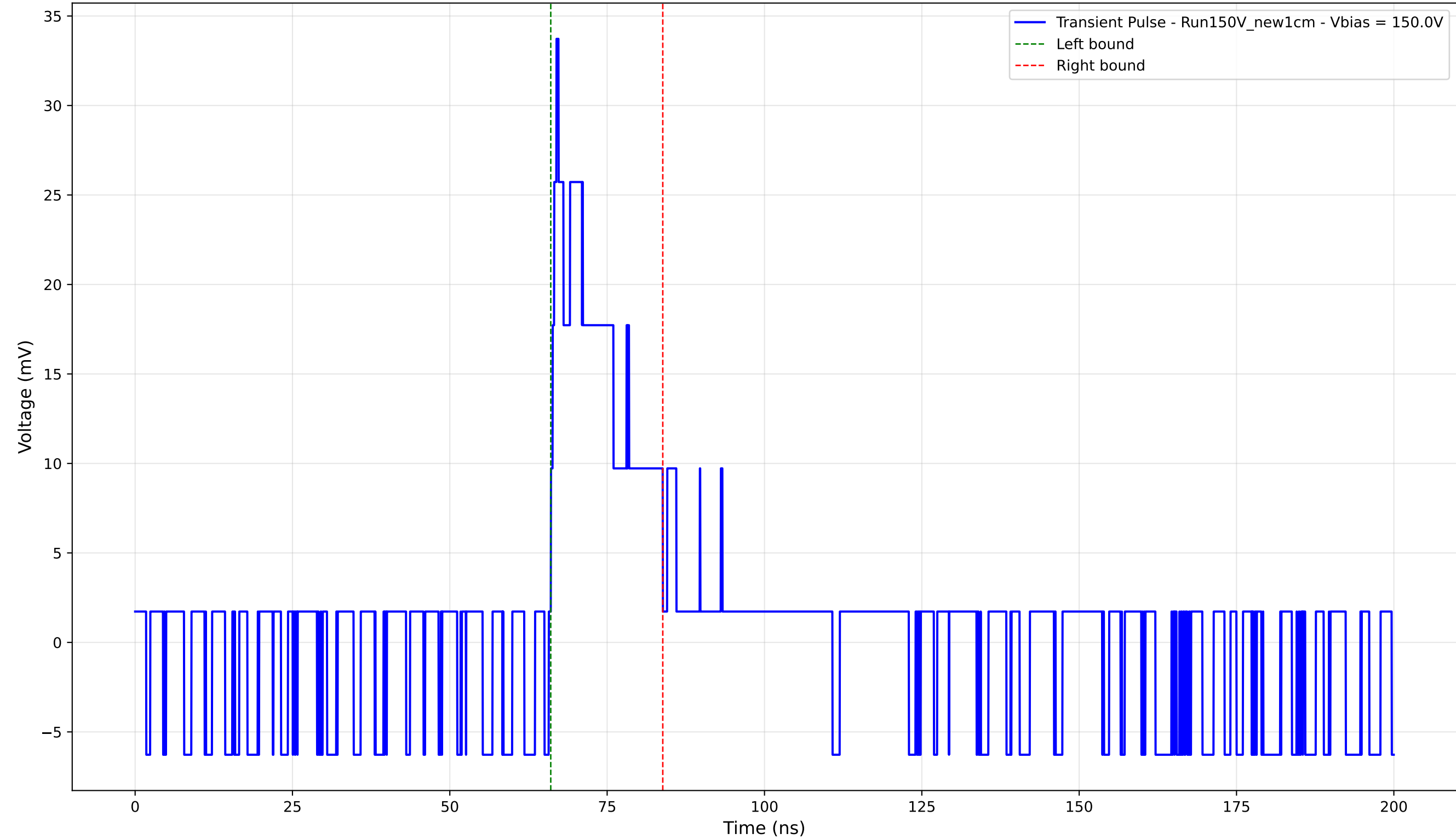
Transient Pulse - Sample: New1cm - Position: 3040.0 \mu\text{m} - Charge: 5.67 pC - Rise Time: 0.90 ns
