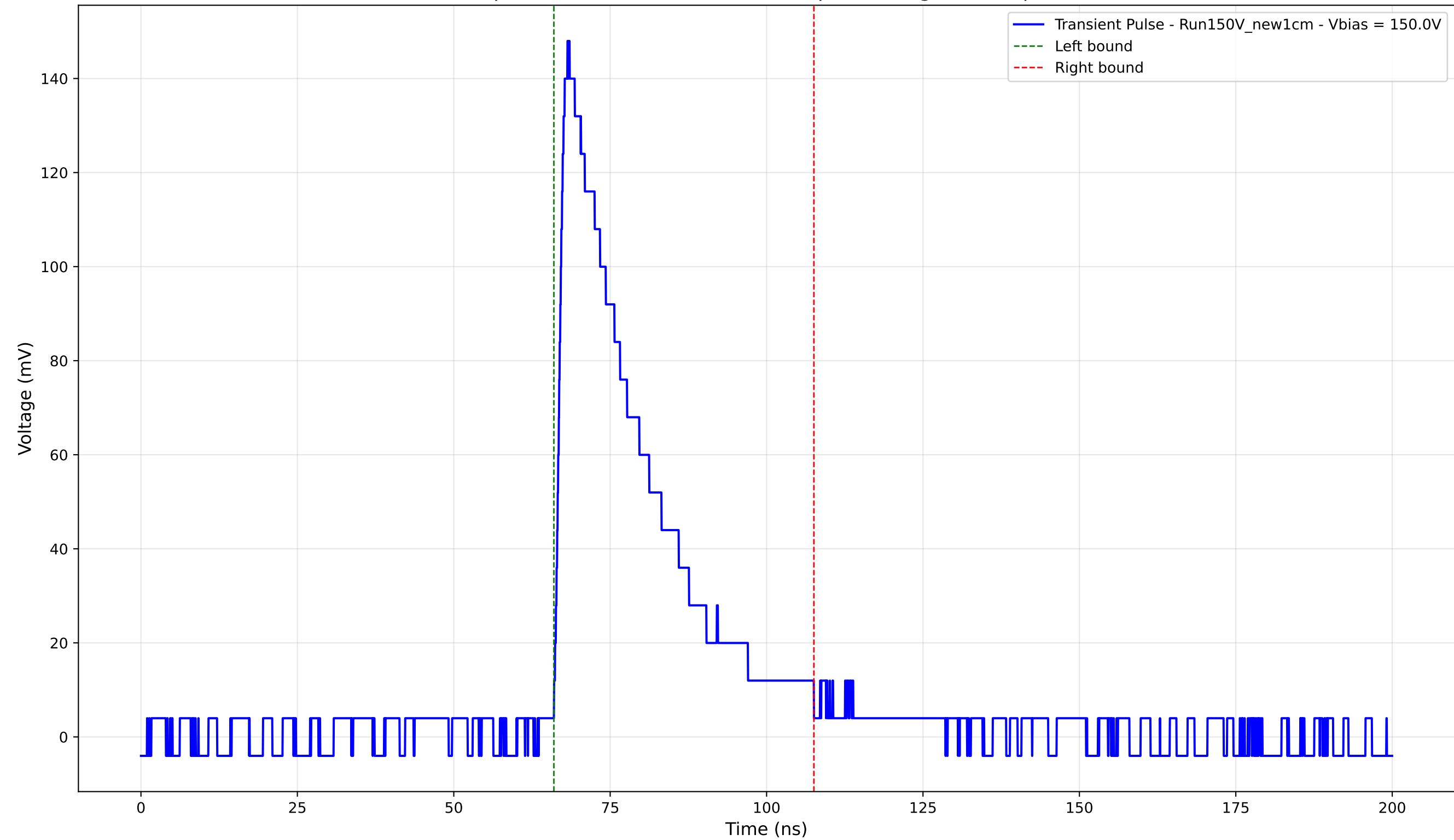
Transient Pulse - Sample: New1cm - Position: 3935.0 \mu\text{m} - Charge: 41.27 pC - Rise Time: 1.55 ns
