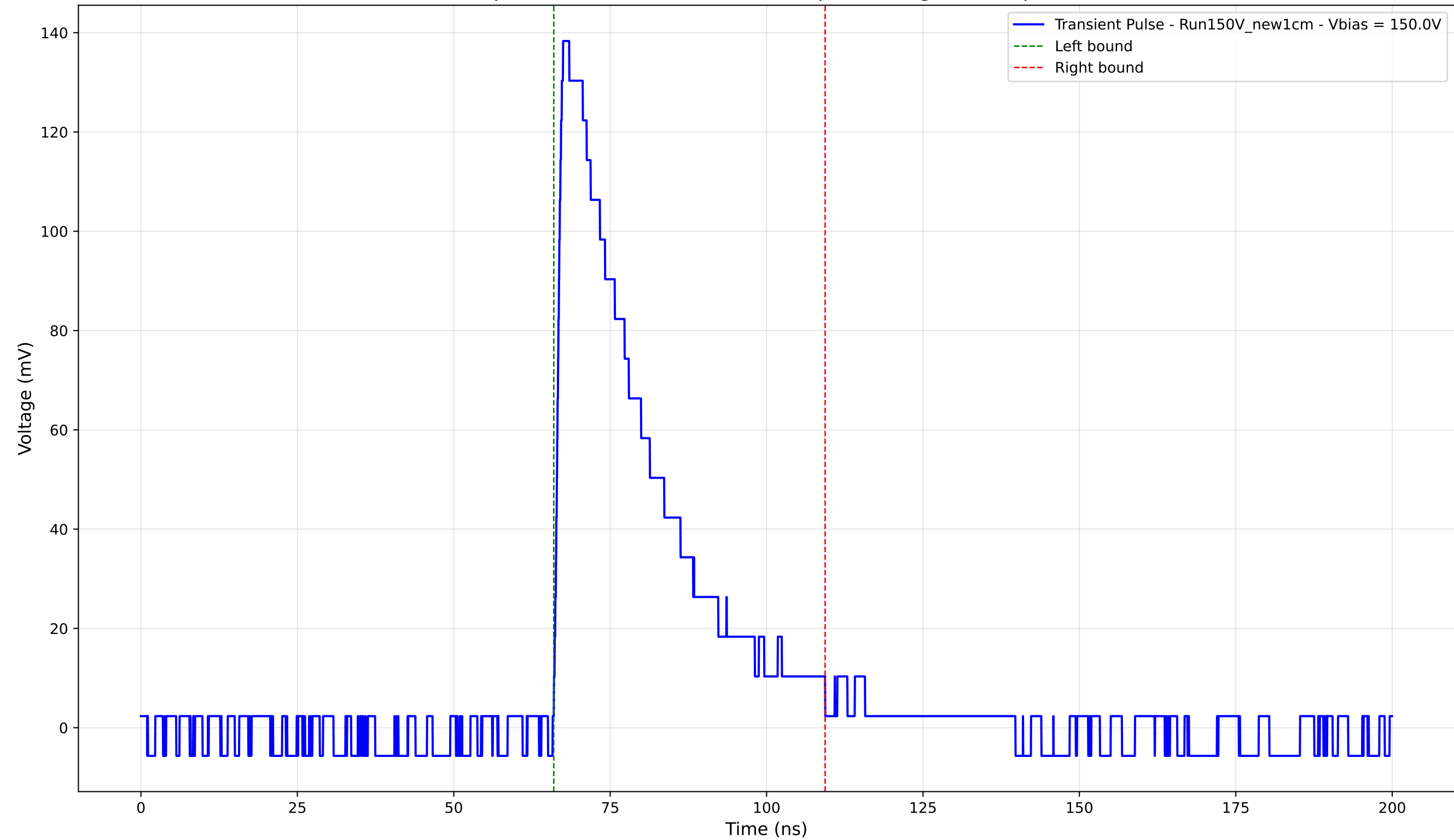
Transient Pulse - Sample: New1cm - Position: 3400.0 \mu\text{m} - Charge: 41.71 pC - Rise Time: 1.15 ns
