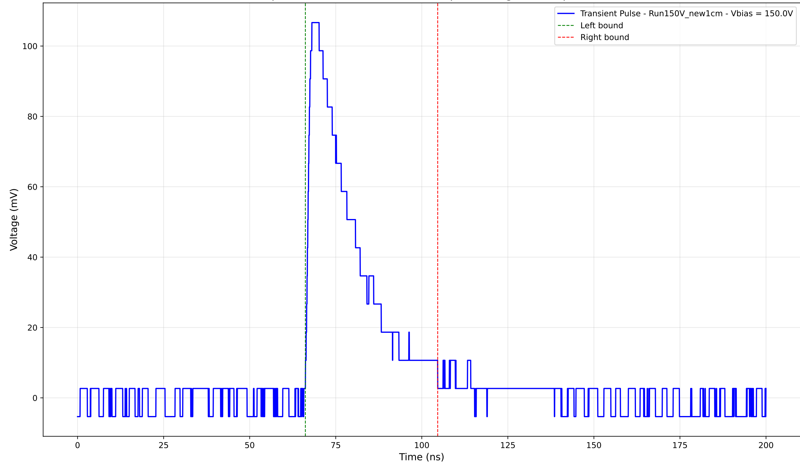
Transient Pulse - Sample: New1cm - Position: 1350.0 \mu\text{m} - Charge: 31.06 pC - Rise Time: 1.30 ns
