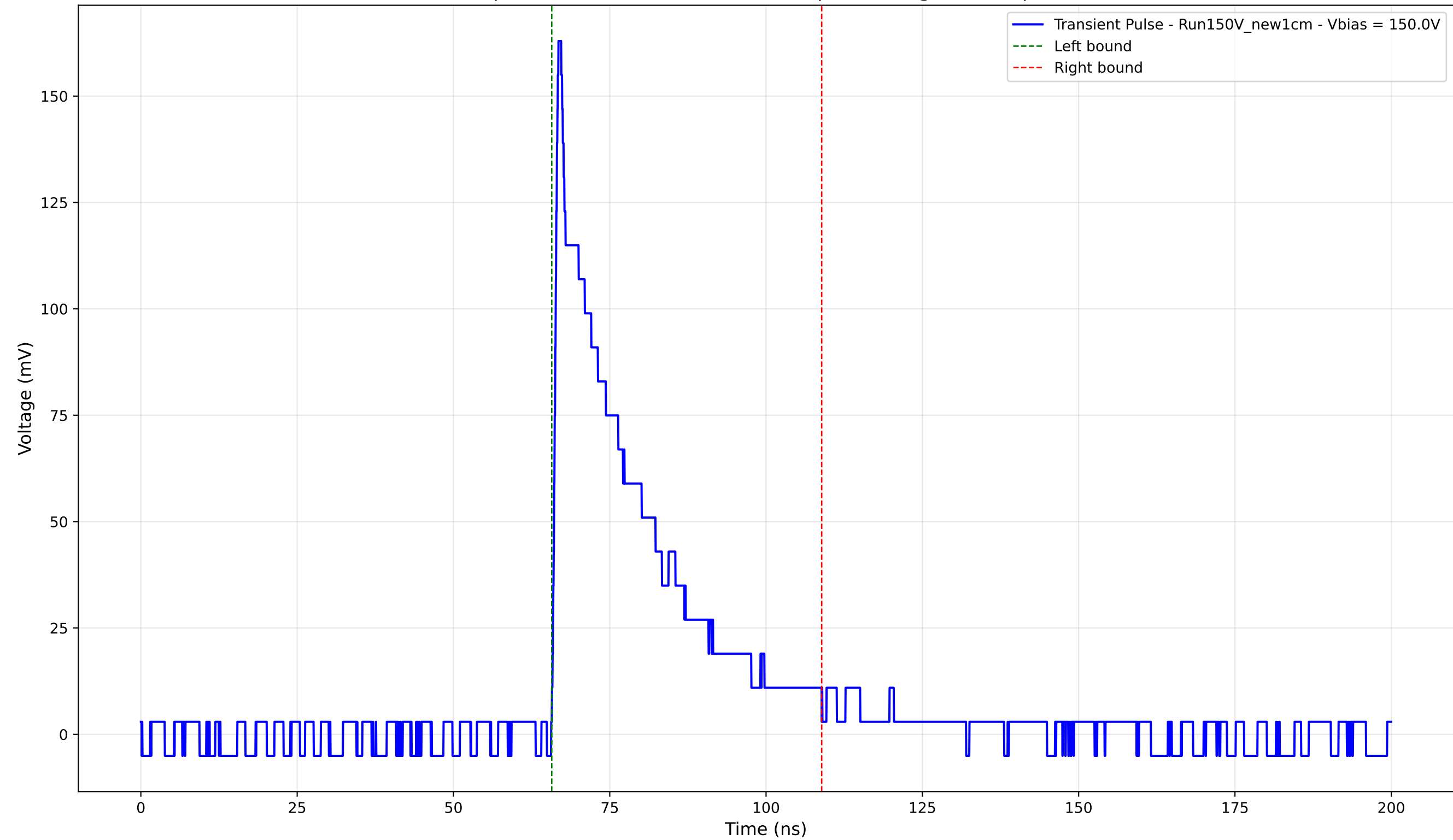
Transient Pulse - Sample: New1cm - Position: 2890.0 \mu\text{m} - Charge: 38.79 pC - Rise Time: 0.79 ns
