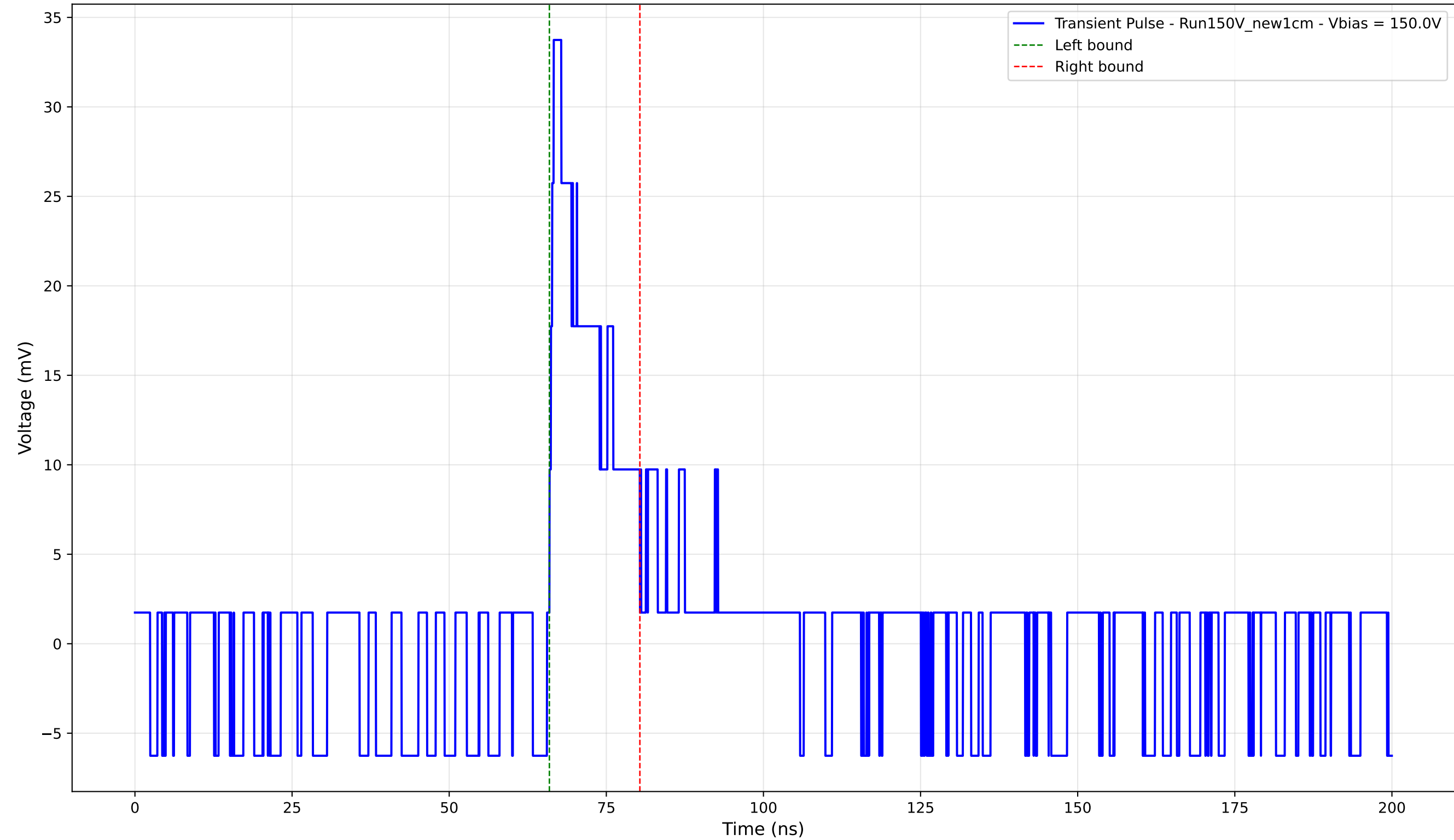
Transient Pulse - Sample: New1cm - Position: 60.0 \mu\text{m} - Charge: 4.93 pC - Rise Time: 0.68 ns
