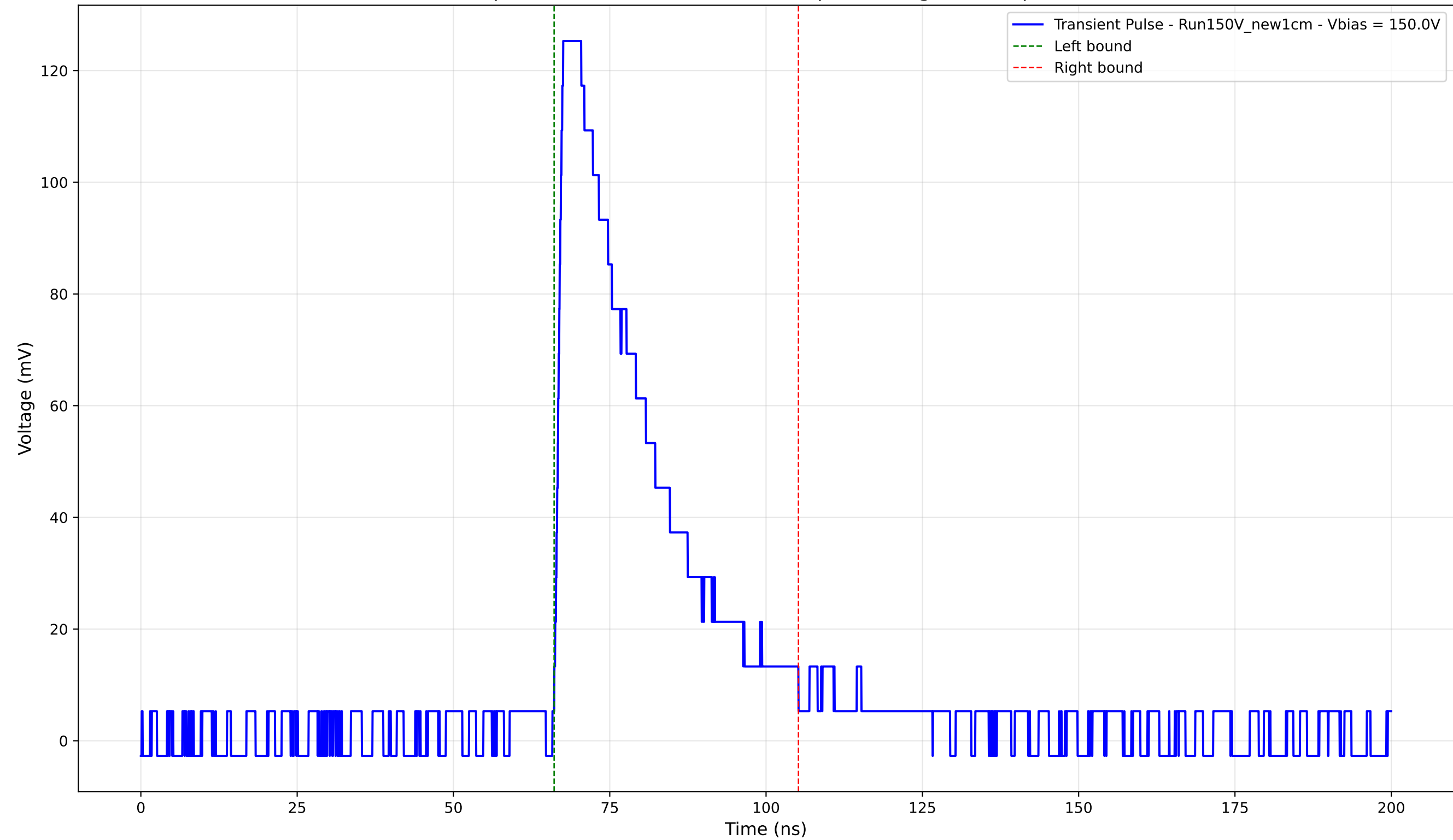
Transient Pulse - Sample: New1cm - Position: 3665.0 \mu\text{m} - Charge: 39.24 pC - Rise Time: 1.28 ns
