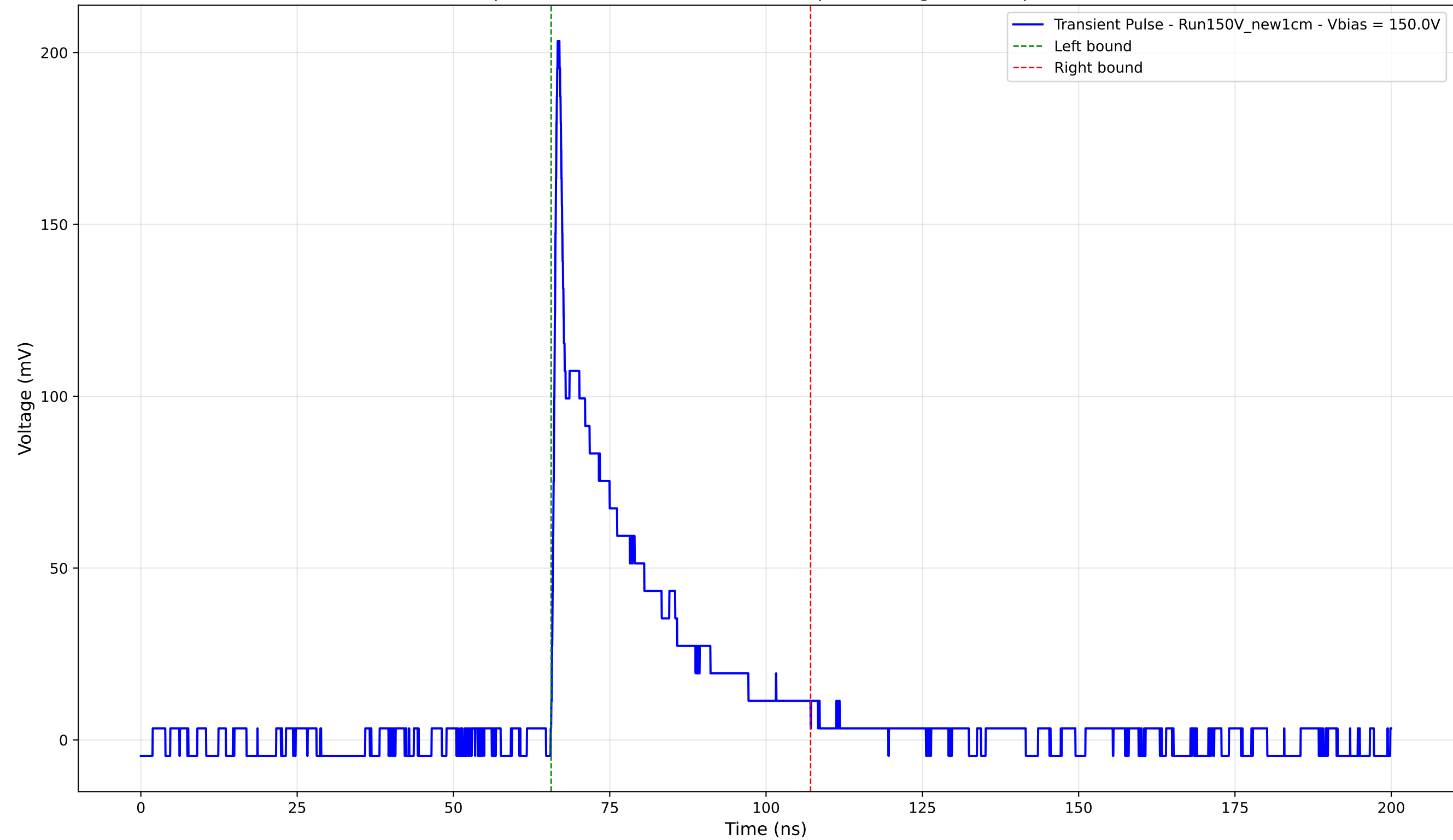
Transient Pulse - Sample: New1cm - Position: 2685.0 \mu\text{m} - Charge: 37.32 pC - Rise Time: 0.78 ns
