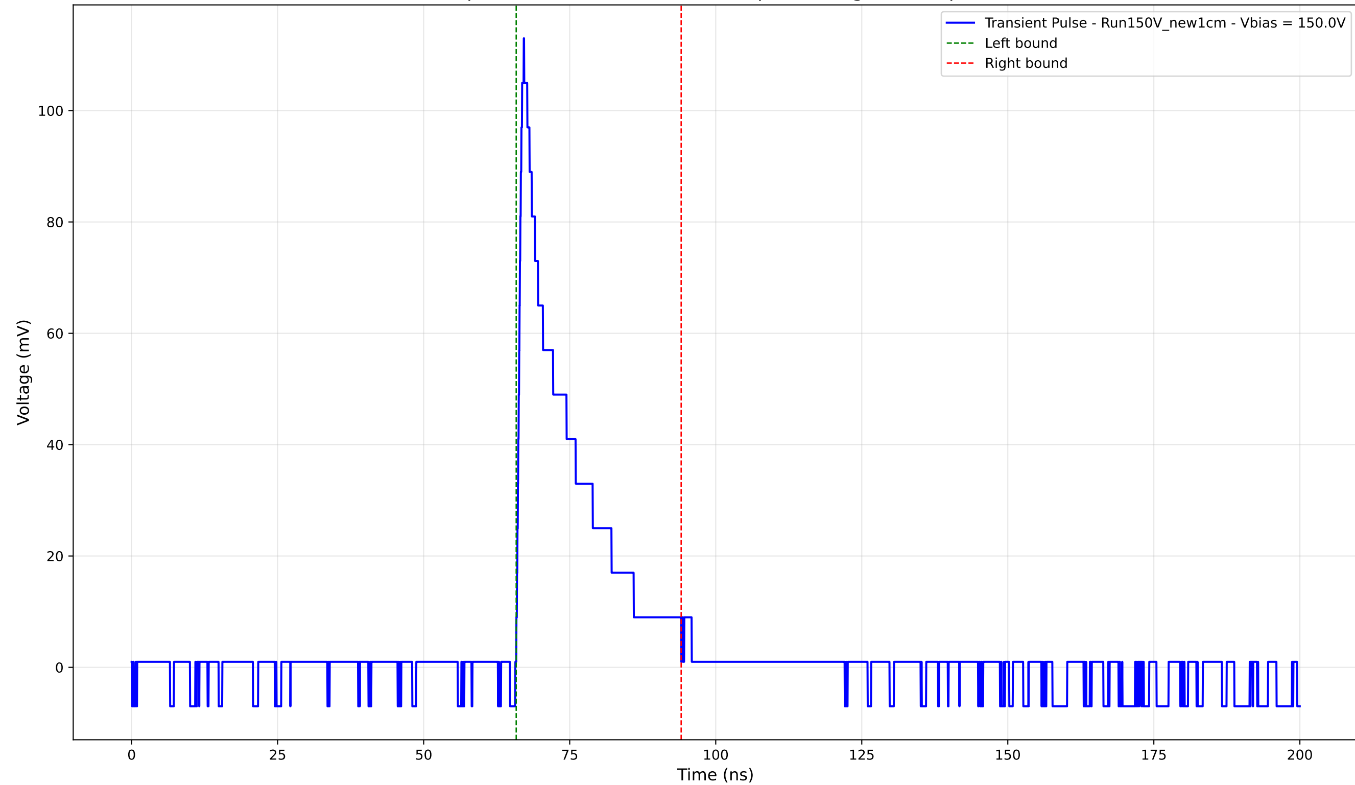
Transient Pulse - Sample: New1cm - Position: 125.0 \mu\text{m} - Charge: 18.95 pC - Rise Time: 0.89 ns
