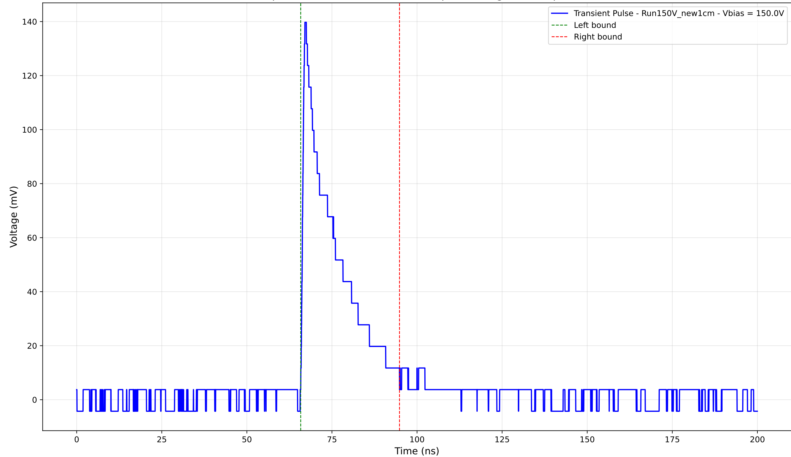
Transient Pulse - Sample: New1cm - Position: 235.0 \mu\text{m} - Charge: 28.21 pC - Rise Time: 0.95 ns
