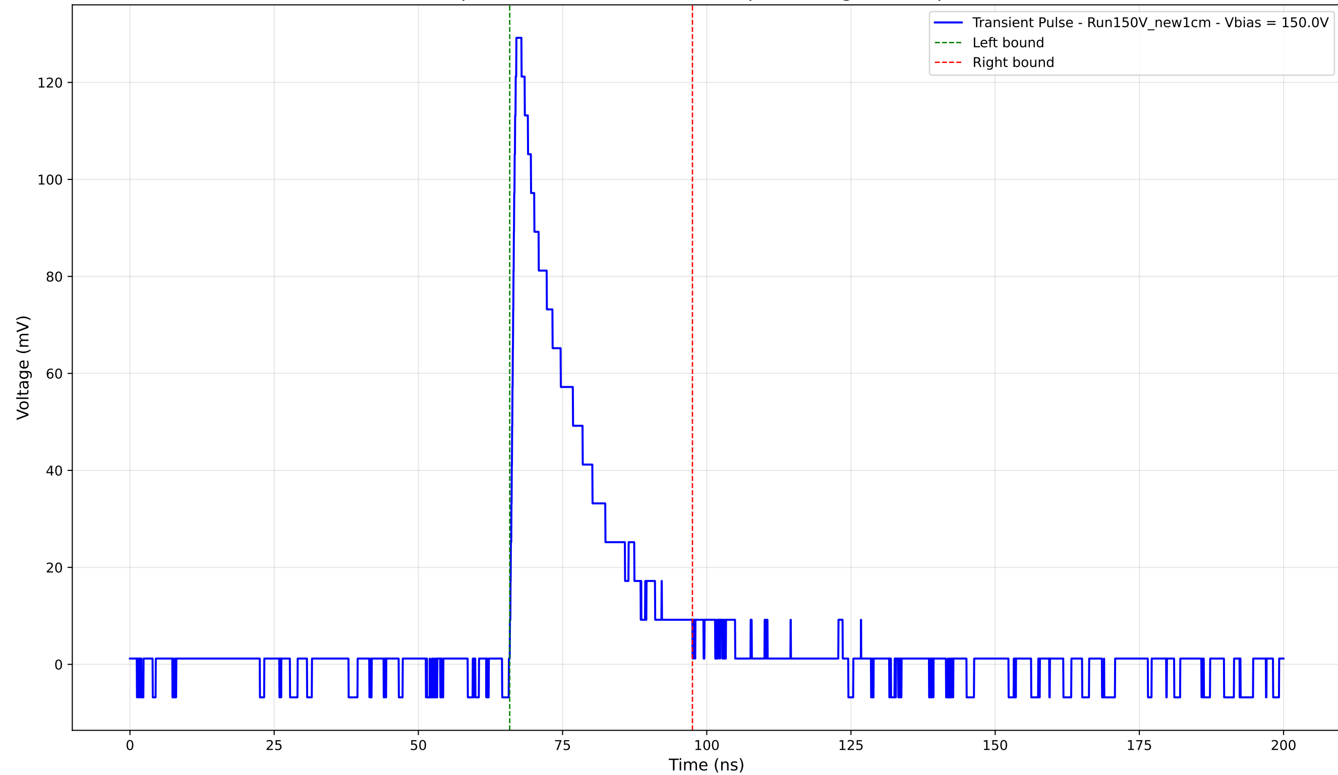
Transient Pulse - Sample: New1cm - Position: 260.0 \mu\text{m} - Charge: 27.33 pC - Rise Time: 0.91 ns
