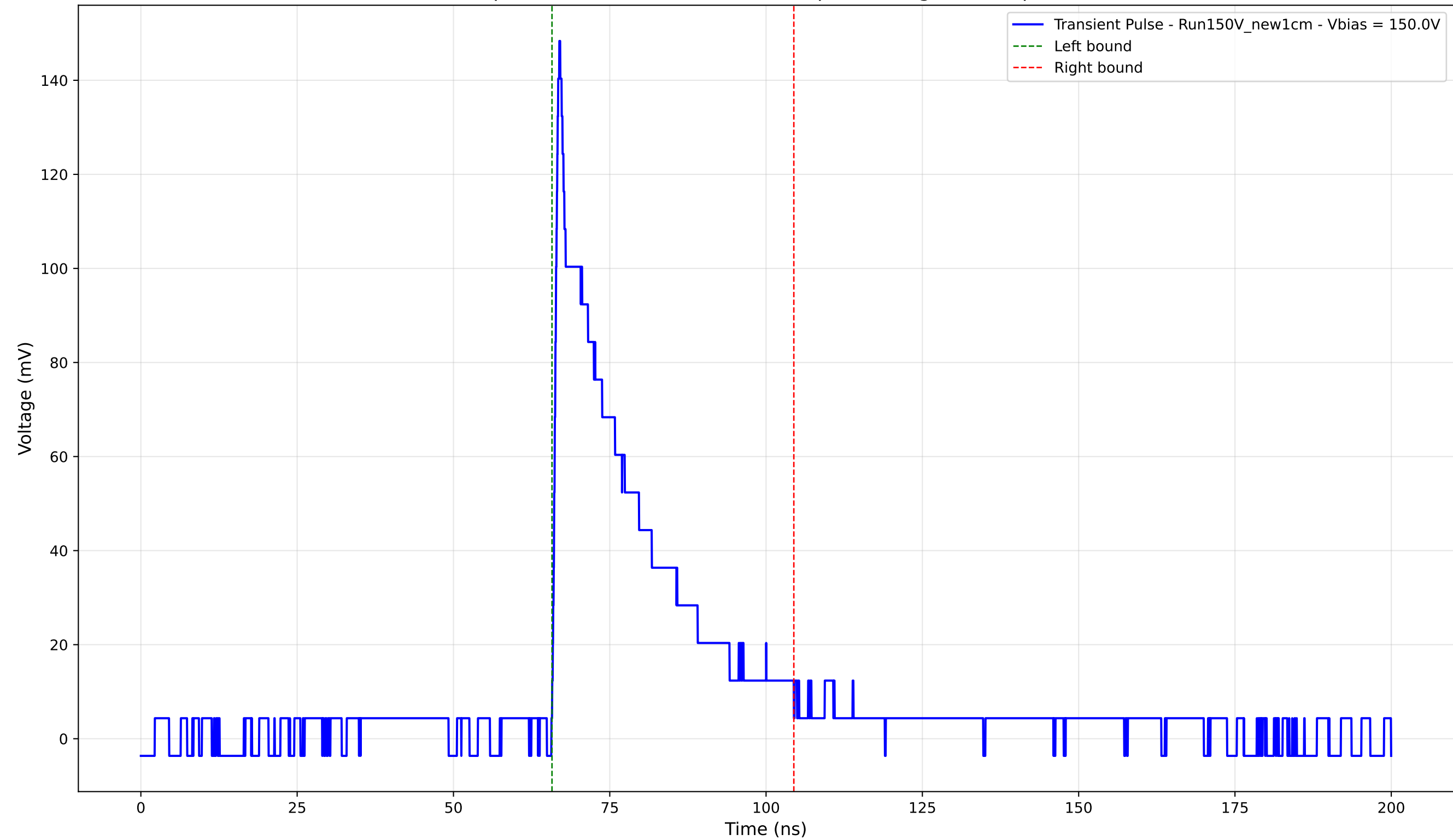
Transient Pulse - Sample: New1cm - Position: 2205.0 \mu\text{m} - Charge: 33.53 pC - Rise Time: 0.87 ns
