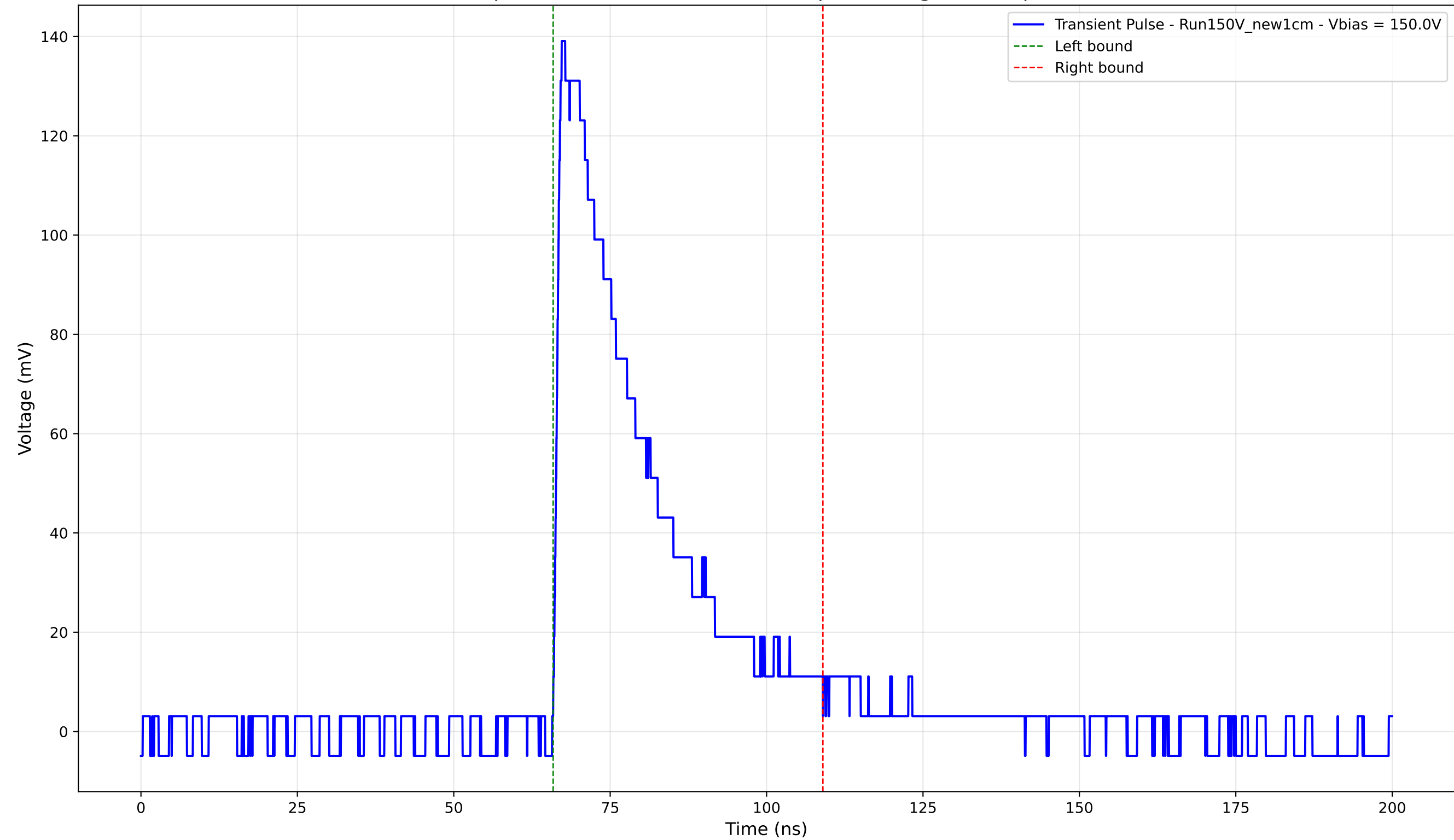
Transient Pulse - Sample: New1cm - Position: 3255.0 \mu\text{m} - Charge: 41.26 pC - Rise Time: 1.05 ns
