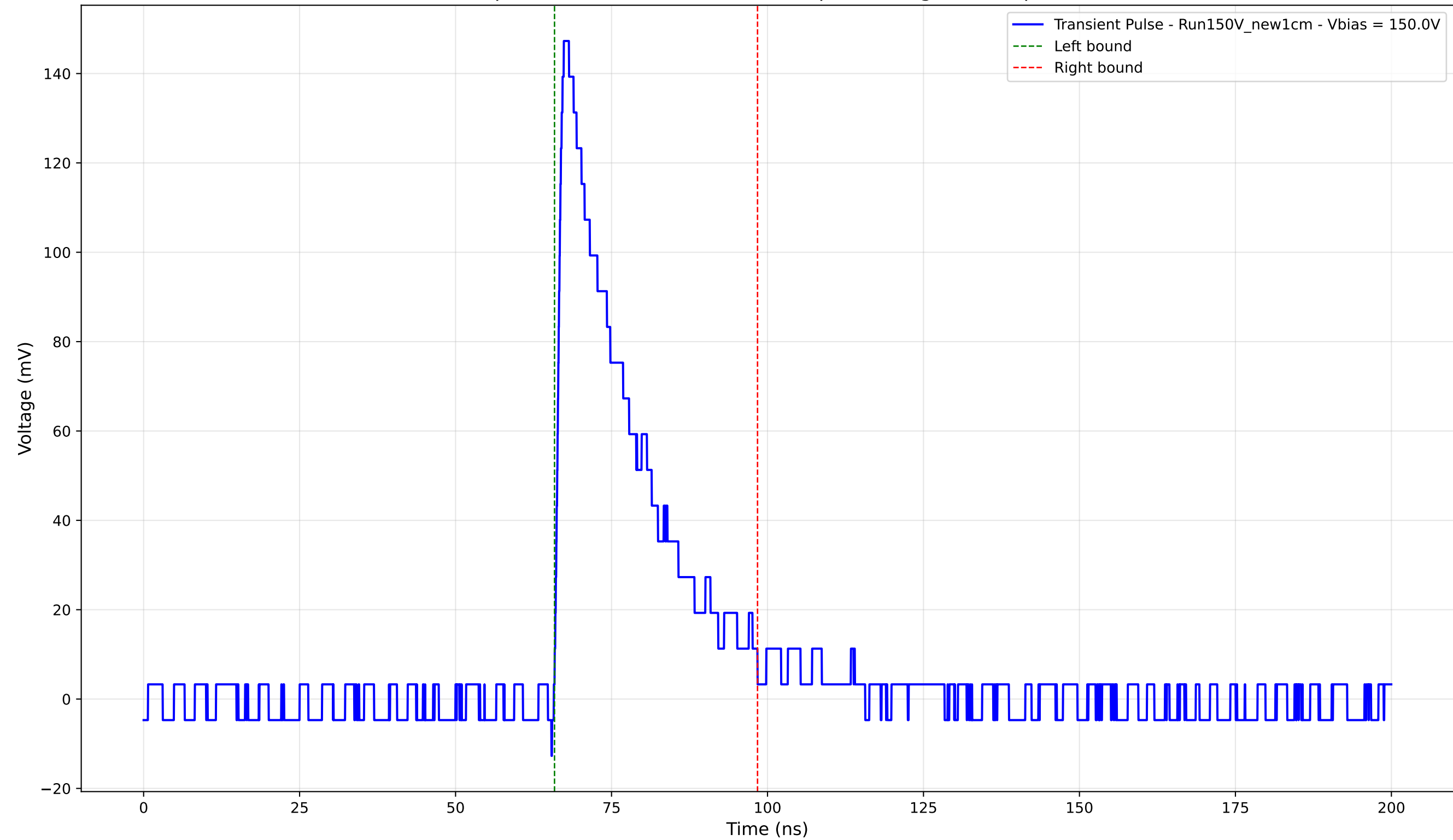
Transient Pulse - Sample: New1cm - Position: 4465.0 \mu\text{m} - Charge: 35.78 pC - Rise Time: 1.17 ns
