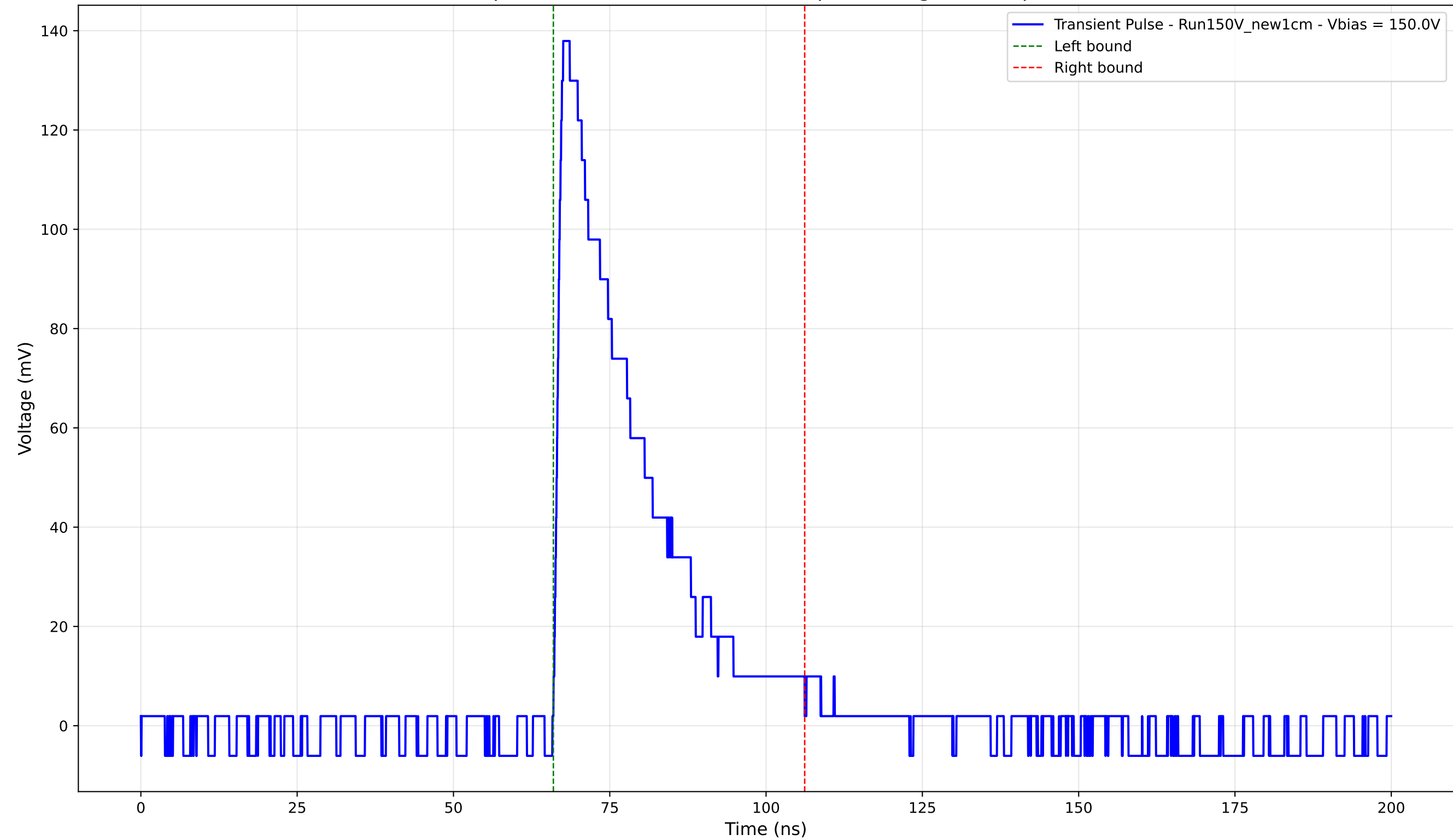
Transient Pulse - Sample: New1cm - Position: 4215.0 \mu\text{m} - Charge: 37.20 pC - Rise Time: 1.21 ns
