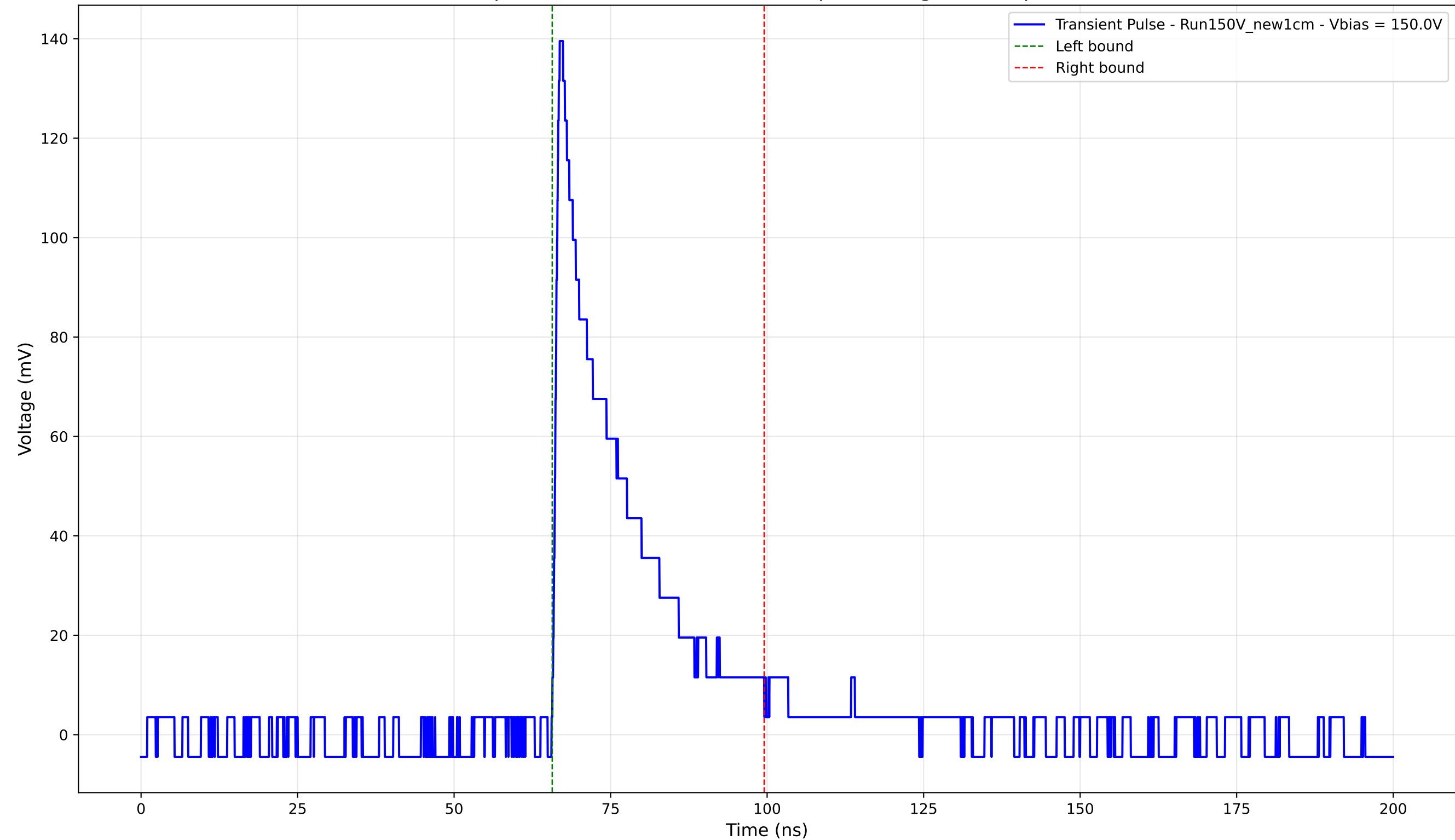
Transient Pulse - Sample: New1cm - Position: 4805.0 \mu\text{m} - Charge: 28.51 pC - Rise Time: 0.91 ns
