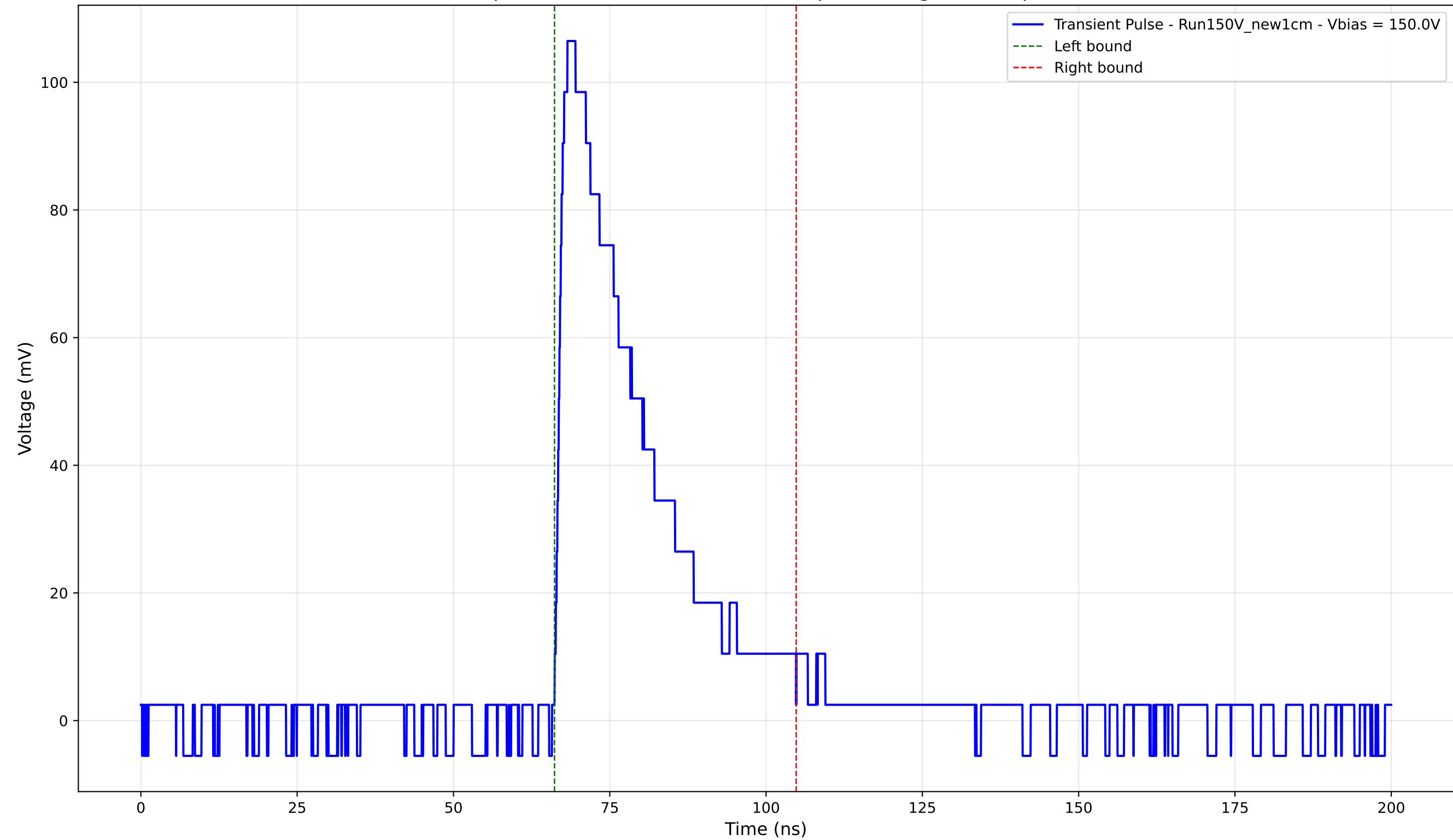
Transient Pulse - Sample: New1cm - Position: 1400.0 \mu\text{m} - Charge: 30.81 pC - Rise Time: 1.36 ns
