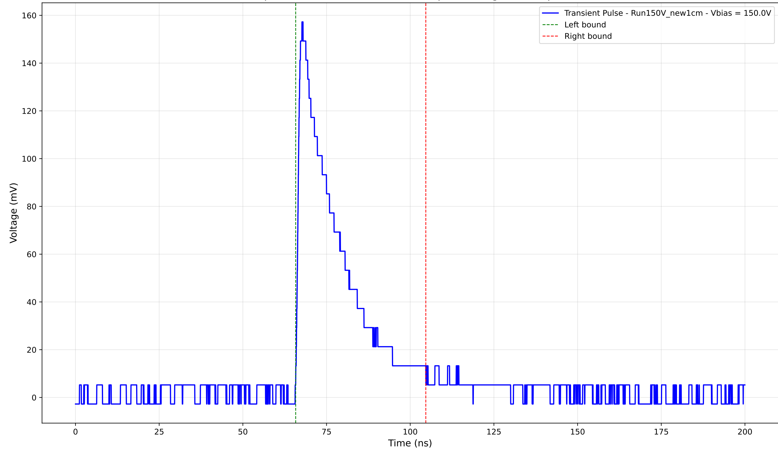
Transient Pulse - Sample: New1cm - Position: 4455.0 \mu\text{m} - Charge: 40.57 pC - Rise Time: 1.27 ns
