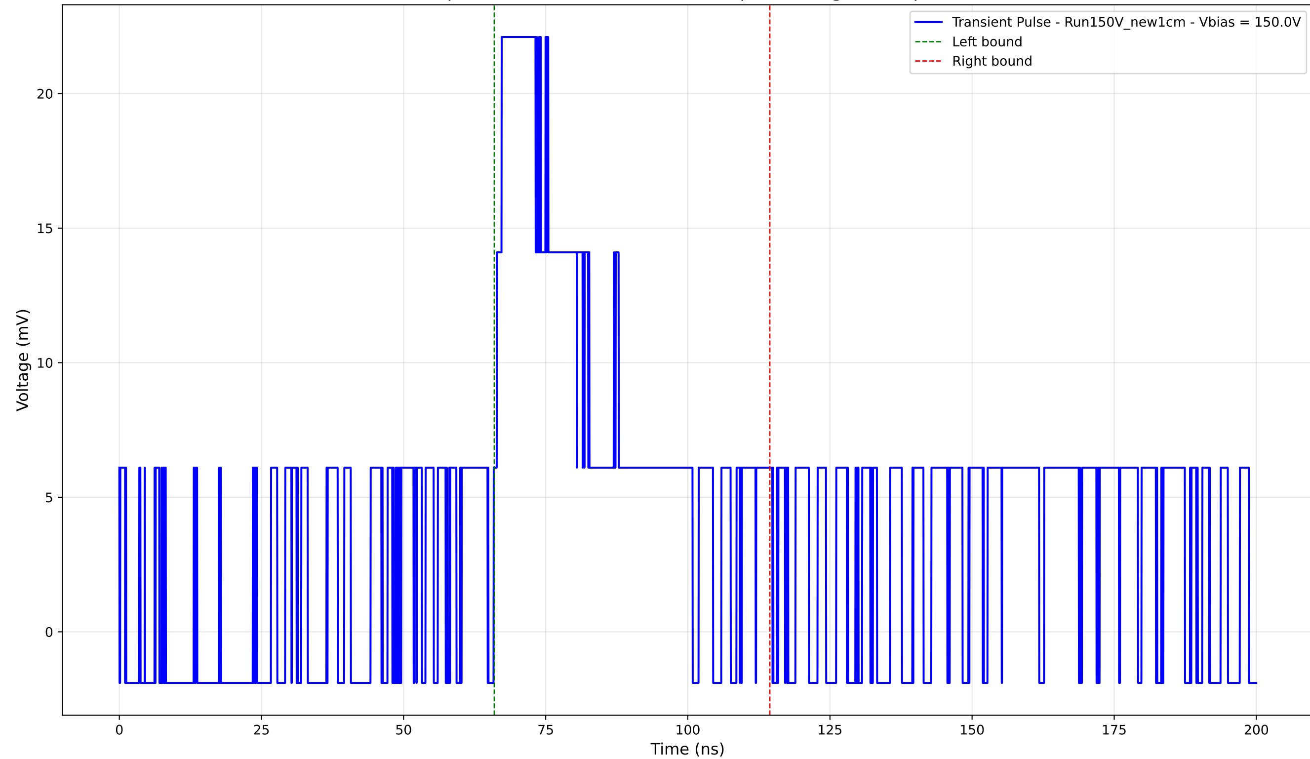
Transient Pulse - Sample: New1cm - Position: 3565.0 \mu\text{m} - Charge: 9.09 pC - Rise Time: 1.42 ns
