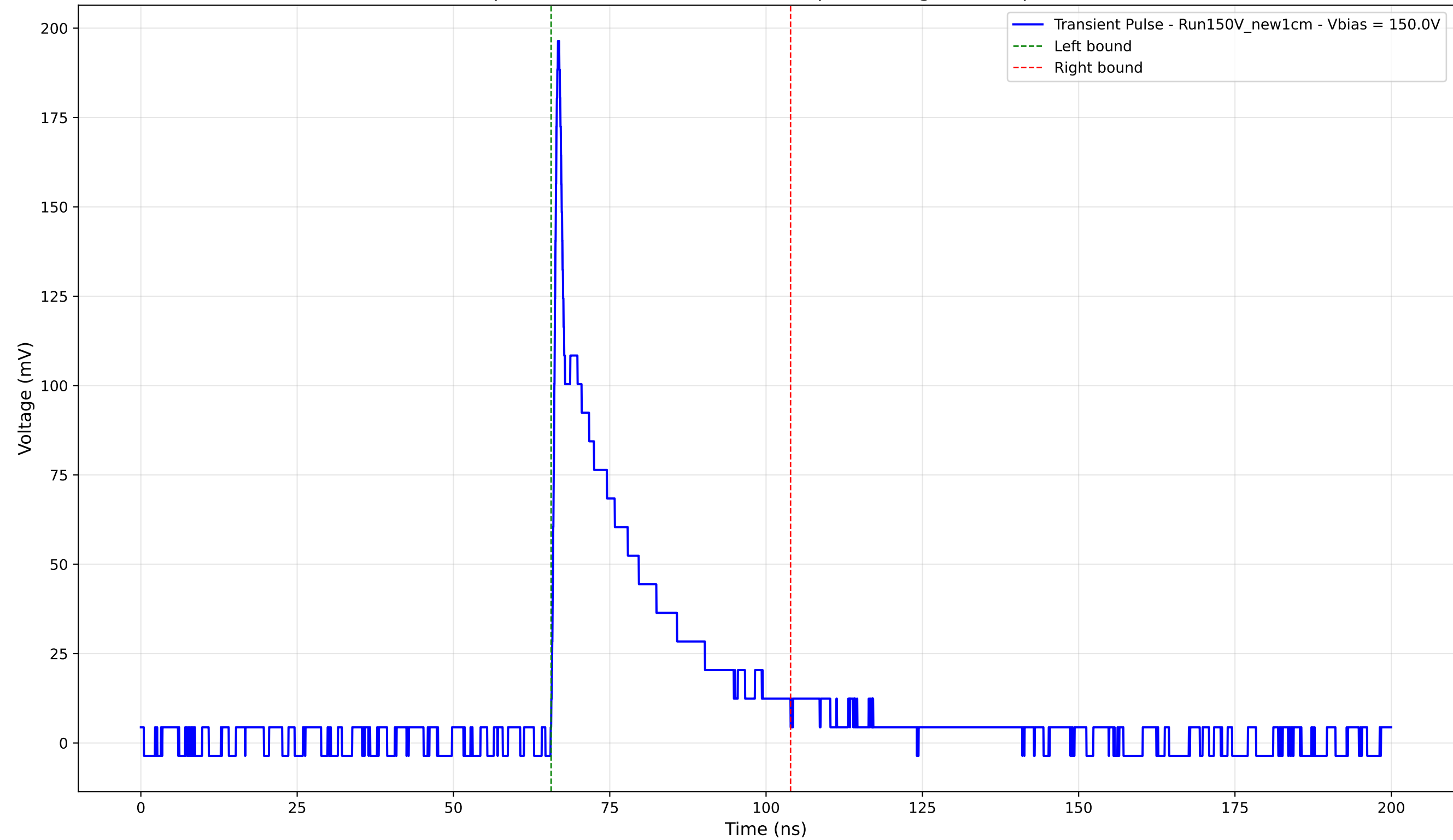
Transient Pulse - Sample: New1cm - Position: 2400.0 \mu\text{m} - Charge: 35.96 pC - Rise Time: 0.80 ns
