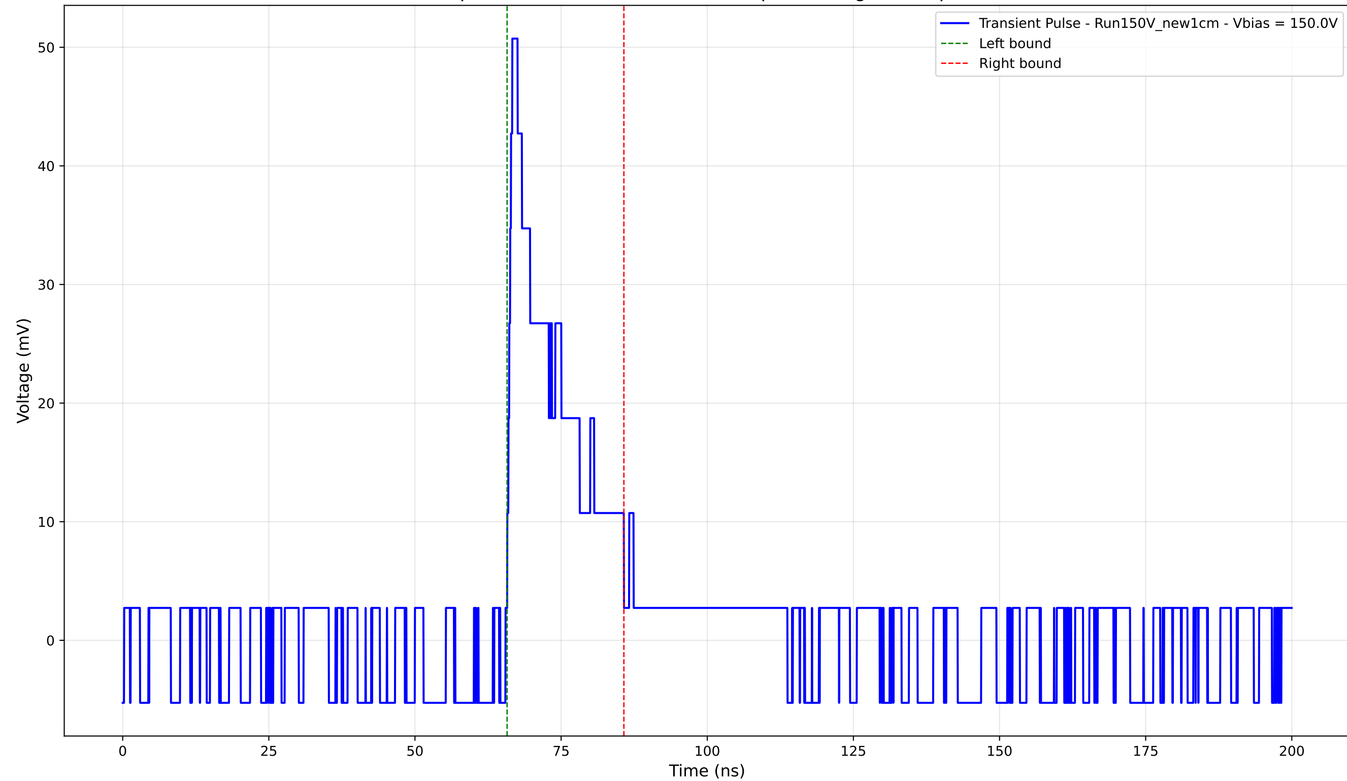
Transient Pulse - Sample: New1cm - Position: 4865.0 \mu\text{m} - Charge: 8.64 pC - Rise Time: 0.87 ns
