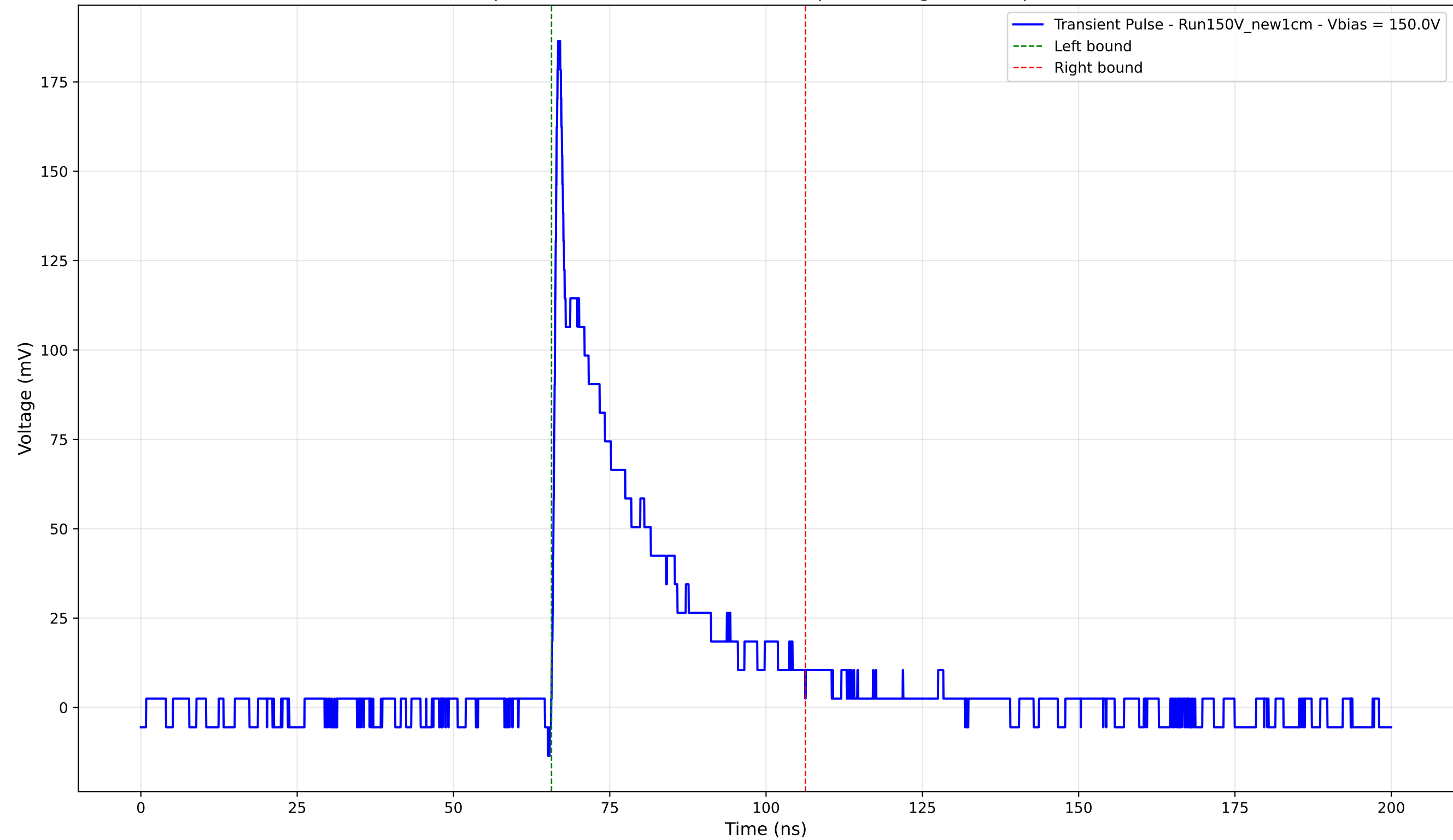
Transient Pulse - Sample: New1cm - Position: 2795.0 \mu\text{m} - Charge: 38.20 pC - Rise Time: 0.76 ns
