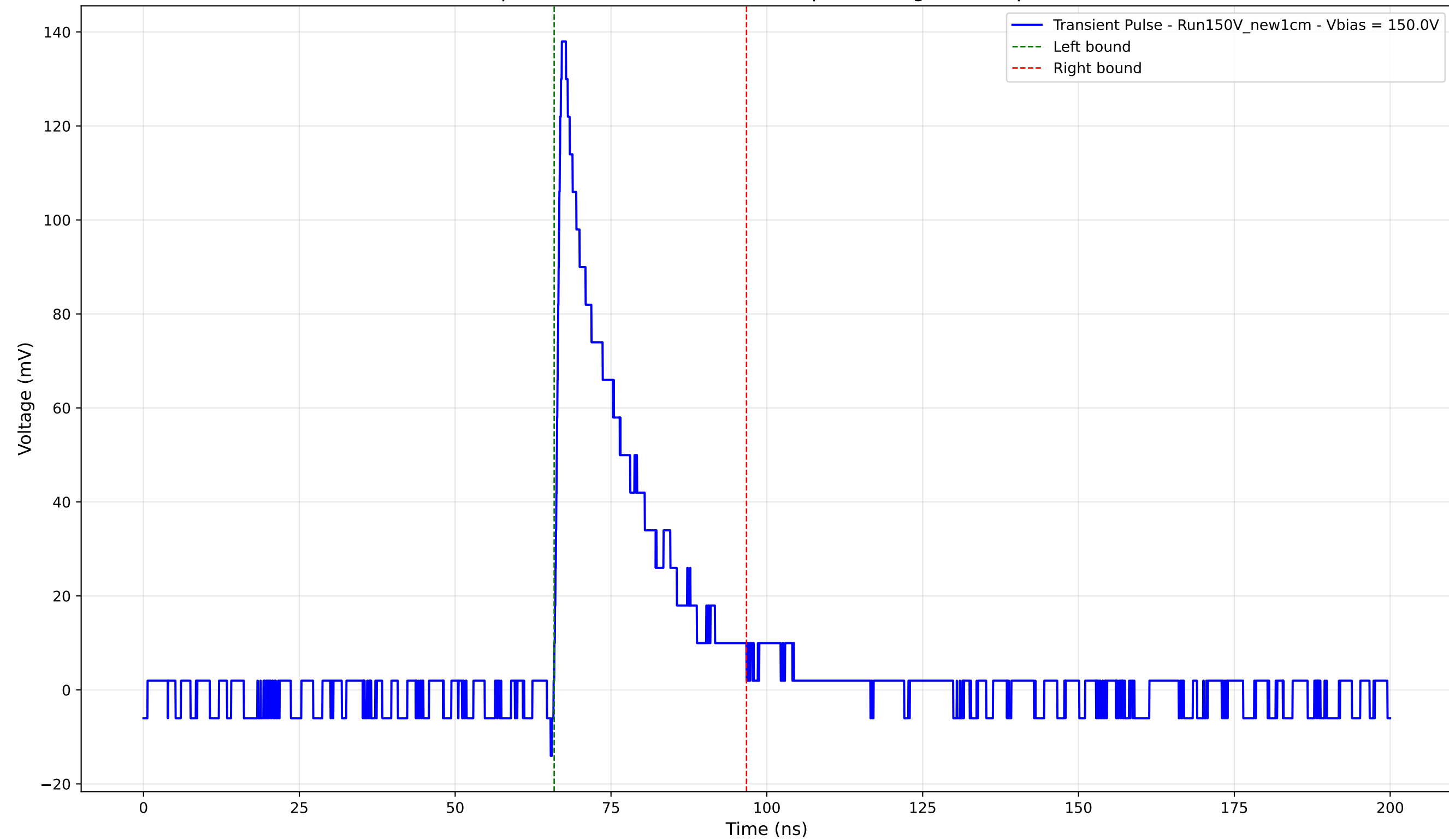
Transient Pulse - Sample: New1cm - Position: 290.0 \mu\text{m} - Charge: 27.67 pC - Rise Time: 0.97 ns
