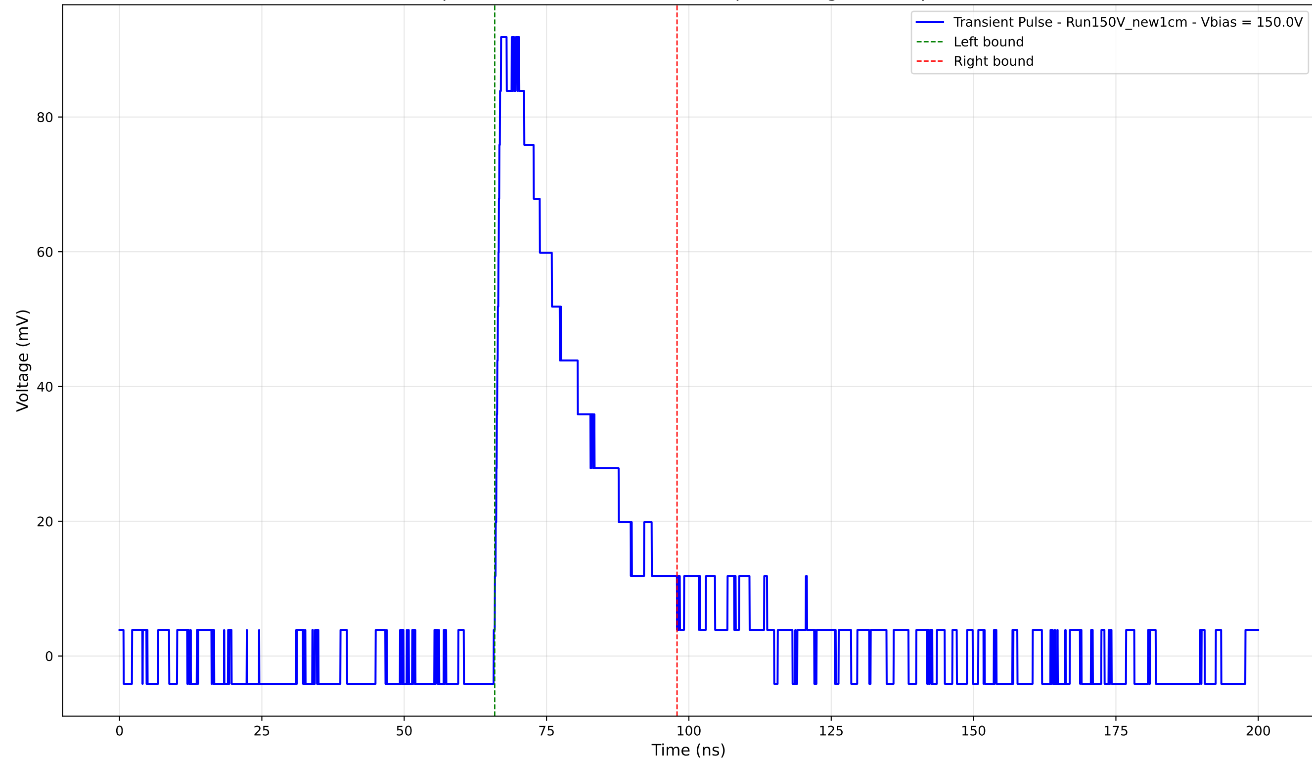
Transient Pulse - Sample: New1cm - Position: 1935.0 \mu\text{m} - Charge: 26.38 pC - Rise Time: 0.91 ns
