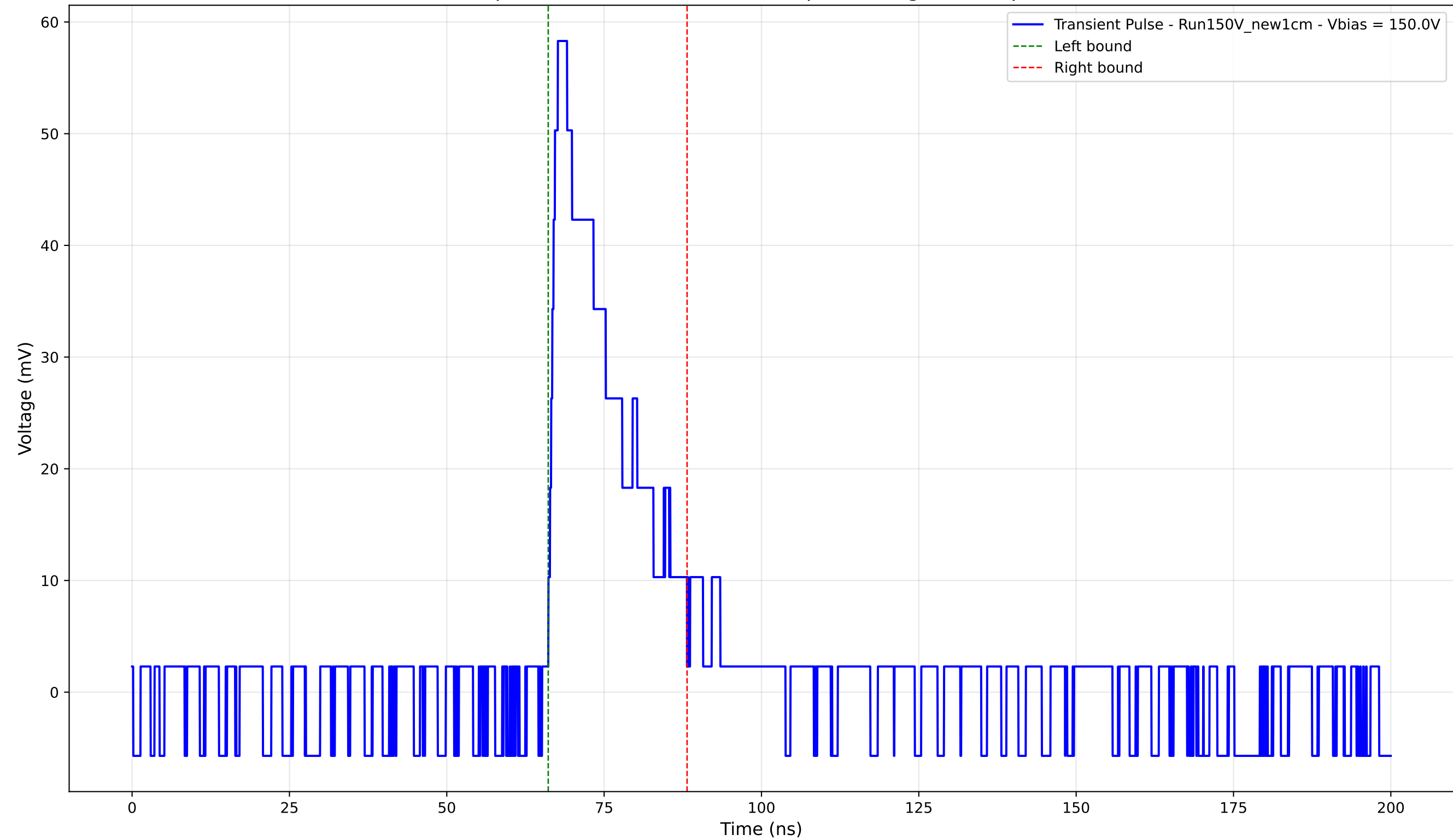
Transient Pulse - Sample: New1cm - Position: 580.0 \mu\text{m} - Charge: 12.28 pC - Rise Time: 1.51 ns
