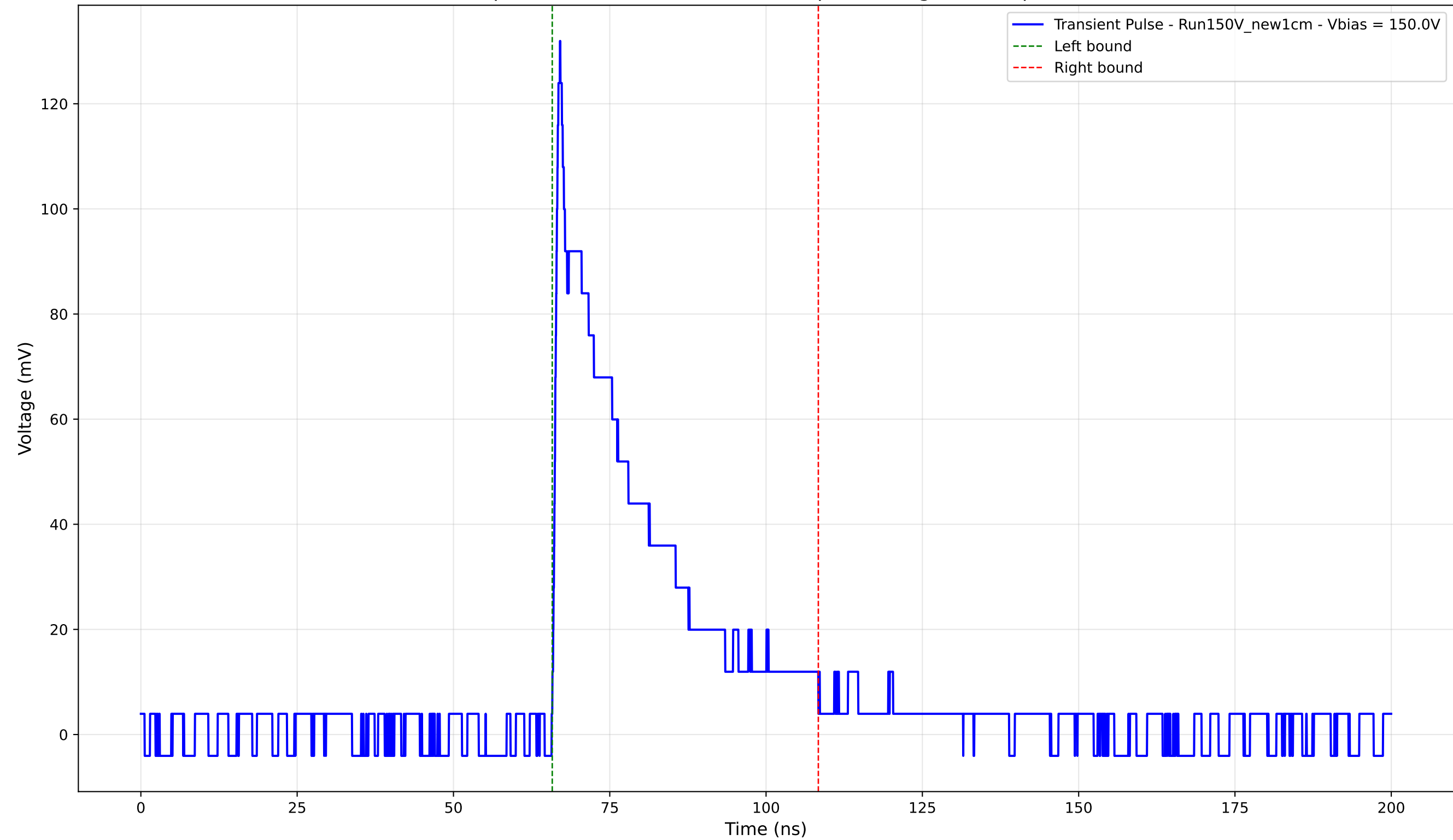
Transient Pulse - Sample: New1cm - Position: 2155.0 \mu\text{m} - Charge: 31.80 pC - Rise Time: 0.86 ns
