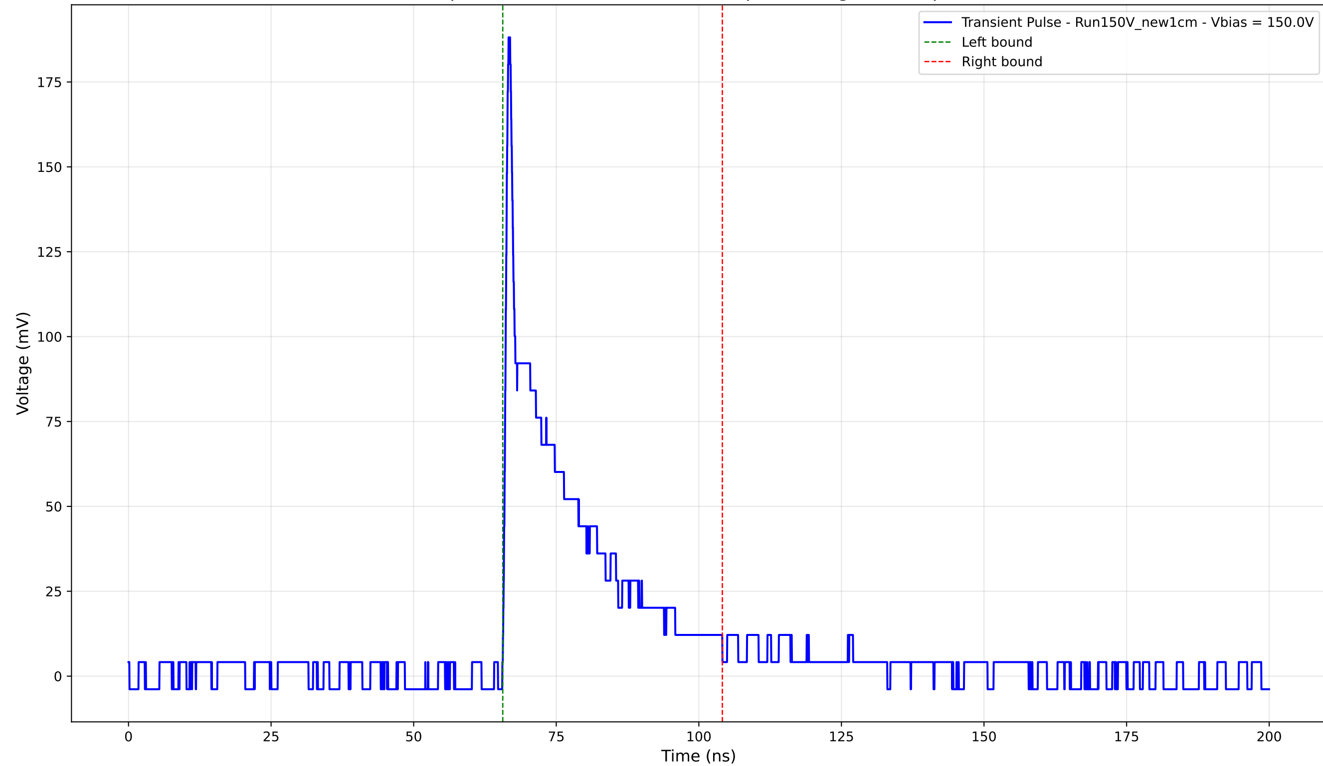
Transient Pulse - Sample: New1cm - Position: 2650.0 \mu\text{m} - Charge: 32.95 pC - Rise Time: 0.78 ns
