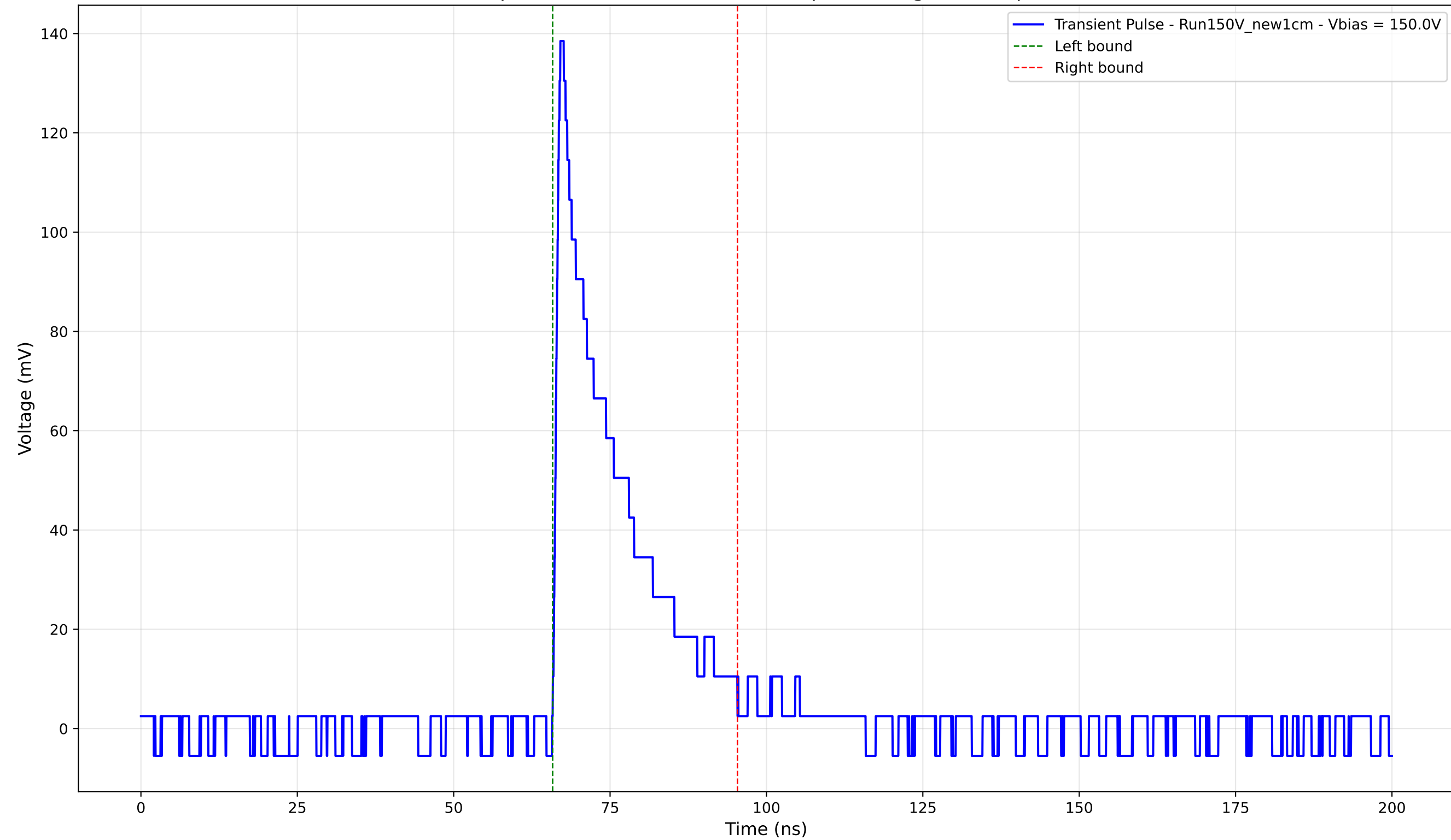
Transient Pulse - Sample: New1cm - Position: 225.0 \mu\text{m} - Charge: 26.37 pC - Rise Time: 0.97 ns
