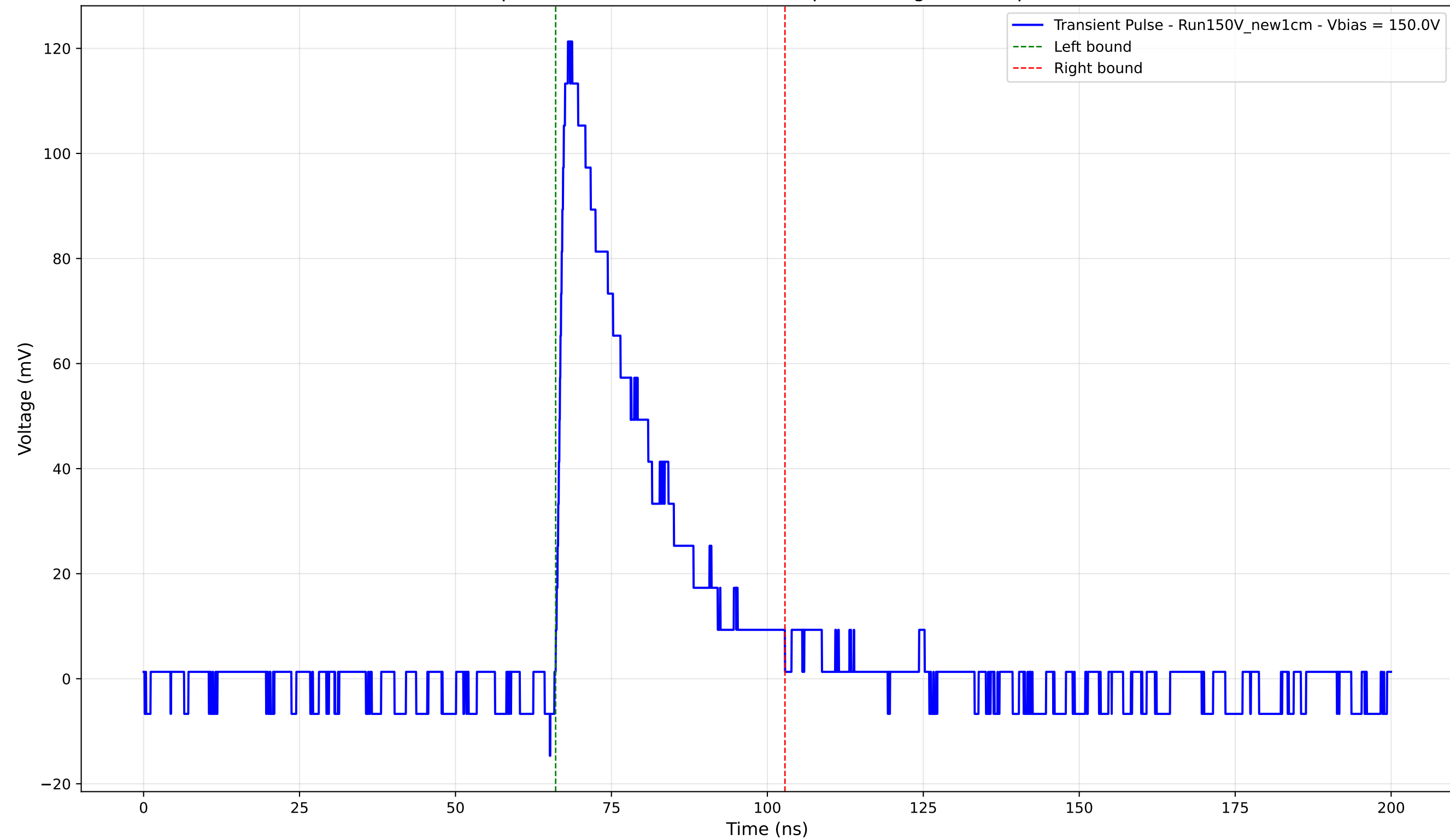
Transient Pulse - Sample: New1cm - Position: 800.0 \mu\text{m} - Charge: 30.91 pC - Rise Time: 1.35 ns
