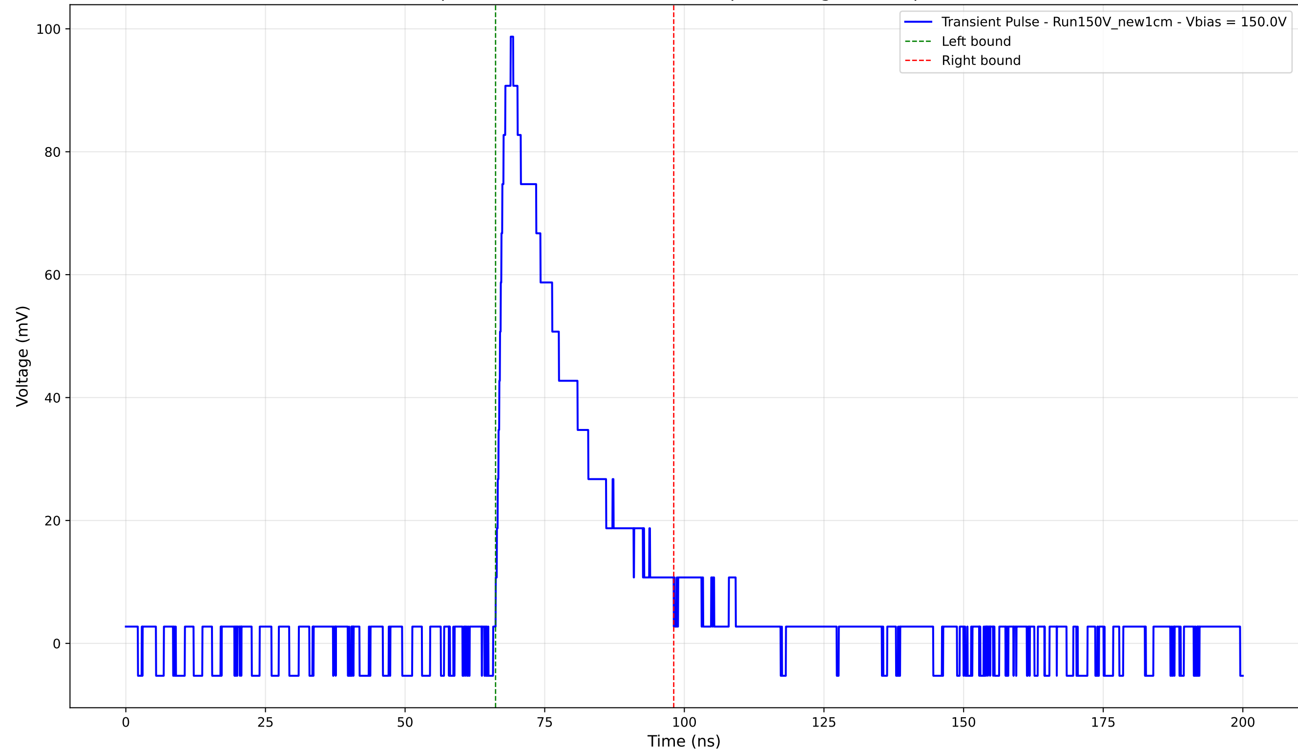
Transient Pulse - Sample: New1cm - Position: 1130.0 \mu\text{m} - Charge: 25.19 pC - Rise Time: 1.72 ns
