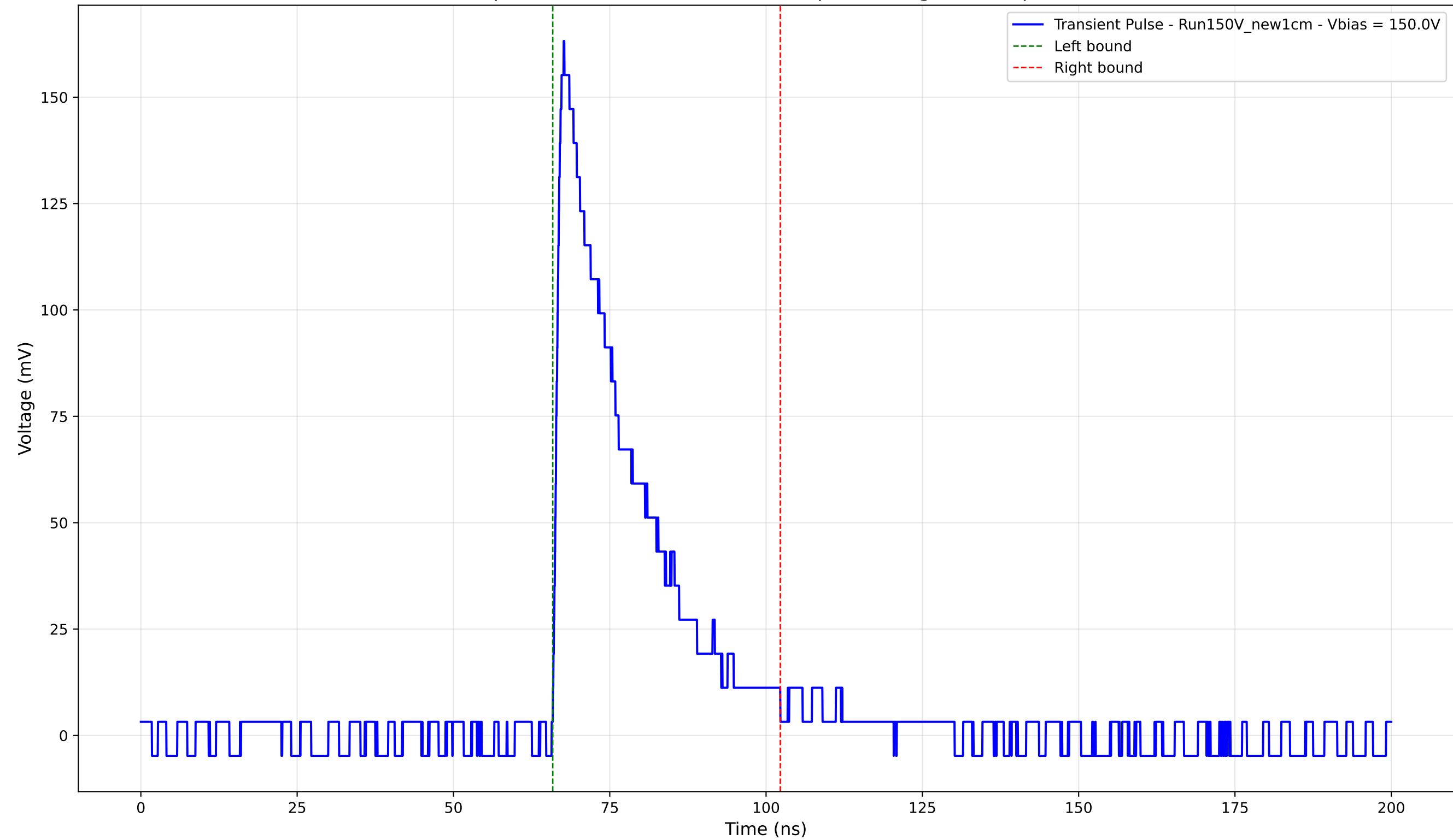
Transient Pulse - Sample: New1cm - Position: 4430.0 \mu\text{m} - Charge: 39.10 pC - Rise Time: 1.15 ns
