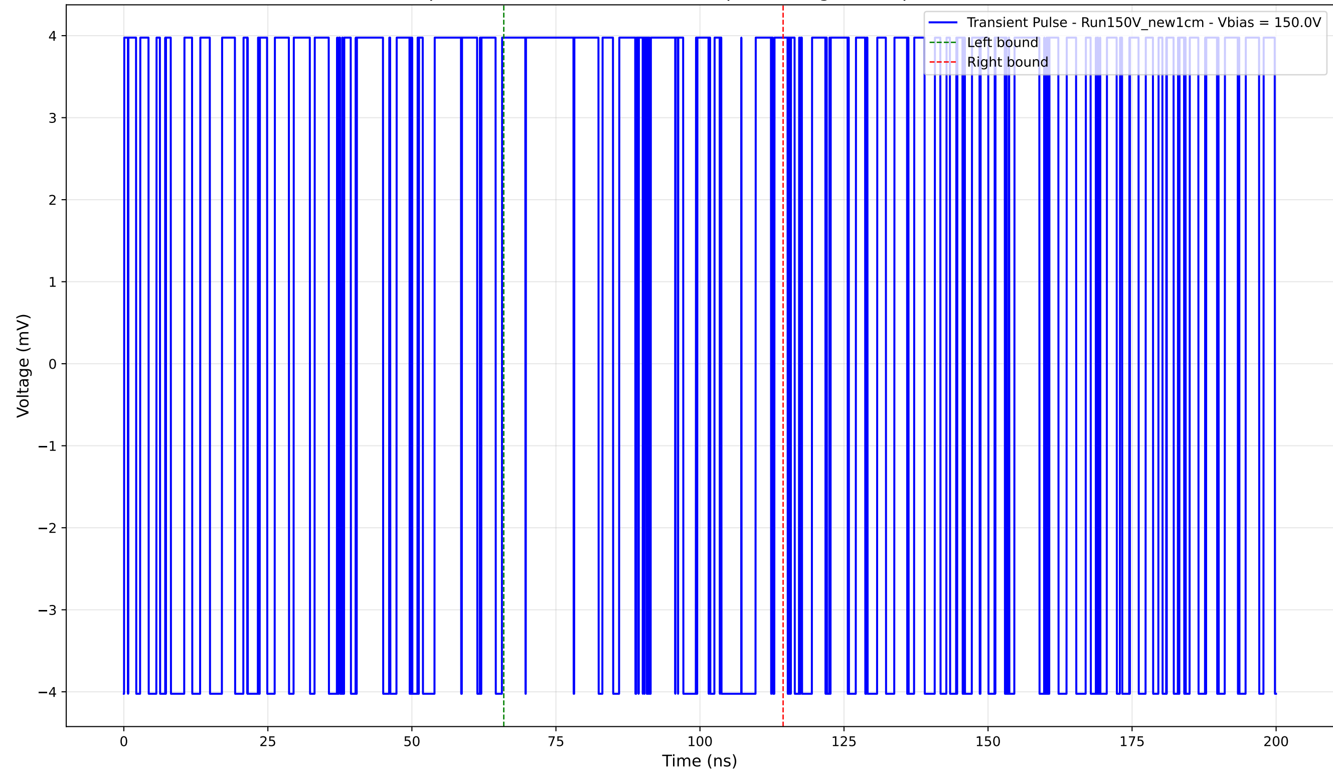
Transient Pulse - Sample: New1cm - Position: 4925.0 \mu\text{m} - Charge: 1.90 pC - Rise Time: 0.00 ns (N/A)
