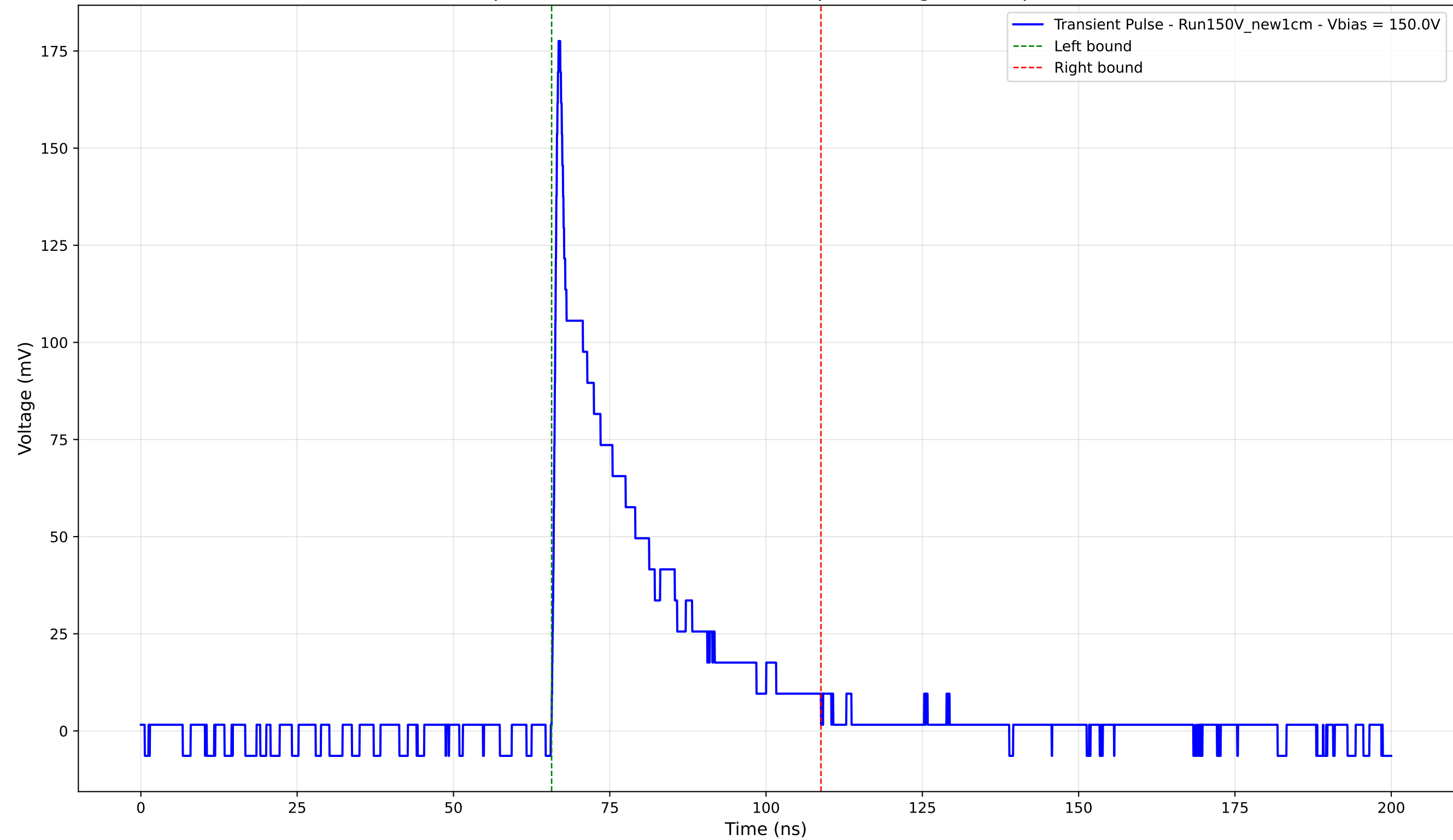
Transient Pulse - Sample: New1cm - Position: 2820.0 \mu\text{m} - Charge: 37.14 pC - Rise Time: 0.80 ns
