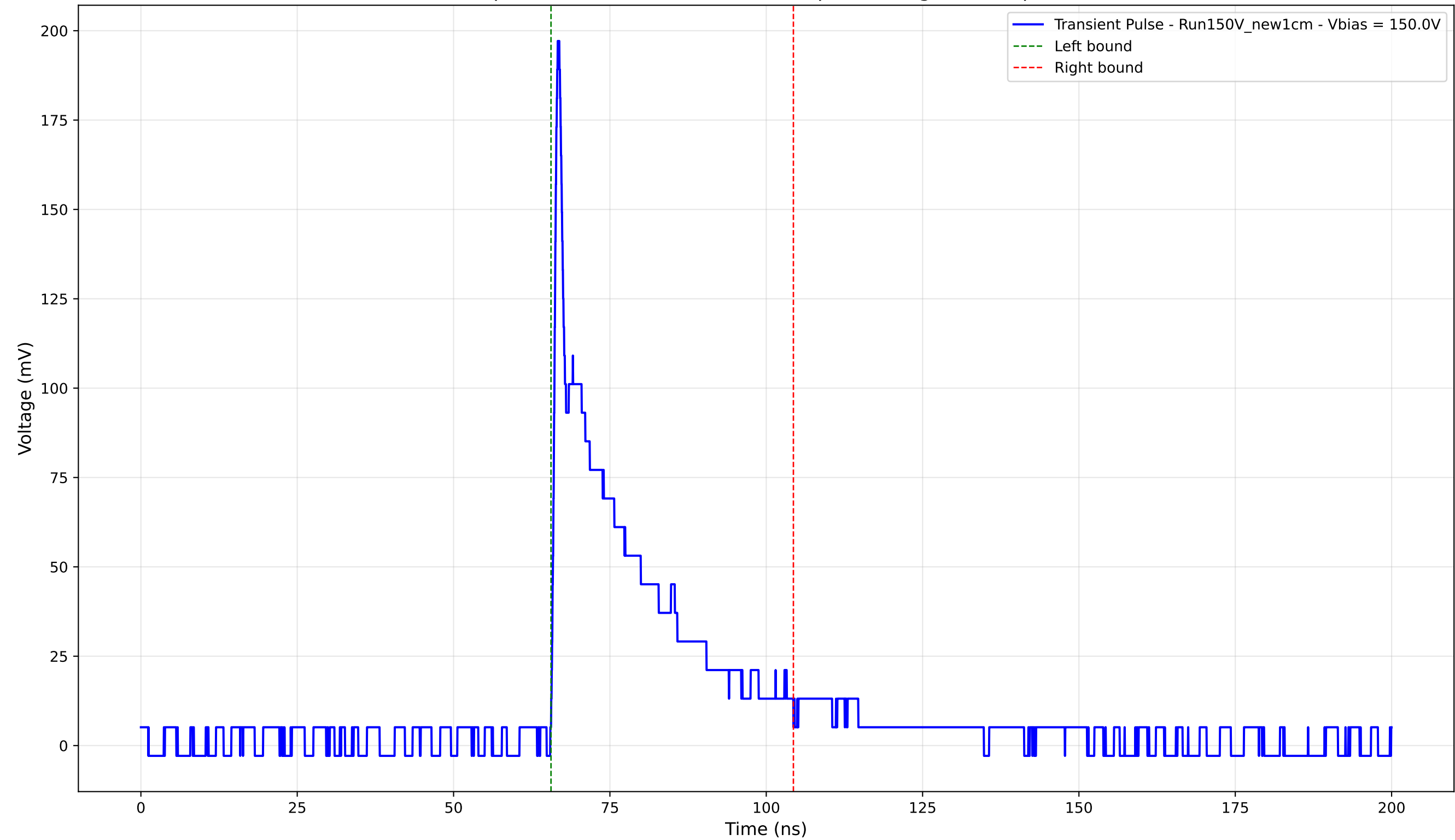
Transient Pulse - Sample: New1cm - Position: 2665.0 \mu\text{m} - Charge: 36.40 pC - Rise Time: 0.82 ns
