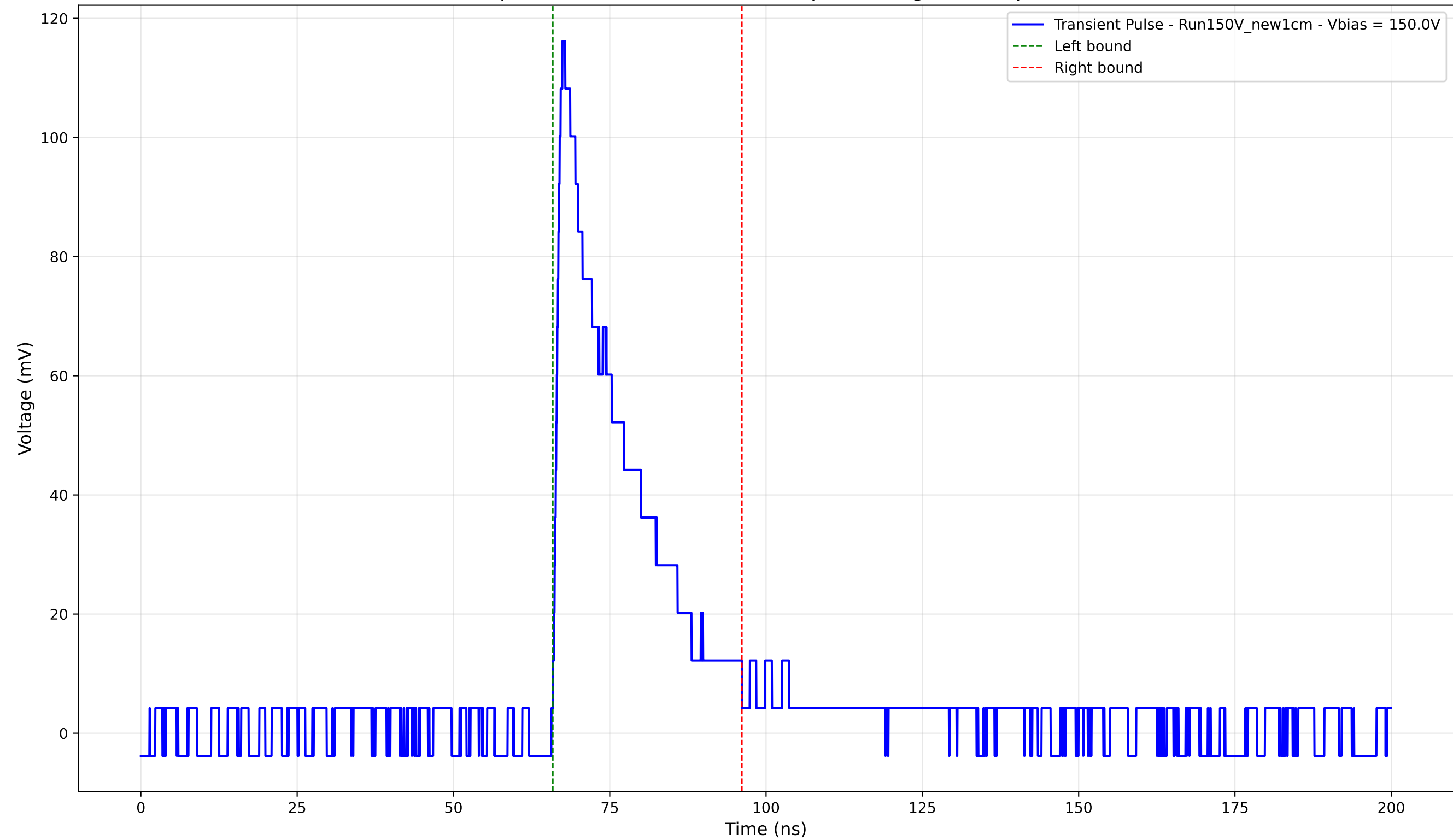
Transient Pulse - Sample: New1cm - Position: 430.0 \mu\text{m} - Charge: 25.83 pC - Rise Time: 1.22 ns
