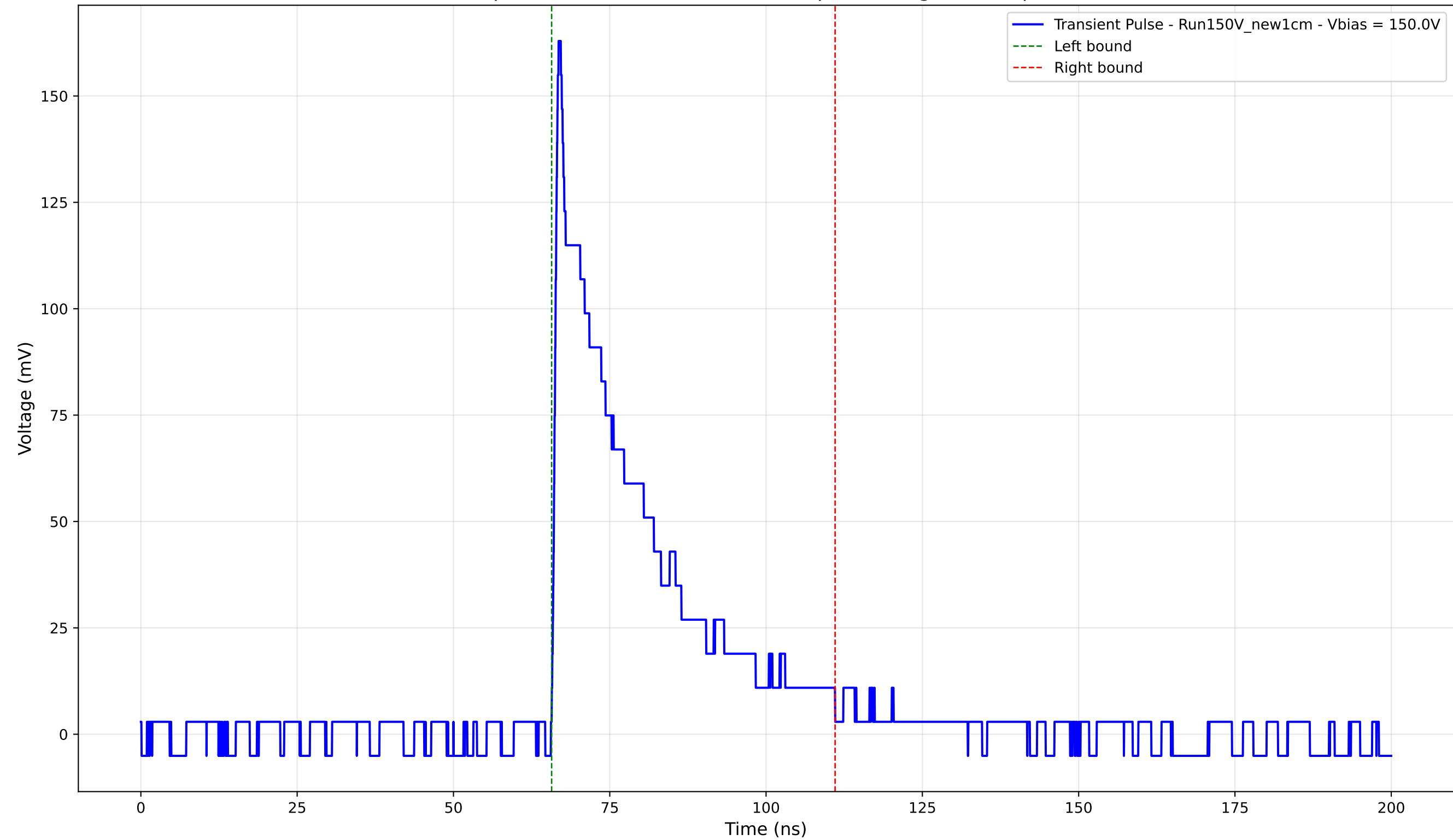
Transient Pulse - Sample: New1cm - Position: 2870.0 \mu\text{m} - Charge: 39.40 pC - Rise Time: 0.83 ns
