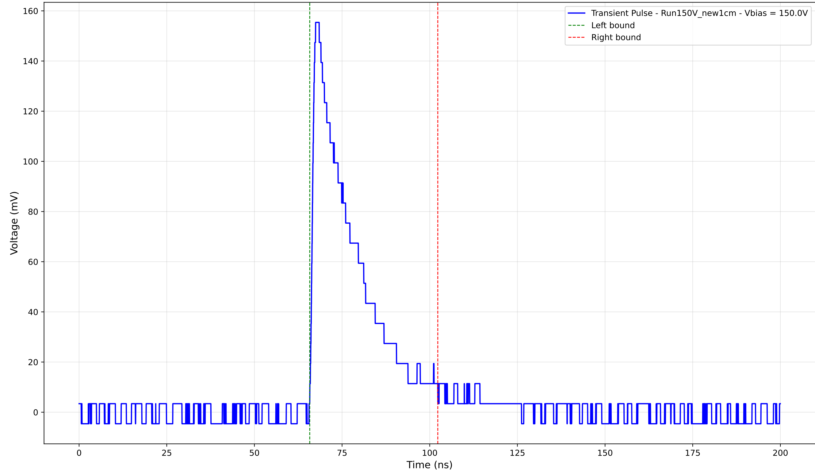
Transient Pulse - Sample: New1cm - Position: 4425.0 \mu\text{m} - Charge: 39.40 pC - Rise Time: 1.27 ns
