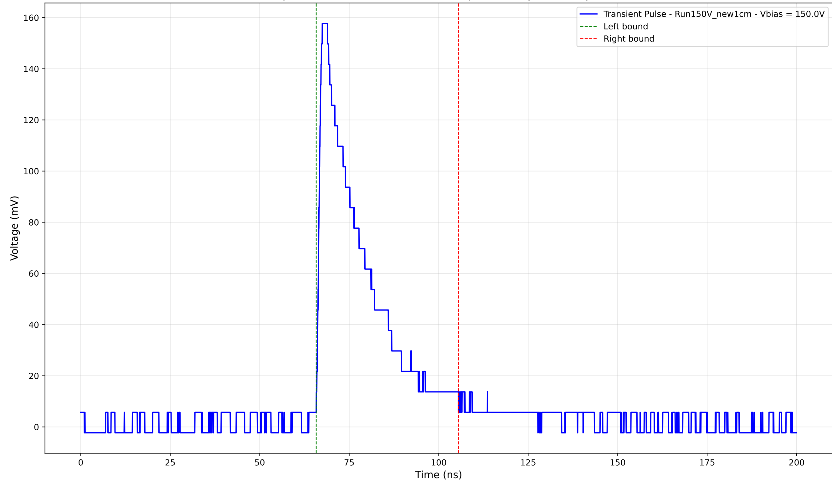
Transient Pulse - Sample: New1cm - Position: 4400.0 \mu\text{m} - Charge: 42.60 pC - Rise Time: 1.29 ns
