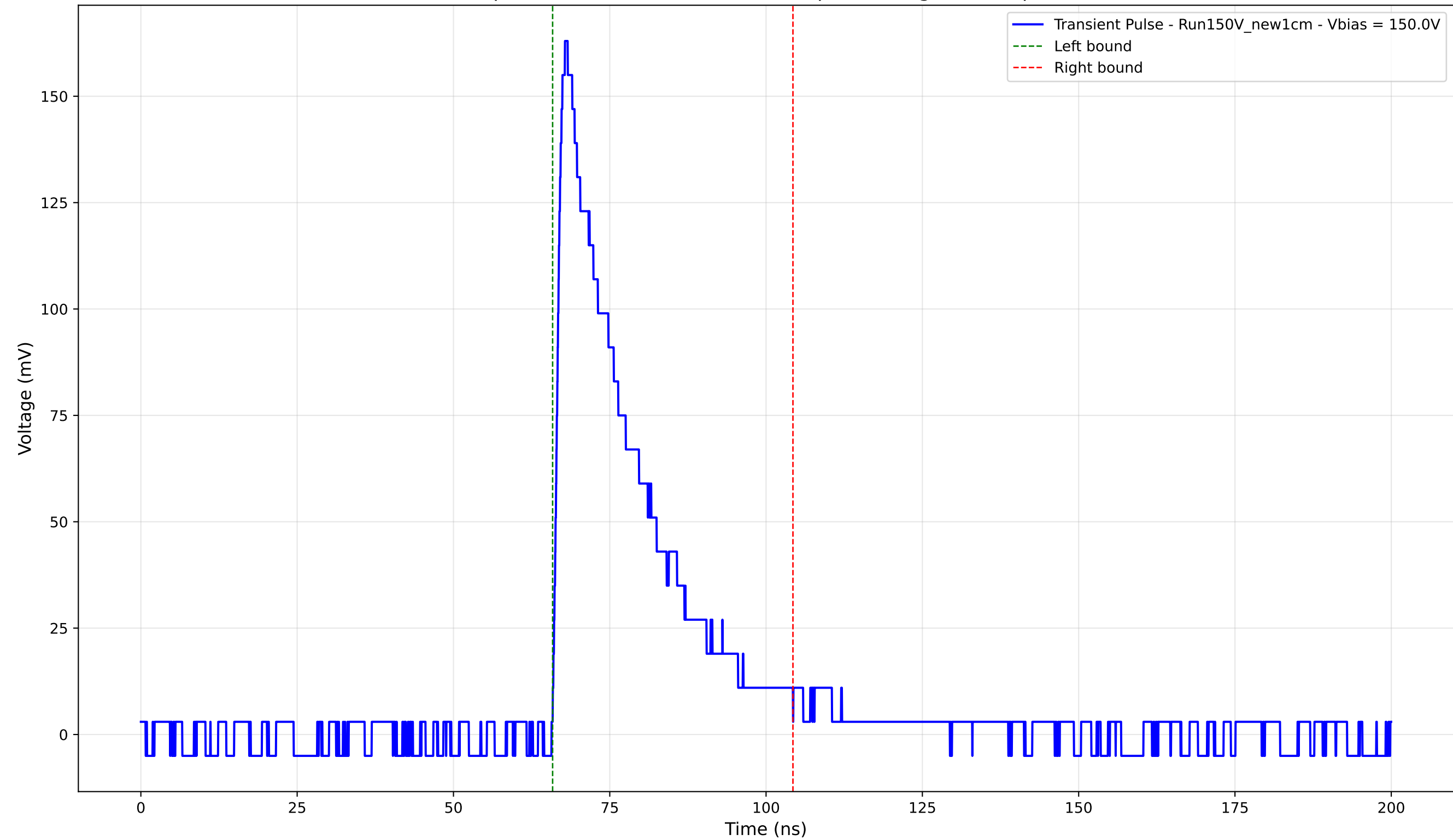
Transient Pulse - Sample: New1cm - Position: 4360.0 \mu\text{m} - Charge: 40.93 pC - Rise Time: 1.31 ns
