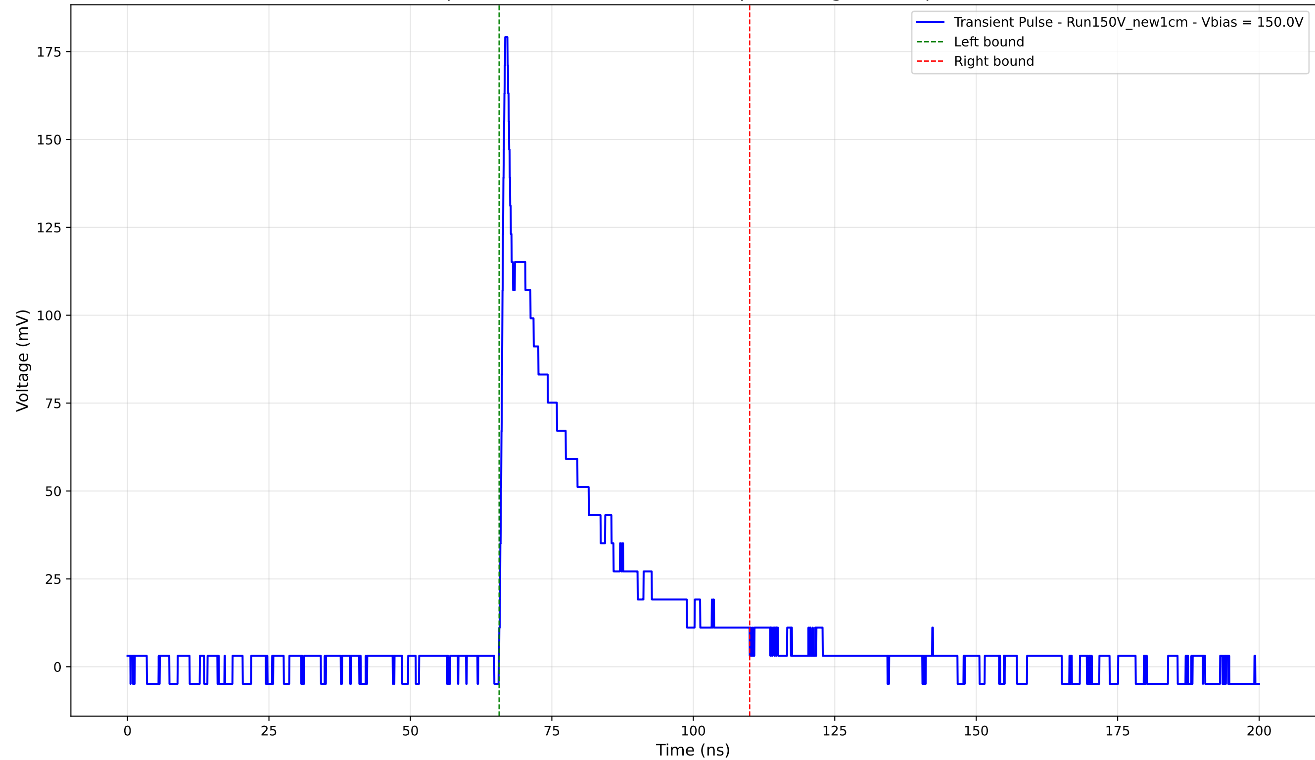
Transient Pulse - Sample: New1cm - Position: 2835.0 \mu\text{m} - Charge: 39.57 pC - Rise Time: 0.80 ns
