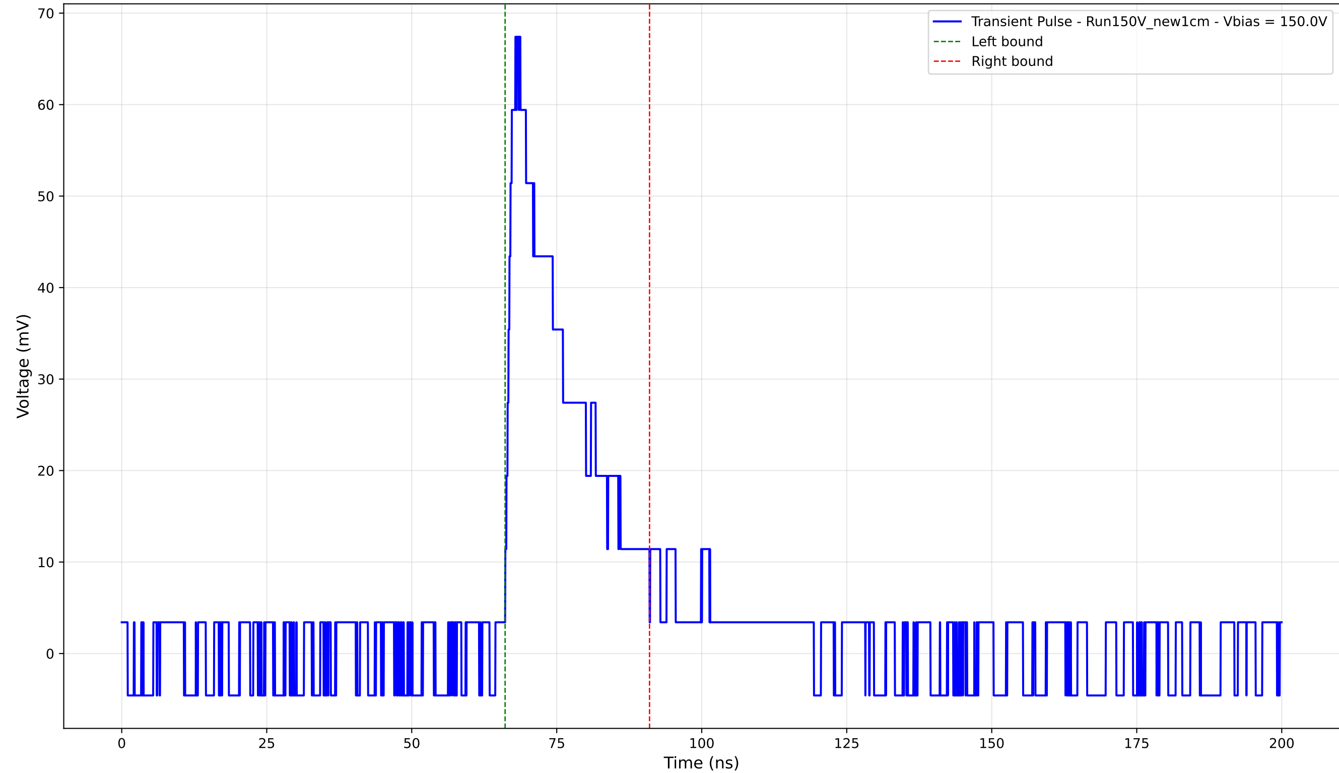
Transient Pulse - Sample: New1cm - Position: 585.0 \mu\text{m} - Charge: 14.92 pC - Rise Time: 1.75 ns
