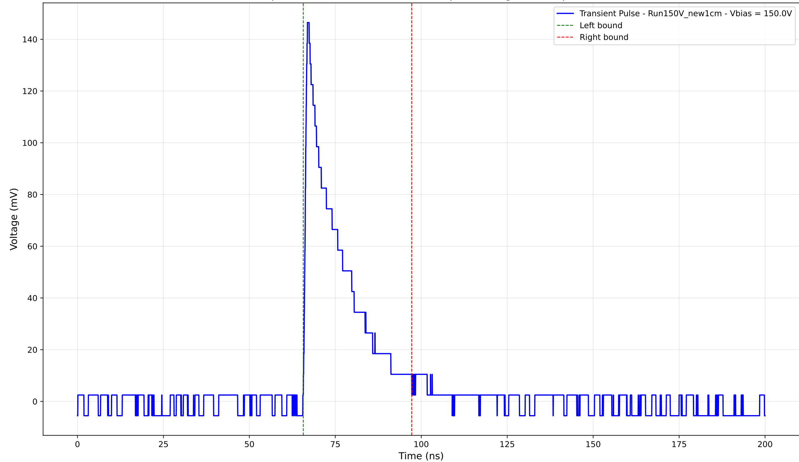
Transient Pulse - Sample: New1cm - Position: 4745.0 \mu\text{m} - Charge: 29.70 pC - Rise Time: 0.97 ns
