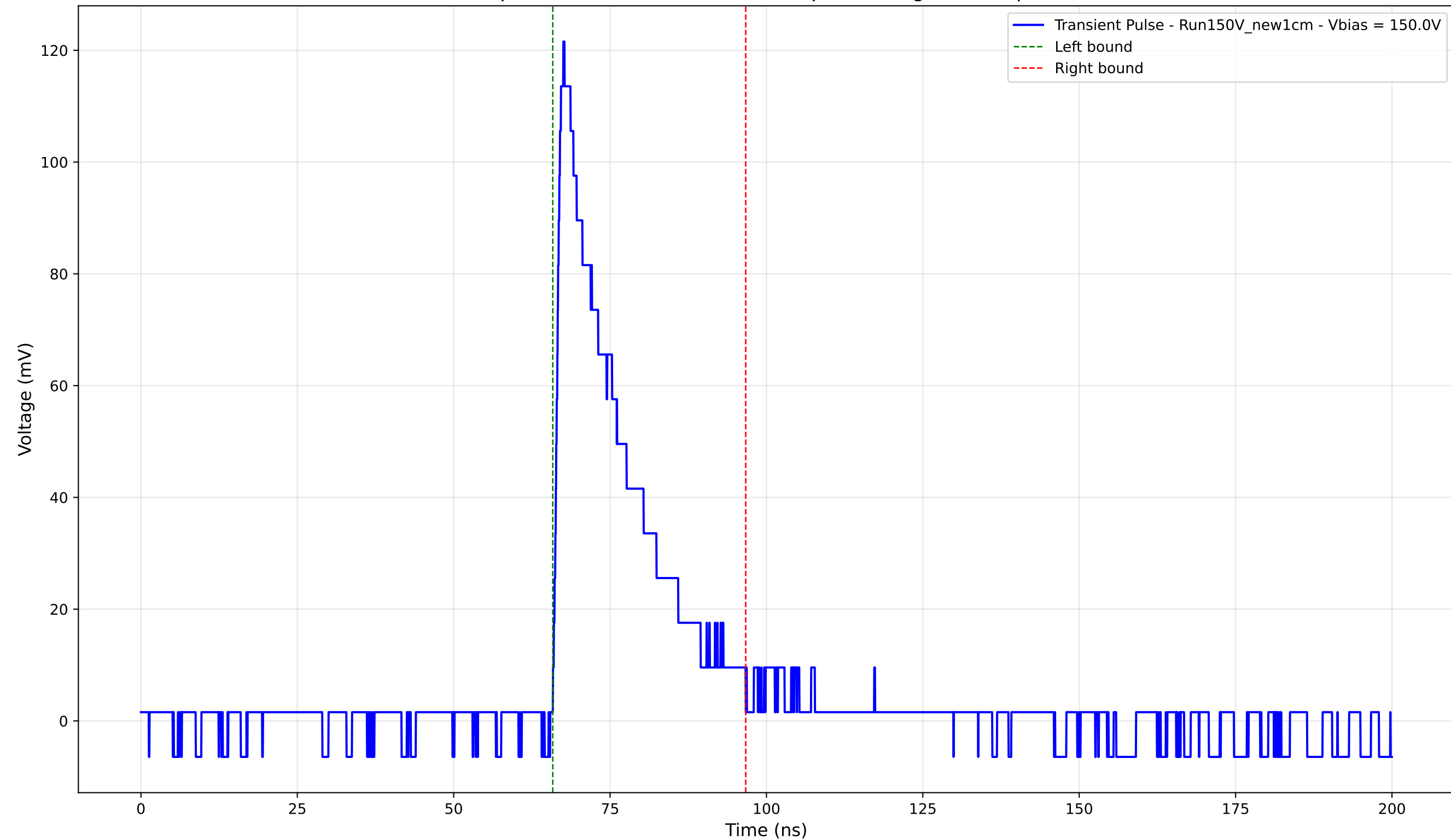
Transient Pulse - Sample: New1cm - Position: 405.0 \mu\text{m} - Charge: 26.04 pC - Rise Time: 1.15 ns
