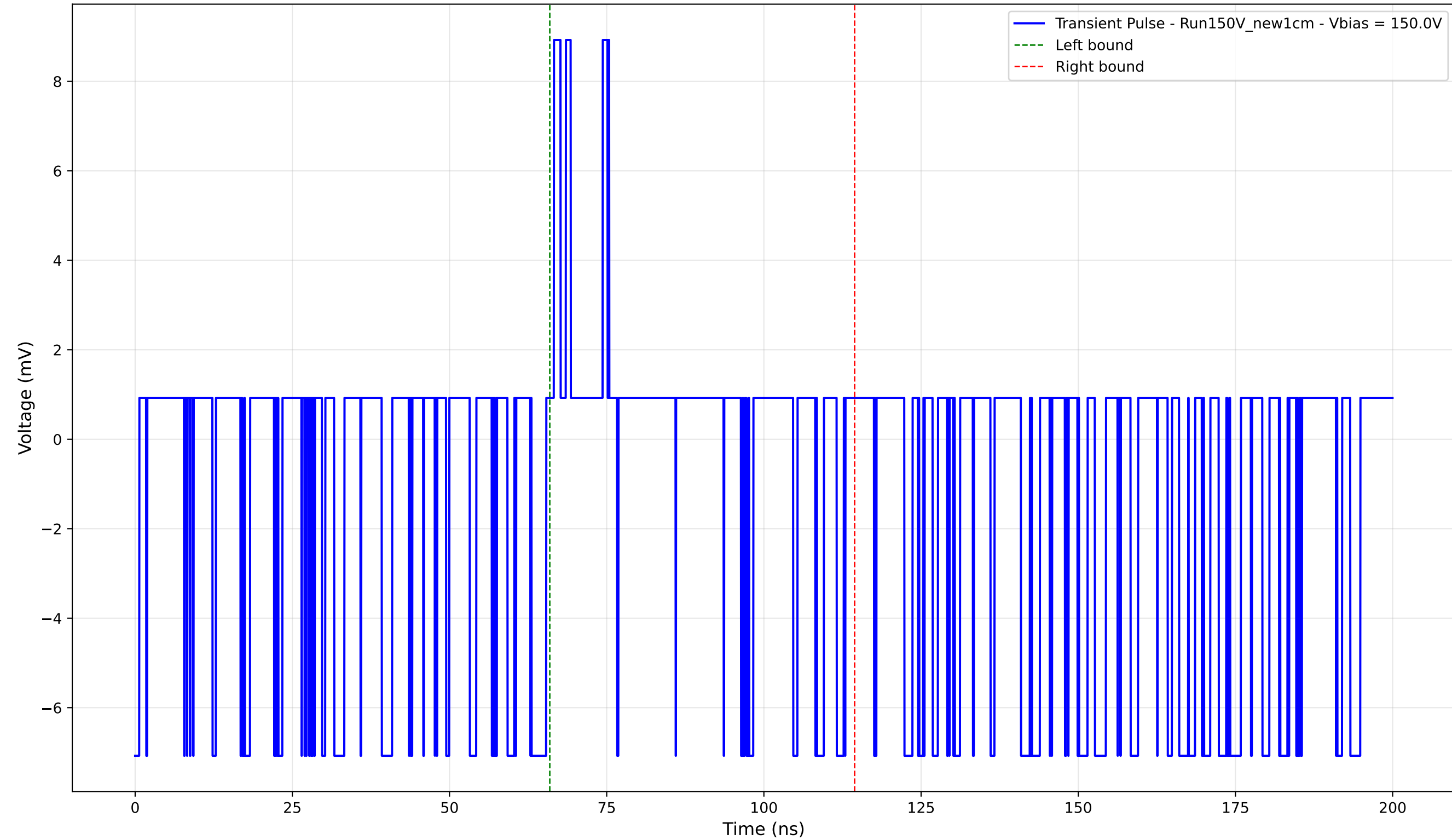
Transient Pulse - Sample: New1cm - Position: 10.0 \mu\text{m} - Charge: 0.56 pC - Rise Time: 0.00 ns (N/A)
