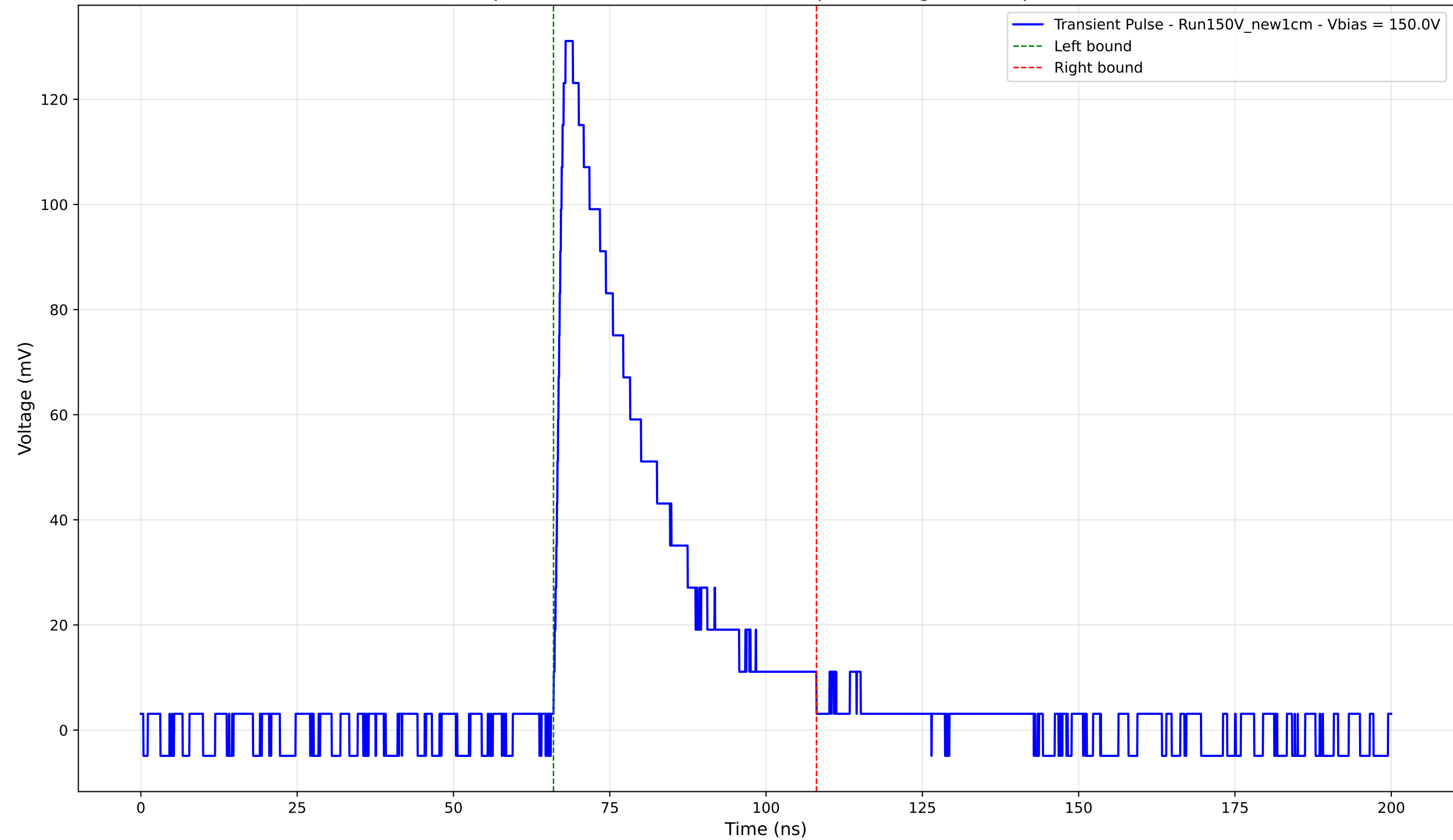
Transient Pulse - Sample: New1cm - Position: 3975.0 \mu\text{m} - Charge: 37.79 pC - Rise Time: 1.45 ns
