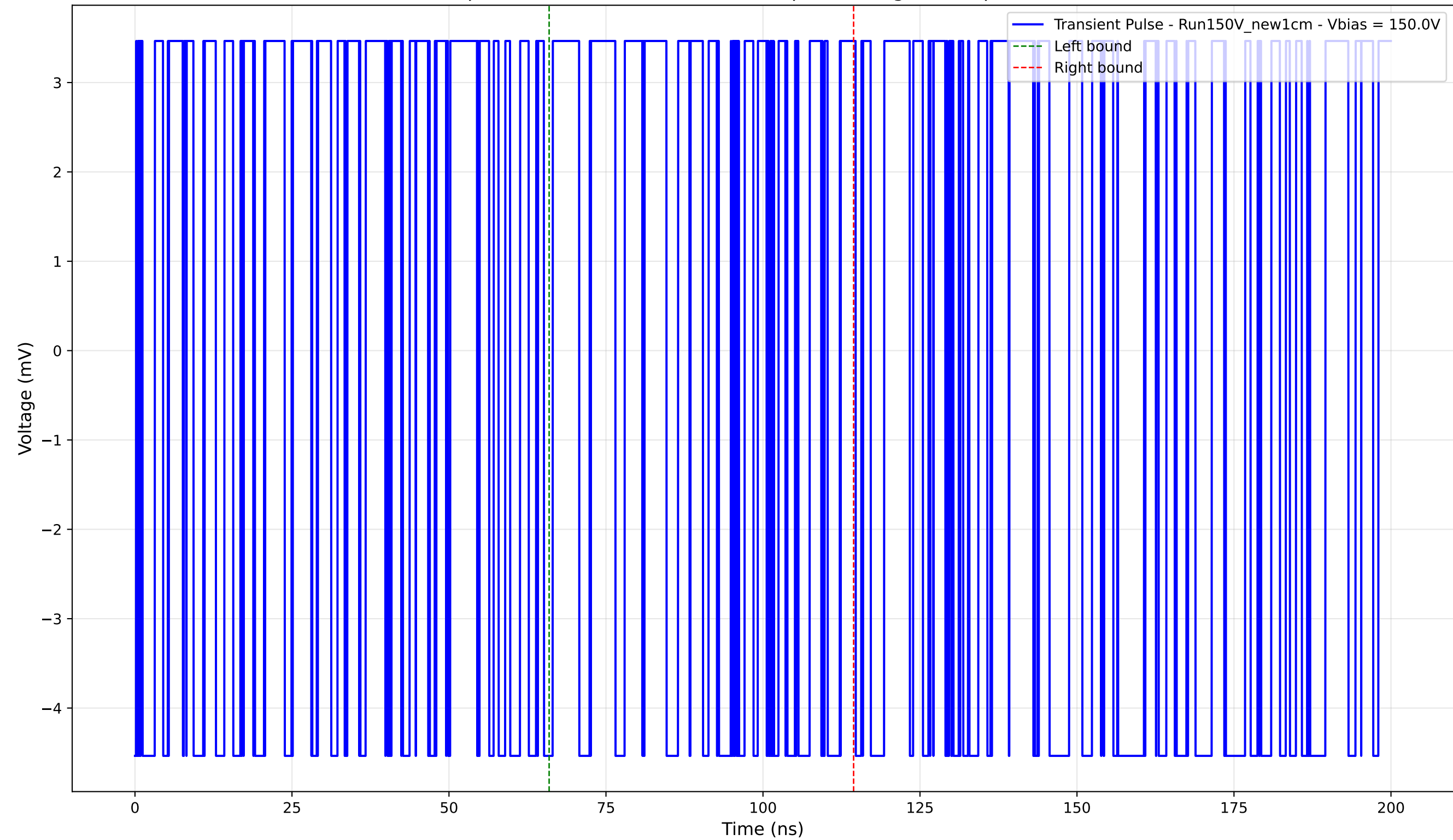
Transient Pulse - Sample: New1cm - Position: 4950.0 \mu\text{m} - Charge: 0.45 pC - Rise Time: 0.00 ns (N/A)
