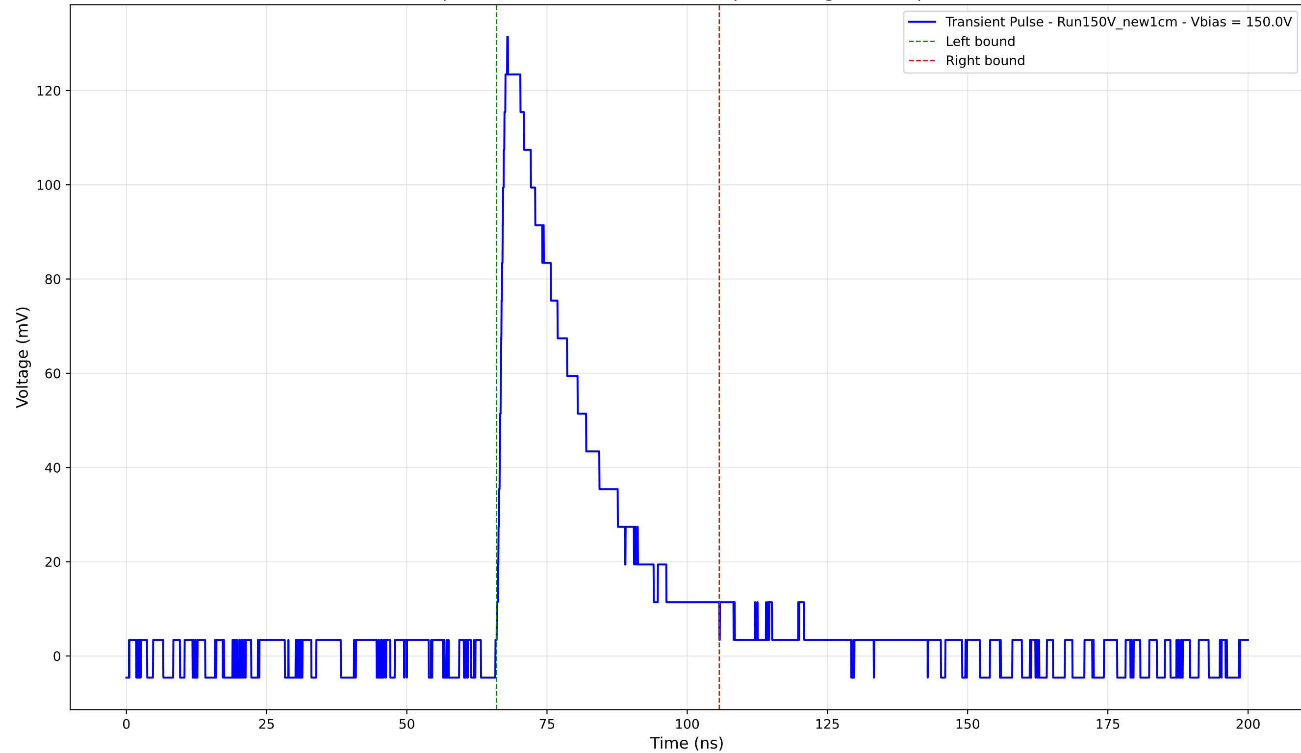
Transient Pulse - Sample: New1cm - Position: 3660.0 \mu\text{m} - Charge: 37.27 pC - Rise Time: 1.36 ns
