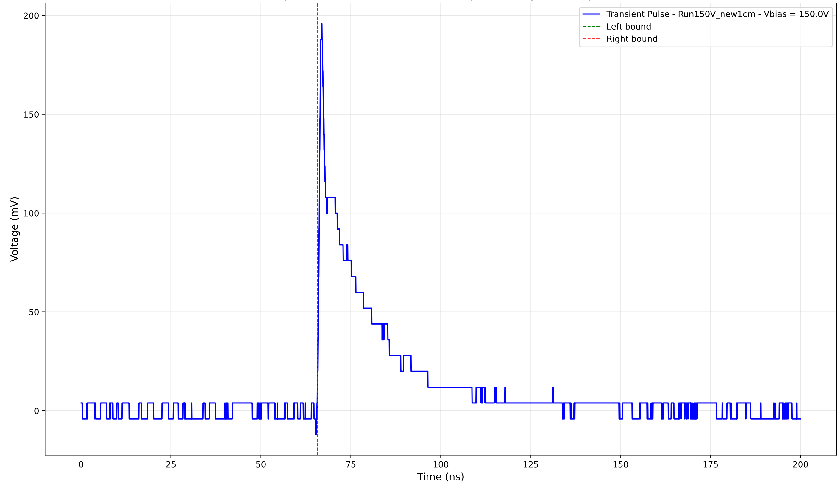
Transient Pulse - Sample: New1cm - Position: 2755.0 \mu\text{m} - Charge: 38.11 pC - Rise Time: 0.82 ns
