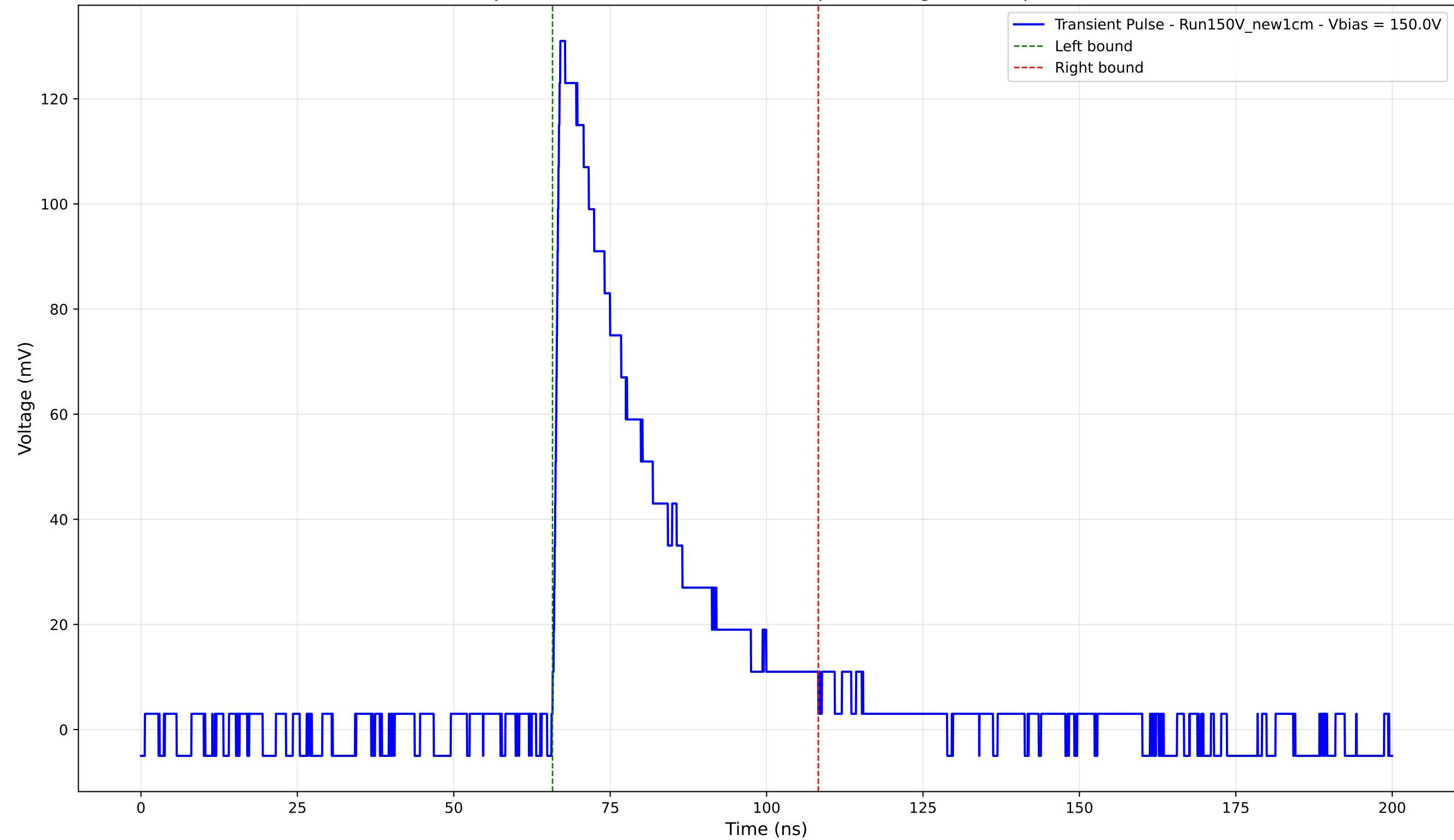
Transient Pulse - Sample: New1cm - Position: 3165.0 \mu\text{m} - Charge: 38.44 pC - Rise Time: 0.95 ns
