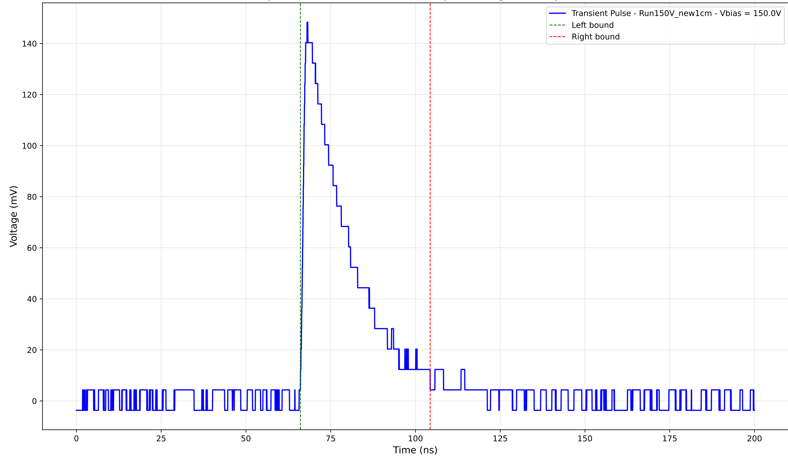
Transient Pulse - Sample: New1cm - Position: 3925.0 \mu\text{m} - Charge: 41.18 pC - Rise Time: 1.39 ns
