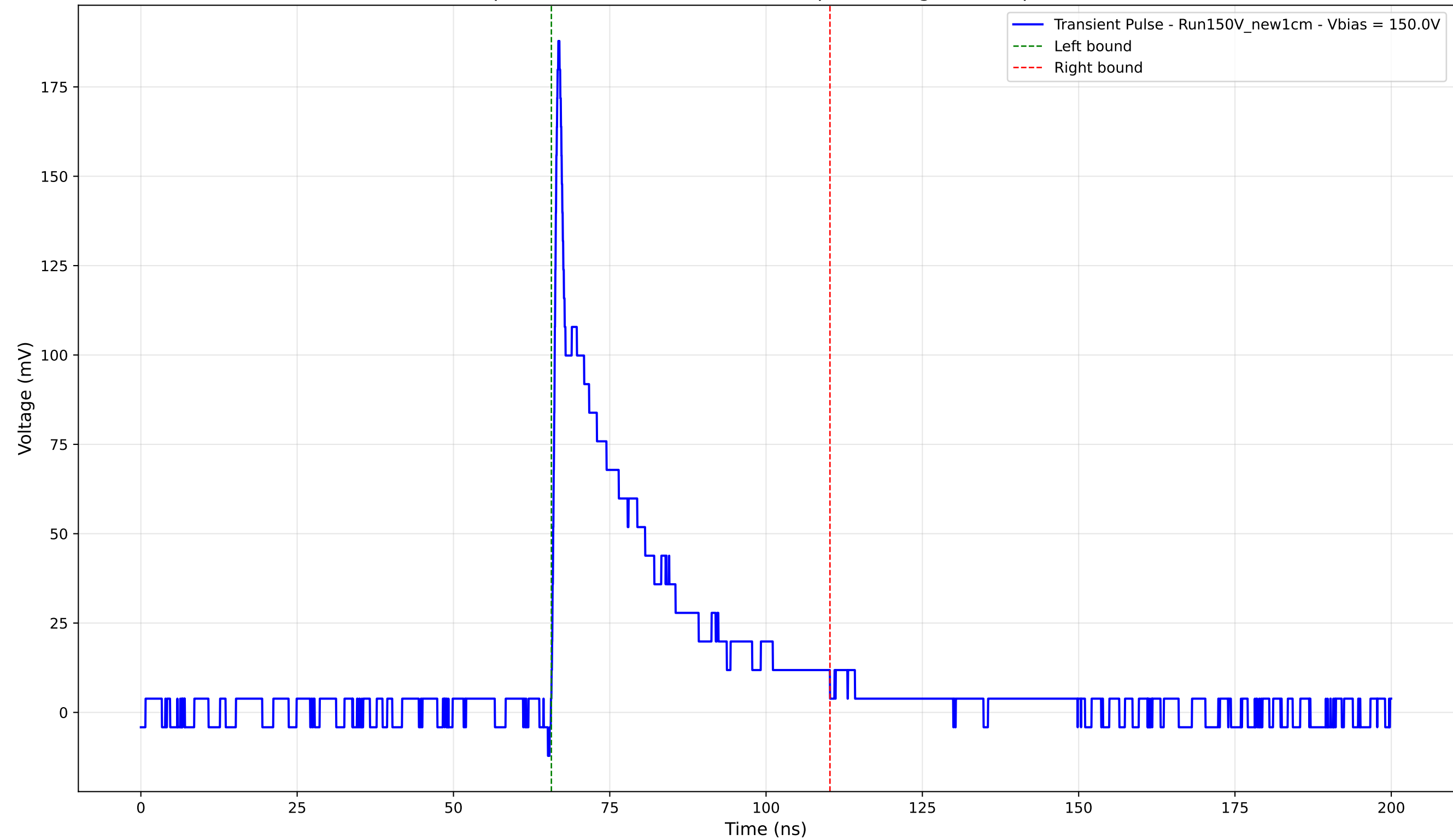
Transient Pulse - Sample: New1cm - Position: 2345.0 \mu\text{m} - Charge: 37.71 pC - Rise Time: 0.82 ns
