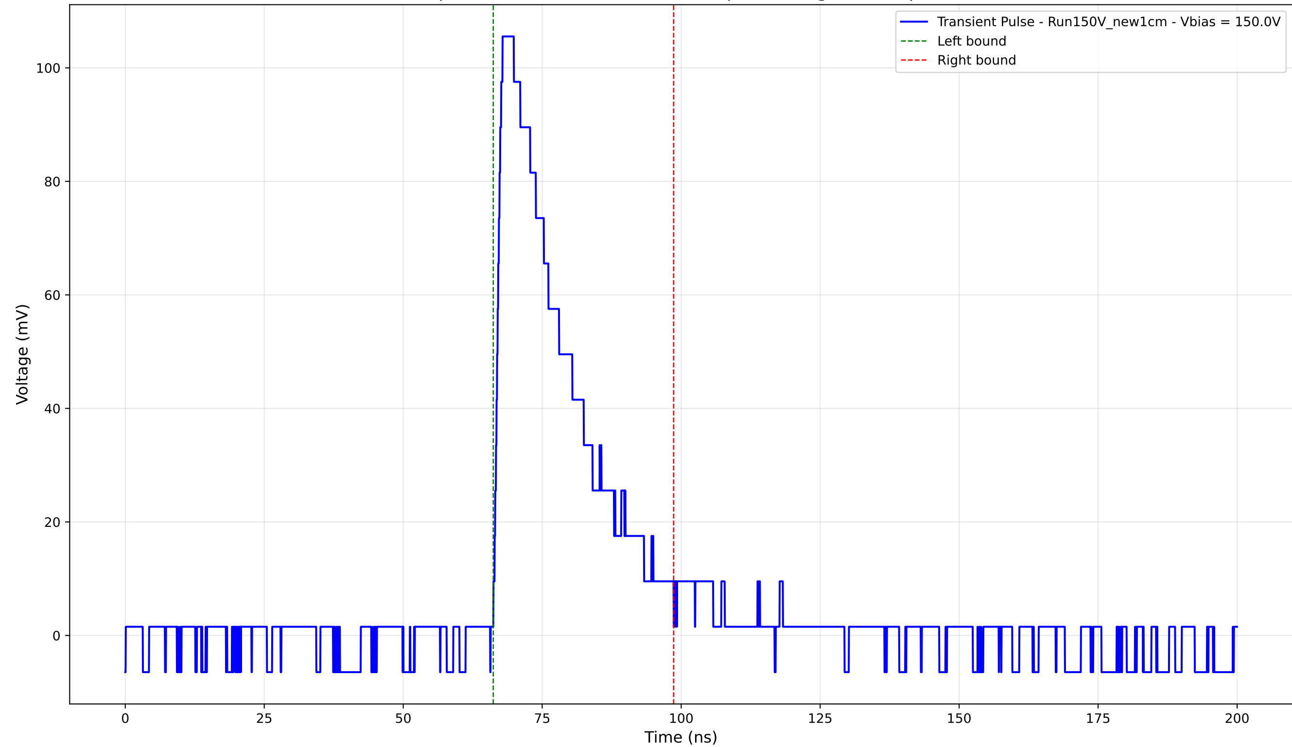
Transient Pulse - Sample: New1cm - Position: 1190.0 \mu\text{m} - Charge: 28.82 pC - Rise Time: 1.20 ns
