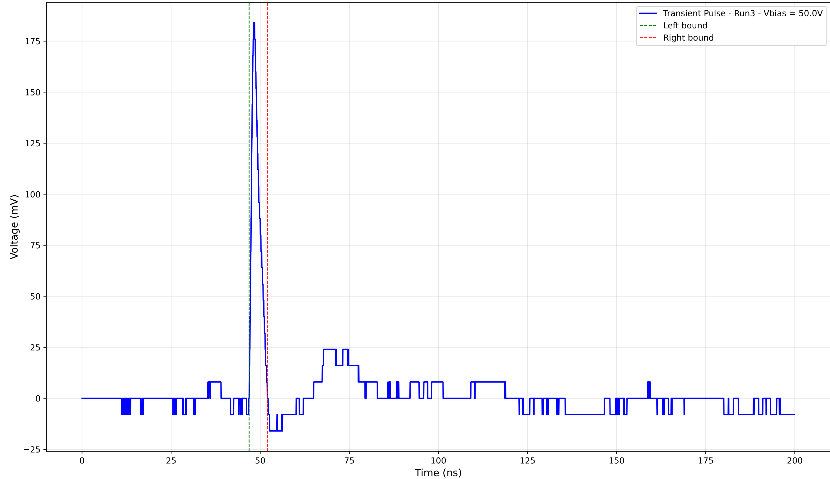
Transient Pulse - Sample: 4003 - Position: 530.0 \mu\text{m} - Charge: 9.23 pC - Rise Time: 0.87 ns
