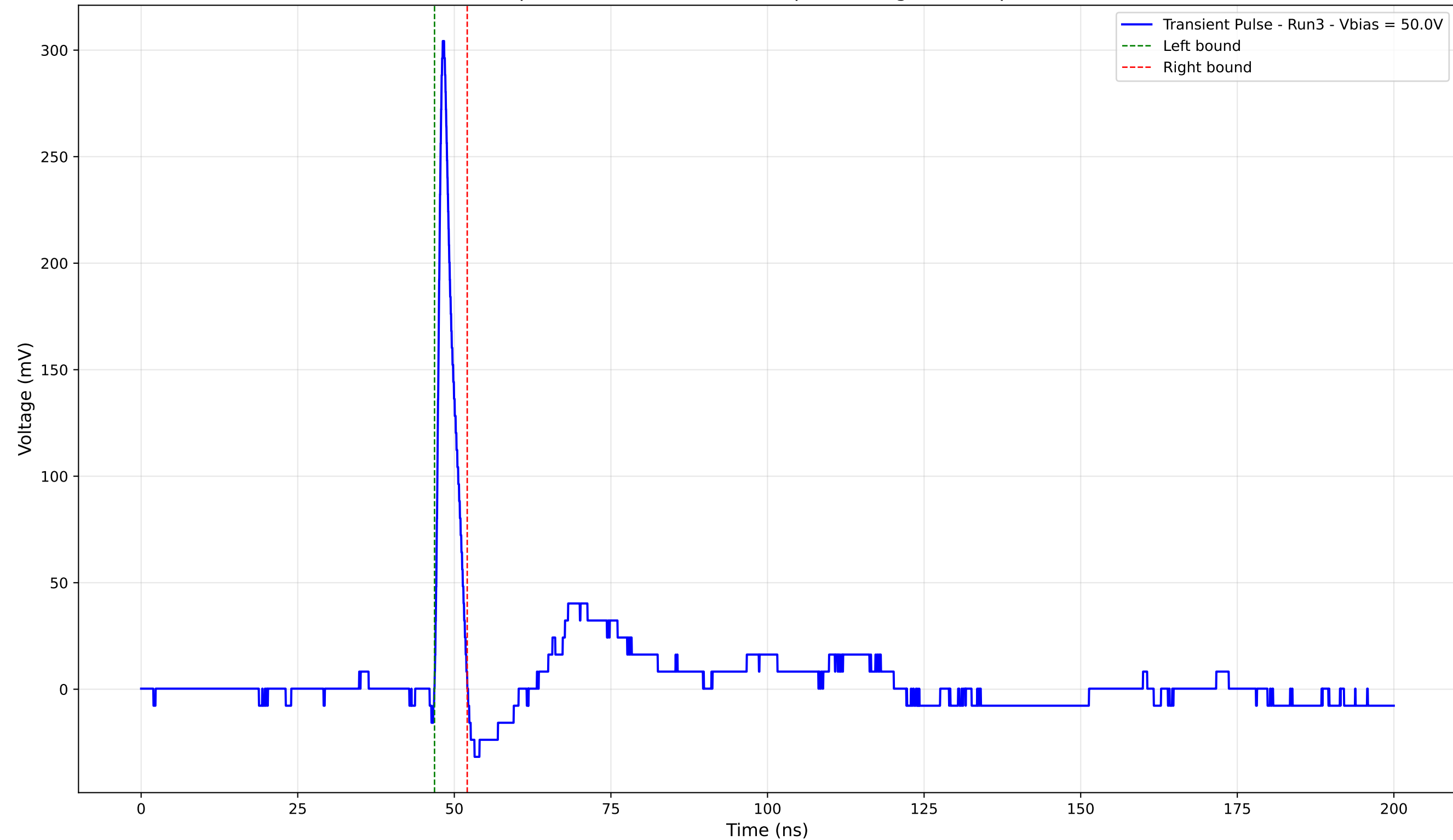
Transient Pulse - Sample: 4003 - Position: 415.0 \mu\text{m} - Charge: 15.32 pC - Rise Time: 0.92 ns
