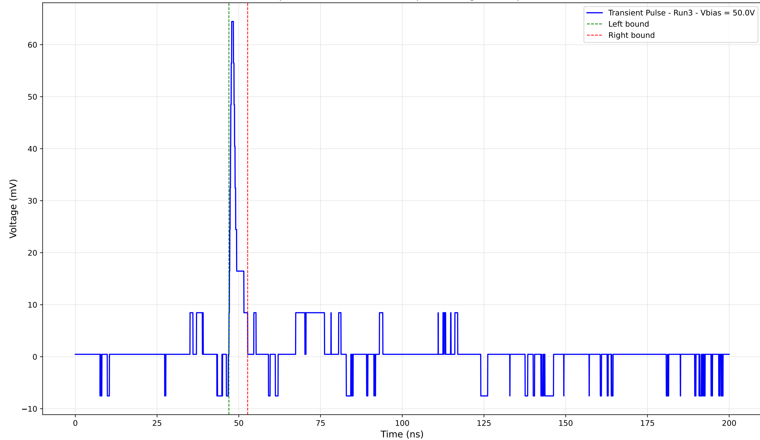
Transient Pulse - Sample: 4003 - Position: 75.0 \mu\text{m} - Charge: 2.92 pC - Rise Time: 0.83 ns
