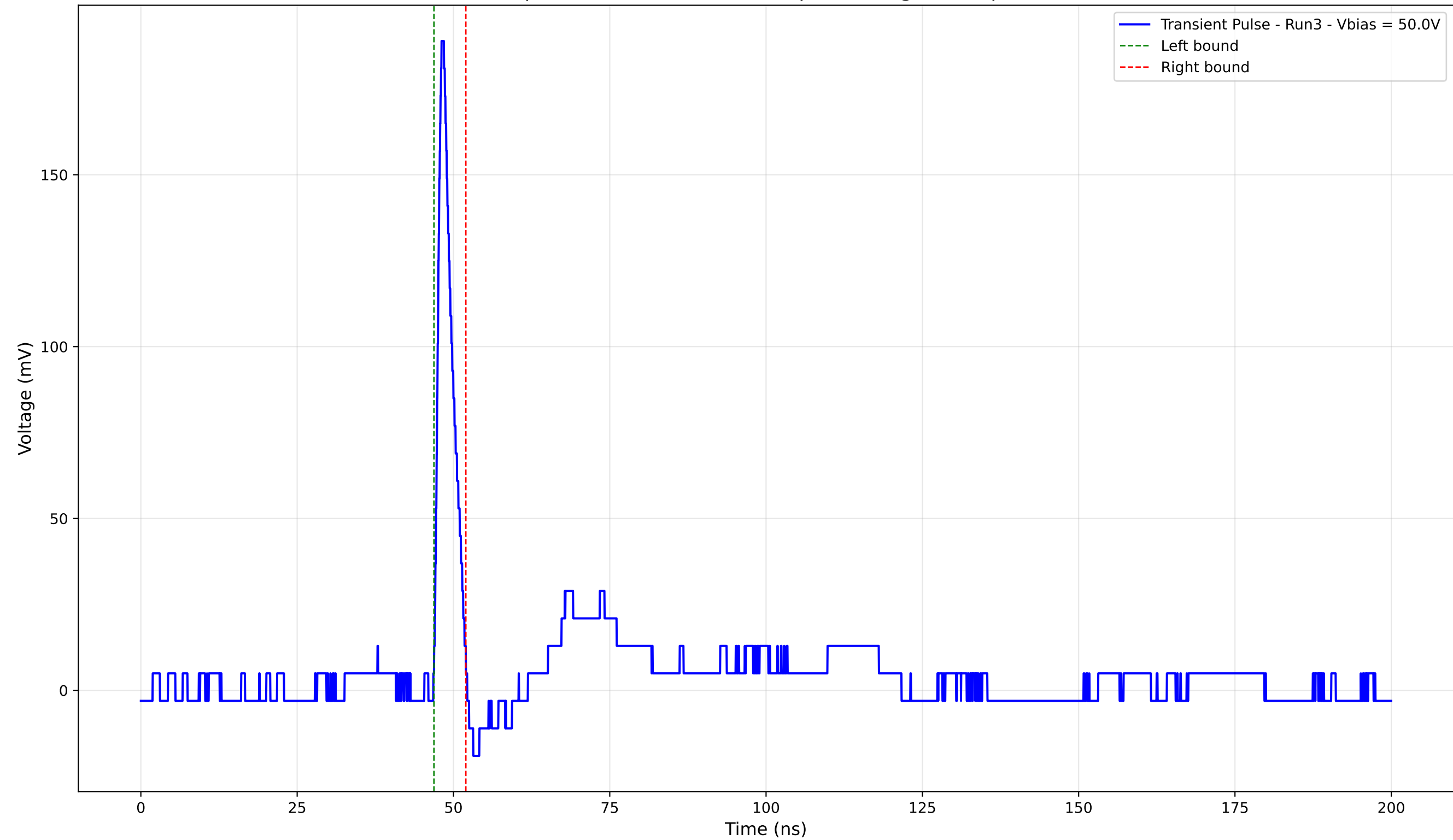
Transient Pulse - Sample: 4003 - Position: 515.0 \mu\text{m} - Charge: 9.76 pC - Rise Time: 0.93 ns
