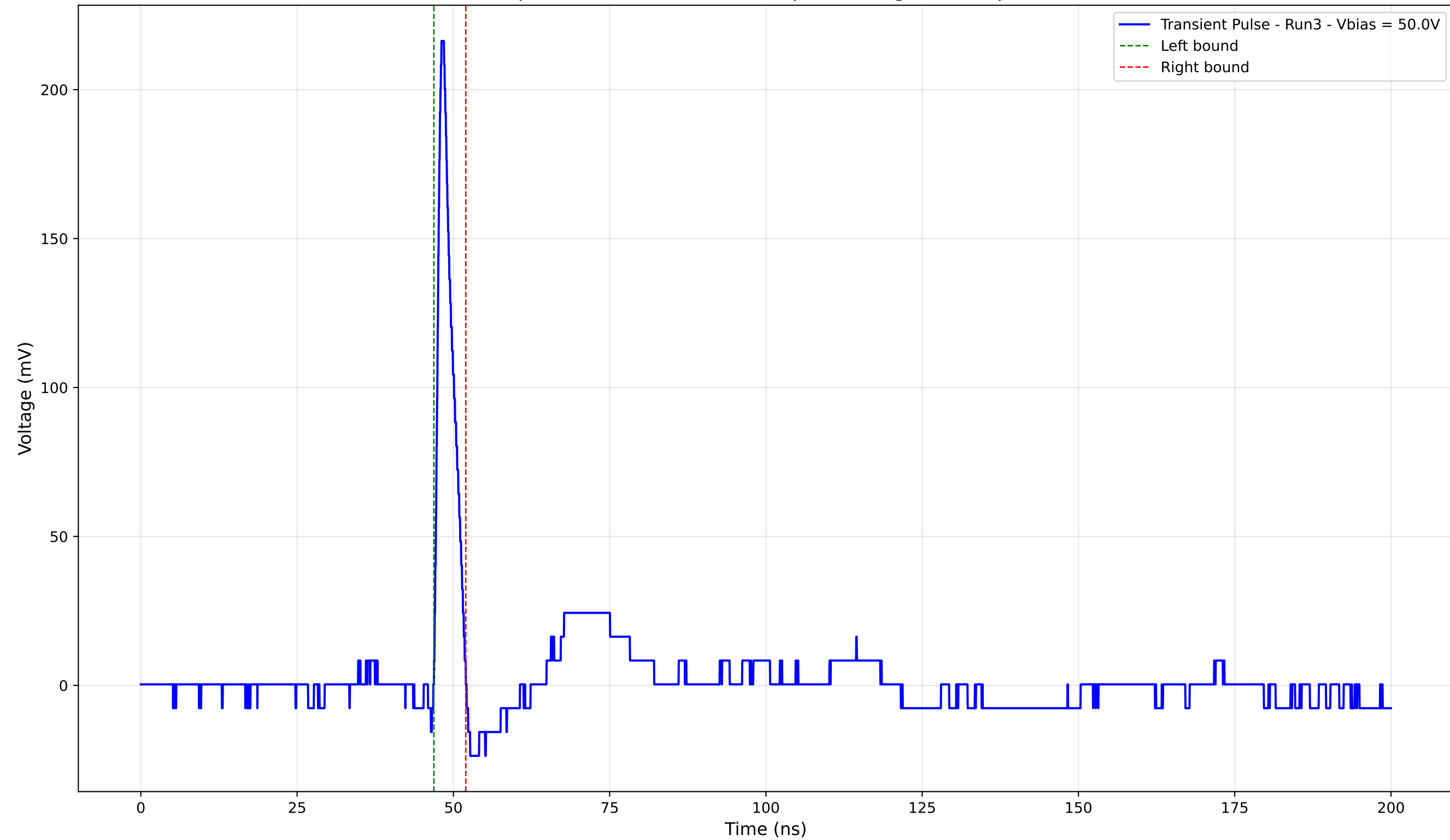
Transient Pulse - Sample: 4003 - Position: 485.0 \mu\text{m} - Charge: 11.23 pC - Rise Time: 0.91 ns
