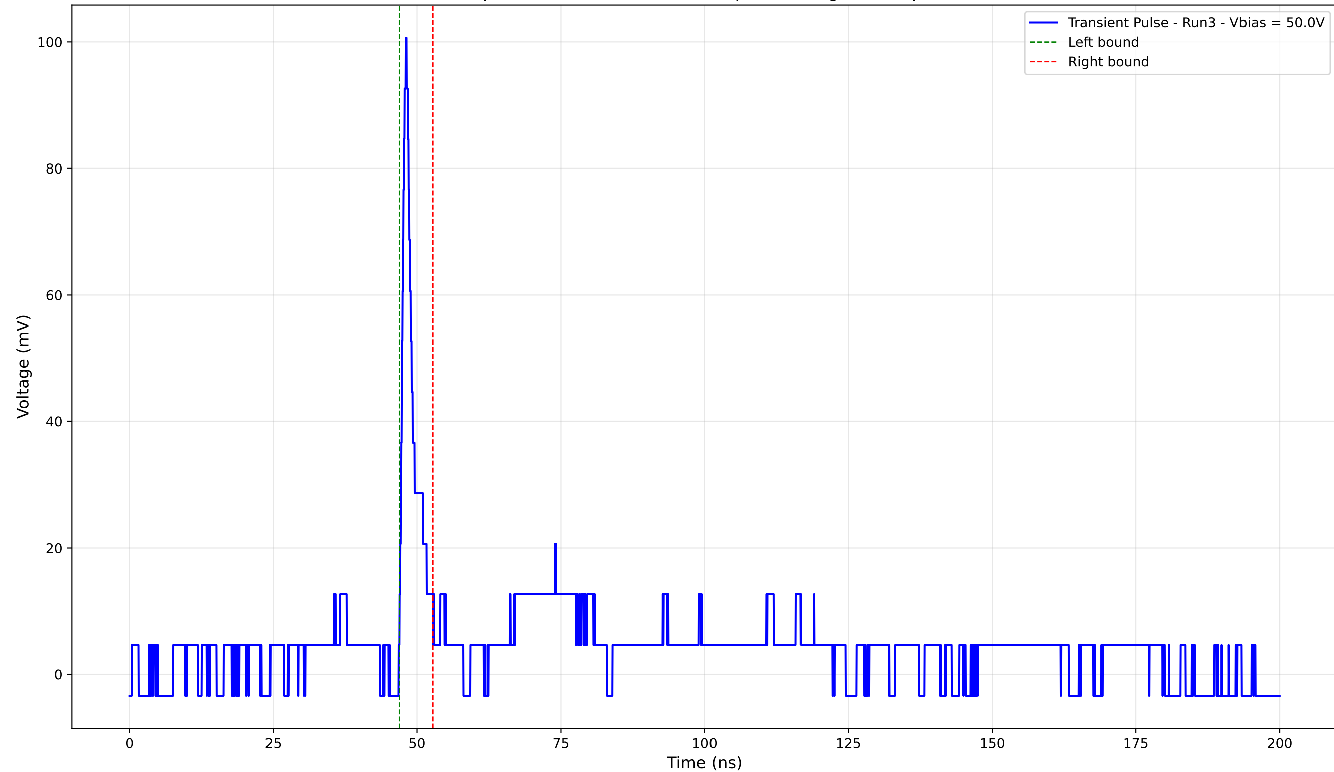
Transient Pulse - Sample: 4003 - Position: 100.0 \mu\text{m} - Charge: 4.62 pC - Rise Time: 0.89 ns
