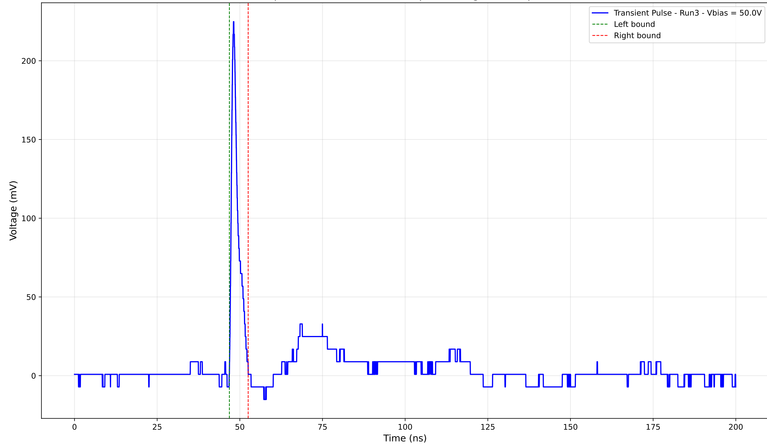
Transient Pulse - Sample: 4003 - Position: 190.0 \mu\text{m} - Charge: 10.43 pC - Rise Time: 0.89 ns
