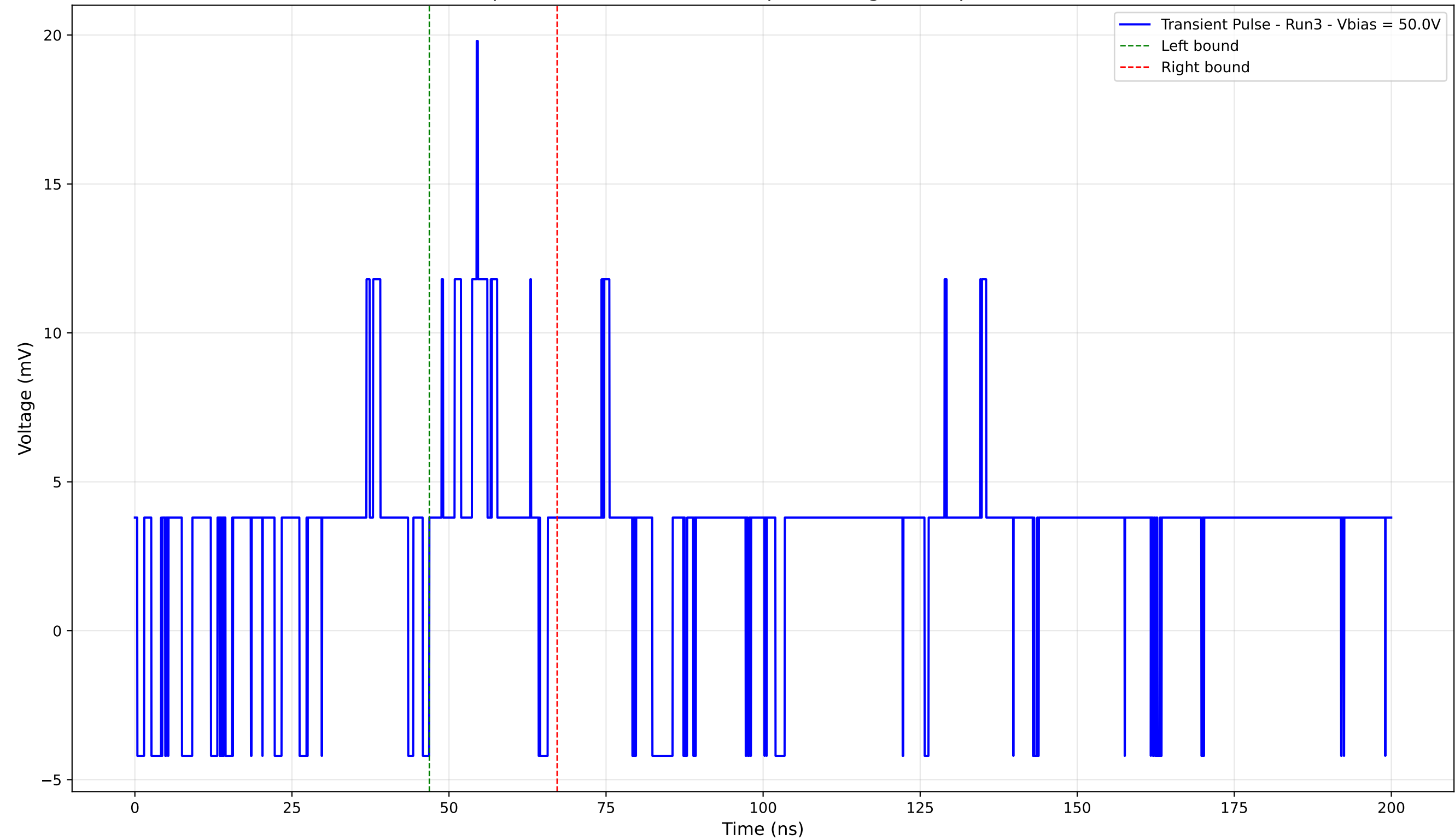
Transient Pulse - Sample: 4003 - Position: 645.0 \mu\text{m} - Charge: 2.11 pC - Rise Time: 0.00 ns (N/A)
