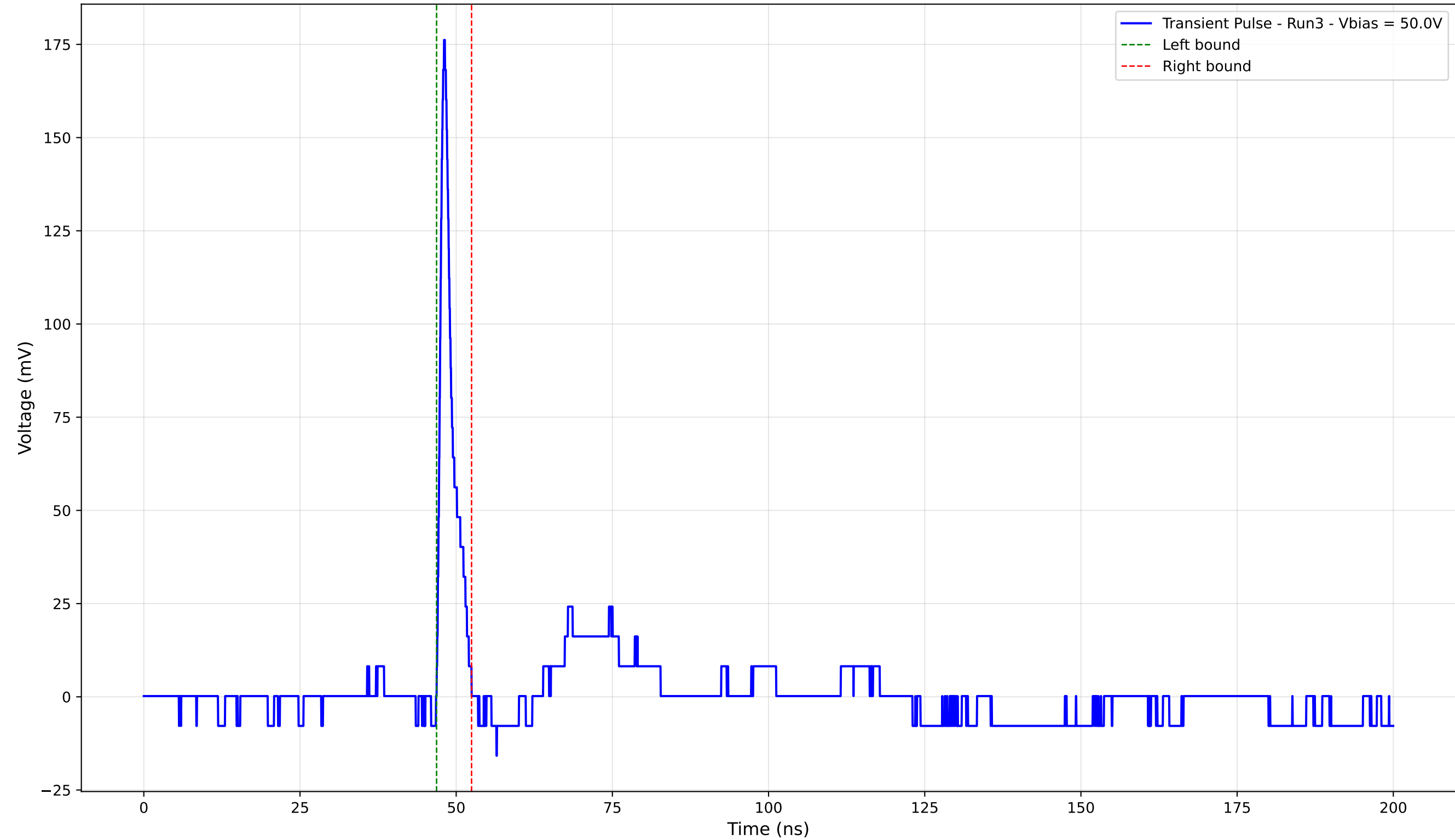
Transient Pulse - Sample: 4003 - Position: 160.0 \mu\text{m} - Charge: 7.93 pC - Rise Time: 0.80 ns
