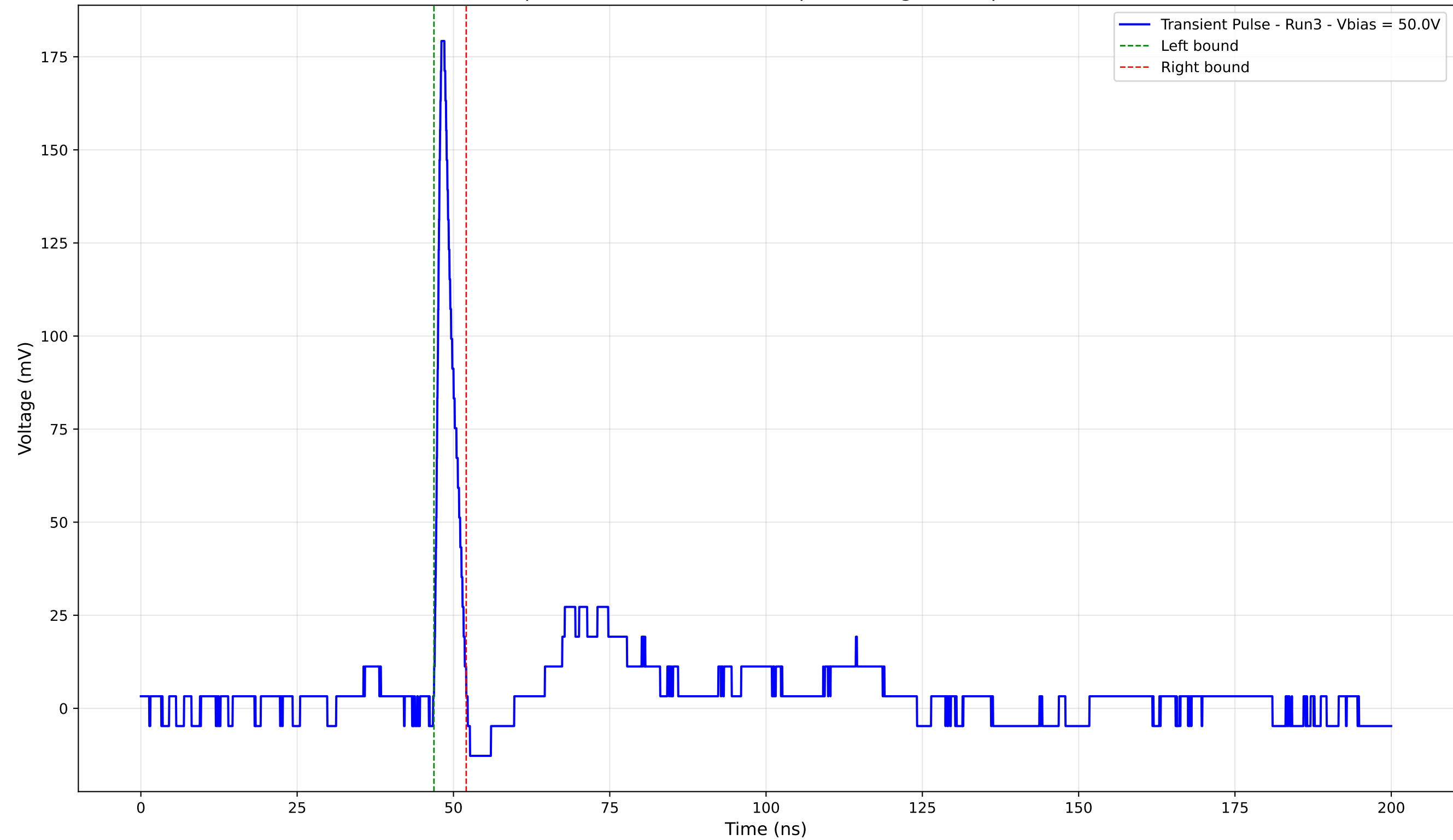
Transient Pulse - Sample: 4003 - Position: 520.0 \mu\text{m} - Charge: 9.53 pC - Rise Time: 0.90 ns
