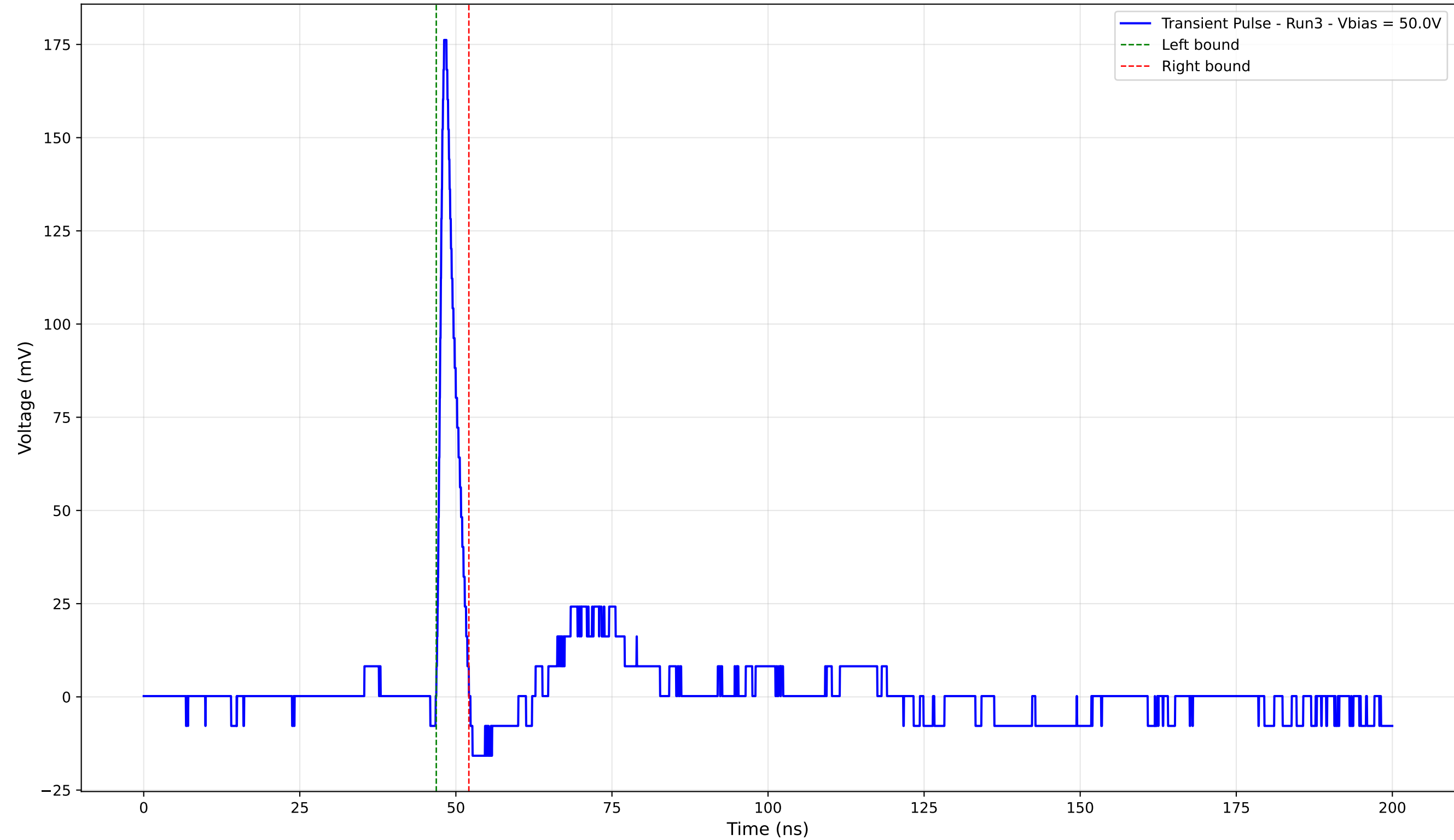
Transient Pulse - Sample: 4003 - Position: 525.0 \mu\text{m} - Charge: 9.12 pC - Rise Time: 0.88 ns
