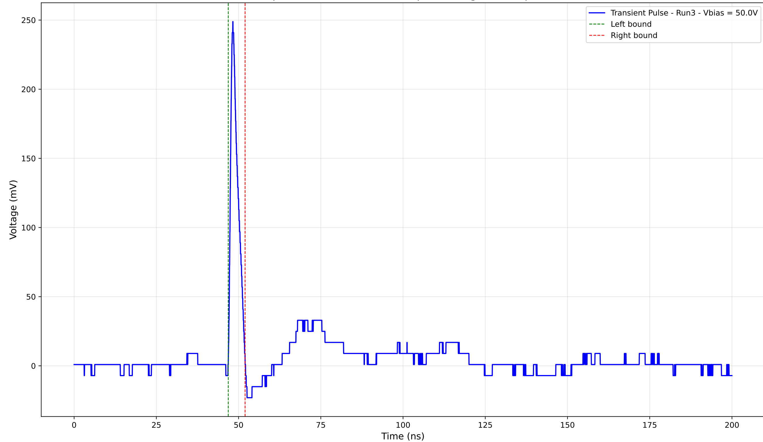
Transient Pulse - Sample: 4003 - Position: 465.0 \mu\text{m} - Charge: 12.55 pC - Rise Time: 0.92 ns
