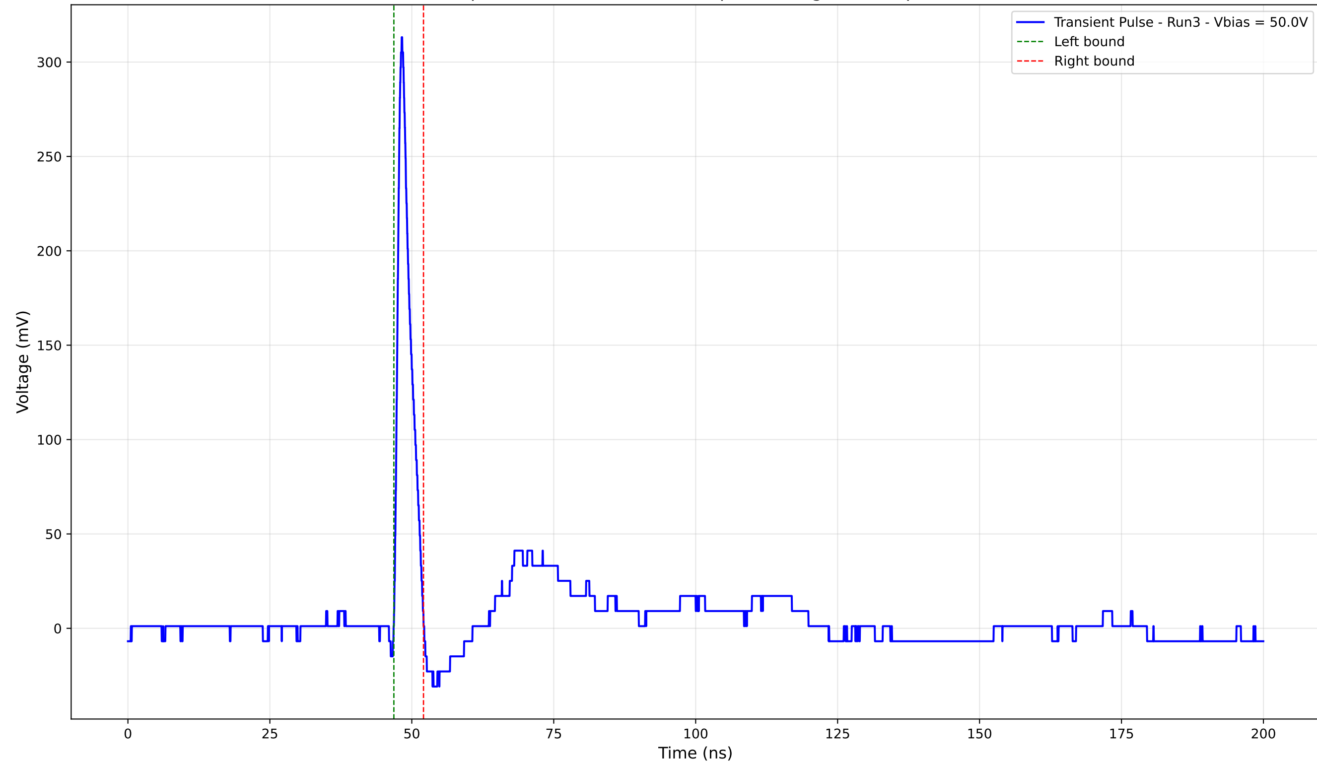
Transient Pulse - Sample: 4003 - Position: 405.0 \mu\text{m} - Charge: 15.75 pC - Rise Time: 0.92 ns
