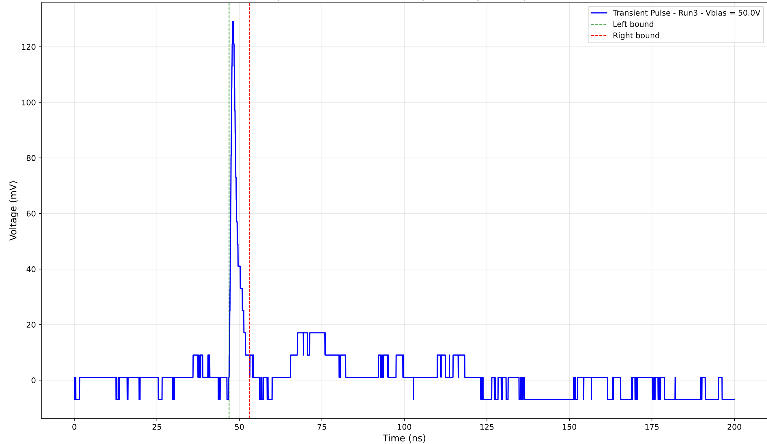
Transient Pulse - Sample: 4003 - Position: 125.0 \mu\text{m} - Charge: 5.92 pC - Rise Time: 0.81 ns
