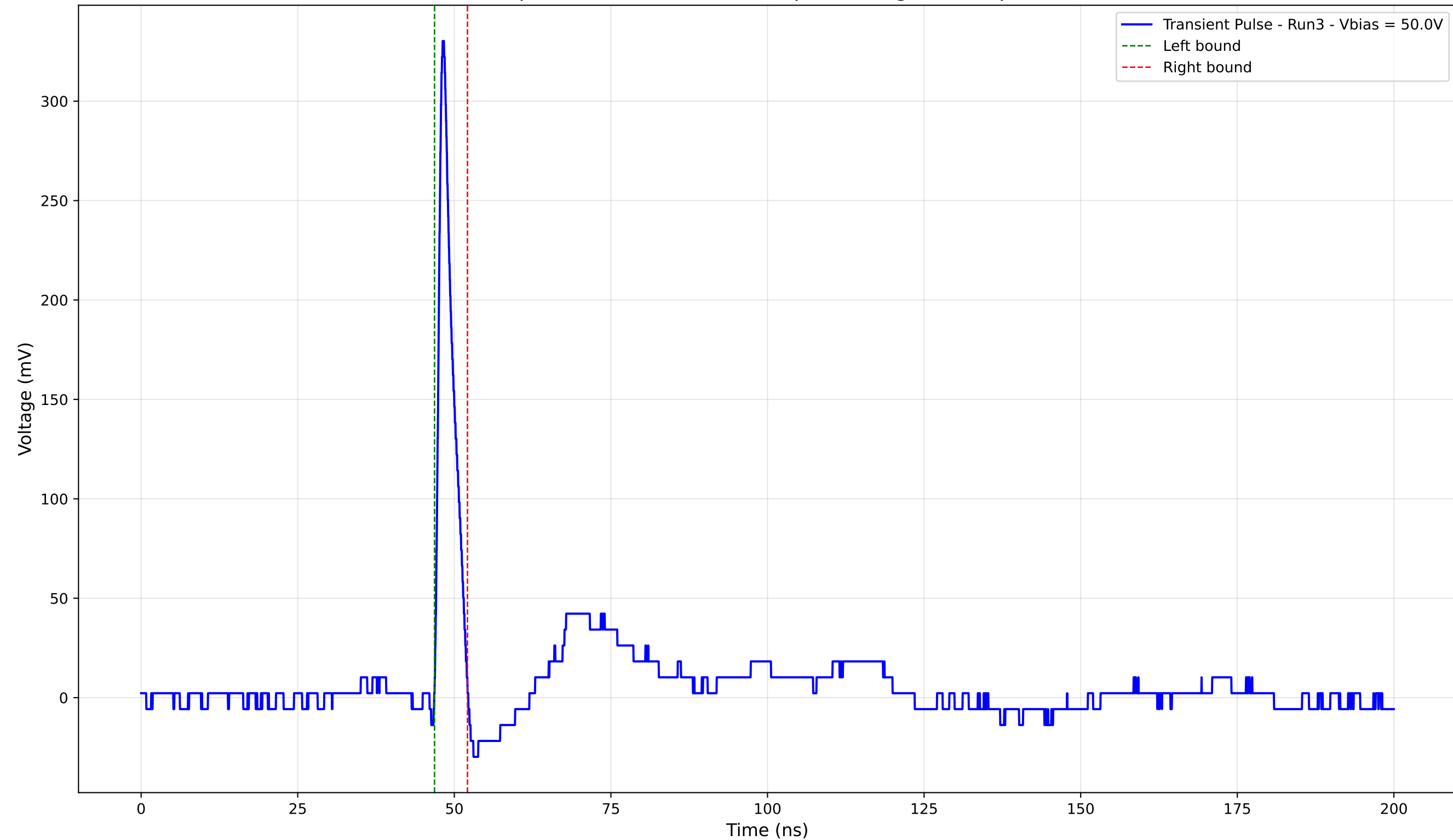
Transient Pulse - Sample: 4003 - Position: 370.0 \mu\text{m} - Charge: 16.78 pC - Rise Time: 0.88 ns
