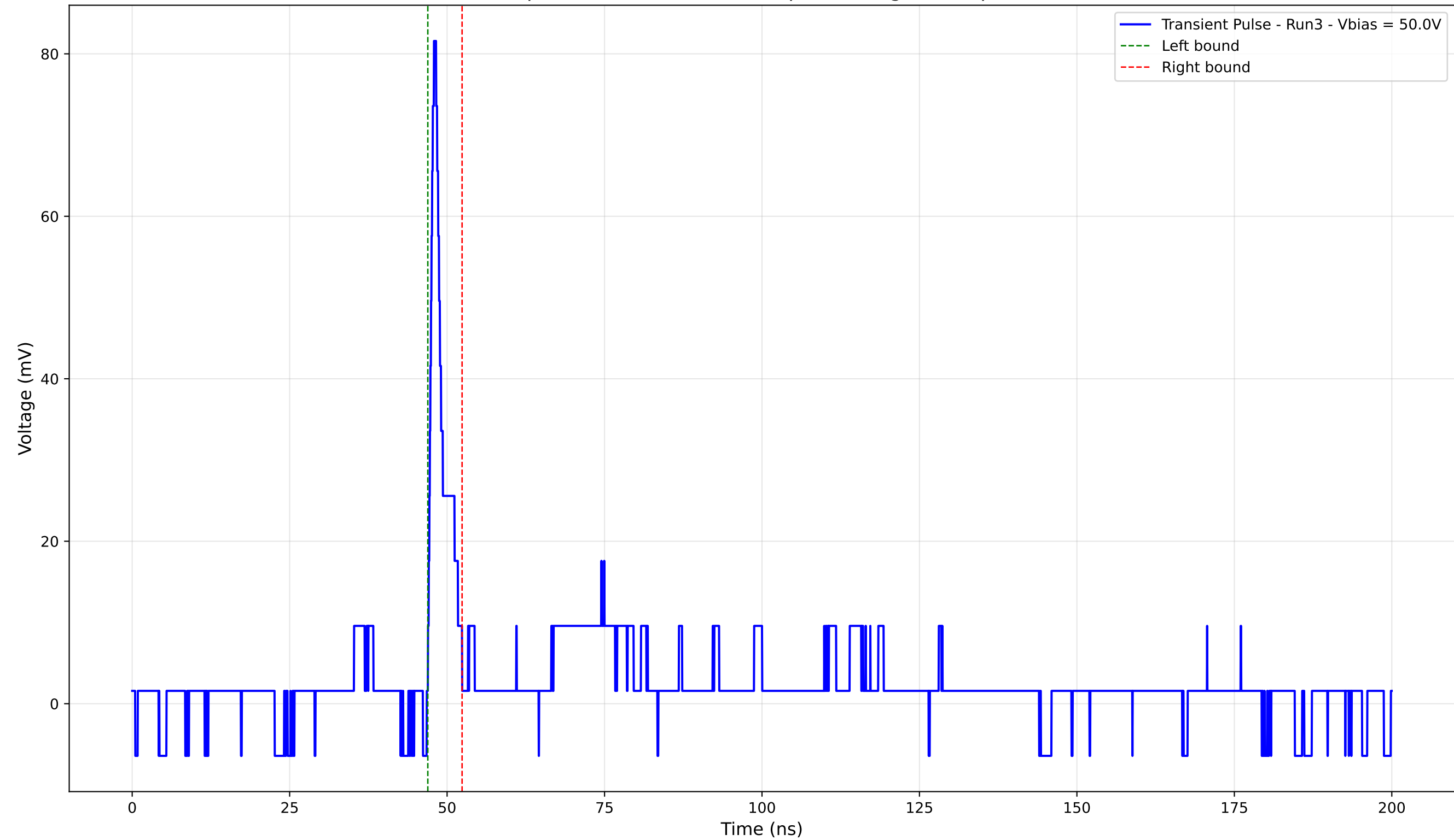
Transient Pulse - Sample: 4003 - Position: 85.0 \mu\text{m} - Charge: 3.77 pC - Rise Time: 0.76 ns
