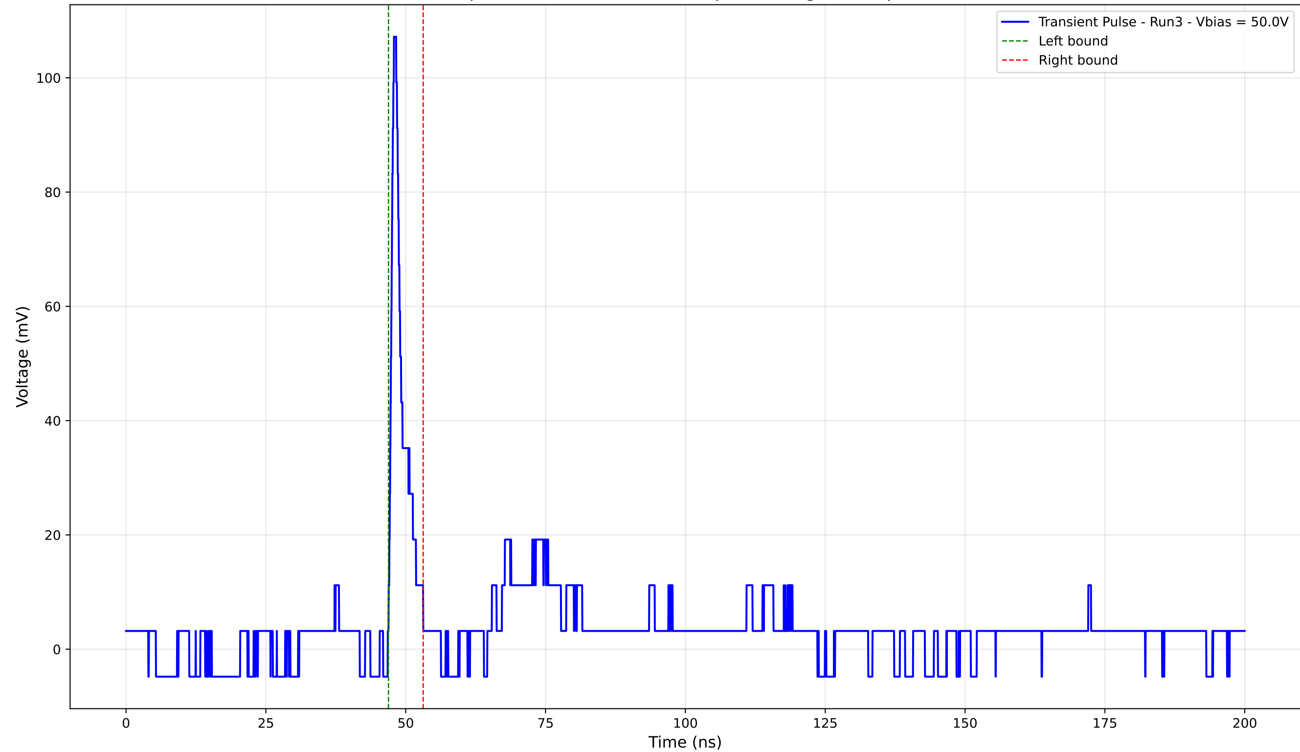
Transient Pulse - Sample: 4003 - Position: 110.0 \mu\text{m} - Charge: 5.15 pC - Rise Time: 0.84 ns
