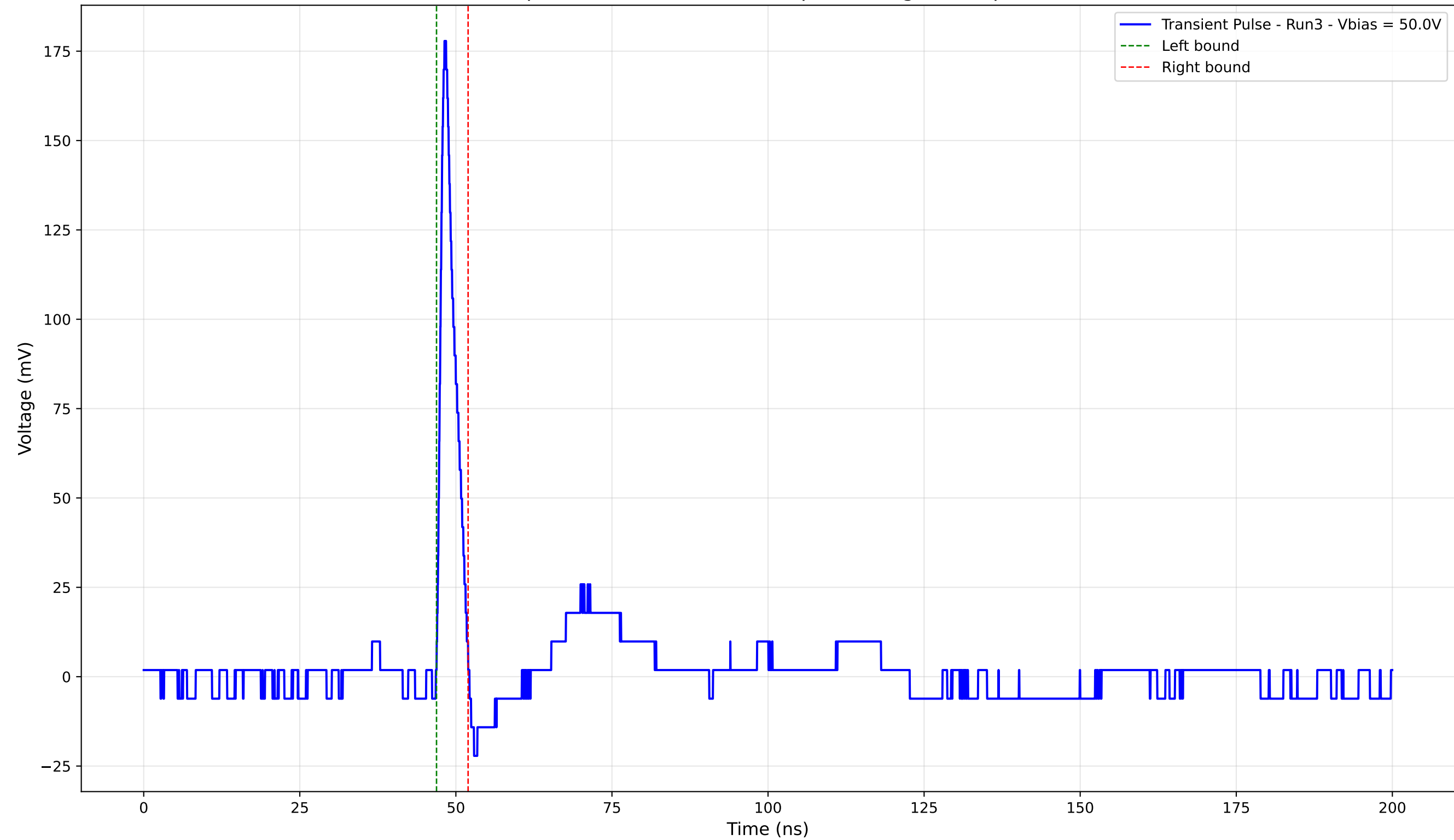
Transient Pulse - Sample: 4003 - Position: 535.0 \mu\text{m} - Charge: 9.08 pC - Rise Time: 0.94 ns
