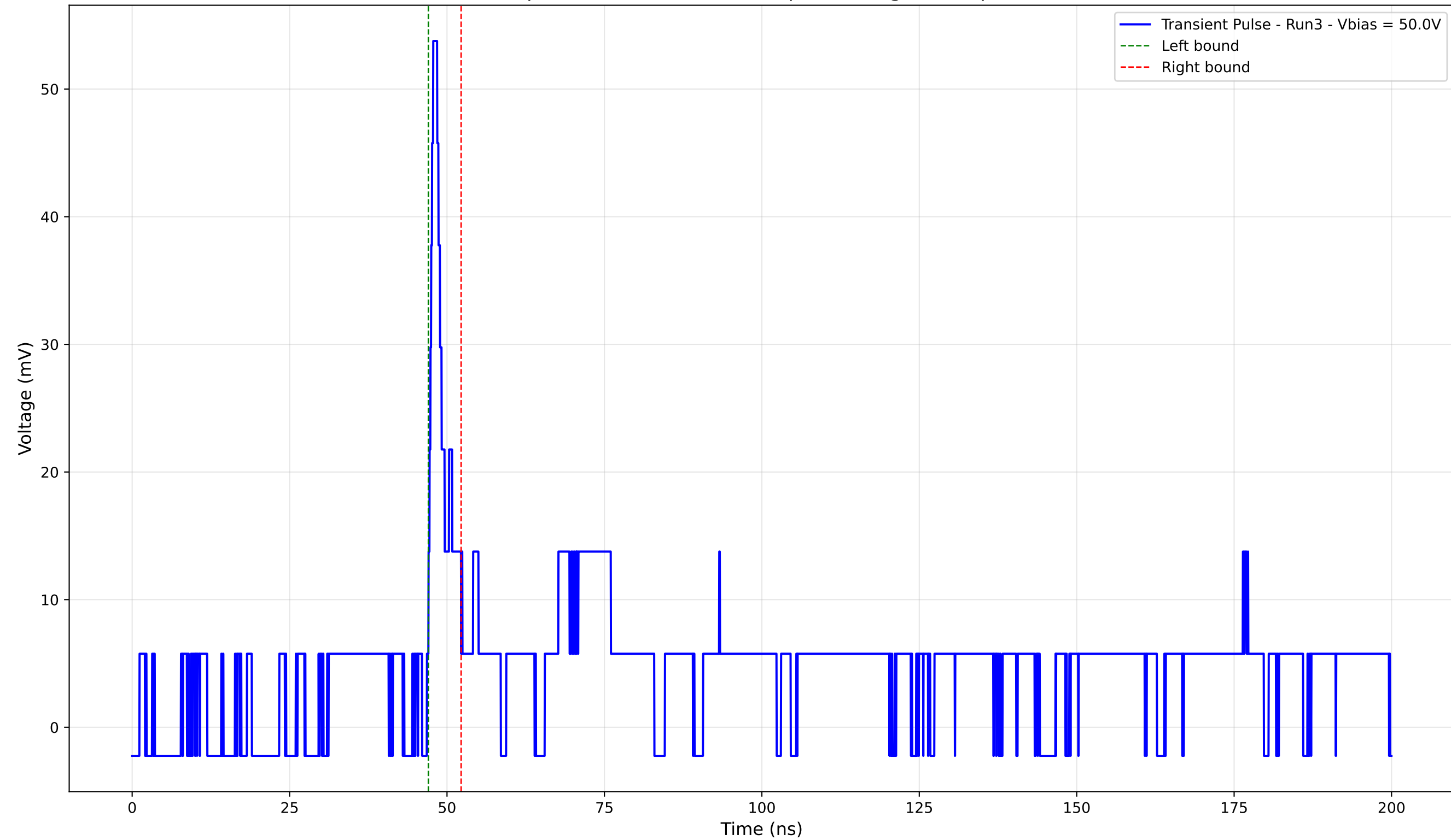
Transient Pulse - Sample: 4003 - Position: 60.0 \mu\text{m} - Charge: 2.67 pC - Rise Time: 1.00 ns
