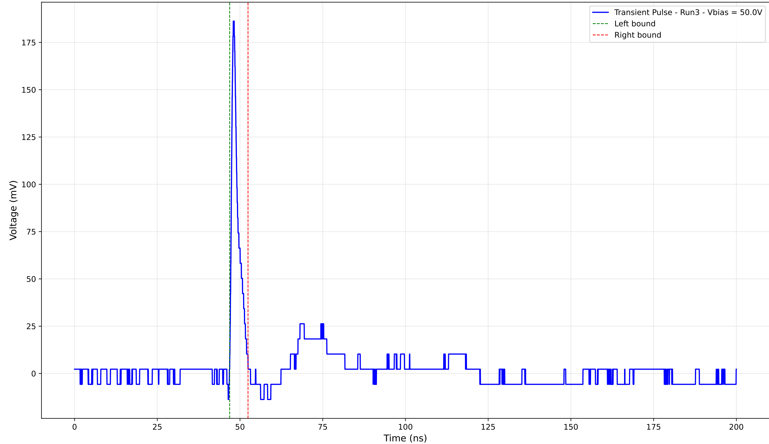
Transient Pulse - Sample: 4003 - Position: 170.0 \mu\text{m} - Charge: 8.59 pC - Rise Time: 0.80 ns
