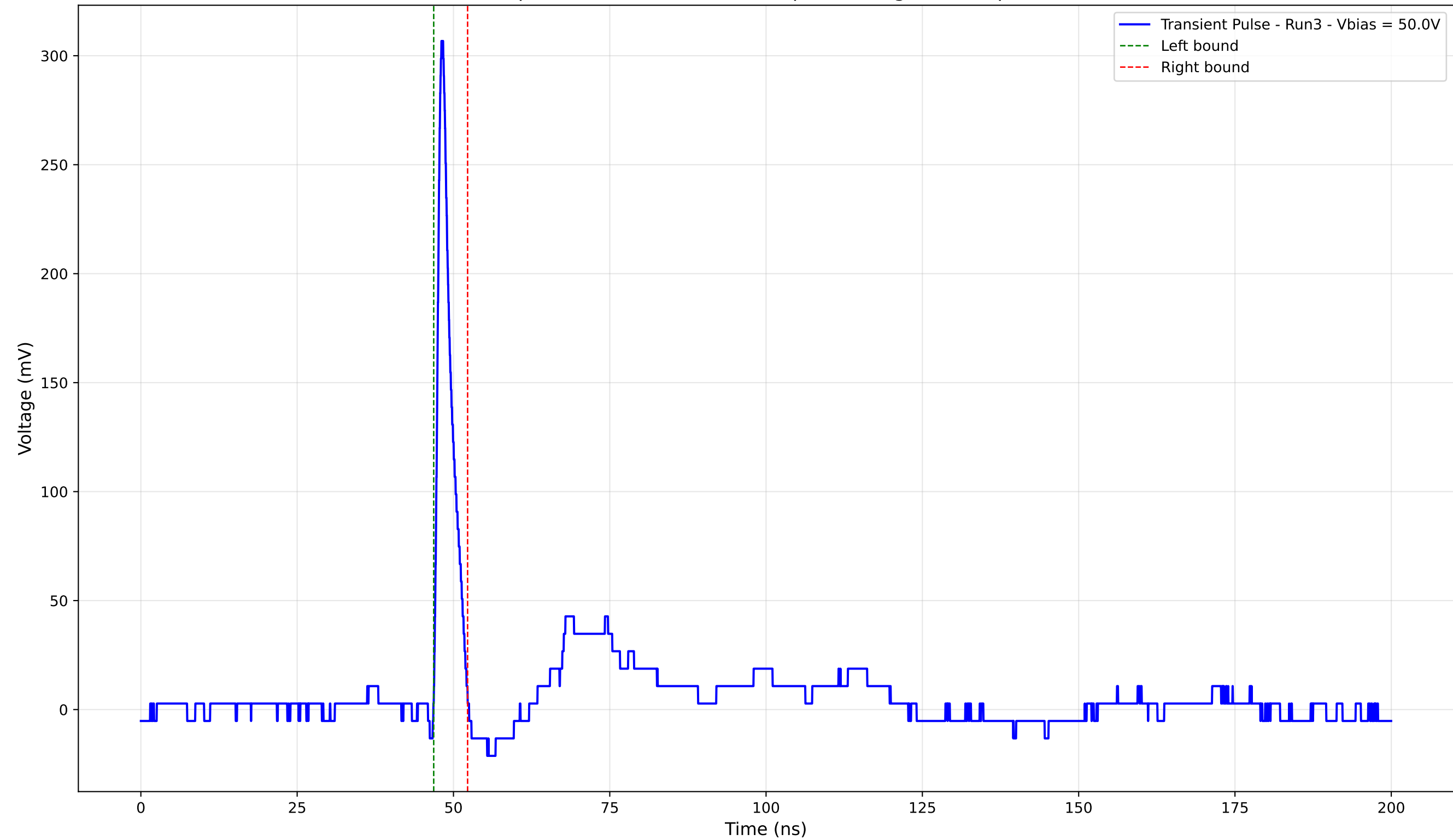
Transient Pulse - Sample: 4003 - Position: 270.0 \mu\text{m} - Charge: 15.10 pC - Rise Time: 0.89 ns
