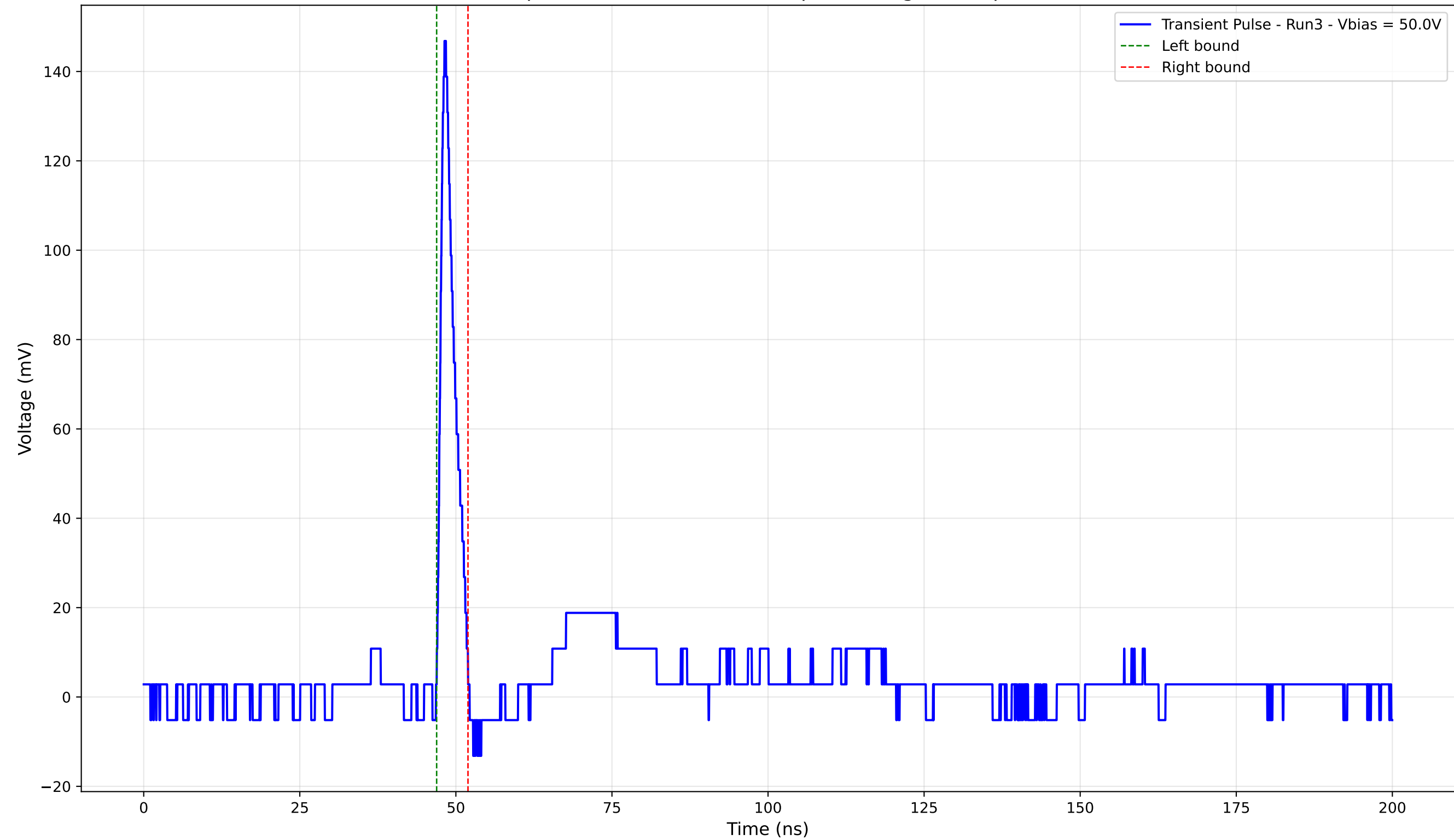
Transient Pulse - Sample: 4003 - Position: 565.0 \mu\text{m} - Charge: 7.42 pC - Rise Time: 0.99 ns
