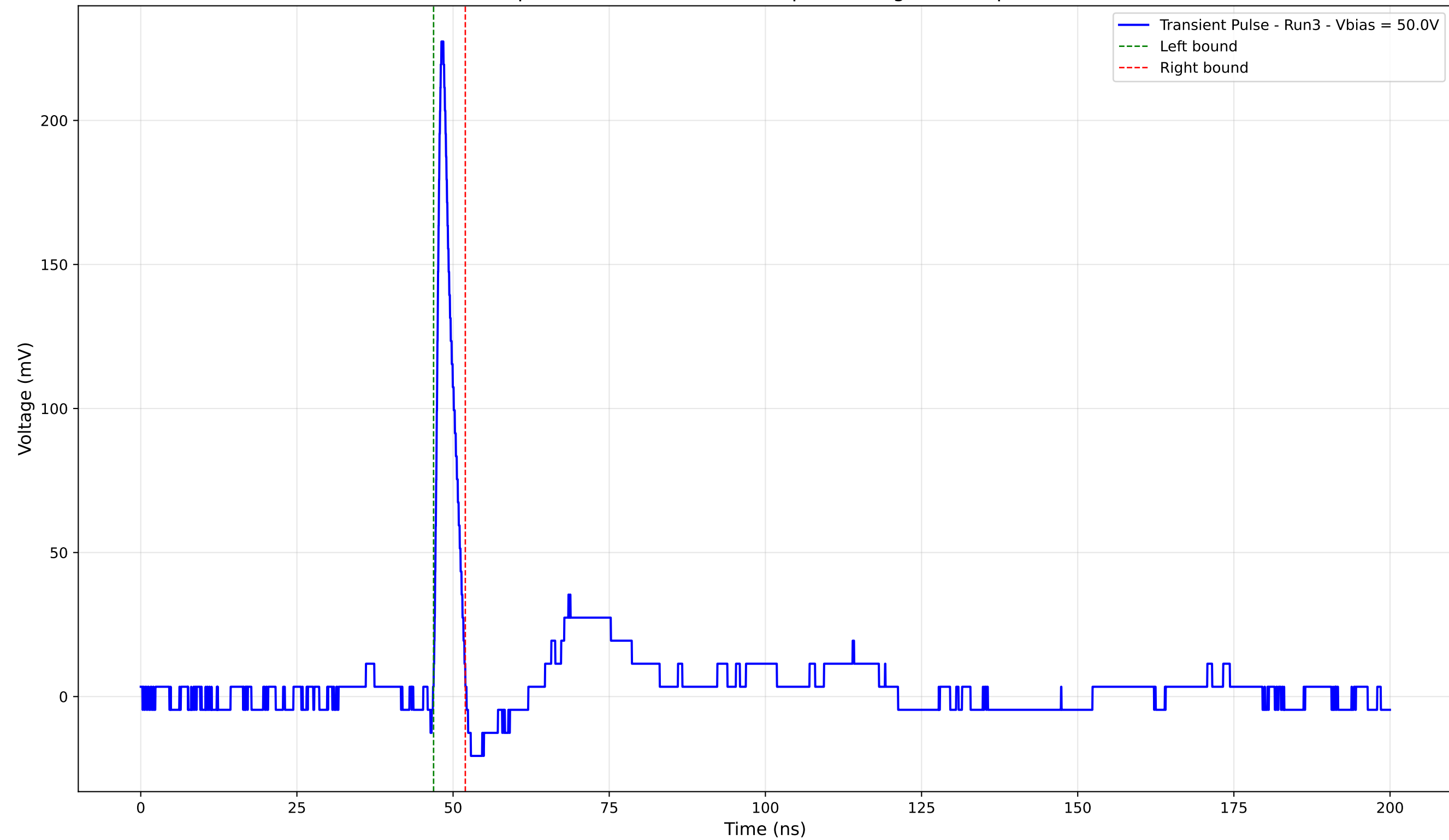
Transient Pulse - Sample: 4003 - Position: 480.0 \mu\text{m} - Charge: 11.69 pC - Rise Time: 0.93 ns
