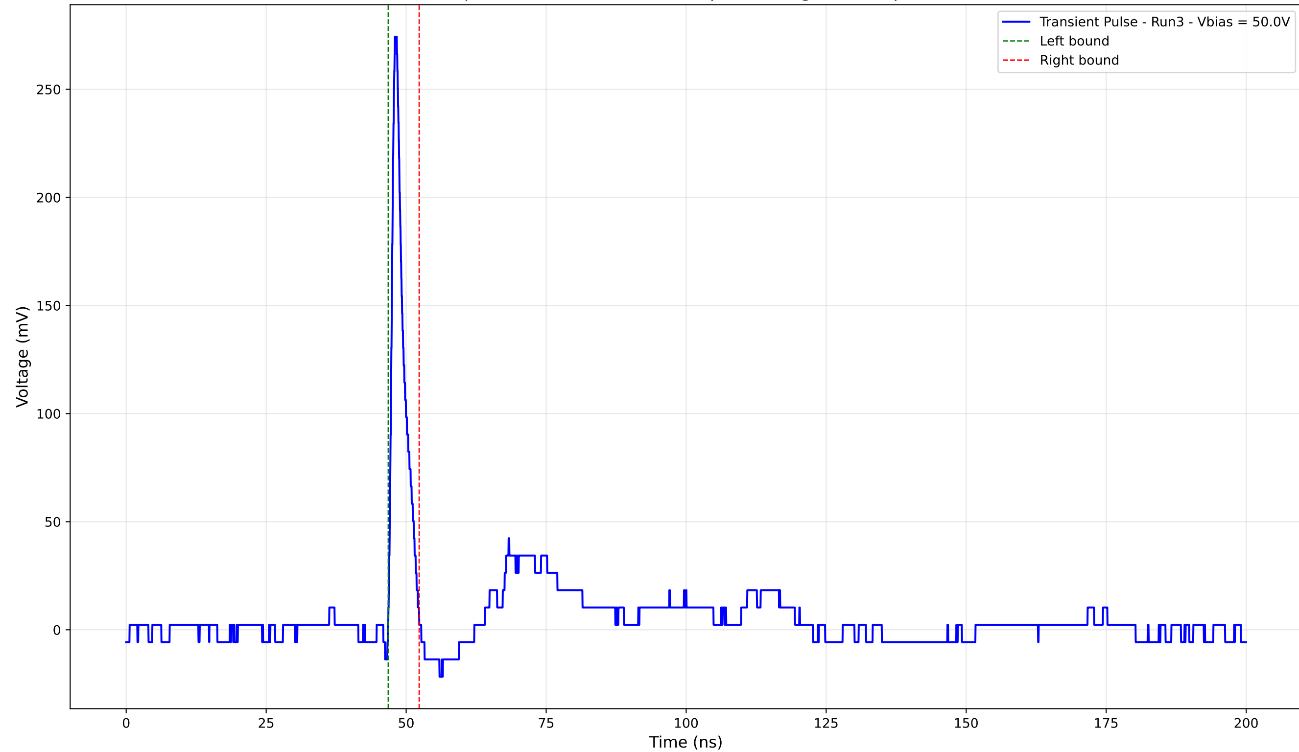
Transient Pulse - Sample: 4003 - Position: 235.0 \mu\text{m} - Charge: 13.33 pC - Rise Time: 0.86 ns
