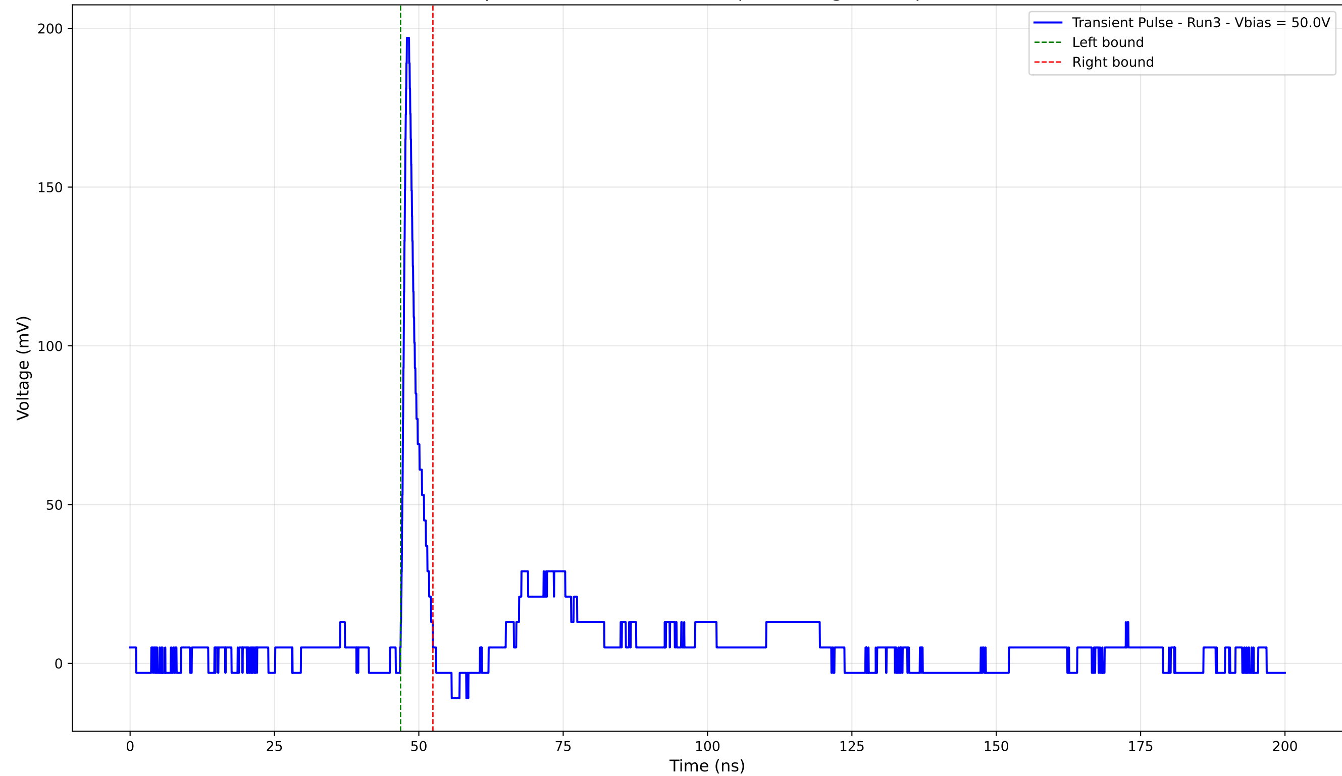
Transient Pulse - Sample: 4003 - Position: 175.0 \mu\text{m} - Charge: 9.59 pC - Rise Time: 0.84 ns
