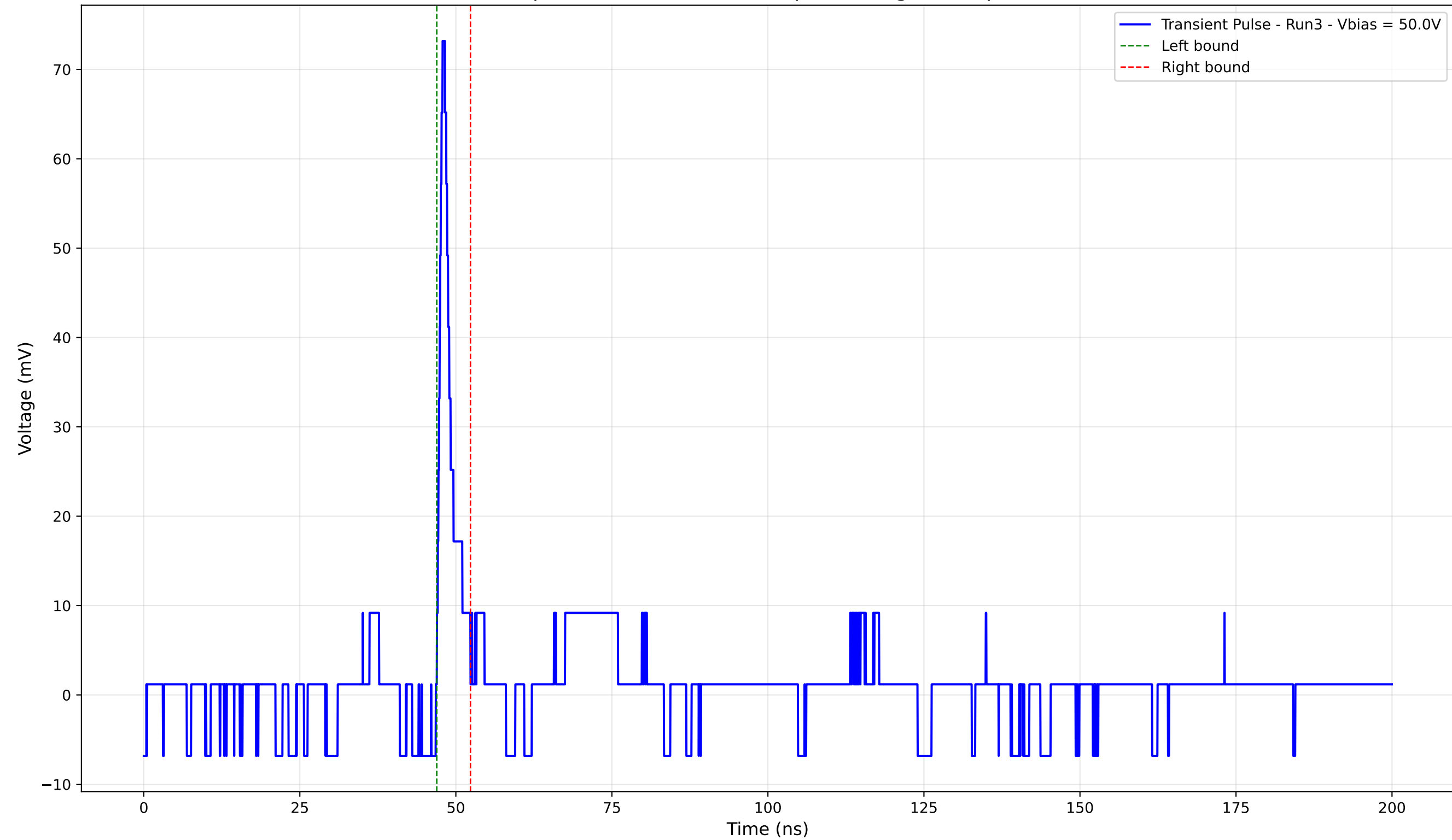
Transient Pulse - Sample: 4003 - Position: 80.0 \mu\text{m} - Charge: 3.10 pC - Rise Time: 0.90 ns
