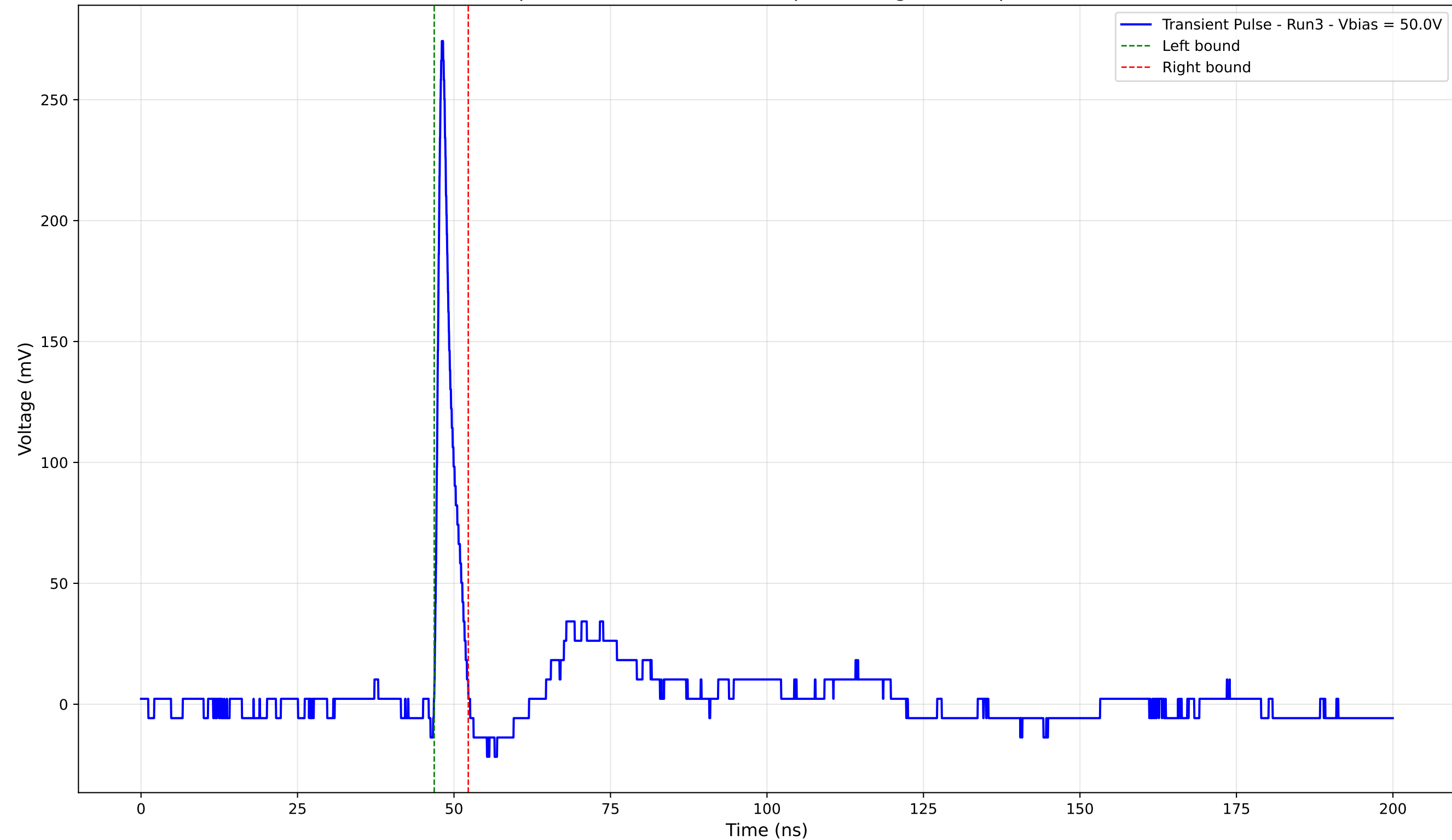
Transient Pulse - Sample: 4003 - Position: 230.0 \mu\text{m} - Charge: 13.02 pC - Rise Time: 0.86 ns
