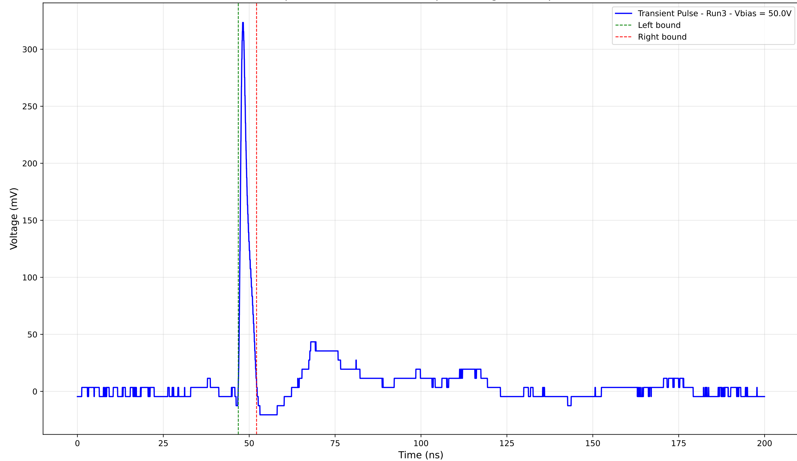
Transient Pulse - Sample: 4003 - Position: 285.0 \mu\text{m} - Charge: 15.84 pC - Rise Time: 0.85 ns
