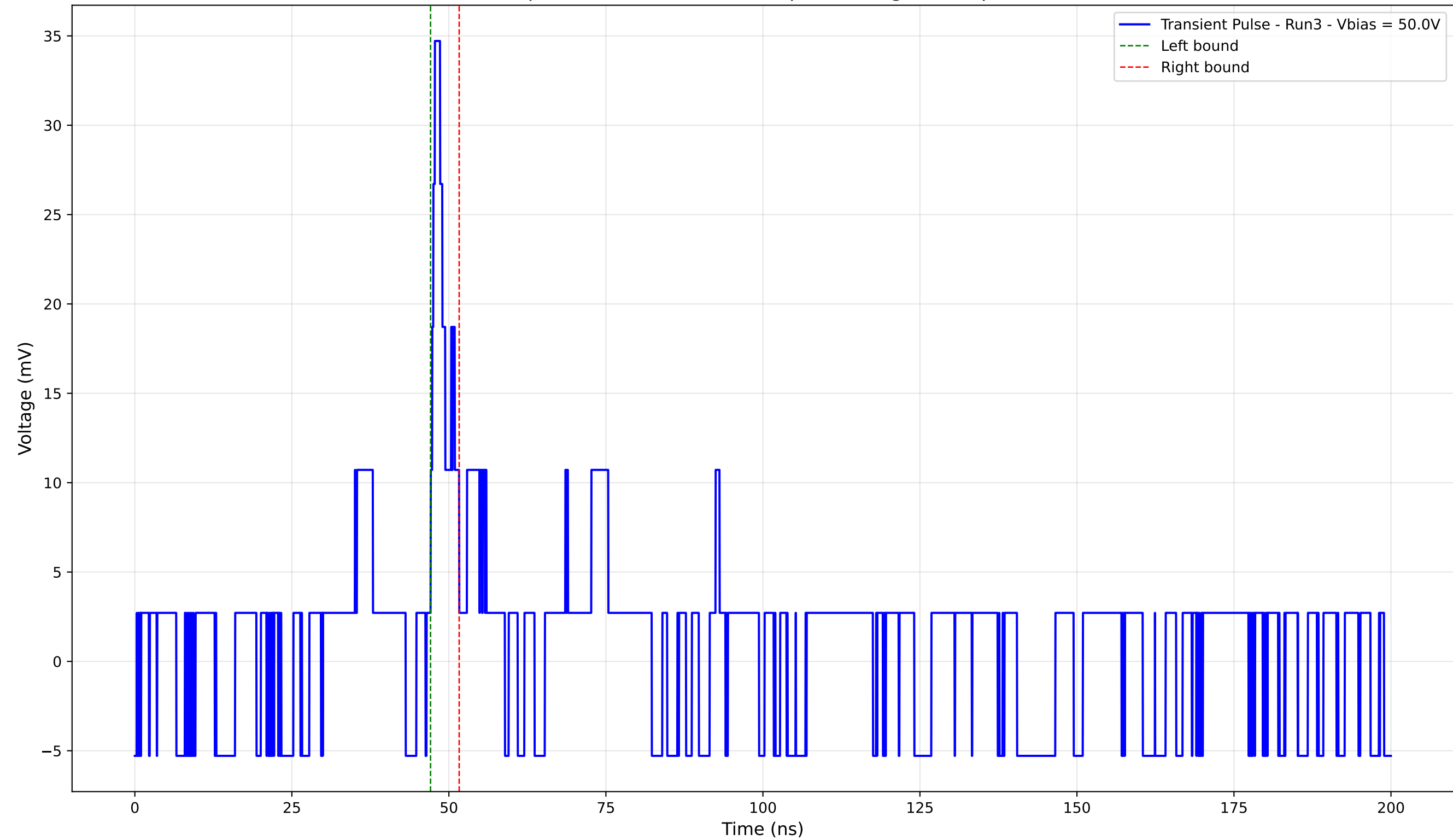
Transient Pulse - Sample: 4003 - Position: 50.0 \mu\text{m} - Charge: 1.74 pC - Rise Time: 0.68 ns
