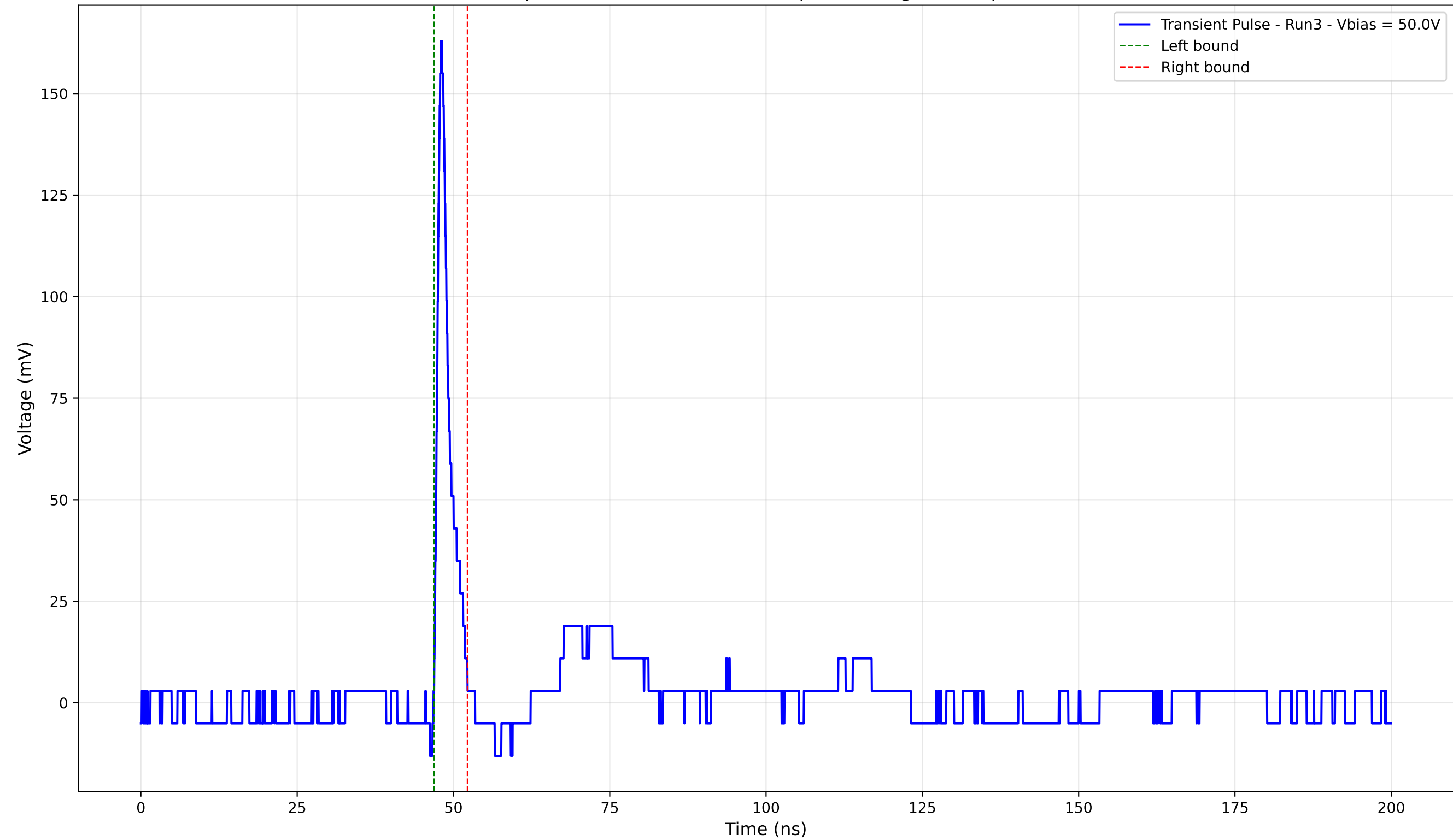
Transient Pulse - Sample: 4003 - Position: 150.0 \mu\text{m} - Charge: 7.19 pC - Rise Time: 0.81 ns
