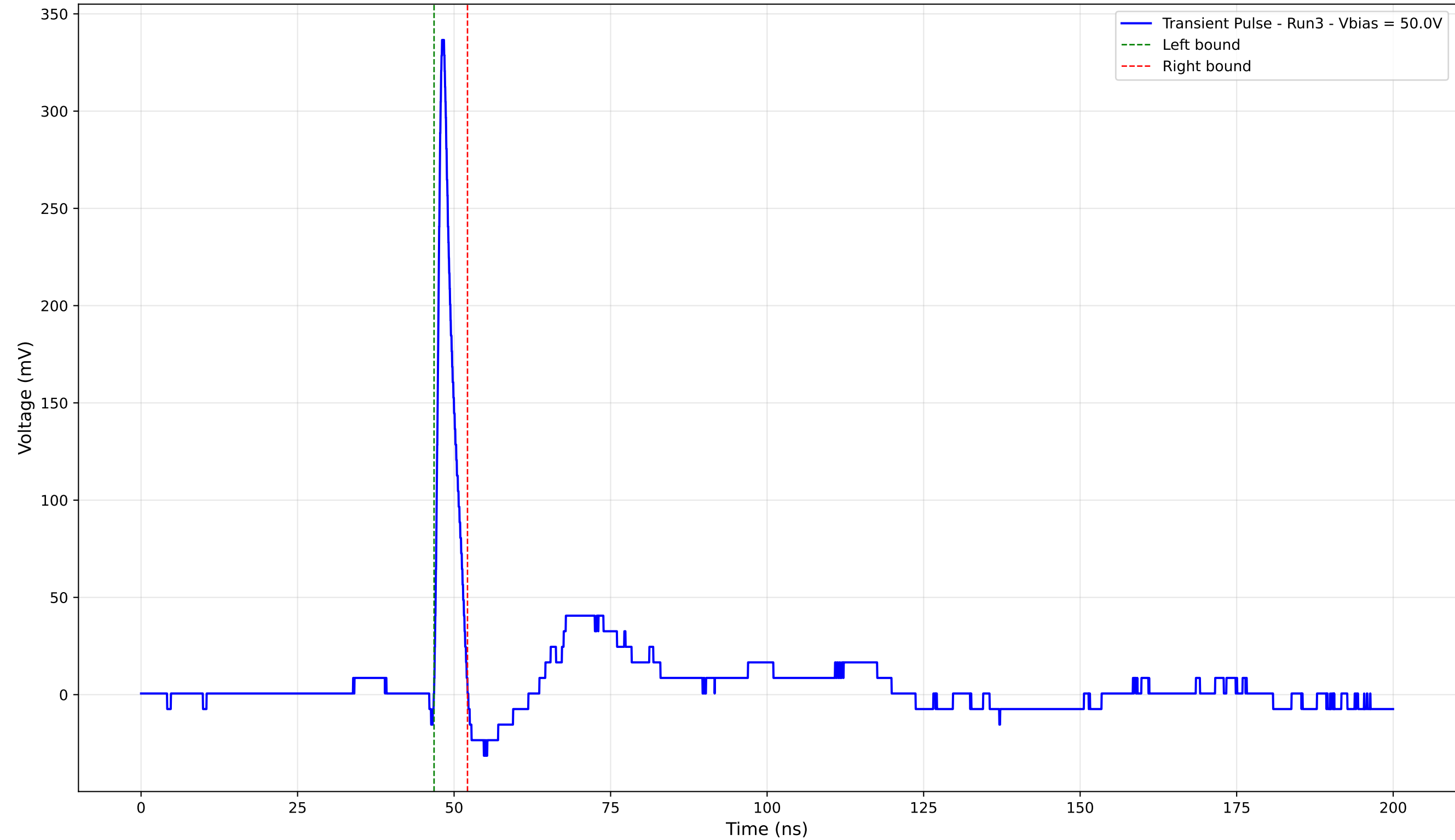
Transient Pulse - Sample: 4003 - Position: 350.0 \mu\text{m} - Charge: 17.16 pC - Rise Time: 0.88 ns
