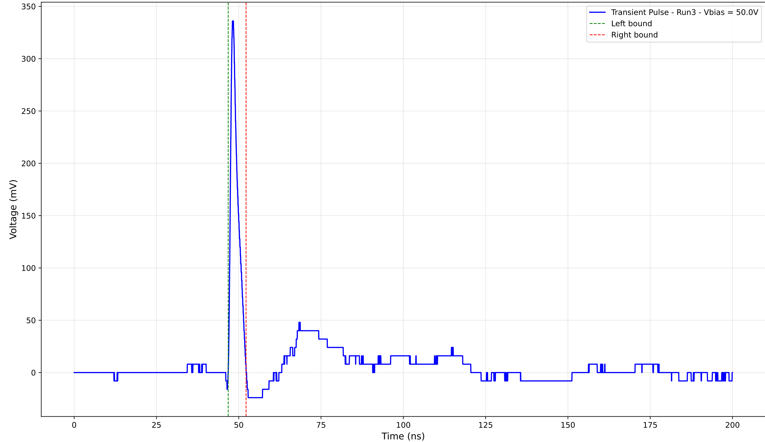
Transient Pulse - Sample: 4003 - Position: 360.0 \mu\text{m} - Charge: 17.06 pC - Rise Time: 0.86 ns
