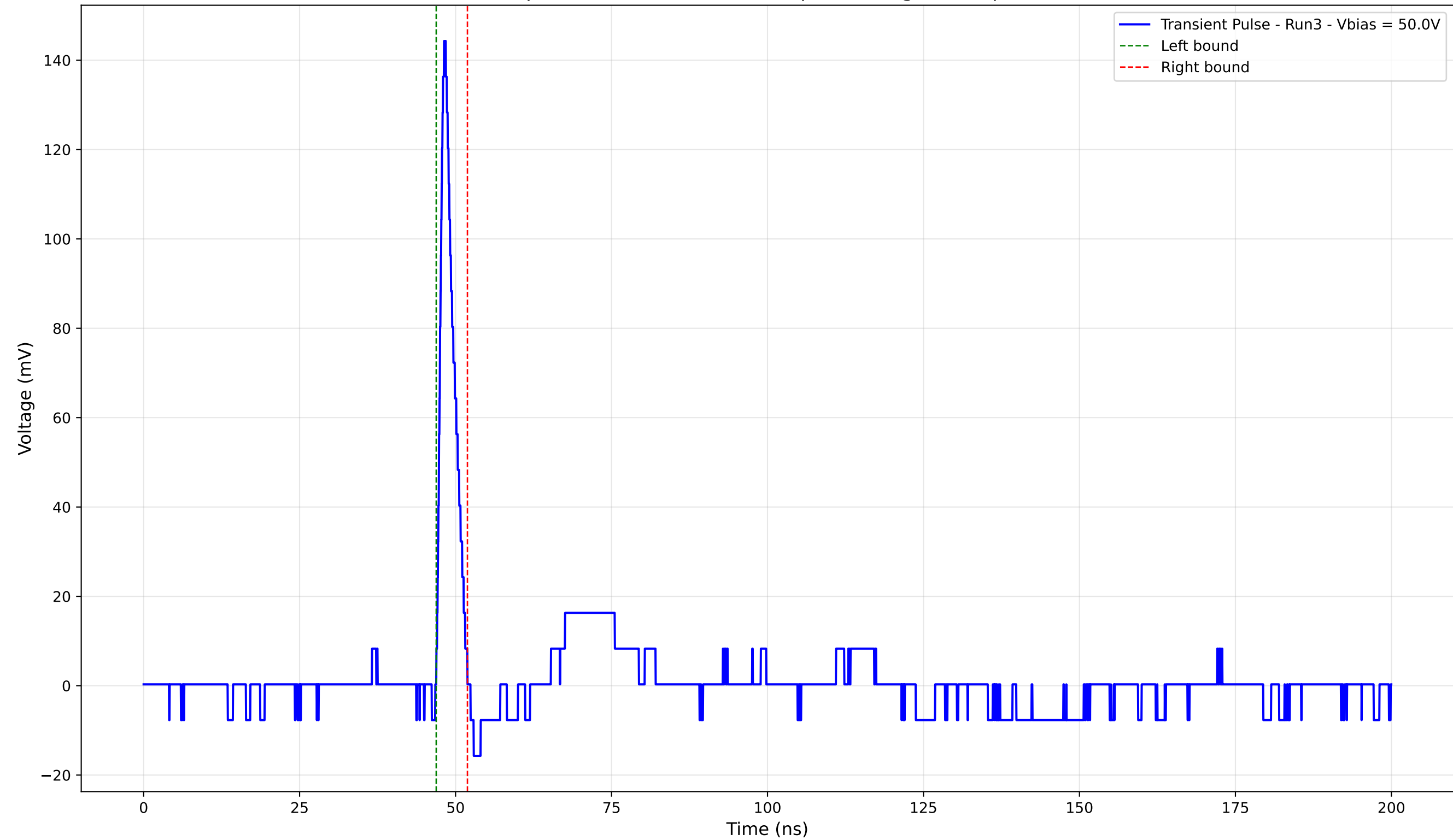
Transient Pulse - Sample: 4003 - Position: 600.0 \mu\text{m} - Charge: 6.99 pC - Rise Time: 0.94 ns
