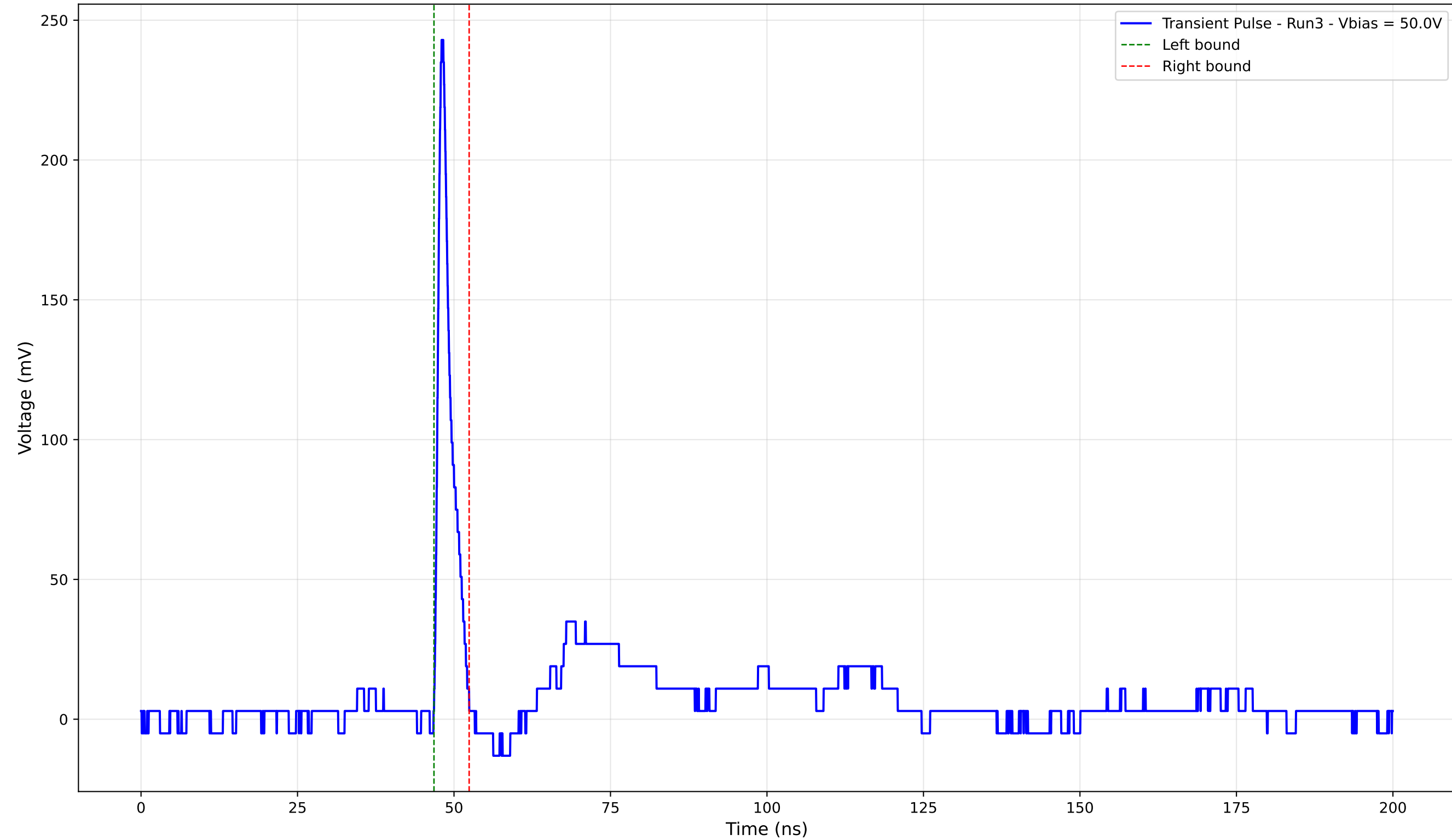
Transient Pulse - Sample: 4003 - Position: 205.0 \mu\text{m} - Charge: 11.71 pC - Rise Time: 0.85 ns
