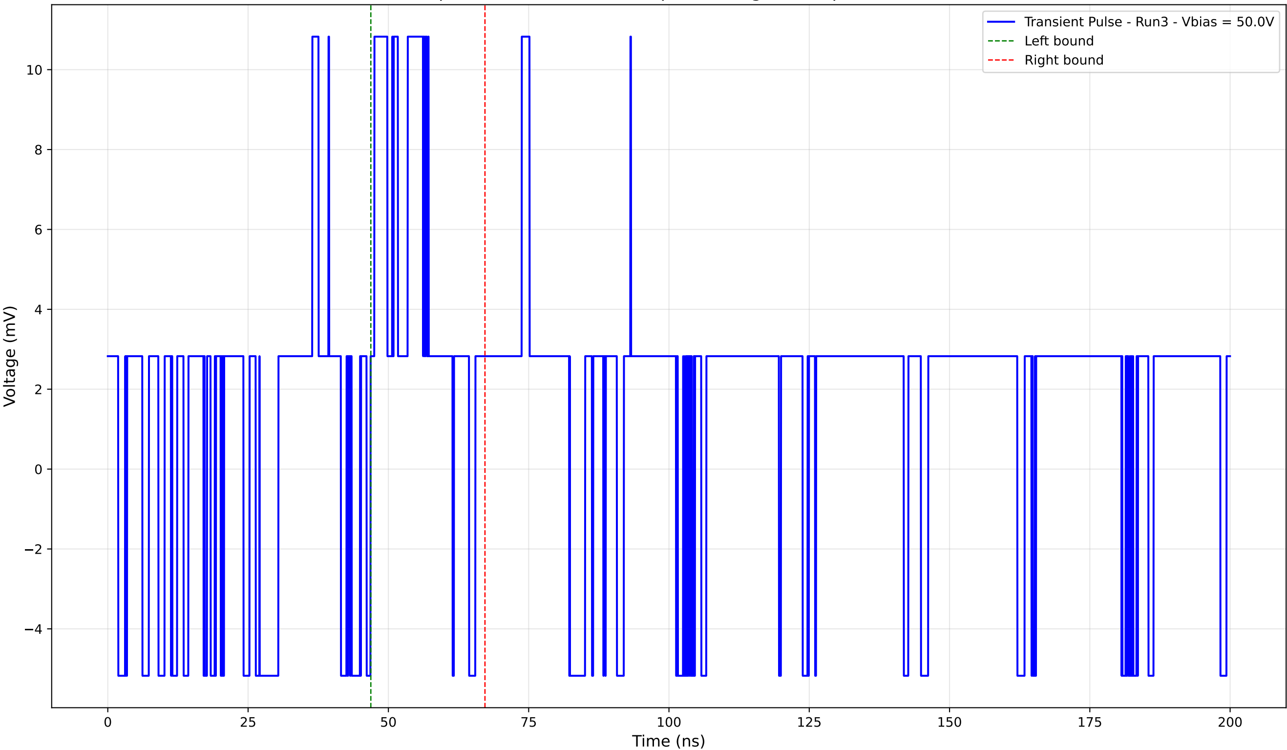
Transient Pulse - Sample: 4003 - Position: 5.0 \mu\text{m} - Charge: 1.96 pC - Rise Time: 0.00 ns (N/A)
