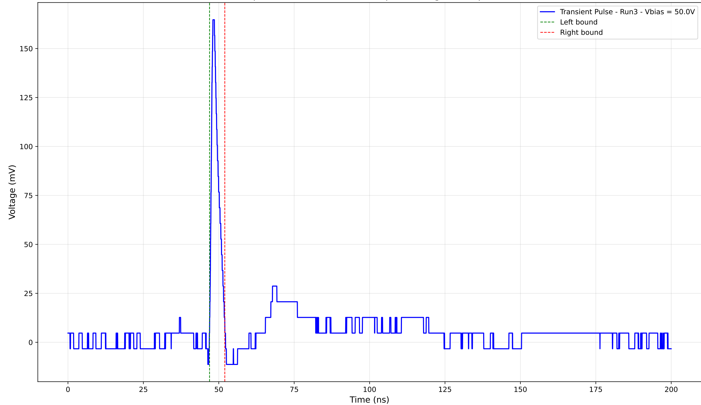
Transient Pulse - Sample: 4003 - Position: 575.0 \mu\text{m} - Charge: 8.68 pC - Rise Time: 0.85 ns
