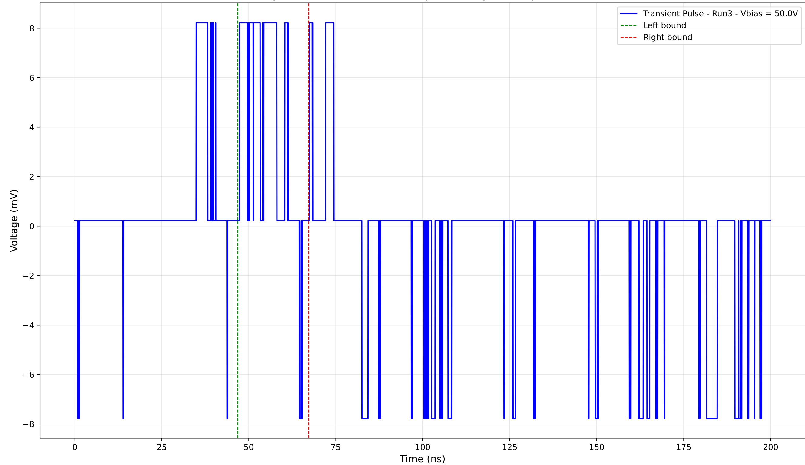
Transient Pulse - Sample: 4003 - Position: 630.0 \mu\text{m} - Charge: 1.58 pC - Rise Time: 0.00 ns (N/A)
