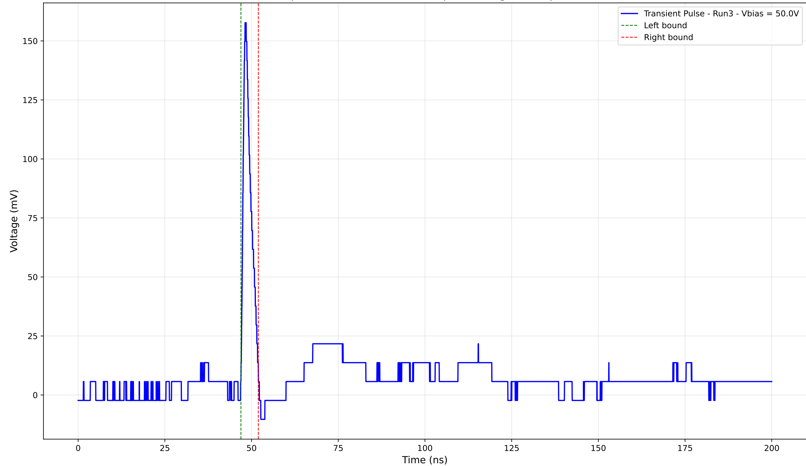
Transient Pulse - Sample: 4003 - Position: 570.0 \mu\text{m} - Charge: 8.23 pC - Rise Time: 0.95 ns
