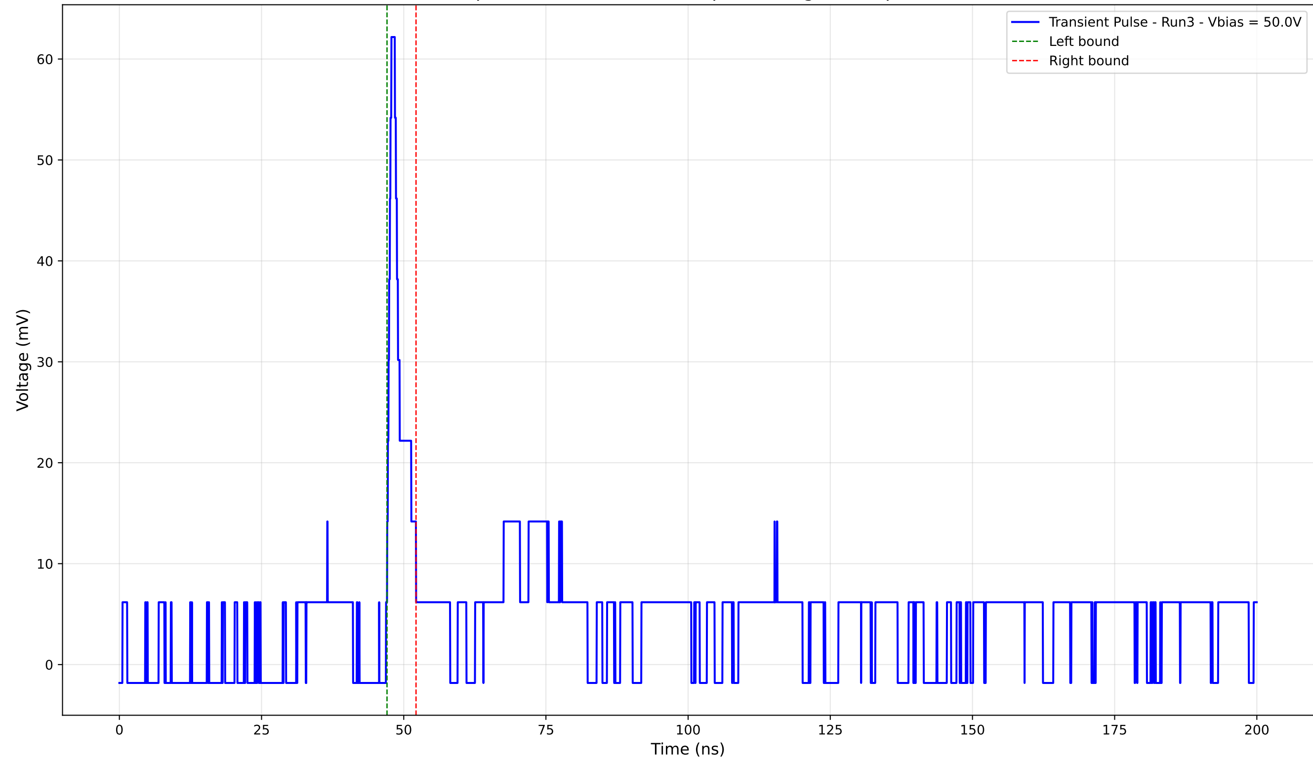
Transient Pulse - Sample: 4003 - Position: 70.0 \mu\text{m} - Charge: 3.12 pC - Rise Time: 0.76 ns
