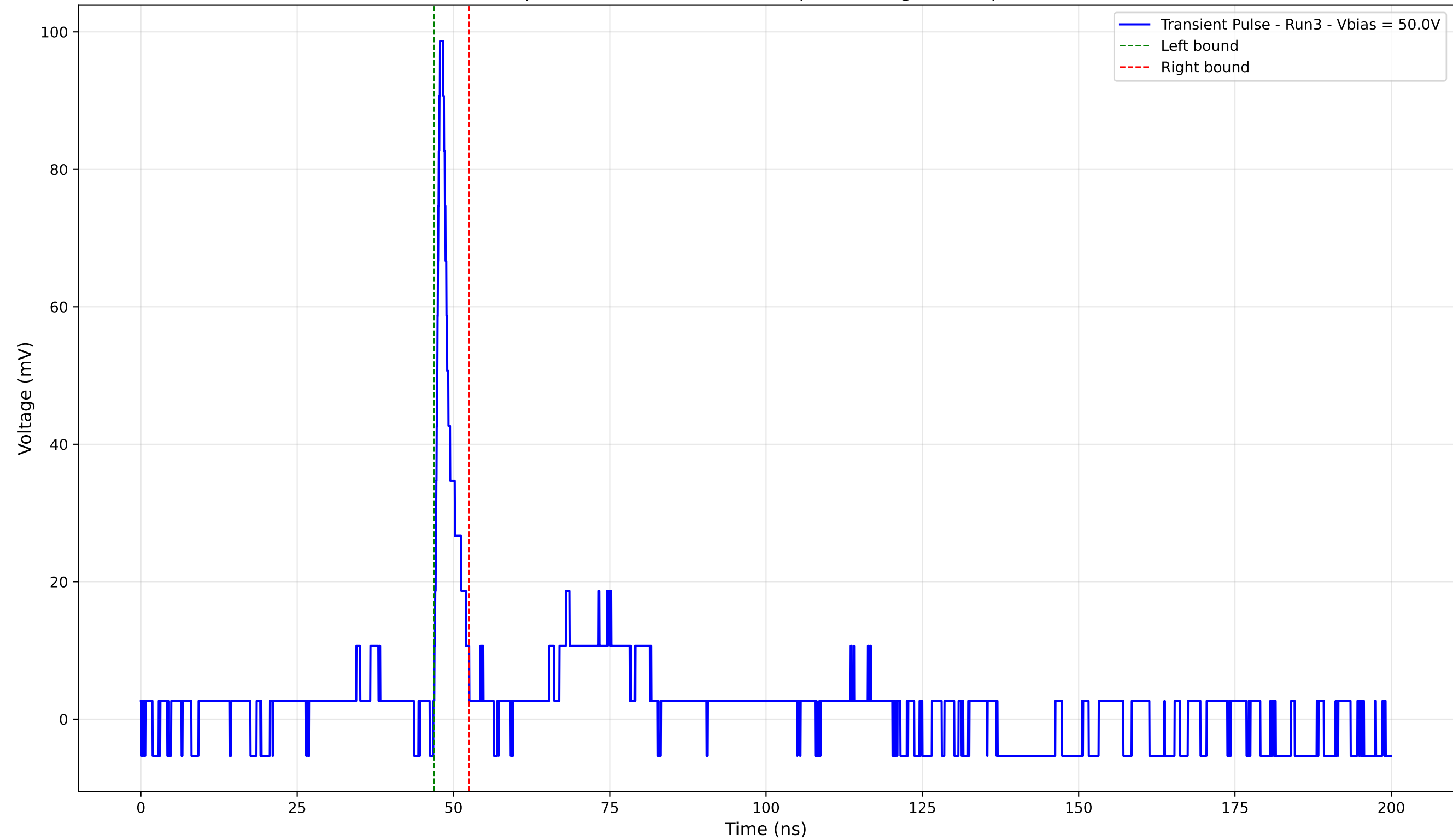
Transient Pulse - Sample: 4003 - Position: 105.0 \mu\text{m} - Charge: 4.76 pC - Rise Time: 0.80 ns
