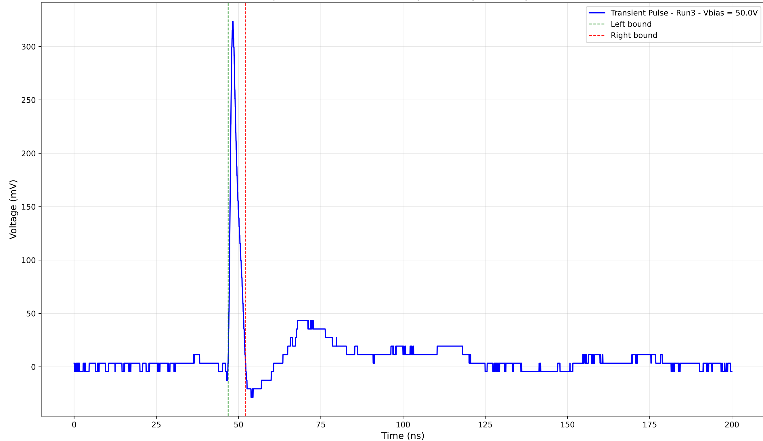
Transient Pulse - Sample: 4003 - Position: 390.0 \mu\text{m} - Charge: 16.39 pC - Rise Time: 0.91 ns
