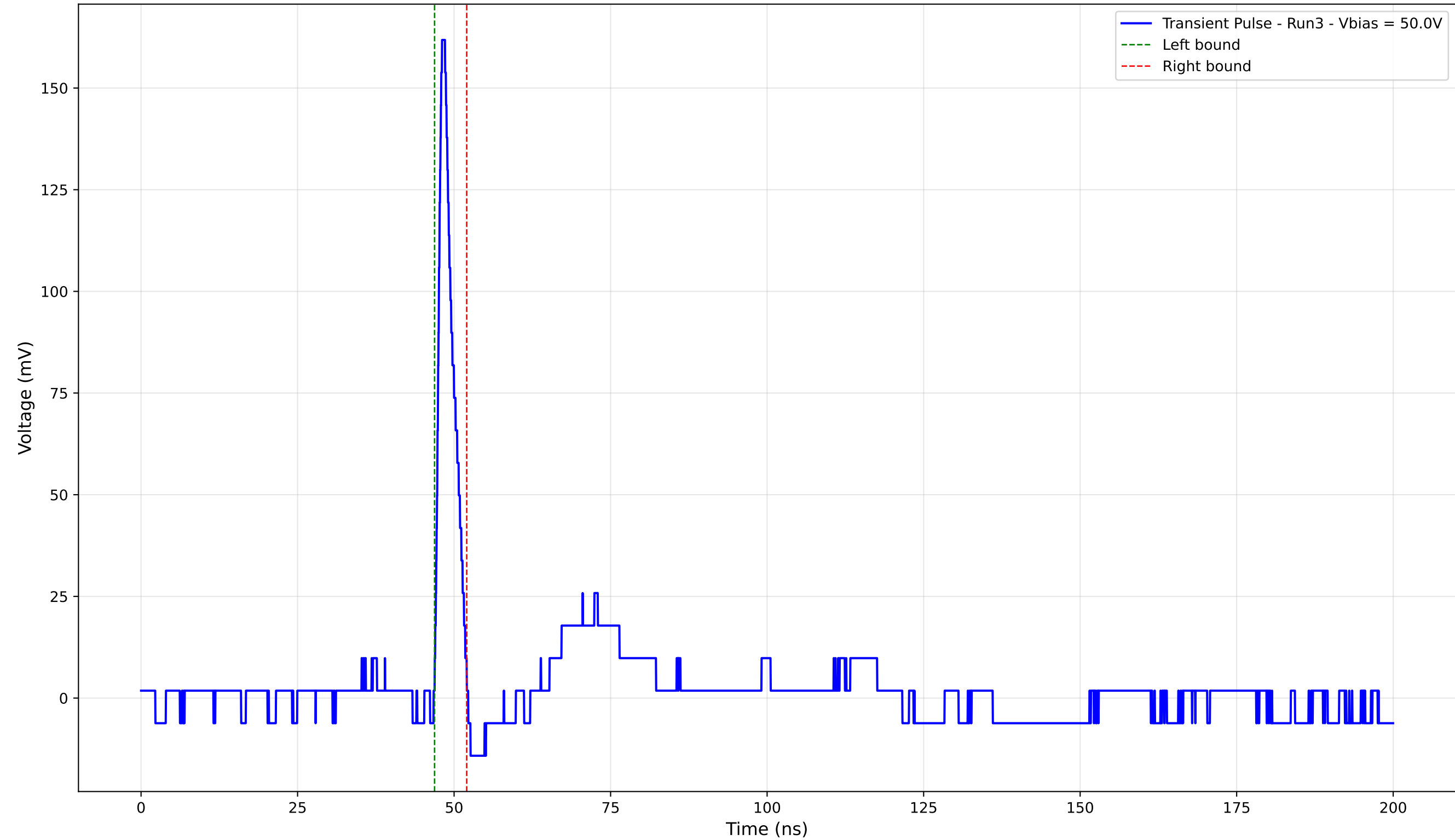
Transient Pulse - Sample: 4003 - Position: 540.0 \mu\text{m} - Charge: 8.47 pC - Rise Time: 0.90 ns
