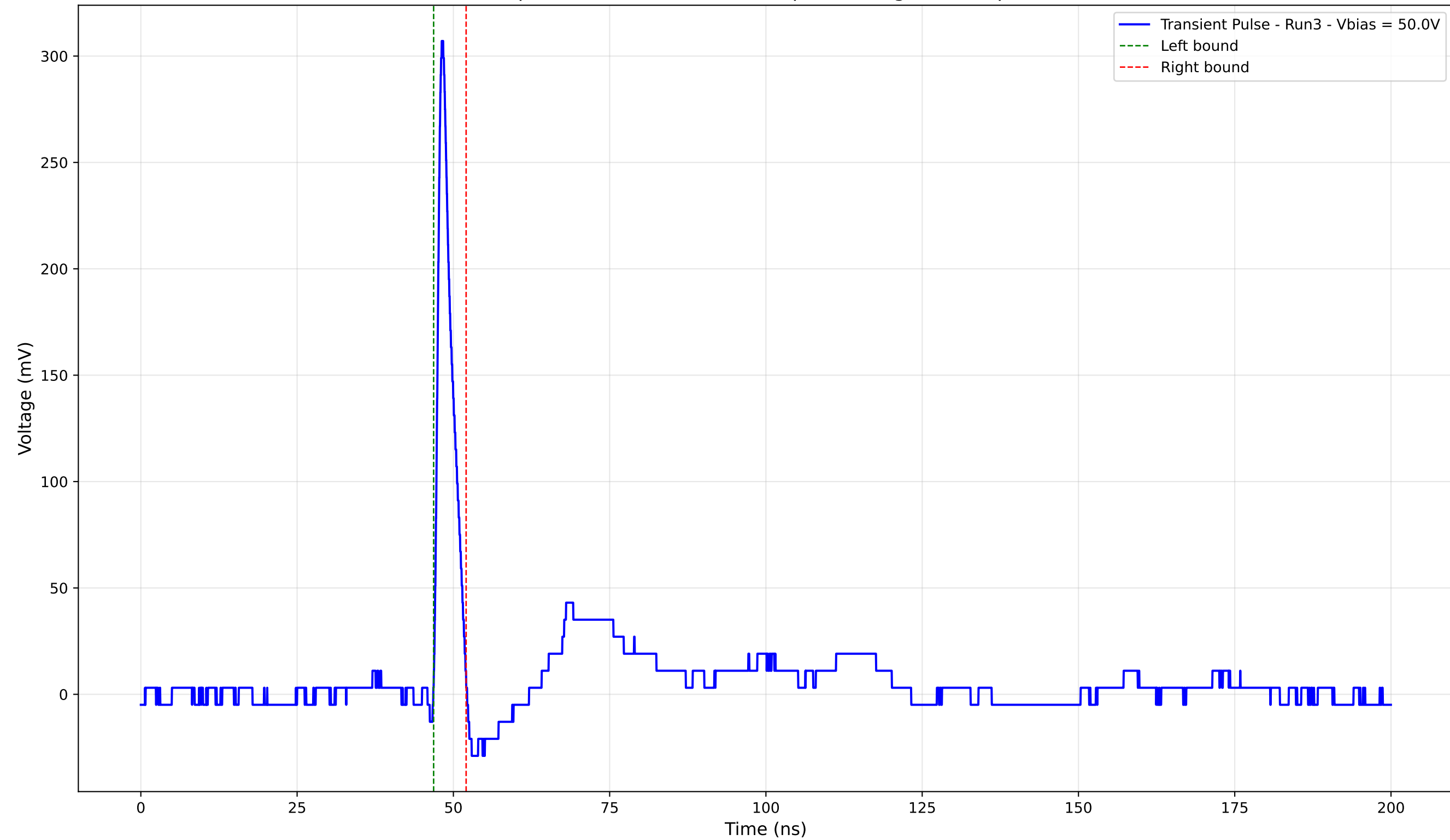
Transient Pulse - Sample: 4003 - Position: 410.0 \mu\text{m} - Charge: 15.59 pC - Rise Time: 0.91 ns
