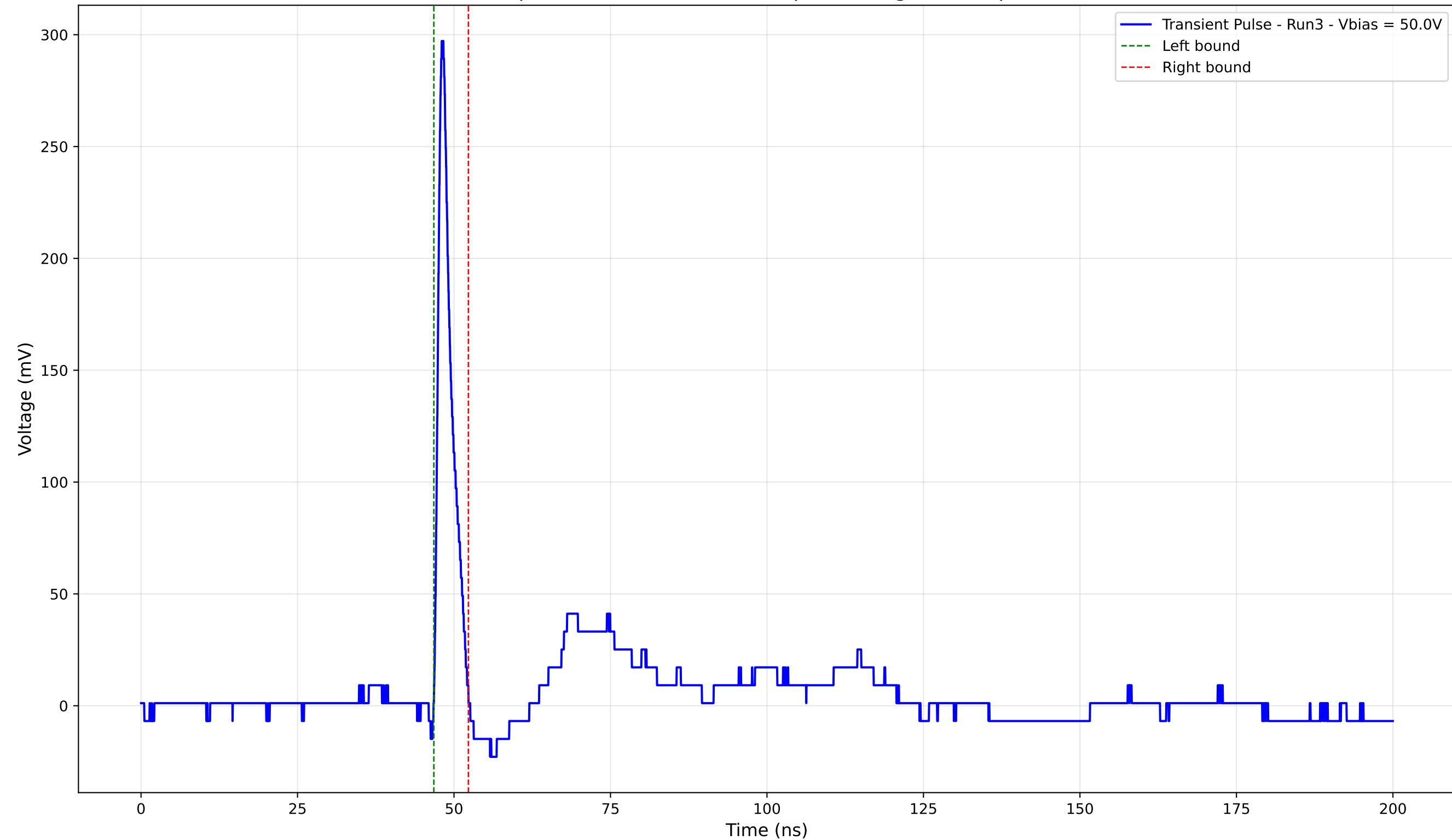
Transient Pulse - Sample: 4003 - Position: 260.0 \mu\text{m} - Charge: 14.61 pC - Rise Time: 0.89 ns
