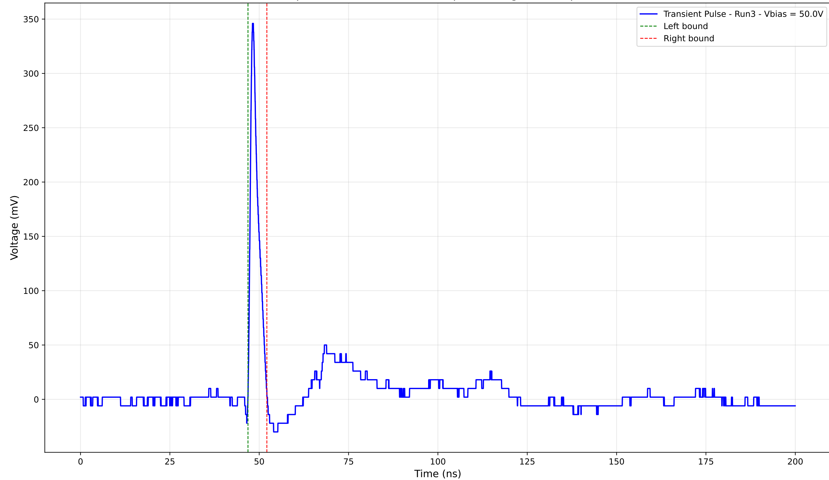
Transient Pulse - Sample: 4003 - Position: 340.0 \mu\text{m} - Charge: 17.31 pC - Rise Time: 0.86 ns
