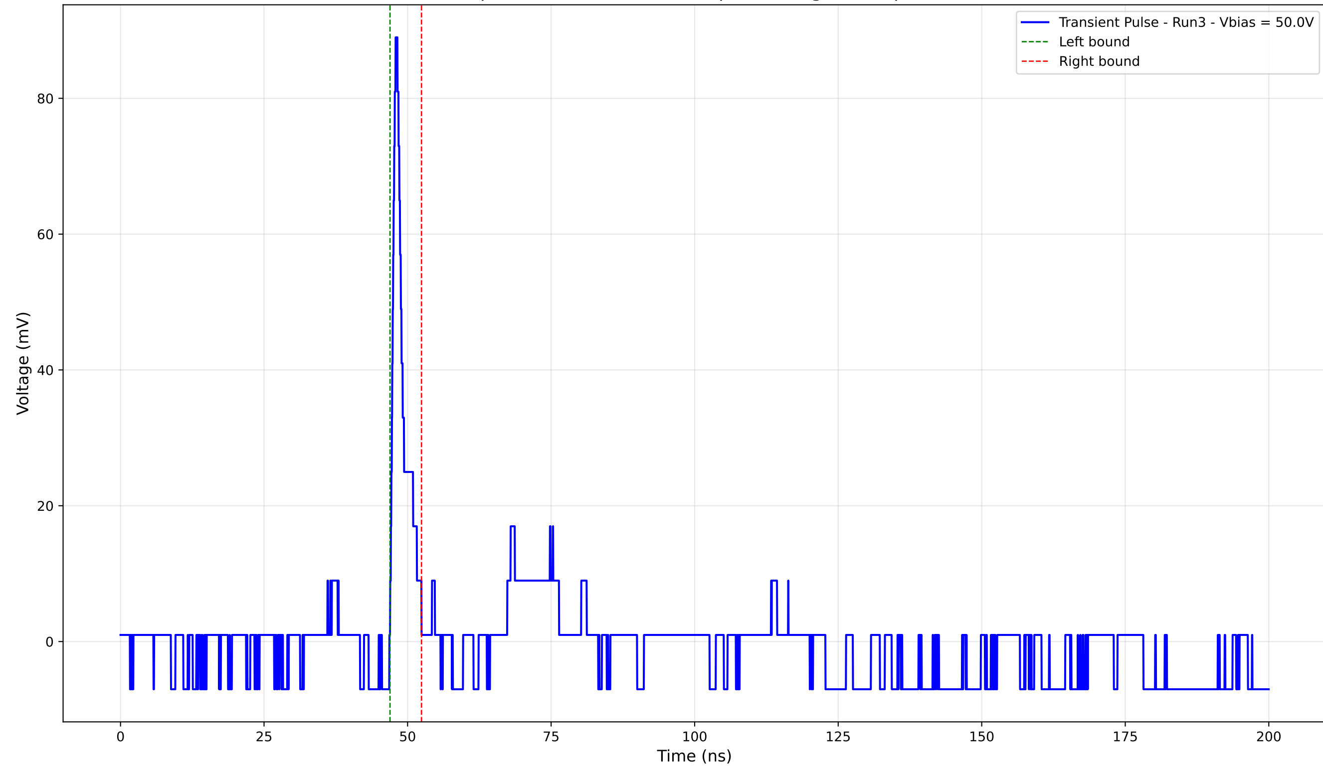
Transient Pulse - Sample: 4003 - Position: 95.0 \mu\text{m} - Charge: 3.89 pC - Rise Time: 0.80 ns
