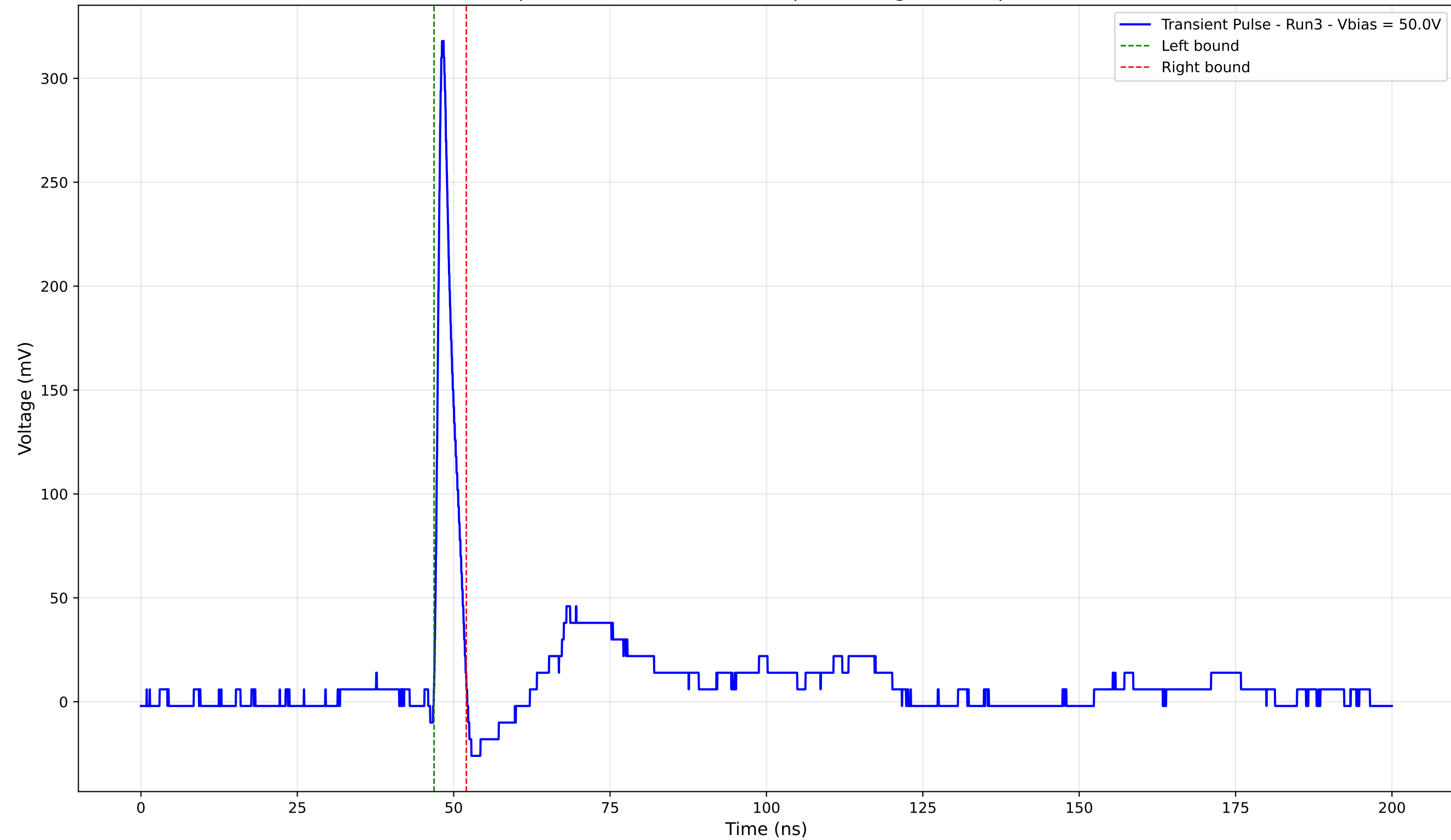
Transient Pulse - Sample: 4003 - Position: 395.0 \mu\text{m} - Charge: 16.19 pC - Rise Time: 0.92 ns
