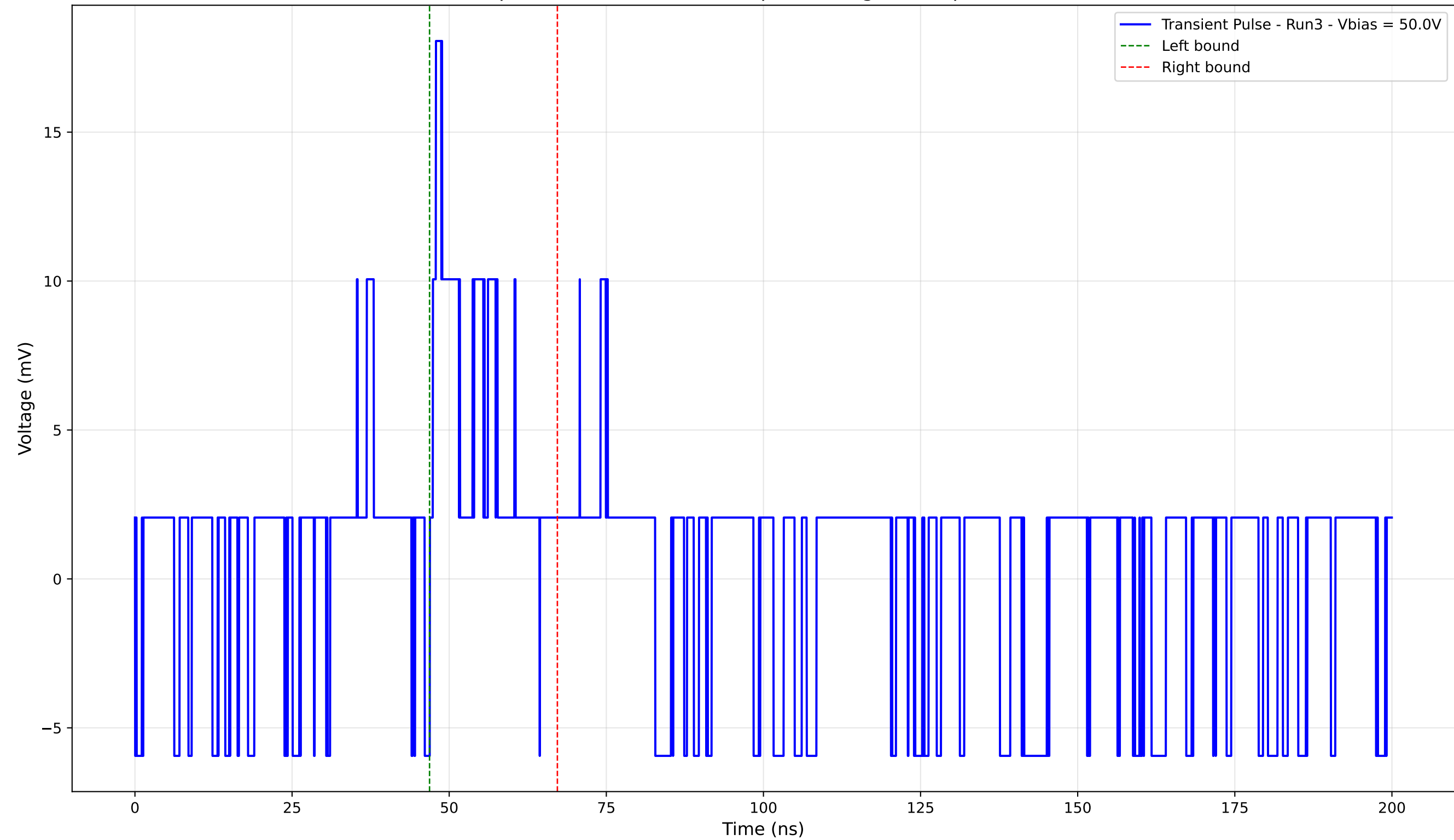
Transient Pulse - Sample: 4003 - Position: 20.0 \mu\text{m} - Charge: 2.21 pC - Rise Time: 0.00 ns (N/A)
