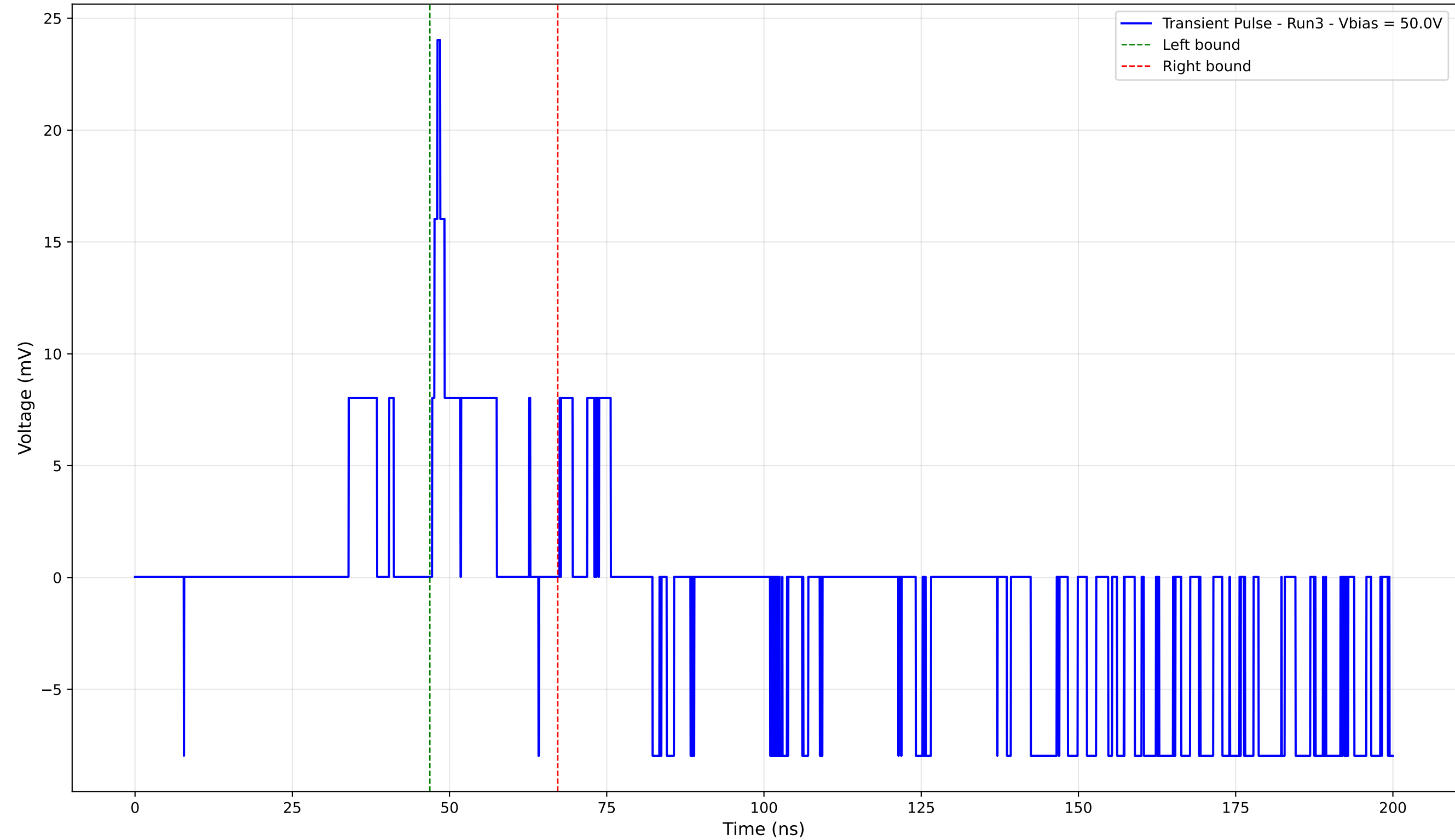
Transient Pulse - Sample: 4003 - Position: 25.0 \mu\text{m} - Charge: 1.98 pC - Rise Time: 0.85 ns
