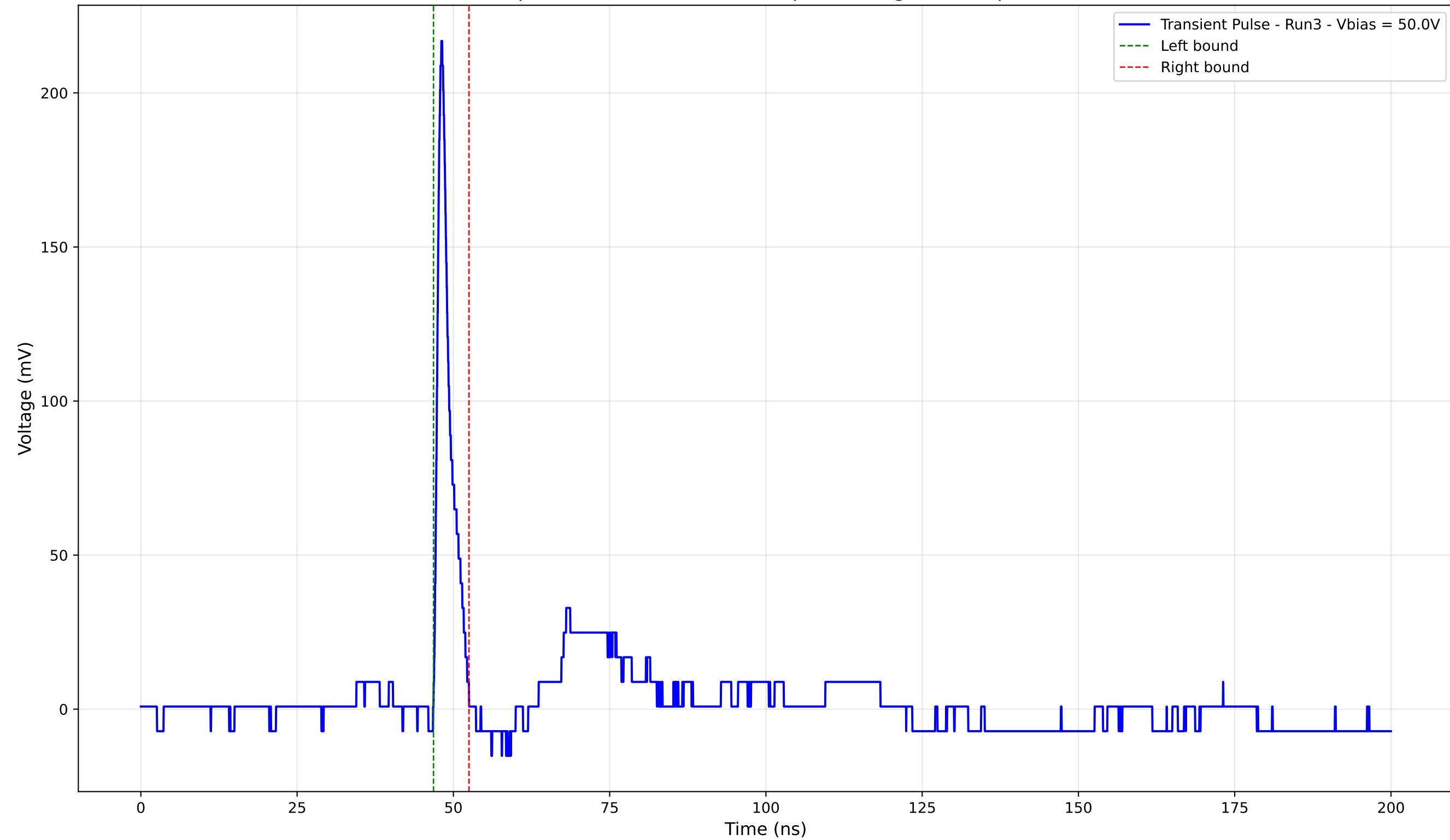
Transient Pulse - Sample: 4003 - Position: 185.0 \mu\text{m} - Charge: 10.13 pC - Rise Time: 0.89 ns
