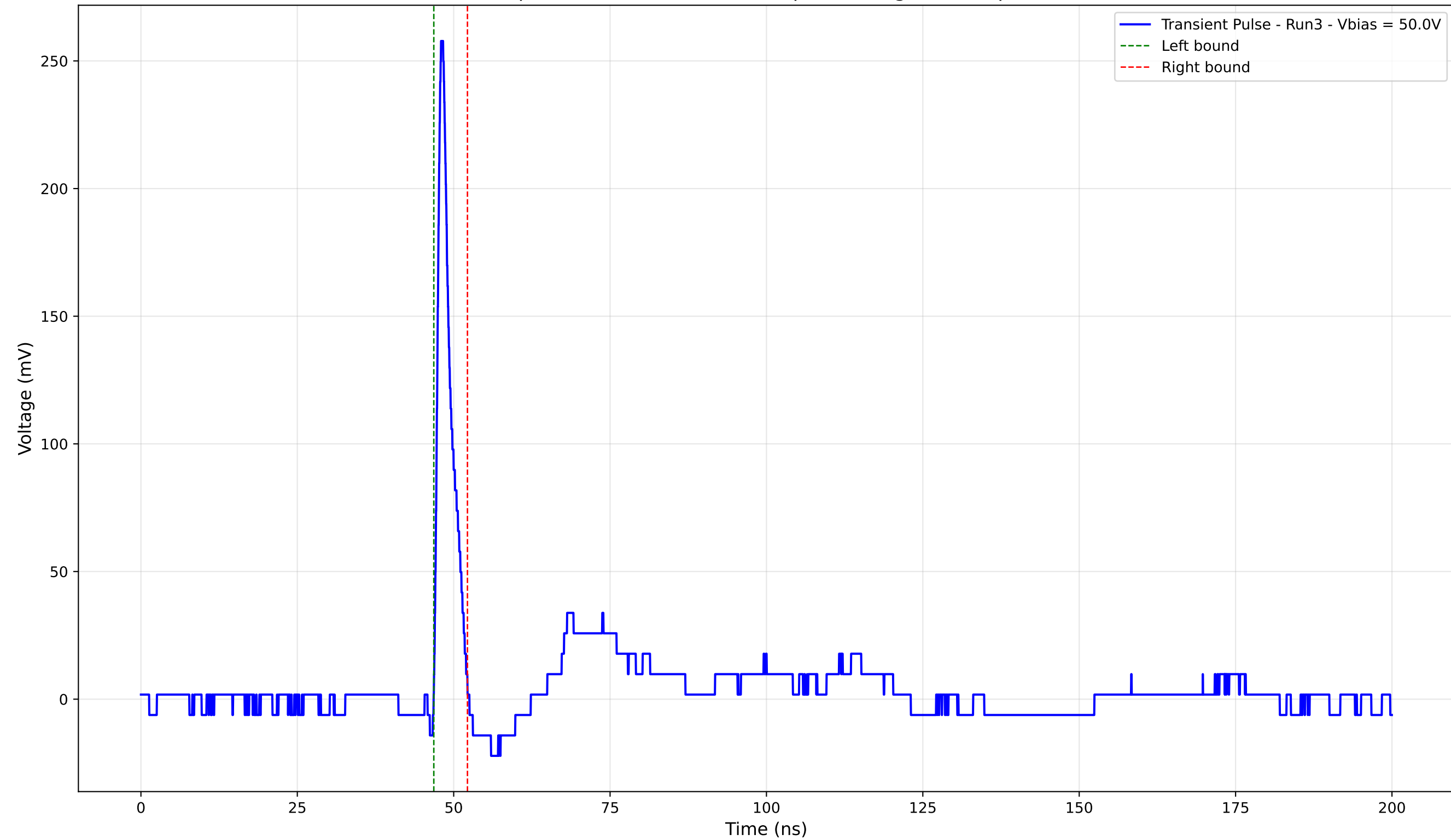
Transient Pulse - Sample: 4003 - Position: 225.0 \mu\text{m} - Charge: 12.33 pC - Rise Time: 0.84 ns
