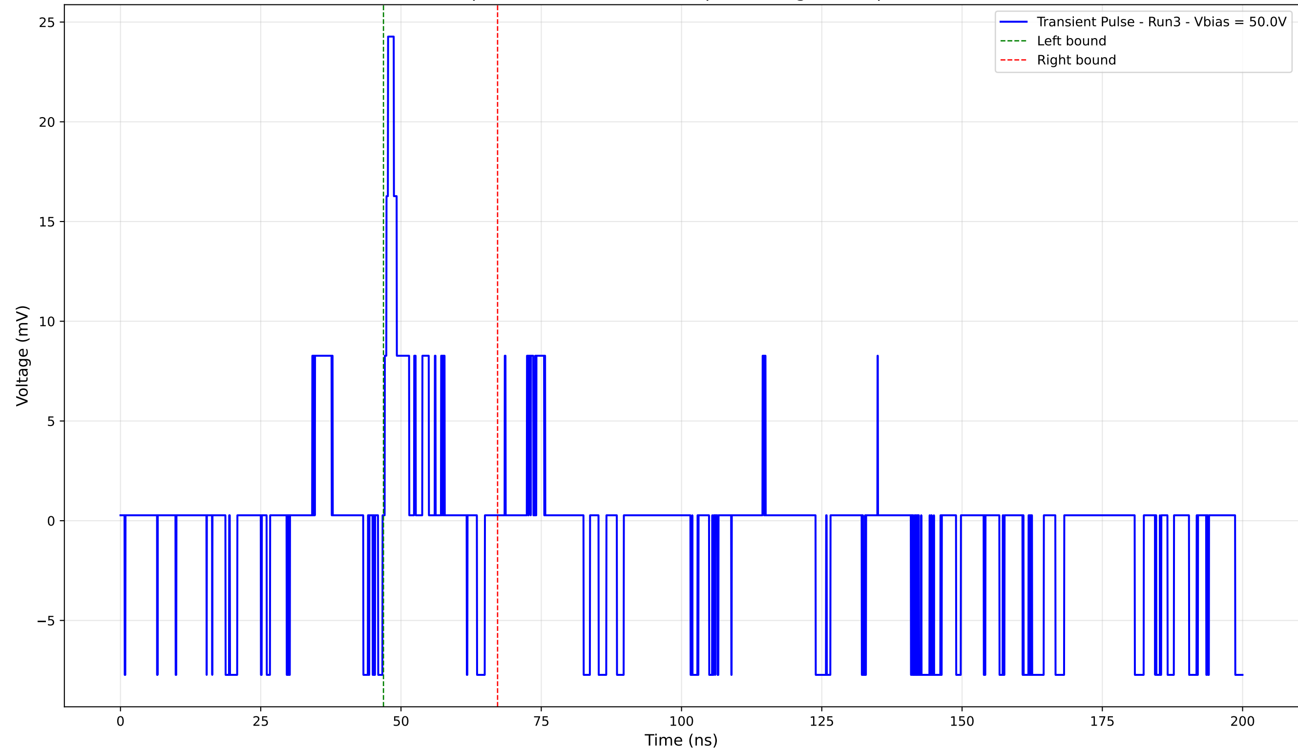
Transient Pulse - Sample: 4003 - Position: 40.0 \mu\text{m} - Charge: 1.35 pC - Rise Time: 0.59 ns
