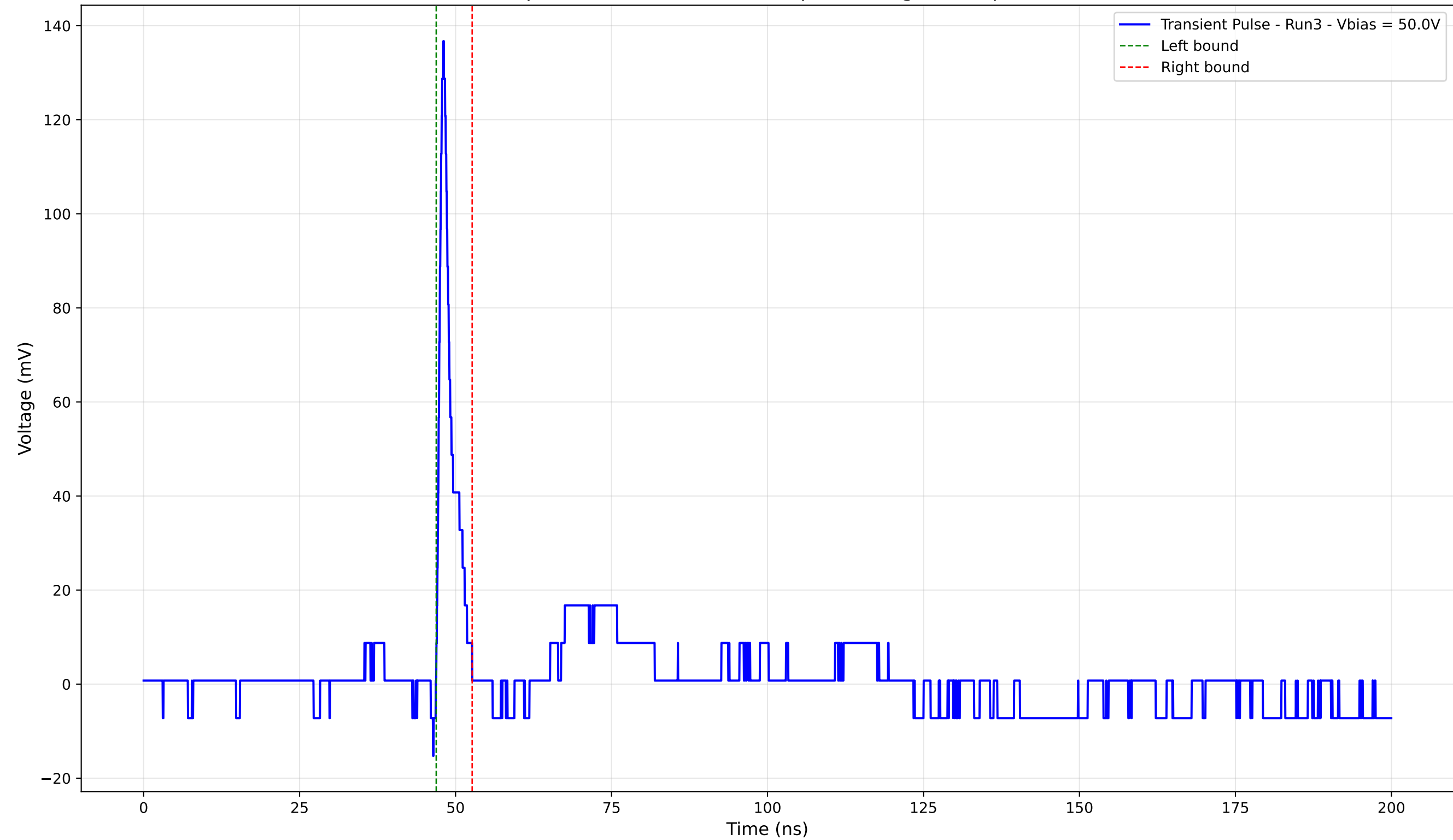
Transient Pulse - Sample: 4003 - Position: 130.0 \mu\text{m} - Charge: 6.01 pC - Rise Time: 0.85 ns
