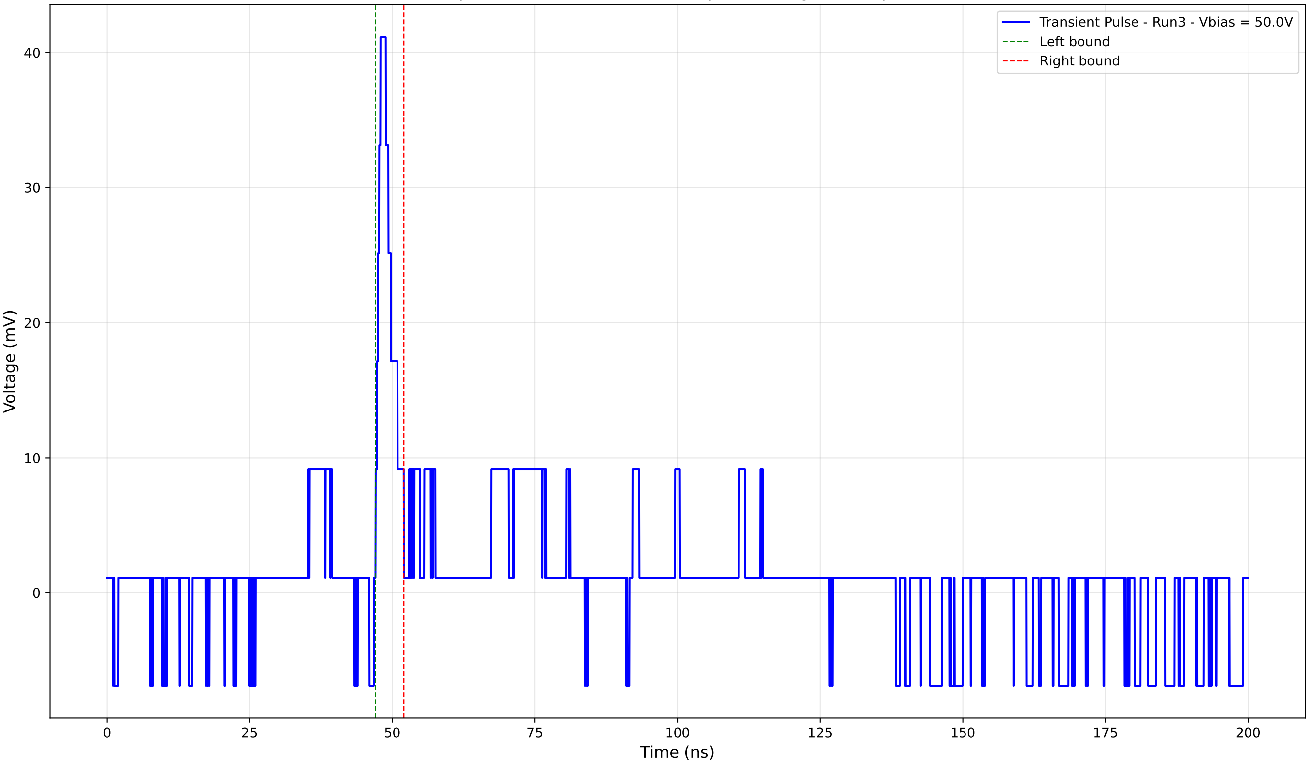
Transient Pulse - Sample: 4003 - Position: 615.0 \mu\text{m} - Charge: 2.25 pC - Rise Time: 0.87 ns
