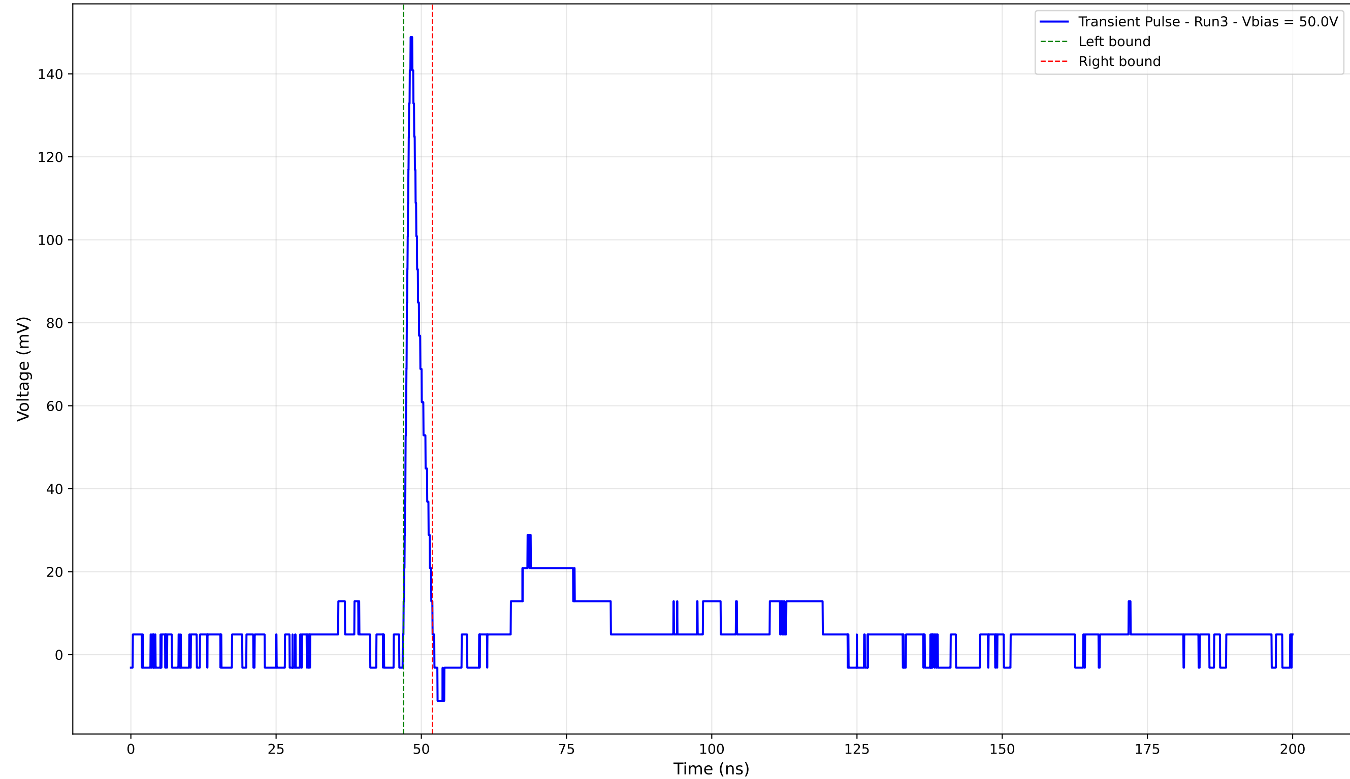
Transient Pulse - Sample: 4003 - Position: 560.0 \mu\text{m} - Charge: 7.57 pC - Rise Time: 0.97 ns
