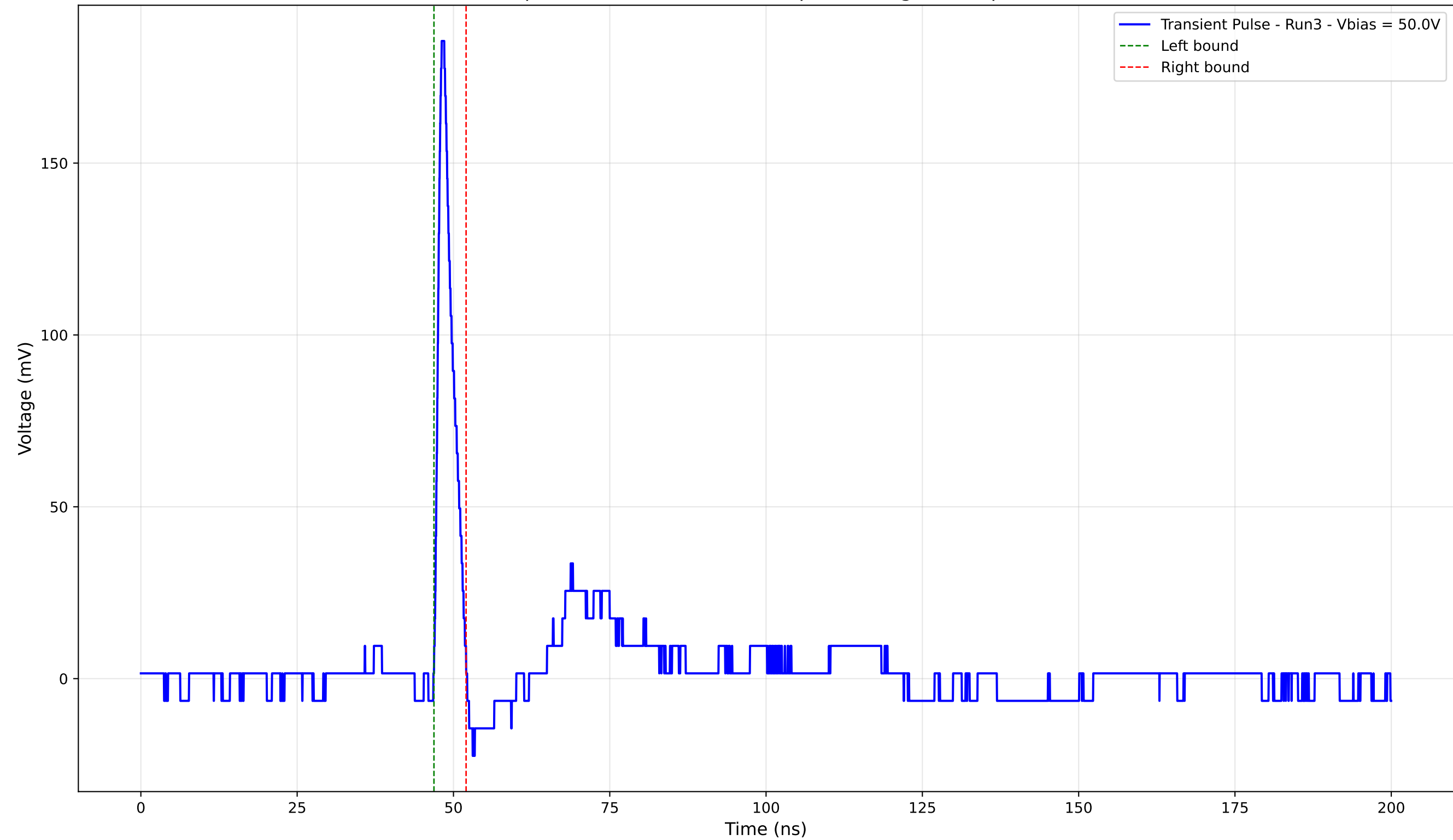
Transient Pulse - Sample: 4003 - Position: 510.0 \mu\text{m} - Charge: 9.64 pC - Rise Time: 0.86 ns
