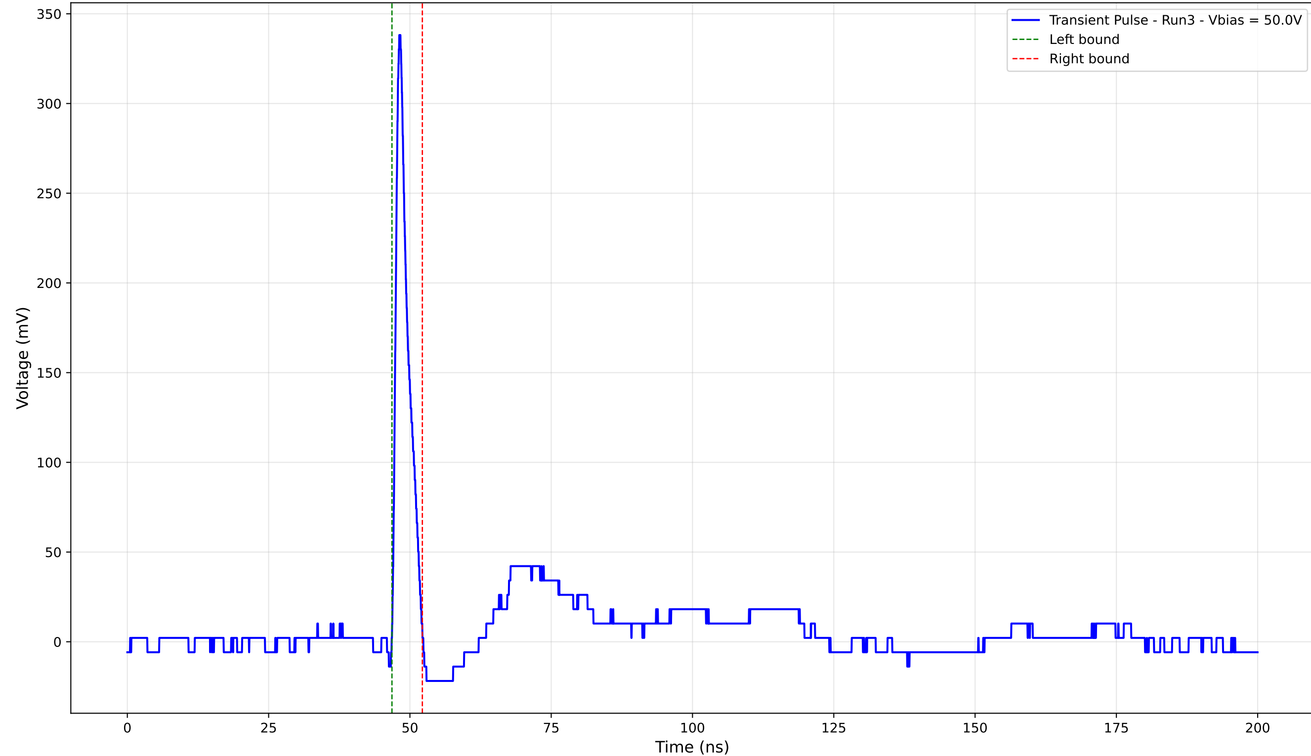
Transient Pulse - Sample: 4003 - Position: 315.0 \mu\text{m} - Charge: 16.91 pC - Rise Time: 0.90 ns
