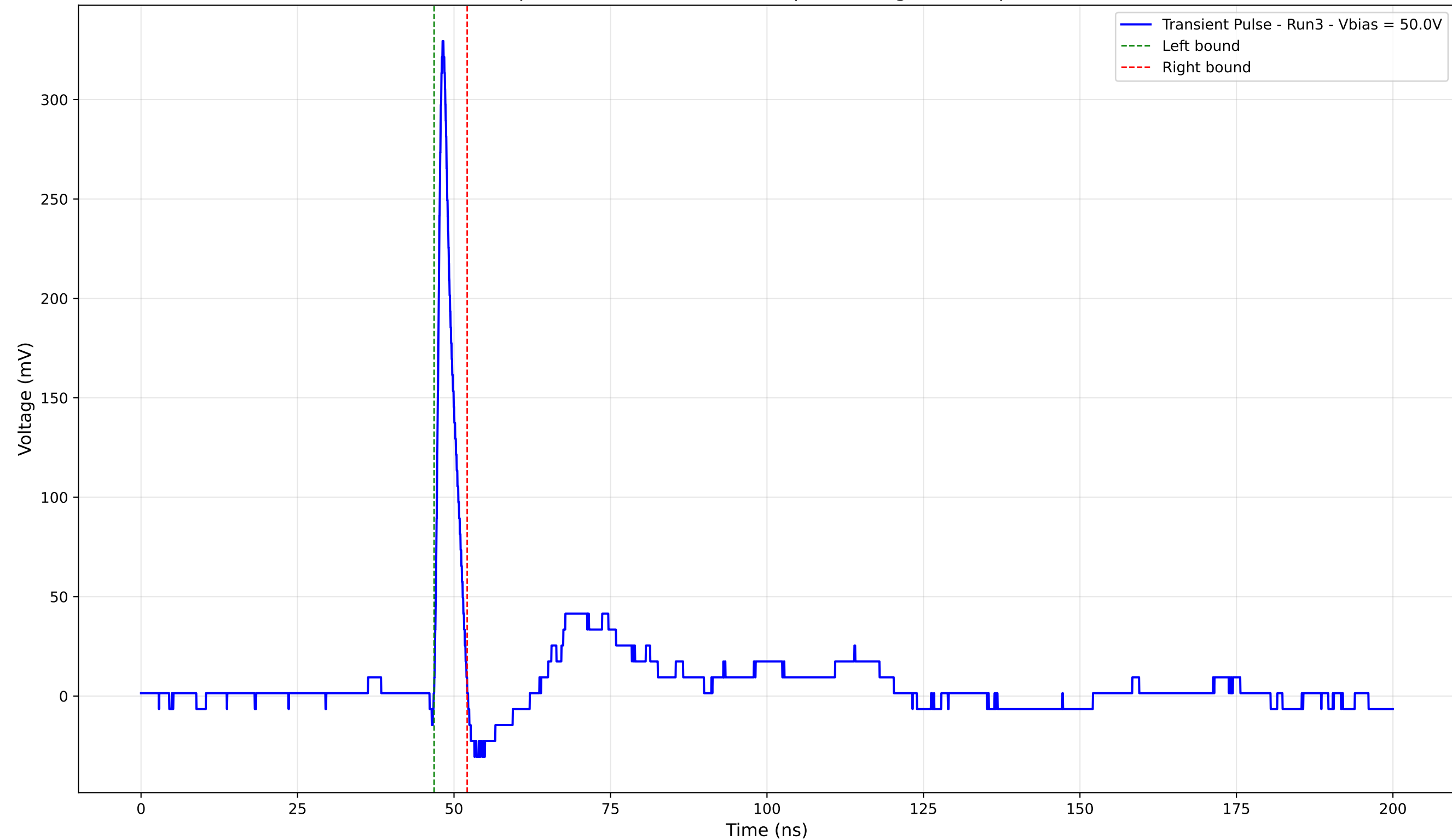
Transient Pulse - Sample: 4003 - Position: 385.0 \mu\text{m} - Charge: 16.44 pC - Rise Time: 0.90 ns
