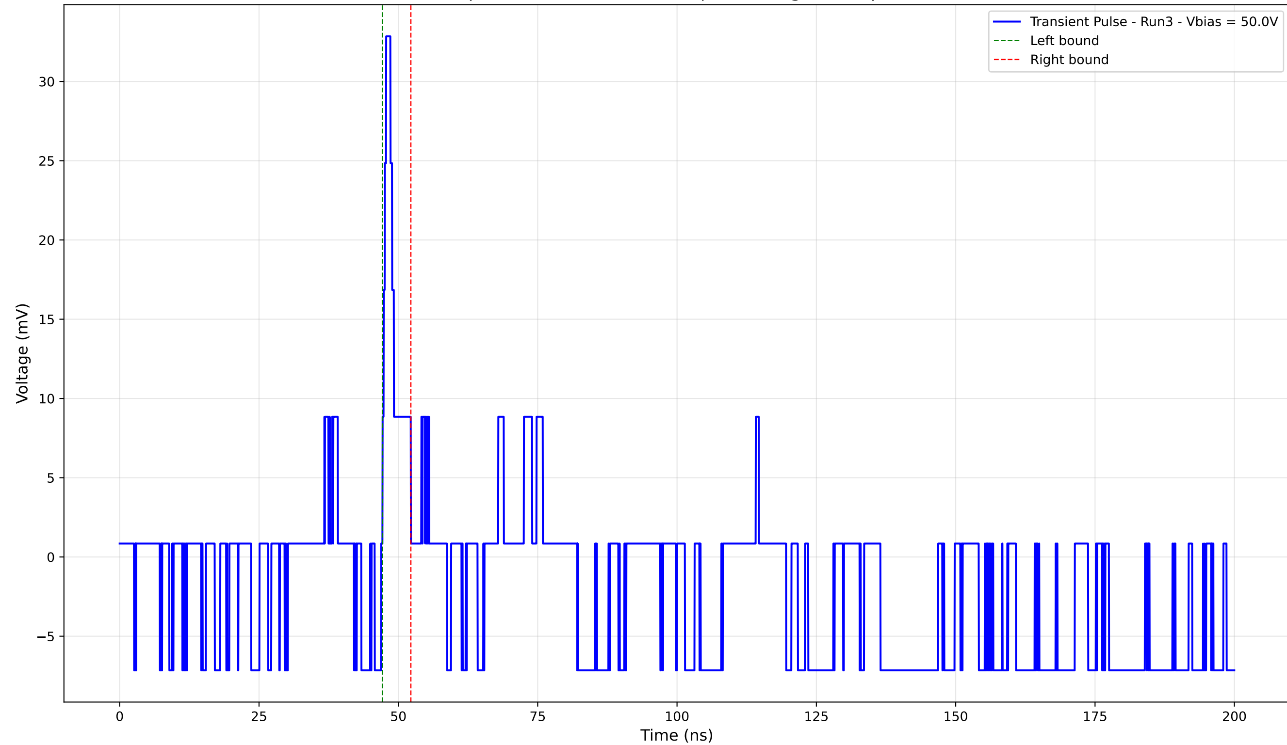
Transient Pulse - Sample: 4003 - Position: 45.0 \mu\text{m} - Charge: 1.53 pC - Rise Time: 0.65 ns
