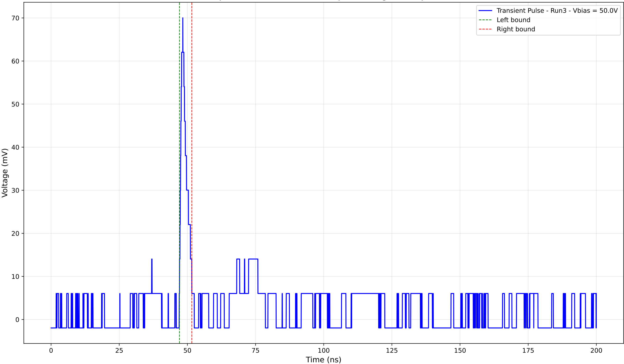
Transient Pulse - Sample: 4003 - Position: 610.0 \mu\text{m} - Charge: 3.30 pC - Rise Time: 1.22 ns
