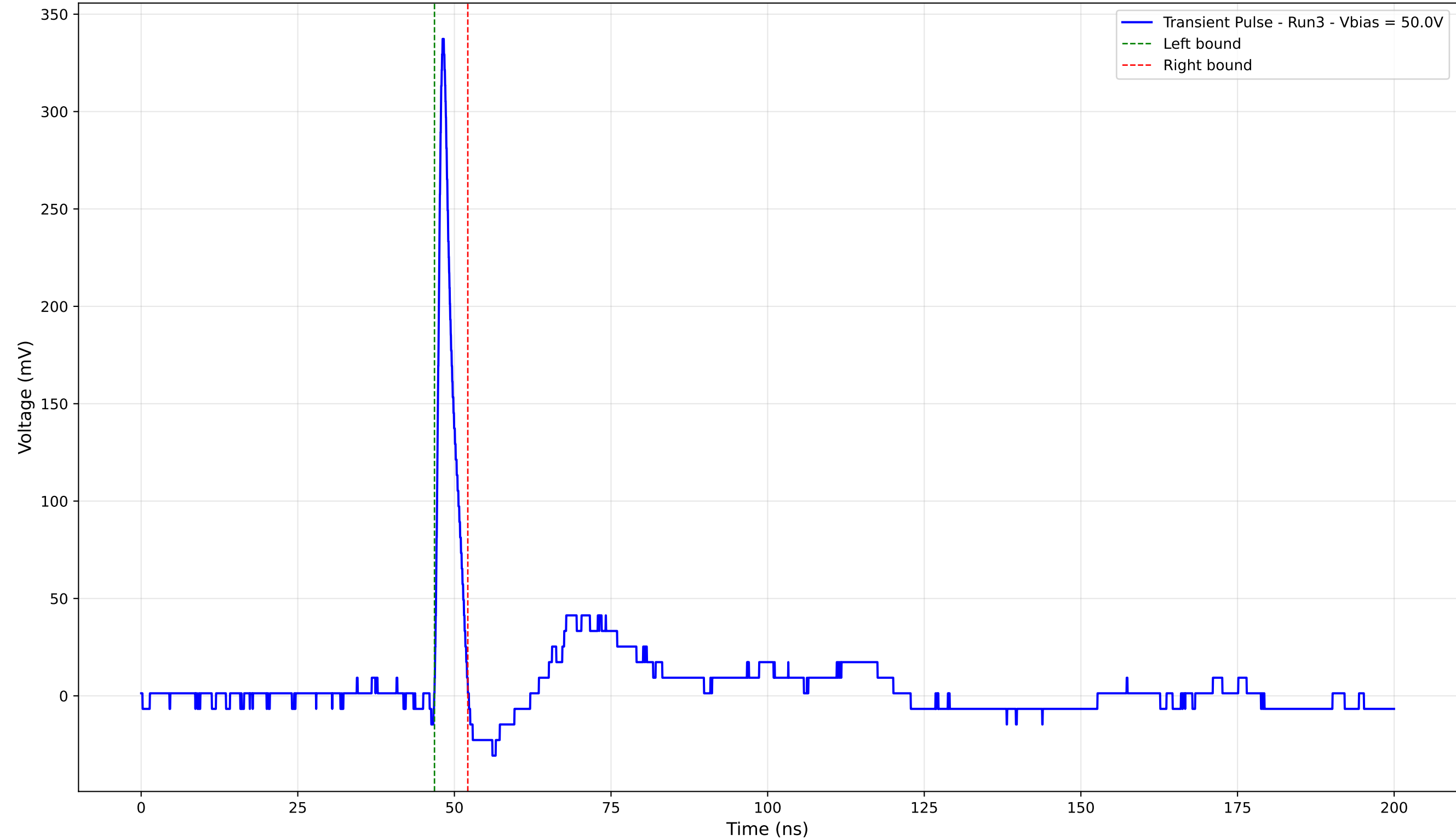
Transient Pulse - Sample: 4003 - Position: 310.0 \mu\text{m} - Charge: 16.68 pC - Rise Time: 0.86 ns
