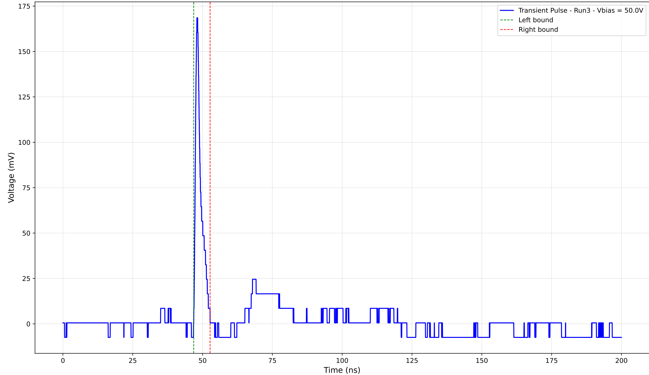
Transient Pulse - Sample: 4003 - Position: 155.0 \mu\text{m} - Charge: 7.76 pC - Rise Time: 0.78 ns
