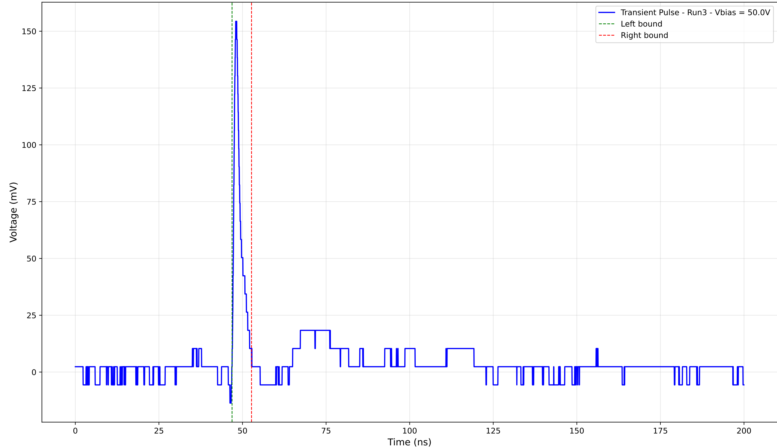
Transient Pulse - Sample: 4003 - Position: 145.0 \mu\text{m} - Charge: 7.19 pC - Rise Time: 0.85 ns
