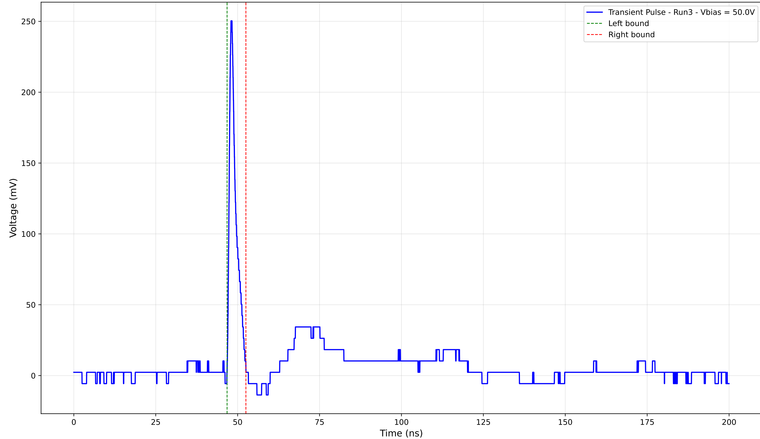
Transient Pulse - Sample: 4003 - Position: 210.0 \mu\text{m} - Charge: 12.10 pC - Rise Time: 0.84 ns
