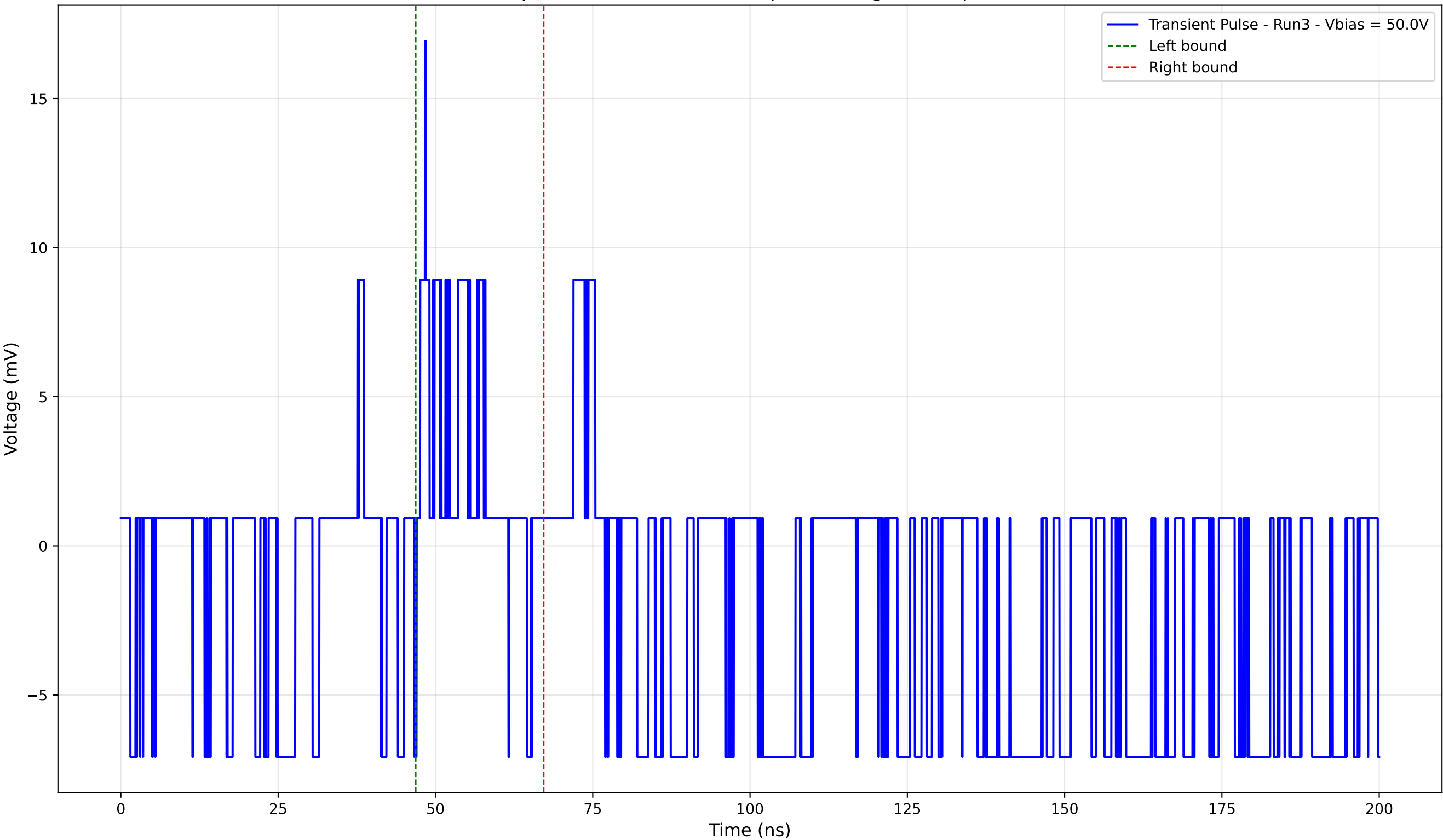
Transient Pulse - Sample: 4003 - Position: 0.0 \mu\text{m} - Charge: 1.17 pC - Rise Time: 0.80 ns
