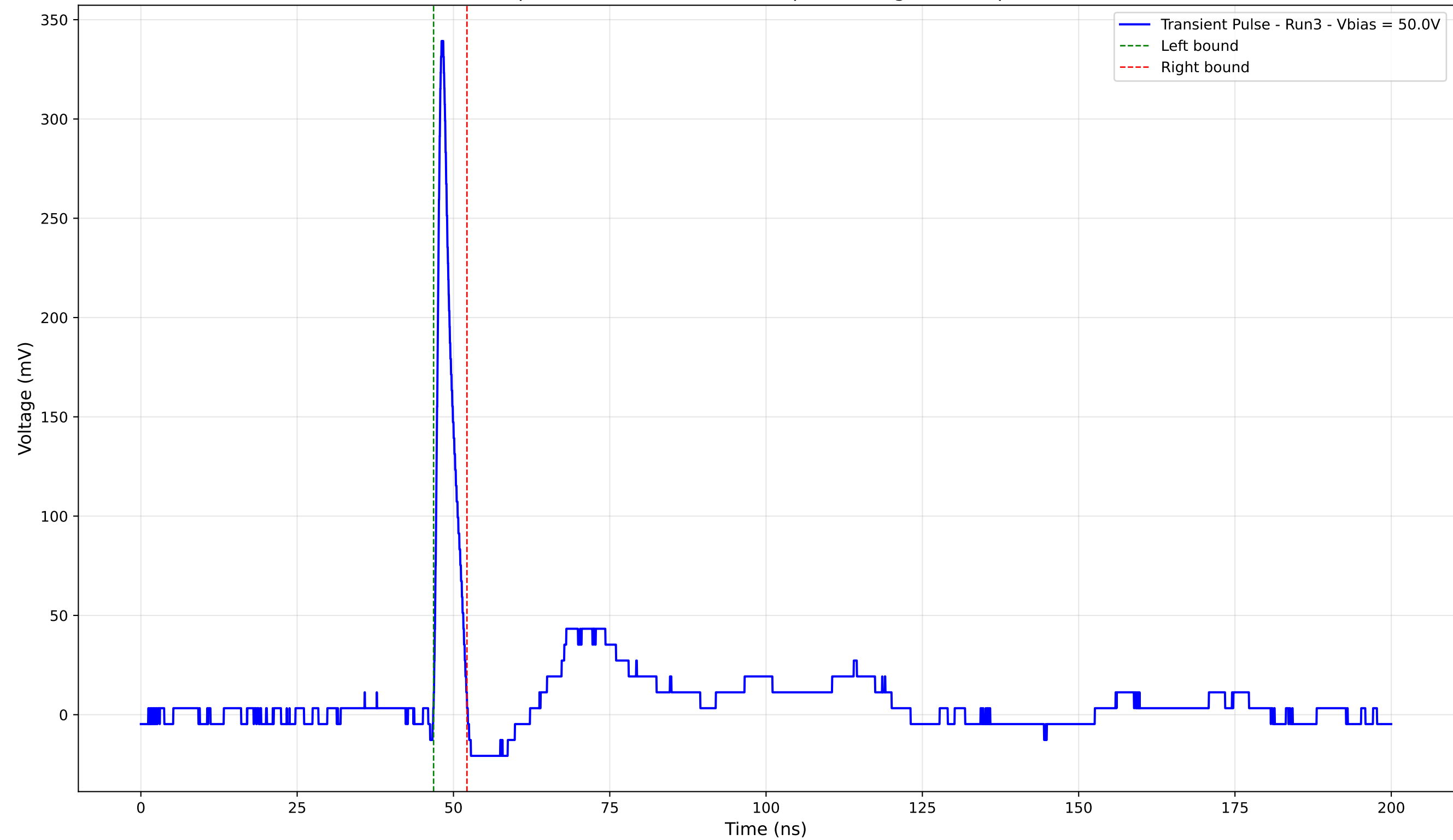
Transient Pulse - Sample: 4003 - Position: 325.0 \mu\text{m} - Charge: 17.12 pC - Rise Time: 0.88 ns
