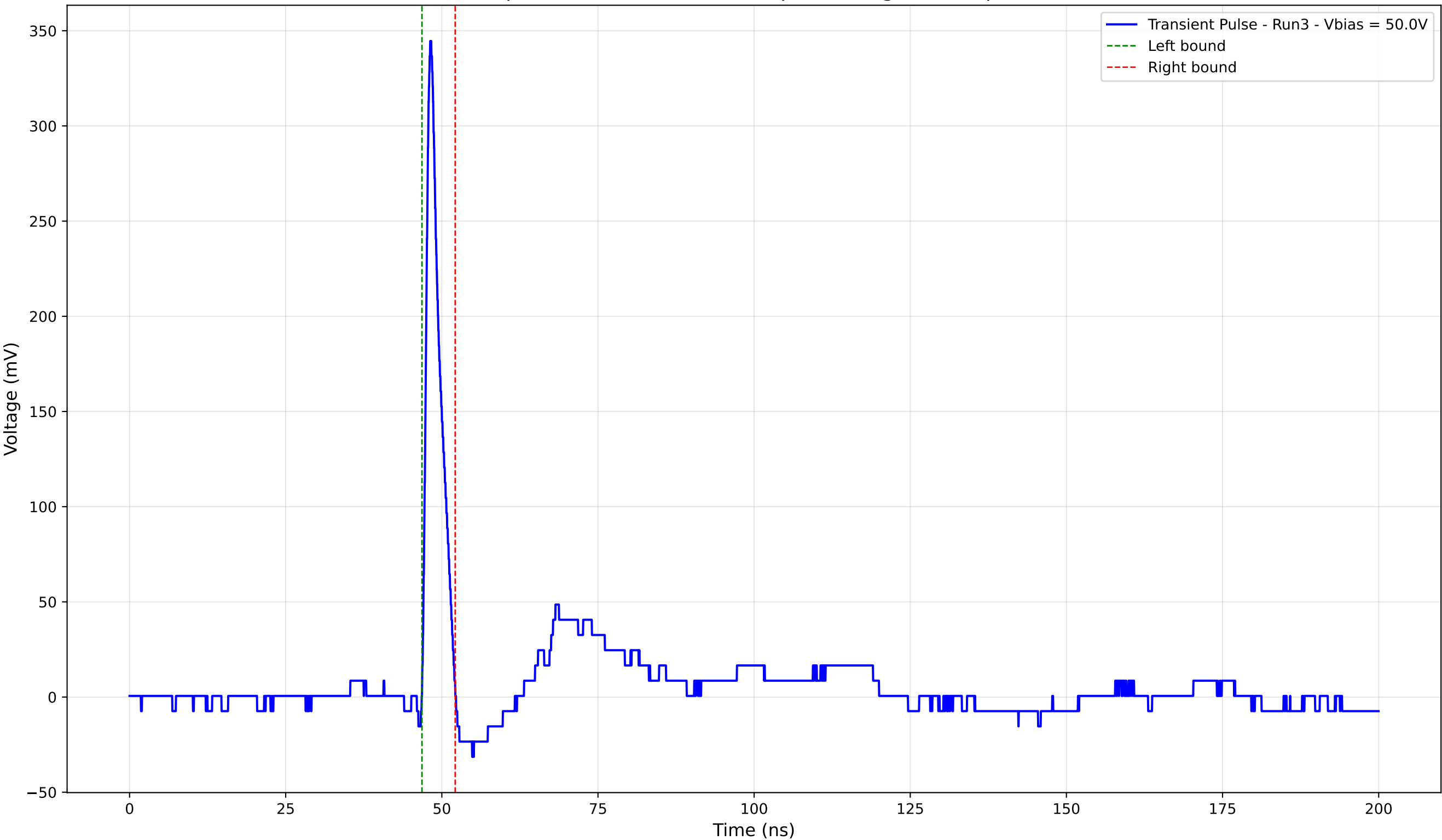
Transient Pulse - Sample: 4003 - Position: 355.0 \mu\text{m} - Charge: 17.23 pC - Rise Time: 0.88 ns
