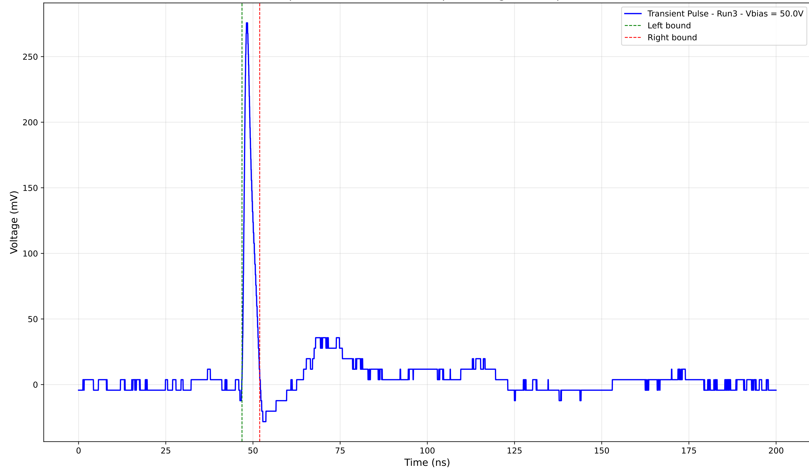
Transient Pulse - Sample: 4003 - Position: 440.0 \mu\text{m} - Charge: 14.04 pC - Rise Time: 0.92 ns
