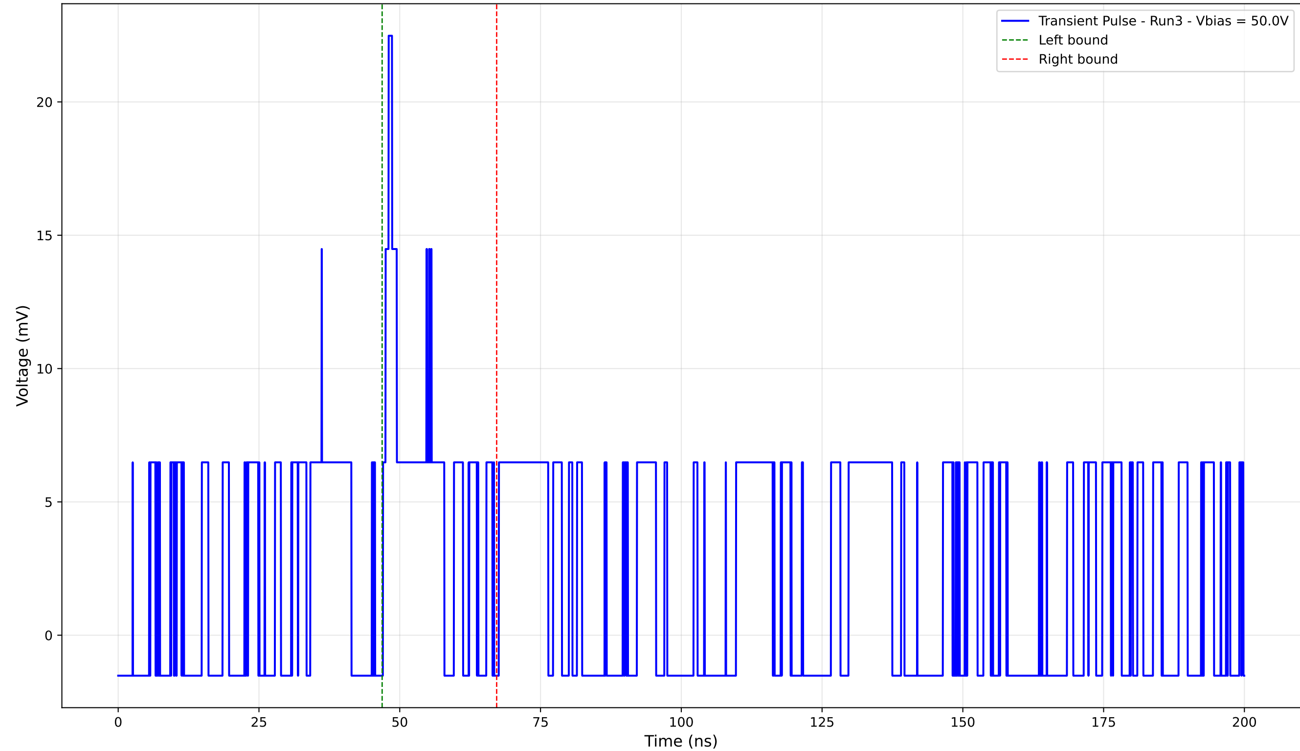
Transient Pulse - Sample: 4003 - Position: 15.0 \mu\text{m} - Charge: 2.29 pC - Rise Time: 1.02 ns
