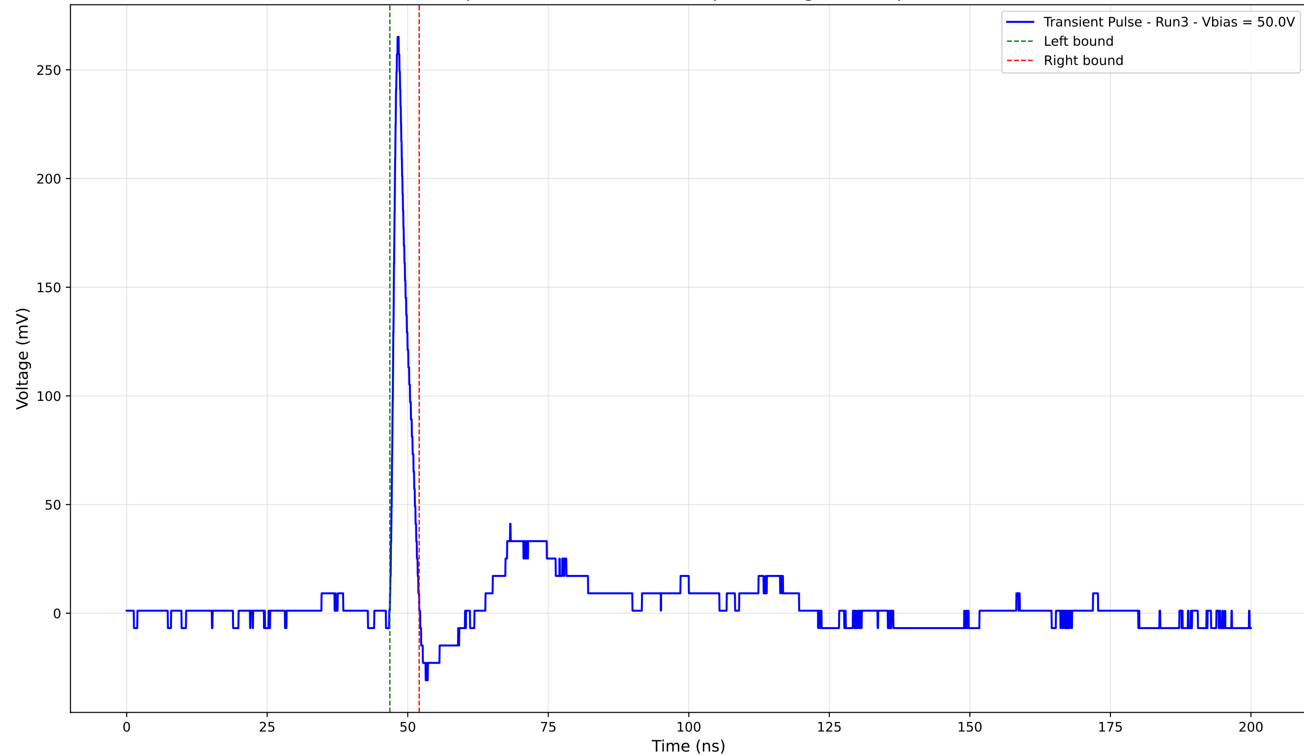
Transient Pulse - Sample: 4003 - Position: 450.0 \mu\text{m} - Charge: 13.59 pC - Rise Time: 0.92 ns
