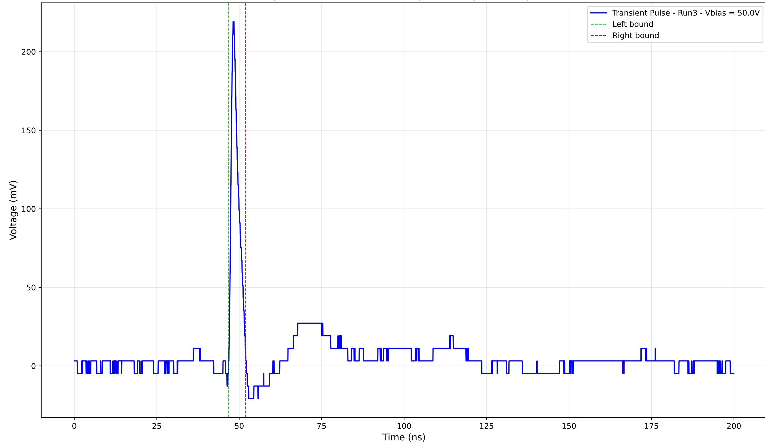
Transient Pulse - Sample: 4003 - Position: 490.0 \mu\text{m} - Charge: 11.16 pC - Rise Time: 0.93 ns
