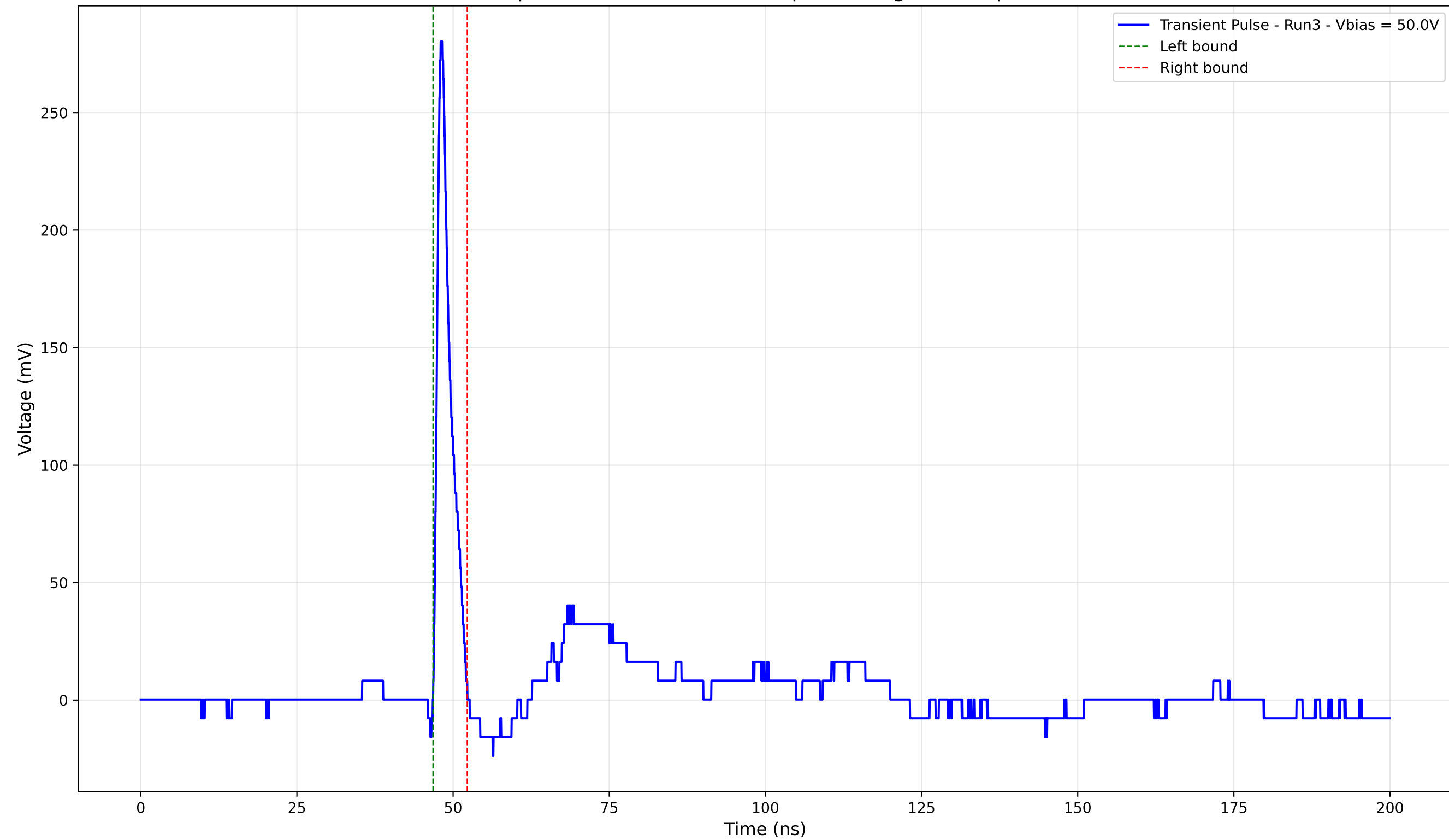
Transient Pulse - Sample: 4003 - Position: 245.0 \mu\text{m} - Charge: 13.78 pC - Rise Time: 0.85 ns
