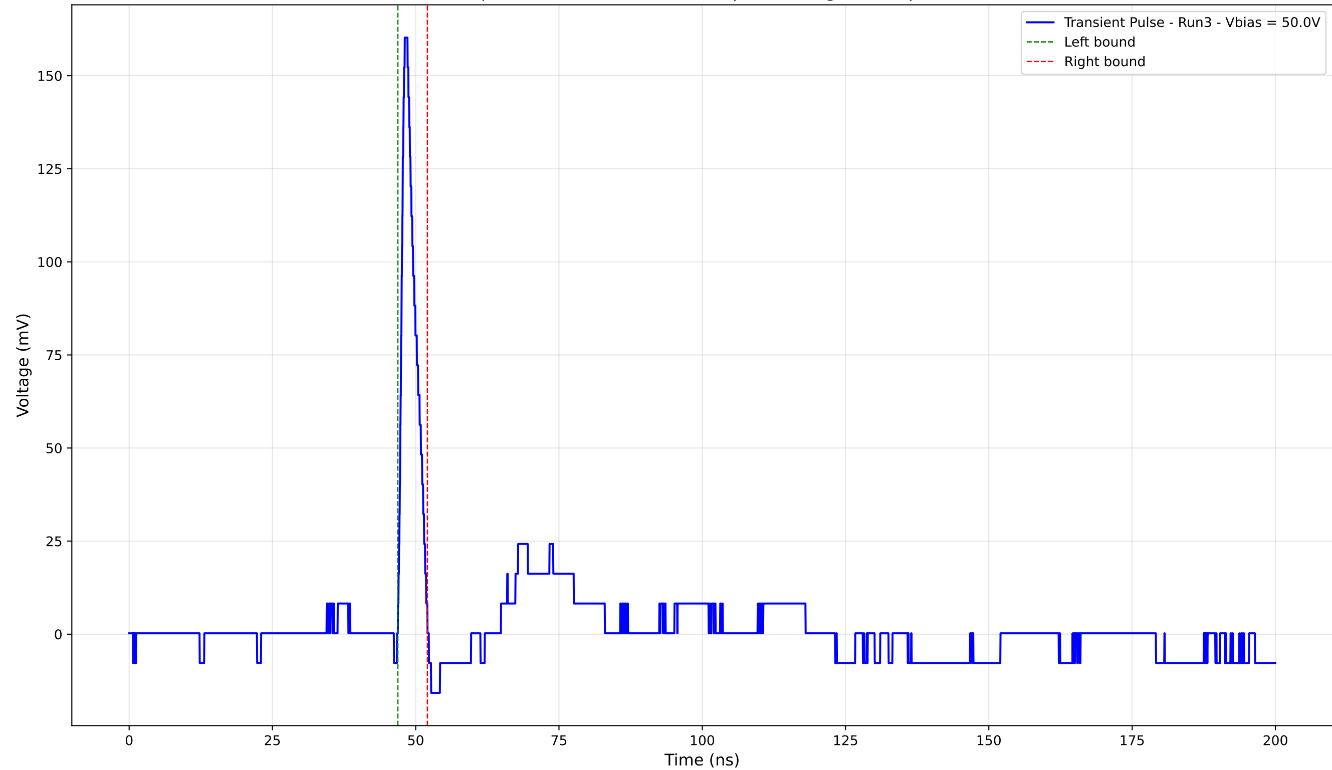
Transient Pulse - Sample: 4003 - Position: 550.0 \mu\text{m} - Charge: 8.65 pC - Rise Time: 0.88 ns
