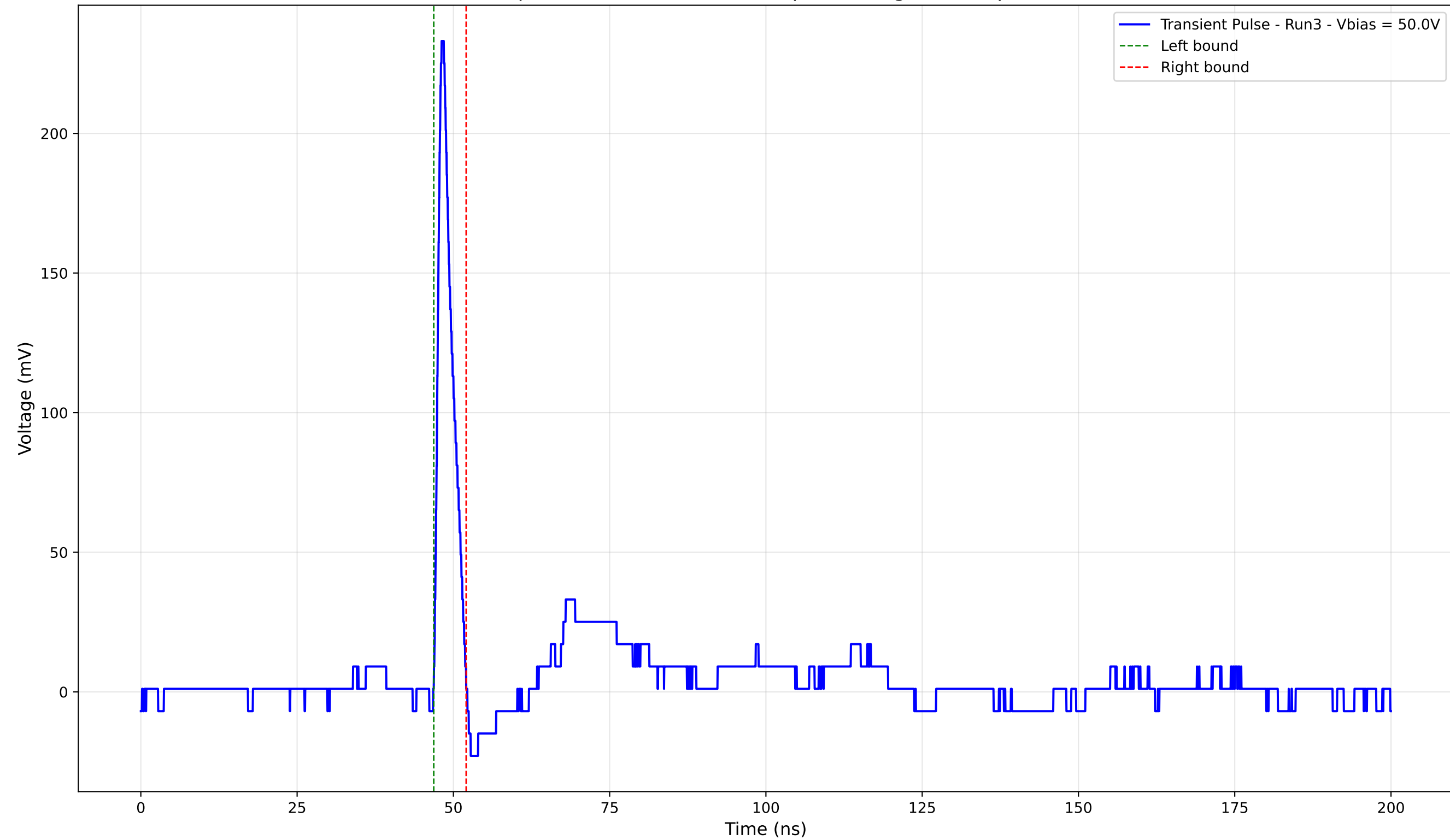
Transient Pulse - Sample: 4003 - Position: 475.0 \mu\text{m} - Charge: 12.02 pC - Rise Time: 0.92 ns
