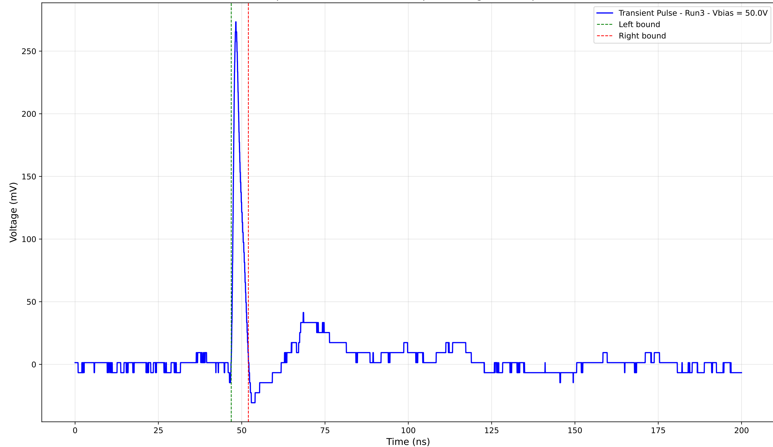
Transient Pulse - Sample: 4003 - Position: 445.0 \mu\text{m} - Charge: 13.80 pC - Rise Time: 0.92 ns
