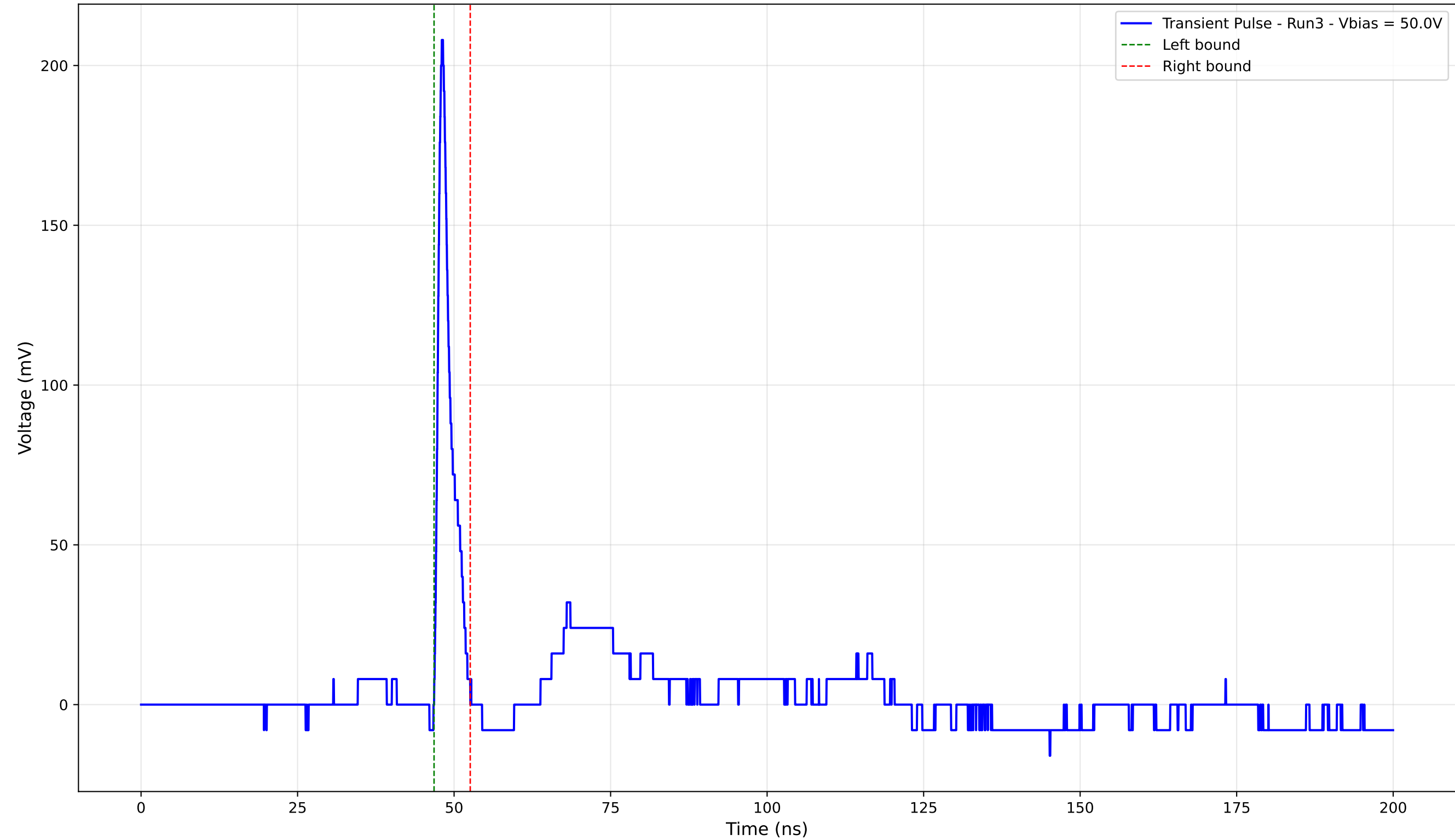
Transient Pulse - Sample: 4003 - Position: 180.0 \mu\text{m} - Charge: 9.86 pC - Rise Time: 0.89 ns
