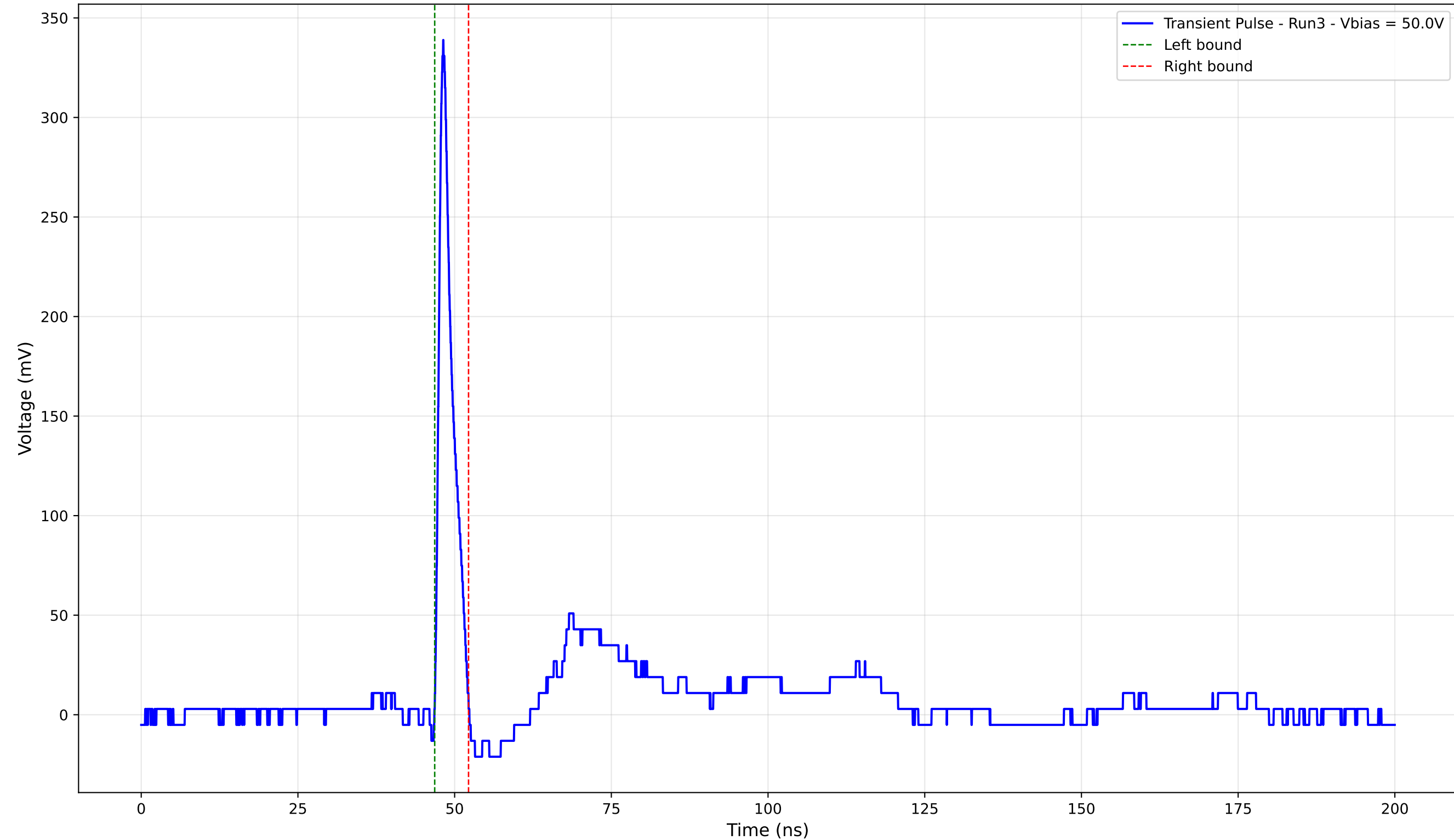
Transient Pulse - Sample: 4003 - Position: 300.0 \mu\text{m} - Charge: 16.69 pC - Rise Time: 0.90 ns
