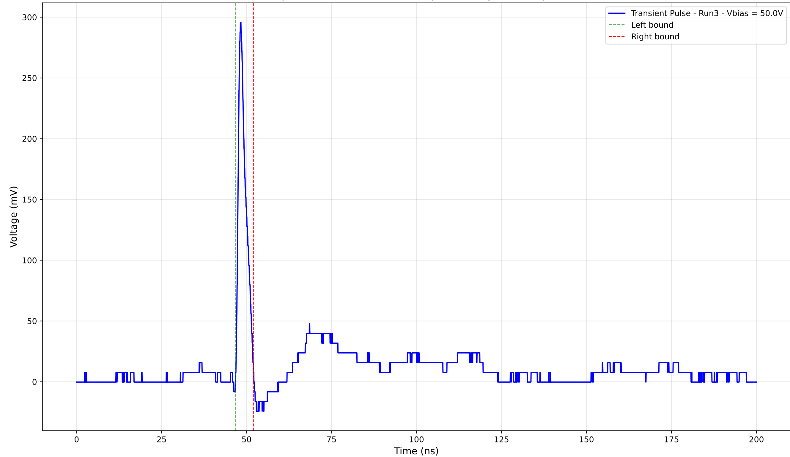
Transient Pulse - Sample: 4003 - Position: 425.0 \mu\text{m} - Charge: 15.18 pC - Rise Time: 0.97 ns
