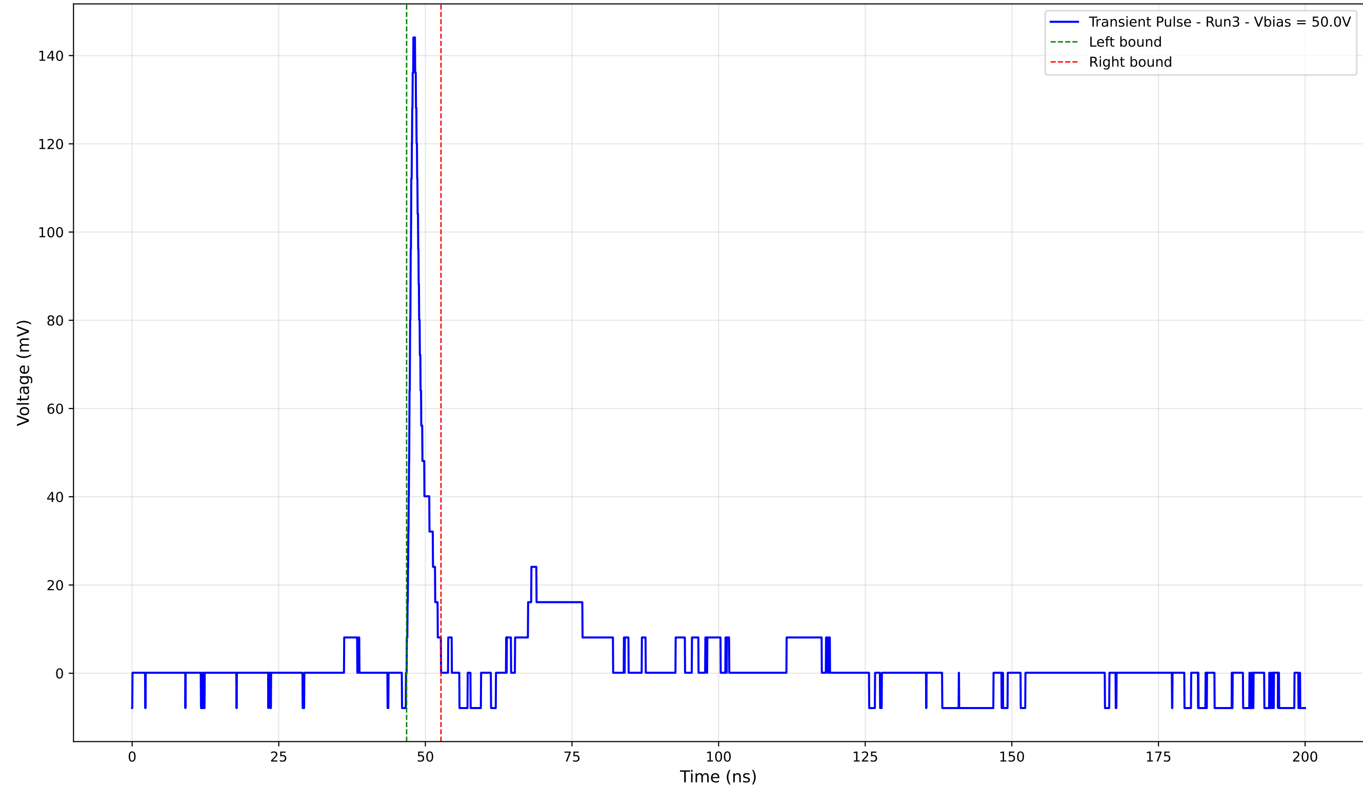
Transient Pulse - Sample: 4003 - Position: 135.0 \mu\text{m} - Charge: 6.61 pC - Rise Time: 0.88 ns
