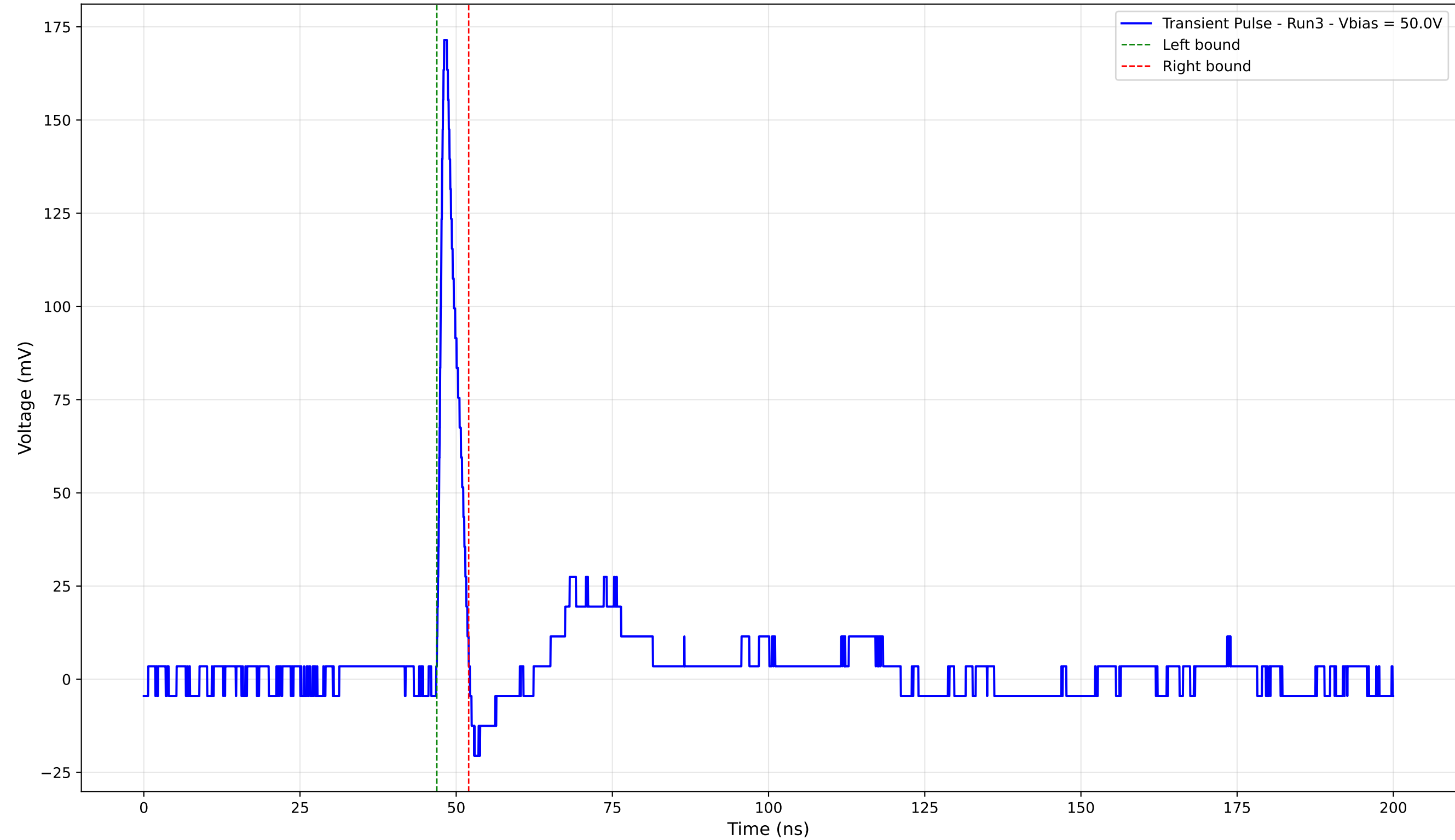
Transient Pulse - Sample: 4003 - Position: 585.0 \mu\text{m} - Charge: 9.33 pC - Rise Time: 0.89 ns
