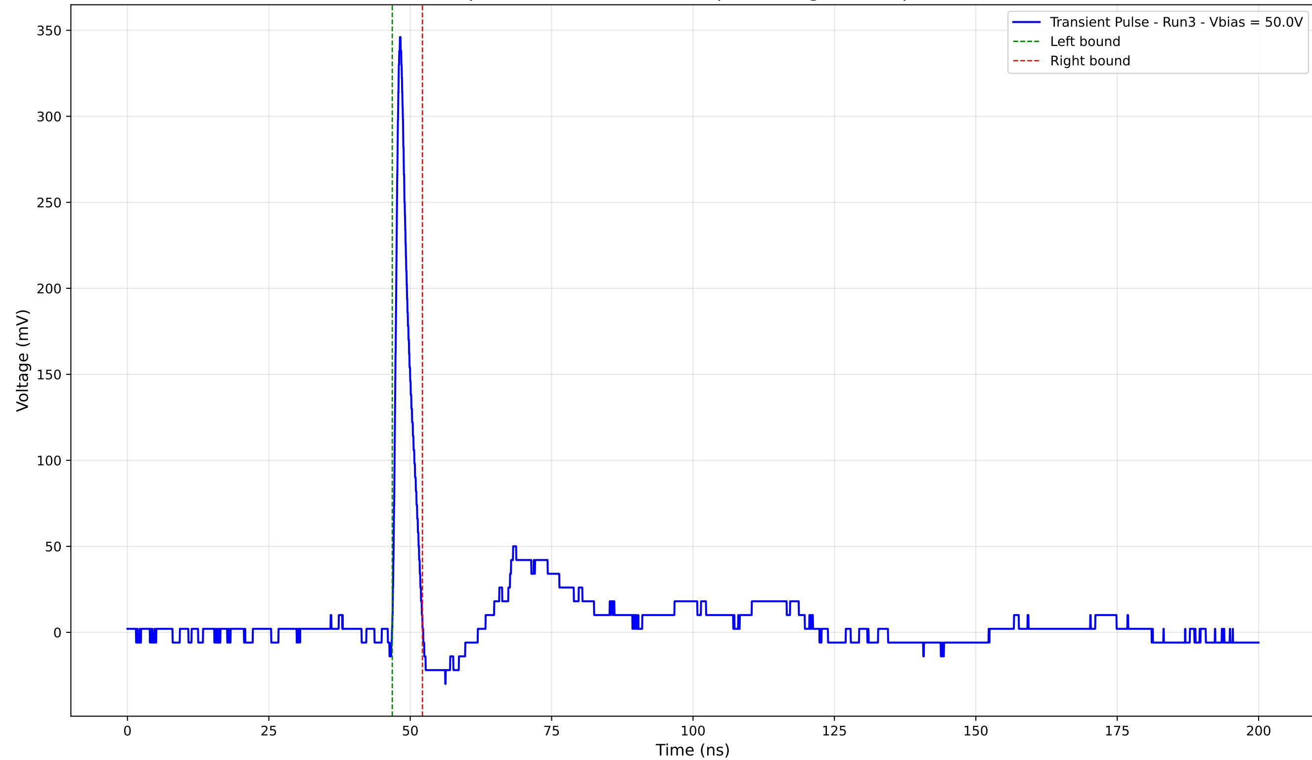
Transient Pulse - Sample: 4003 - Position: 345.0 \mu\text{m} - Charge: 17.33 pC - Rise Time: 0.90 ns
