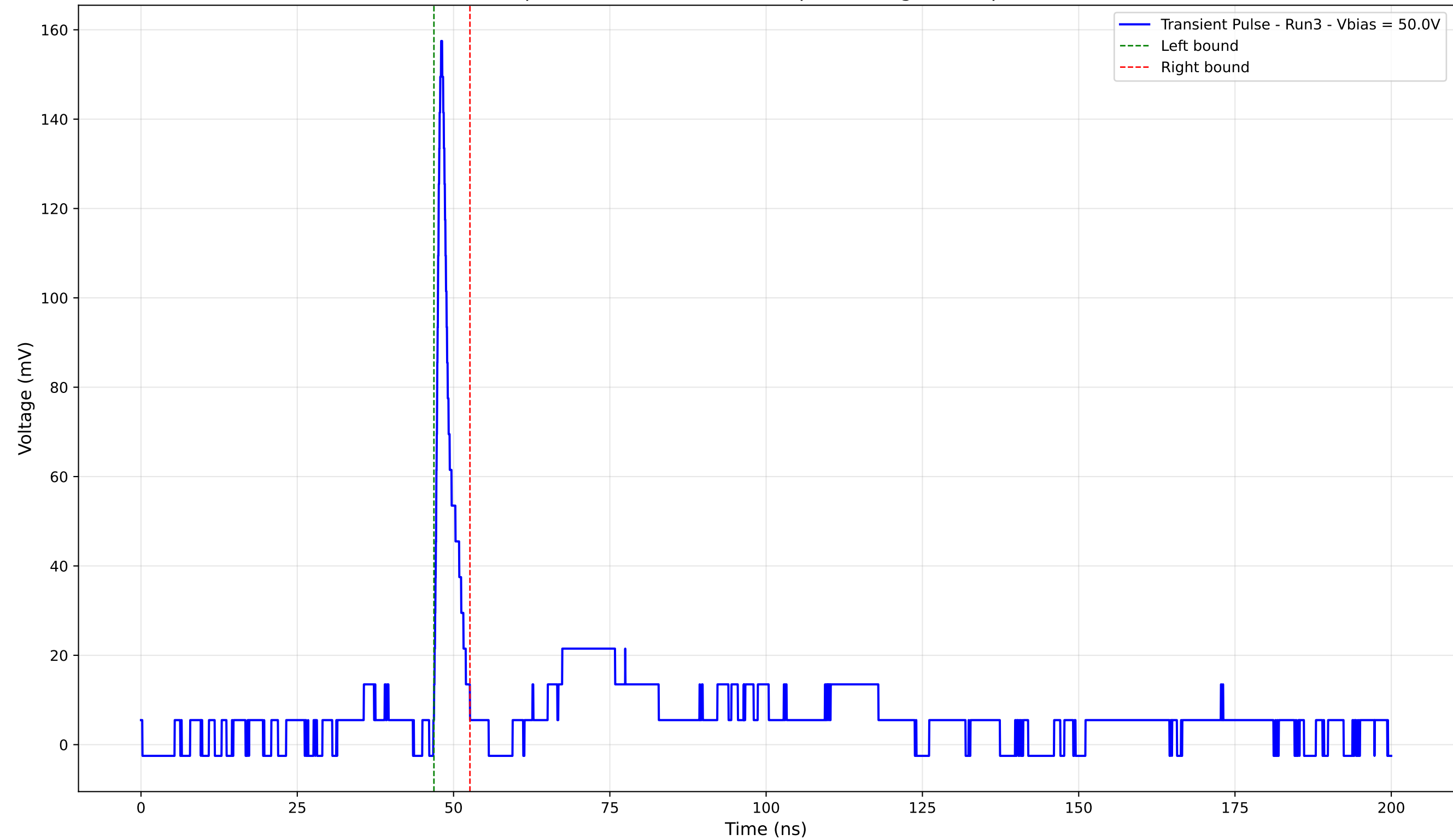
Transient Pulse - Sample: 4003 - Position: 140.0 \mu\text{m} - Charge: 7.45 pC - Rise Time: 0.91 ns
