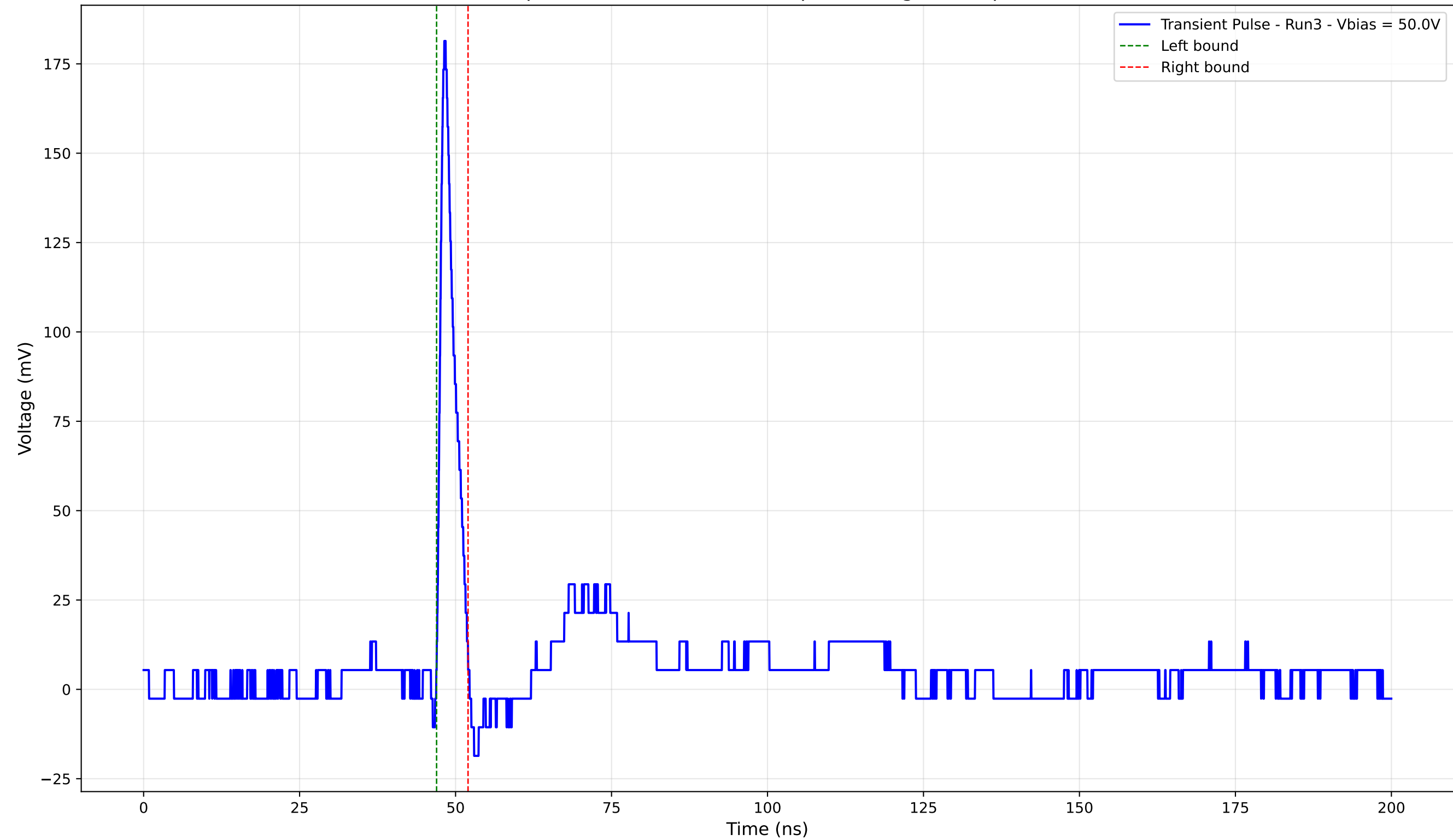
Transient Pulse - Sample: 4003 - Position: 580.0 \mu\text{m} - Charge: 9.31 pC - Rise Time: 0.89 ns
