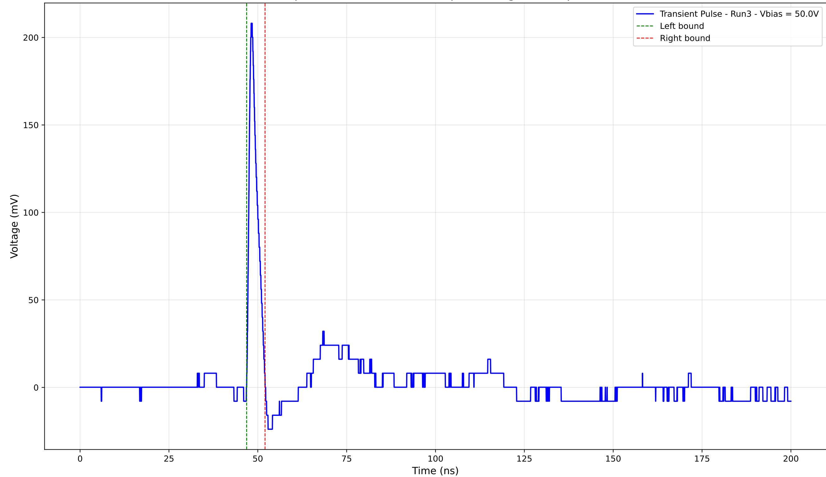
Transient Pulse - Sample: 4003 - Position: 495.0 \mu\text{m} - Charge: 10.81 pC - Rise Time: 0.91 ns
