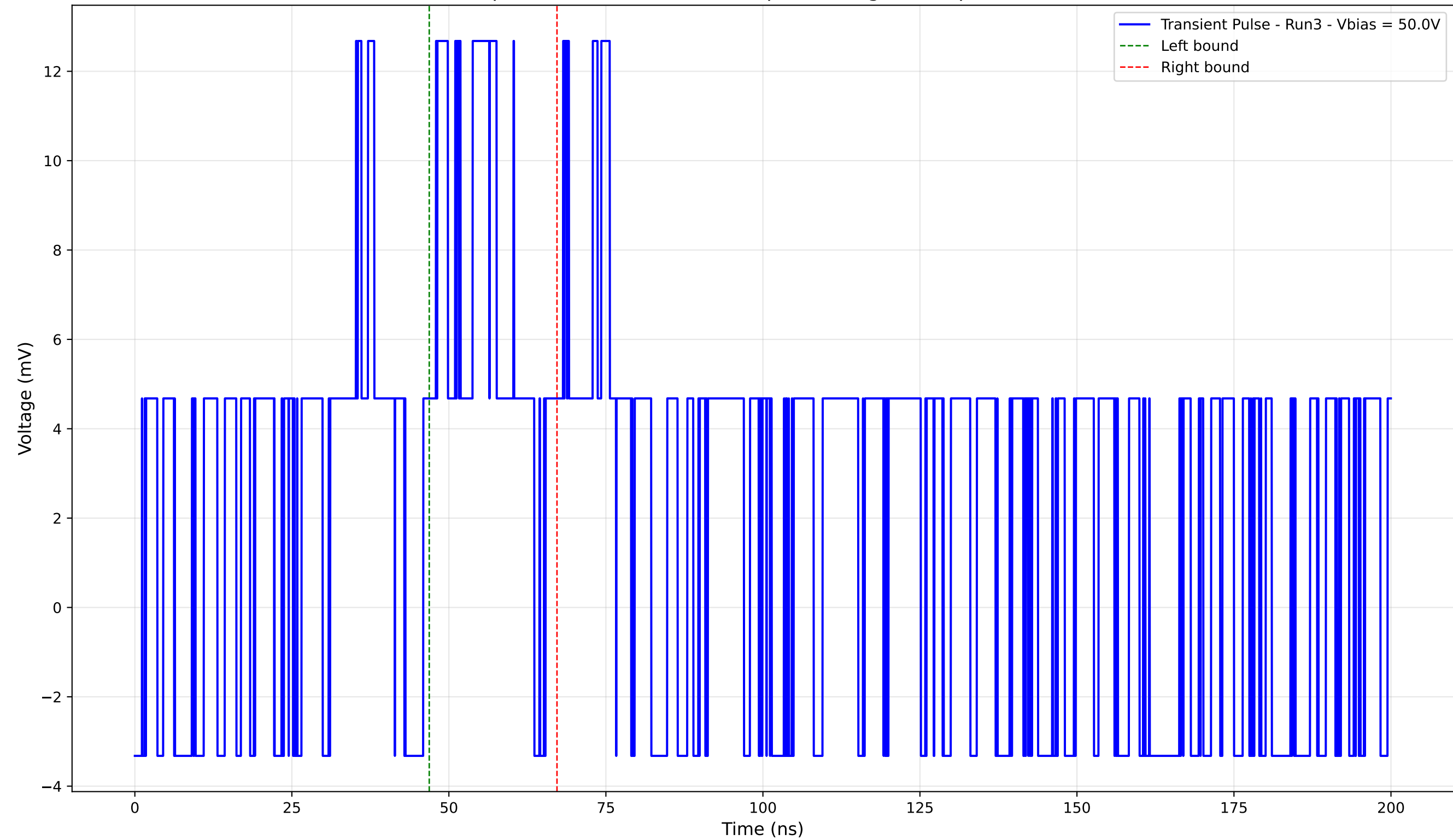
Transient Pulse - Sample: 4003 - Position: 640.0 \mu\text{m} - Charge: 2.64 pC - Rise Time: 0.00 ns (N/A)
