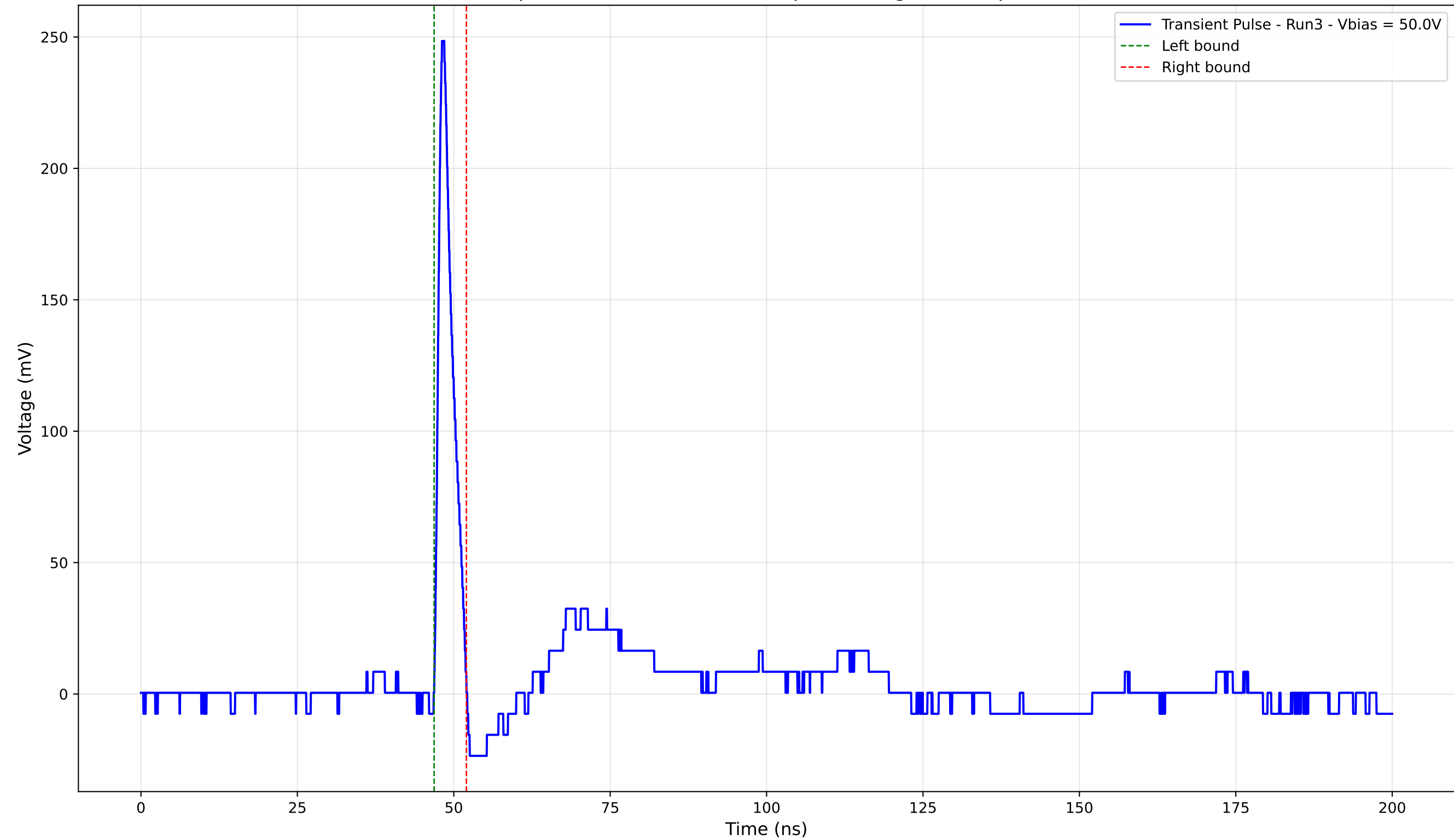
Transient Pulse - Sample: 4003 - Position: 460.0 \mu\text{m} - Charge: 12.84 pC - Rise Time: 0.86 ns
