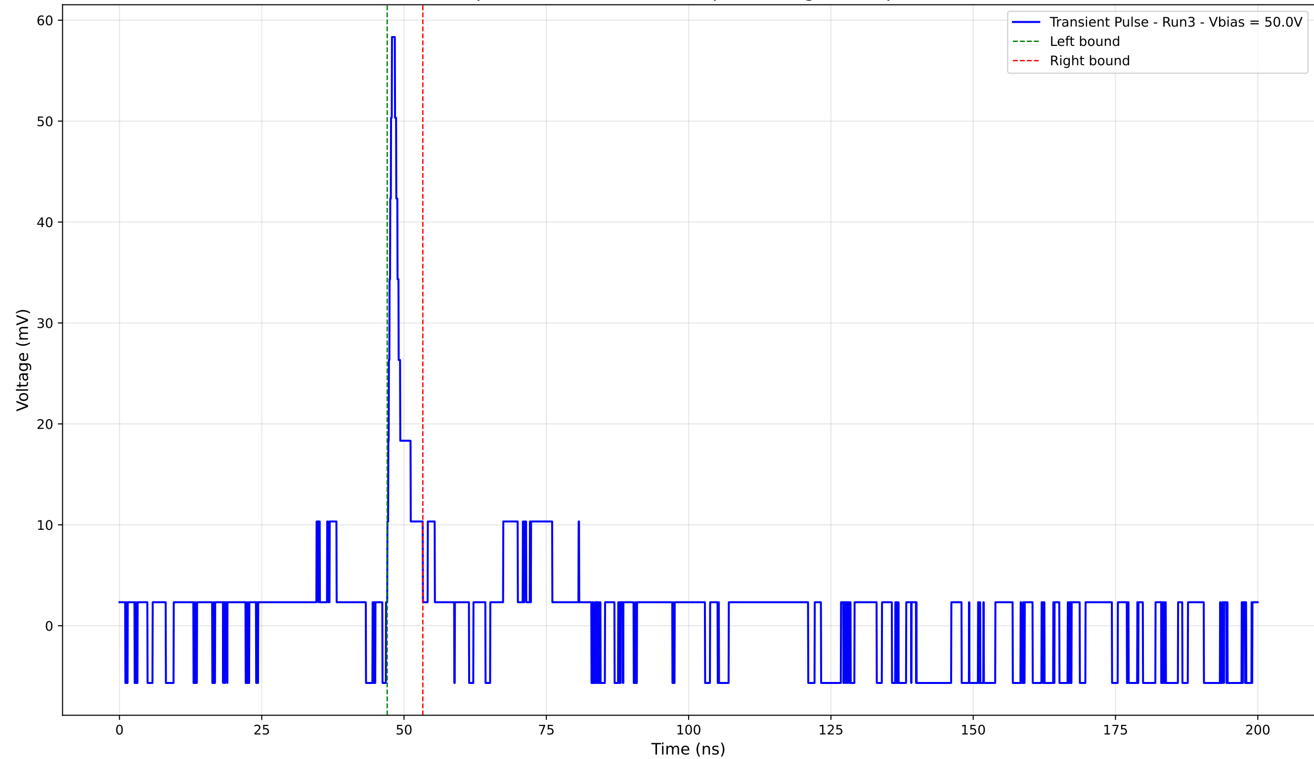
Transient Pulse - Sample: 4003 - Position: 65.0 \mu\text{m} - Charge: 2.94 pC - Rise Time: 0.81 ns
