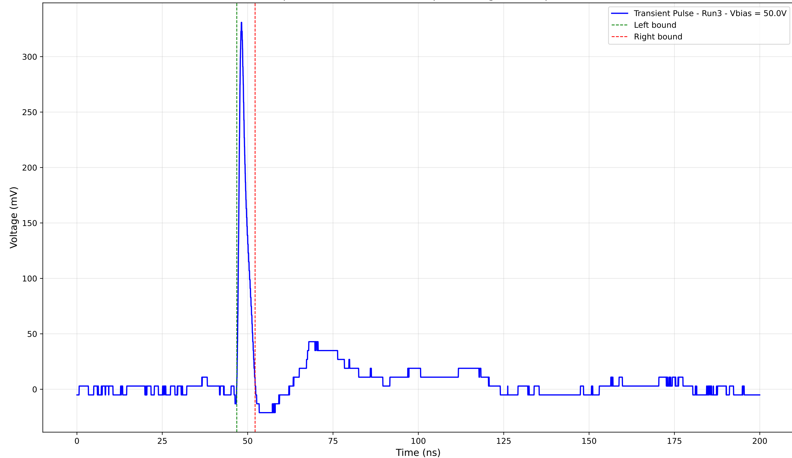
Transient Pulse - Sample: 4003 - Position: 295.0 \mu\text{m} - Charge: 16.30 pC - Rise Time: 0.88 ns
