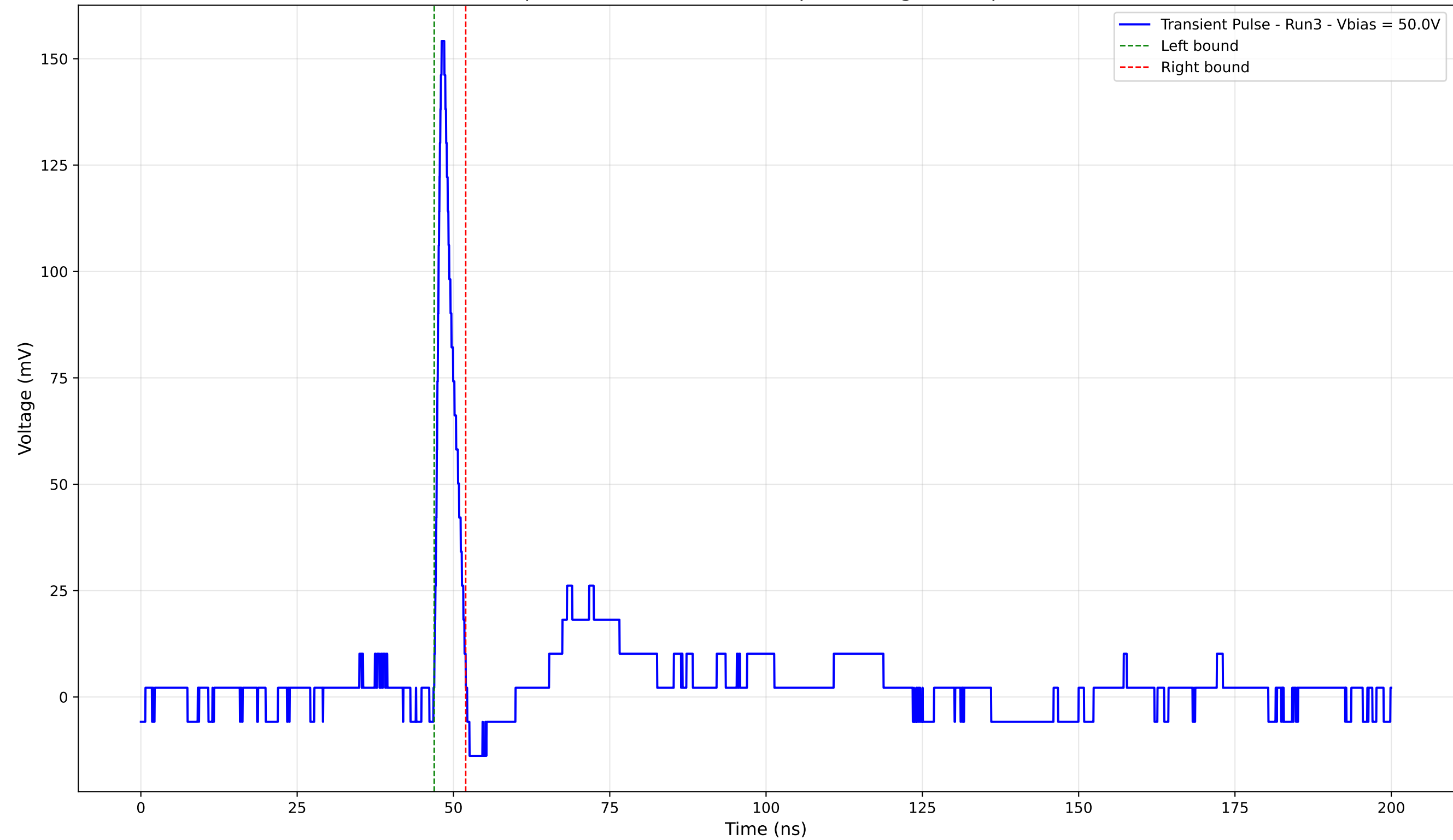
Transient Pulse - Sample: 4003 - Position: 555.0 \mu\text{m} - Charge: 8.09 pC - Rise Time: 0.95 ns
