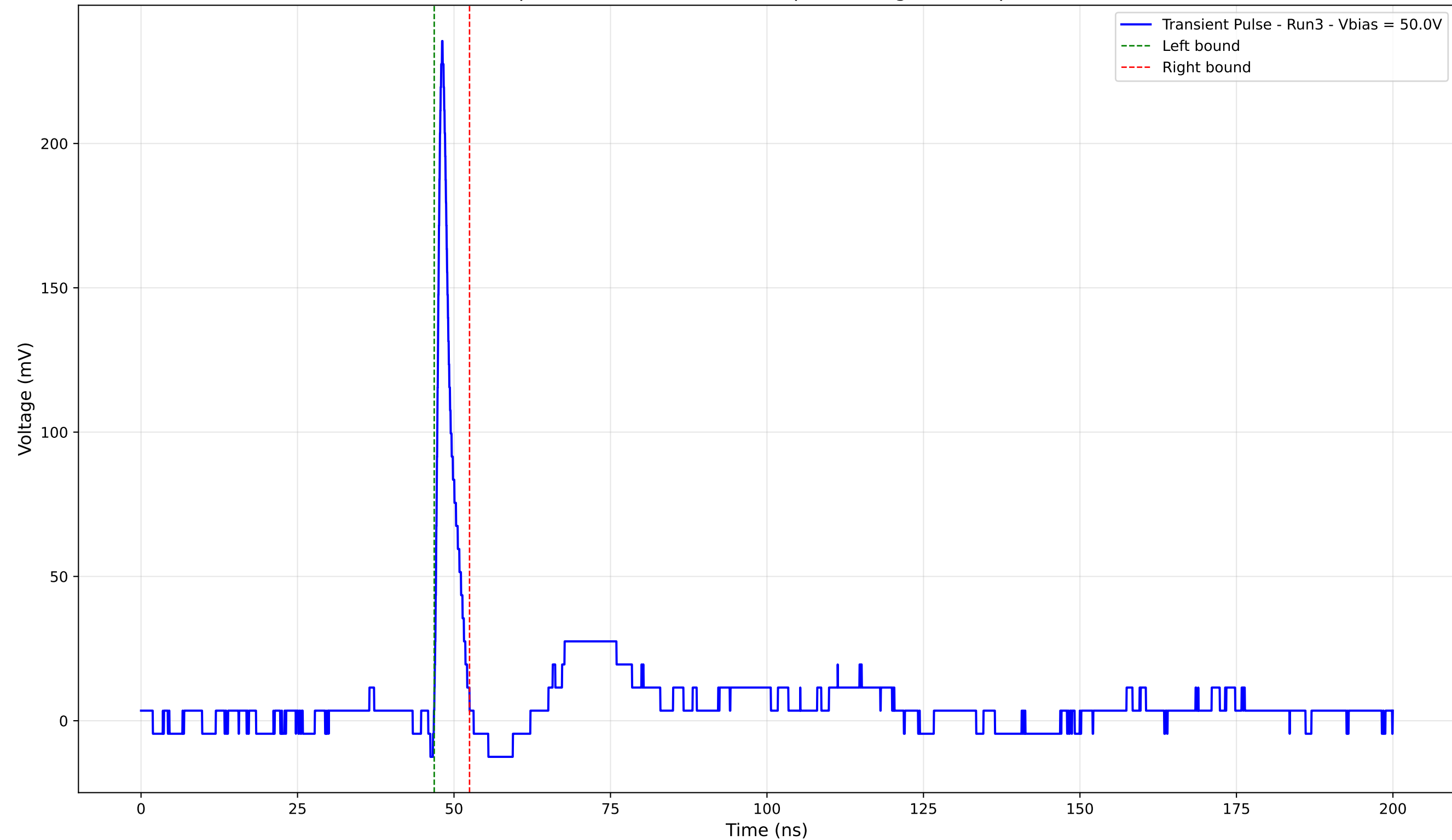
Transient Pulse - Sample: 4003 - Position: 200.0 \mu\text{m} - Charge: 11.05 pC - Rise Time: 0.89 ns
