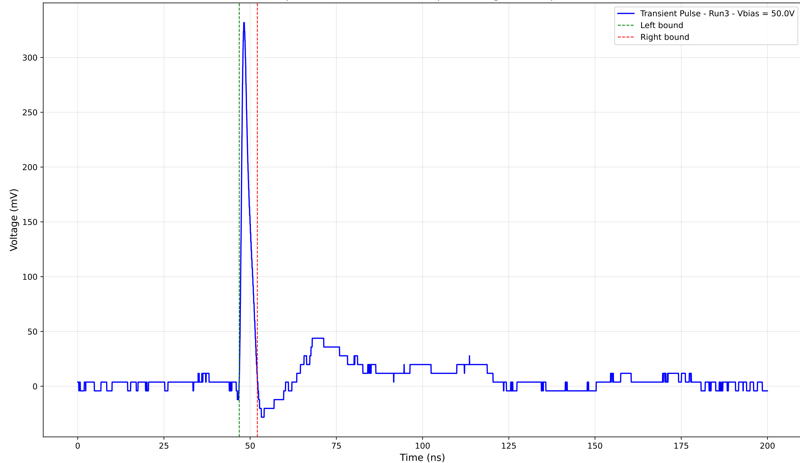
Transient Pulse - Sample: 4003 - Position: 380.0 \mu\text{m} - Charge: 16.80 pC - Rise Time: 0.91 ns
