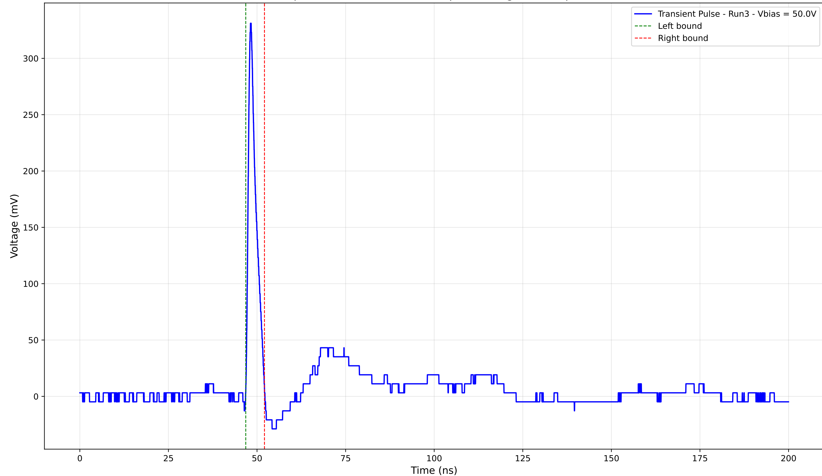
Transient Pulse - Sample: 4003 - Position: 375.0 \mu\text{m} - Charge: 16.68 pC - Rise Time: 0.91 ns
