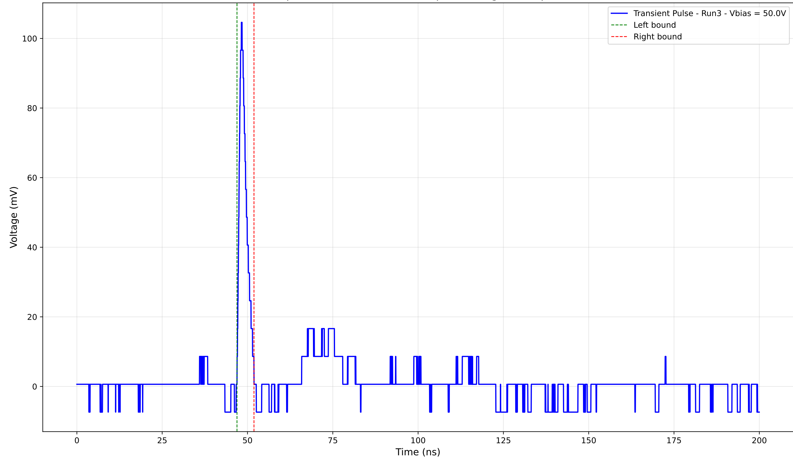
Transient Pulse - Sample: 4003 - Position: 605.0 \mu\text{m} - Charge: 5.03 pC - Rise Time: 0.92 ns
