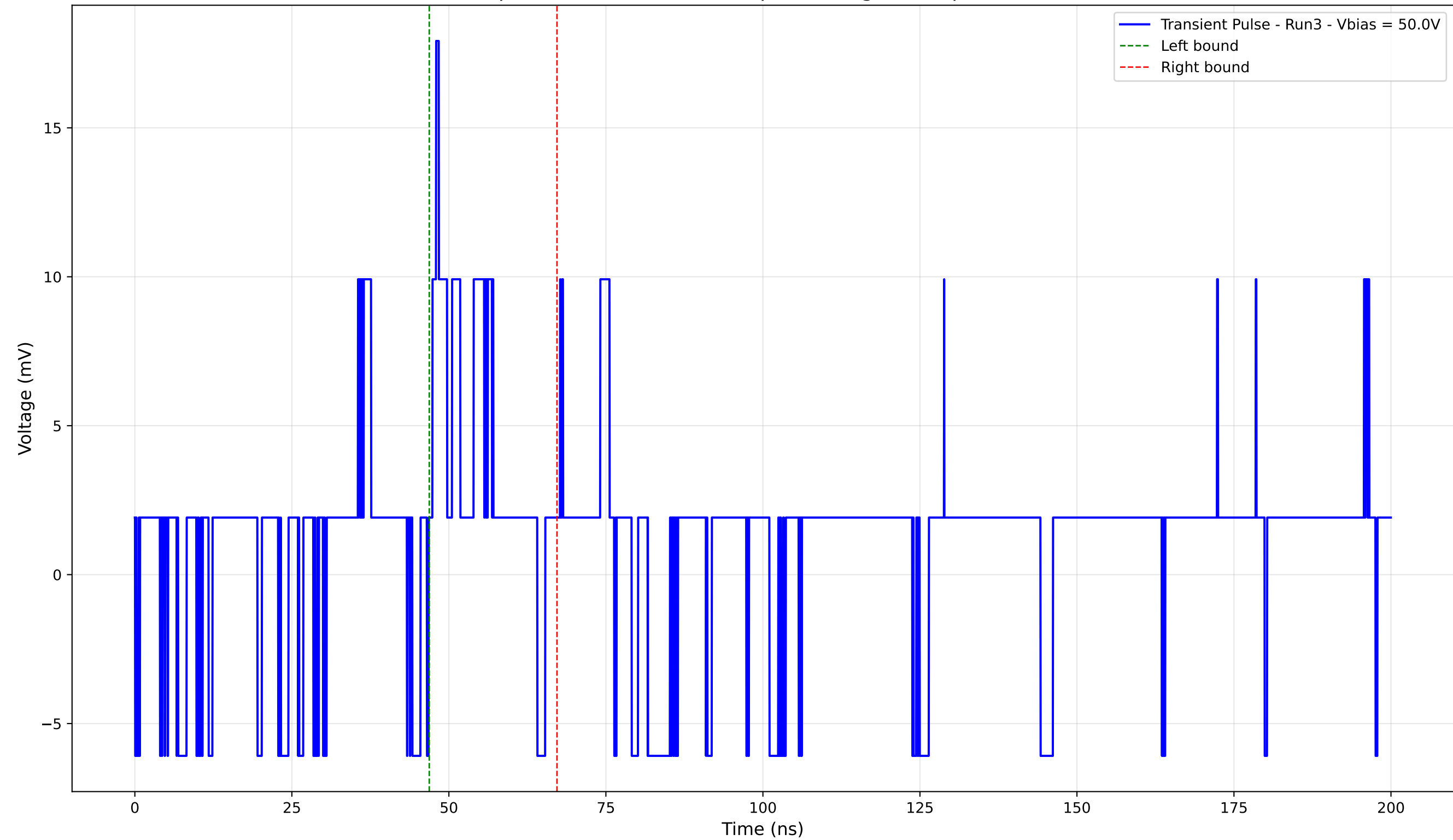
Transient Pulse - Sample: 4003 - Position: 10.0 \mu\text{m} - Charge: 1.68 pC - Rise Time: 0.00 ns (N/A)
