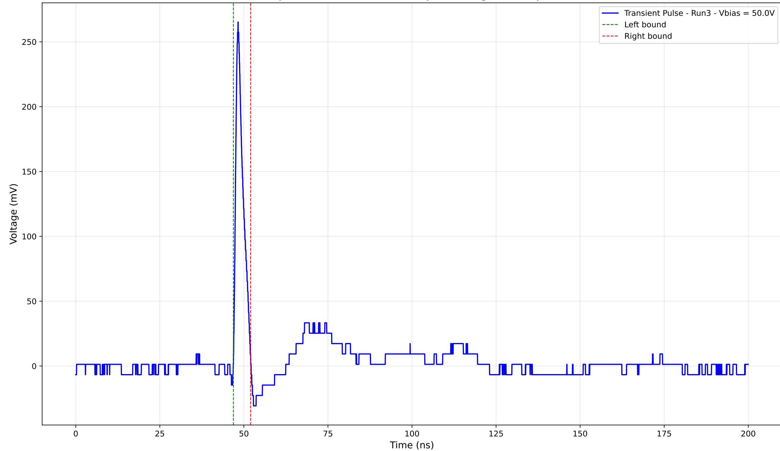
Transient Pulse - Sample: 4003 - Position: 455.0 \mu\text{m} - Charge: 13.23 pC - Rise Time: 0.90 ns
