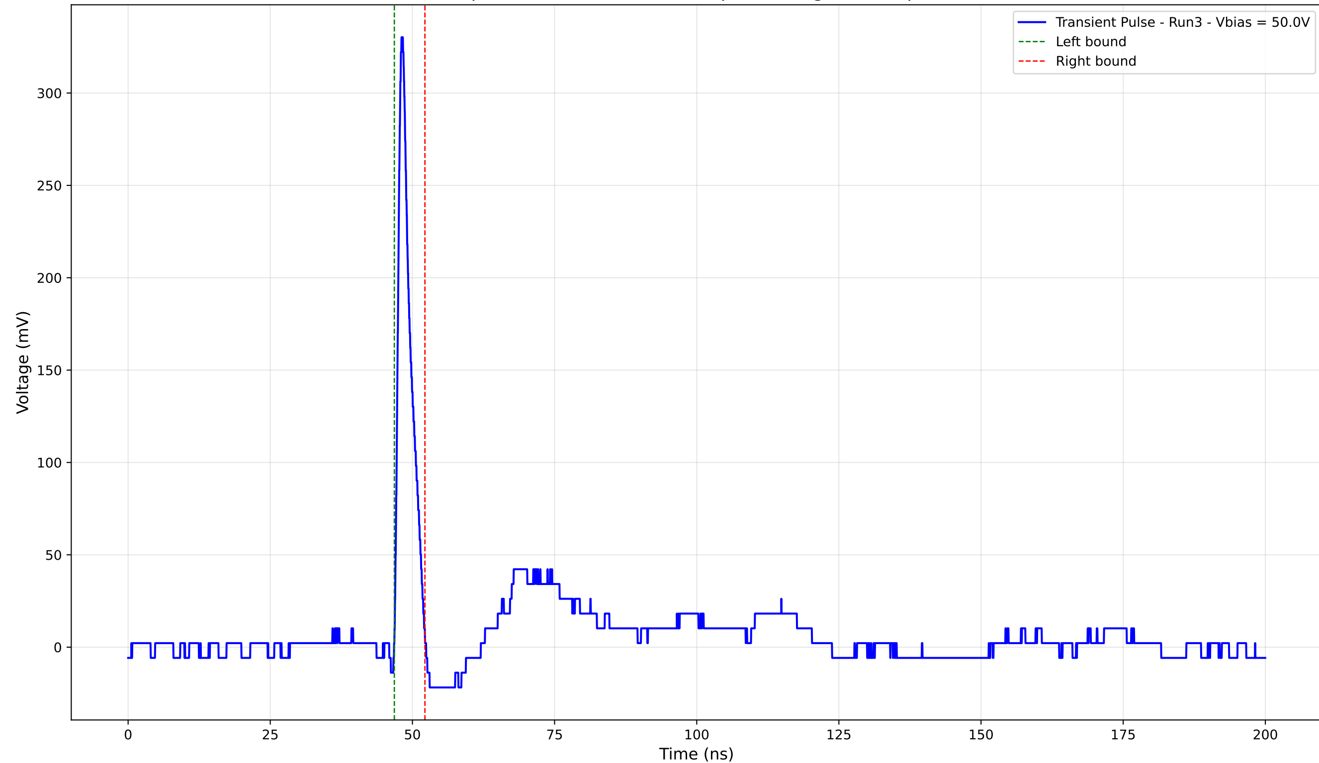
Transient Pulse - Sample: 4003 - Position: 305.0 \mu\text{m} - Charge: 16.50 pC - Rise Time: 0.86 ns
