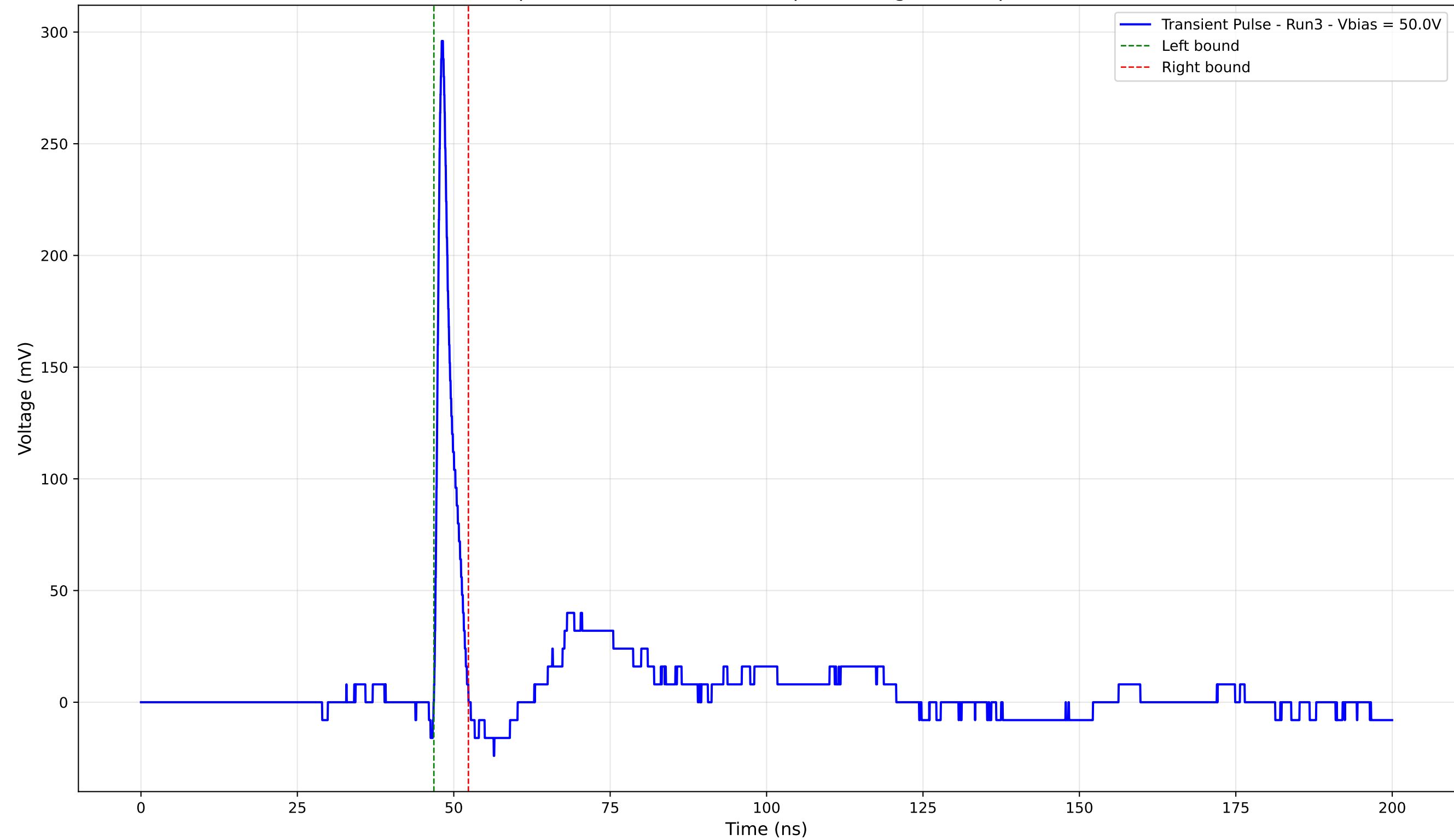
Transient Pulse - Sample: 4003 - Position: 250.0 \mu\text{m} - Charge: 14.20 pC - Rise Time: 0.87 ns
