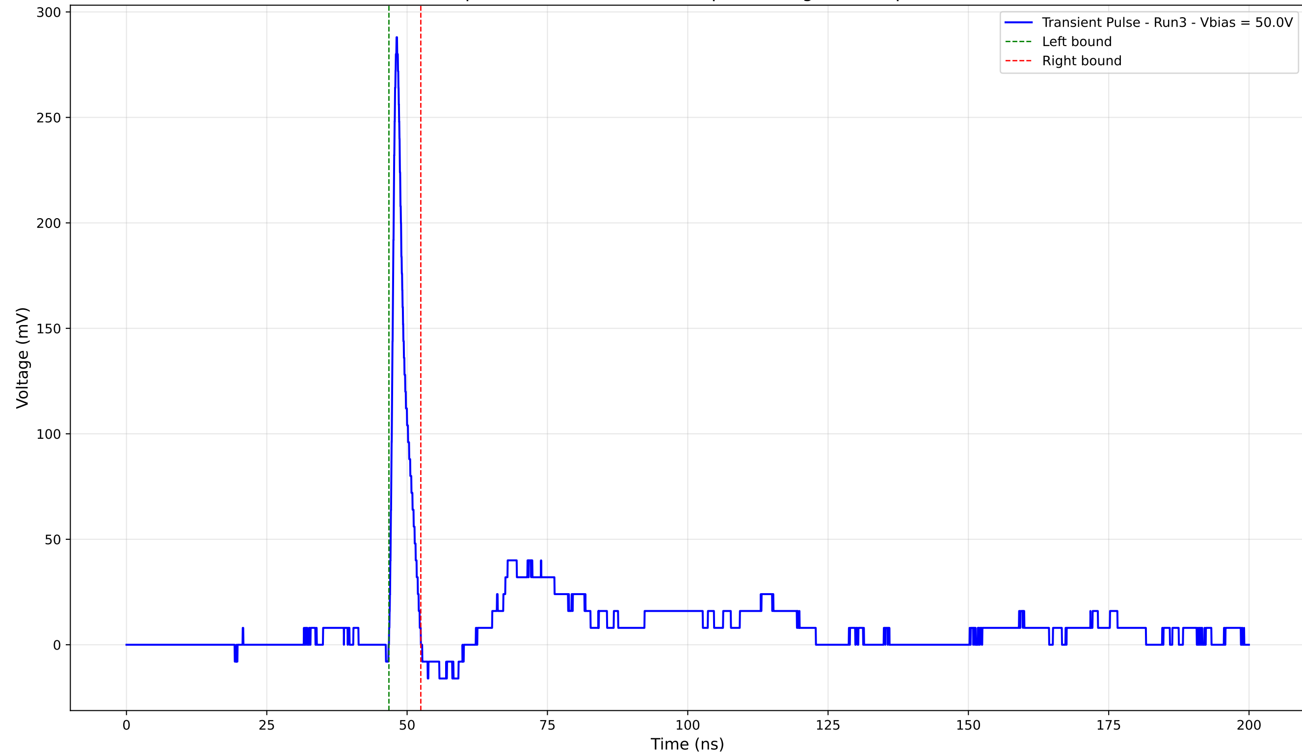
Transient Pulse - Sample: 4003 - Position: 240.0 \mu\text{m} - Charge: 13.89 pC - Rise Time: 0.89 ns
