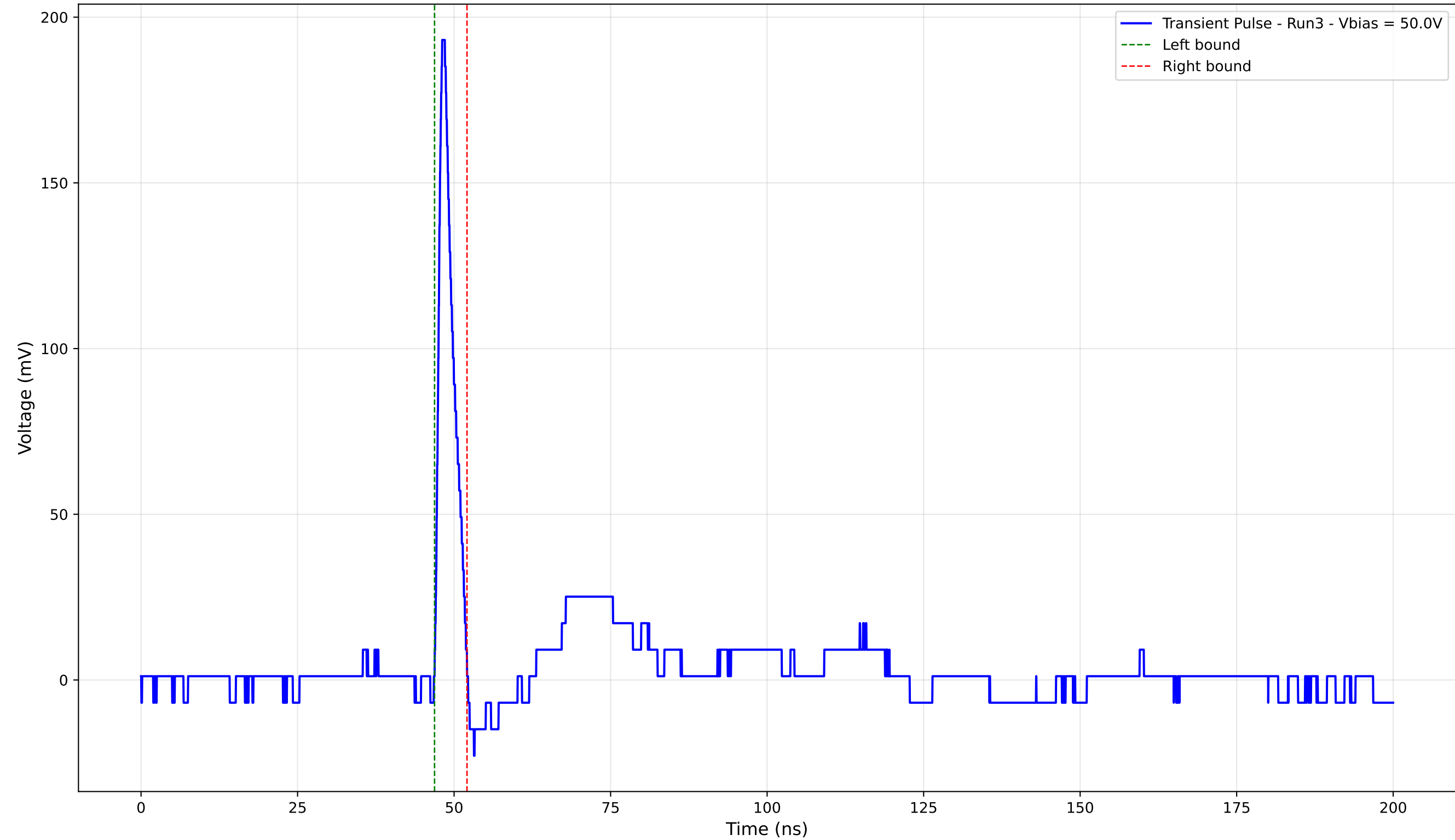
Transient Pulse - Sample: 4003 - Position: 505.0 \mu\text{m} - Charge: 10.14 pC - Rise Time: 0.87 ns
