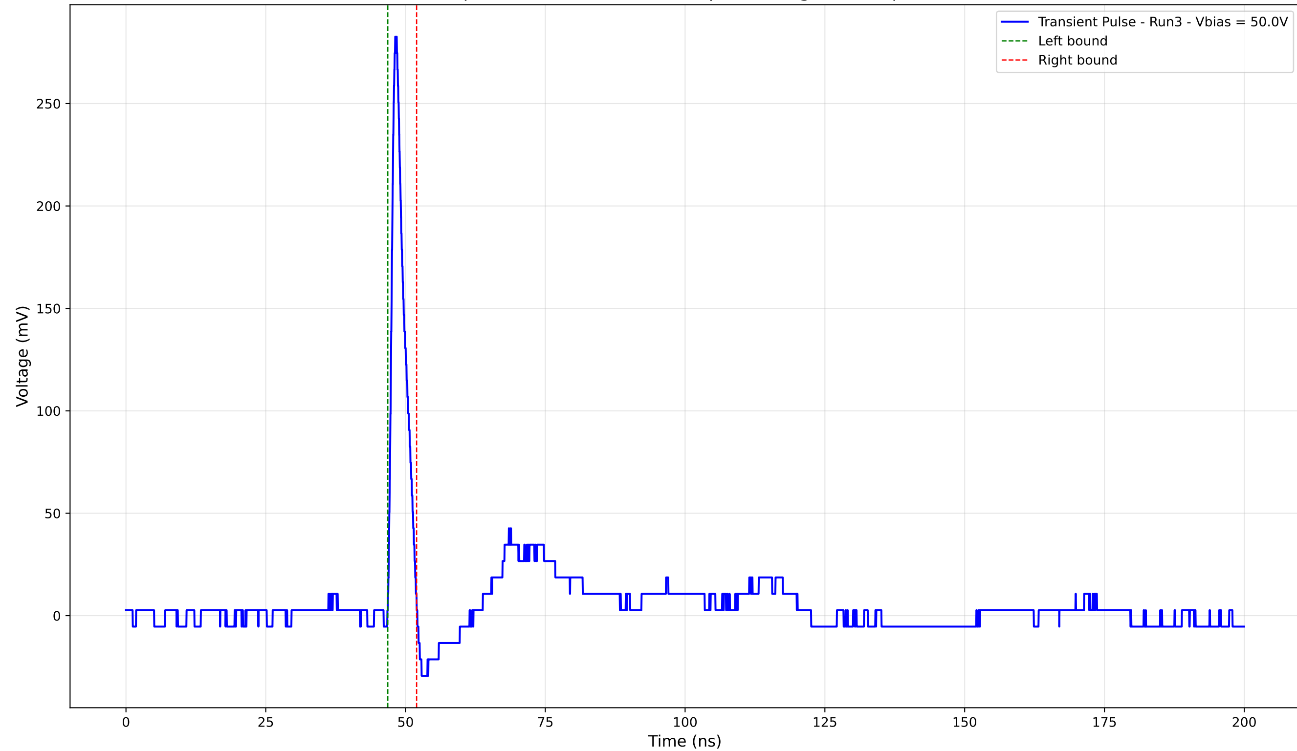
Transient Pulse - Sample: 4003 - Position: 435.0 \mu\text{m} - Charge: 14.40 pC - Rise Time: 0.92 ns
