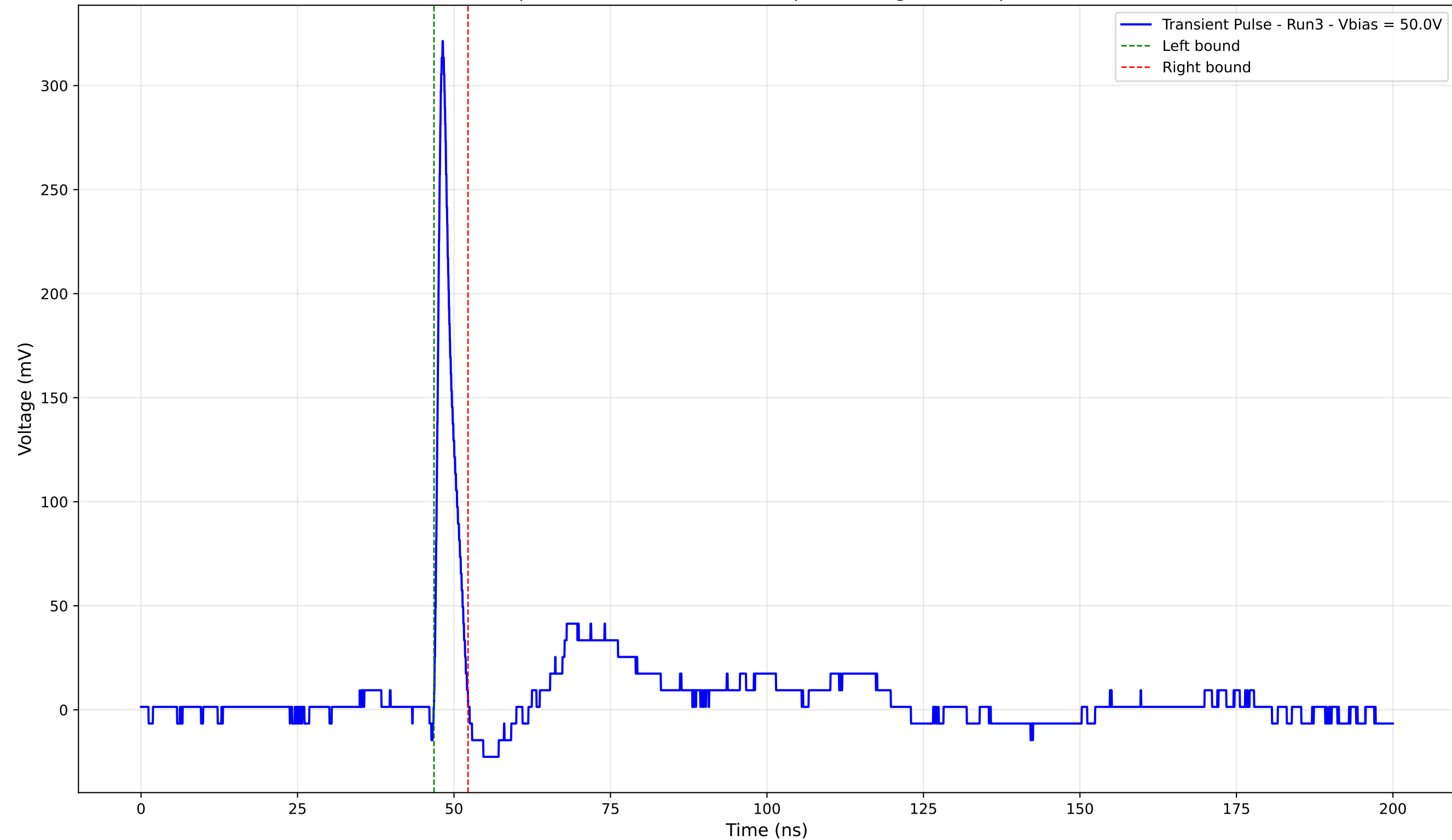
Transient Pulse - Sample: 4003 - Position: 280.0 \mu\text{m} - Charge: 15.69 pC - Rise Time: 0.88 ns
