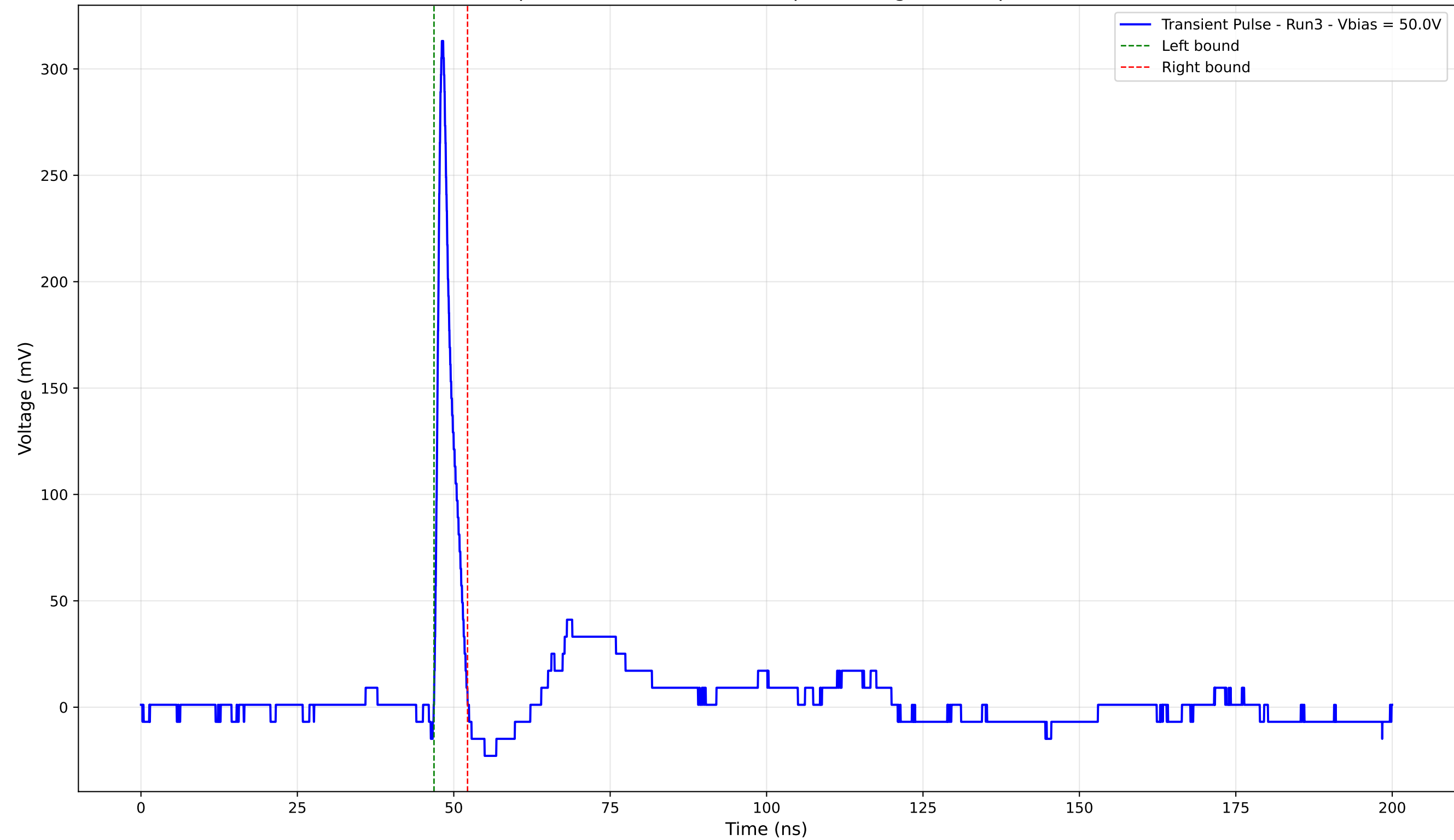
Transient Pulse - Sample: 4003 - Position: 275.0 \mu\text{m} - Charge: 15.23 pC - Rise Time: 0.88 ns
