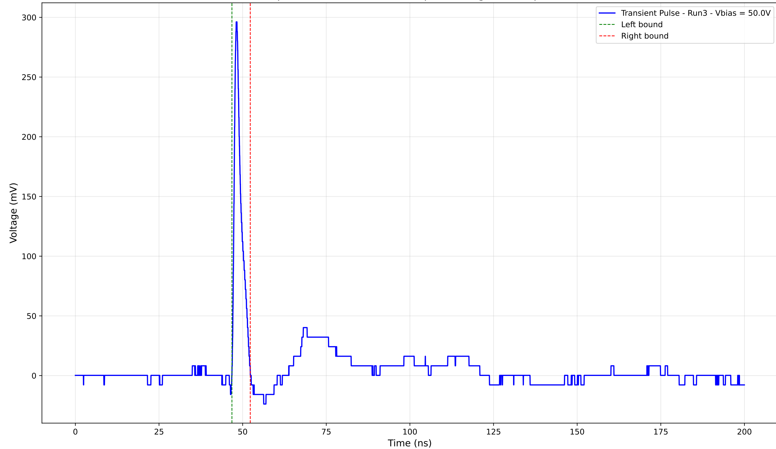
Transient Pulse - Sample: 4003 - Position: 255.0 \mu\text{m} - Charge: 14.27 pC - Rise Time: 0.89 ns
