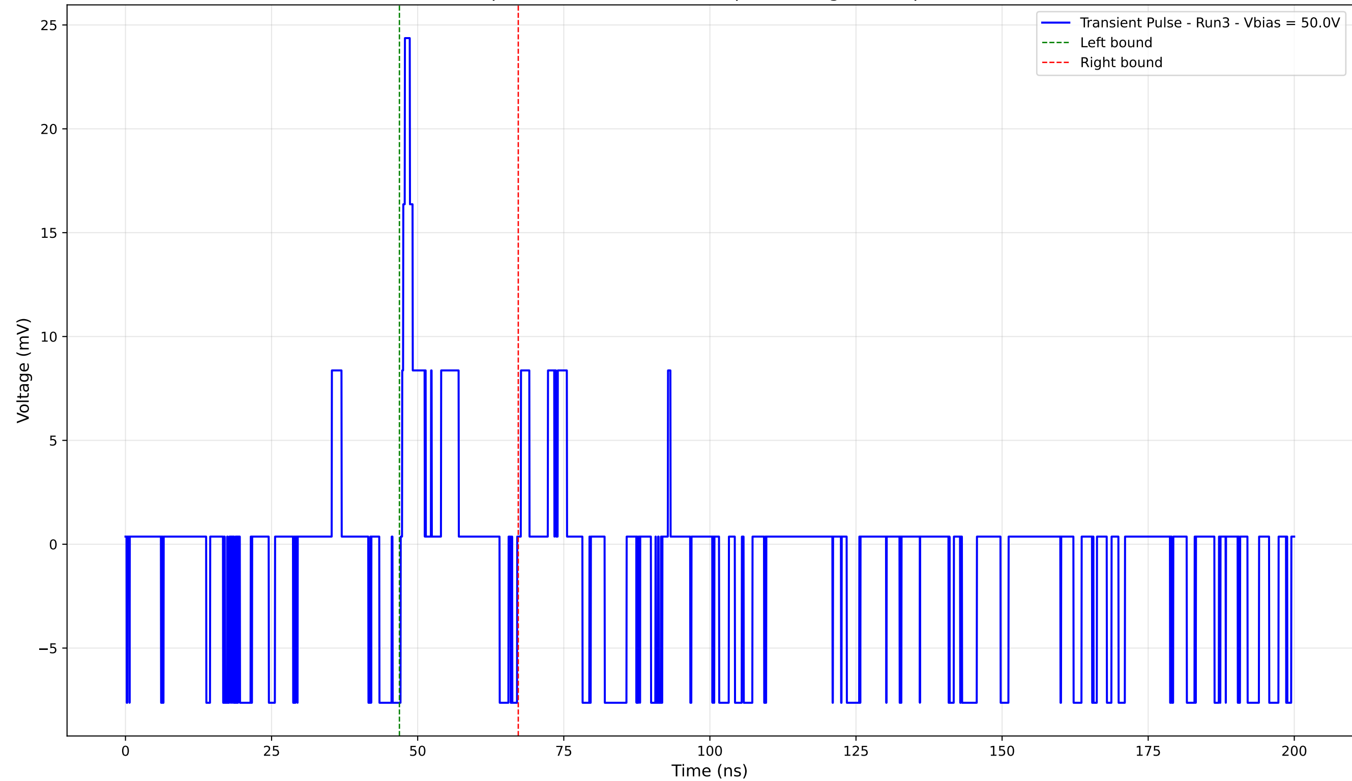
Transient Pulse - Sample: 4003 - Position: 30.0 \mu\text{m} - Charge: 1.25 pC - Rise Time: 0.47 ns
