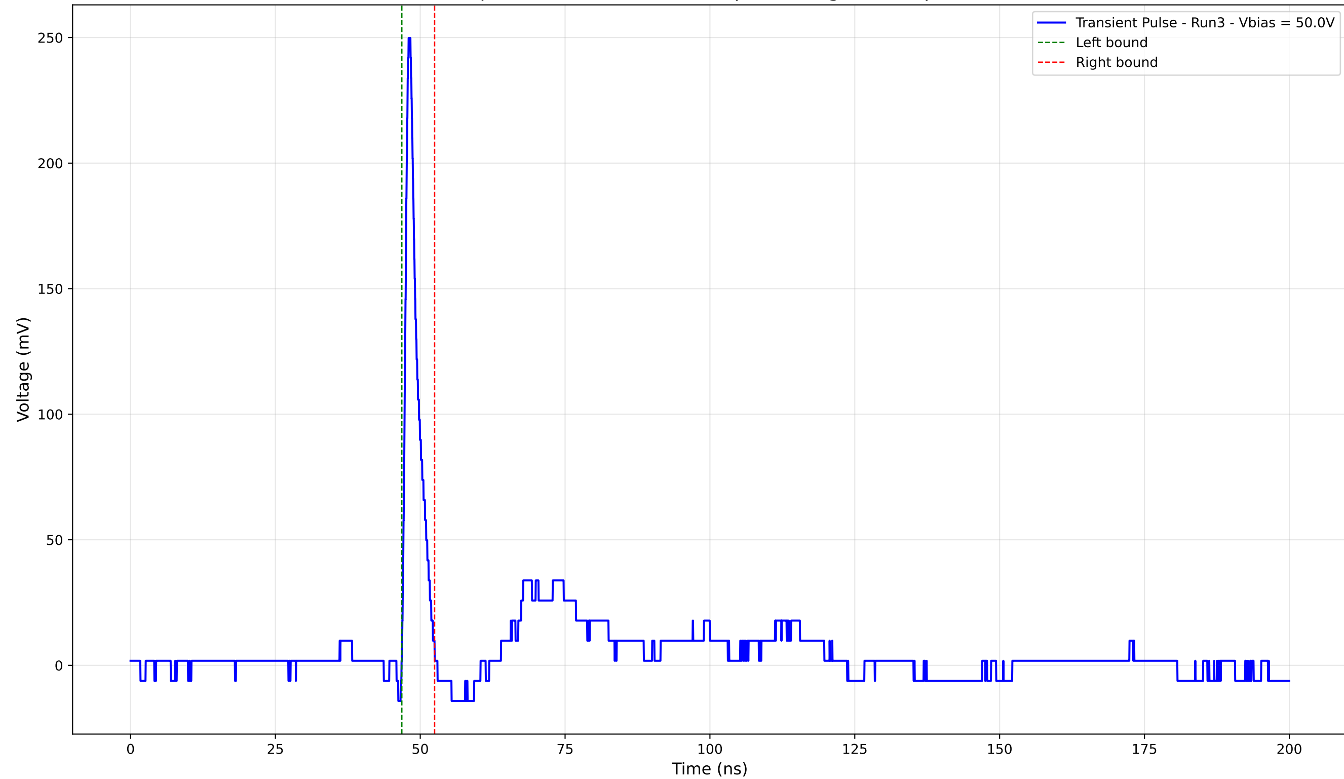
Transient Pulse - Sample: 4003 - Position: 215.0 \mu\text{m} - Charge: 12.07 pC - Rise Time: 0.84 ns
