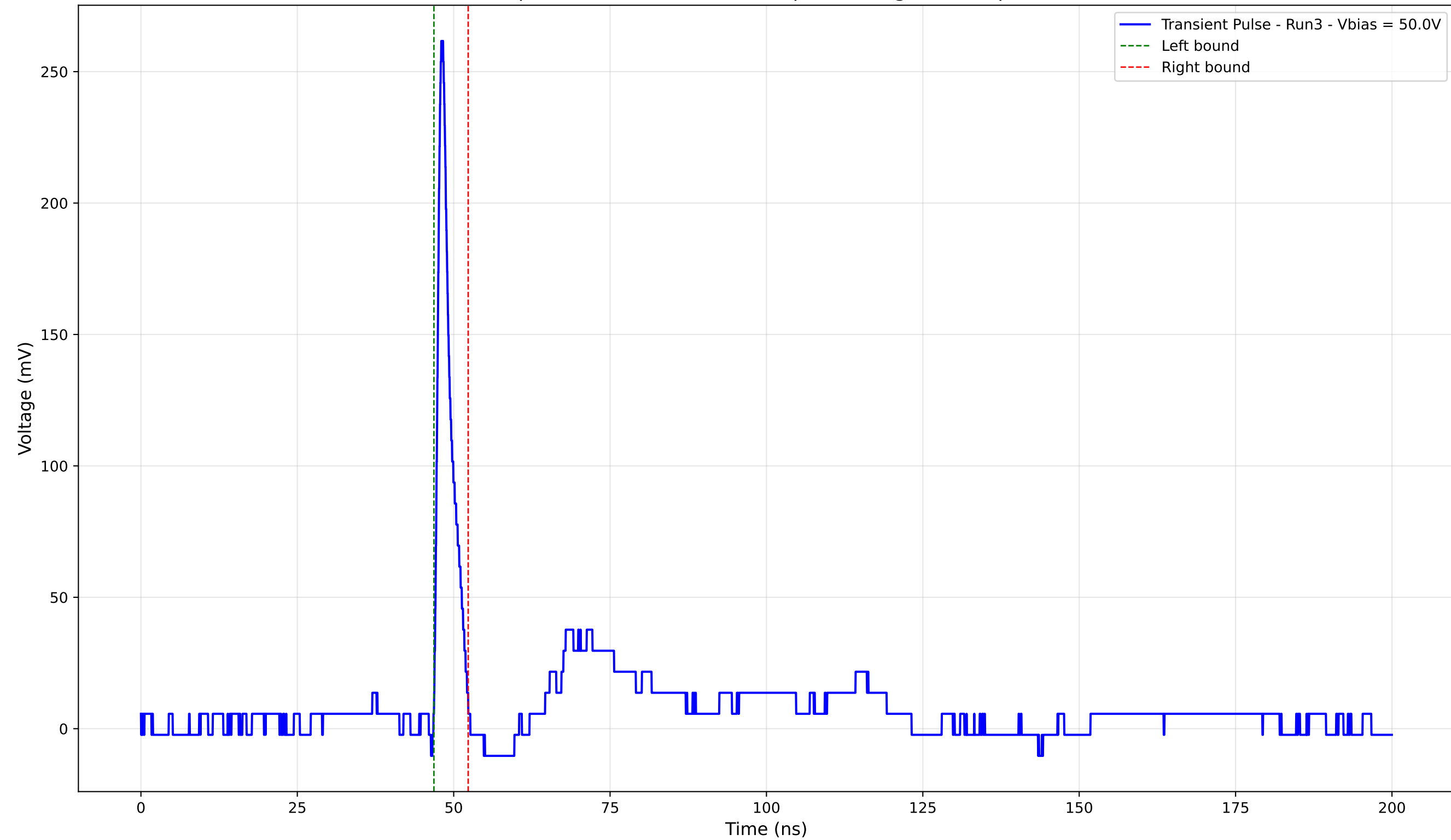
Transient Pulse - Sample: 4003 - Position: 220.0 \mu\text{m} - Charge: 12.71 pC - Rise Time: 0.87 ns
