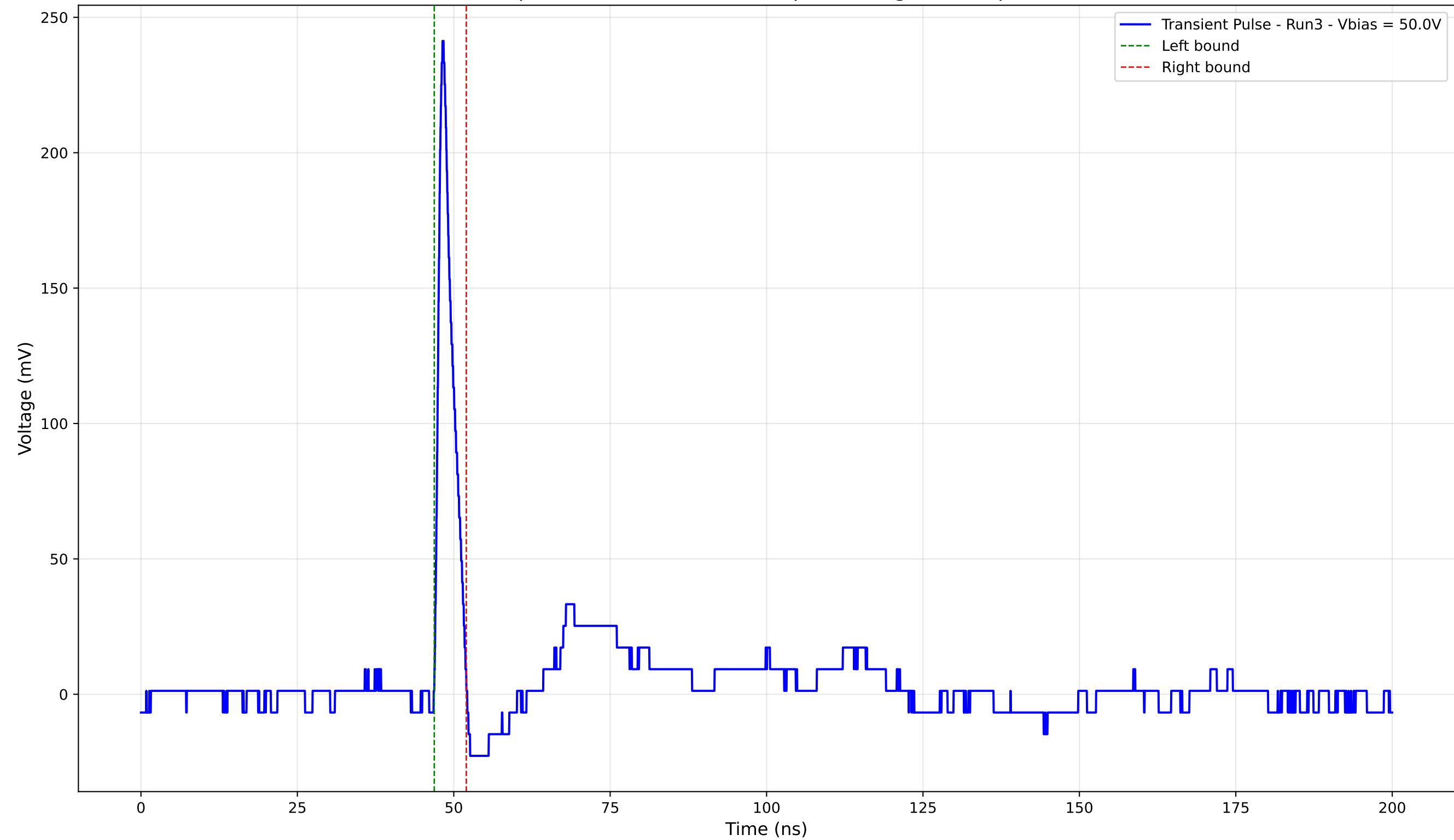
Transient Pulse - Sample: 4003 - Position: 470.0 \mu\text{m} - Charge: 12.23 pC - Rise Time: 0.90 ns
