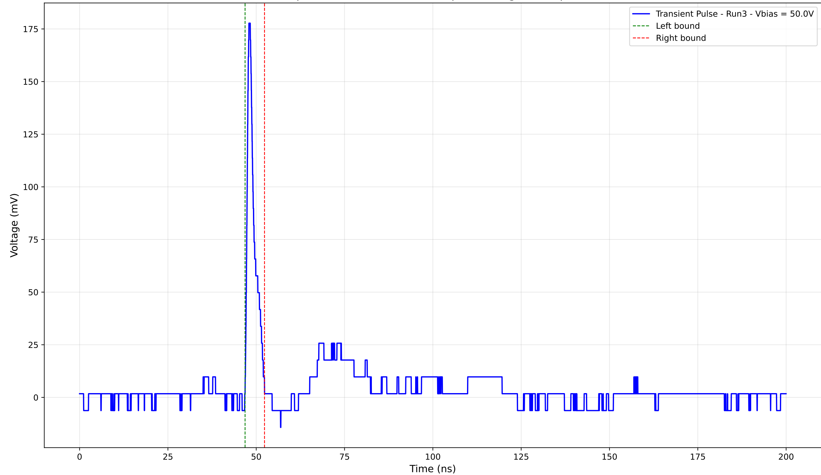
Transient Pulse - Sample: 4003 - Position: 165.0 \mu\text{m} - Charge: 8.46 pC - Rise Time: 0.78 ns
