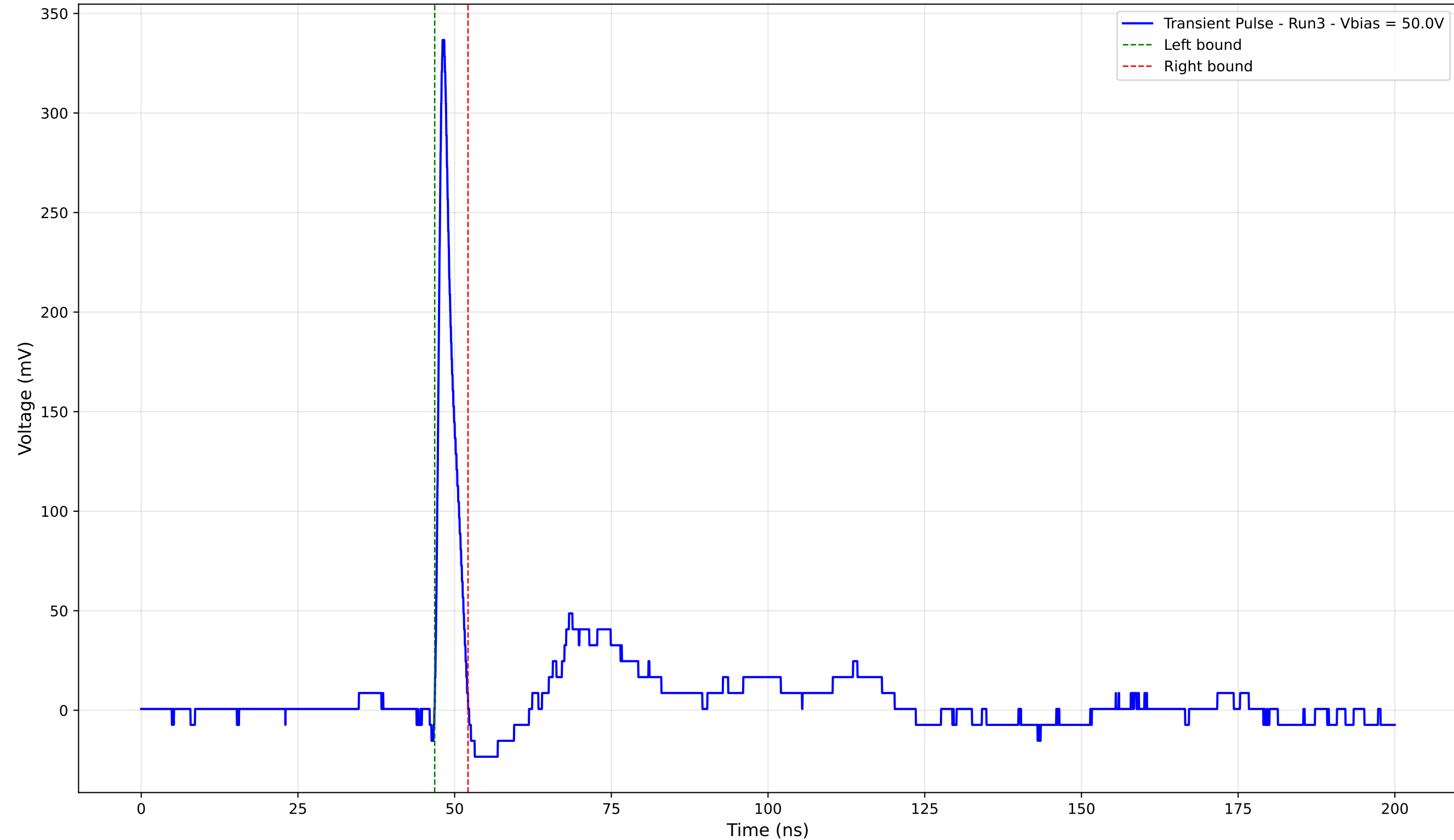
Transient Pulse - Sample: 4003 - Position: 320.0 \mu\text{m} - Charge: 16.79 pC - Rise Time: 0.86 ns
