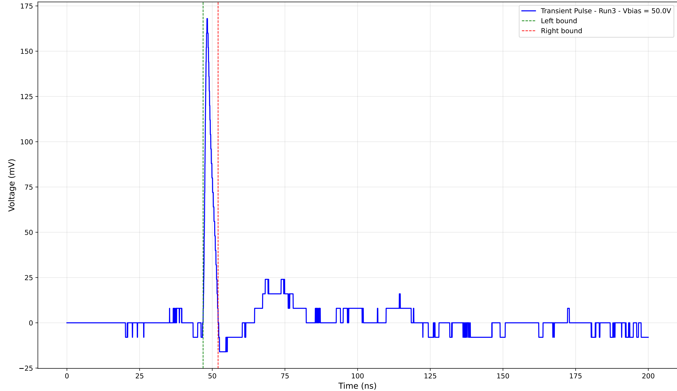
Transient Pulse - Sample: 4003 - Position: 545.0 \mu\text{m} - Charge: 8.63 pC - Rise Time: 0.90 ns
