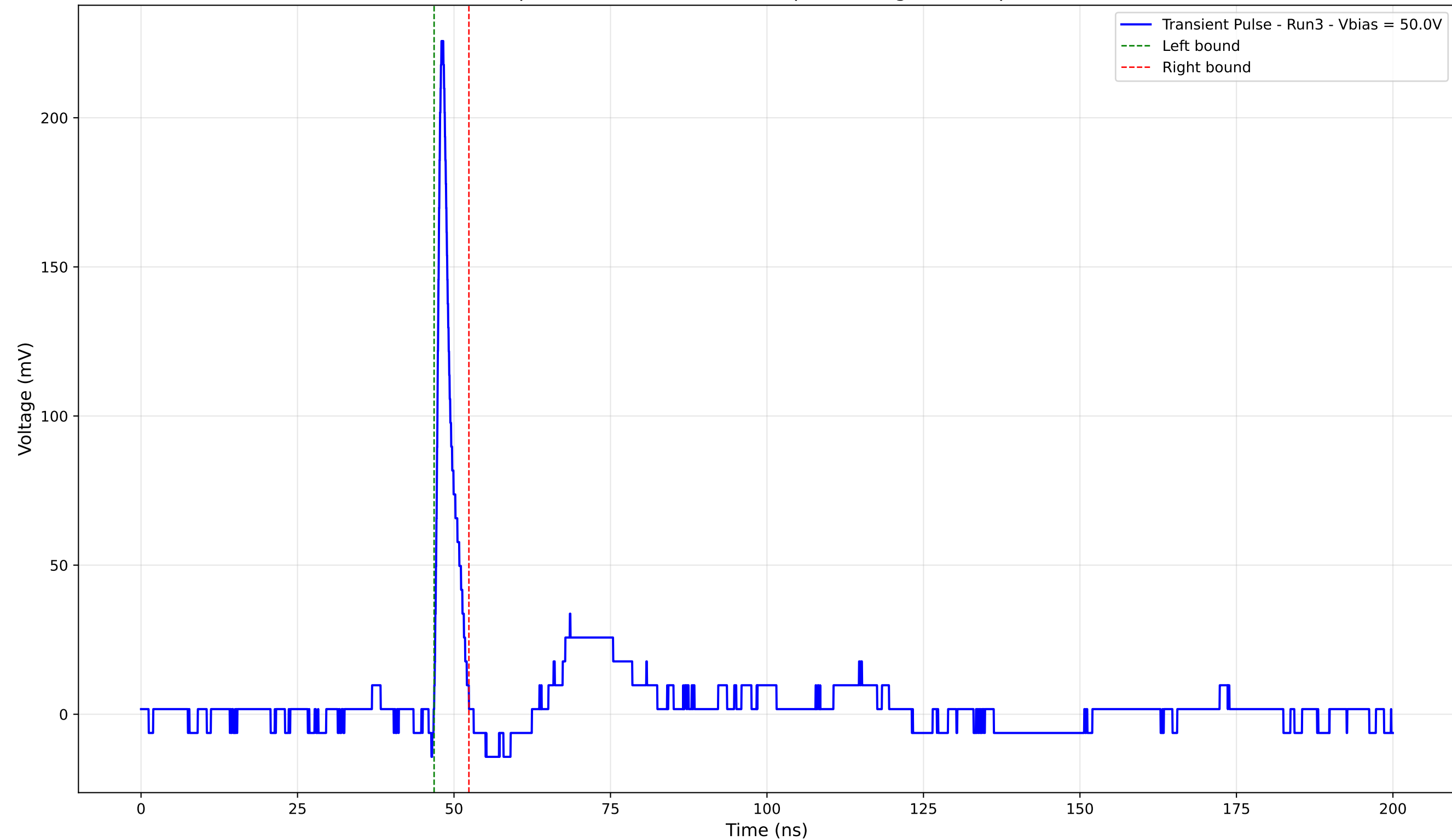
Transient Pulse - Sample: 4003 - Position: 195.0 \mu\text{m} - Charge: 10.59 pC - Rise Time: 0.87 ns
