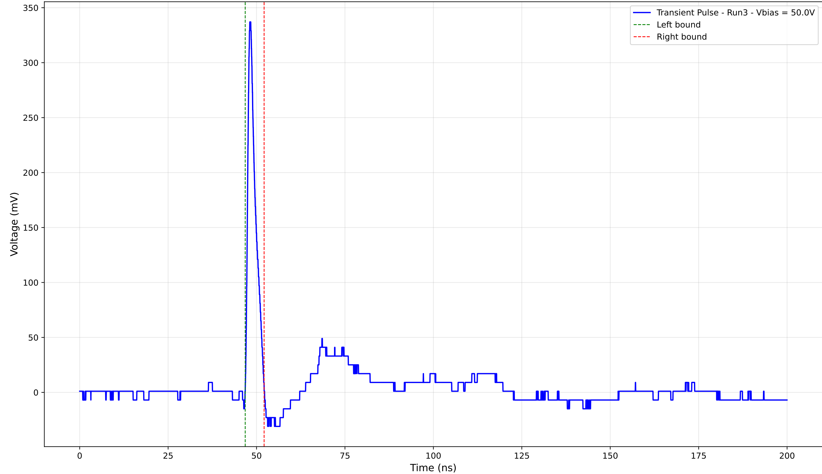
Transient Pulse - Sample: 4003 - Position: 330.0 \mu\text{m} - Charge: 16.97 pC - Rise Time: 0.86 ns
