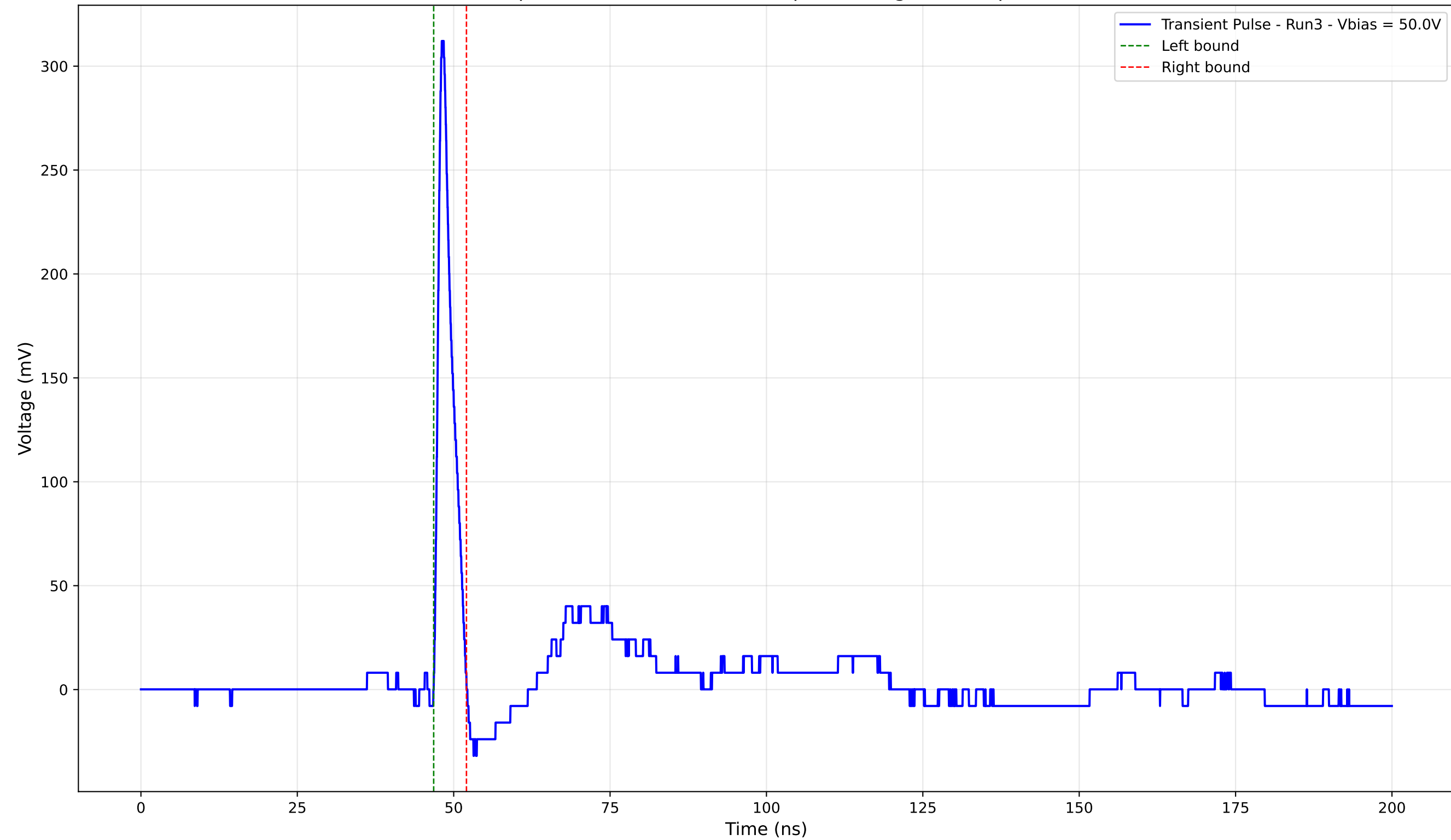
Transient Pulse - Sample: 4003 - Position: 400.0 \mu\text{m} - Charge: 15.86 pC - Rise Time: 0.90 ns
