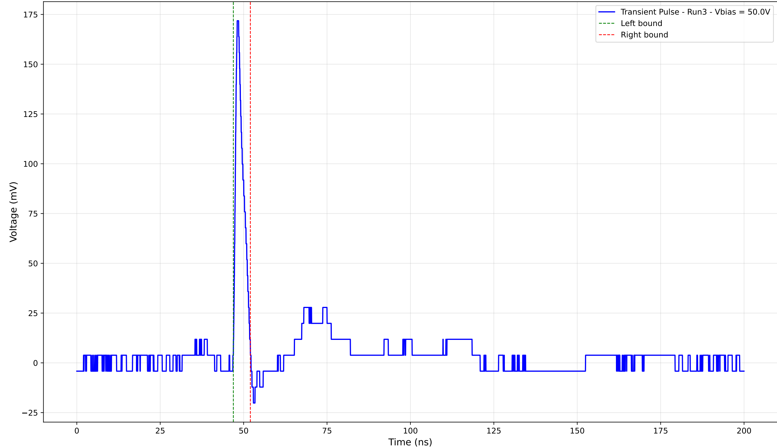
Transient Pulse - Sample: 4003 - Position: 590.0 \mu\text{m} - Charge: 9.26 pC - Rise Time: 0.89 ns
