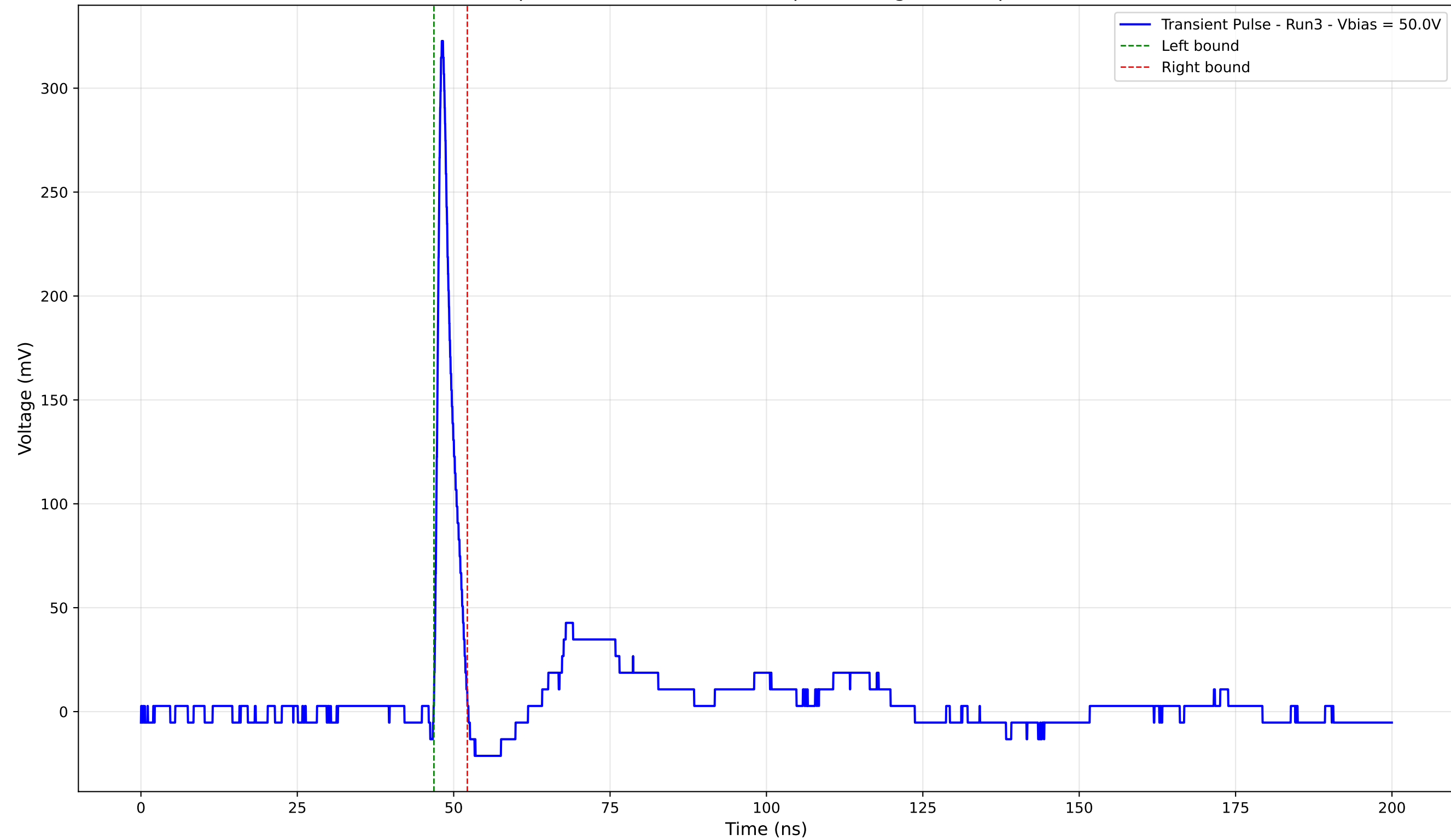
Transient Pulse - Sample: 4003 - Position: 290.0 \mu\text{m} - Charge: 15.86 pC - Rise Time: 0.85 ns
