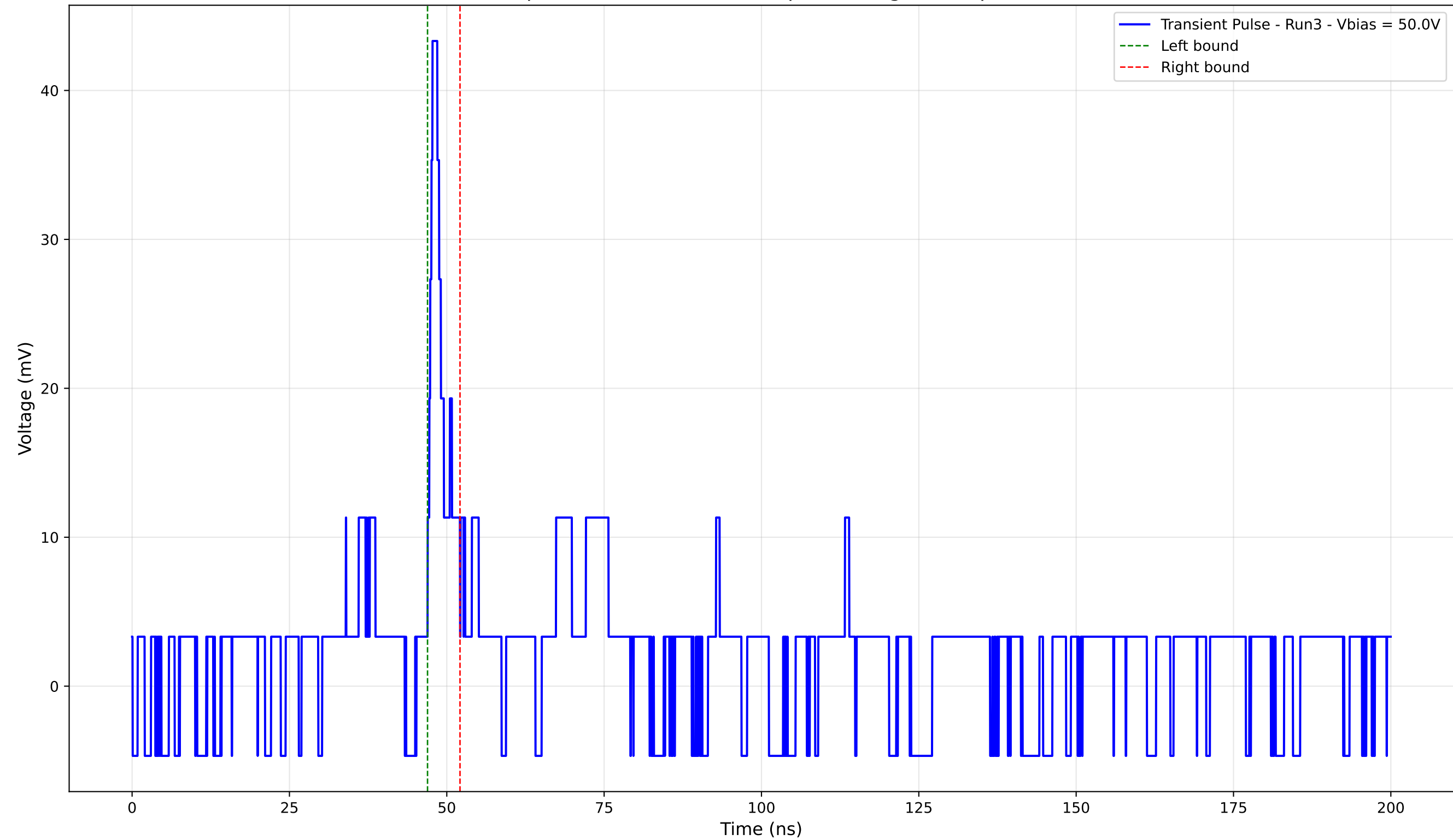
Transient Pulse - Sample: 4003 - Position: 55.0 \mu\text{m} - Charge: 2.18 pC - Rise Time: 0.78 ns
