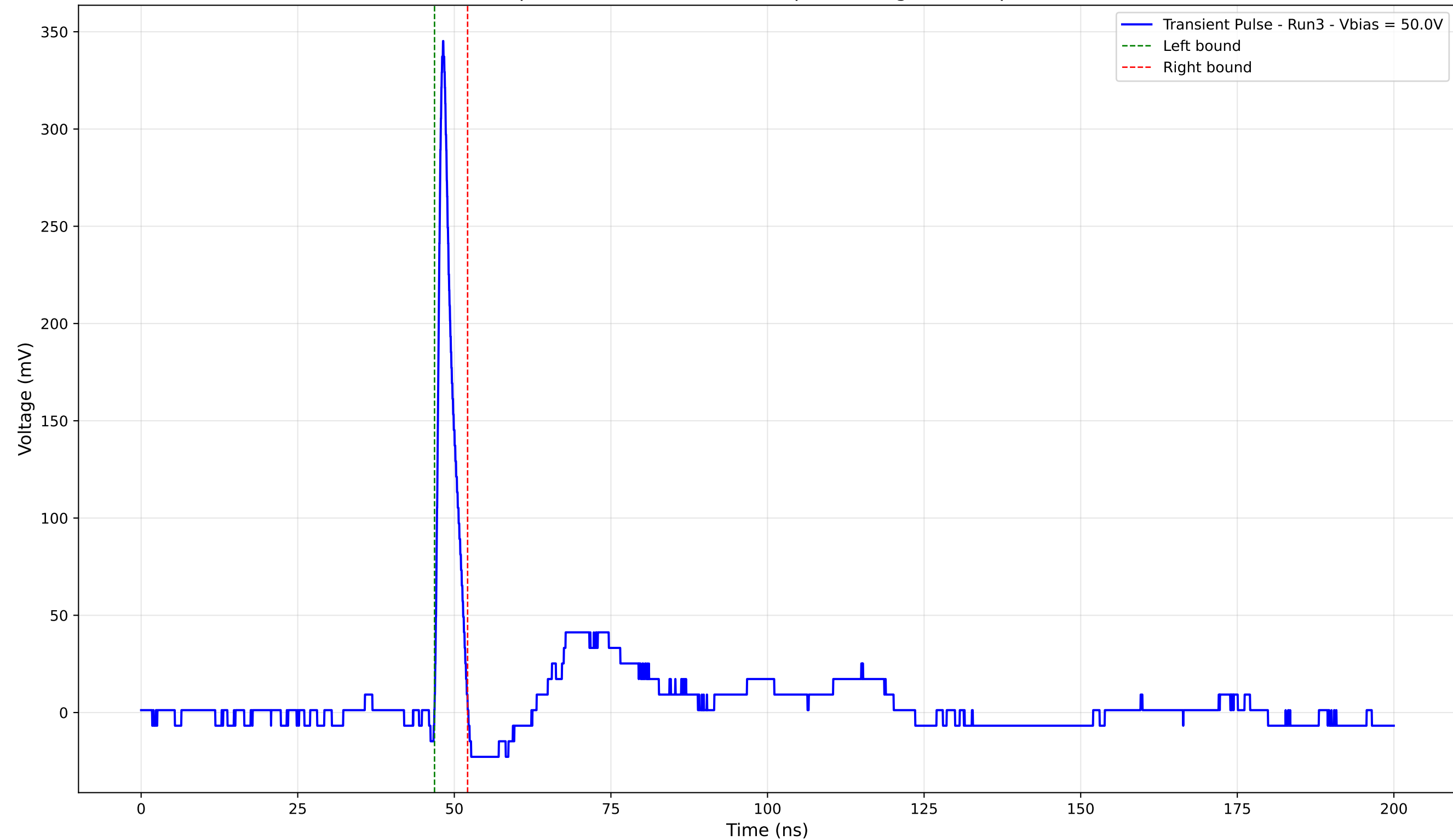
Transient Pulse - Sample: 4003 - Position: 335.0 \mu\text{m} - Charge: 16.93 pC - Rise Time: 0.90 ns
