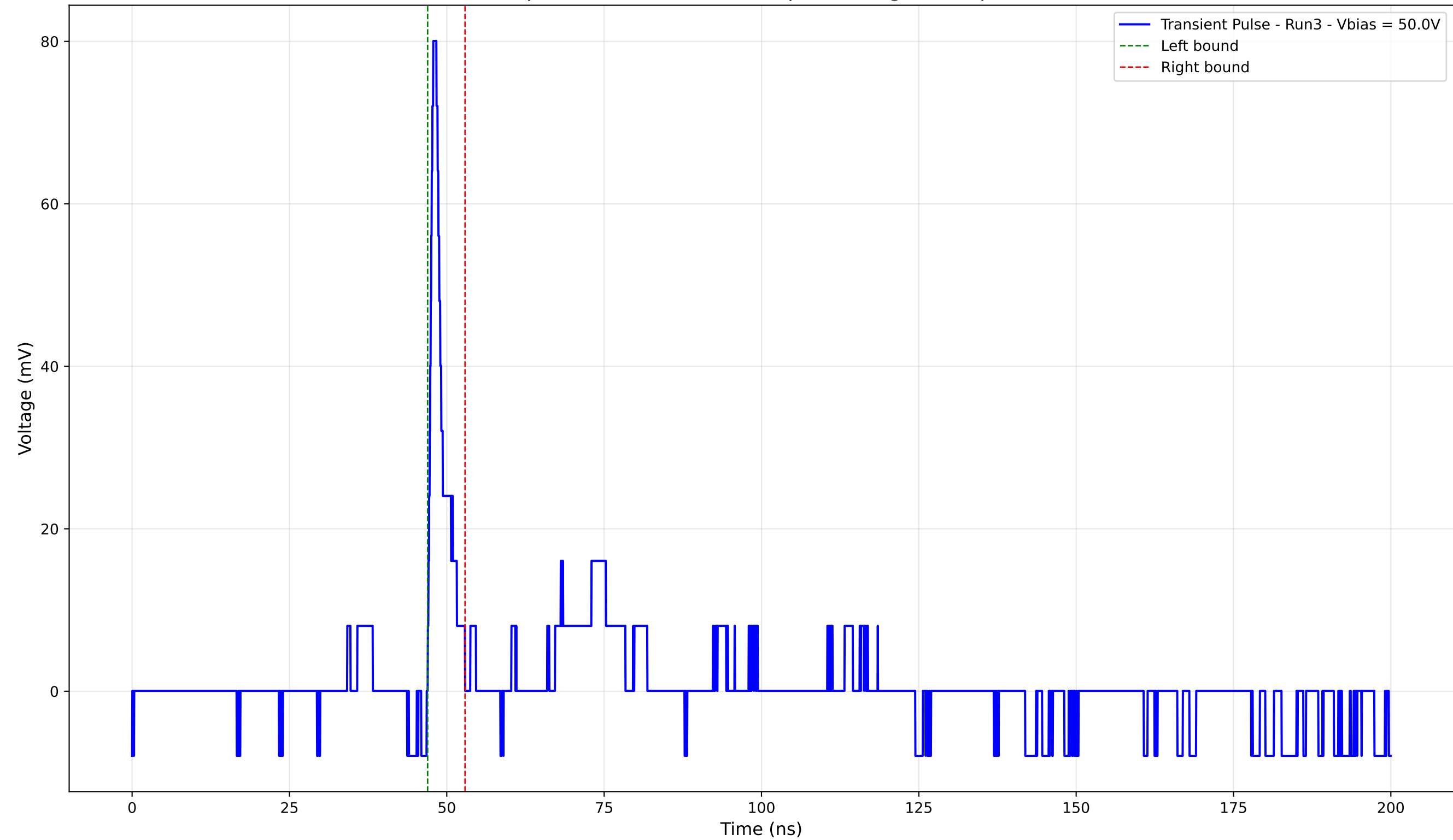
Transient Pulse - Sample: 4003 - Position: 90.0 \mu\text{m} - Charge: 3.71 pC - Rise Time: 0.72 ns
