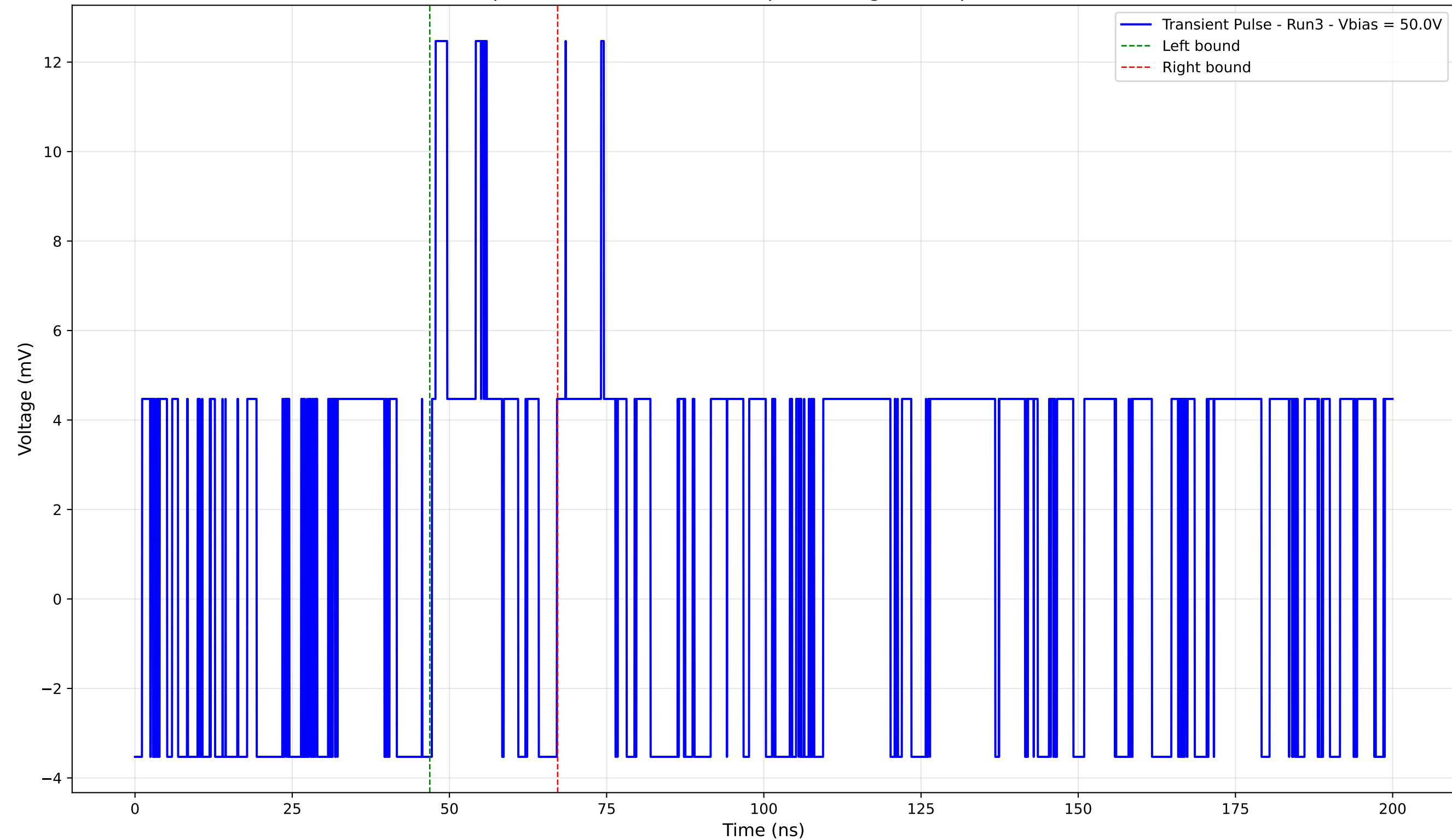
Transient Pulse - Sample: 4003 - Position: 625.0 \mu\text{m} - Charge: 1.59 pC - Rise Time: 0.00 ns (N/A)
