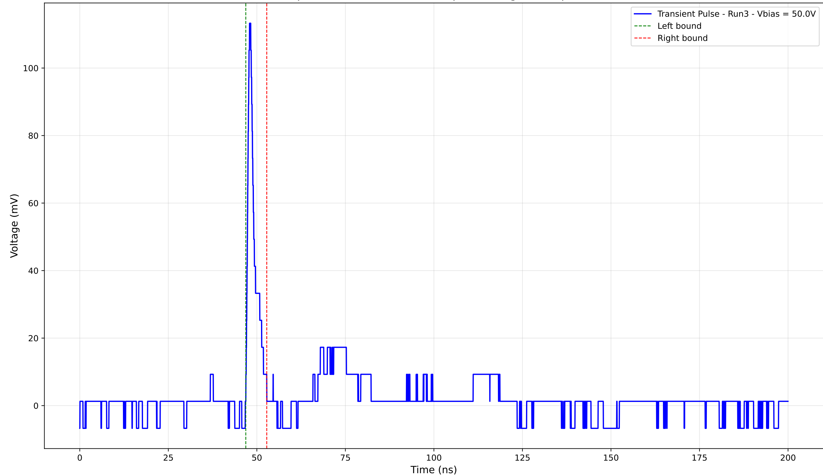
Transient Pulse - Sample: 4003 - Position: 115.0 \mu\text{m} - Charge: 5.26 pC - Rise Time: 0.79 ns
