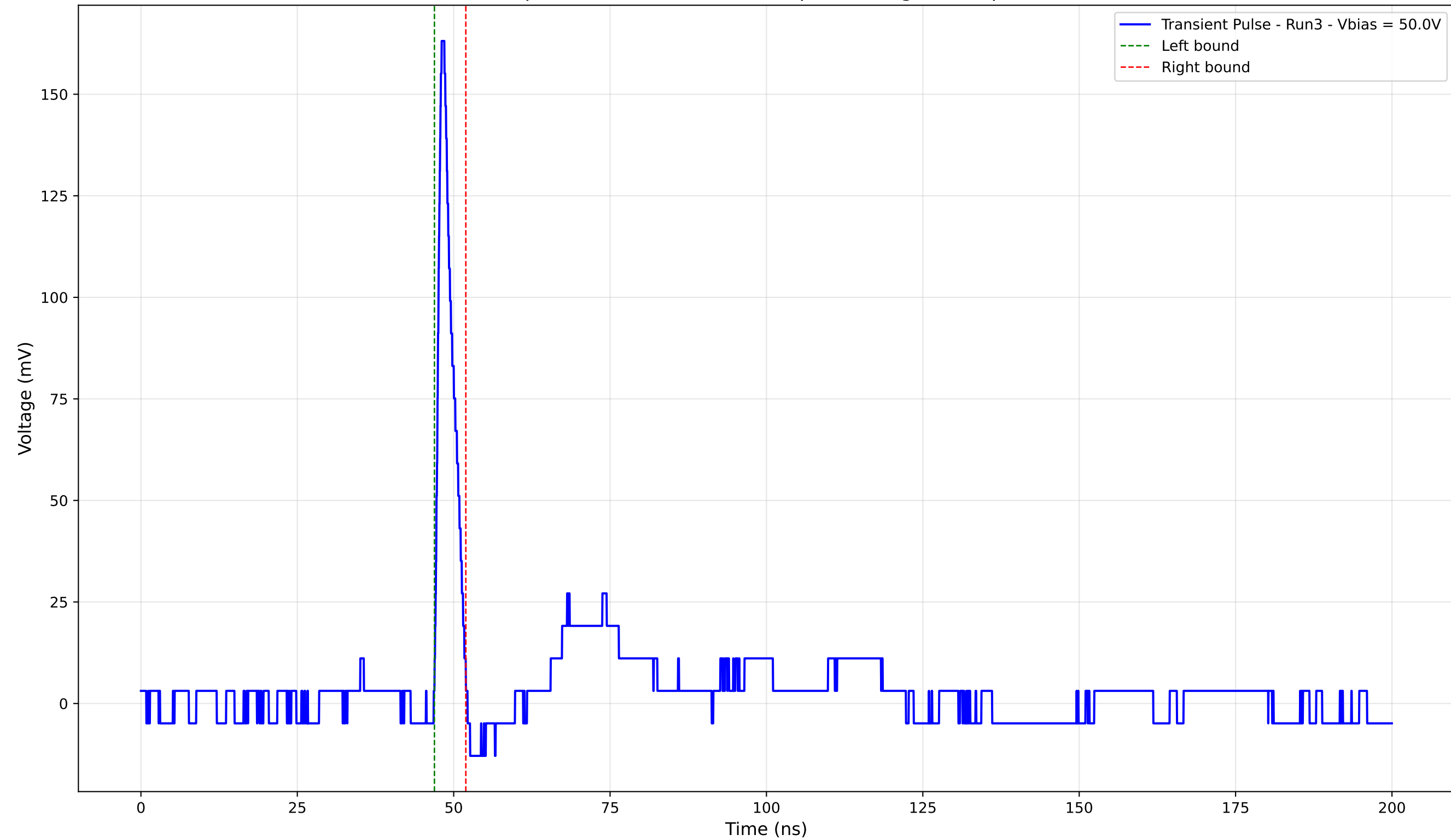
Transient Pulse - Sample: 4003 - Position: 595.0 \mu\text{m} - Charge: 8.50 pC - Rise Time: 0.87 ns
