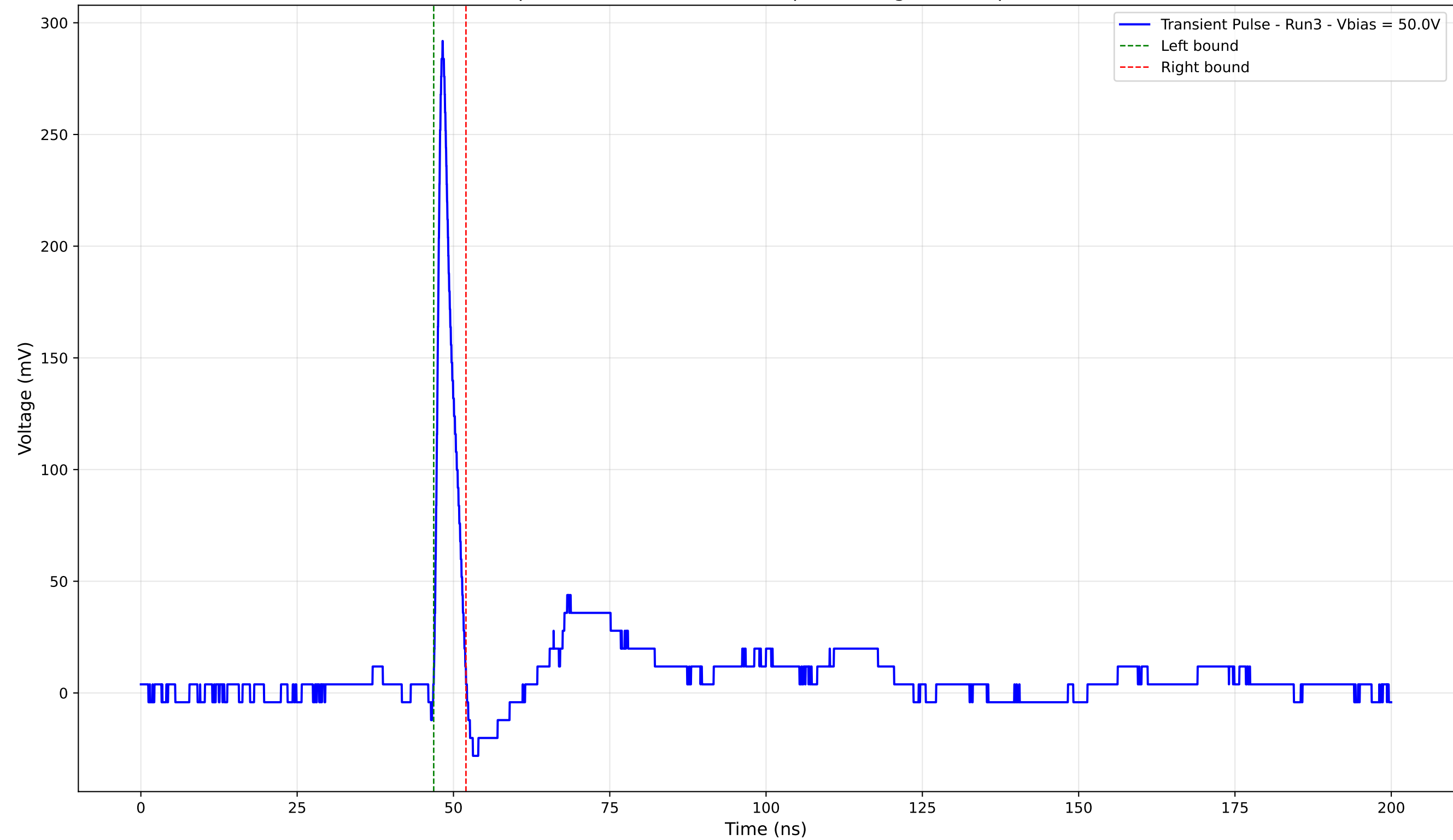
Transient Pulse - Sample: 4003 - Position: 430.0 \mu\text{m} - Charge: 14.70 pC - Rise Time: 0.96 ns
