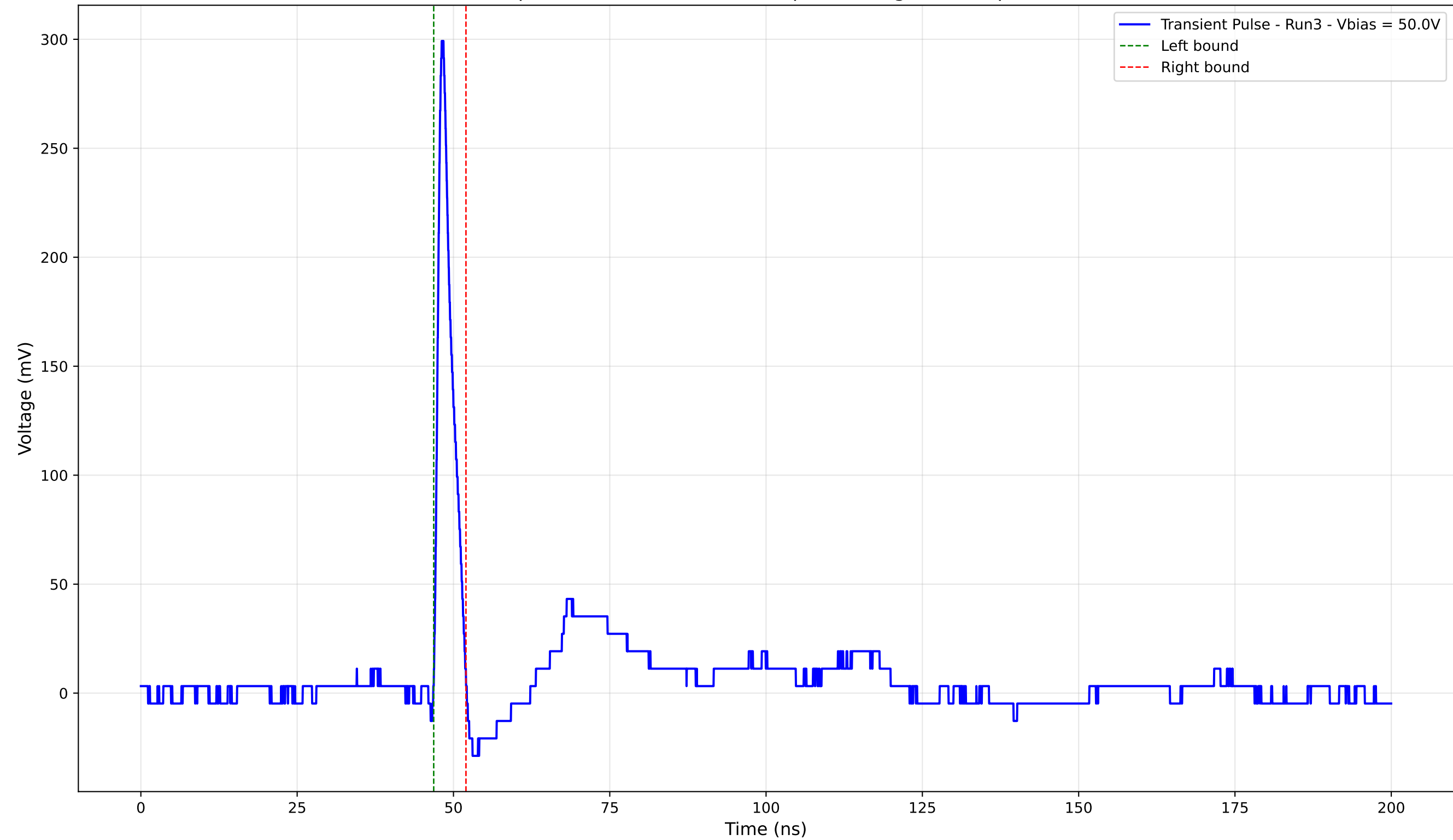
Transient Pulse - Sample: 4003 - Position: 420.0 \mu\text{m} - Charge: 15.21 pC - Rise Time: 0.91 ns
