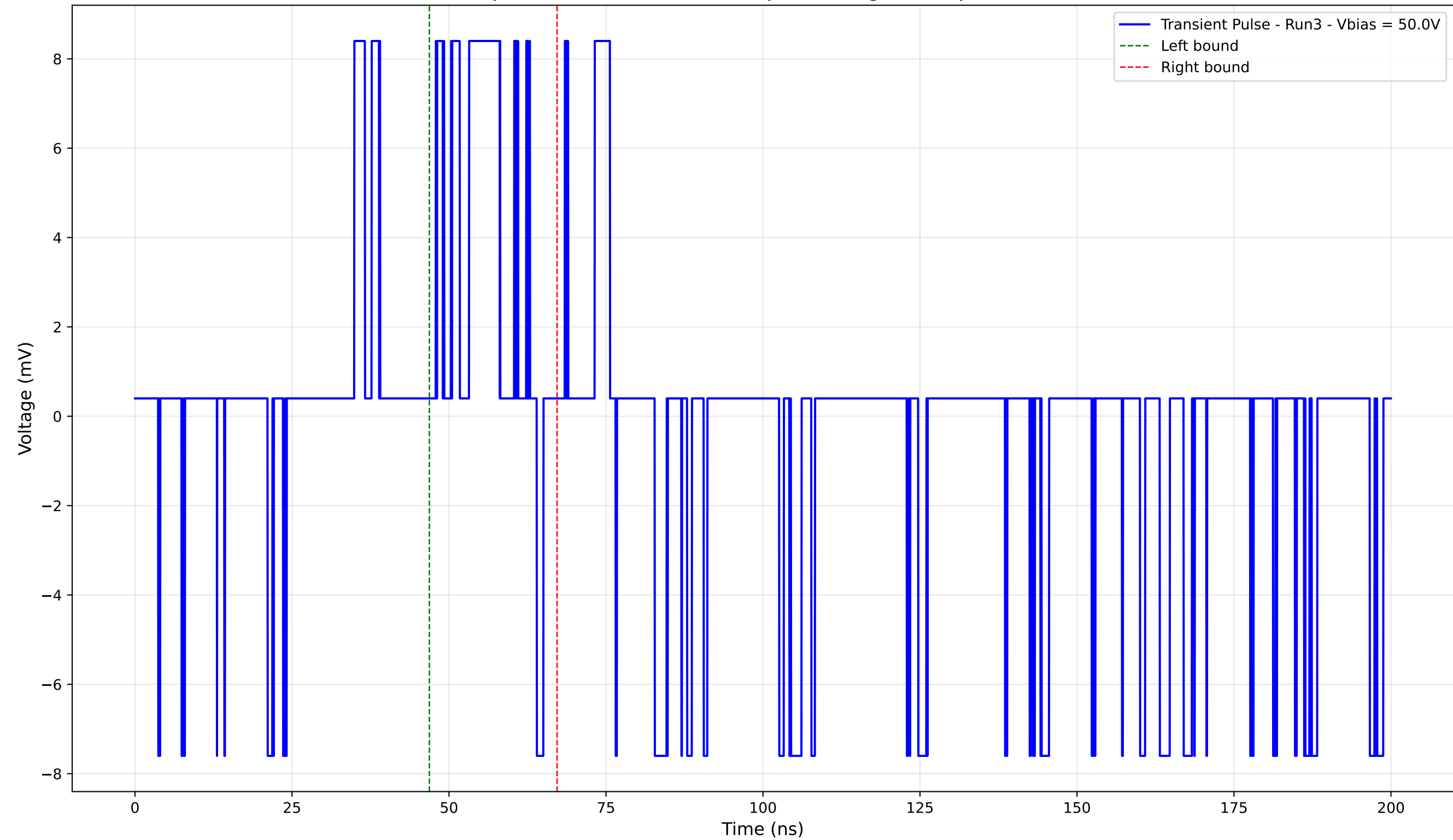
Transient Pulse - Sample: 4003 - Position: 650.0 \mu\text{m} - Charge: 1.30 pC - Rise Time: 0.00 ns (N/A)
