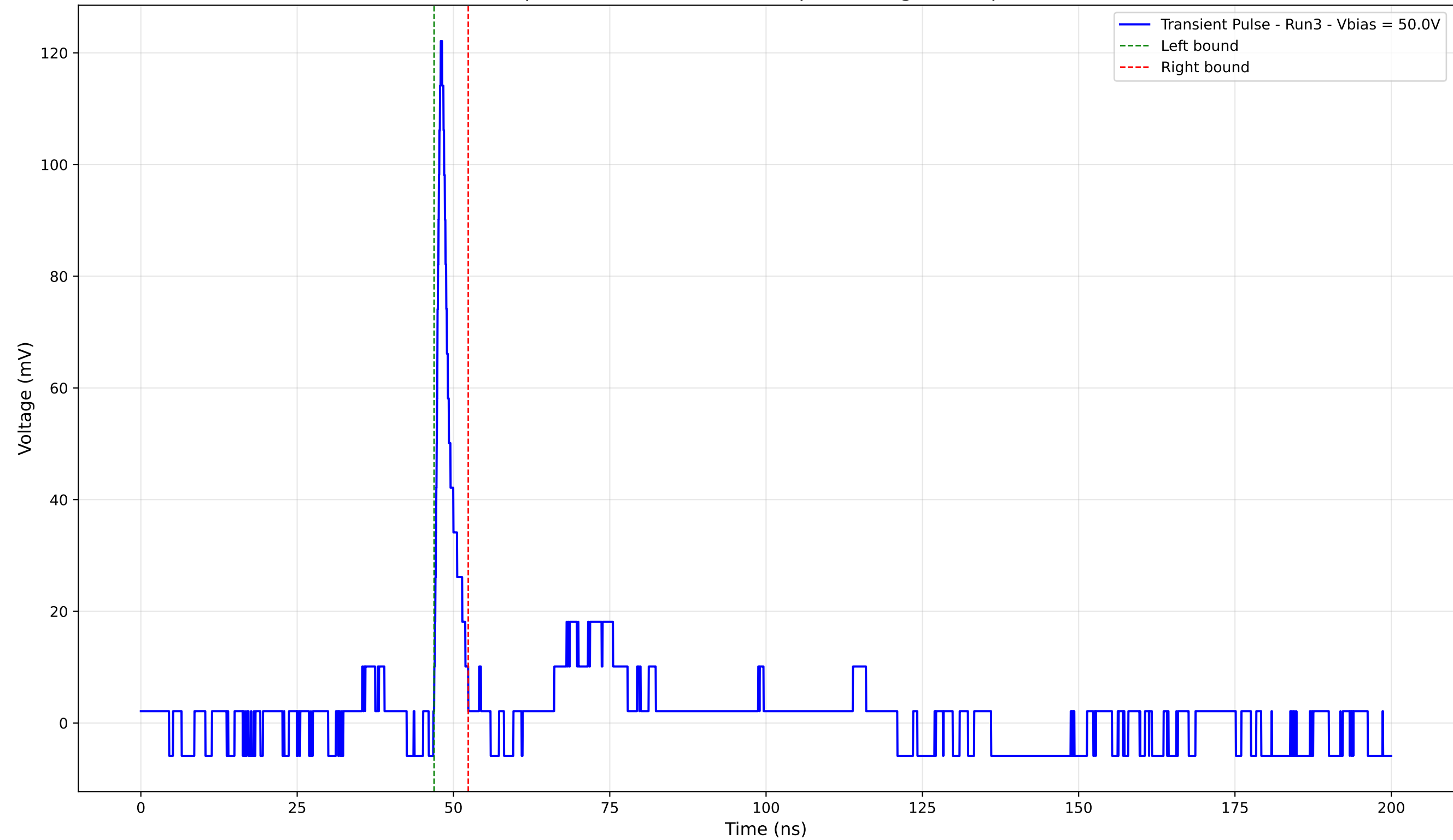
Transient Pulse - Sample: 4003 - Position: 120.0 \mu\text{m} - Charge: 5.51 pC - Rise Time: 0.83 ns
