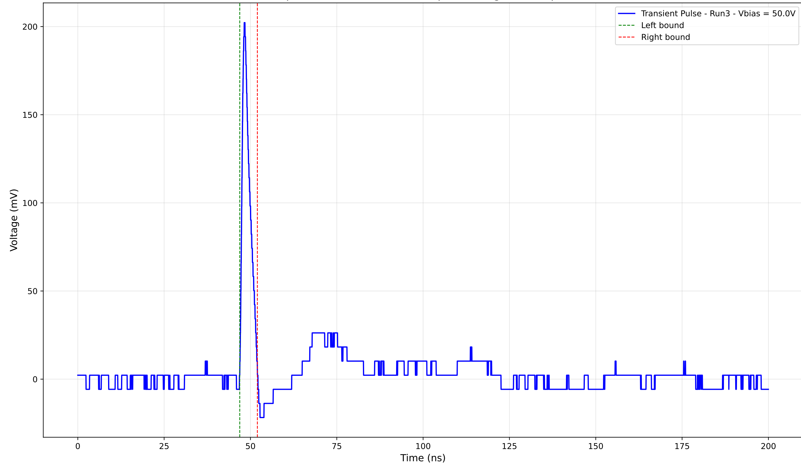
Transient Pulse - Sample: 4003 - Position: 500.0 \mu\text{m} - Charge: 10.32 pC - Rise Time: 0.92 ns
