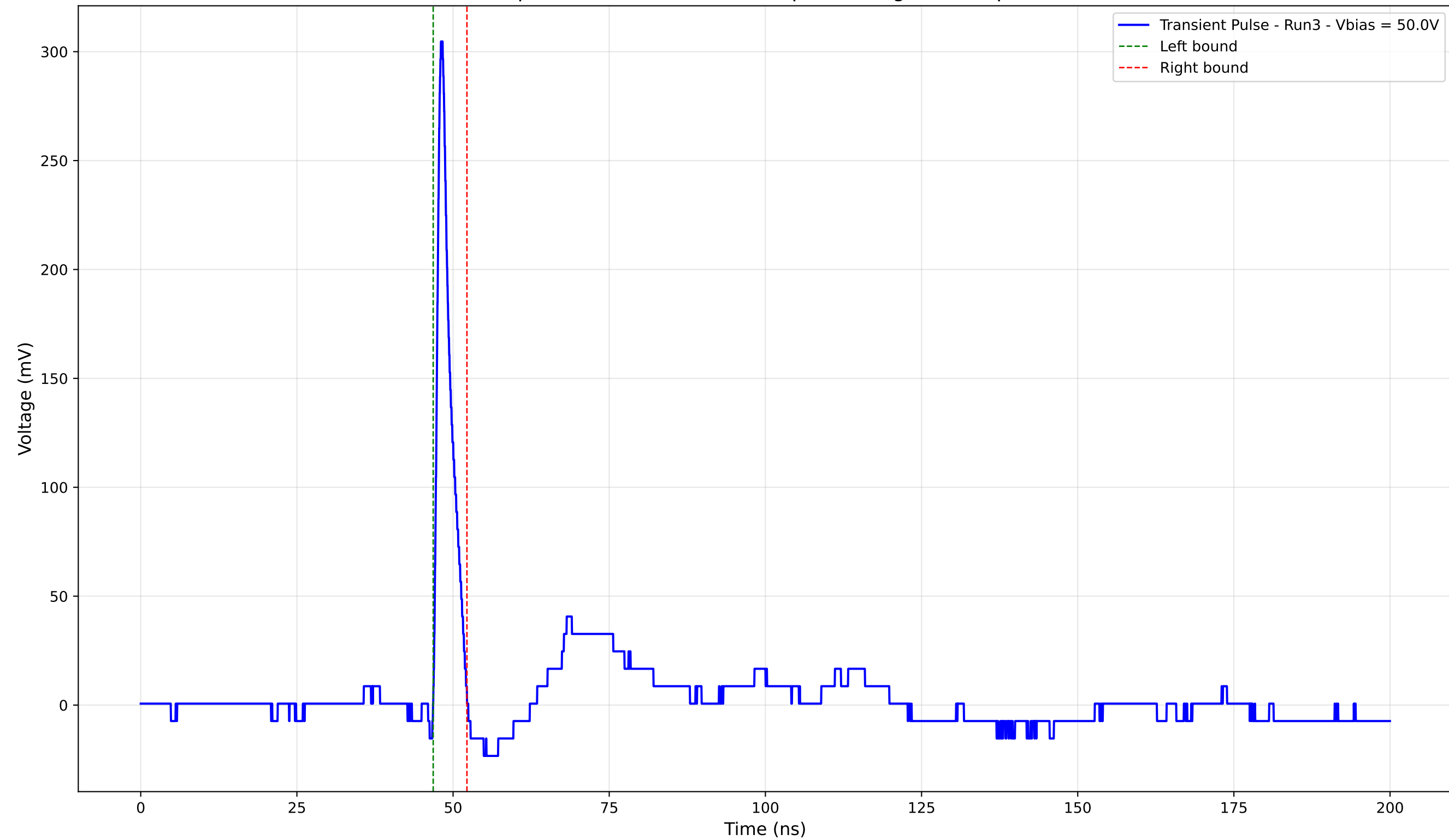
Transient Pulse - Sample: 4003 - Position: 265.0 \mu\text{m} - Charge: 14.81 pC - Rise Time: 0.87 ns
