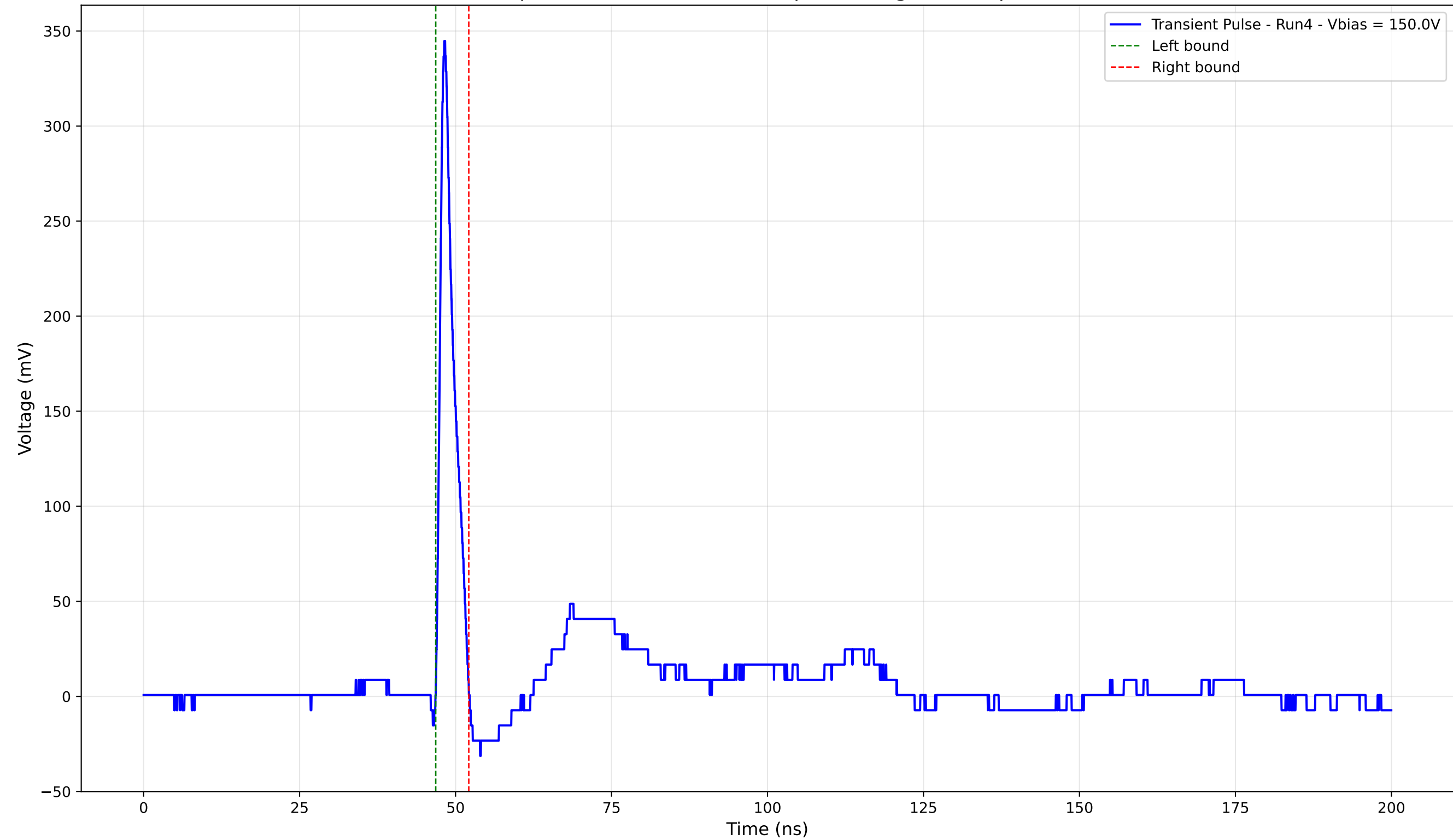
Transient Pulse - Sample: 4003 - Position: 365.0 \mu\text{m} - Charge: 17.41 pC - Rise Time: 0.90 ns
