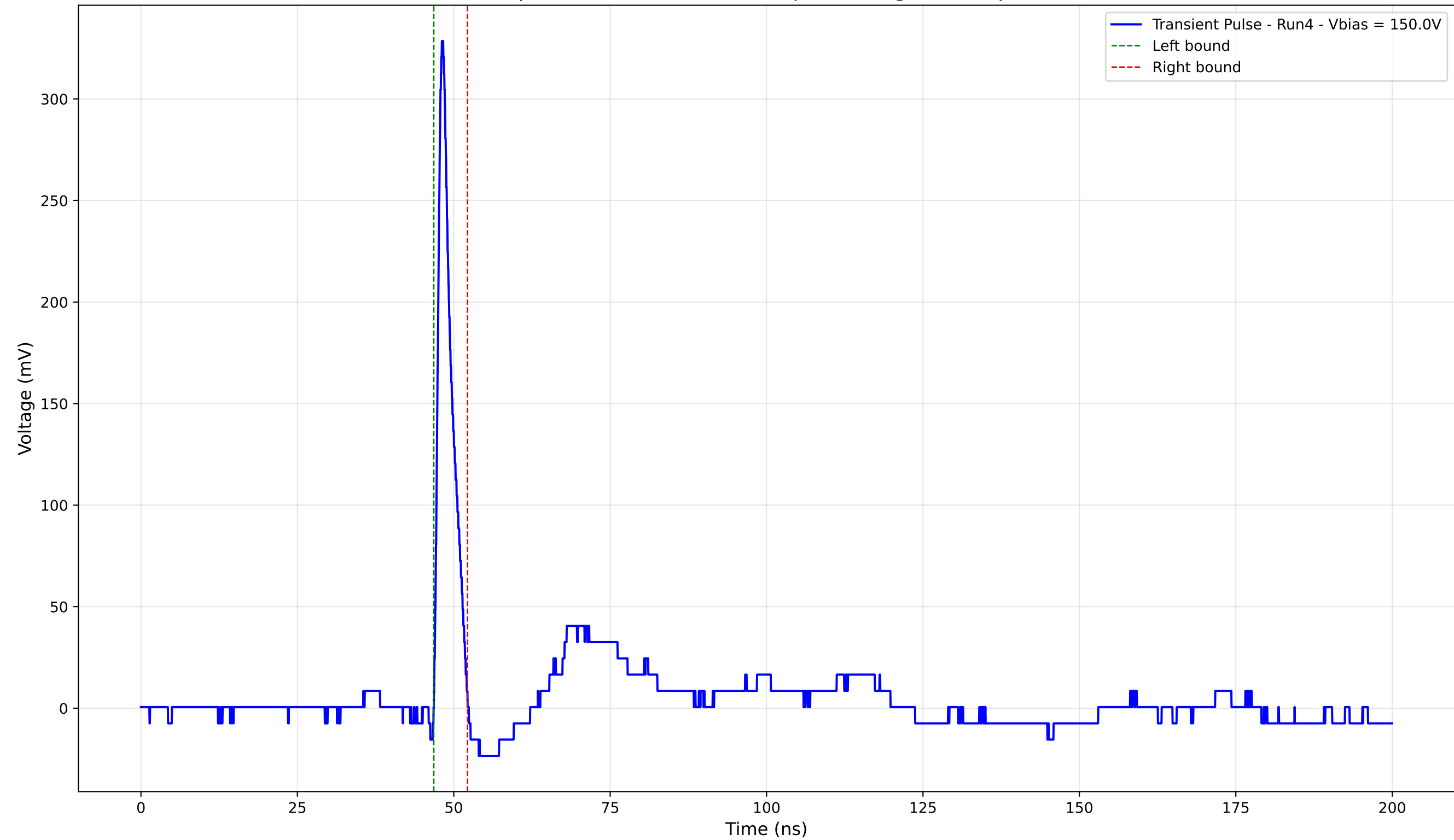
Transient Pulse - Sample: 4003 - Position: 290.0 \mu\text{m} - Charge: 16.28 pC - Rise Time: 0.84 ns
