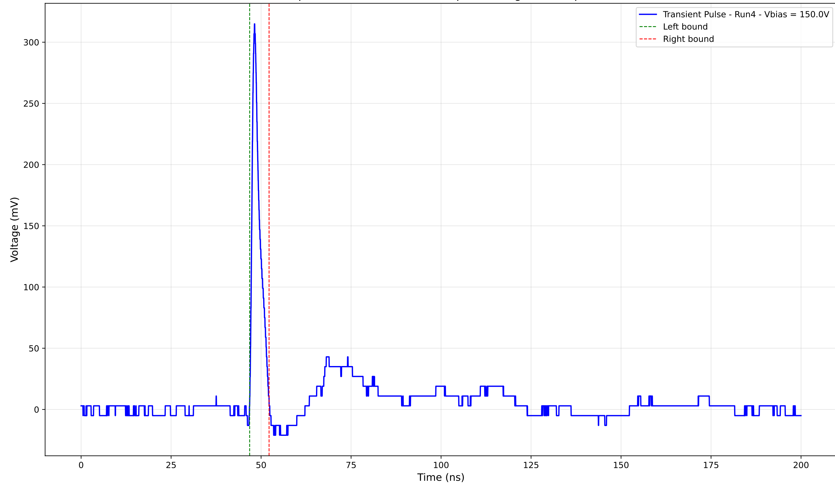
Transient Pulse - Sample: 4003 - Position: 270.0 \mu\text{m} - Charge: 15.37 pC - Rise Time: 0.91 ns
