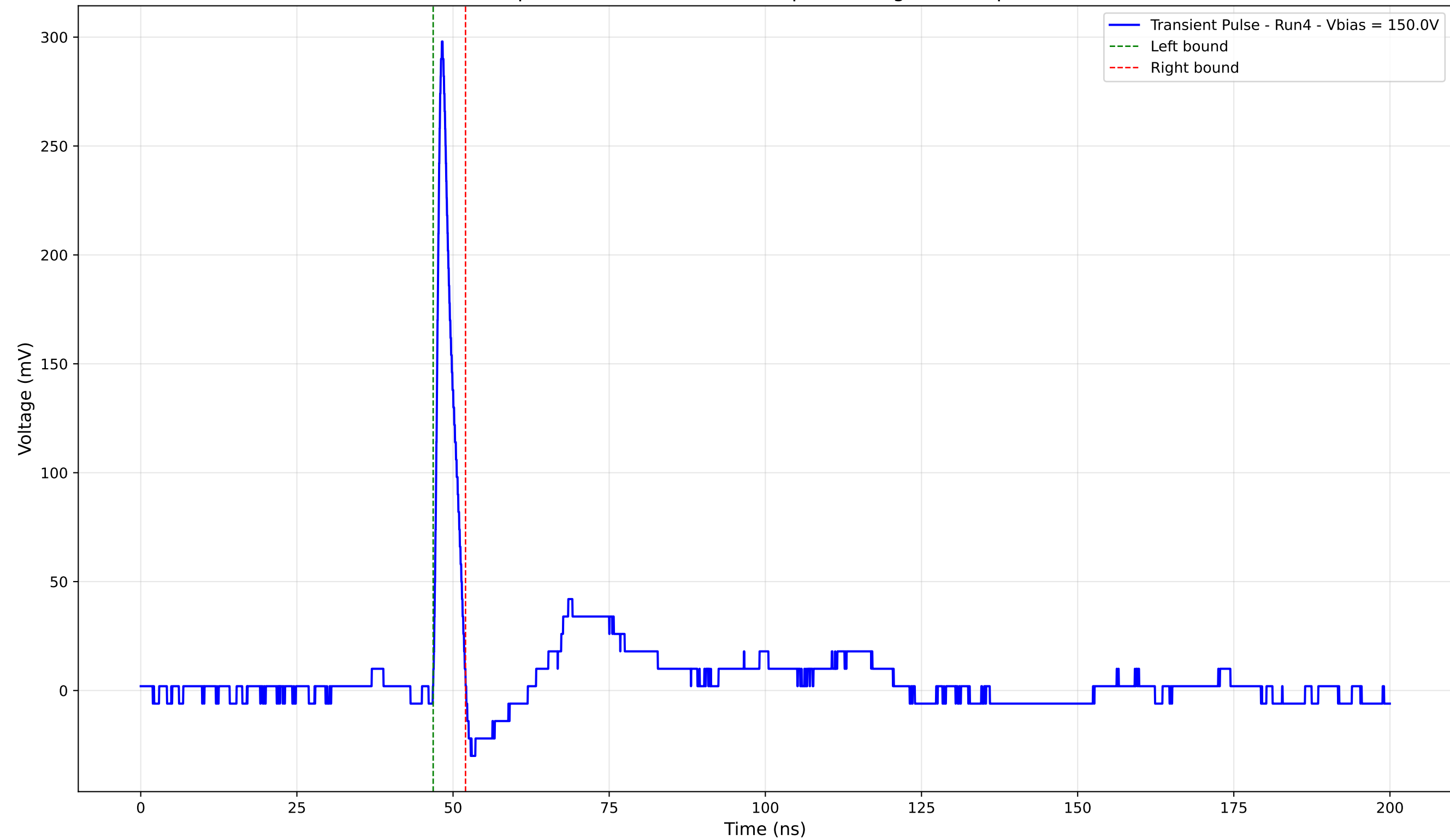
Transient Pulse - Sample: 4003 - Position: 425.0 \mu\text{m} - Charge: 15.09 pC - Rise Time: 0.93 ns
