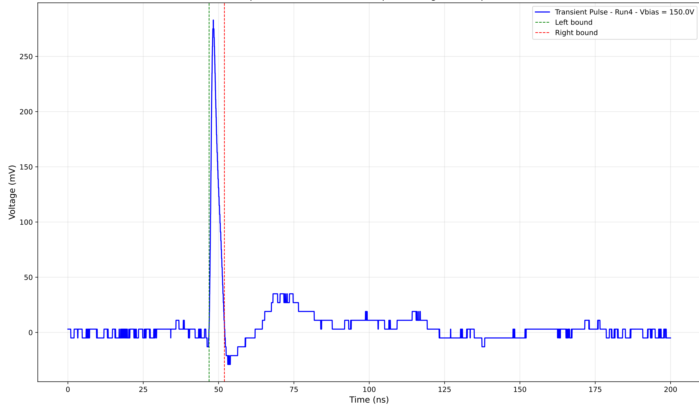
Transient Pulse - Sample: 4003 - Position: 440.0 \mu\text{m} - Charge: 14.23 pC - Rise Time: 0.92 ns
