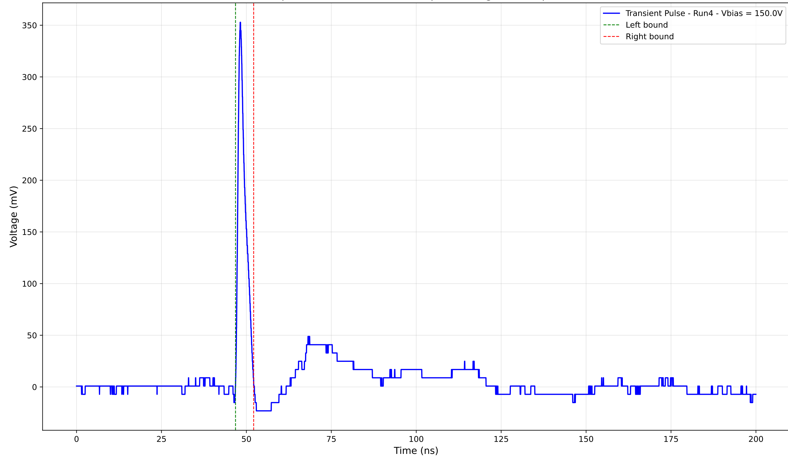
Transient Pulse - Sample: 4003 - Position: 345.0 \mu\text{m} - Charge: 17.61 pC - Rise Time: 0.89 ns
