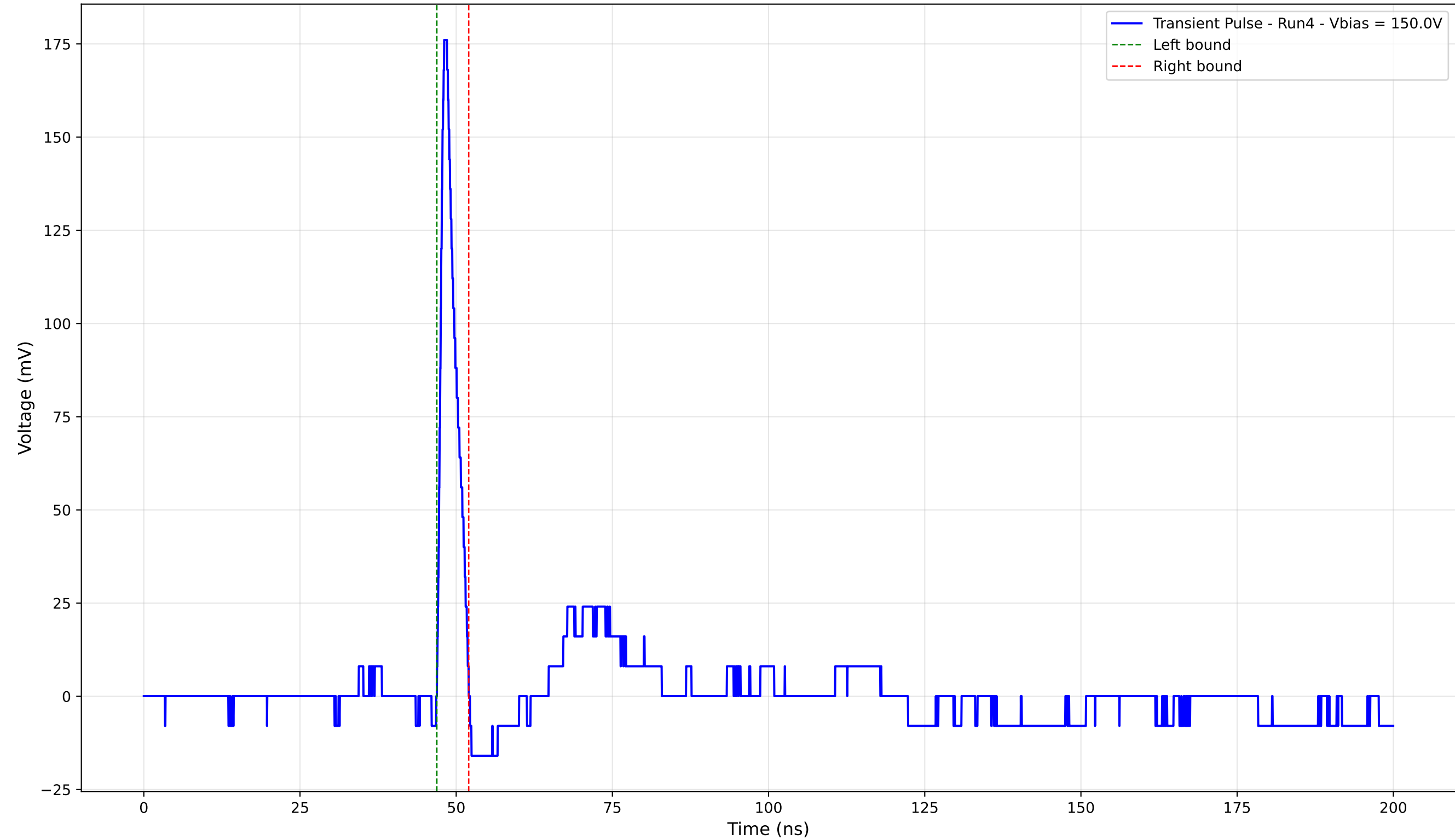
Transient Pulse - Sample: 4003 - Position: 580.0 \mu\text{m} - Charge: 9.35 pC - Rise Time: 0.86 ns
