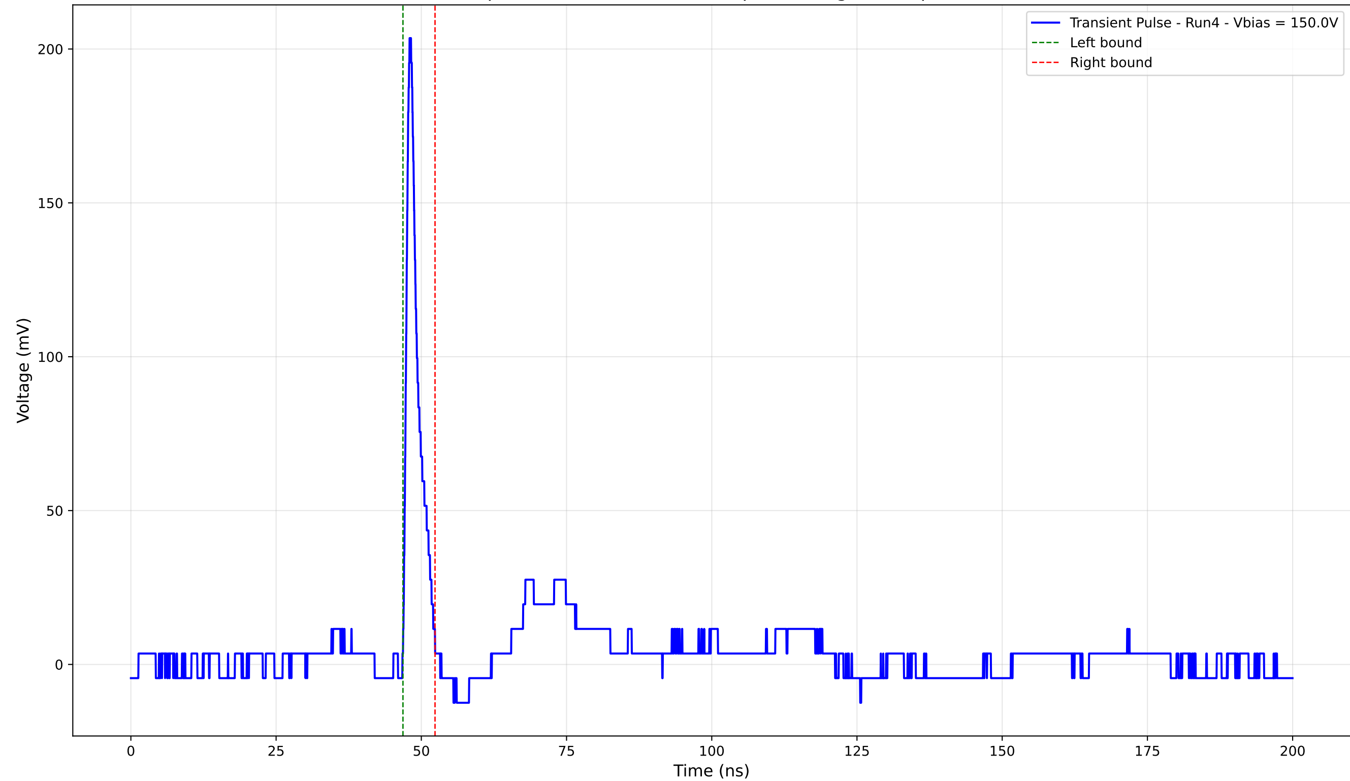
Transient Pulse - Sample: 4003 - Position: 175.0 \mu\text{m} - Charge: 9.59 pC - Rise Time: 0.82 ns
