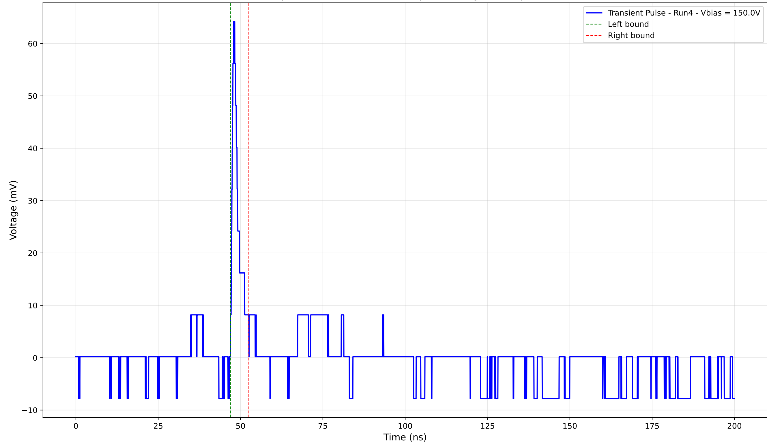
Transient Pulse - Sample: 4003 - Position: 70.0 \mu\text{m} - Charge: 2.87 pC - Rise Time: 0.96 ns
