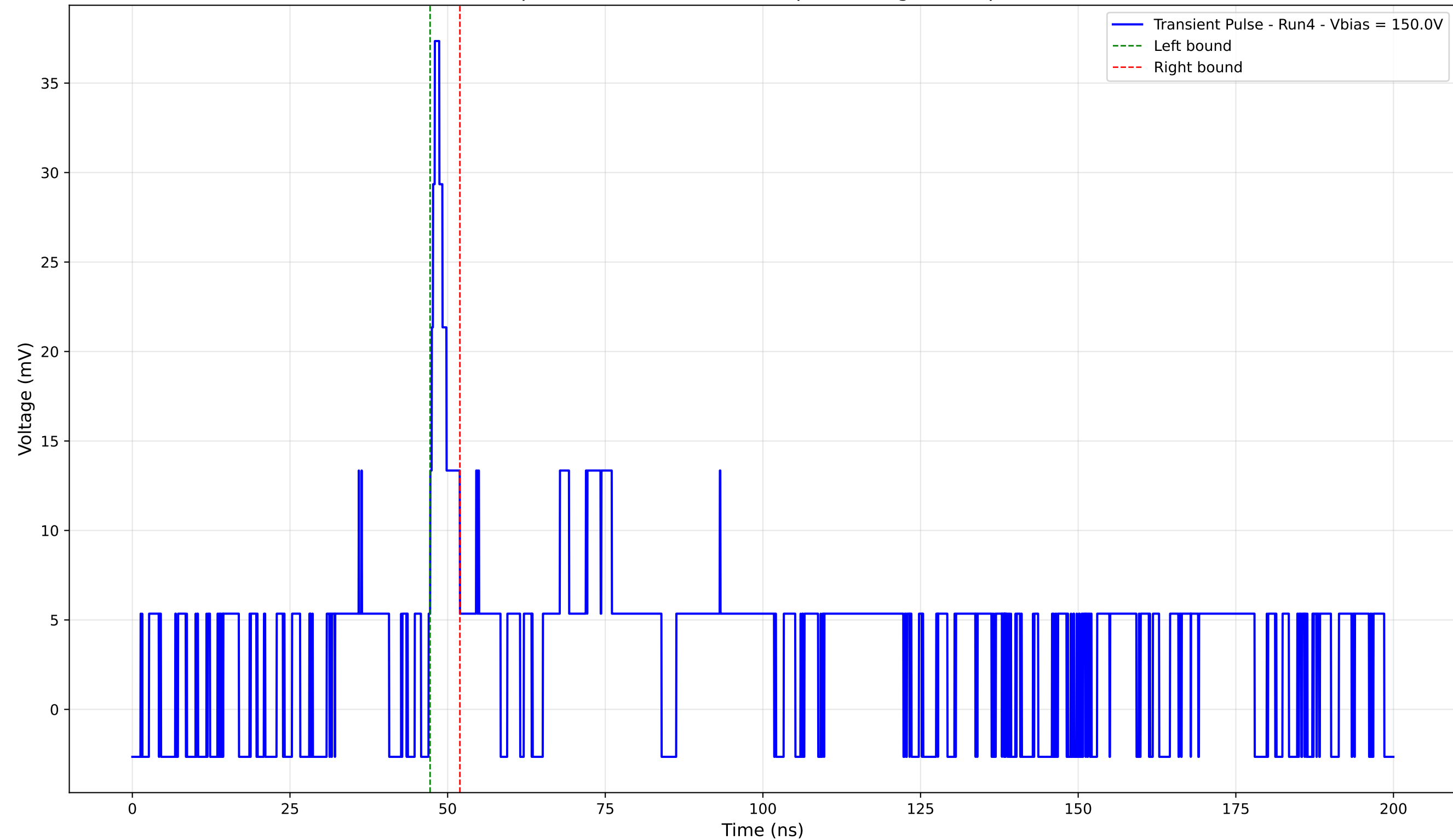
Transient Pulse - Sample: 4003 - Position: 615.0 \mu\text{m} - Charge: 1.99 pC - Rise Time: 0.99 ns
