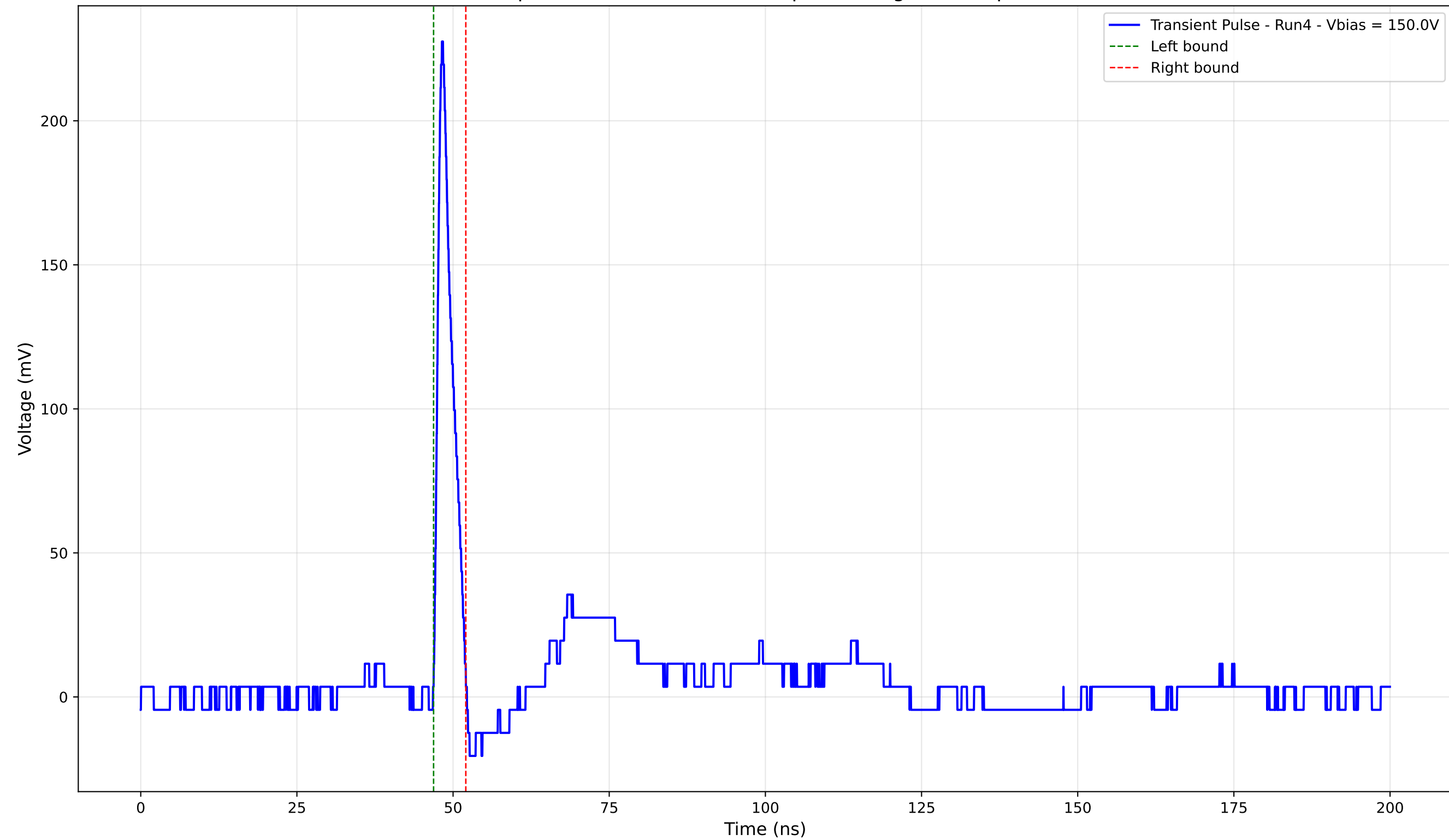
Transient Pulse - Sample: 4003 - Position: 485.0 \mu\text{m} - Charge: 11.82 pC - Rise Time: 0.95 ns
