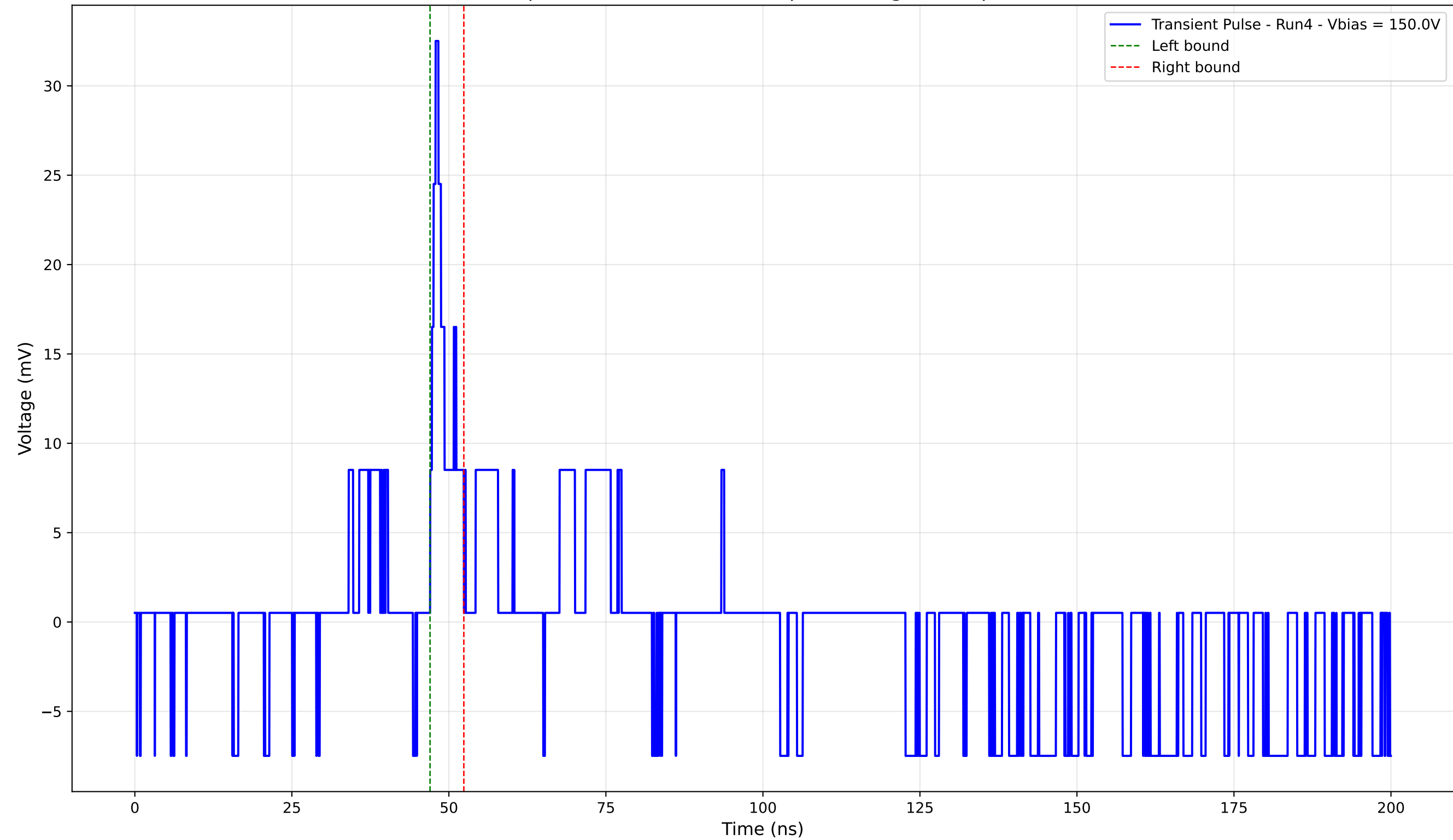
Transient Pulse - Sample: 4003 - Position: 40.0 \mu\text{m} - Charge: 1.53 pC - Rise Time: 0.87 ns
