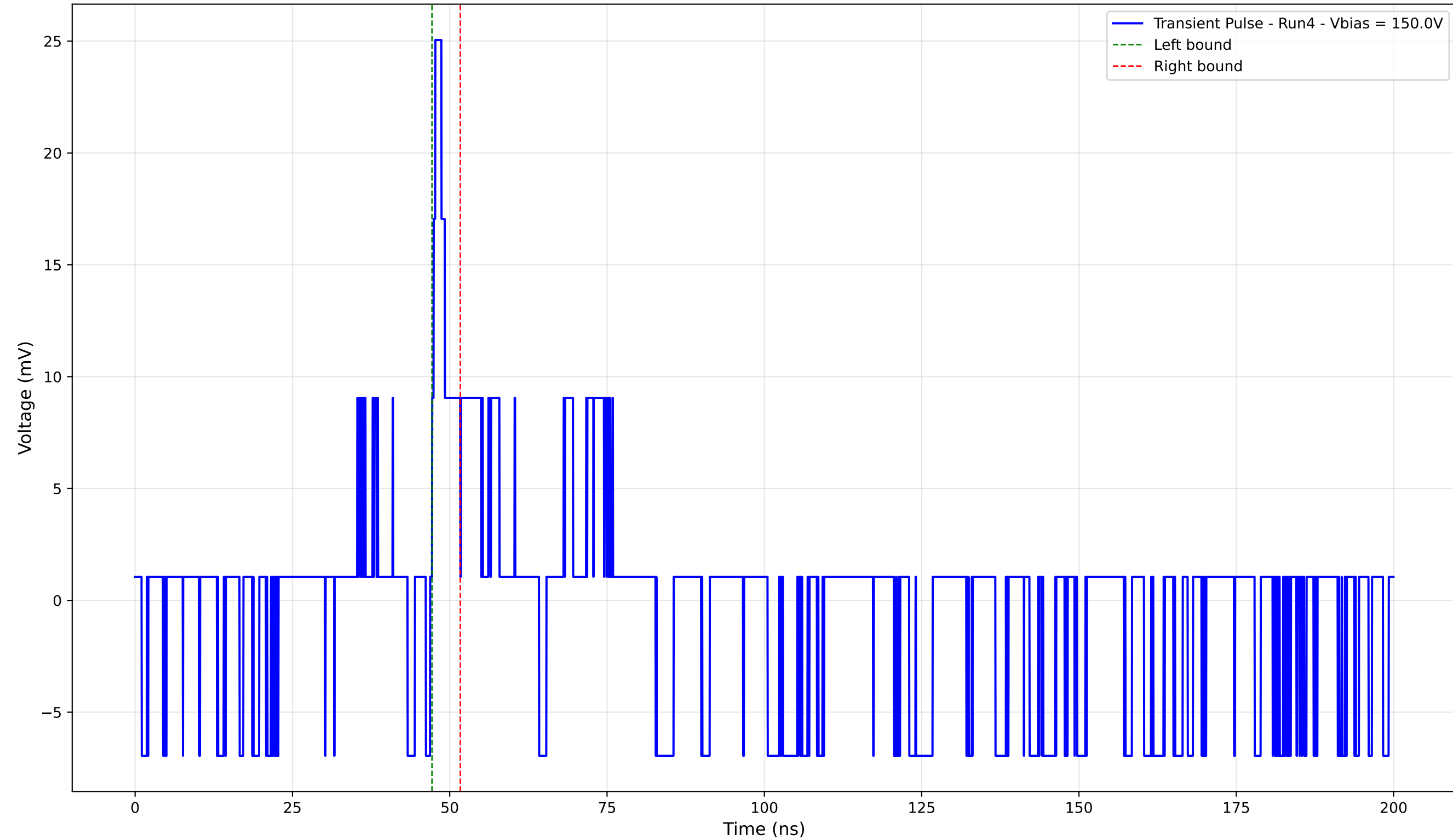
Transient Pulse - Sample: 4003 - Position: 35.0 \mu\text{m} - Charge: 1.25 pC - Rise Time: 0.52 ns
