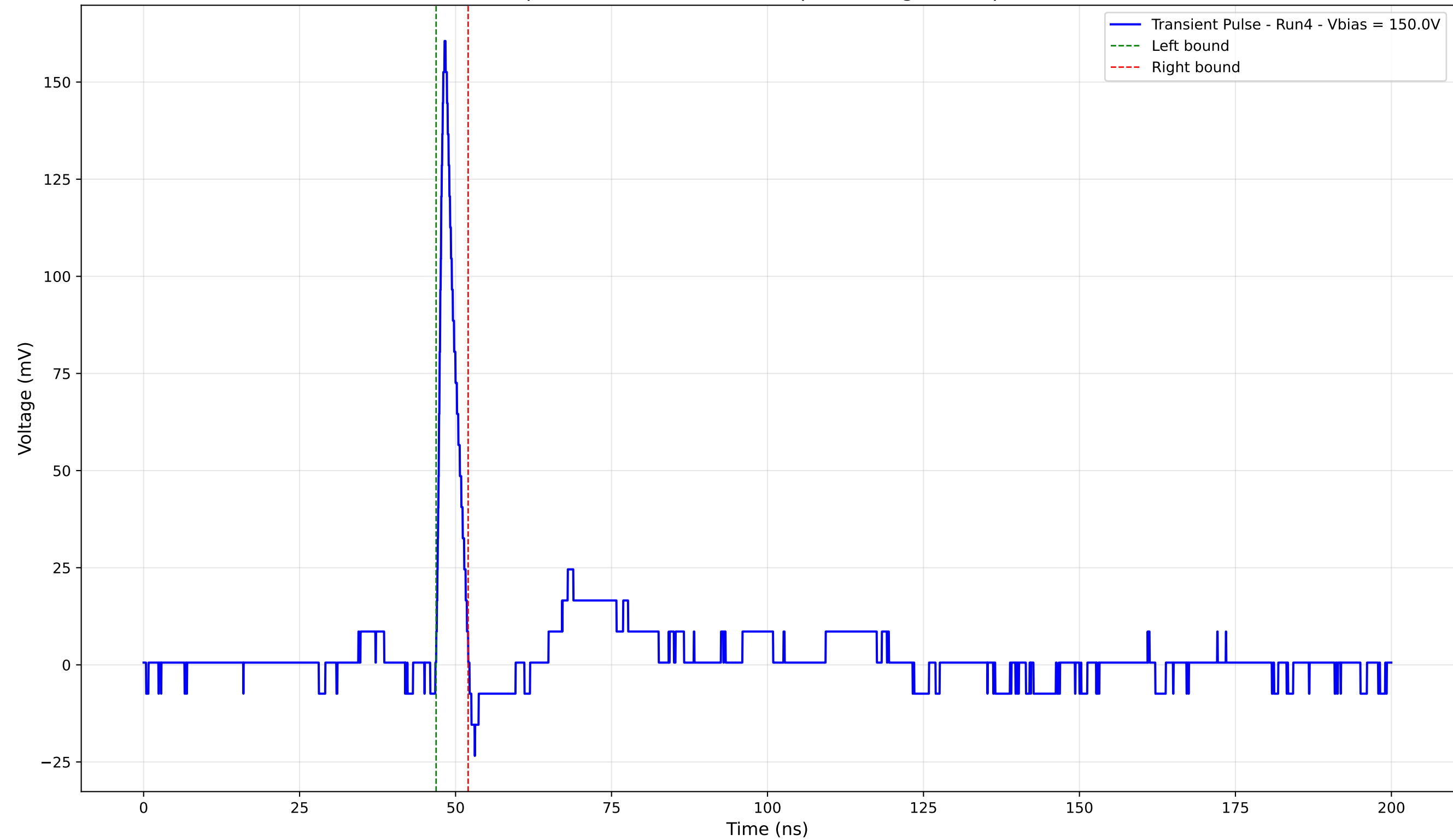
Transient Pulse - Sample: 4003 - Position: 555.0 \mu\text{m} - Charge: 8.20 pC - Rise Time: 0.94 ns
