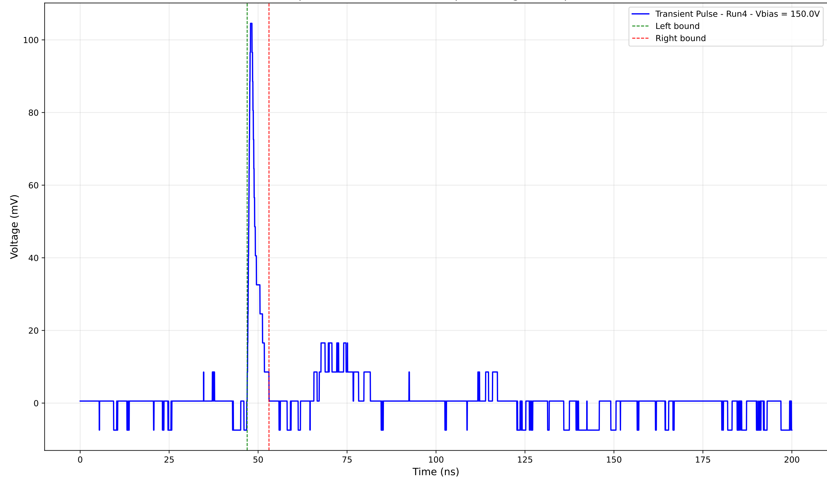
Transient Pulse - Sample: 4003 - Position: 110.0 \mu\text{m} - Charge: 4.83 pC - Rise Time: 0.72 ns
