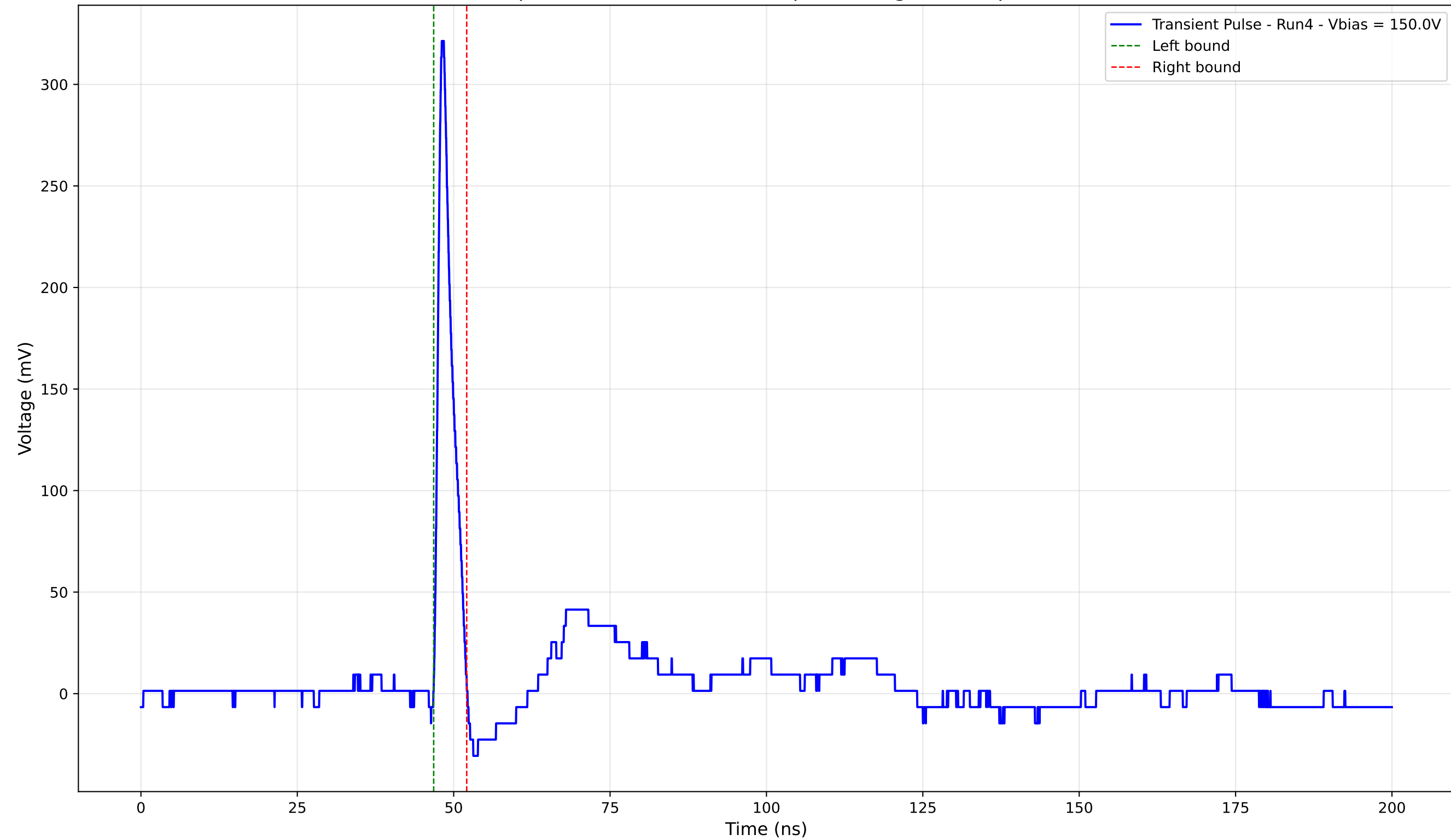
Transient Pulse - Sample: 4003 - Position: 385.0 \mu\text{m} - Charge: 16.42 pC - Rise Time: 0.90 ns
