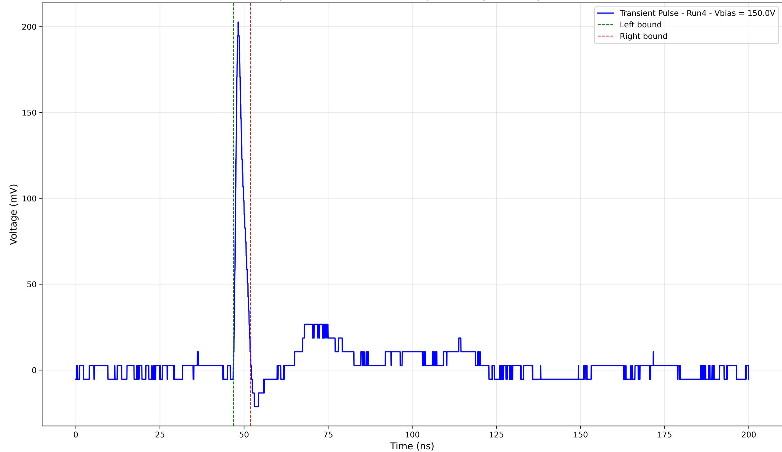
Transient Pulse - Sample: 4003 - Position: 505.0 \mu\text{m} - Charge: 10.17 pC - Rise Time: 0.96 ns
