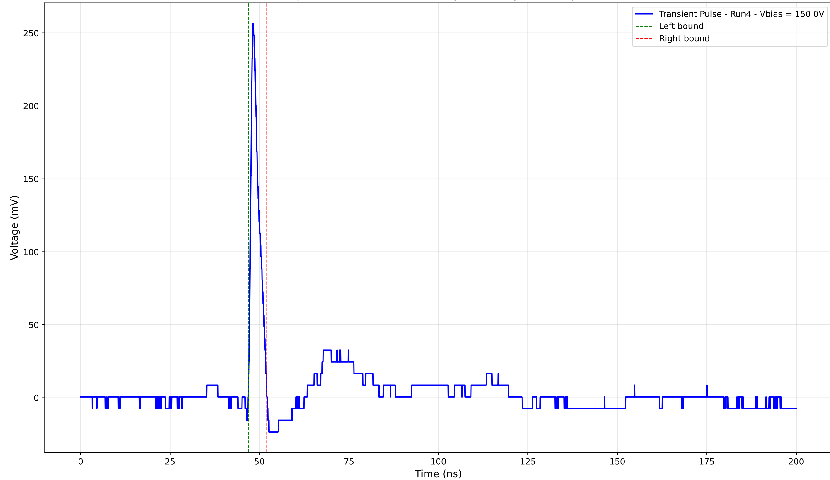
Transient Pulse - Sample: 4003 - Position: 460.0 \mu\text{m} - Charge: 13.06 pC - Rise Time: 0.86 ns
