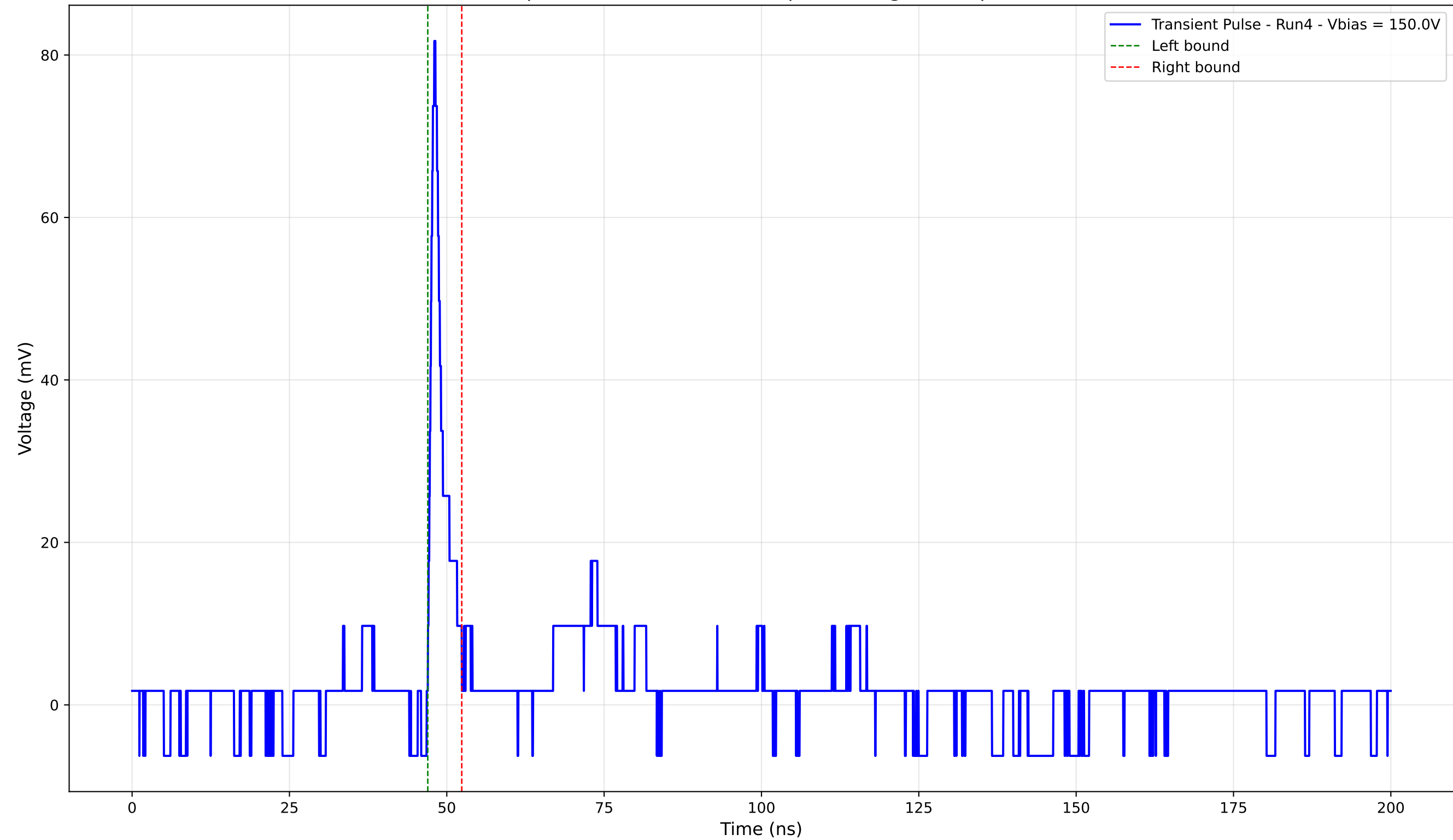
Transient Pulse - Sample: 4003 - Position: 85.0 \mu\text{m} - Charge: 3.59 pC - Rise Time: 0.78 ns
