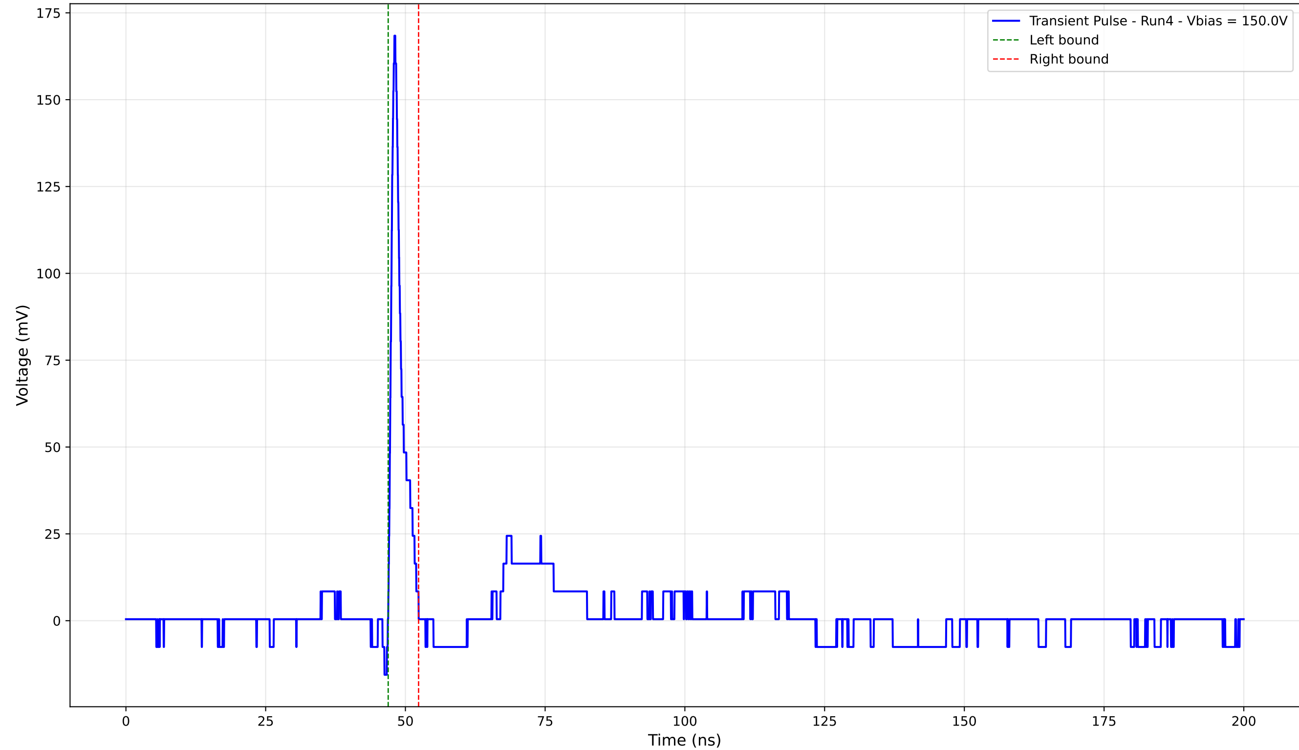
Transient Pulse - Sample: 4003 - Position: 150.0 \mu\text{m} - Charge: 7.28 pC - Rise Time: 0.78 ns
