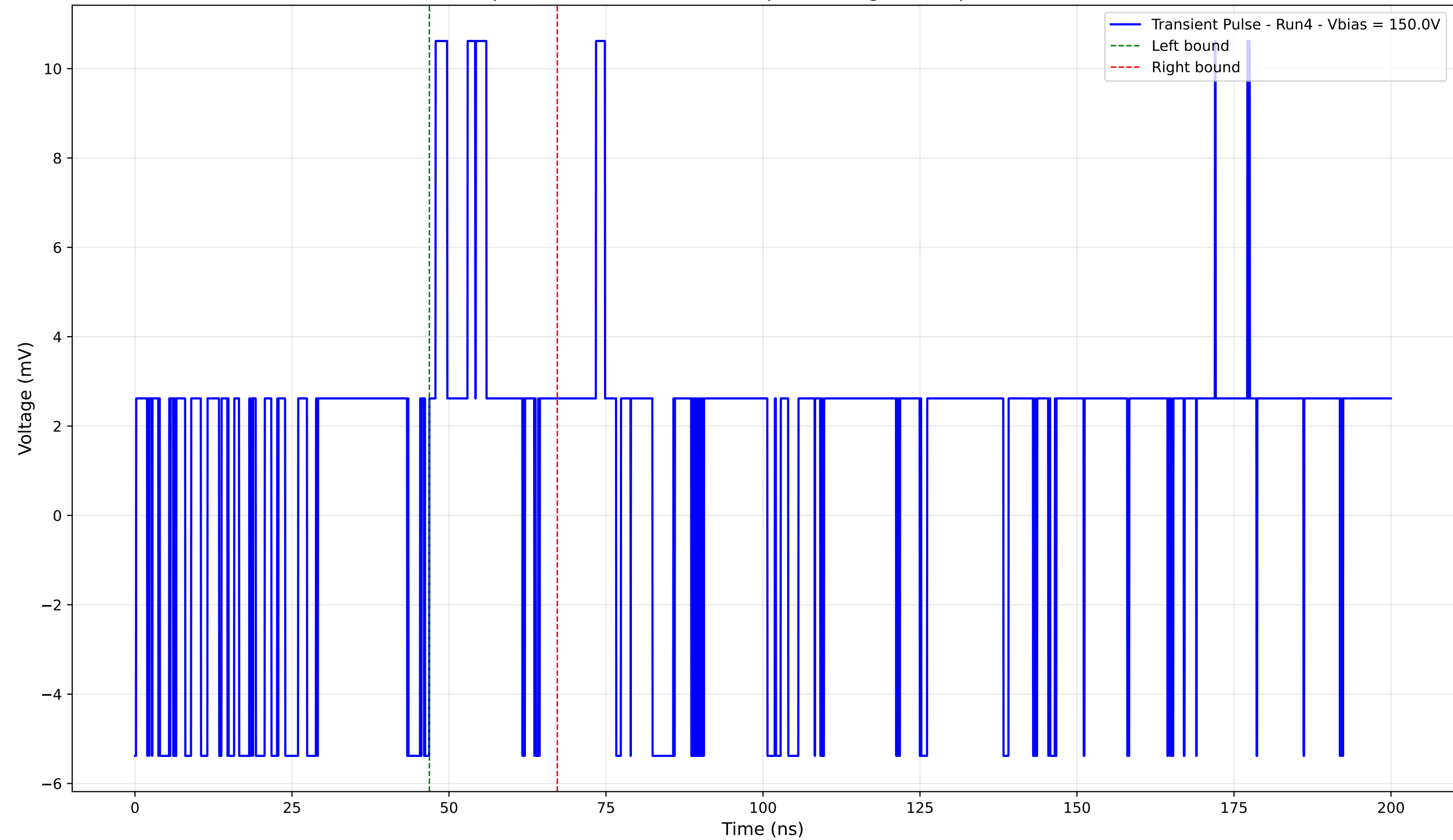
Transient Pulse - Sample: 4003 - Position: 625.0 \mu\text{m} - Charge: 1.69 pC - Rise Time: 0.00 ns (N/A)
