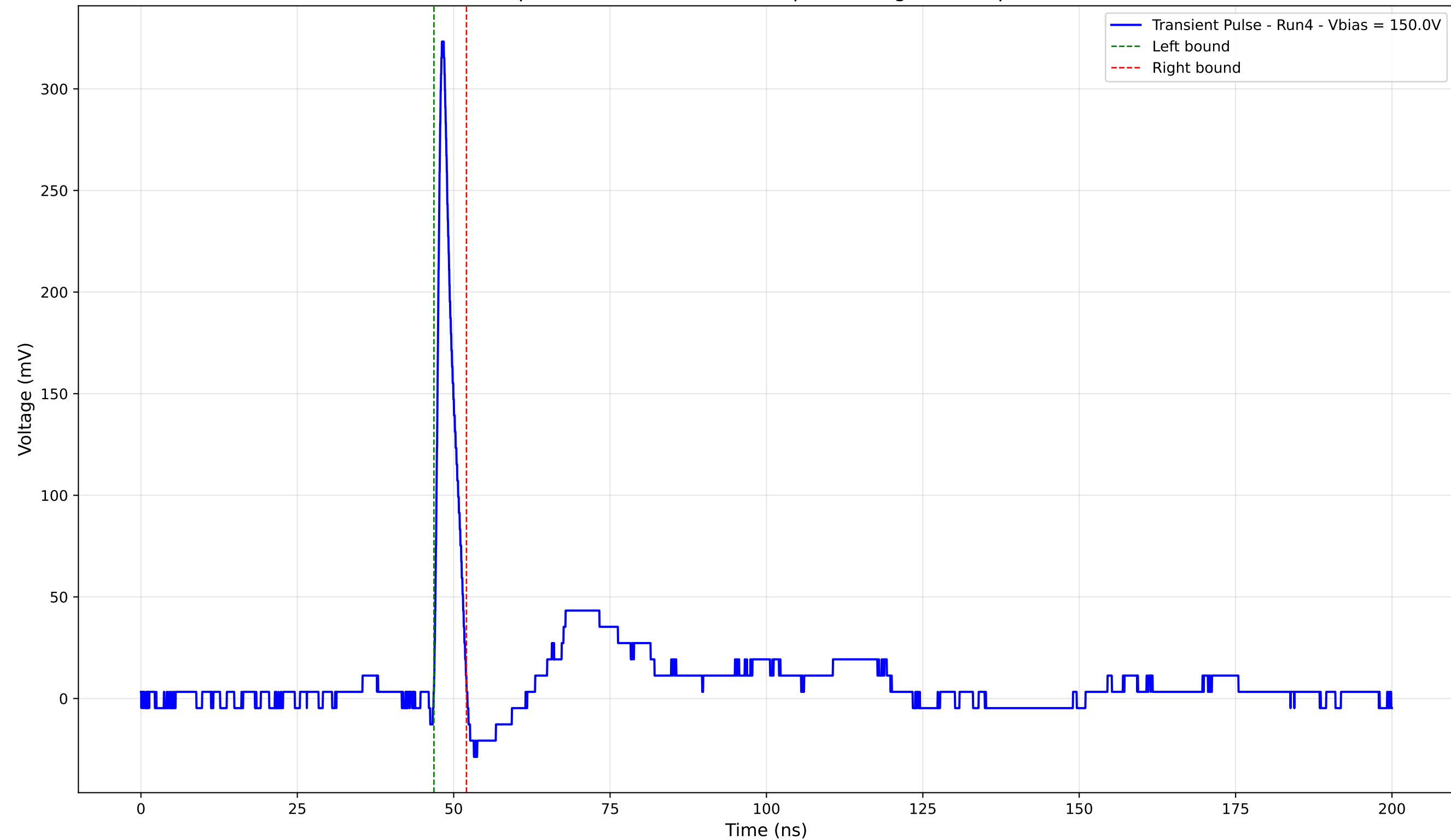
Transient Pulse - Sample: 4003 - Position: 395.0 \mu\text{m} - Charge: 16.61 pC - Rise Time: 0.89 ns
