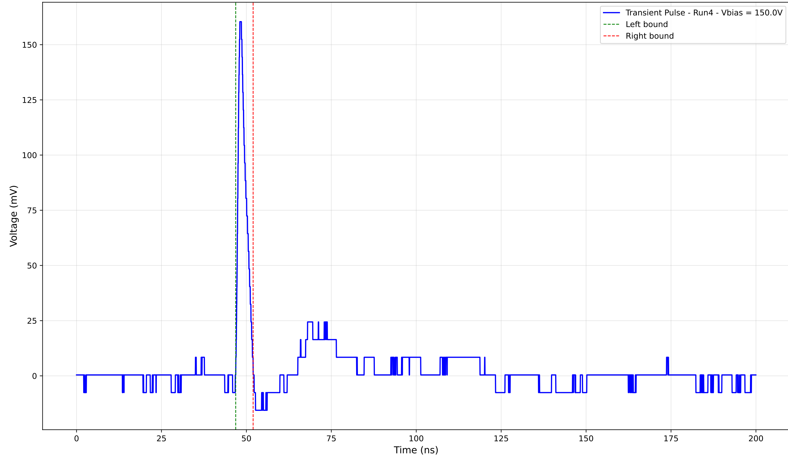
Transient Pulse - Sample: 4003 - Position: 540.0 \mu\text{m} - Charge: 8.44 pC - Rise Time: 0.90 ns
