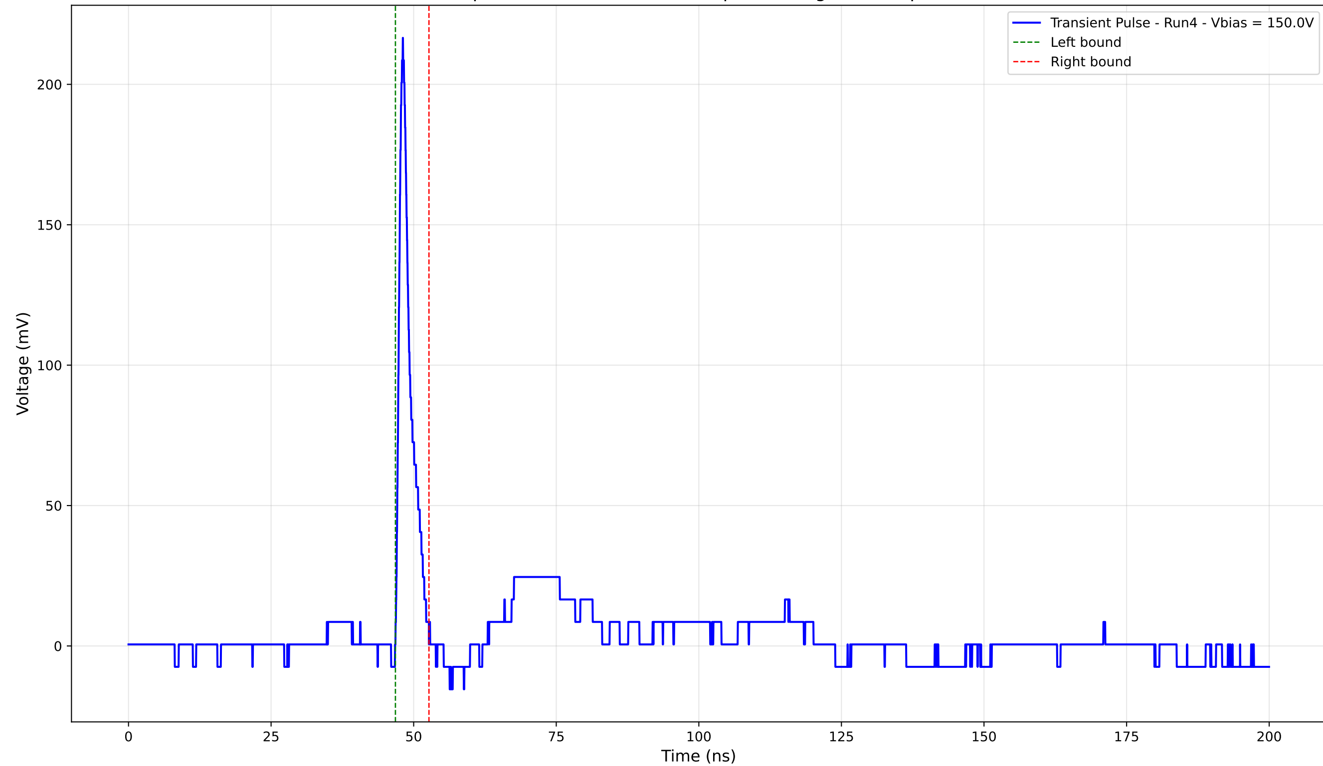
Transient Pulse - Sample: 4003 - Position: 180.0 \mu\text{m} - Charge: 10.00 pC - Rise Time: 0.89 ns
