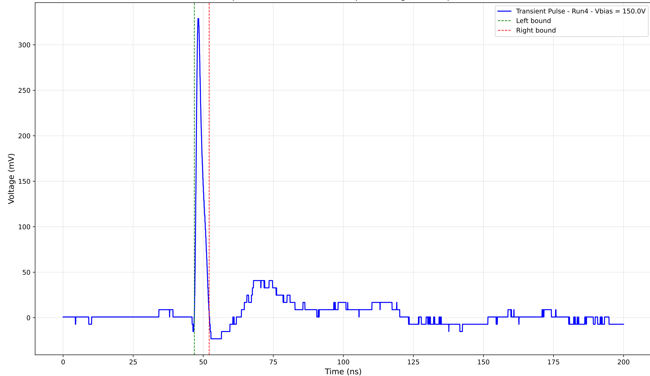
Transient Pulse - Sample: 4003 - Position: 375.0 \mu\text{m} - Charge: 16.68 pC - Rise Time: 0.86 ns
