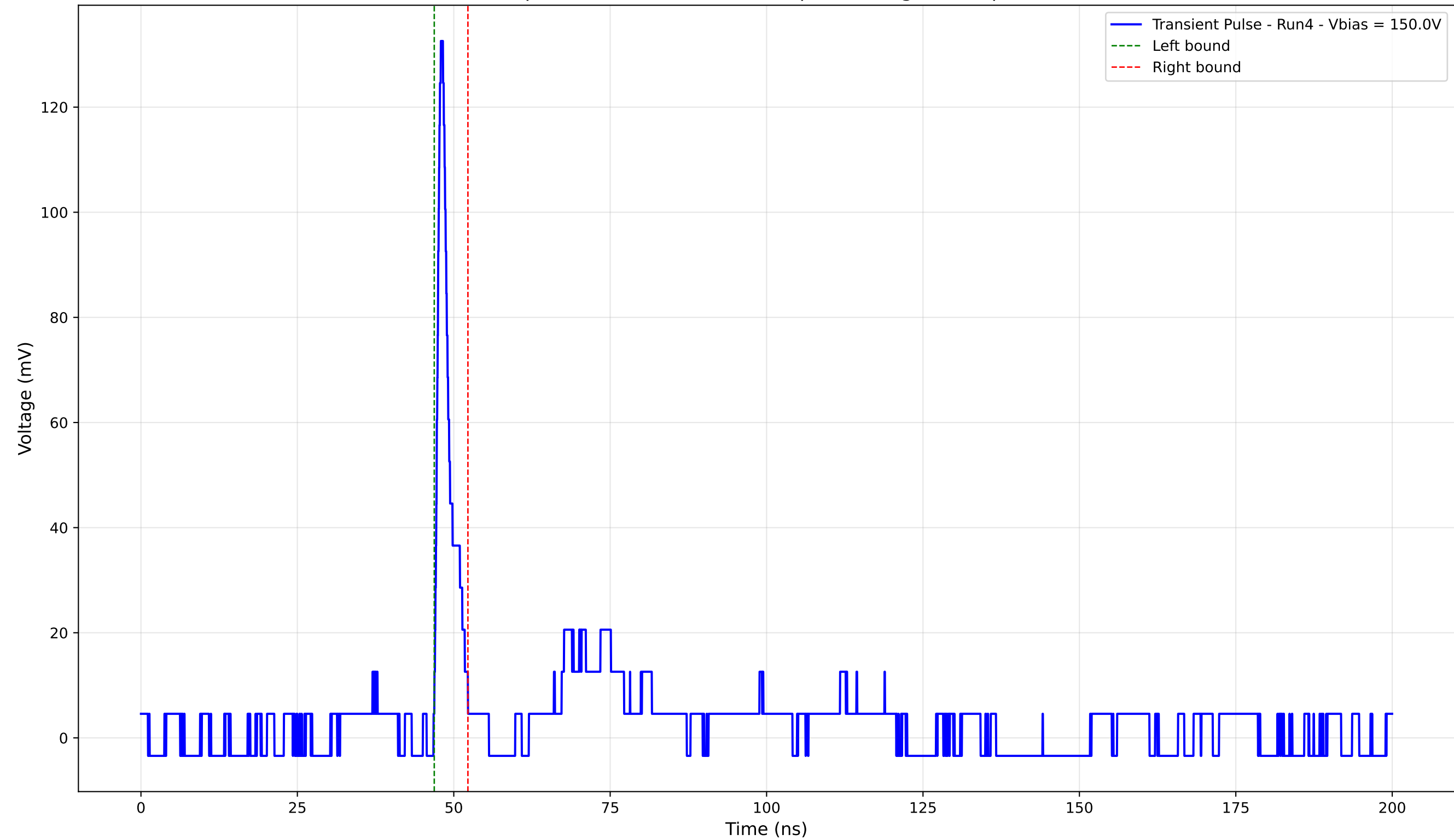
Transient Pulse - Sample: 4003 - Position: 125.0 \mu\text{m} - Charge: 6.07 pC - Rise Time: 0.80 ns
