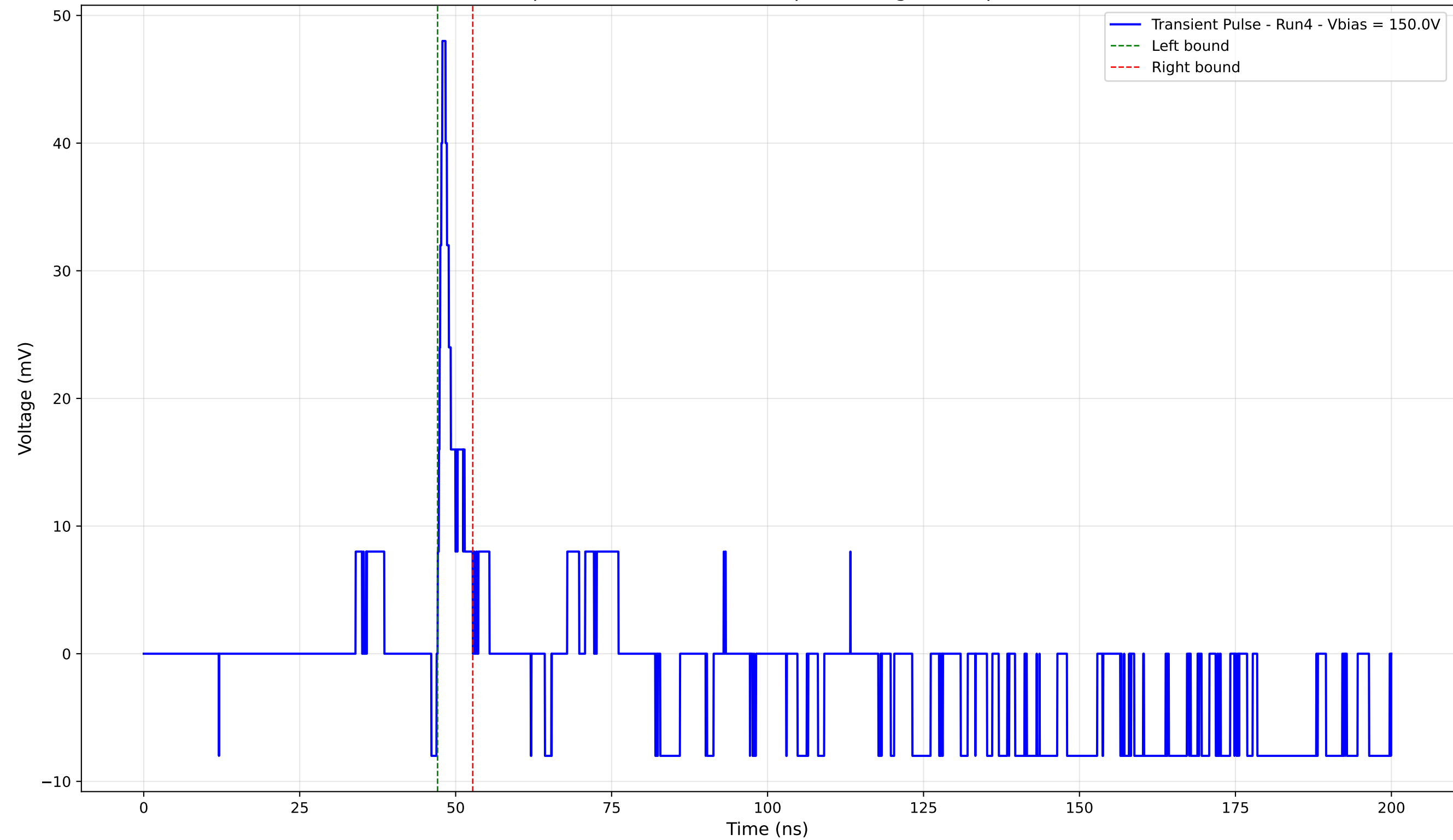
Transient Pulse - Sample: 4003 - Position: 55.0 \mu\text{m} - Charge: 2.27 pC - Rise Time: 0.75 ns
