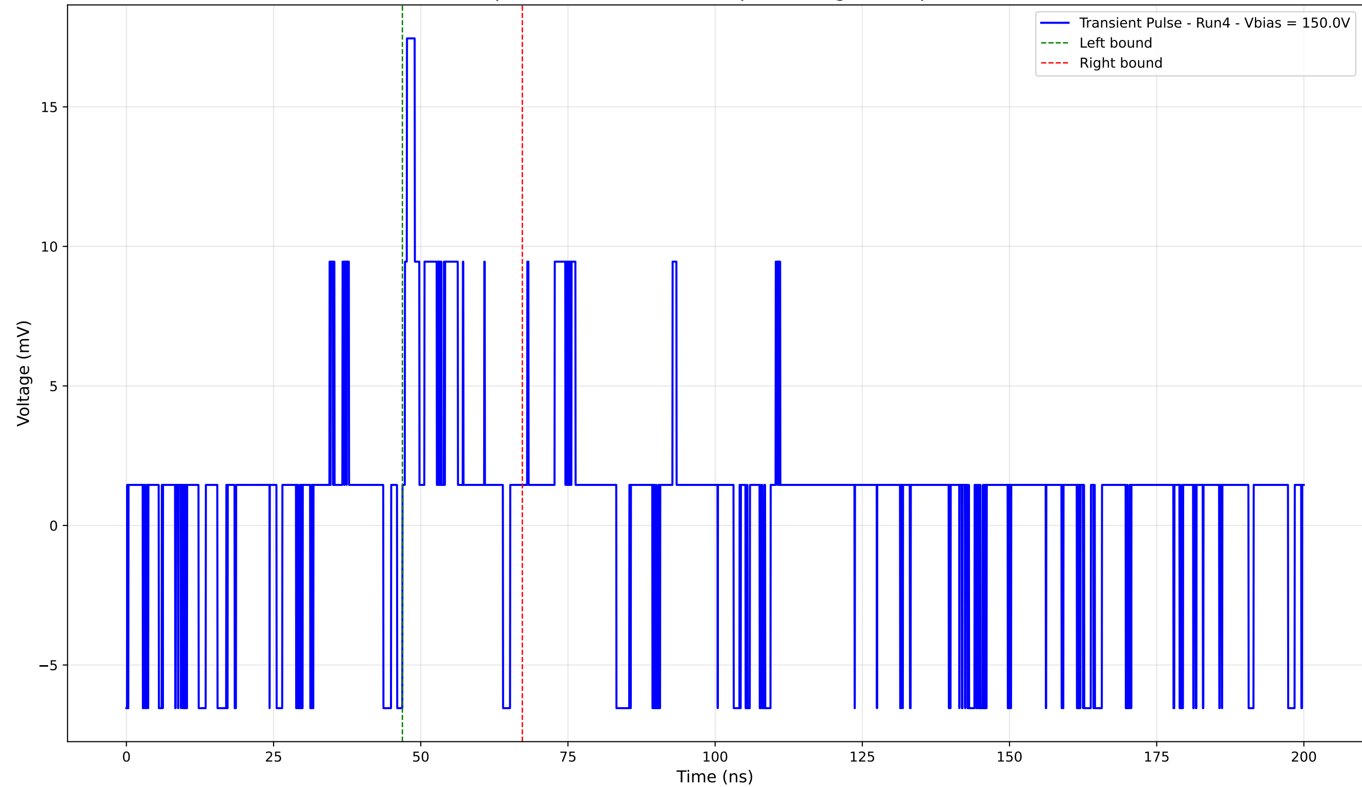
Transient Pulse - Sample: 4003 - Position: 25.0 \mu\text{m} - Charge: 1.79 pC - Rise Time: 0.36 ns
