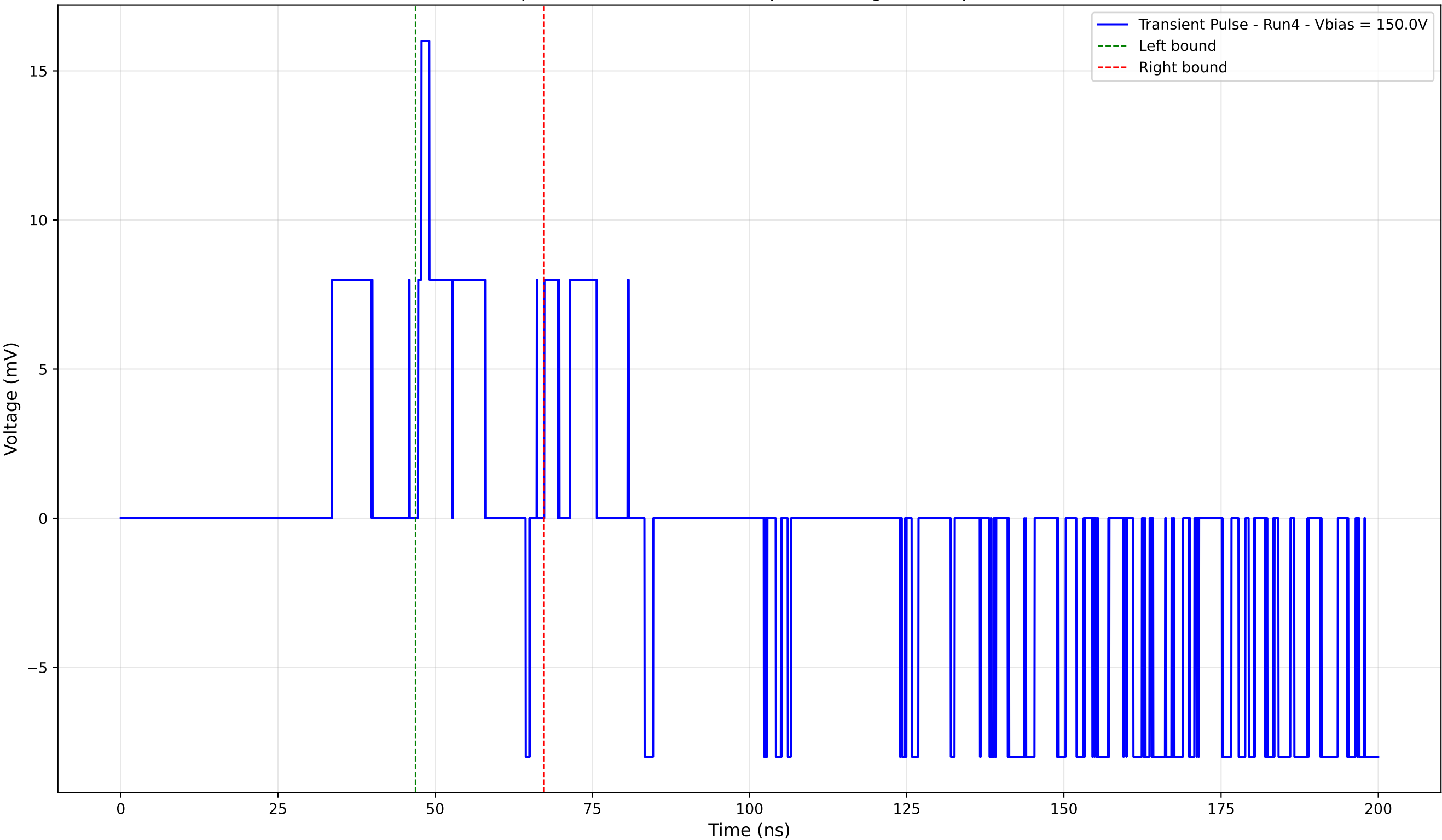
Transient Pulse - Sample: 4003 - Position: 5.0 \mu\text{m} - Charge: 1.80 pC - Rise Time: 0.54 ns
