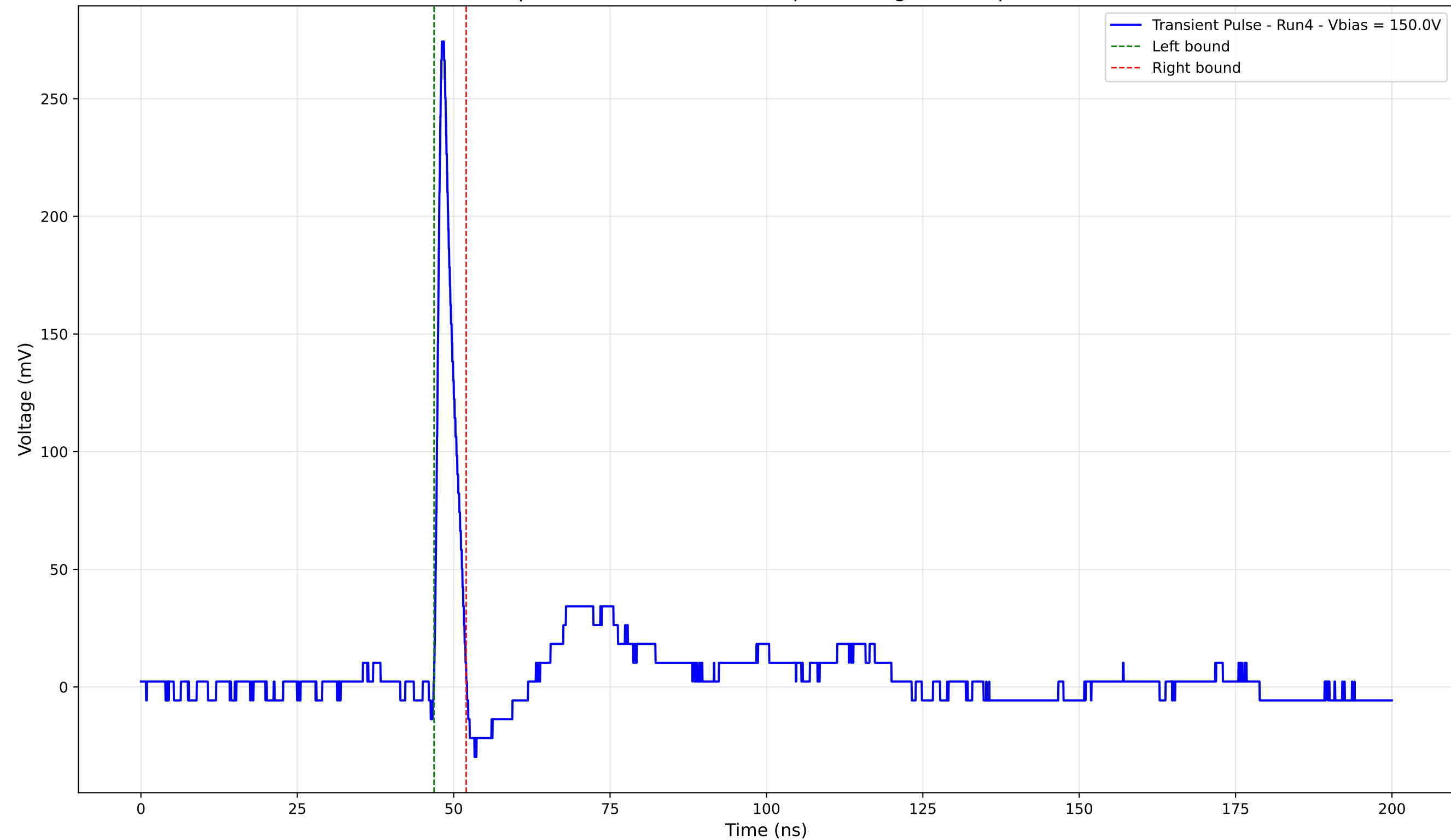
Transient Pulse - Sample: 4003 - Position: 445.0 \mu\text{m} - Charge: 14.12 pC - Rise Time: 0.90 ns
