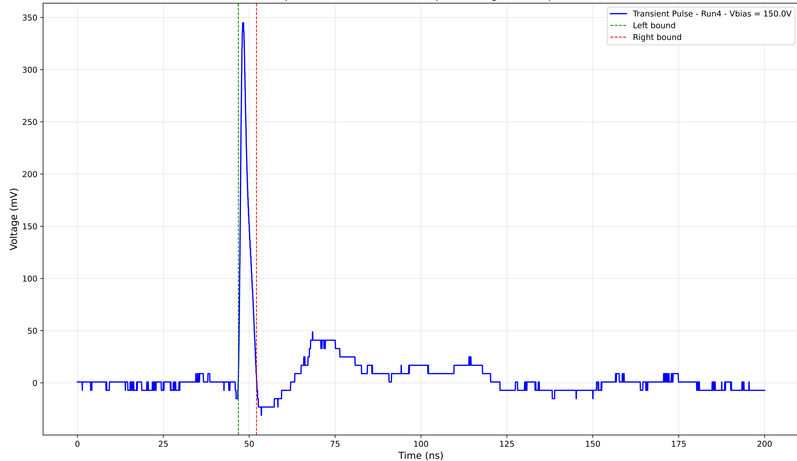
Transient Pulse - Sample: 4003 - Position: 350.0 \mu\text{m} - Charge: 17.42 pC - Rise Time: 0.87 ns
