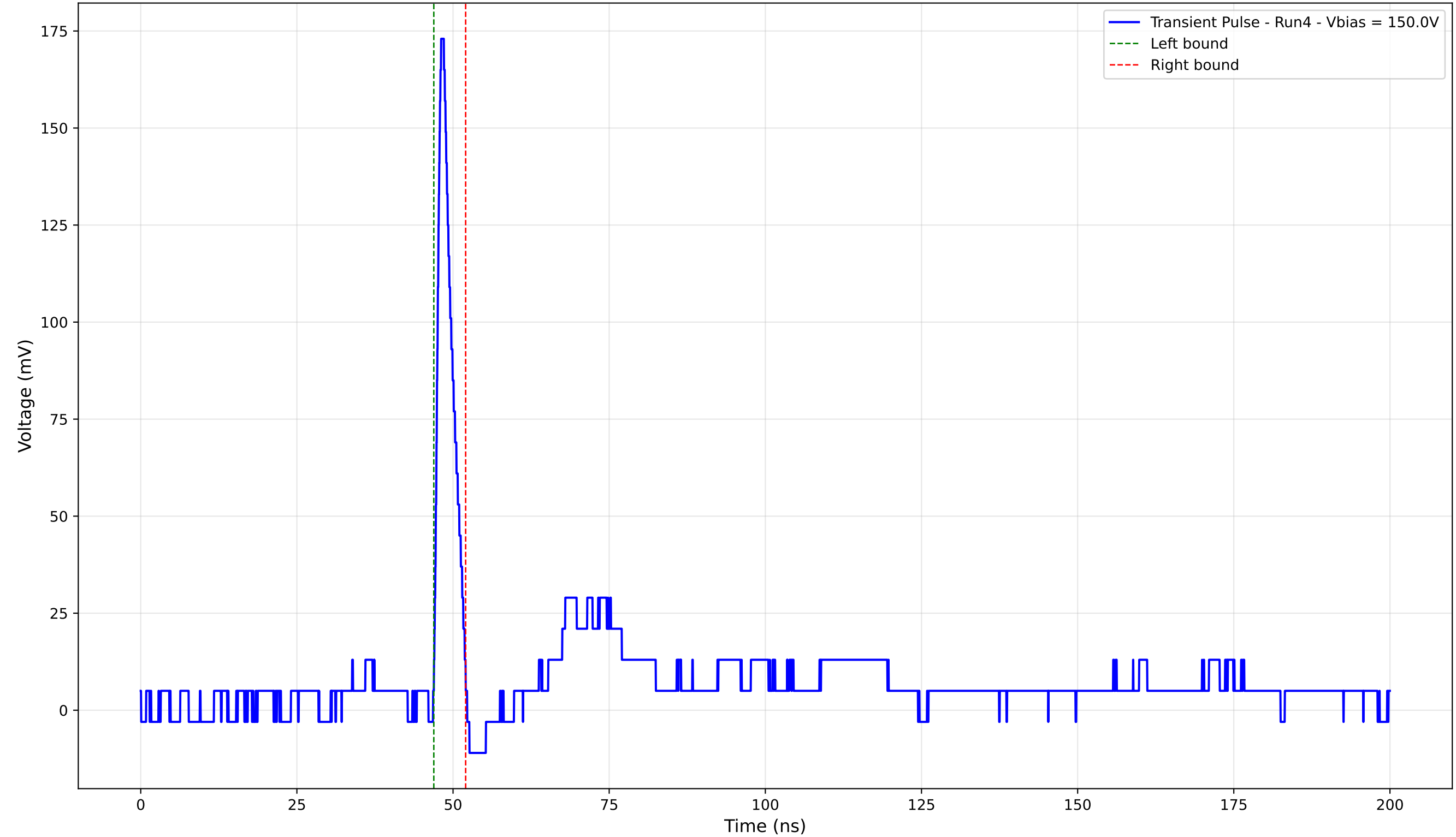
Transient Pulse - Sample: 4003 - Position: 575.0 \mu\text{m} - Charge: 9.22 pC - Rise Time: 0.89 ns
