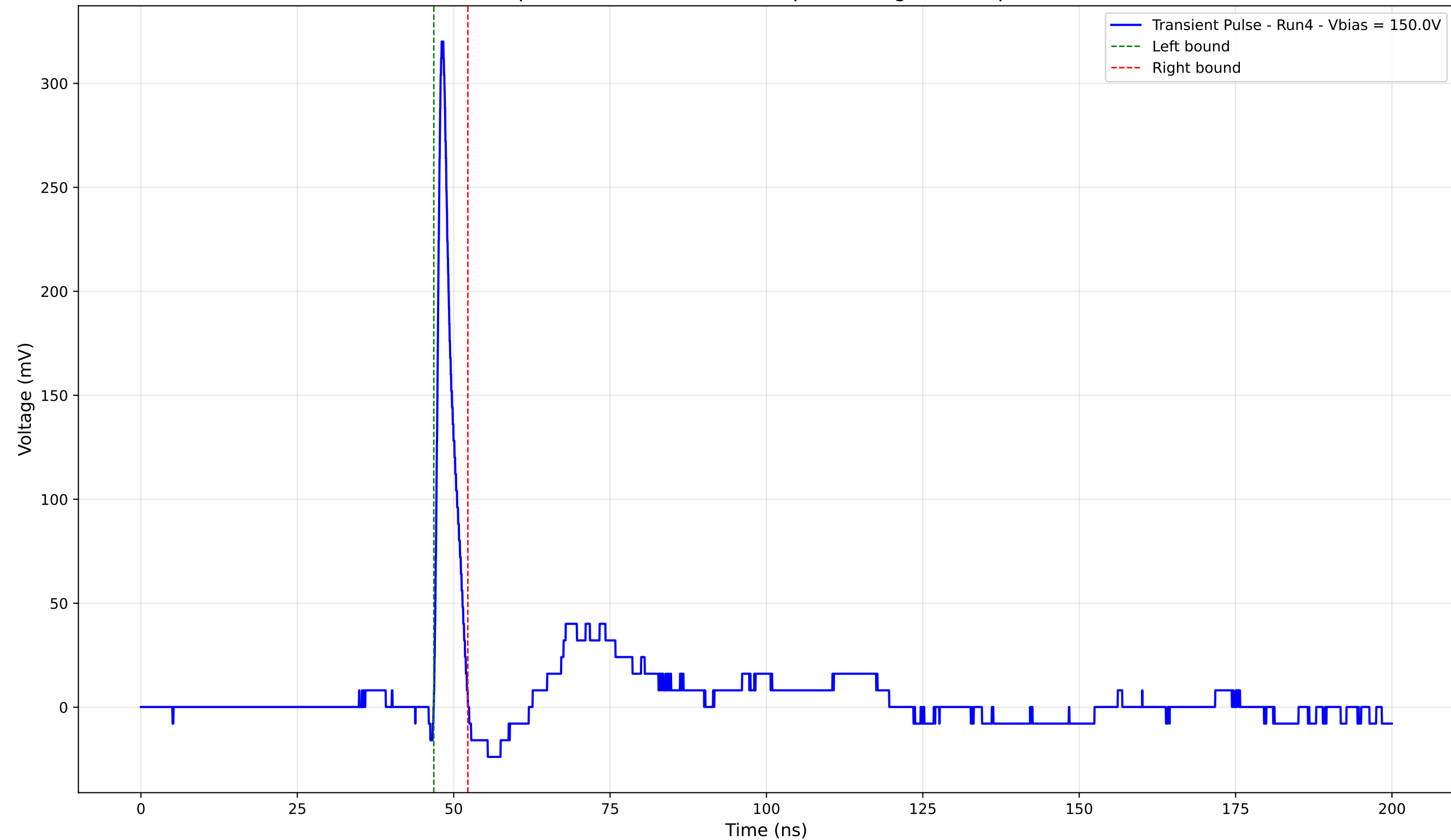
Transient Pulse - Sample: 4003 - Position: 280.0 \mu\text{m} - Charge: 15.88 pC - Rise Time: 0.86 ns
