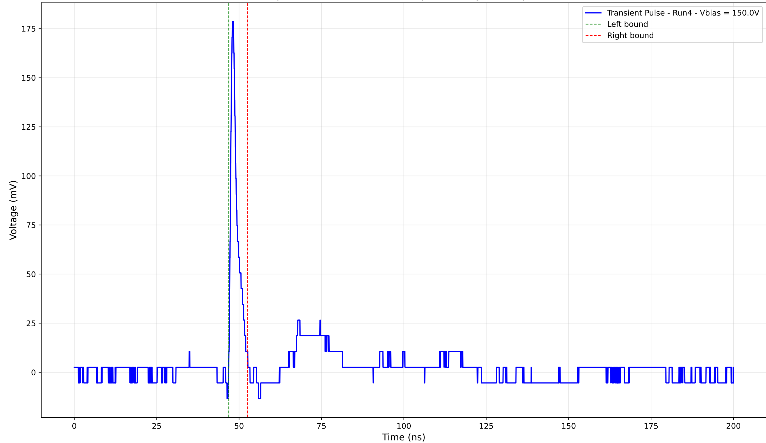
Transient Pulse - Sample: 4003 - Position: 160.0 \mu\text{m} - Charge: 8.34 pC - Rise Time: 0.80 ns
