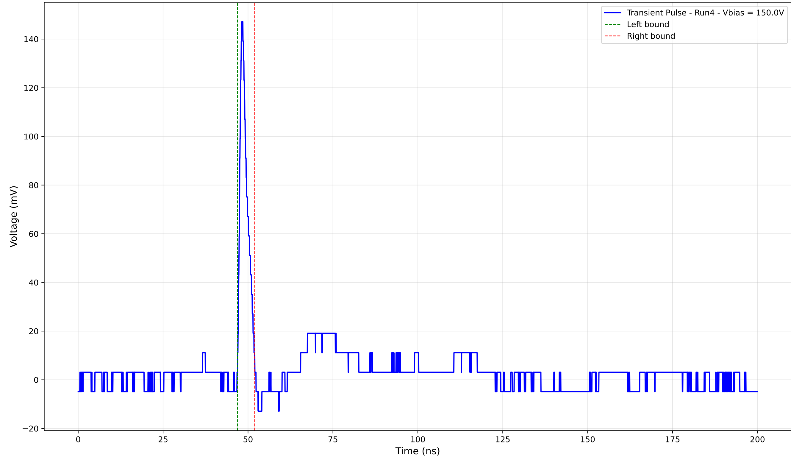
Transient Pulse - Sample: 4003 - Position: 560.0 \mu\text{m} - Charge: 7.47 pC - Rise Time: 0.97 ns
