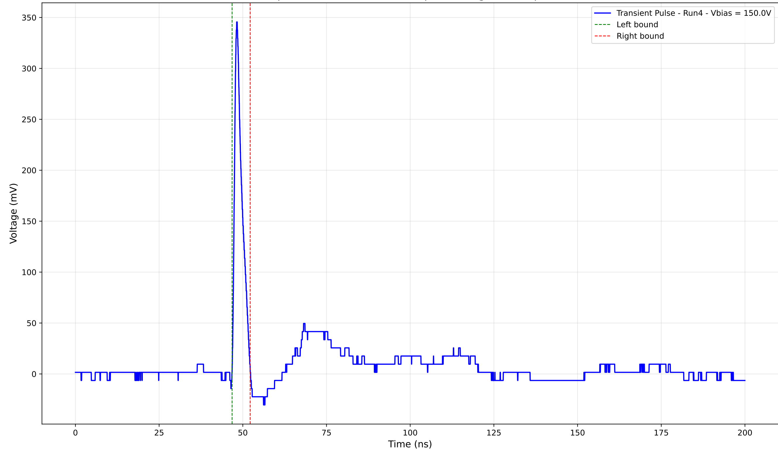
Transient Pulse - Sample: 4003 - Position: 355.0 \mu\text{m} - Charge: 17.56 pC - Rise Time: 0.90 ns
