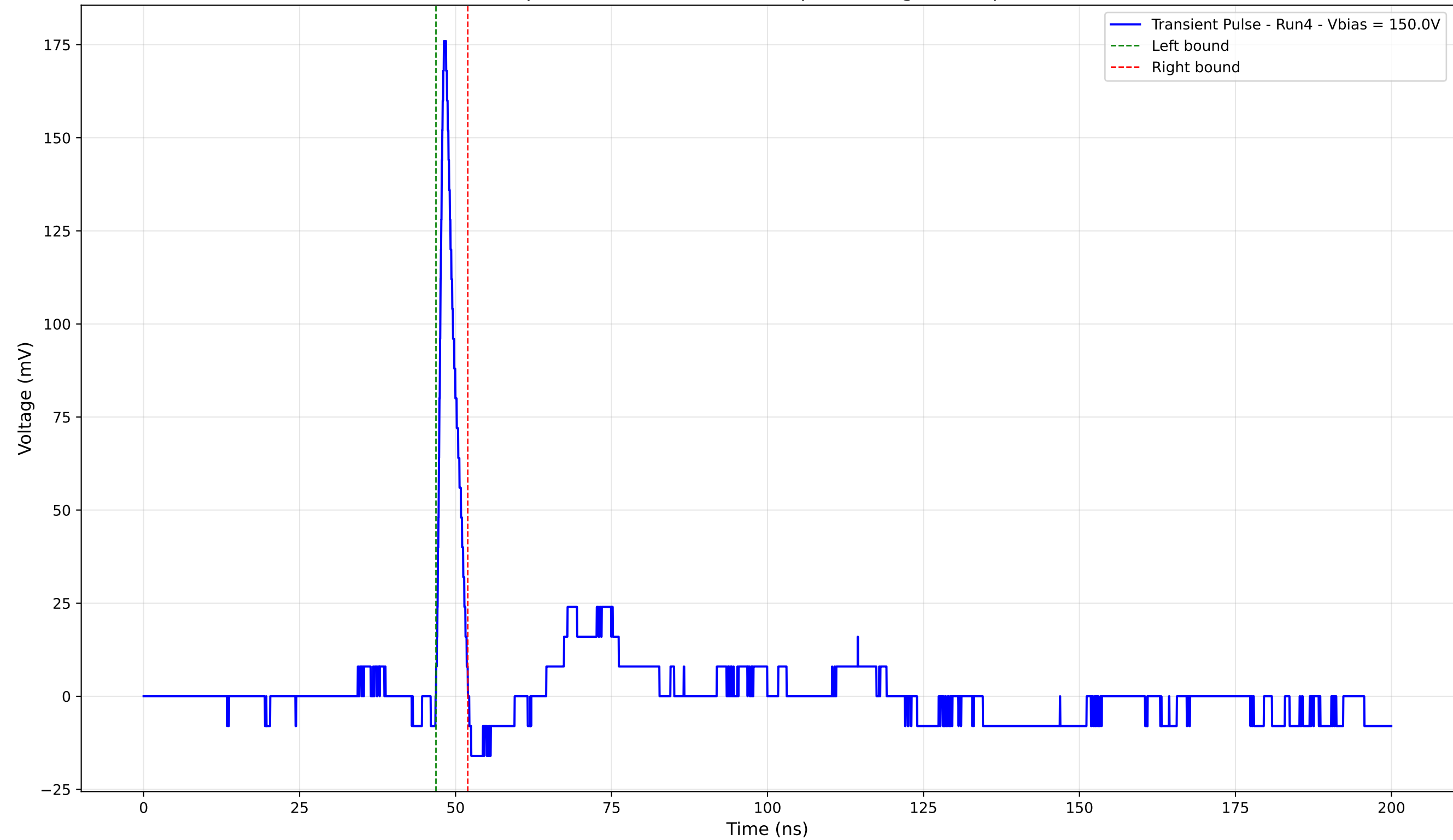
Transient Pulse - Sample: 4003 - Position: 535.0 \mu\text{m} - Charge: 8.98 pC - Rise Time: 0.86 ns
