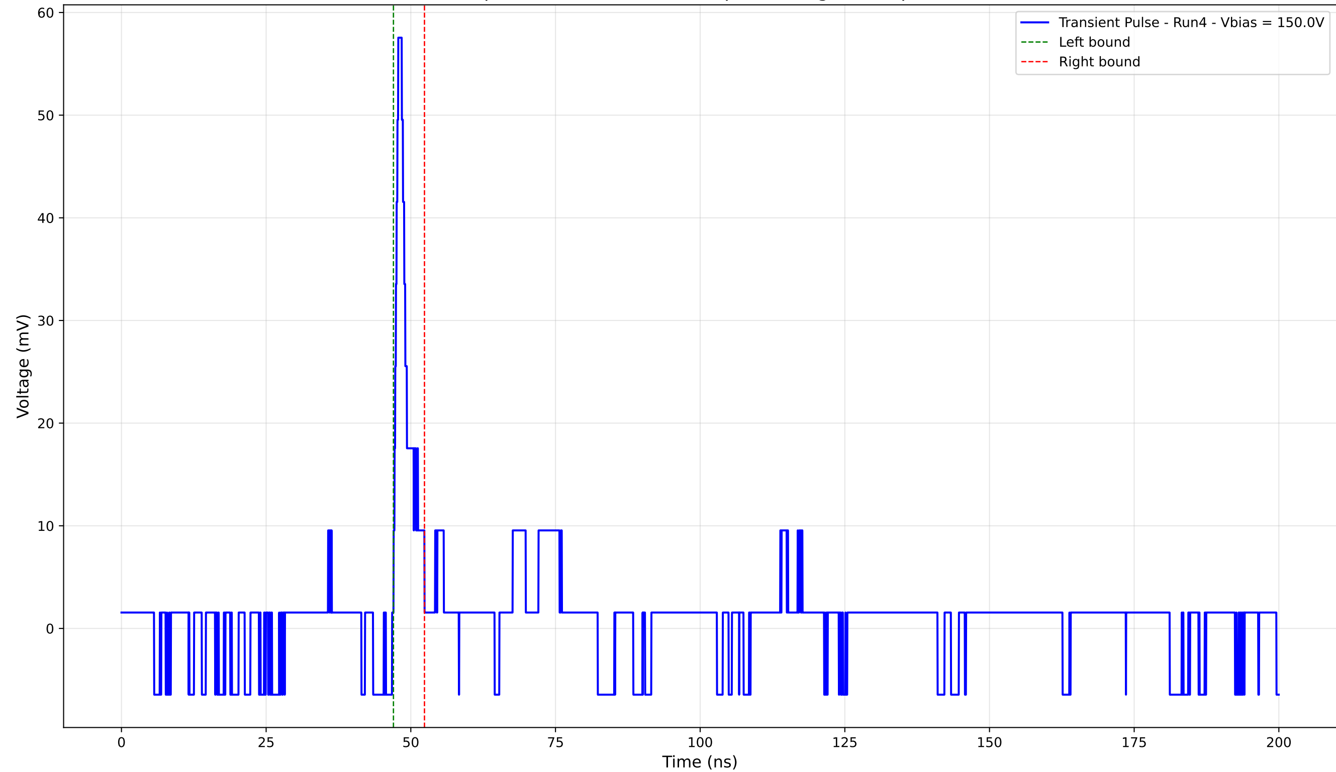
Transient Pulse - Sample: 4003 - Position: 65.0 \mu\text{m} - Charge: 2.67 pC - Rise Time: 0.81 ns
