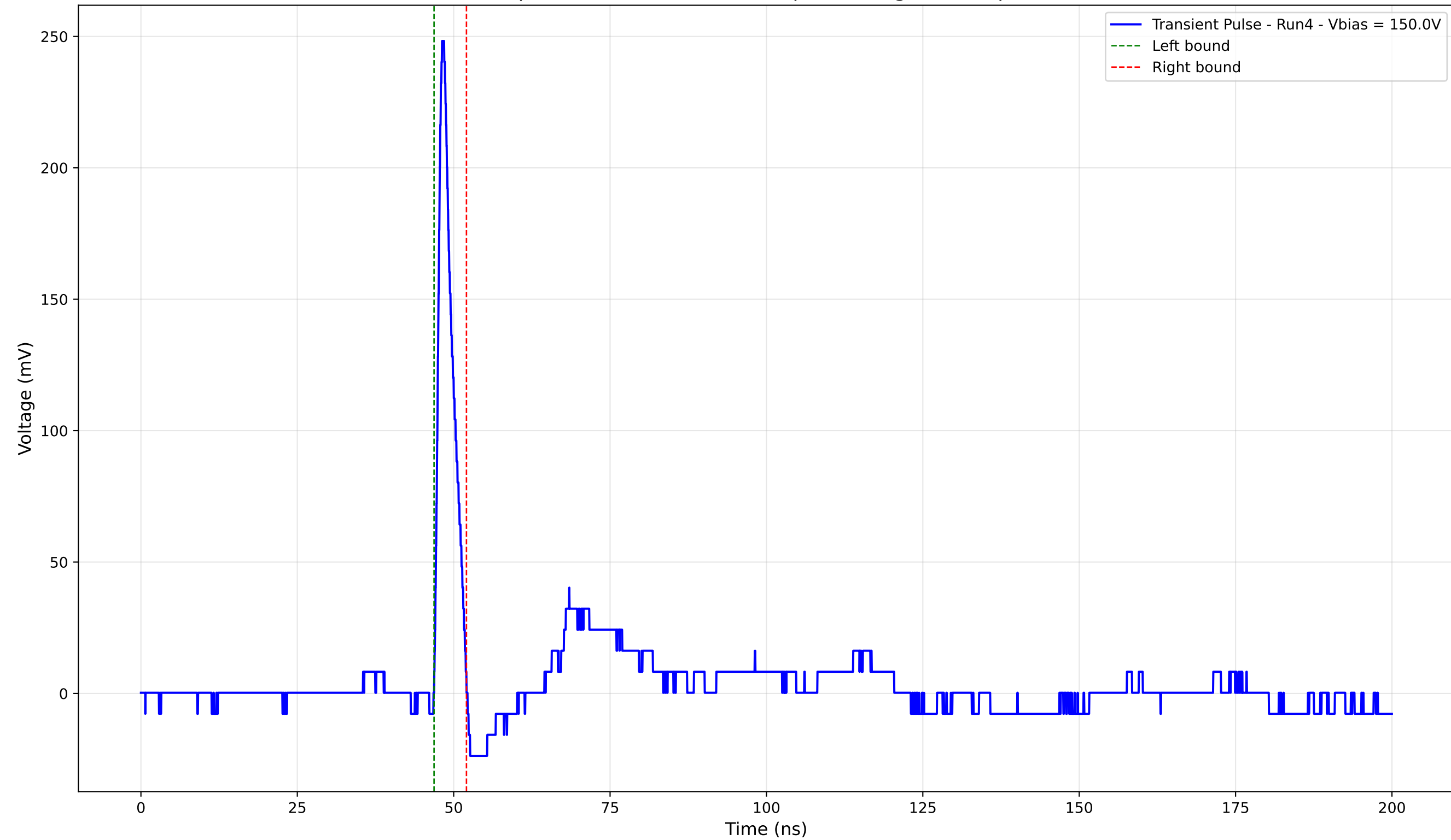
Transient Pulse - Sample: 4003 - Position: 465.0 \mu\text{m} - Charge: 12.77 pC - Rise Time: 0.88 ns
