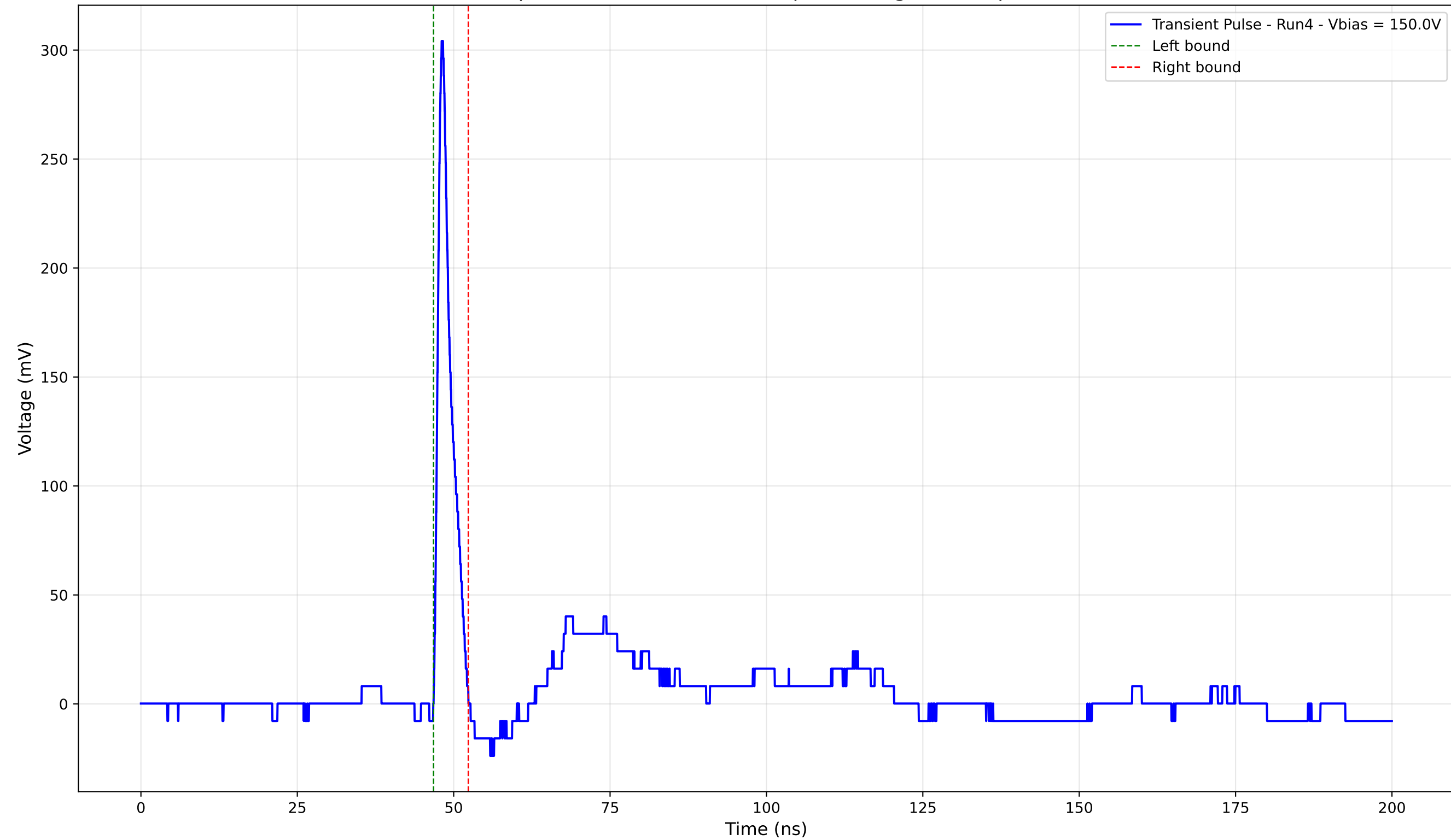
Transient Pulse - Sample: 4003 - Position: 260.0 \mu\text{m} - Charge: 14.82 pC - Rise Time: 0.90 ns
