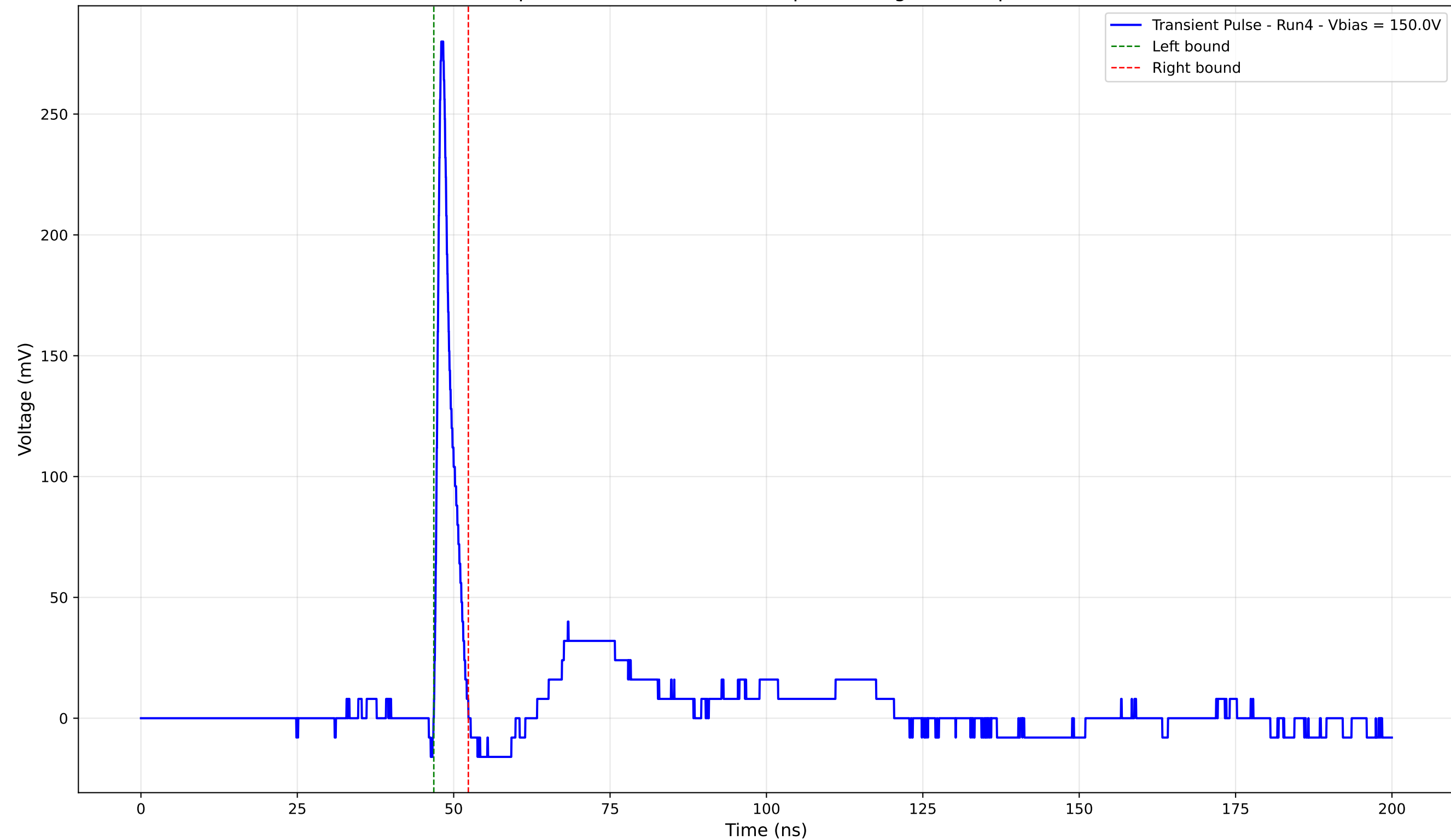
Transient Pulse - Sample: 4003 - Position: 240.0 \mu\text{m} - Charge: 13.59 pC - Rise Time: 0.83 ns
