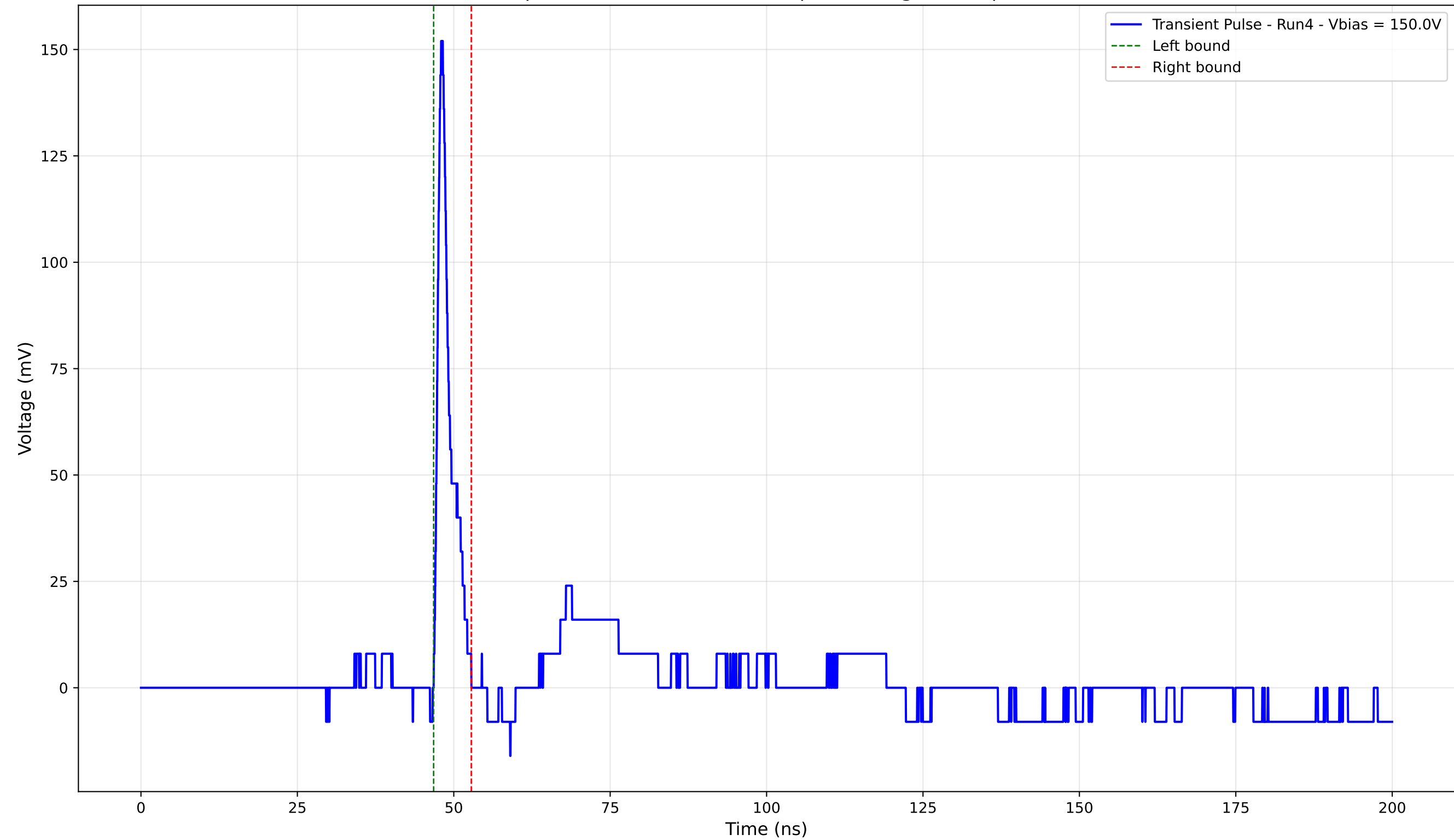
Transient Pulse - Sample: 4003 - Position: 140.0 \mu\text{m} - Charge: 7.14 pC - Rise Time: 0.92 ns
