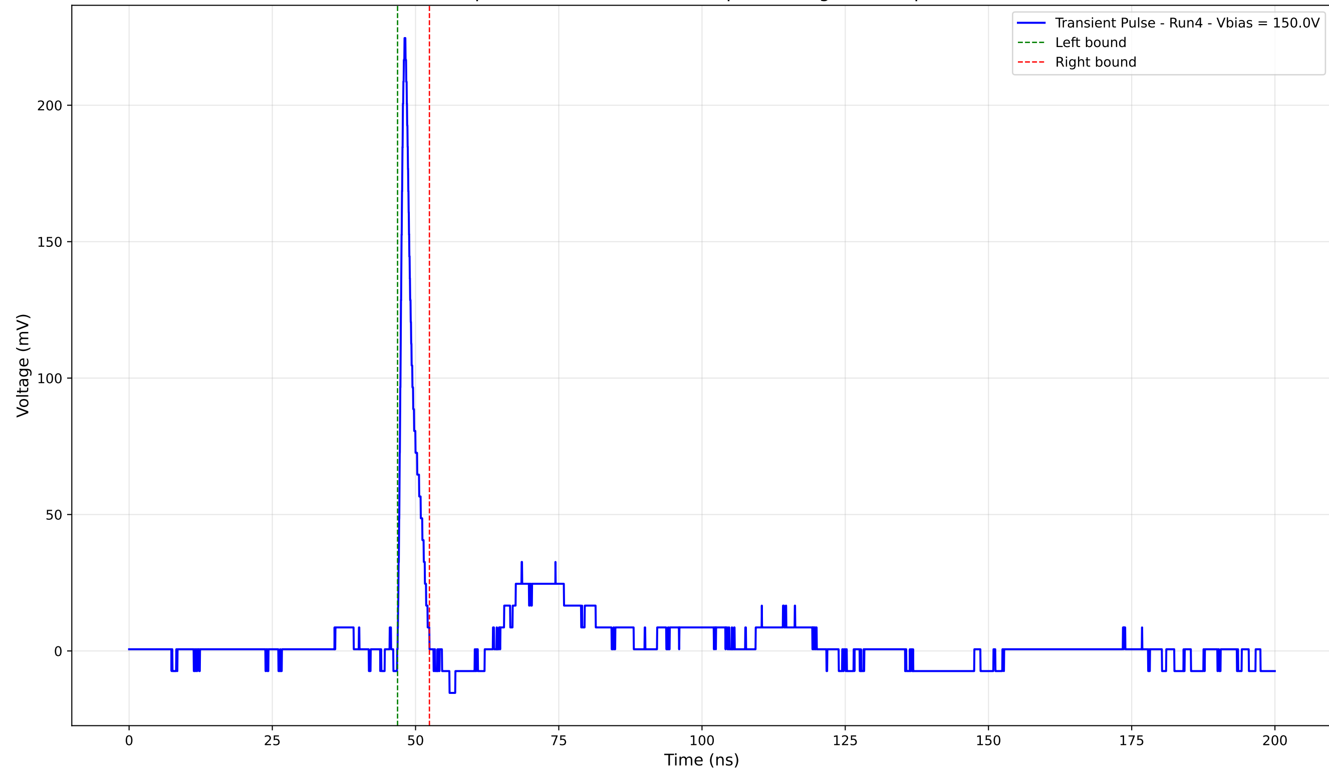
Transient Pulse - Sample: 4003 - Position: 190.0 \mu\text{m} - Charge: 10.45 pC - Rise Time: 0.87 ns
