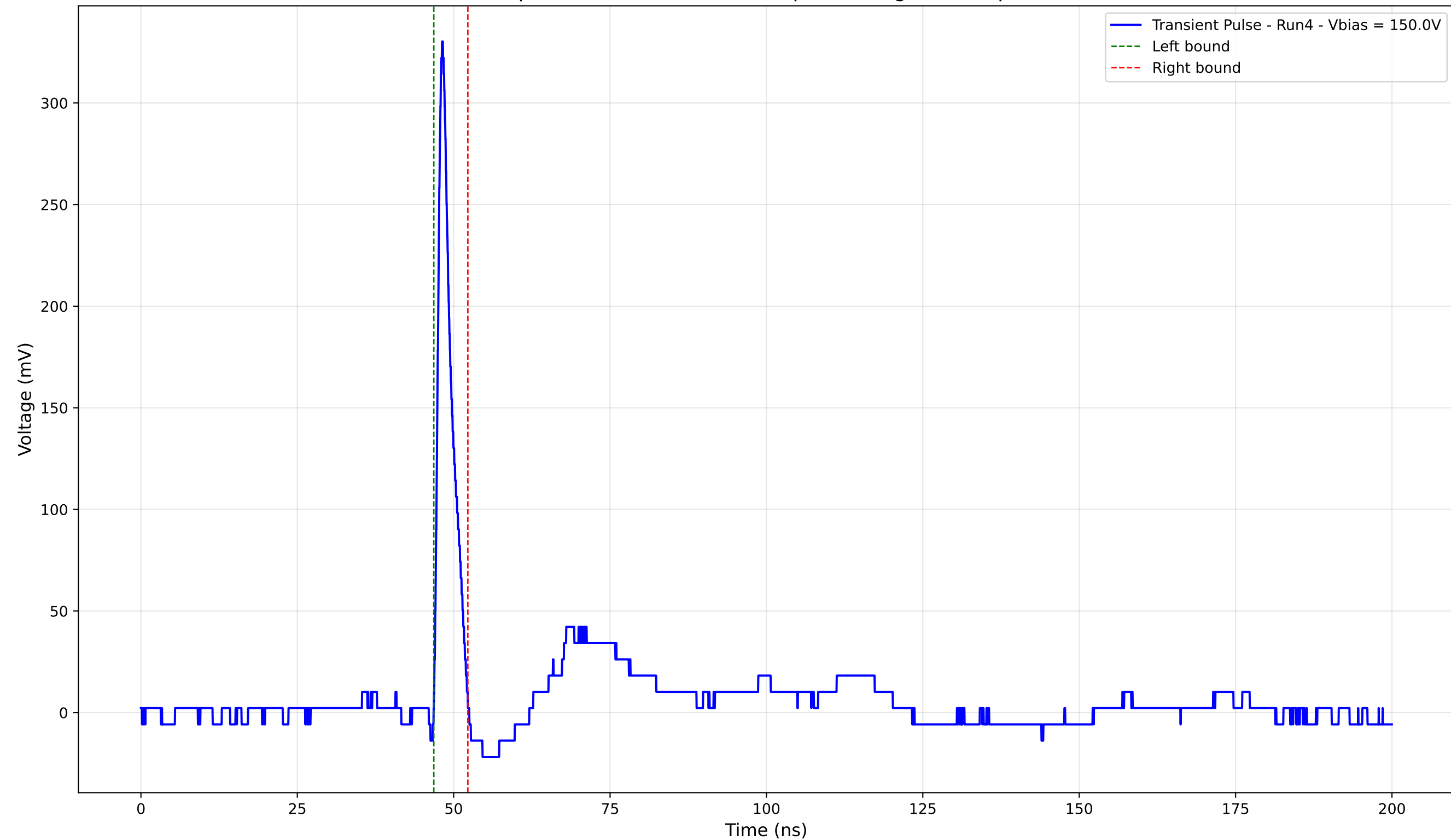
Transient Pulse - Sample: 4003 - Position: 285.0 \mu\text{m} - Charge: 16.21 pC - Rise Time: 0.88 ns
