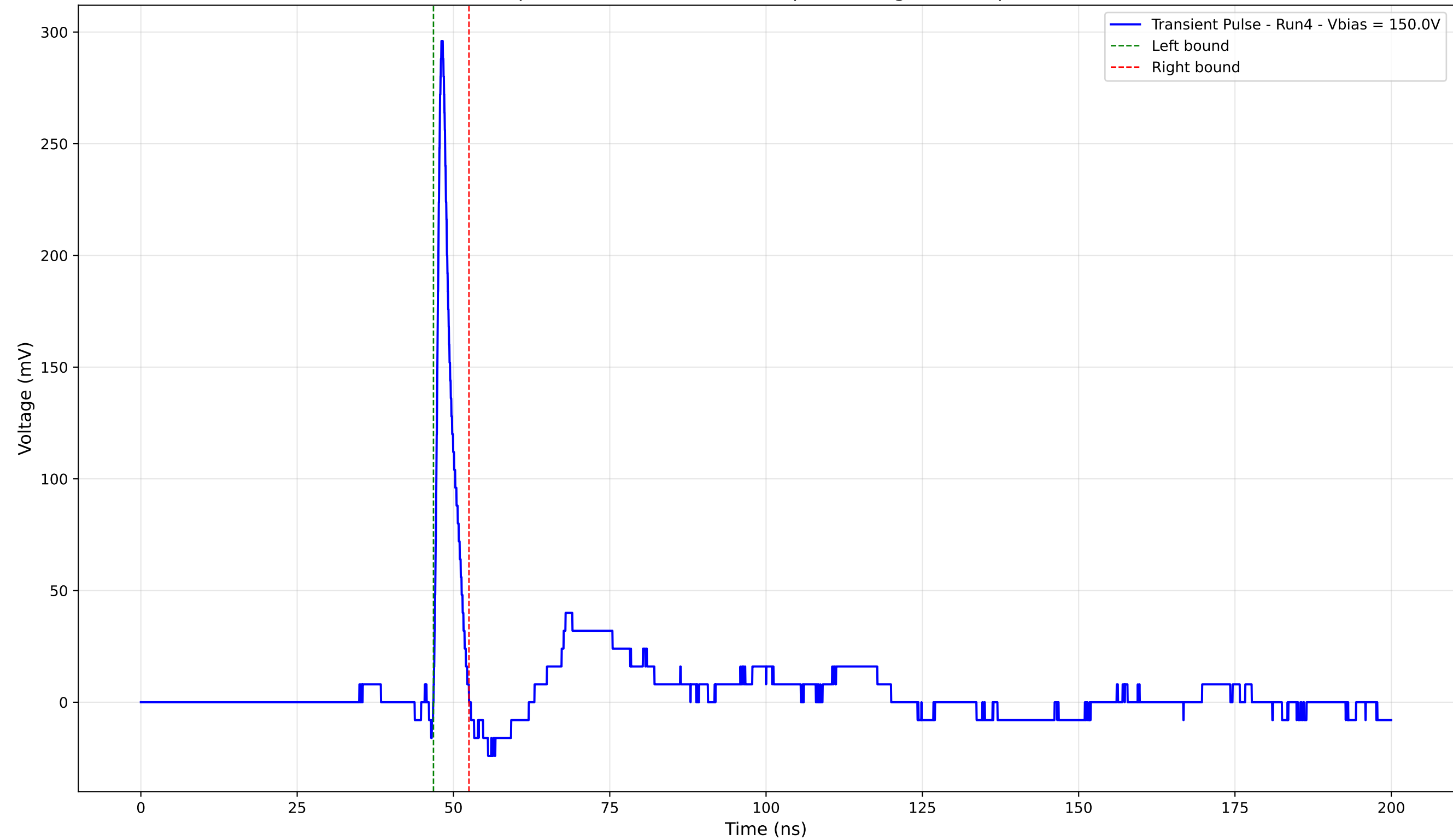
Transient Pulse - Sample: 4003 - Position: 250.0 \mu\text{m} - Charge: 14.39 pC - Rise Time: 0.89 ns
