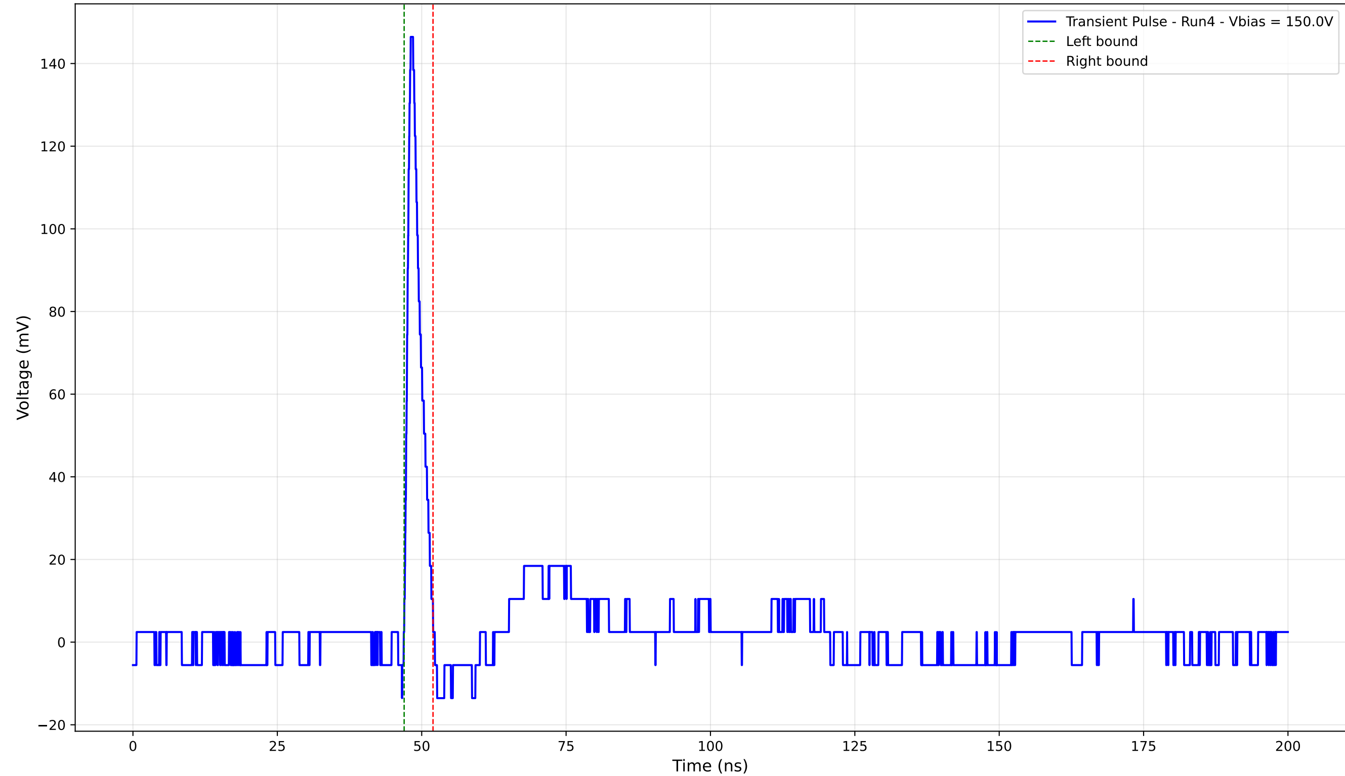
Transient Pulse - Sample: 4003 - Position: 565.0 \mu\text{m} - Charge: 7.37 pC - Rise Time: 0.91 ns
