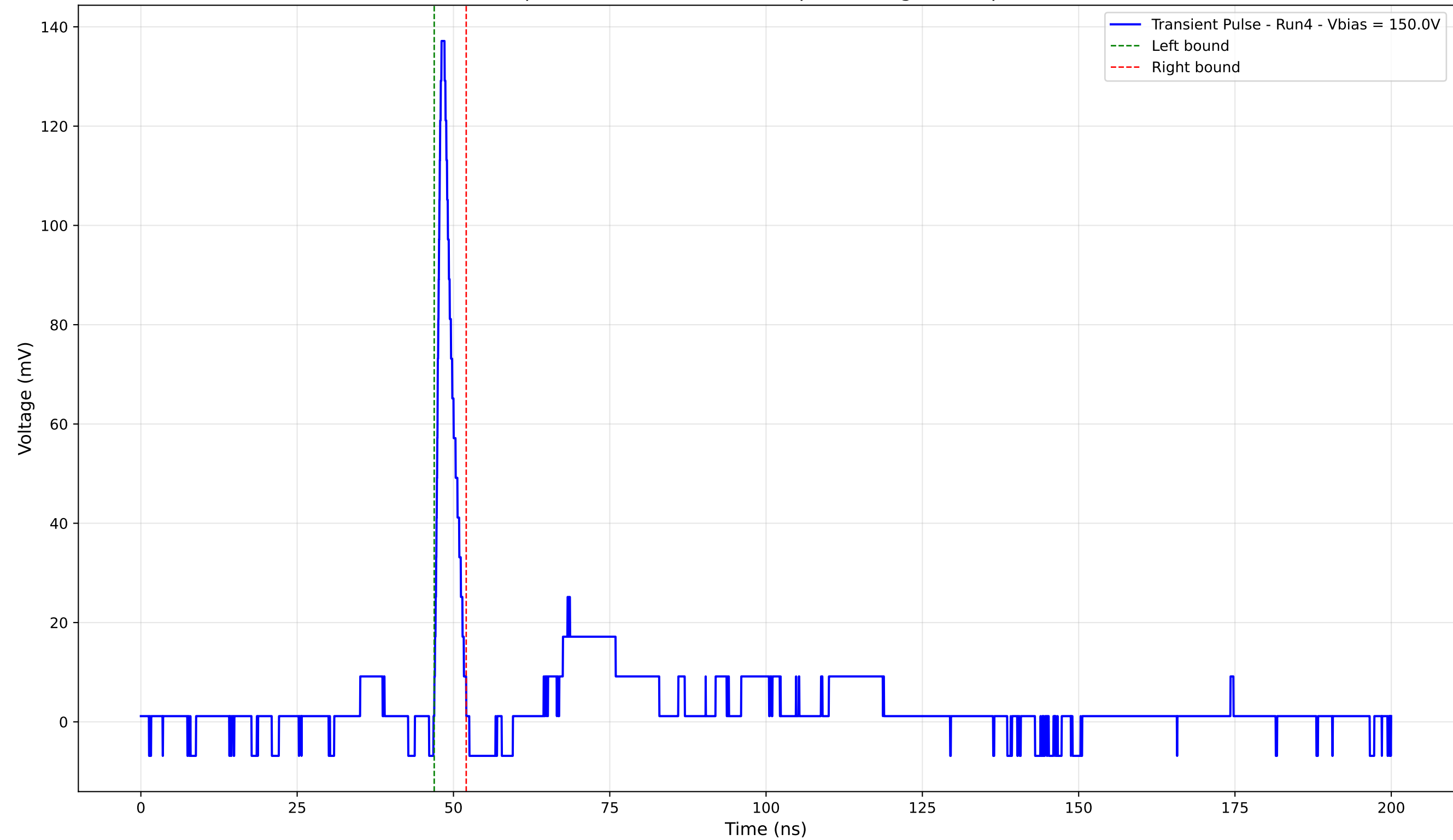
Transient Pulse - Sample: 4003 - Position: 600.0 \mu\text{m} - Charge: 6.98 pC - Rise Time: 0.93 ns
