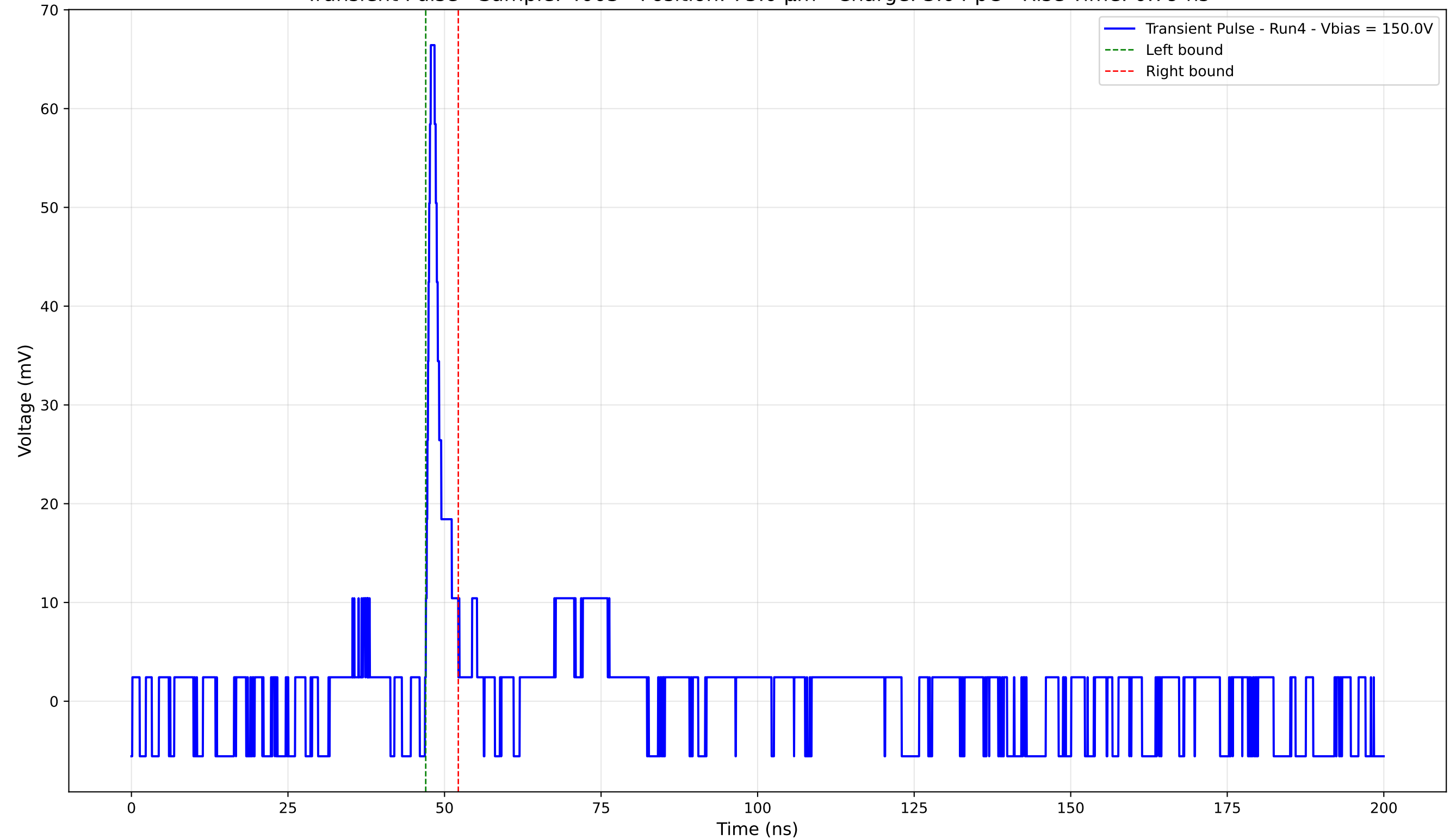
Transient Pulse - Sample: 4003 - Position: 75.0 \mu\text{m} - Charge: 3.04 pC - Rise Time: 0.79 ns
