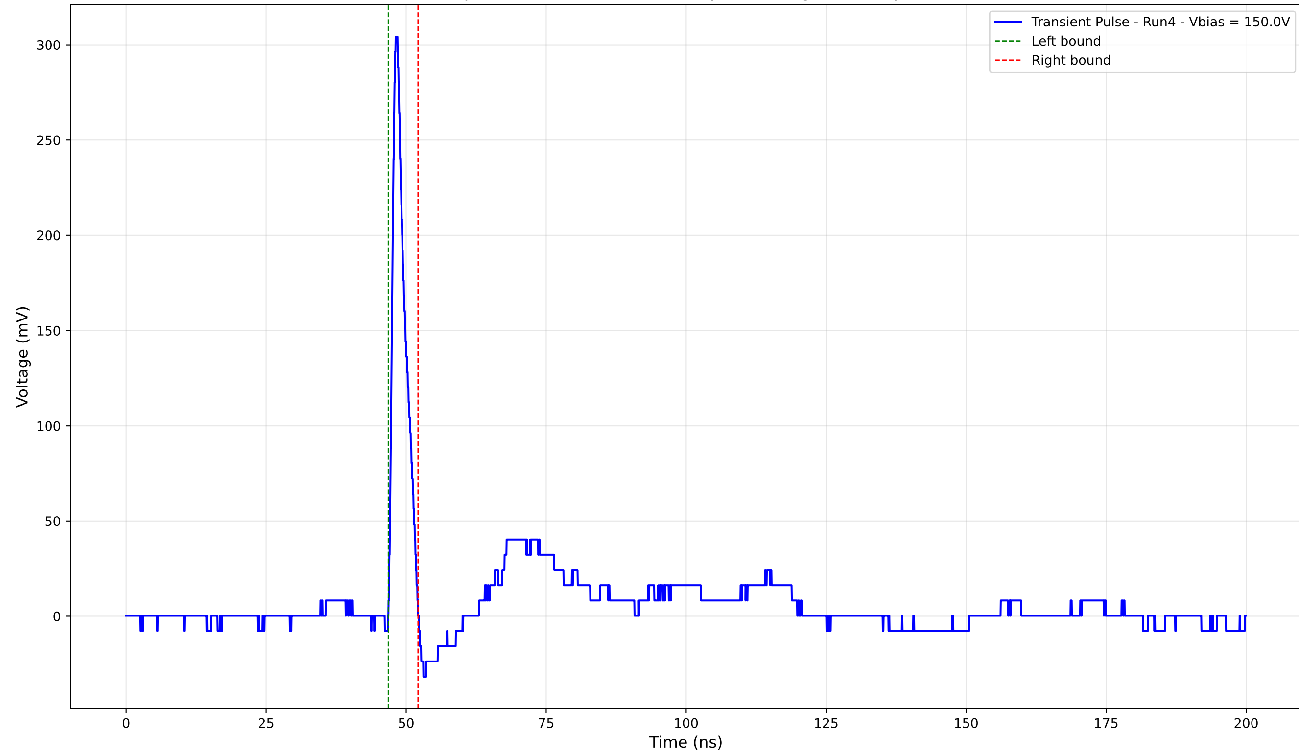
Transient Pulse - Sample: 4003 - Position: 415.0 \mu\text{m} - Charge: 15.77 pC - Rise Time: 0.92 ns
