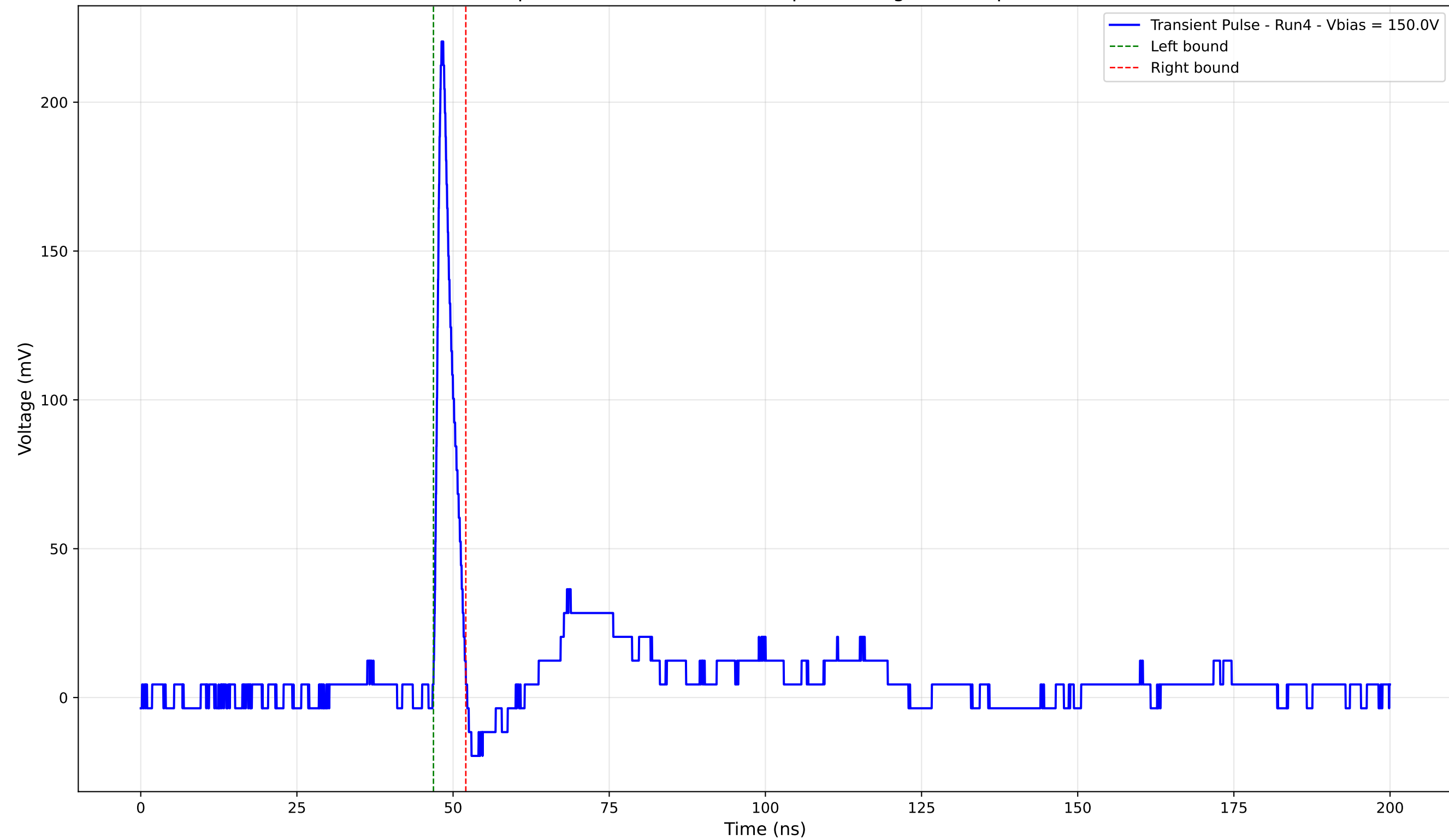
Transient Pulse - Sample: 4003 - Position: 490.0 \mu\text{m} - Charge: 11.46 pC - Rise Time: 0.96 ns
