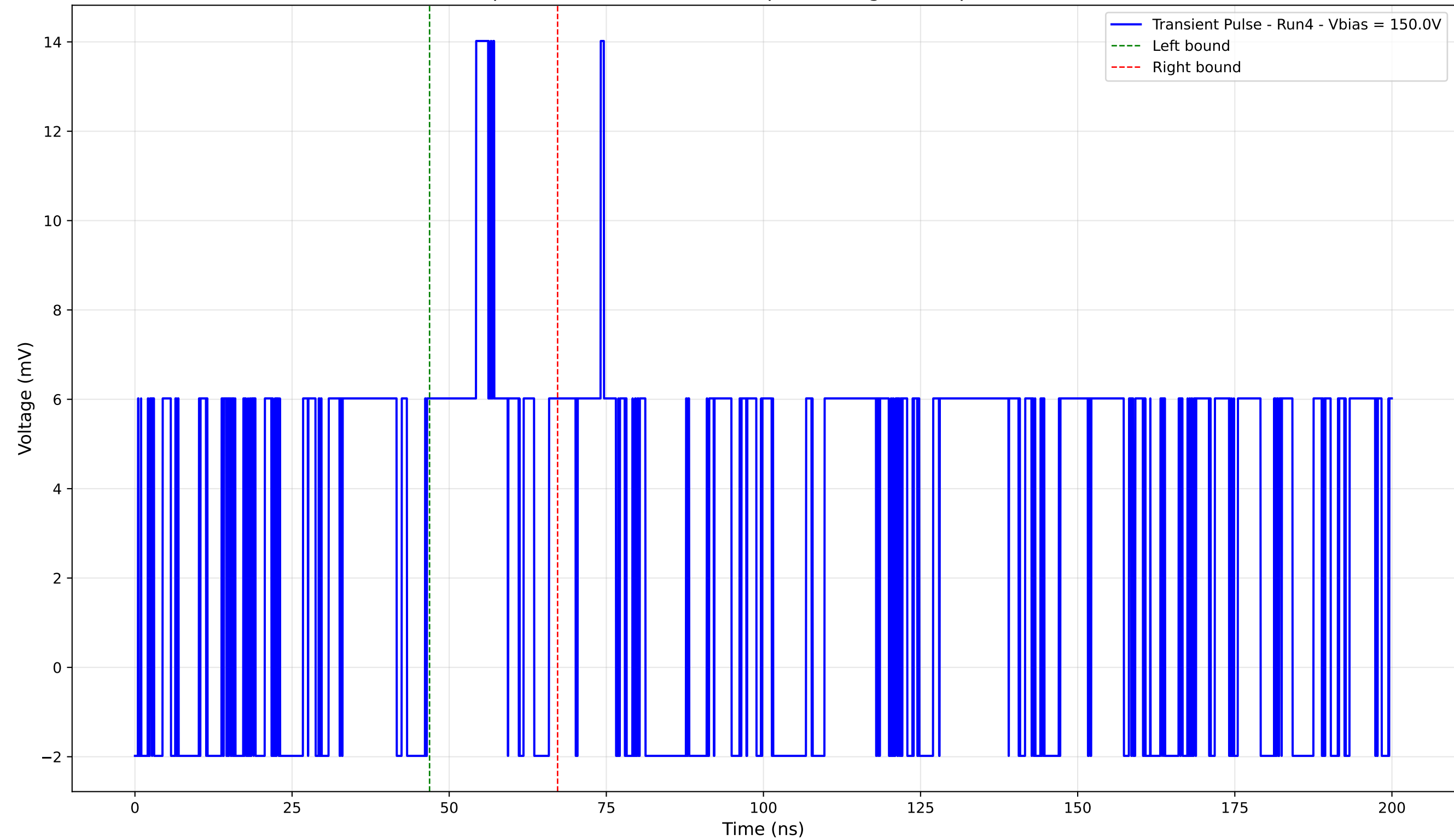
Transient Pulse - Sample: 4003 - Position: 650.0 \mu\text{m} - Charge: 2.30 pC - Rise Time: 0.00 ns (N/A)
