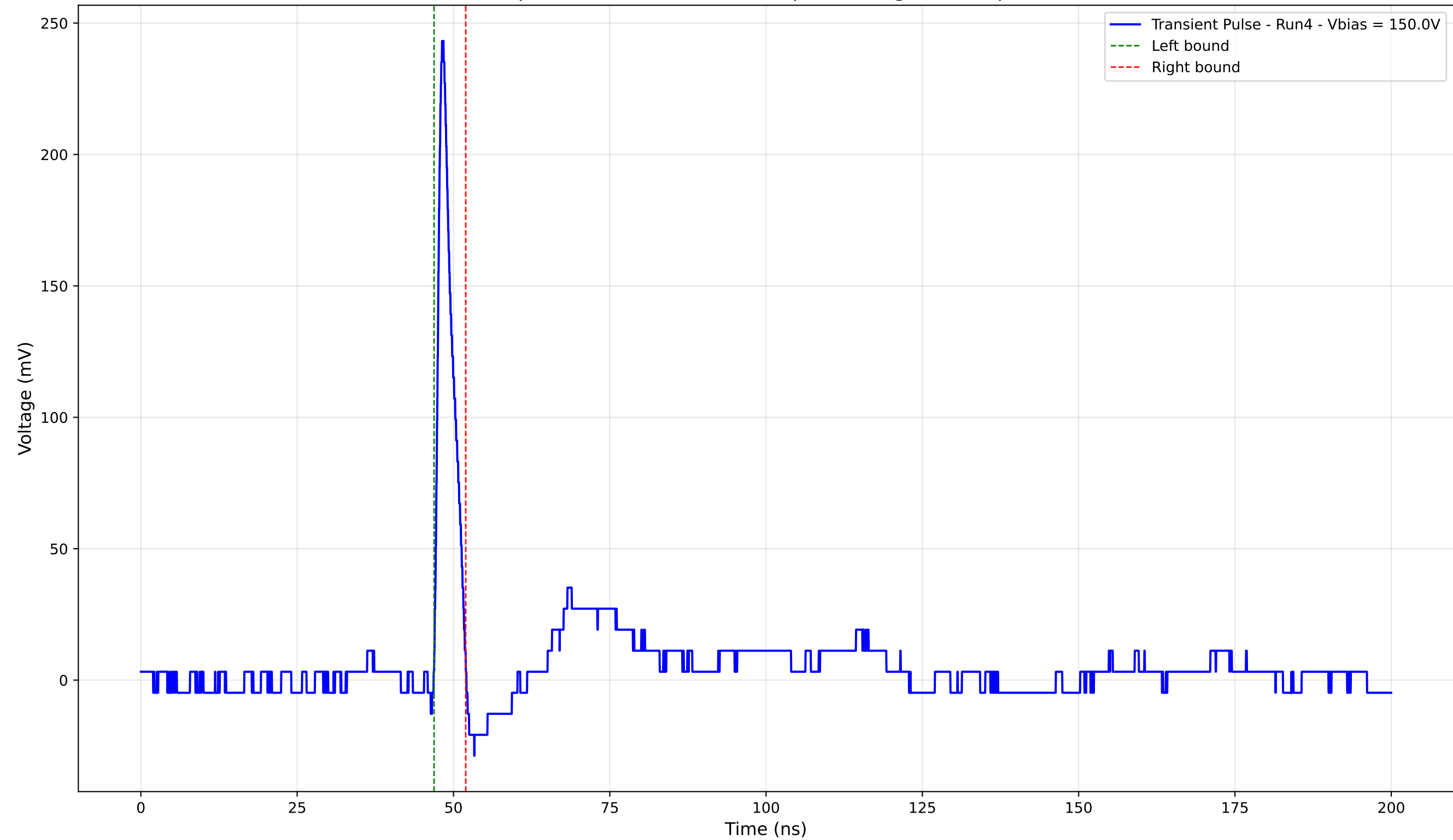
Transient Pulse - Sample: 4003 - Position: 470.0 \mu\text{m} - Charge: 12.51 pC - Rise Time: 0.91 ns
