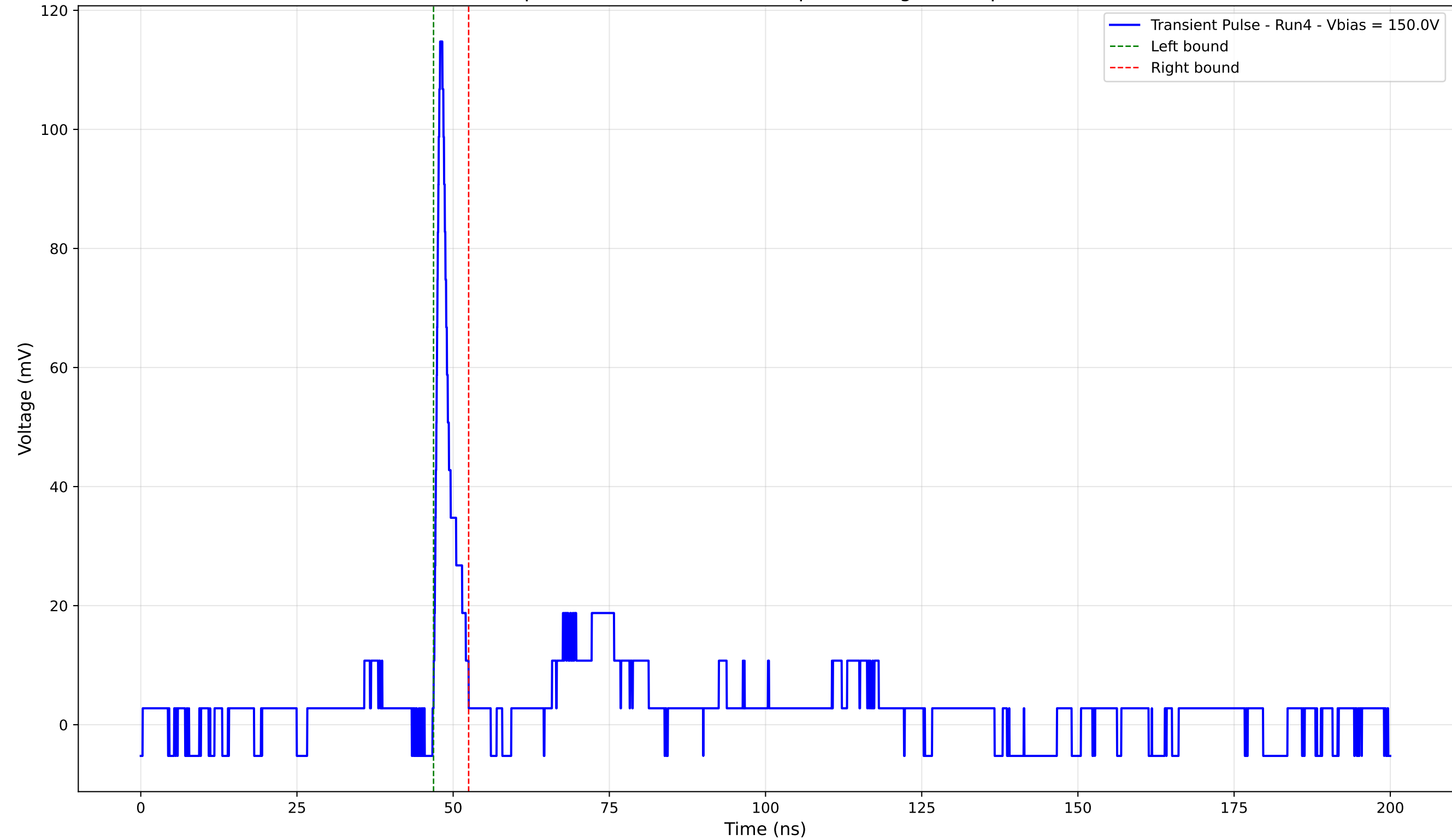
Transient Pulse - Sample: 4003 - Position: 115.0 \mu\text{m} - Charge: 5.37 pC - Rise Time: 0.80 ns
