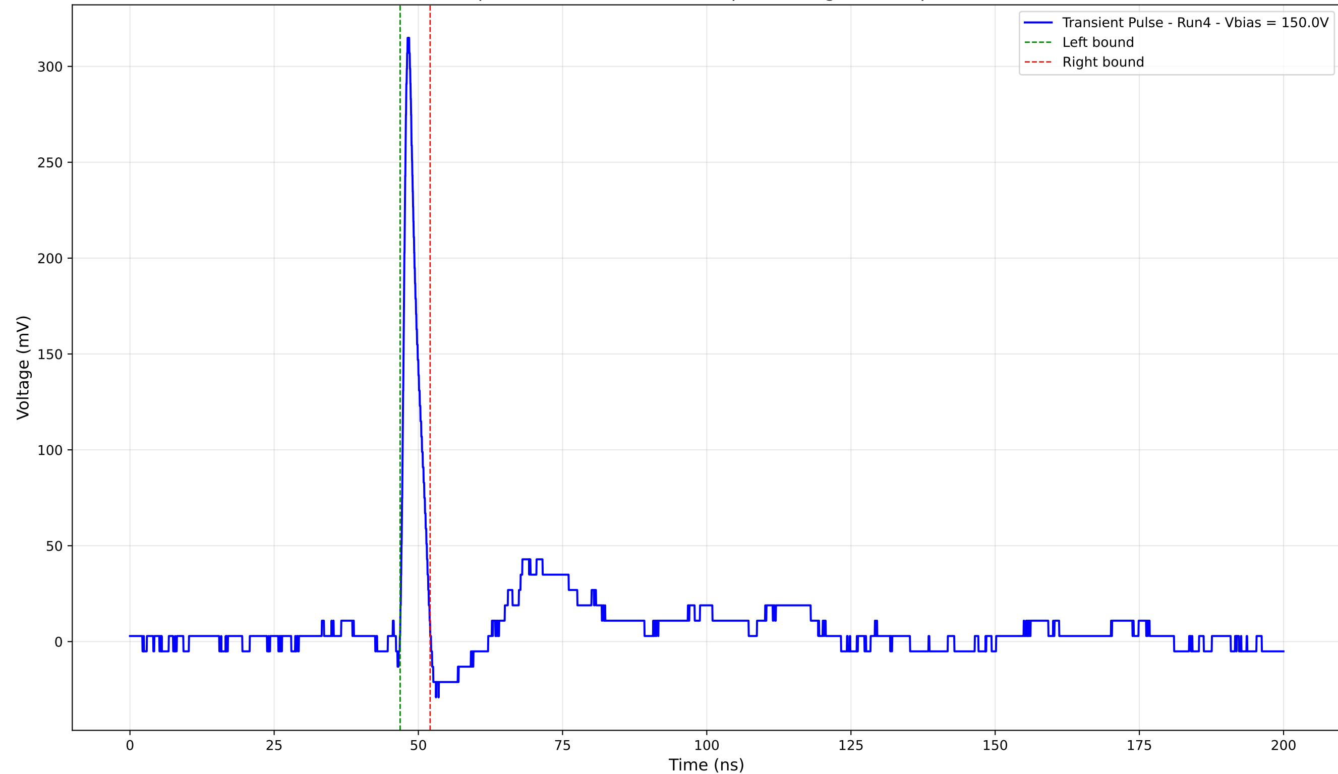
Transient Pulse - Sample: 4003 - Position: 405.0 \mu\text{m} - Charge: 16.08 pC - Rise Time: 0.93 ns
