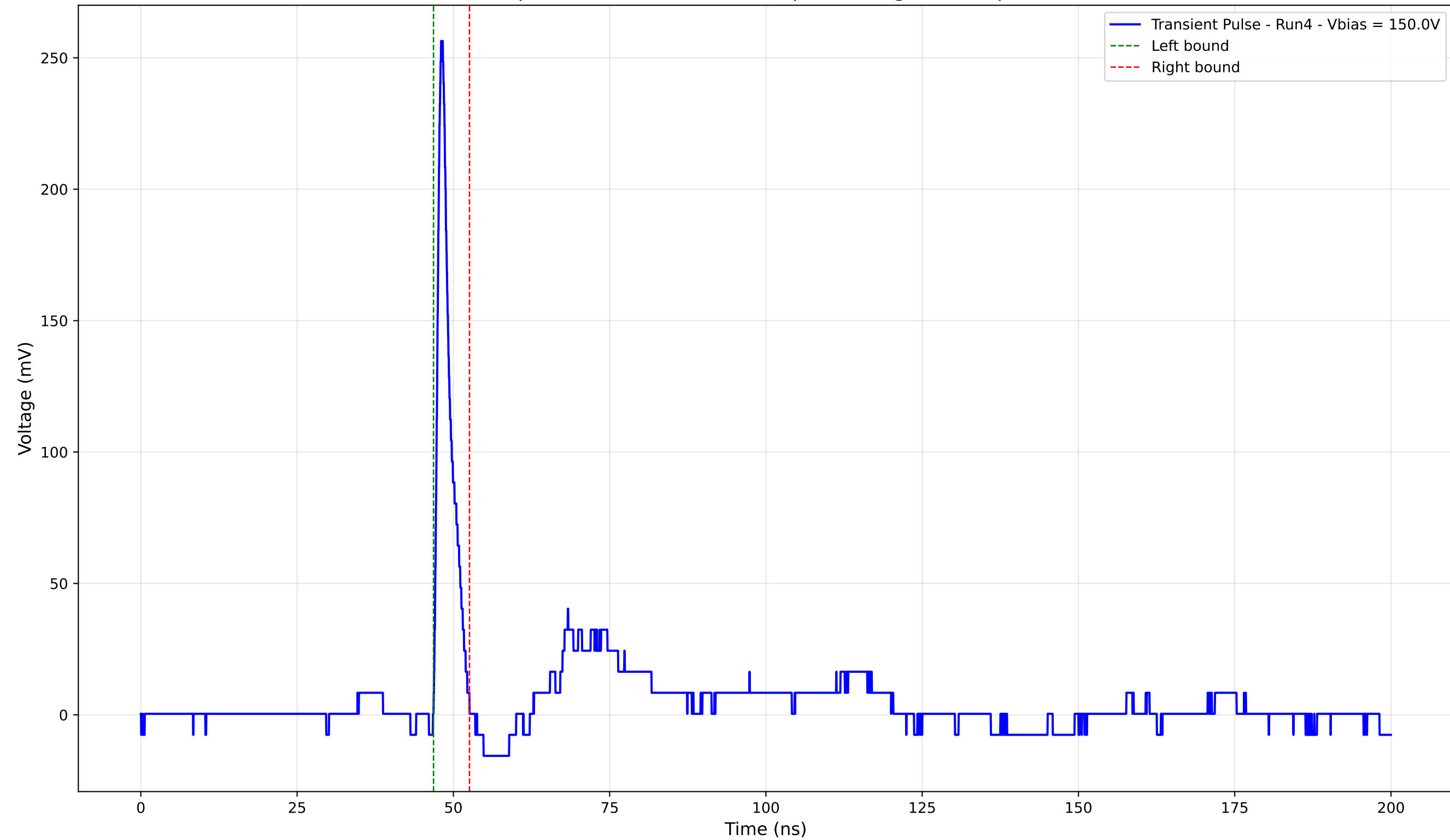
Transient Pulse - Sample: 4003 - Position: 215.0 \mu\text{m} - Charge: 12.24 pC - Rise Time: 0.84 ns
