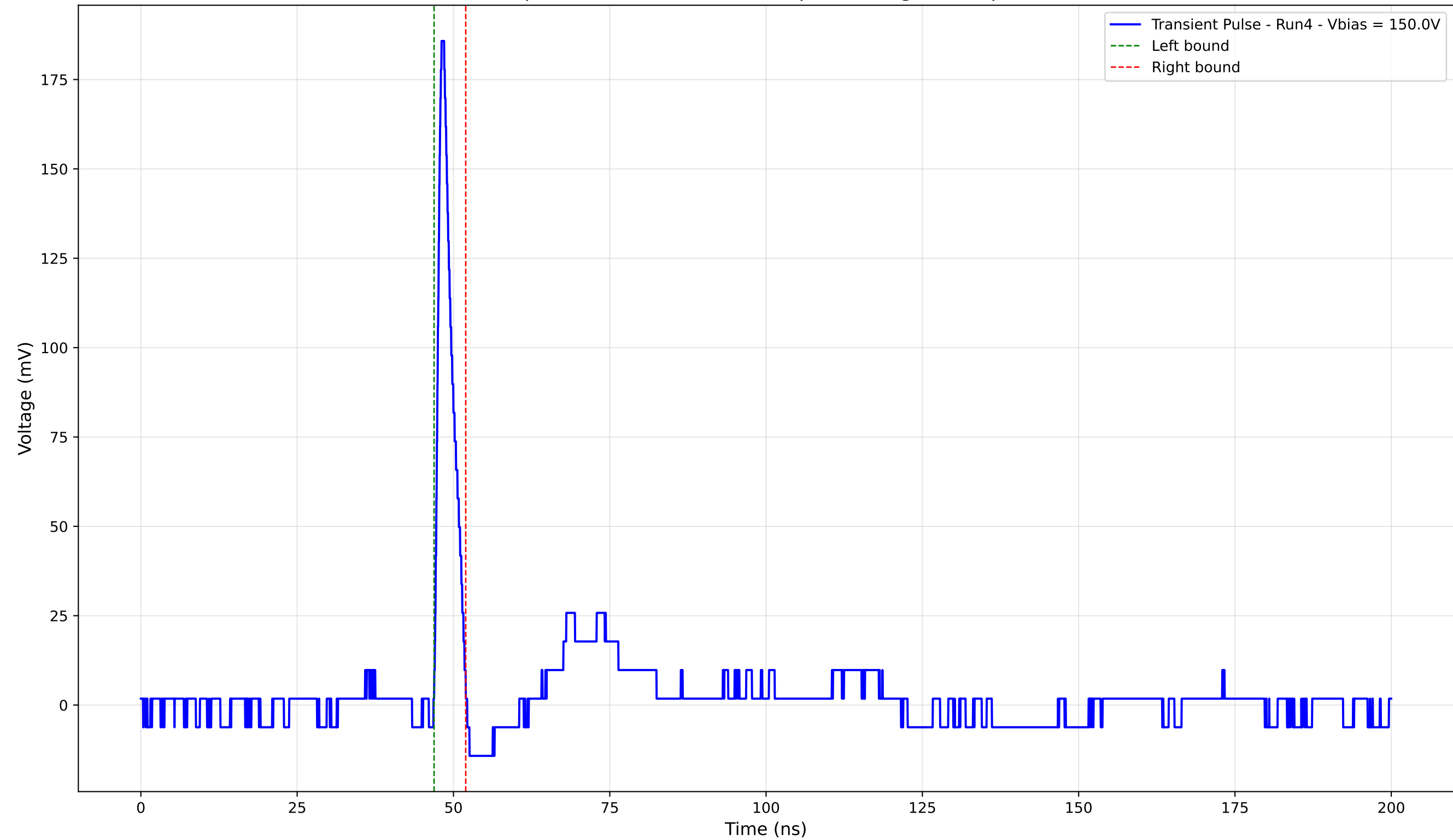
Transient Pulse - Sample: 4003 - Position: 530.0 \mu\text{m} - Charge: 9.51 pC - Rise Time: 0.84 ns
