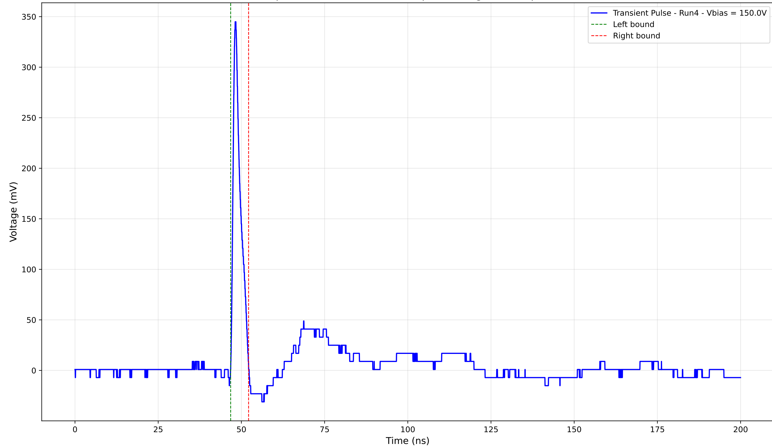
Transient Pulse - Sample: 4003 - Position: 325.0 \mu\text{m} - Charge: 17.37 pC - Rise Time: 0.90 ns
