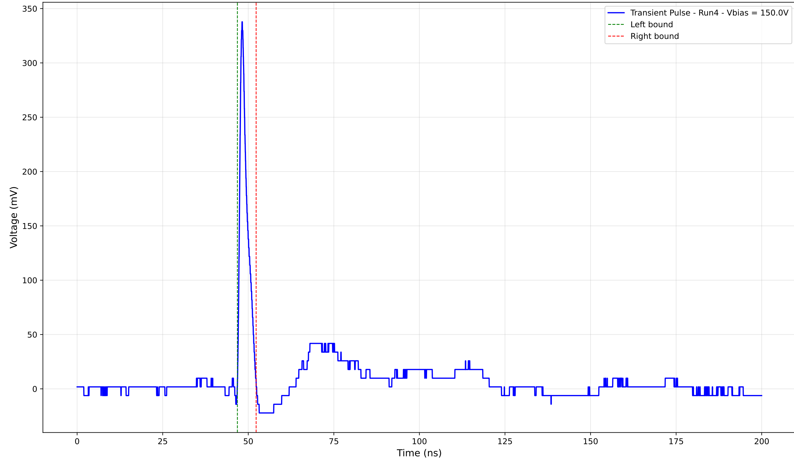
Transient Pulse - Sample: 4003 - Position: 300.0 \mu\text{m} - Charge: 16.79 pC - Rise Time: 0.90 ns
