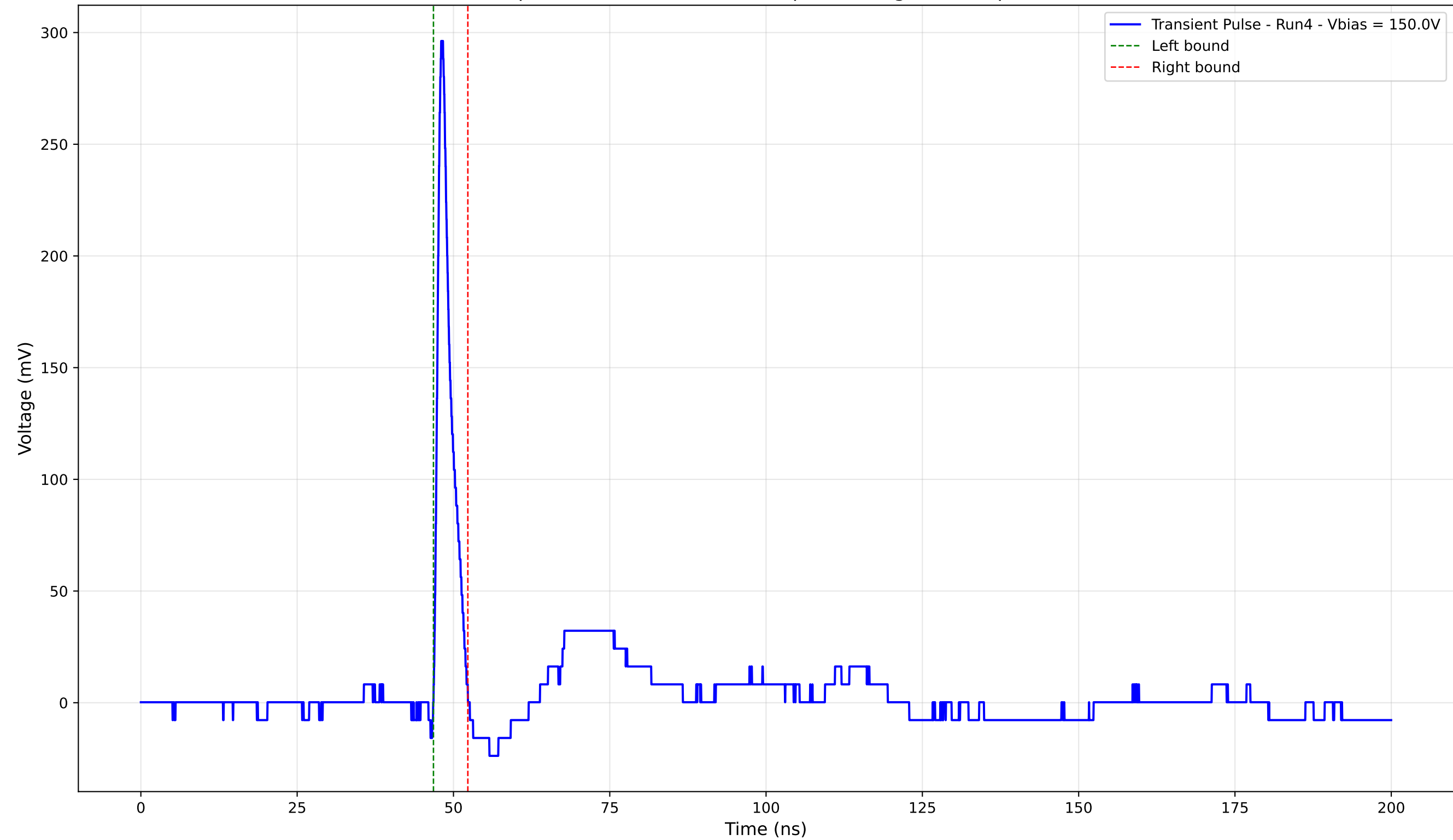
Transient Pulse - Sample: 4003 - Position: 255.0 \mu\text{m} - Charge: 14.39 pC - Rise Time: 0.89 ns
