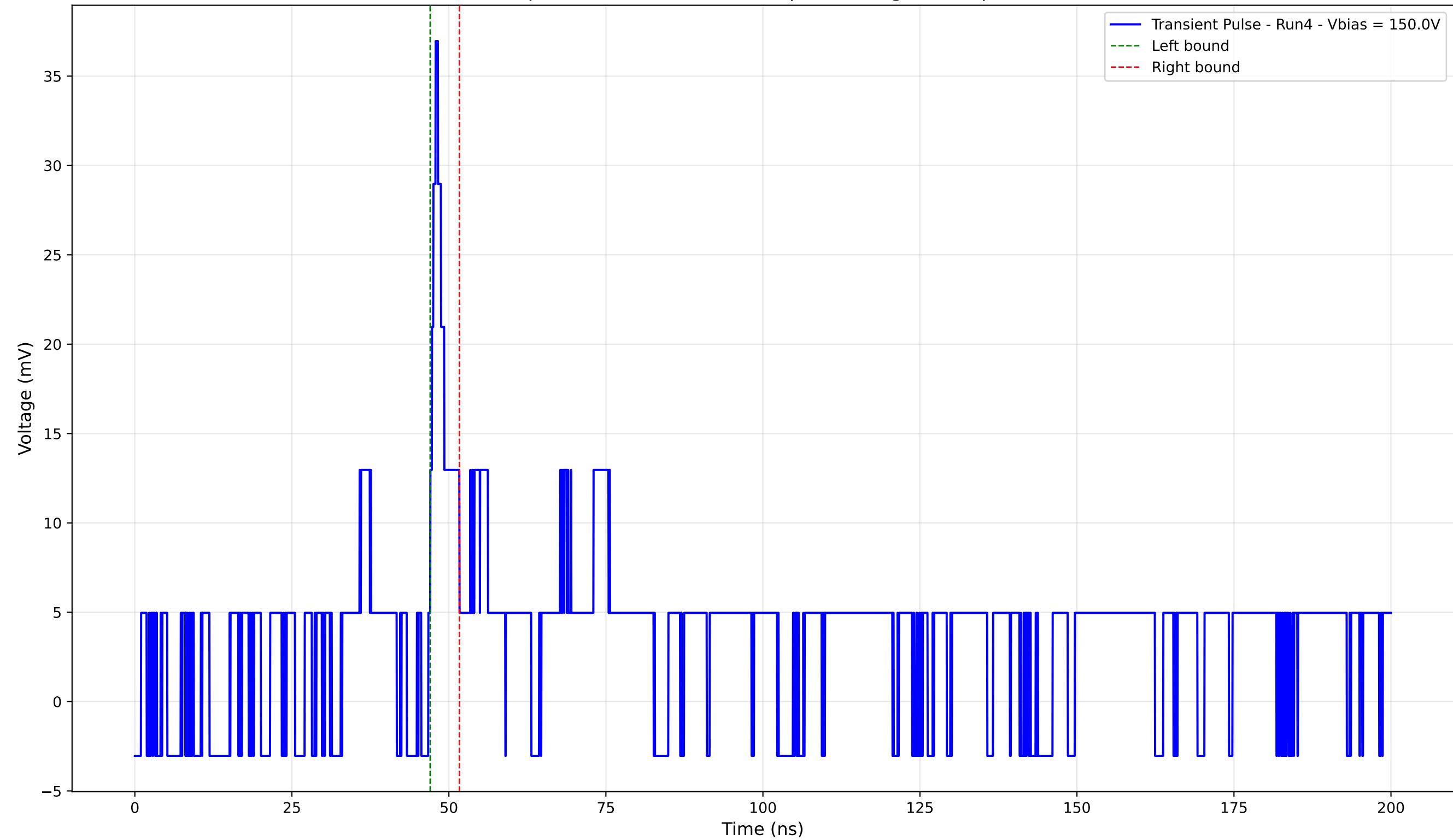
Transient Pulse - Sample: 4003 - Position: 45.0 \mu\text{m} - Charge: 1.77 pC - Rise Time: 1.17 ns
