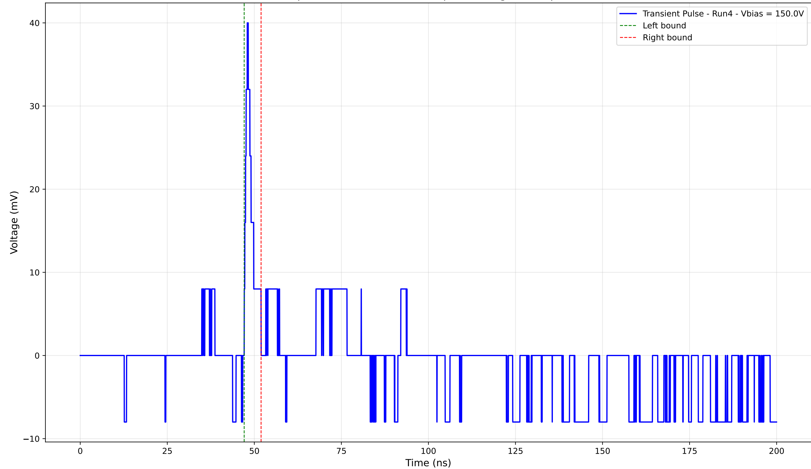
Transient Pulse - Sample: 4003 - Position: 50.0 \mu\text{m} - Charge: 1.66 pC - Rise Time: 0.87 ns
