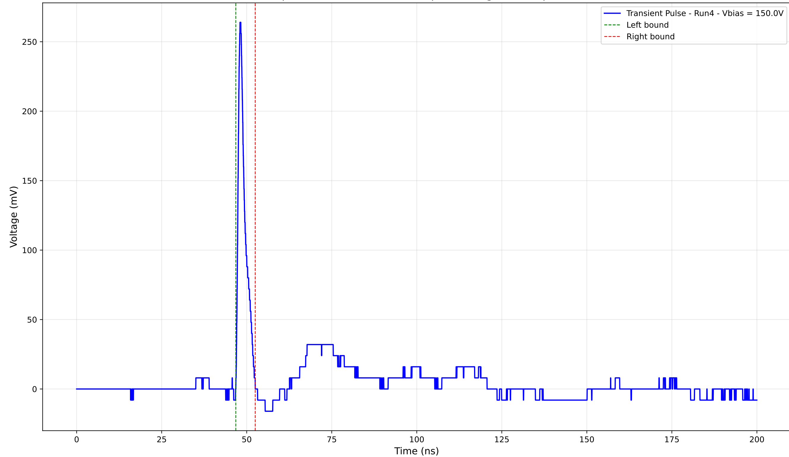
Transient Pulse - Sample: 4003 - Position: 220.0 \mu\text{m} - Charge: 12.66 pC - Rise Time: 0.83 ns
