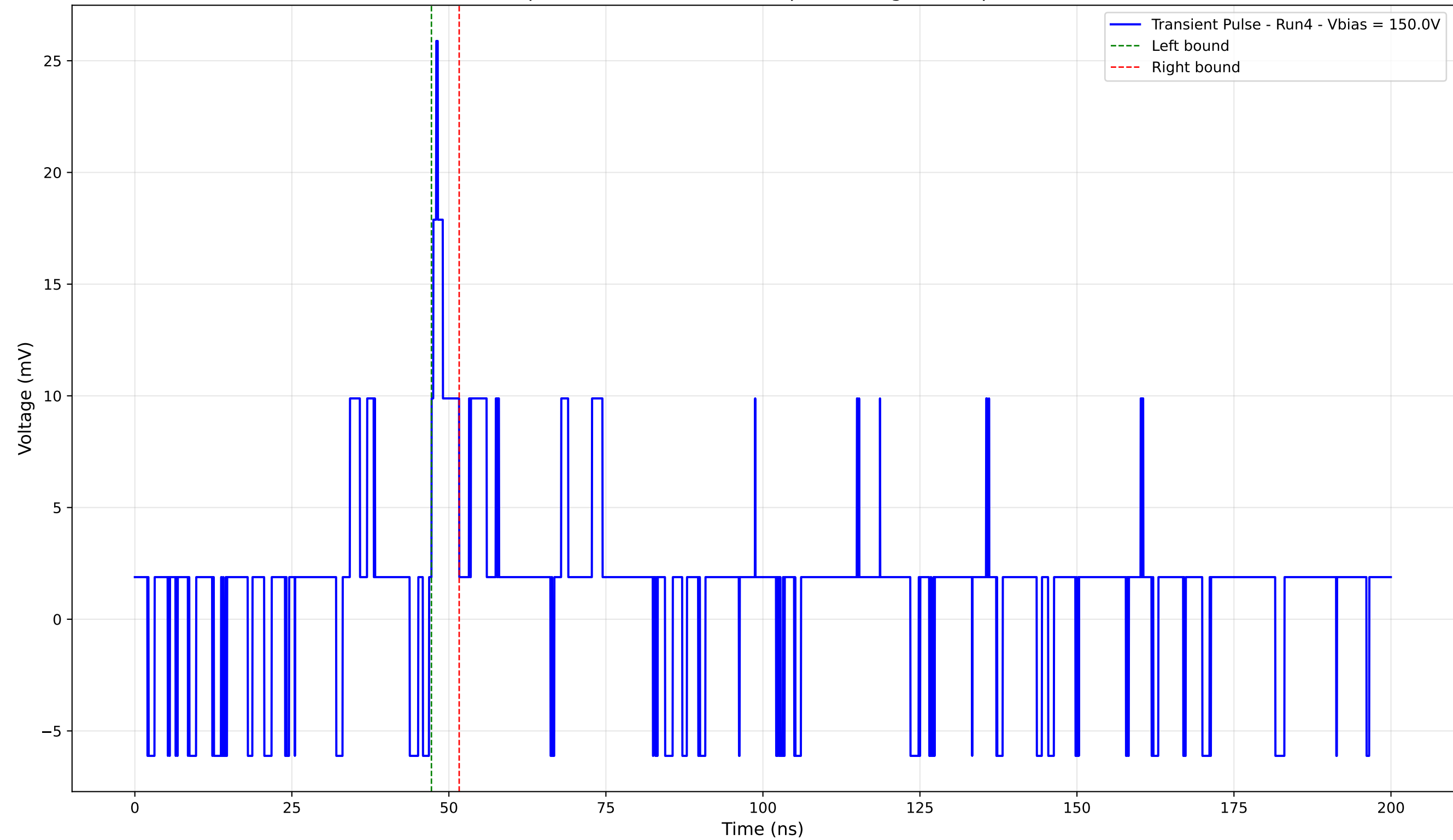
Transient Pulse - Sample: 4003 - Position: 30.0 \mu\text{m} - Charge: 1.16 pC - Rise Time: 0.76 ns
