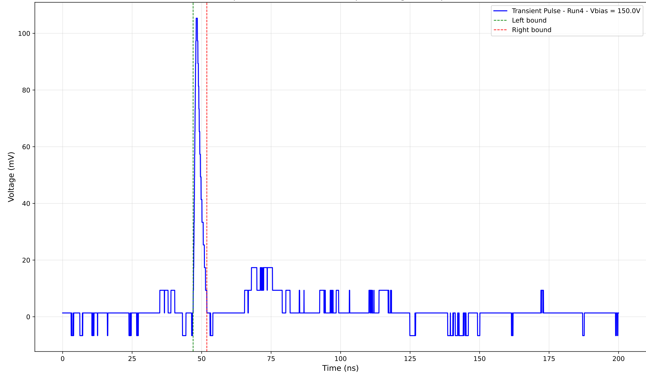
Transient Pulse - Sample: 4003 - Position: 605.0 \mu\text{m} - Charge: 5.00 pC - Rise Time: 0.86 ns
