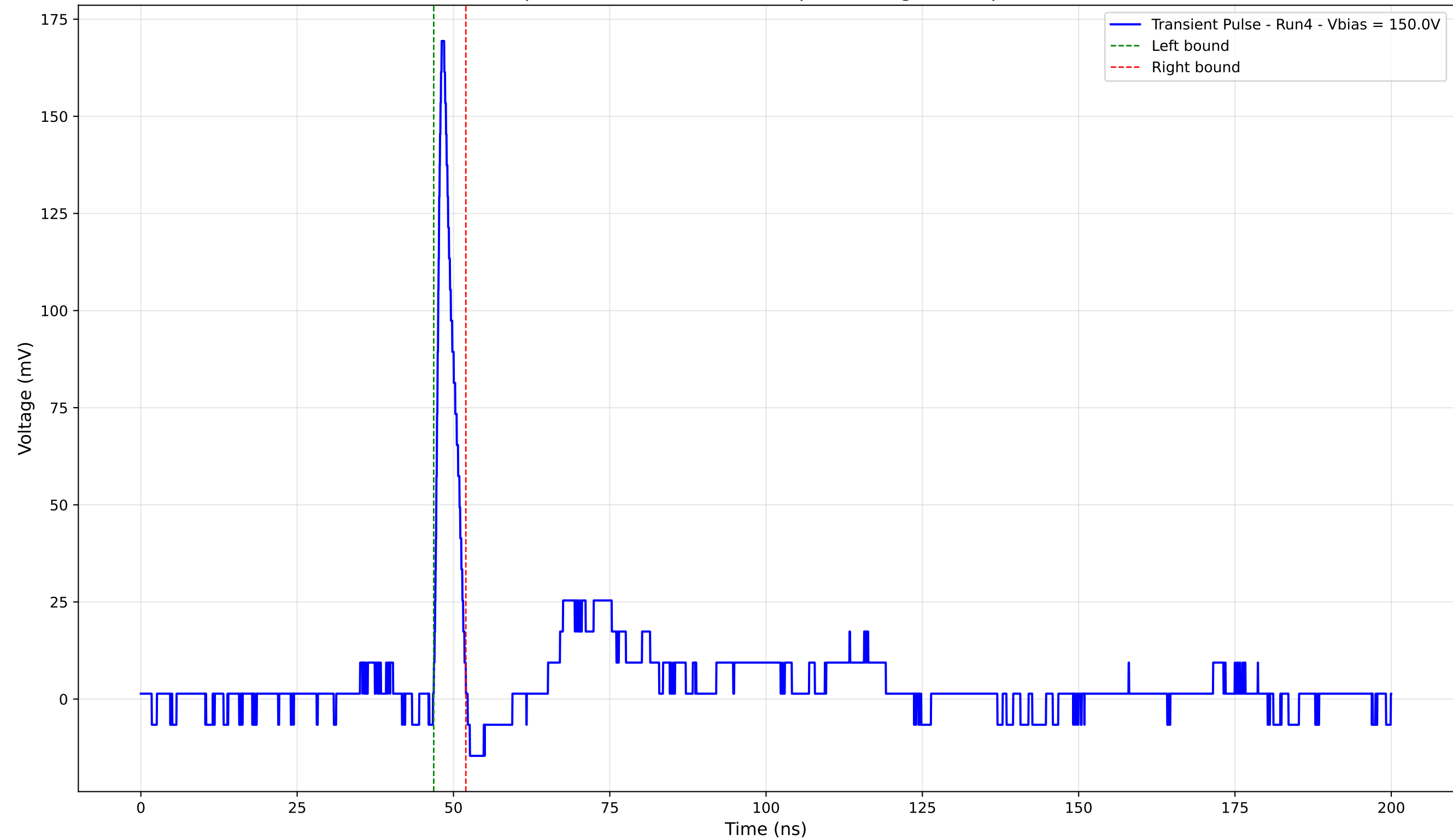
Transient Pulse - Sample: 4003 - Position: 550.0 \mu\text{m} - Charge: 9.04 pC - Rise Time: 0.94 ns
