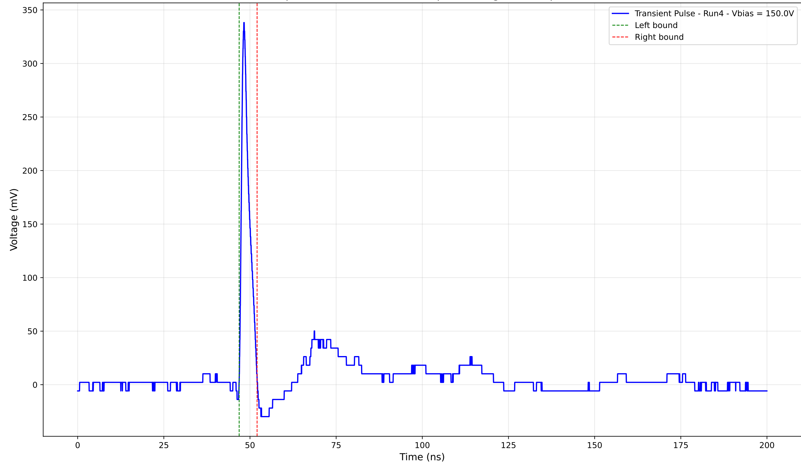
Transient Pulse - Sample: 4003 - Position: 380.0 \mu\text{m} - Charge: 16.87 pC - Rise Time: 0.90 ns
