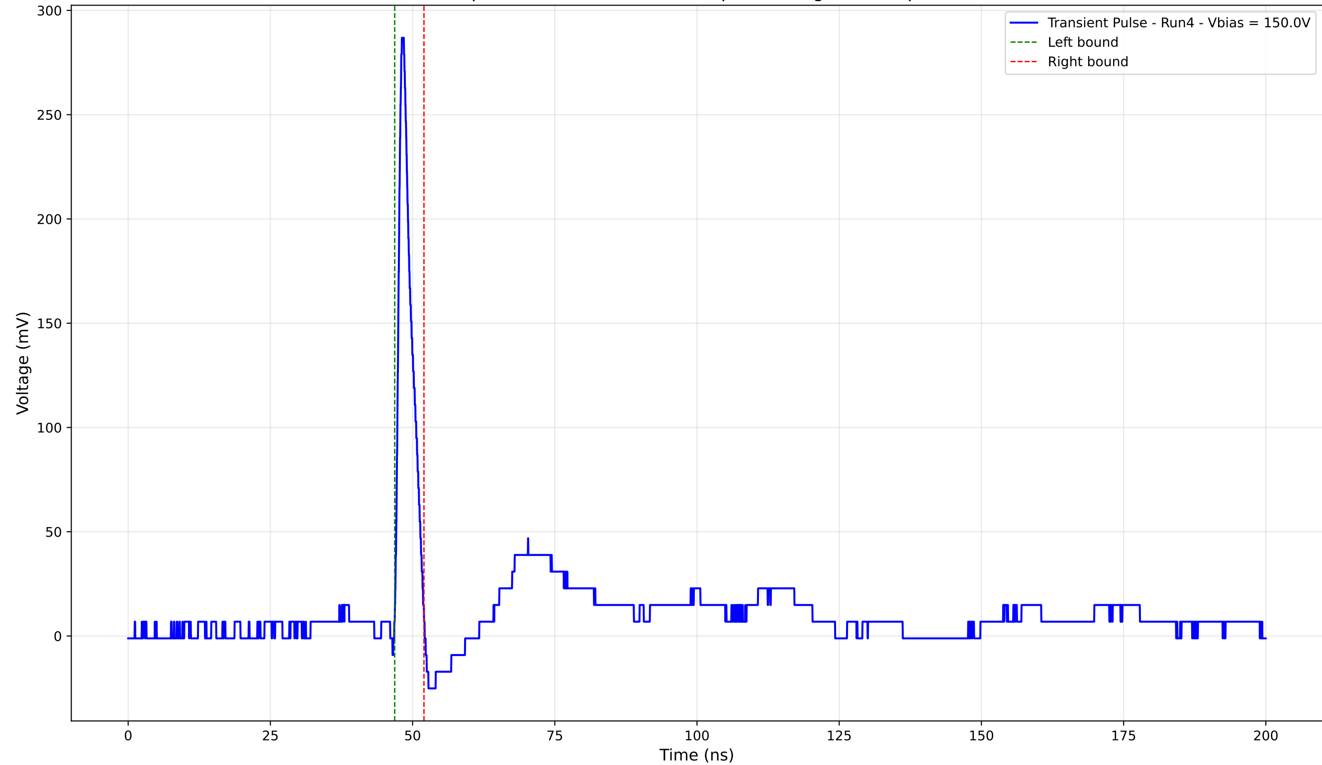
Transient Pulse - Sample: 4003 - Position: 435.0 \mu\text{m} - Charge: 14.87 pC - Rise Time: 0.93 ns
