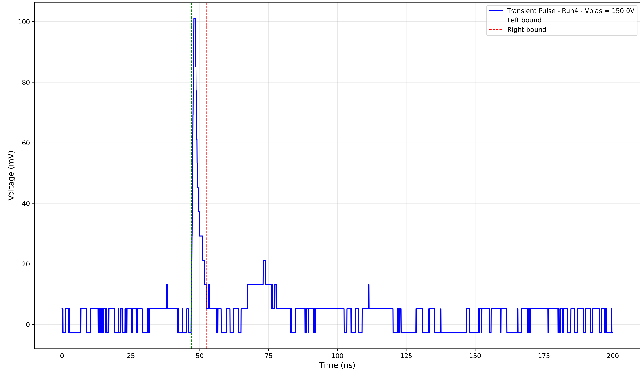
Transient Pulse - Sample: 4003 - Position: 105.0 \mu\text{m} - Charge: 4.86 pC - Rise Time: 0.75 ns
