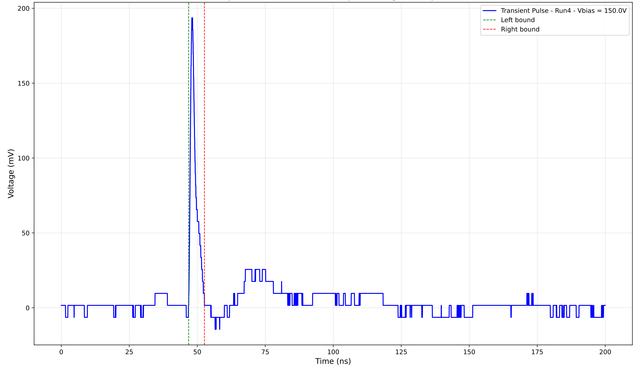
Transient Pulse - Sample: 4003 - Position: 170.0 \mu\text{m} - Charge: 9.11 pC - Rise Time: 0.84 ns
