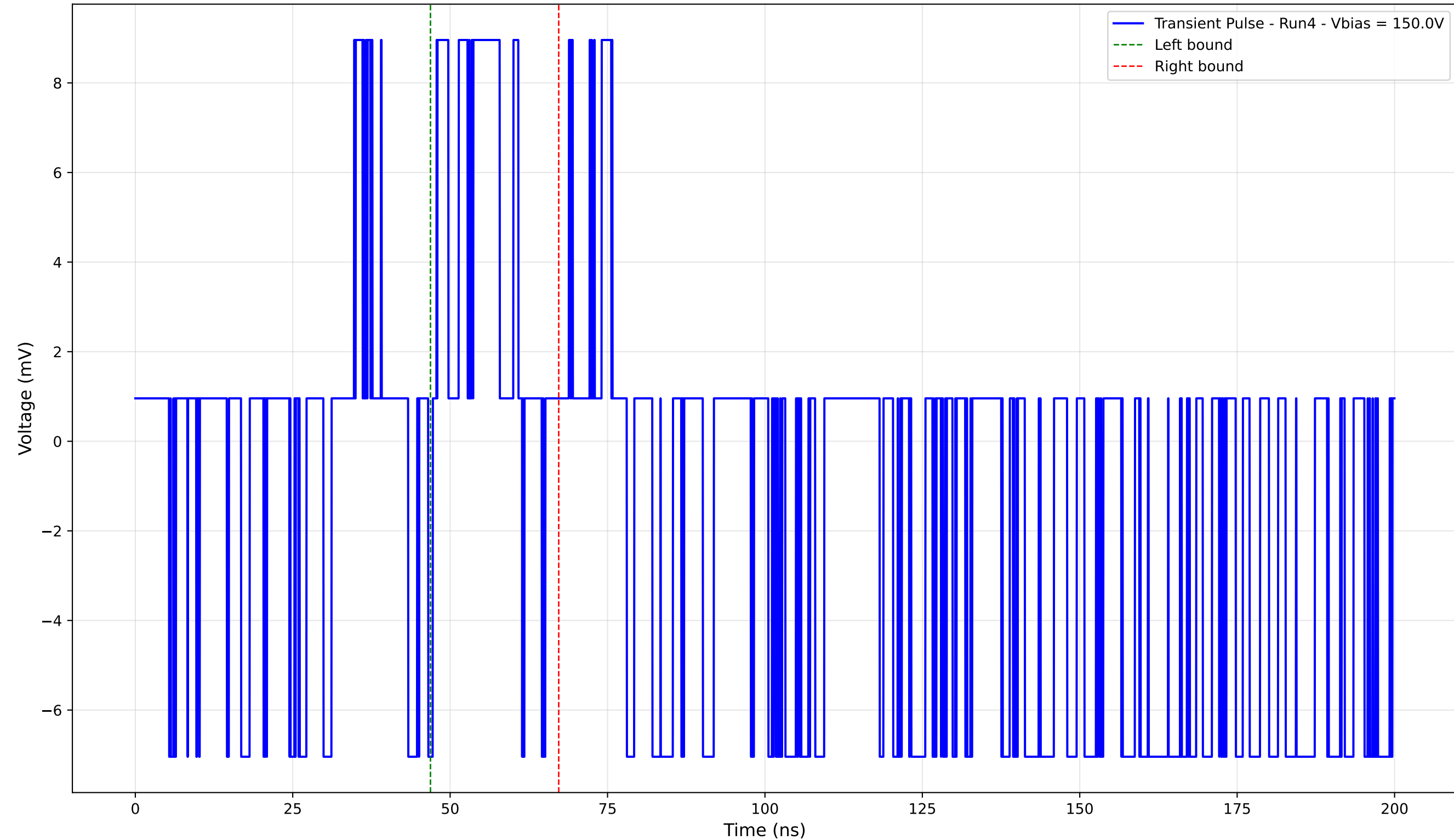
Transient Pulse - Sample: 4003 - Position: 635.0 \mu\text{m} - Charge: 1.61 pC - Rise Time: 0.00 ns (N/A)
