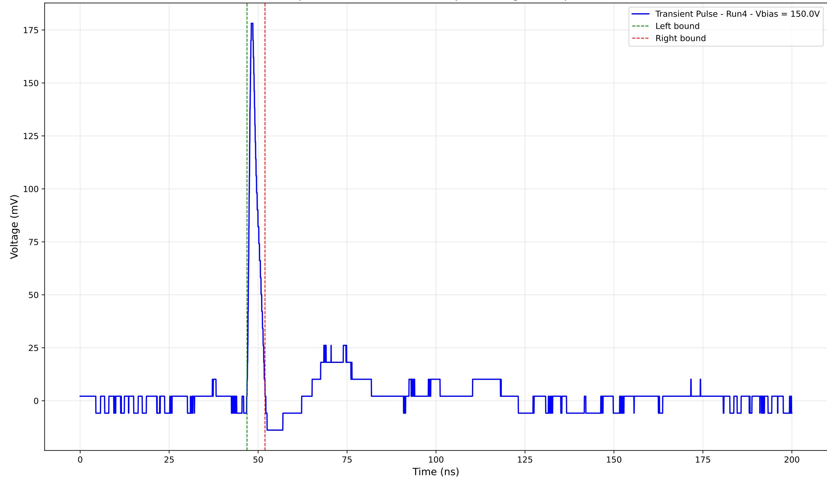
Transient Pulse - Sample: 4003 - Position: 525.0 \mu\text{m} - Charge: 9.24 pC - Rise Time: 0.90 ns
