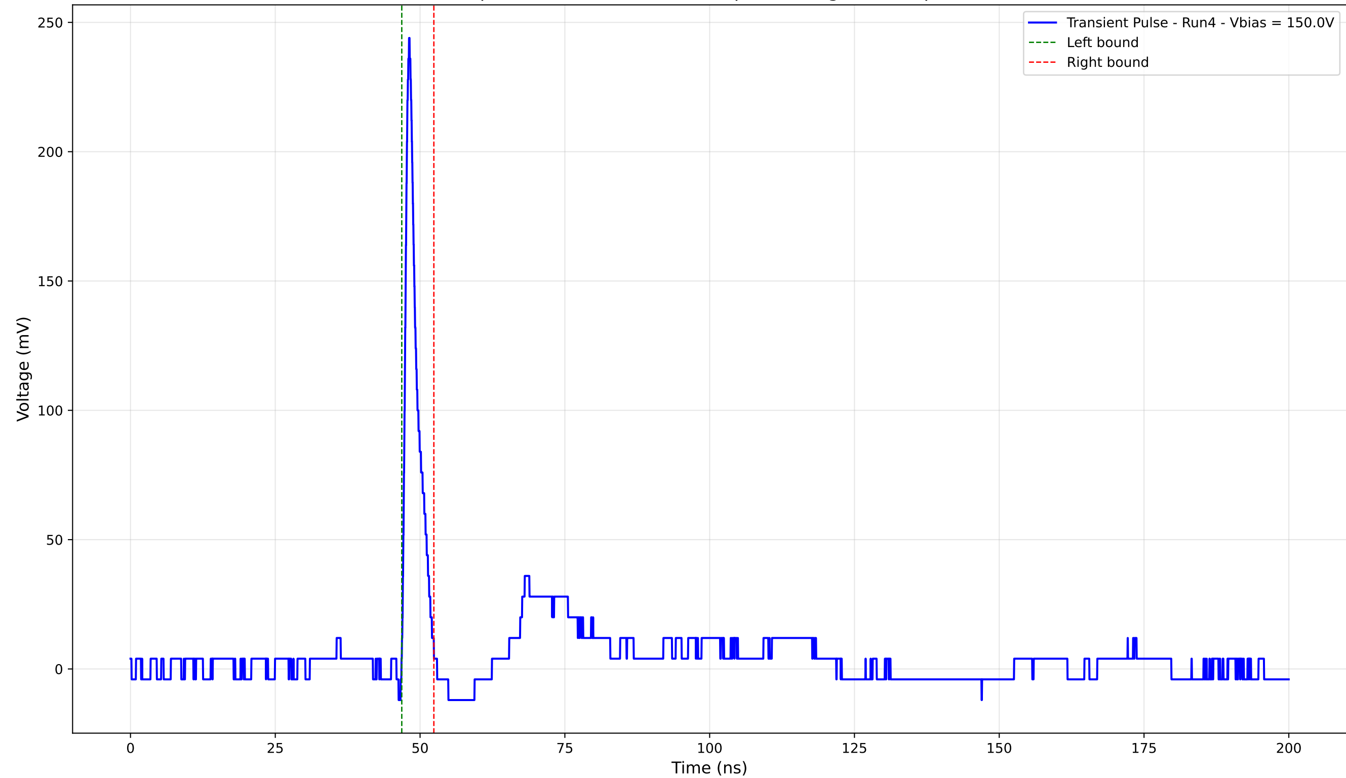
Transient Pulse - Sample: 4003 - Position: 200.0 \mu\text{m} - Charge: 11.39 pC - Rise Time: 0.83 ns
