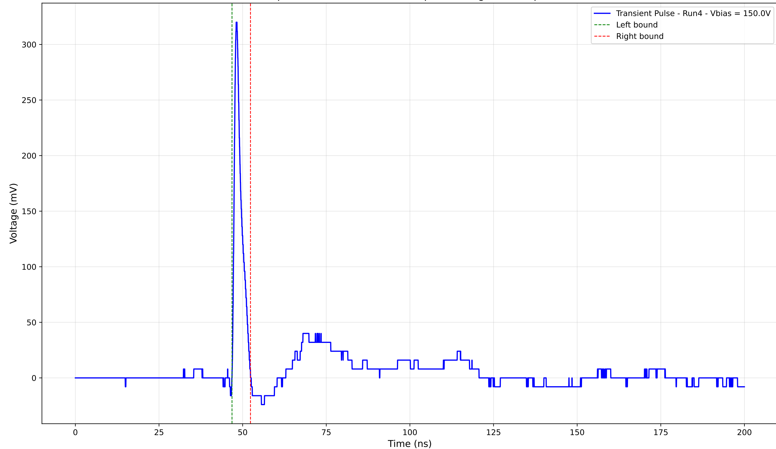
Transient Pulse - Sample: 4003 - Position: 275.0 \mu\text{m} - Charge: 15.66 pC - Rise Time: 0.82 ns
