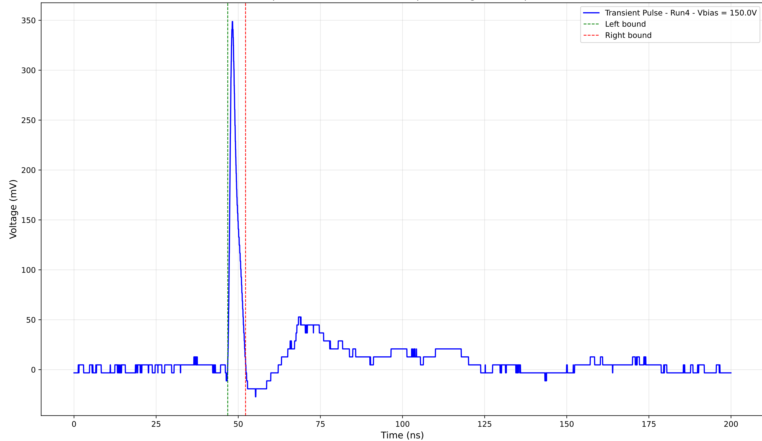
Transient Pulse - Sample: 4003 - Position: 315.0 \mu\text{m} - Charge: 17.41 pC - Rise Time: 0.92 ns
