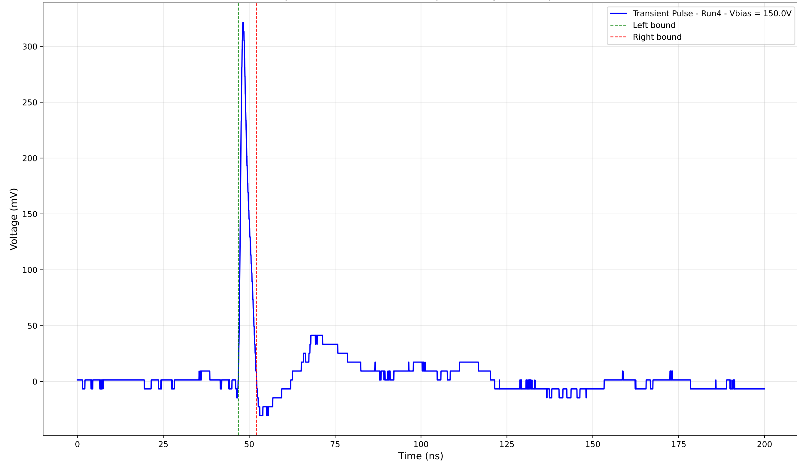
Transient Pulse - Sample: 4003 - Position: 400.0 \mu\text{m} - Charge: 16.24 pC - Rise Time: 0.90 ns
