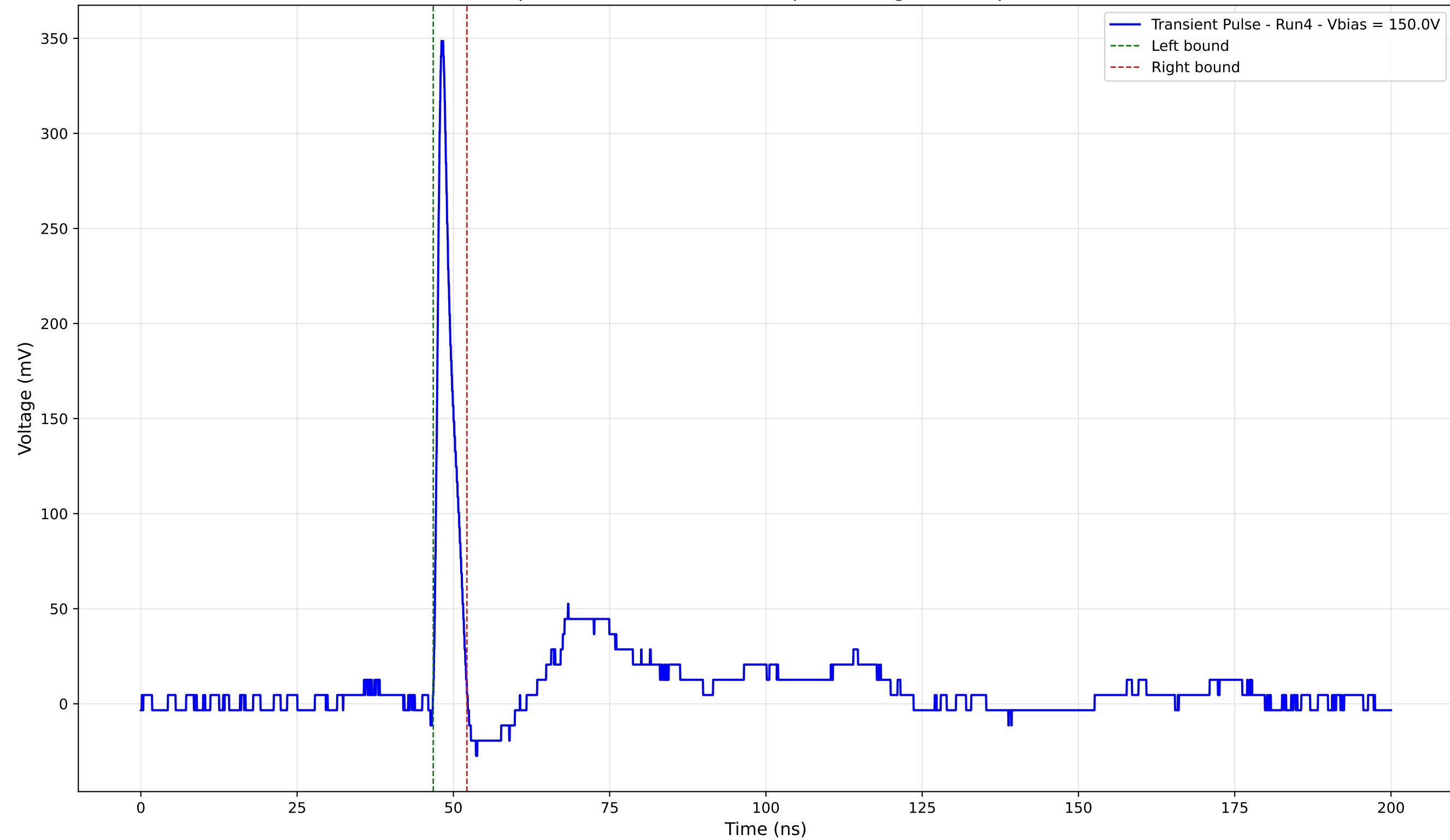
Transient Pulse - Sample: 4003 - Position: 335.0 \mu\text{m} - Charge: 17.92 pC - Rise Time: 0.92 ns
