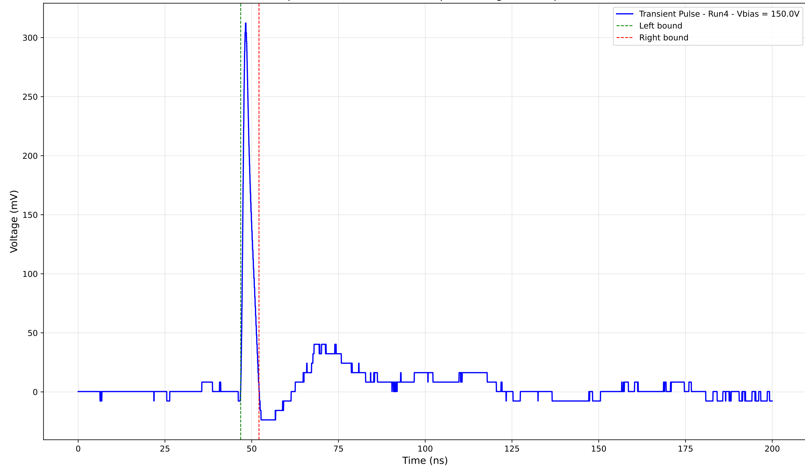
Transient Pulse - Sample: 4003 - Position: 410.0 \mu\text{m} - Charge: 15.68 pC - Rise Time: 0.96 ns
