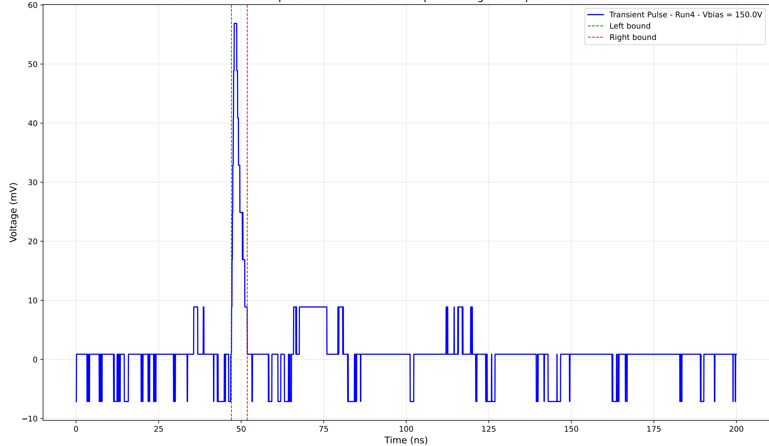
Transient Pulse - Sample: 4003 - Position: 610.0 \mu\text{m} - Charge: 2.88 pC - Rise Time: 0.81 ns
