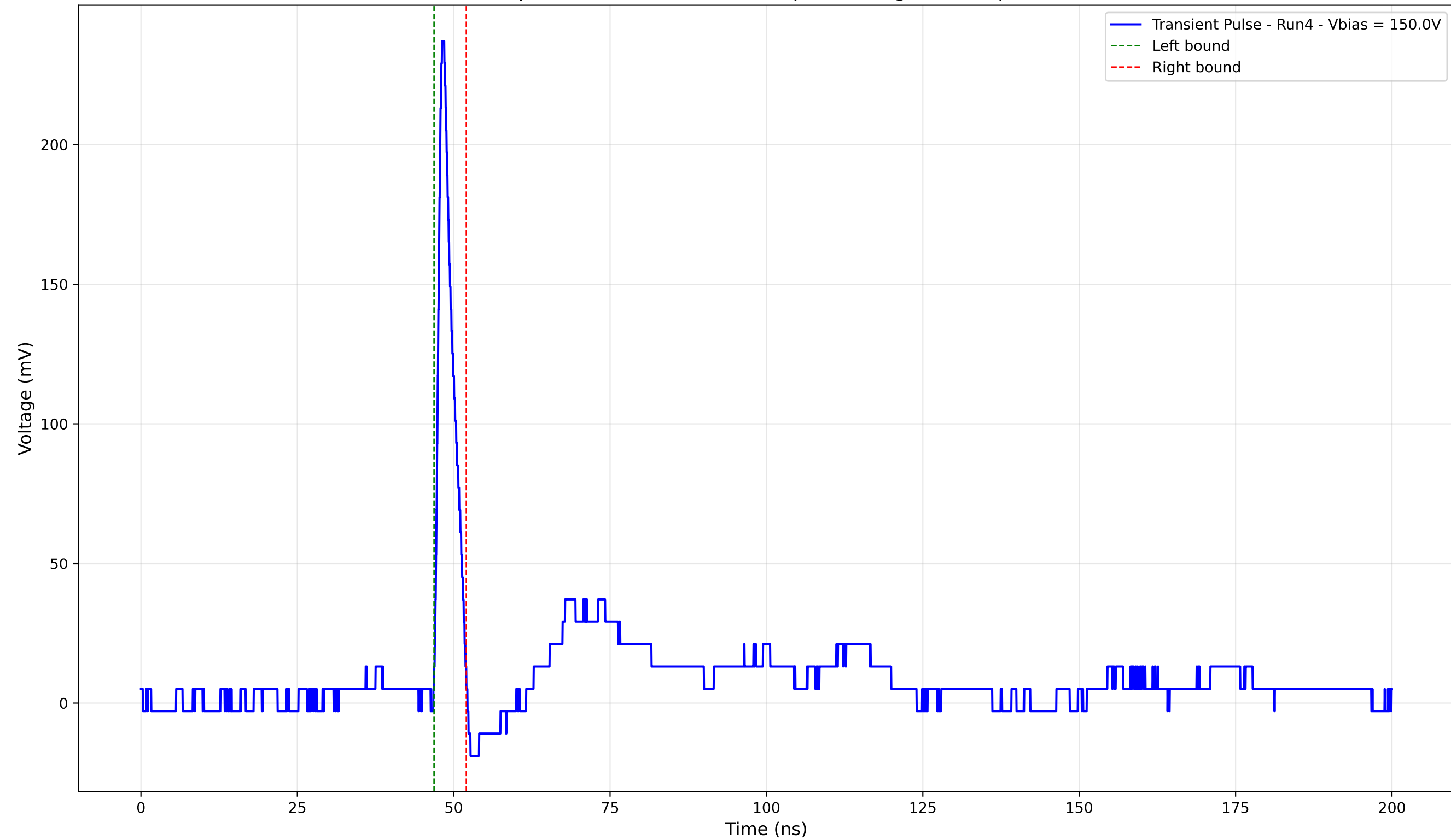
Transient Pulse - Sample: 4003 - Position: 475.0 \mu\text{m} - Charge: 12.52 pC - Rise Time: 0.95 ns
