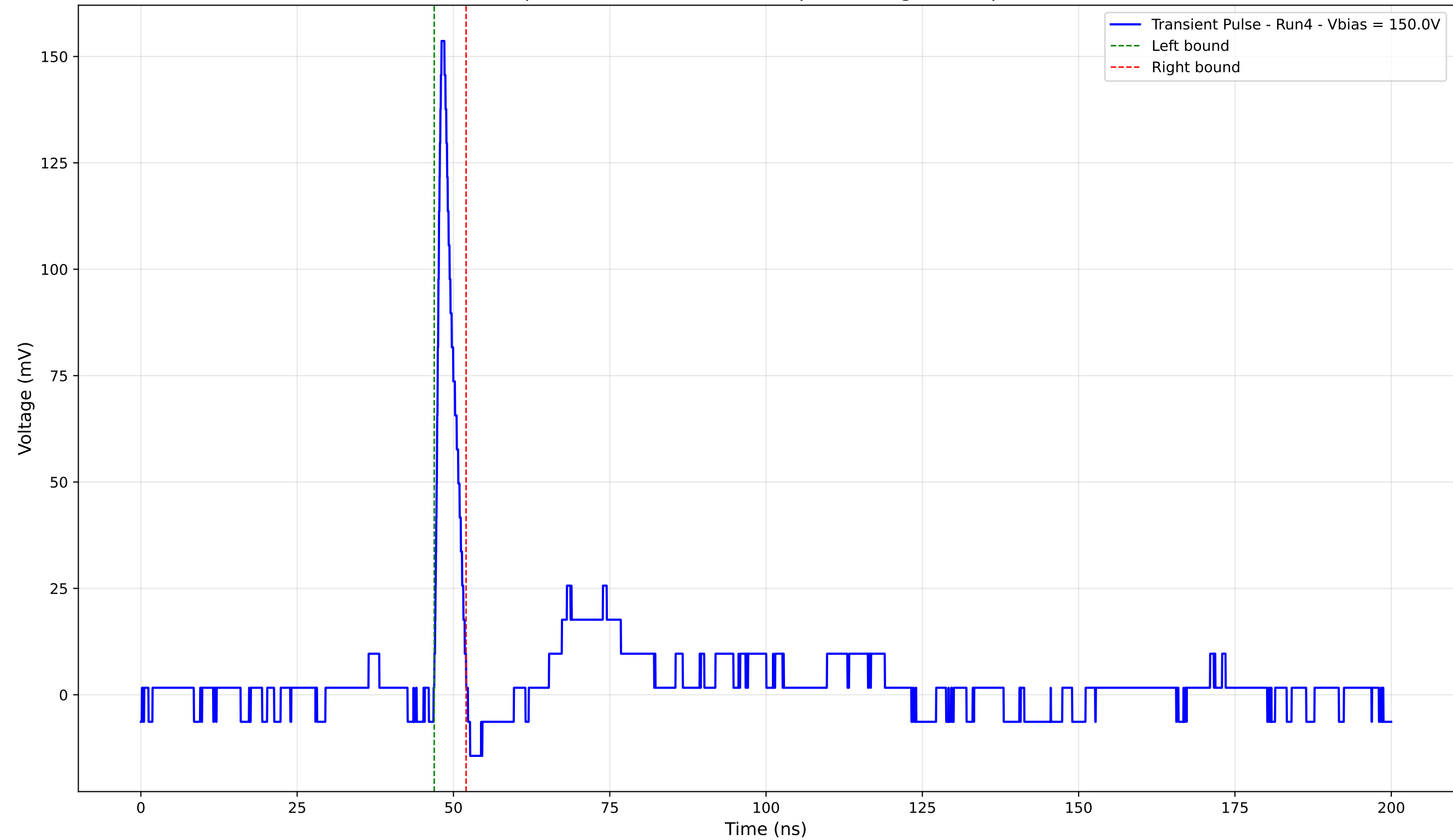
Transient Pulse - Sample: 4003 - Position: 570.0 \mu\text{m} - Charge: 8.14 pC - Rise Time: 0.93 ns
