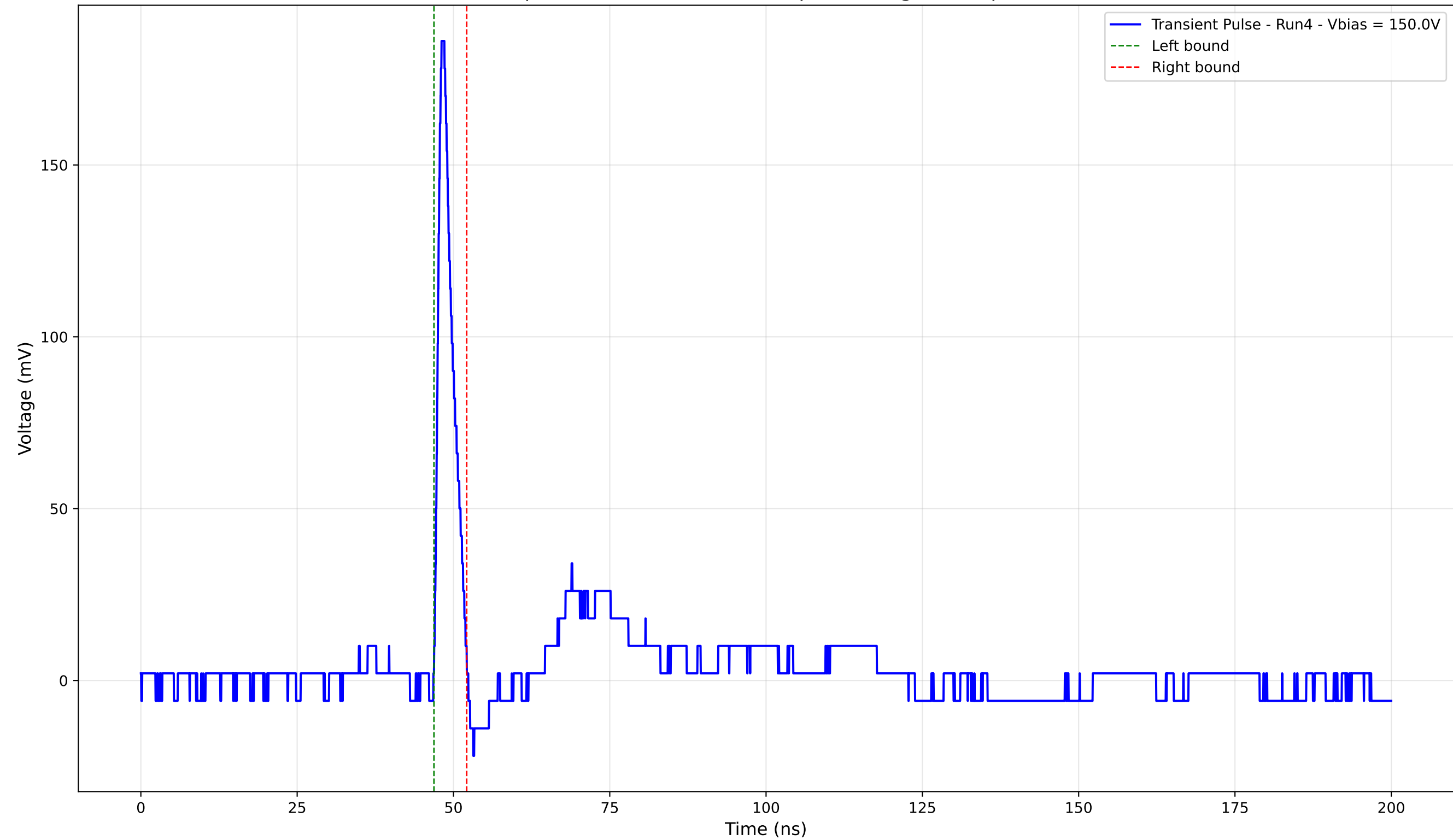
Transient Pulse - Sample: 4003 - Position: 515.0 \mu\text{m} - Charge: 9.88 pC - Rise Time: 0.88 ns
