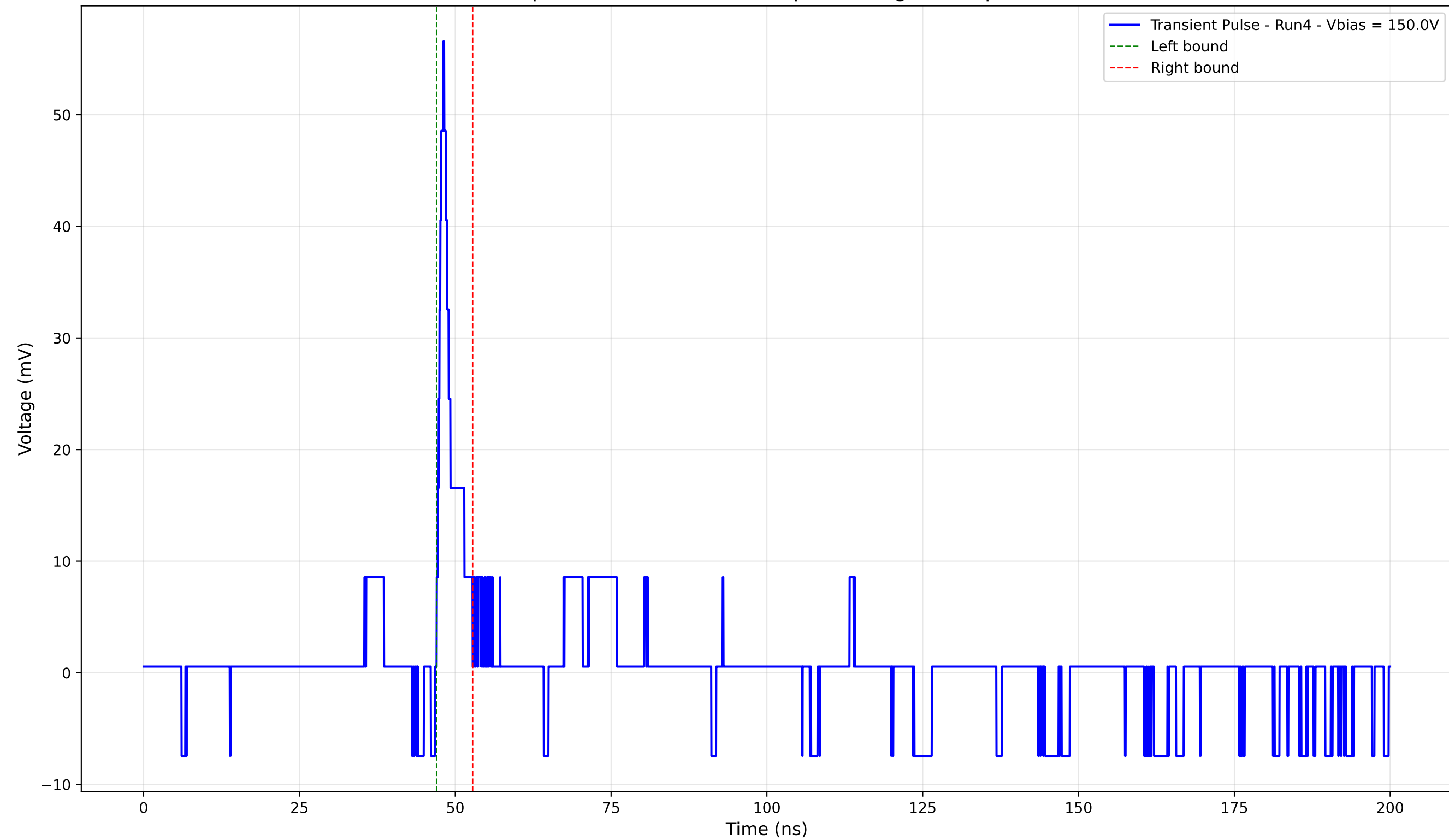
Transient Pulse - Sample: 4003 - Position: 60.0 \mu\text{m} - Charge: 2.53 pC - Rise Time: 1.05 ns
