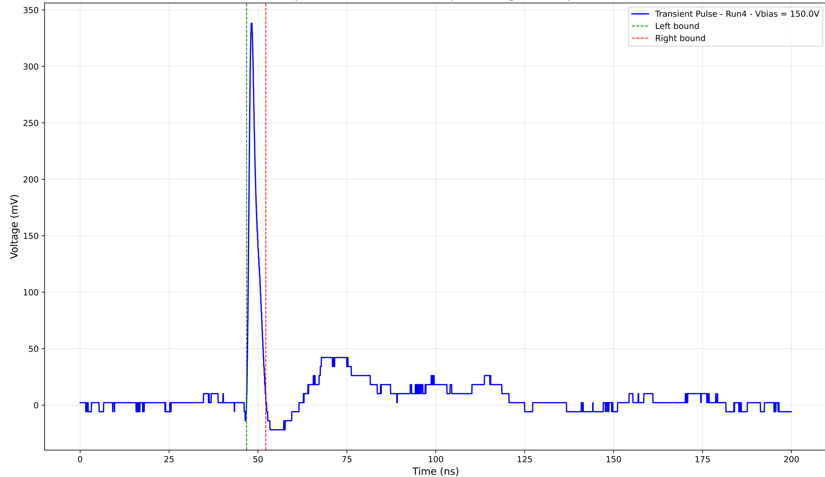
Transient Pulse - Sample: 4003 - Position: 305.0 \mu\text{m} - Charge: 16.85 pC - Rise Time: 0.88 ns
