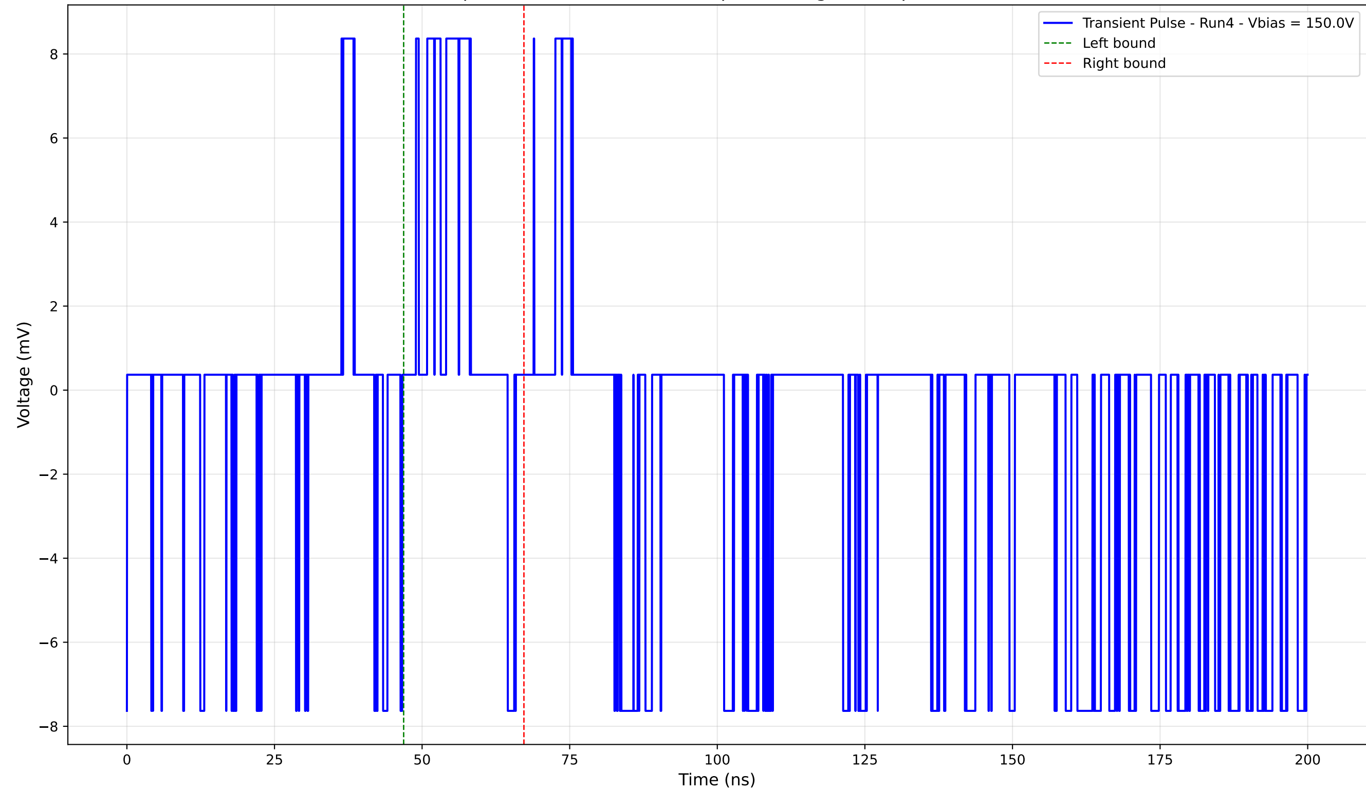
Transient Pulse - Sample: 4003 - Position: 640.0 \mu\text{m} - Charge: 1.01 pC - Rise Time: 0.00 ns (N/A)
