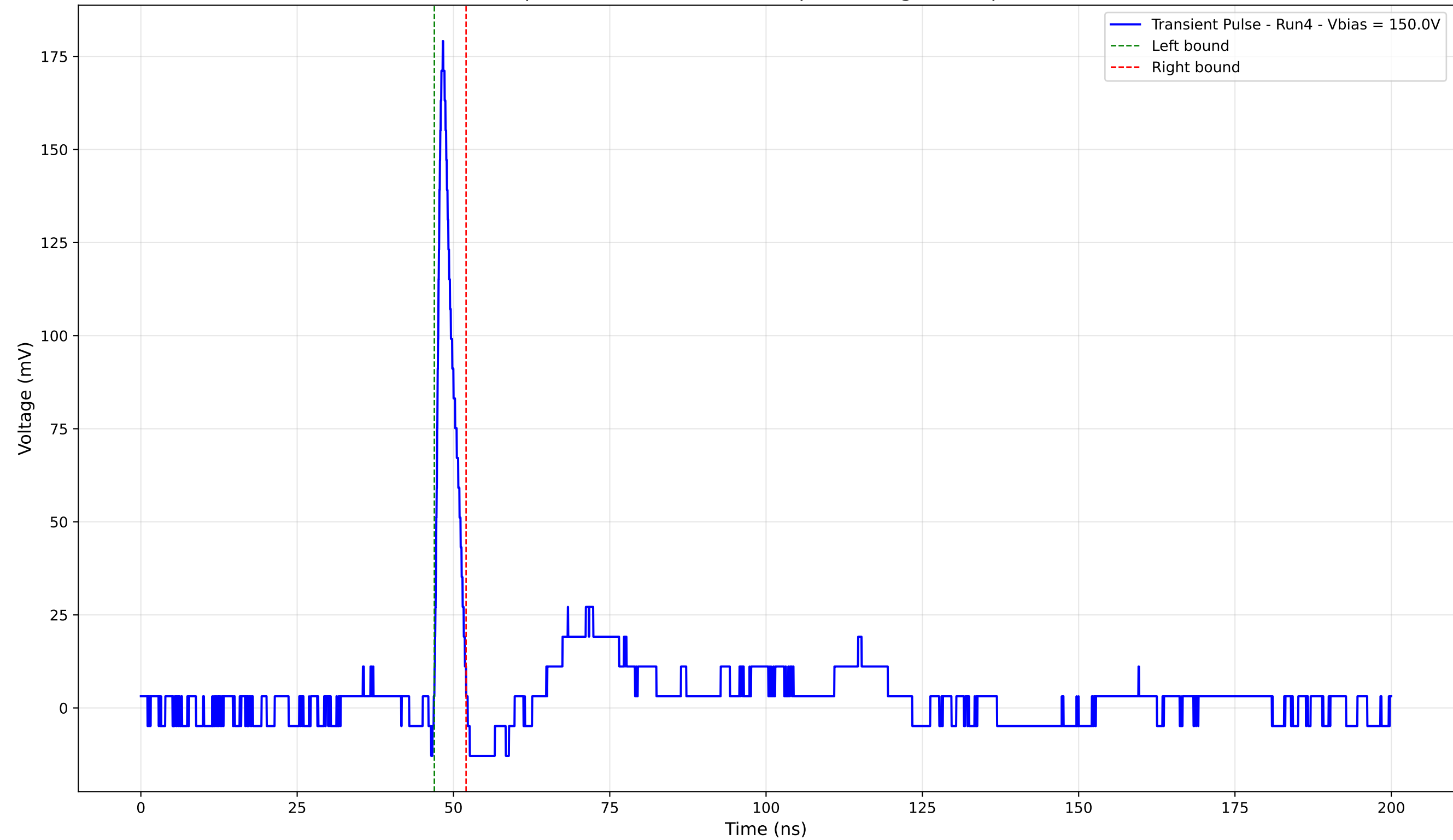
Transient Pulse - Sample: 4003 - Position: 590.0 \mu\text{m} - Charge: 9.30 pC - Rise Time: 0.92 ns
