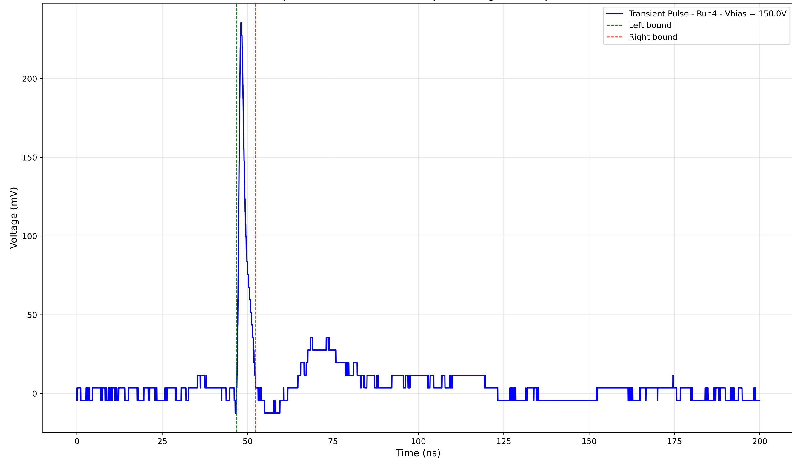
Transient Pulse - Sample: 4003 - Position: 195.0 \mu\text{m} - Charge: 11.05 pC - Rise Time: 0.87 ns
