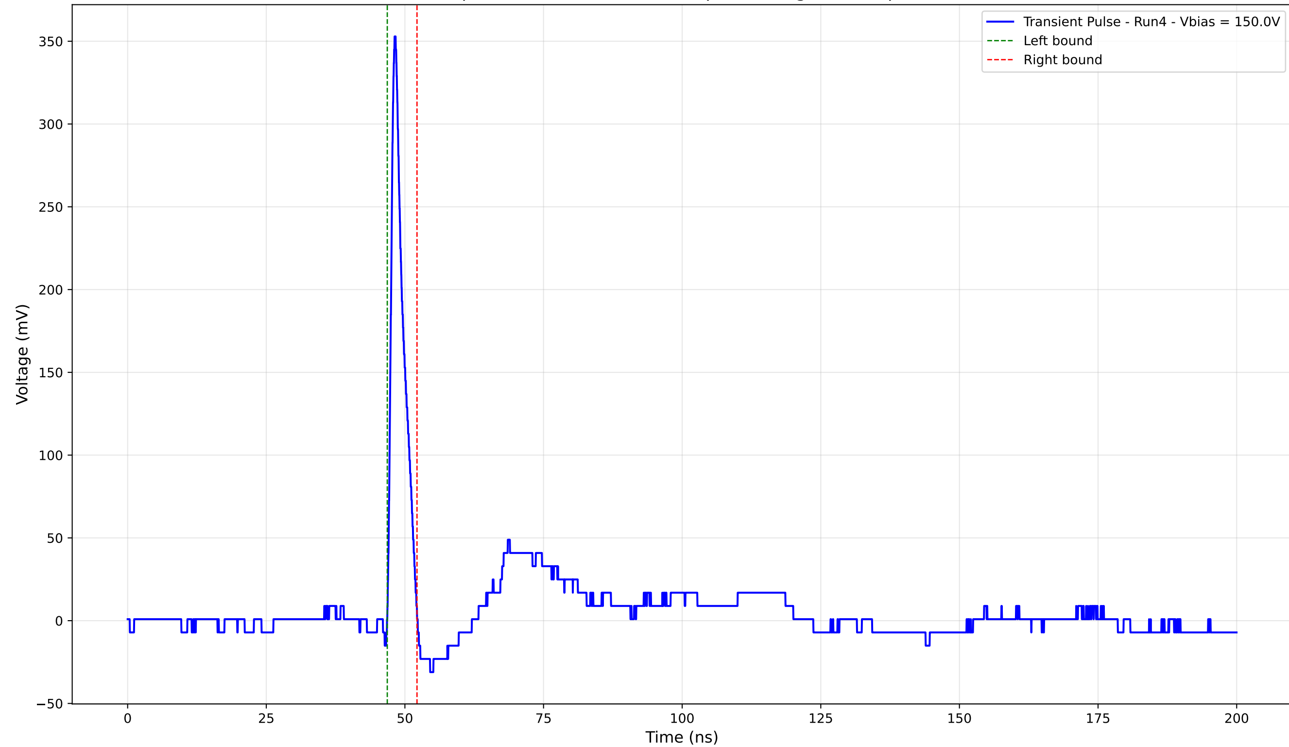
Transient Pulse - Sample: 4003 - Position: 340.0 \mu\text{m} - Charge: 17.69 pC - Rise Time: 0.89 ns
