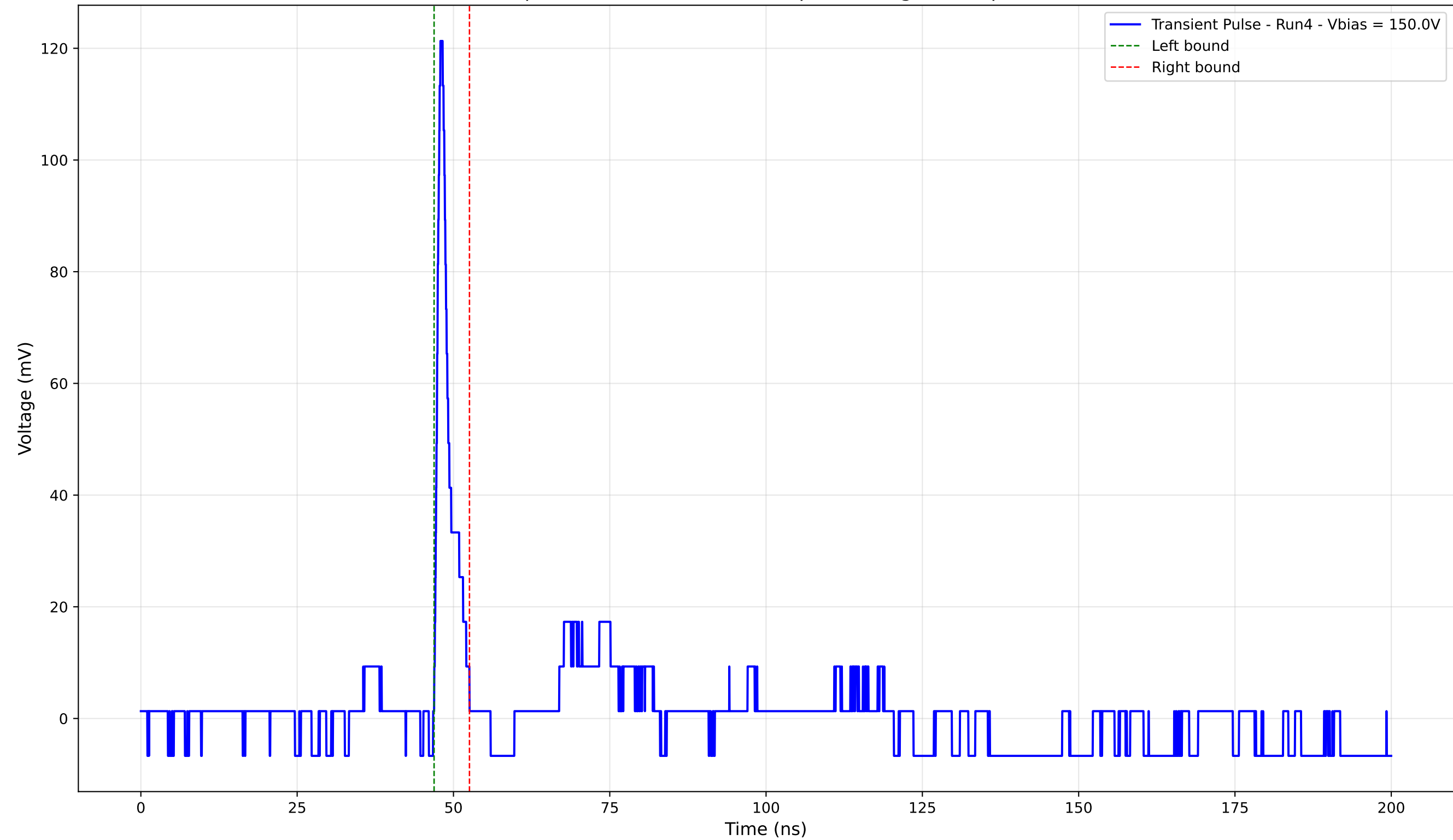
Transient Pulse - Sample: 4003 - Position: 120.0 \mu\text{m} - Charge: 5.50 pC - Rise Time: 0.77 ns
