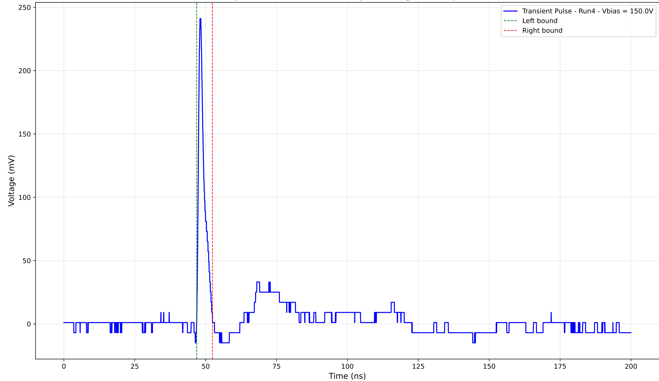
Transient Pulse - Sample: 4003 - Position: 205.0 \mu\text{m} - Charge: 11.50 pC - Rise Time: 0.82 ns
