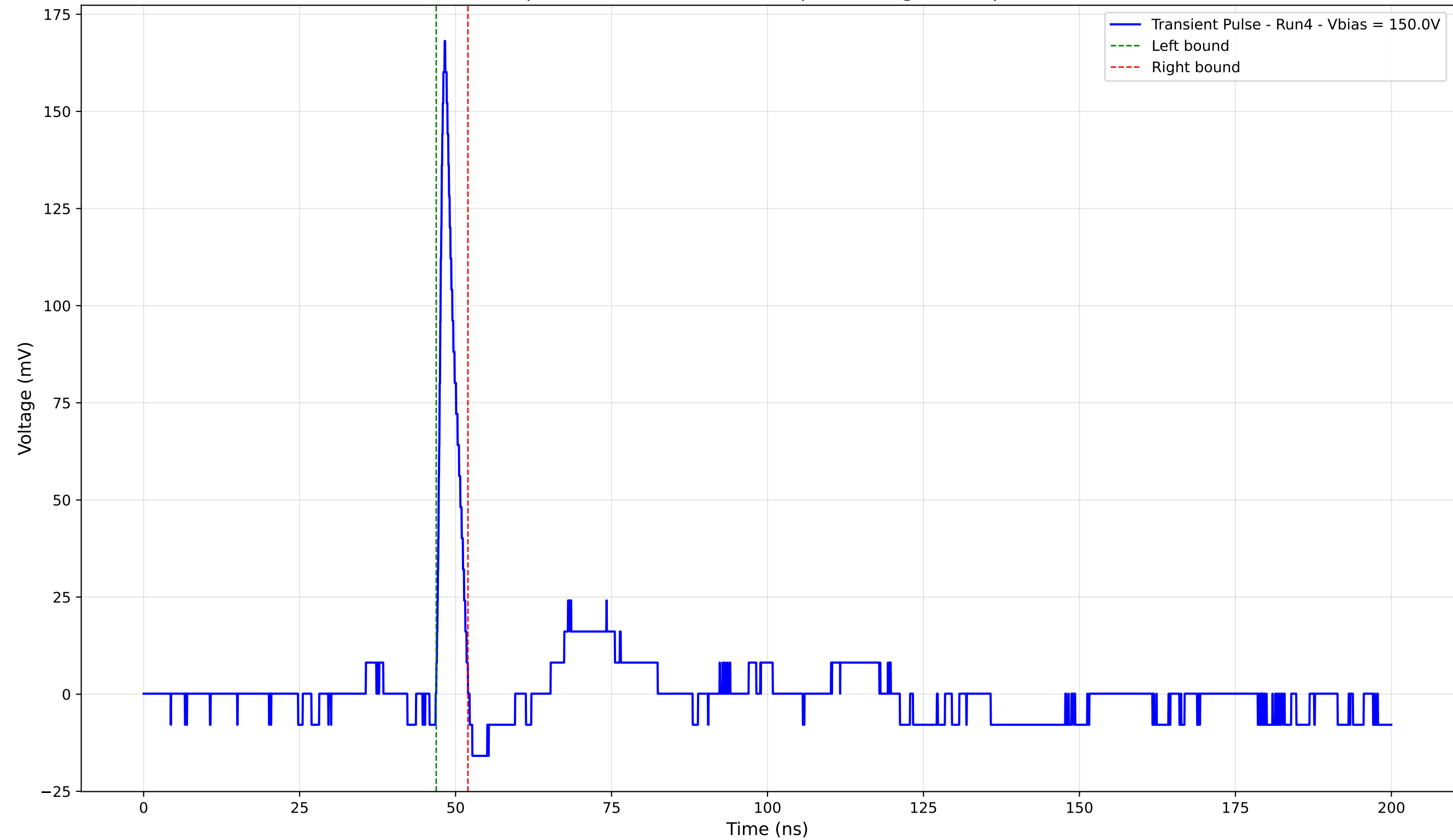
Transient Pulse - Sample: 4003 - Position: 595.0 \mu\text{m} - Charge: 8.42 pC - Rise Time: 0.86 ns
