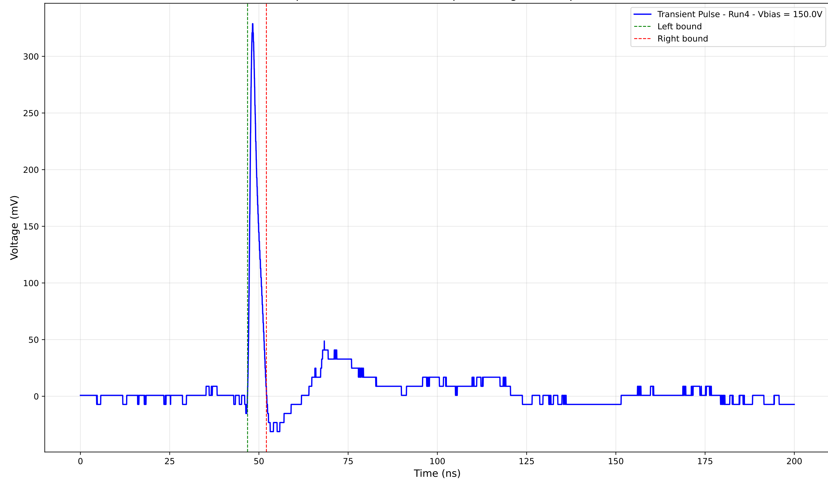
Transient Pulse - Sample: 4003 - Position: 390.0 \mu\text{m} - Charge: 16.40 pC - Rise Time: 0.90 ns
