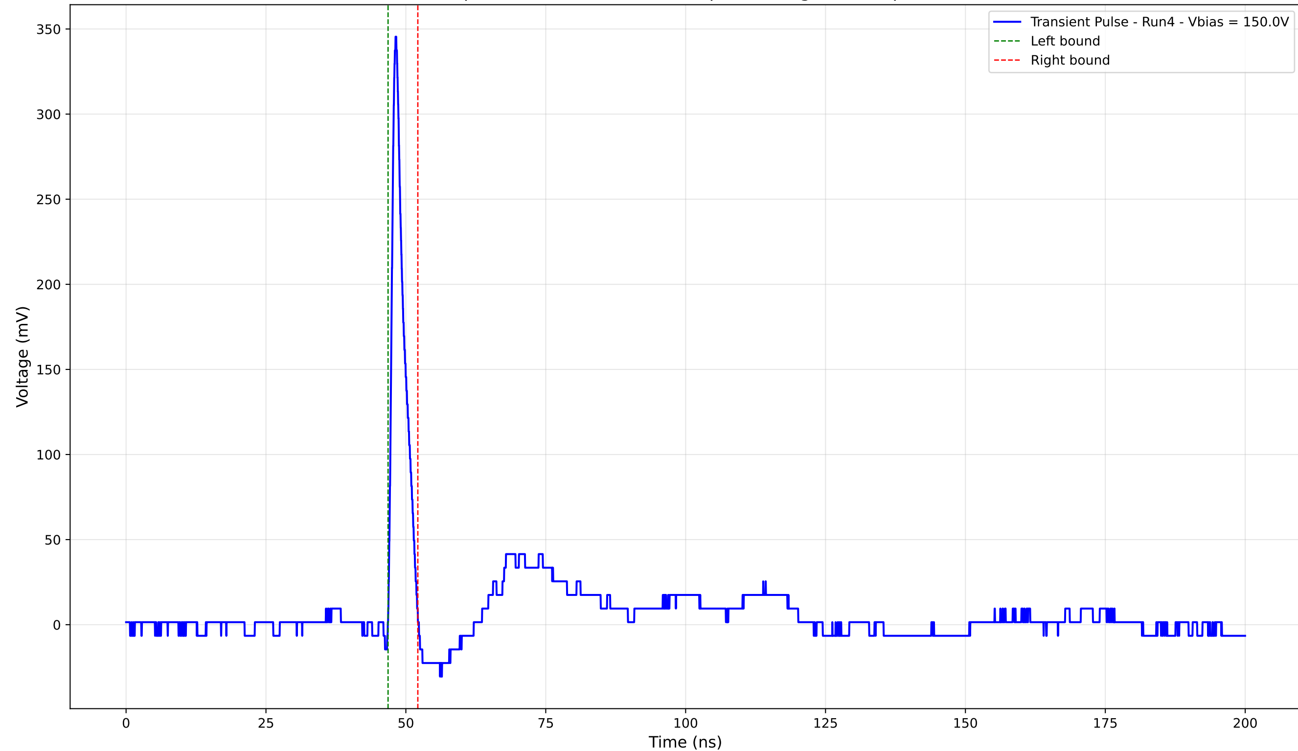
Transient Pulse - Sample: 4003 - Position: 320.0 \mu\text{m} - Charge: 17.16 pC - Rise Time: 0.88 ns
