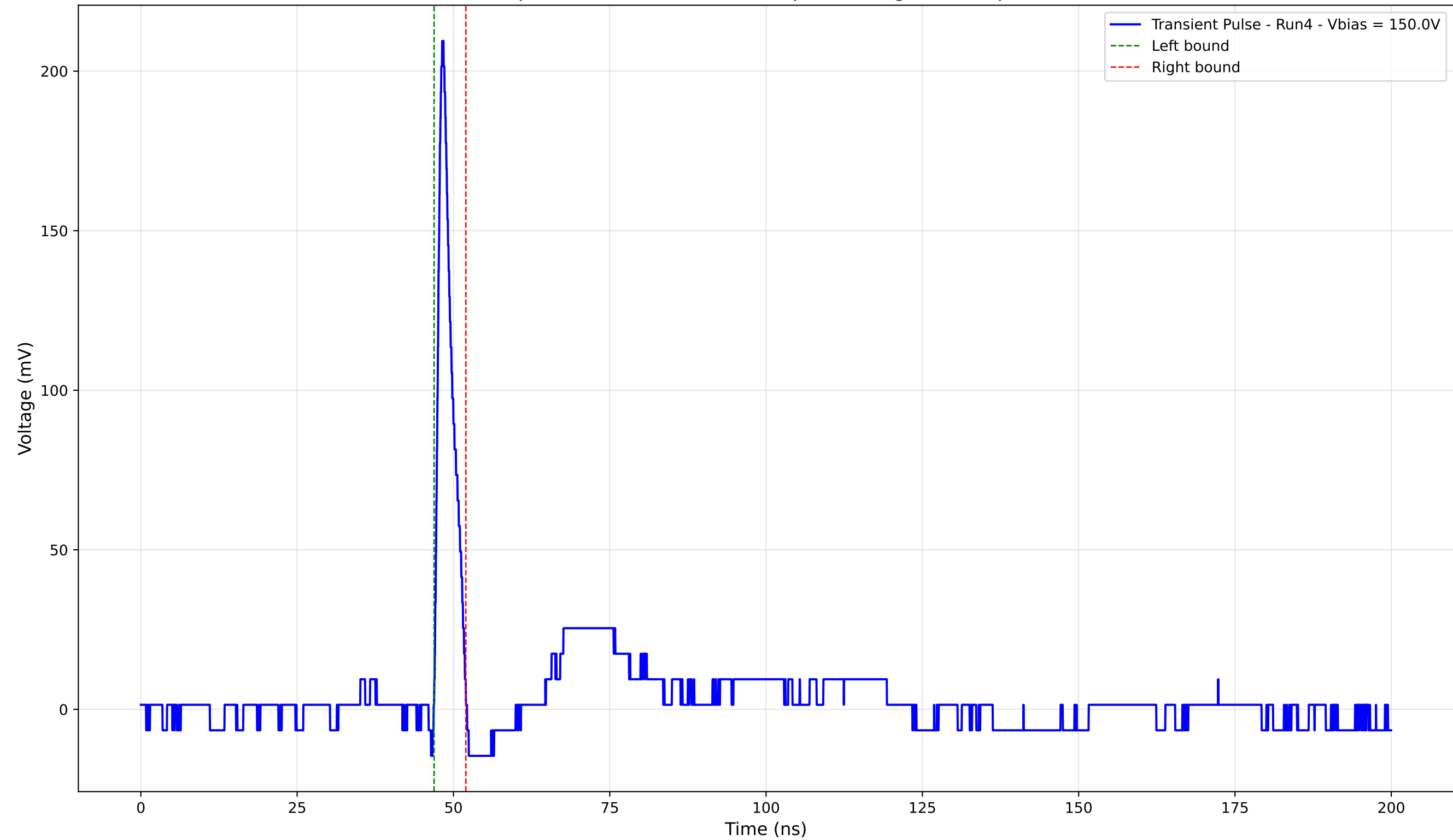
Transient Pulse - Sample: 4003 - Position: 500.0 \mu\text{m} - Charge: 10.54 pC - Rise Time: 0.91 ns
