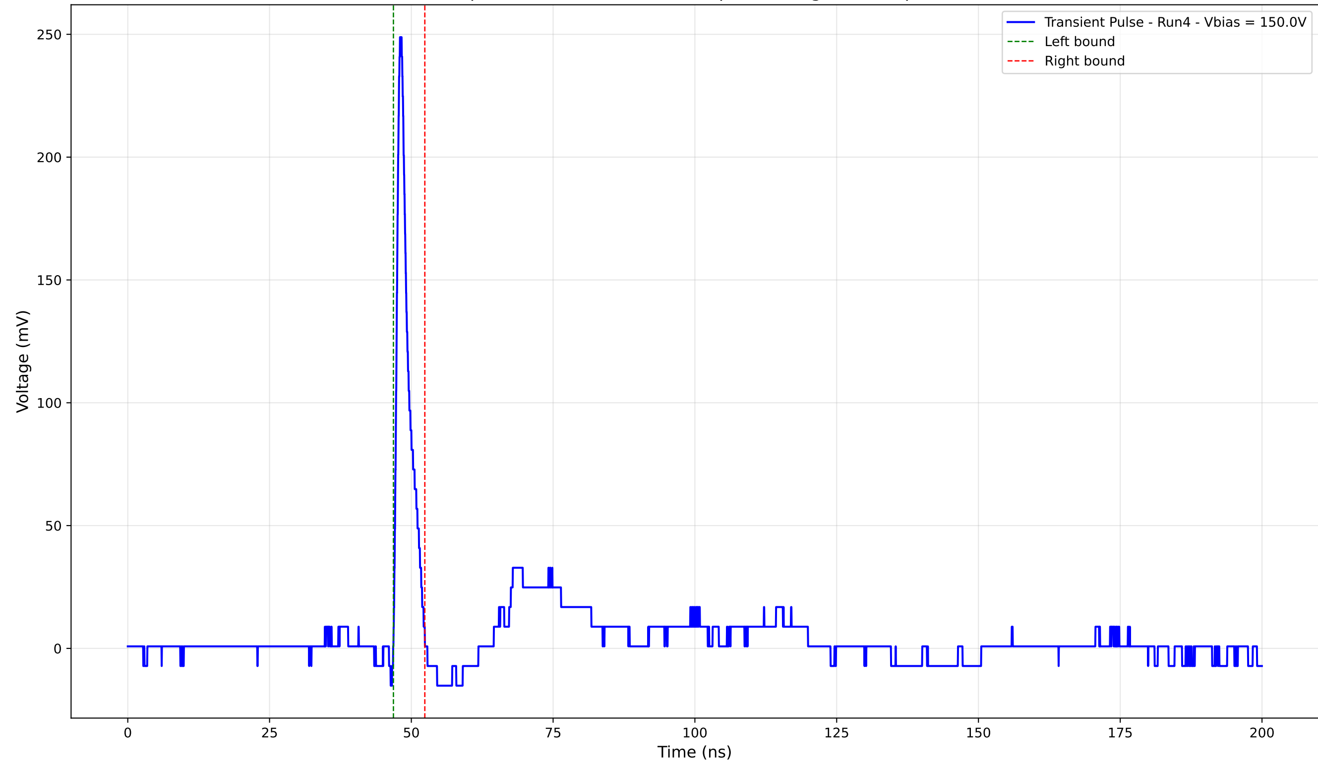
Transient Pulse - Sample: 4003 - Position: 210.0 \mu\text{m} - Charge: 11.82 pC - Rise Time: 0.80 ns
