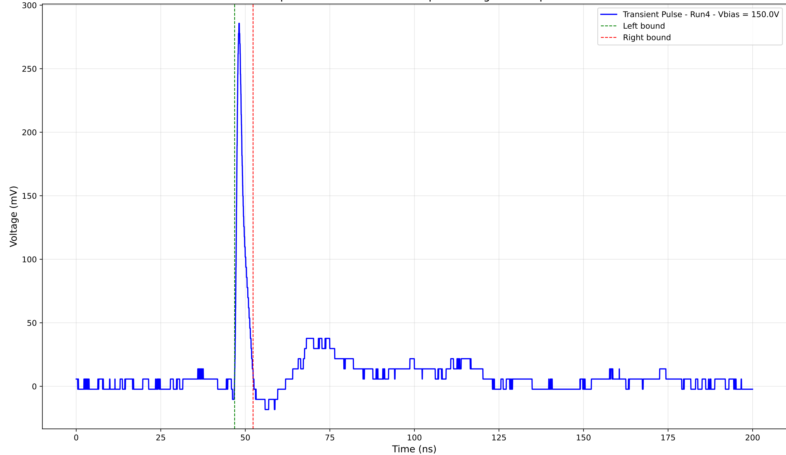
Transient Pulse - Sample: 4003 - Position: 235.0 \mu\text{m} - Charge: 13.62 pC - Rise Time: 0.88 ns
