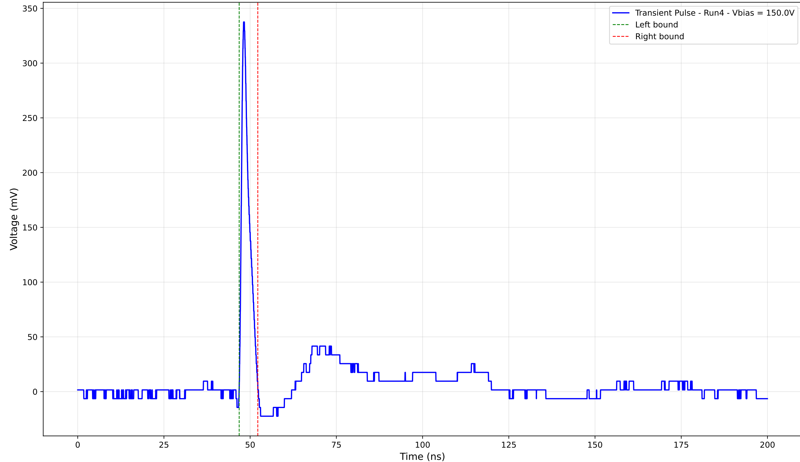
Transient Pulse - Sample: 4003 - Position: 310.0 \mu\text{m} - Charge: 16.84 pC - Rise Time: 0.86 ns
