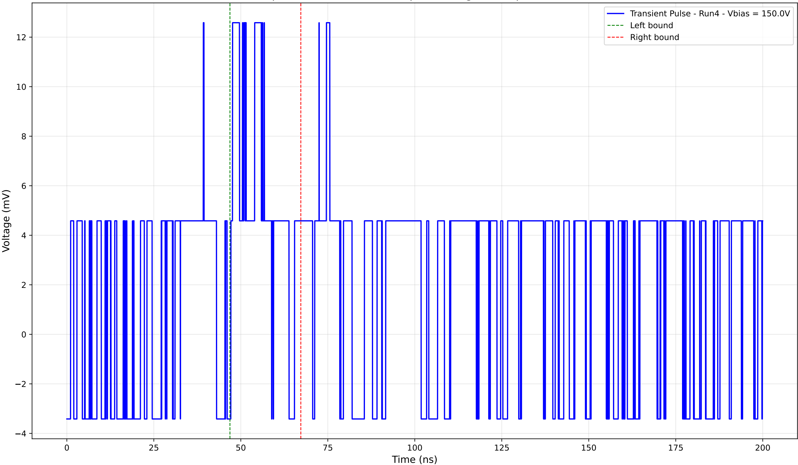
Transient Pulse - Sample: 4003 - Position: 0.0 \mu\text{m} - Charge: 2.31 pC - Rise Time: 0.00 ns (N/A)
