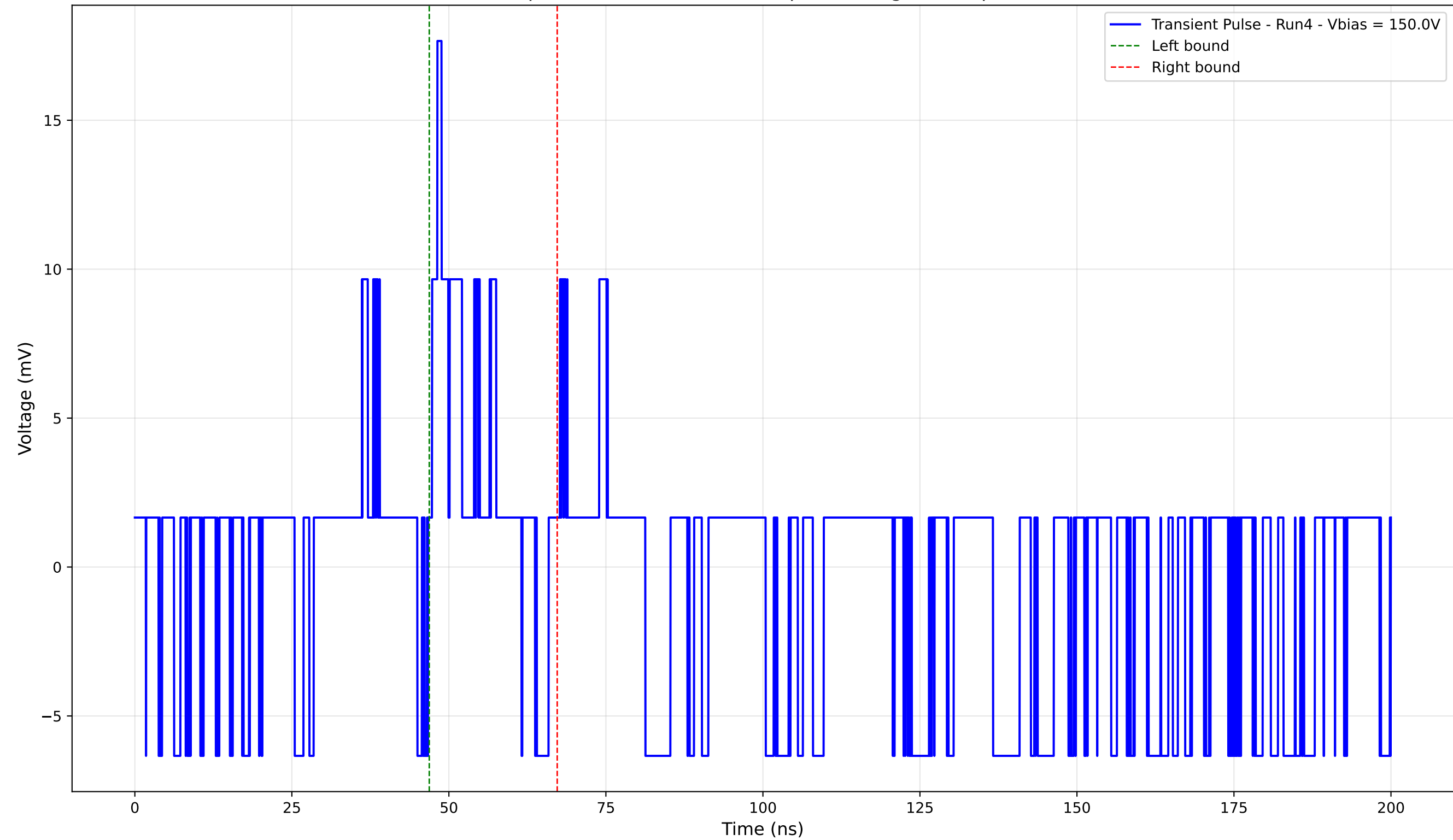
Transient Pulse - Sample: 4003 - Position: 15.0 \mu\text{m} - Charge: 1.45 pC - Rise Time: 0.86 ns
