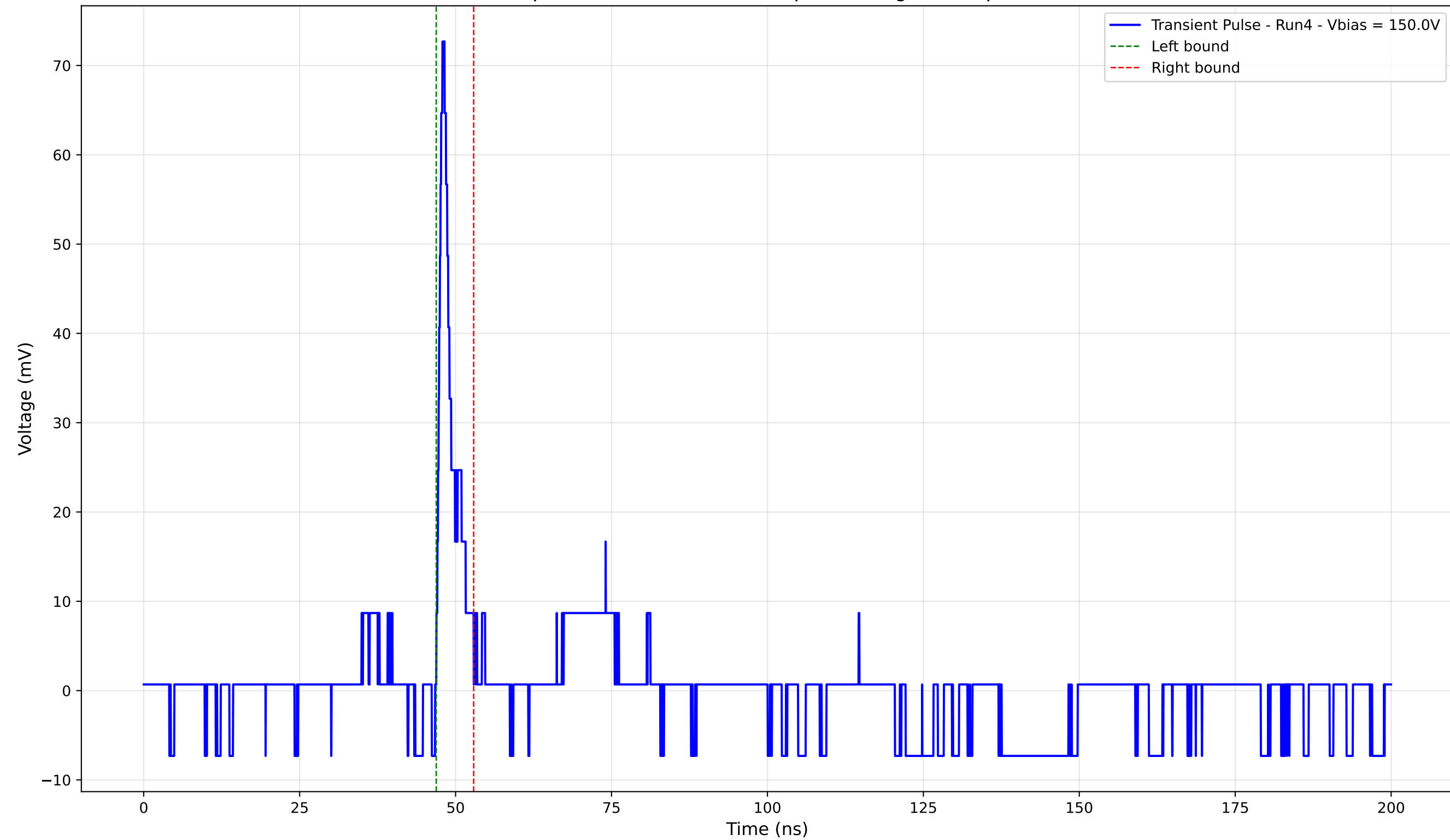
Transient Pulse - Sample: 4003 - Position: 80.0 \mu\text{m} - Charge: 3.47 pC - Rise Time: 0.96 ns
