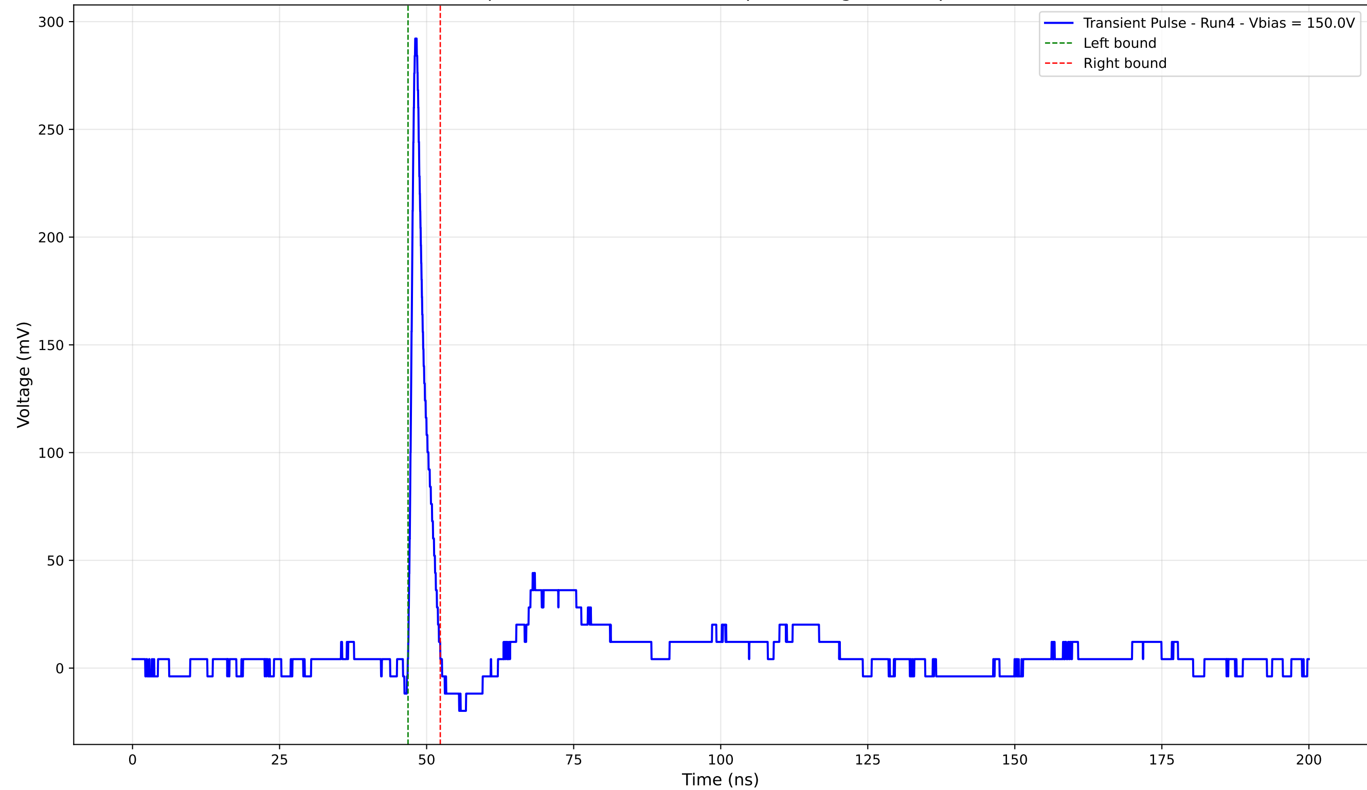
Transient Pulse - Sample: 4003 - Position: 245.0 \mu\text{m} - Charge: 14.29 pC - Rise Time: 0.88 ns
