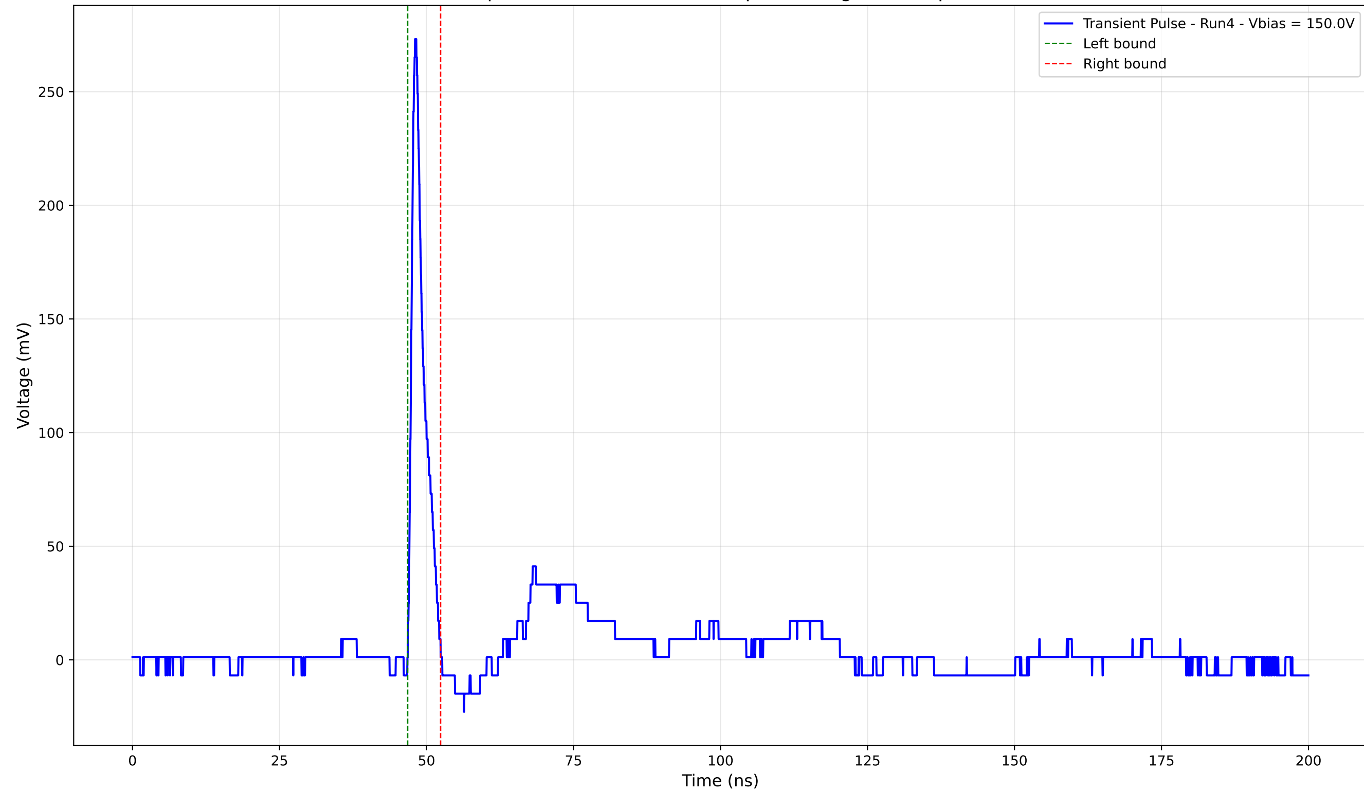
Transient Pulse - Sample: 4003 - Position: 230.0 \mu\text{m} - Charge: 13.23 pC - Rise Time: 0.85 ns
