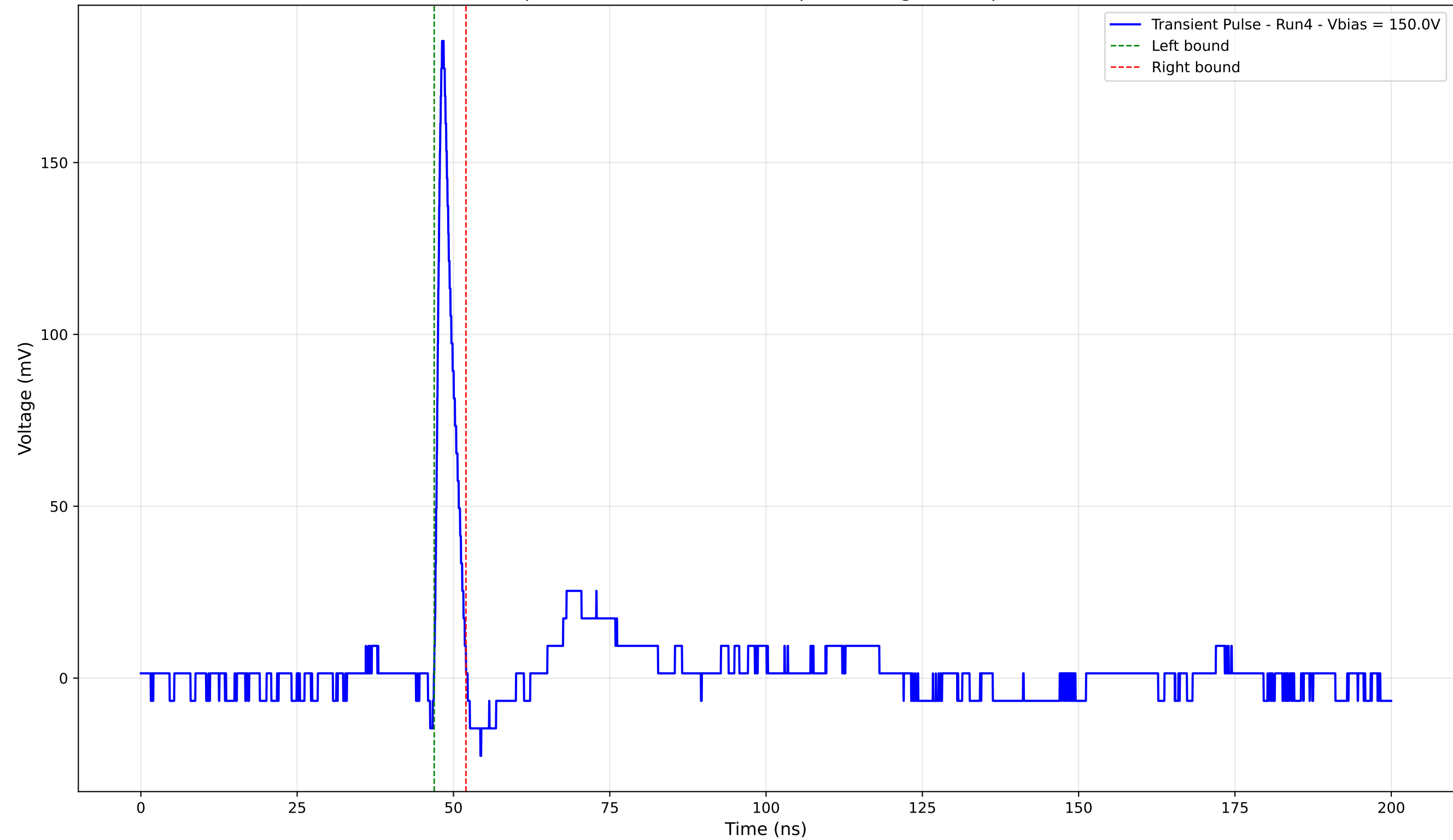
Transient Pulse - Sample: 4003 - Position: 520.0 \mu\text{m} - Charge: 9.40 pC - Rise Time: 0.88 ns
