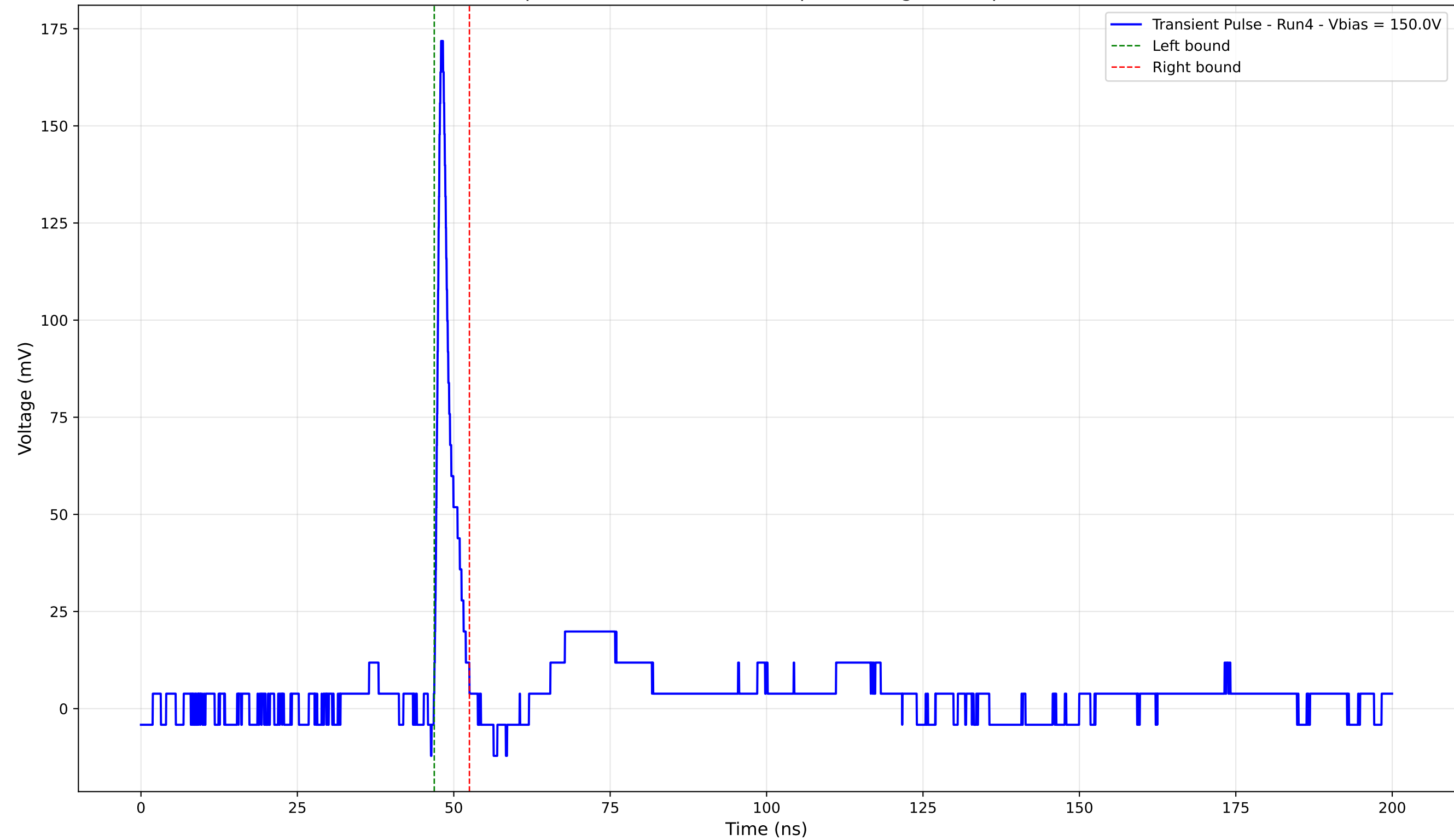
Transient Pulse - Sample: 4003 - Position: 155.0 \mu\text{m} - Charge: 7.97 pC - Rise Time: 0.81 ns
