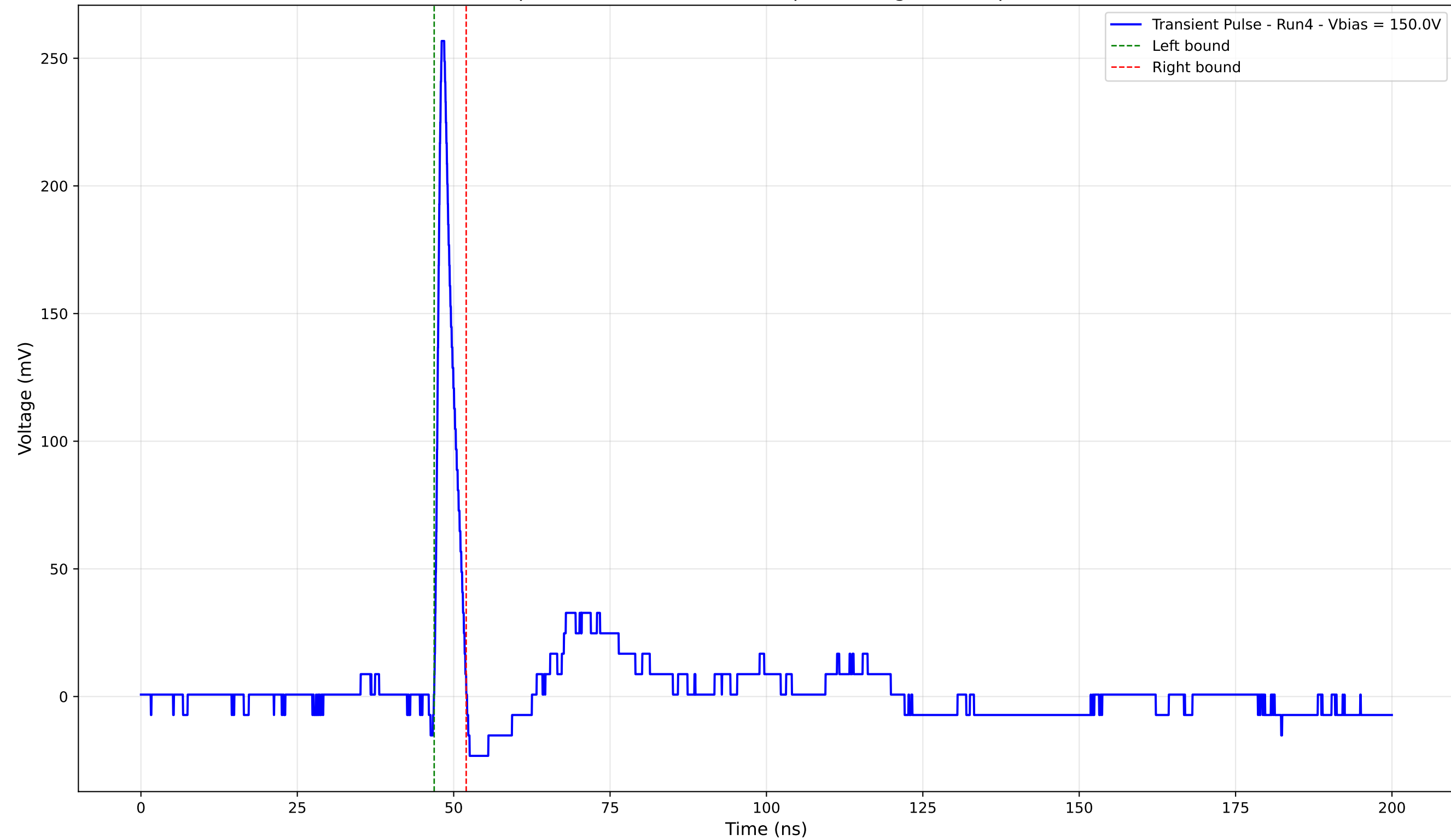
Transient Pulse - Sample: 4003 - Position: 455.0 \mu\text{m} - Charge: 13.23 pC - Rise Time: 0.86 ns
