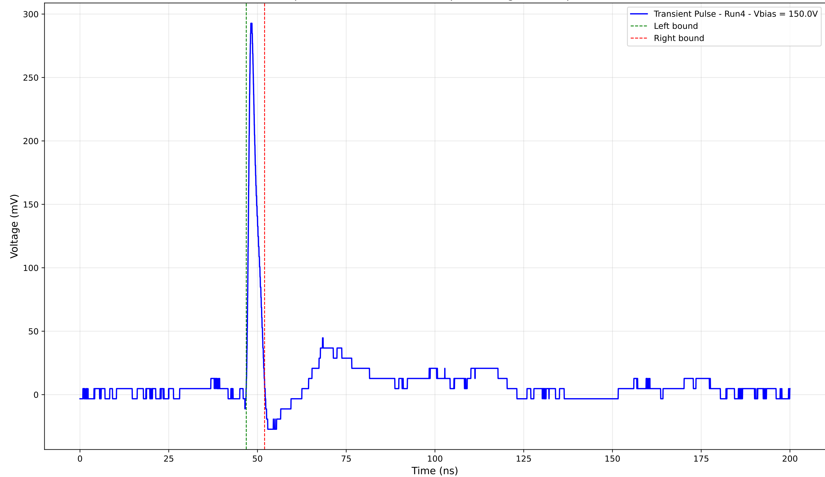
Transient Pulse - Sample: 4003 - Position: 430.0 \mu\text{m} - Charge: 15.09 pC - Rise Time: 0.92 ns
