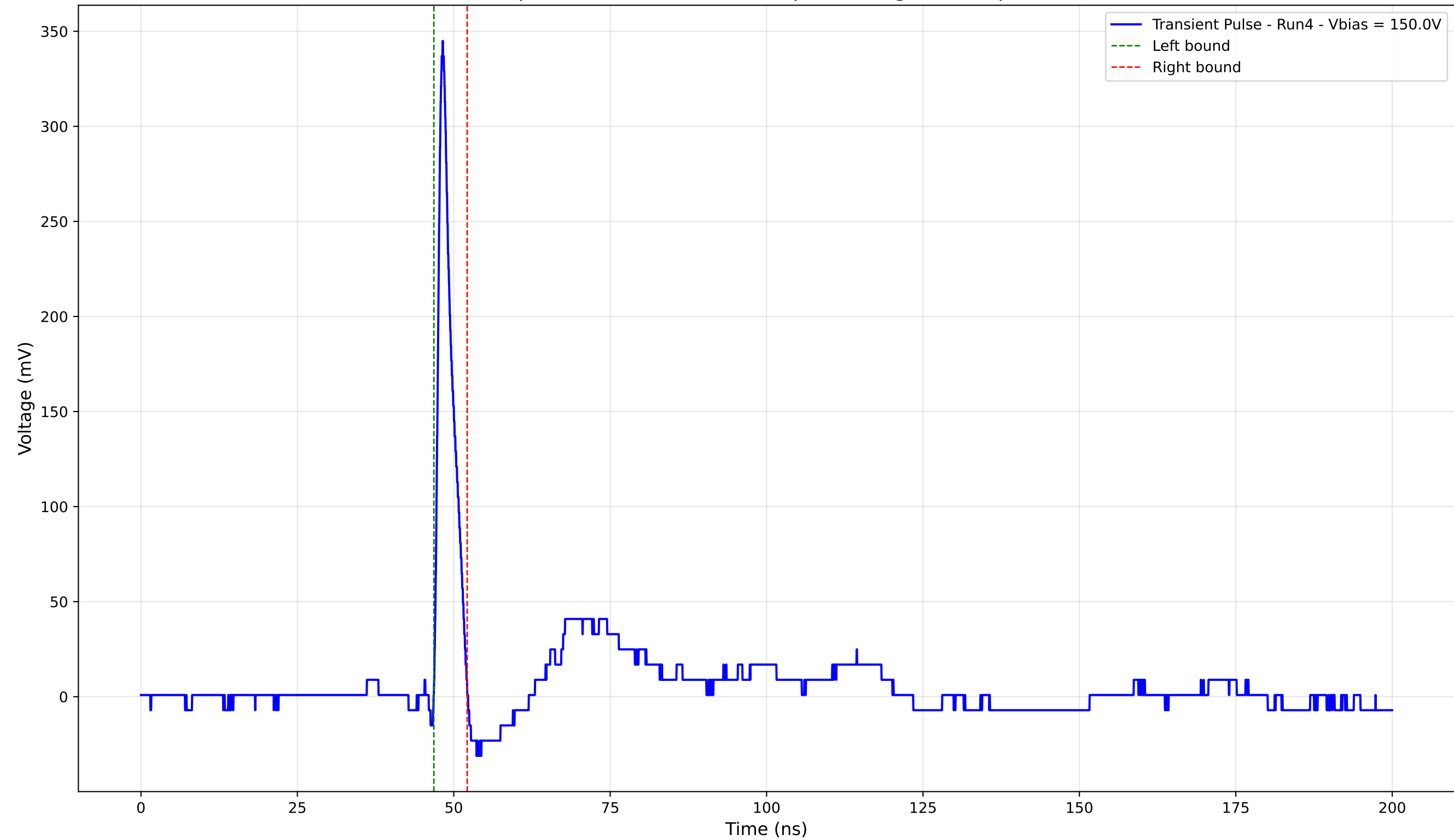
Transient Pulse - Sample: 4003 - Position: 360.0 \mu\text{m} - Charge: 17.21 pC - Rise Time: 0.90 ns
