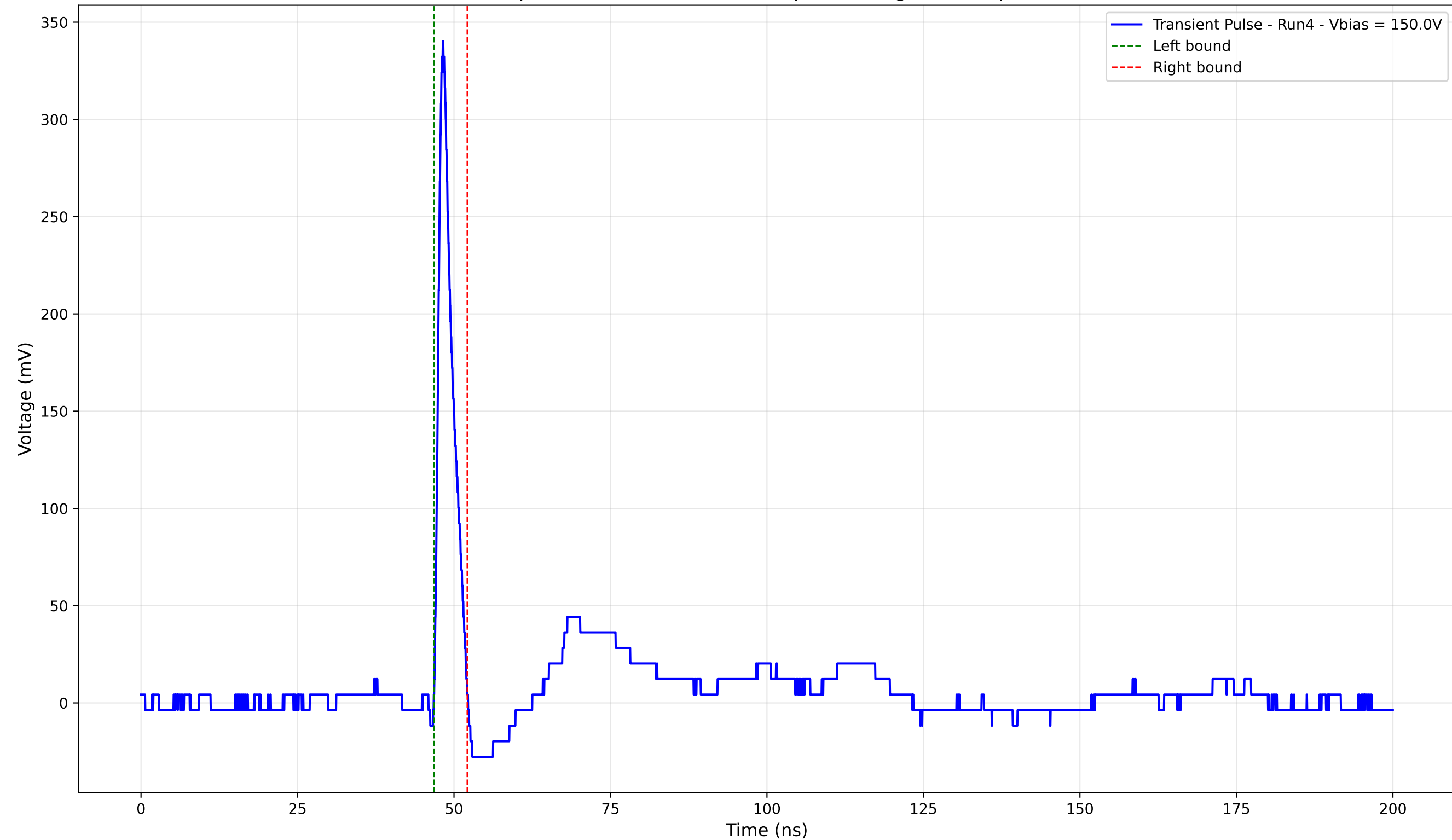
Transient Pulse - Sample: 4003 - Position: 370.0 \mu\text{m} - Charge: 17.16 pC - Rise Time: 0.95 ns
