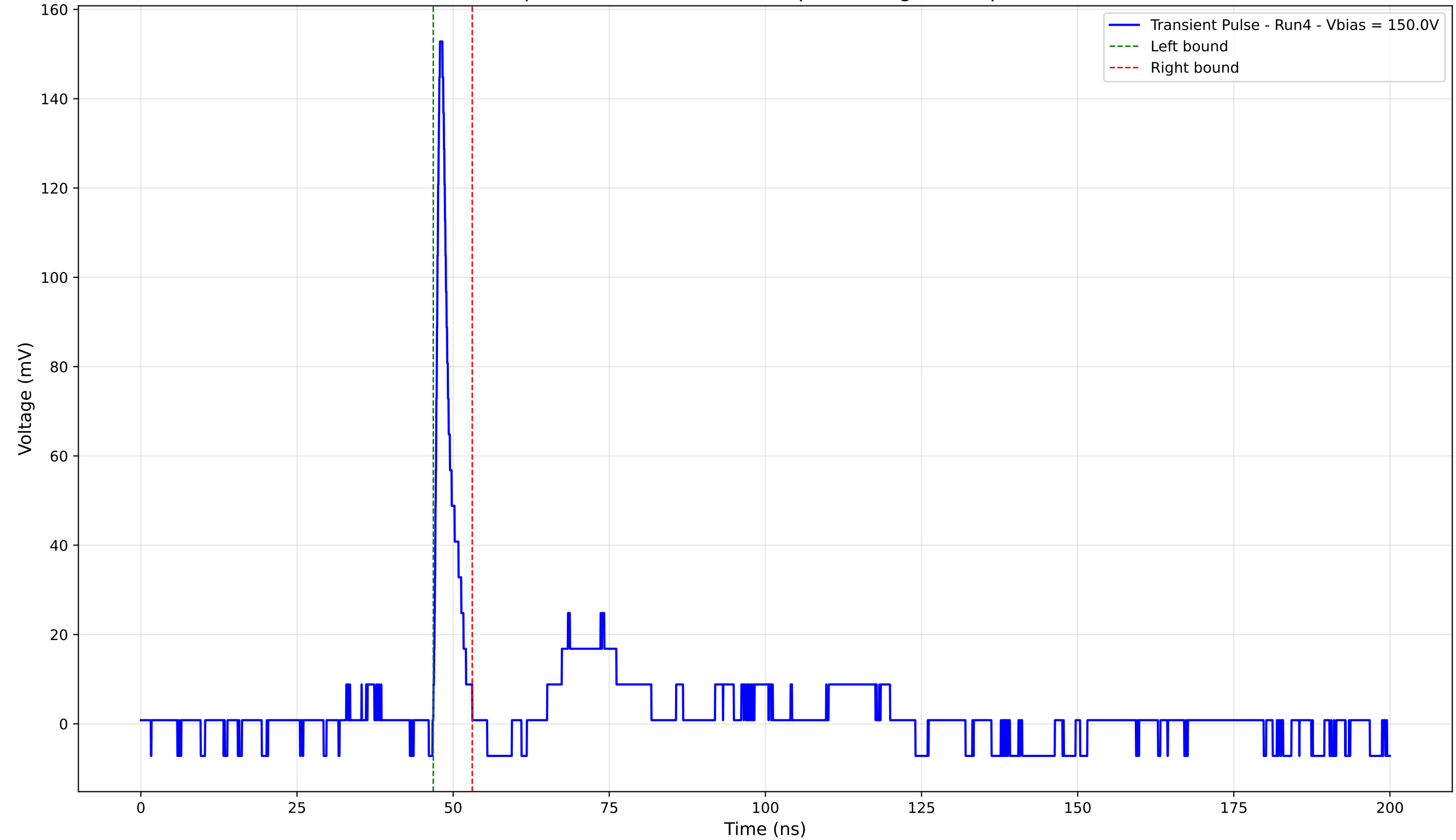
Transient Pulse - Sample: 4003 - Position: 145.0 \mu\text{m} - Charge: 7.30 pC - Rise Time: 0.84 ns
