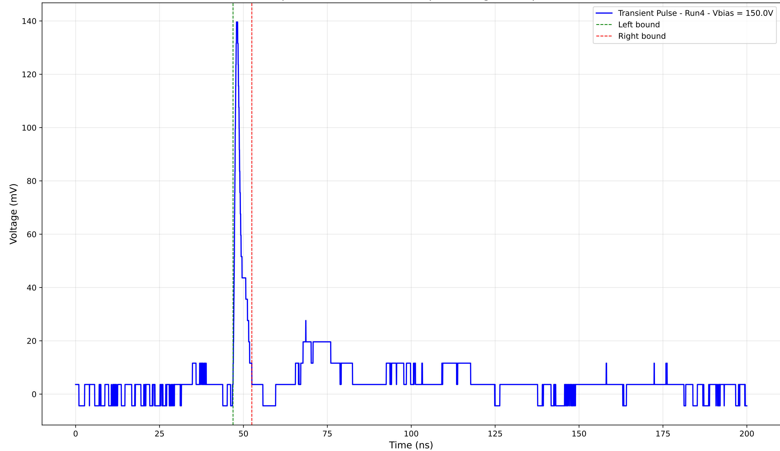
Transient Pulse - Sample: 4003 - Position: 130.0 \mu\text{m} - Charge: 6.48 pC - Rise Time: 0.83 ns
