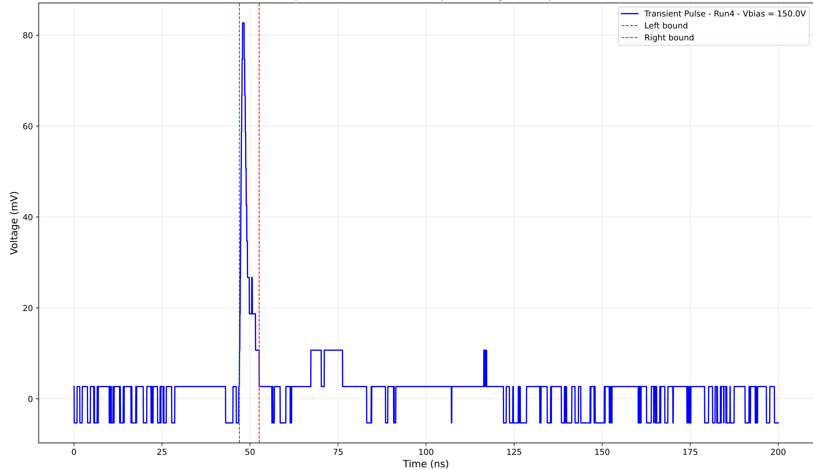
Transient Pulse - Sample: 4003 - Position: 90.0 \mu\text{m} - Charge: 3.73 pC - Rise Time: 0.75 ns
