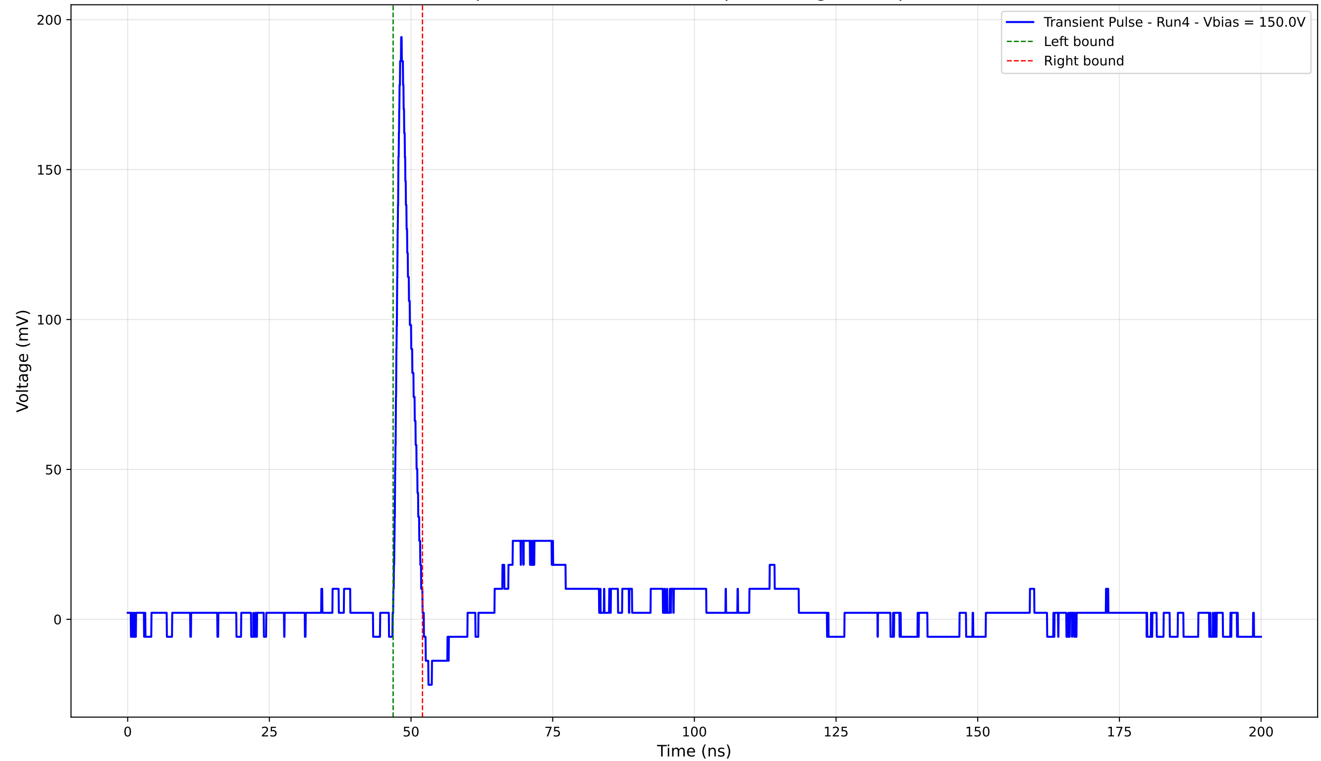
Transient Pulse - Sample: 4003 - Position: 510.0 \mu\text{m} - Charge: 9.99 pC - Rise Time: 0.94 ns
