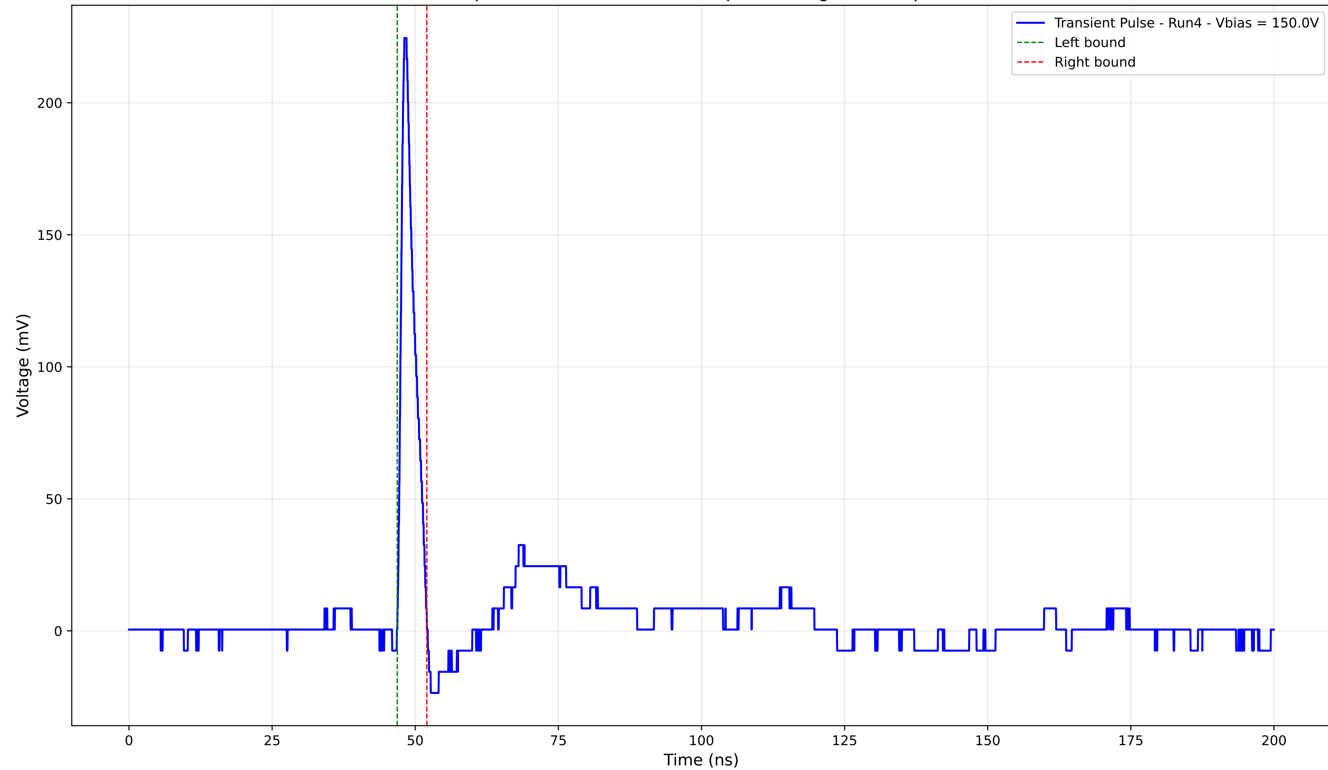
Transient Pulse - Sample: 4003 - Position: 480.0 \mu\text{m} - Charge: 11.72 pC - Rise Time: 0.93 ns
