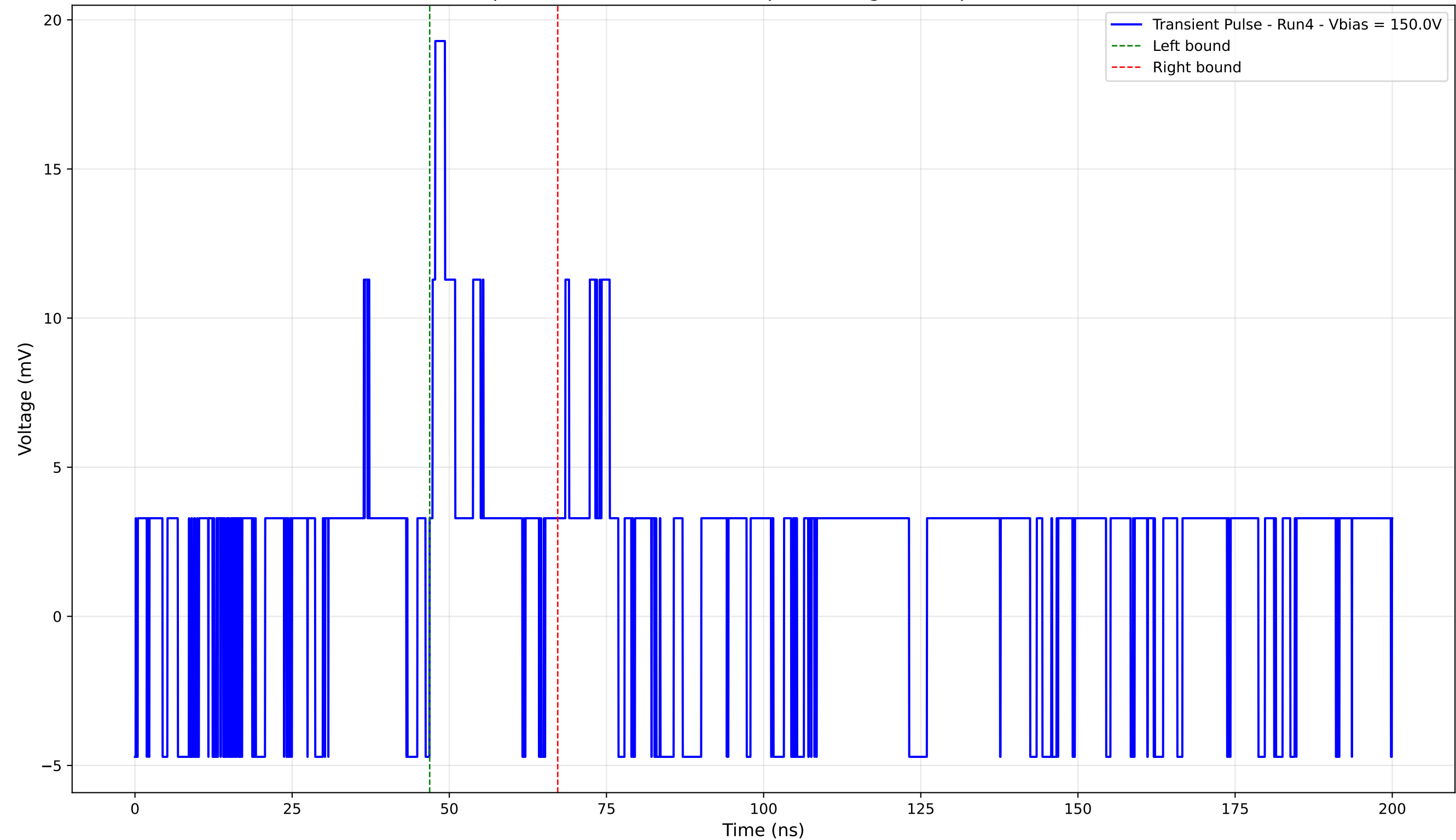
Transient Pulse - Sample: 4003 - Position: 620.0 \mu\text{m} - Charge: 2.20 pC - Rise Time: 0.00 ns (N/A)
