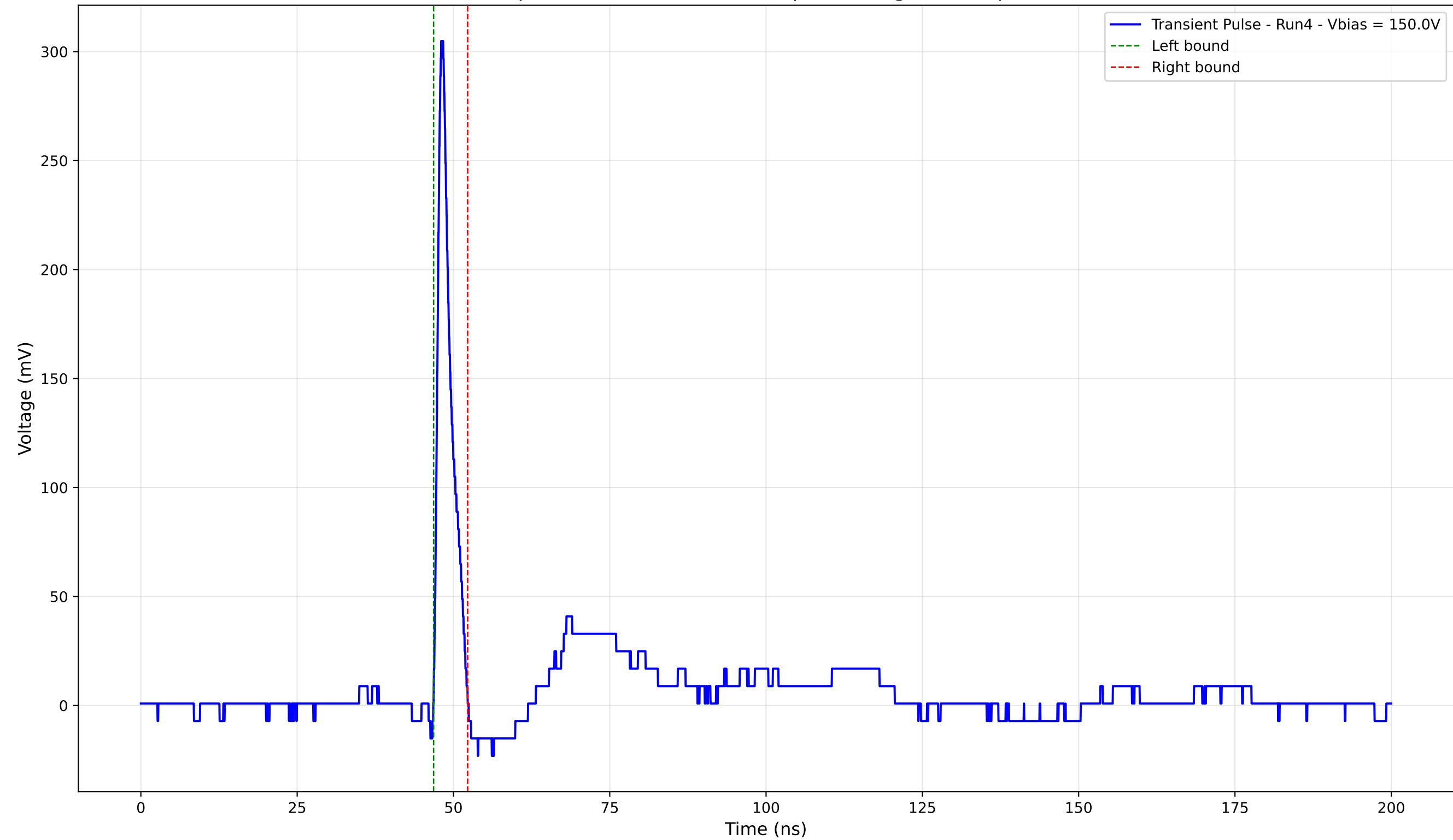
Transient Pulse - Sample: 4003 - Position: 265.0 \mu\text{m} - Charge: 14.95 pC - Rise Time: 0.89 ns
