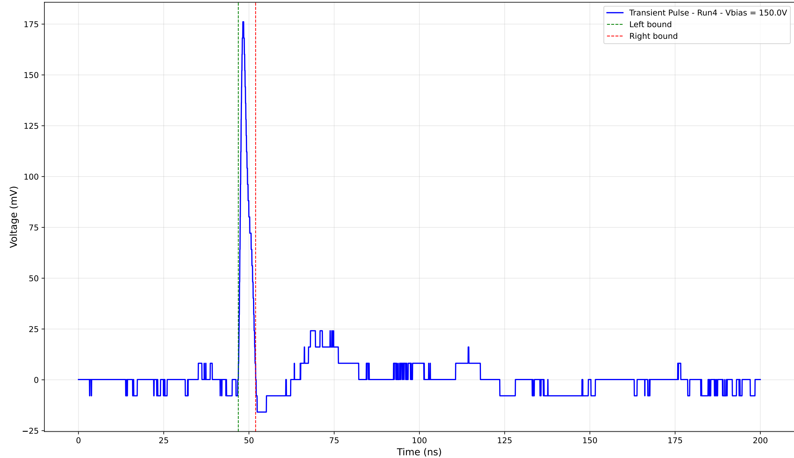
Transient Pulse - Sample: 4003 - Position: 585.0 \mu\text{m} - Charge: 9.13 pC - Rise Time: 0.92 ns
