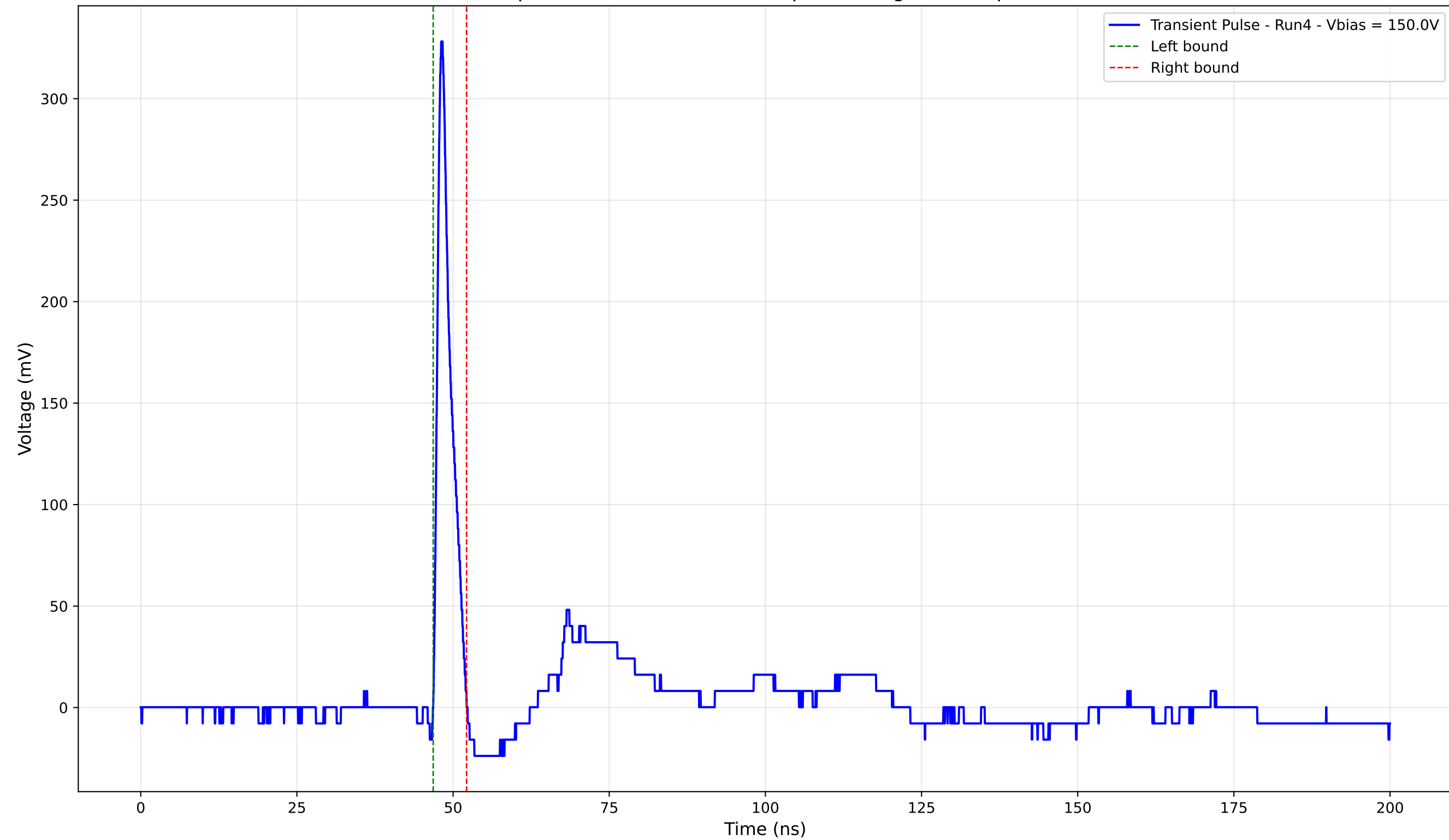
Transient Pulse - Sample: 4003 - Position: 295.0 \mu\text{m} - Charge: 16.14 pC - Rise Time: 0.86 ns
