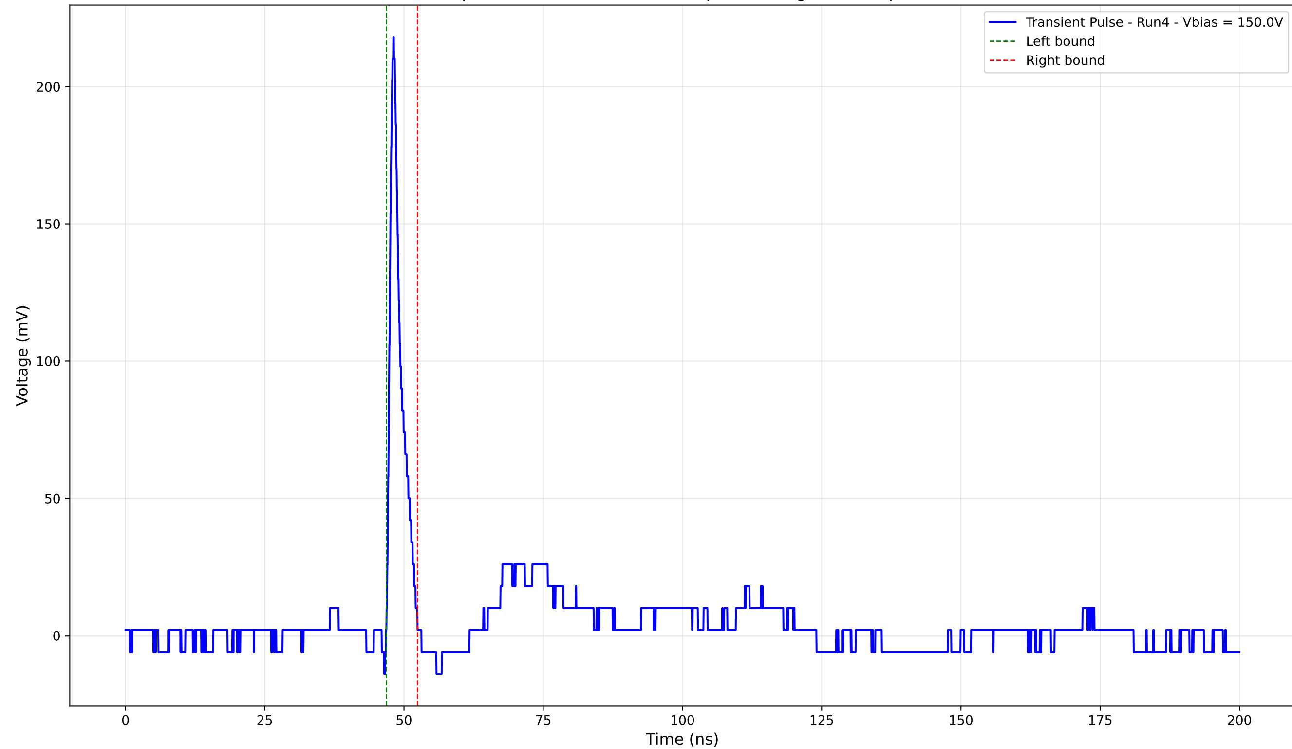
Transient Pulse - Sample: 4003 - Position: 185.0 \mu\text{m} - Charge: 10.12 pC - Rise Time: 0.87 ns
