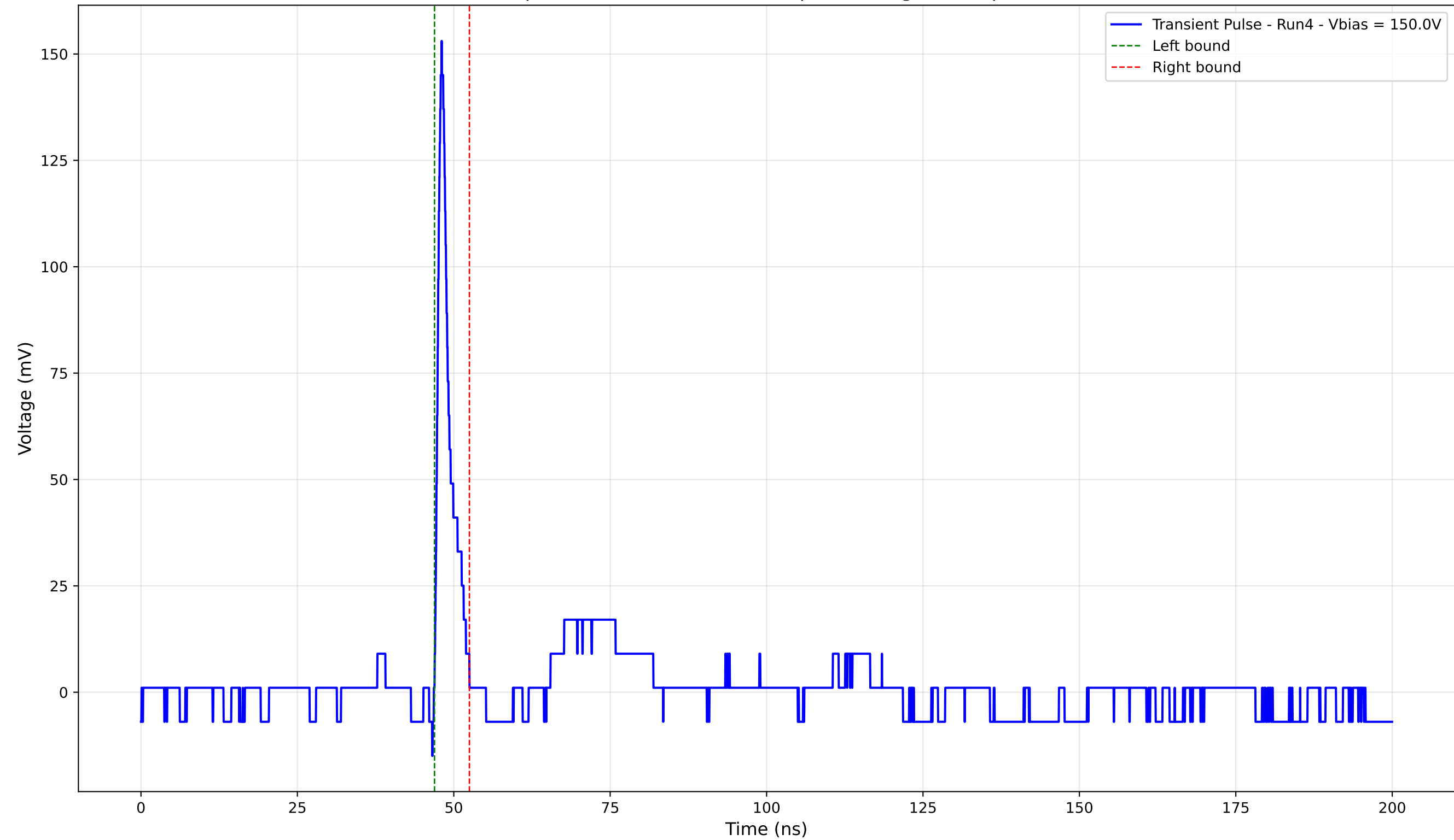
Transient Pulse - Sample: 4003 - Position: 135.0 \mu\text{m} - Charge: 6.60 pC - Rise Time: 0.88 ns
