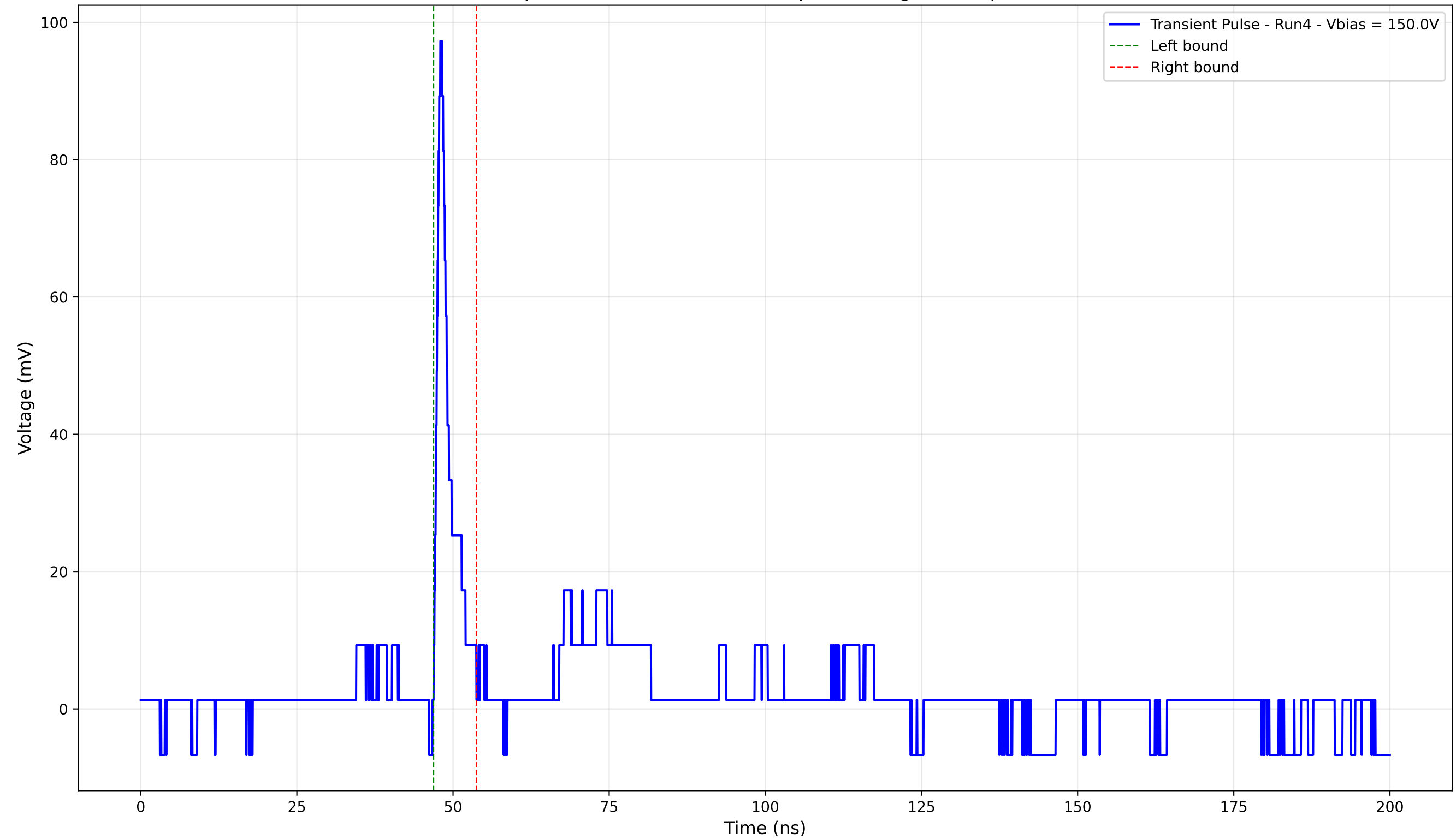
Transient Pulse - Sample: 4003 - Position: 100.0 \mu\text{m} - Charge: 4.67 pC - Rise Time: 0.78 ns
