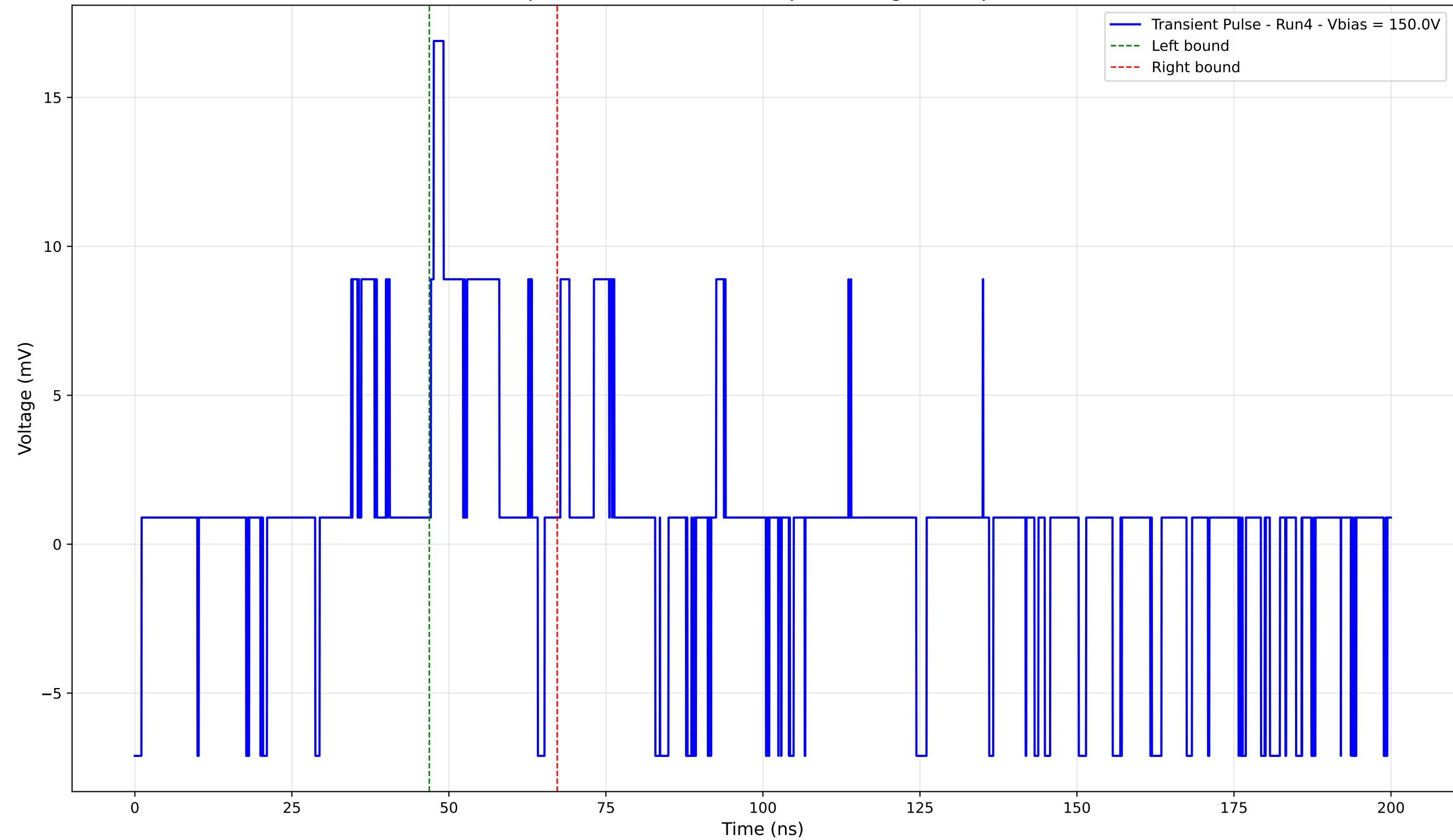
Transient Pulse - Sample: 4003 - Position: 20.0 \mu\text{m} - Charge: 2.14 pC - Rise Time: 0.46 ns
