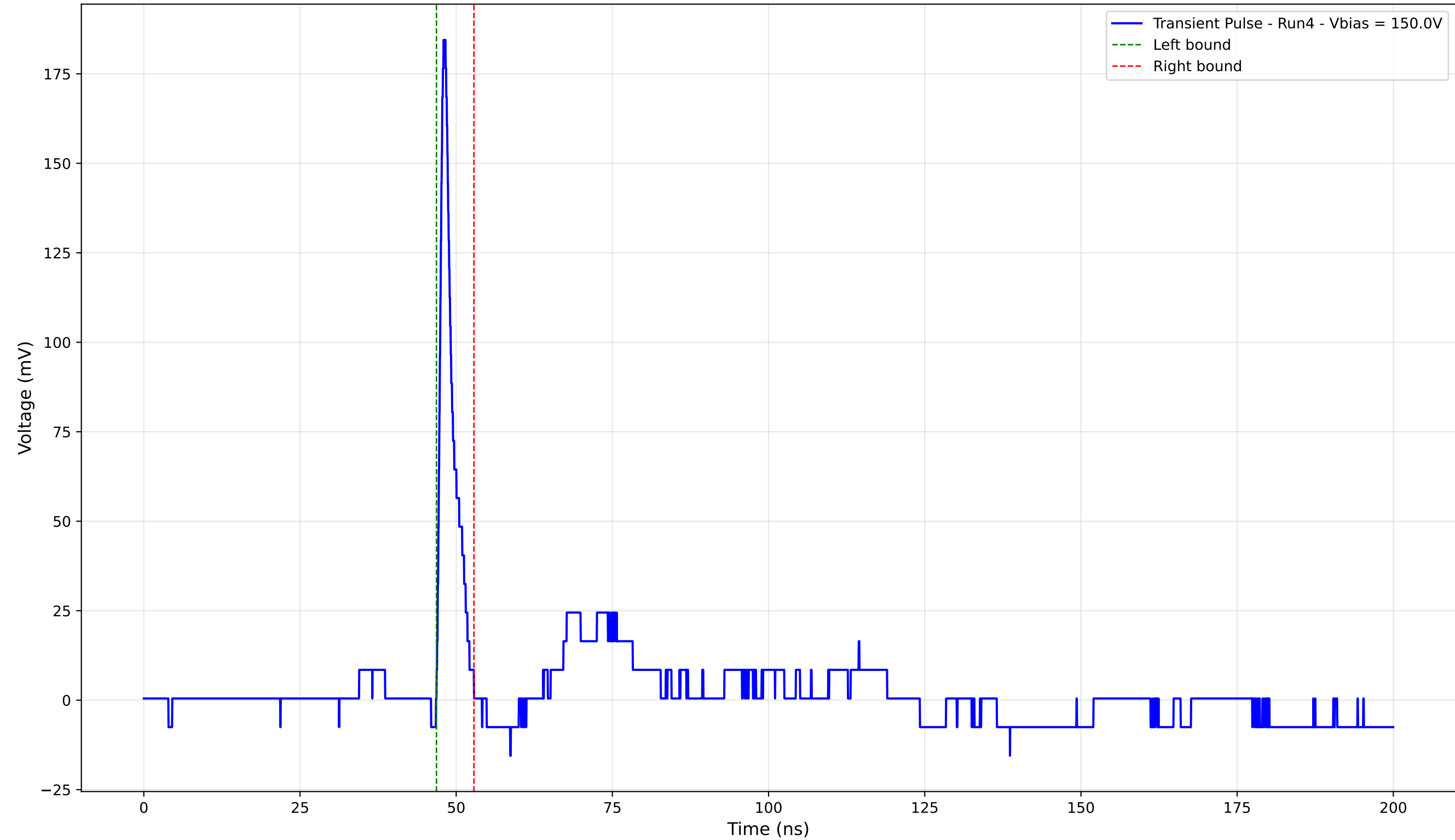
Transient Pulse - Sample: 4003 - Position: 165.0 \mu\text{m} - Charge: 8.75 pC - Rise Time: 0.78 ns
