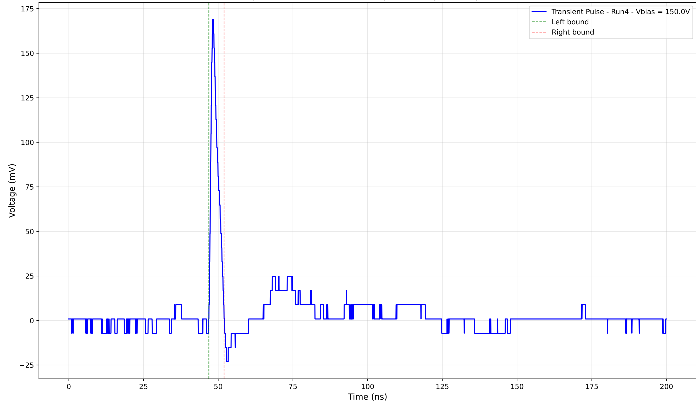
Transient Pulse - Sample: 4003 - Position: 545.0 \mu\text{m} - Charge: 8.76 pC - Rise Time: 0.86 ns
