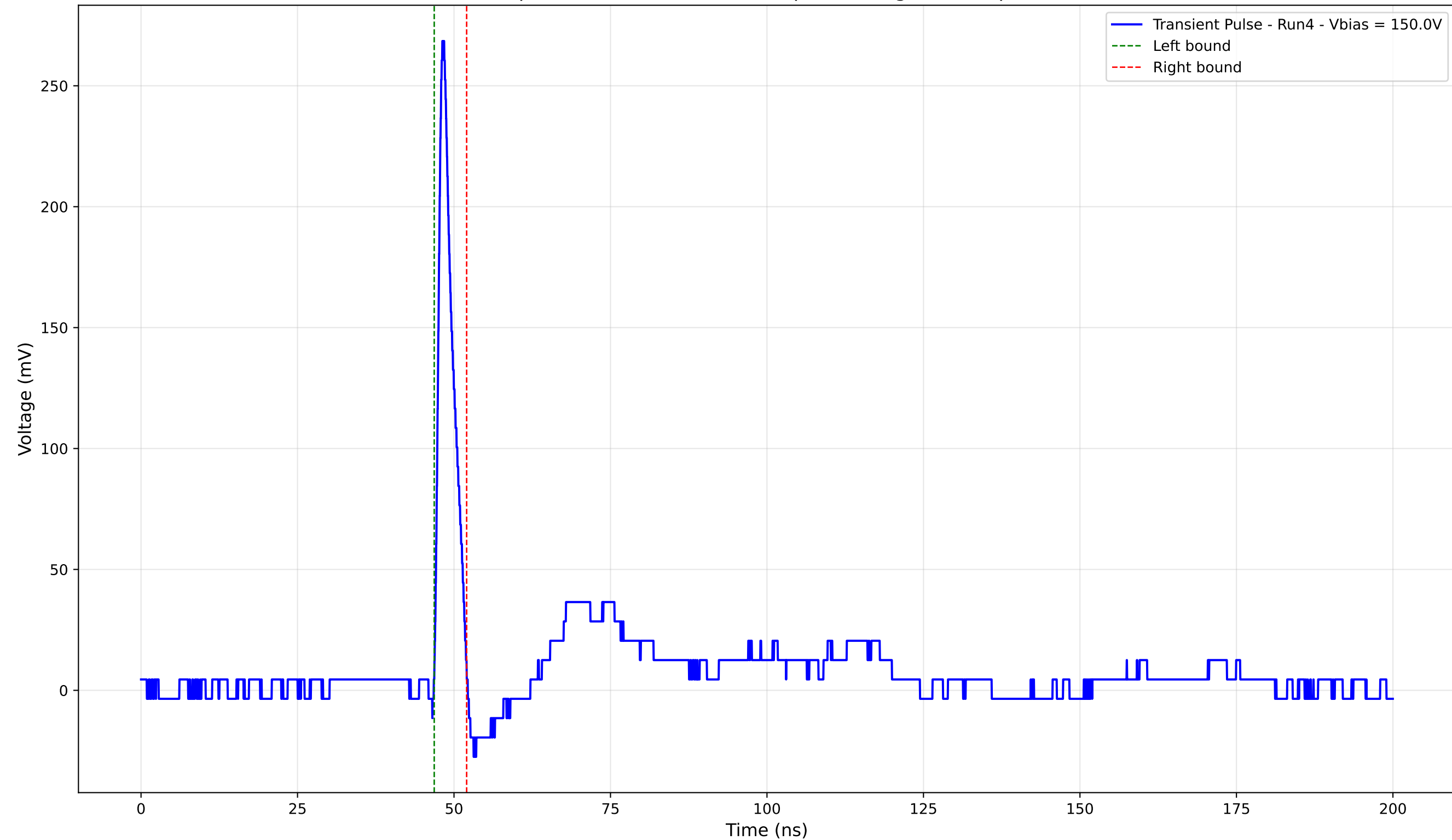
Transient Pulse - Sample: 4003 - Position: 450.0 \mu\text{m} - Charge: 13.95 pC - Rise Time: 0.94 ns
