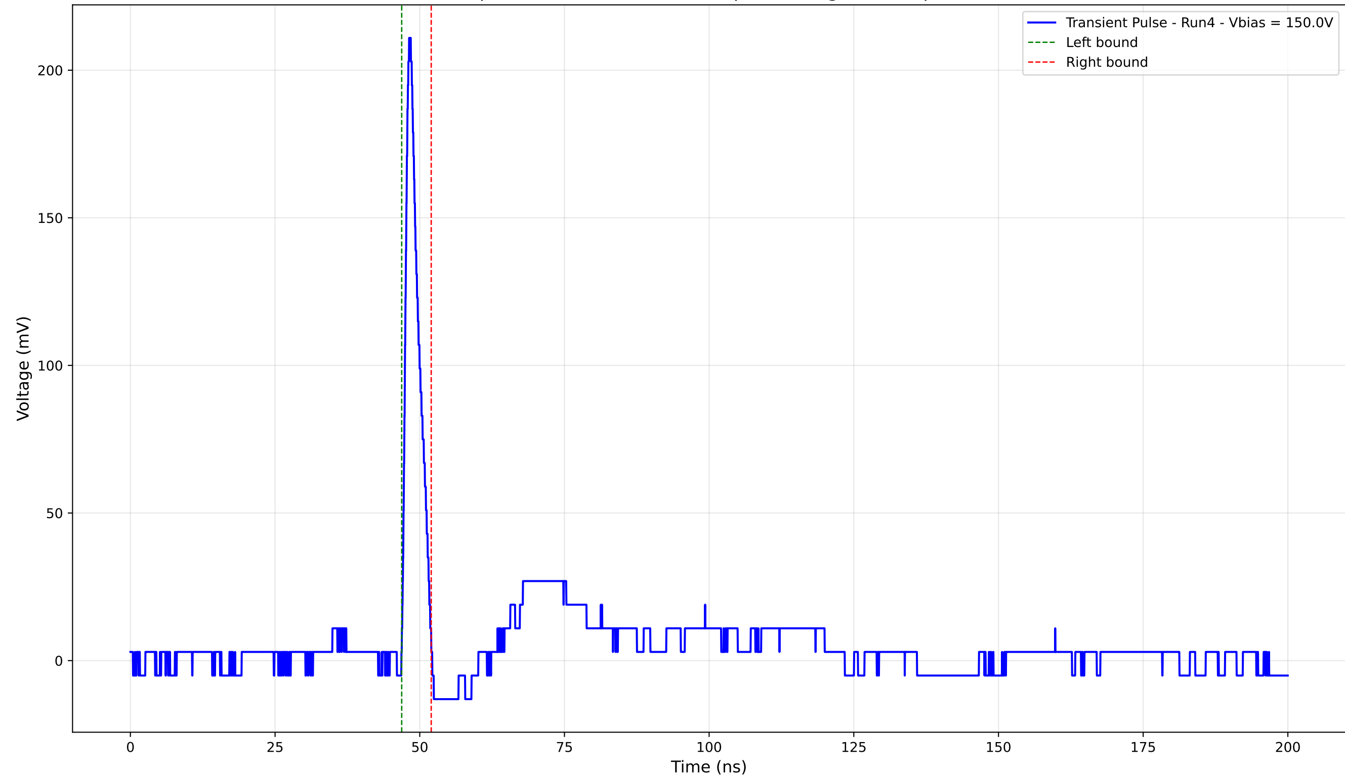
Transient Pulse - Sample: 4003 - Position: 495.0 \mu\text{m} - Charge: 10.95 pC - Rise Time: 0.91 ns
