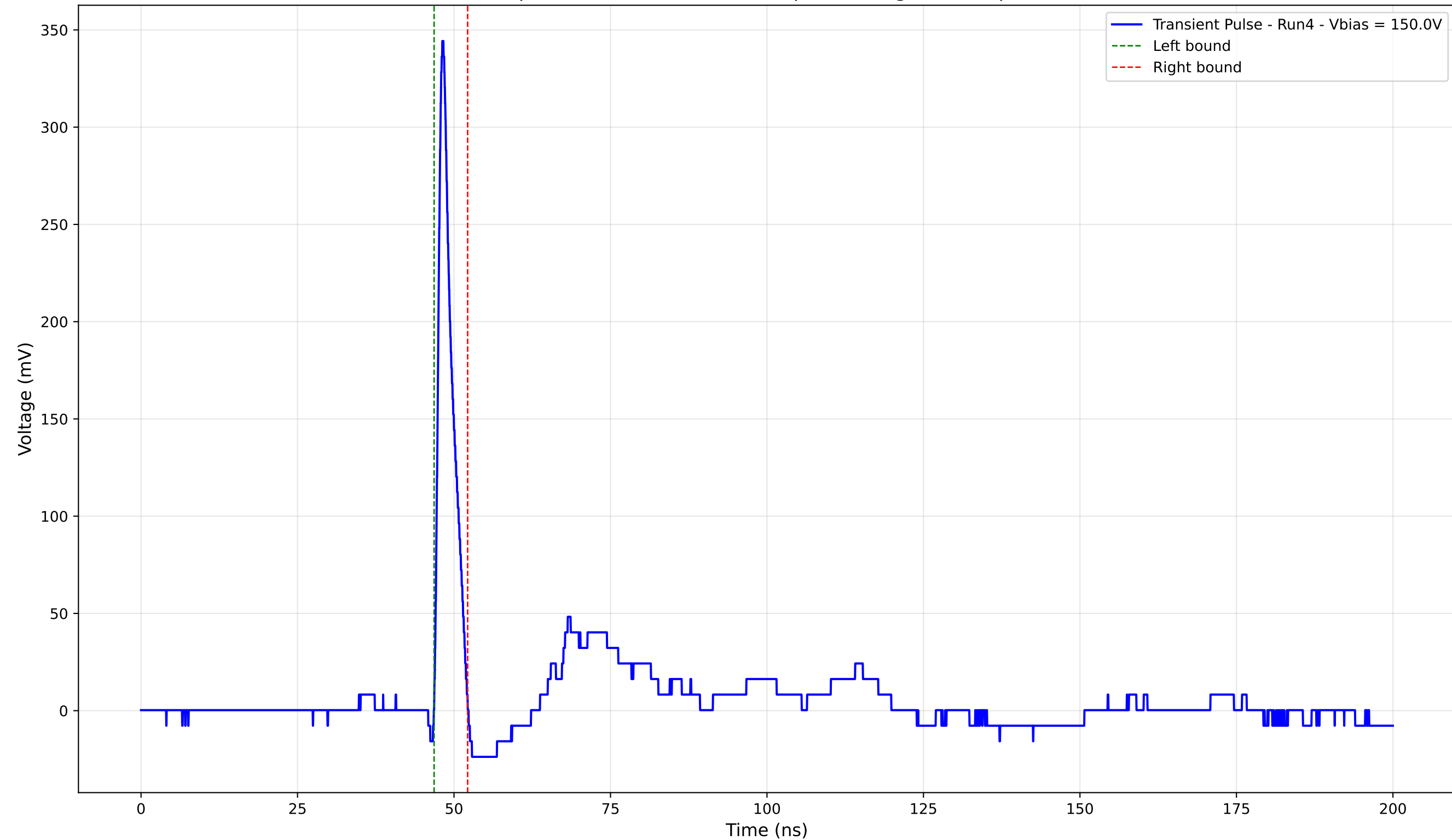
Transient Pulse - Sample: 4003 - Position: 330.0 \mu\text{m} - Charge: 17.19 pC - Rise Time: 0.87 ns
