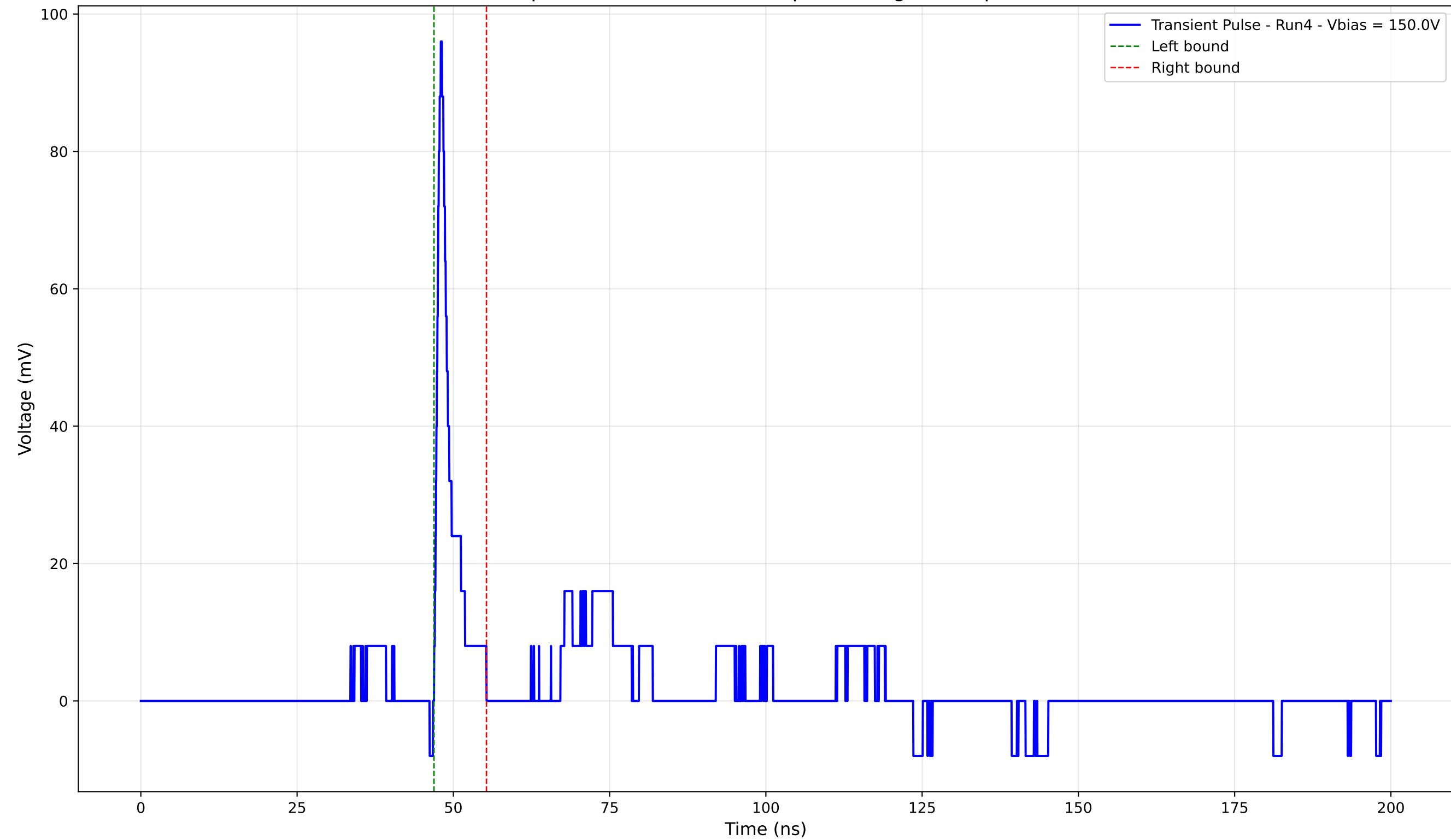
Transient Pulse - Sample: 4003 - Position: 95.0 \mu\text{m} - Charge: 4.66 pC - Rise Time: 0.78 ns
