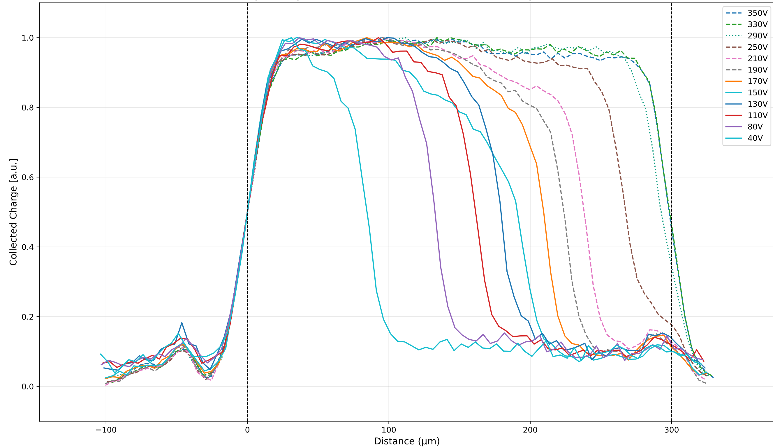
Shape Comparison — Individual Normalization — Sample: 4003
