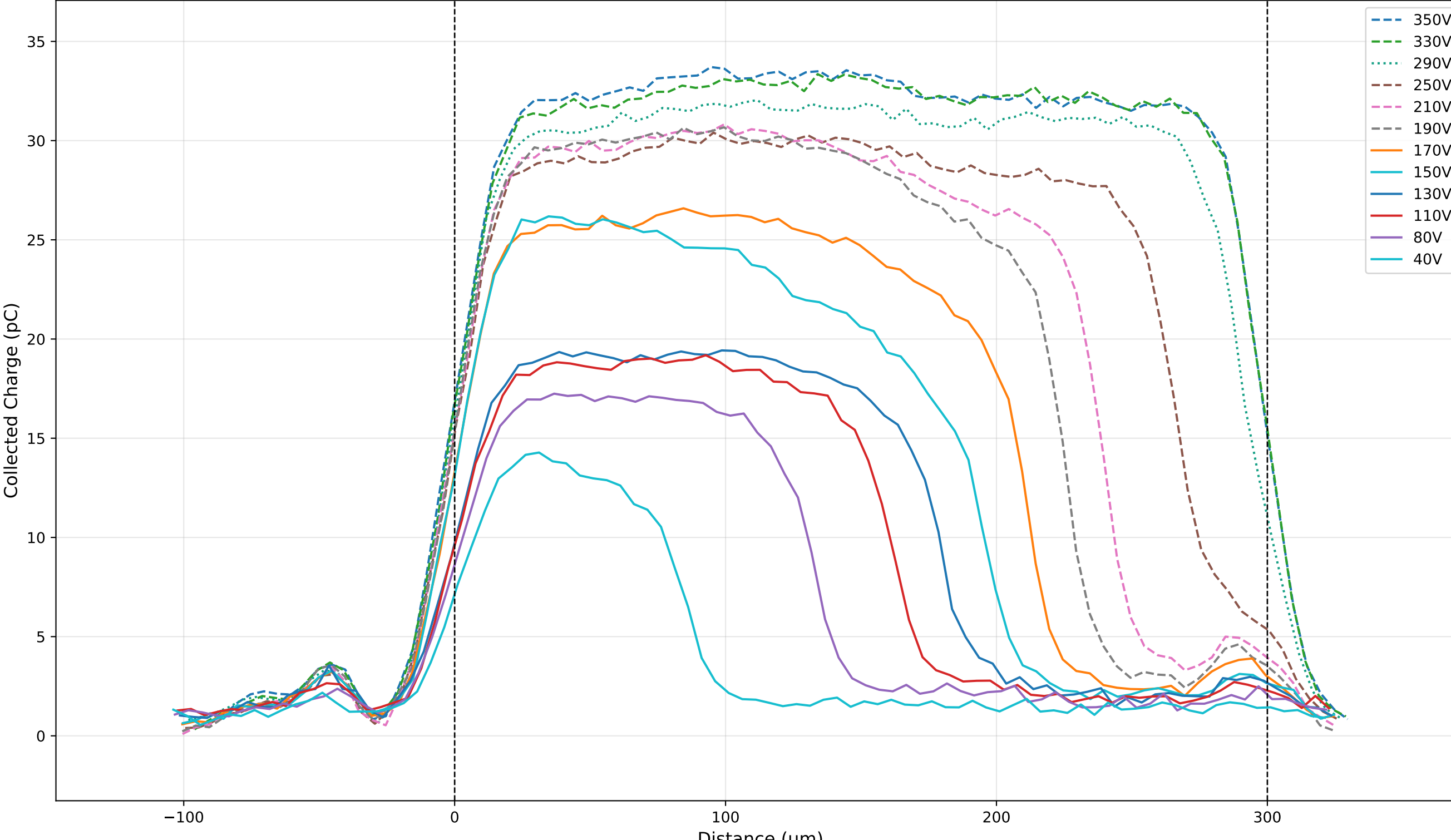
Collected Charge - Sample: 4003
