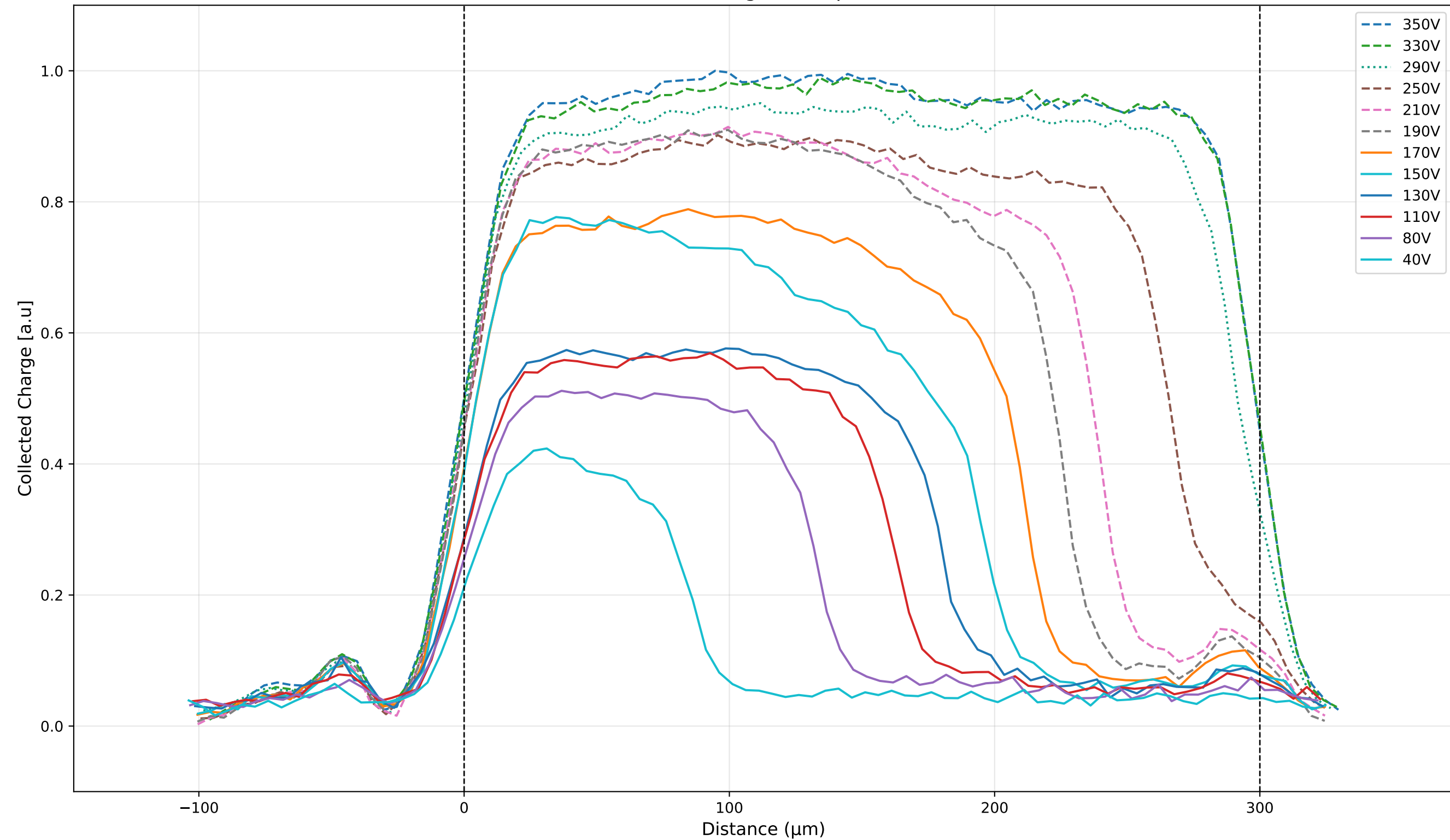
Collected Charge - Sample: 4003
