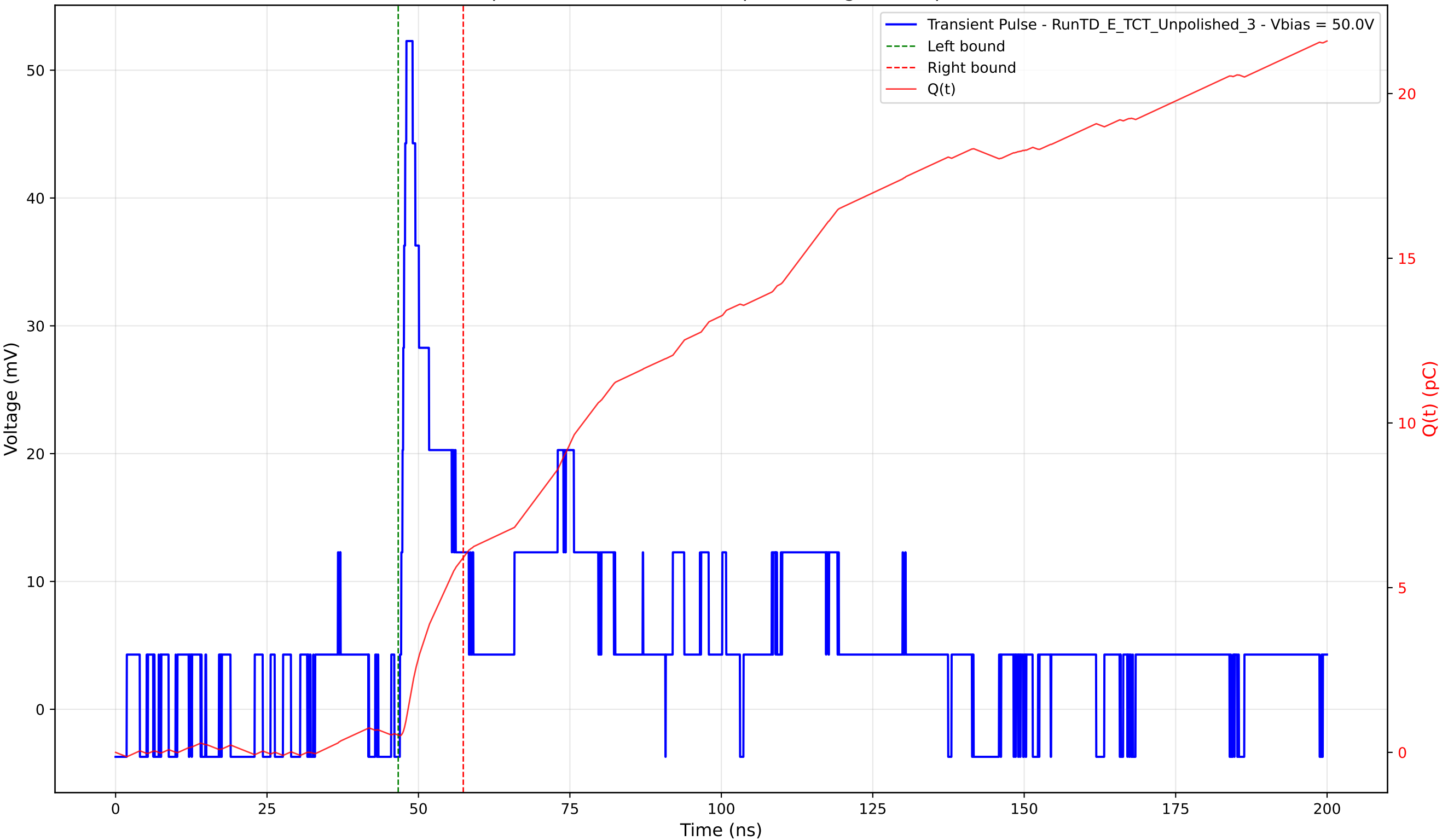
Transient Pulse - Sample: TD - Position: 210.0 \mu\text{m} - Charge: 5.40 pC - Rise Time: 0.86 ns
