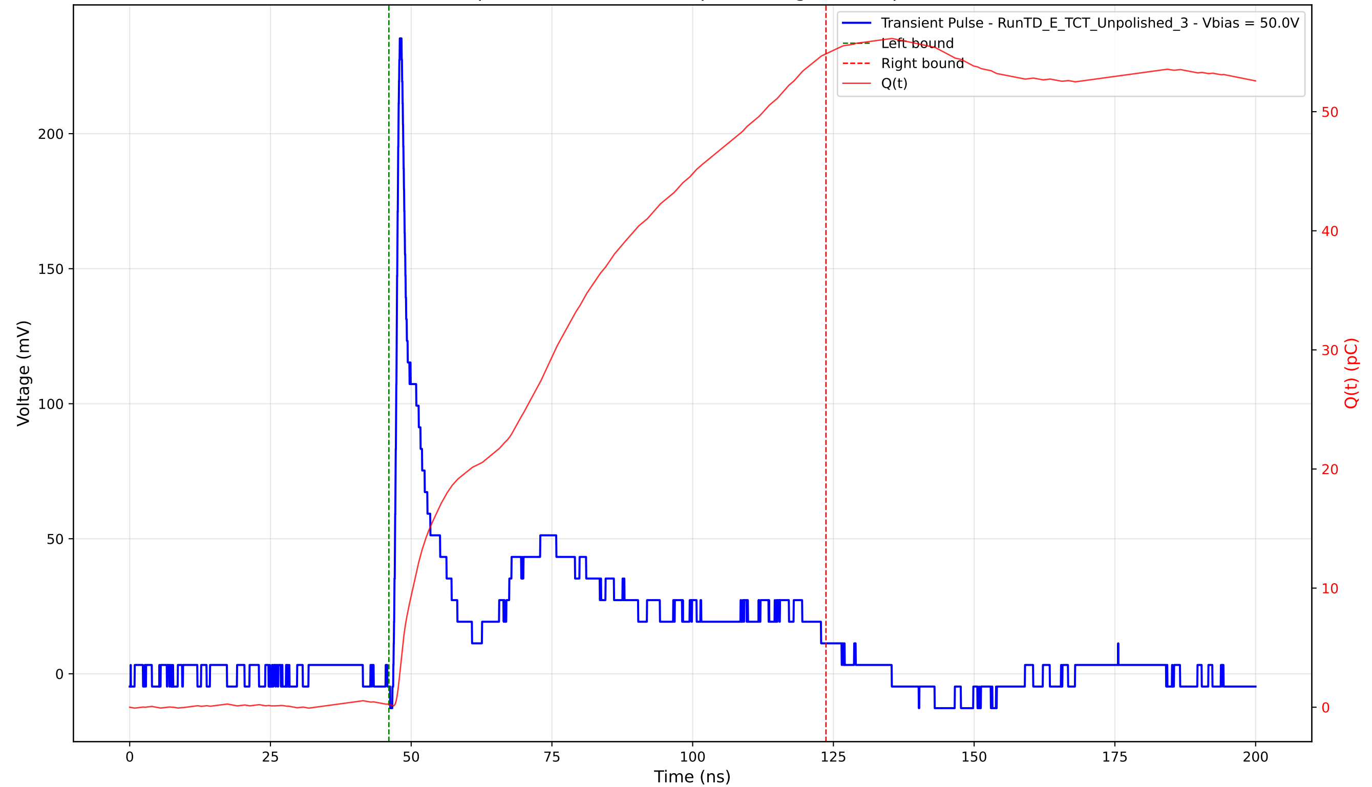
Transient Pulse - Sample: TD - Position: 40.0 \mu\text{m} - Charge: 54.62 pC - Rise Time: 0.83 ns
