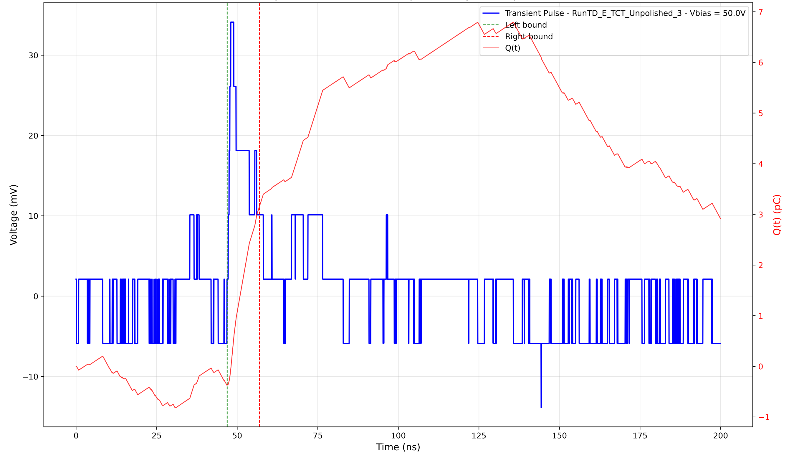
Transient Pulse - Sample: TD - Position: 375.0 \mu\text{m} - Charge: 3.54 pC - Rise Time: 0.82 ns
