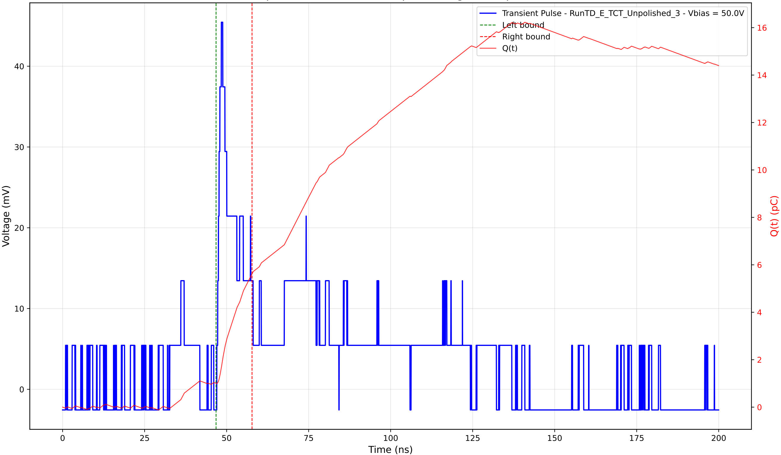
Transient Pulse - Sample: TD - Position: 380.0 \mu\text{m} - Charge: 4.62 pC - Rise Time: 1.39 ns
