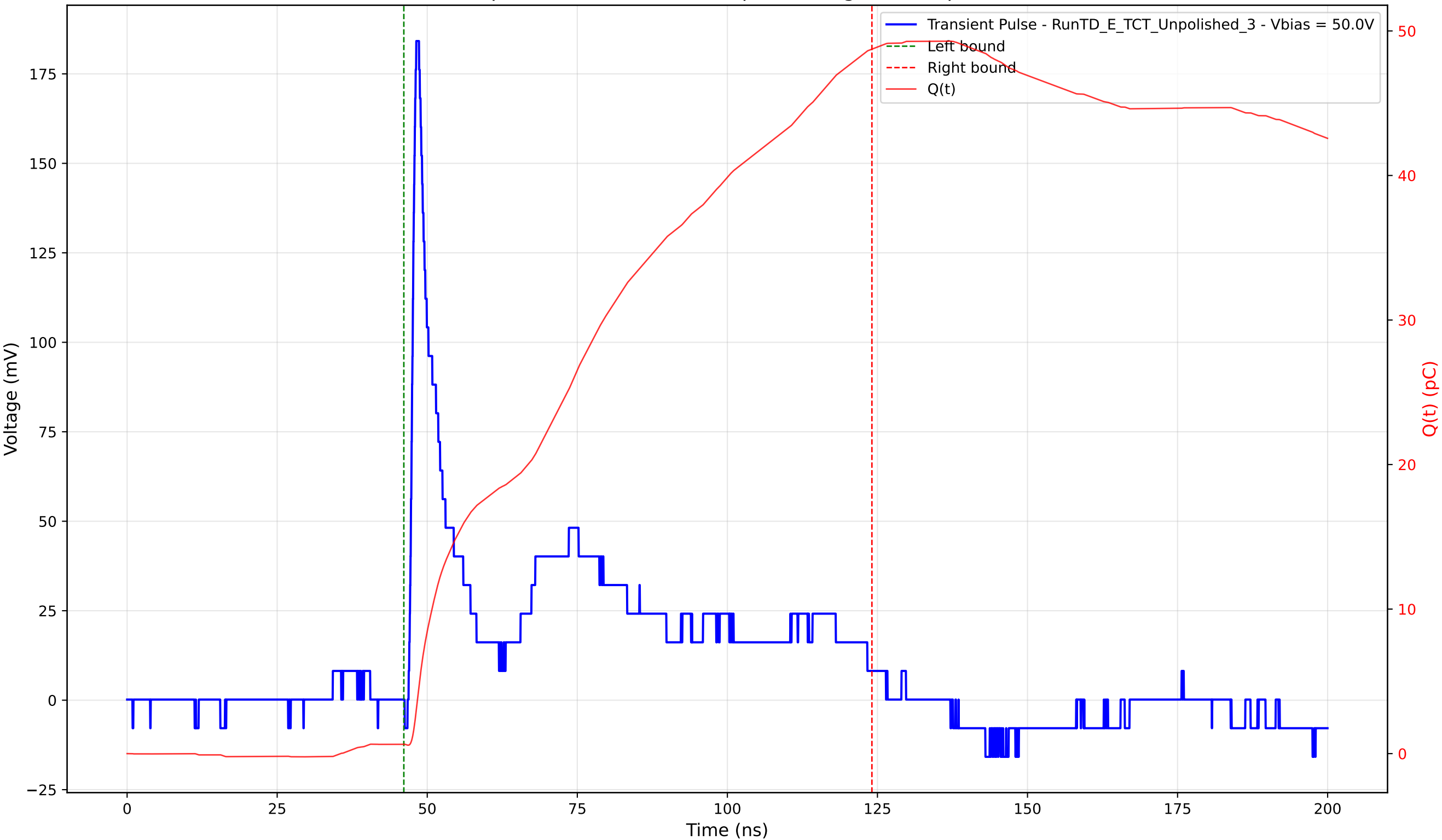
Transient Pulse - Sample: TD - Position: 120.0 \mu\text{m} - Charge: 48.09 pC - Rise Time: 0.91 ns
