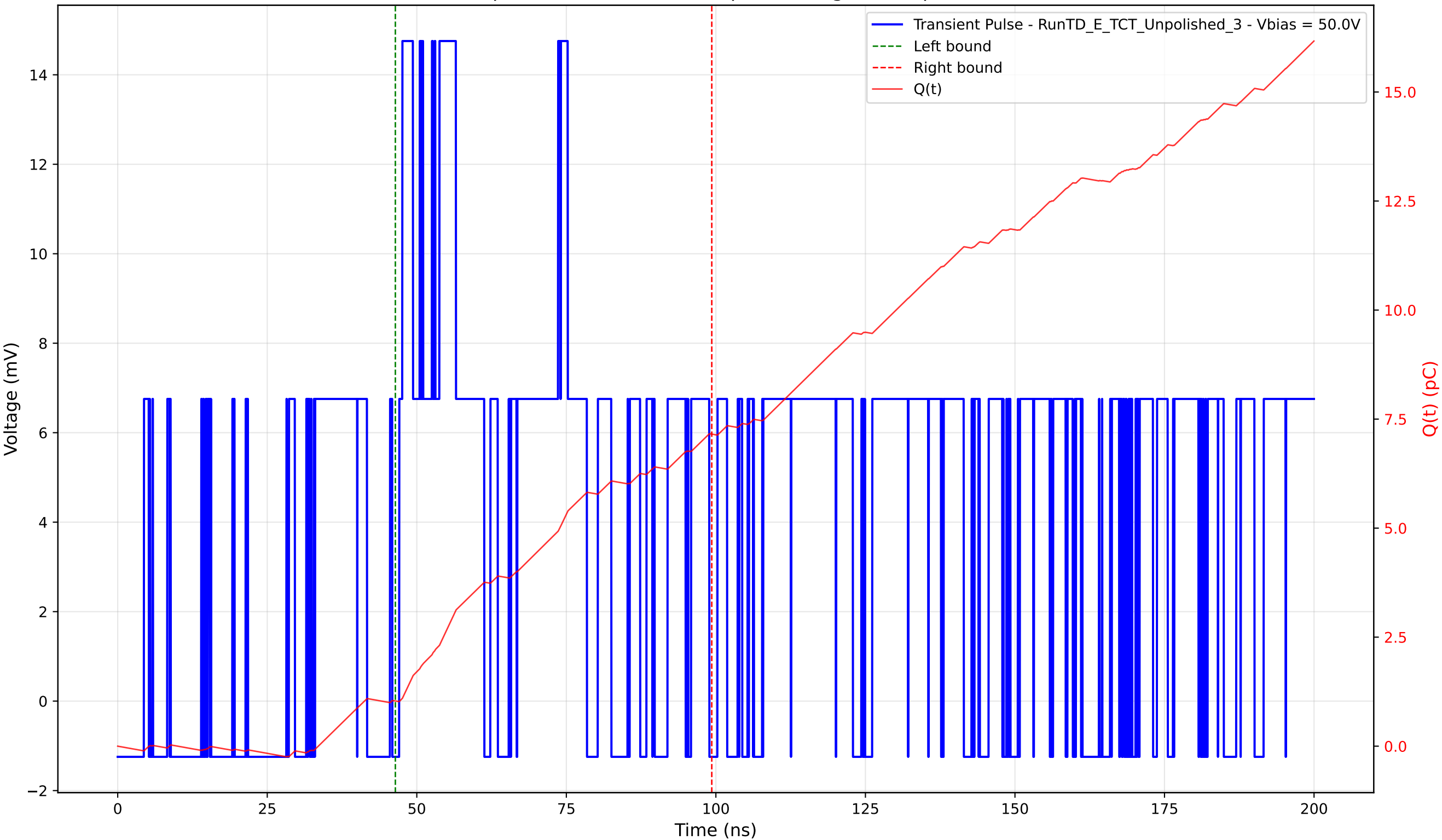
Transient Pulse - Sample: TD - Position: 10.0 \mu\text{m} - Charge: 6.12 pC - Rise Time: 0.54 ns
