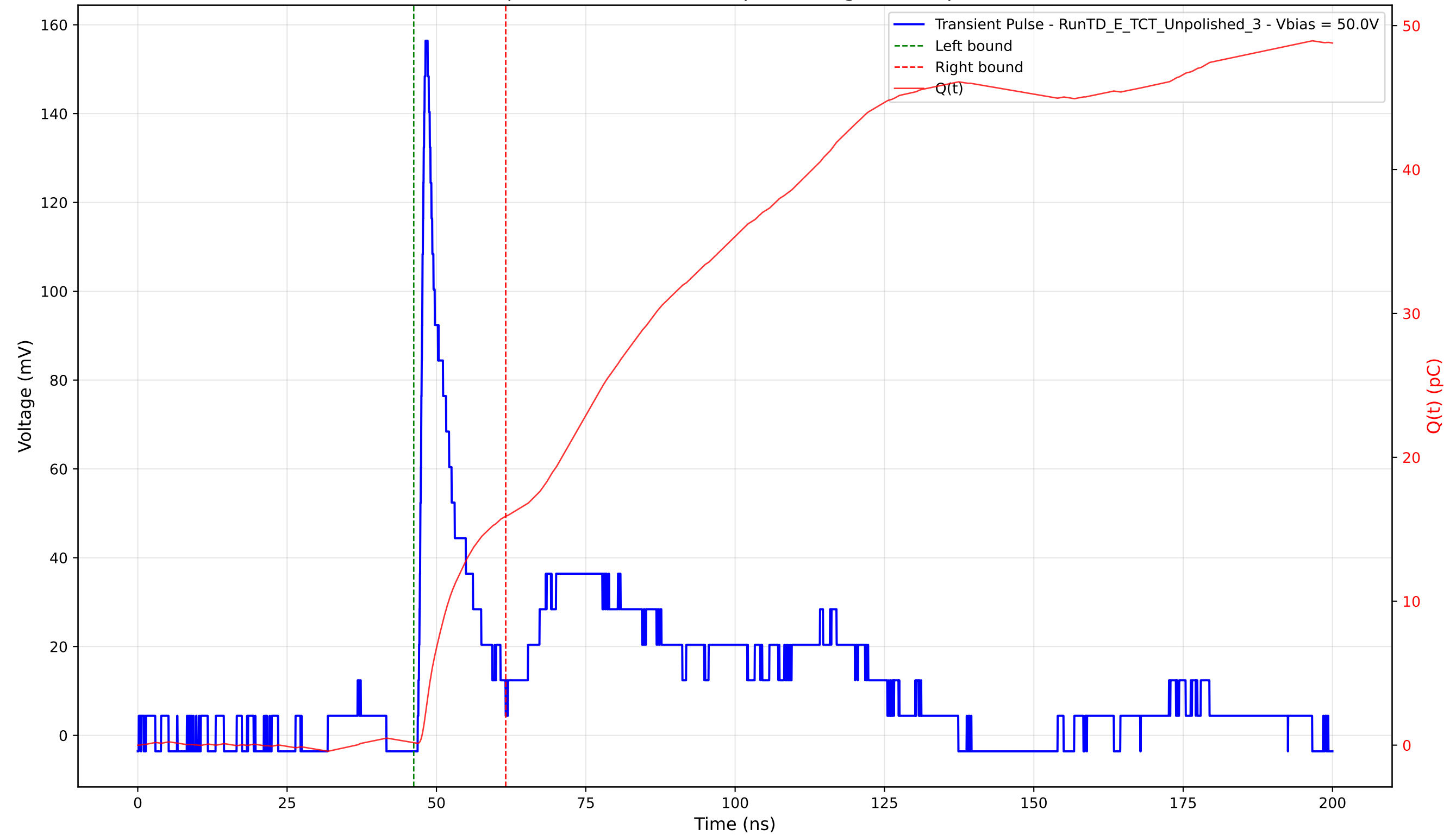
Transient Pulse - Sample: TD - Position: 95.0 \mu\text{m} - Charge: 15.74 pC - Rise Time: 0.95 ns
