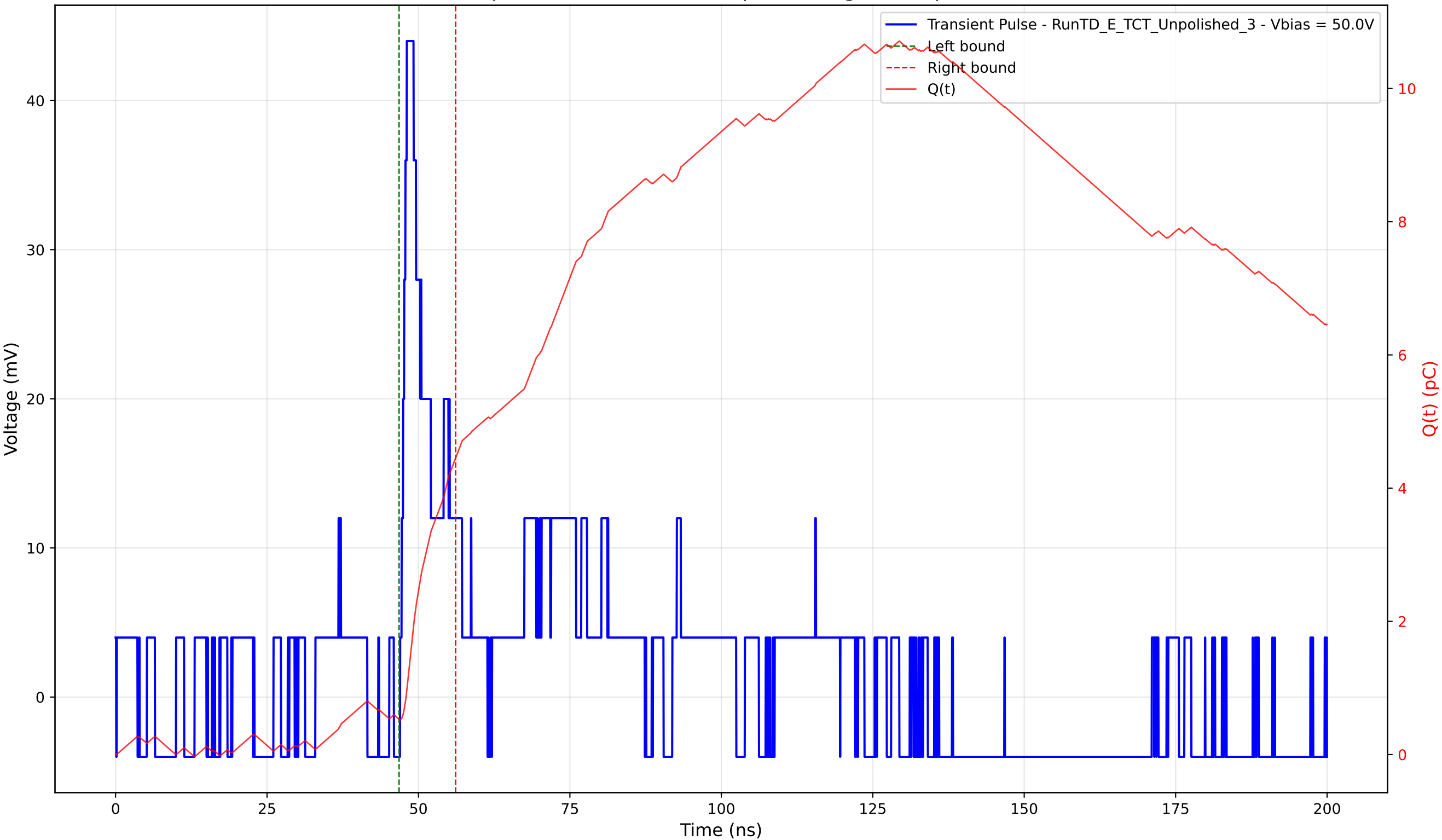
Transient Pulse - Sample: TD - Position: 255.0 \mu\text{m} - Charge: 3.93 pC - Rise Time: 0.86 ns
