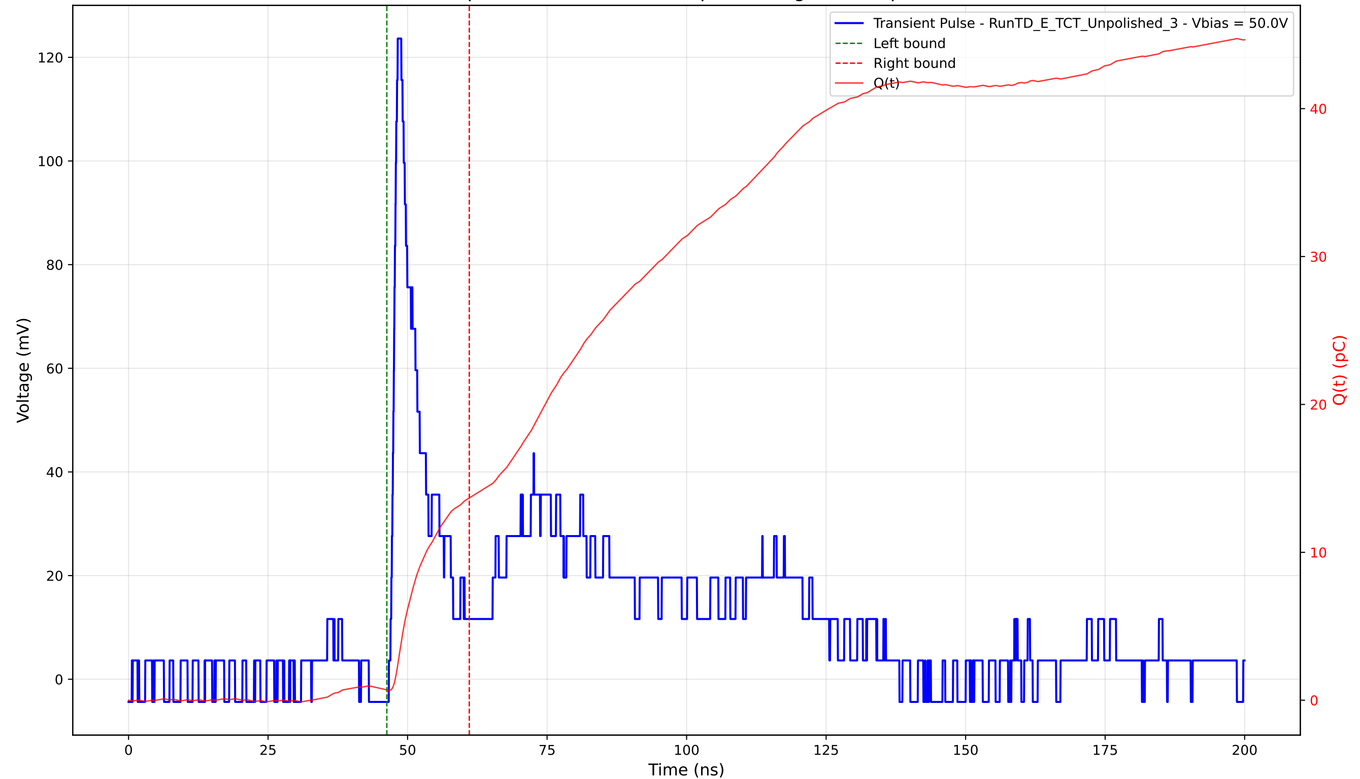
Transient Pulse - Sample: TD - Position: 165.0 \mu\text{m} - Charge: 12.98 pC - Rise Time: 1.04 ns
