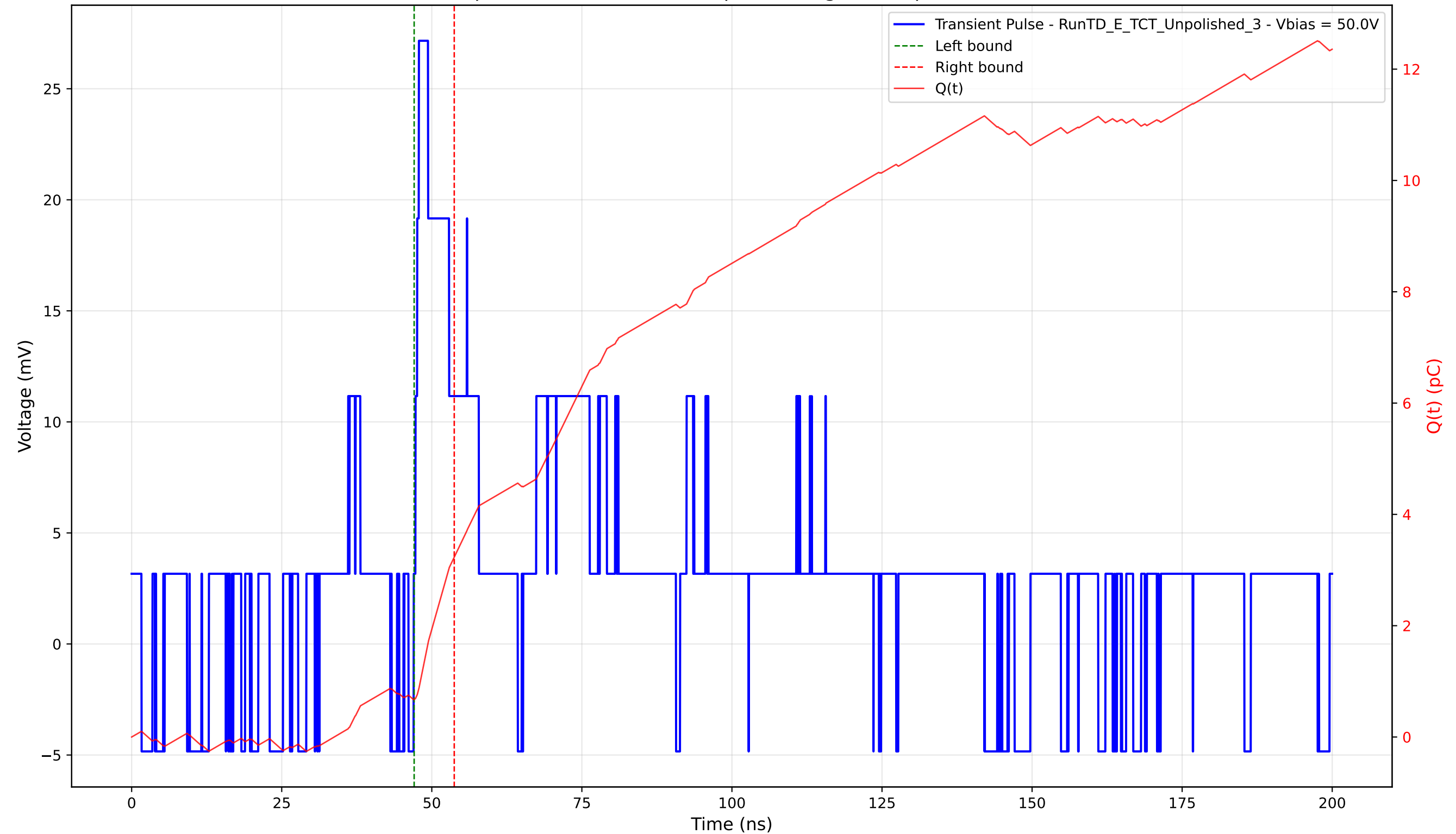
Transient Pulse - Sample: TD - Position: 390.0 \mu\text{m} - Charge: 2.56 pC - Rise Time: 0.00 ns (N/A)
