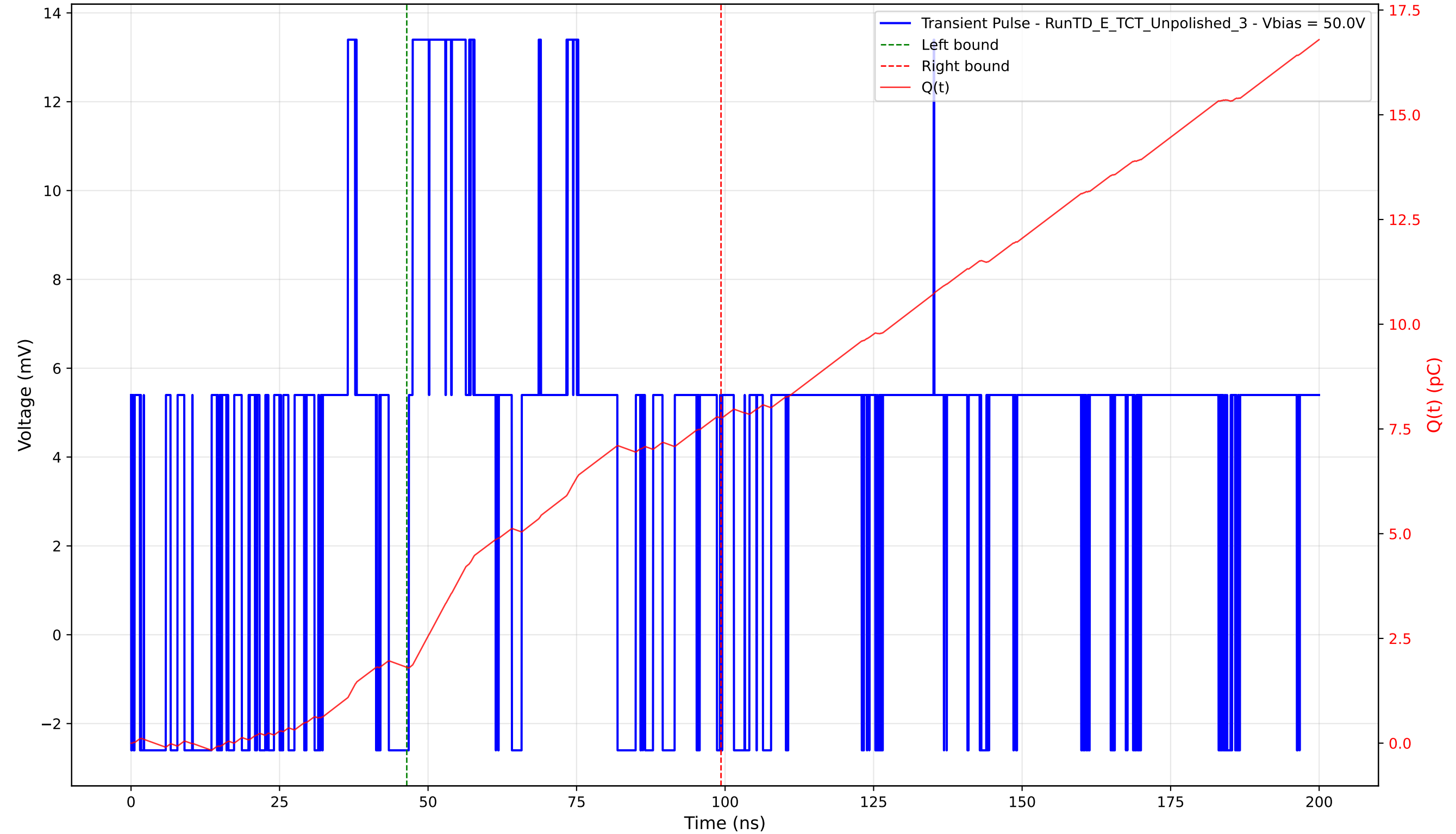
Transient Pulse - Sample: TD - Position: 355.0 \mu\text{m} - Charge: 5.96 pC - Rise Time: 0.00 ns (N/A)
