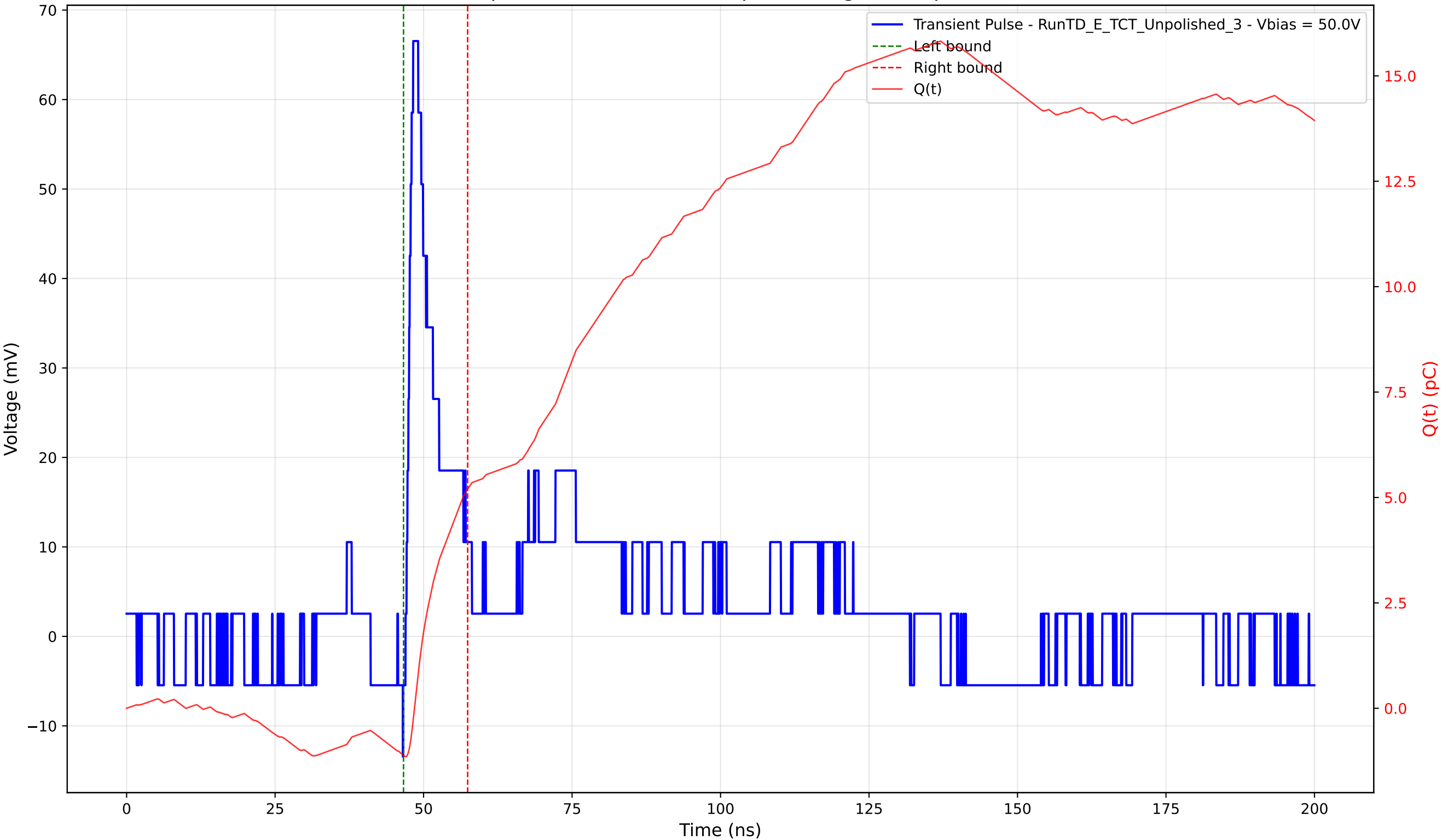
Transient Pulse - Sample: TD - Position: 160.0 \mu\text{m} - Charge: 6.32 pC - Rise Time: 1.11 ns
