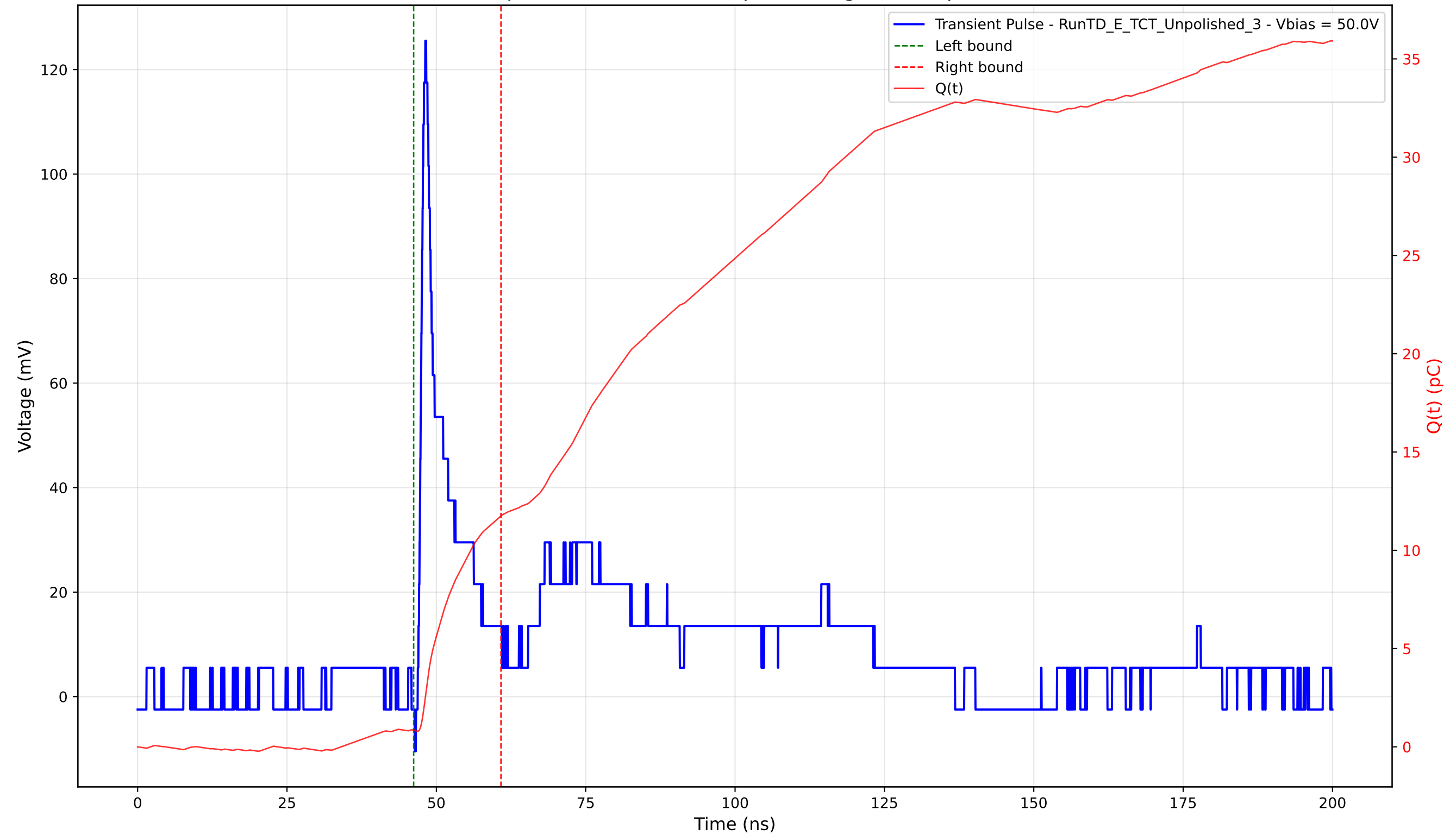
Transient Pulse - Sample: TD - Position: 35.0 \mu\text{m} - Charge: 10.90 pC - Rise Time: 0.92 ns
