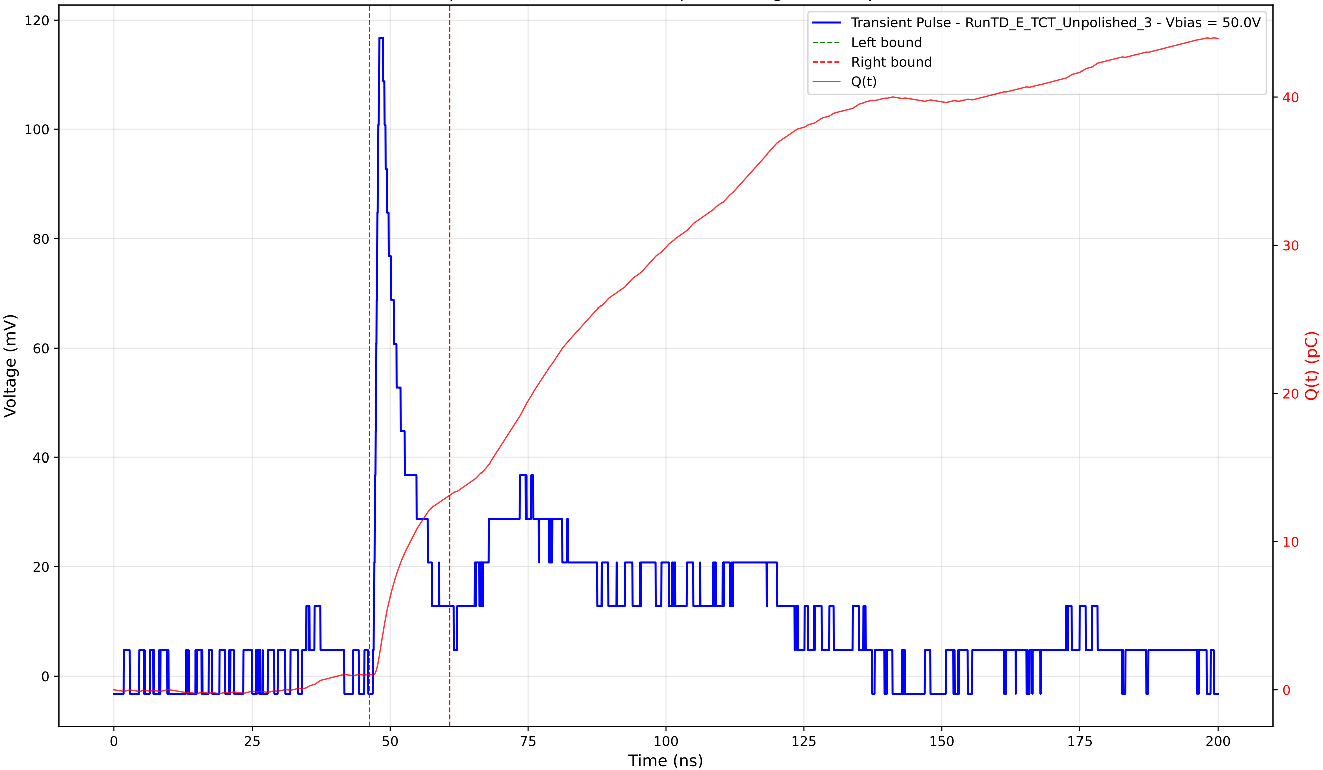
Transient Pulse - Sample: TD - Position: 200.0 \mu\text{m} - Charge: 12.11 pC - Rise Time: 0.92 ns
