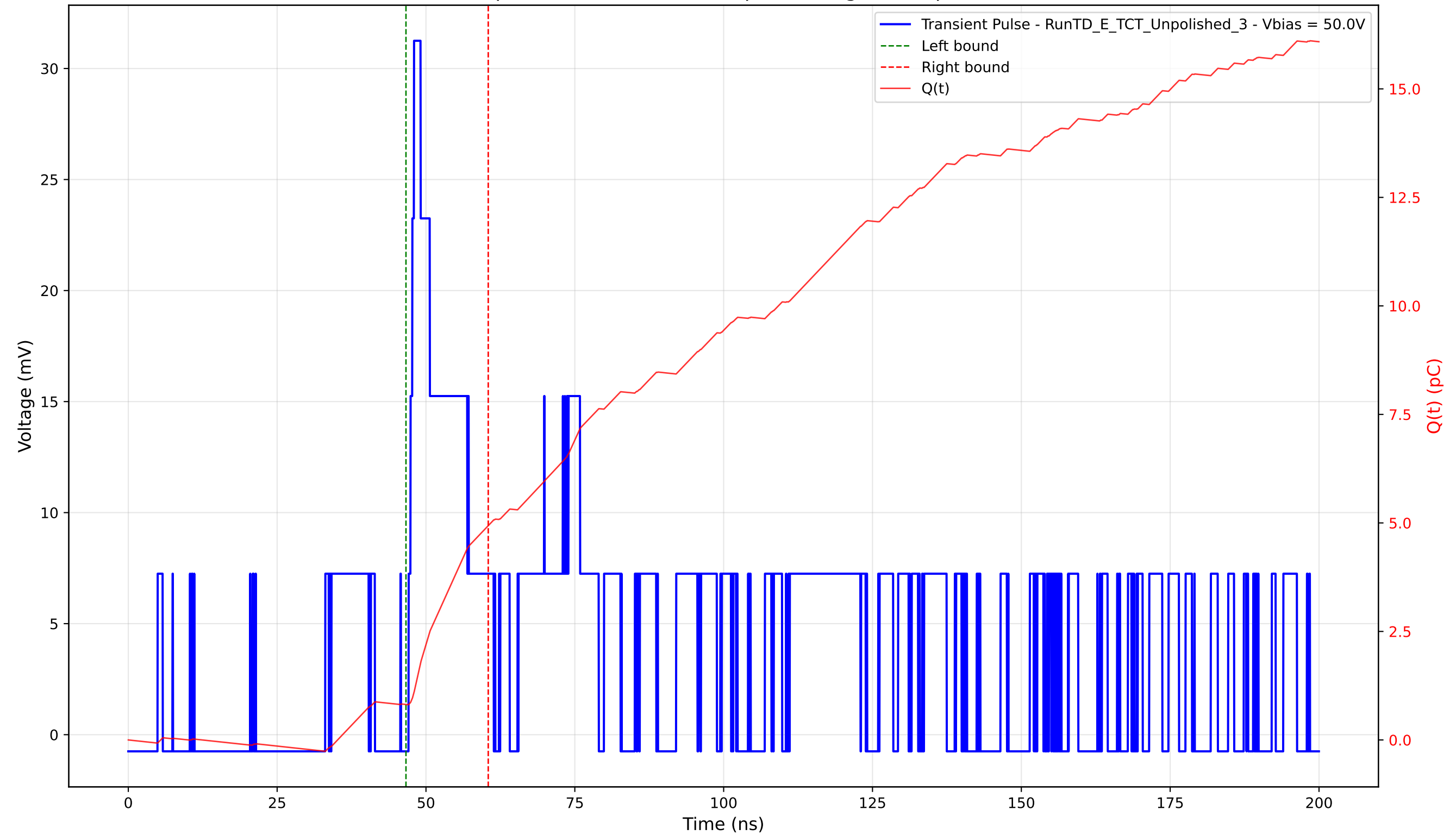
Transient Pulse - Sample: TD - Position: 300.0 \mu\text{m} - Charge: 4.12 pC - Rise Time: 0.91 ns
