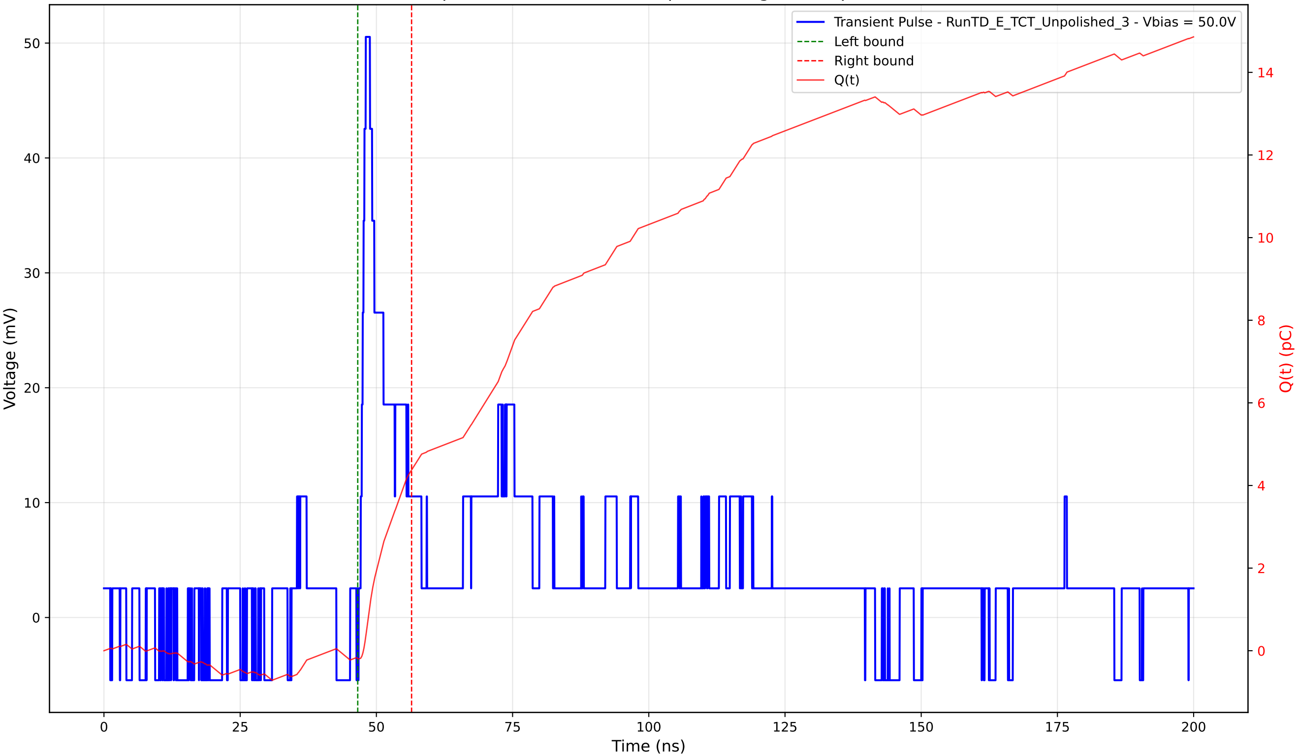
Transient Pulse - Sample: TD - Position: 250.0 \mu\text{m} - Charge: 4.56 pC - Rise Time: 0.93 ns
