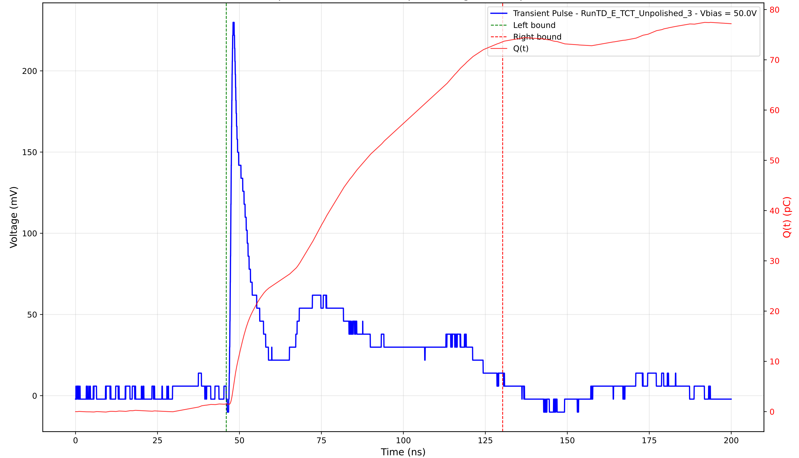
Transient Pulse - Sample: TD - Position: 80.0 \mu\text{m} - Charge: 72.05 pC - Rise Time: 0.88 ns
