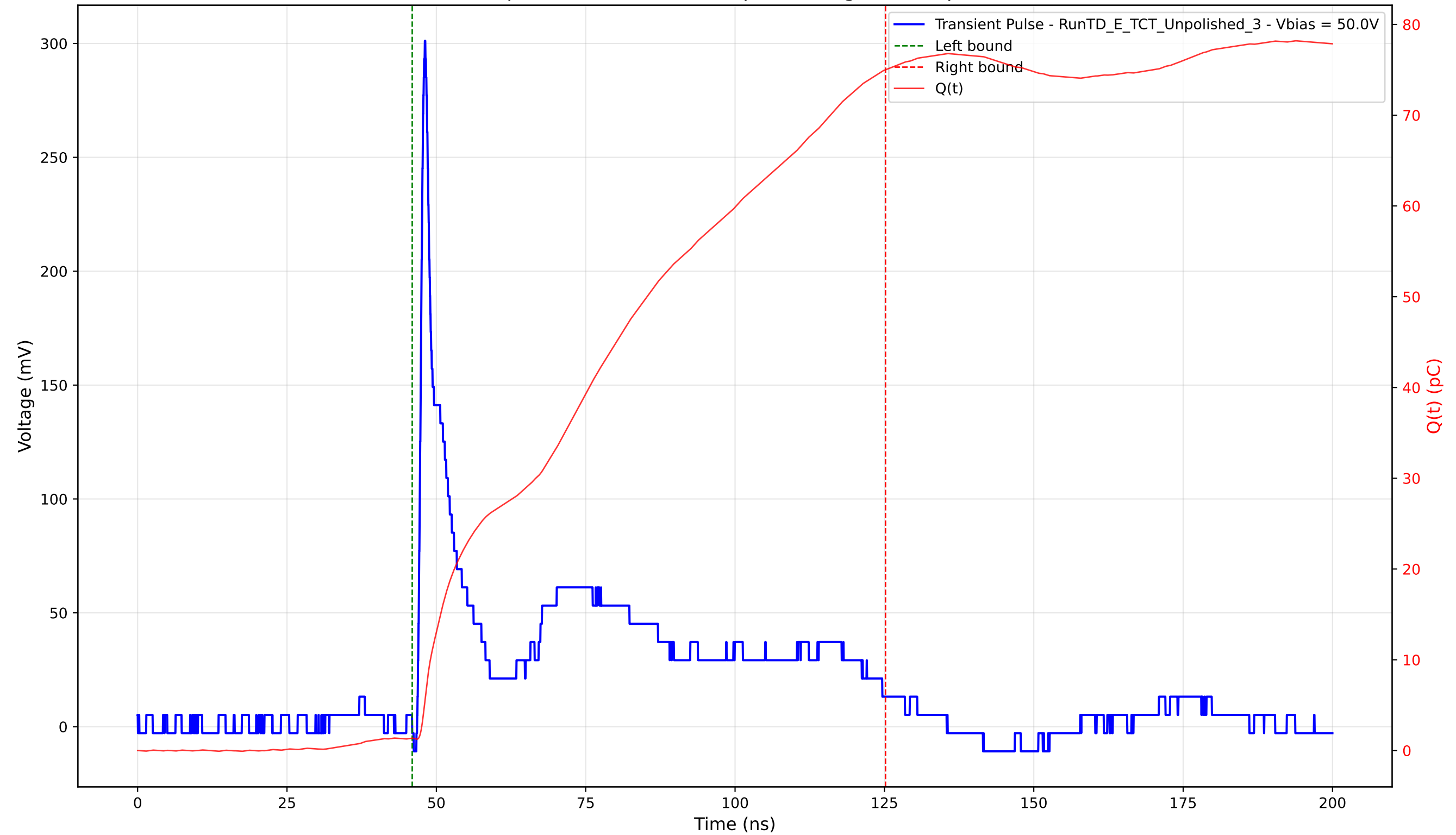
Transient Pulse - Sample: TD - Position: 45.0 \mu\text{m} - Charge: 73.63 pC - Rise Time: 0.86 ns
