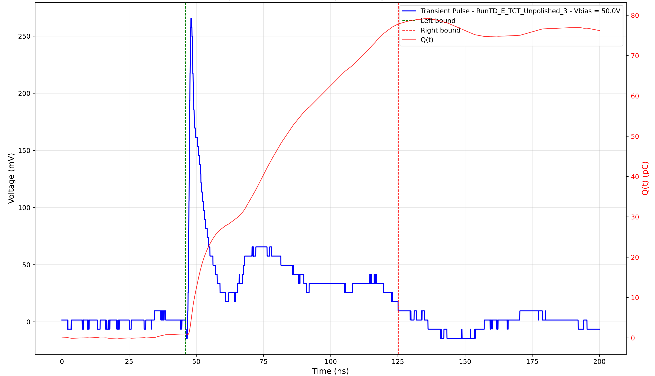
Transient Pulse - Sample: TD - Position: 75.0 \mu\text{m} - Charge: 76.89 pC - Rise Time: 0.82 ns
