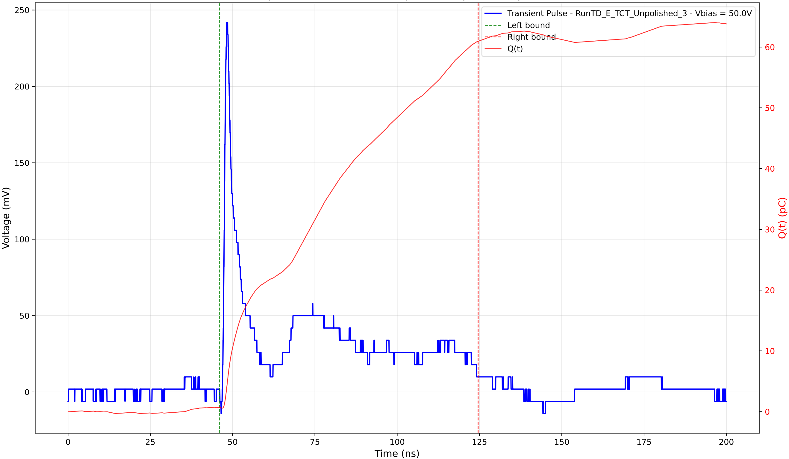
Transient Pulse - Sample: TD - Position: 115.0 \mu\text{m} - Charge: 60.26 pC - Rise Time: 0.90 ns
