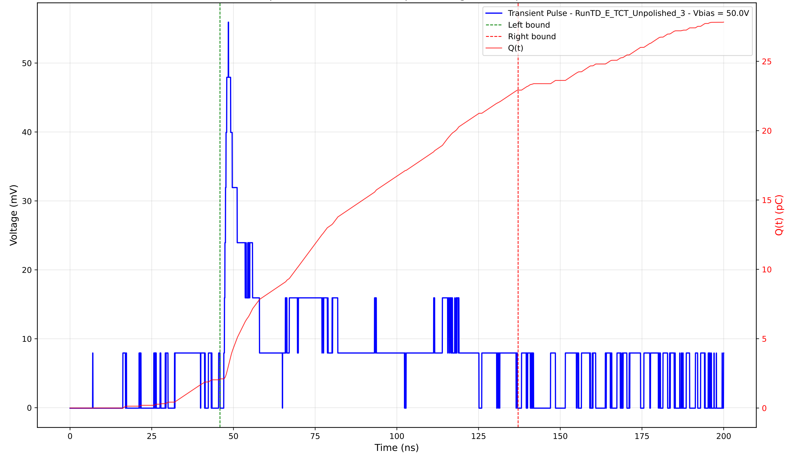
Transient Pulse - Sample: TD - Position: 240.0 \mu\text{m} - Charge: 20.82 pC - Rise Time: 1.39 ns
