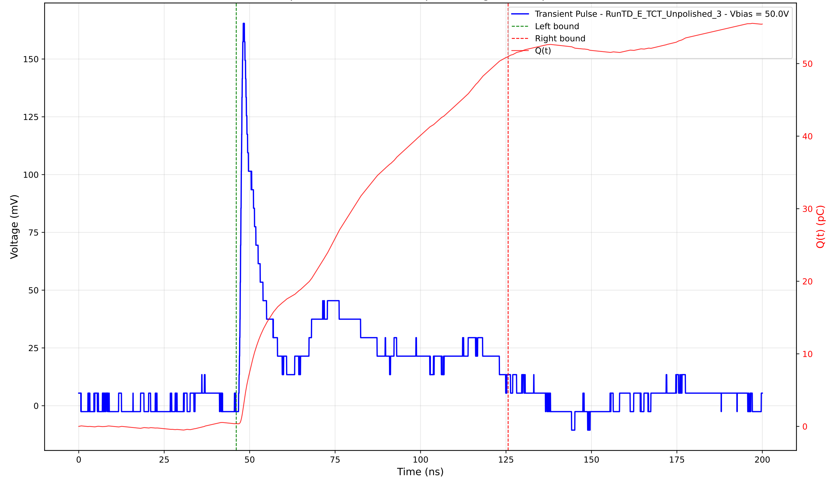
Transient Pulse - Sample: TD - Position: 85.0 \mu\text{m} - Charge: 50.59 pC - Rise Time: 0.91 ns
