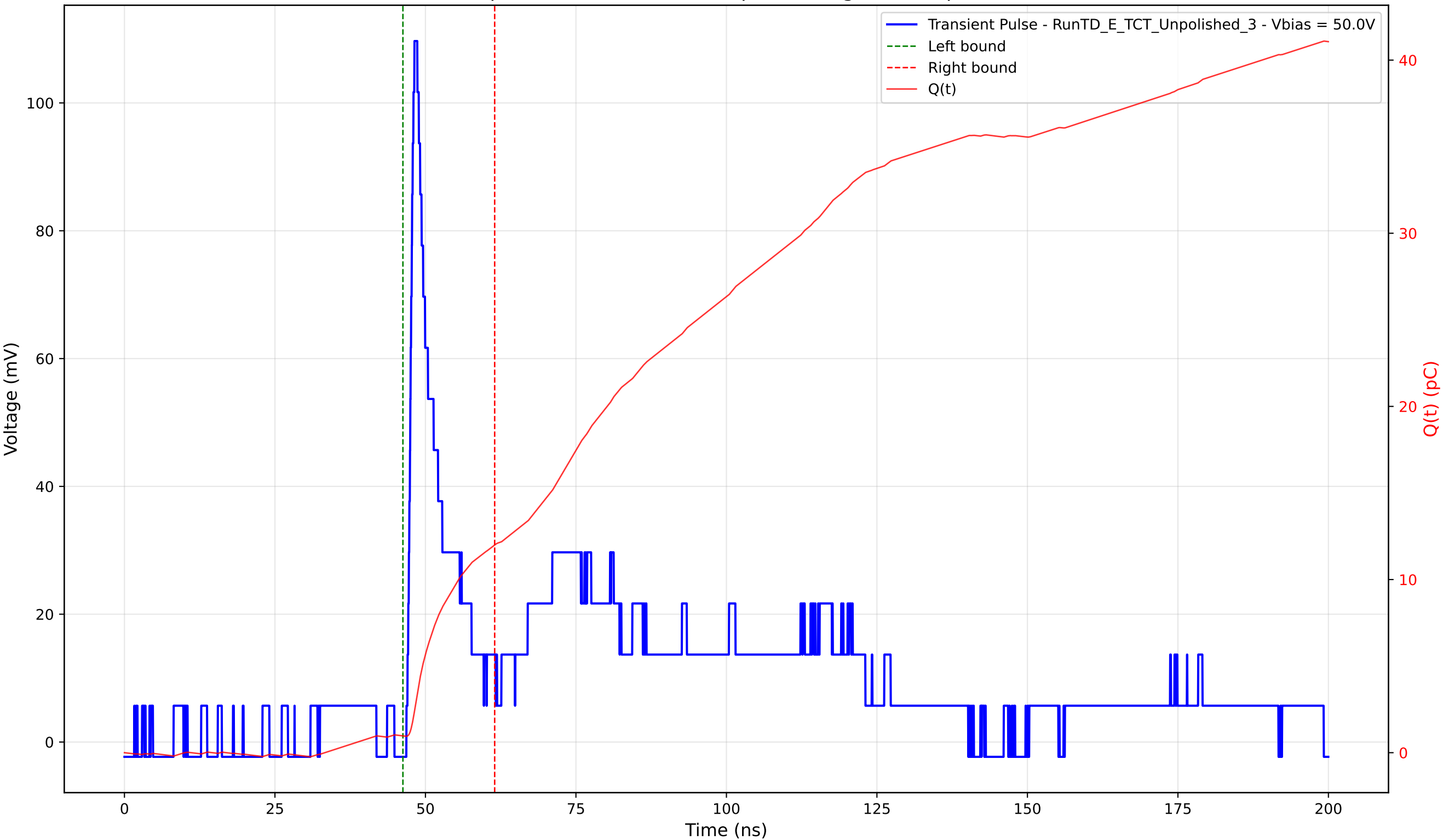
Transient Pulse - Sample: TD - Position: 205.0 \mu\text{m} - Charge: 11.04 pC - Rise Time: 0.99 ns
