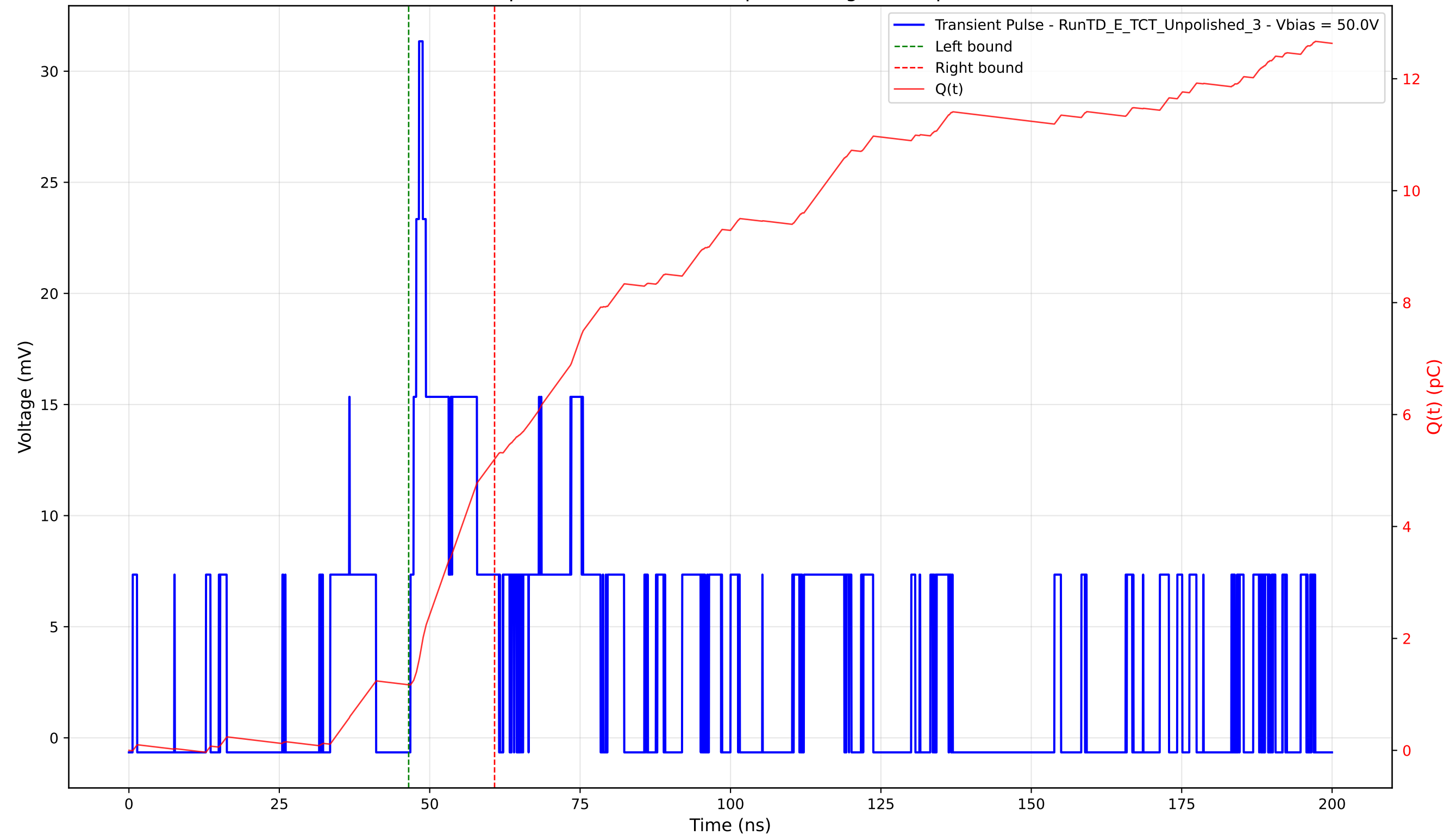
Transient Pulse - Sample: TD - Position: 25.0 \mu\text{m} - Charge: 4.04 pC - Rise Time: 1.43 ns
