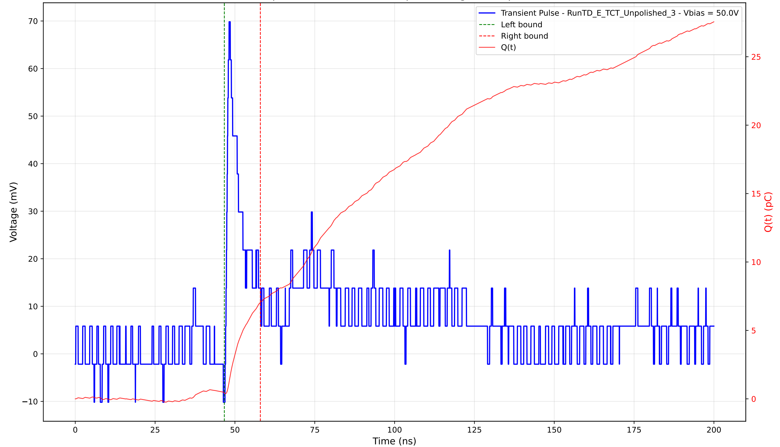
Transient Pulse - Sample: TD - Position: 190.0 \mu\text{m} - Charge: 6.63 pC - Rise Time: 0.96 ns
