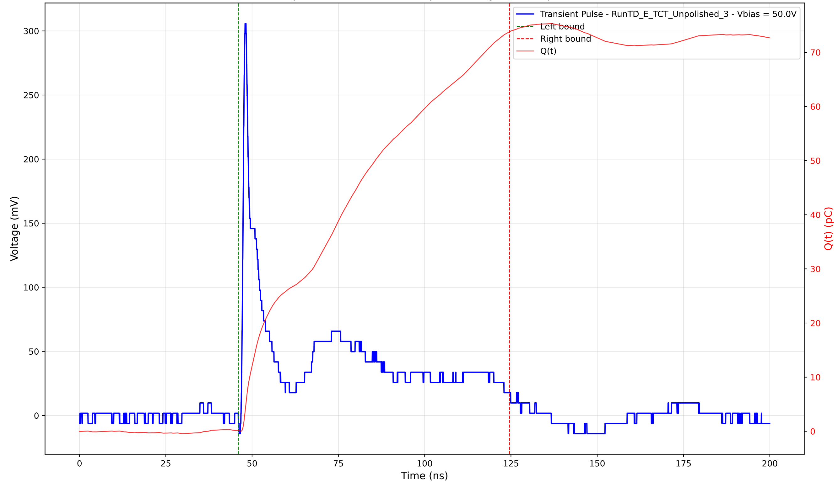
Transient Pulse - Sample: TD - Position: 50.0 \mu\text{m} - Charge: 73.63 pC - Rise Time: 0.83 ns
