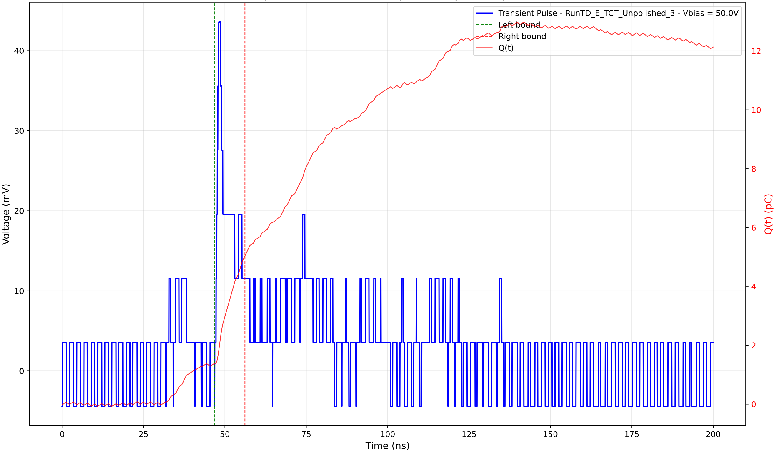
Transient Pulse - Sample: TD - Position: 245.0 \mu\text{m} - Charge: 3.67 pC - Rise Time: 0.86 ns
