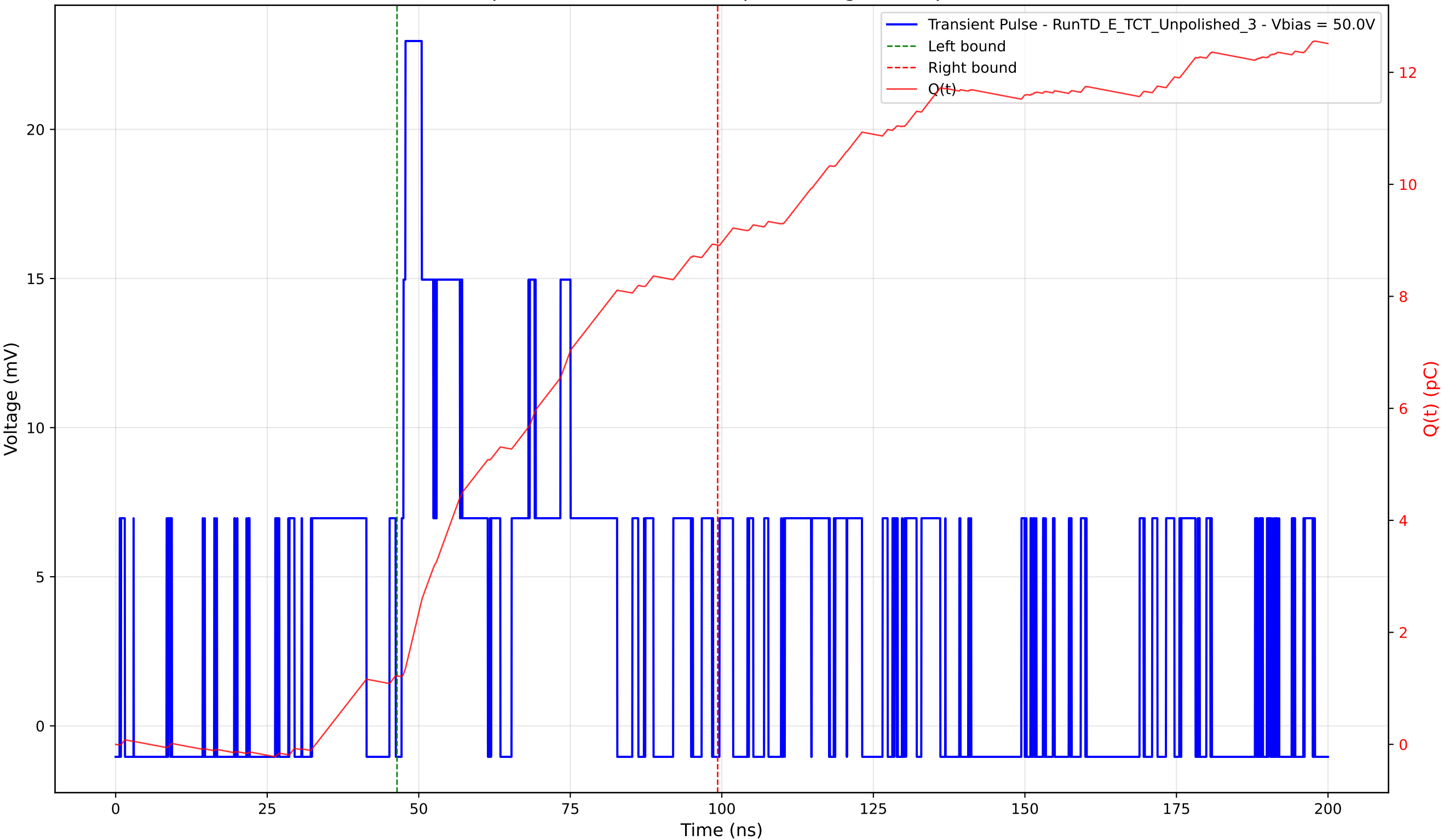
Transient Pulse - Sample: TD - Position: 290.0 \mu\text{m} - Charge: 7.69 pC - Rise Time: 0.64 ns
