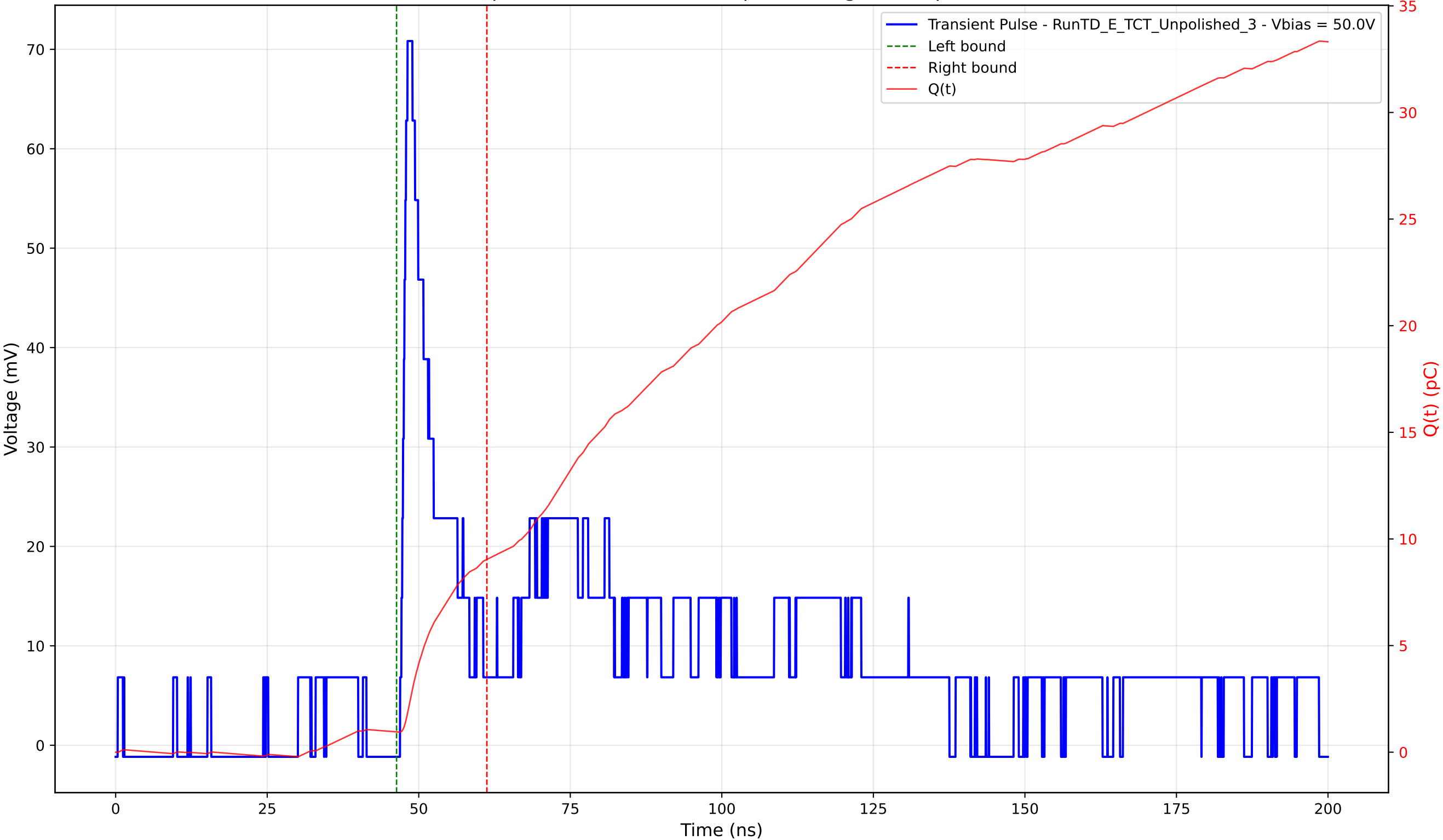
Transient Pulse - Sample: TD - Position: 180.0 \mu\text{m} - Charge: 8.09 pC - Rise Time: 1.02 ns
