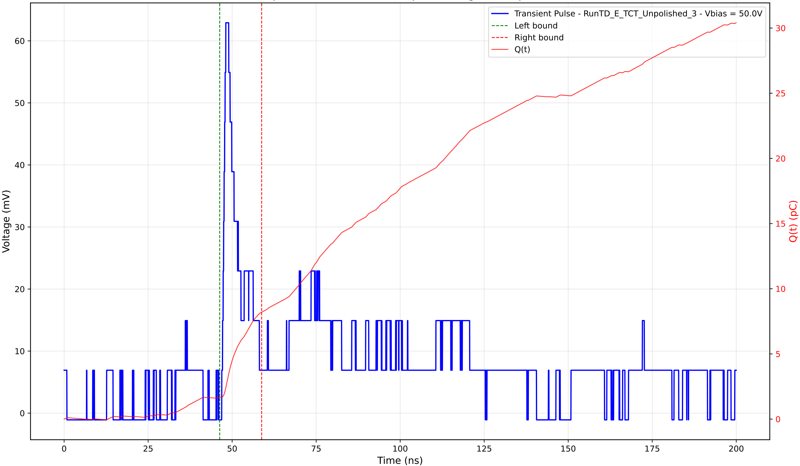
Transient Pulse - Sample: TD - Position: 315.0 \mu\text{m} - Charge: 6.52 pC - Rise Time: 1.20 ns
