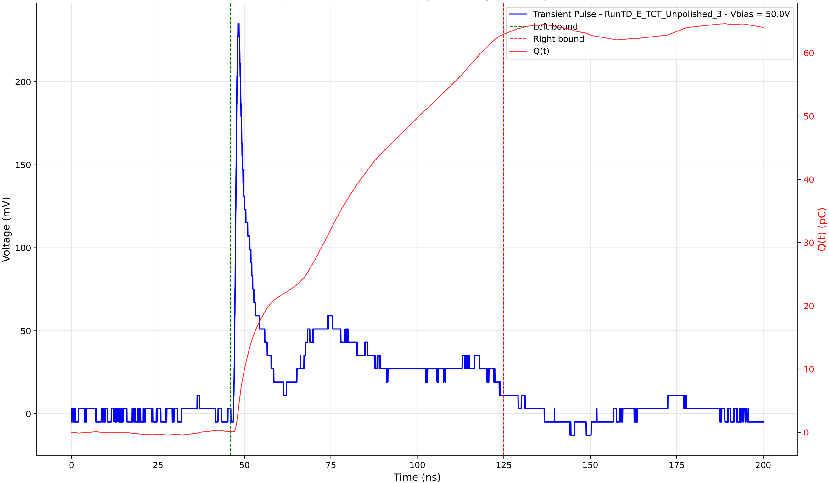
Transient Pulse - Sample: TD - Position: 105.0 \mu\text{m} - Charge: 62.78 pC - Rise Time: 0.93 ns
