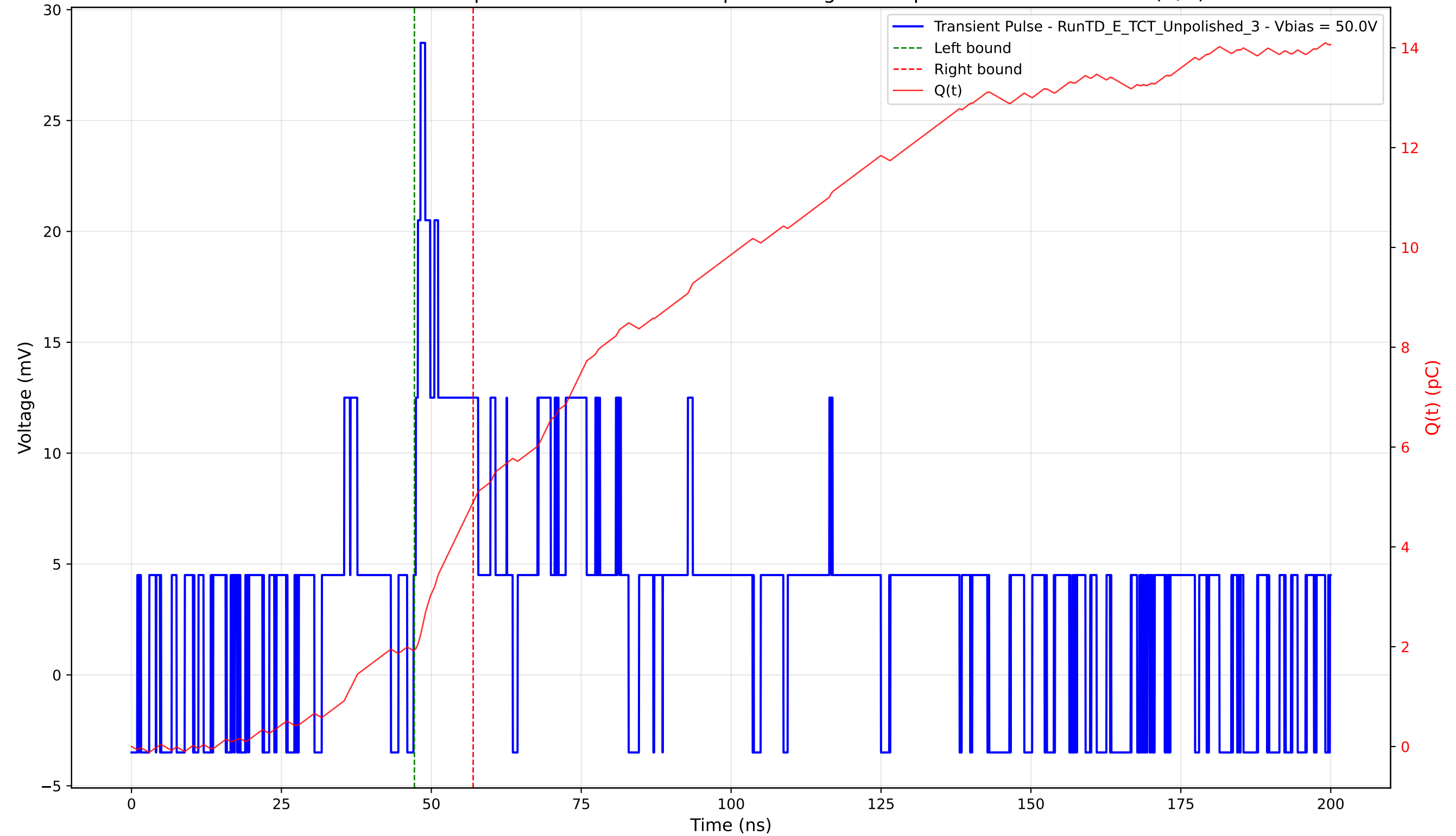
Transient Pulse - Sample: TD - Position: 400.0 \mu\text{m} - Charge: 2.97 pC - Rise Time: 0.00 ns (N/A)
