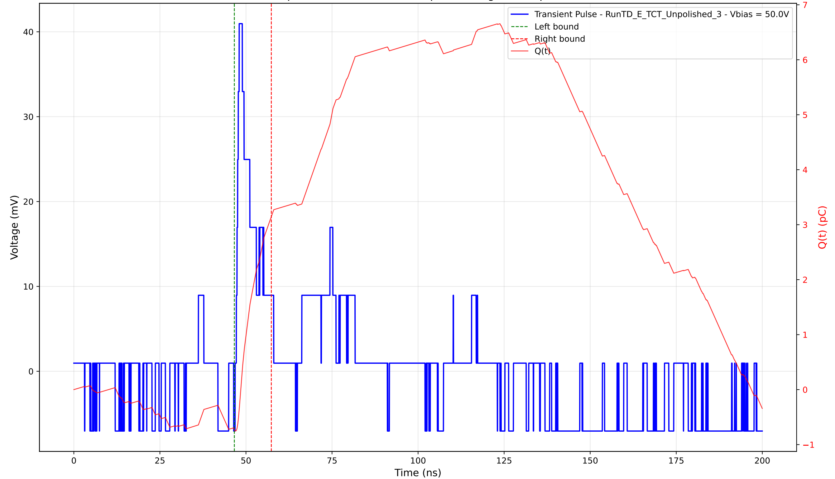
Transient Pulse - Sample: TD - Position: 340.0 \mu\text{m} - Charge: 3.87 pC - Rise Time: 0.83 ns
