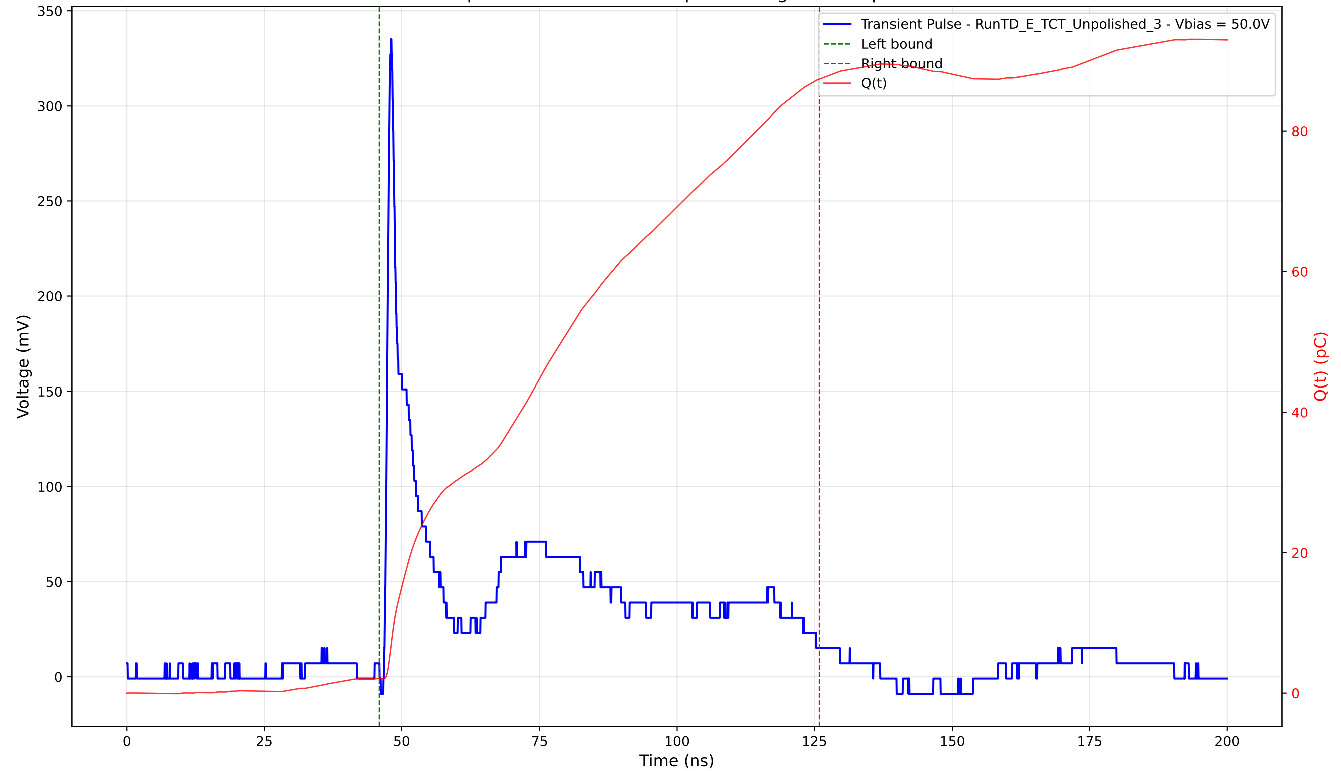
Transient Pulse - Sample: TD - Position: 60.0 \mu\text{m} - Charge: 85.29 pC - Rise Time: 0.83 ns
