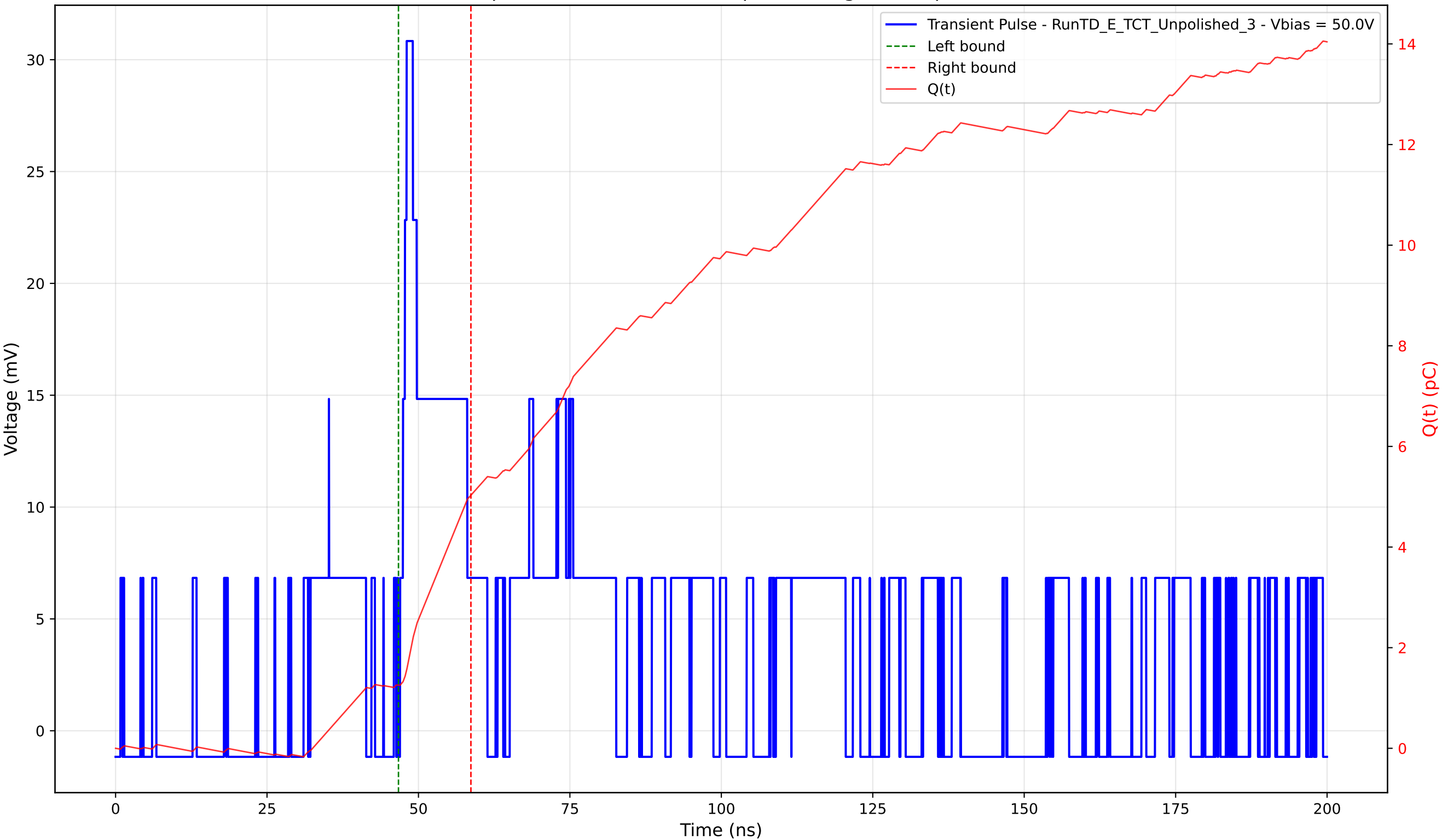
Transient Pulse - Sample: TD - Position: 330.0 \mu\text{m} - Charge: 3.77 pC - Rise Time: 1.09 ns
