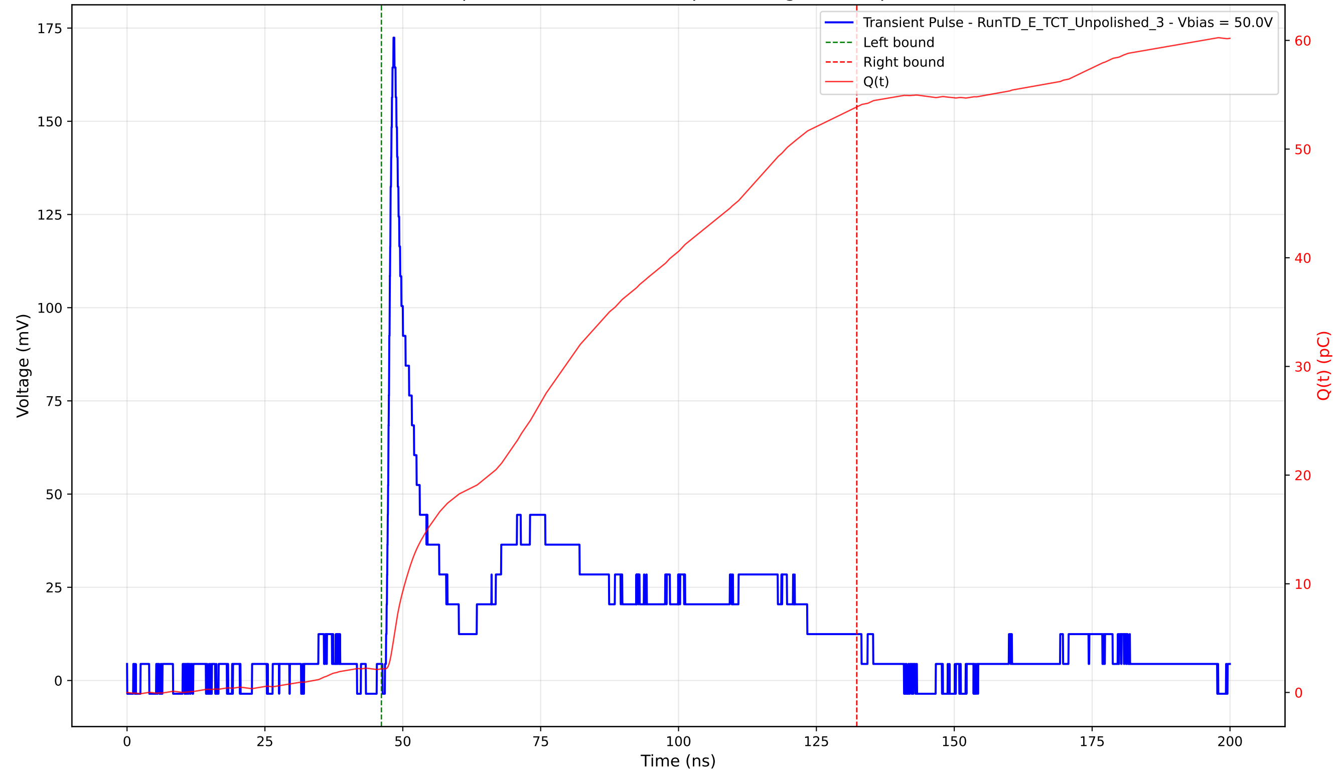
Transient Pulse - Sample: TD - Position: 140.0 \mu\text{m} - Charge: 51.71 pC - Rise Time: 0.97 ns
