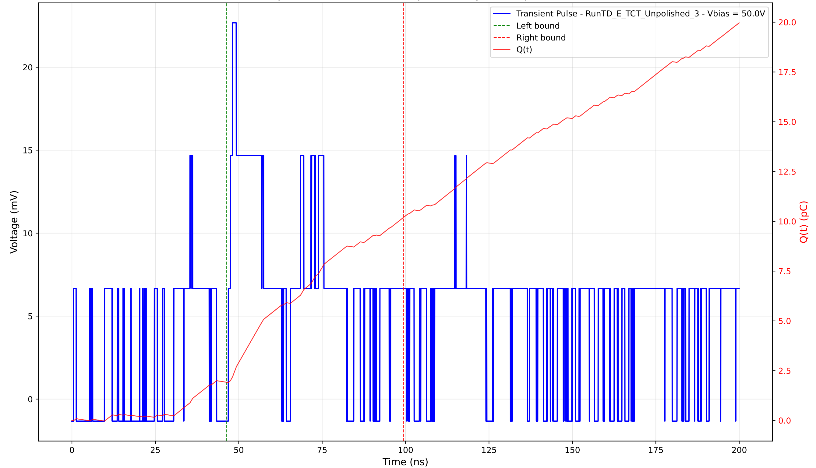
Transient Pulse - Sample: TD - Position: 410.0 \mu\text{m} - Charge: 8.27 pC - Rise Time: 1.26 ns
