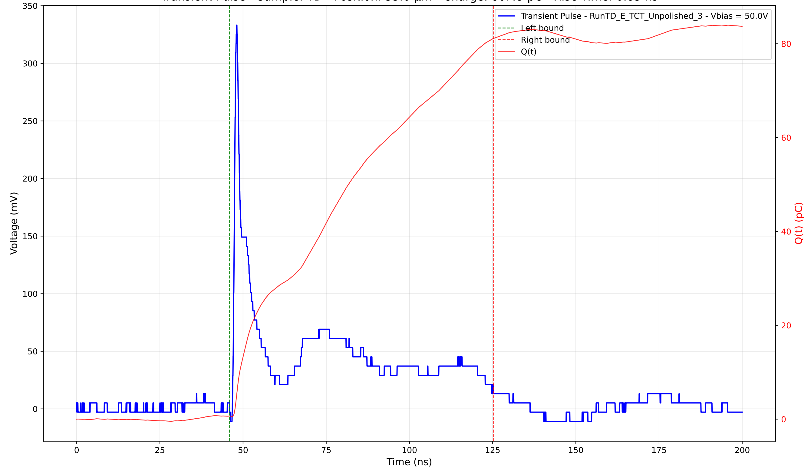
Transient Pulse - Sample: TD - Position: 55.0 \mu\text{m} - Charge: 80.43 pC - Rise Time: 0.83 ns
