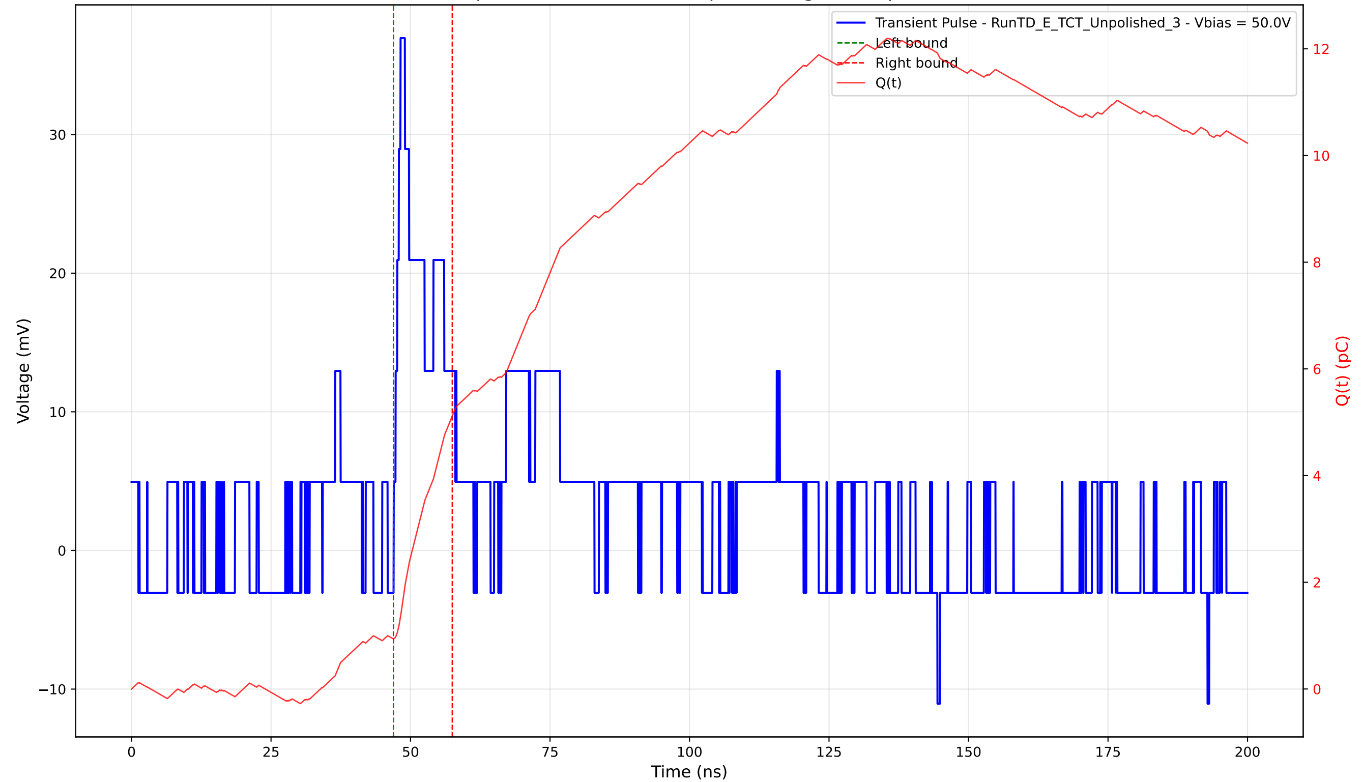
Transient Pulse - Sample: TD - Position: 345.0 \mu\text{m} - Charge: 4.18 pC - Rise Time: 1.23 ns
