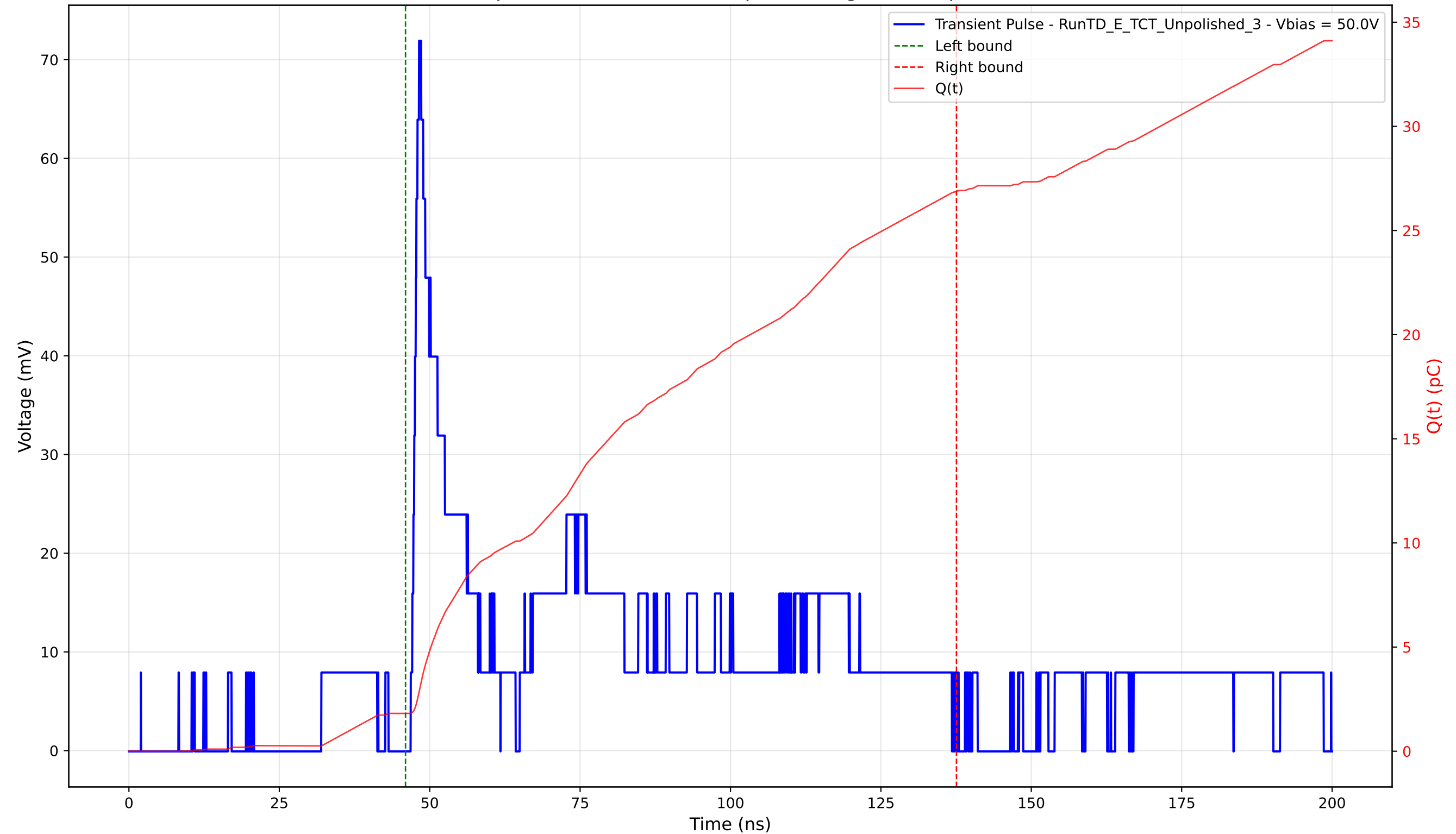
Transient Pulse - Sample: TD - Position: 235.0 \mu\text{m} - Charge: 25.08 pC - Rise Time: 1.38 ns
