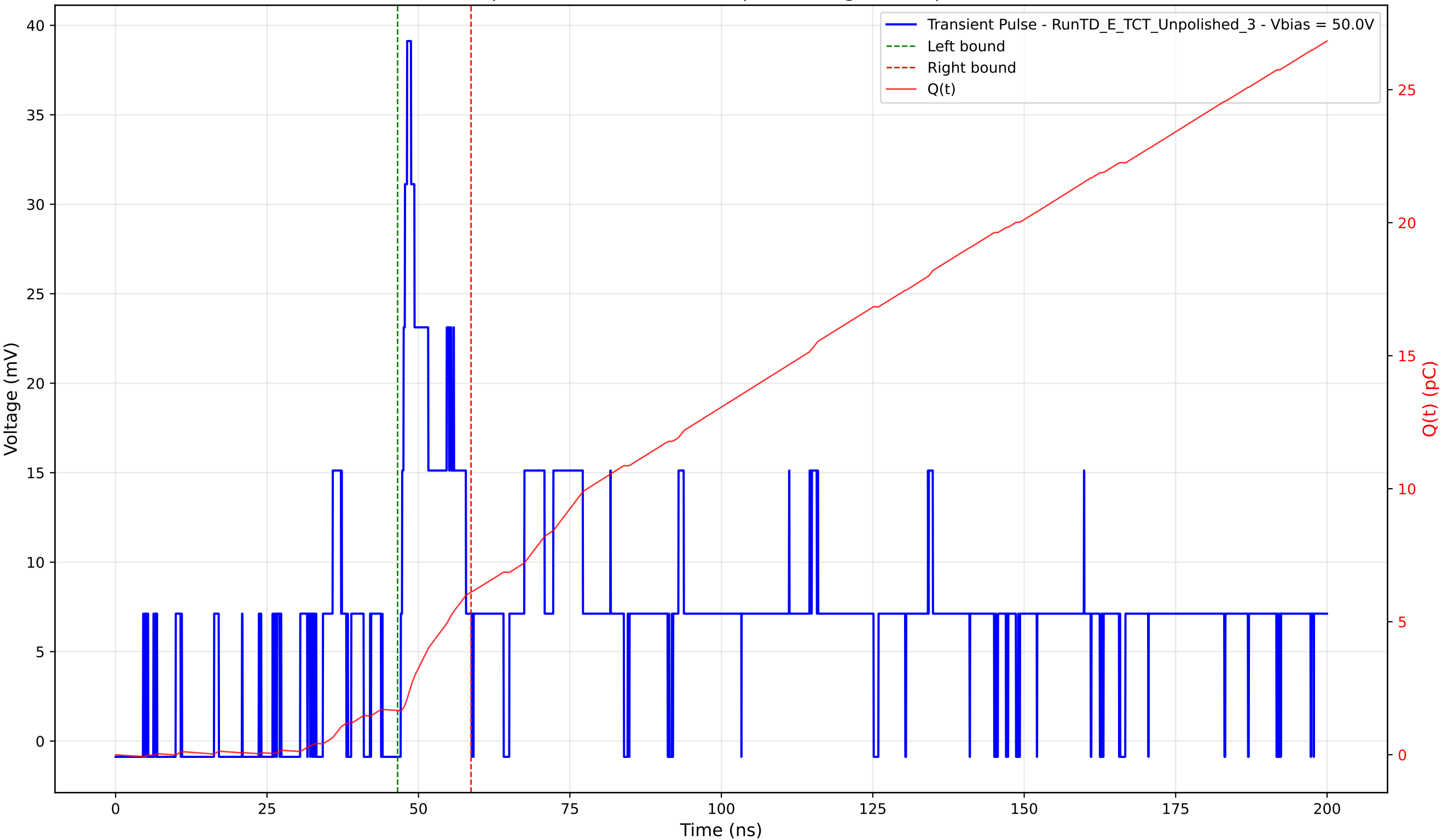
Transient Pulse - Sample: TD - Position: 265.0 \mu\text{m} - Charge: 4.45 pC - Rise Time: 1.05 ns
