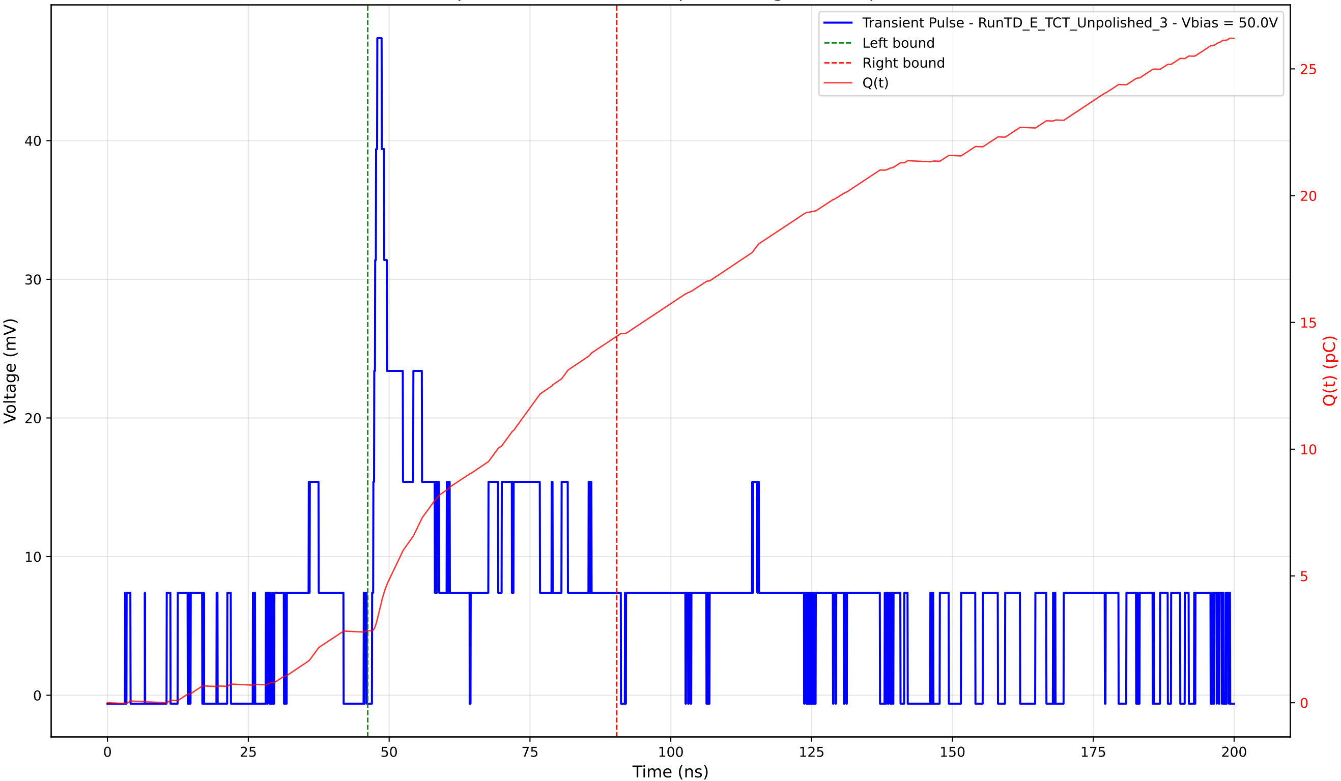
Transient Pulse - Sample: TD - Position: 30.0 \mu\text{m} - Charge: 11.62 pC - Rise Time: 0.93 ns
