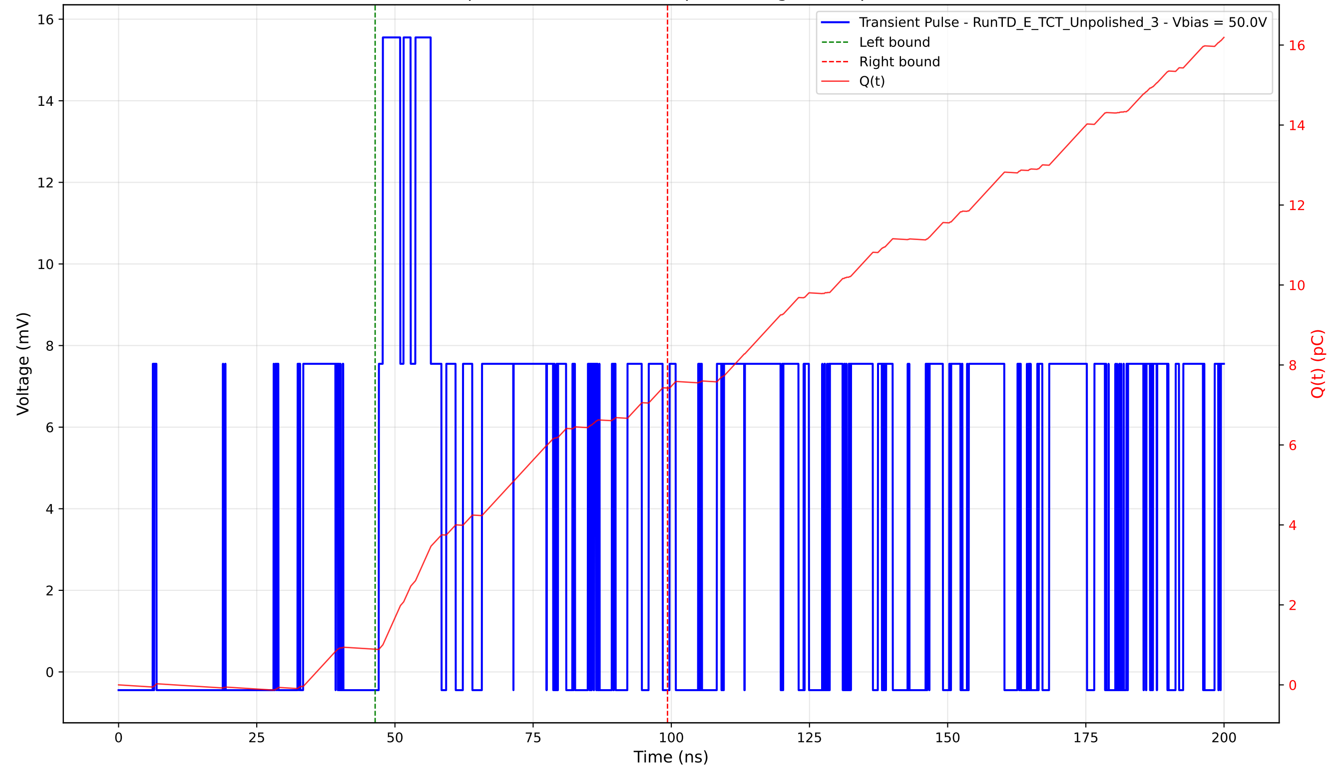
Transient Pulse - Sample: TD - Position: 15.0 \mu\text{m} - Charge: 6.53 pC - Rise Time: 0.74 ns
