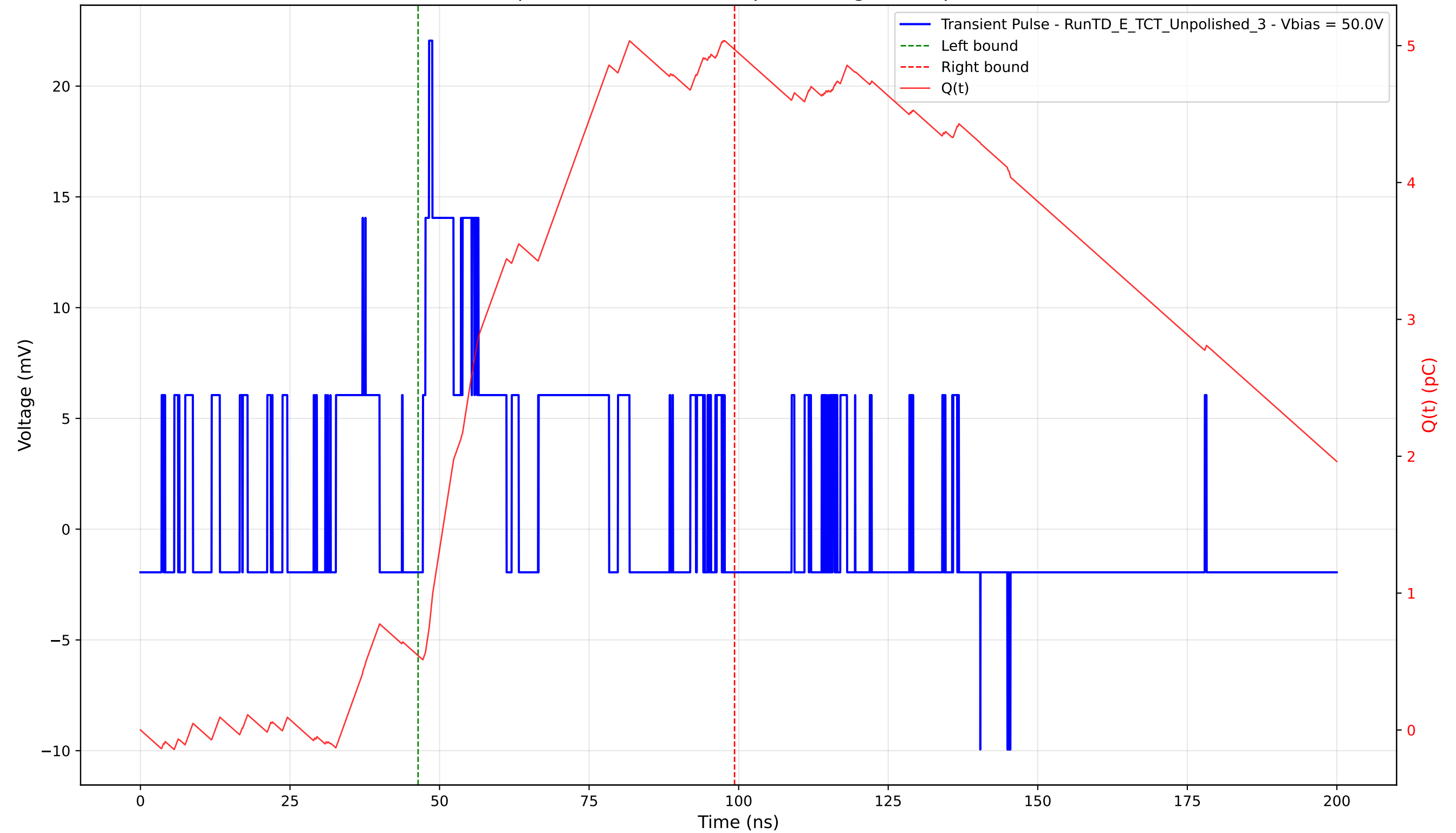
Transient Pulse - Sample: TD - Position: 20.0 \mu\text{m} - Charge: 4.43 pC - Rise Time: 1.04 ns
