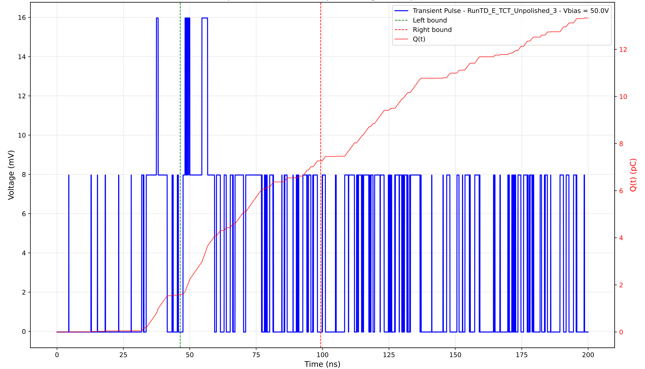
Transient Pulse - Sample: TD - Position: 0.0 \mu\text{m} - Charge: 5.68 pC - Rise Time: 3.86 ns
