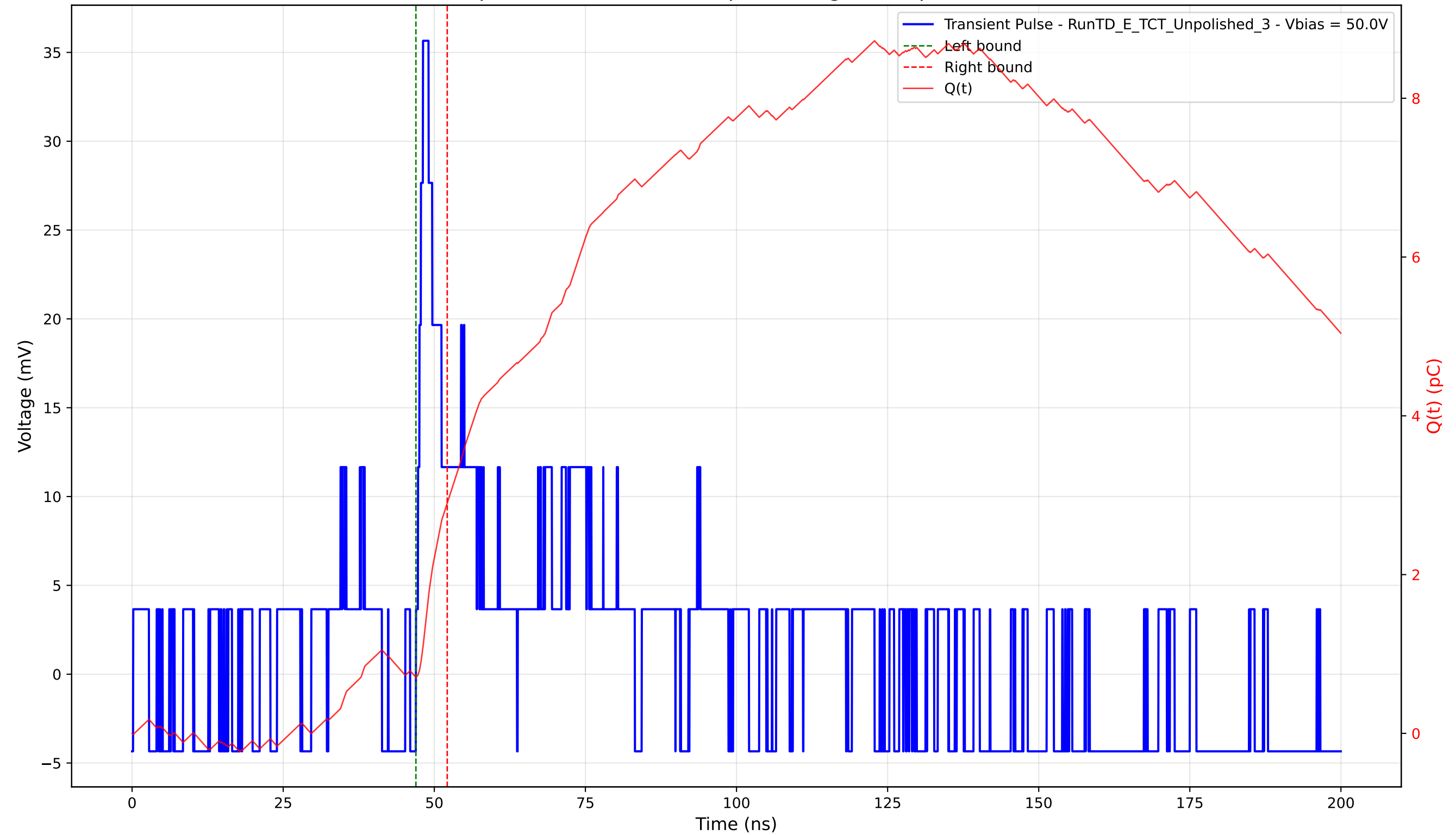
Transient Pulse - Sample: TD - Position: 285.0 \mu\text{m} - Charge: 2.19 pC - Rise Time: 0.00 ns (N/A)
