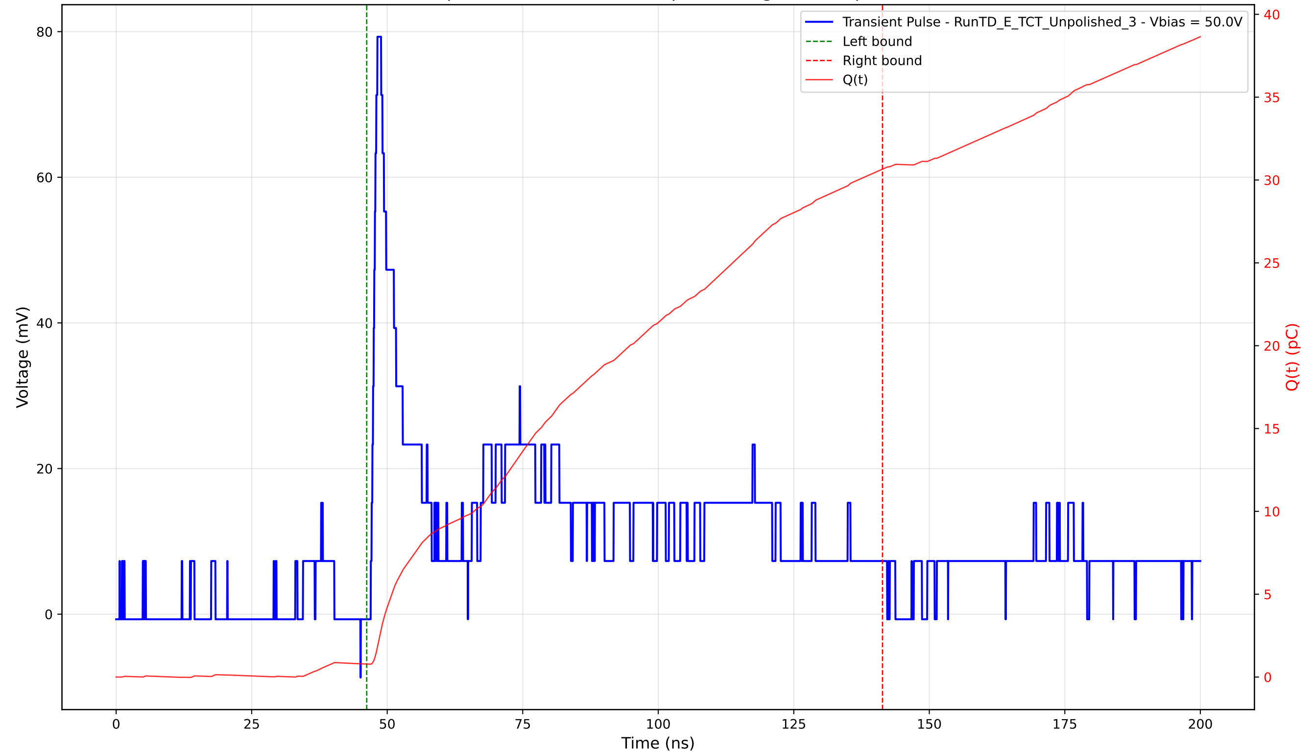
Transient Pulse - Sample: TD - Position: 195.0 \mu\text{m} - Charge: 29.88 pC - Rise Time: 1.08 ns
