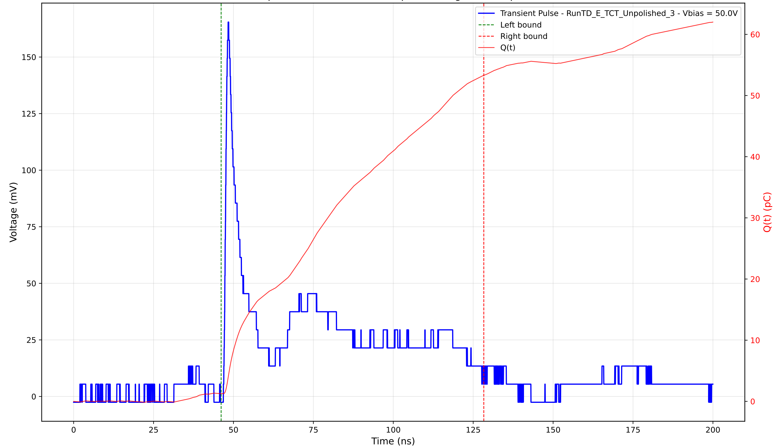
Transient Pulse - Sample: TD - Position: 135.0 \mu\text{m} - Charge: 52.02 pC - Rise Time: 0.97 ns
