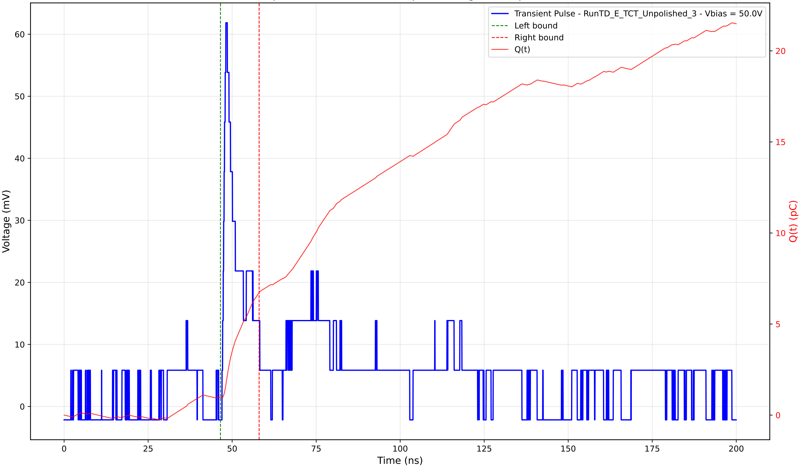
Transient Pulse - Sample: TD - Position: 275.0 \mu\text{m} - Charge: 5.77 pC - Rise Time: 0.98 ns
