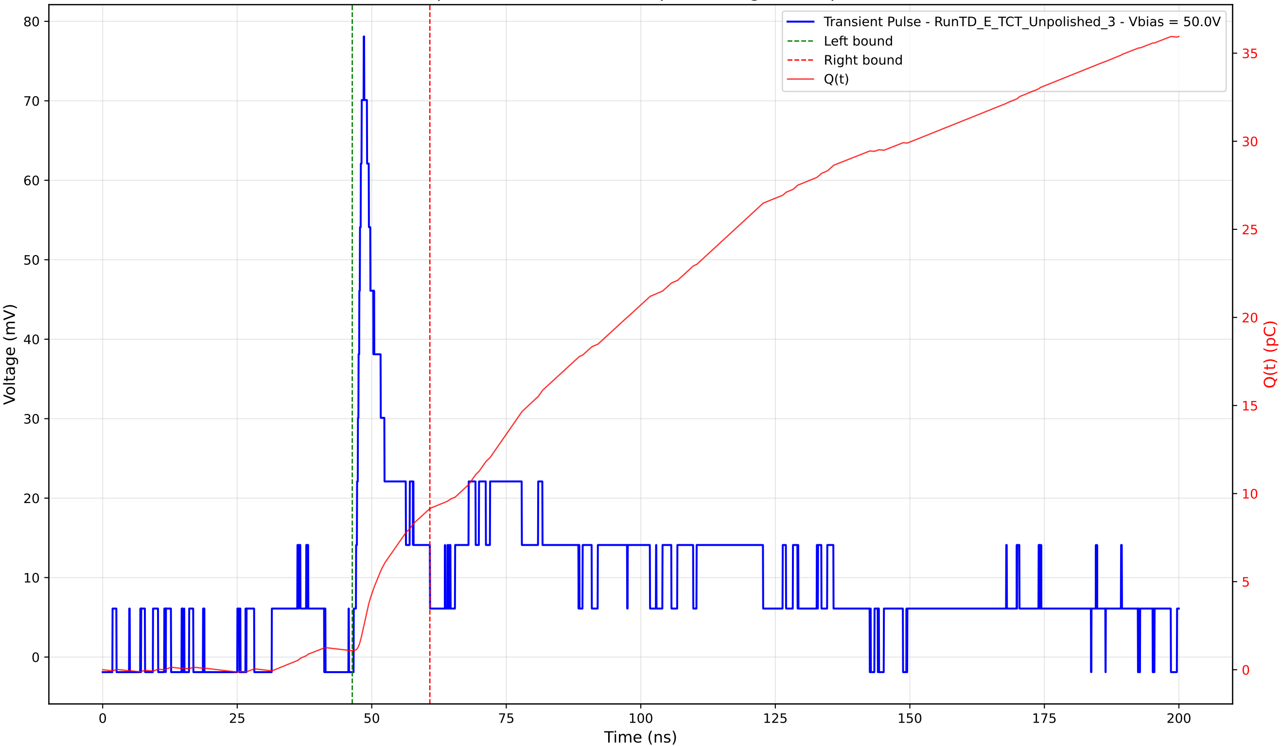
Transient Pulse - Sample: TD - Position: 185.0 \mu\text{m} - Charge: 8.08 pC - Rise Time: 1.44 ns
