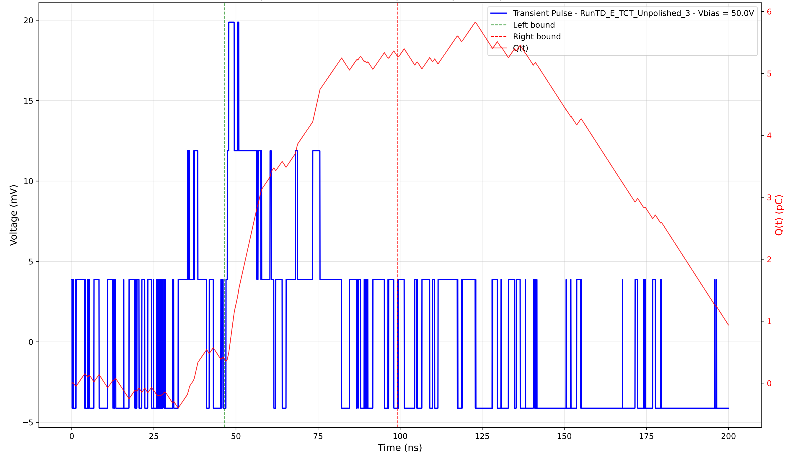
Transient Pulse - Sample: TD - Position: 370.0 \mu\text{m} - Charge: 4.89 pC - Rise Time: 0.00 ns (N/A)
