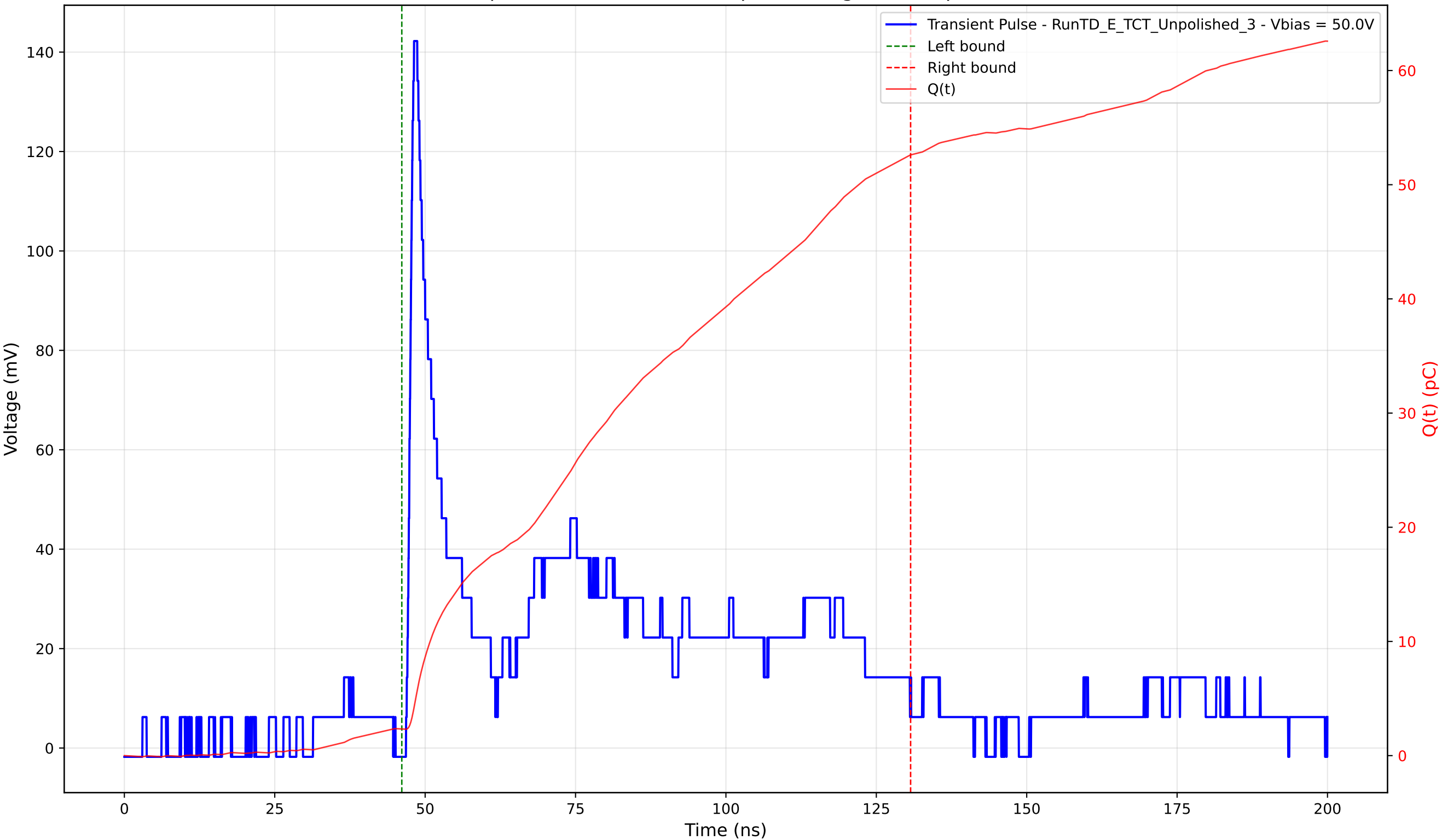
Transient Pulse - Sample: TD - Position: 170.0 \mu\text{m} - Charge: 50.28 pC - Rise Time: 1.08 ns
