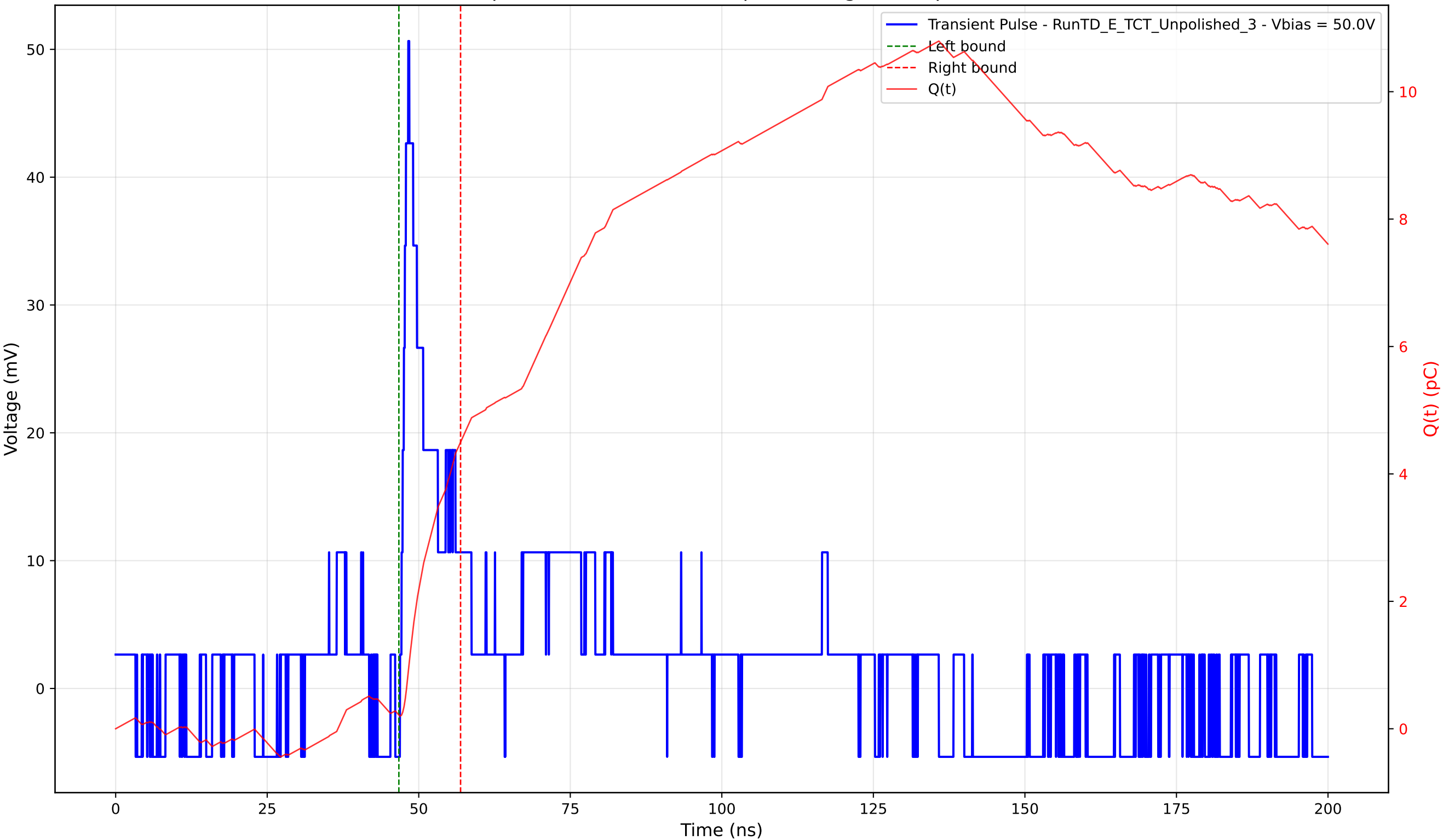
Transient Pulse - Sample: TD - Position: 270.0 \mu\text{m} - Charge: 4.28 pC - Rise Time: 1.11 ns
