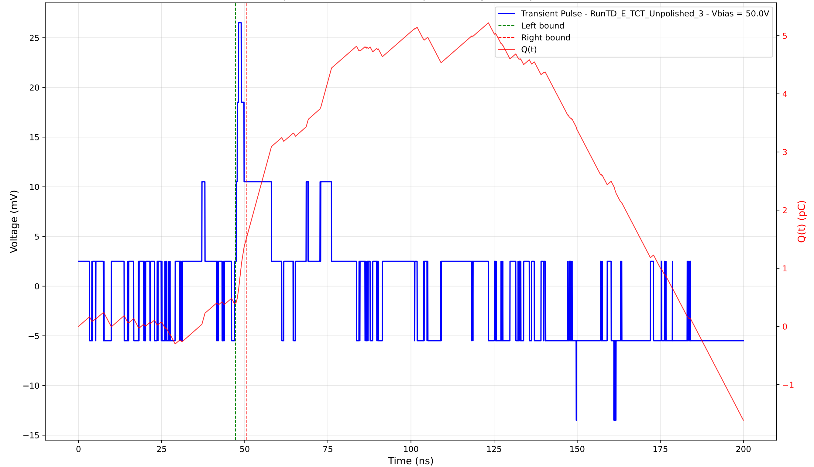
Transient Pulse - Sample: TD - Position: 325.0 \mu\text{m} - Charge: 1.14 pC - Rise Time: 0.70 ns
