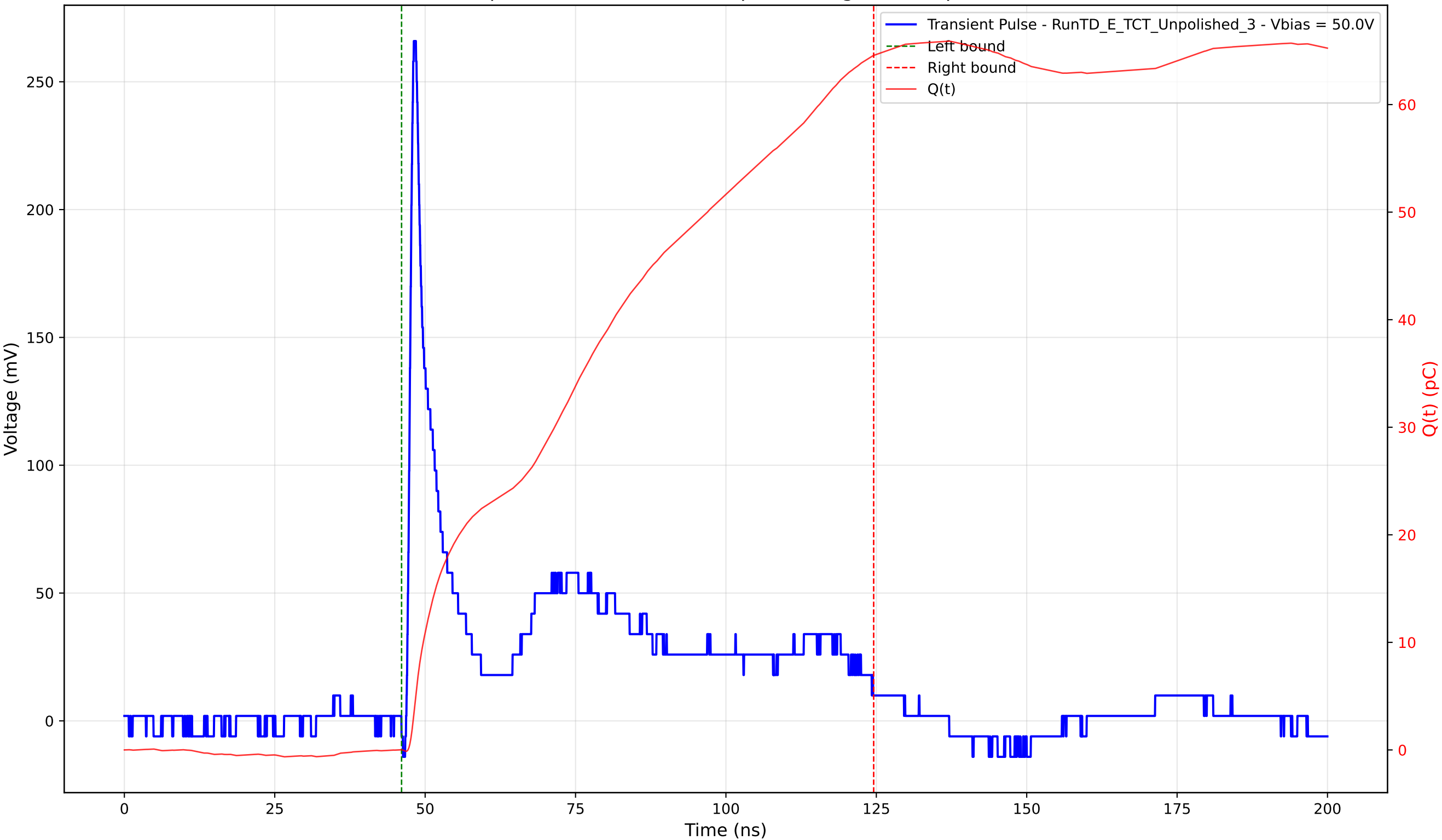
Transient Pulse - Sample: TD - Position: 110.0 \mu\text{m} - Charge: 64.55 pC - Rise Time: 0.88 ns
