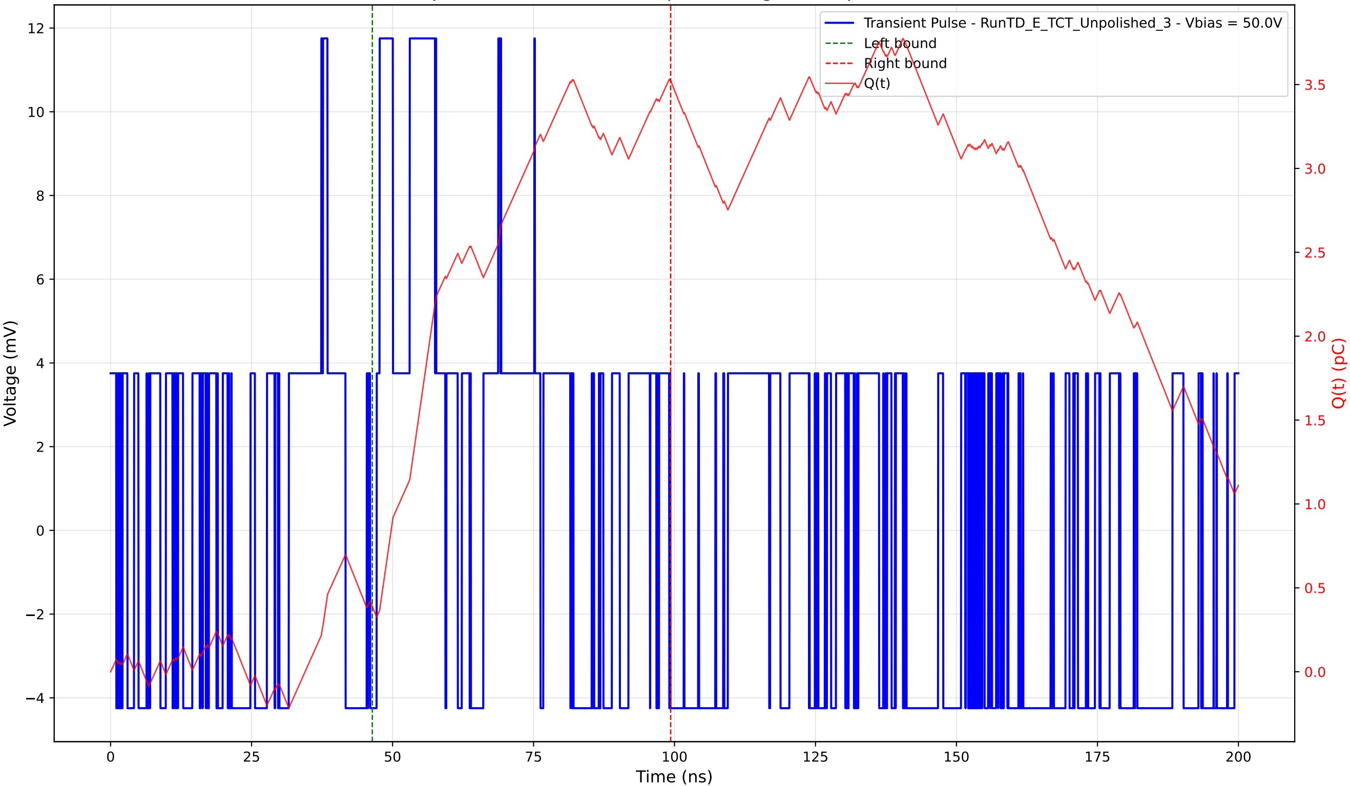
Transient Pulse - Sample: TD - Position: 365.0 \mu\text{m} - Charge: 3.14 pC - Rise Time: 0.00 ns (N/A)
