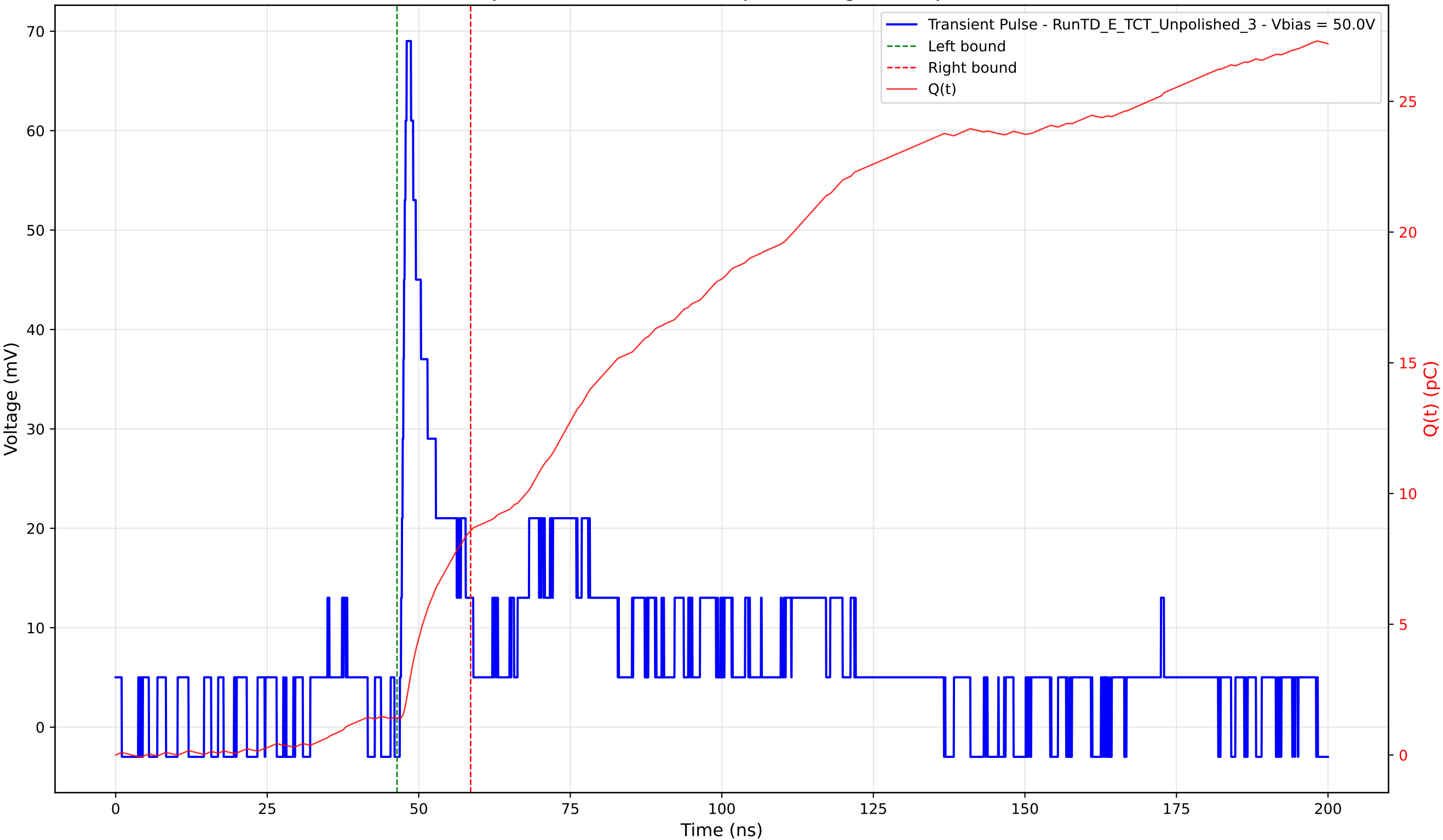
Transient Pulse - Sample: TD - Position: 225.0 \mu\text{m} - Charge: 7.16 pC - Rise Time: 0.94 ns
