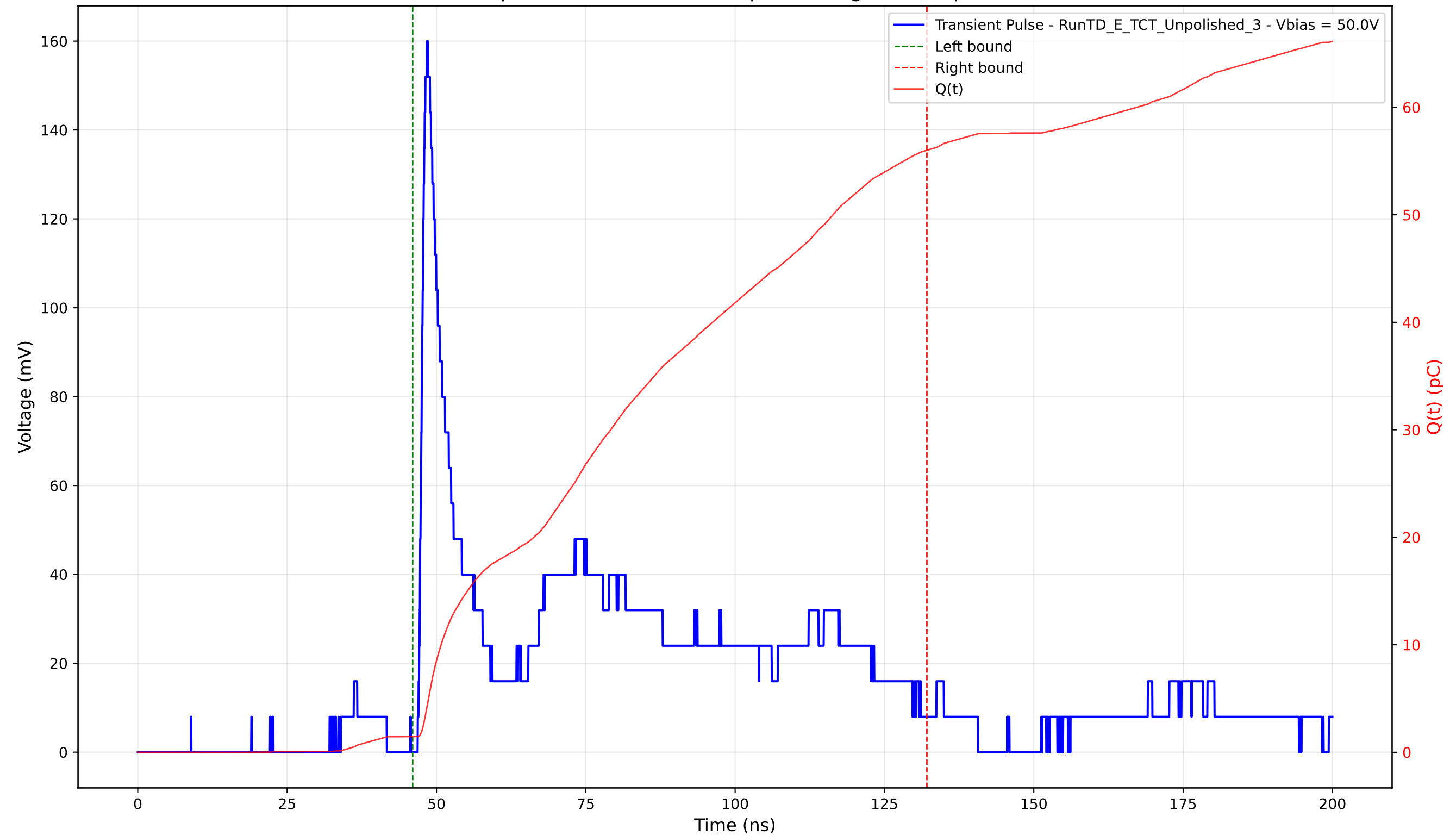
Transient Pulse - Sample: TD - Position: 130.0 \mu\text{m} - Charge: 54.53 pC - Rise Time: 1.06 ns
