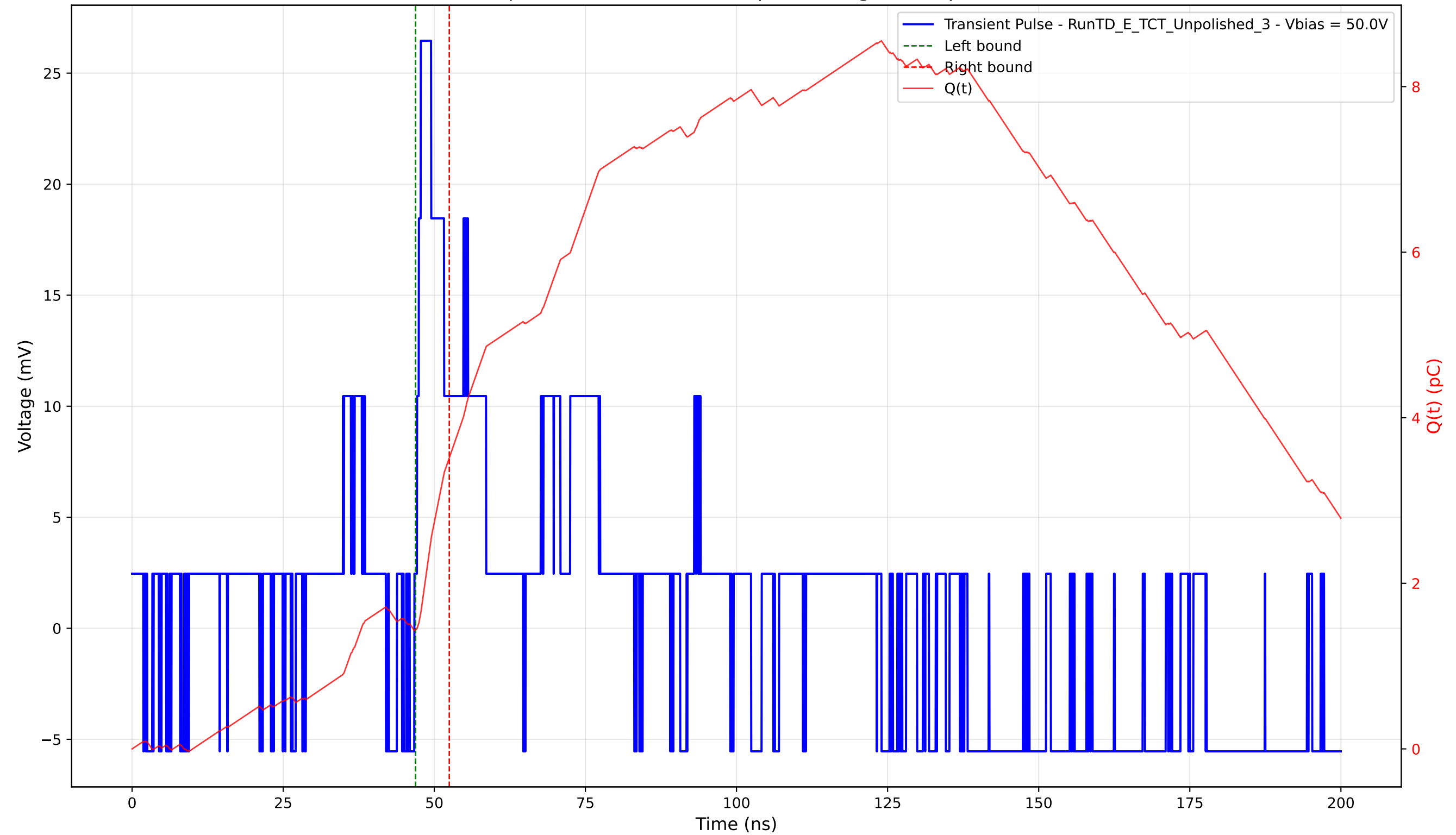
Transient Pulse - Sample: TD - Position: 305.0 \mu\text{m} - Charge: 2.07 pC - Rise Time: 0.64 ns
