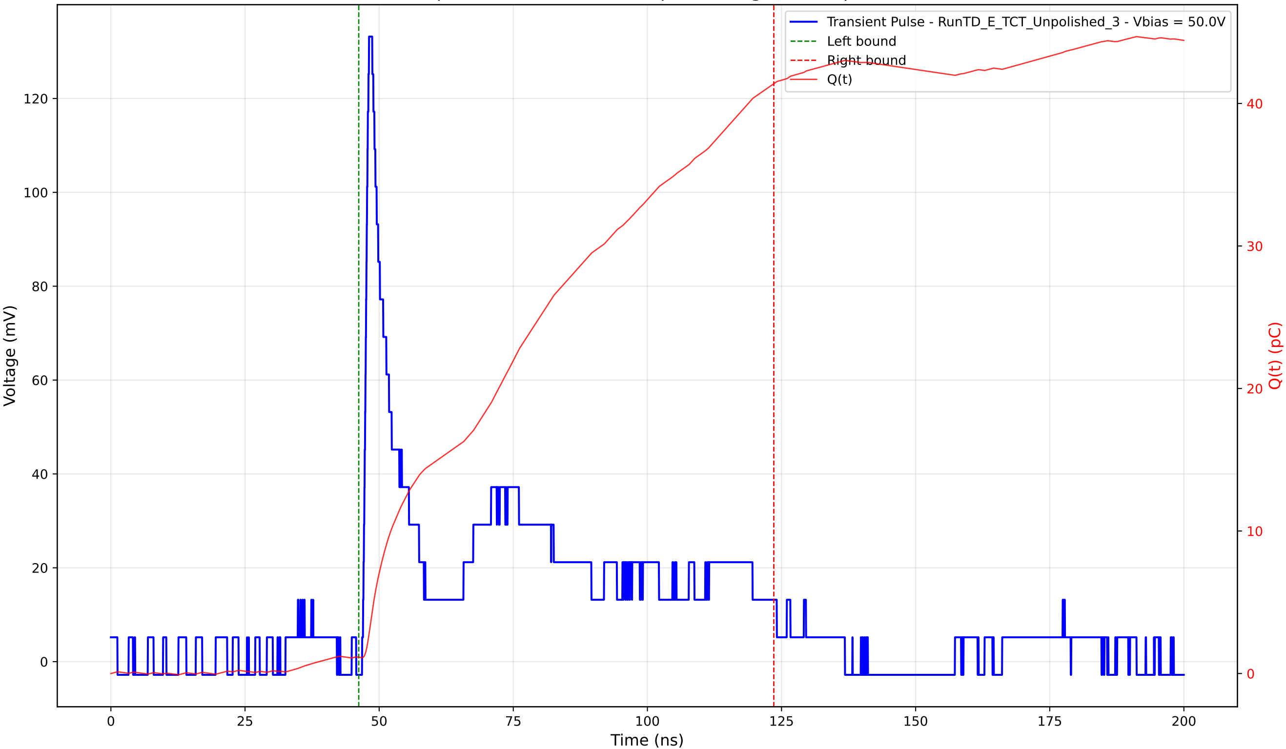
Transient Pulse - Sample: TD - Position: 145.0 \mu\text{m} - Charge: 40.25 pC - Rise Time: 0.94 ns
