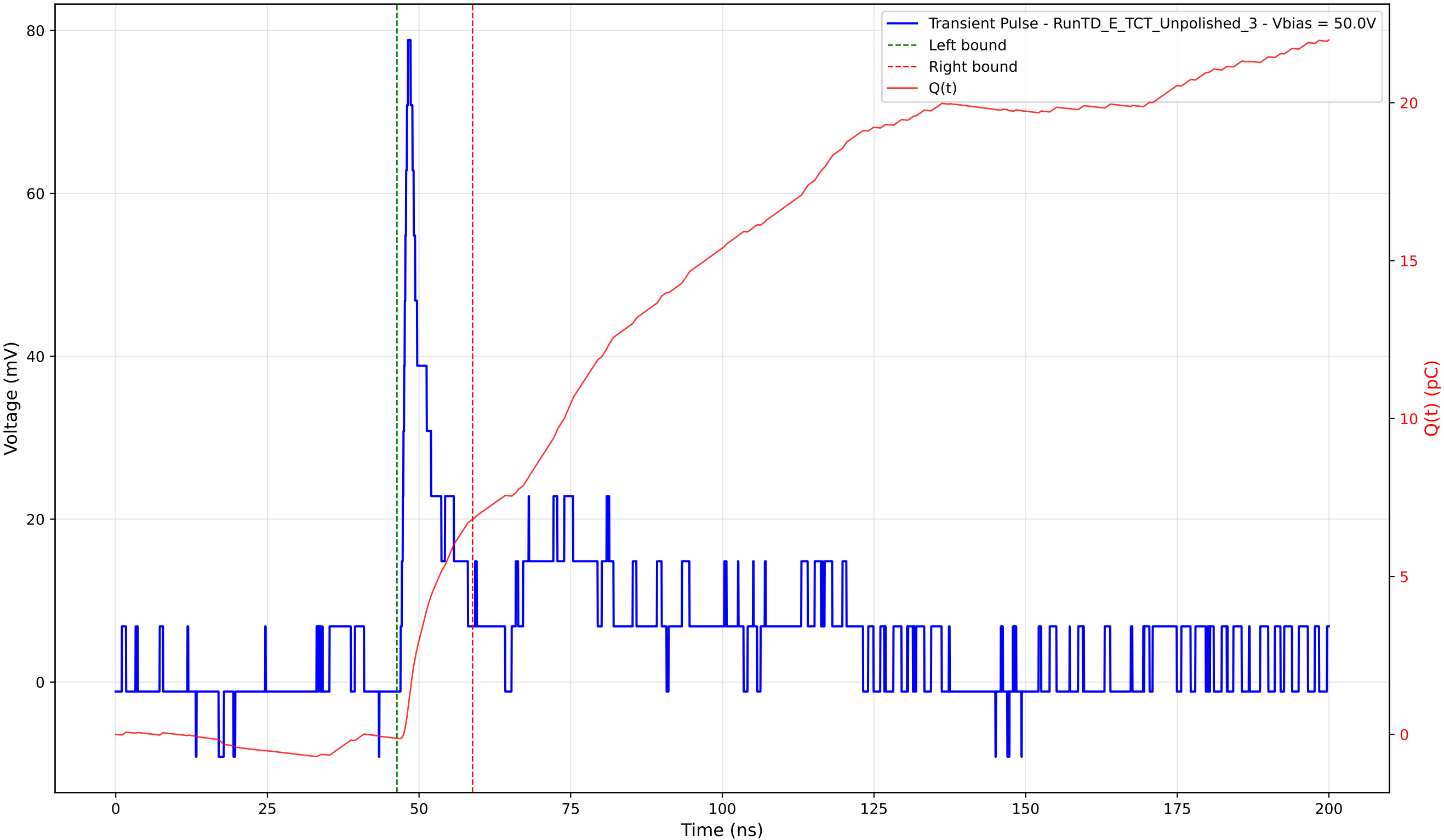
Transient Pulse - Sample: TD - Position: 230.0 \mu\text{m} - Charge: 6.93 pC - Rise Time: 1.04 ns
