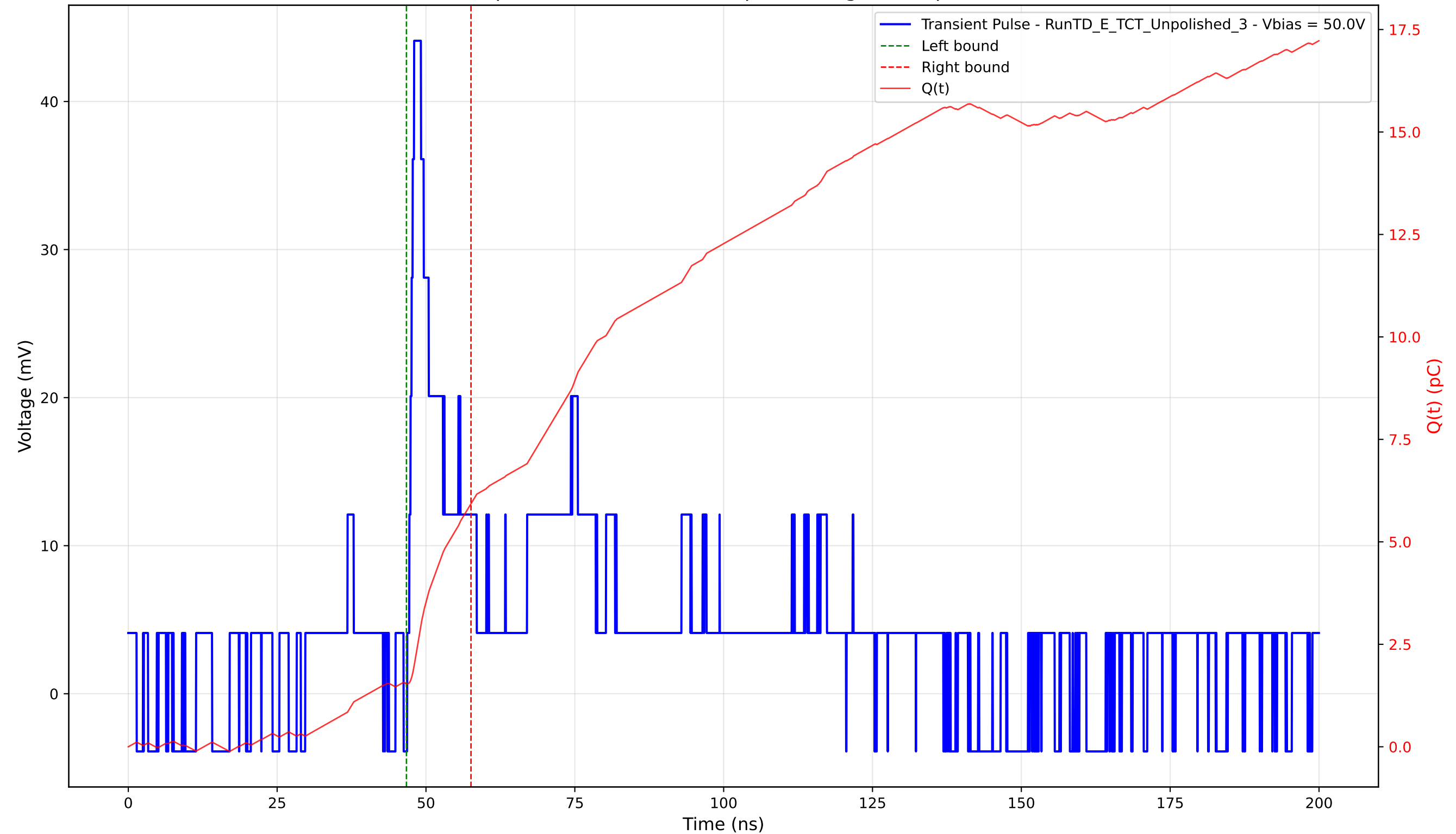
Transient Pulse - Sample: TD - Position: 280.0 \mu\text{m} - Charge: 4.40 pC - Rise Time: 0.82 ns
