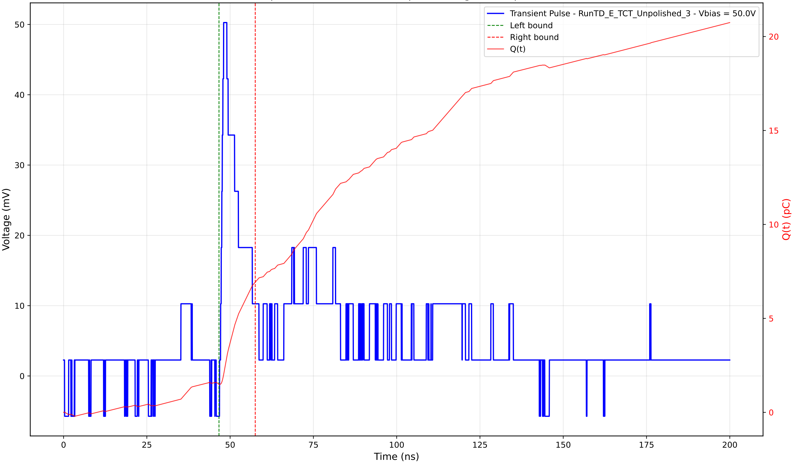
Transient Pulse - Sample: TD - Position: 155.0 \mu\text{m} - Charge: 5.43 pC - Rise Time: 0.91 ns
