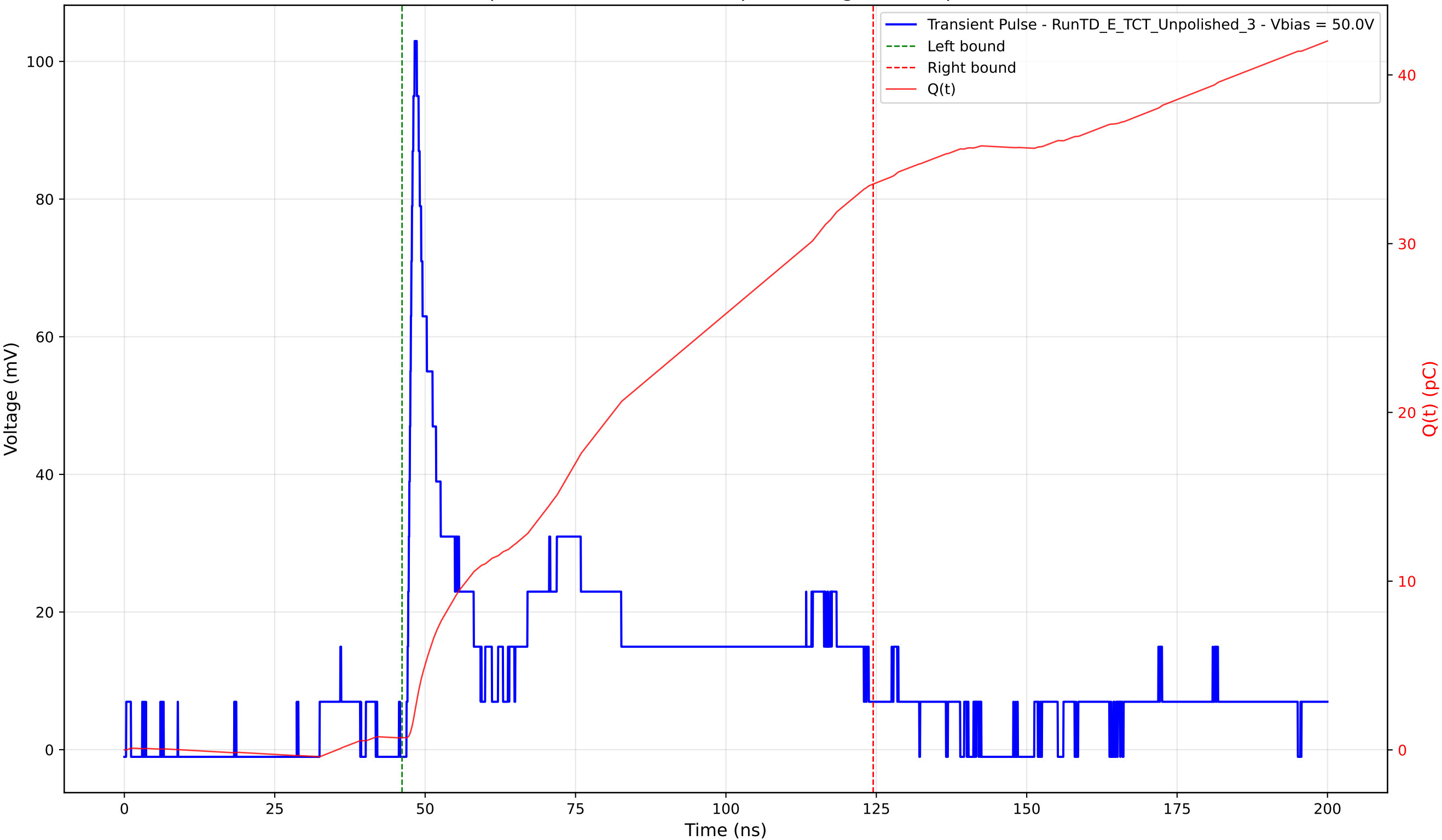
Transient Pulse - Sample: TD - Position: 175.0 \mu\text{m} - Charge: 32.80 pC - Rise Time: 0.97 ns
