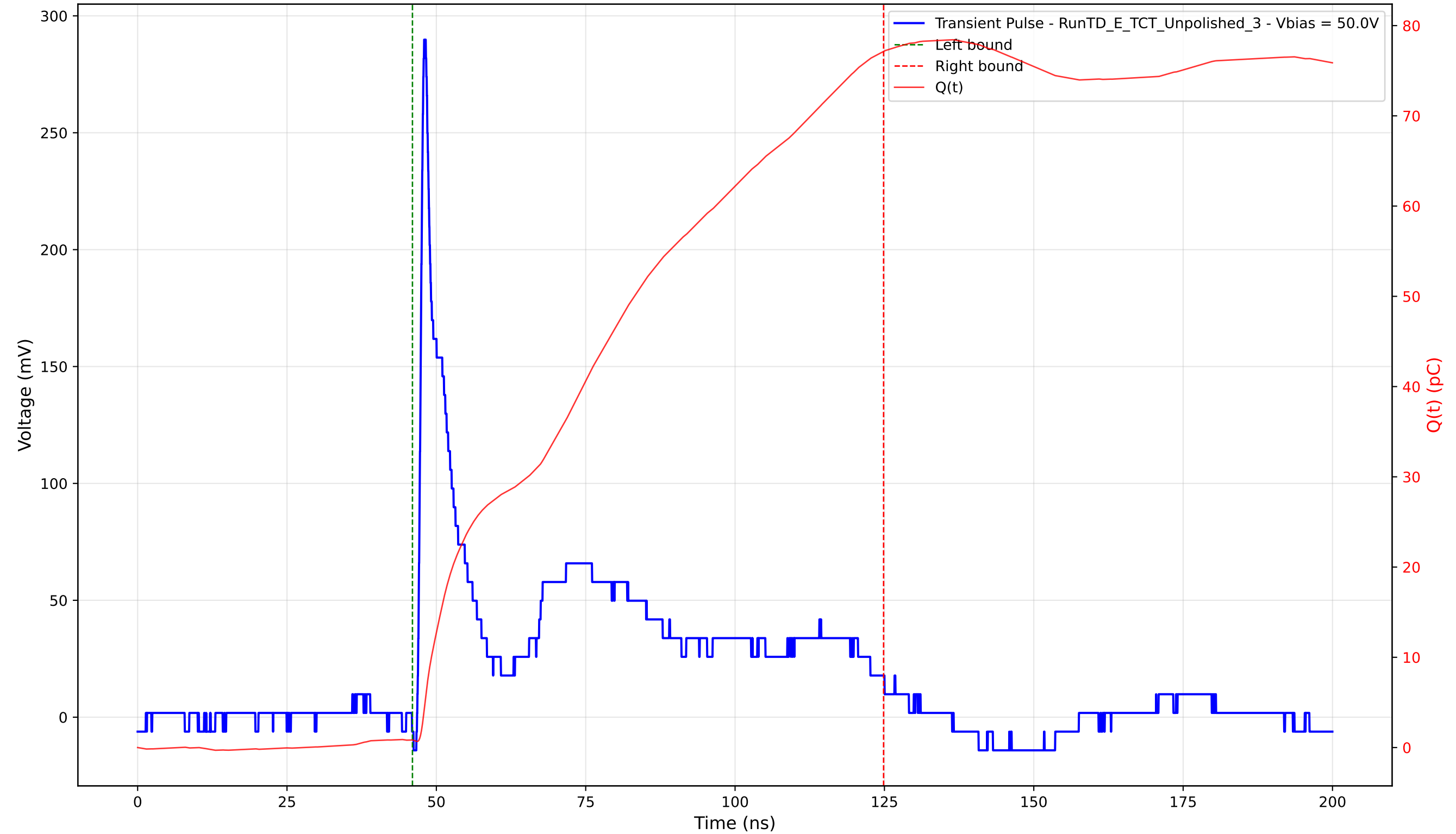
Transient Pulse - Sample: TD - Position: 70.0 \mu\text{m} - Charge: 76.31 pC - Rise Time: 0.81 ns
