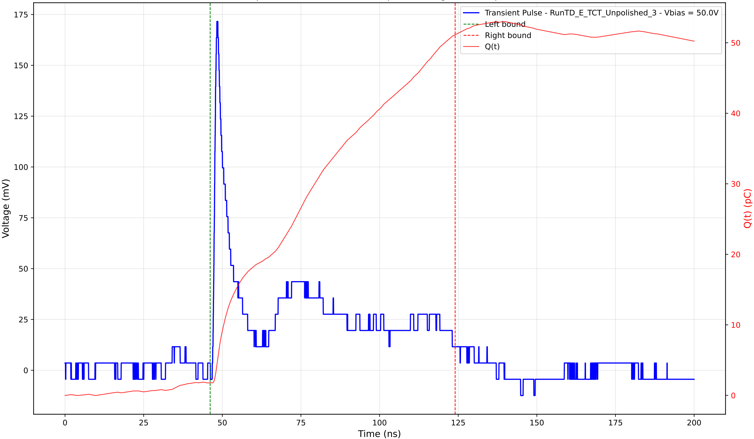
Transient Pulse - Sample: TD - Position: 125.0 \mu\text{m} - Charge: 49.33 pC - Rise Time: 0.97 ns
