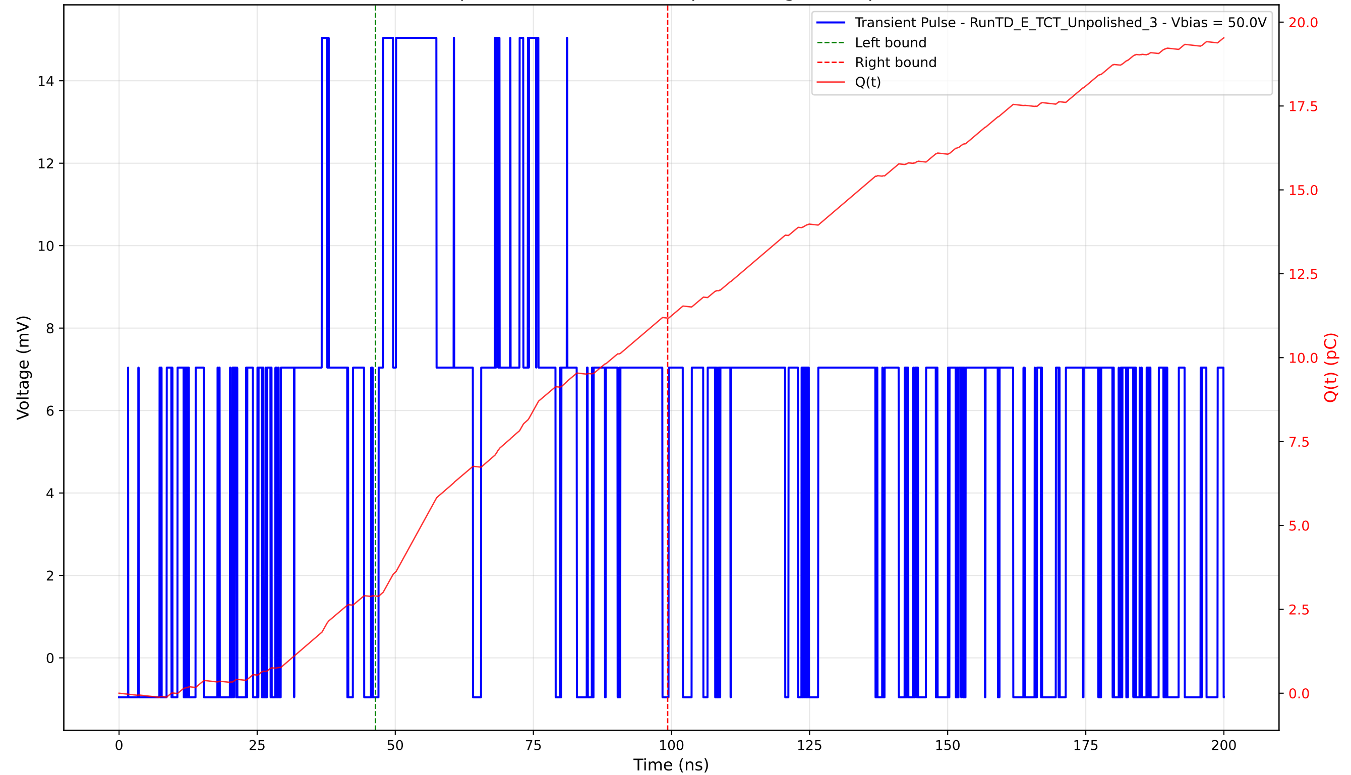
Transient Pulse - Sample: TD - Position: 360.0 \mu\text{m} - Charge: 8.28 pC - Rise Time: 5.00 ns
