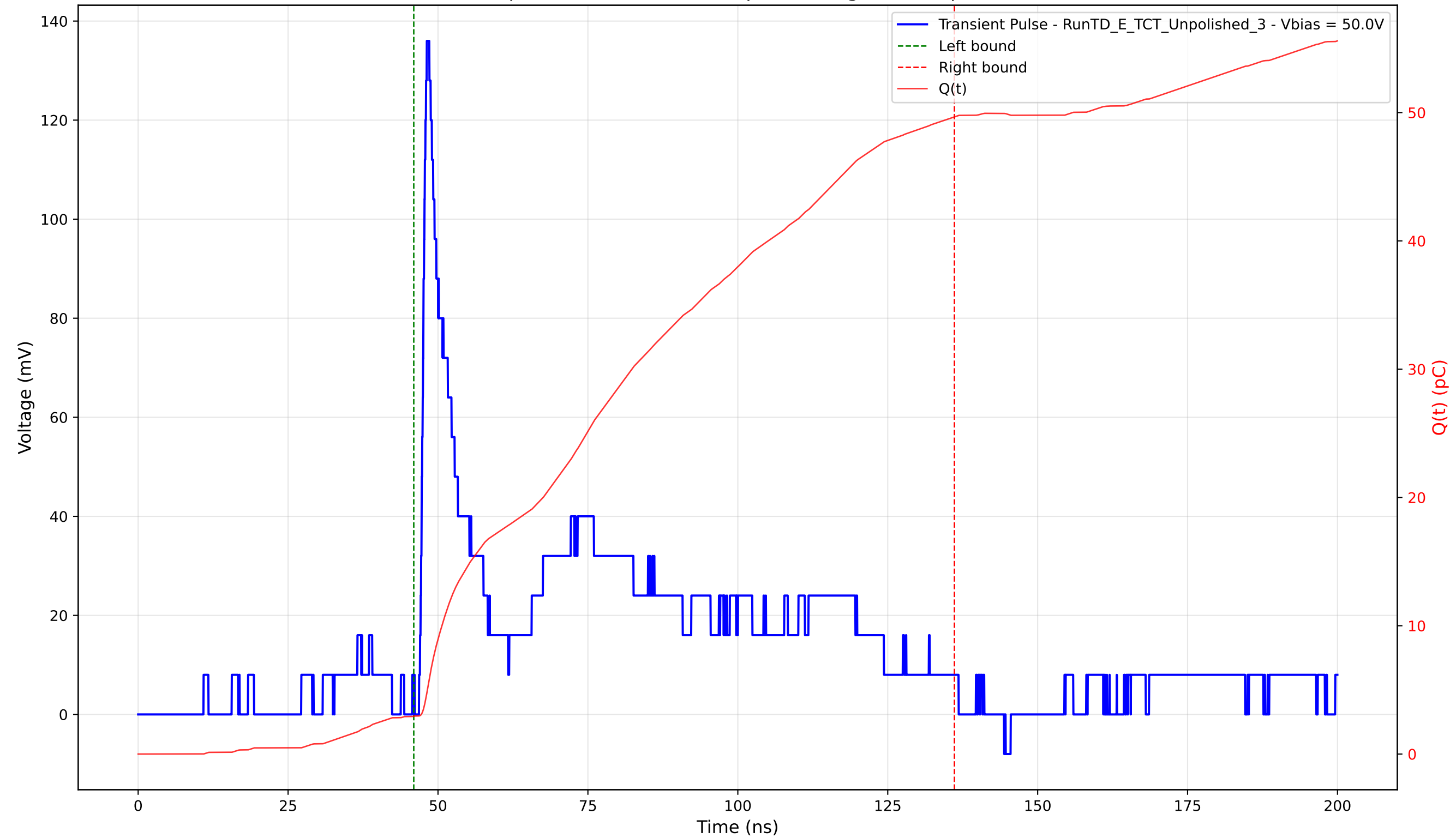
Transient Pulse - Sample: TD - Position: 90.0 \mu\text{m} - Charge: 46.71 pC - Rise Time: 1.01 ns
