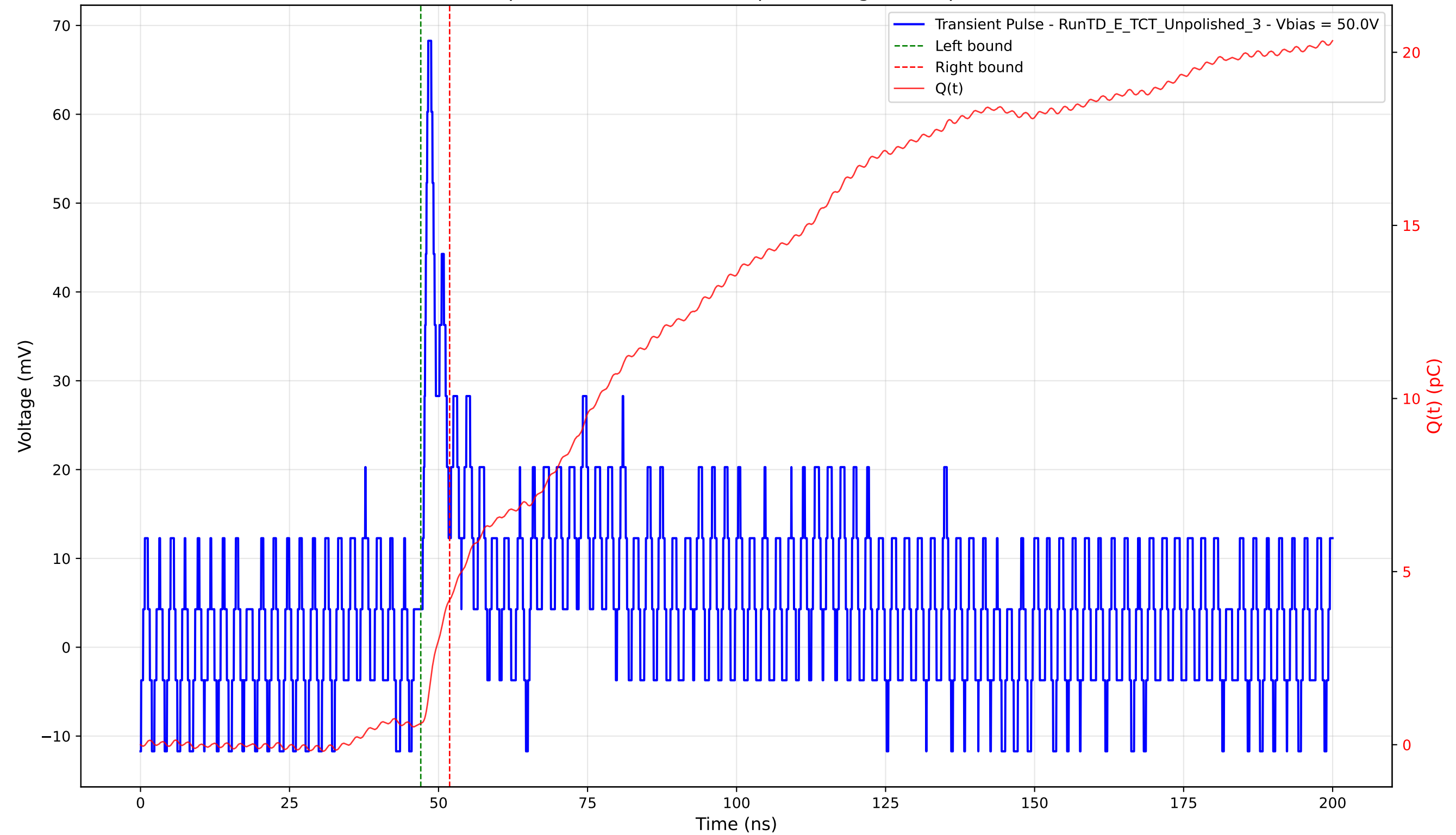
Transient Pulse - Sample: TD - Position: 220.0 \mu\text{m} - Charge: 3.57 pC - Rise Time: 0.93 ns
