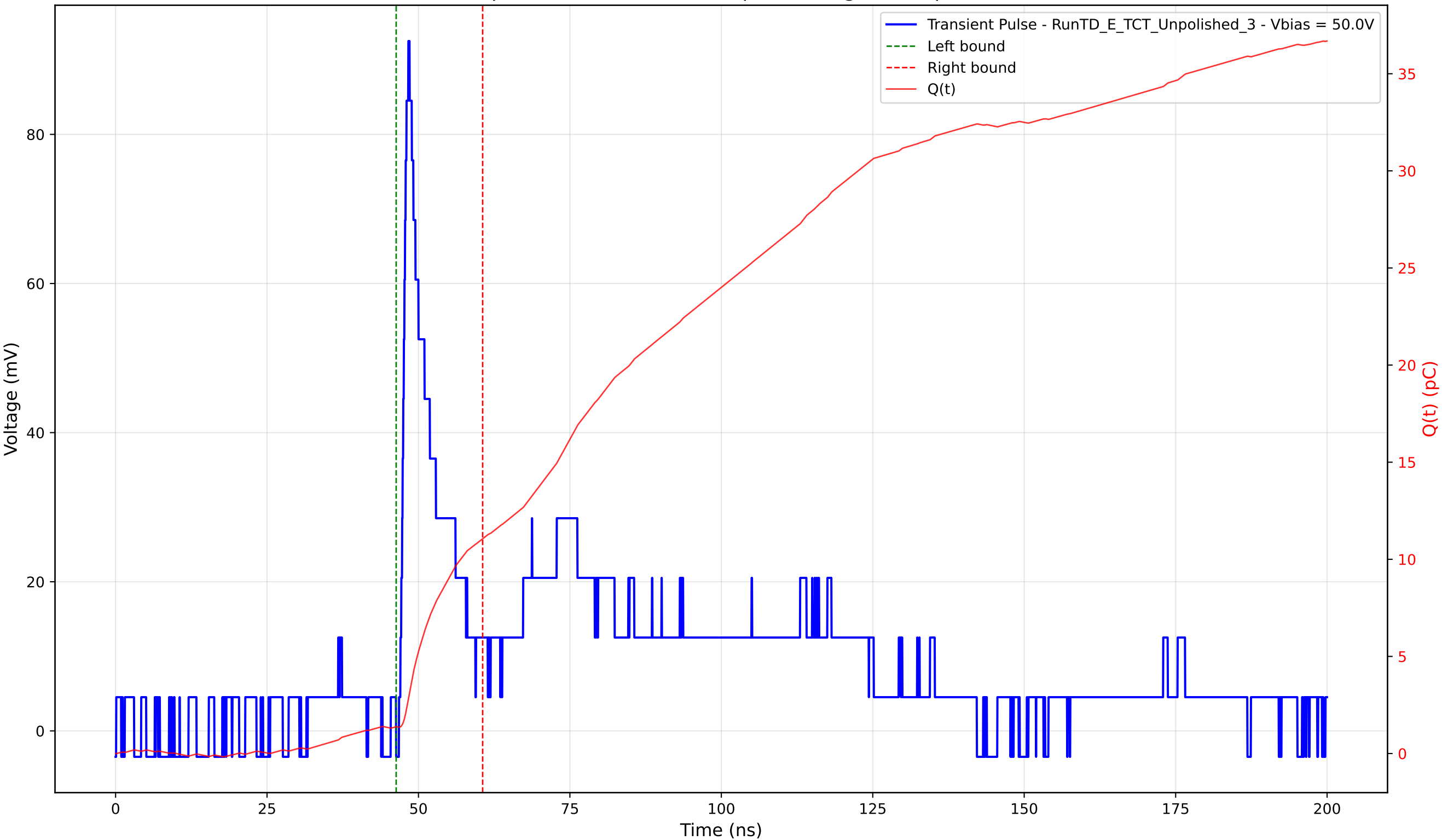
Transient Pulse - Sample: TD - Position: 150.0 \mu\text{m} - Charge: 9.68 pC - Rise Time: 1.01 ns
