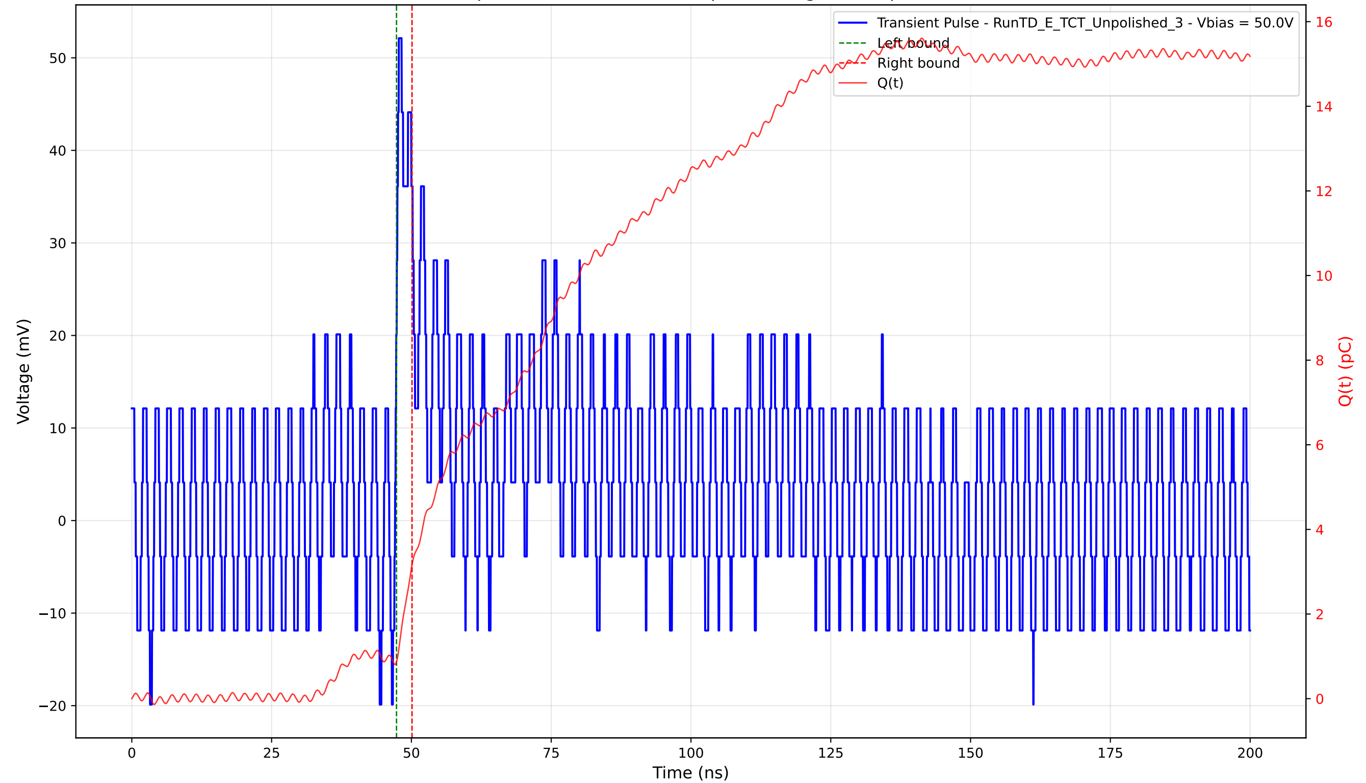
Transient Pulse - Sample: TD - Position: 215.0 \mu\text{m} - Charge: 2.31 pC - Rise Time: 0.58 ns
