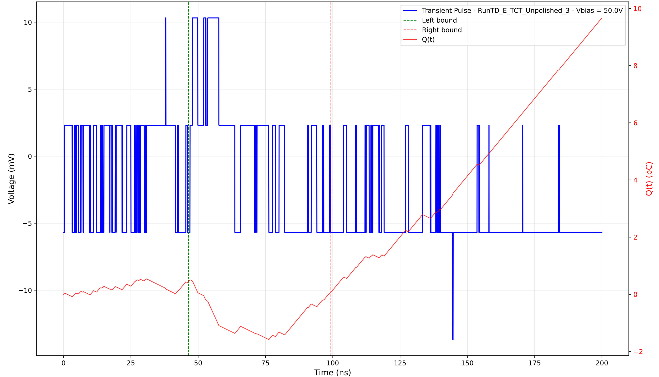
Transient Pulse - Sample: TD - Position: 5.0 \mu\text{m} - Charge: 0.38 pC - Rise Time: 0.00 ns (N/A)
