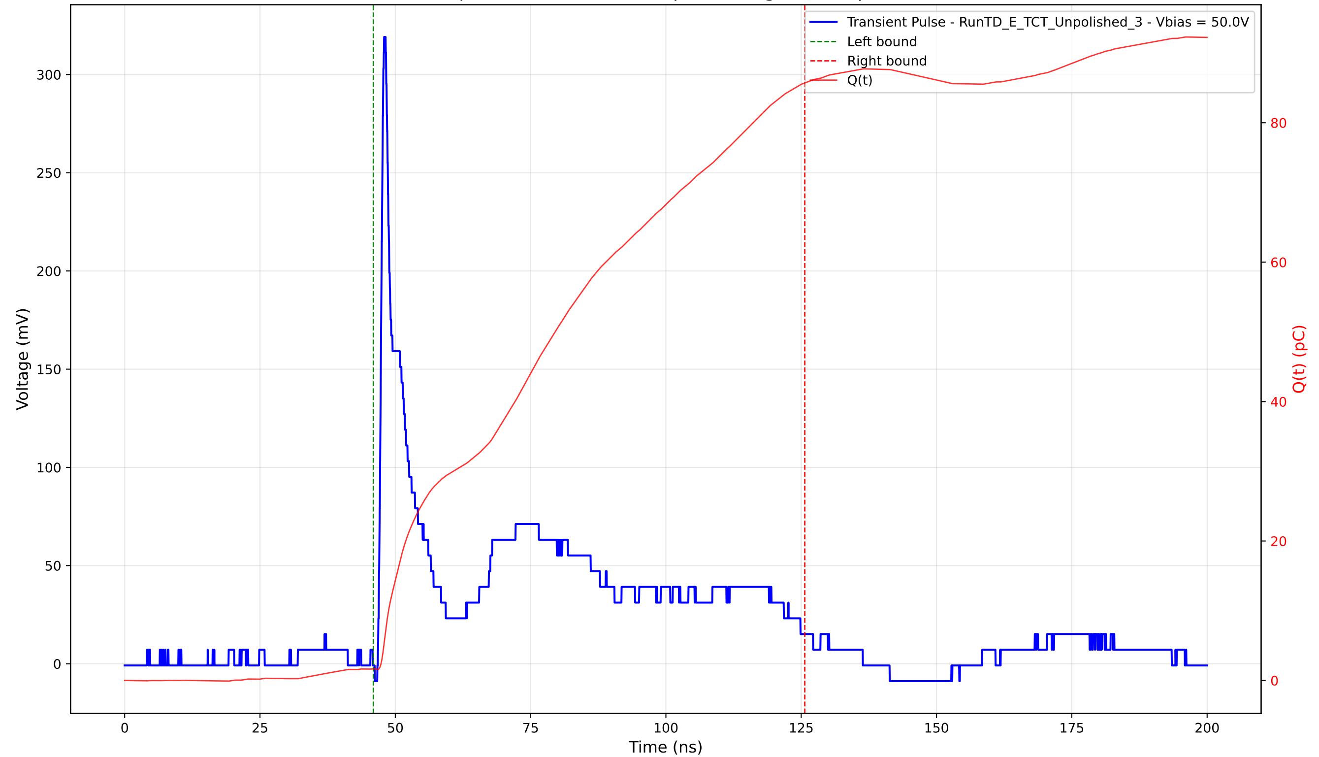
Transient Pulse - Sample: TD - Position: 65.0 \mu\text{m} - Charge: 84.04 pC - Rise Time: 0.80 ns
