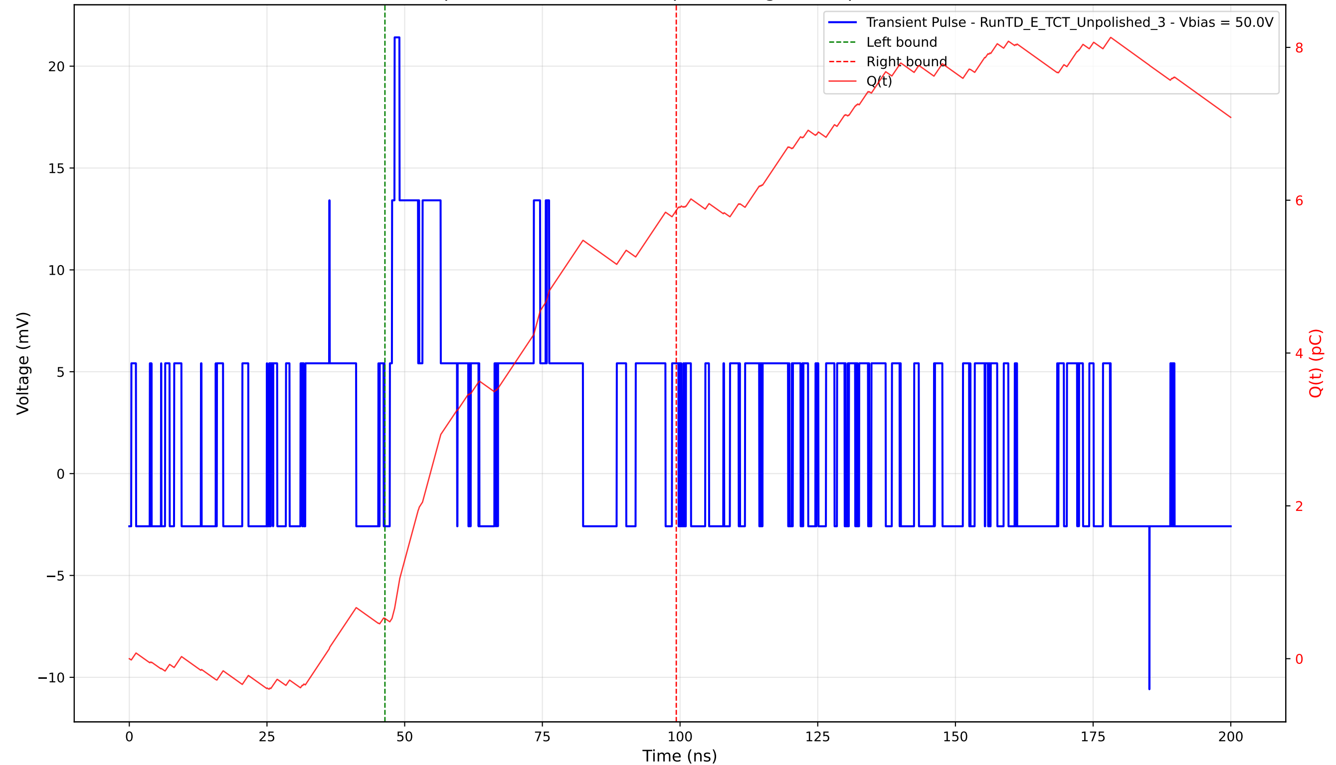
Transient Pulse - Sample: TD - Position: 350.0 \mu\text{m} - Charge: 5.34 pC - Rise Time: 0.00 ns (N/A)
