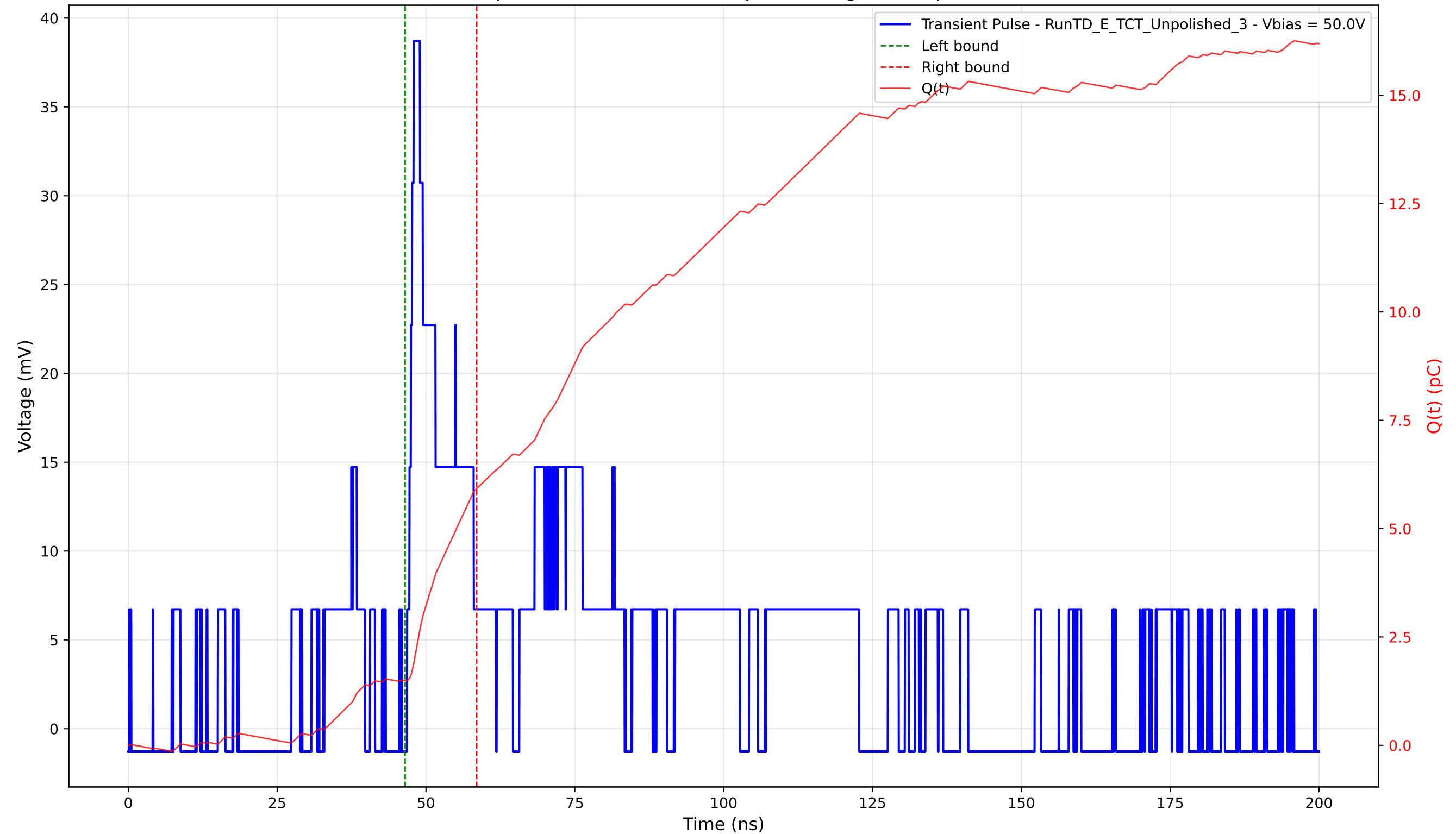
Transient Pulse - Sample: TD - Position: 335.0 \mu\text{m} - Charge: 4.43 pC - Rise Time: 1.11 ns
