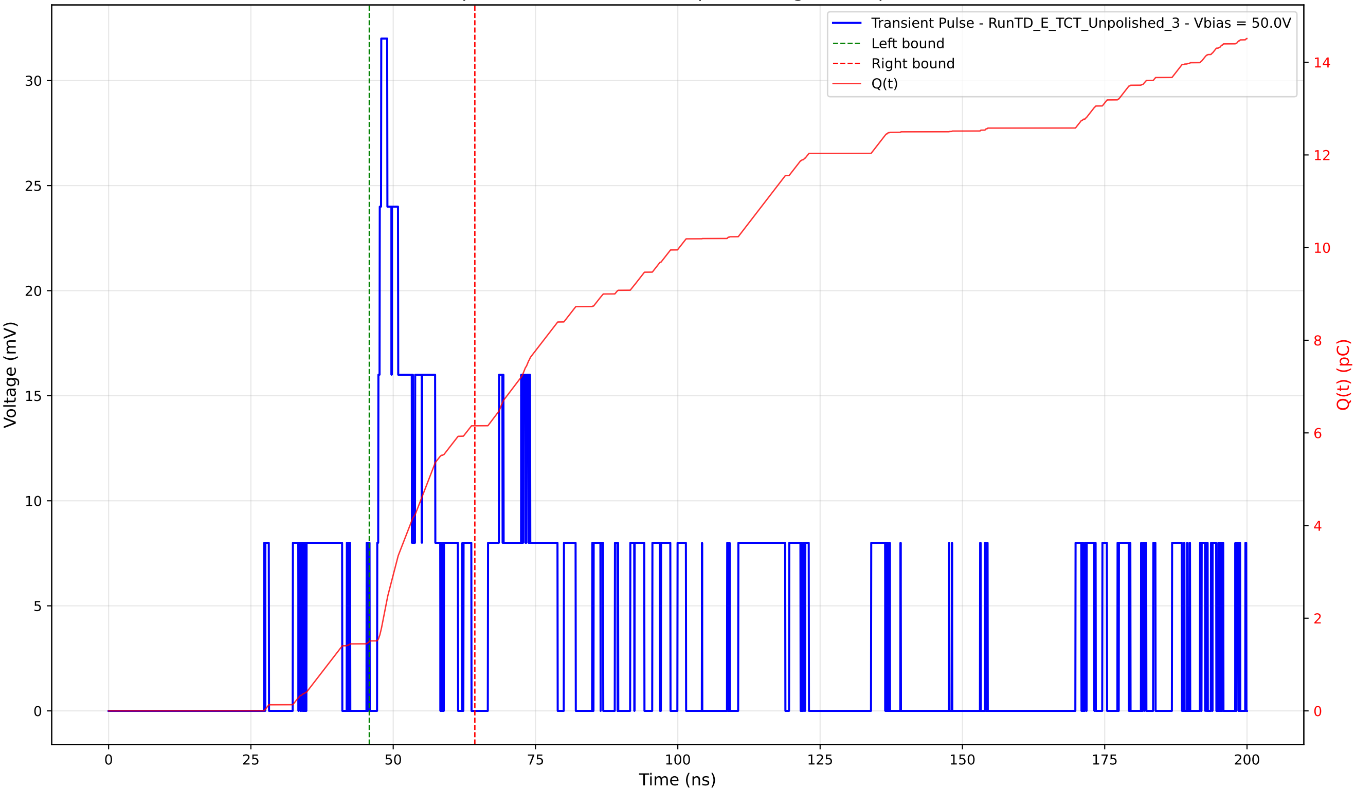
Transient Pulse - Sample: TD - Position: 260.0 \mu\text{m} - Charge: 4.65 pC - Rise Time: 0.71 ns
