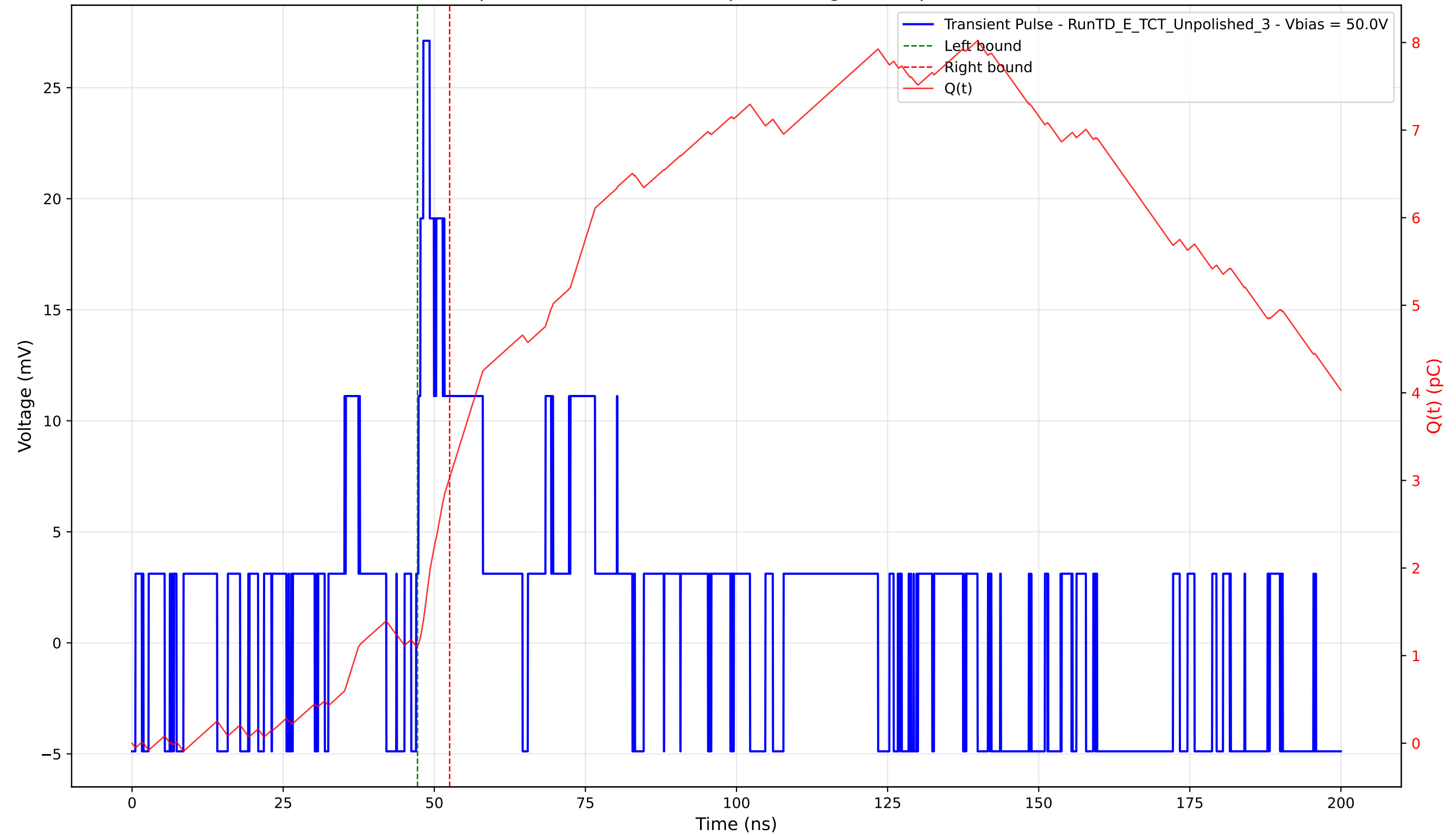
Transient Pulse - Sample: TD - Position: 395.0 \mu\text{m} - Charge: 1.91 pC - Rise Time: 0.00 ns (N/A)
