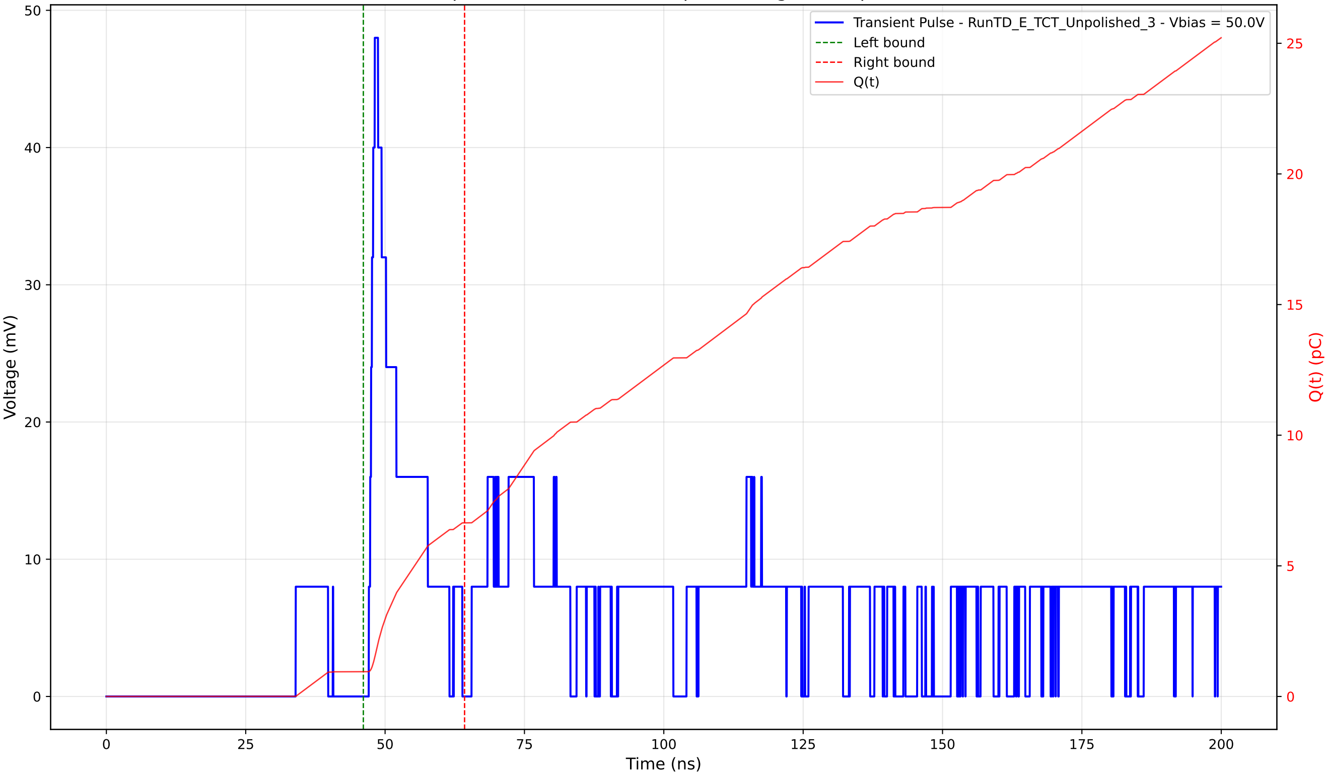
Transient Pulse - Sample: TD - Position: 310.0 \mu\text{m} - Charge: 5.70 pC - Rise Time: 1.07 ns
