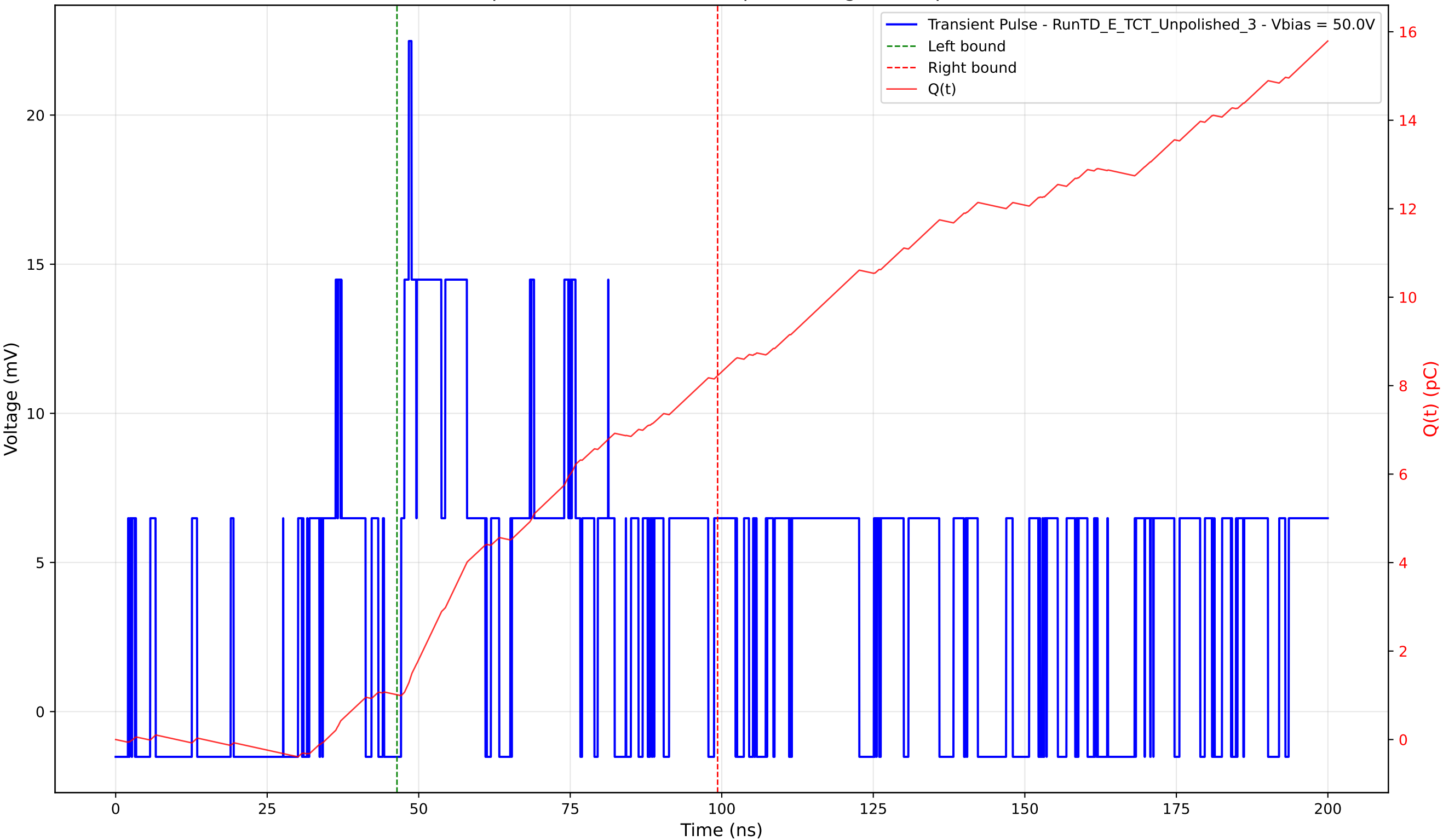
Transient Pulse - Sample: TD - Position: 415.0 \mu\text{m} - Charge: 7.21 pC - Rise Time: 1.28 ns
