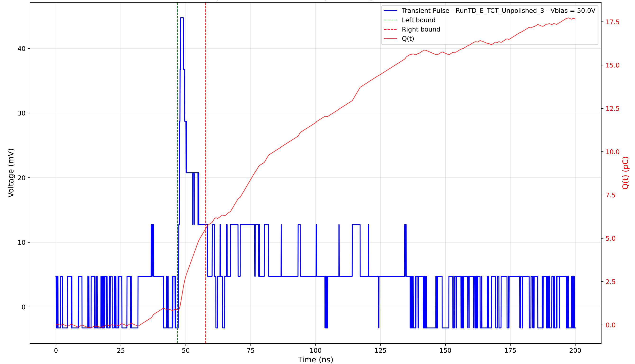
Transient Pulse - Sample: TD - Position: 320.0 \mu\text{m} - Charge: 4.68 pC - Rise Time: 0.88 ns
