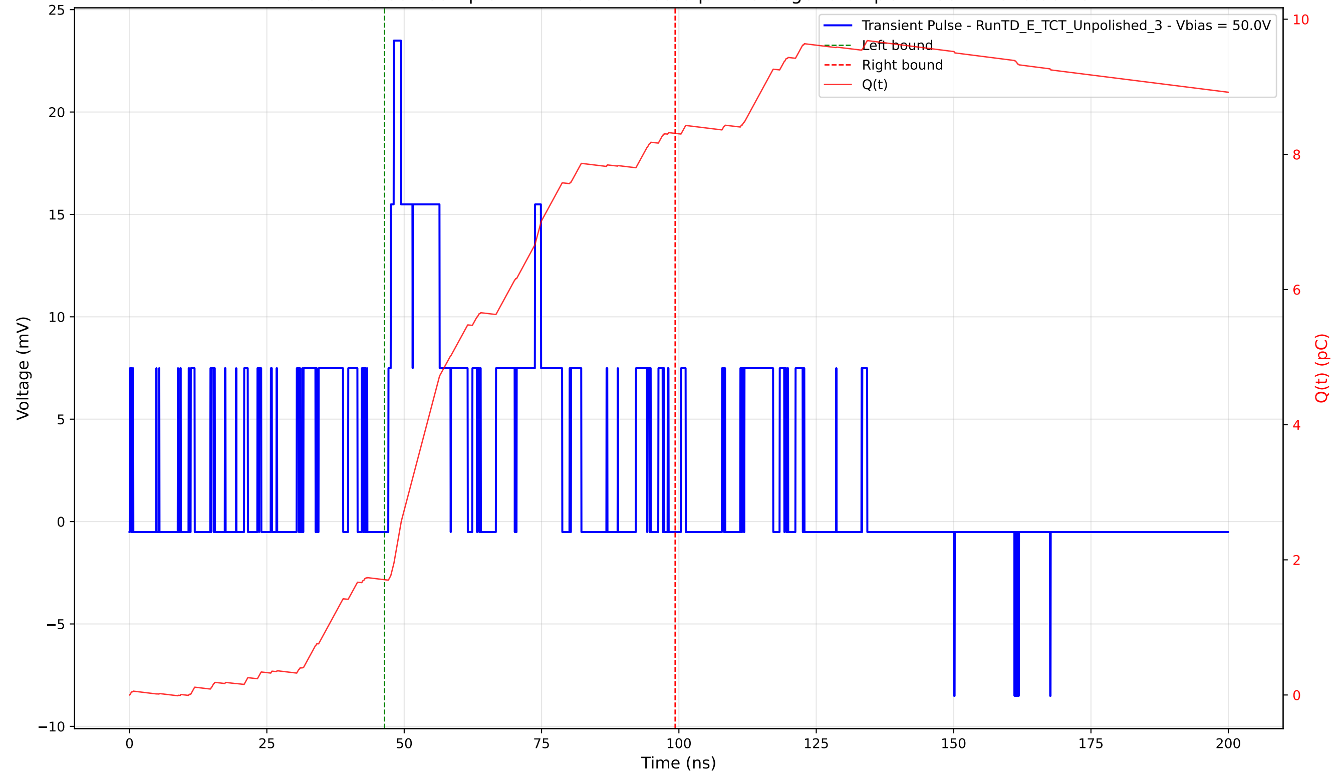
Transient Pulse - Sample: TD - Position: 405.0 \mu\text{m} - Charge: 6.61 pC - Rise Time: 0.99 ns
