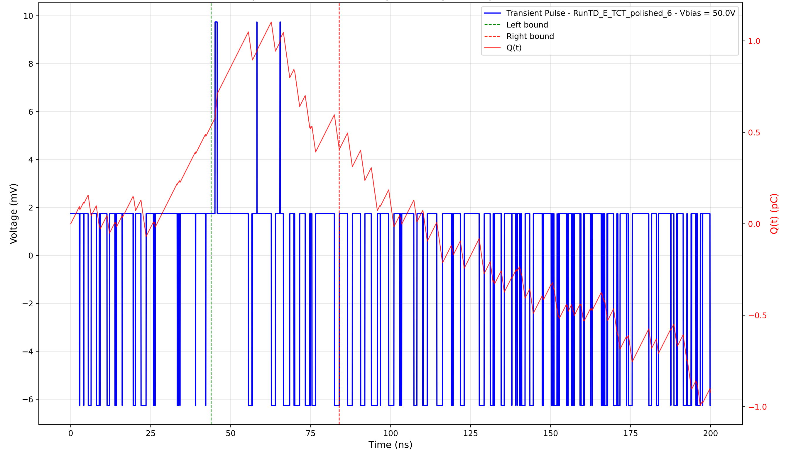
Transient Pulse - Sample: 4003 - Position: 5.0 \mu\text{m} - Charge: 0.13 pC - Rise Time: 0.00 ns (N/A)
