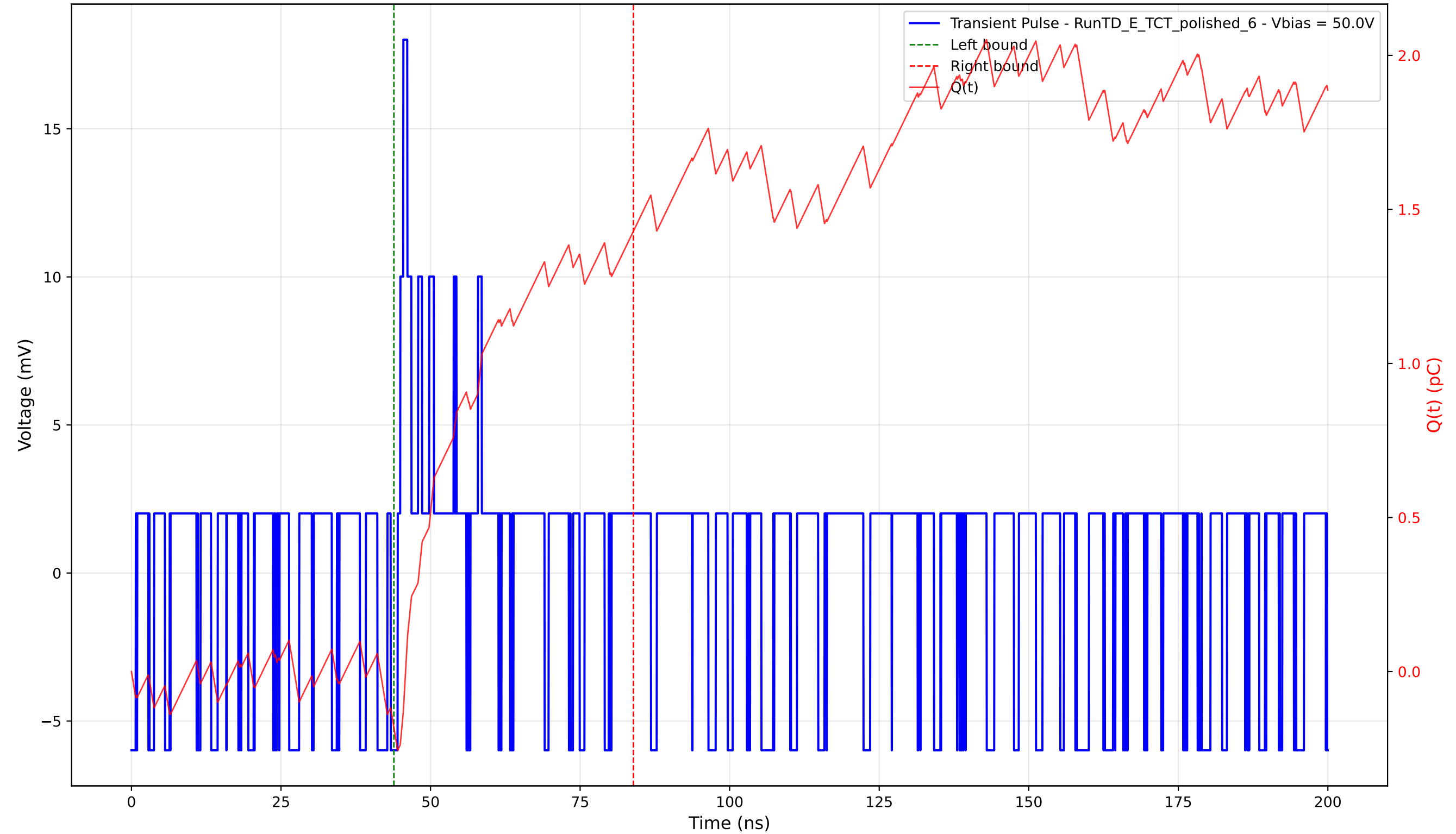
Transient Pulse - Sample: 4003 - Position: 335.0 \mu\text{m} - Charge: 1.61 pC - Rise Time: 0.00 ns (N/A)
