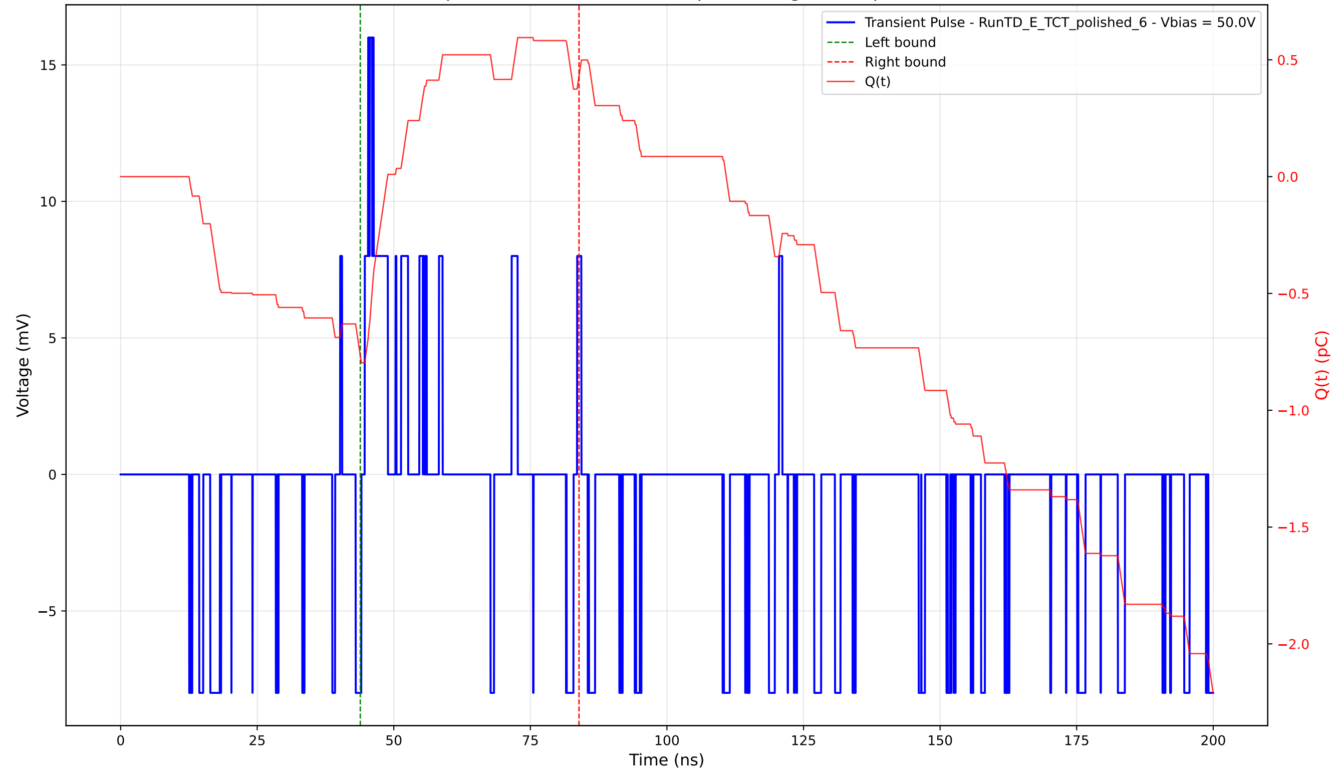
Transient Pulse - Sample: 4003 - Position: 365.0 \mu\text{m} - Charge: 1.20 pC - Rise Time: 0.64 ns
