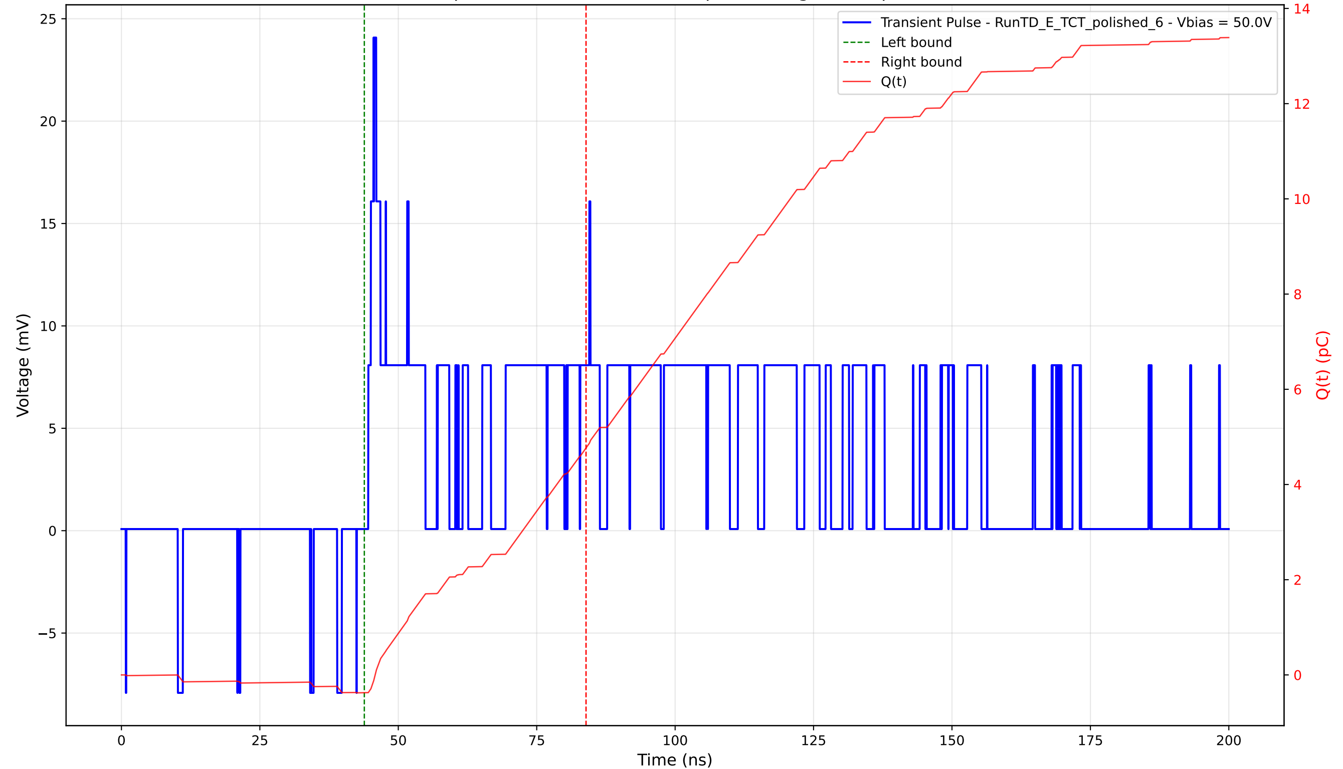
Transient Pulse - Sample: 4003 - Position: 230.0 \mu\text{m} - Charge: 5.14 pC - Rise Time: 0.95 ns
