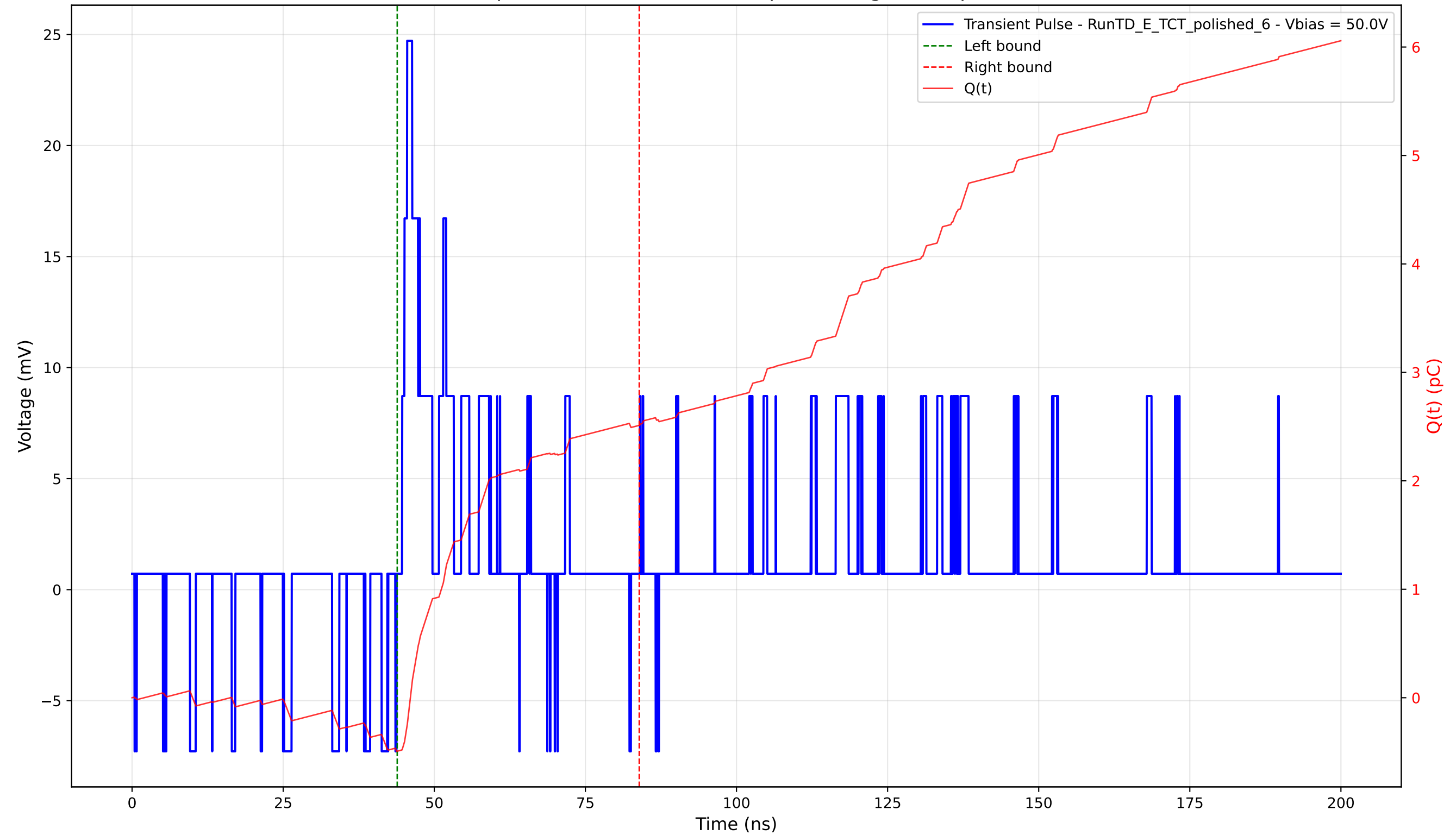
Transient Pulse - Sample: 4003 - Position: 245.0 \mu\text{m} - Charge: 3.00 pC - Rise Time: 0.84 ns
