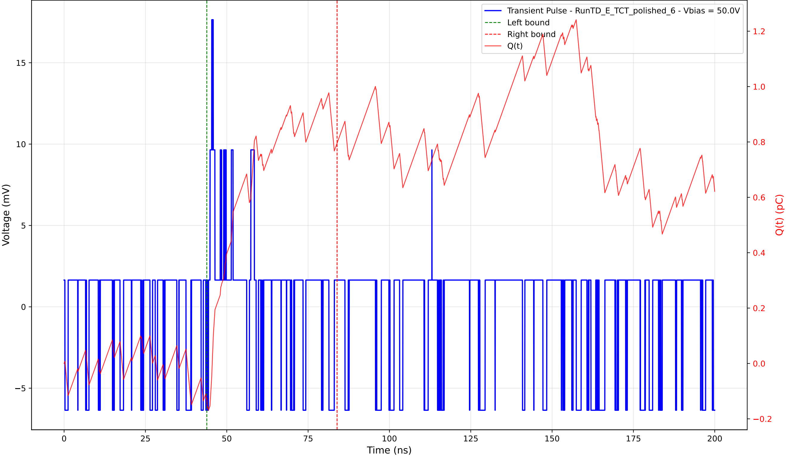
Transient Pulse - Sample: 4003 - Position: 25.0 \mu\text{m} - Charge: 0.93 pC - Rise Time: 0.54 ns
