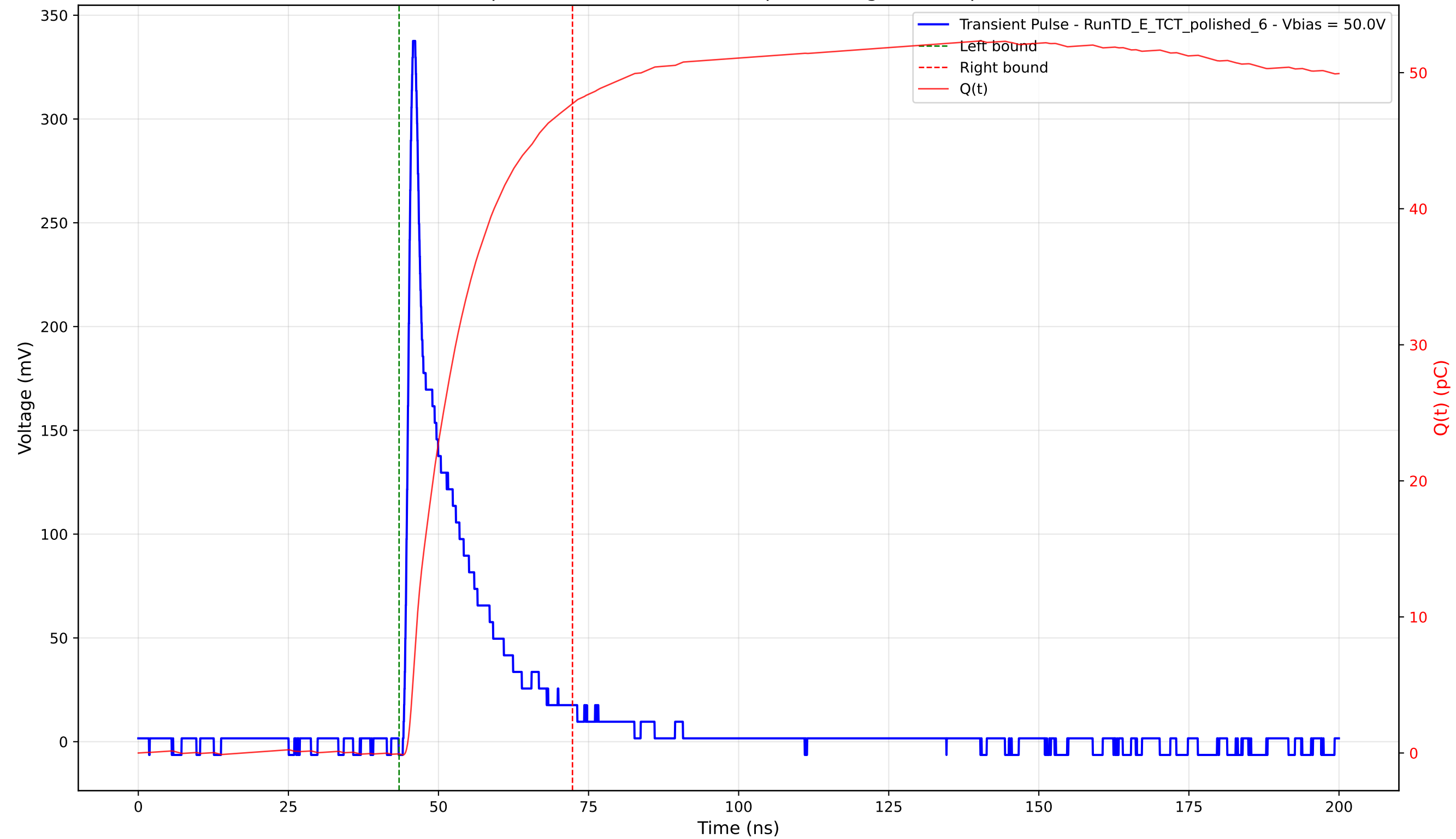
Transient Pulse - Sample: 4003 - Position: 140.0 \mu\text{m} - Charge: 47.80 pC - Rise Time: 1.08 ns
