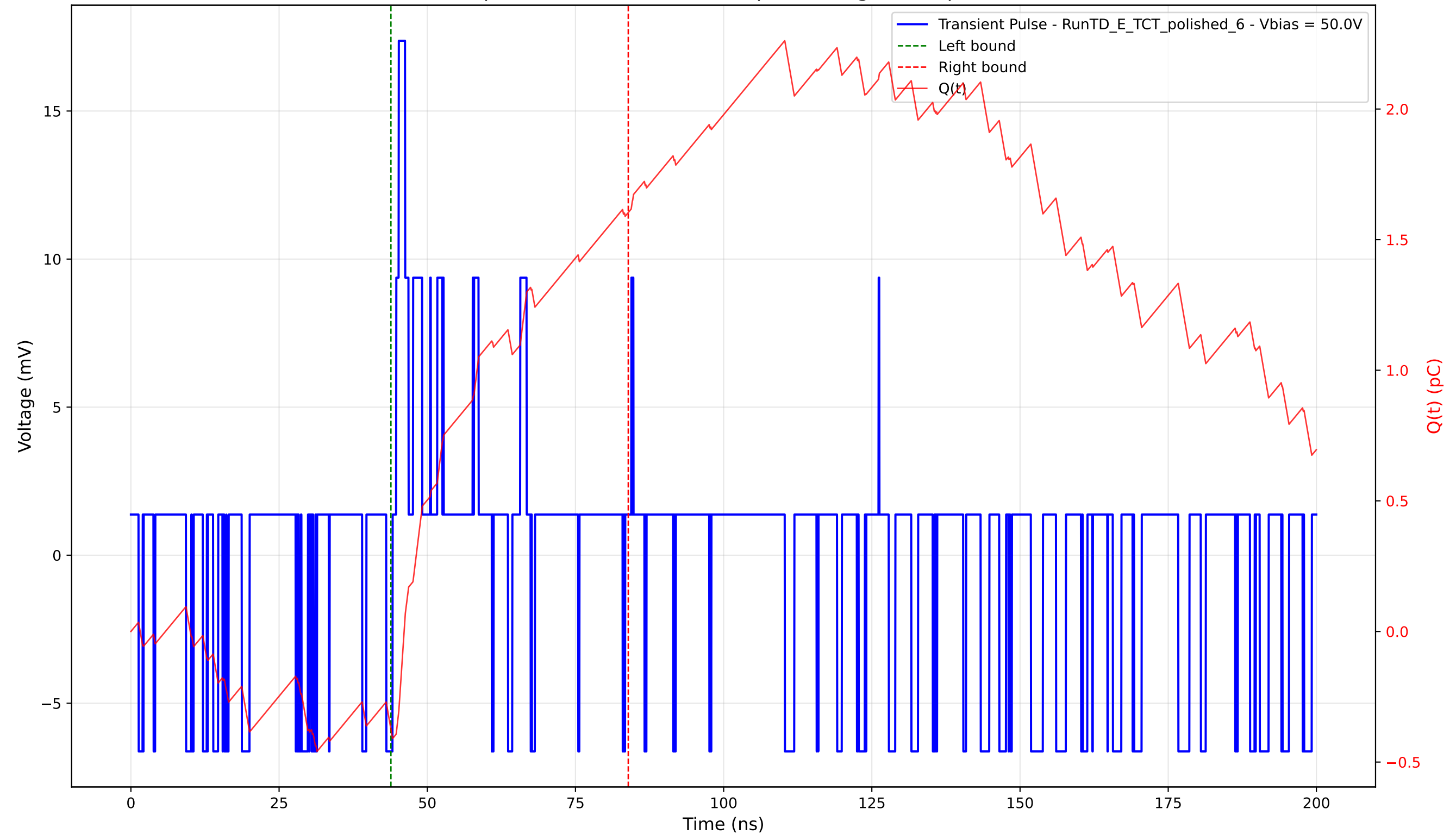
Transient Pulse - Sample: 4003 - Position: 370.0 \mu\text{m} - Charge: 1.98 pC - Rise Time: 0.44 ns
