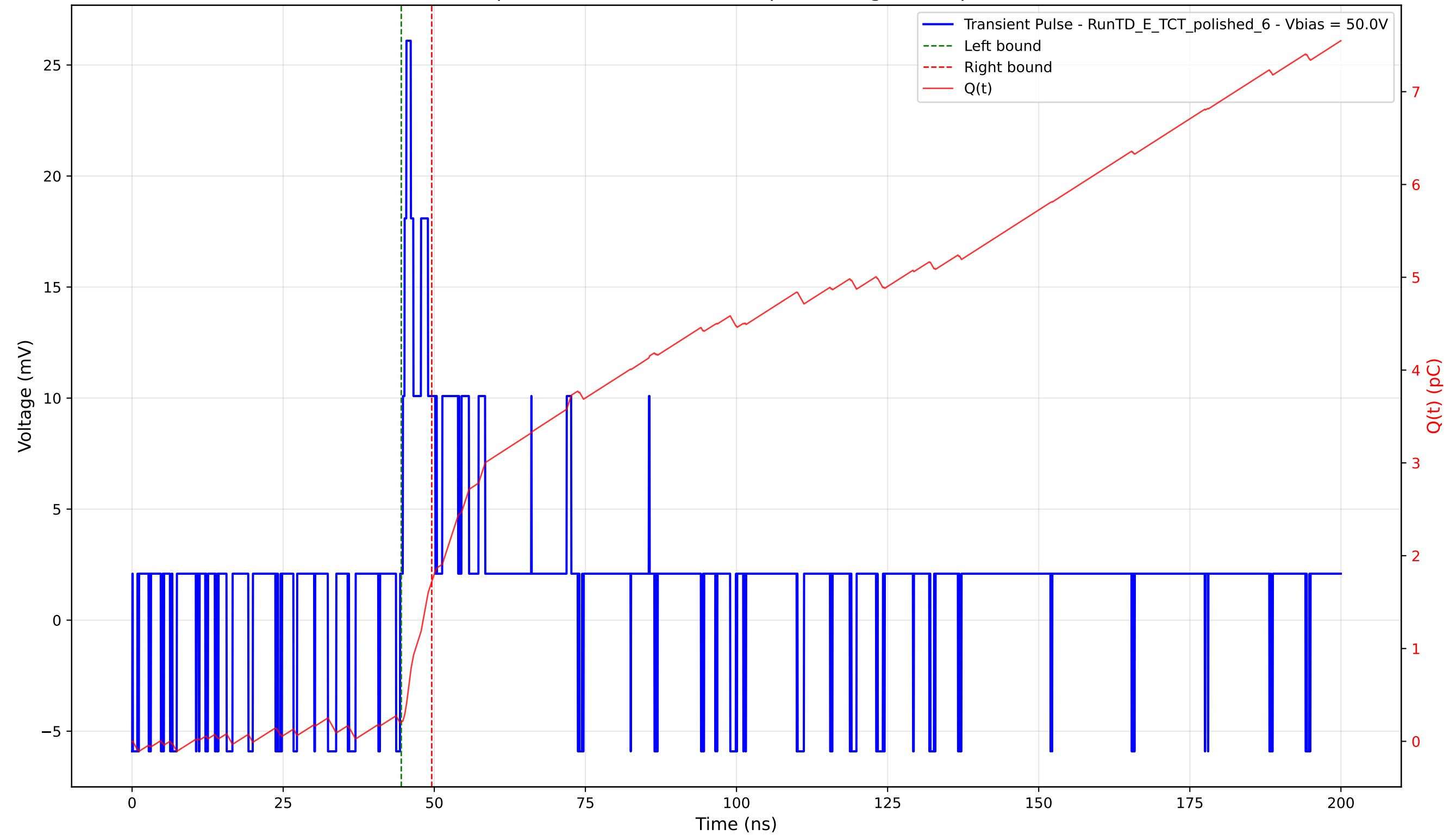
Transient Pulse - Sample: 4003 - Position: 290.0 \mu\text{m} - Charge: 1.51 pC - Rise Time: 0.60 ns
