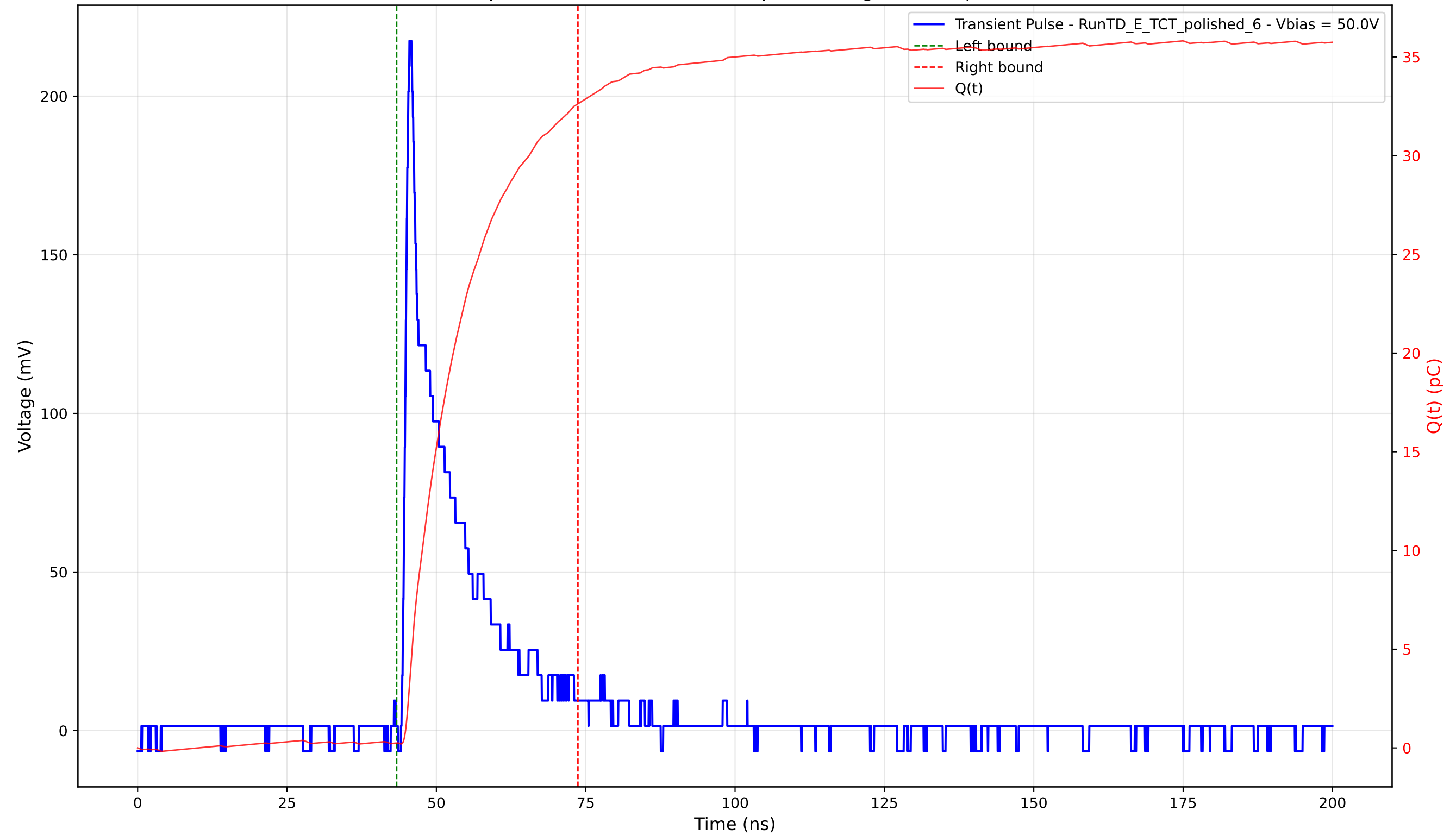
Transient Pulse - Sample: 4003 - Position: 105.0 \mu\text{m} - Charge: 32.37 pC - Rise Time: 0.95 ns
