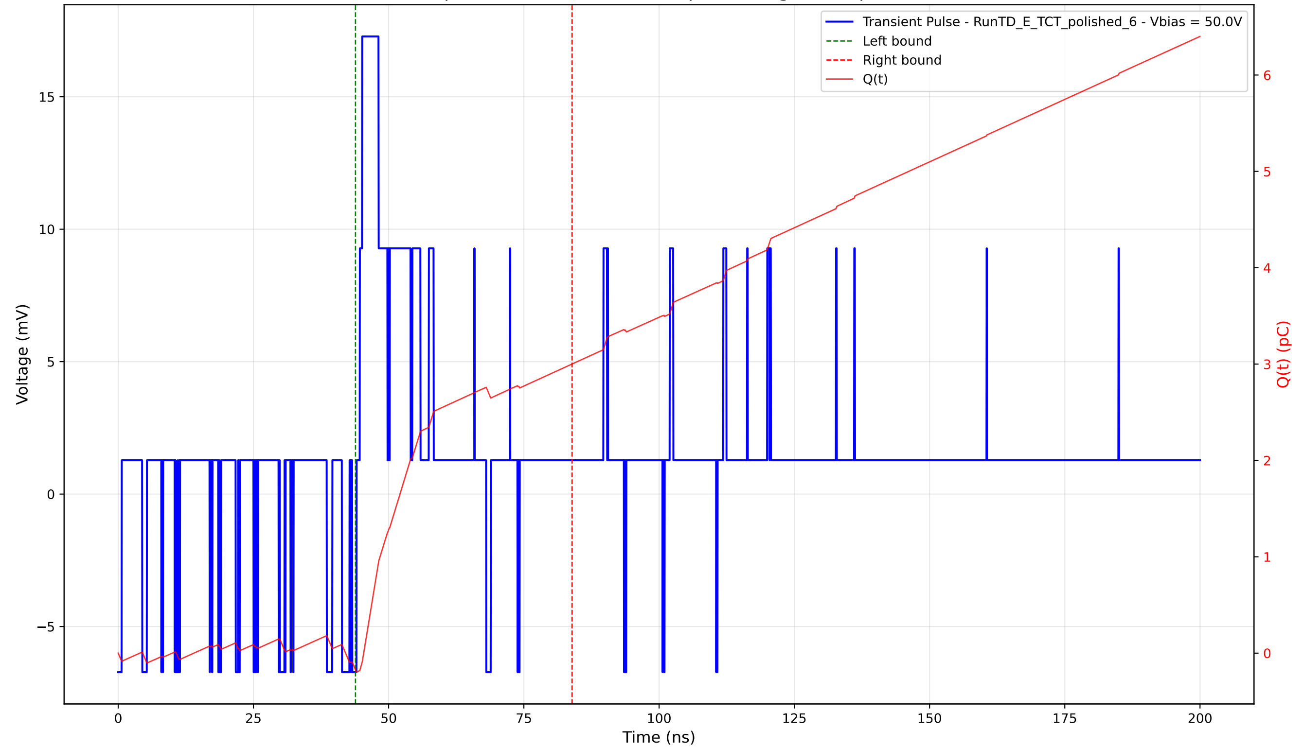
Transient Pulse - Sample: 4003 - Position: 250.0 \mu\text{m} - Charge: 3.17 pC - Rise Time: 0.46 ns
