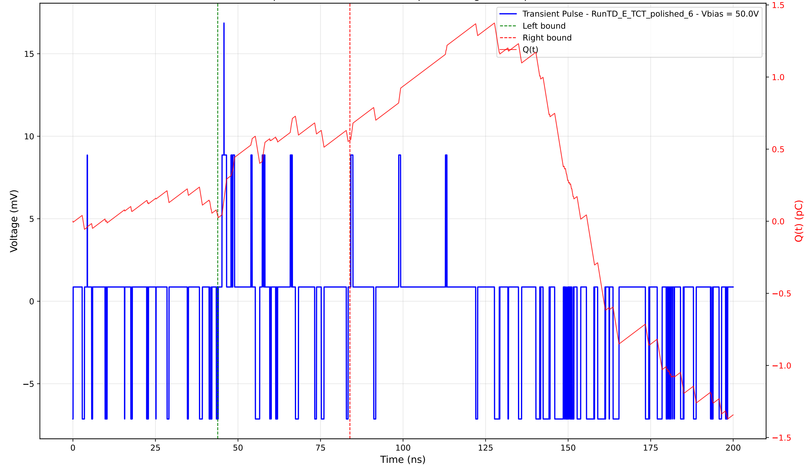
Transient Pulse - Sample: 4003 - Position: 75.0 \mu\text{m} - Charge: 0.52 pC - Rise Time: 0.62 ns
