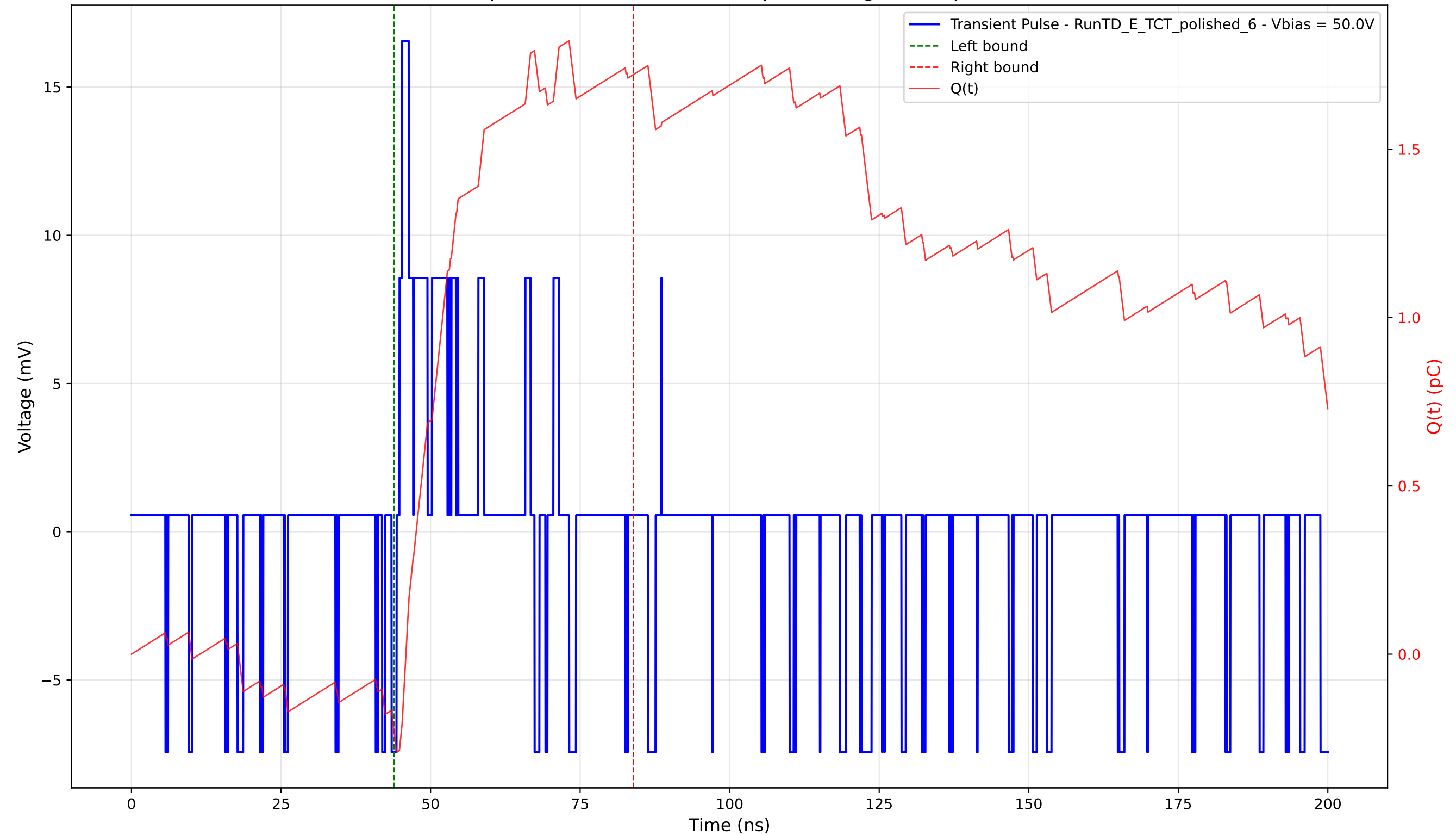
Transient Pulse - Sample: 4003 - Position: 375.0 \mu\text{m} - Charge: 1.95 pC - Rise Time: 0.46 ns
