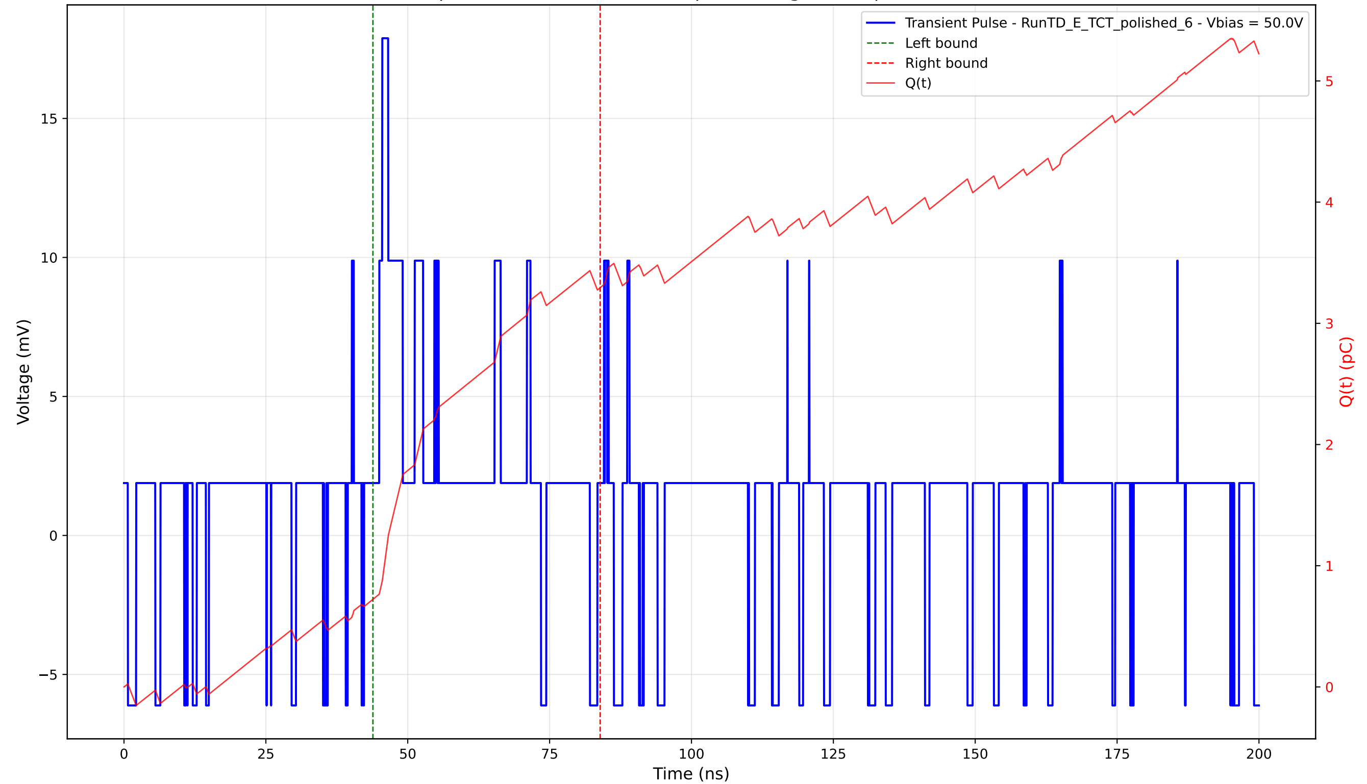
Transient Pulse - Sample: 4003 - Position: 330.0 \mu\text{m} - Charge: 2.57 pC - Rise Time: 0.00 ns (N/A)
