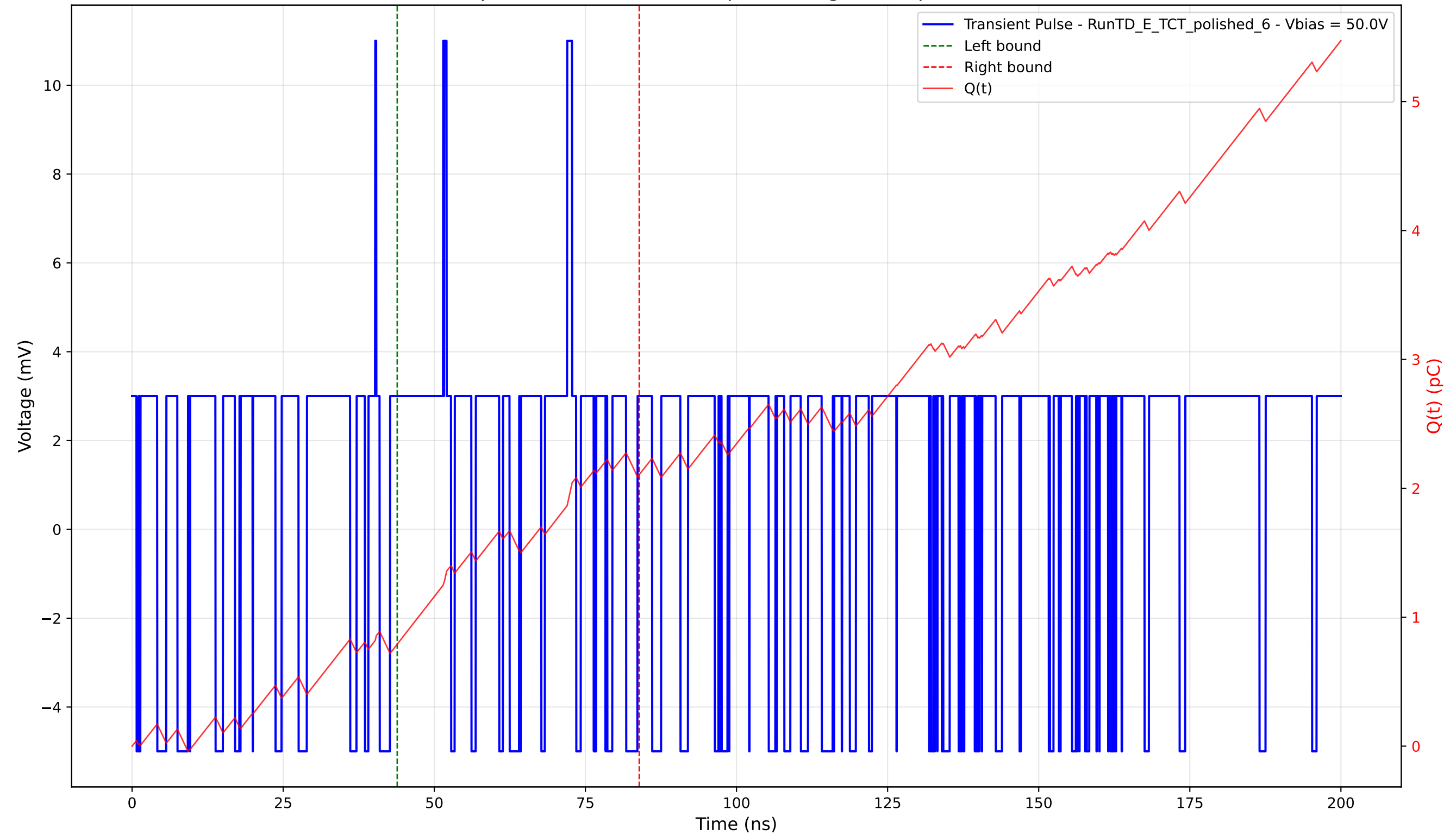
Transient Pulse - Sample: 4003 - Position: 0.0 \mu\text{m} - Charge: 1.31 pC - Rise Time: 0.00 ns (N/A)
