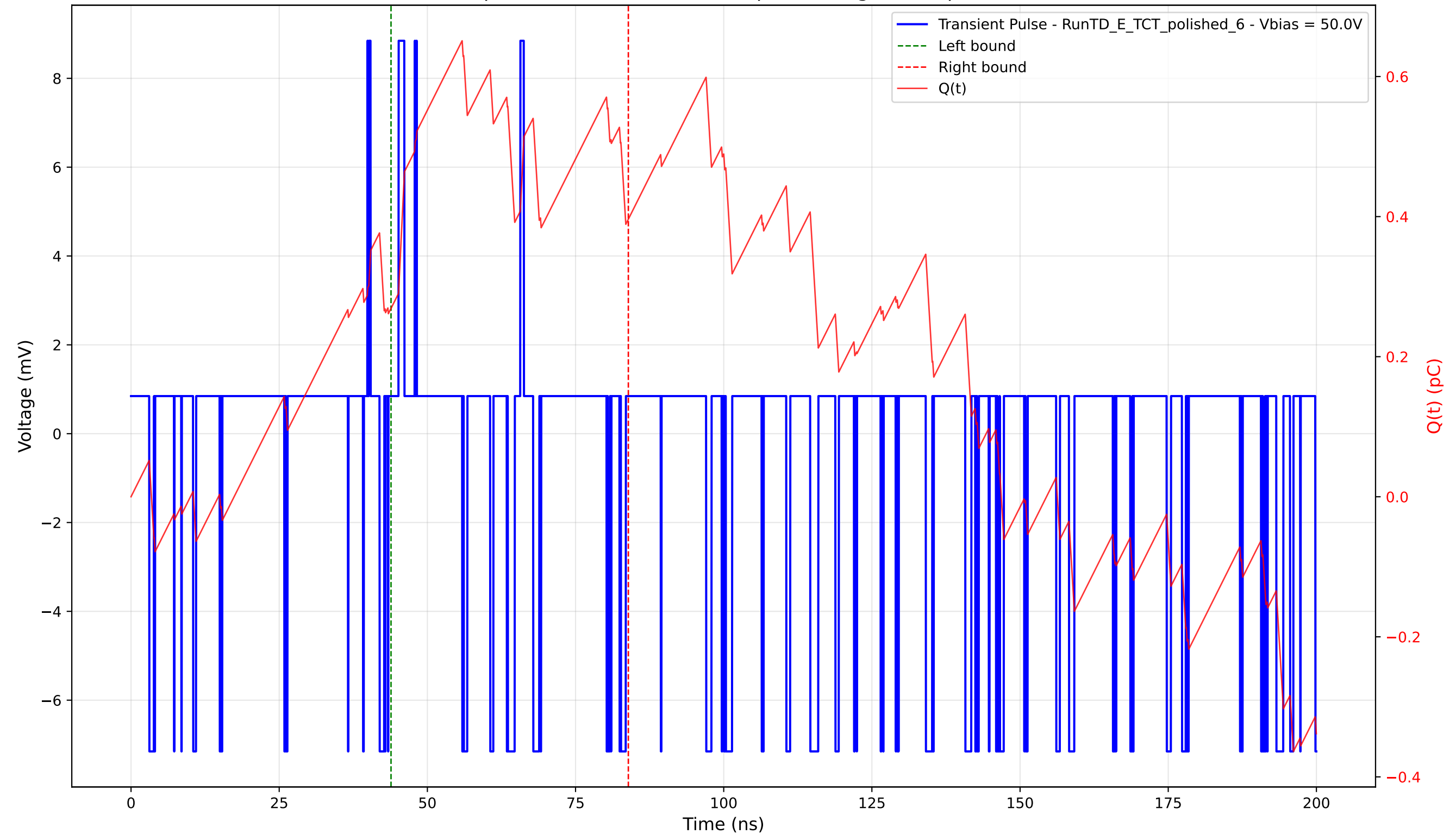
Transient Pulse - Sample: 4003 - Position: 420.0 \mu\text{m} - Charge: 0.13 pC - Rise Time: 0.02 ns
