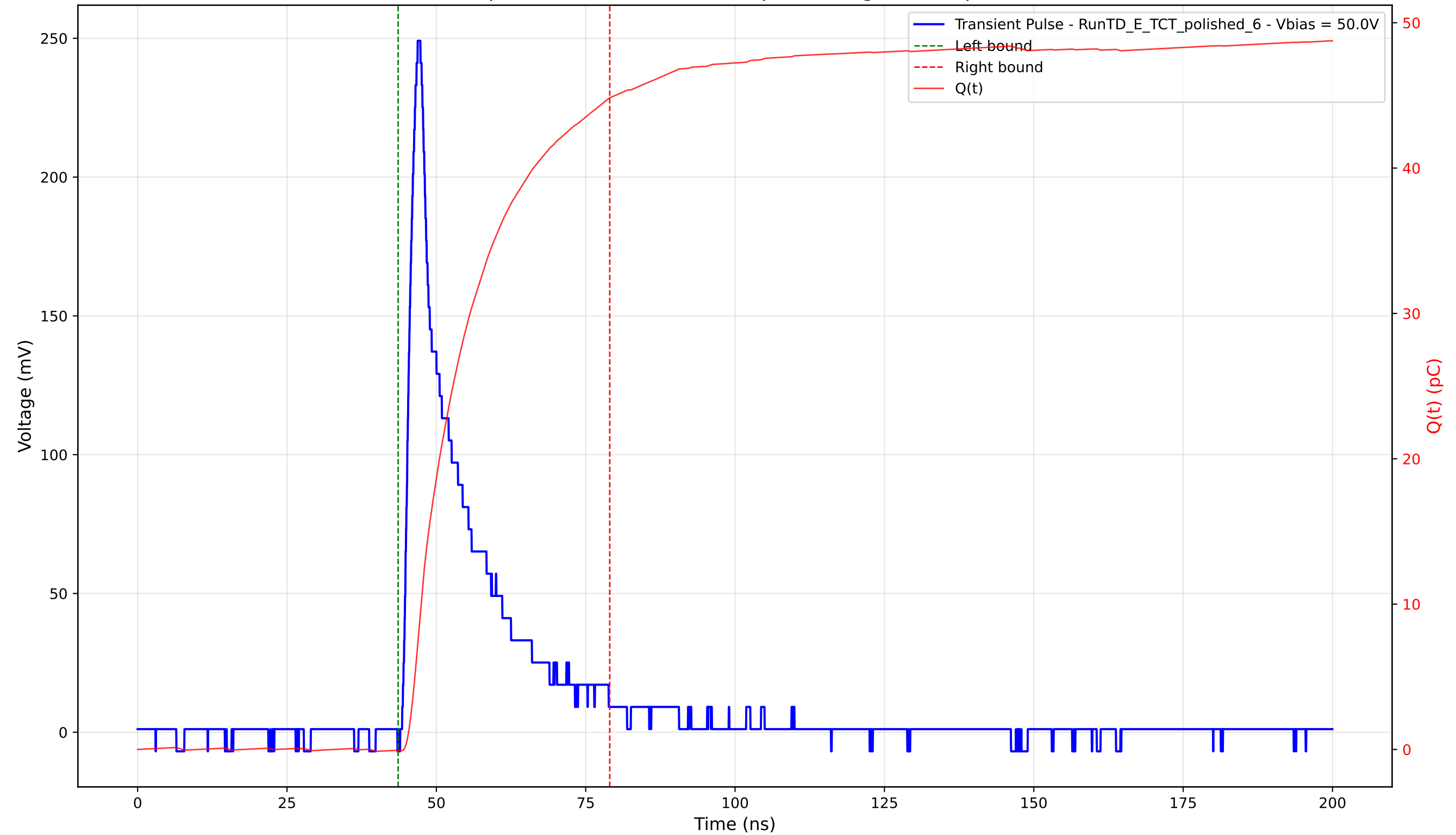
Transient Pulse - Sample: 4003 - Position: 180.0 \mu\text{m} - Charge: 44.90 pC - Rise Time: 1.90 ns
