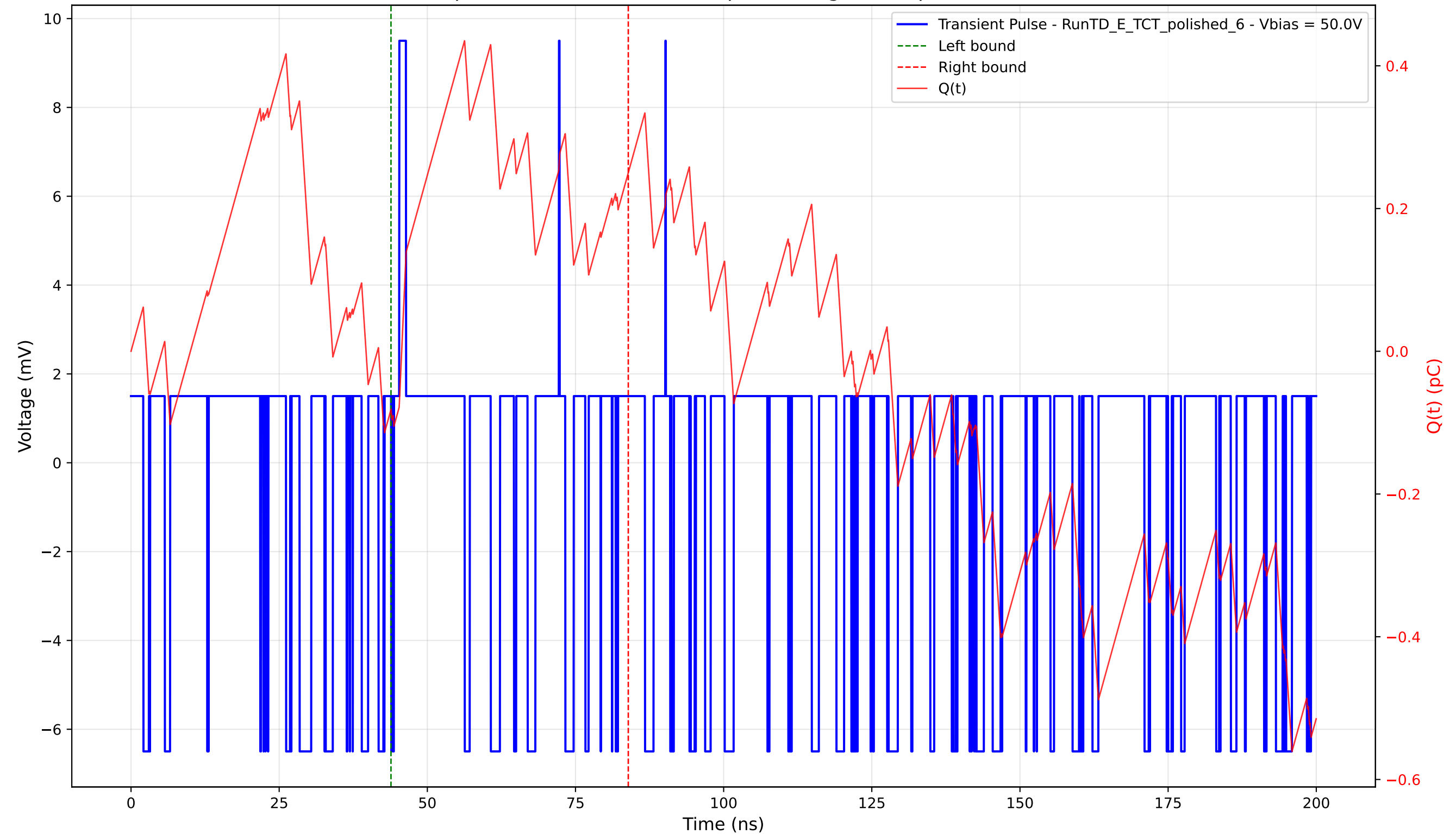
Transient Pulse - Sample: 4003 - Position: 415.0 \mu\text{m} - Charge: 0.33 pC - Rise Time: 0.00 ns (N/A)
