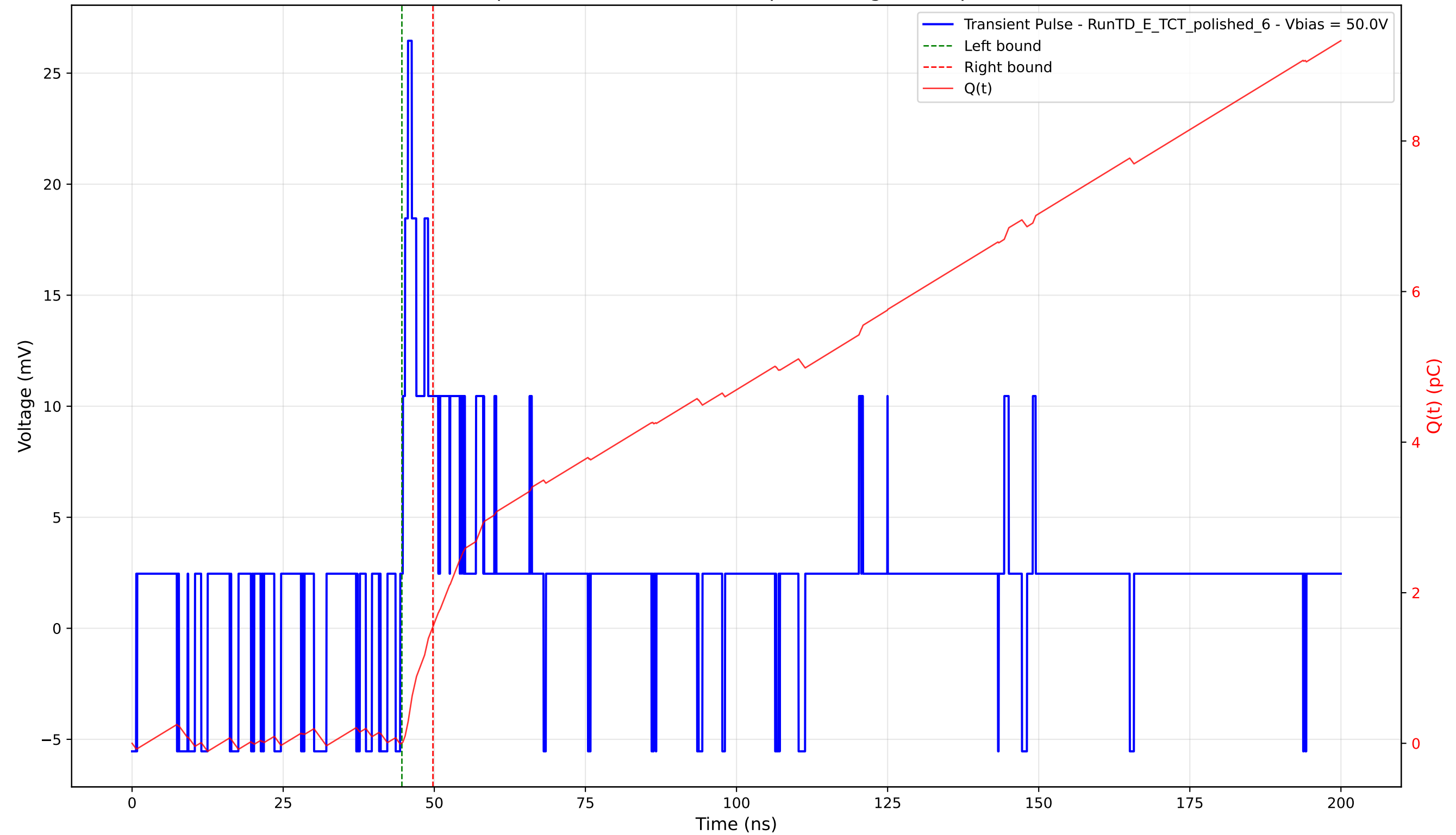
Transient Pulse - Sample: 4003 - Position: 260.0 \mu\text{m} - Charge: 1.55 pC - Rise Time: 0.86 ns
