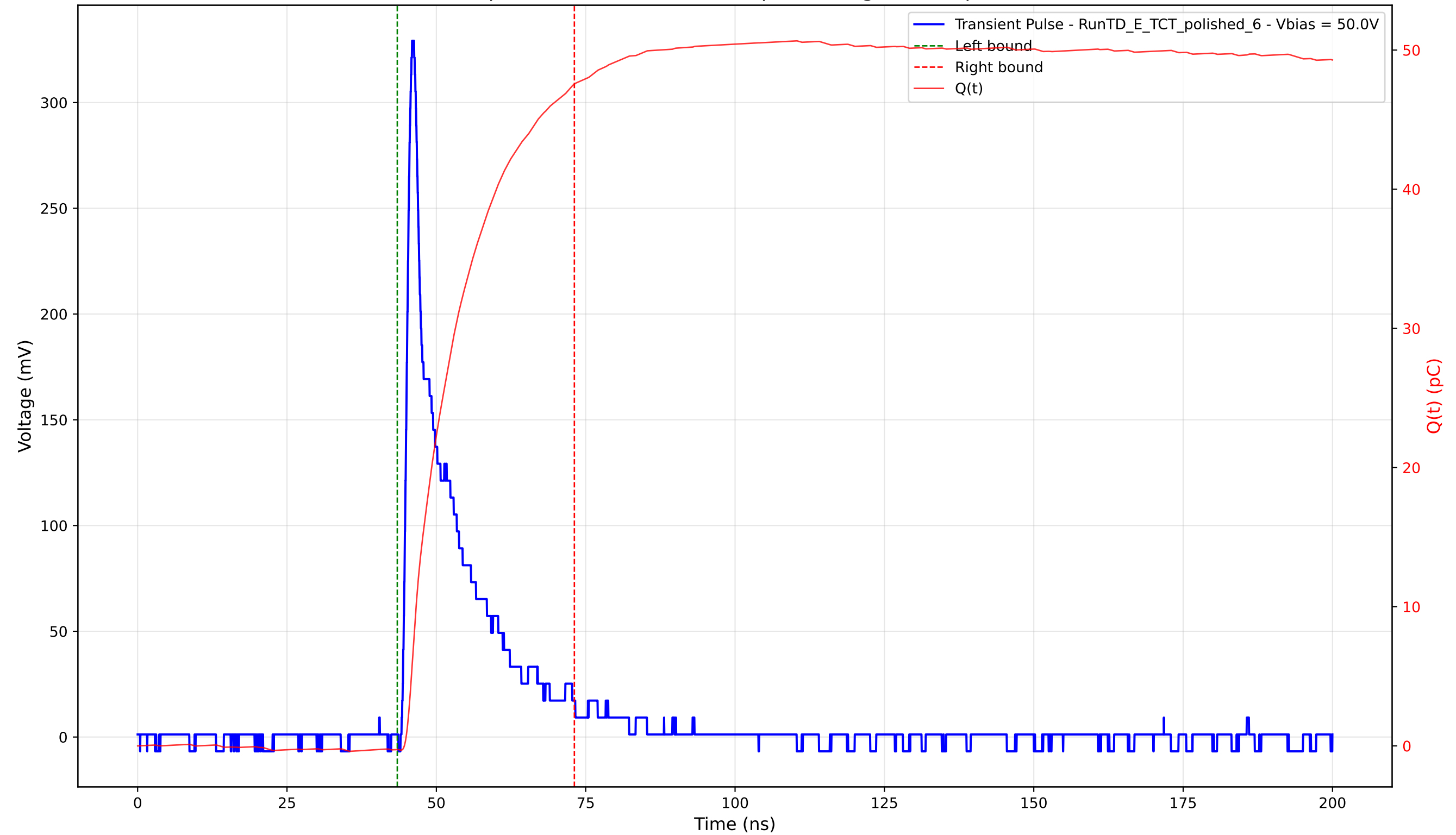
Transient Pulse - Sample: 4003 - Position: 150.0 \mu\text{m} - Charge: 47.82 pC - Rise Time: 1.20 ns
