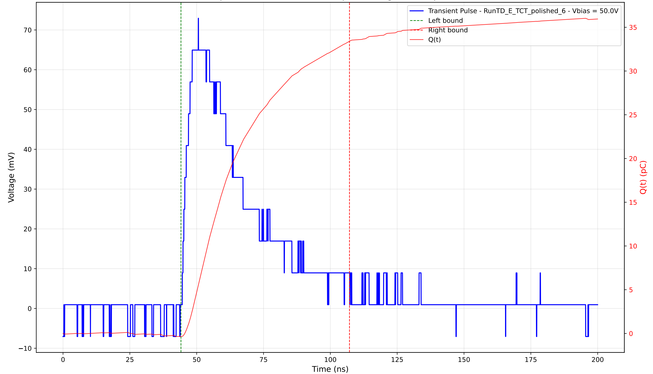
Transient Pulse - Sample: 4003 - Position: 205.0 \mu\text{m} - Charge: 33.76 pC - Rise Time: 5.98 ns
