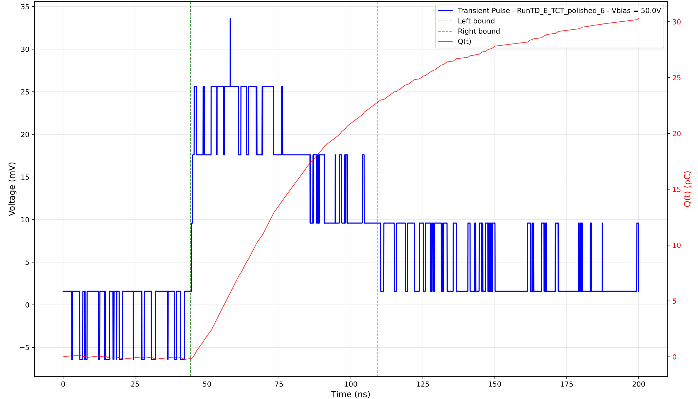
Transient Pulse - Sample: 4003 - Position: 215.0 \mu\text{m} - Charge: 22.97 pC - Rise Time: 13.44 ns
