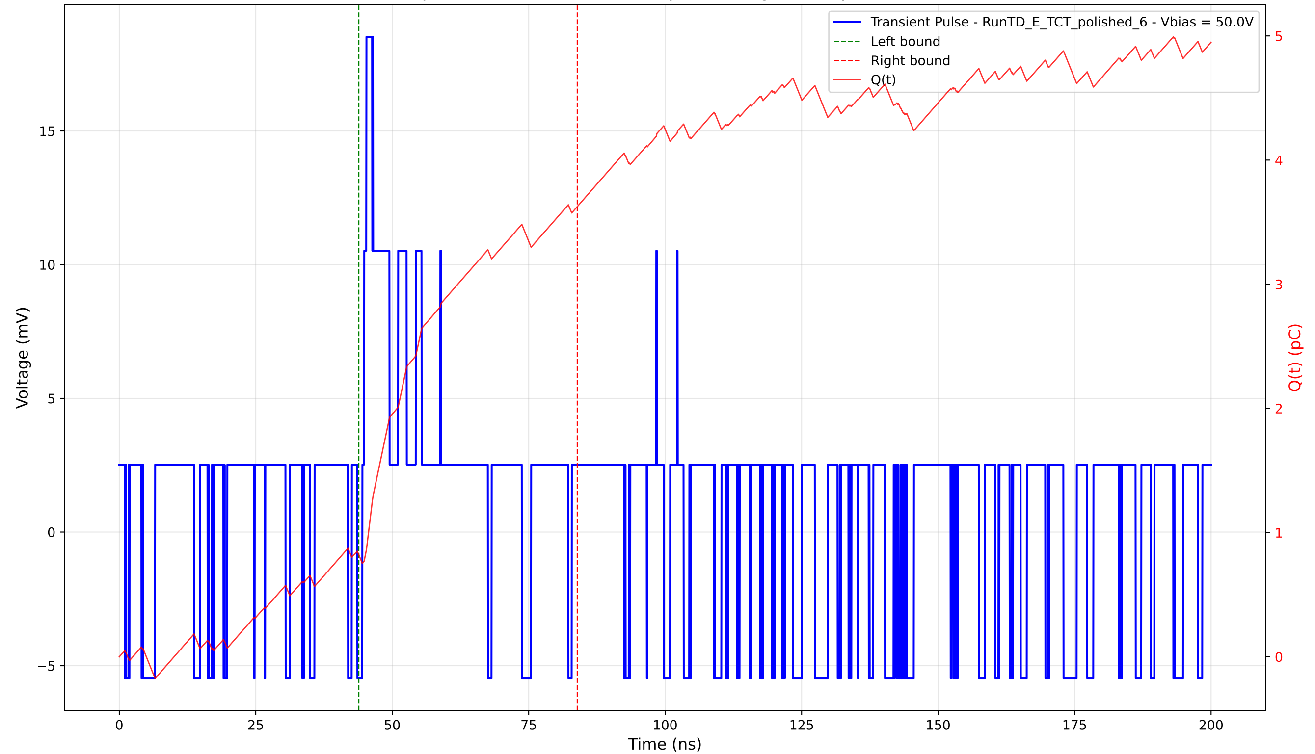
Transient Pulse - Sample: 4003 - Position: 310.0 \mu\text{m} - Charge: 2.80 pC - Rise Time: 0.00 ns (N/A)
