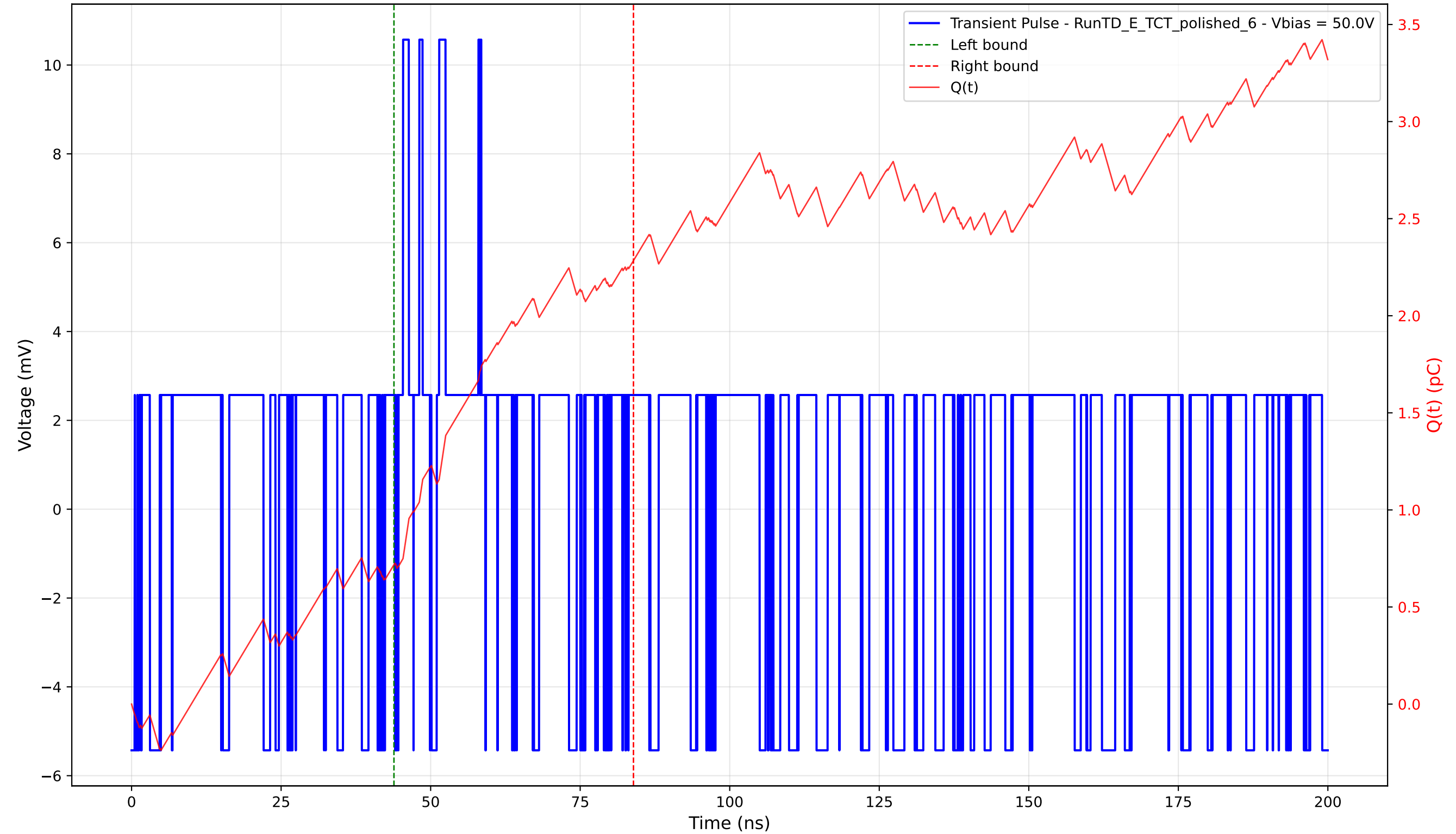
Transient Pulse - Sample: 4003 - Position: 10.0 \mu\text{m} - Charge: 1.56 pC - Rise Time: 0.00 ns (N/A)
