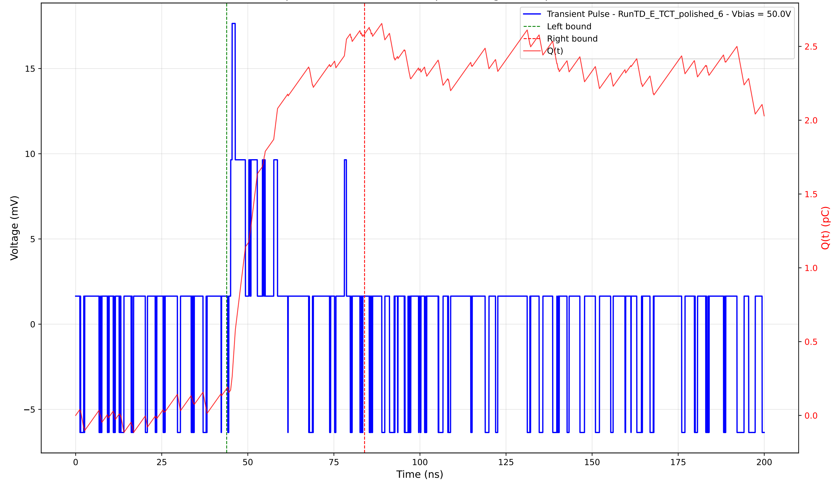
Transient Pulse - Sample: 4003 - Position: 40.0 \mu\text{m} - Charge: 2.40 pC - Rise Time: 0.44 ns
