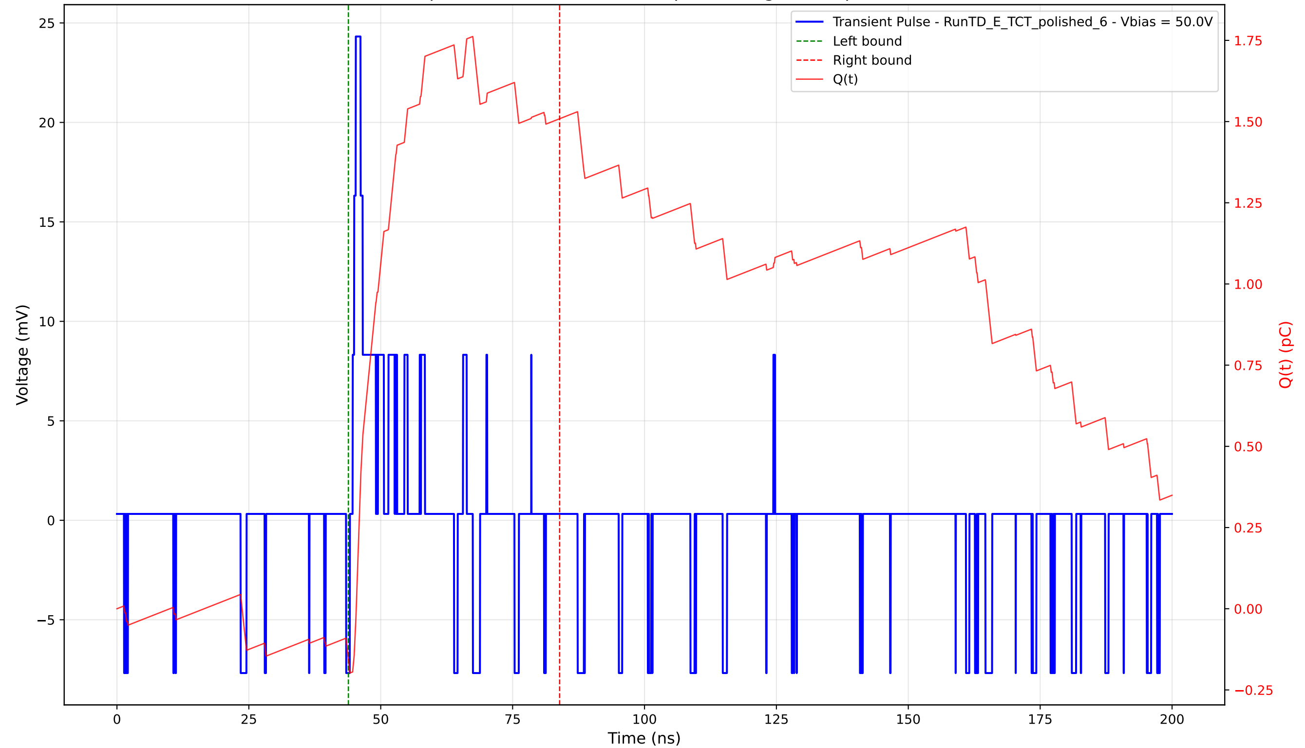
Transient Pulse - Sample: 4003 - Position: 400.0 \mu\text{m} - Charge: 1.67 pC - Rise Time: 0.59 ns
