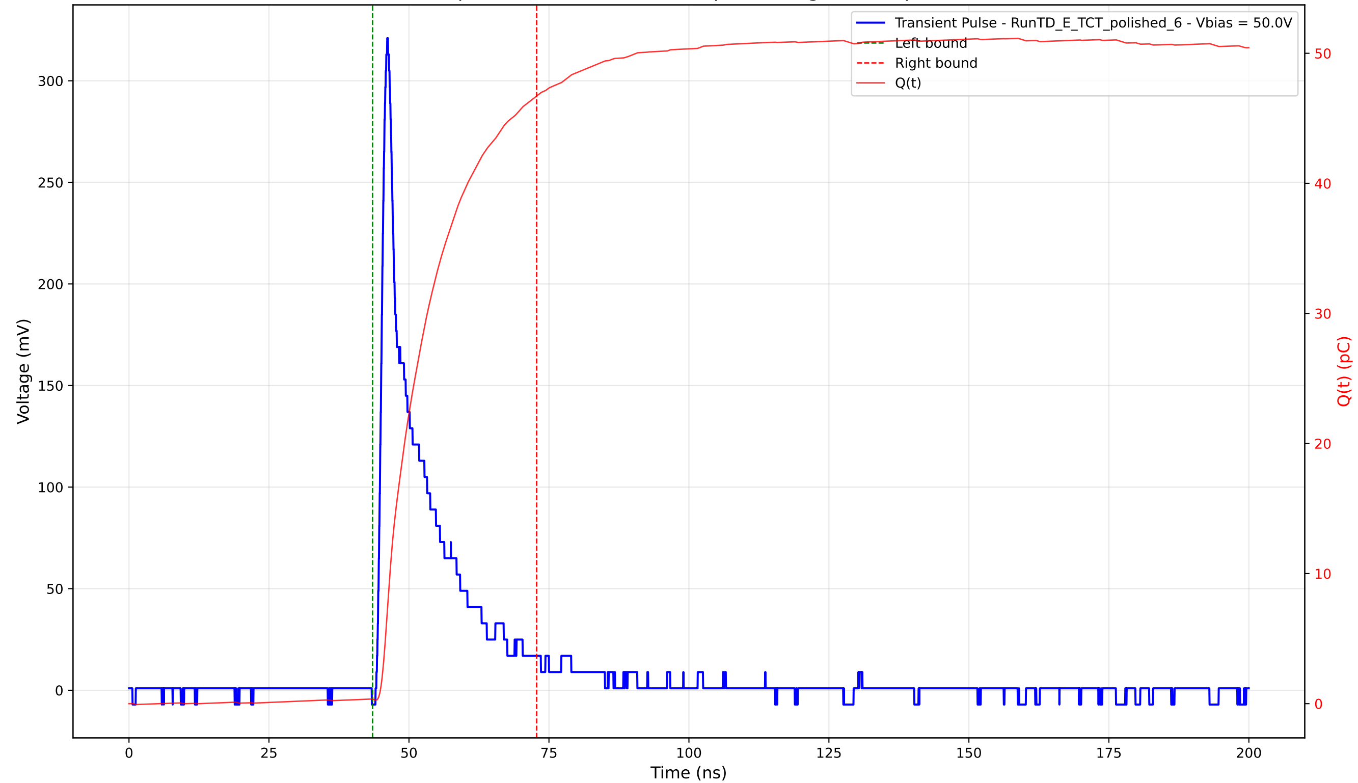
Transient Pulse - Sample: 4003 - Position: 155.0 \mu\text{m} - Charge: 46.38 pC - Rise Time: 1.28 ns
