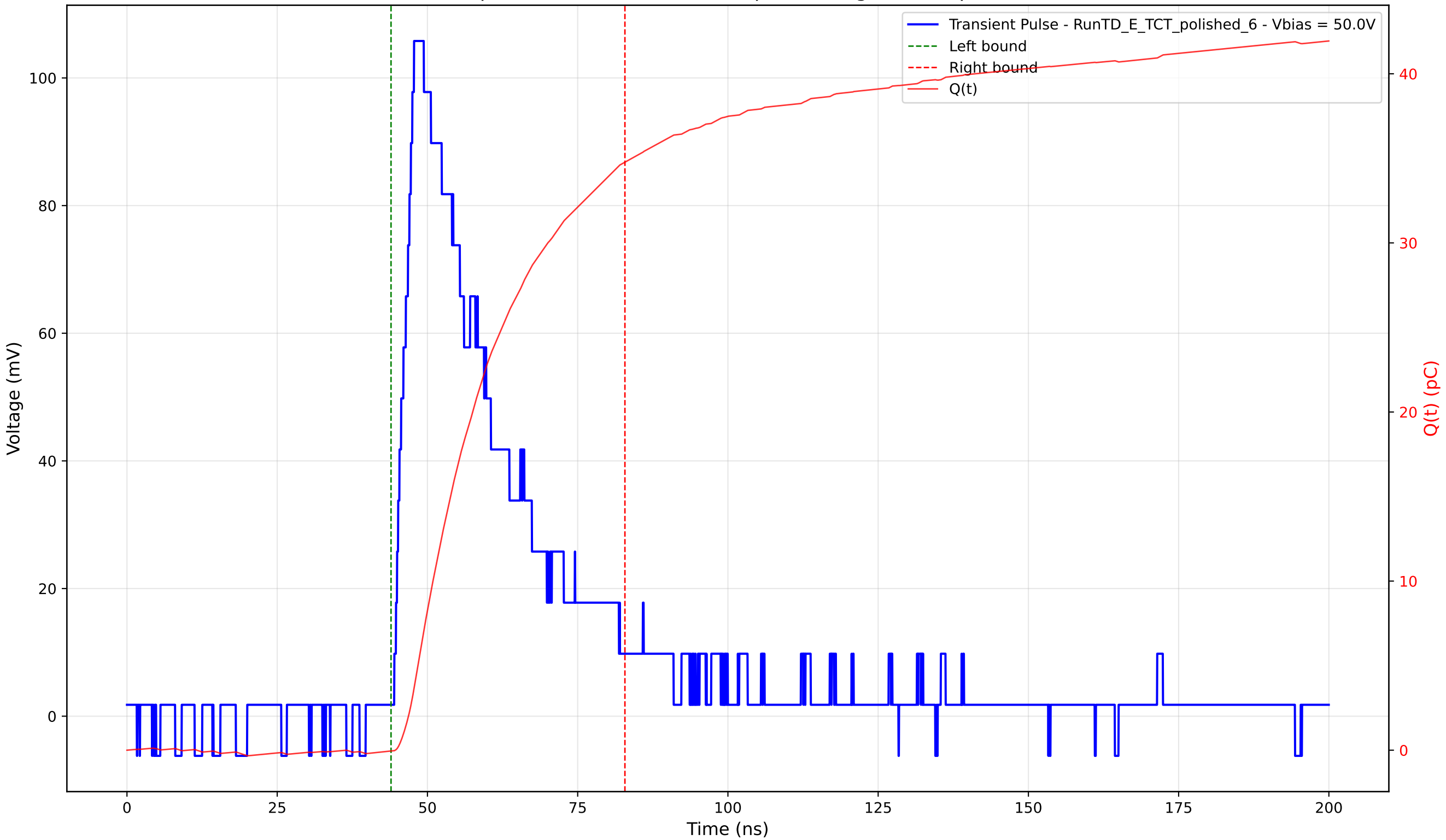
Transient Pulse - Sample: 4003 - Position: 200.0 \mu\text{m} - Charge: 34.82 pC - Rise Time: 2.74 ns
