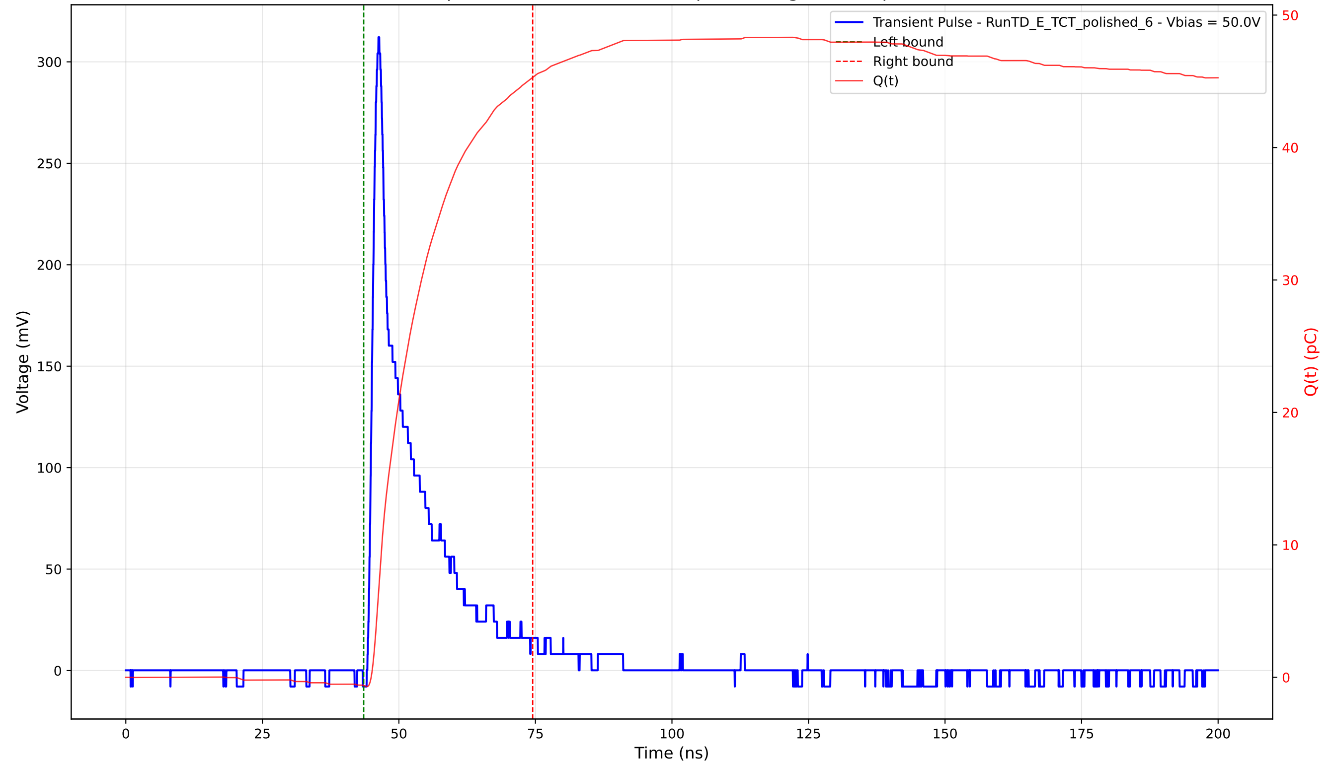
Transient Pulse - Sample: 4003 - Position: 160.0 \mu\text{m} - Charge: 45.90 pC - Rise Time: 1.40 ns
