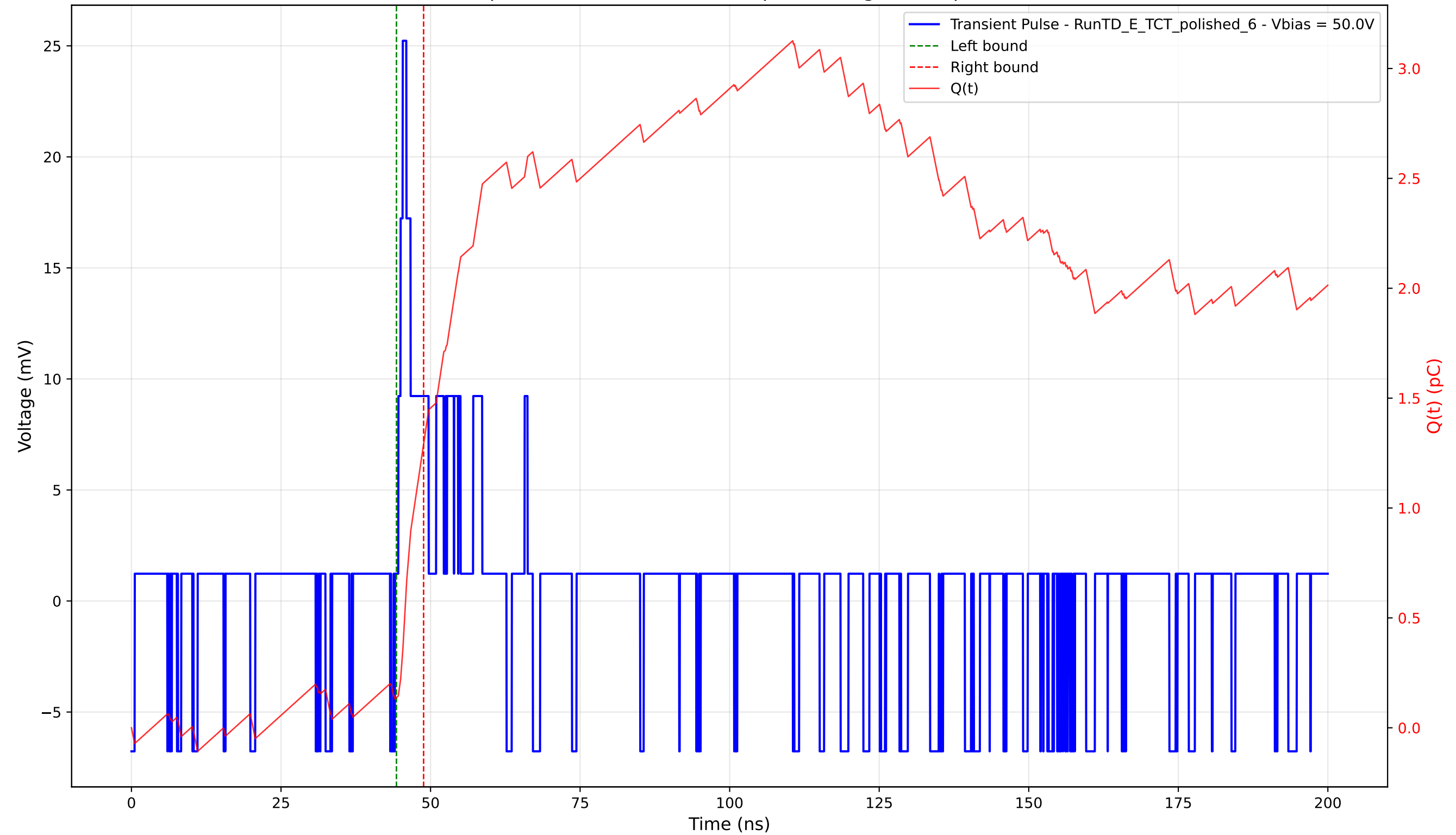
Transient Pulse - Sample: 4003 - Position: 395.0 \mu\text{m} - Charge: 1.16 pC - Rise Time: 0.74 ns
