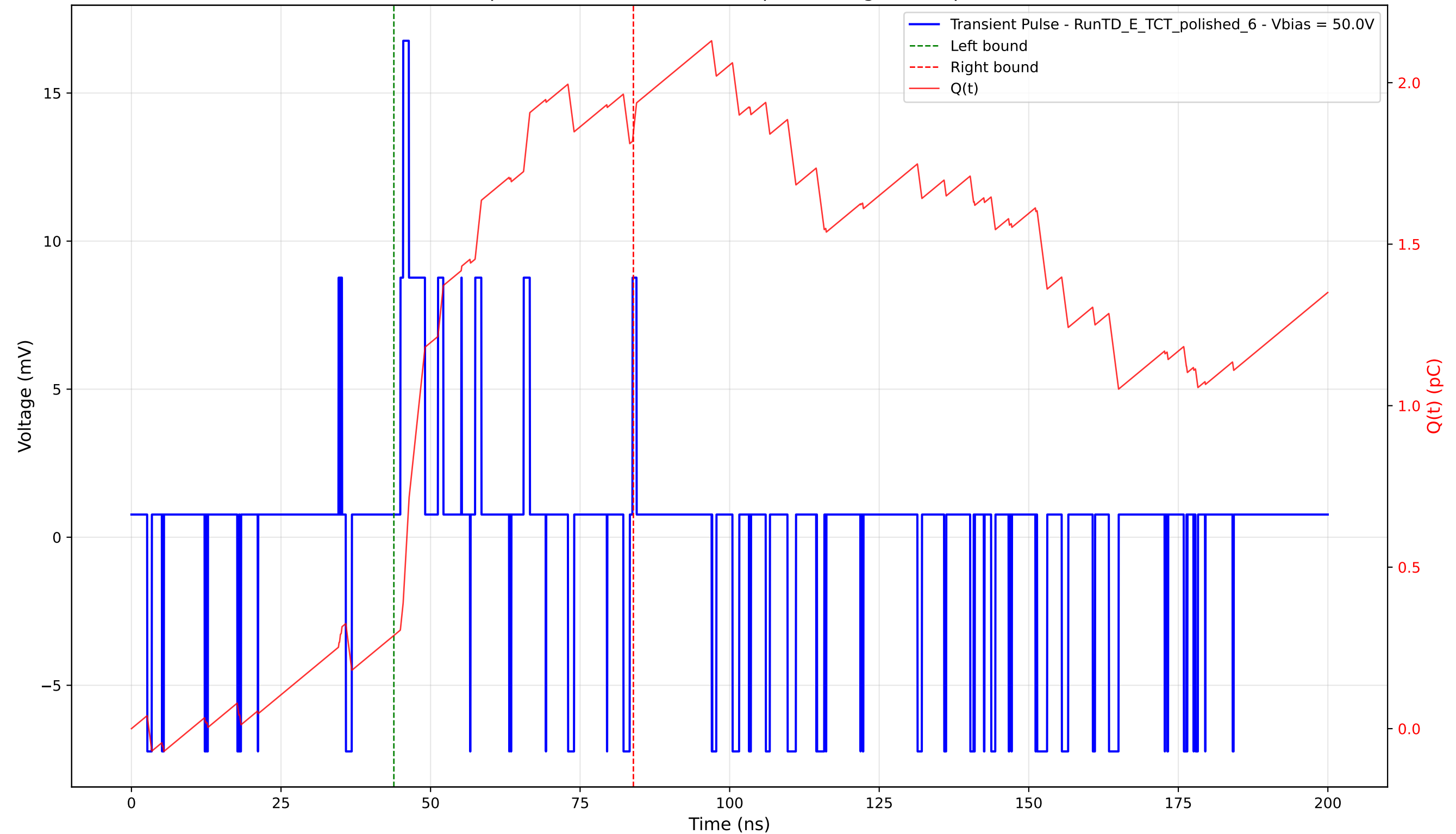
Transient Pulse - Sample: 4003 - Position: 350.0 \mu\text{m} - Charge: 1.56 pC - Rise Time: 0.48 ns
