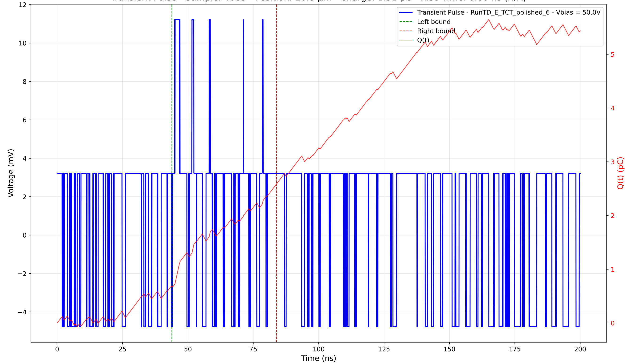
Transient Pulse - Sample: 4003 - Position: 20.0 \mu\text{m} - Charge: 1.91 pC - Rise Time: 0.00 ns (N/A)
