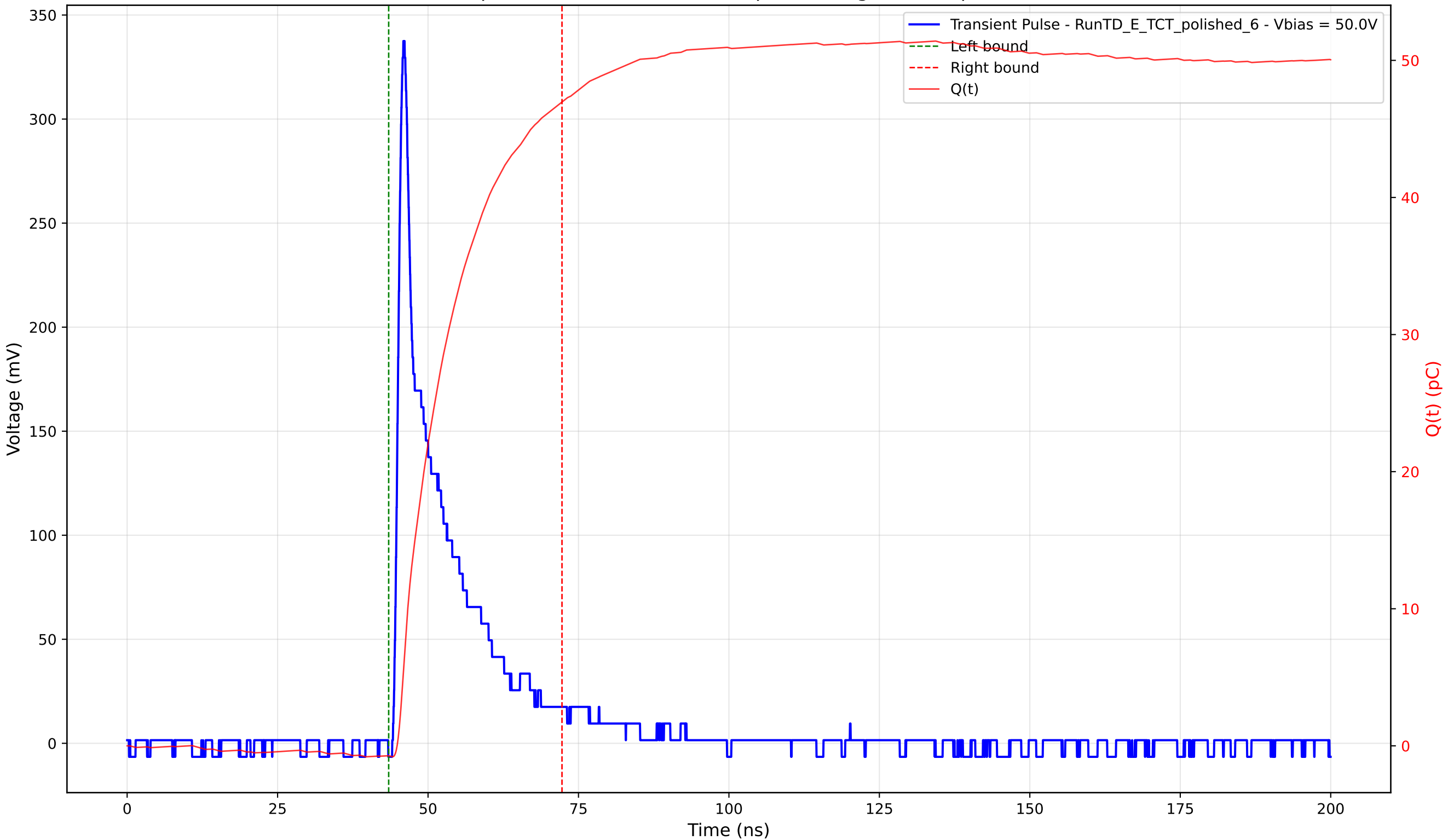
Transient Pulse - Sample: 4003 - Position: 145.0 \mu\text{m} - Charge: 47.70 pC - Rise Time: 1.14 ns
