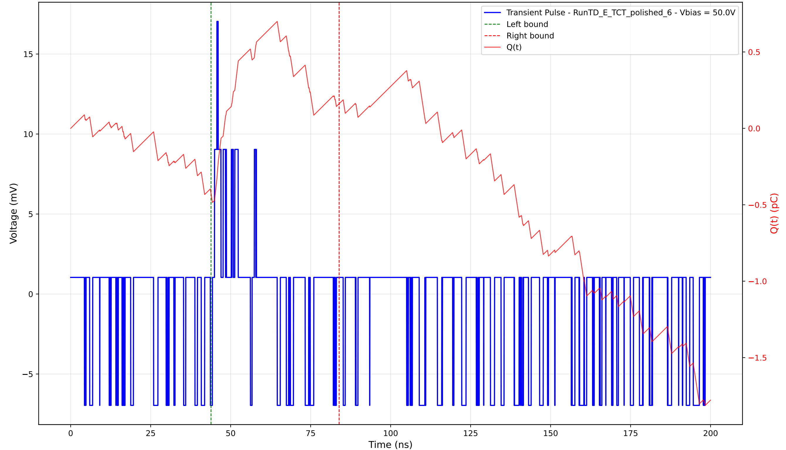
Transient Pulse - Sample: 4003 - Position: 355.0 \mu\text{m} - Charge: 0.59 pC - Rise Time: 0.76 ns
