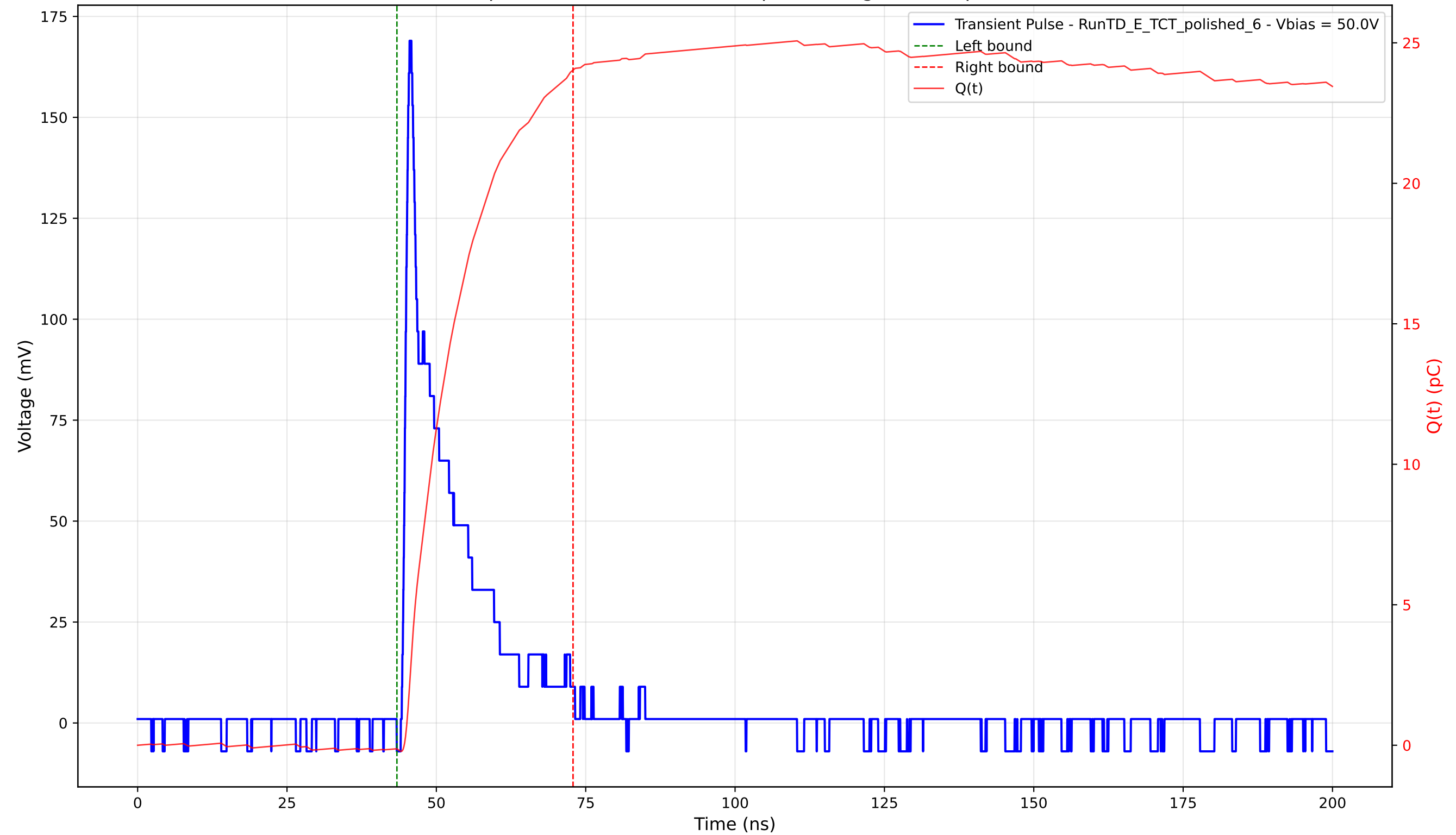
Transient Pulse - Sample: 4003 - Position: 100.0 \mu\text{m} - Charge: 24.16 pC - Rise Time: 0.98 ns
