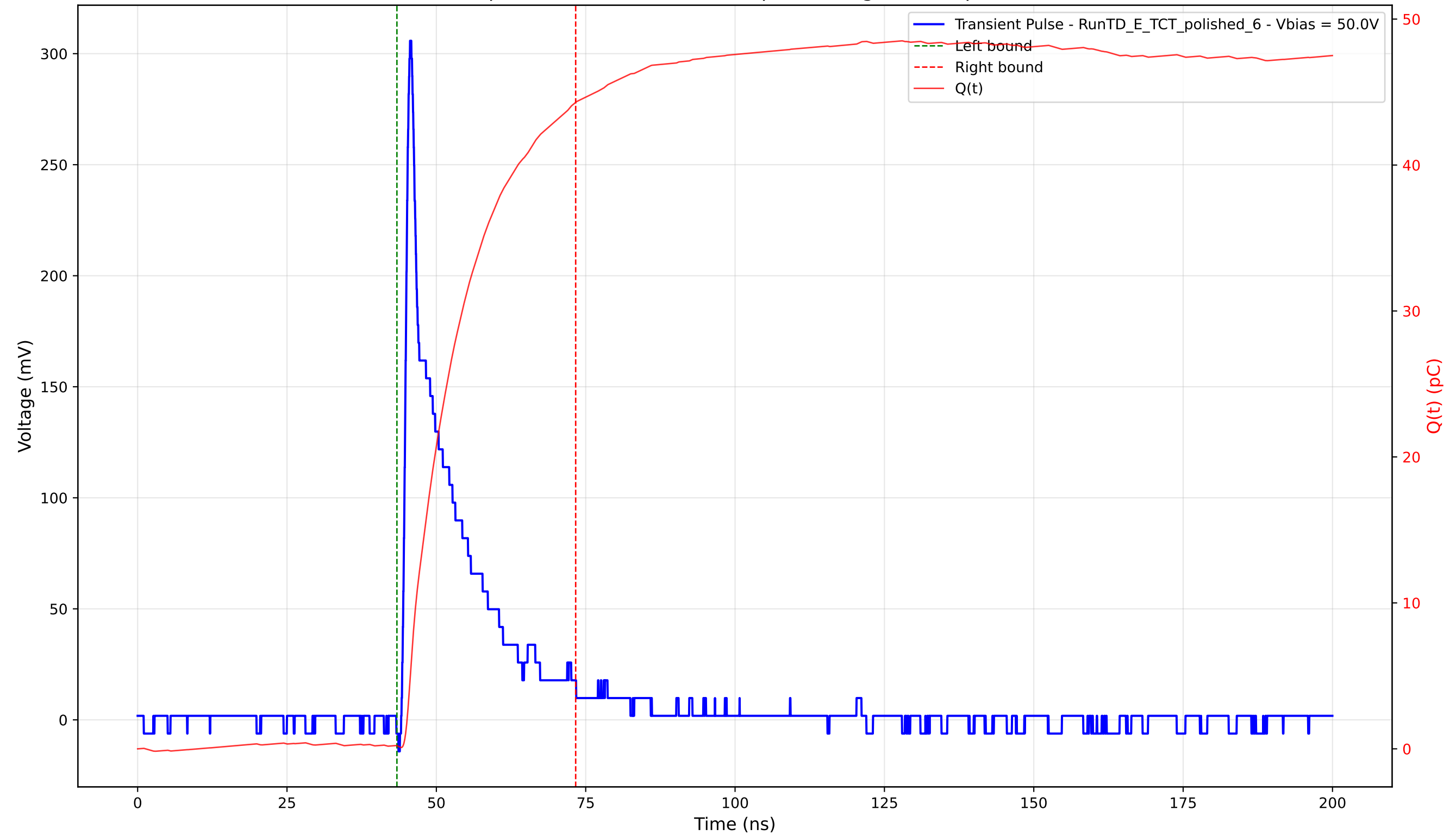
Transient Pulse - Sample: 4003 - Position: 115.0 \mu\text{m} - Charge: 44.09 pC - Rise Time: 1.01 ns
