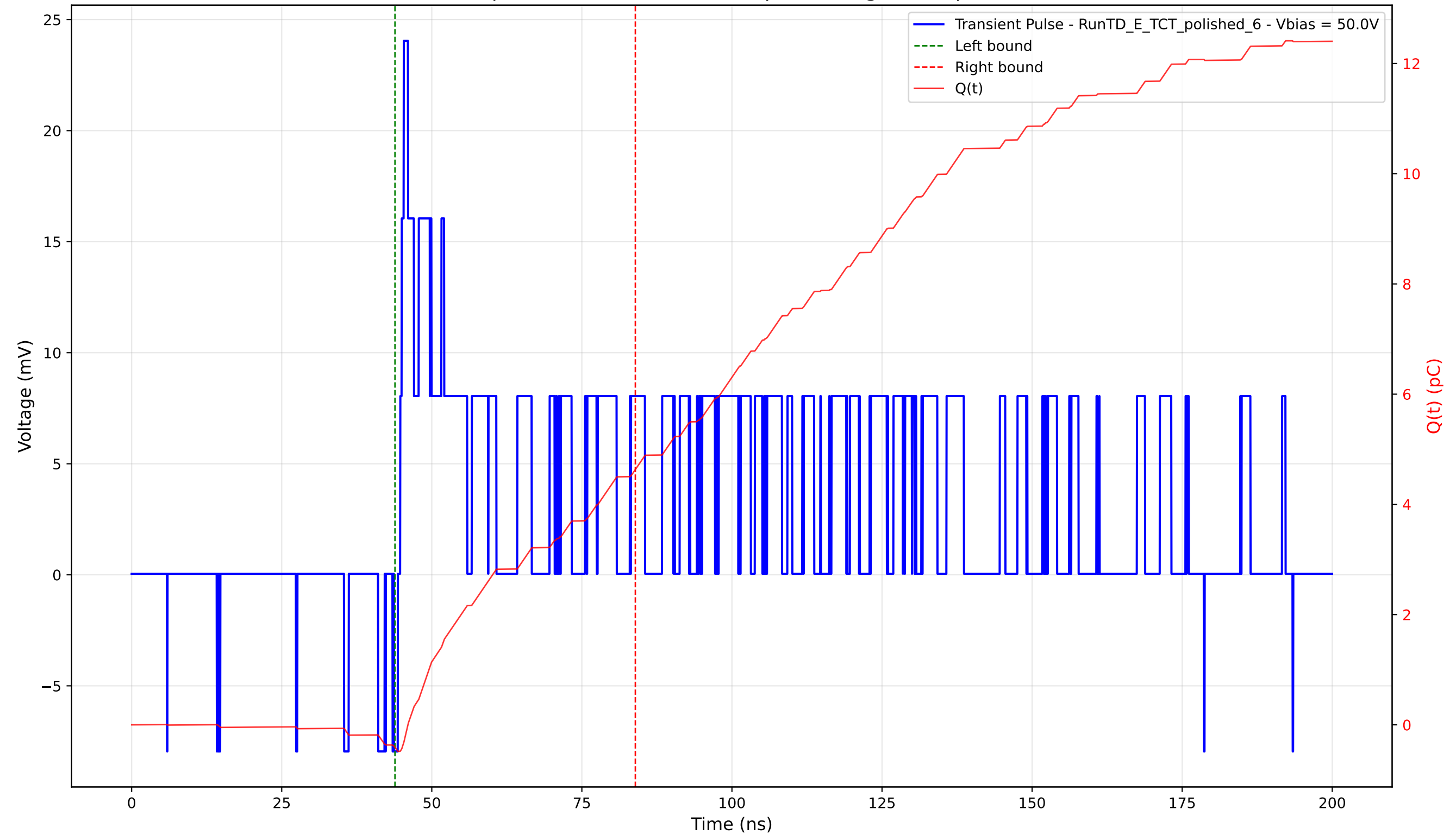
Transient Pulse - Sample: 4003 - Position: 235.0 \mu\text{m} - Charge: 5.04 pC - Rise Time: 0.59 ns
