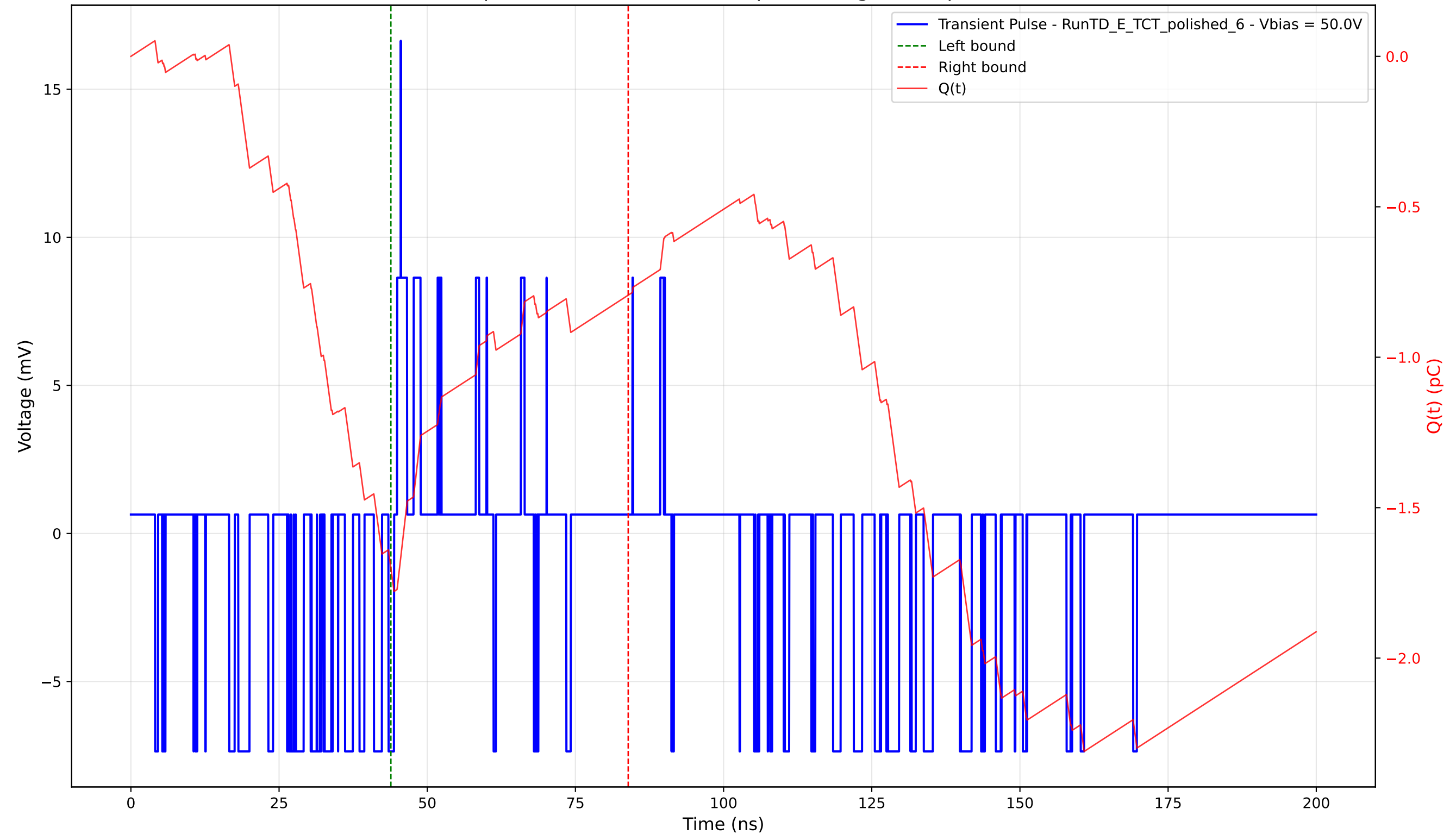
Transient Pulse - Sample: 4003 - Position: 340.0 \mu\text{m} - Charge: 0.91 pC - Rise Time: 0.64 ns
