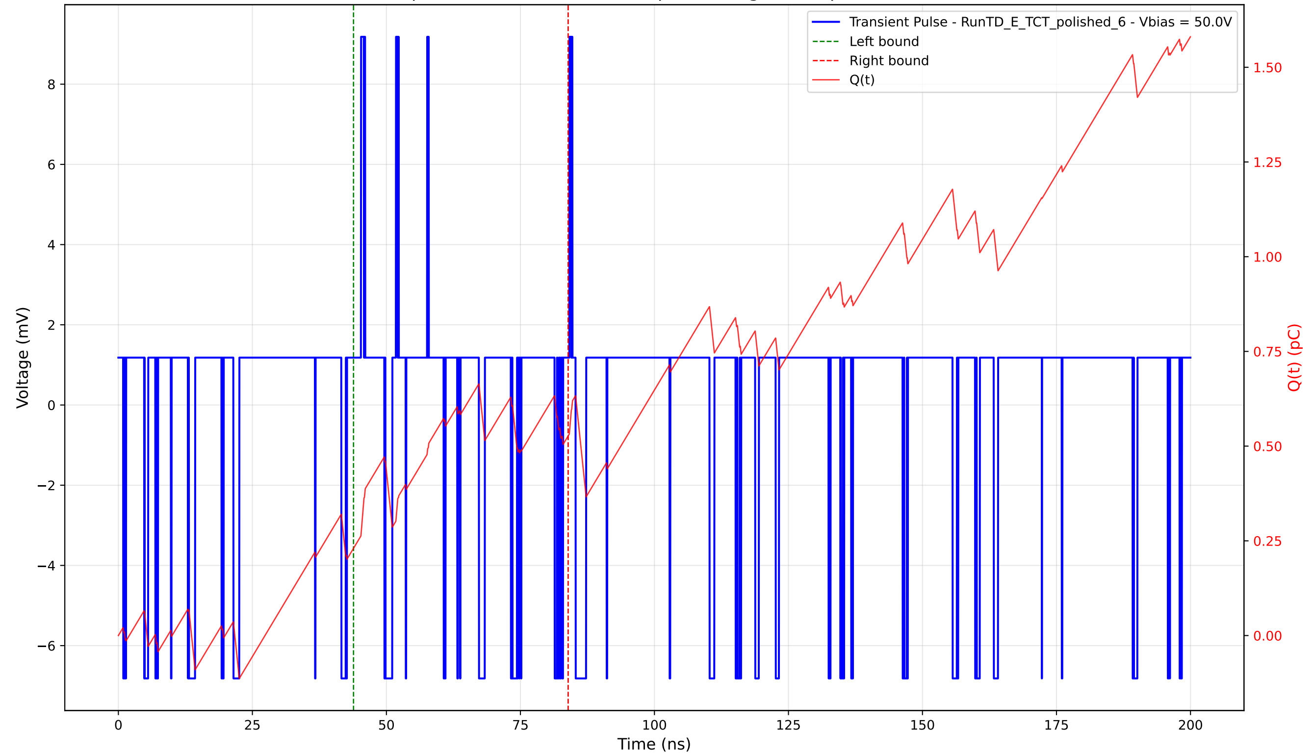
Transient Pulse - Sample: 4003 - Position: 425.0 \mu\text{m} - Charge: 0.30 pC - Rise Time: 0.00 ns (N/A)
