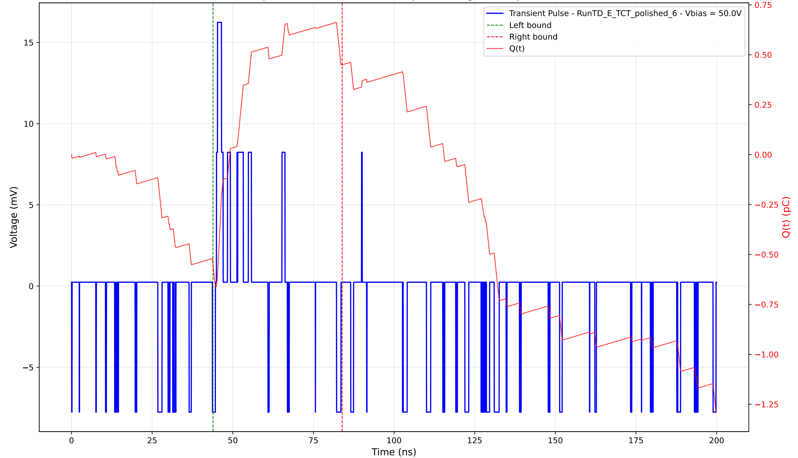
Transient Pulse - Sample: 4003 - Position: 405.0 \mu\text{m} - Charge: 1.00 pC - Rise Time: 0.34 ns
