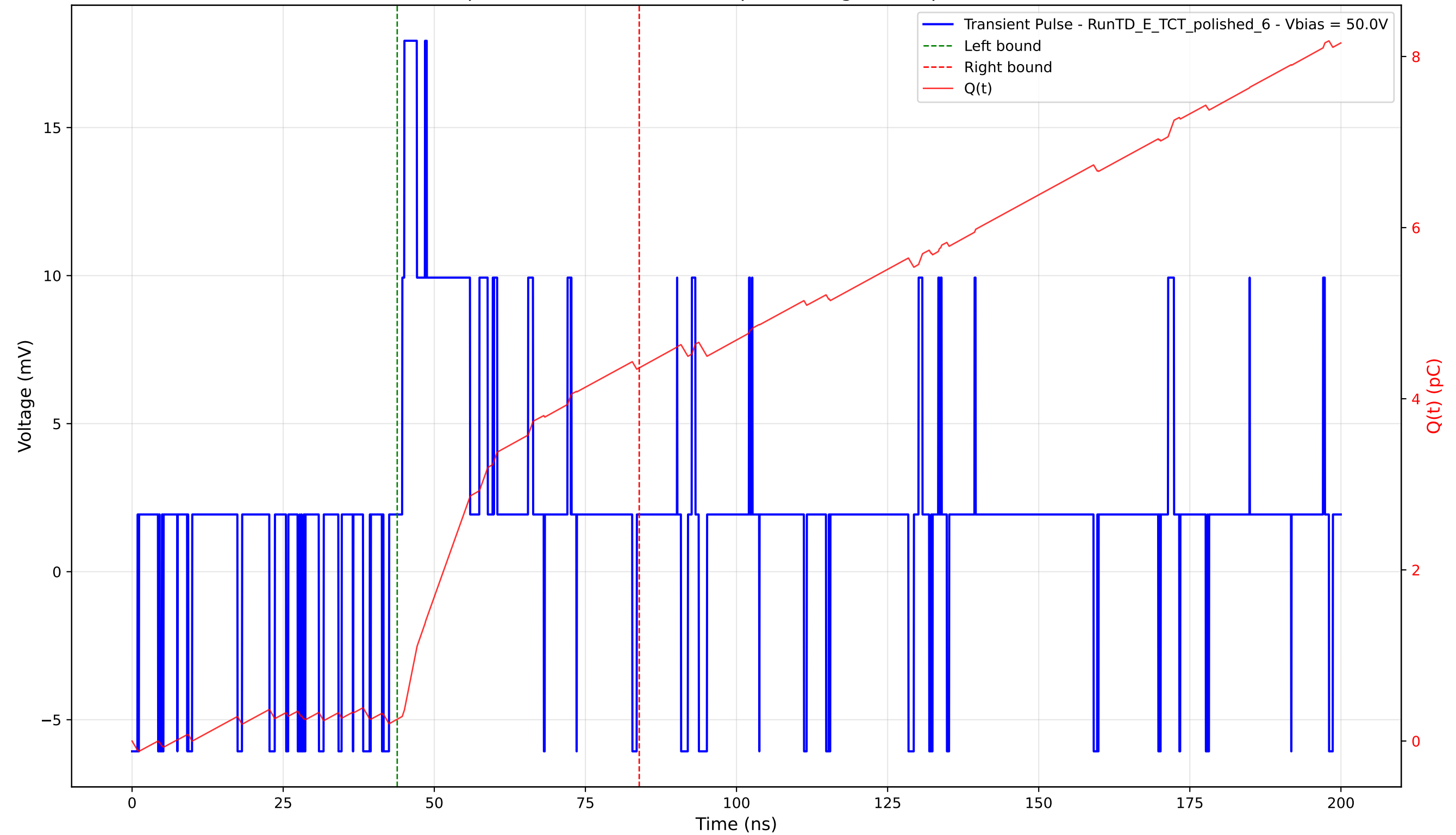
Transient Pulse - Sample: 4003 - Position: 255.0 \mu\text{m} - Charge: 4.11 pC - Rise Time: 0.00 ns (N/A)
