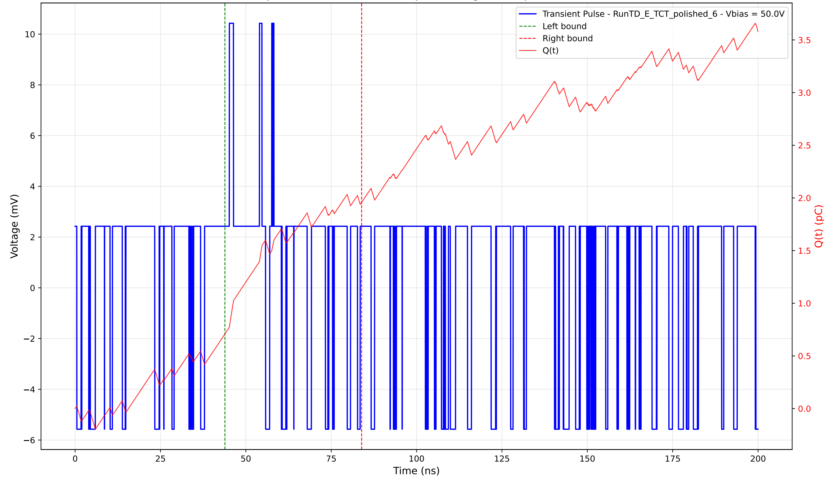
Transient Pulse - Sample: 4003 - Position: 15.0 \mu\text{m} - Charge: 1.25 pC - Rise Time: 0.00 ns (N/A)
