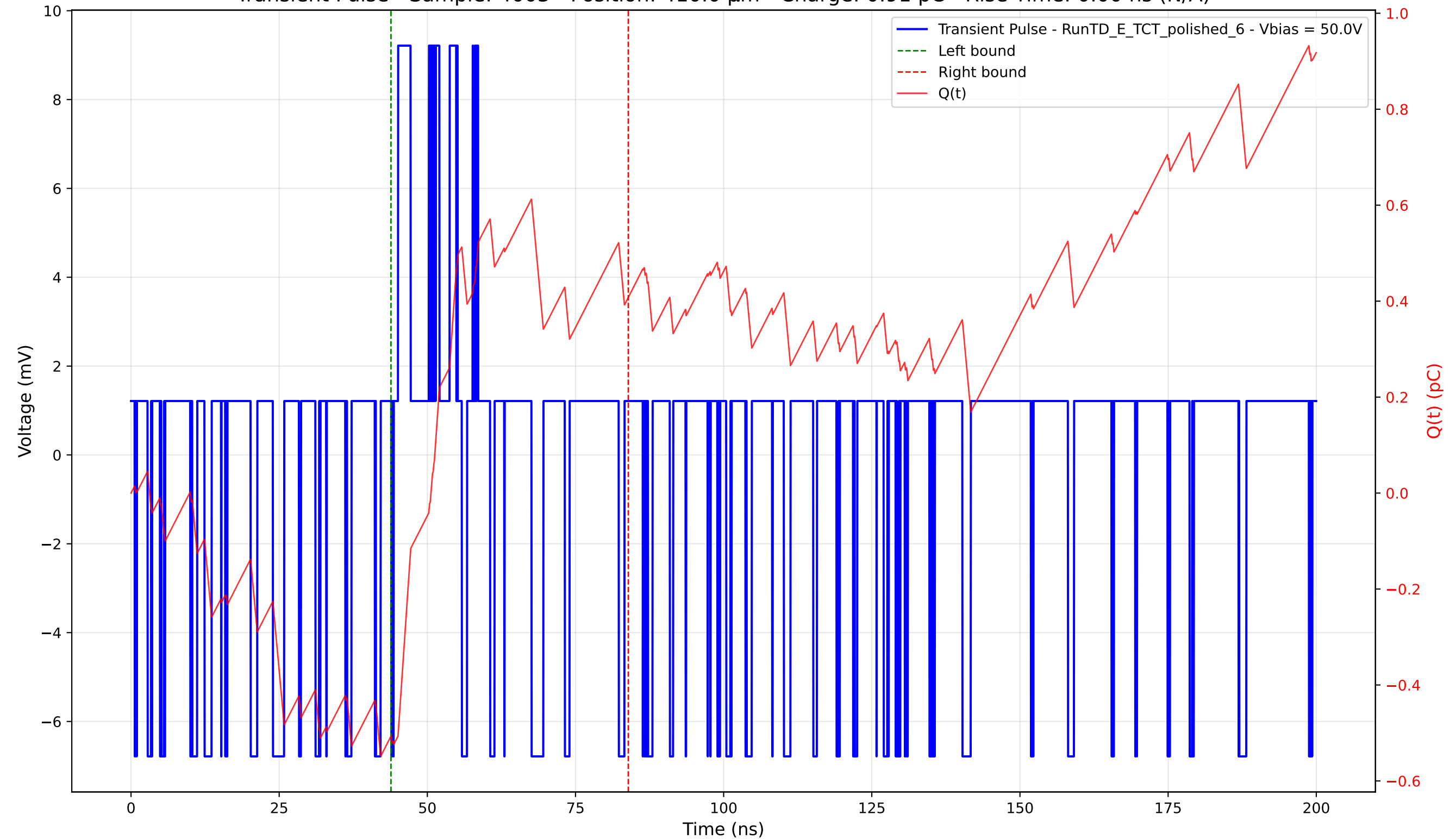
Transient Pulse - Sample: 4003 - Position: 410.0 \mu\text{m} - Charge: 0.91 pC - Rise Time: 0.00 ns (N/A)
