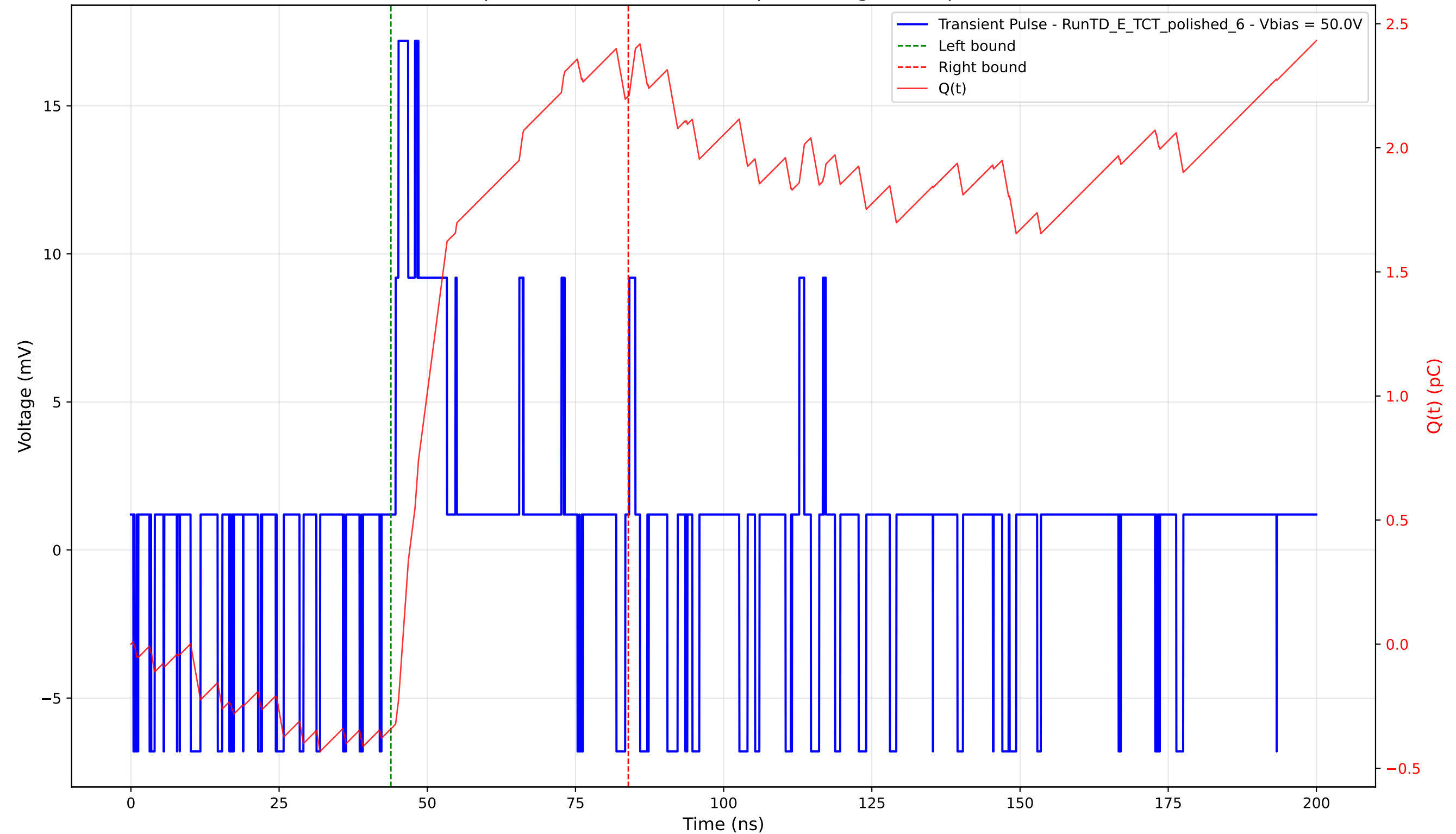
Transient Pulse - Sample: 4003 - Position: 295.0 \mu\text{m} - Charge: 2.55 pC - Rise Time: 0.50 ns
