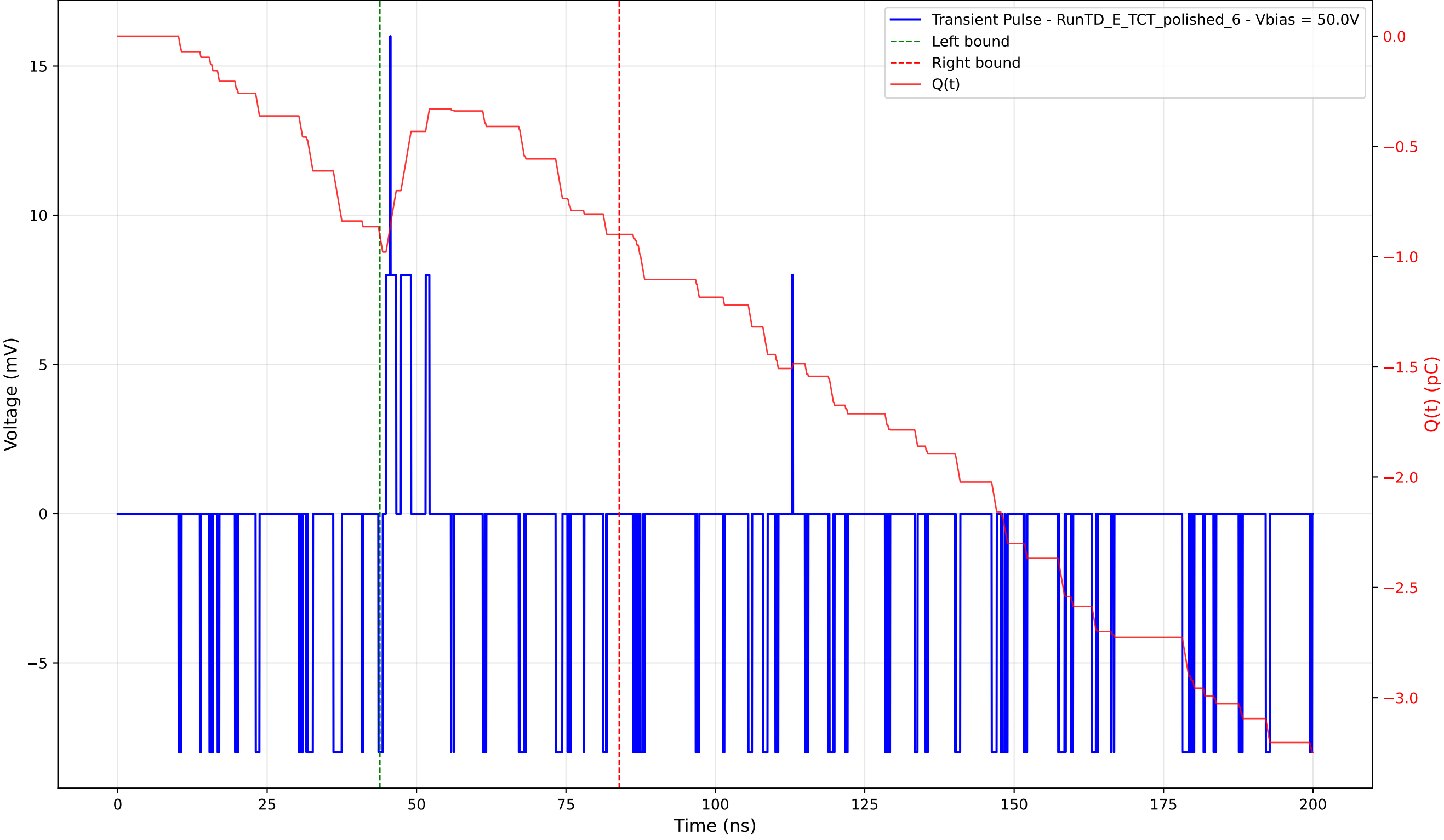
Transient Pulse - Sample: 4003 - Position: 30.0 \mu\text{m} - Charge: 0.01 pC - Rise Time: 0.72 ns
