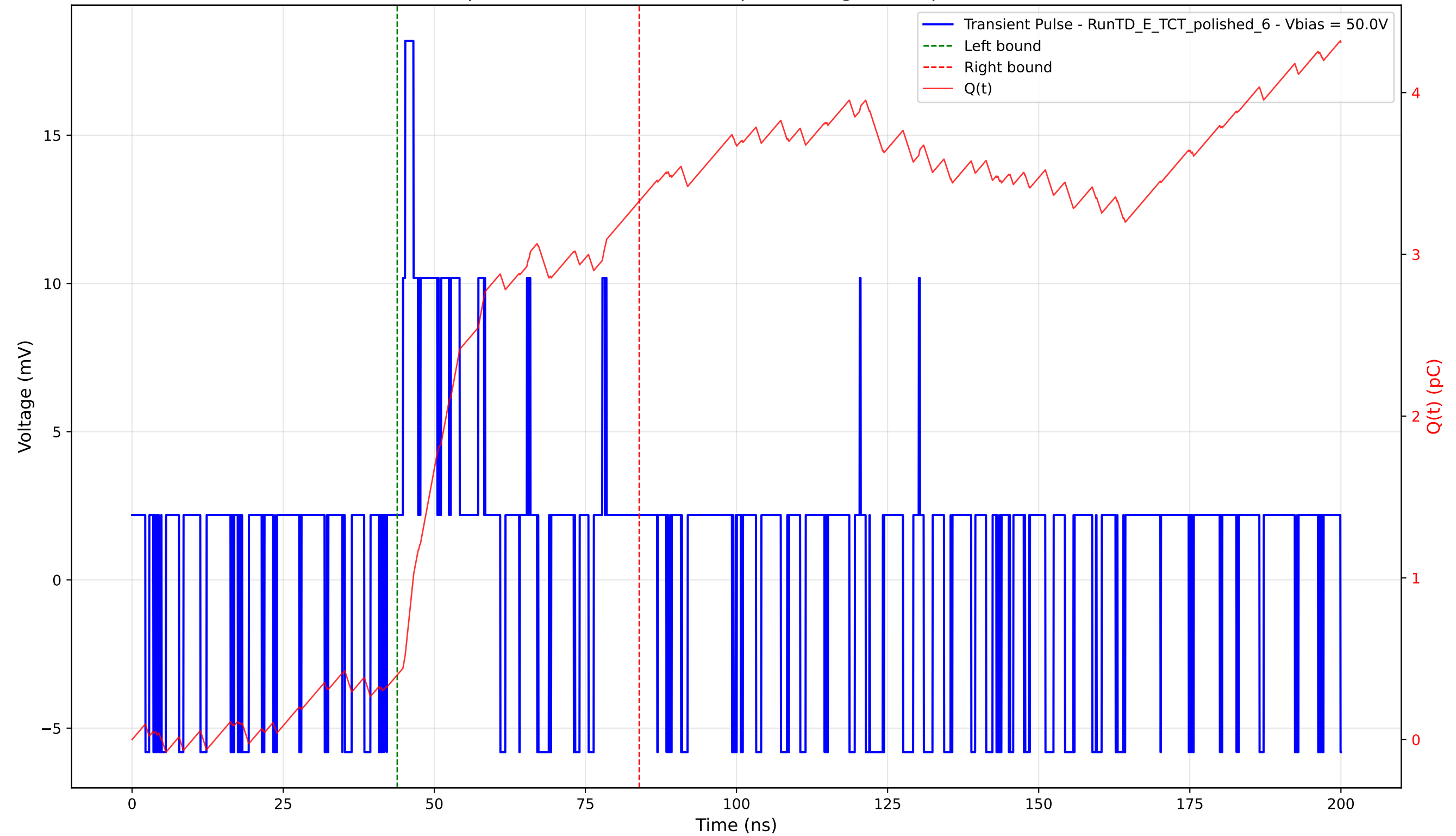
Transient Pulse - Sample: 4003 - Position: 305.0 \mu\text{m} - Charge: 2.93 pC - Rise Time: 0.00 ns (N/A)
