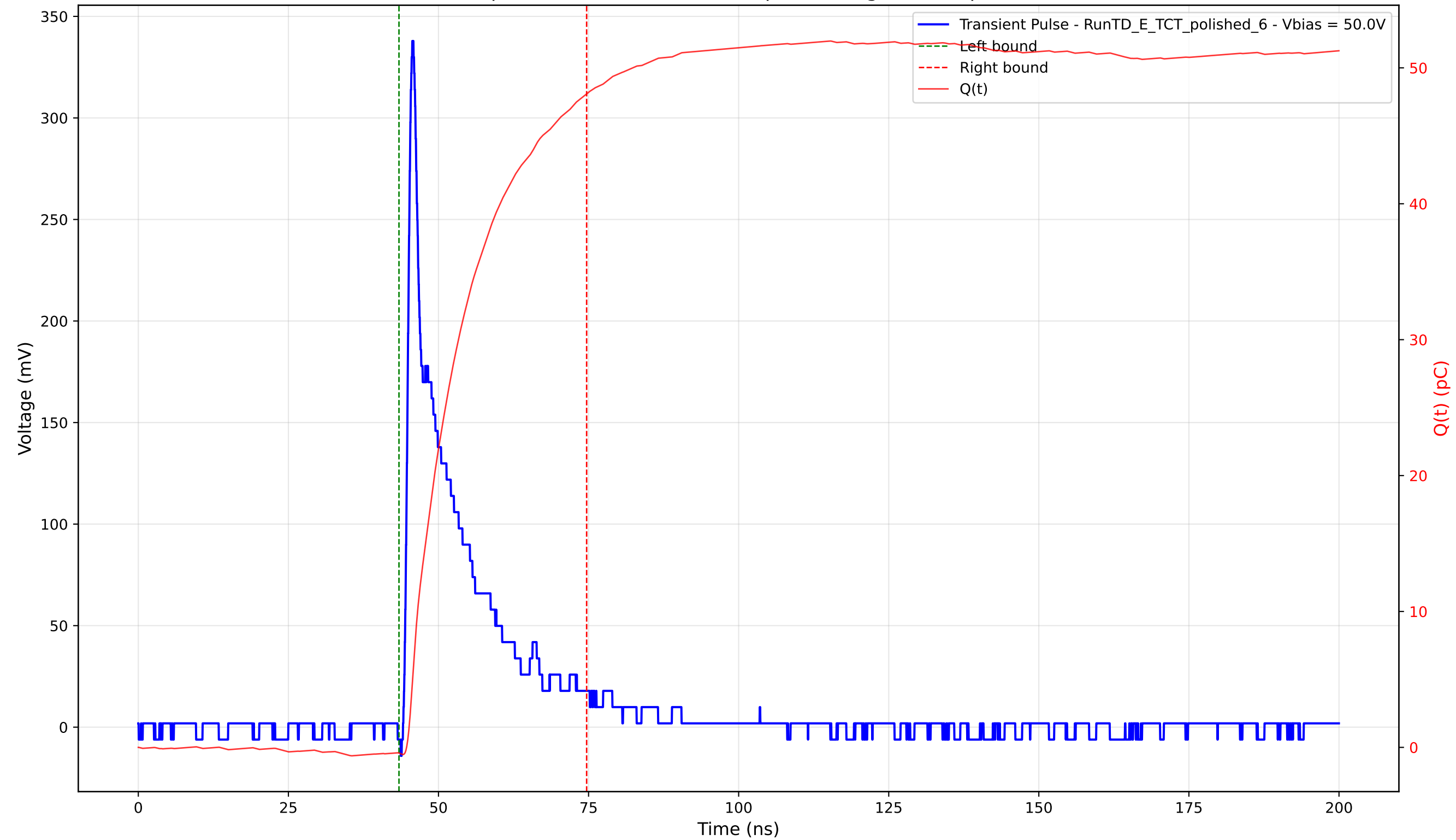
Transient Pulse - Sample: 4003 - Position: 120.0 \mu\text{m} - Charge: 48.52 pC - Rise Time: 1.00 ns
