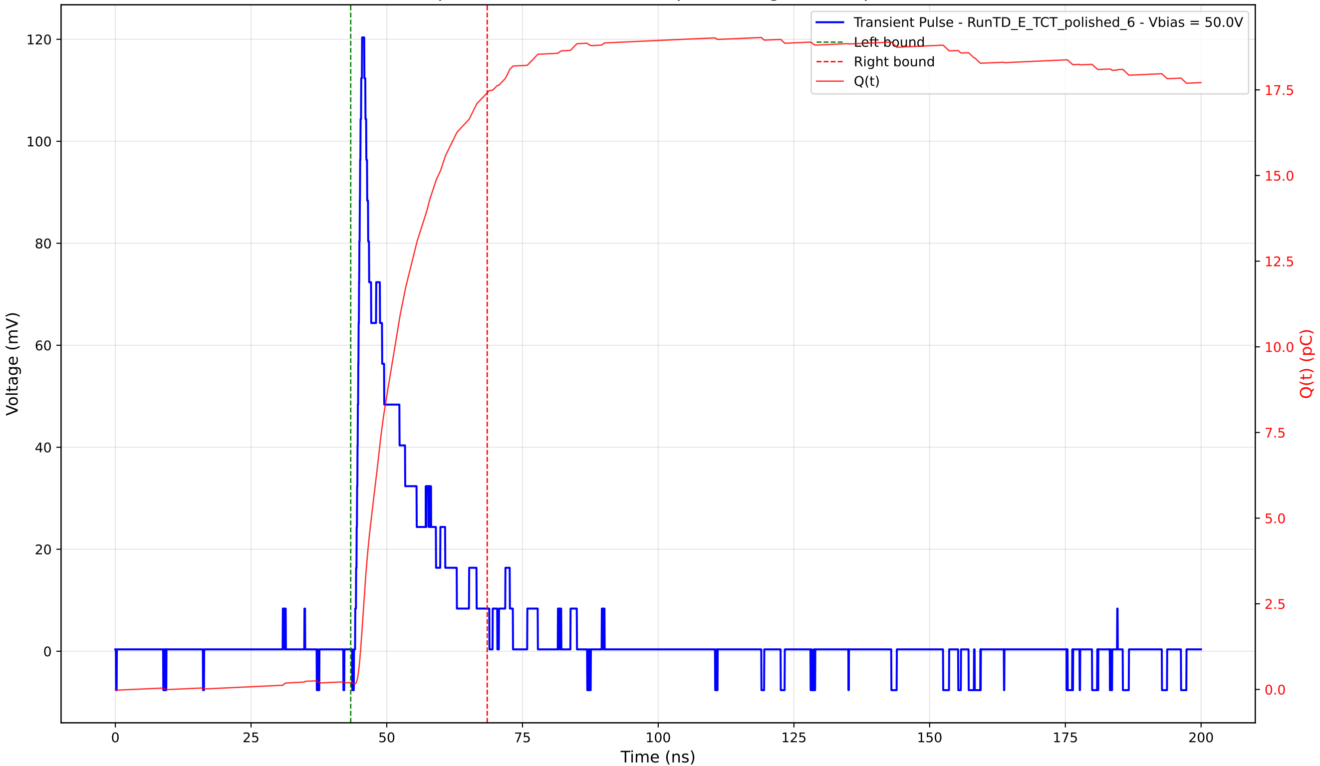
Transient Pulse - Sample: 4003 - Position: 95.0 \mu\text{m} - Charge: 17.21 pC - Rise Time: 0.95 ns
