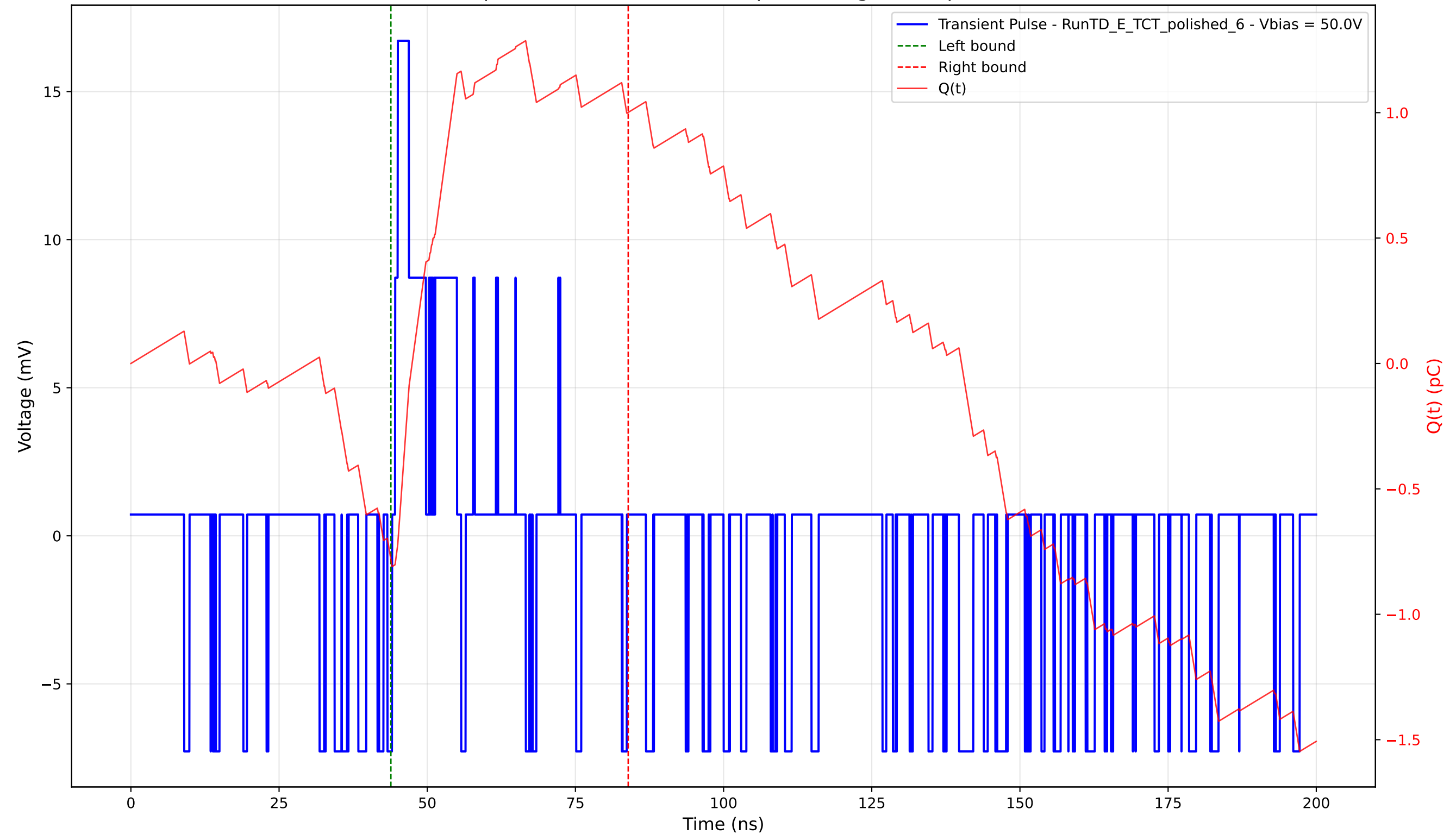
Transient Pulse - Sample: 4003 - Position: 380.0 \mu\text{m} - Charge: 1.79 pC - Rise Time: 0.46 ns
