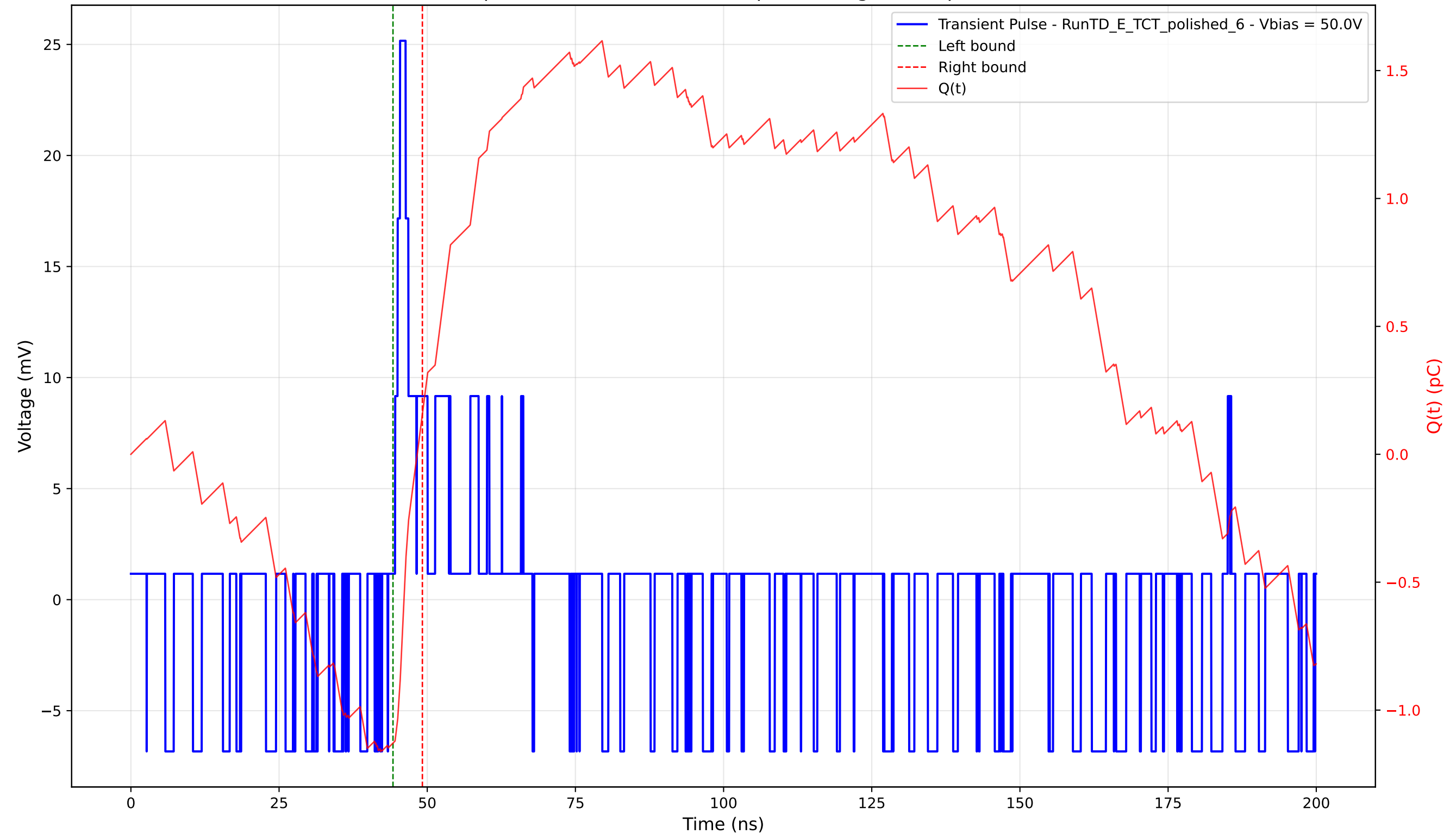
Transient Pulse - Sample: 4003 - Position: 385.0 \mu\text{m} - Charge: 1.29 pC - Rise Time: 0.84 ns
