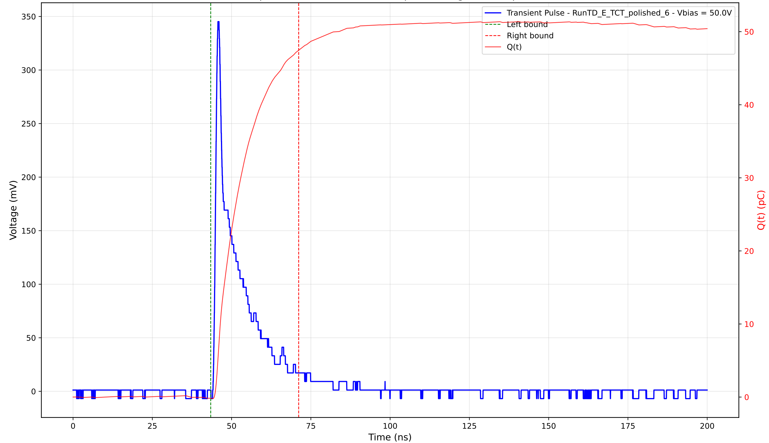
Transient Pulse - Sample: 4003 - Position: 135.0 \mu\text{m} - Charge: 47.61 pC - Rise Time: 1.06 ns
