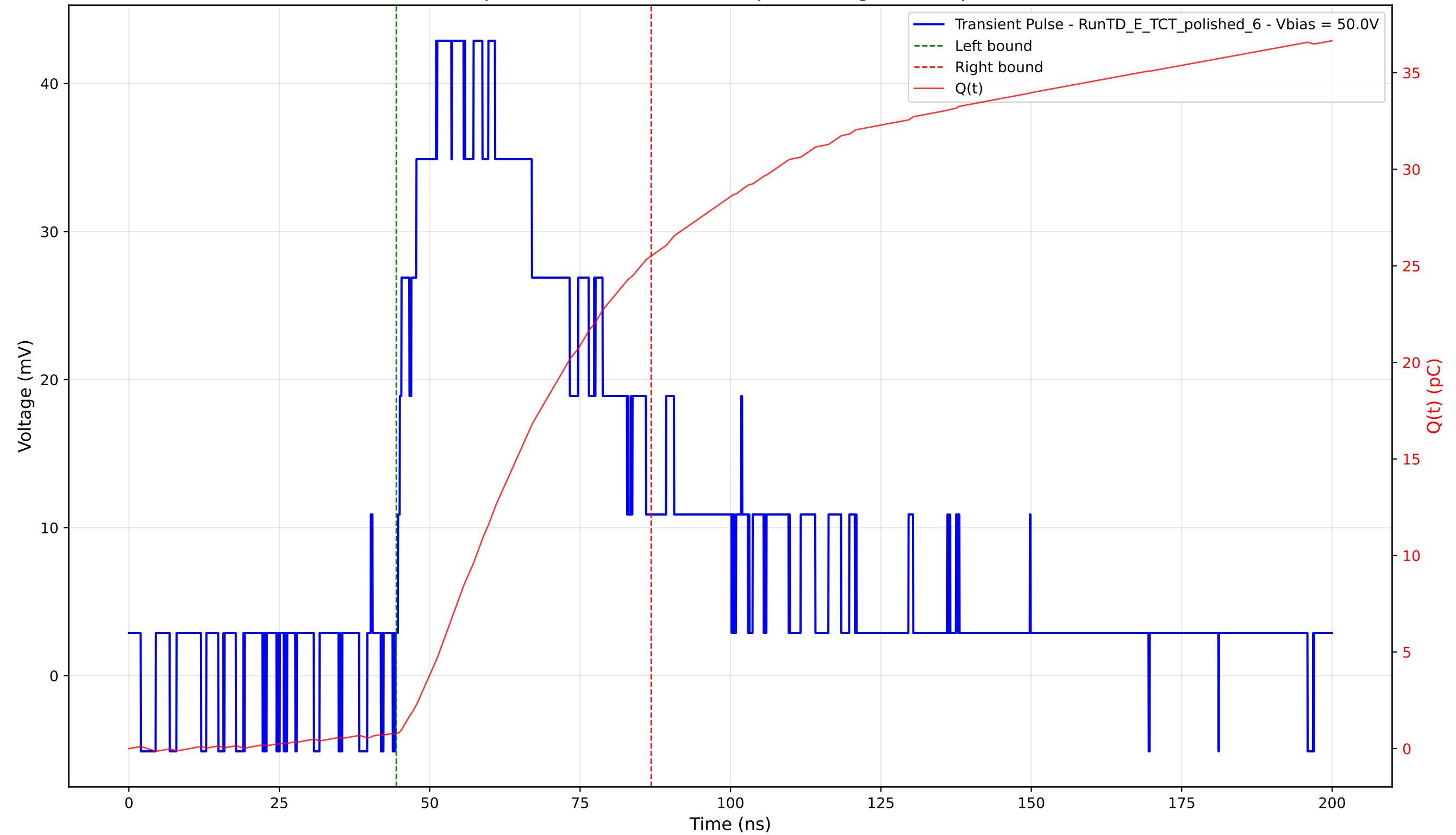
Transient Pulse - Sample: 4003 - Position: 210.0 \mu\text{m} - Charge: 24.73 pC - Rise Time: 6.36 ns
