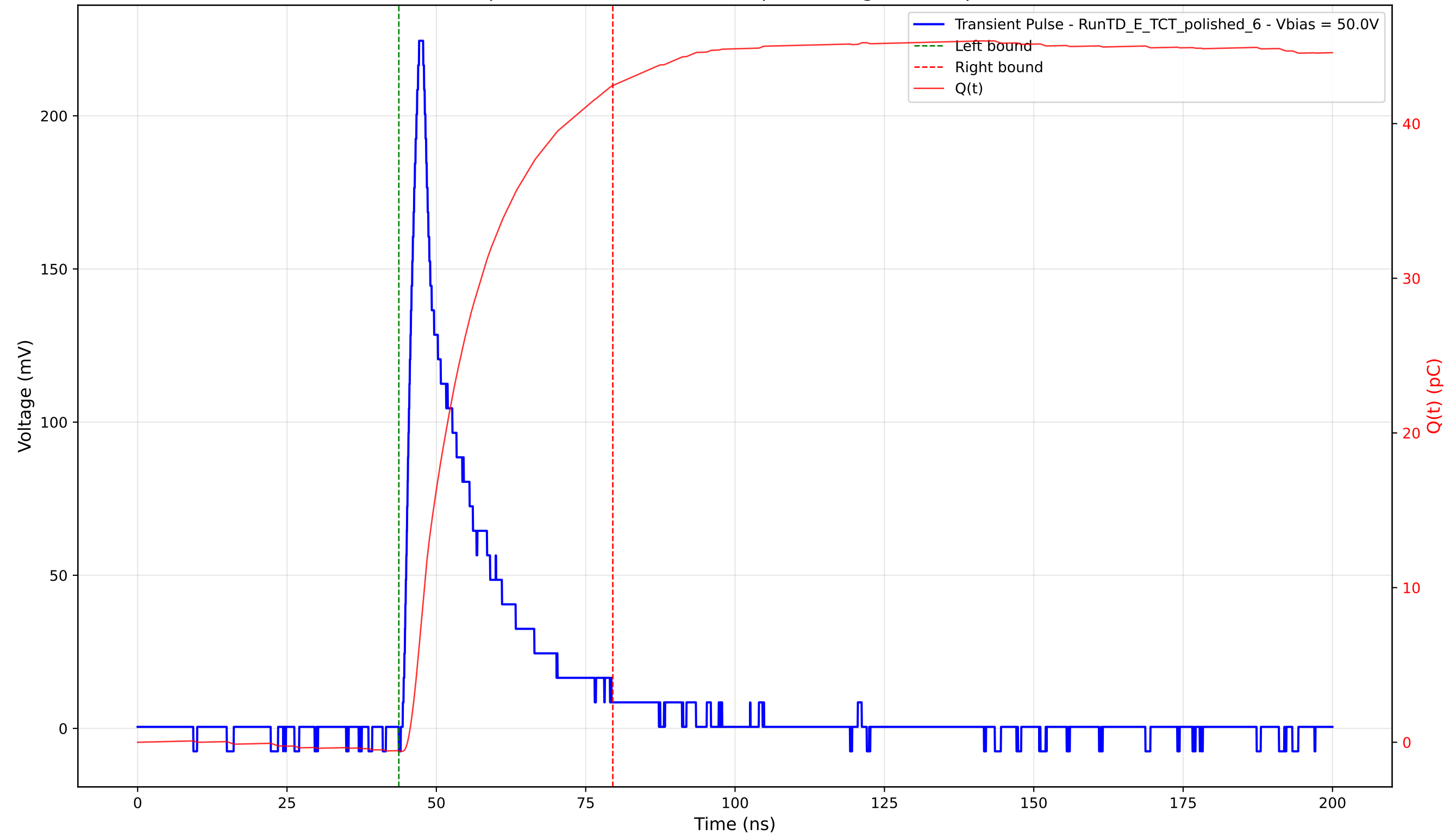
Transient Pulse - Sample: 4003 - Position: 185.0 \mu\text{m} - Charge: 43.00 pC - Rise Time: 2.15 ns
