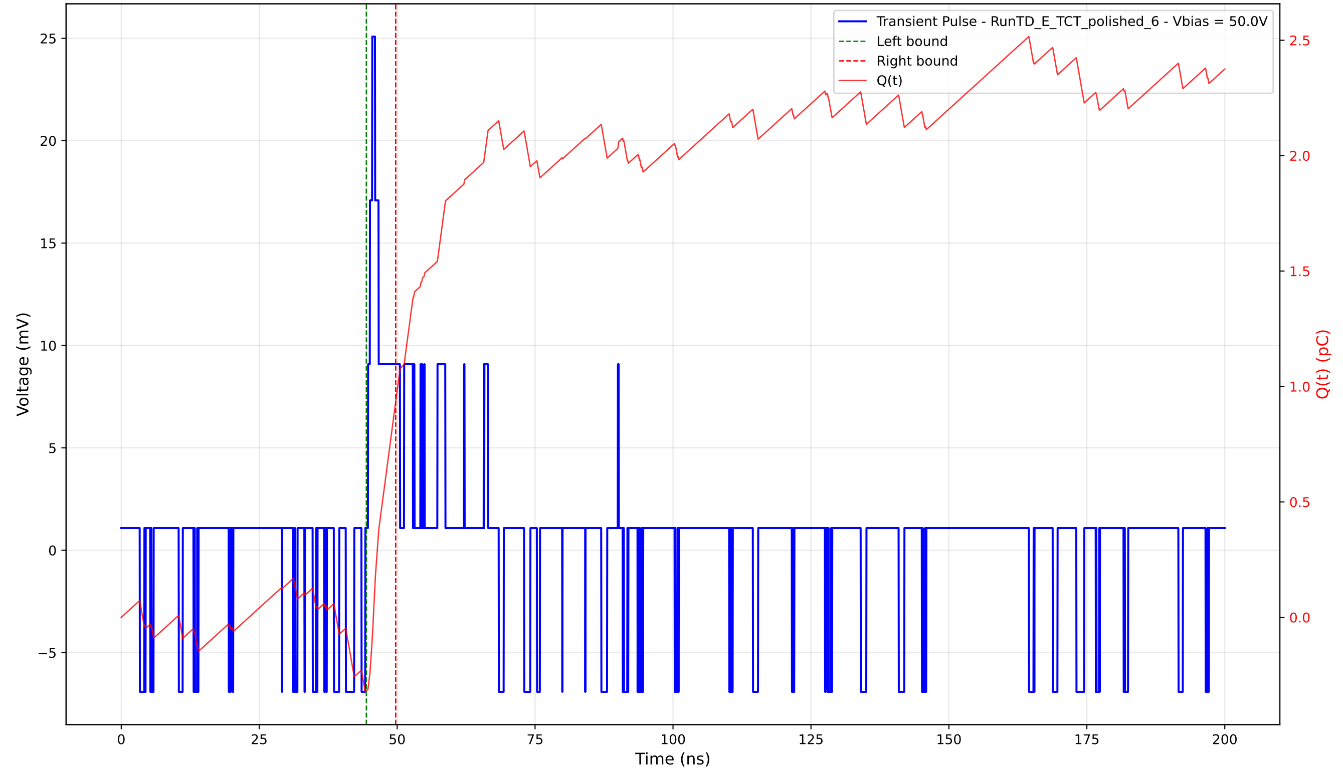
Transient Pulse - Sample: 4003 - Position: 275.0 \mu\text{m} - Charge: 1.26 pC - Rise Time: 0.78 ns
