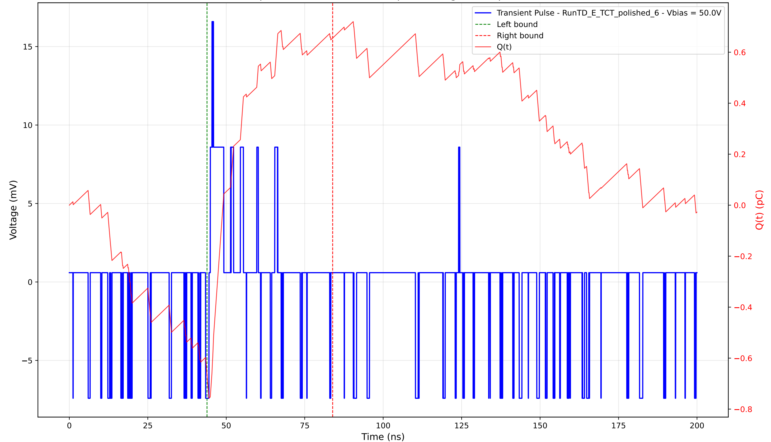
Transient Pulse - Sample: 4003 - Position: 35.0 \mu\text{m} - Charge: 1.32 pC - Rise Time: 0.56 ns
