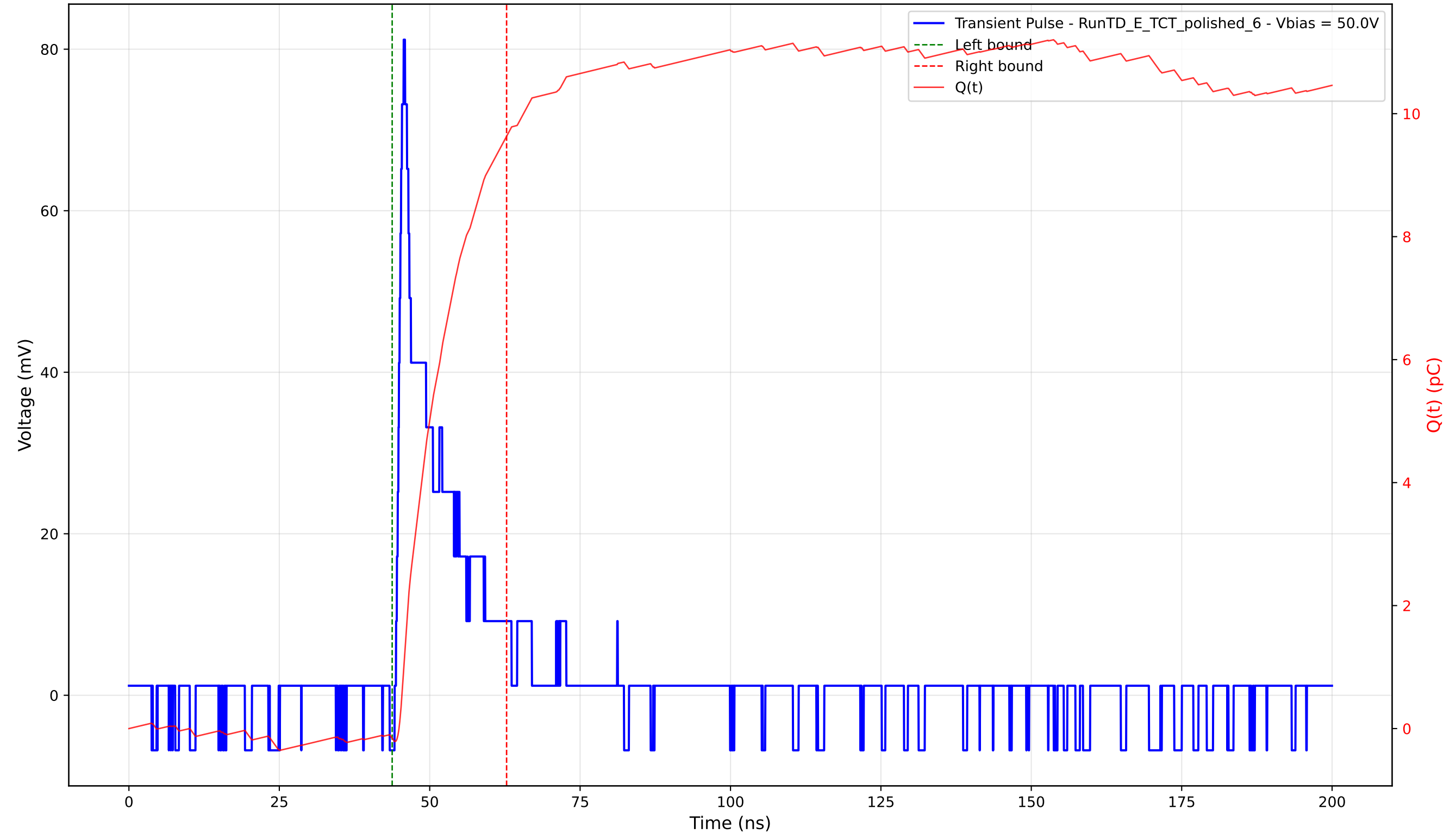
Transient Pulse - Sample: 4003 - Position: 90.0 \mu\text{m} - Charge: 9.79 pC - Rise Time: 0.98 ns
