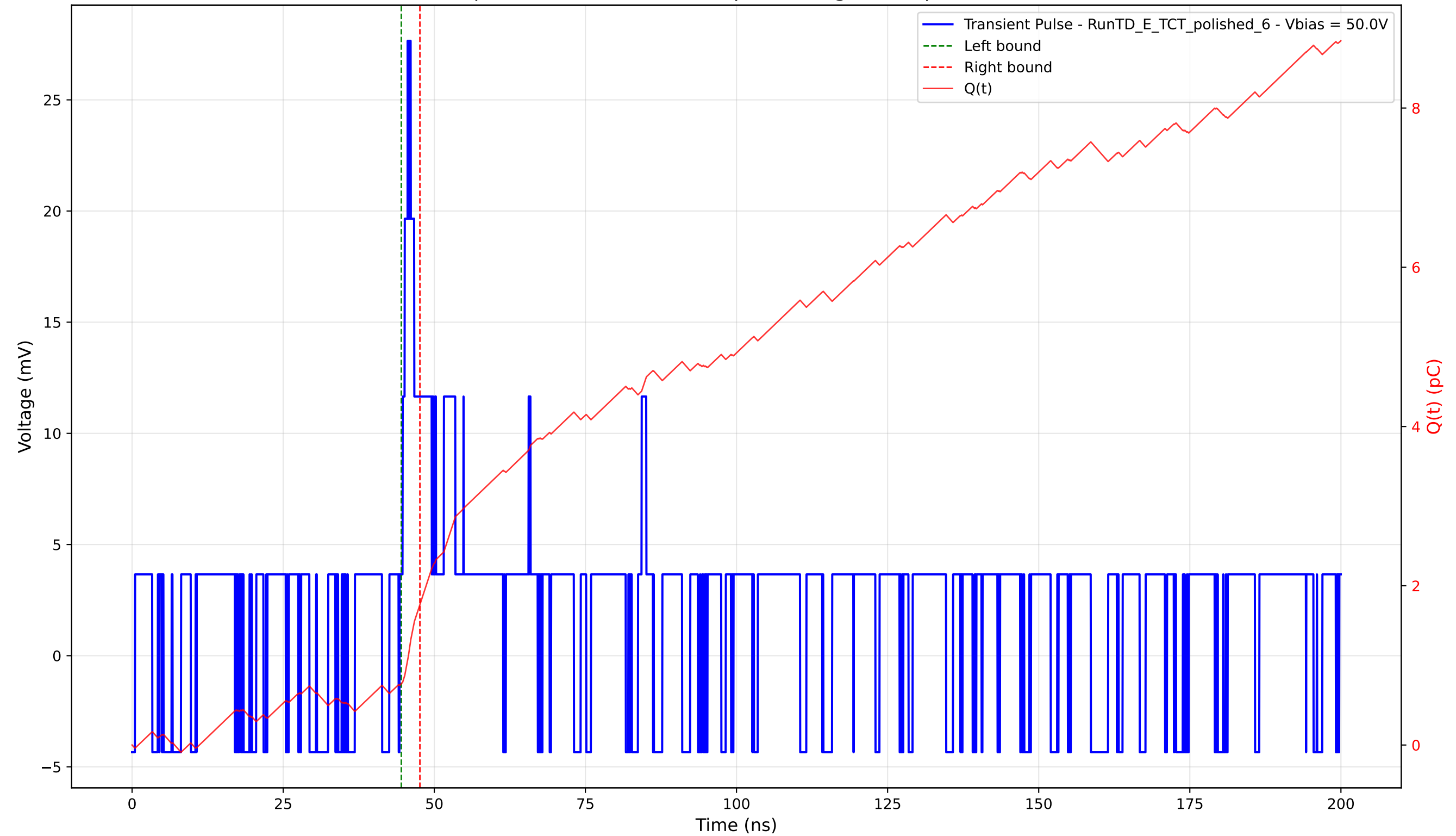
Transient Pulse - Sample: 4003 - Position: 80.0 \mu\text{m} - Charge: 0.99 pC - Rise Time: 0.00 ns (N/A)
