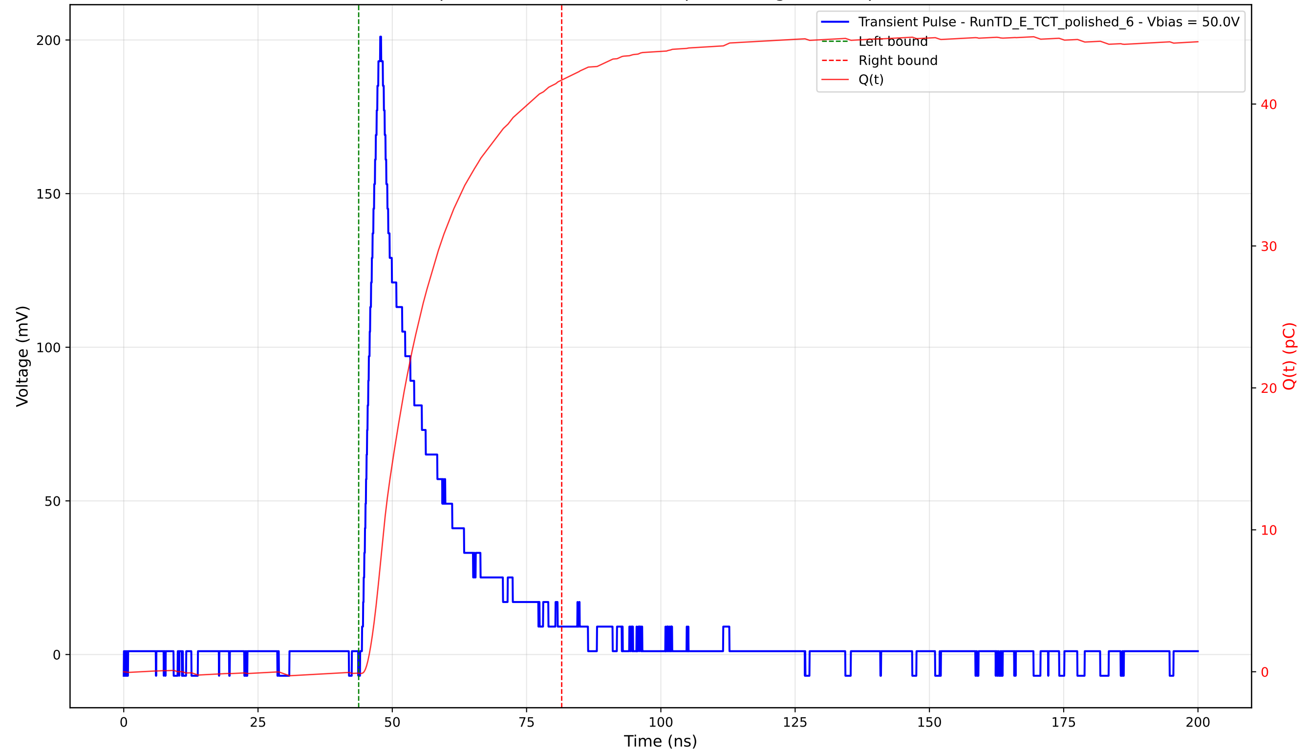
Transient Pulse - Sample: 4003 - Position: 190.0 \mu\text{m} - Charge: 41.78 pC - Rise Time: 2.57 ns
