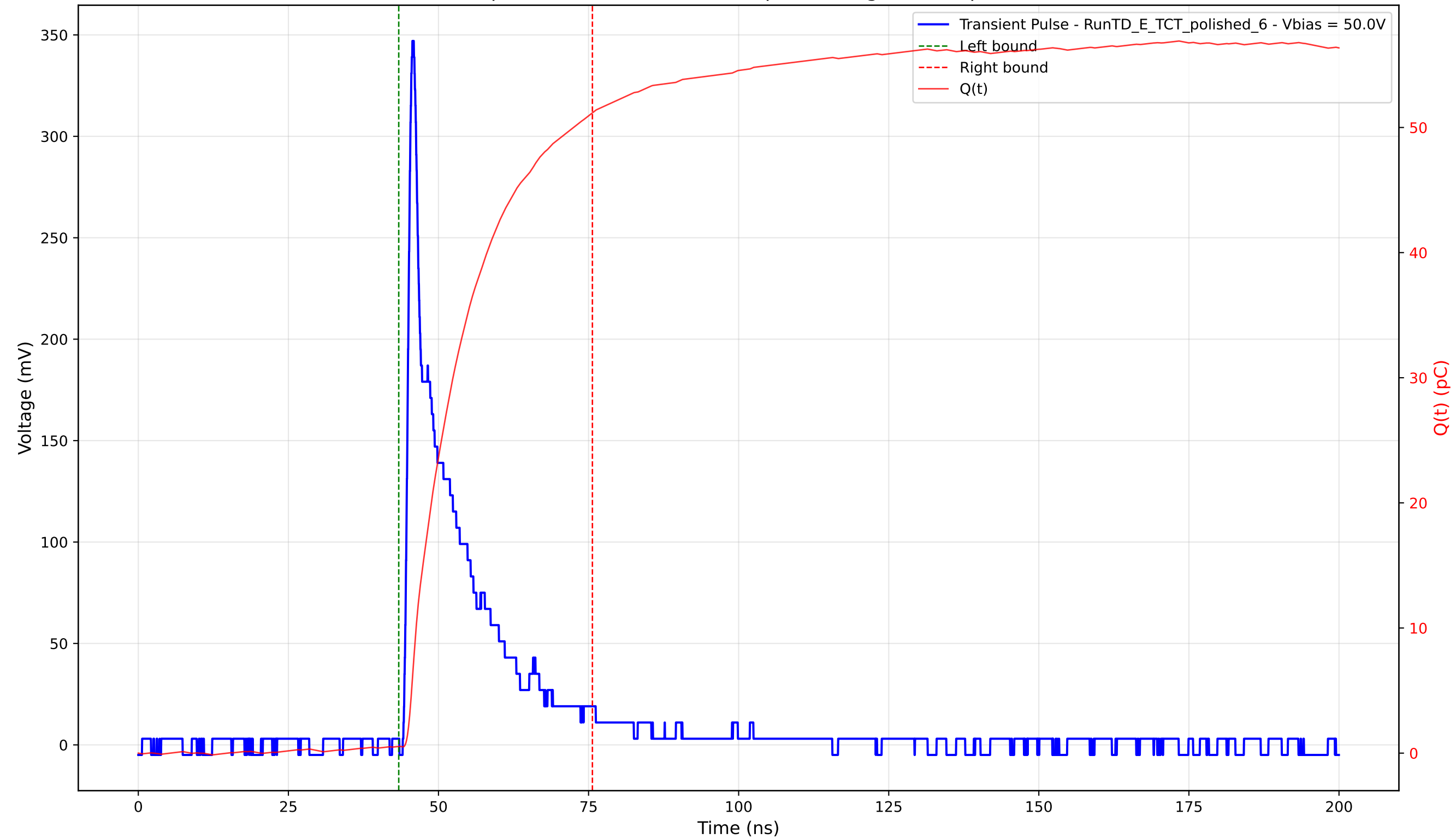
Transient Pulse - Sample: 4003 - Position: 125.0 \mu\text{m} - Charge: 50.63 pC - Rise Time: 1.04 ns
