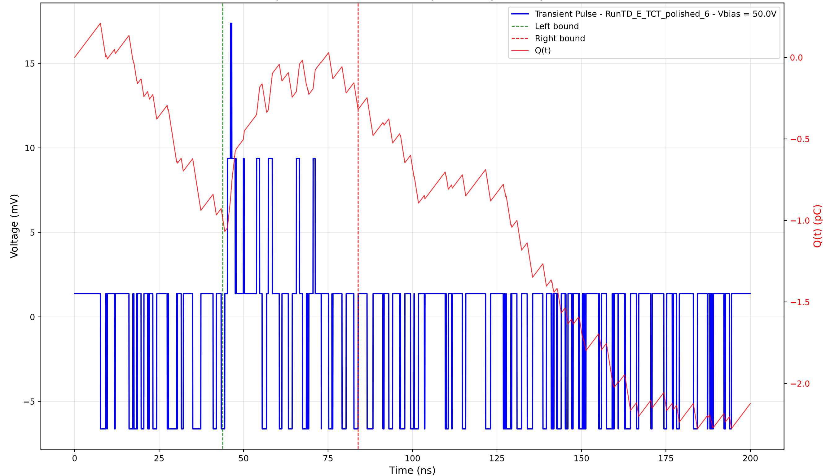
Transient Pulse - Sample: 4003 - Position: 345.0 \mu\text{m} - Charge: 0.68 pC - Rise Time: 0.90 ns
