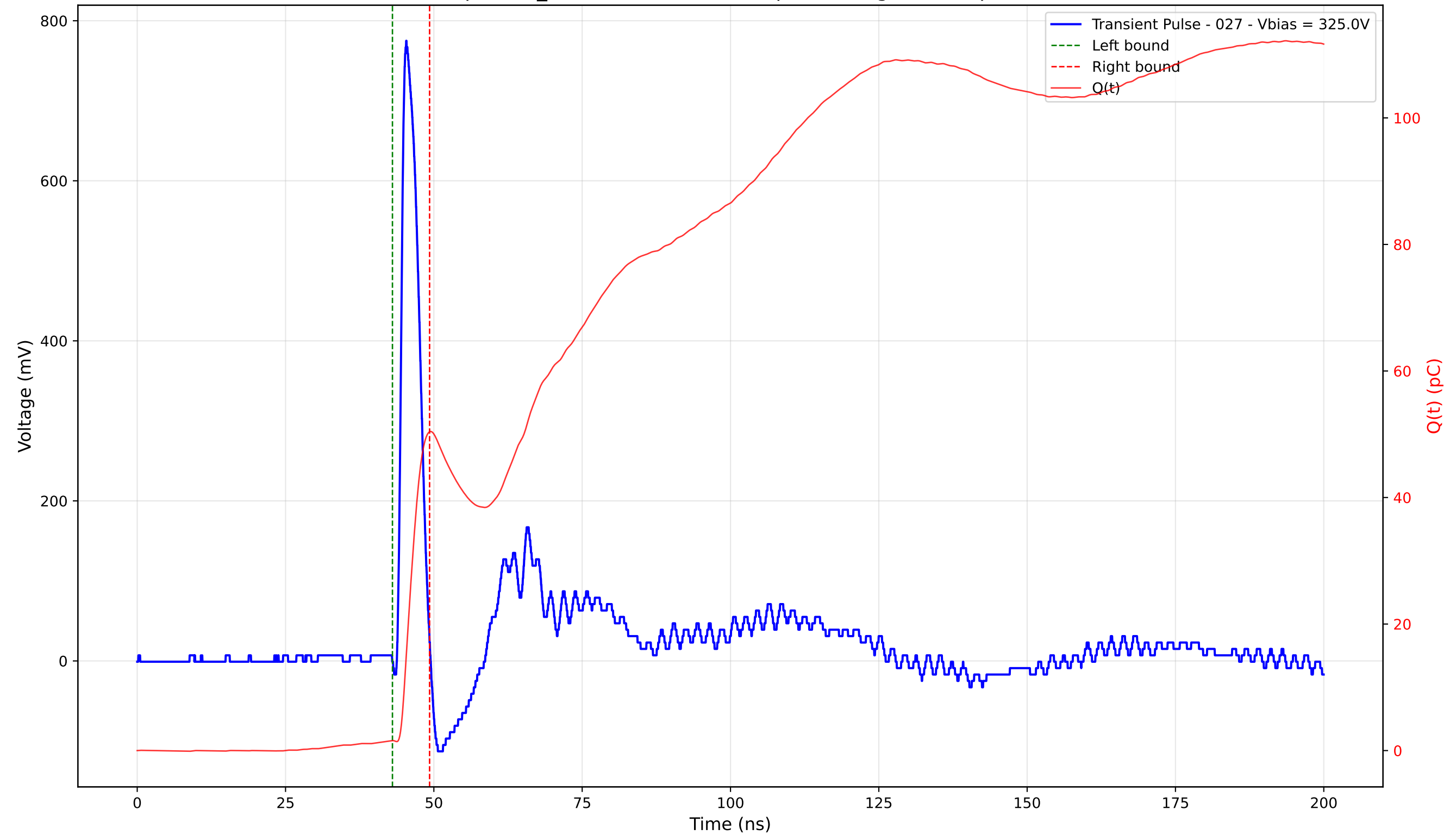
Transient Pulse - Sample: TD_4004 - Position: 300.0 \mu\text{m} - Charge: 48.81 pC - Rise Time: 0.95 ns
