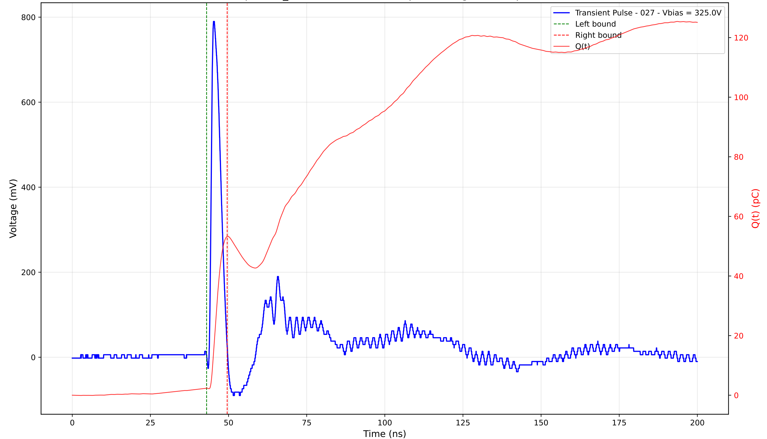
Transient Pulse - Sample: TD_4004 - Position: 160.0 \mu\text{m} - Charge: 50.91 pC - Rise Time: 0.88 ns
