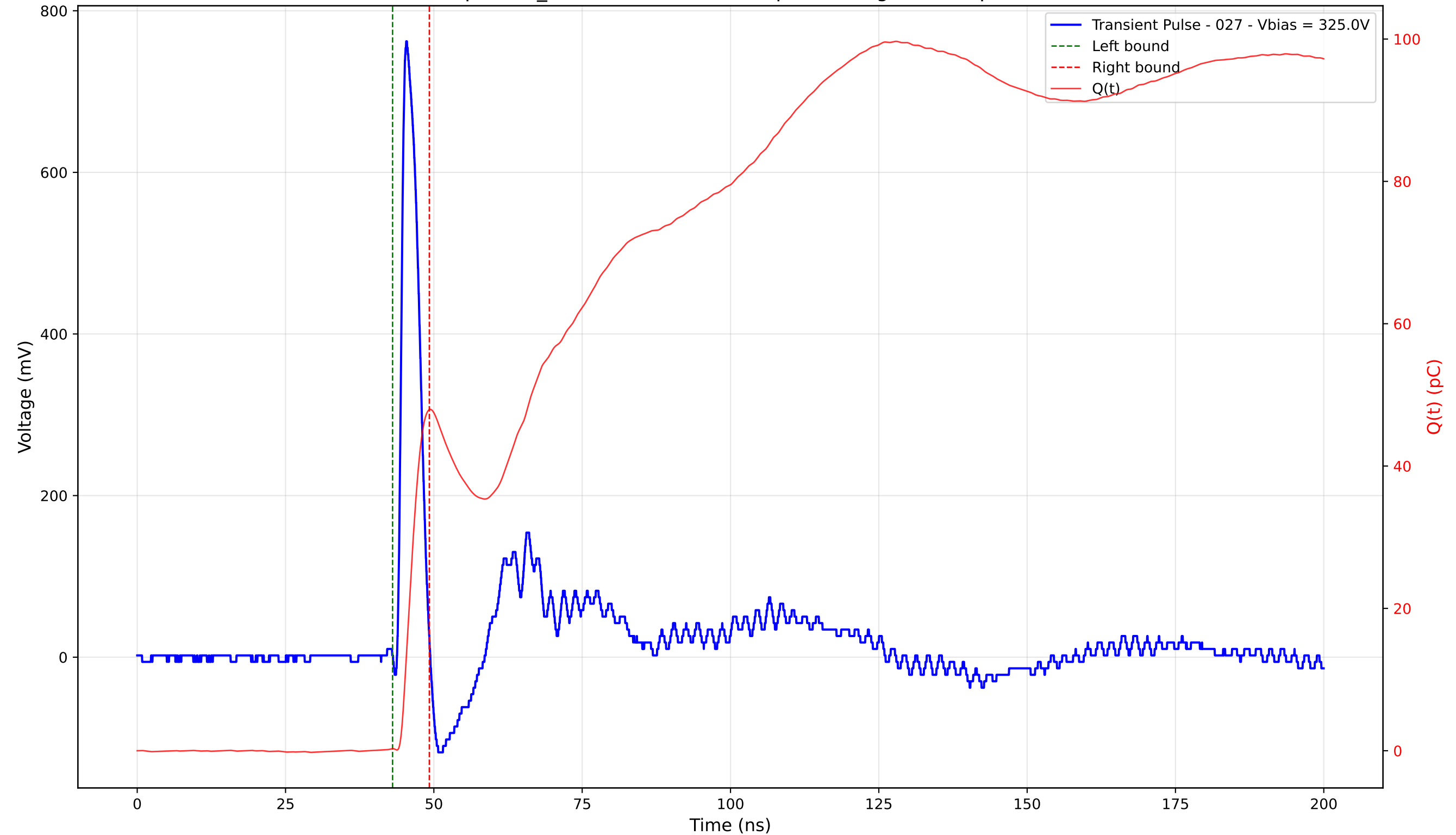
Transient Pulse - Sample: TD_4004 - Position: 305.0 \mu\text{m} - Charge: 47.64 pC - Rise Time: 0.94 ns
