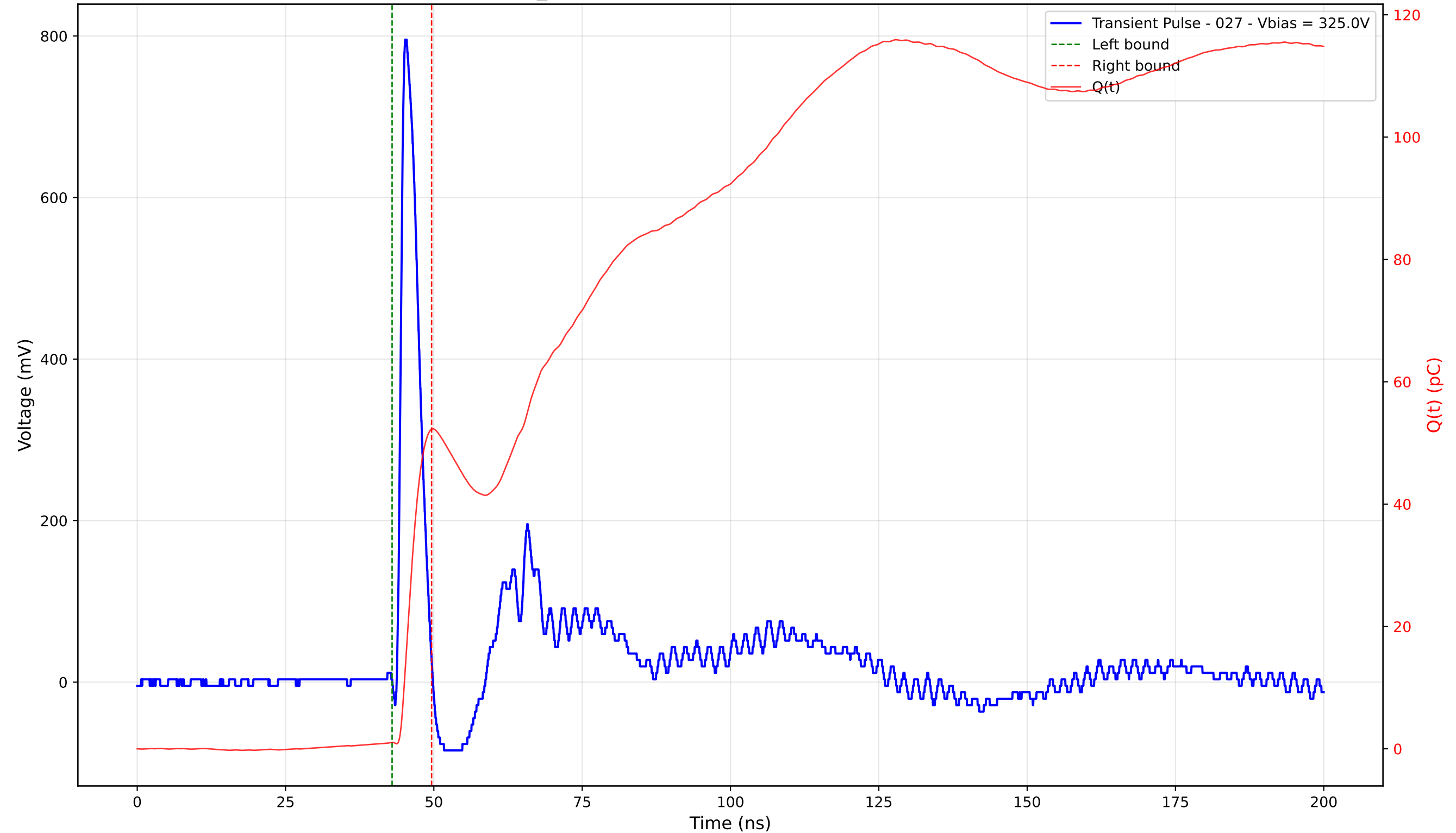
Transient Pulse - Sample: TD_4004 - Position: 220.0 \mu\text{m} - Charge: 51.19 pC - Rise Time: 0.91 ns
