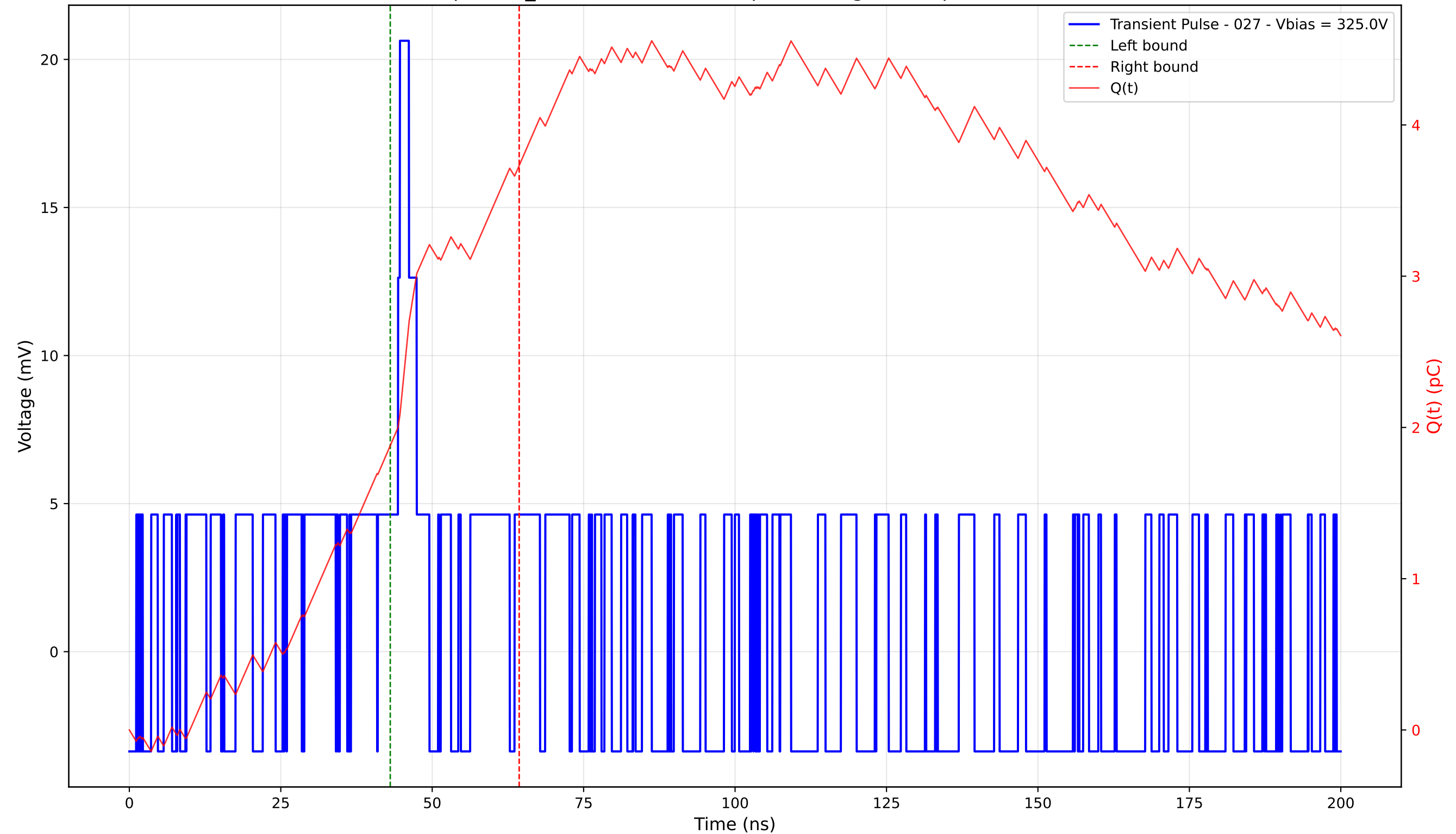
Transient Pulse - Sample: TD_4004 - Position: 20.0 \mu\text{m} - Charge: 1.85 pC - Rise Time: 0.00 ns (N/A)
