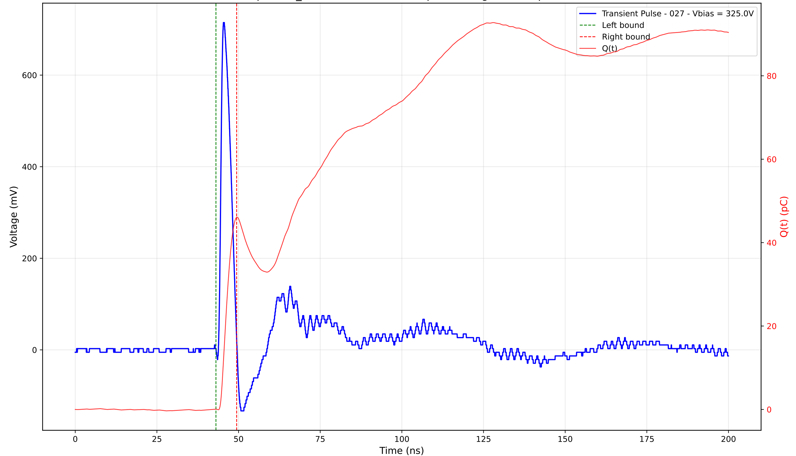
Transient Pulse - Sample: TD_4004 - Position: 330.0 \mu\text{m} - Charge: 46.01 pC - Rise Time: 0.97 ns
