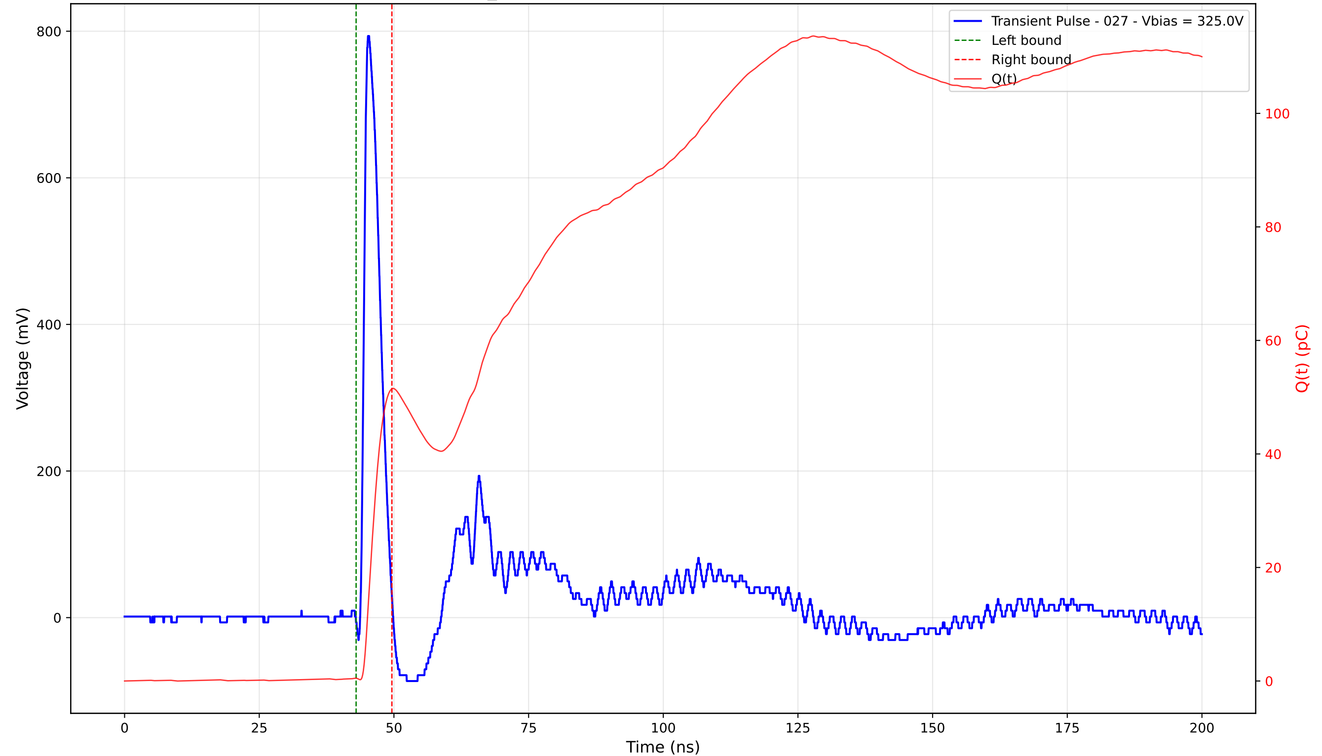
Transient Pulse - Sample: TD_4004 - Position: 215.0 \mu\text{m} - Charge: 50.99 pC - Rise Time: 0.89 ns
