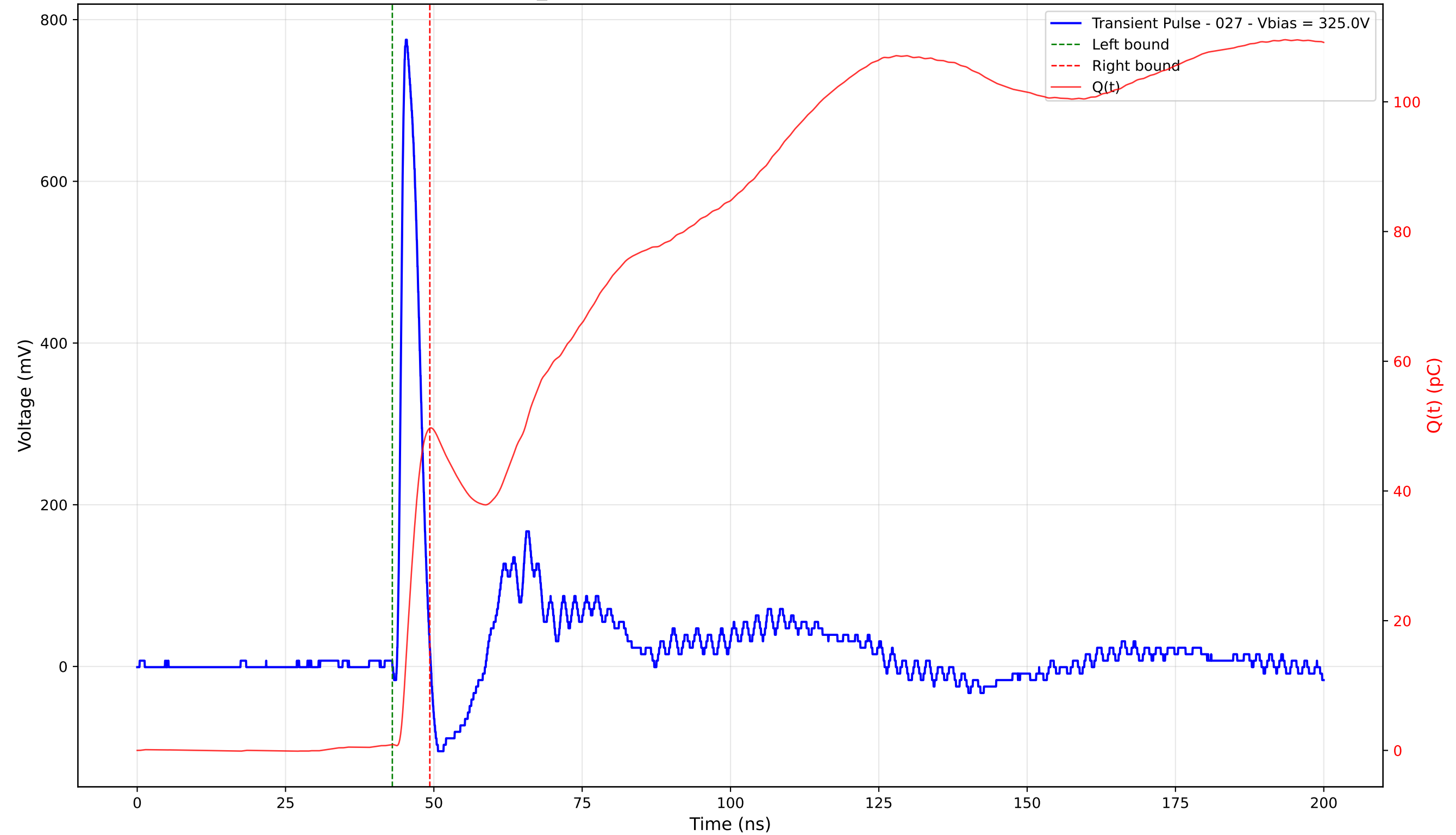
Transient Pulse - Sample: TD_4004 - Position: 255.0 \mu\text{m} - Charge: 48.79 pC - Rise Time: 0.93 ns
