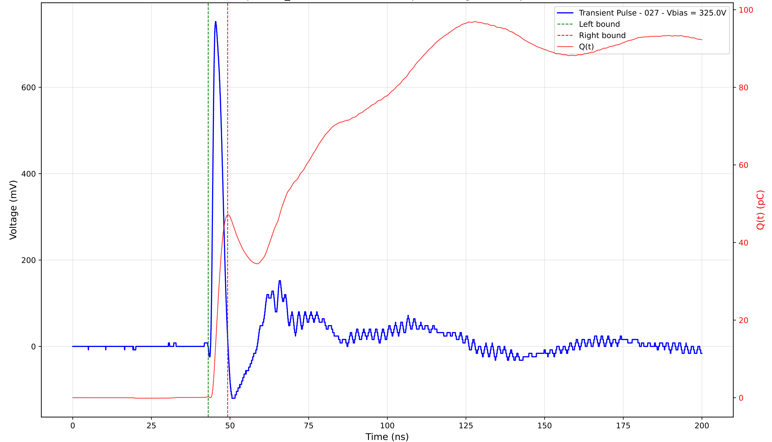
Transient Pulse - Sample: TD_4004 - Position: 310.0 \mu\text{m} - Charge: 46.91 pC - Rise Time: 0.95 ns
