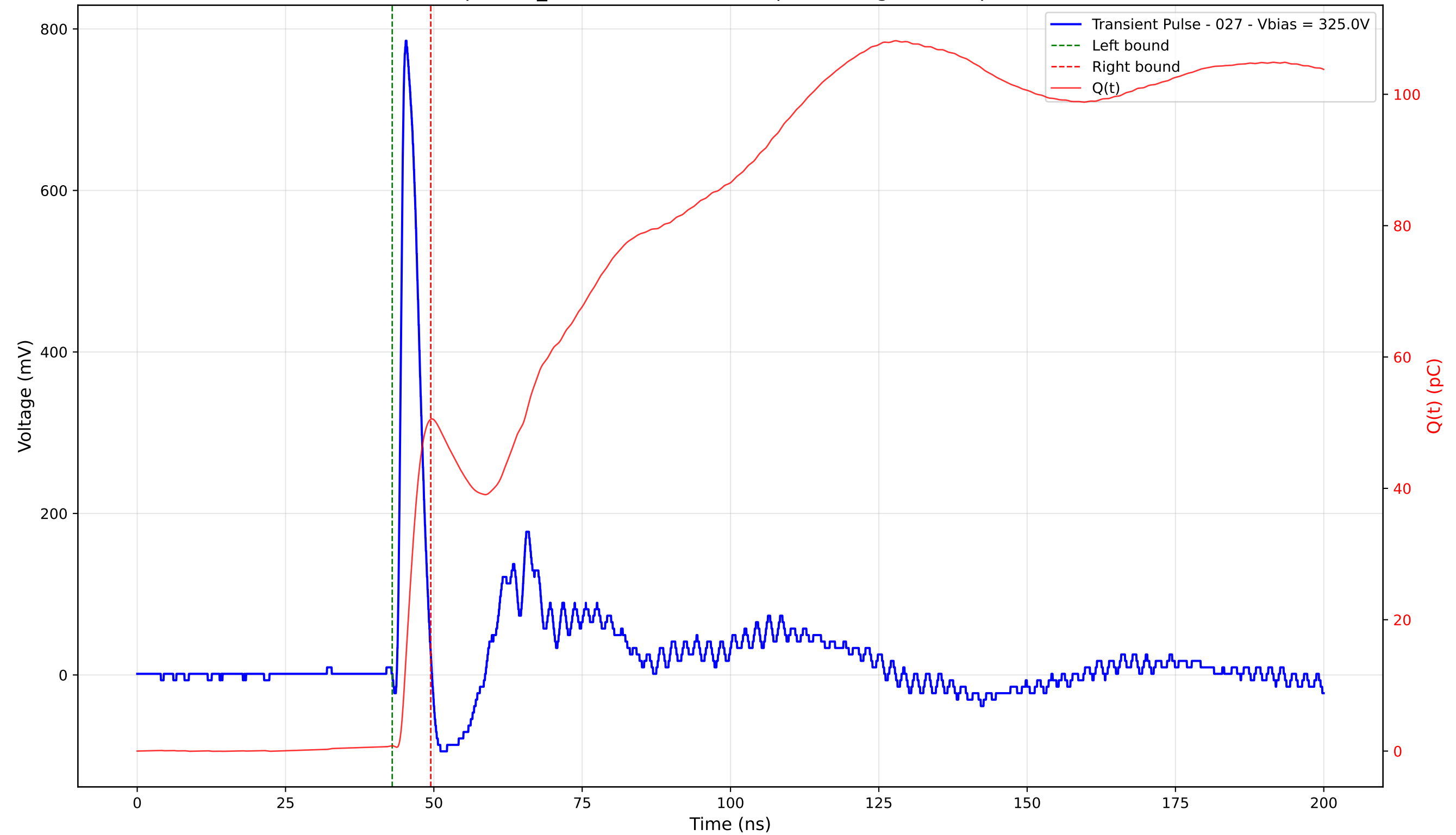
Transient Pulse - Sample: TD_4004 - Position: 230.0 \mu\text{m} - Charge: 49.72 pC - Rise Time: 0.91 ns
