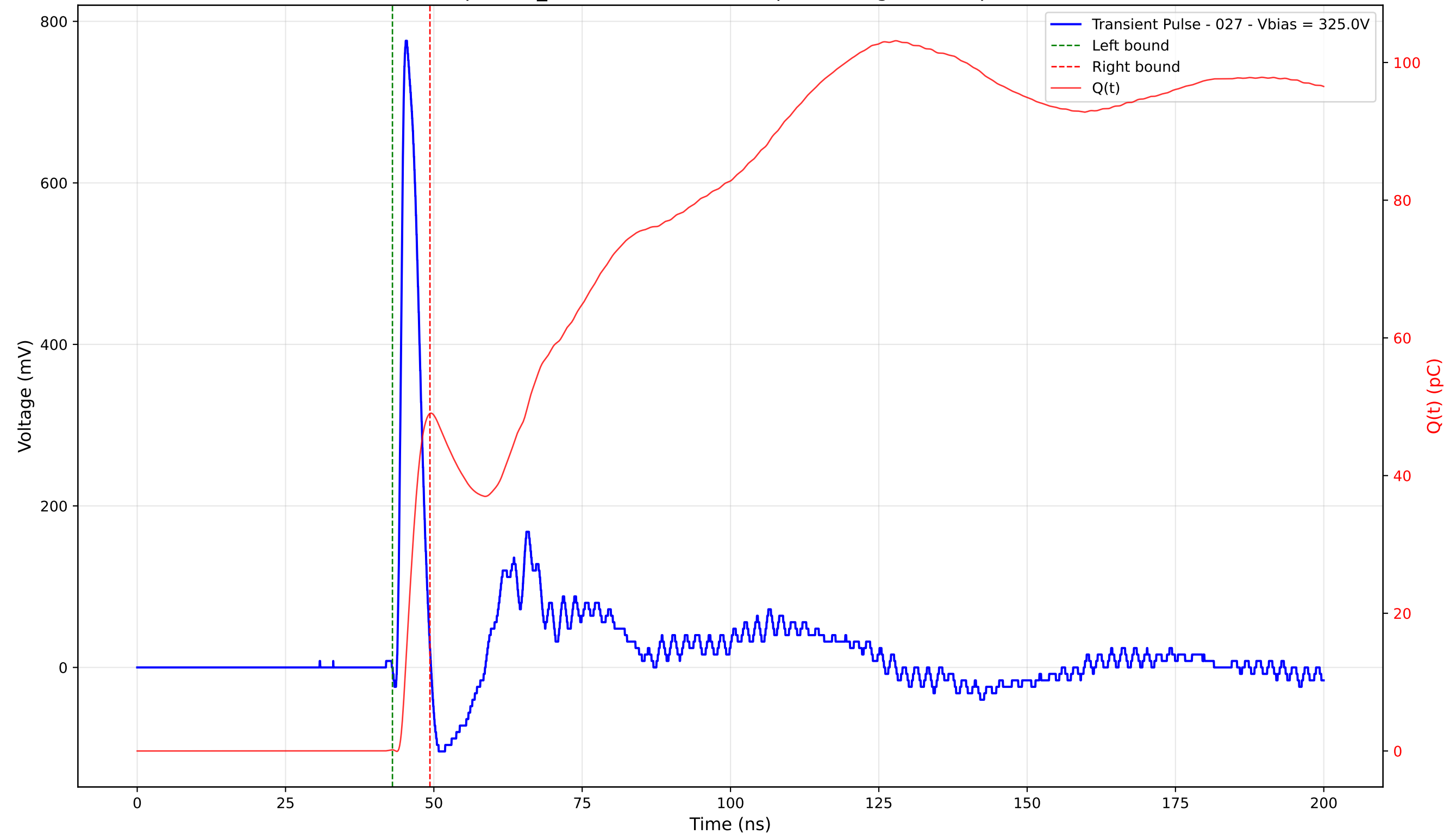
Transient Pulse - Sample: TD_4004 - Position: 250.0 \mu\text{m} - Charge: 48.85 pC - Rise Time: 0.91 ns
