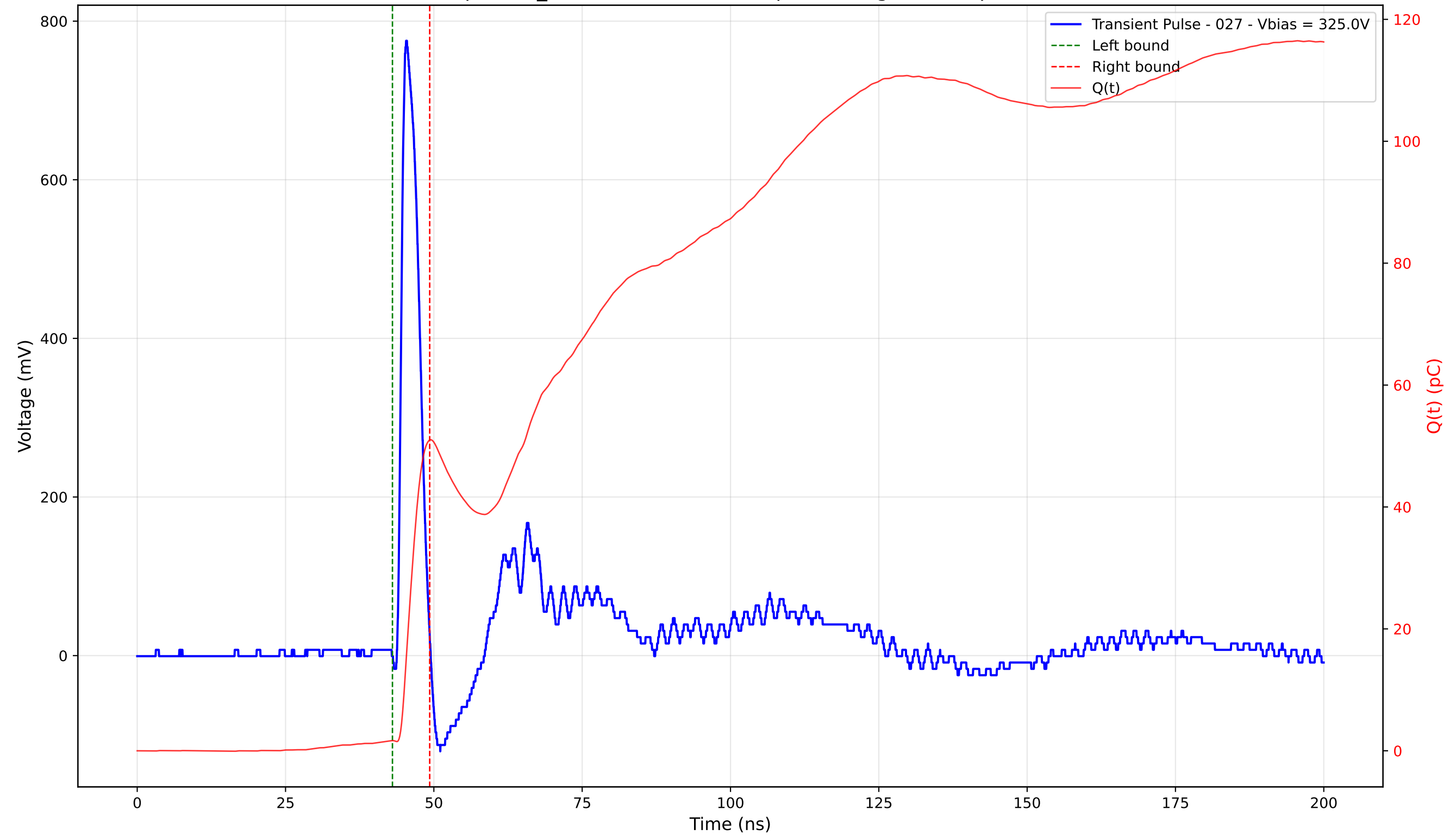
Transient Pulse - Sample: TD_4004 - Position: 295.0 \mu\text{m} - Charge: 49.31 pC - Rise Time: 0.95 ns
