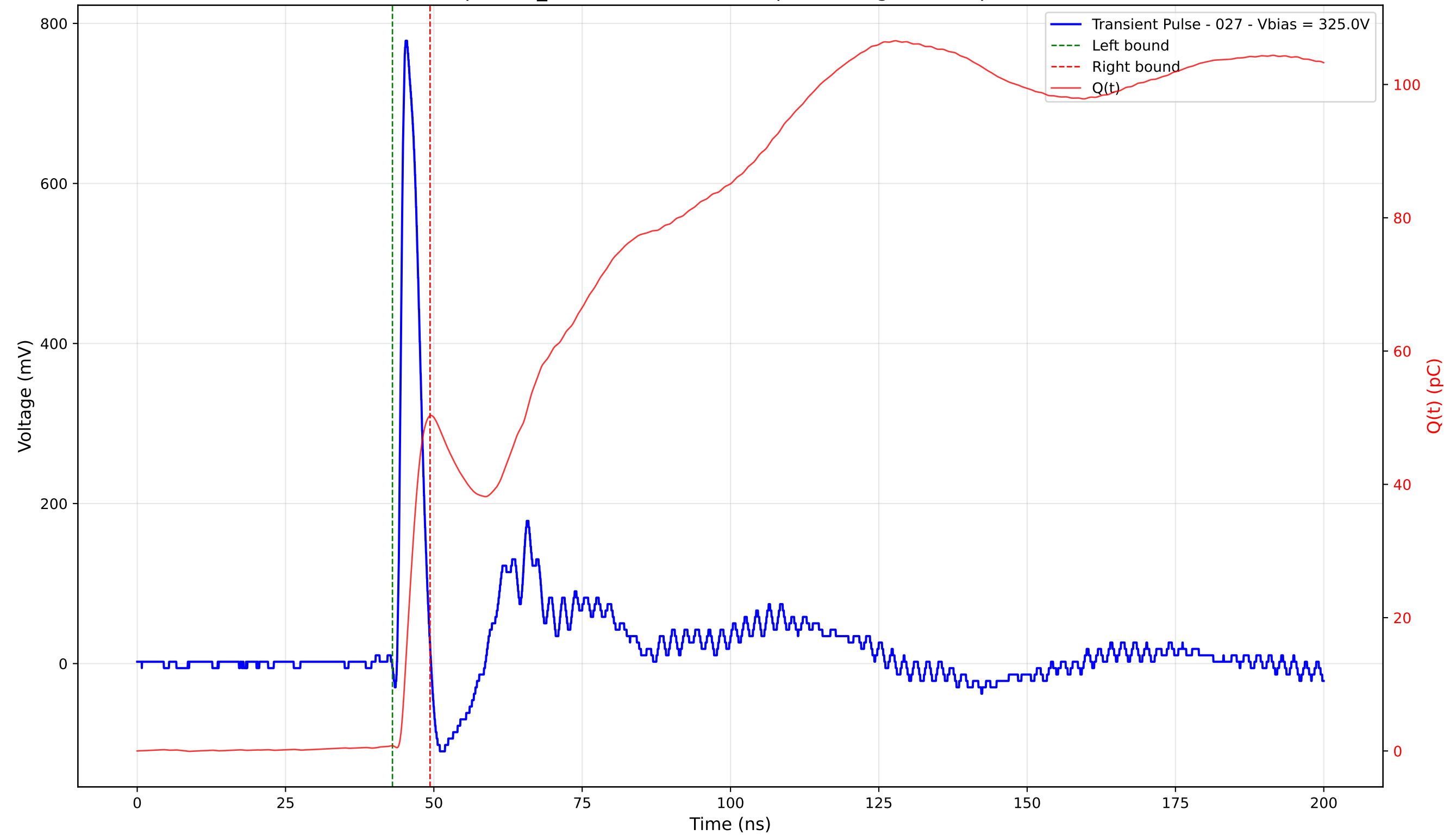
Transient Pulse - Sample: TD_4004 - Position: 270.0 \mu\text{m} - Charge: 49.53 pC - Rise Time: 0.90 ns
