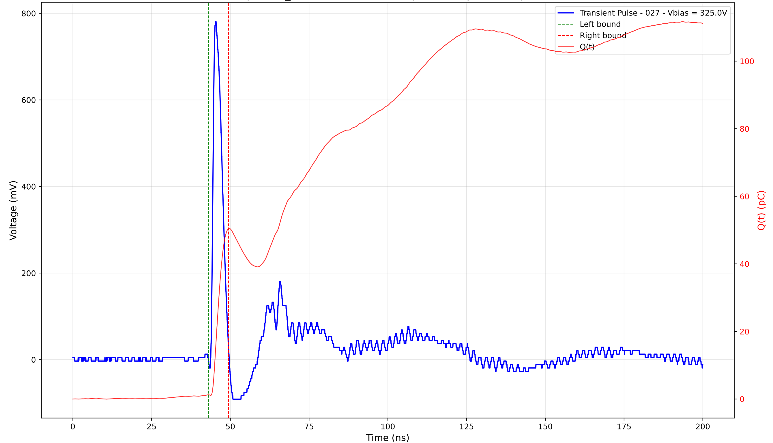
Transient Pulse - Sample: TD_4004 - Position: 235.0 \mu\text{m} - Charge: 49.17 pC - Rise Time: 0.91 ns
