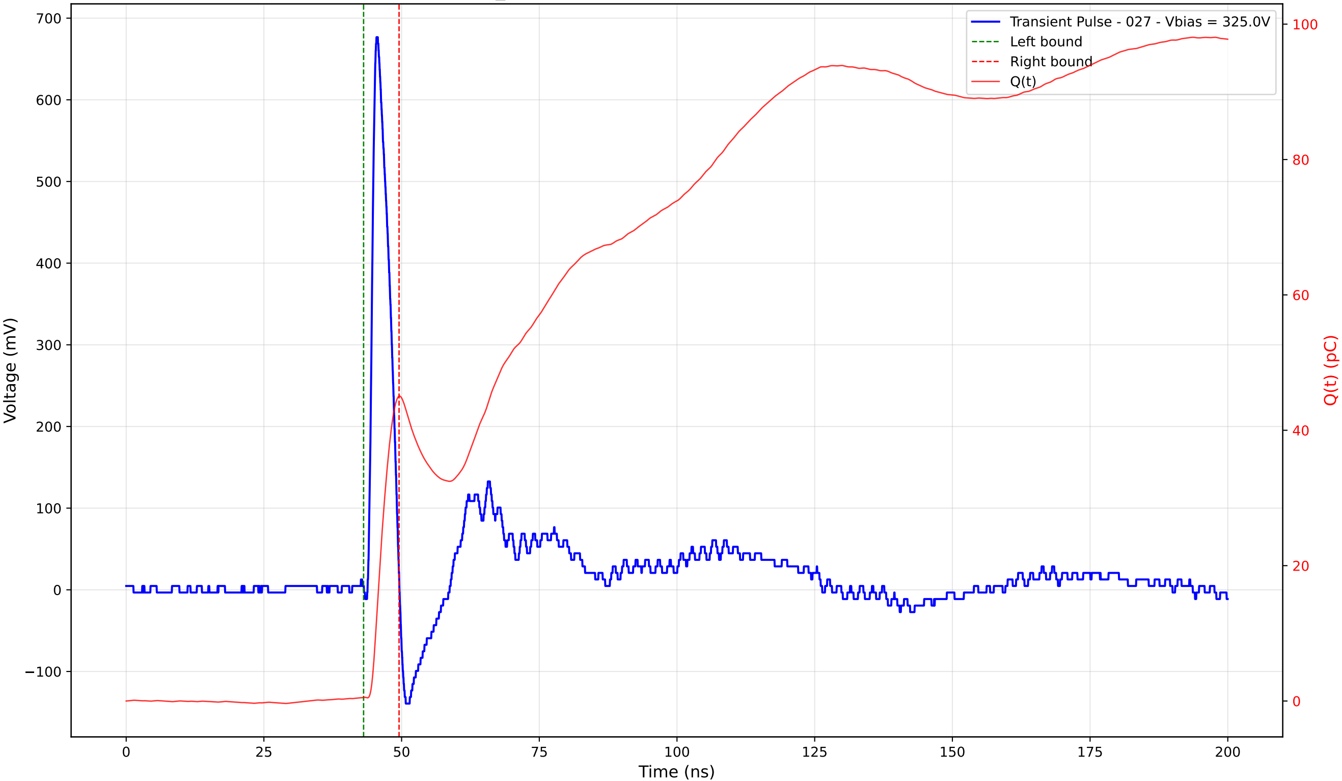
Transient Pulse - Sample: TD_4004 - Position: 370.0 \mu\text{m} - Charge: 44.48 pC - Rise Time: 1.02 ns
