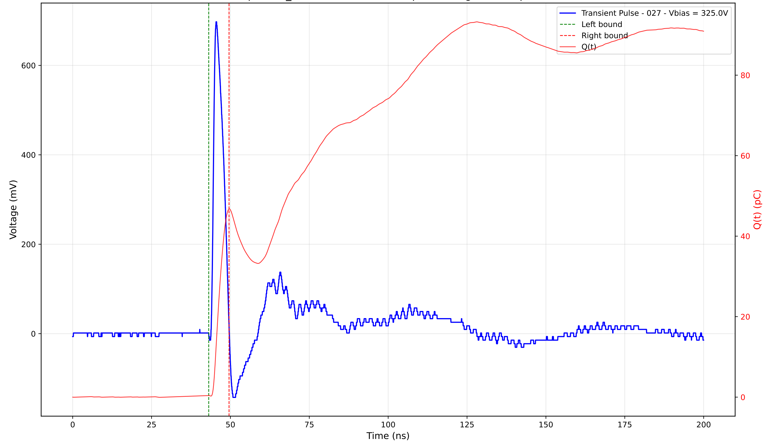
Transient Pulse - Sample: TD_4004 - Position: 360.0 \mu\text{m} - Charge: 46.33 pC - Rise Time: 1.00 ns
