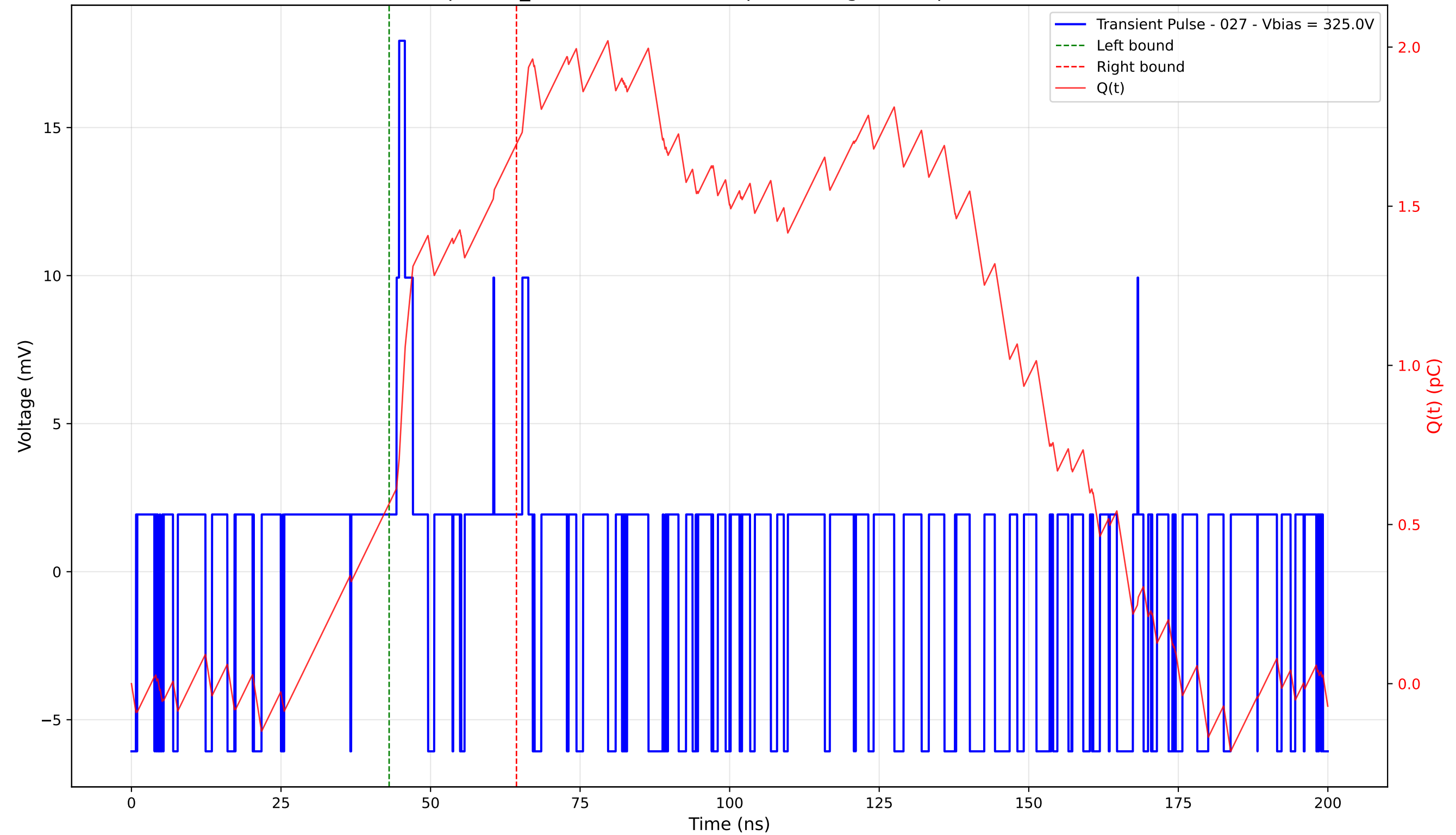
Transient Pulse - Sample: TD_4004 - Position: 10.0 \mu\text{m} - Charge: 1.13 pC - Rise Time: 0.00 ns (N/A)
