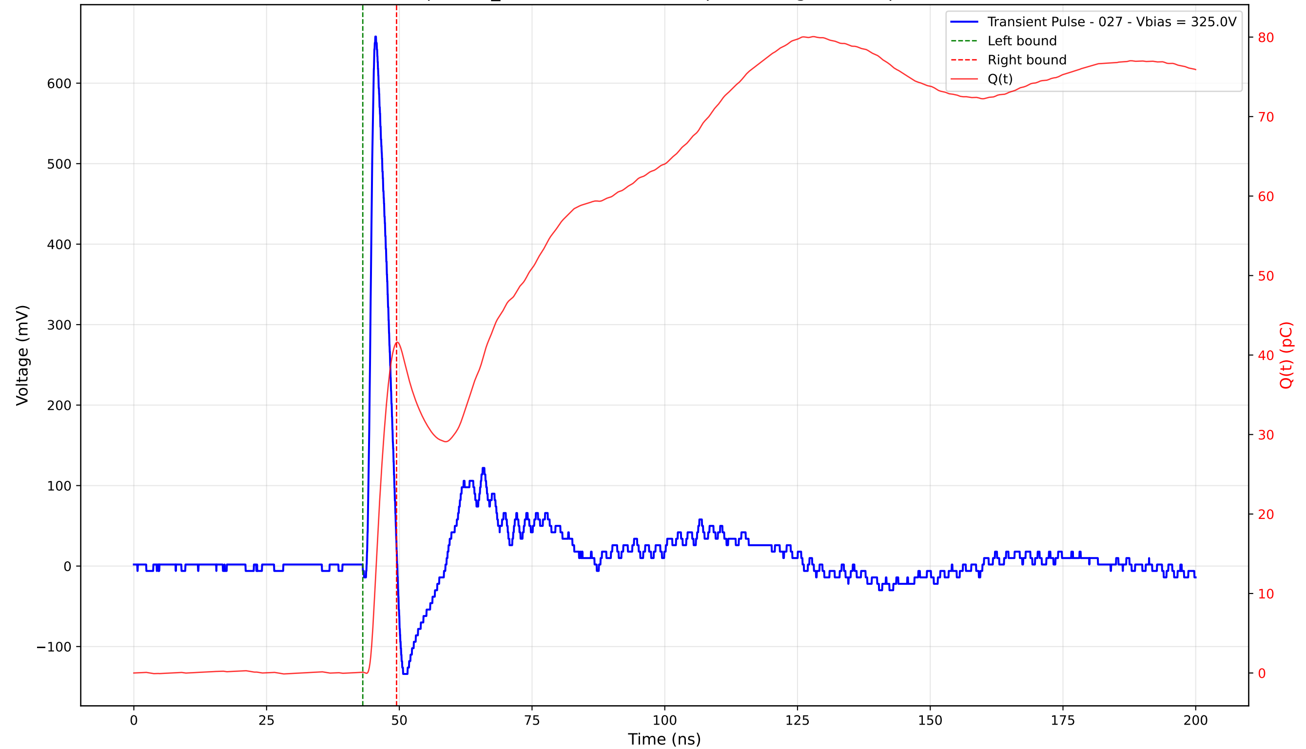
Transient Pulse - Sample: TD_4004 - Position: 380.0 \mu\text{m} - Charge: 41.48 pC - Rise Time: 1.02 ns
