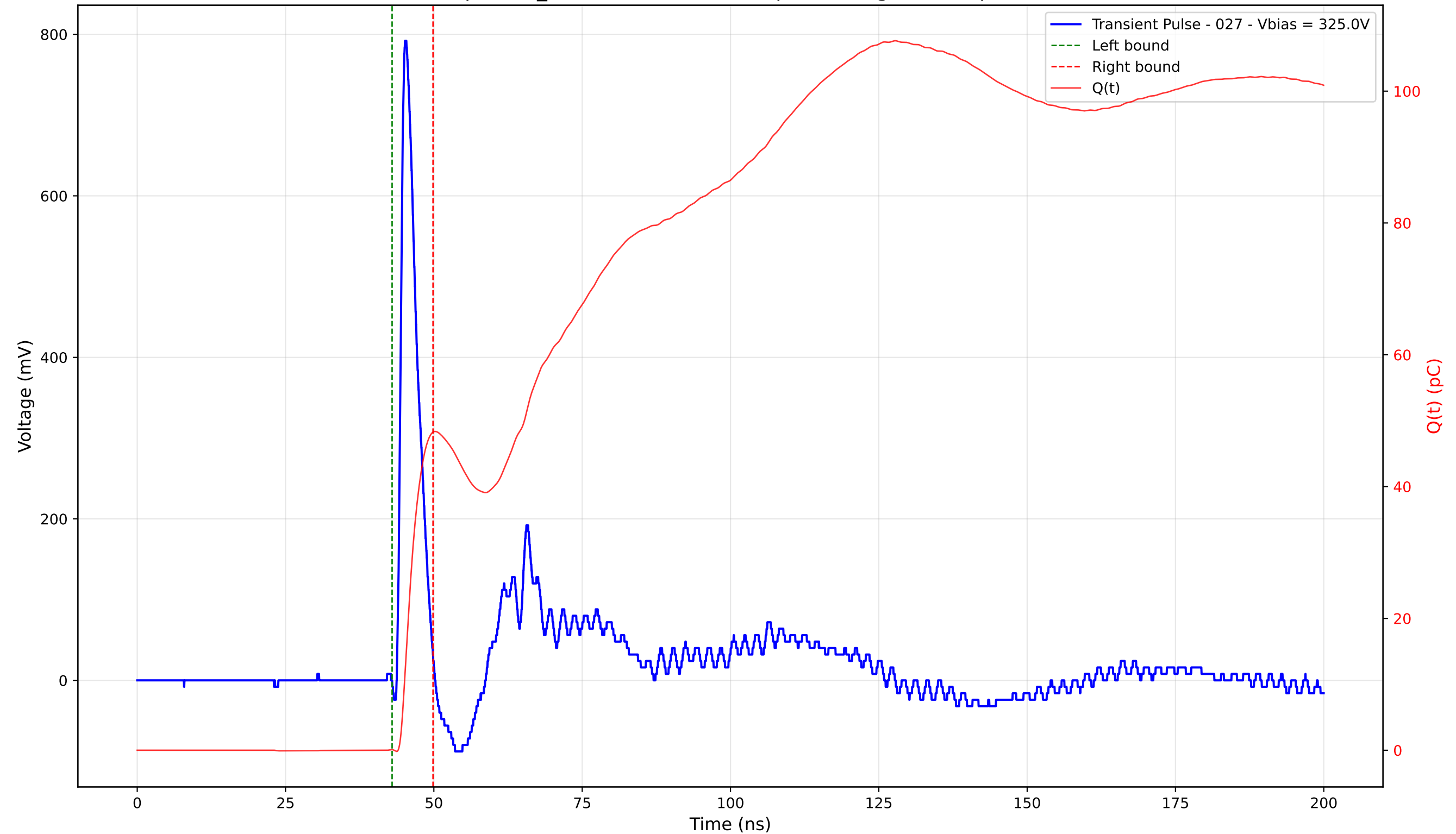
Transient Pulse - Sample: TD_4004 - Position: 100.0 \mu\text{m} - Charge: 48.18 pC - Rise Time: 0.86 ns
