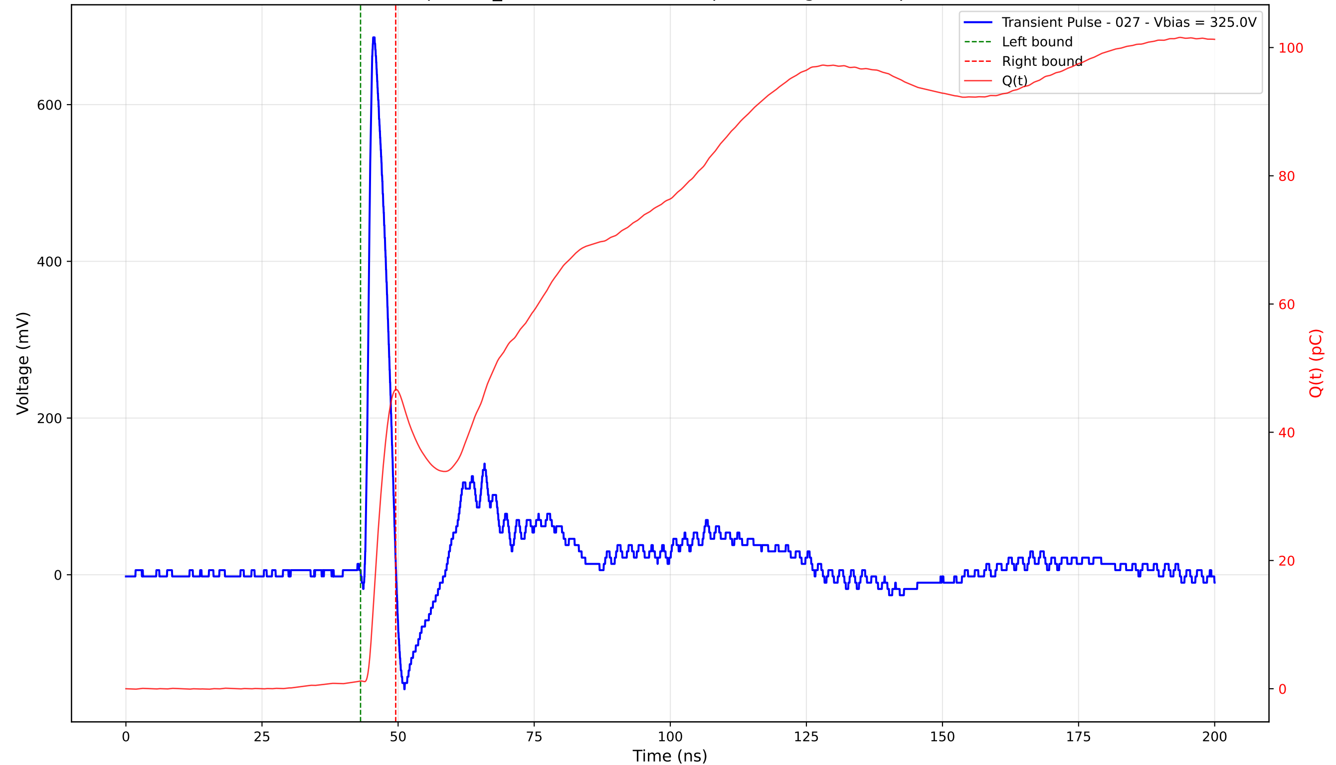
Transient Pulse - Sample: TD_4004 - Position: 365.0 \mu\text{m} - Charge: 45.45 pC - Rise Time: 0.99 ns
