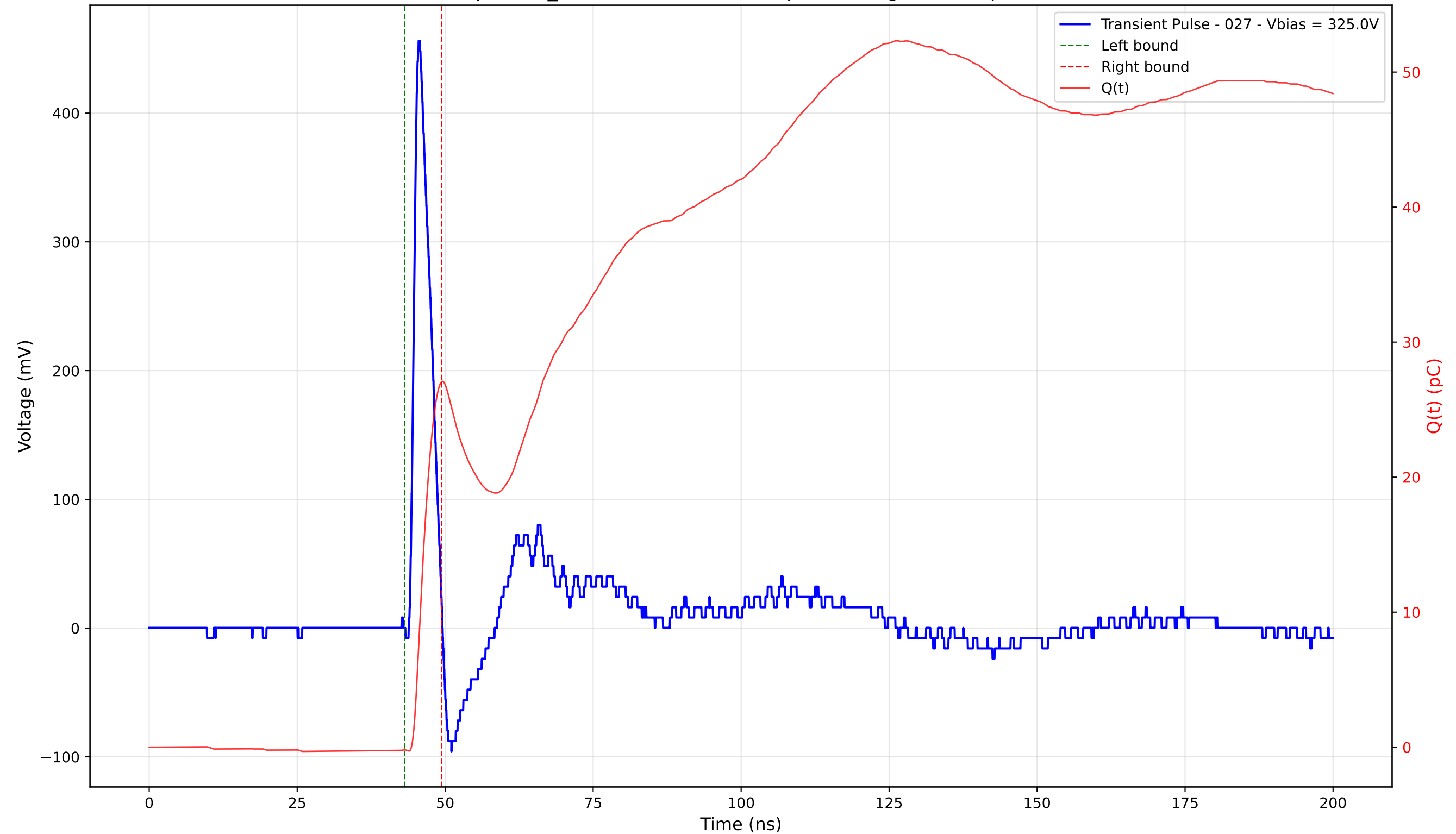
Transient Pulse - Sample: TD_4004 - Position: 395.0 \mu\text{m} - Charge: 27.27 pC - Rise Time: 1.05 ns
