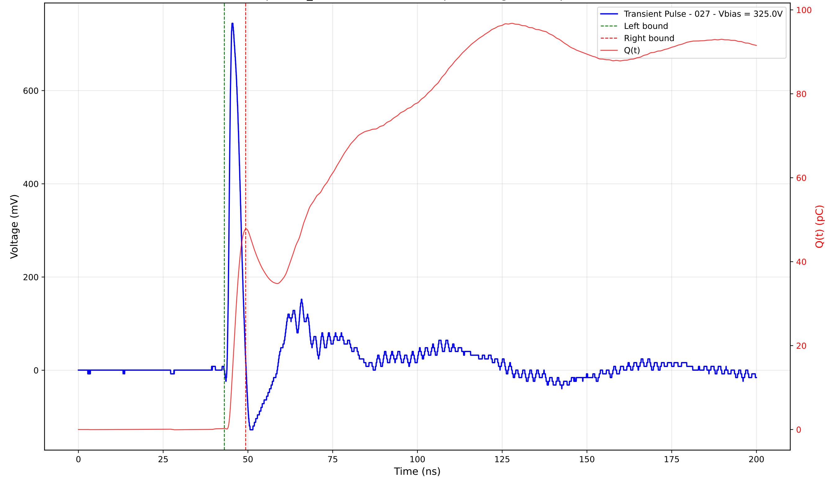
Transient Pulse - Sample: TD_4004 - Position: 320.0 \mu\text{m} - Charge: 47.52 pC - Rise Time: 0.95 ns
