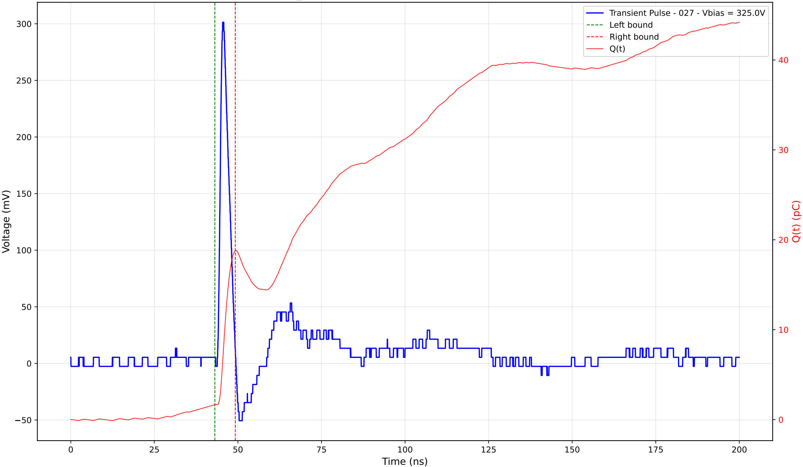
Transient Pulse - Sample: TD_4004 - Position: 405.0 \mu\text{m} - Charge: 17.14 pC - Rise Time: 1.06 ns
