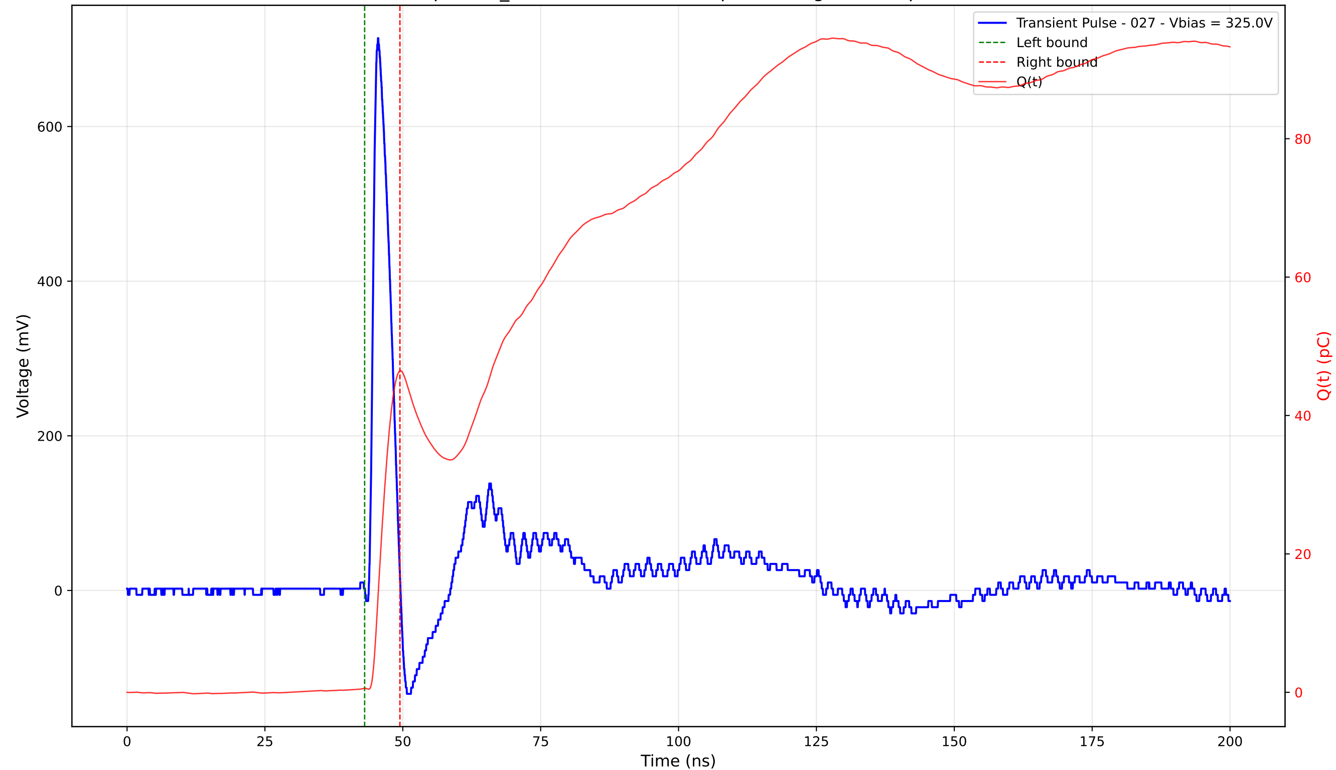
Transient Pulse - Sample: TD_4004 - Position: 335.0 \mu\text{m} - Charge: 45.87 pC - Rise Time: 1.01 ns
