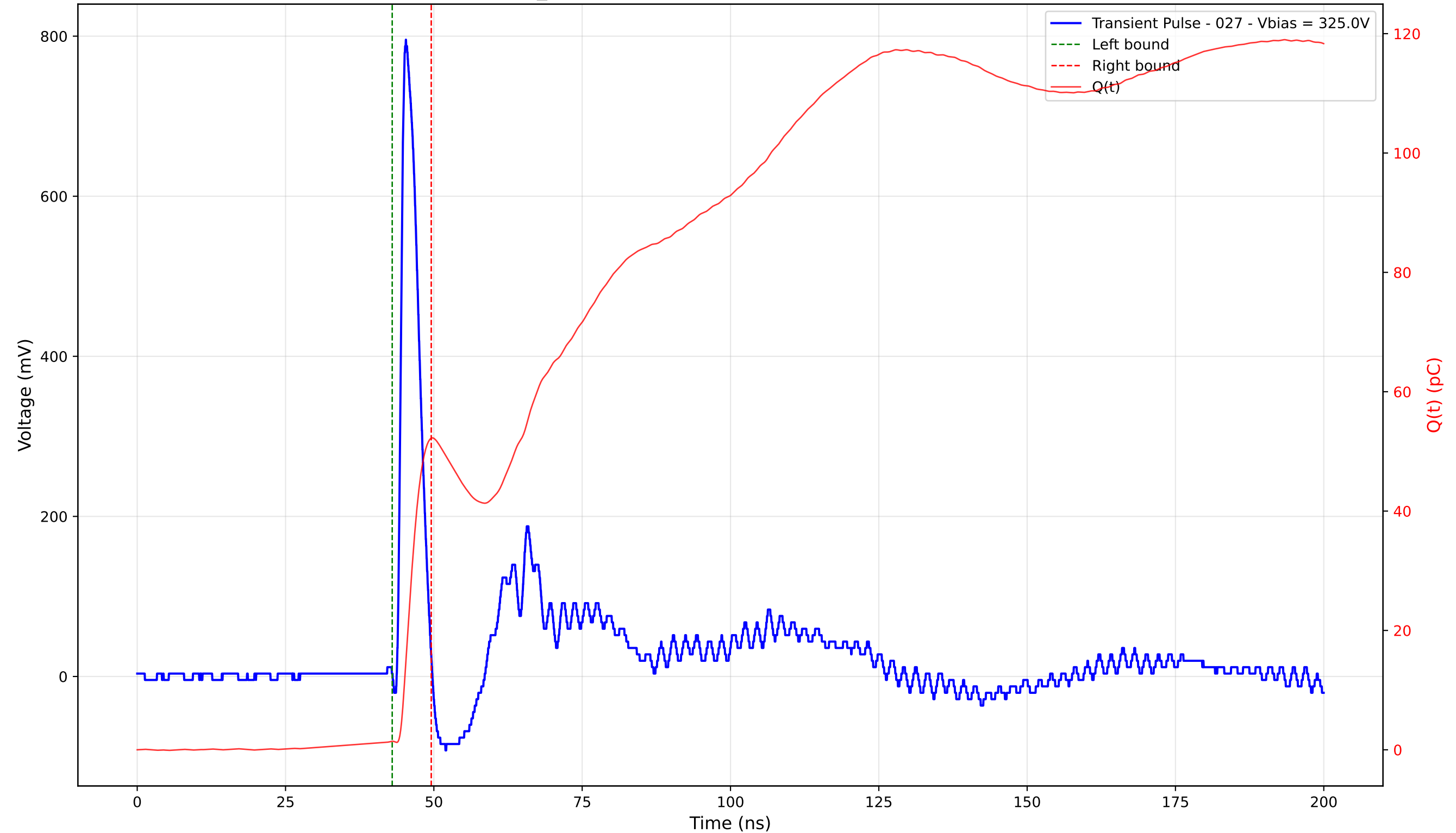
Transient Pulse - Sample: TD_4004 - Position: 225.0 \mu\text{m} - Charge: 50.79 pC - Rise Time: 0.91 ns
