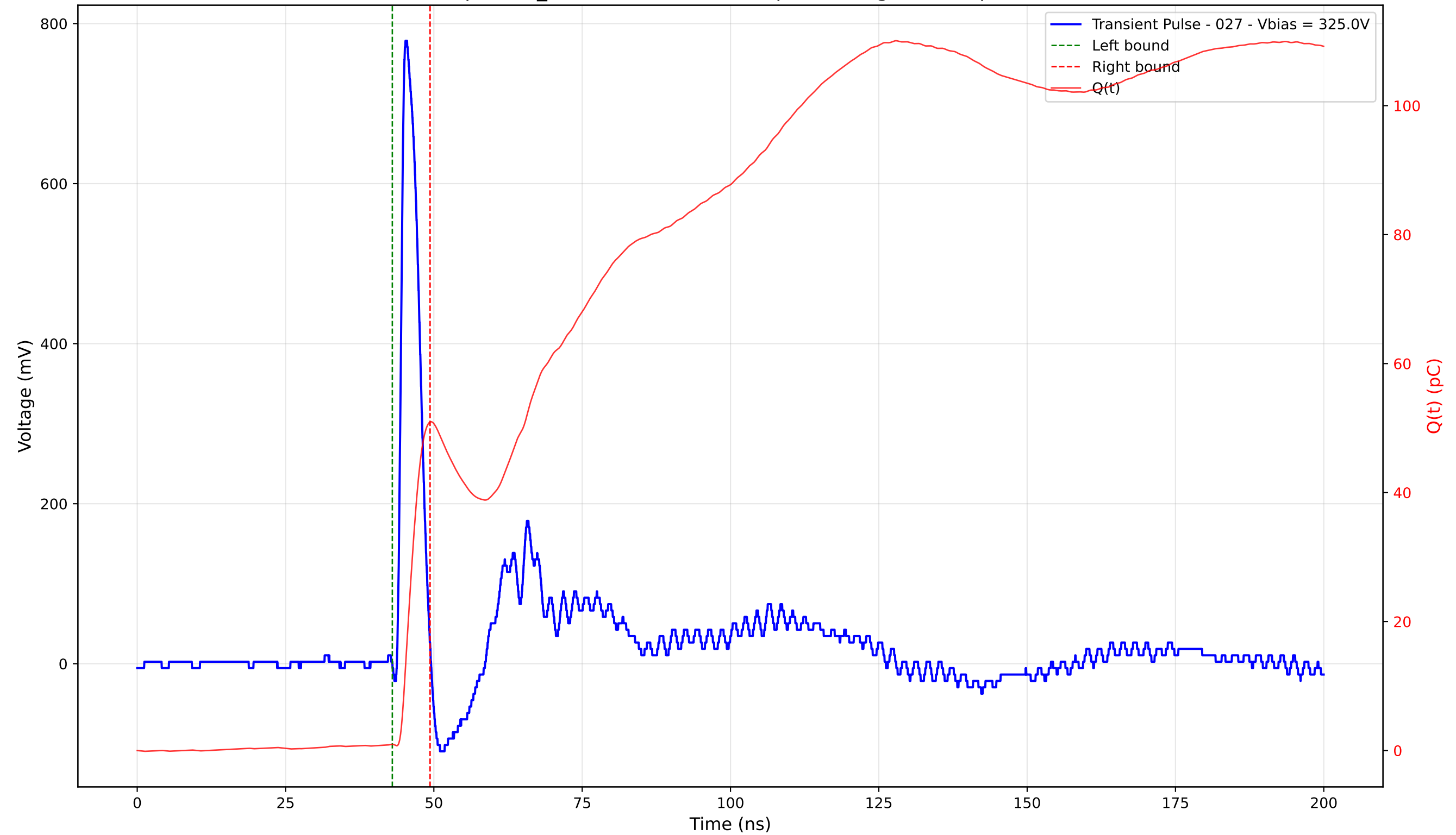
Transient Pulse - Sample: TD_4004 - Position: 275.0 \mu\text{m} - Charge: 49.98 pC - Rise Time: 0.90 ns
