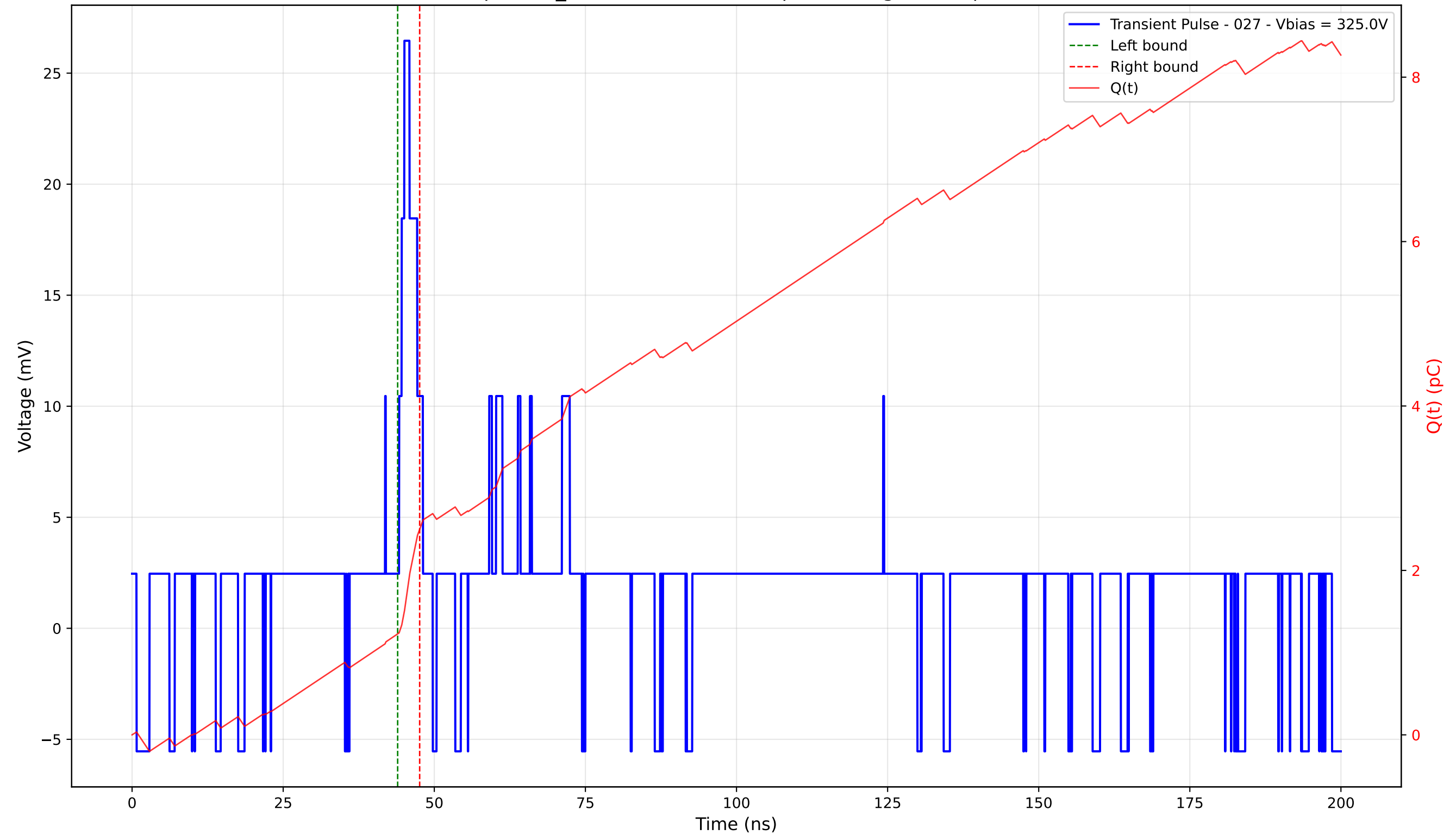
Transient Pulse - Sample: TD_4004 - Position: 25.0 \mu\text{m} - Charge: 1.28 pC - Rise Time: 0.88 ns
