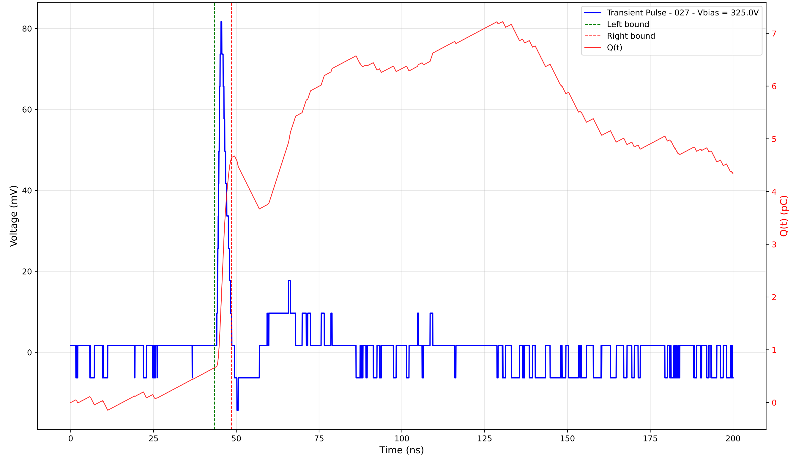
Transient Pulse - Sample: TD_4004 - Position: 435.0 \mu\text{m} - Charge: 3.98 pC - Rise Time: 0.98 ns
