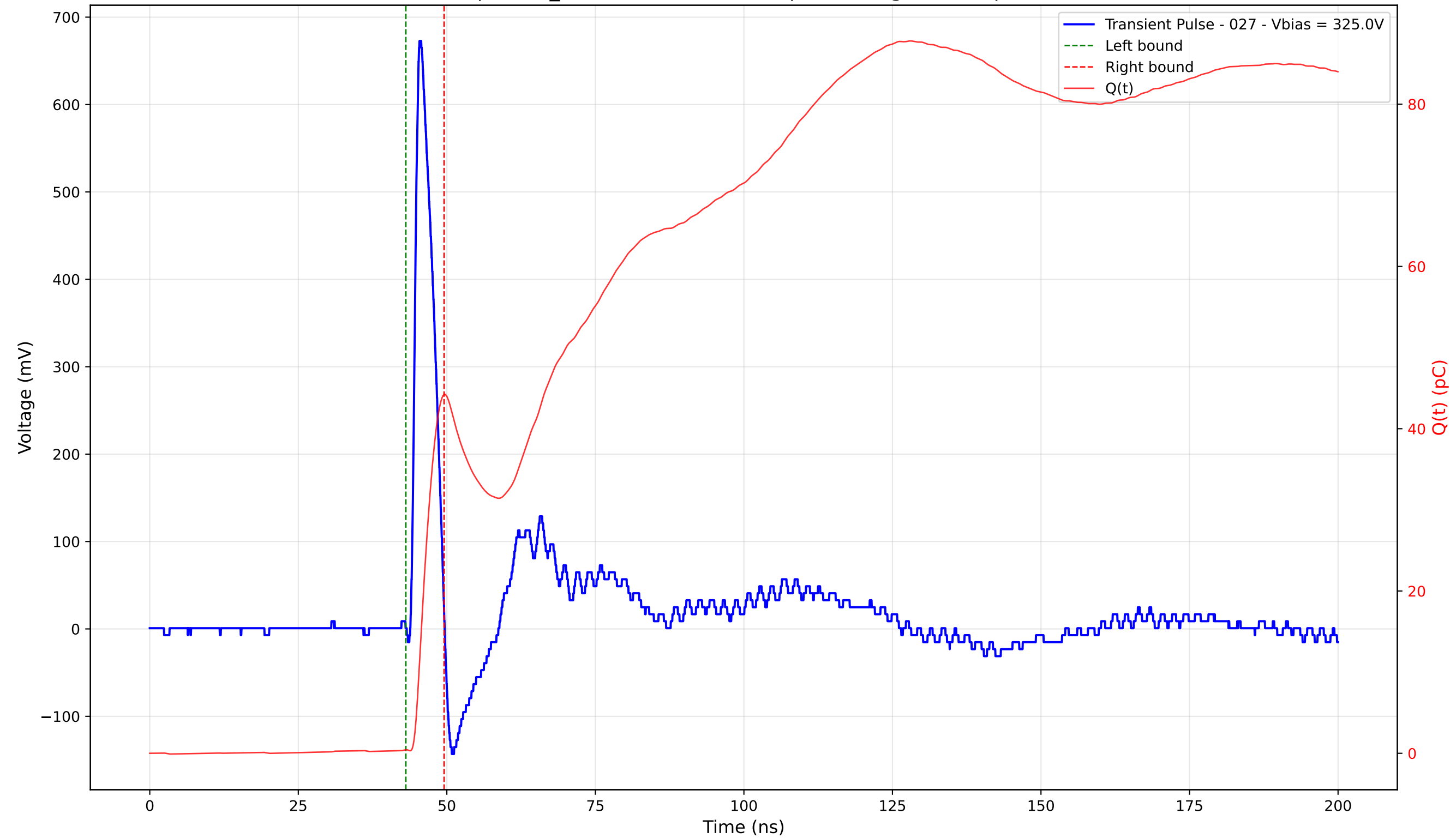
Transient Pulse - Sample: TD_4004 - Position: 375.0 \mu\text{m} - Charge: 43.79 pC - Rise Time: 0.99 ns
