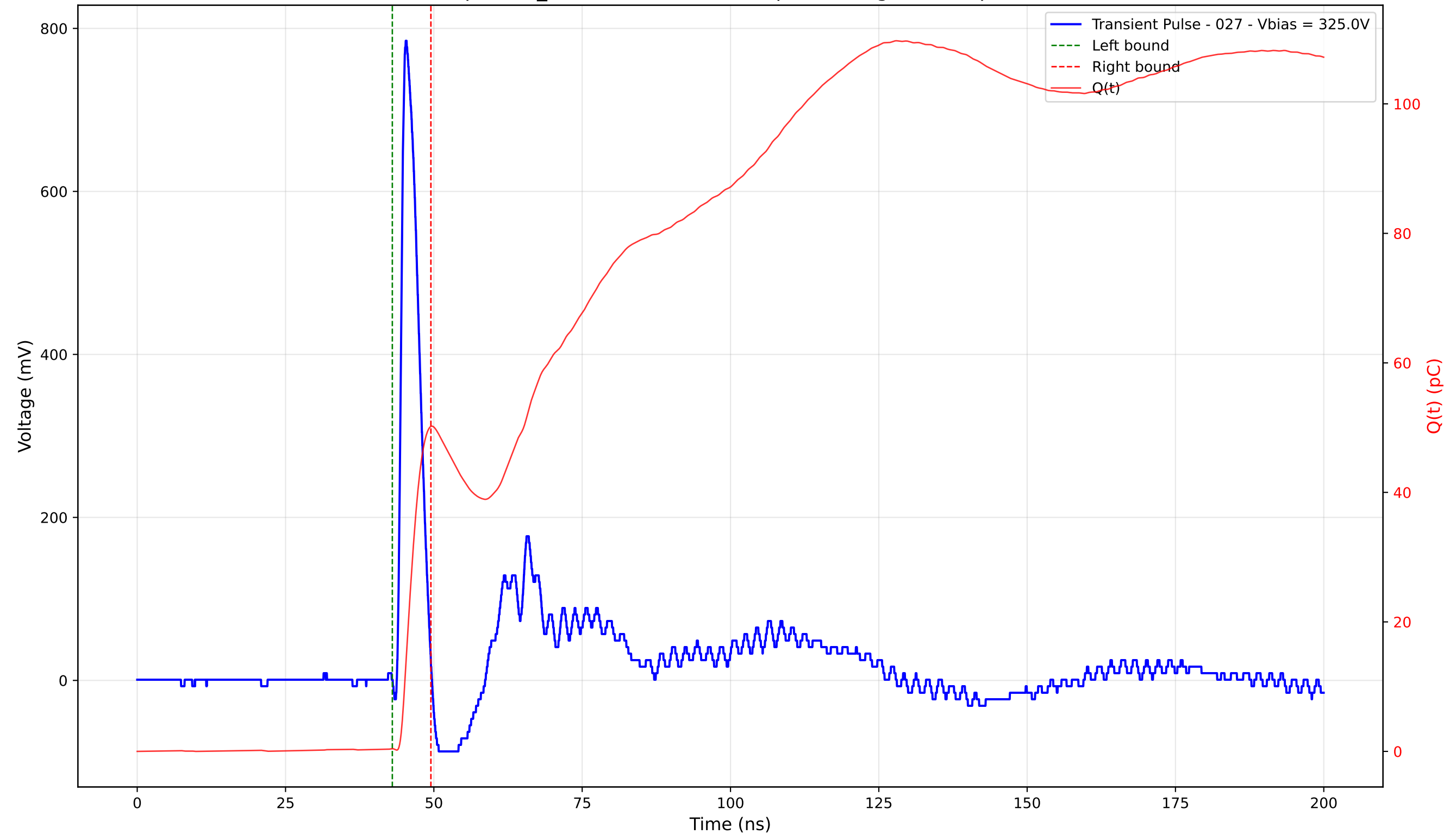
Transient Pulse - Sample: TD_4004 - Position: 155.0 \mu\text{m} - Charge: 49.77 pC - Rise Time: 0.92 ns
