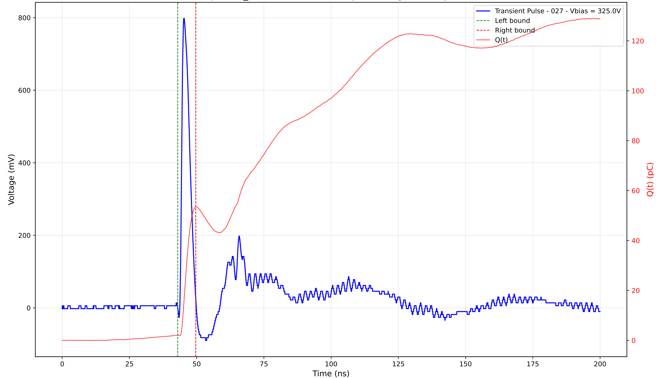
Transient Pulse - Sample: TD_4004 - Position: 210.0 \mu\text{m} - Charge: 51.38 pC - Rise Time: 0.90 ns
