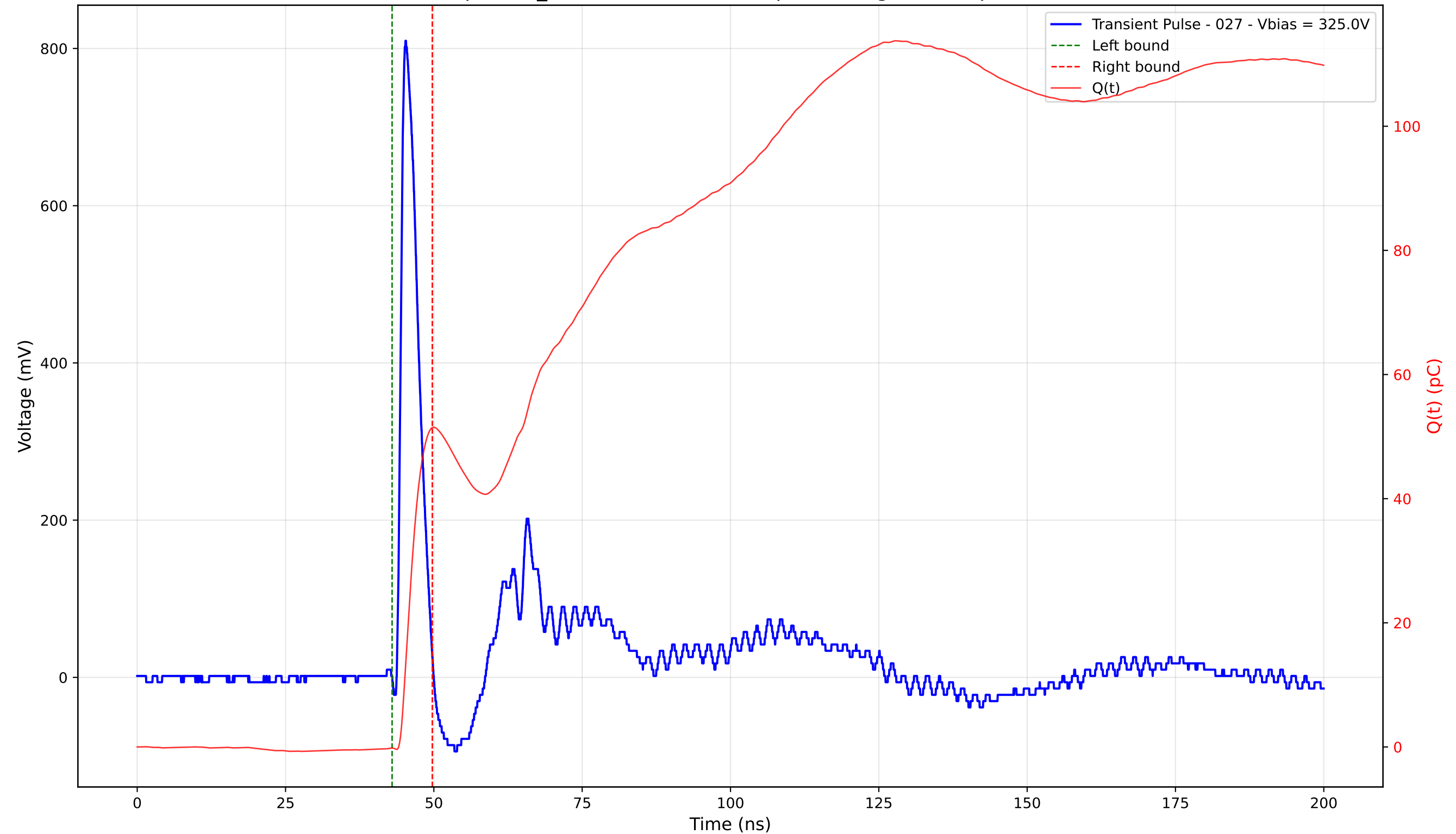
Transient Pulse - Sample: TD_4004 - Position: 180.0 \mu\text{m} - Charge: 51.62 pC - Rise Time: 0.88 ns
