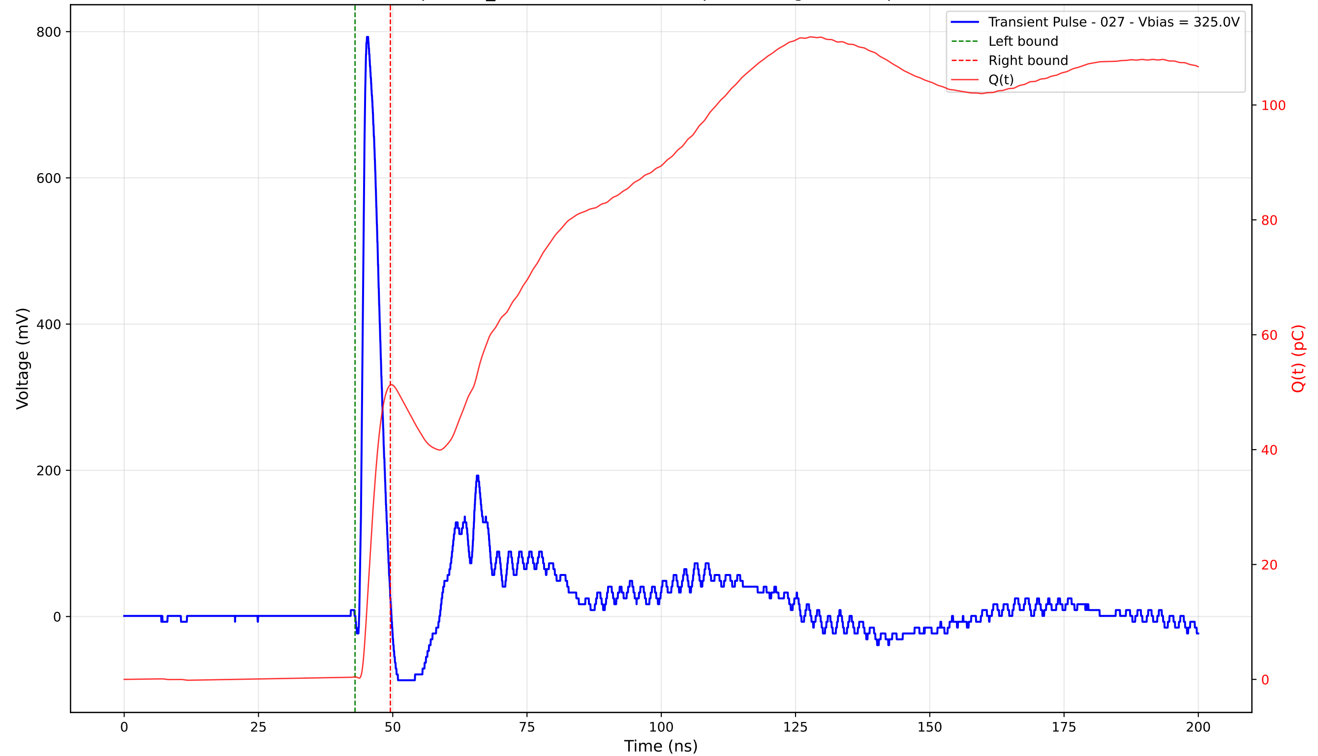
Transient Pulse - Sample: TD_4004 - Position: 165.0 \mu\text{m} - Charge: 50.81 pC - Rise Time: 0.89 ns
