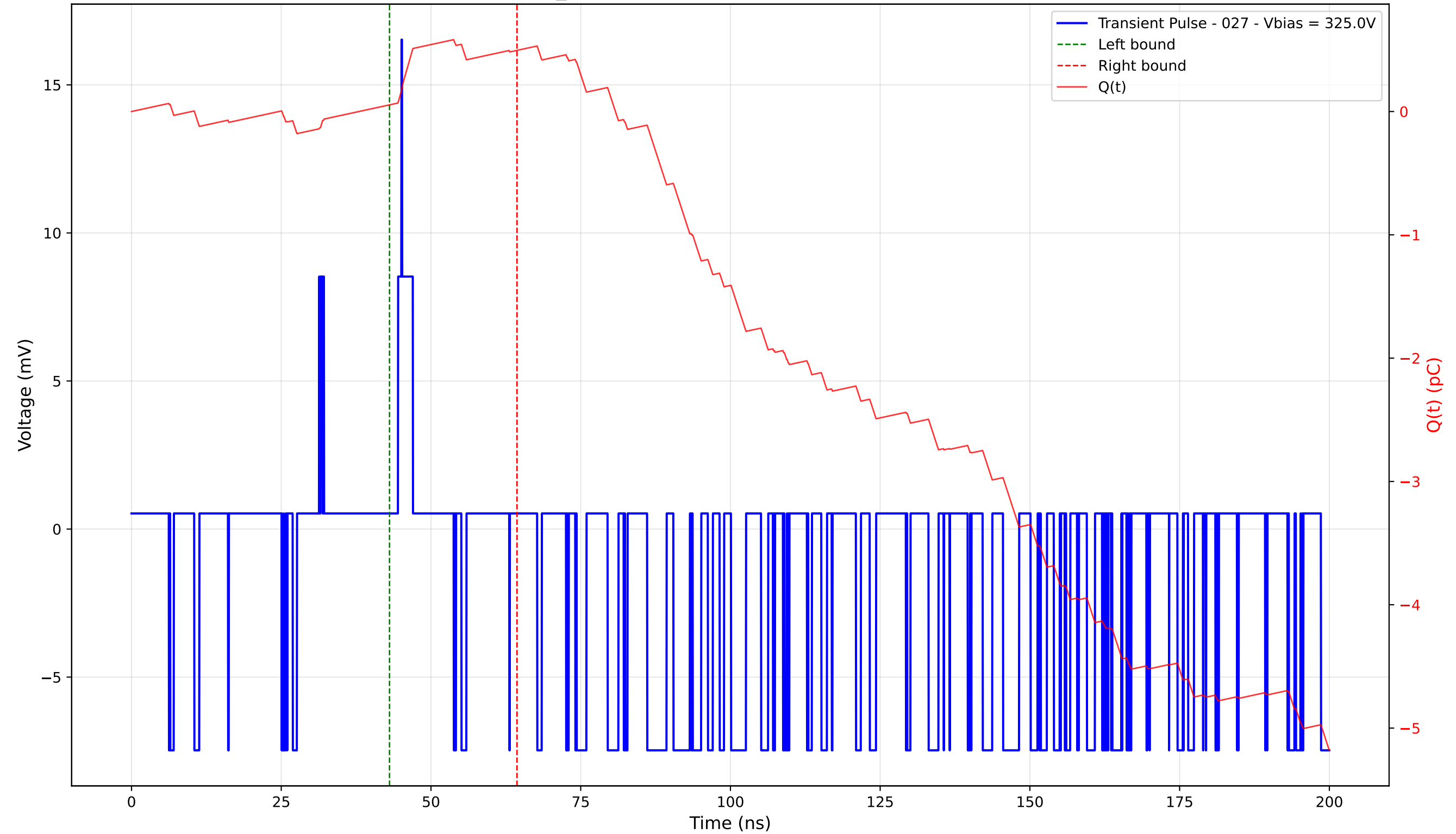
Transient Pulse - Sample: TD_4004 - Position: 0.0 \mu\text{m} - Charge: 0.44 pC - Rise Time: 0.58 ns
