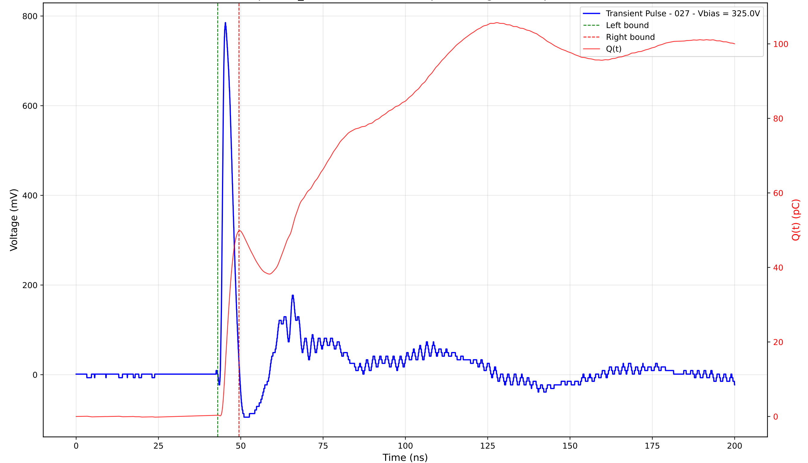
Transient Pulse - Sample: TD_4004 - Position: 145.0 \mu\text{m} - Charge: 49.46 pC - Rise Time: 0.91 ns
