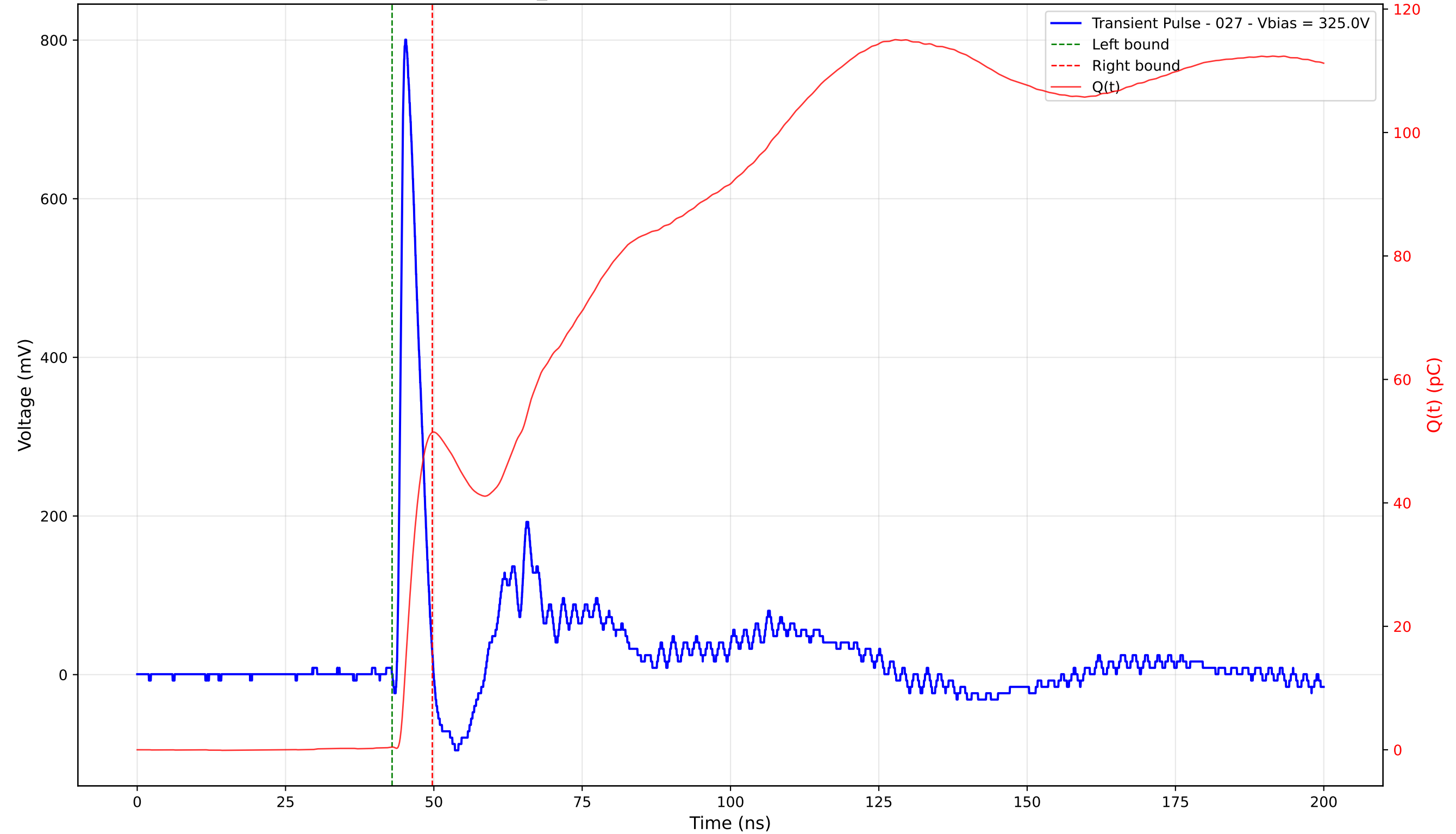
Transient Pulse - Sample: TD_4004 - Position: 115.0 \mu\text{m} - Charge: 50.96 pC - Rise Time: 0.89 ns
