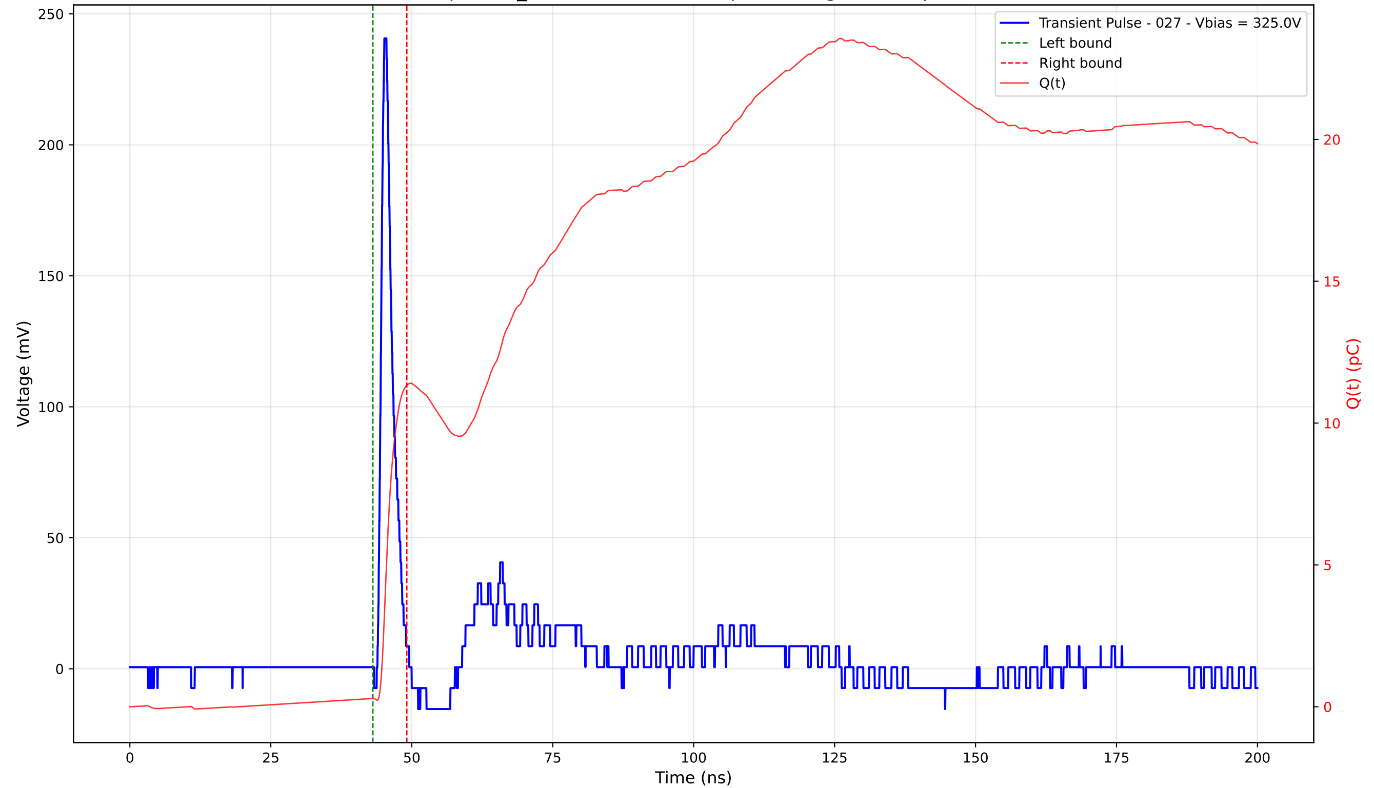
Transient Pulse - Sample: TD_4004 - Position: 55.0 \mu\text{m} - Charge: 11.04 pC - Rise Time: 0.88 ns
