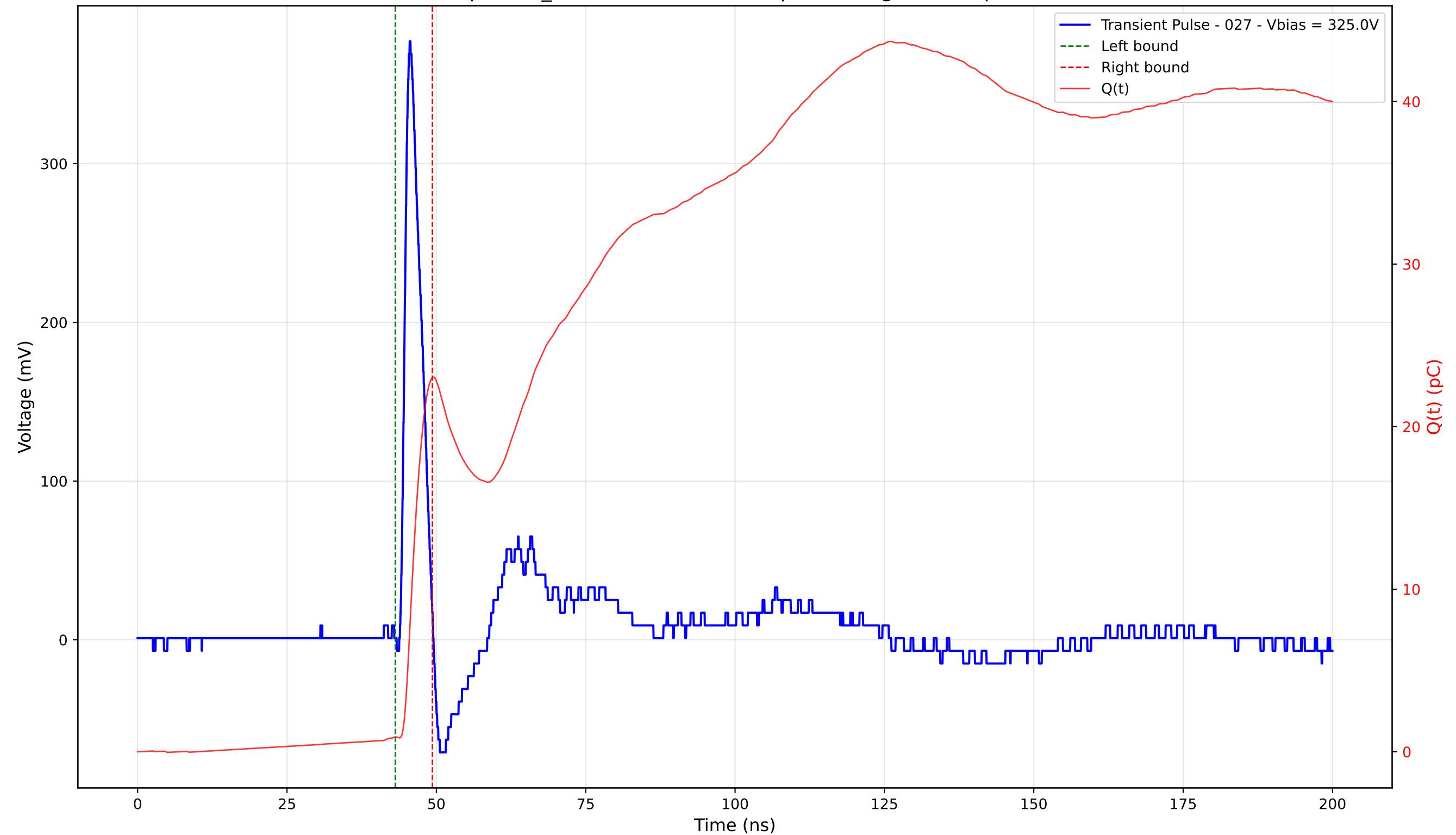
Transient Pulse - Sample: TD_4004 - Position: 400.0 \mu\text{m} - Charge: 22.12 pC - Rise Time: 1.09 ns
