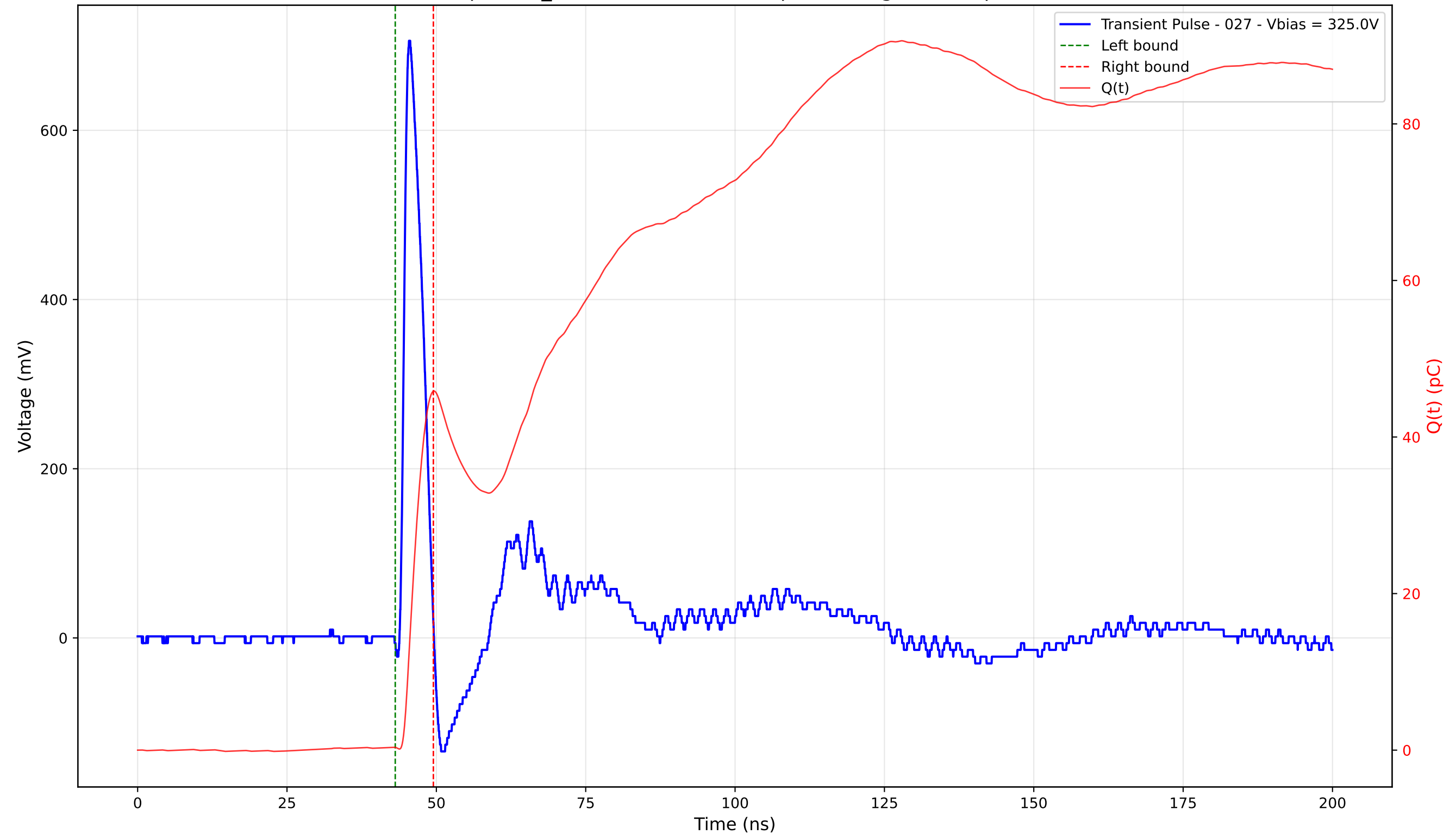
Transient Pulse - Sample: TD_4004 - Position: 345.0 \mu\text{m} - Charge: 45.50 pC - Rise Time: 0.99 ns
