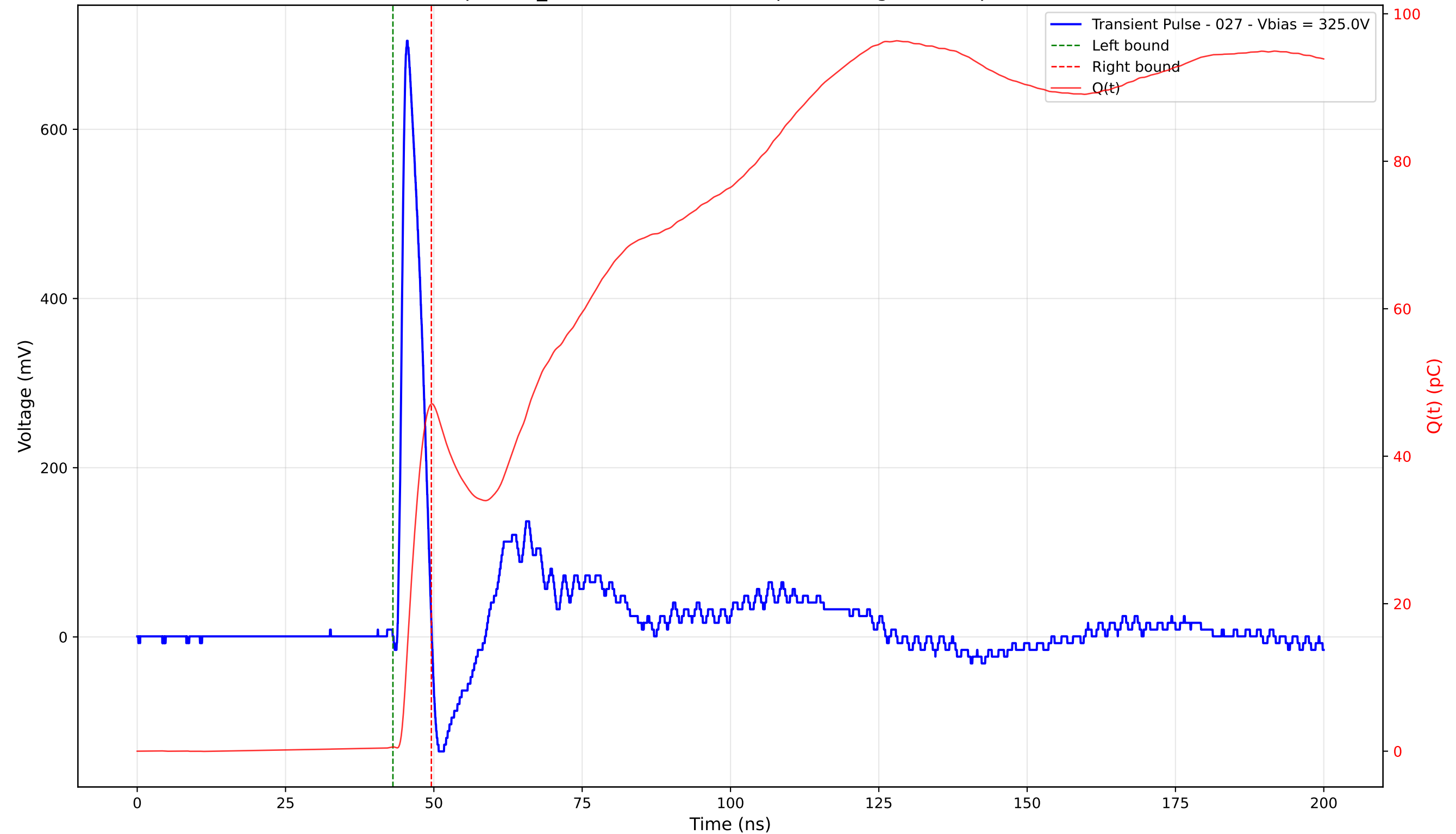
Transient Pulse - Sample: TD_4004 - Position: 355.0 \mu\text{m} - Charge: 46.51 pC - Rise Time: 1.01 ns
