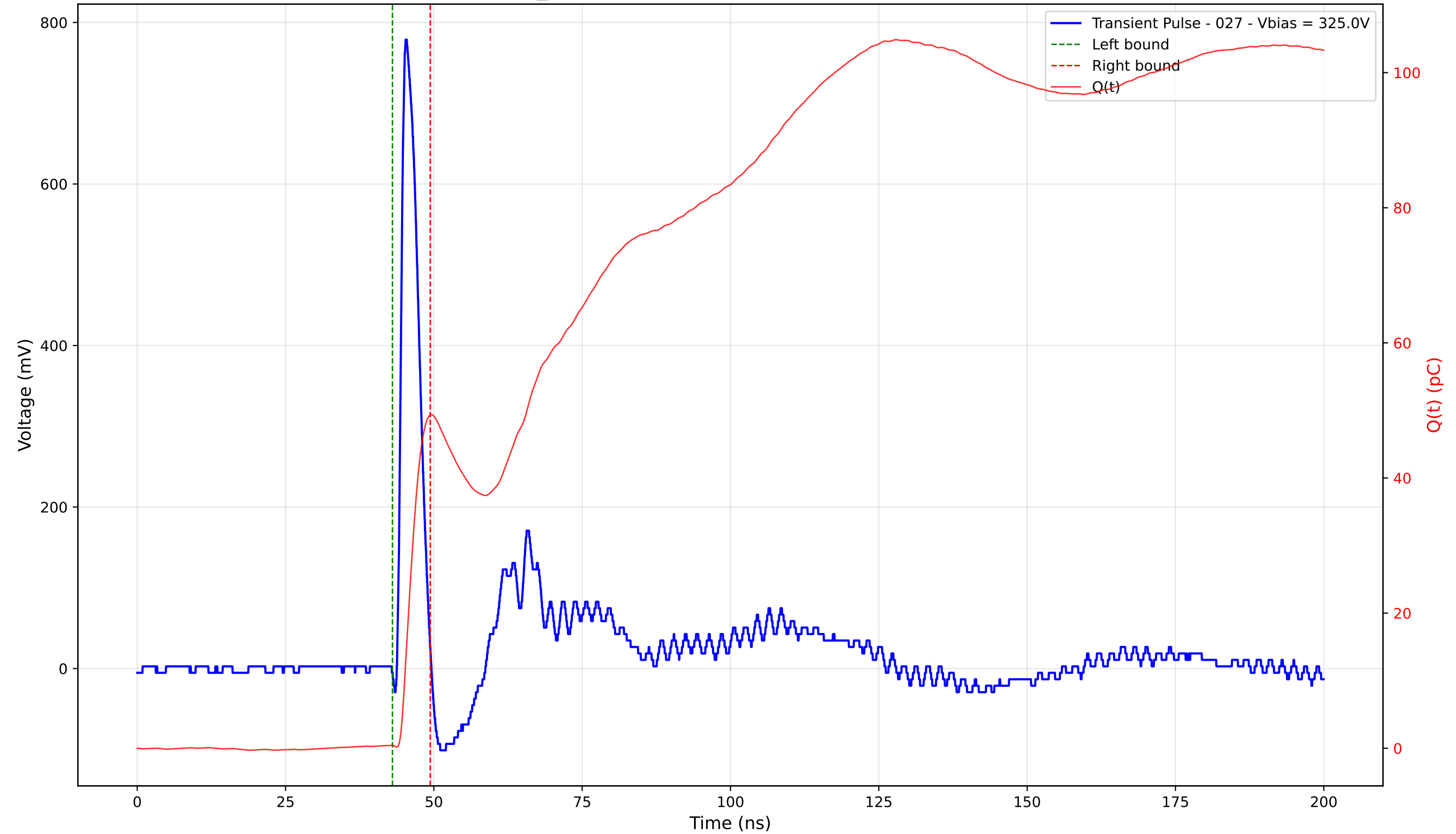
Transient Pulse - Sample: TD_4004 - Position: 240.0 \mu\text{m} - Charge: 48.90 pC - Rise Time: 0.92 ns
