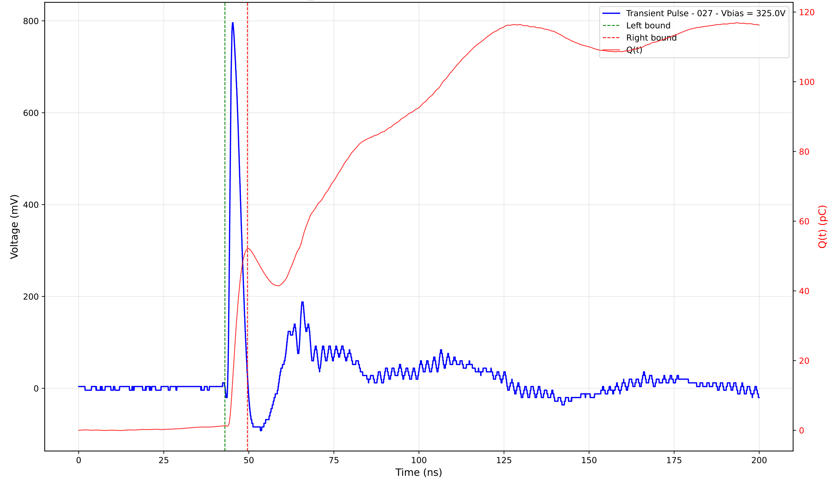
Transient Pulse - Sample: TD_4004 - Position: 125.0 \mu\text{m} - Charge: 50.75 pC - Rise Time: 0.89 ns
