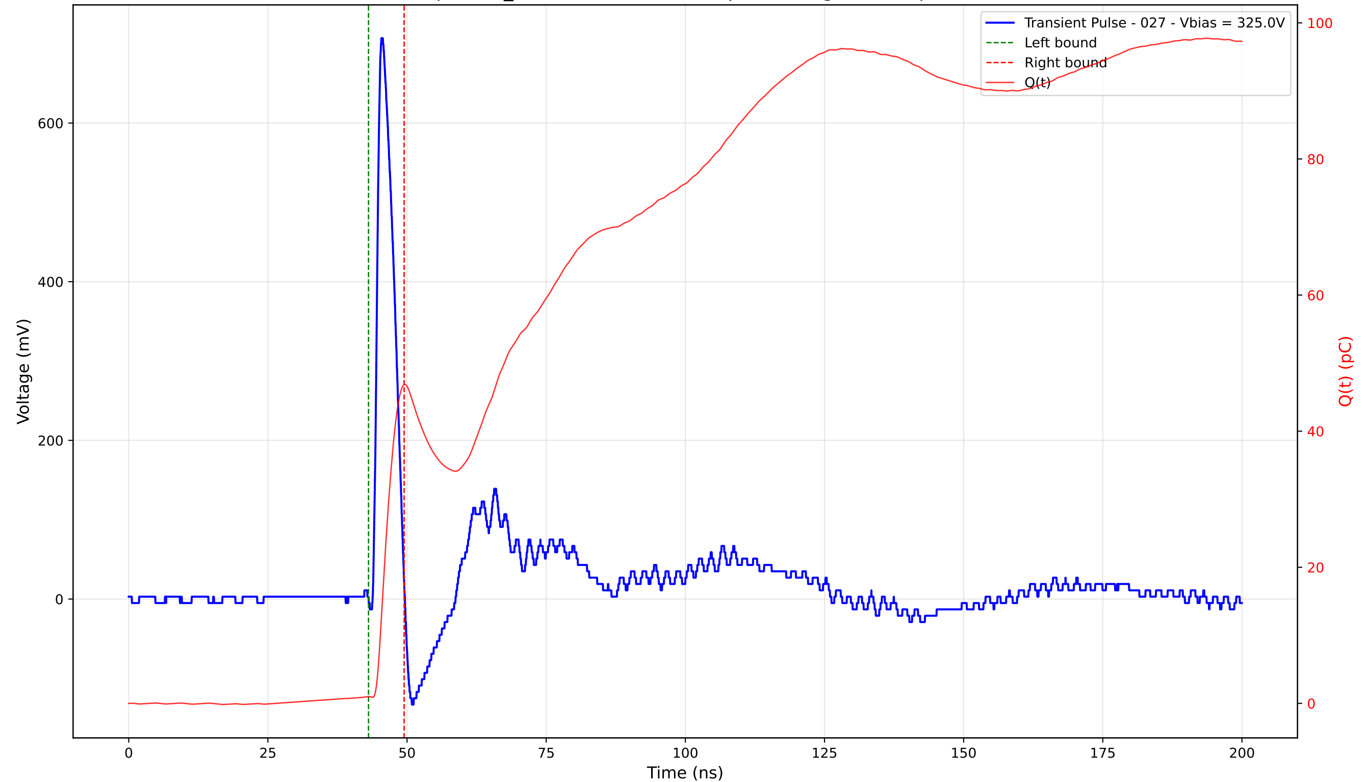
Transient Pulse - Sample: TD_4004 - Position: 340.0 \mu\text{m} - Charge: 45.83 pC - Rise Time: 0.99 ns
