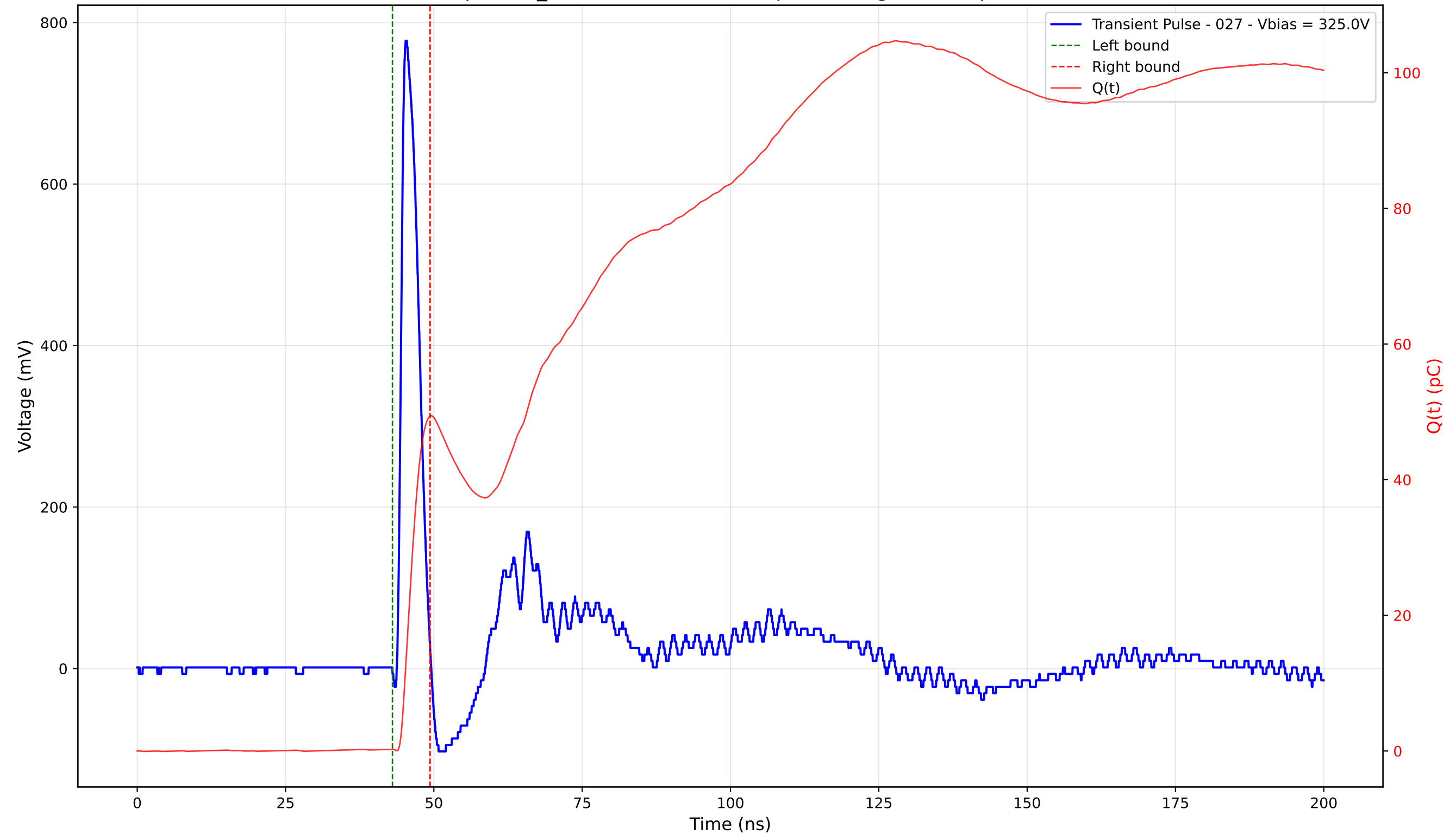
Transient Pulse - Sample: TD_4004 - Position: 245.0 \mu\text{m} - Charge: 49.13 pC - Rise Time: 0.91 ns
