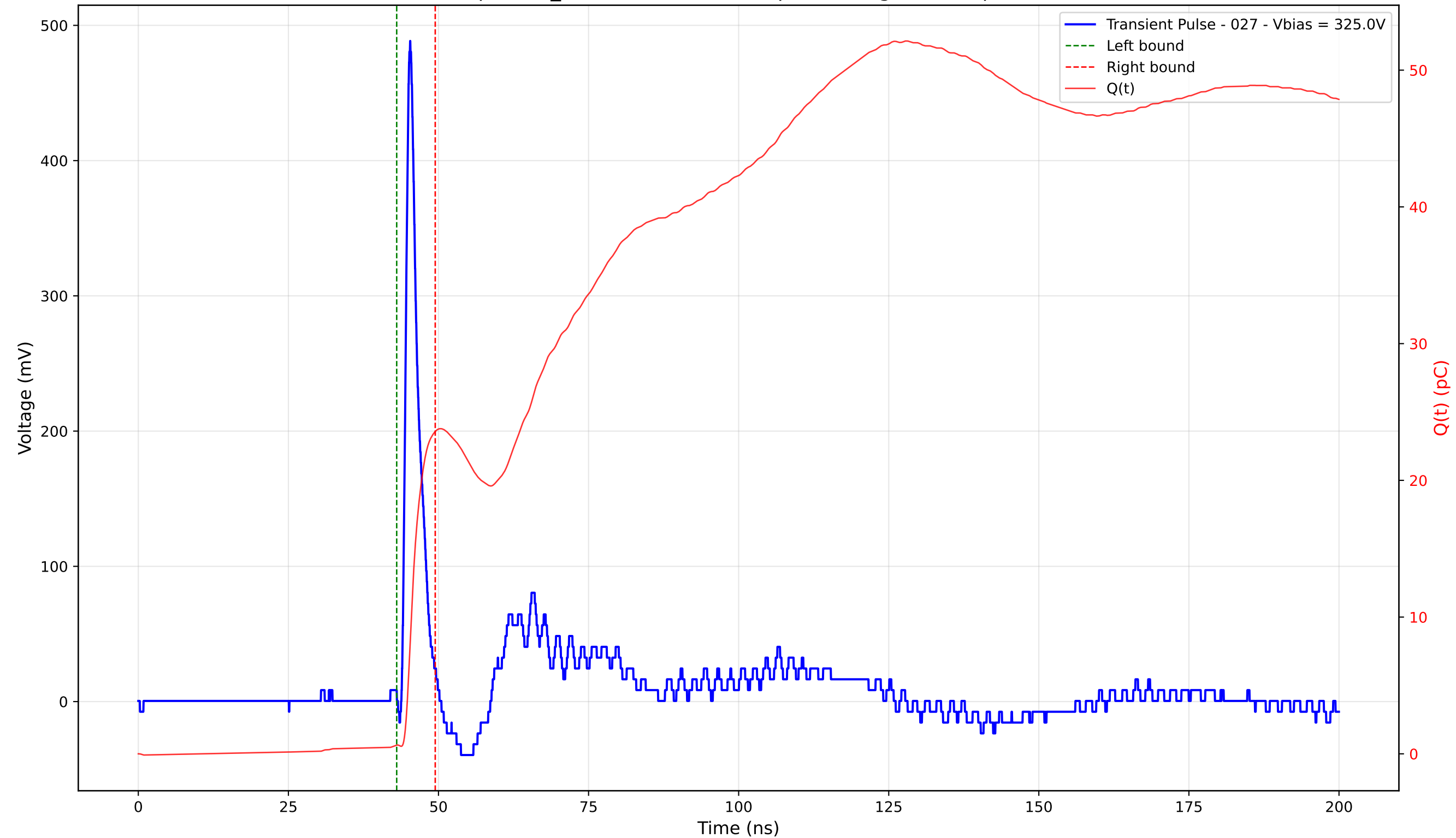
Transient Pulse - Sample: TD_4004 - Position: 65.0 \mu\text{m} - Charge: 22.93 pC - Rise Time: 0.92 ns
