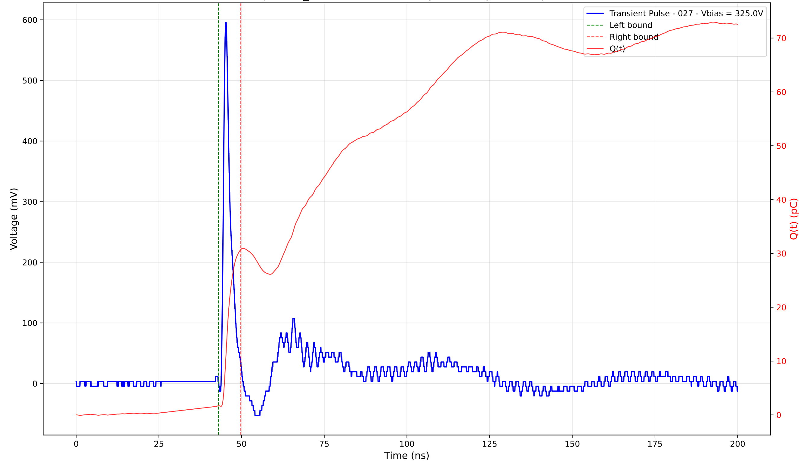
Transient Pulse - Sample: TD_4004 - Position: 70.0 \mu\text{m} - Charge: 29.04 pC - Rise Time: 0.89 ns
