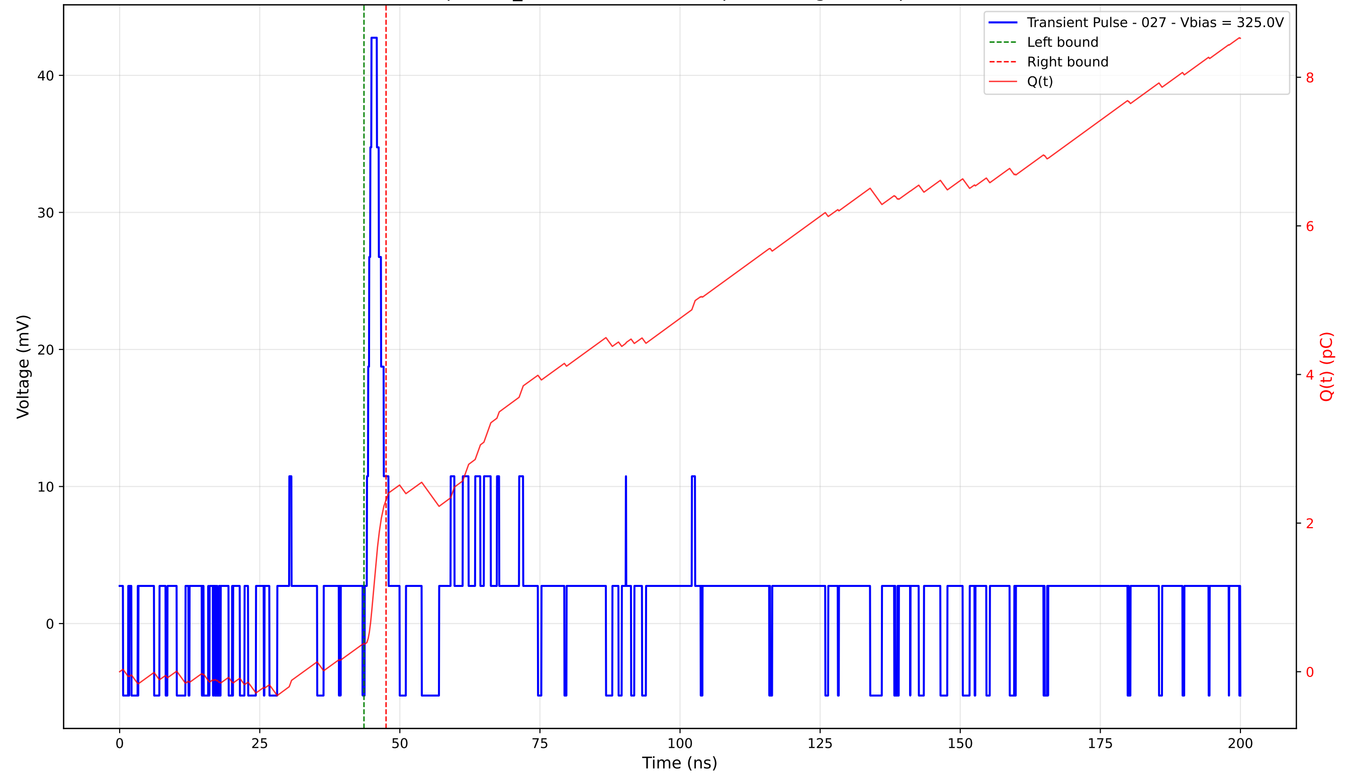
Transient Pulse - Sample: TD_4004 - Position: 35.0 \mu\text{m} - Charge: 1.93 pC - Rise Time: 0.82 ns
