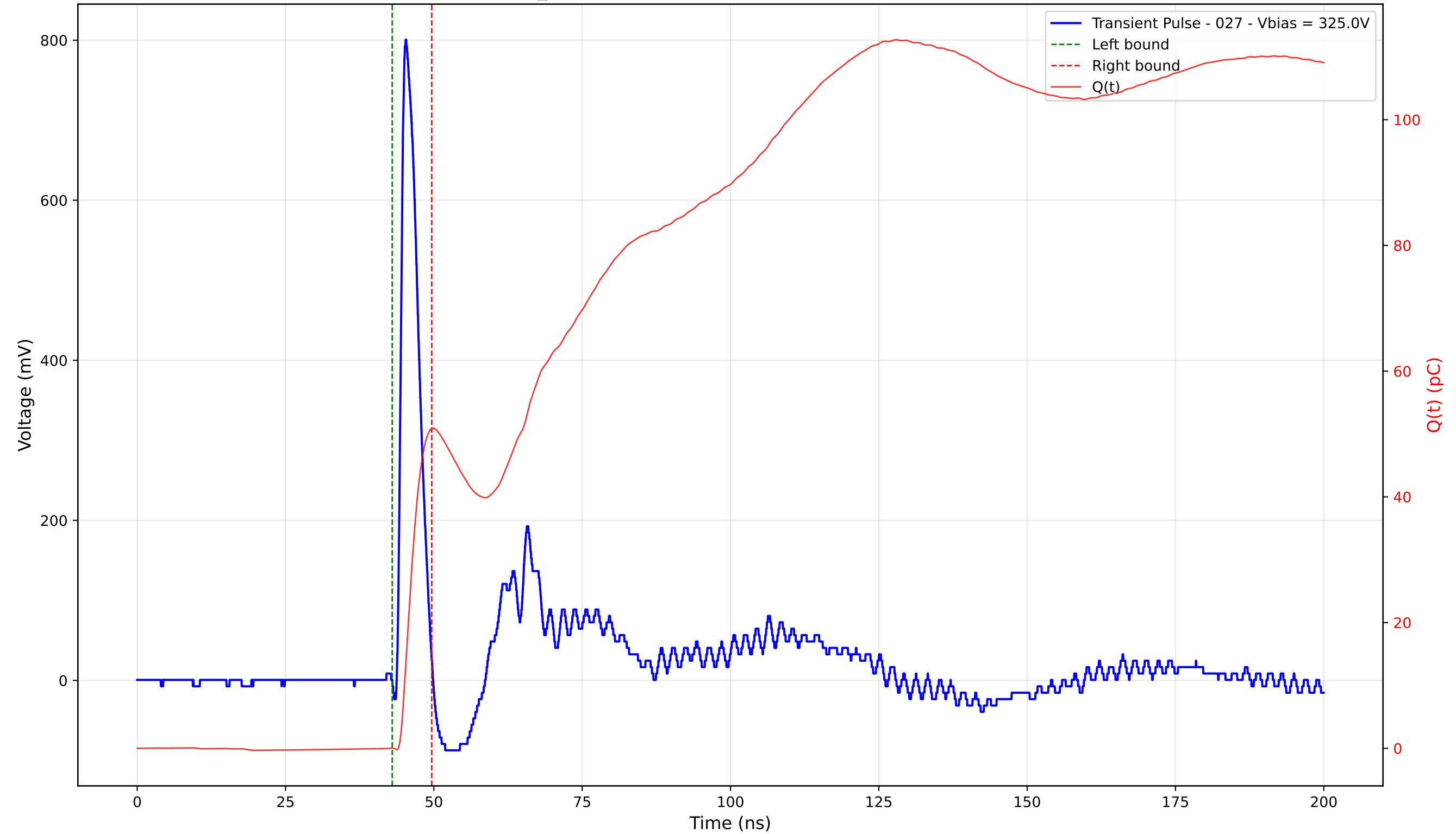
Transient Pulse - Sample: TD_4004 - Position: 205.0 \mu\text{m} - Charge: 50.82 pC - Rise Time: 0.90 ns
