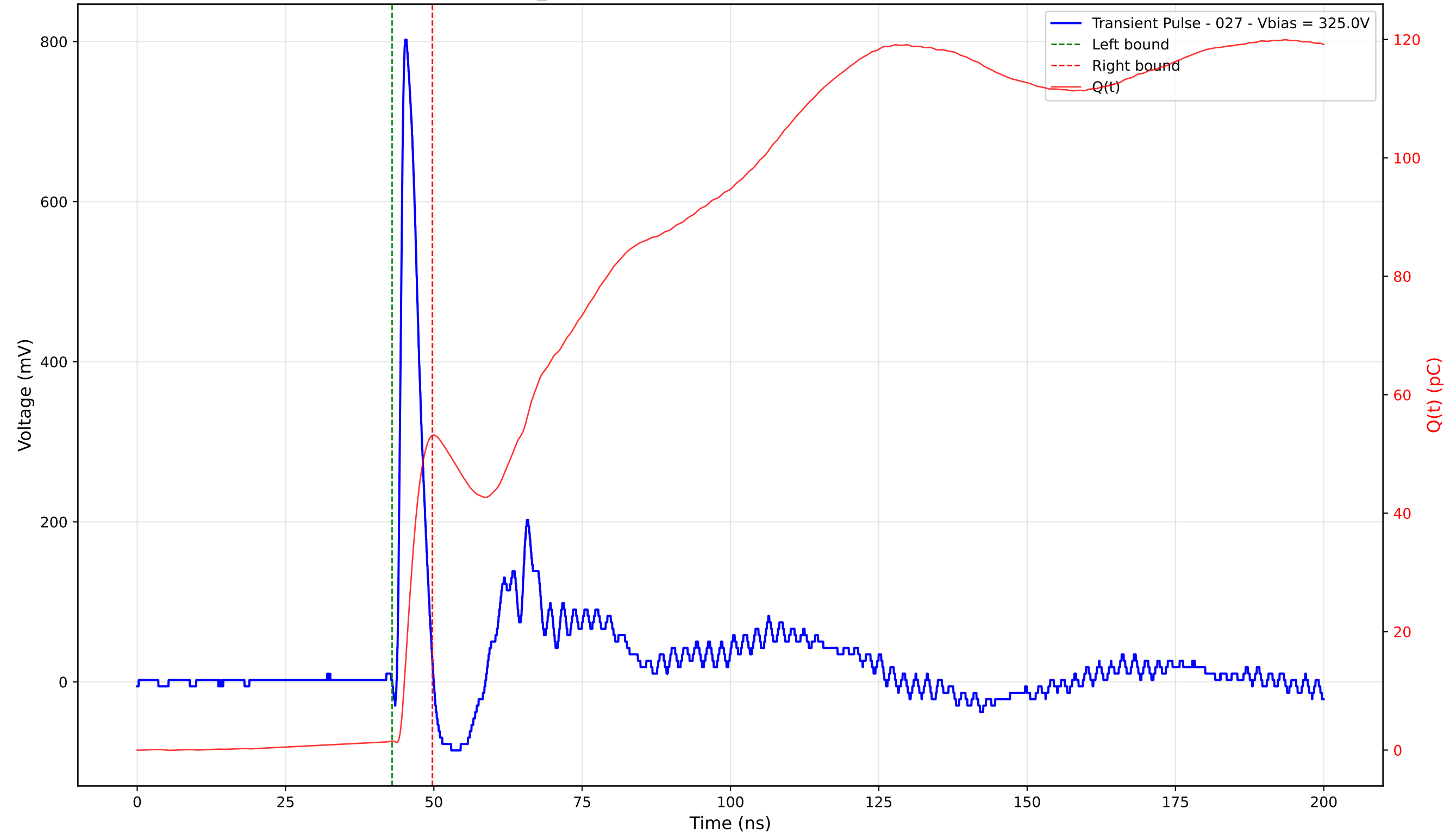
Transient Pulse - Sample: TD_4004 - Position: 200.0 \mu\text{m} - Charge: 51.60 pC - Rise Time: 0.88 ns
