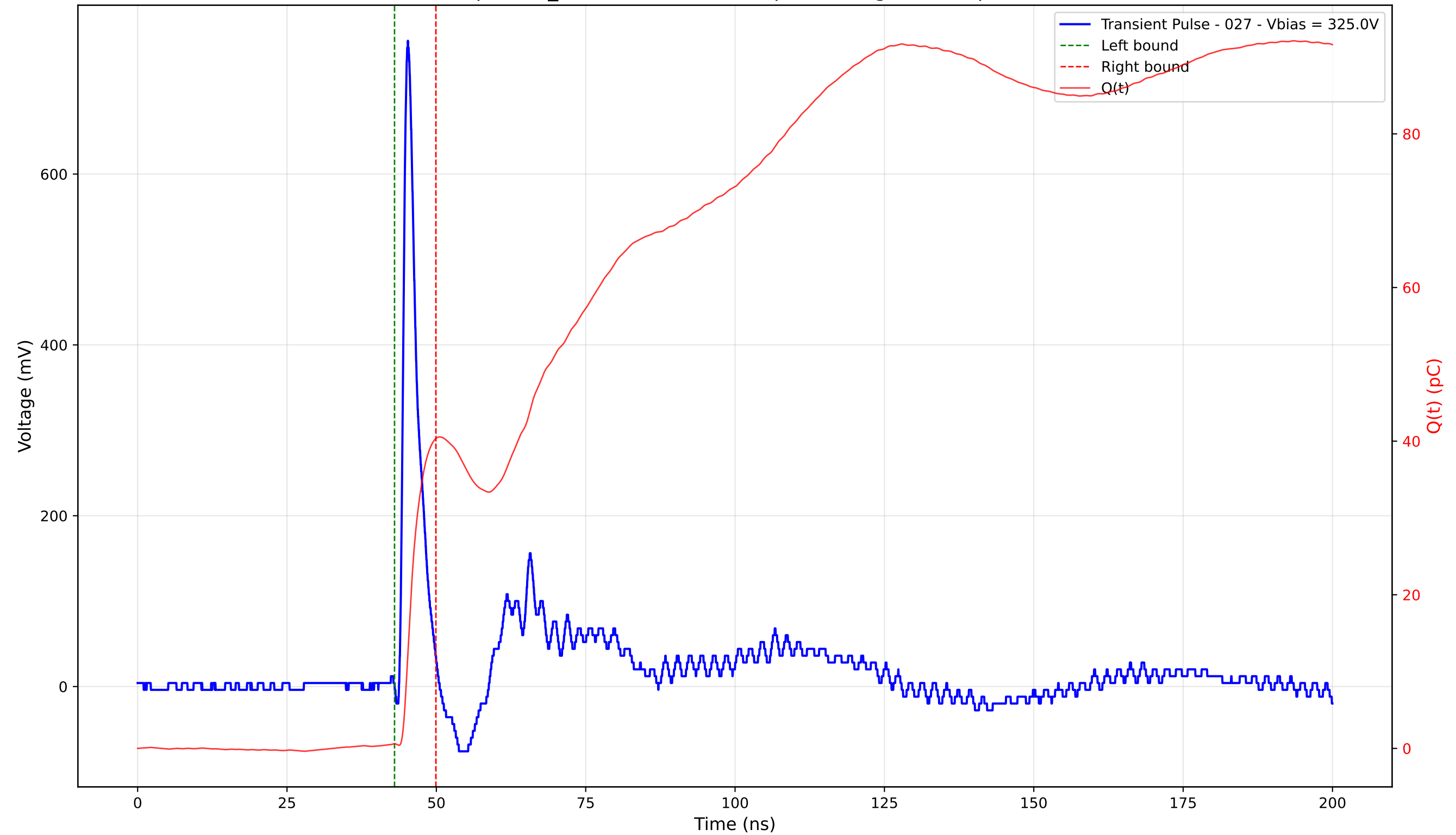
Transient Pulse - Sample: TD_4004 - Position: 85.0 \mu\text{m} - Charge: 39.74 pC - Rise Time: 0.89 ns
