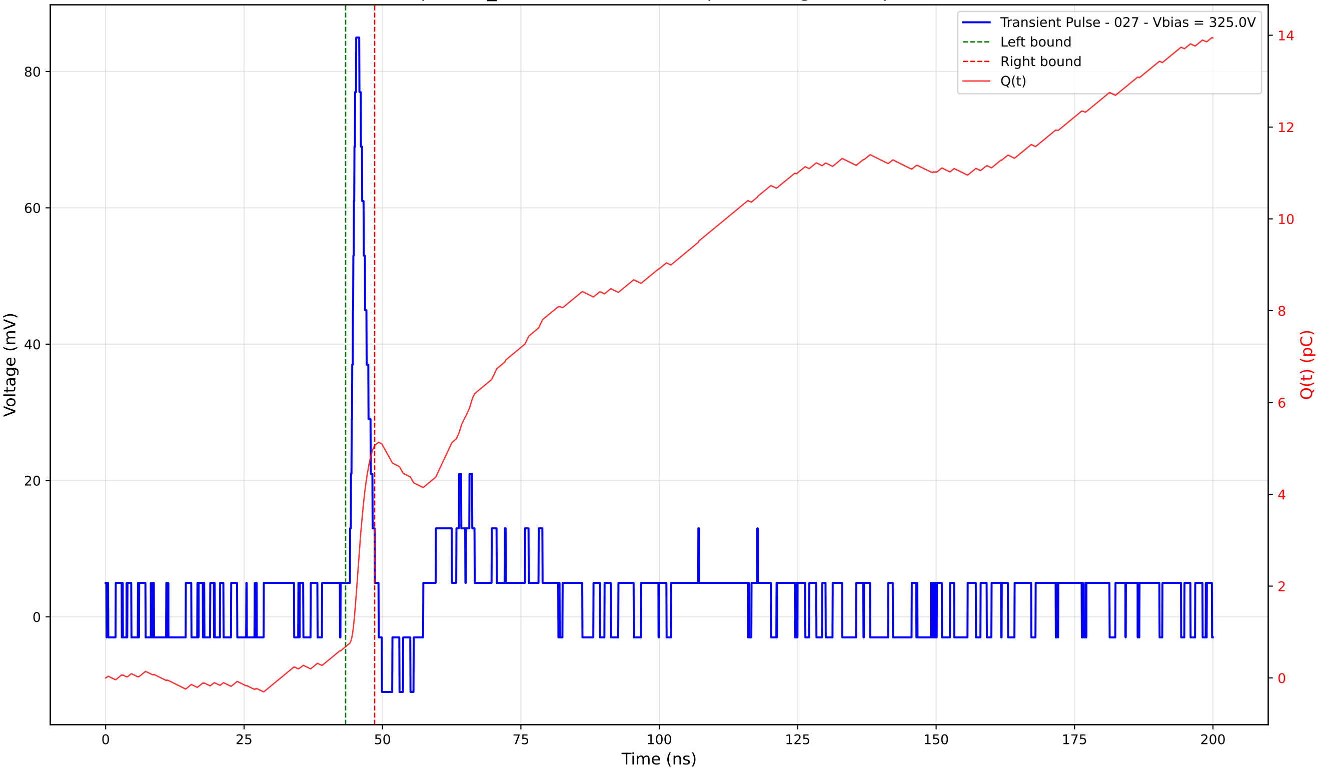
Transient Pulse - Sample: TD_4004 - Position: 425.0 \mu\text{m} - Charge: 4.38 pC - Rise Time: 0.91 ns
