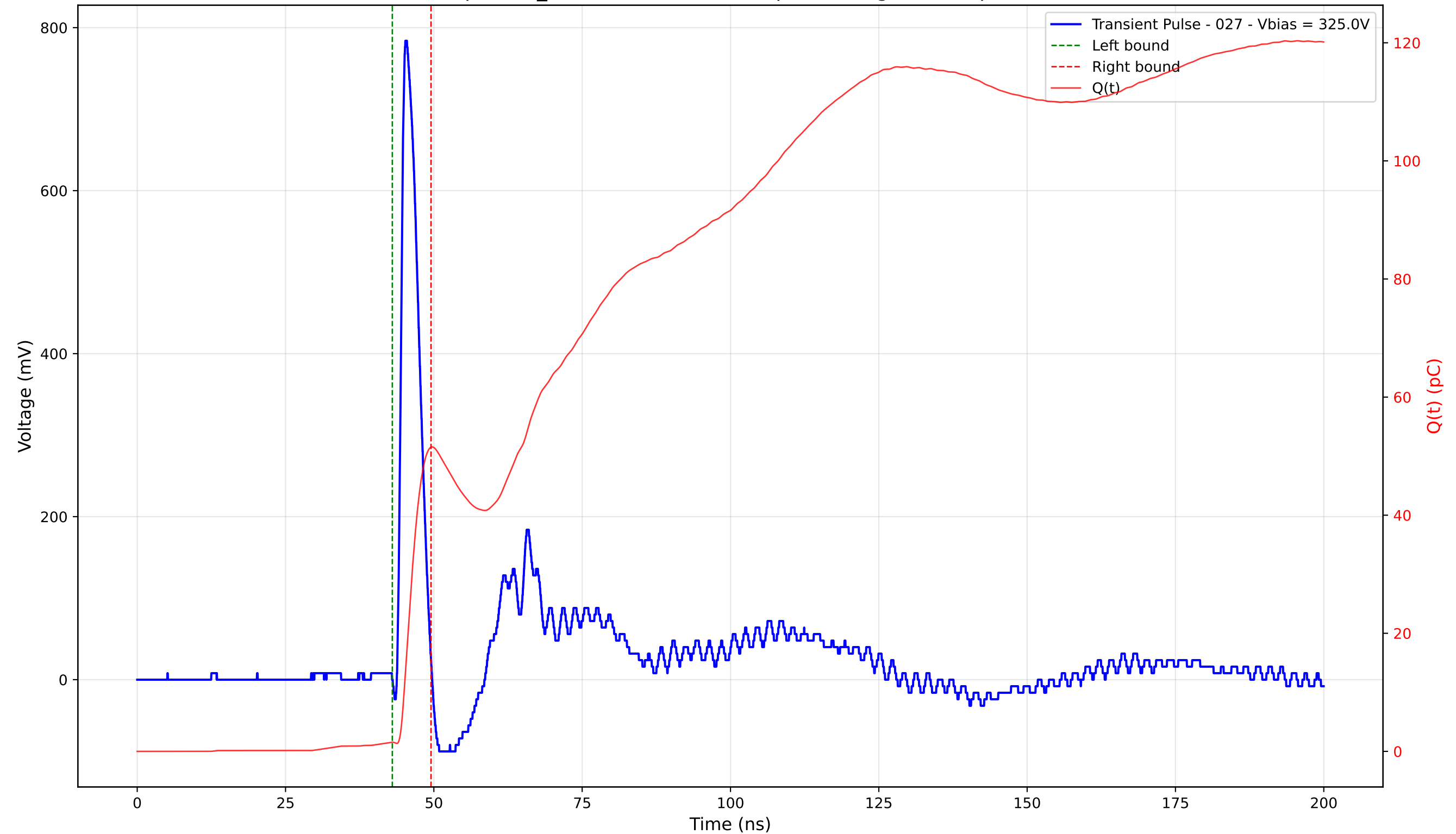
Transient Pulse - Sample: TD_4004 - Position: 150.0 \mu\text{m} - Charge: 49.96 pC - Rise Time: 0.90 ns
