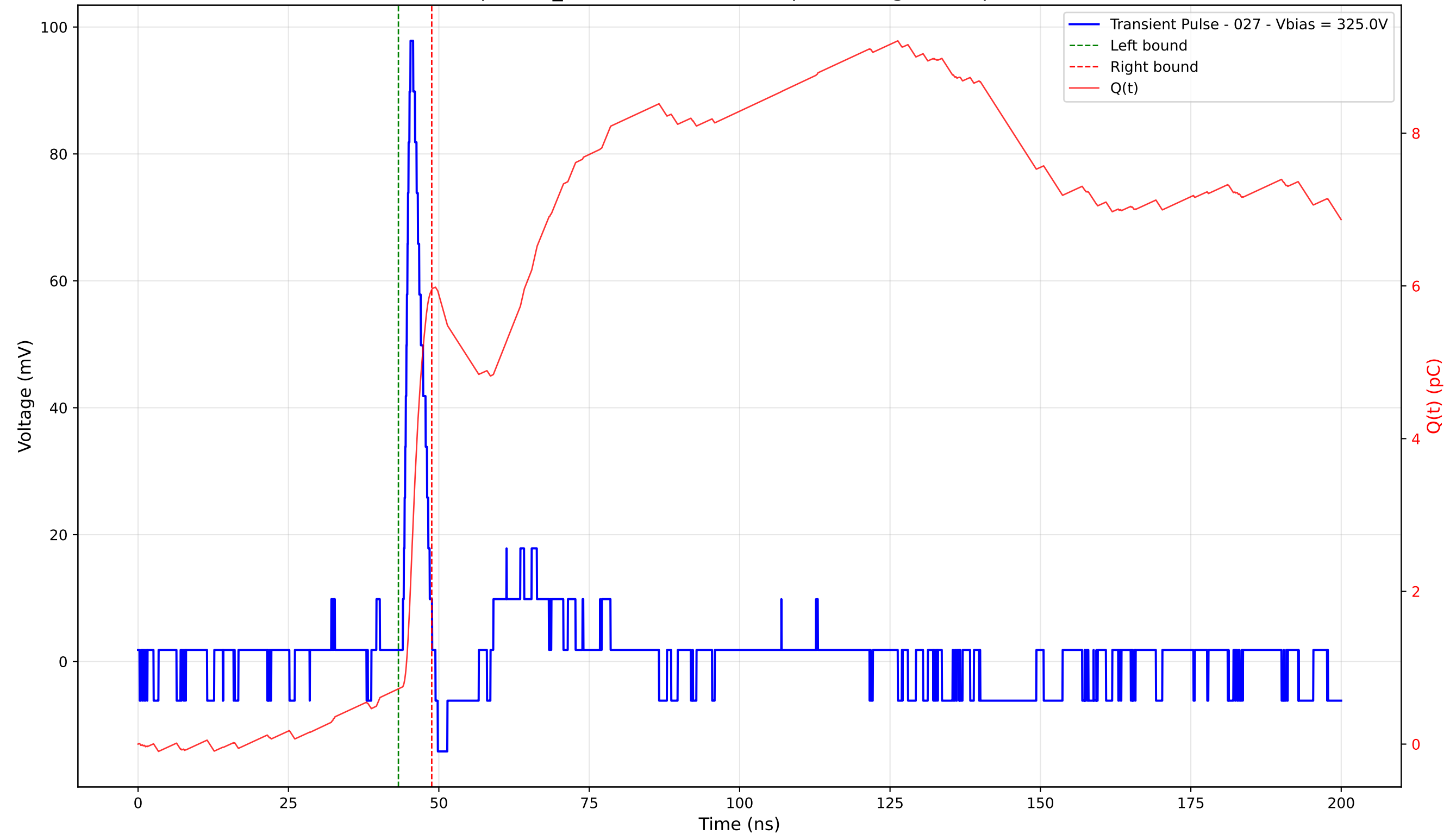
Transient Pulse - Sample: TD_4004 - Position: 420.0 \mu\text{m} - Charge: 5.23 pC - Rise Time: 1.10 ns
