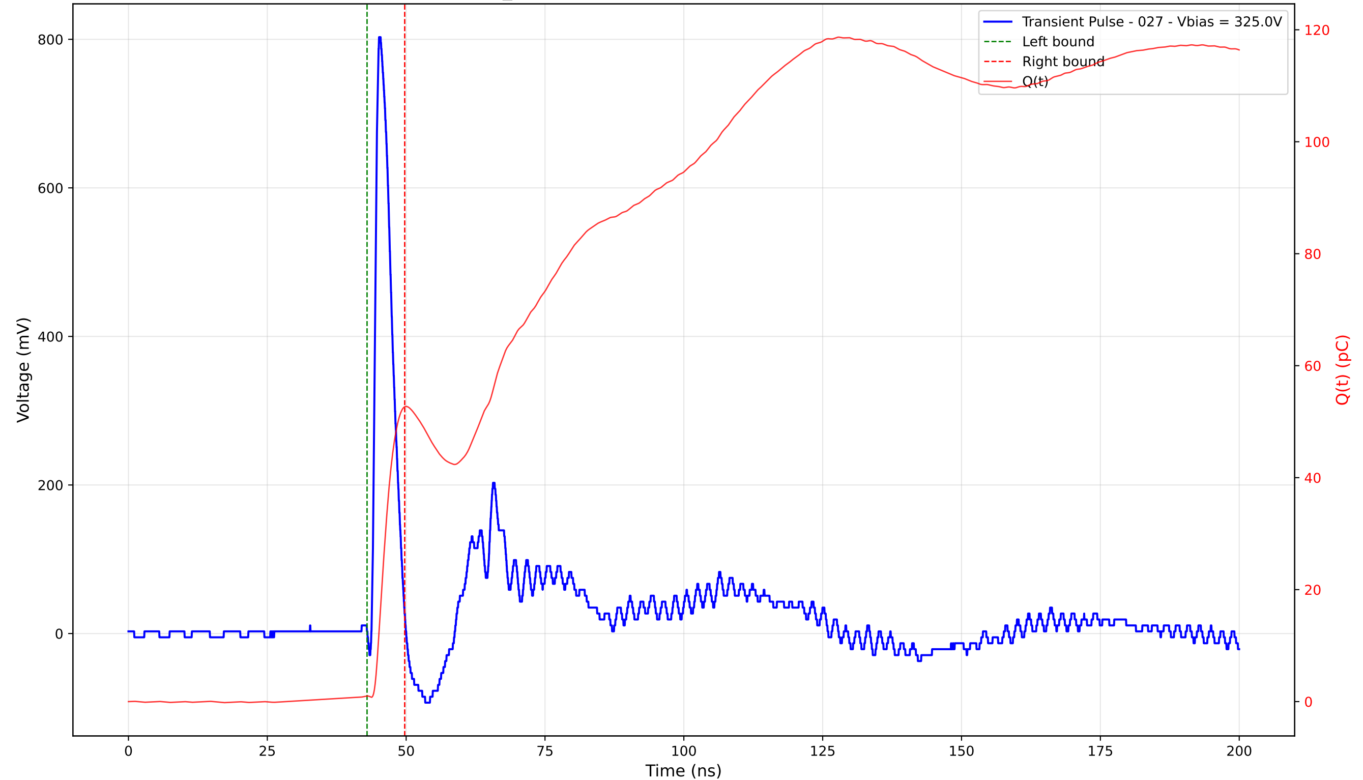
Transient Pulse - Sample: TD_4004 - Position: 195.0 \mu\text{m} - Charge: 51.65 pC - Rise Time: 0.89 ns
