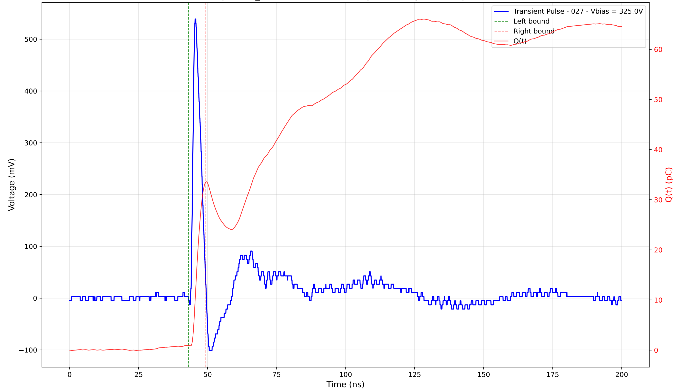
Transient Pulse - Sample: TD_4004 - Position: 390.0 \mu\text{m} - Charge: 32.58 pC - Rise Time: 1.04 ns
