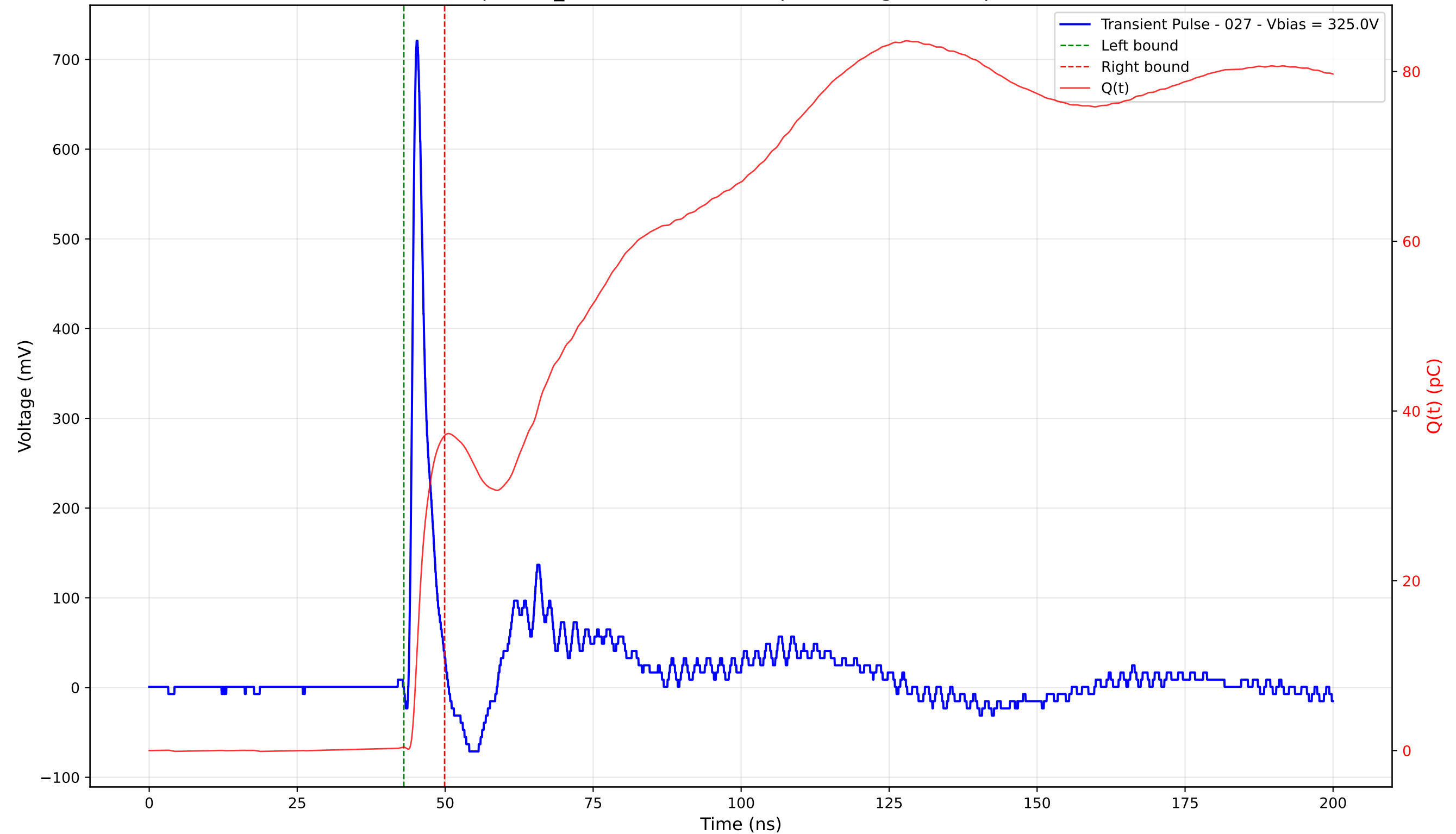
Transient Pulse - Sample: TD_4004 - Position: 80.0 \mu\text{m} - Charge: 36.71 pC - Rise Time: 0.88 ns
