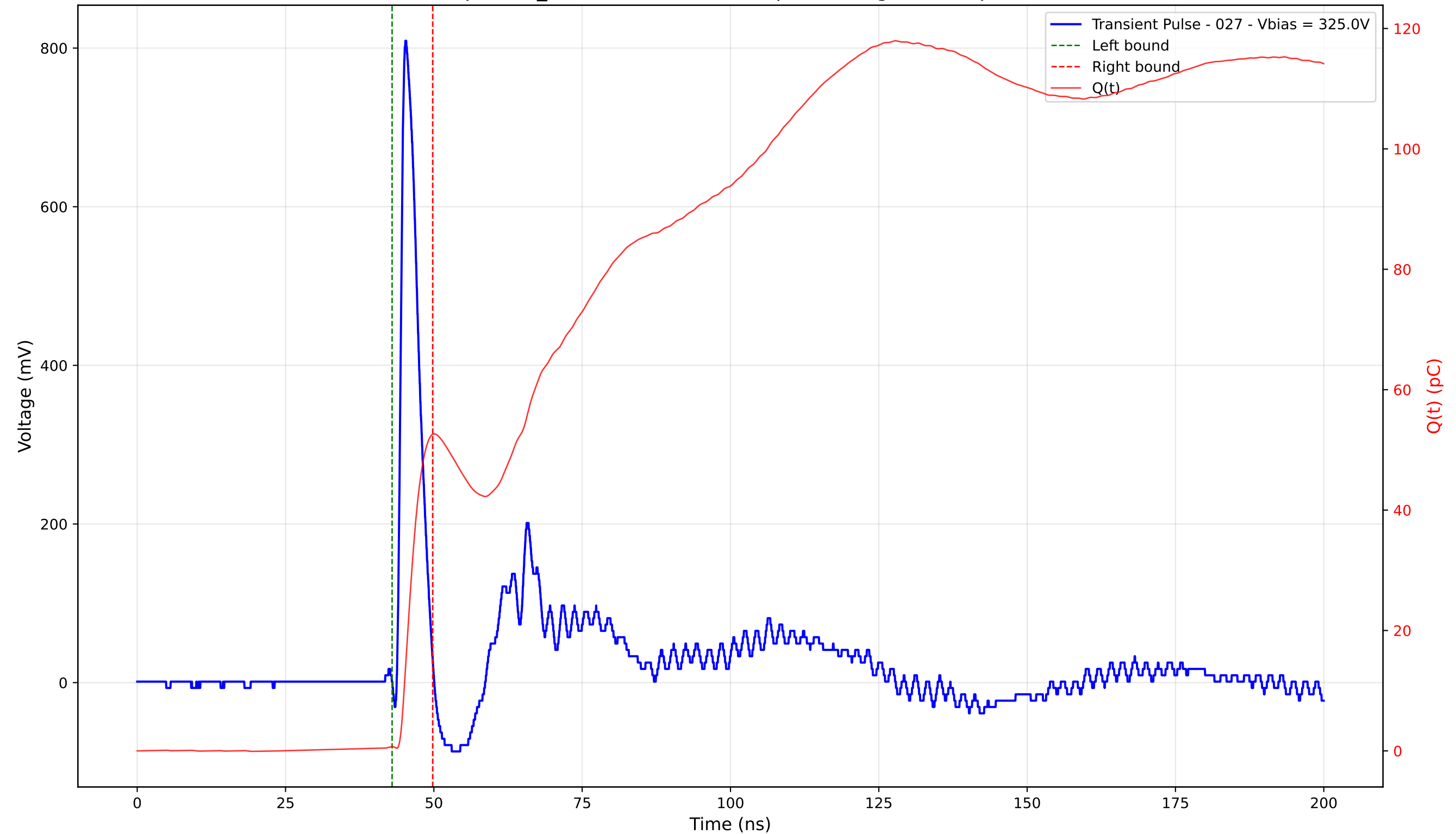
Transient Pulse - Sample: TD_4004 - Position: 190.0 \mu\text{m} - Charge: 51.90 pC - Rise Time: 0.88 ns
