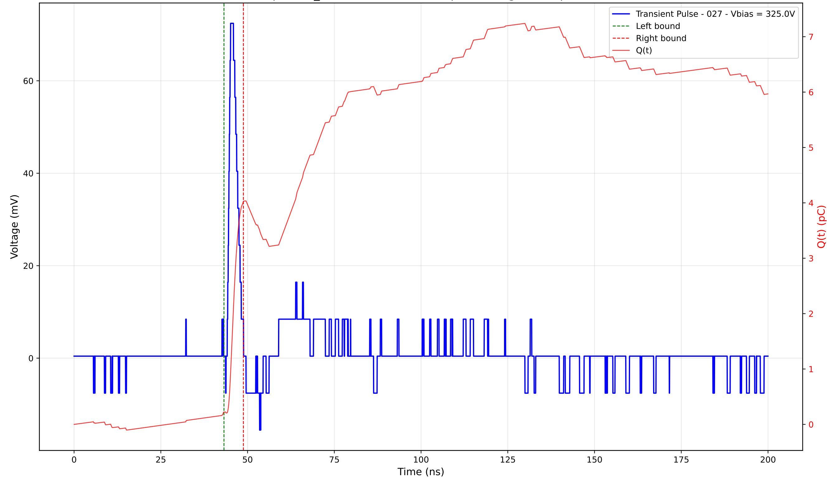
Transient Pulse - Sample: TD_4004 - Position: 430.0 \mu\text{m} - Charge: 3.80 pC - Rise Time: 0.96 ns
