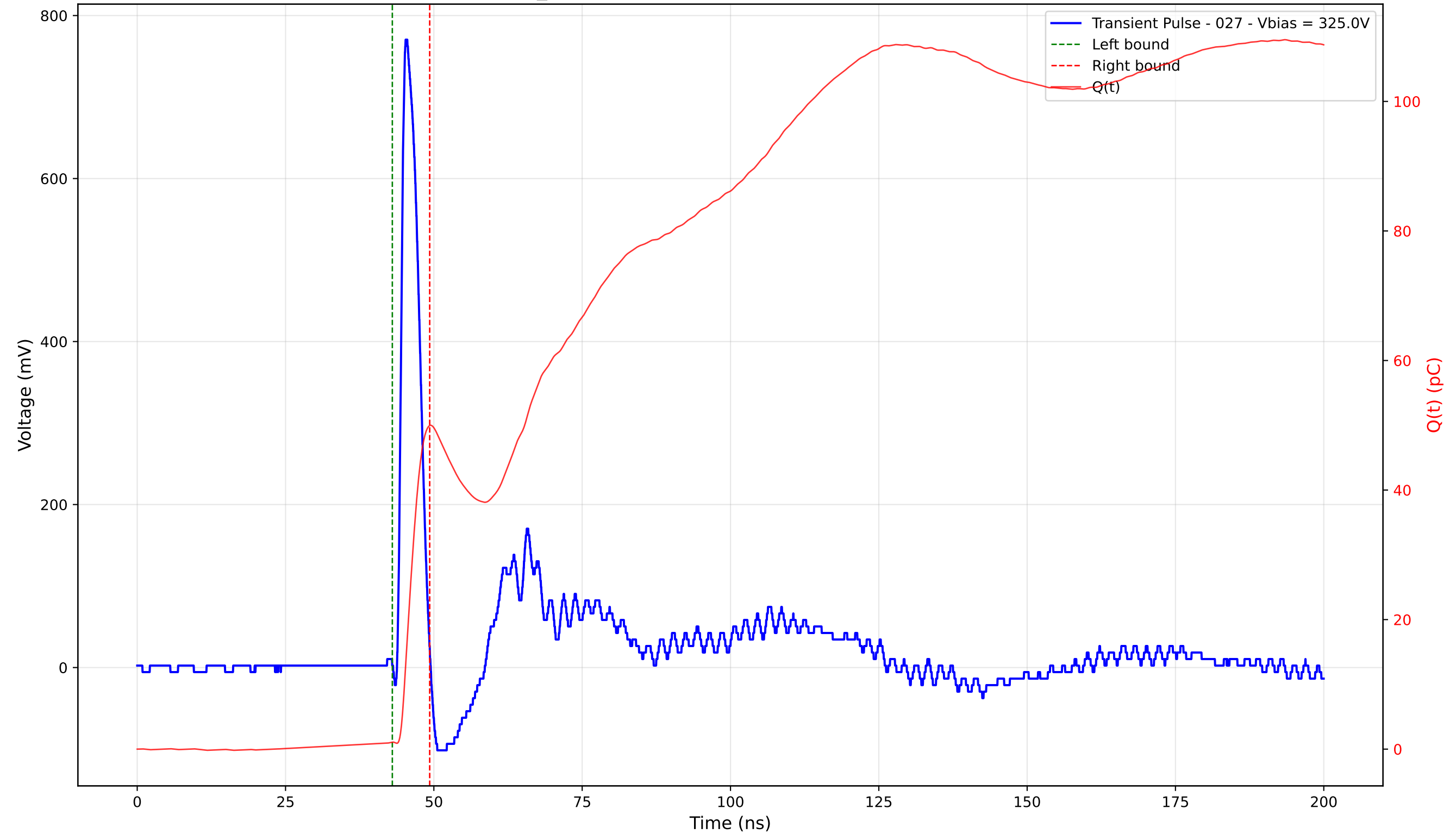
Transient Pulse - Sample: TD_4004 - Position: 260.0 \mu\text{m} - Charge: 48.89 pC - Rise Time: 0.92 ns
