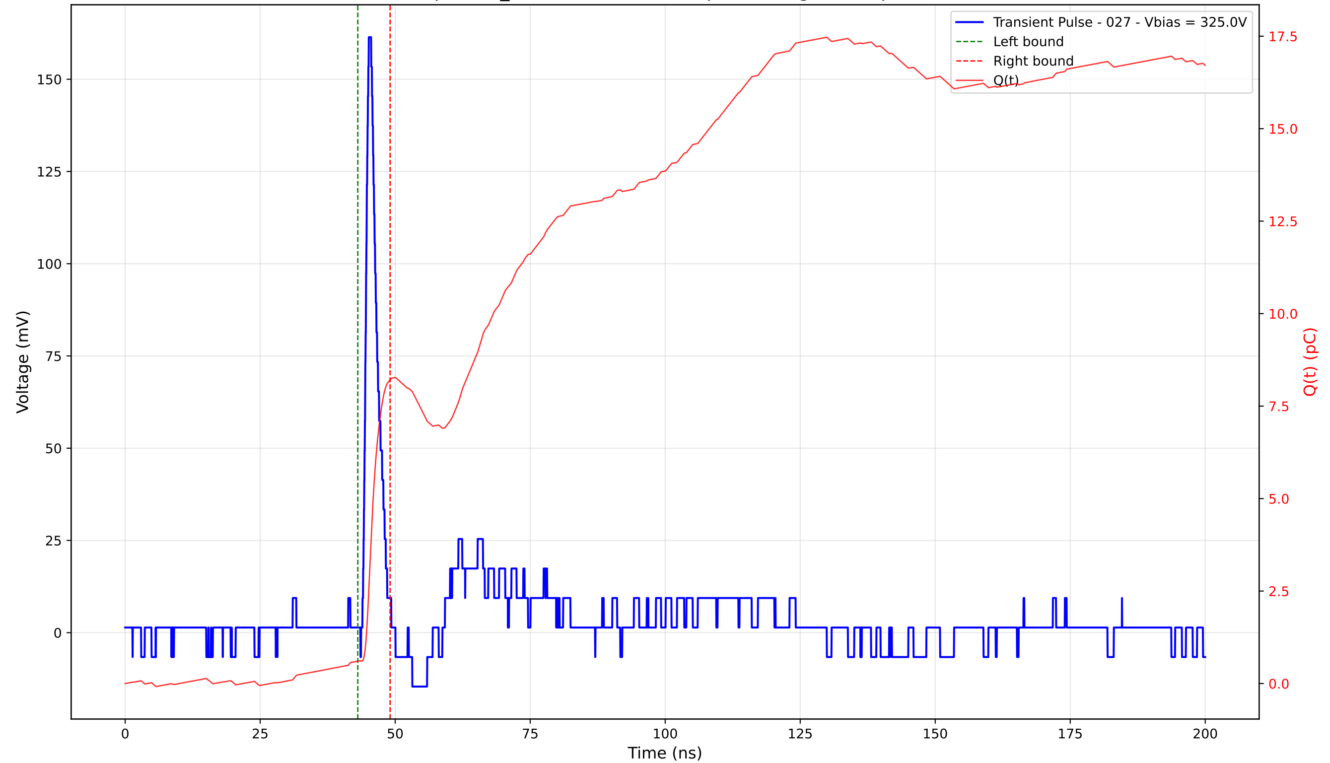
Transient Pulse - Sample: TD_4004 - Position: 50.0 \mu\text{m} - Charge: 7.61 pC - Rise Time: 0.88 ns
