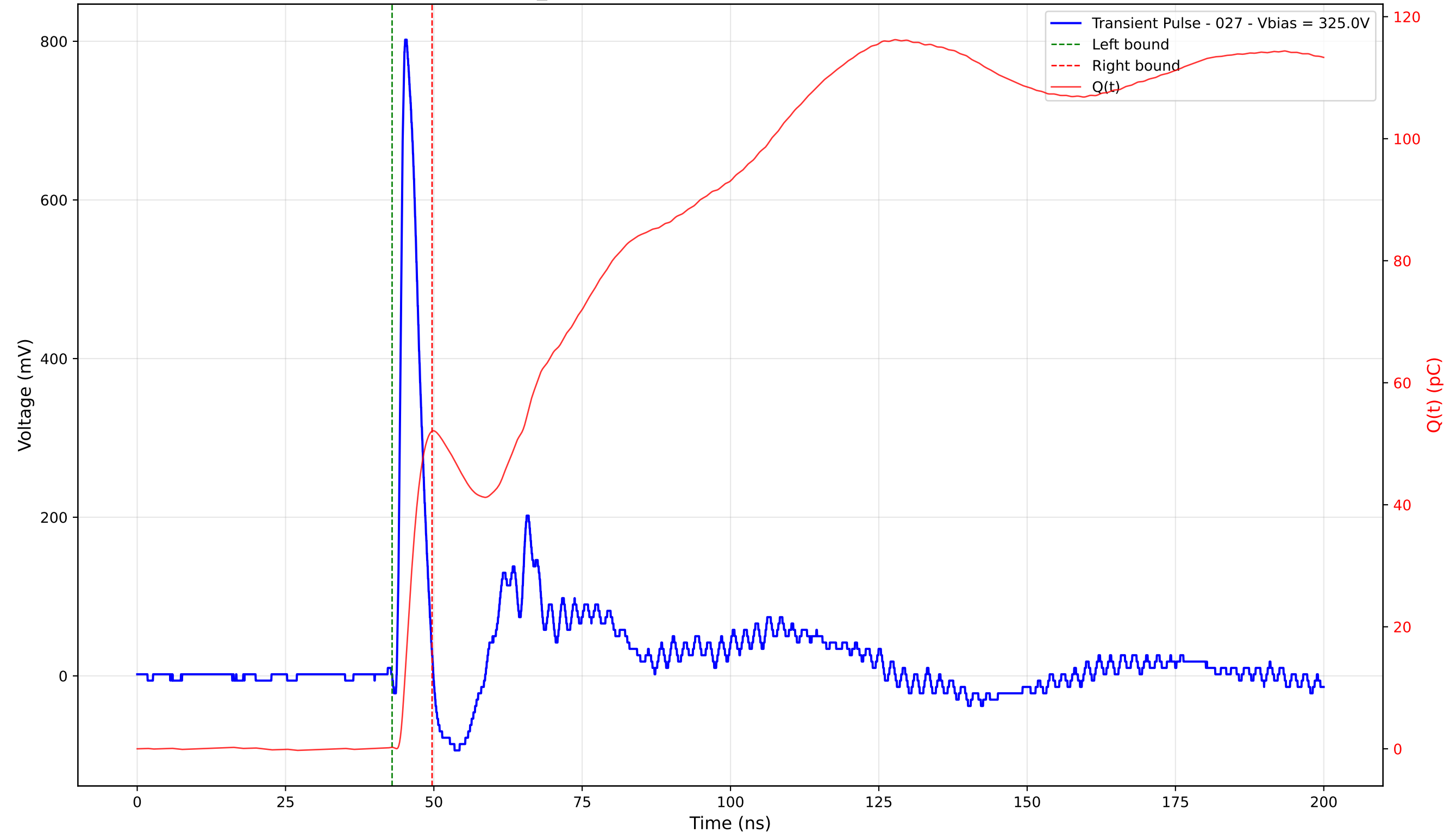
Transient Pulse - Sample: TD_4004 - Position: 175.0 \mu\text{m} - Charge: 51.82 pC - Rise Time: 0.88 ns
