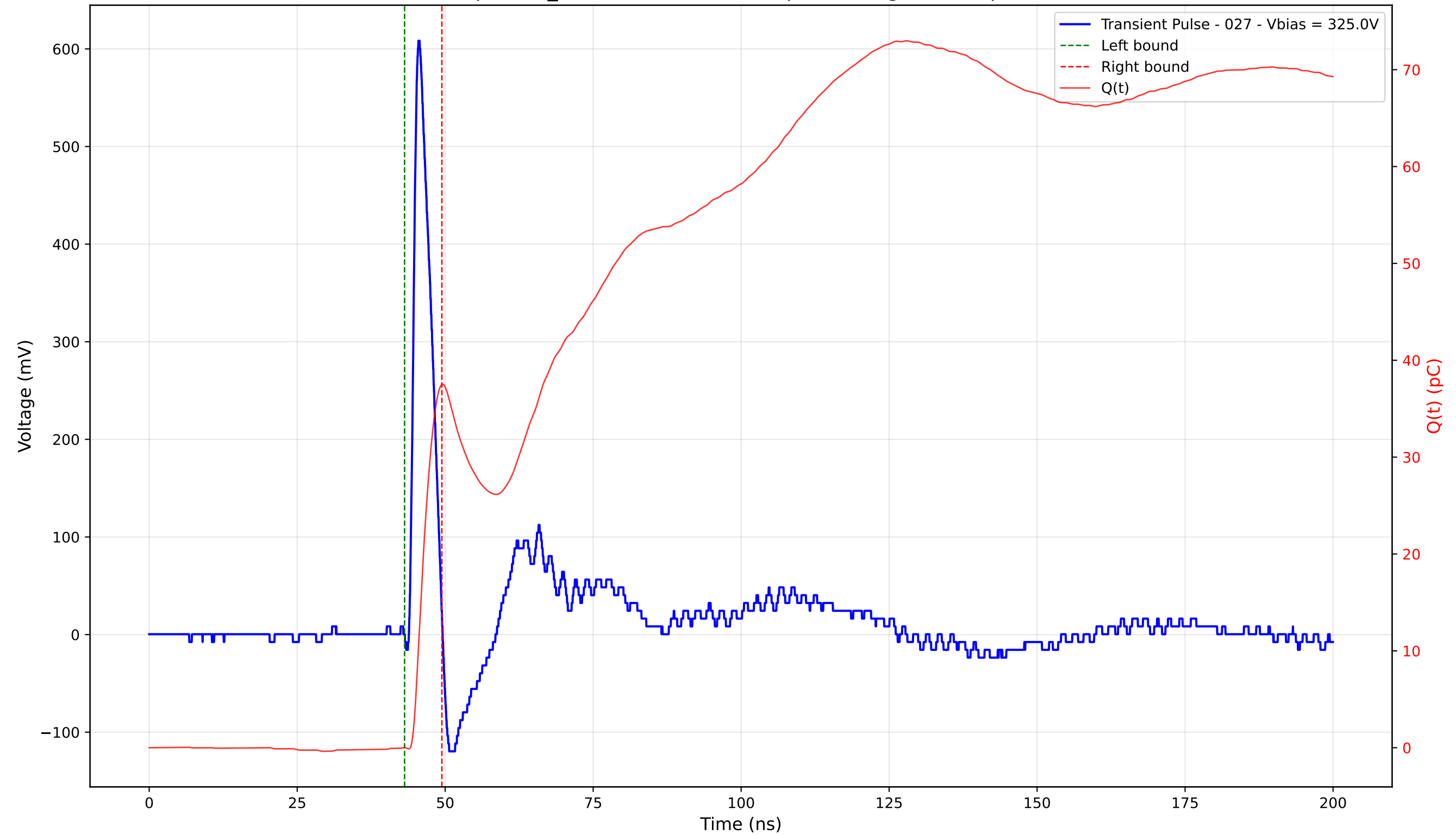
Transient Pulse - Sample: TD_4004 - Position: 385.0 \mu\text{m} - Charge: 37.48 pC - Rise Time: 1.03 ns
