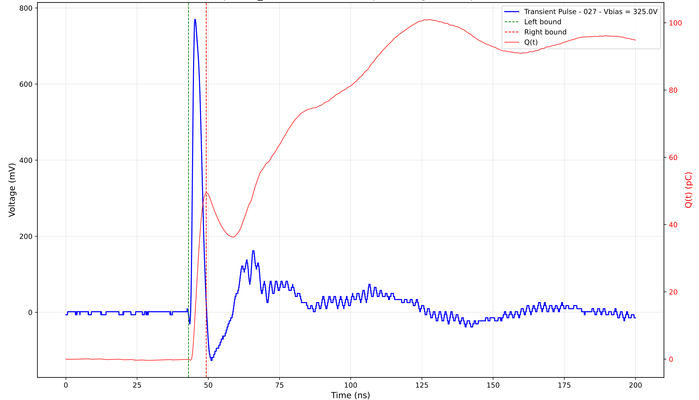
Transient Pulse - Sample: TD_4004 - Position: 290.0 \mu\text{m} - Charge: 49.48 pC - Rise Time: 0.92 ns
