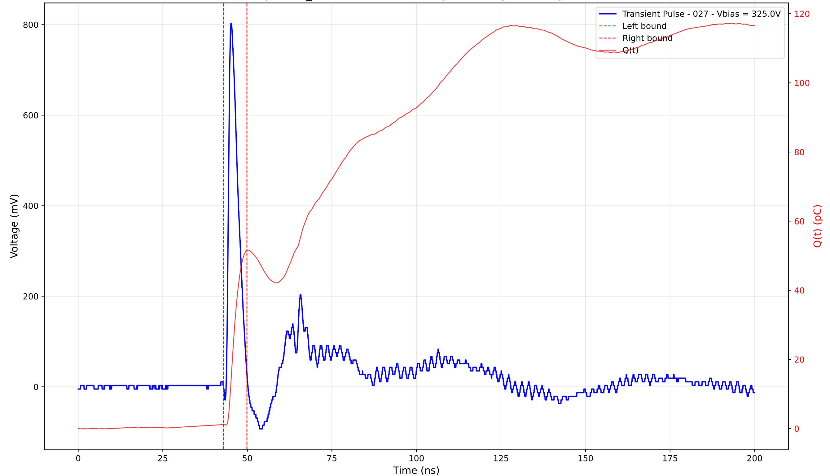
Transient Pulse - Sample: TD_4004 - Position: 105.0 \mu\text{m} - Charge: 50.31 pC - Rise Time: 0.87 ns
