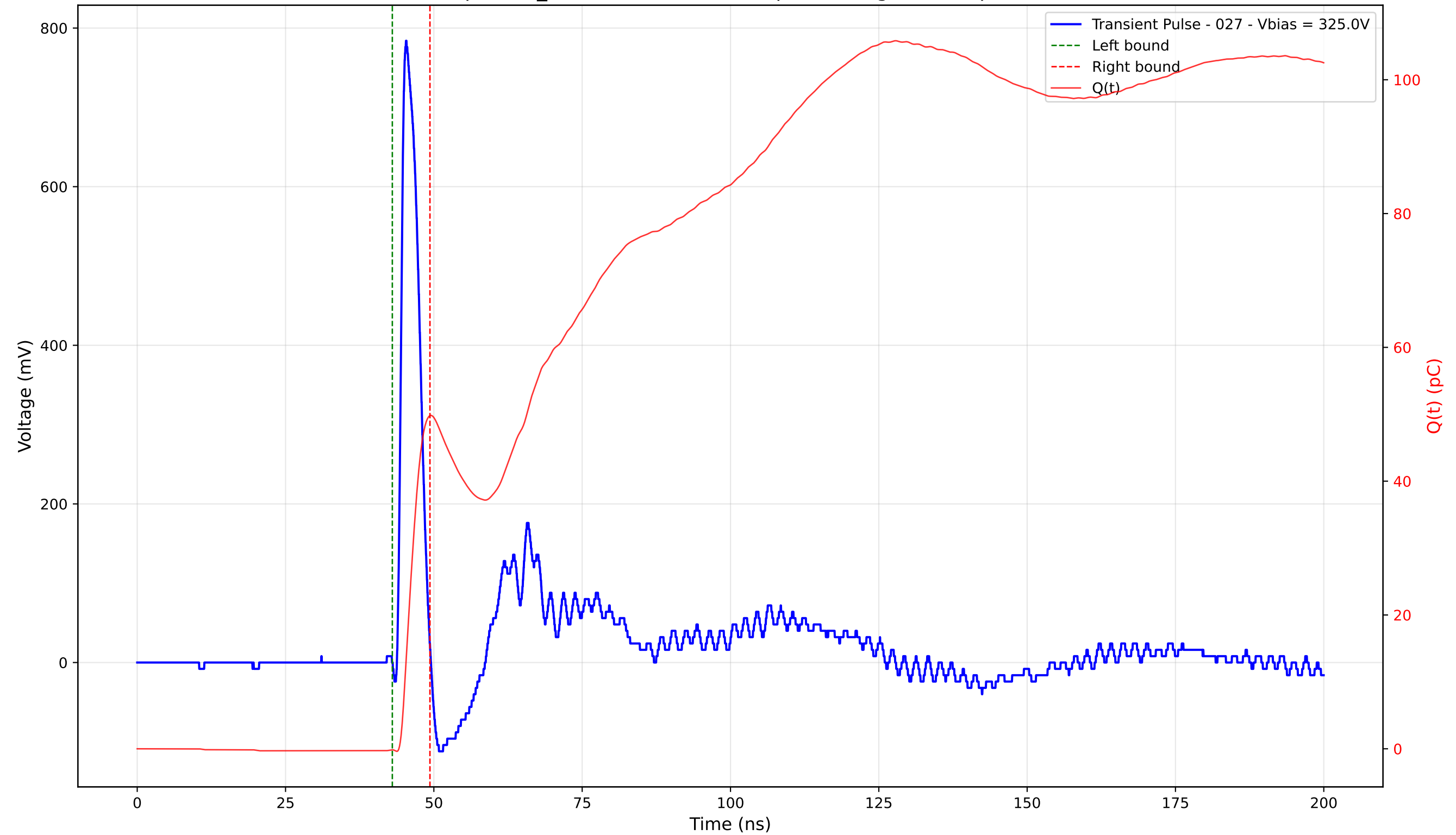
Transient Pulse - Sample: TD_4004 - Position: 280.0 \mu\text{m} - Charge: 49.95 pC - Rise Time: 0.91 ns
