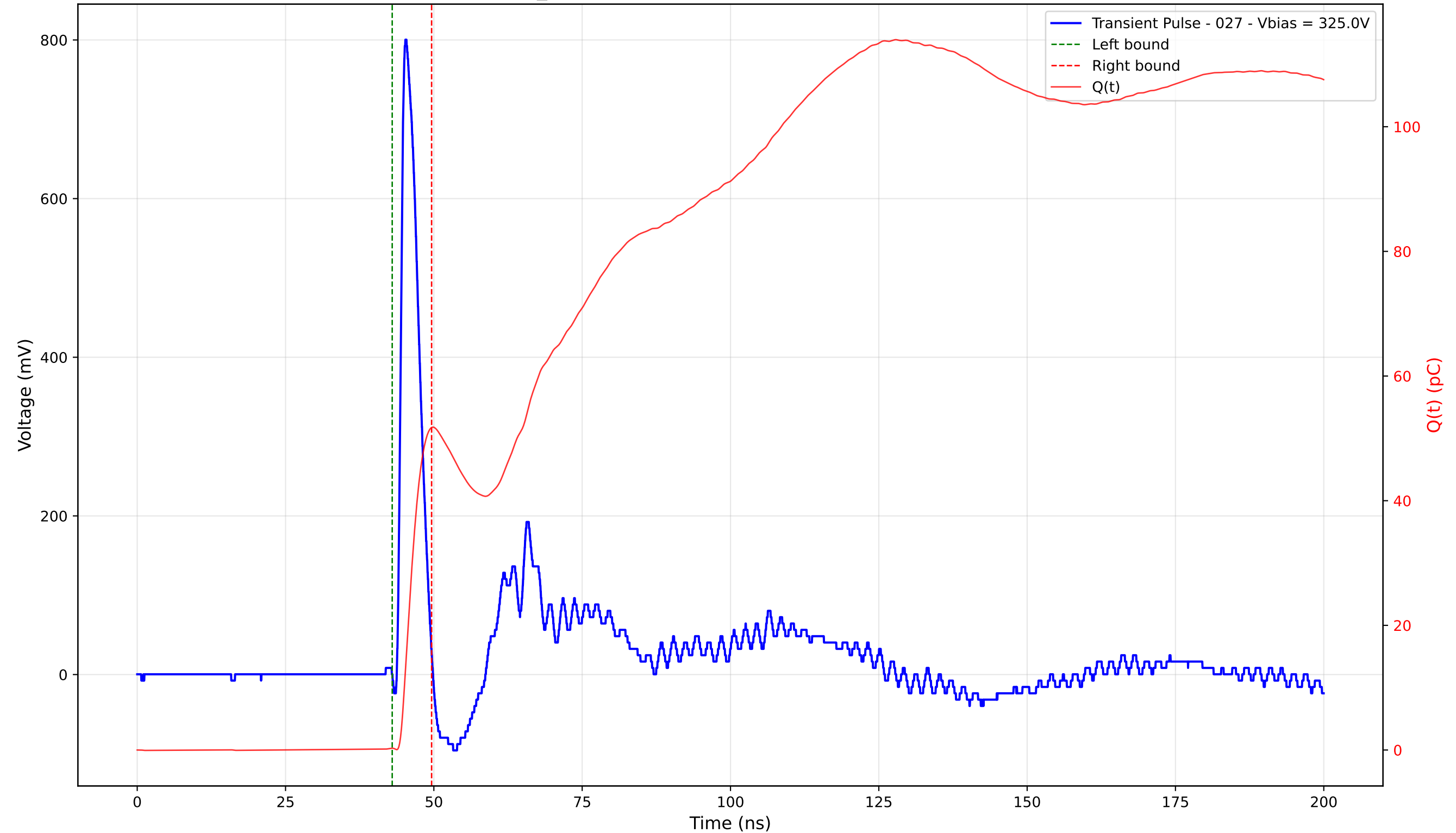
Transient Pulse - Sample: TD_4004 - Position: 170.0 \mu\text{m} - Charge: 51.45 pC - Rise Time: 0.90 ns
