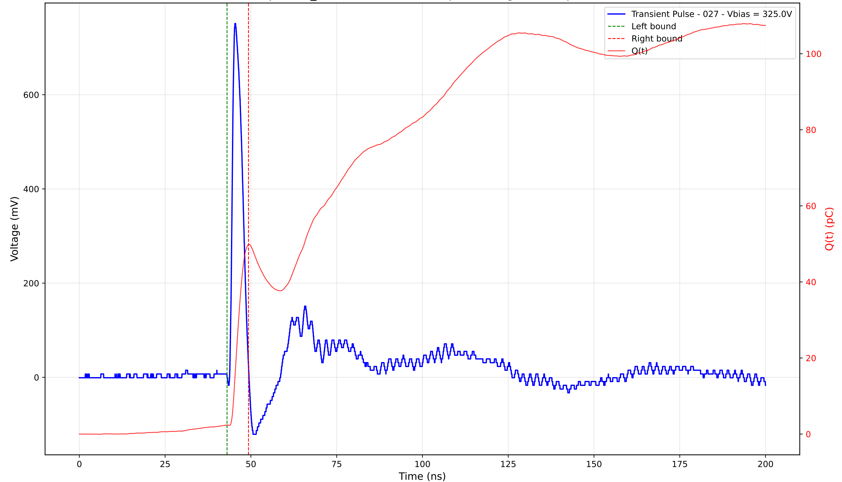
Transient Pulse - Sample: TD_4004 - Position: 315.0 \mu\text{m} - Charge: 47.44 pC - Rise Time: 0.96 ns
