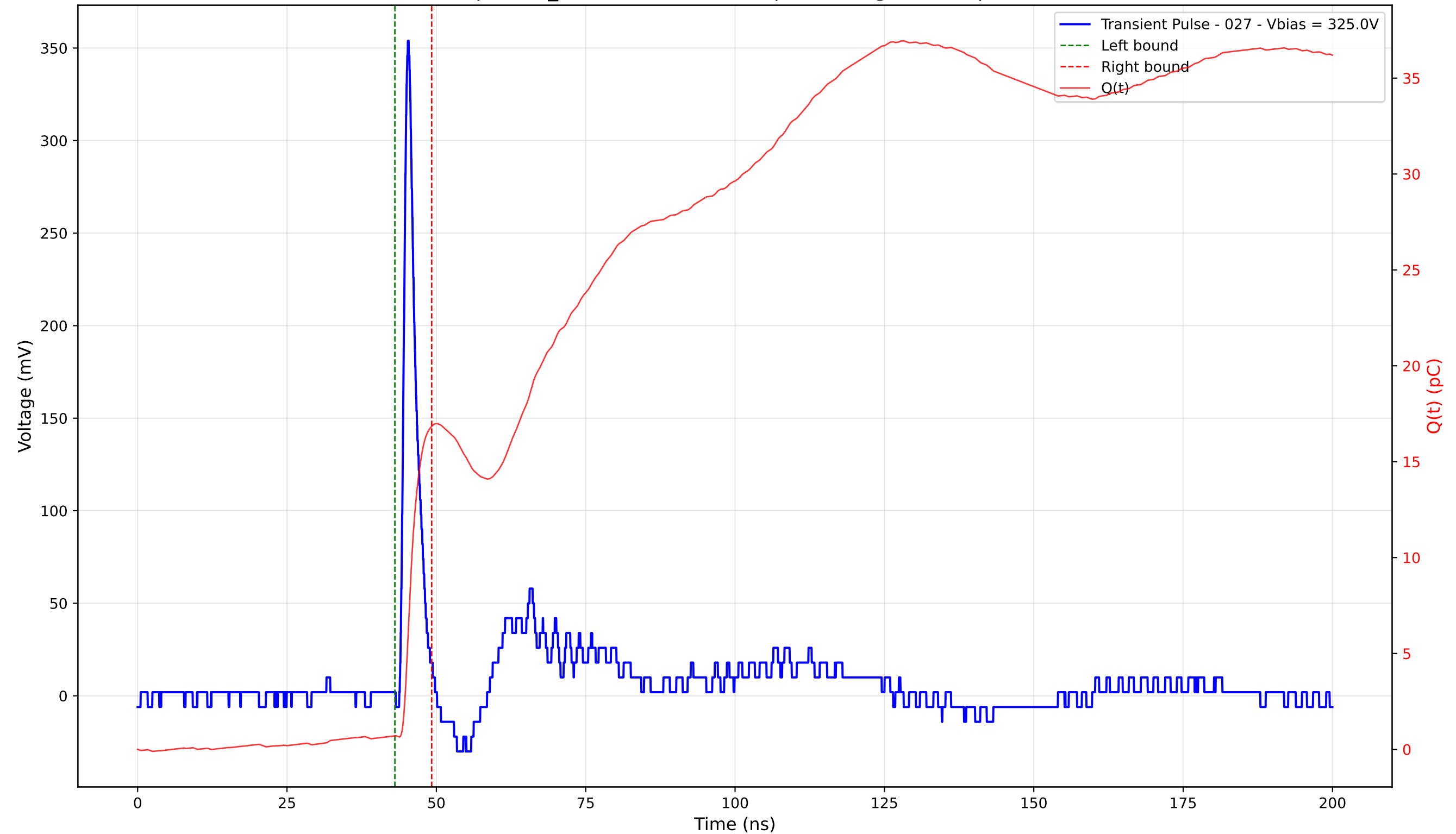
Transient Pulse - Sample: TD_4004 - Position: 60.0 \mu\text{m} - Charge: 16.14 pC - Rise Time: 0.92 ns
