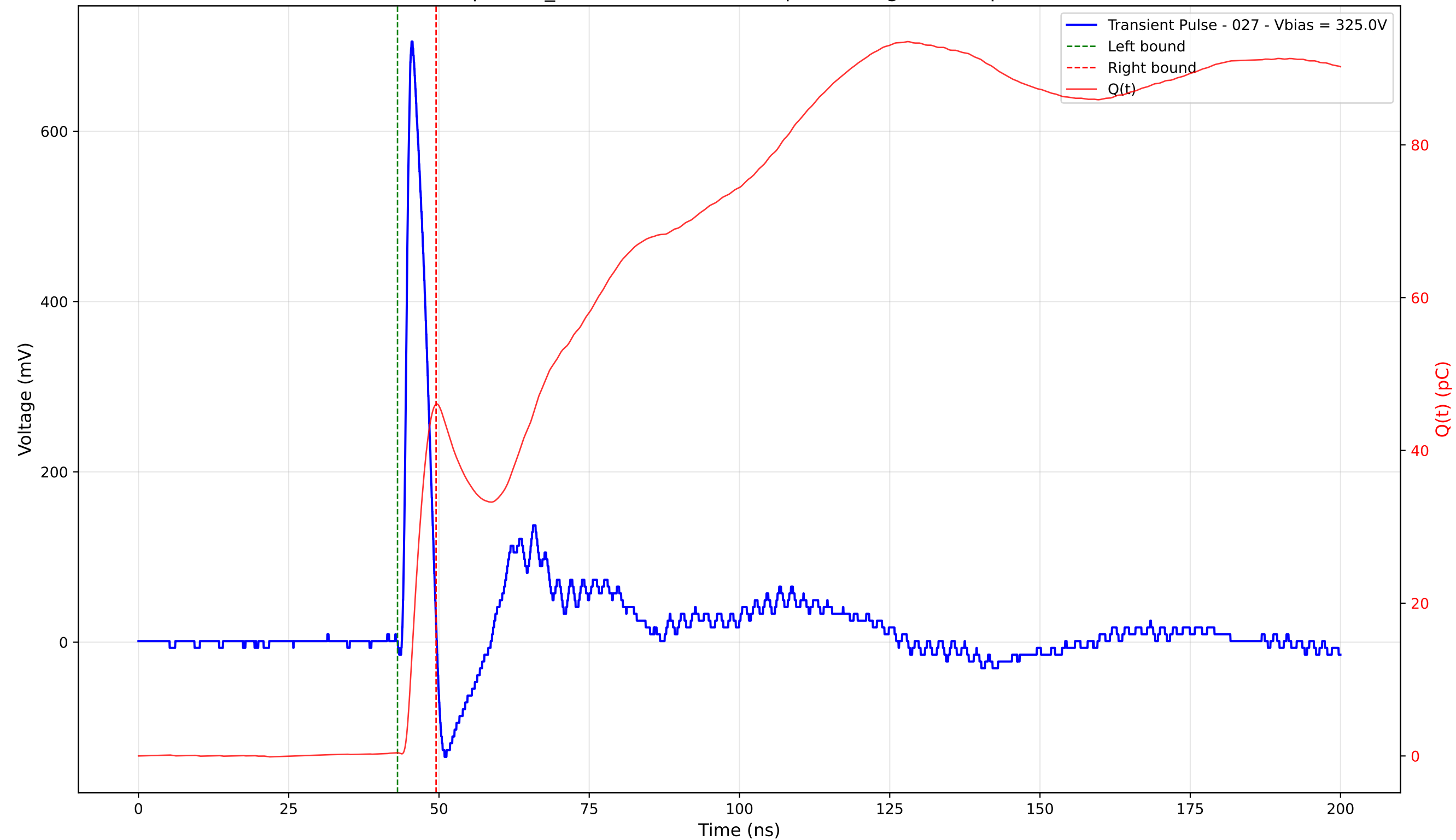
Transient Pulse - Sample: TD_4004 - Position: 350.0 \mu\text{m} - Charge: 45.64 pC - Rise Time: 0.99 ns
