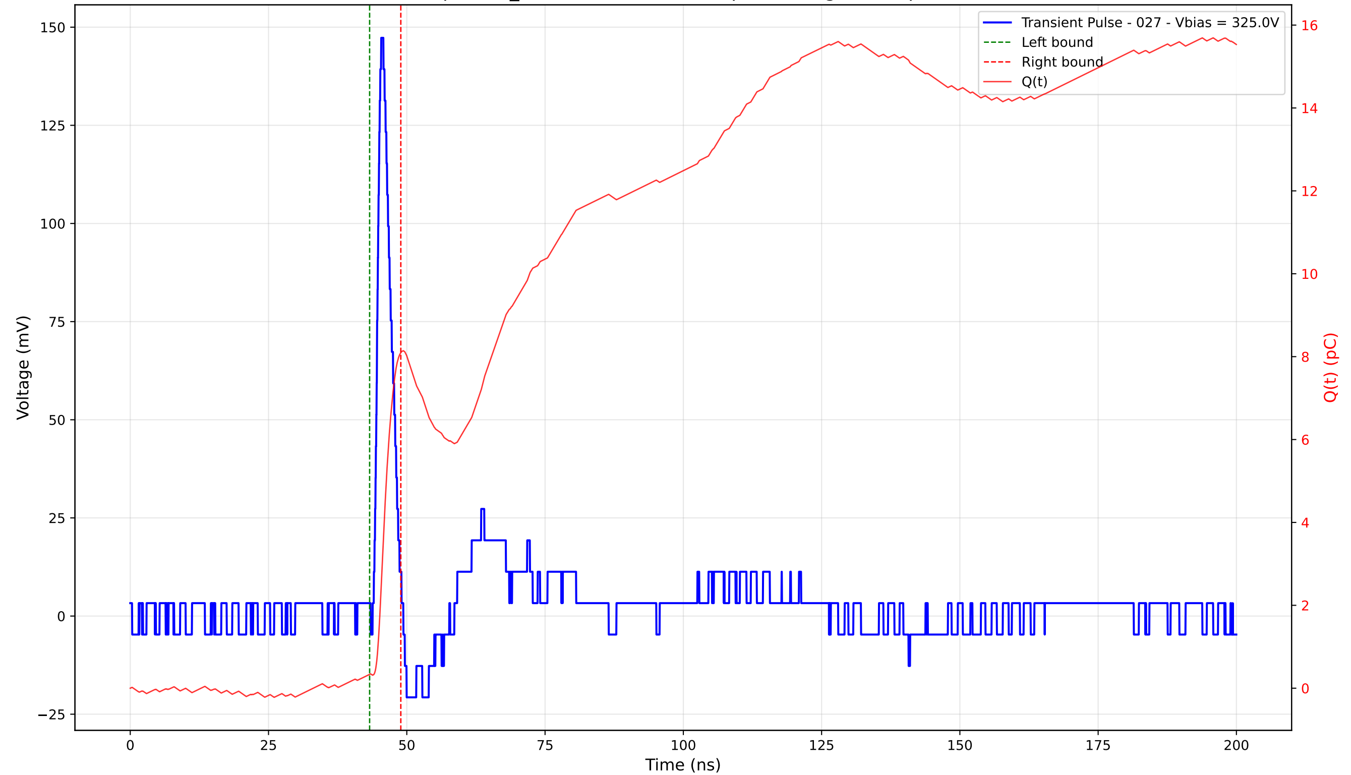
Transient Pulse - Sample: TD_4004 - Position: 415.0 \mu\text{m} - Charge: 7.76 pC - Rise Time: 1.05 ns
