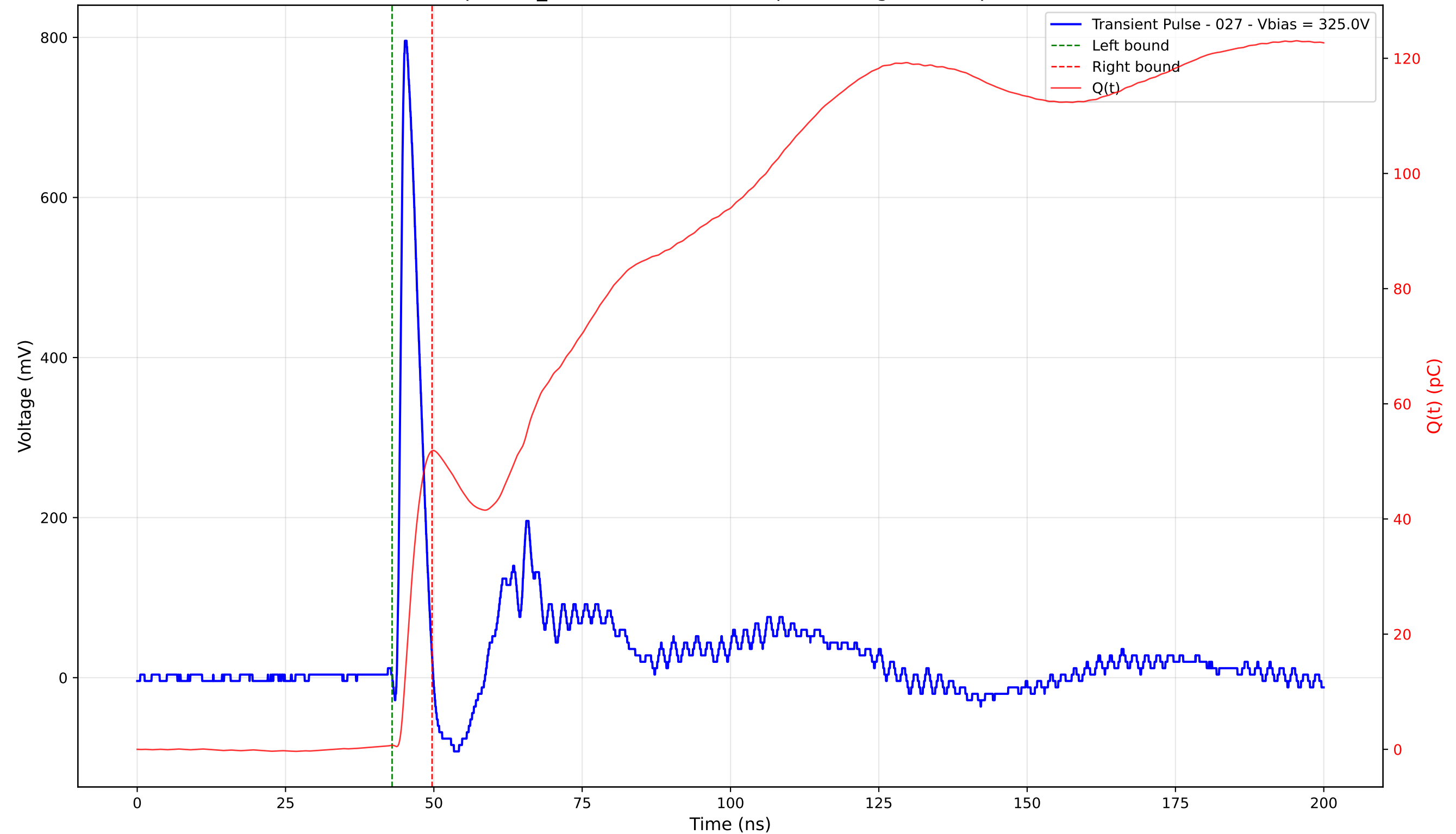
Transient Pulse - Sample: TD_4004 - Position: 120.0 \mu\text{m} - Charge: 51.13 pC - Rise Time: 0.89 ns
