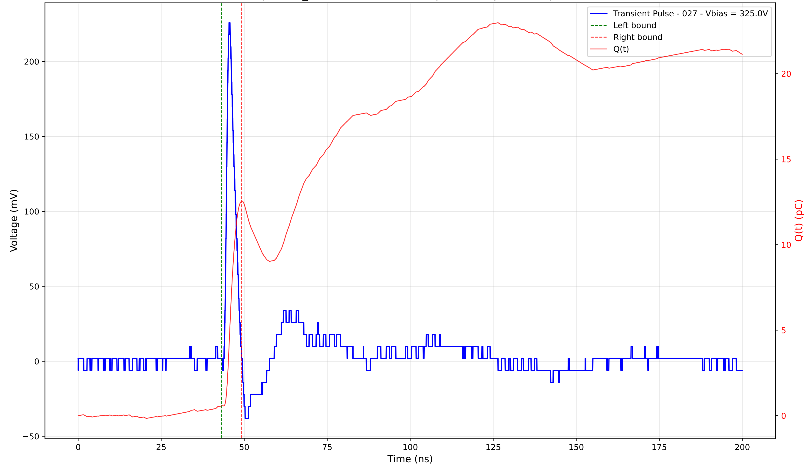
Transient Pulse - Sample: TD_4004 - Position: 410.0 \mu\text{m} - Charge: 11.95 pC - Rise Time: 1.07 ns
