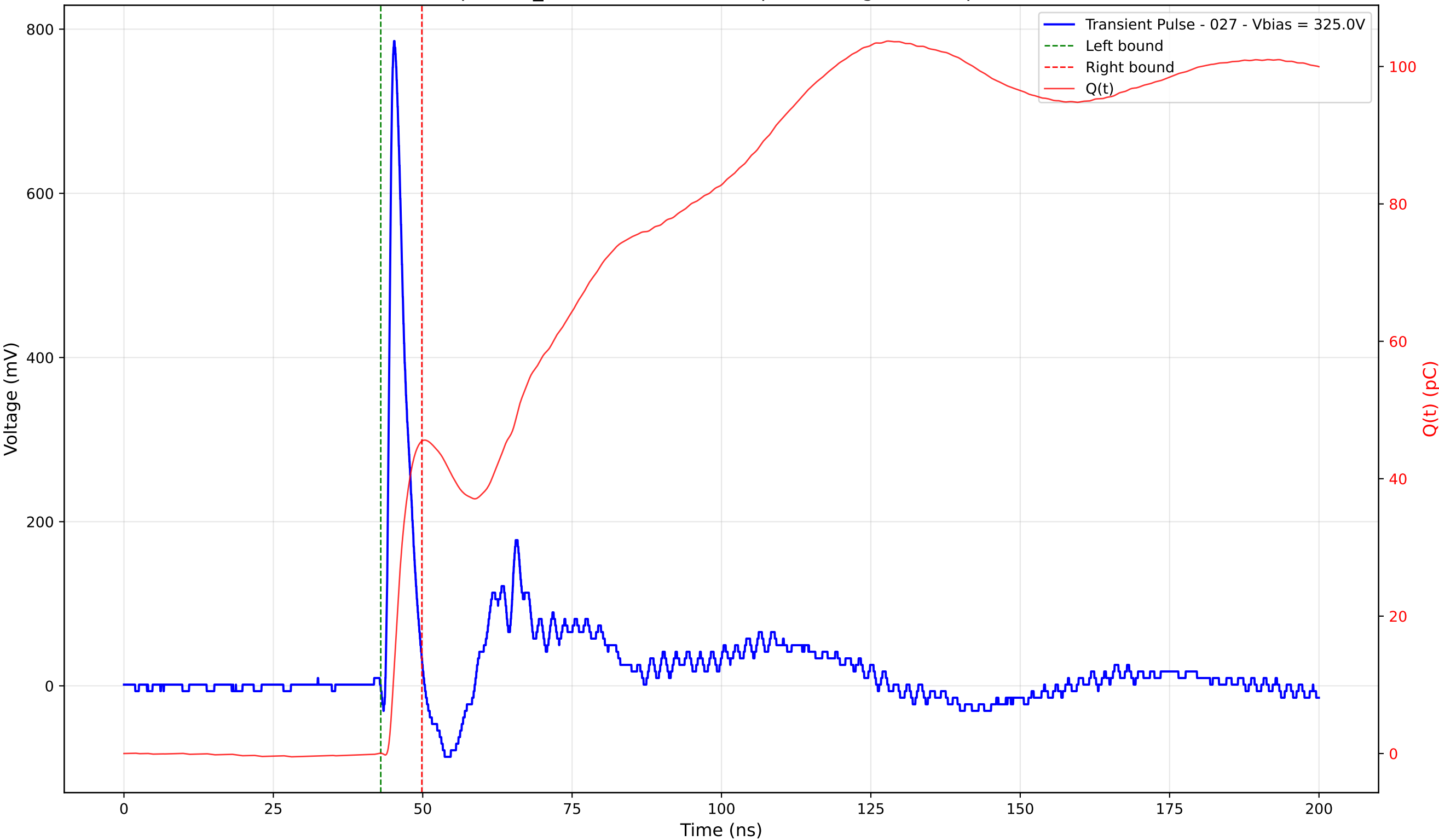
Transient Pulse - Sample: TD_4004 - Position: 95.0 \mu\text{m} - Charge: 45.43 pC - Rise Time: 0.88 ns
