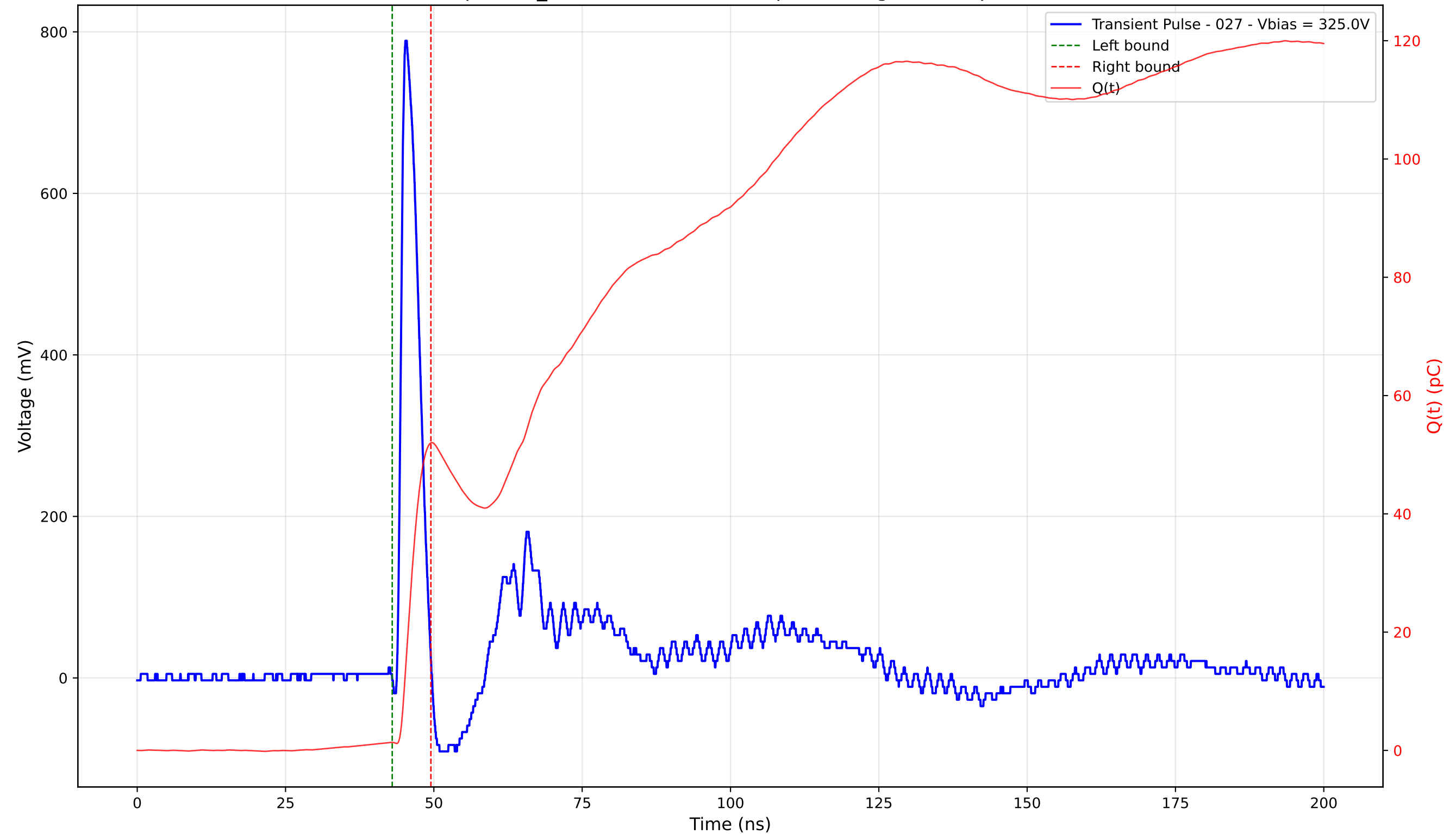
Transient Pulse - Sample: TD_4004 - Position: 135.0 \mu\text{m} - Charge: 50.63 pC - Rise Time: 0.90 ns
