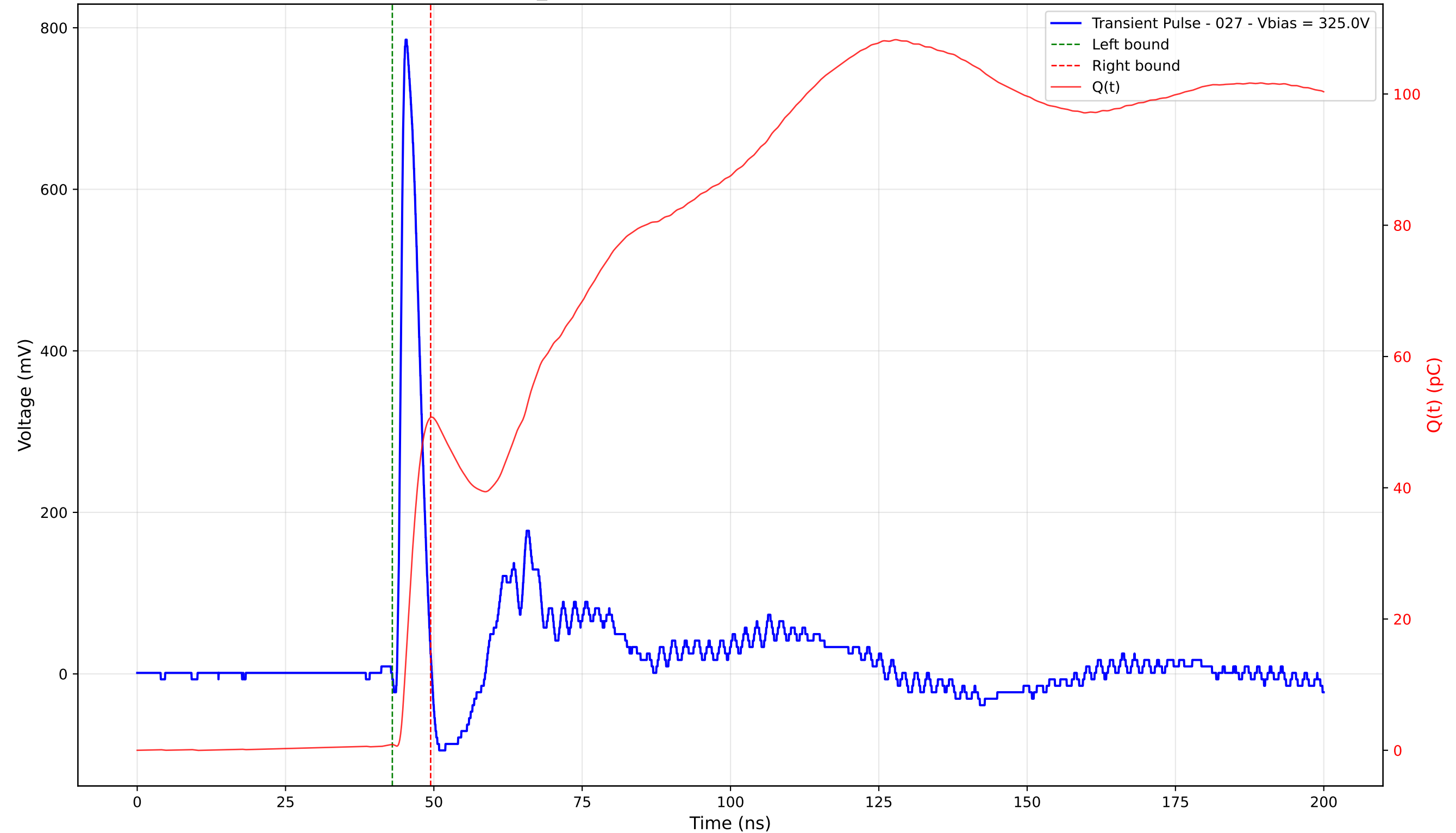
Transient Pulse - Sample: TD_4004 - Position: 140.0 \mu\text{m} - Charge: 49.83 pC - Rise Time: 0.91 ns
