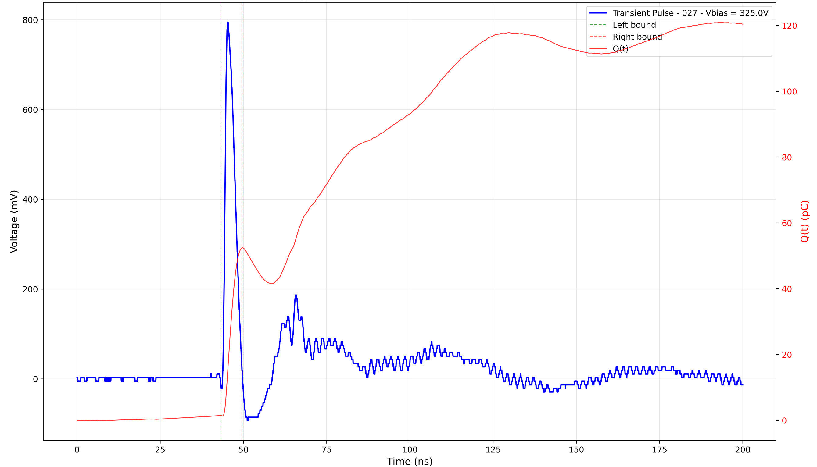
Transient Pulse - Sample: TD_4004 - Position: 130.0 \mu\text{m} - Charge: 50.85 pC - Rise Time: 0.91 ns
