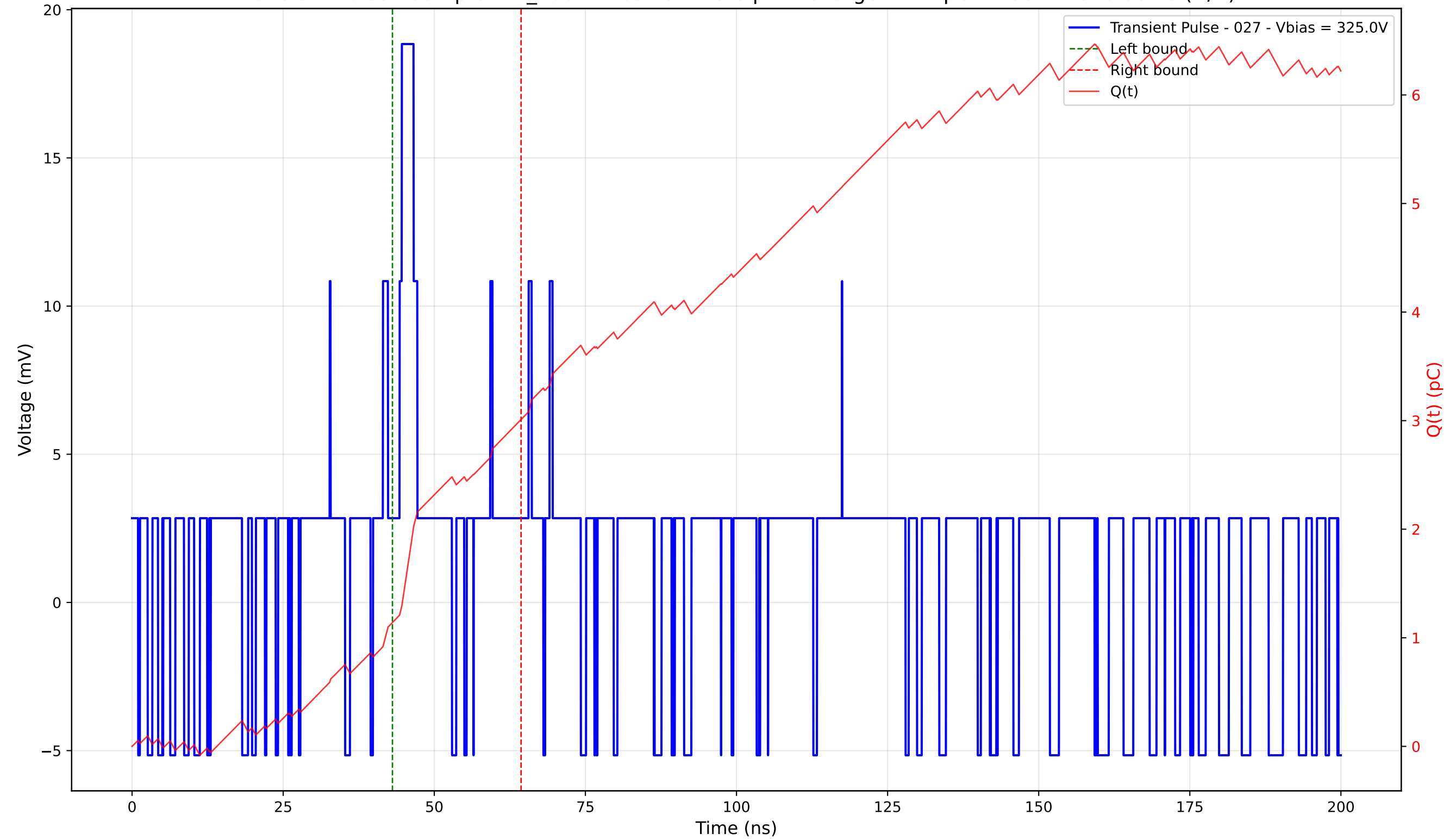
Transient Pulse - Sample: TD_4004 - Position: 15.0 \mu\text{m} - Charge: 1.87 pC - Rise Time: 0.00 ns (N/A)
