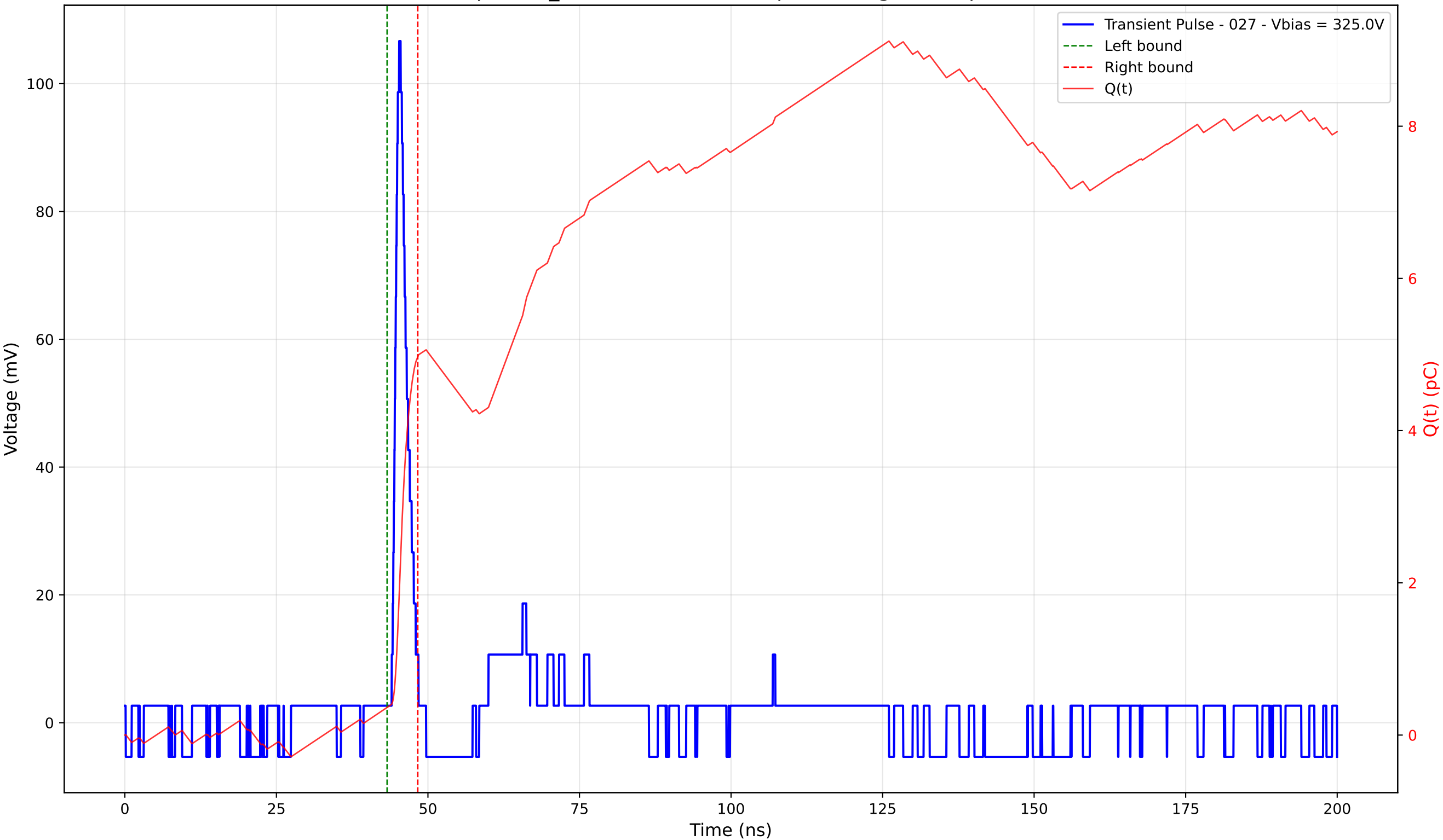
Transient Pulse - Sample: TD_4004 - Position: 45.0 \mu\text{m} - Charge: 4.61 pC - Rise Time: 0.86 ns
