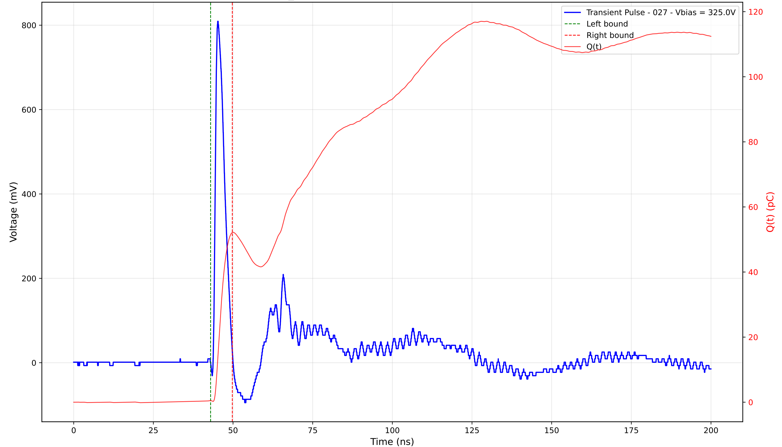
Transient Pulse - Sample: TD_4004 - Position: 185.0 \mu\text{m} - Charge: 51.64 pC - Rise Time: 0.88 ns
