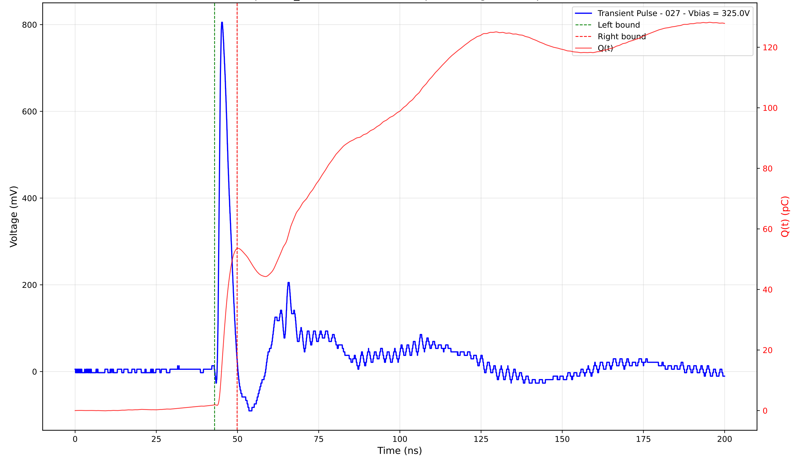
Transient Pulse - Sample: TD_4004 - Position: 110.0 \mu\text{m} - Charge: 51.60 pC - Rise Time: 0.87 ns
