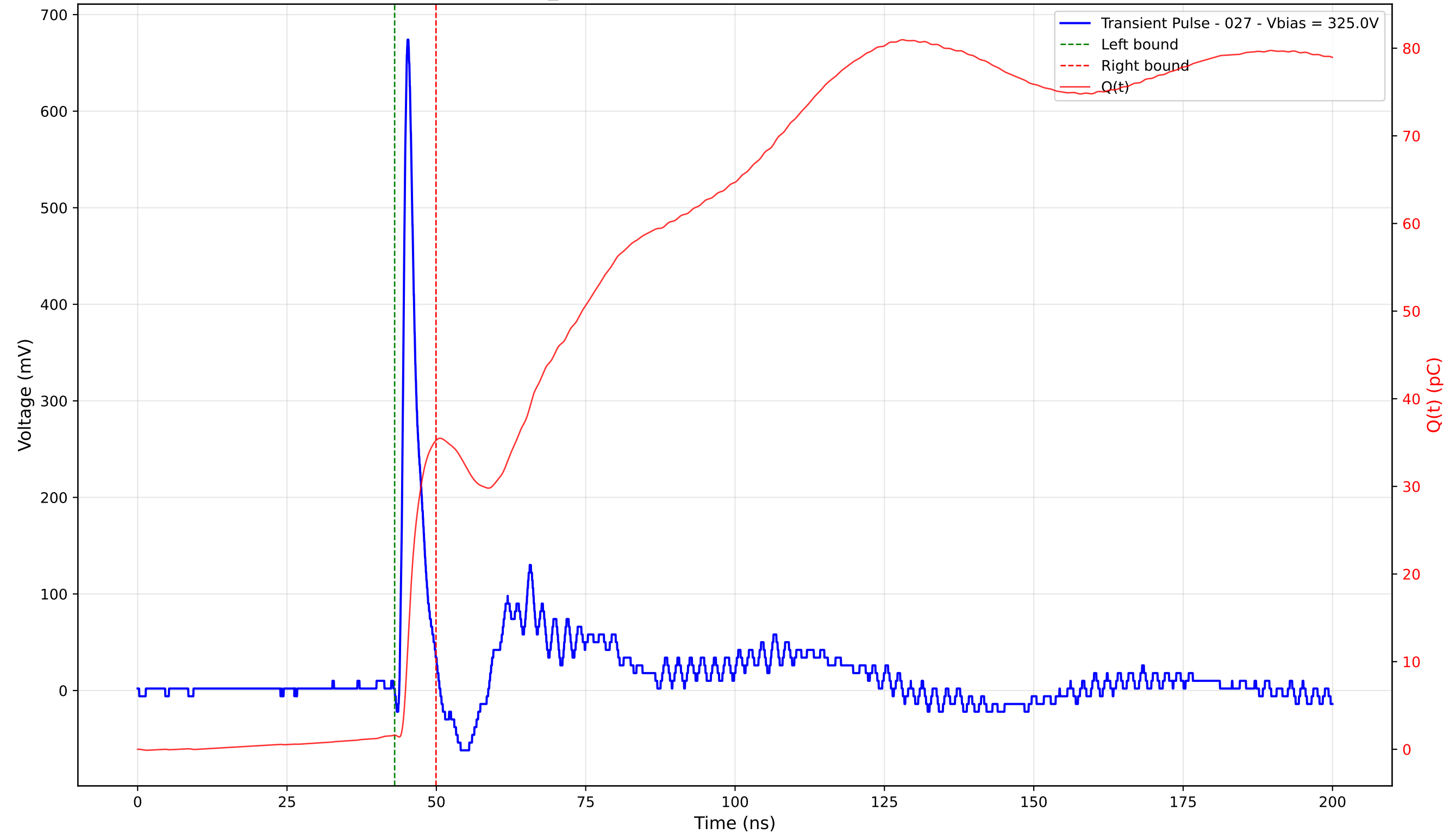
Transient Pulse - Sample: TD_4004 - Position: 75.0 \mu\text{m} - Charge: 33.64 pC - Rise Time: 0.91 ns
