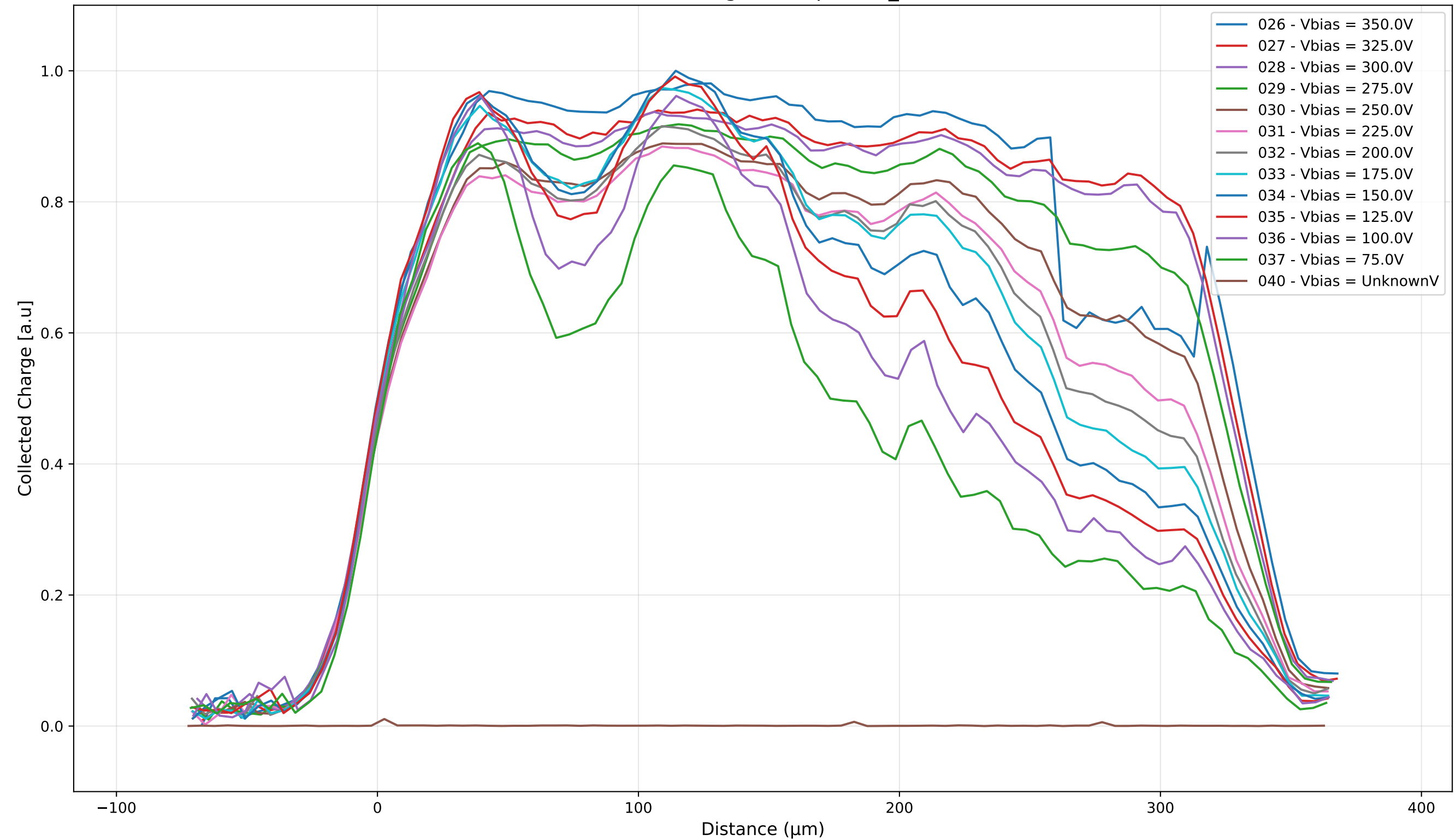
Collected Charge - Sample: TD_4004
