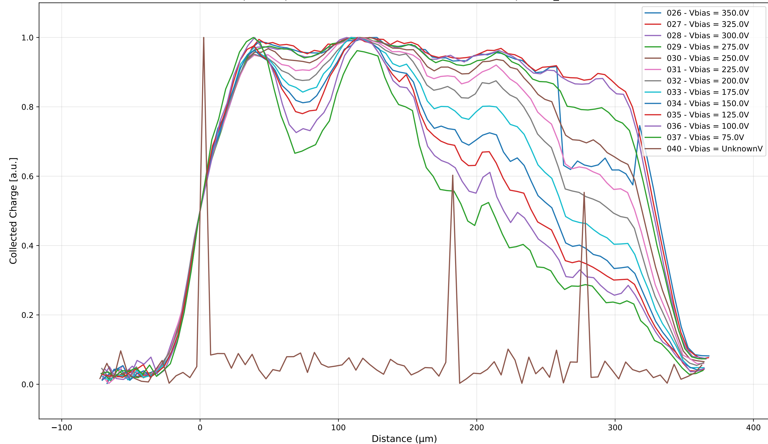
Shape Comparison — Individual Normalization — Sample: TD_4004
