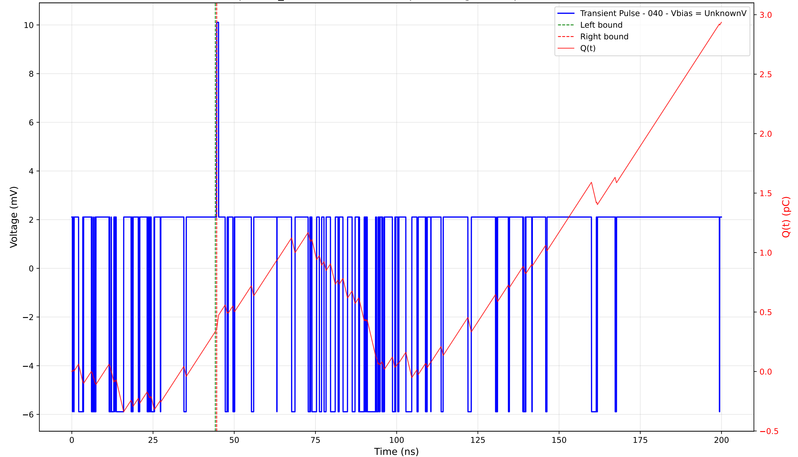
Transient Pulse - Sample: TD_4004 - Position: 130.0 \mu m - Charge: 0.02 pC - Rise Time: 0.00 ns (N/A)
