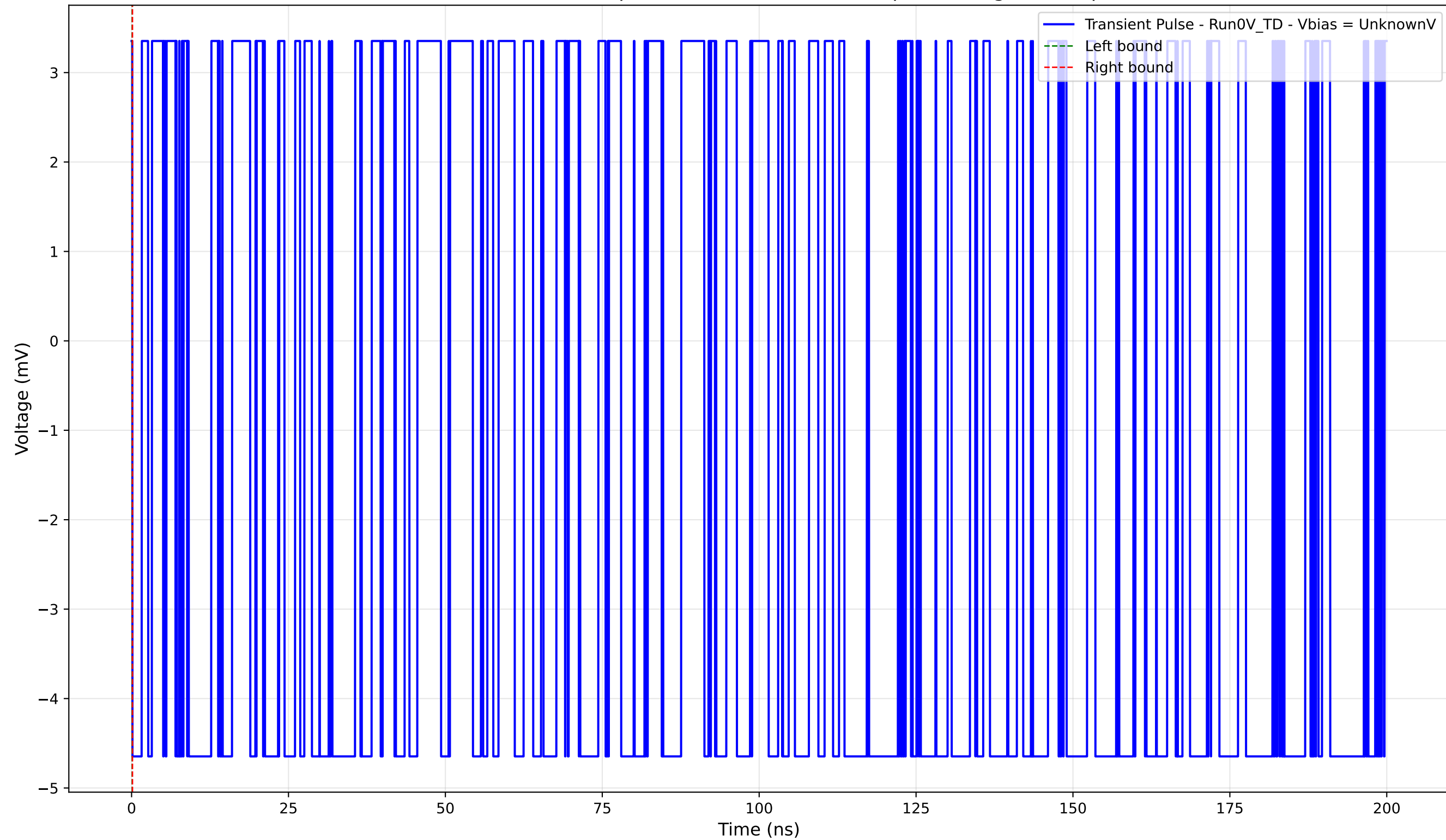
Transient Pulse - Sample: 4004 - Position: 250.0 \mu\text{m} - Charge: -0.00 pC
