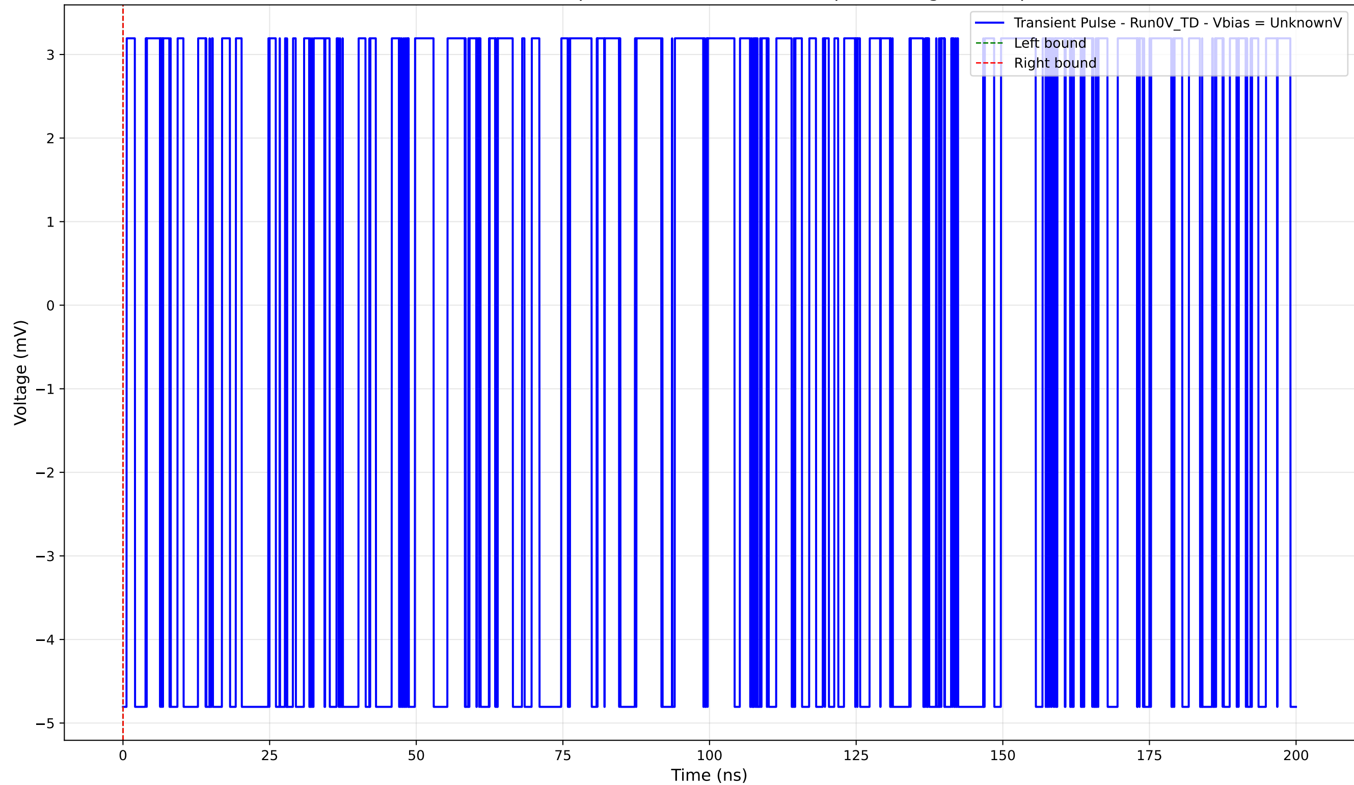
Transient Pulse - Sample: 4004 - Position: 740.0 \mu\text{m} - Charge: -0.00 pC
