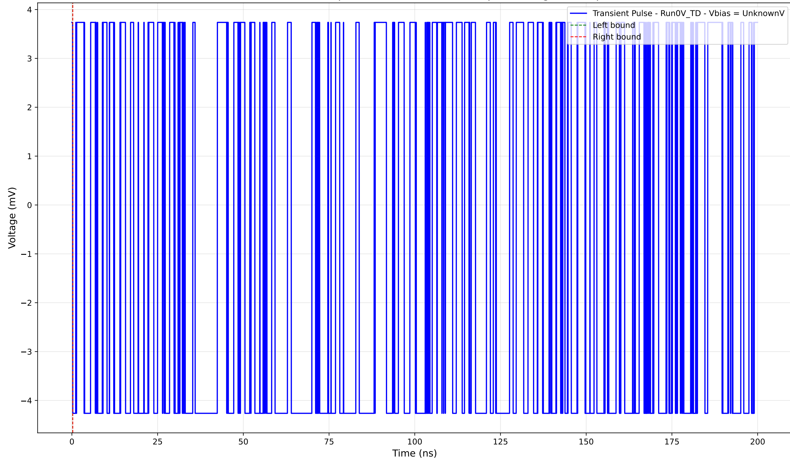
Transient Pulse - Sample: 4004 - Position: 390.0 \mu\text{m} - Charge: -0.00 pC
