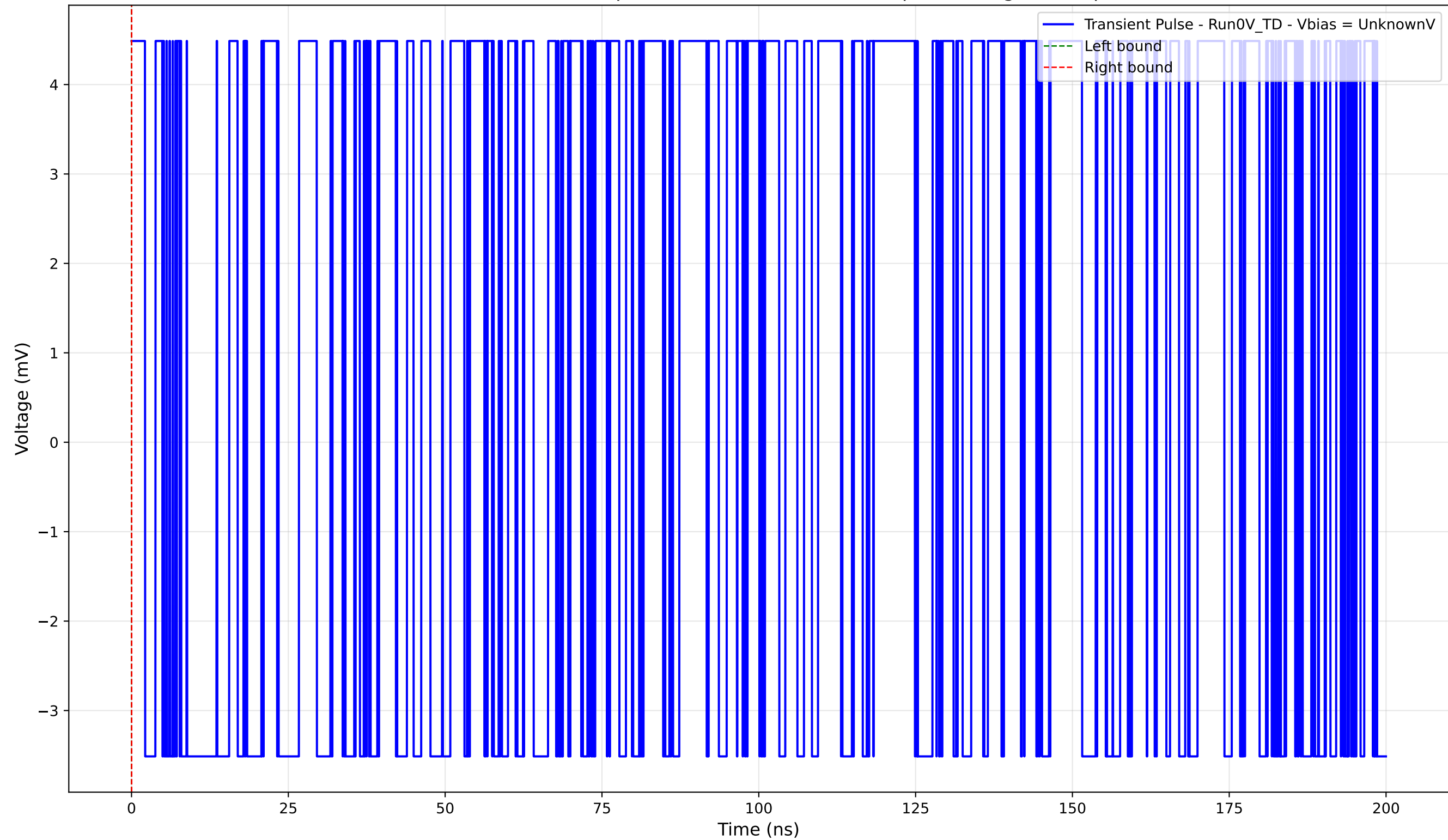
Transient Pulse - Sample: 4004 - Position: 1520.0 \mu\text{m} - Charge: 0.00 pC
