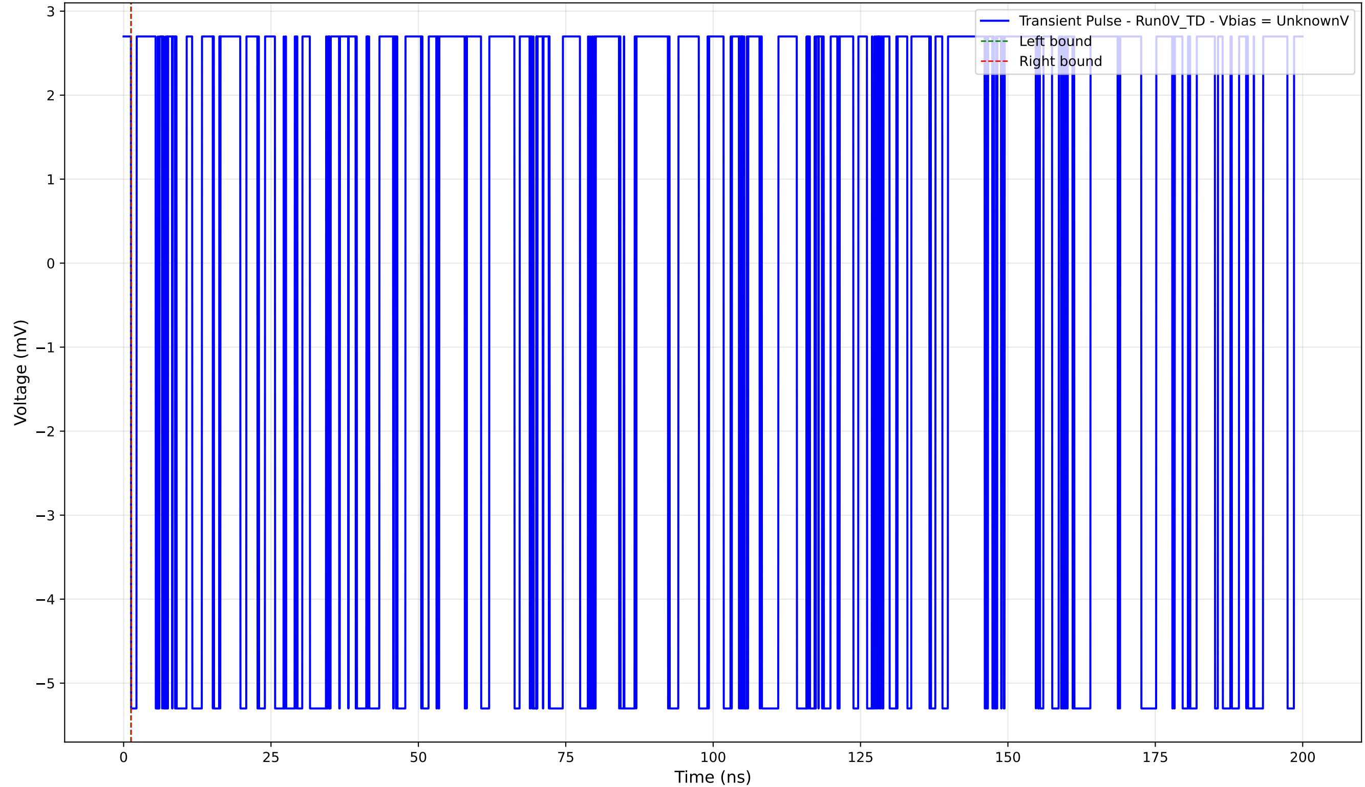
Transient Pulse - Sample: 4004 - Position: 1430.0 \mu\text{m} - Charge: -0.00 pC
