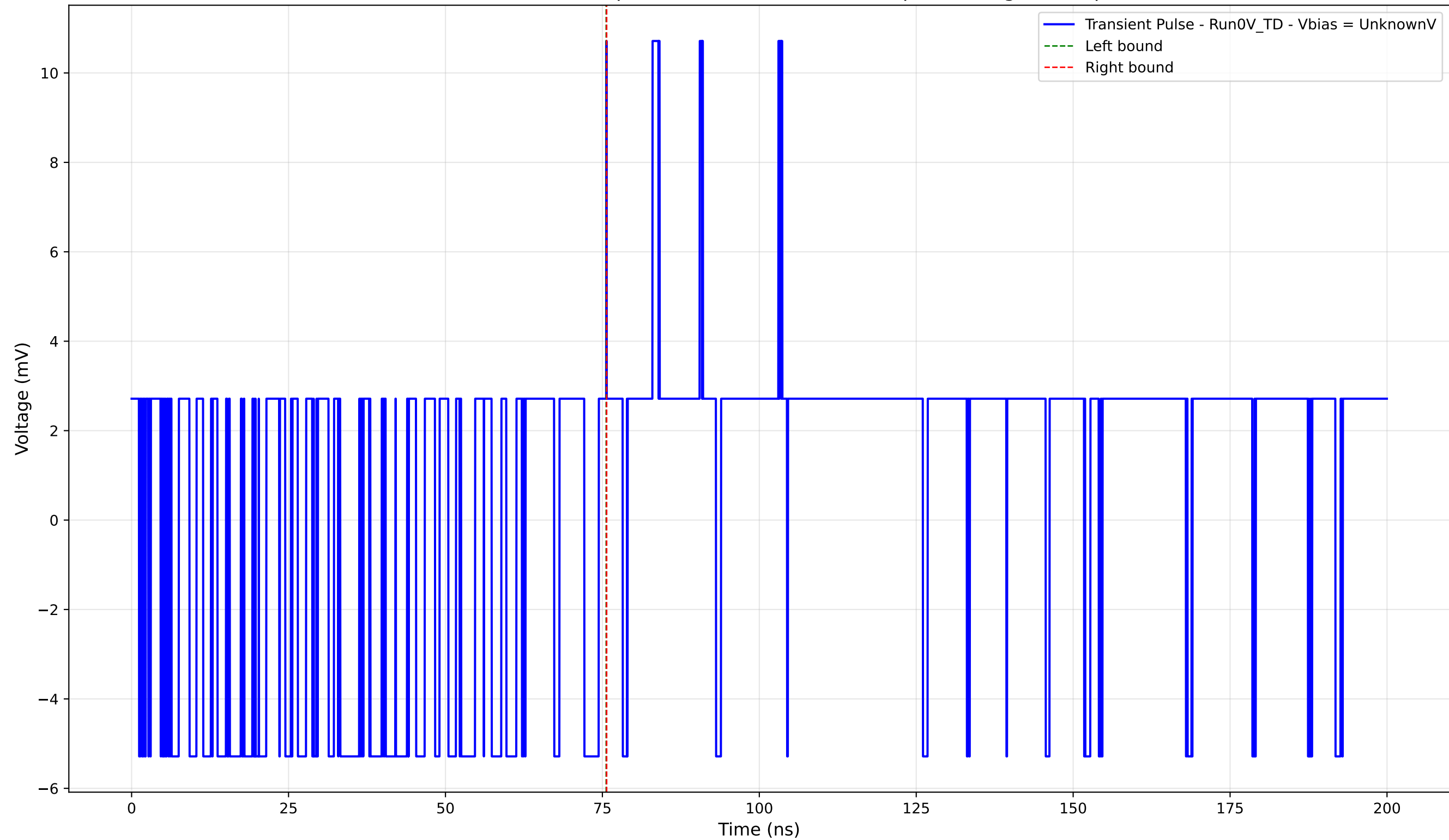
Transient Pulse - Sample: 4004 - Position: 1890.0 \mu\text{m} - Charge: 0.01 pC
