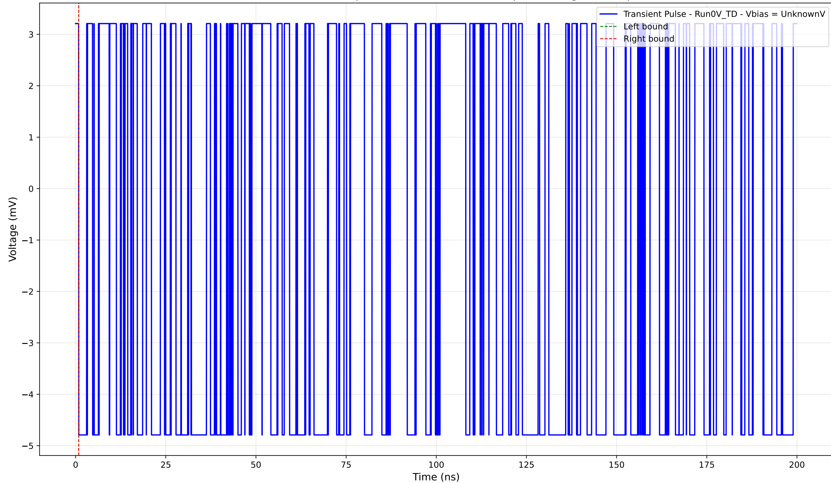
Transient Pulse - Sample: 4004 - Position: 510.0 \mu\text{m} - Charge: -0.00 pC
