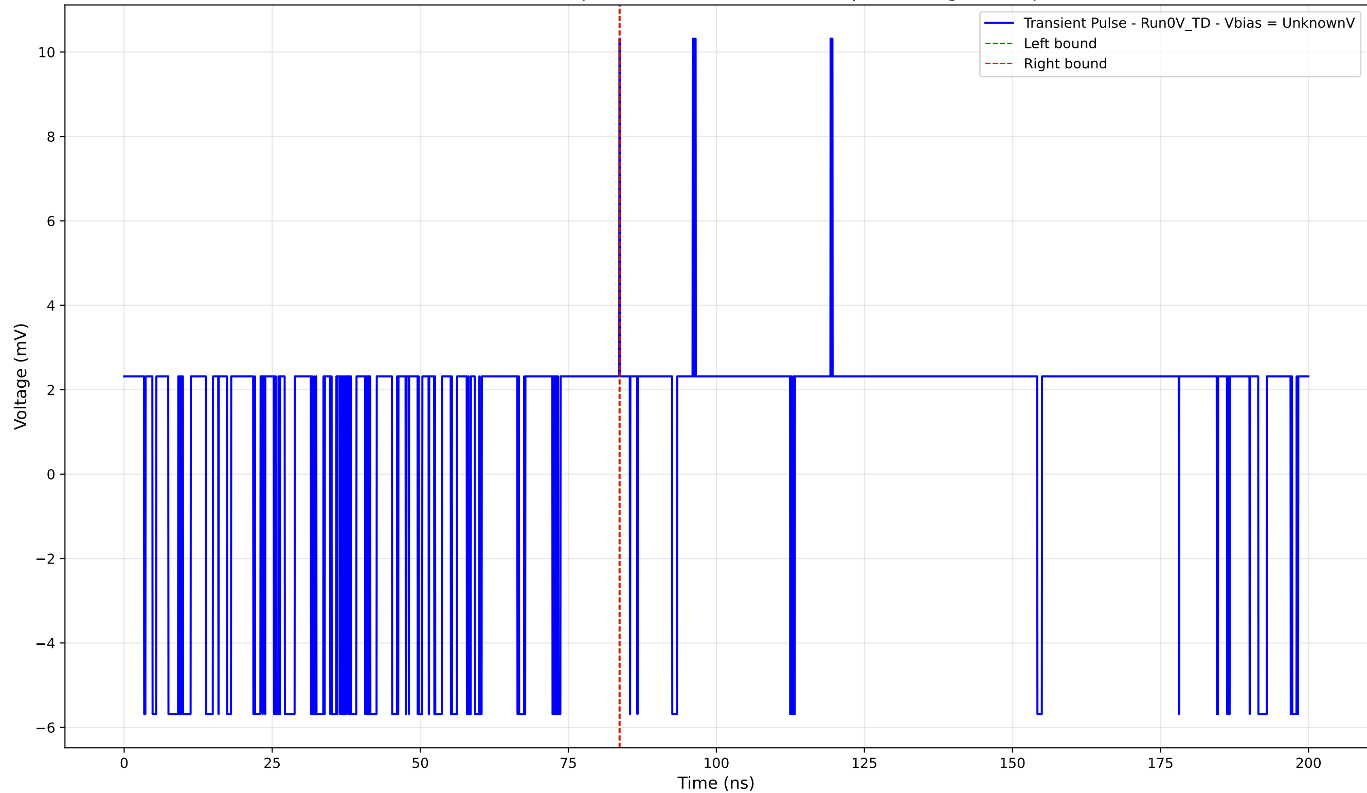
Transient Pulse - Sample: 4004 - Position: 1970.0 \mu\text{m} - Charge: 0.02 pC
