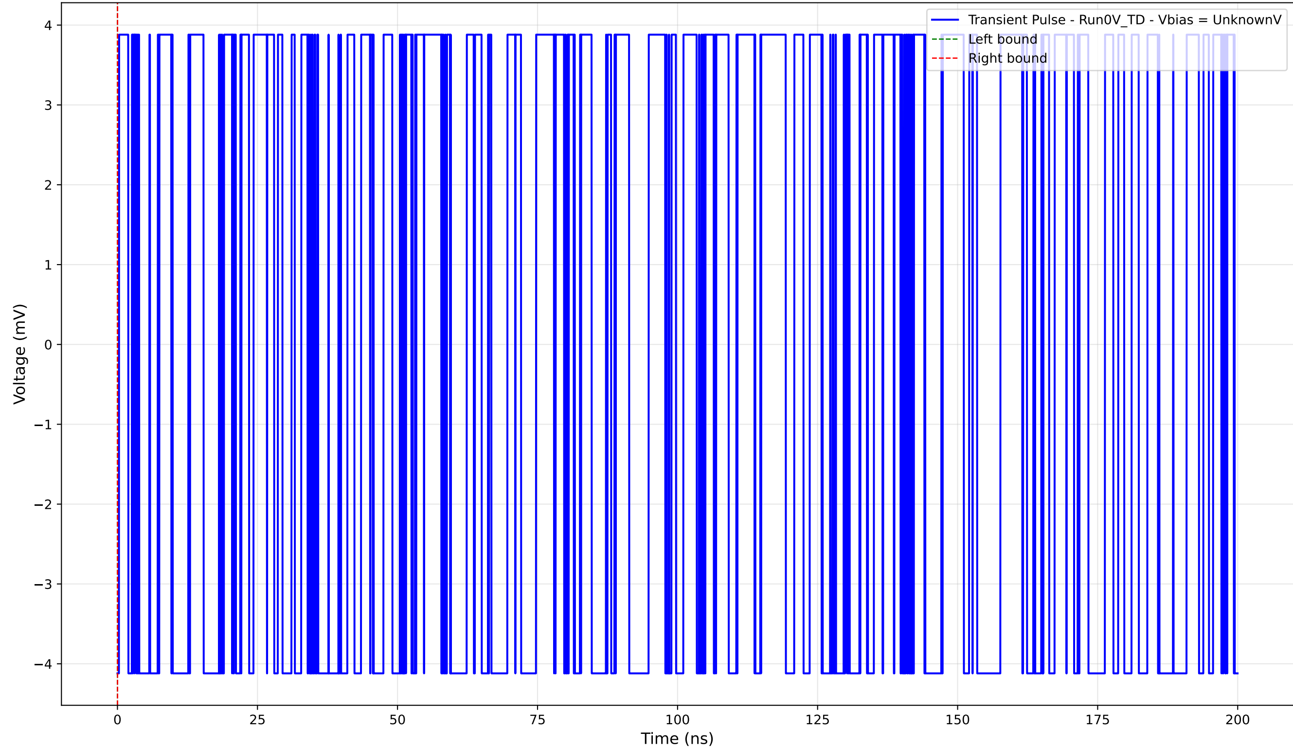
Transient Pulse - Sample: 4004 - Position: 1660.0 \mu\text{m} - Charge: -0.00 pC
