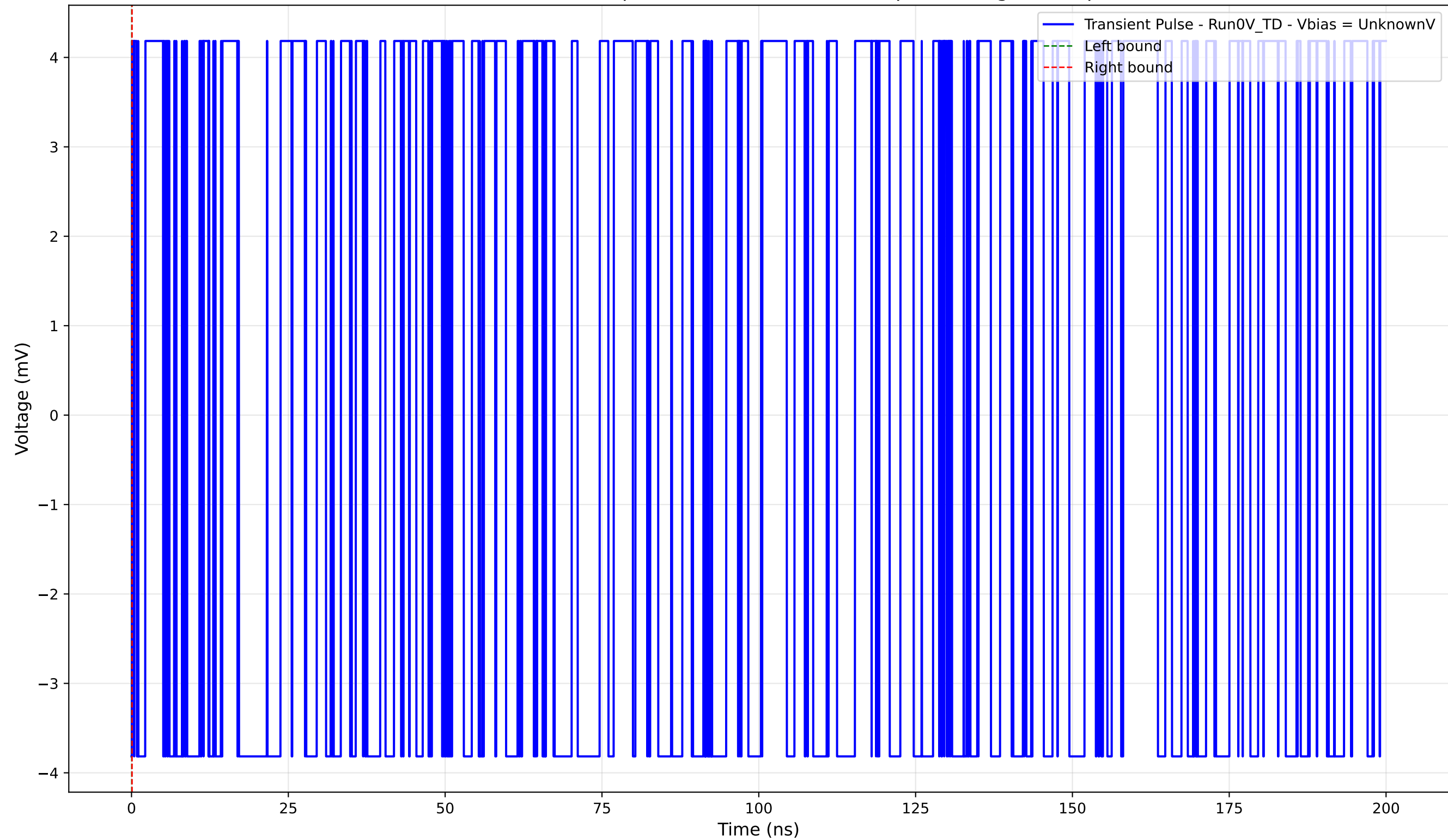
Transient Pulse - Sample: 4004 - Position: 420.0 \mu\text{m} - Charge: 0.00 pC
