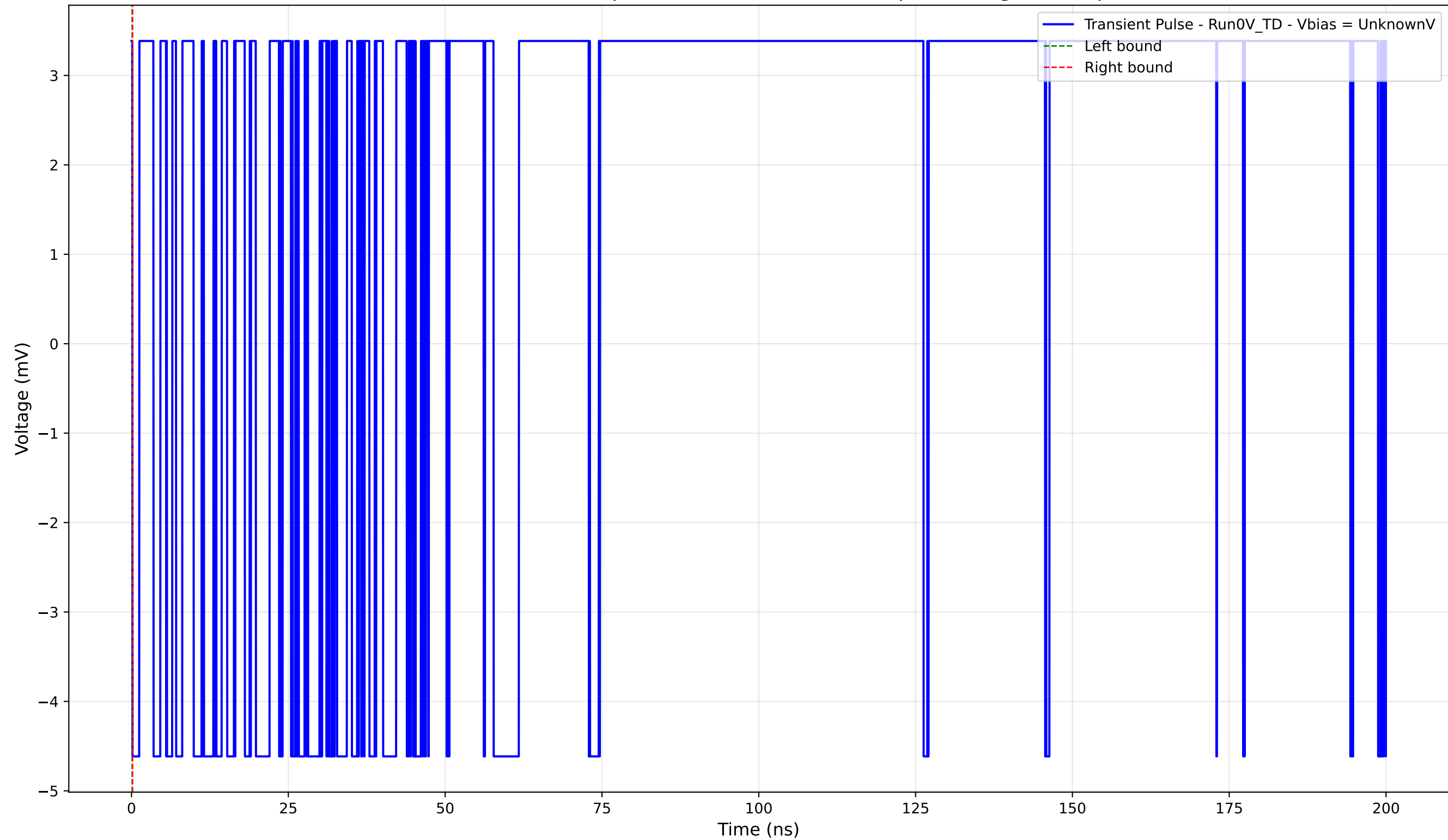
Transient Pulse - Sample: 4004 - Position: 1760.0 \mu\text{m} - Charge: -0.00 pC
