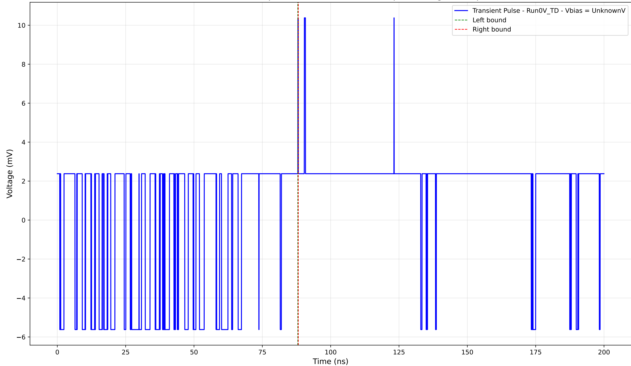
Transient Pulse - Sample: 4004 - Position: 1990.0 \mu\text{m} - Charge: 0.03 pC
