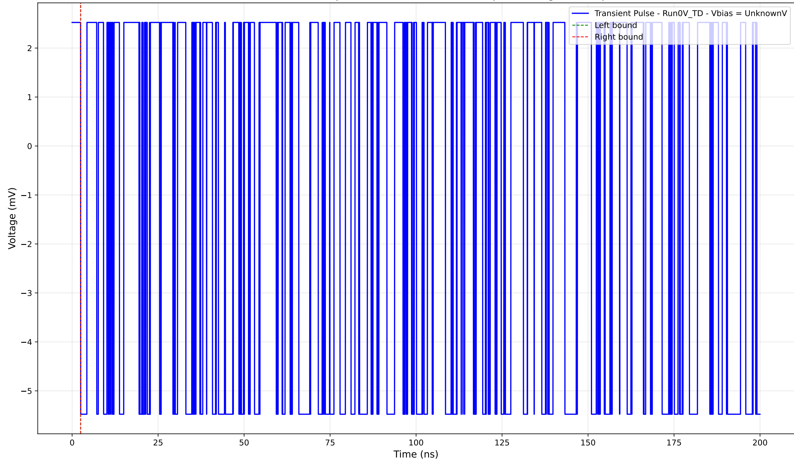
Transient Pulse - Sample: 4004 - Position: 1390.0 \mu\text{m} - Charge: -0.00 pC
