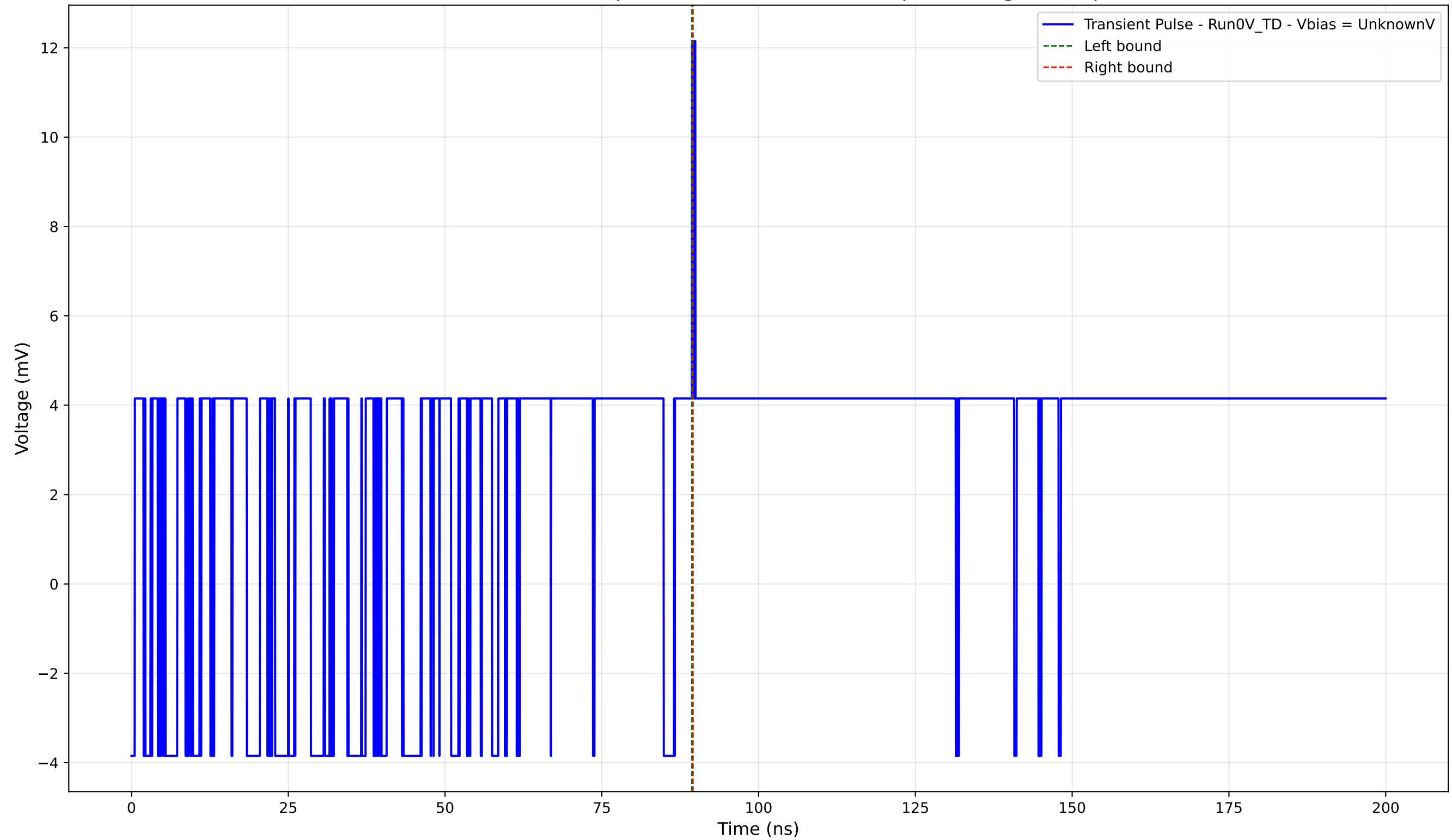
Transient Pulse - Sample: 4004 - Position: 1740.0 \mu\text{m} - Charge: 0.04 pC
