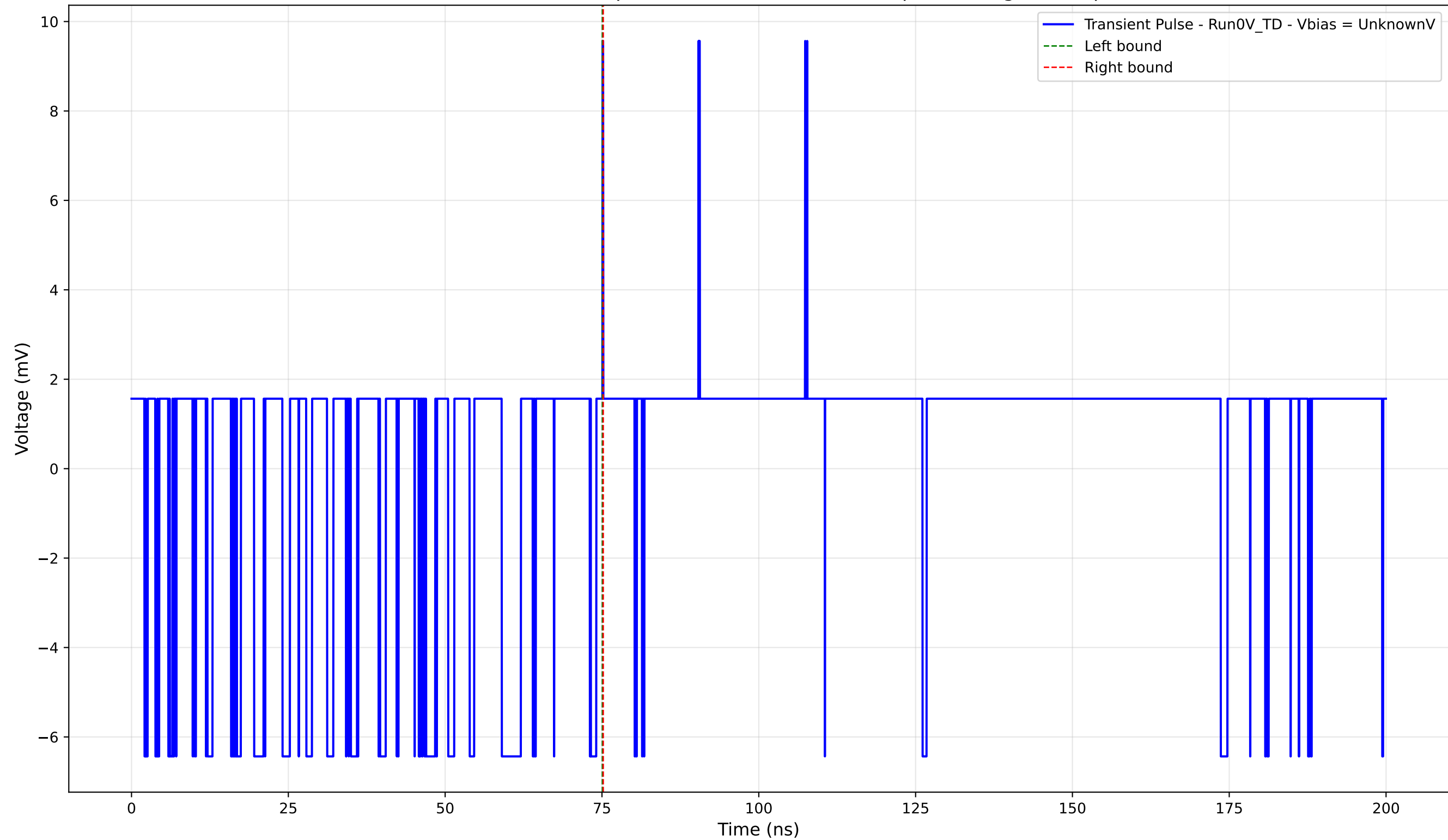
Transient Pulse - Sample: 4004 - Position: 1950.0 \mu\text{m} - Charge: 0.02 pC
