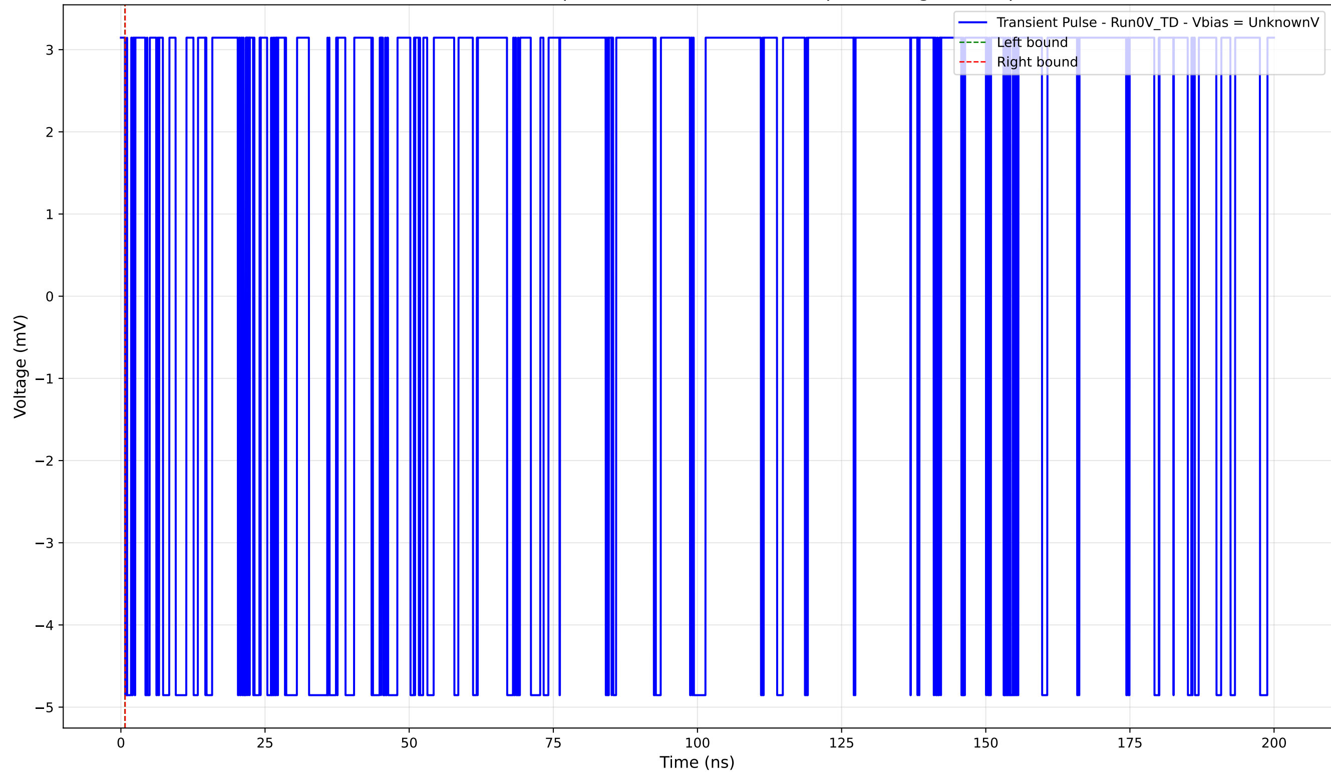
Transient Pulse - Sample: 4004 - Position: 1680.0 \mu\text{m} - Charge: -0.00 pC
