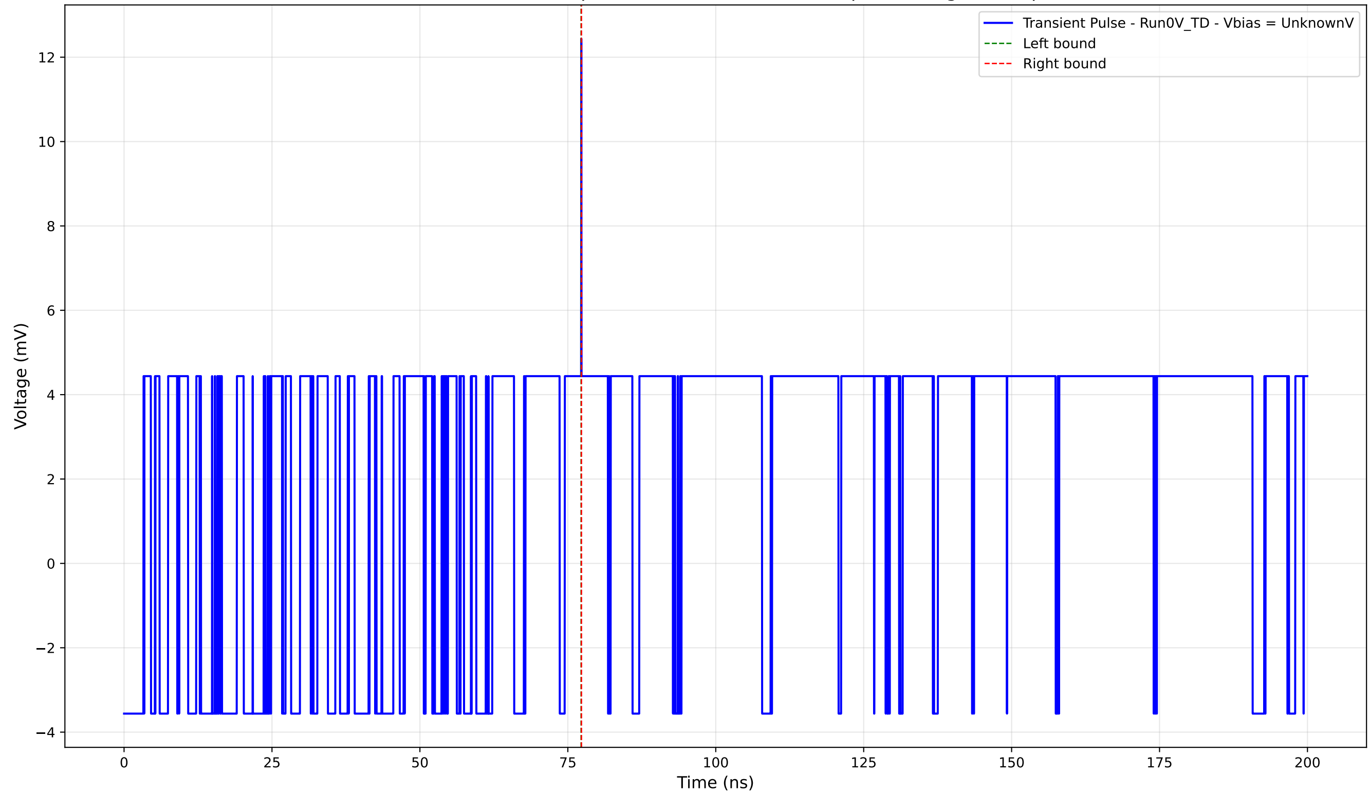
Transient Pulse - Sample: 4004 - Position: 1800.0 \mu\text{m} - Charge: 0.01 pC
