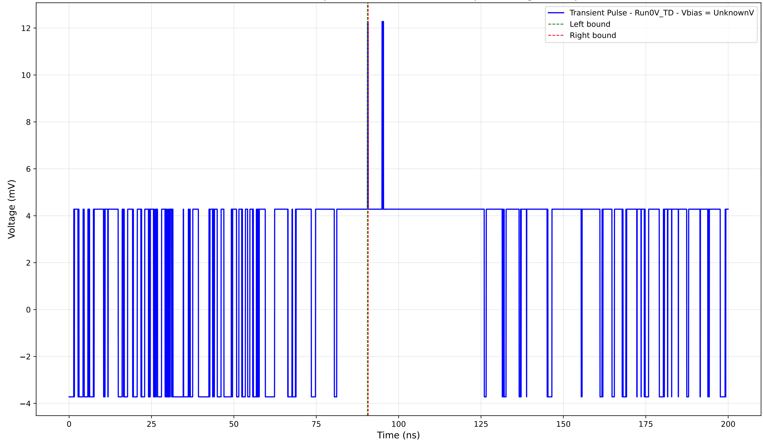
Transient Pulse - Sample: 4004 - Position: 1920.0 \mu\text{m} - Charge: 0.05 pC
