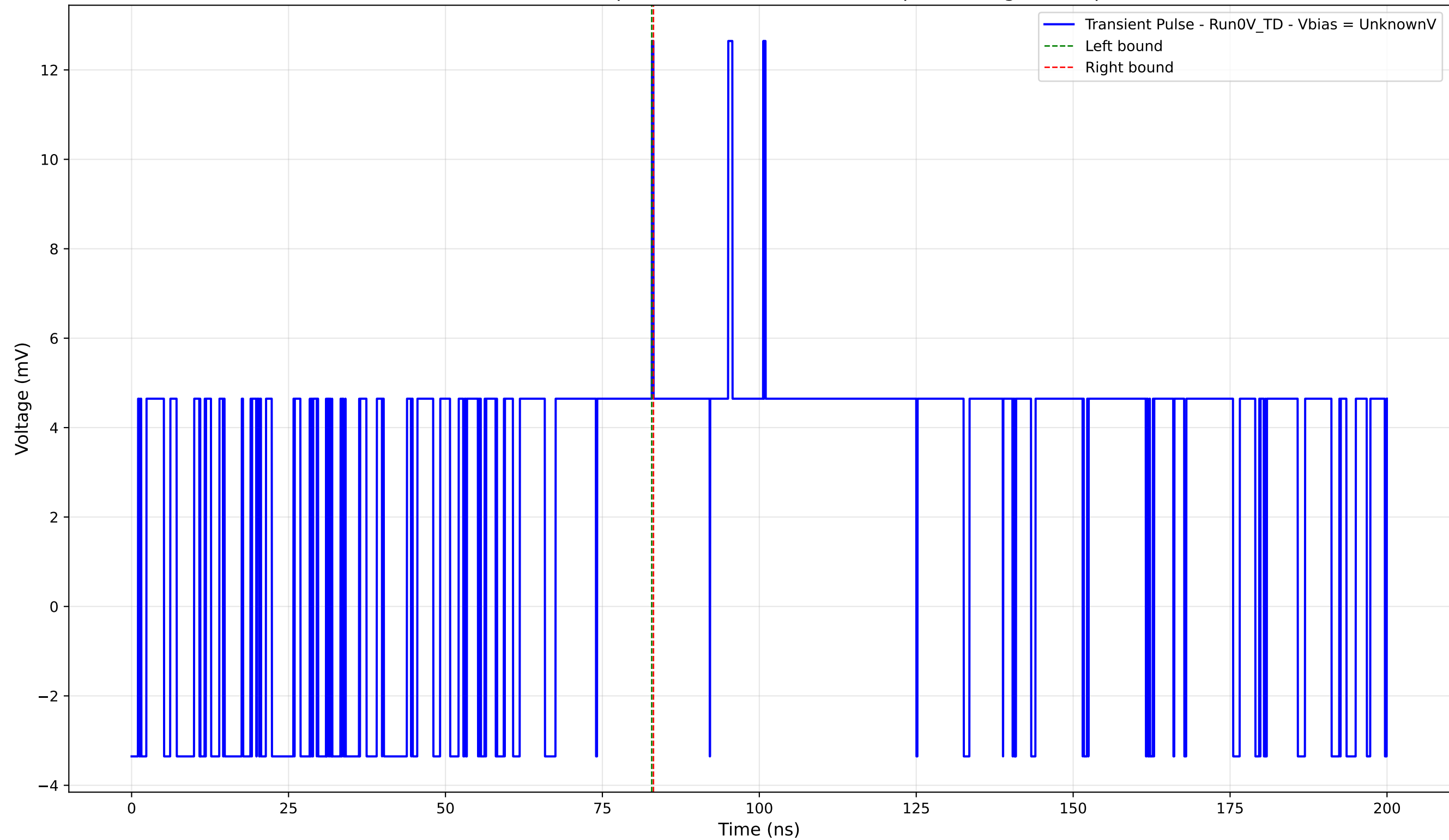
Transient Pulse - Sample: 4004 - Position: 1780.0 \mu\text{m} - Charge: 0.07 pC
