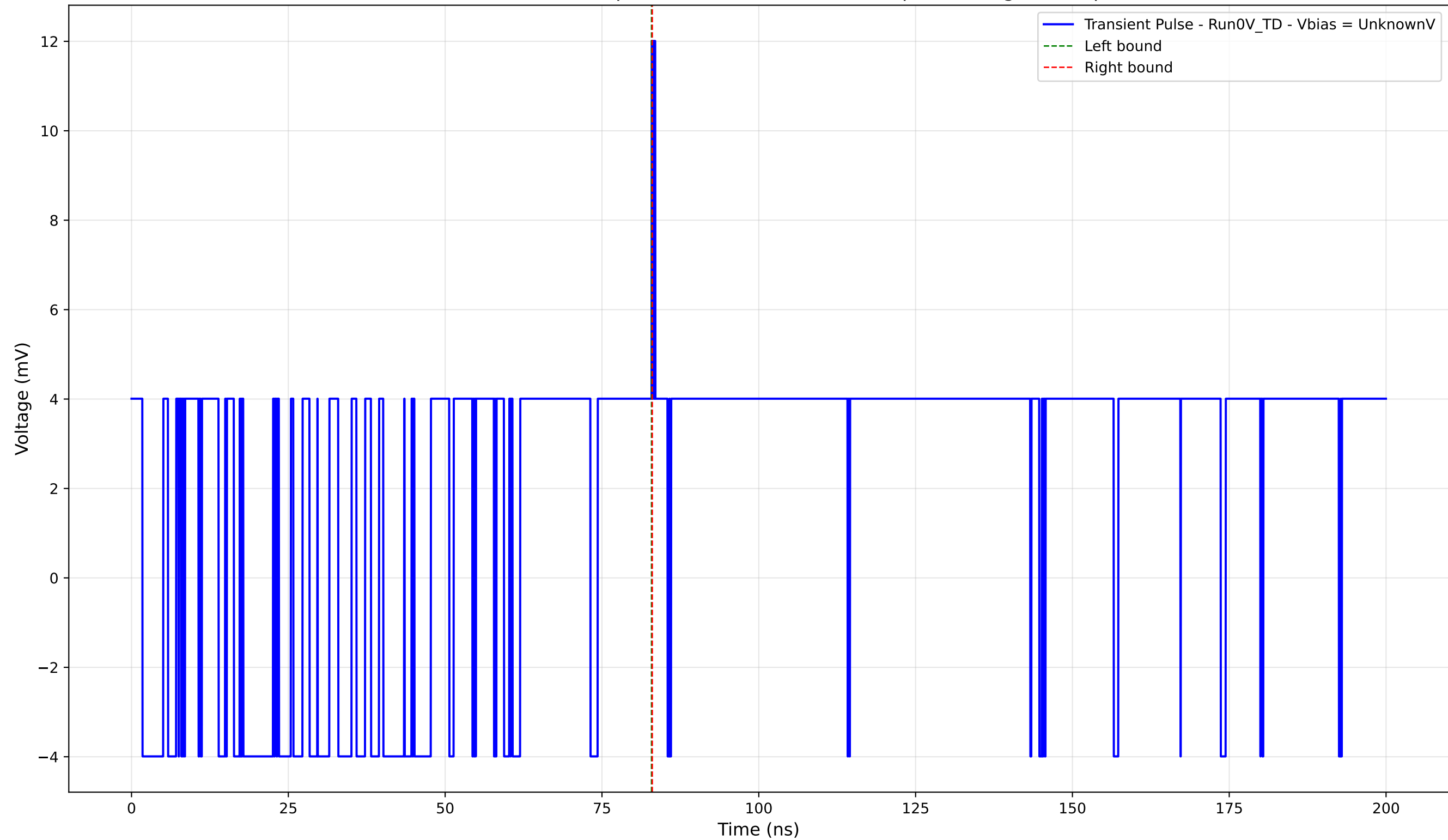
Transient Pulse - Sample: 4004 - Position: 1960.0 \mu\text{m} - Charge: 0.03 pC
