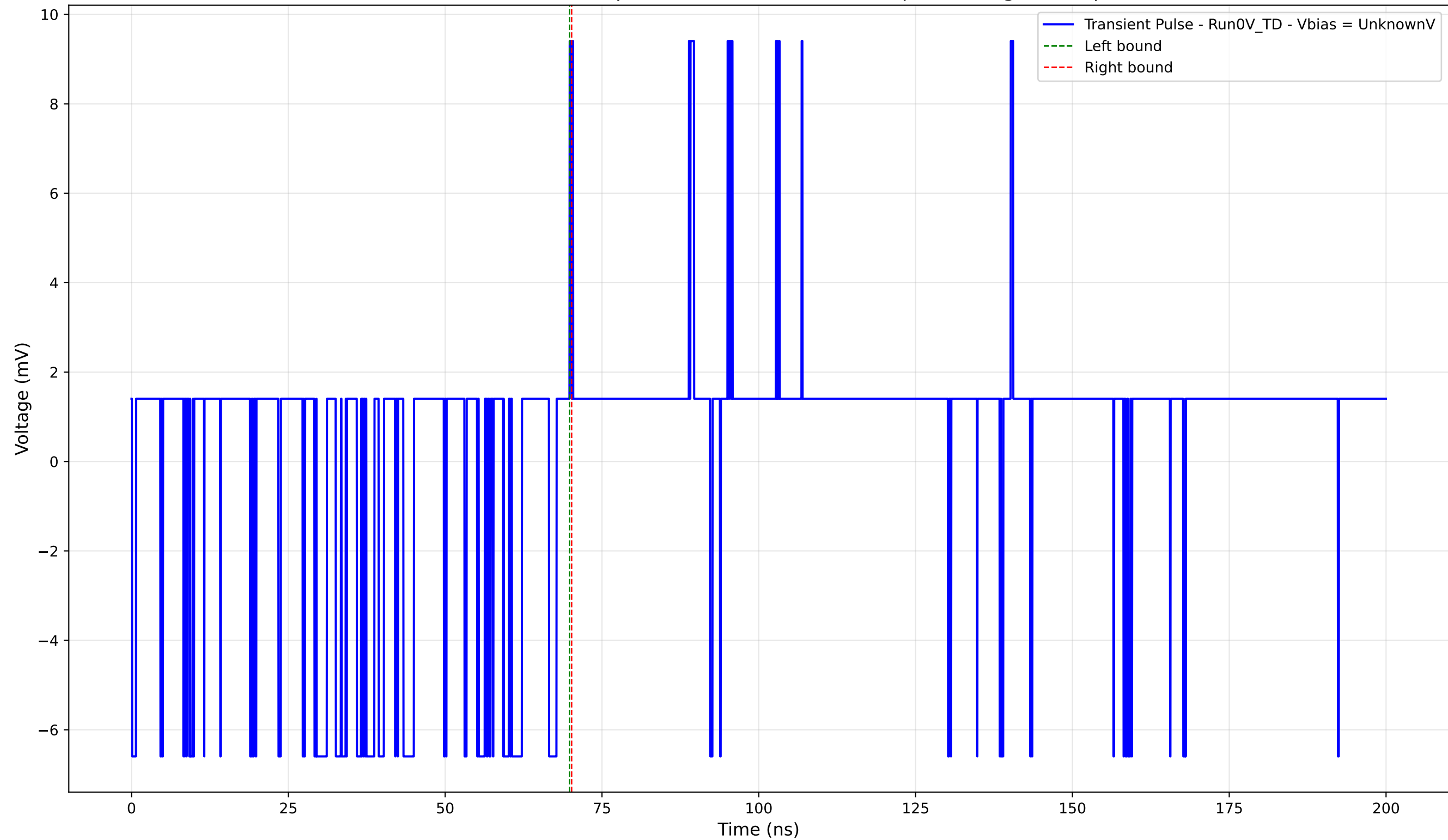
Transient Pulse - Sample: 4004 - Position: 1810.0 \mu\text{m} - Charge: 0.06 pC
