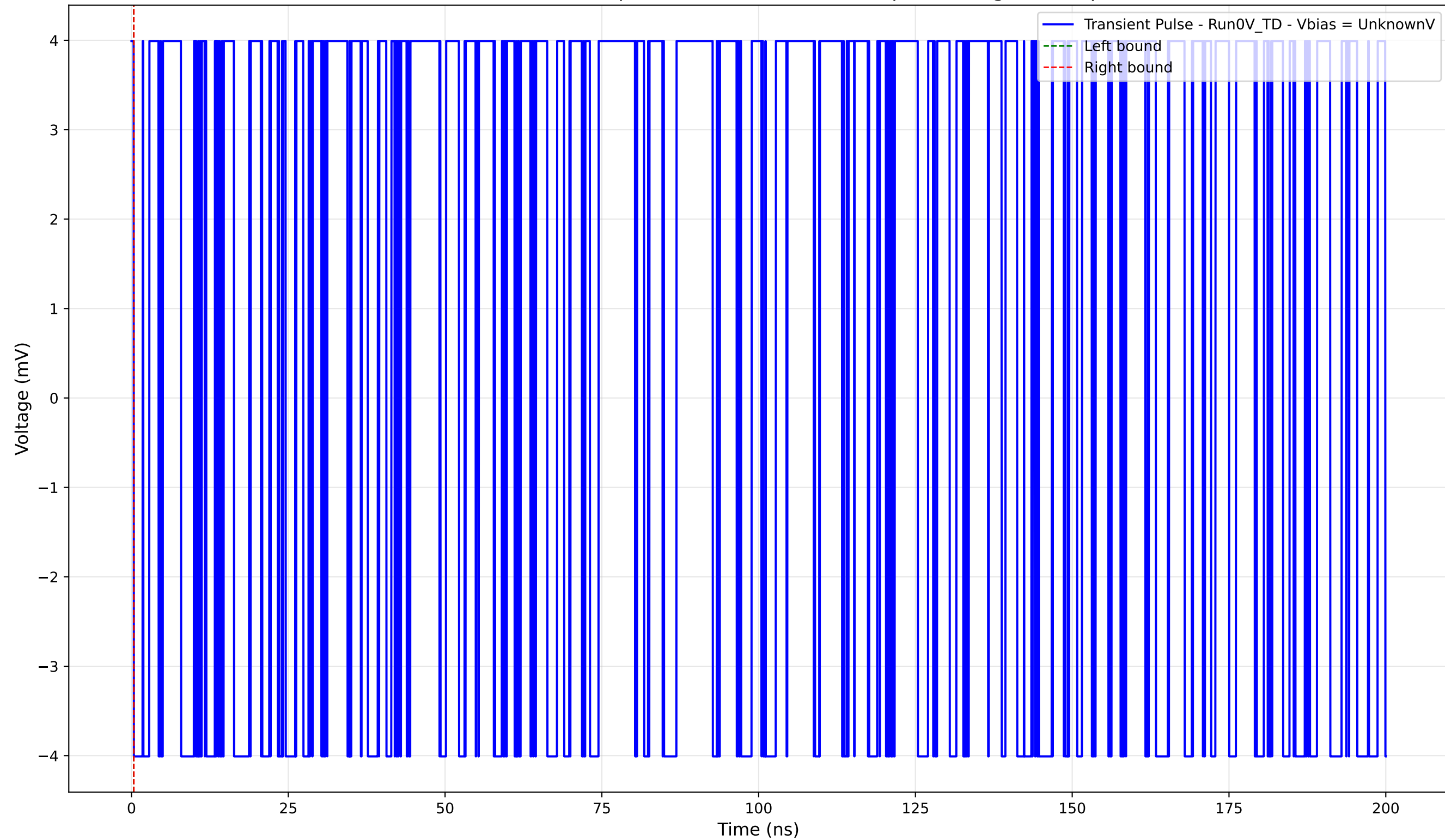
Transient Pulse - Sample: 4004 - Position: 560.0 \mu\text{m} - Charge: -0.00 pC
