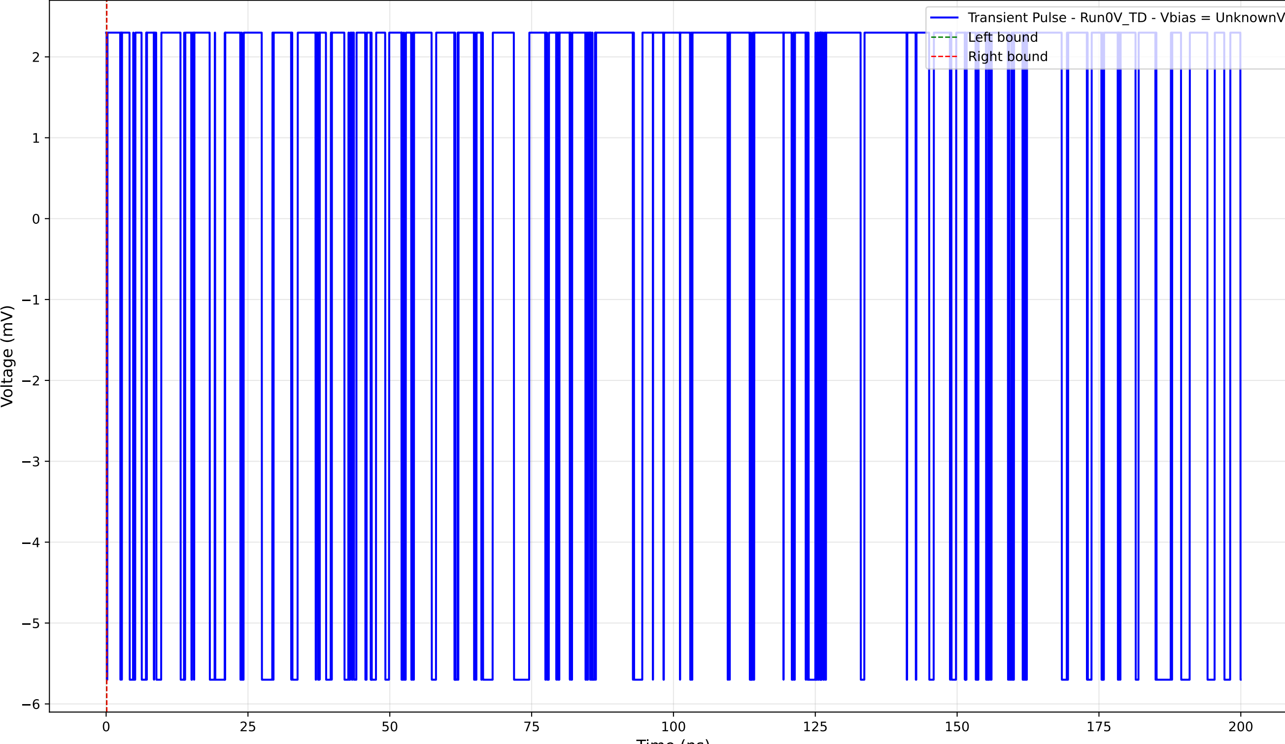
Transient Pulse - Sample: 4004 - Position: 1650.0 \mu\text{m} - Charge: -0.00 pC
