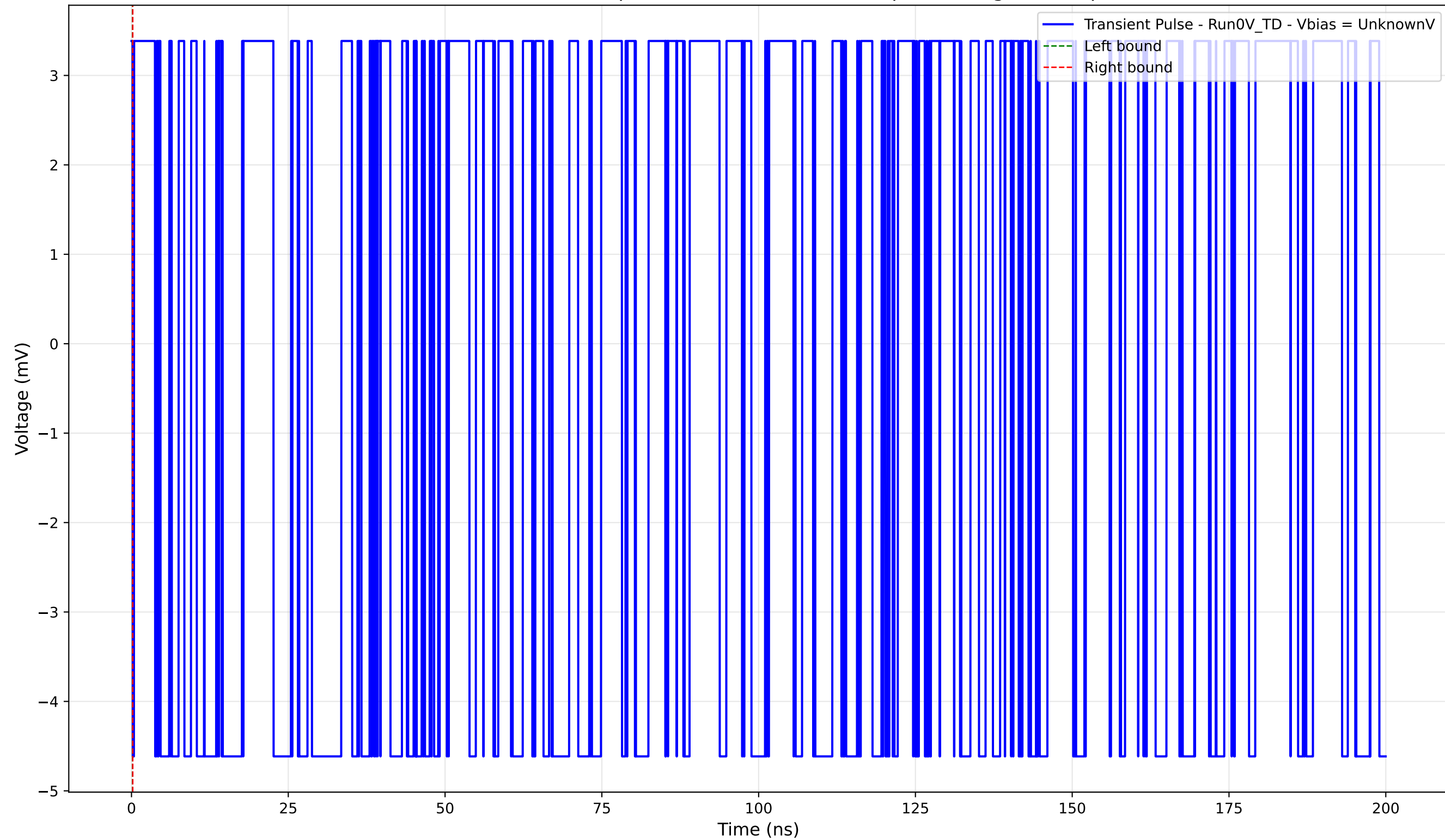
Transient Pulse - Sample: 4004 - Position: 600.0 \mu\text{m} - Charge: -0.00 pC
