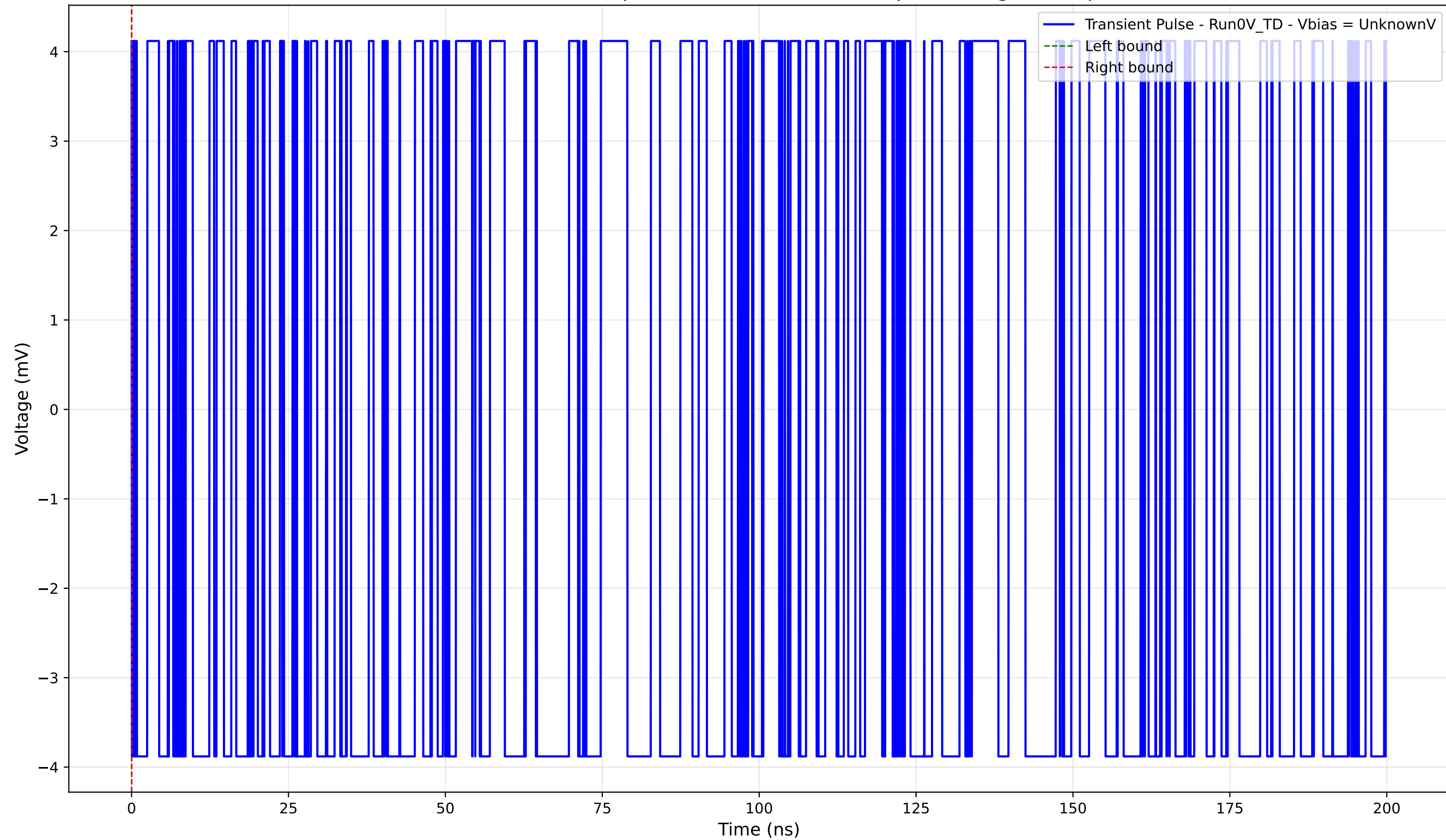
Transient Pulse - Sample: 4004 - Position: 860.0 \mu\text{m} - Charge: 0.00 pC
