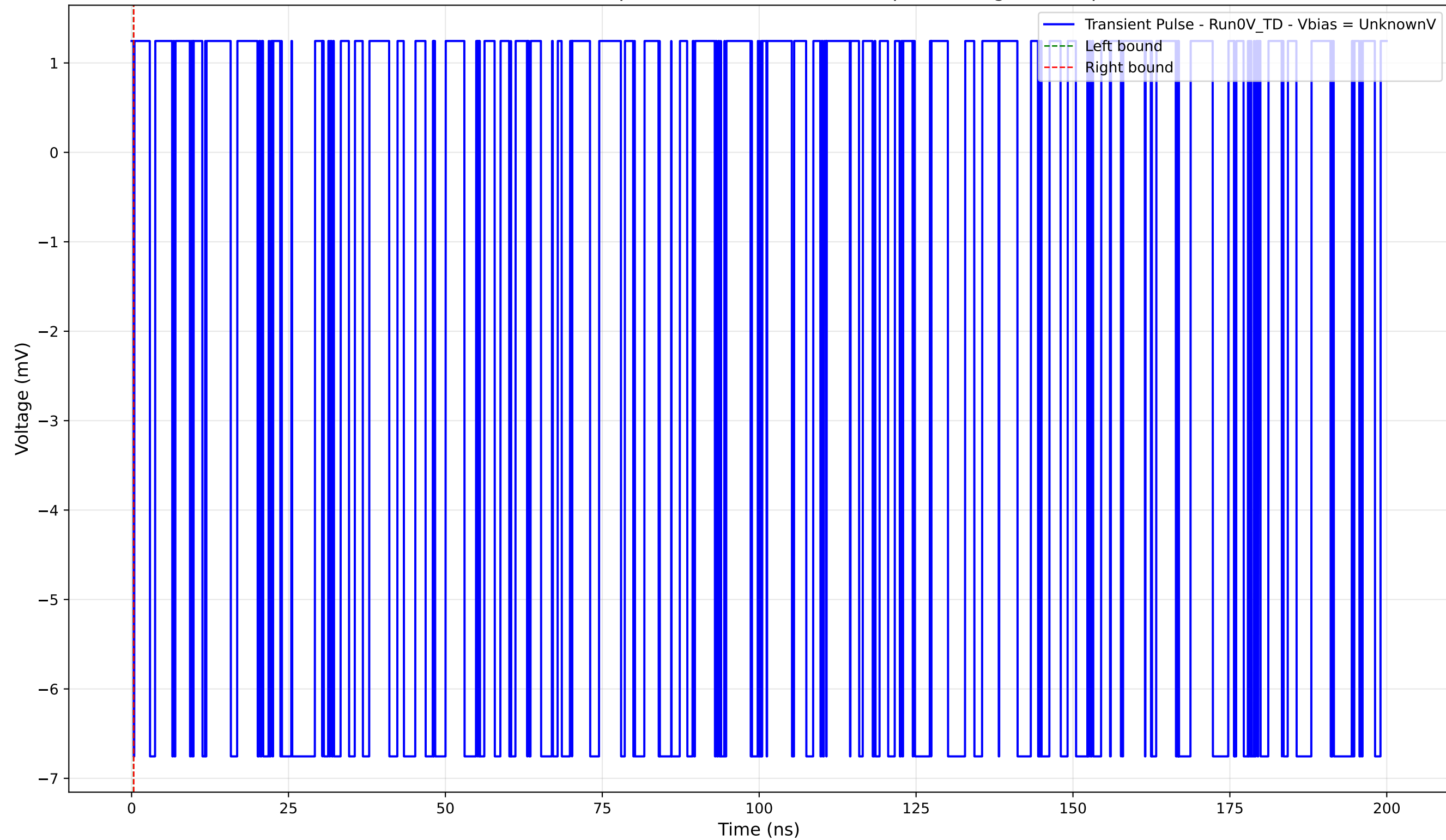
Transient Pulse - Sample: 4004 - Position: 240.0 \mu\text{m} - Charge: -0.00 pC
