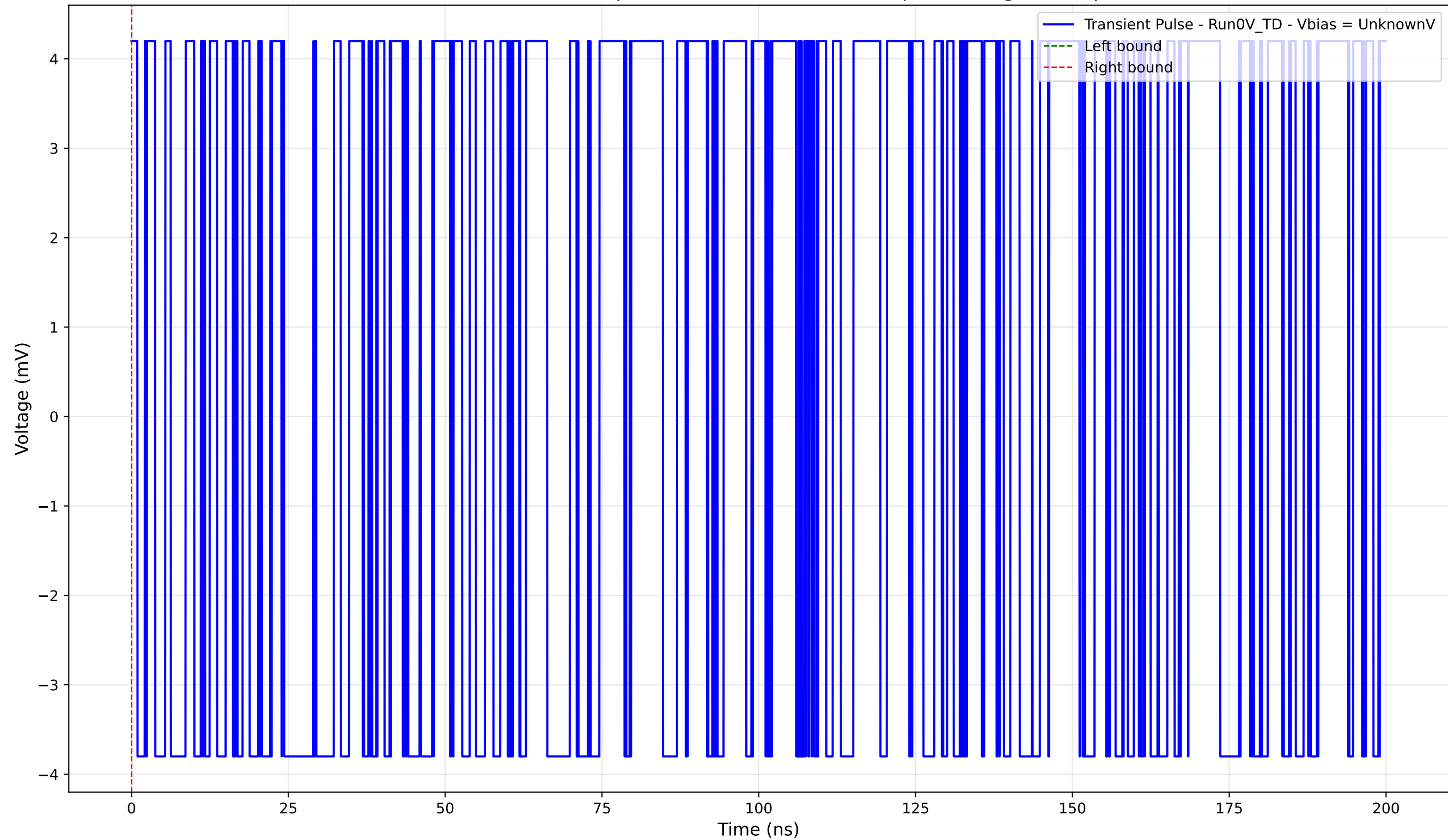
Transient Pulse - Sample: 4004 - Position: 1170.0 \mu\text{m} - Charge: 0.00 pC
