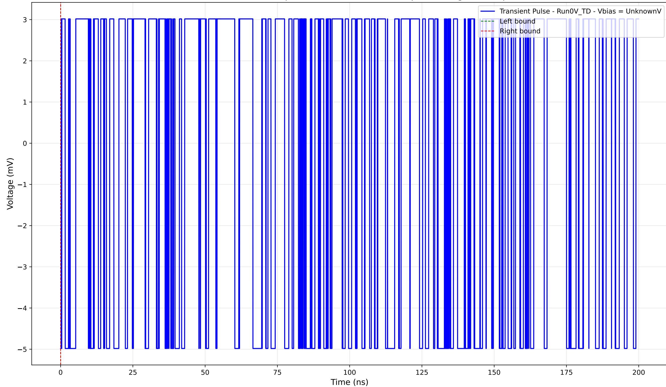
Transient Pulse - Sample: 4004 - Position: 520.0 \mu\text{m} - Charge: -0.00 pC
