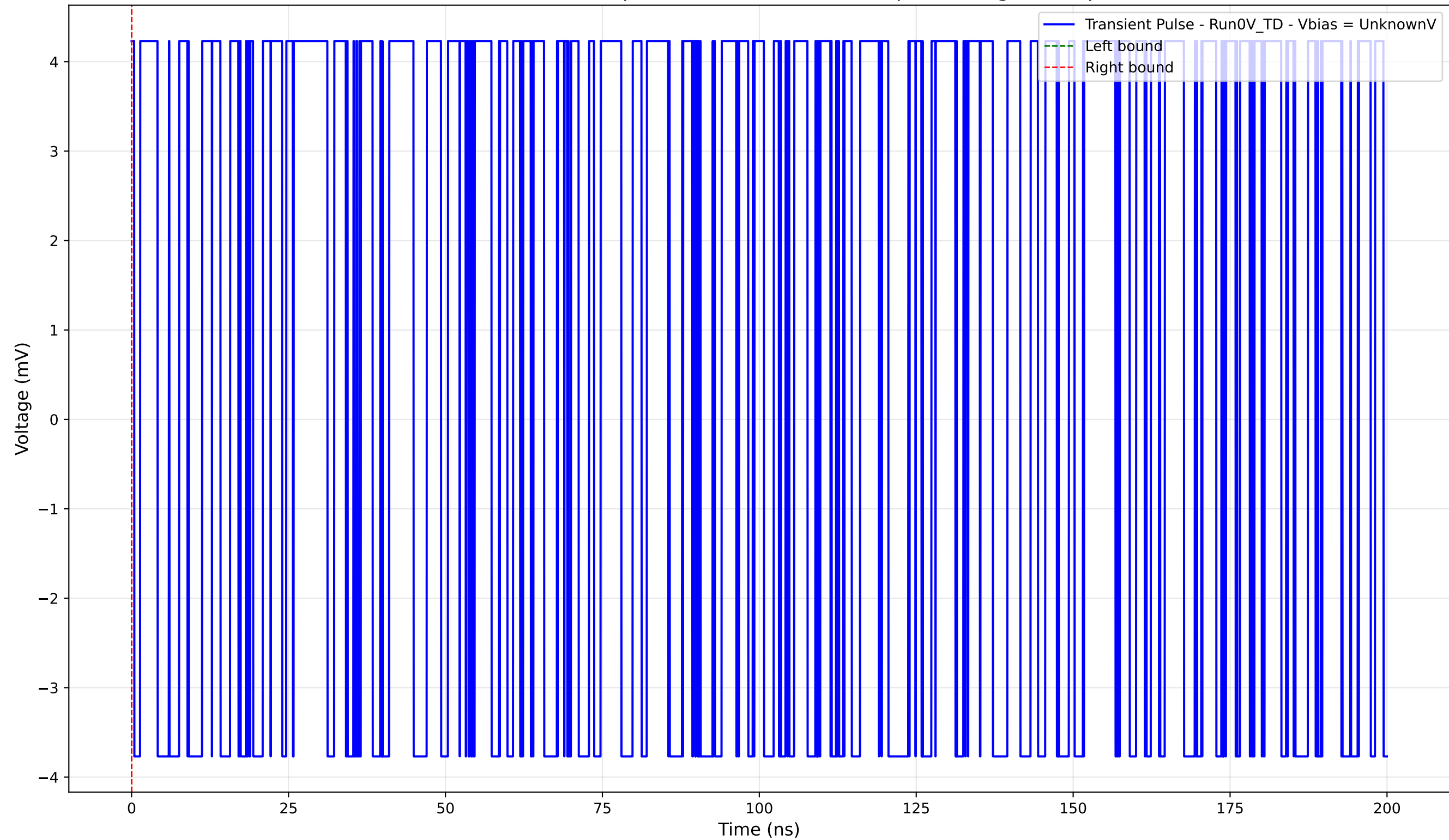
Transient Pulse - Sample: 4004 - Position: 990.0 \mu\text{m} - Charge: 0.00 pC
