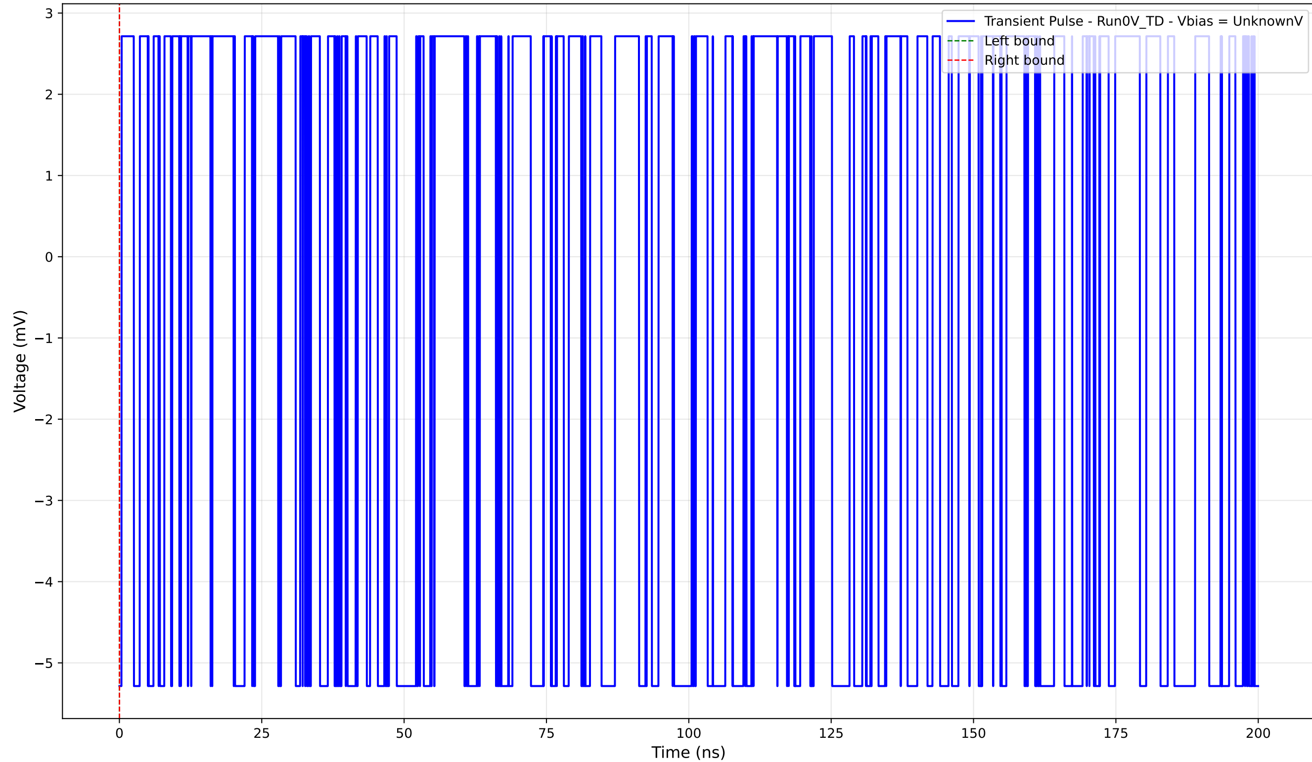
Transient Pulse - Sample: 4004 - Position: 830.0 \mu\text{m} - Charge: -0.00 pC
