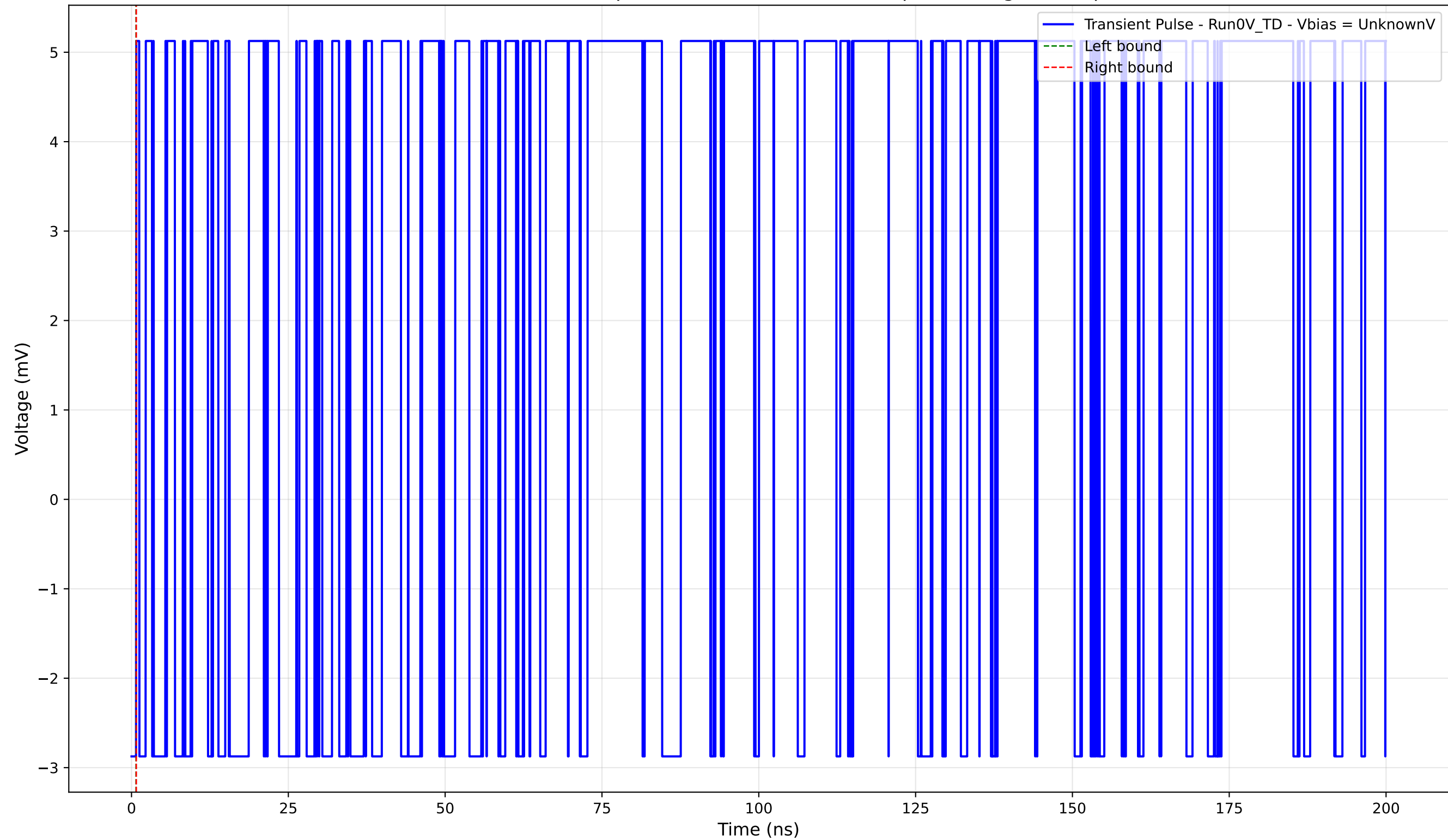
Transient Pulse - Sample: 4004 - Position: 1670.0 \mu\text{m} - Charge: 0.00 pC
