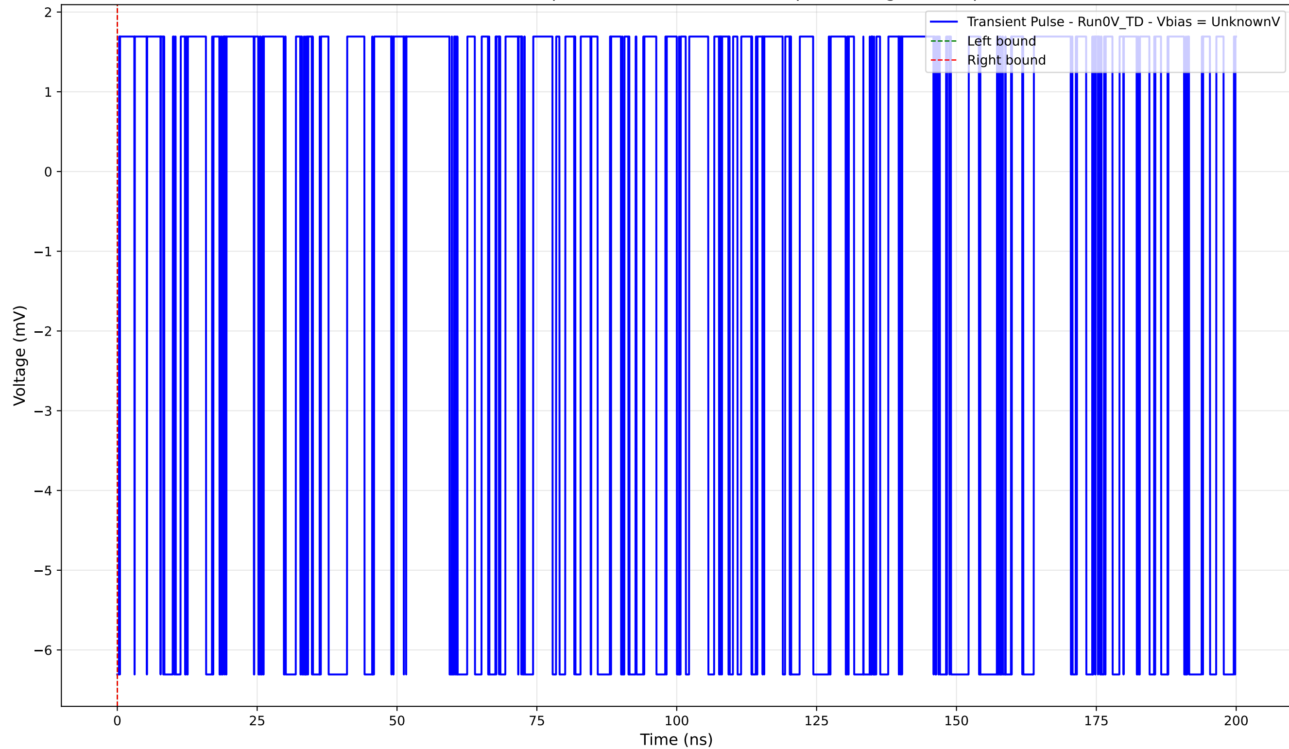
Transient Pulse - Sample: 4004 - Position: 220.0 \mu\text{m} - Charge: -0.00 pC
