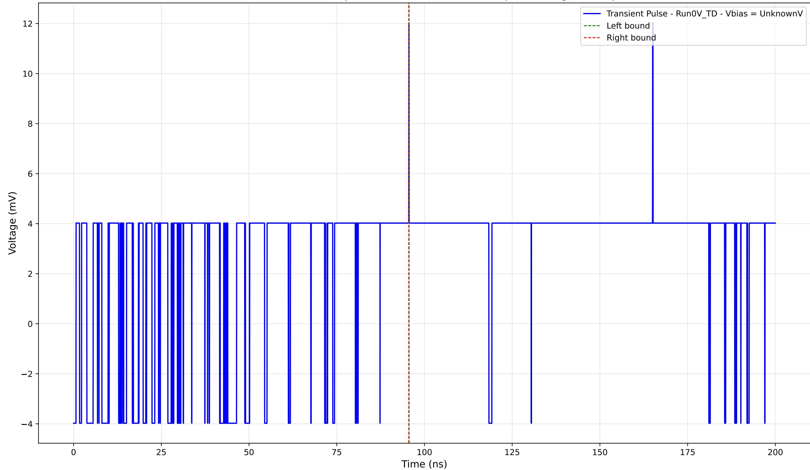
Transient Pulse - Sample: 4004 - Position: 1730.0 \mu\text{m} - Charge: 0.02 pC
