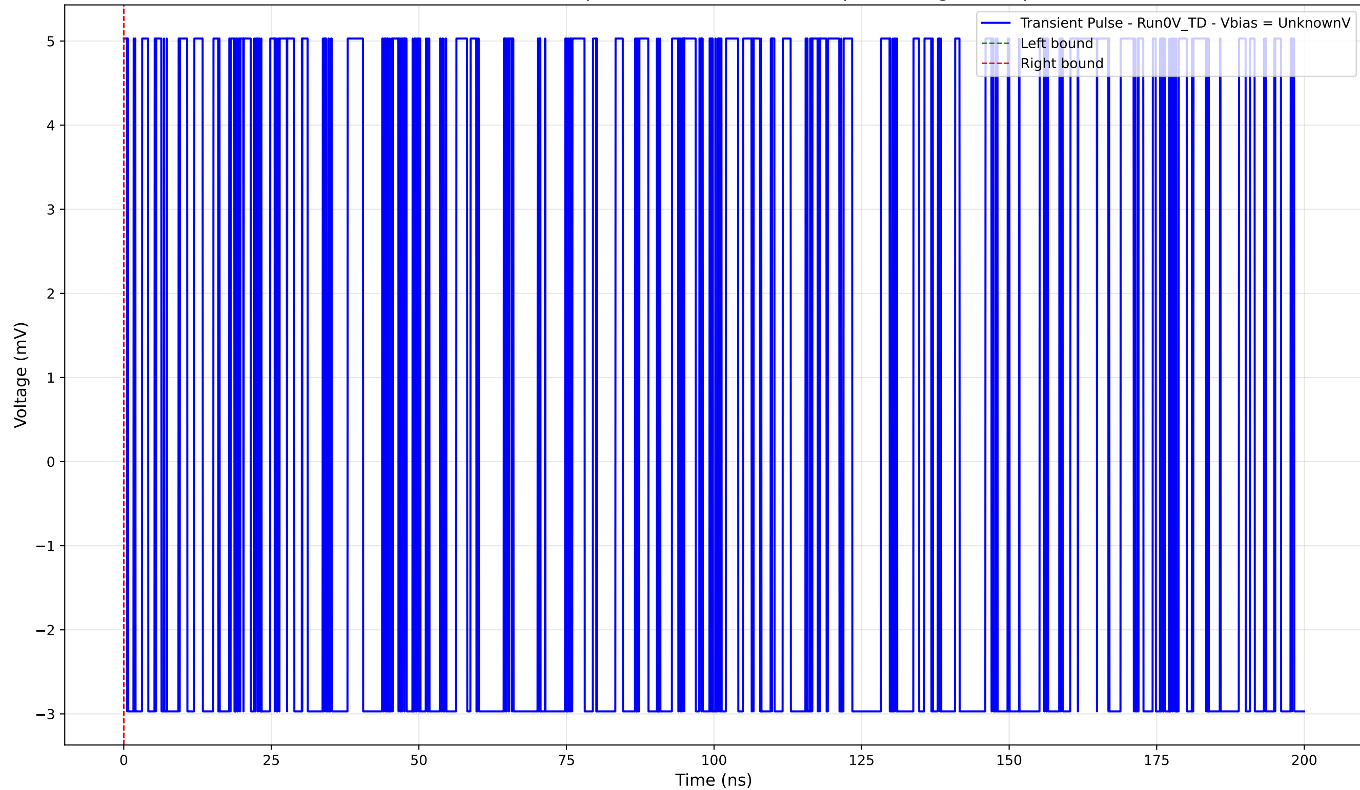
Transient Pulse - Sample: 4004 - Position: 410.0 \mu\text{m} - Charge: 0.00 pC
