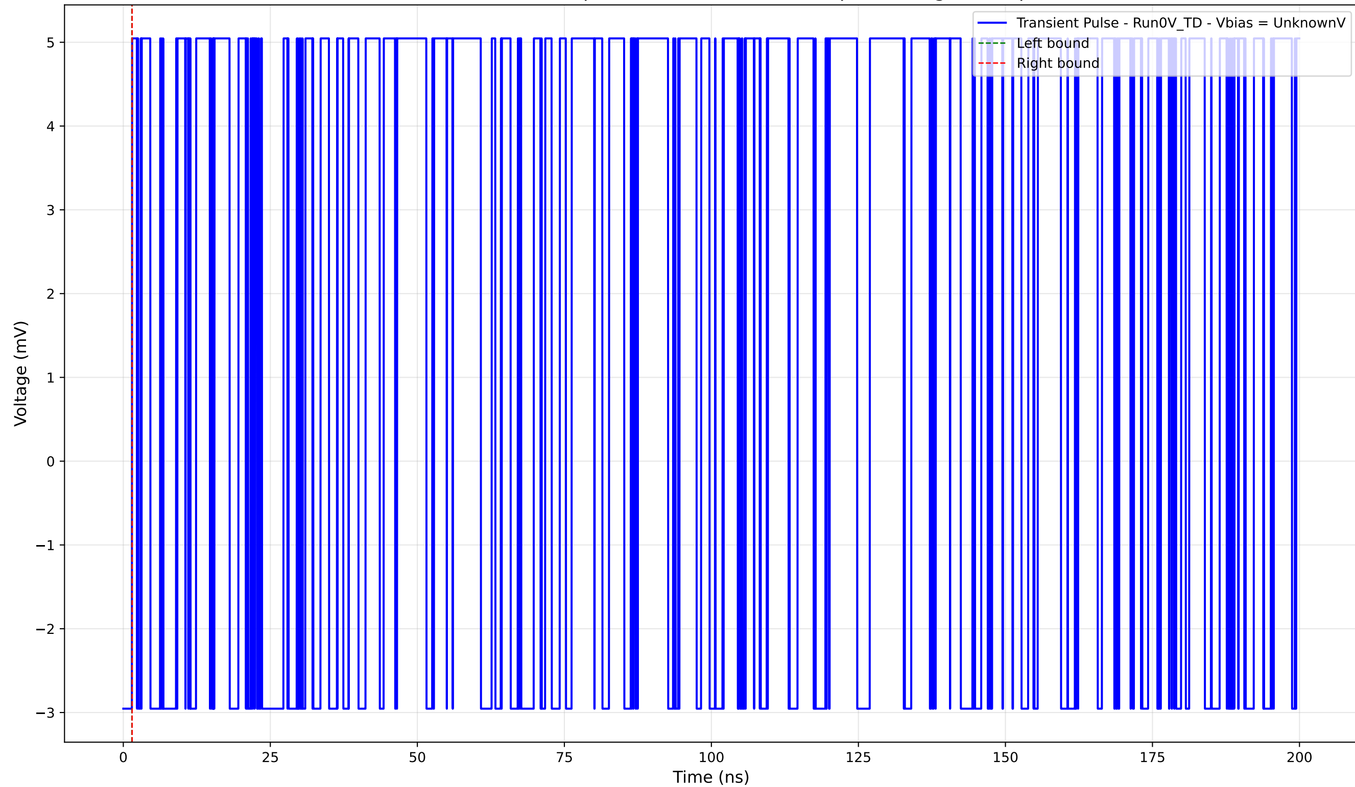
Transient Pulse - Sample: 4004 - Position: 360.0 \mu\text{m} - Charge: 0.00 pC
