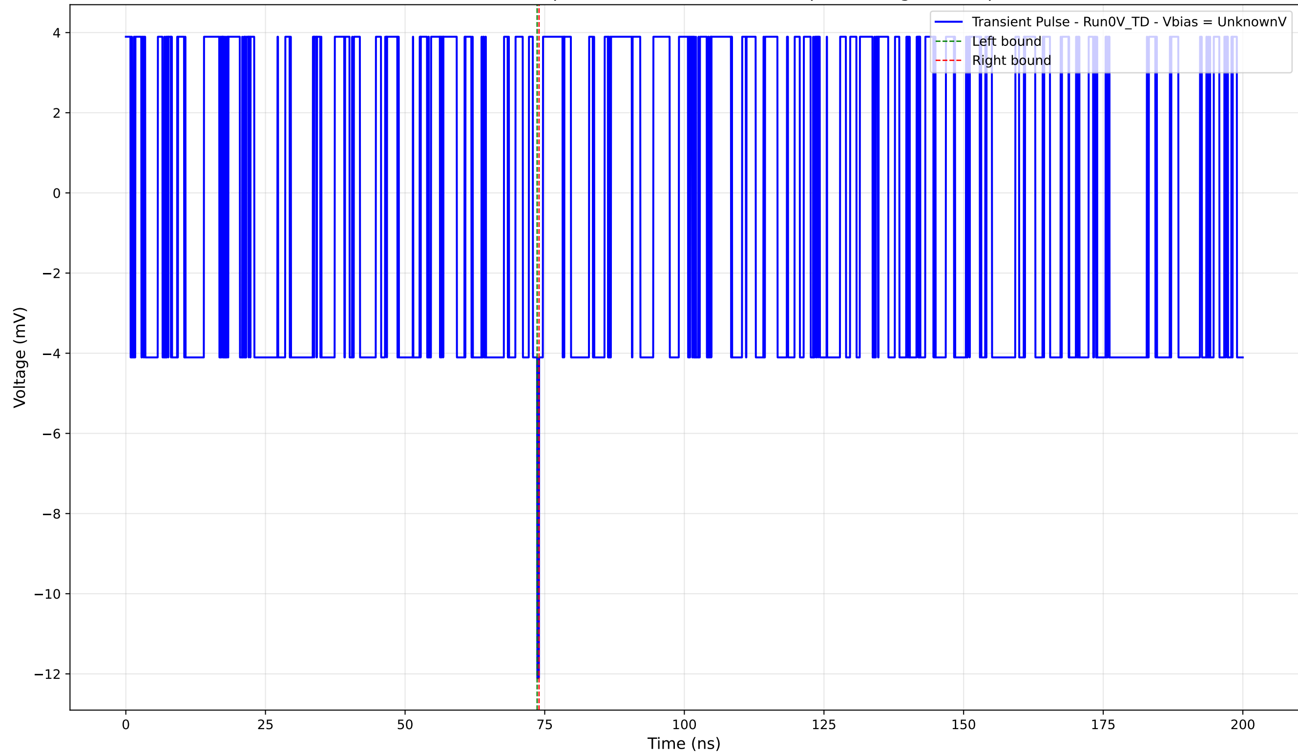
Transient Pulse - Sample: 4004 - Position: 1490.0 \mu\text{m} - Charge: -0.08 pC
