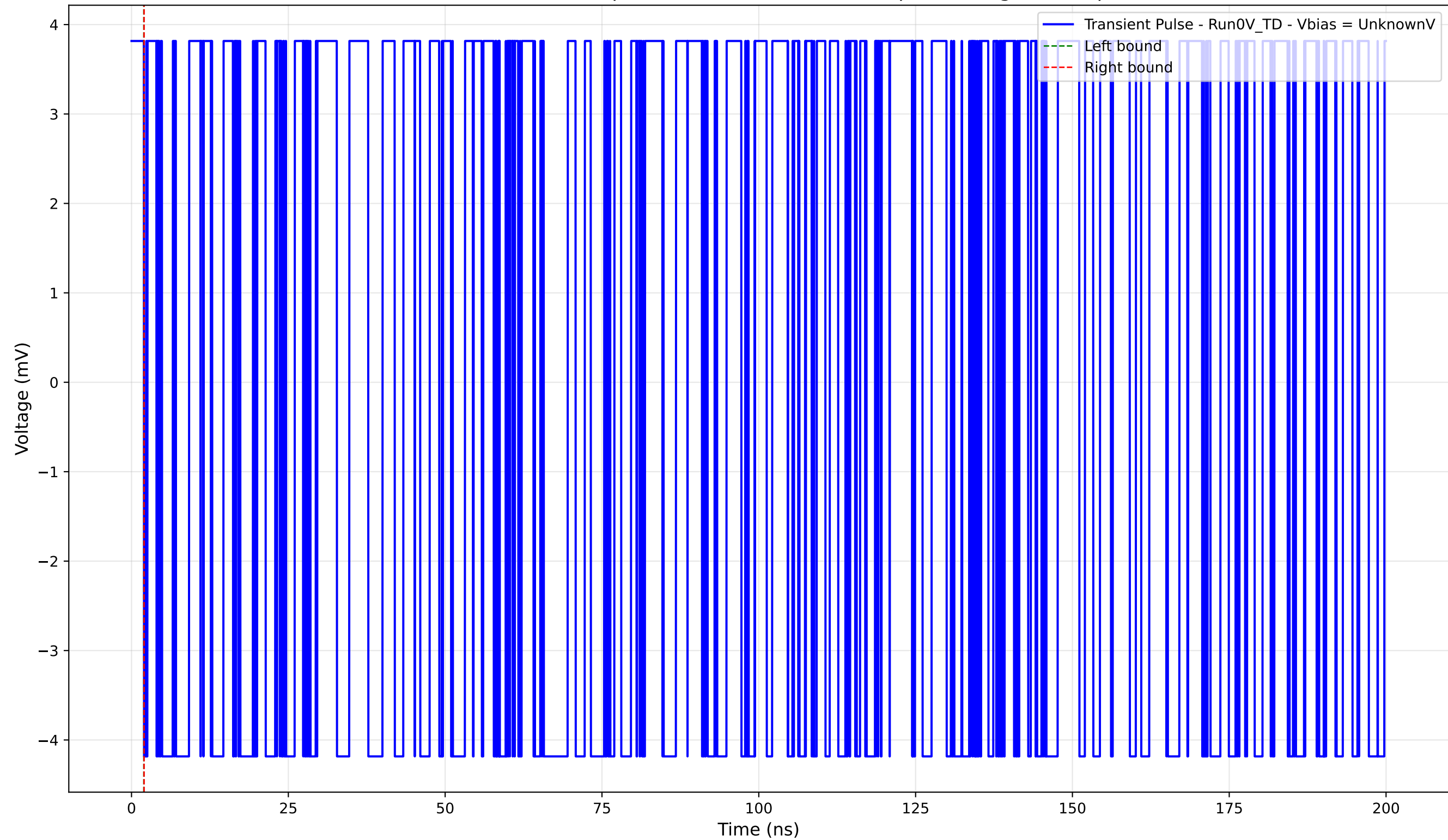
Transient Pulse - Sample: 4004 - Position: 1270.0 \mu\text{m} - Charge: -0.00 pC
