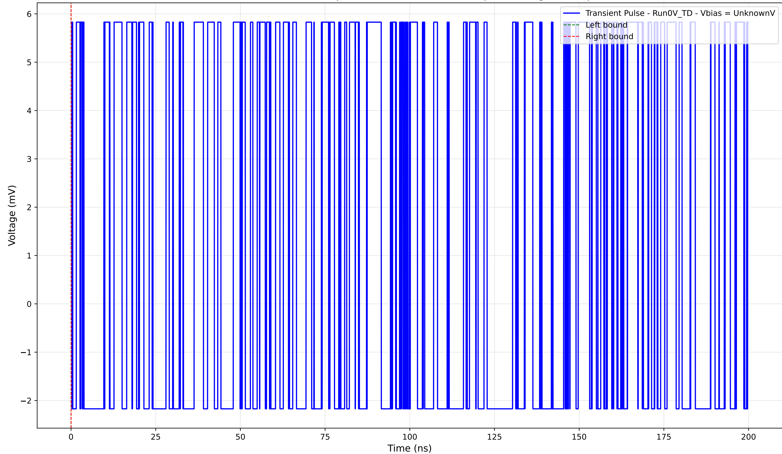
Transient Pulse - Sample: 4004 - Position: 430.0 \mu\text{m} - Charge: 0.00 pC
