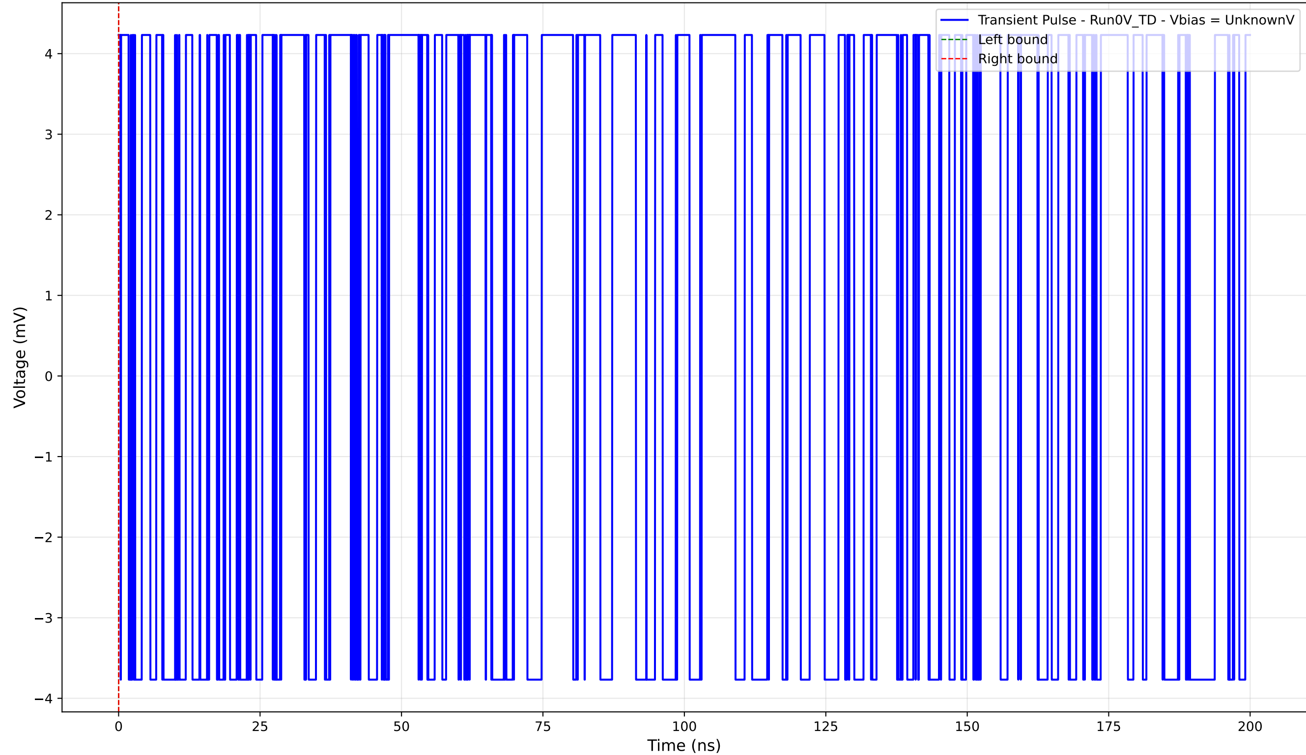
Transient Pulse - Sample: 4004 - Position: 1560.0 \mu\text{m} - Charge: 0.00 pC
