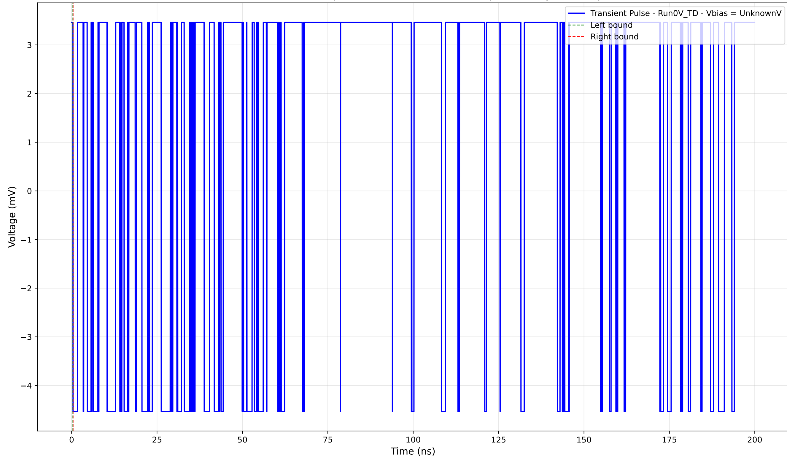
Transient Pulse - Sample: 4004 - Position: 1700.0 \mu\text{m} - Charge: -0.00 pC
