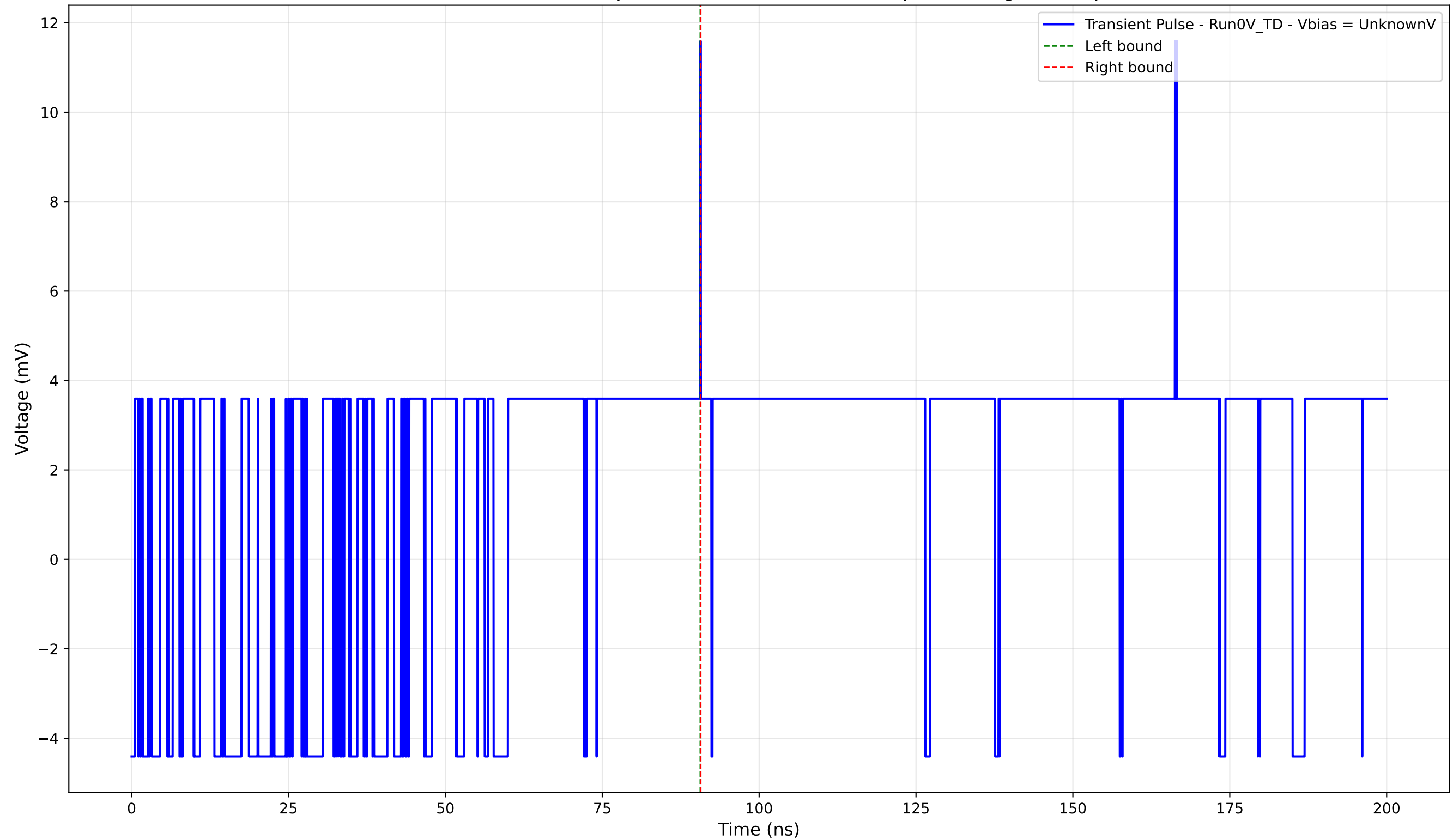
Transient Pulse - Sample: 4004 - Position: 1860.0 \mu\text{m} - Charge: 0.02 pC
