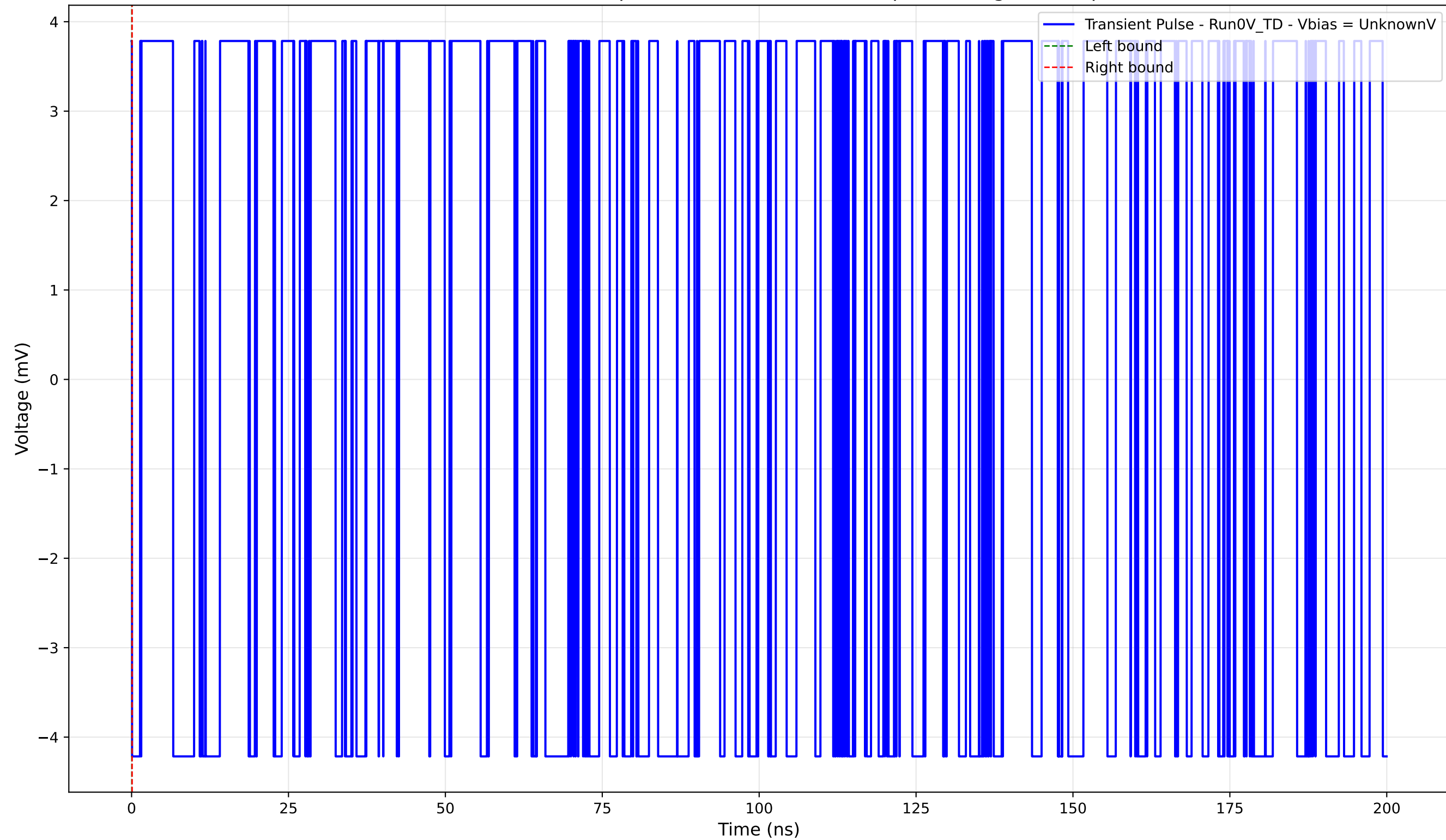
Transient Pulse - Sample: 4004 - Position: 690.0 \mu\text{m} - Charge: -0.00 pC
