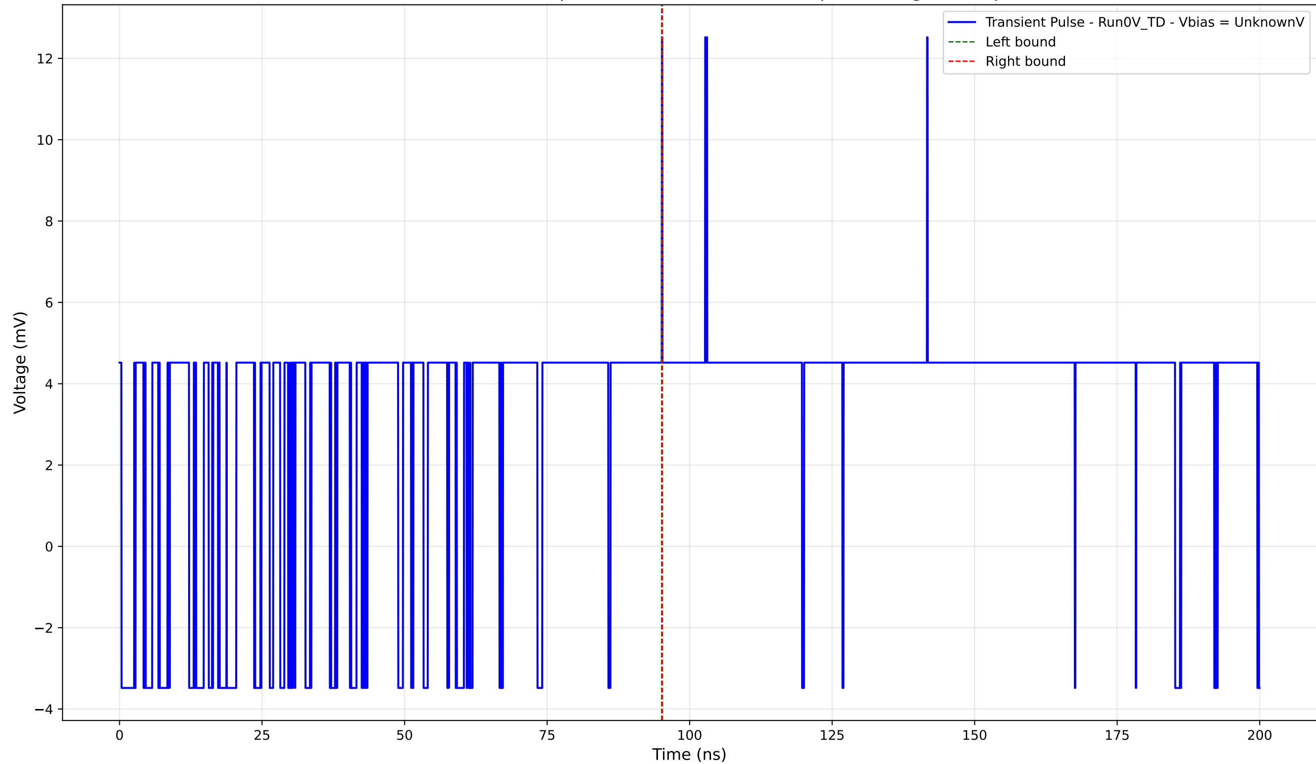
Transient Pulse - Sample: 4004 - Position: 1770.0 \mu\text{m} - Charge: 0.03 pC
