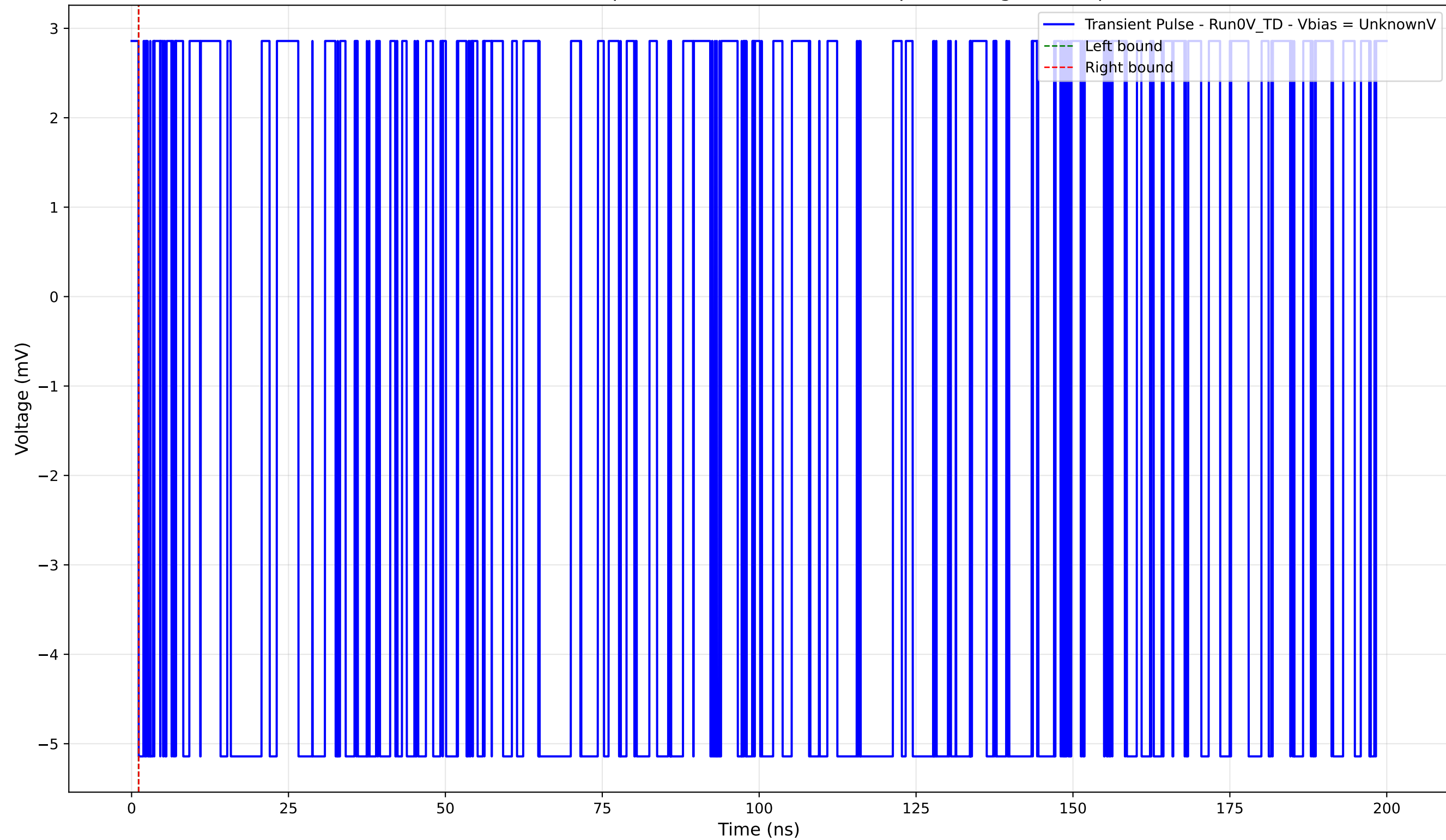
Transient Pulse - Sample: 4004 - Position: 1530.0 \mu\text{m} - Charge: -0.00 pC
