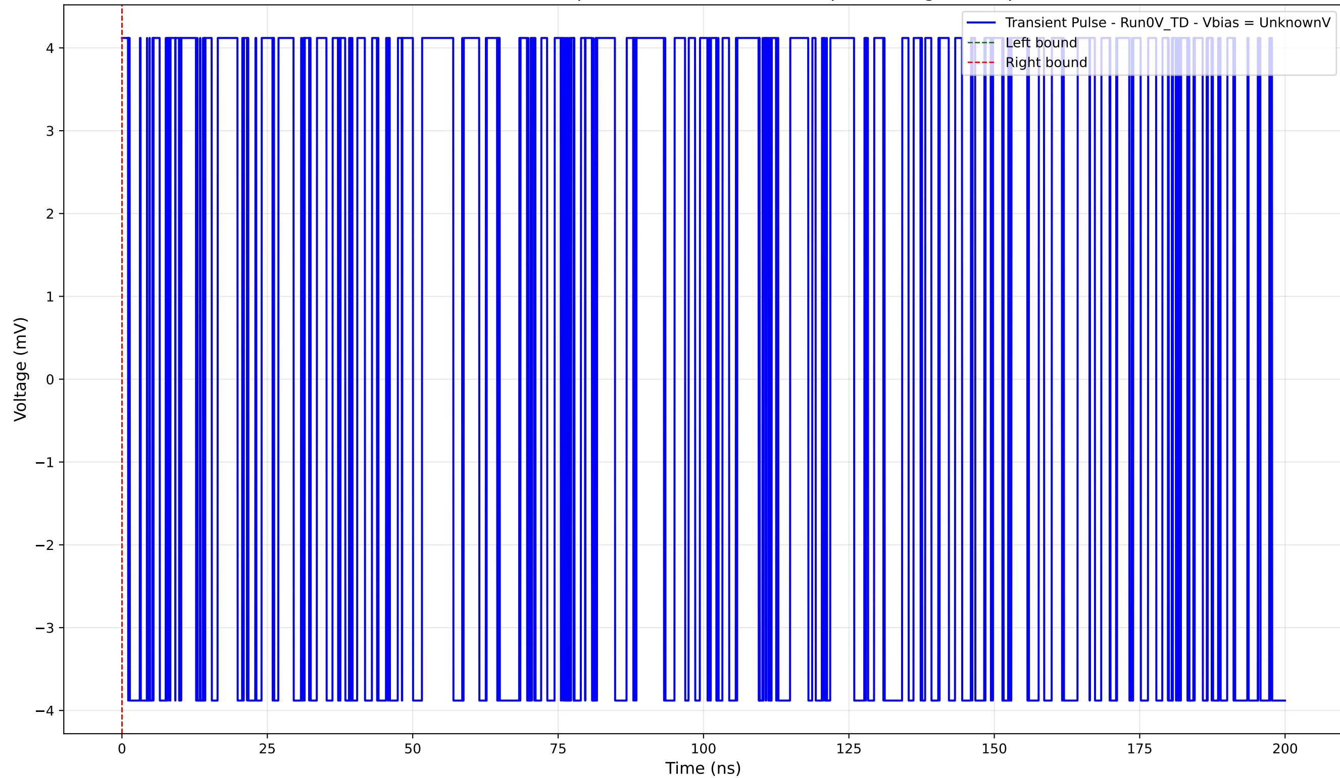
Transient Pulse - Sample: 4004 - Position: 110.0 \mu\text{m} - Charge: 0.00 pC
