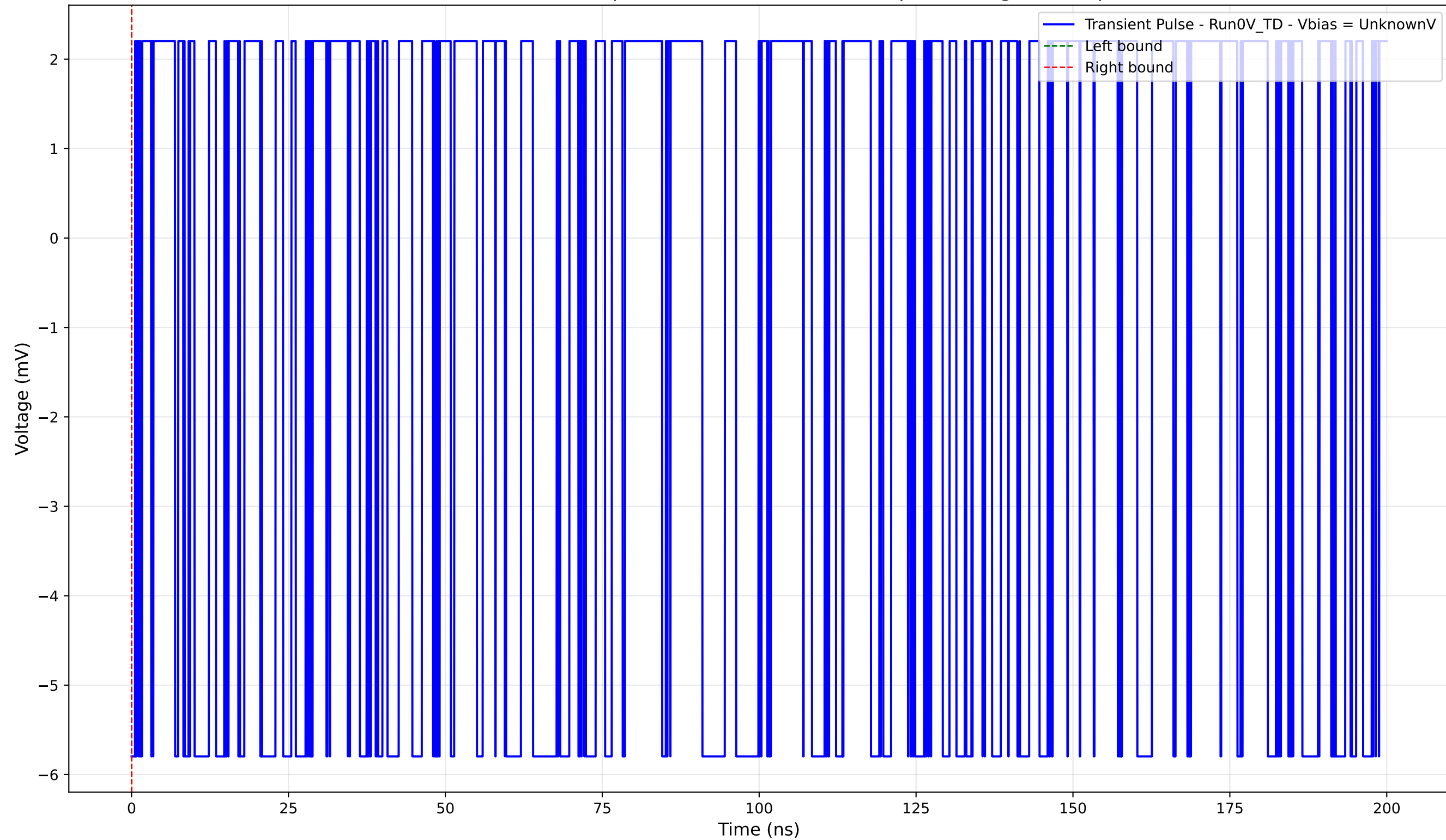
Transient Pulse - Sample: 4004 - Position: 1350.0 \mu\text{m} - Charge: -0.00 pC
