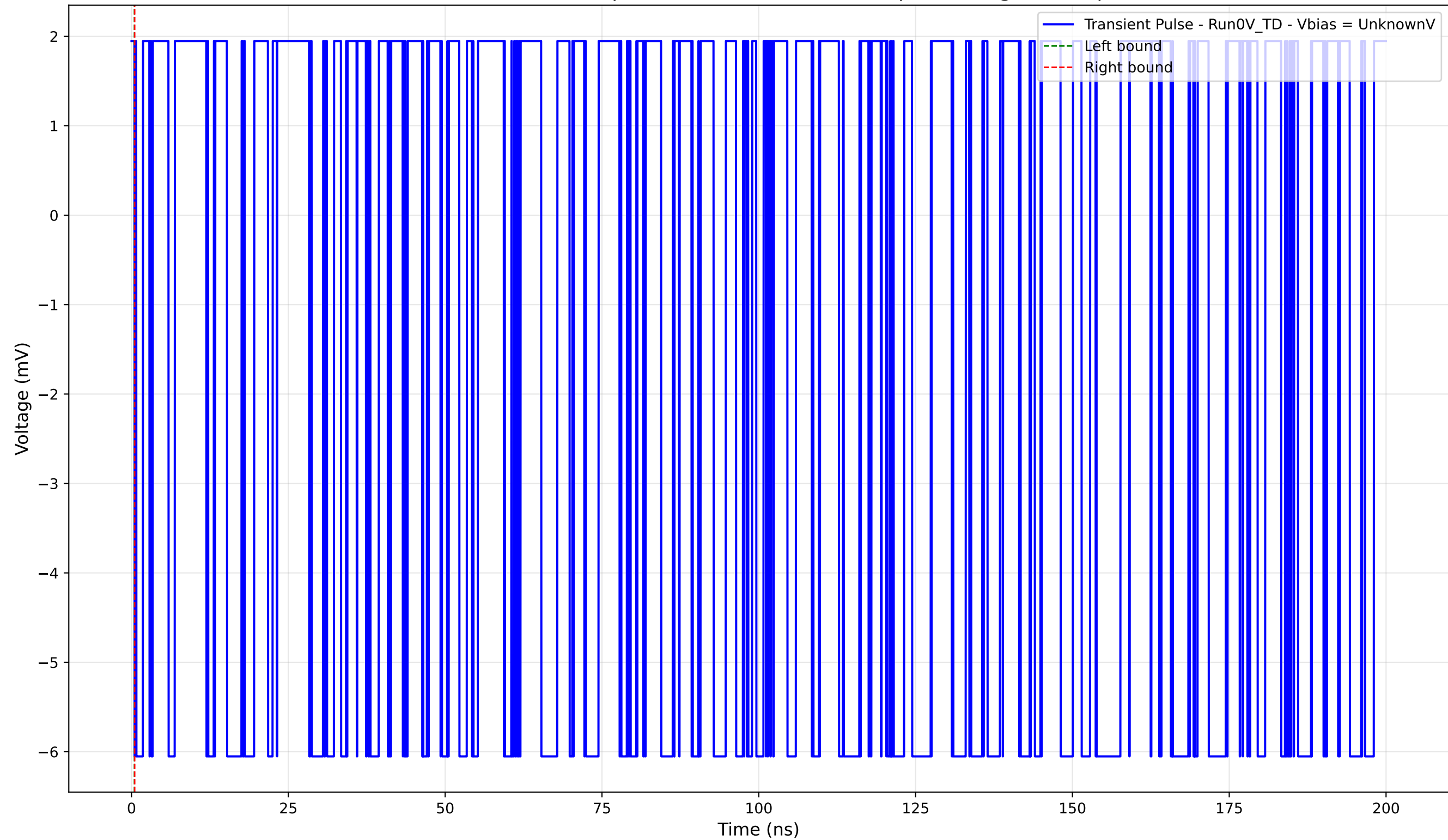
Transient Pulse - Sample: 4004 - Position: 1550.0 \mu\text{m} - Charge: -0.00 pC
