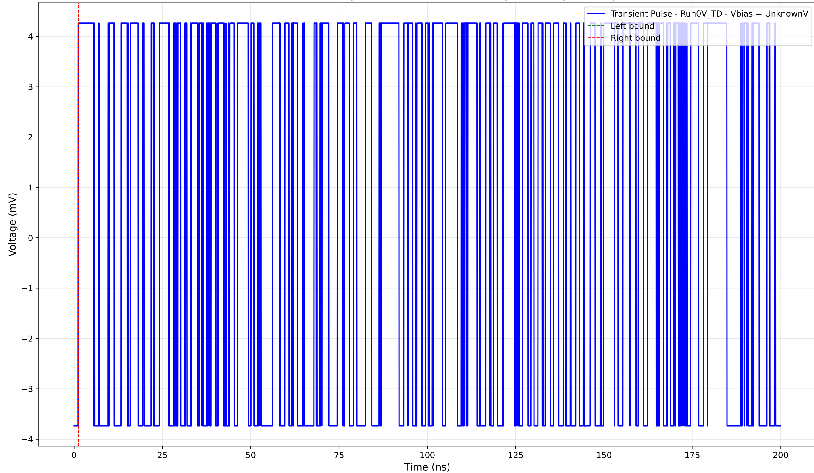
Transient Pulse - Sample: 4004 - Position: 880.0 \mu\text{m} - Charge: 0.00 pC
