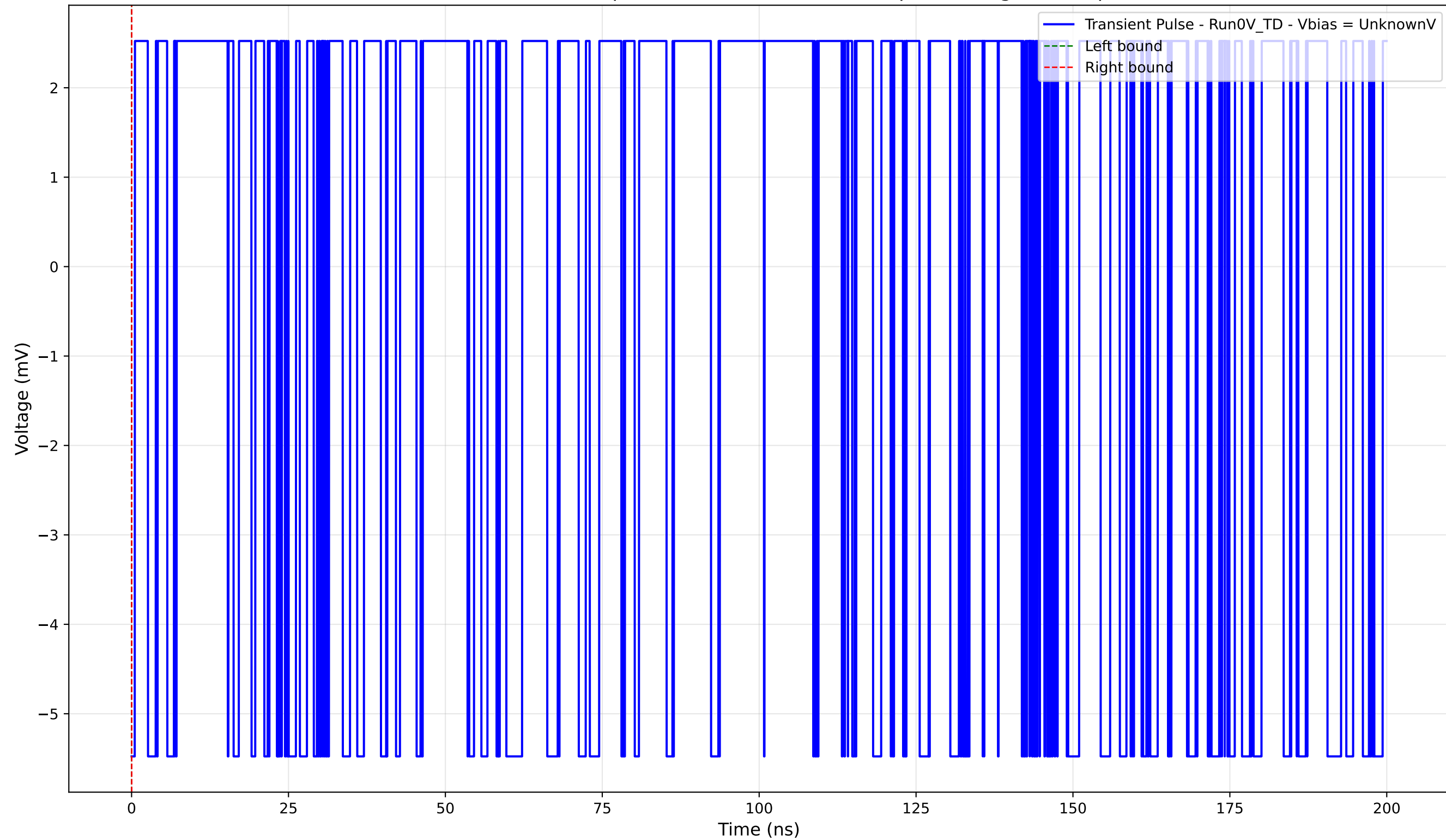
Transient Pulse - Sample: 4004 - Position: 1590.0 \mu\text{m} - Charge: -0.00 pC
