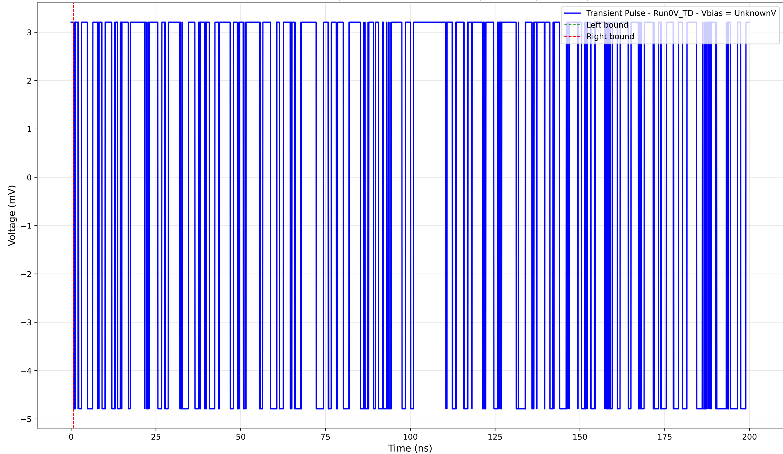
Transient Pulse - Sample: 4004 - Position: 30.0 \mu\text{m} - Charge: -0.00 pC
