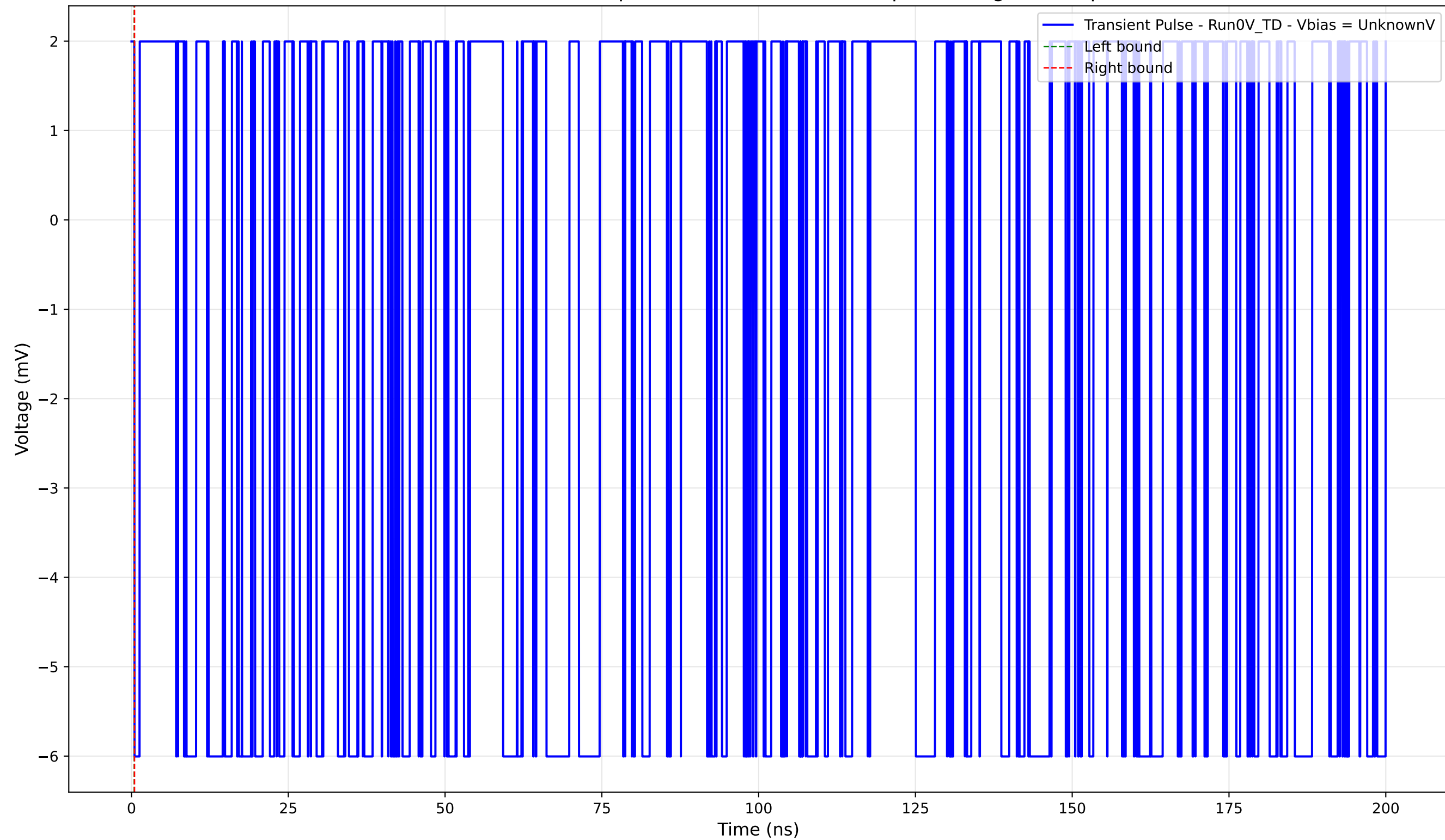
Transient Pulse - Sample: 4004 - Position: 280.0 \mu\text{m} - Charge: -0.00 pC
