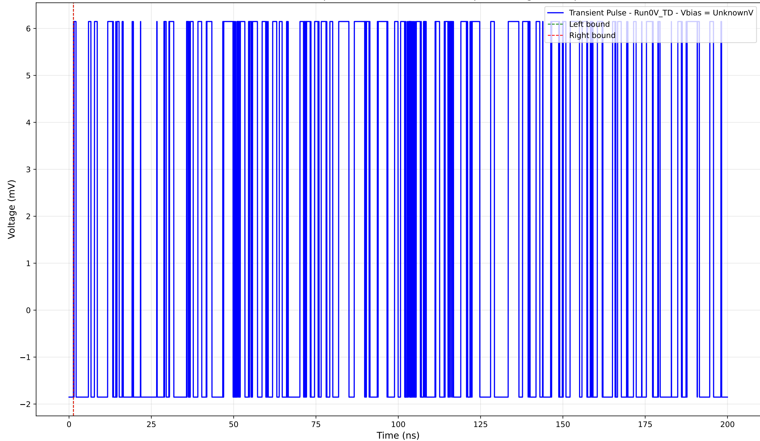
Transient Pulse - Sample: 4004 - Position: 1260.0 \mu\text{m} - Charge: 0.00 pC
