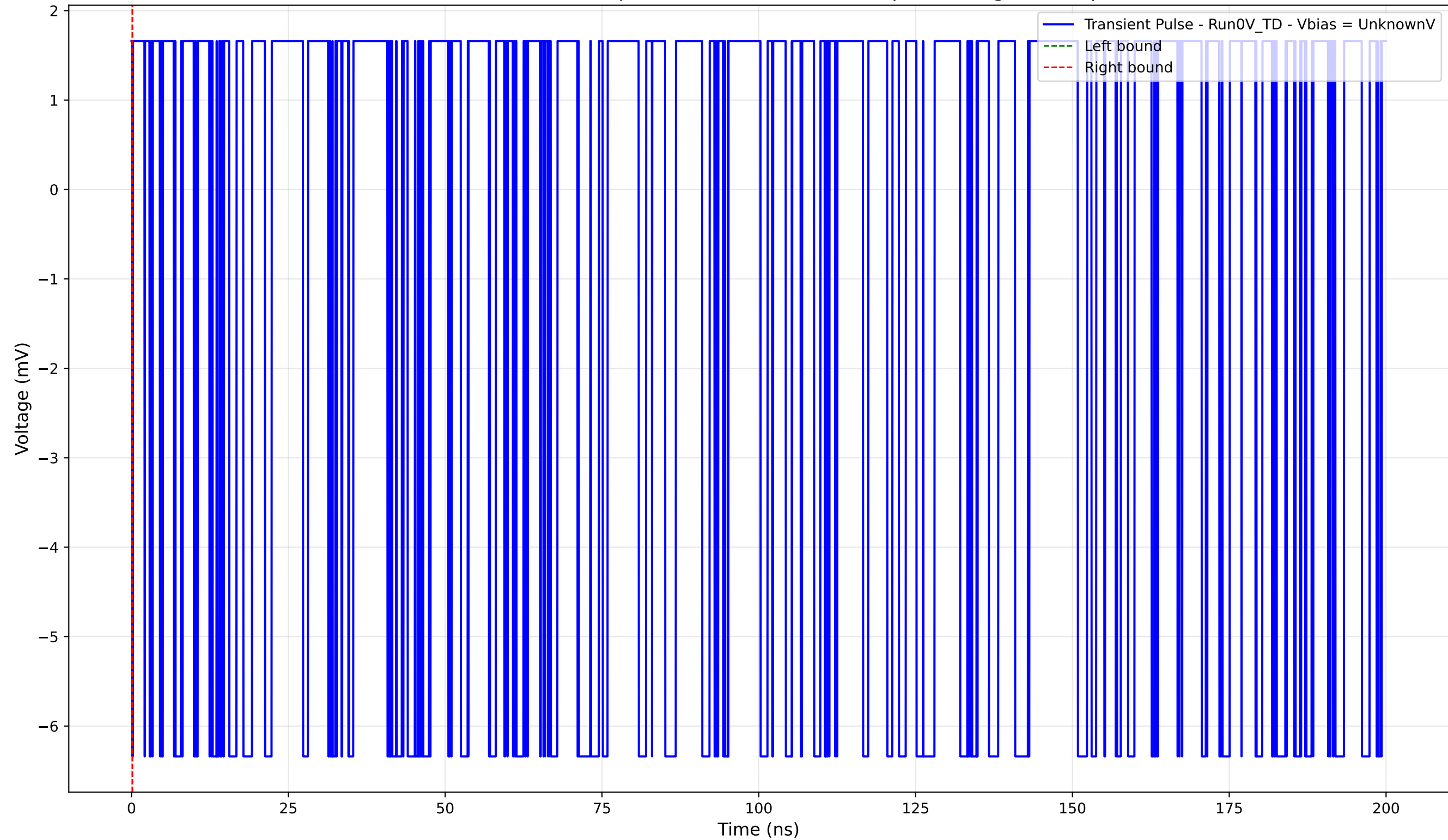
Transient Pulse - Sample: 4004 - Position: 910.0 \mu\text{m} - Charge: -0.00 pC
