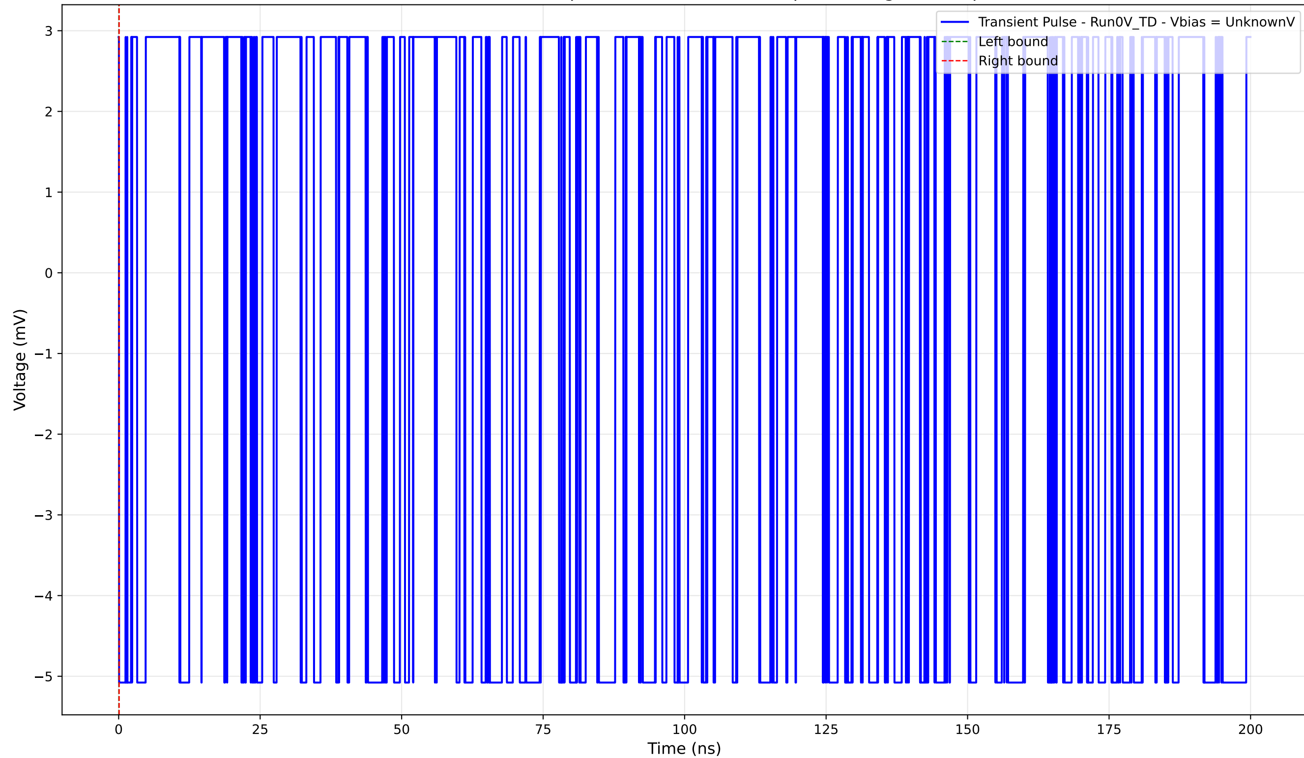
Transient Pulse - Sample: 4004 -Position: 0.0 \mu\text{m} - Charge: -0.00 pC
