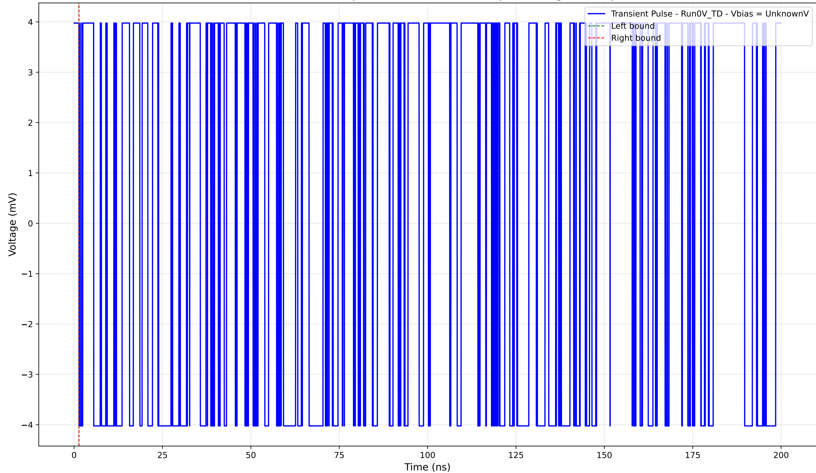
Transient Pulse - Sample: 4004 - Position: 90.0 \mu\text{m} - Charge: -0.00 pC
