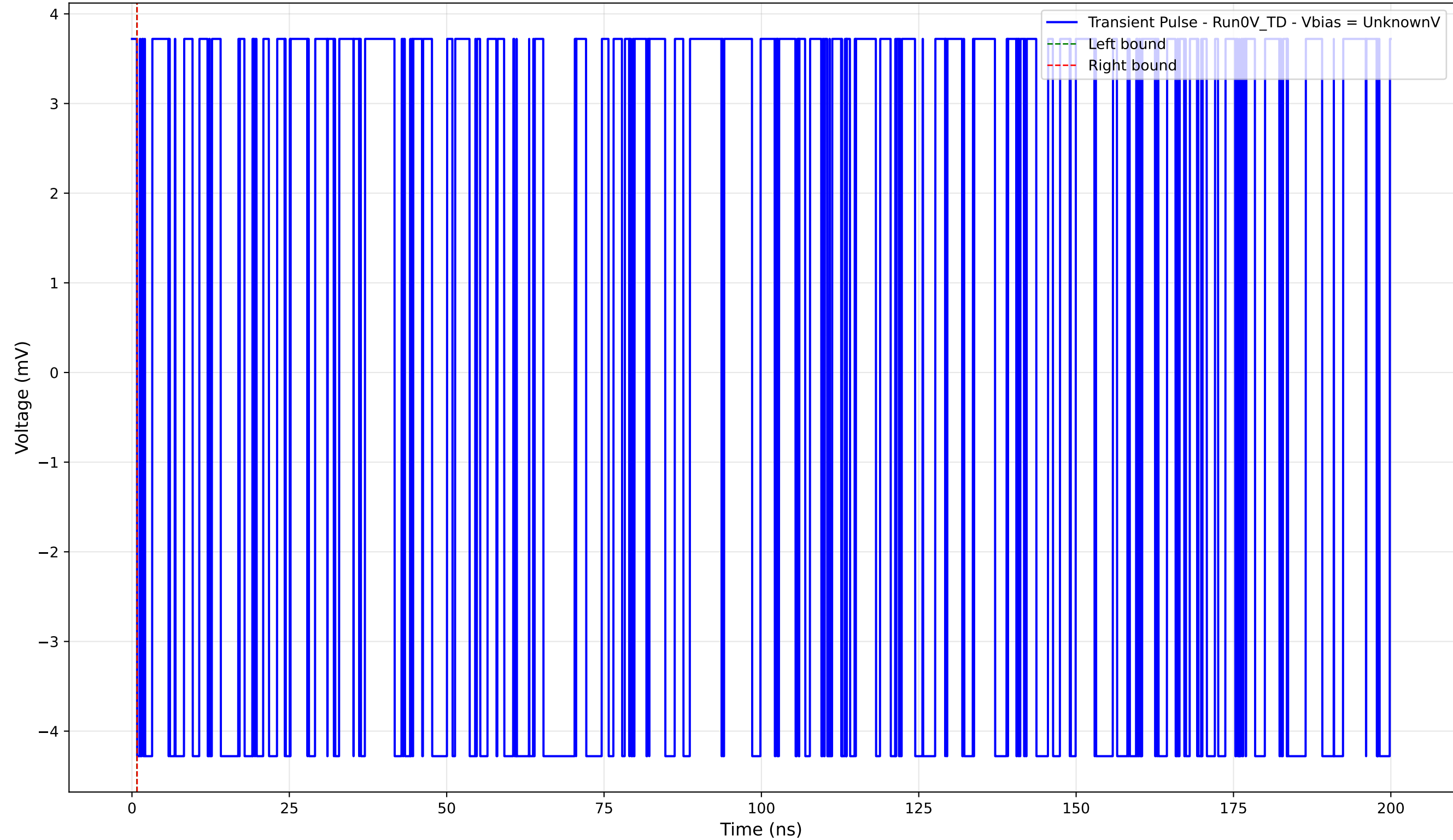
Transient Pulse - Sample: 4004 - Position: 1000.0 \mu\text{m} - Charge: -0.00 pC
