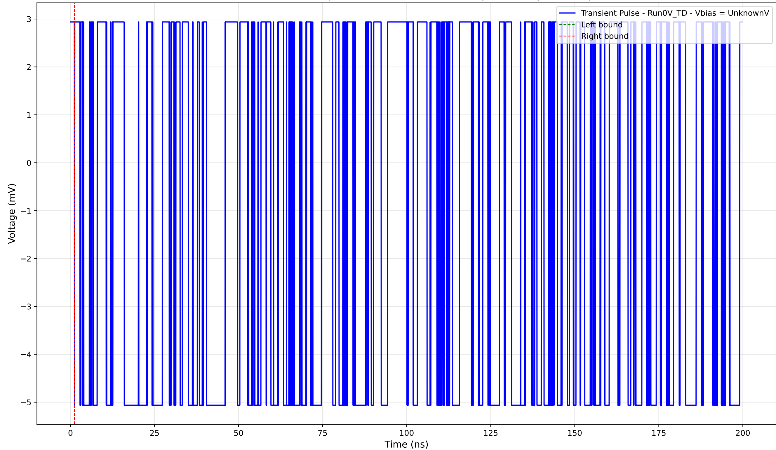
Transient Pulse - Sample: 4004 - Position: 1380.0 \mu\text{m} - Charge: -0.00 pC
