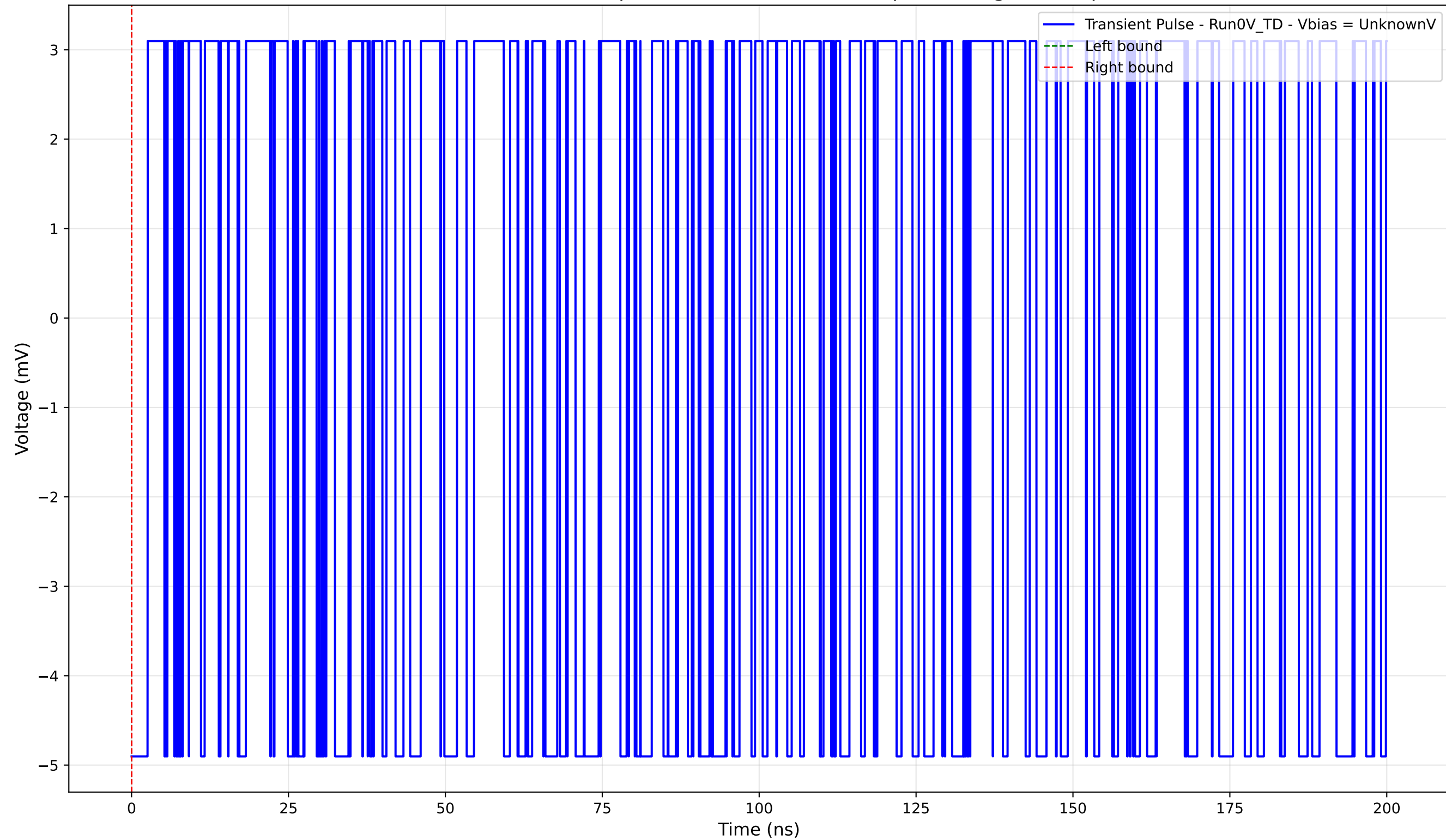
Transient Pulse - Sample: 4004 - Position: 930.0 \mu\text{m} - Charge: -0.00 pC
