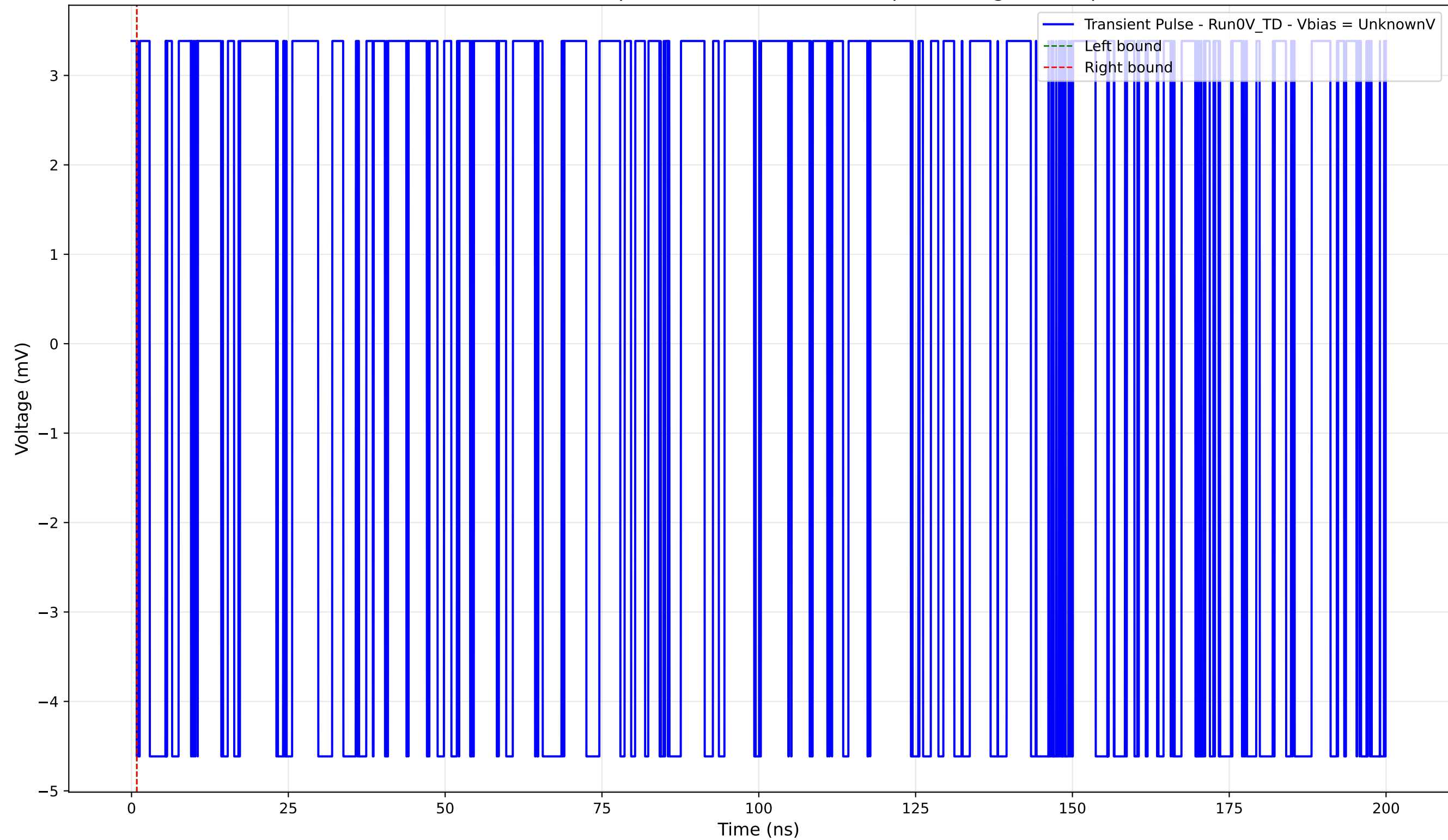
Transient Pulse - Sample: 4004 - Position: 340.0 \mu\text{m} - Charge: -0.00 pC
