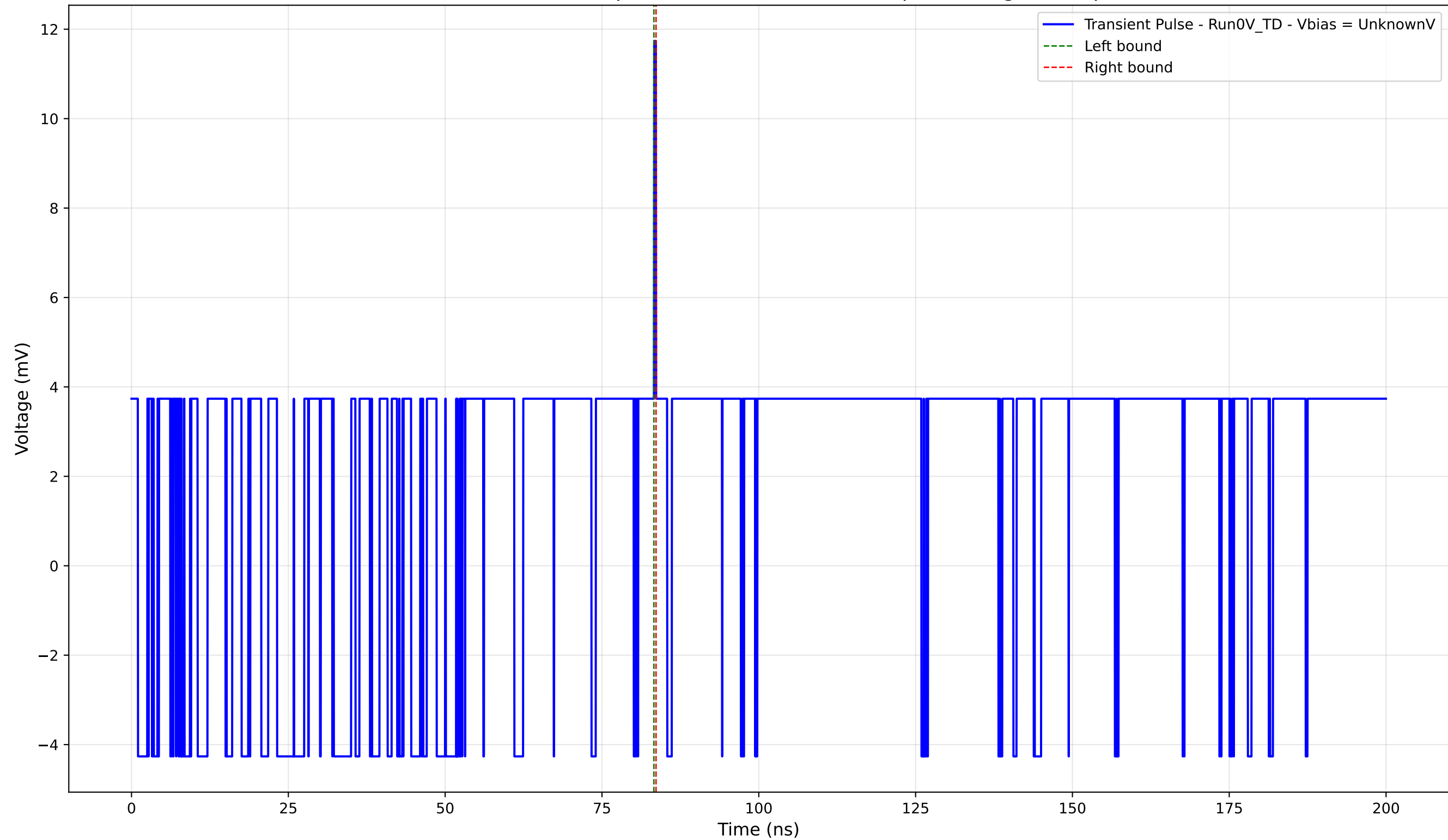
Transient Pulse - Sample: 4004 - Position: 1870.0 \mu\text{m} - Charge: 0.08 pC
