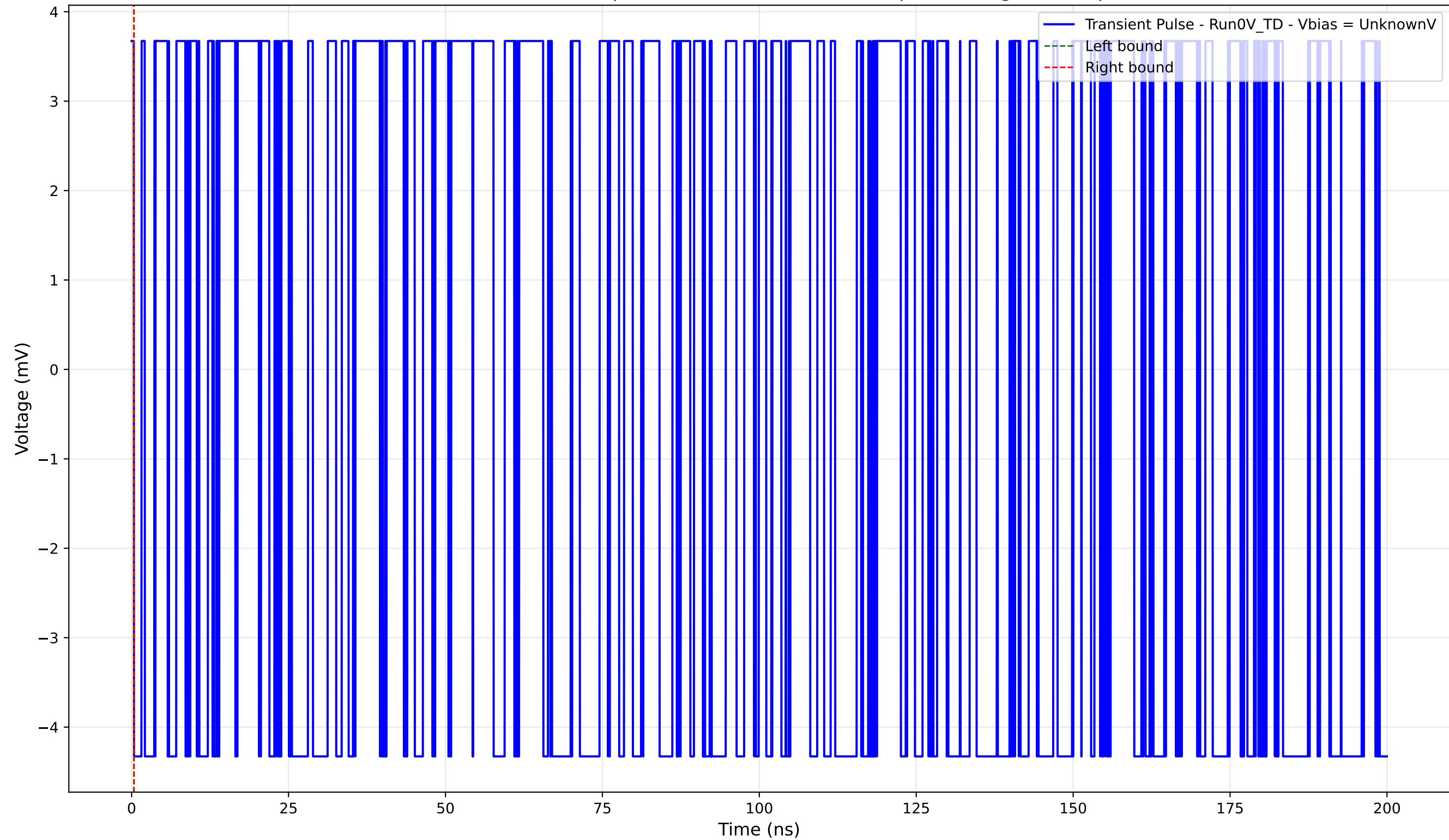
Transient Pulse - Sample: 4004 - Position: 1210.0 \mu\text{m} - Charge: -0.00 pC
