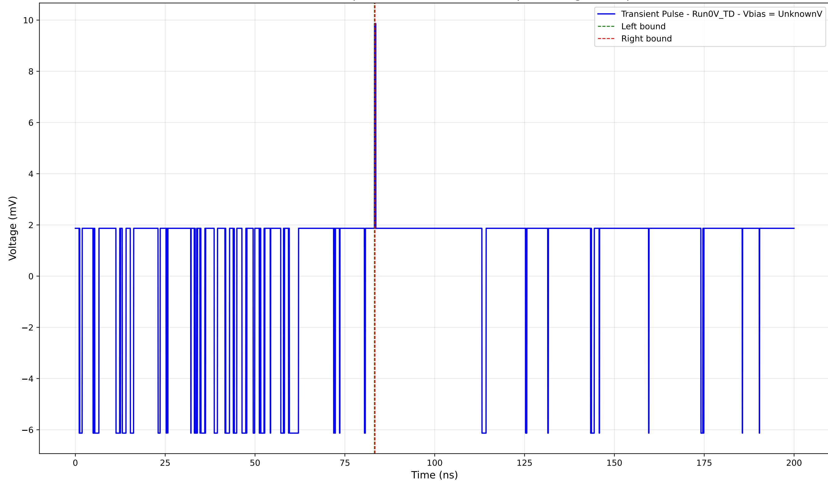
Transient Pulse - Sample: 4004 - Position: 1980.0 \mu\text{m} - Charge: 0.03 pC
