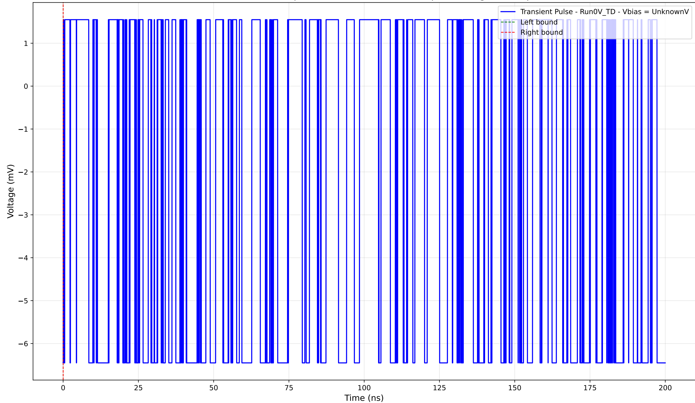
Transient Pulse - Sample: 4004 - Position: 1090.0 \mu\text{m} - Charge: -0.00 pC
