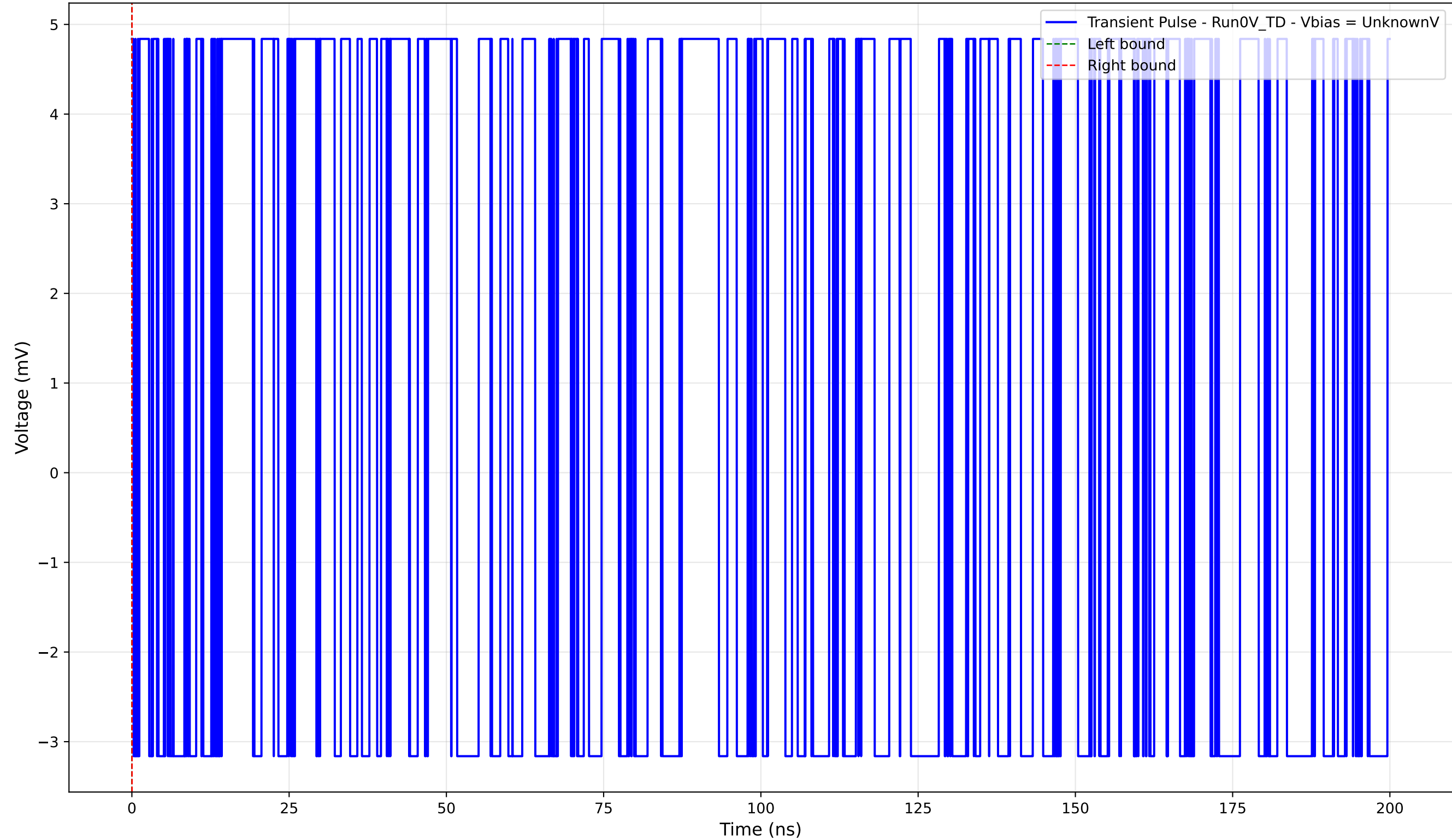
Transient Pulse - Sample: 4004 - Position: 1070.0 \mu\text{m} - Charge: 0.00 pC
