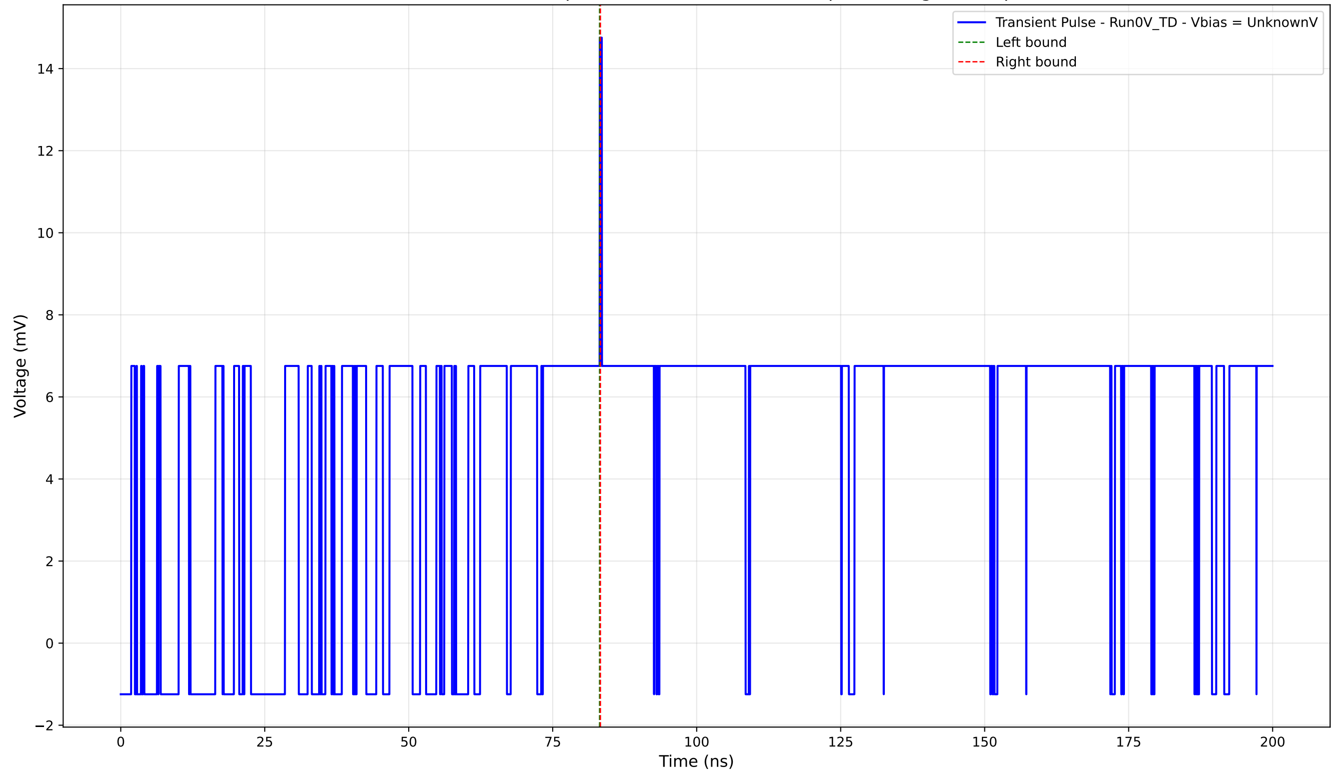
Transient Pulse - Sample: 4004 - Position: 1940.0 \mu\text{m} - Charge: 0.04 pC
