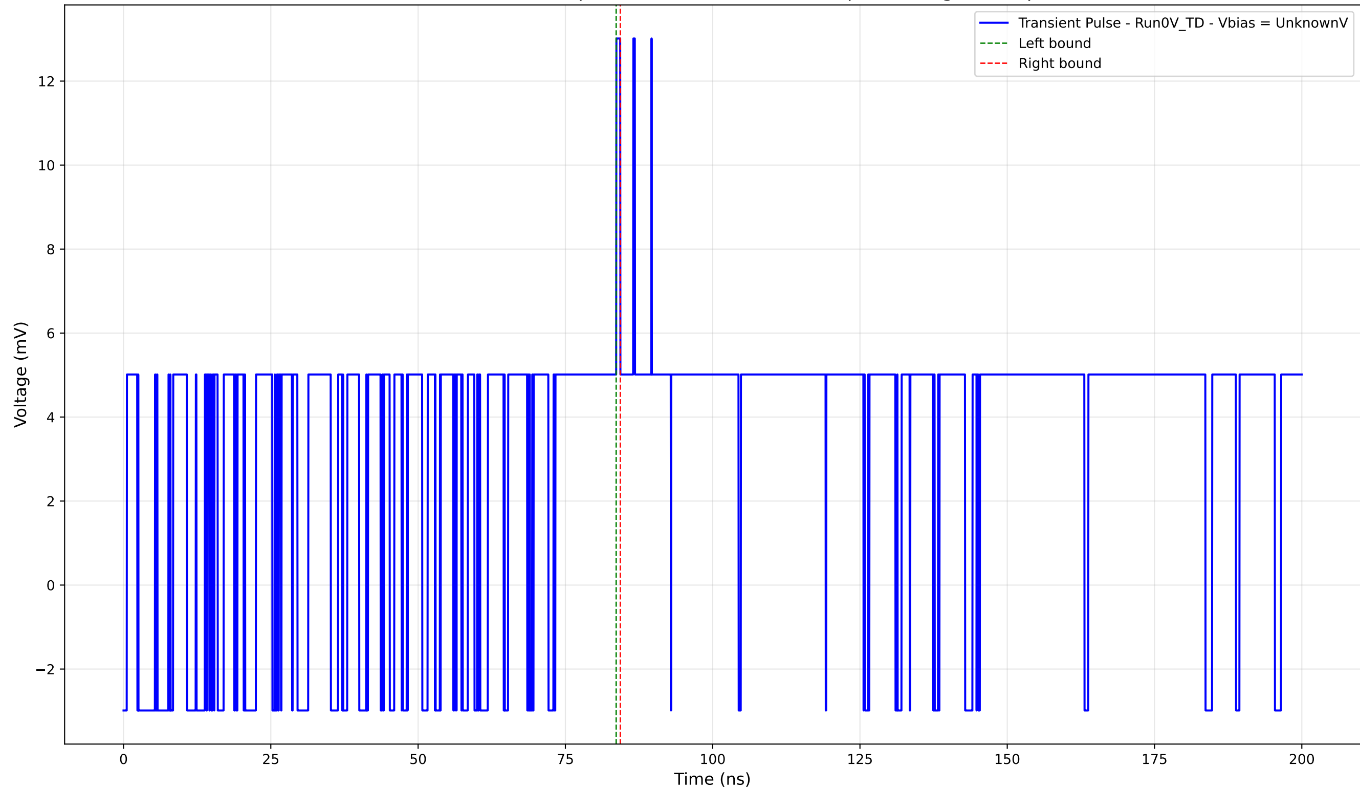
Transient Pulse - Sample: 4004 - Position: 1900.0 \mu\text{m} - Charge: 0.18 pC
