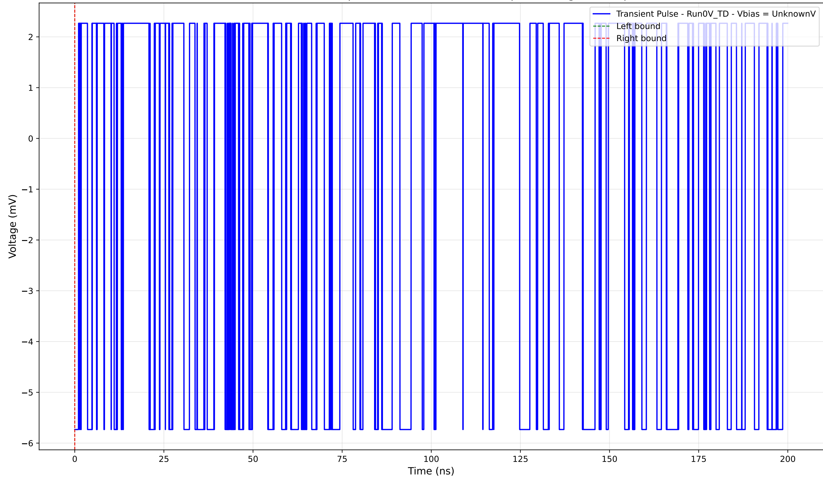
Transient Pulse - Sample: 4004 - Position: 1630.0 \mu\text{m} - Charge: -0.00 pC
