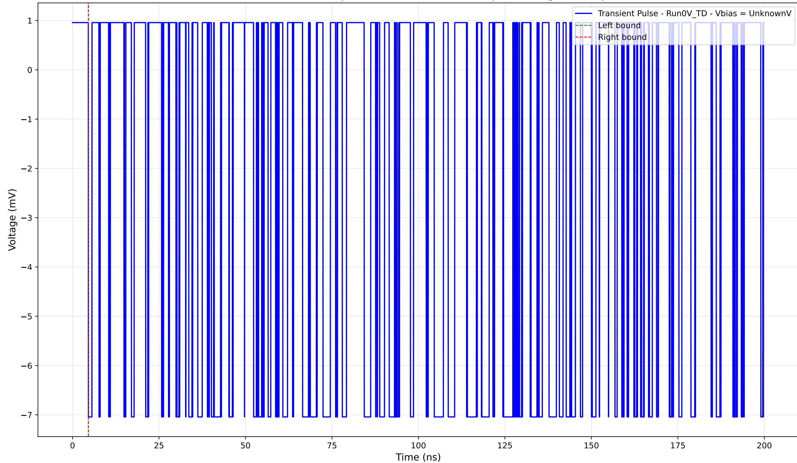
Transient Pulse - Sample: 4004 - Position: 190.0 \mu\text{m} - Charge: -0.00 pC
