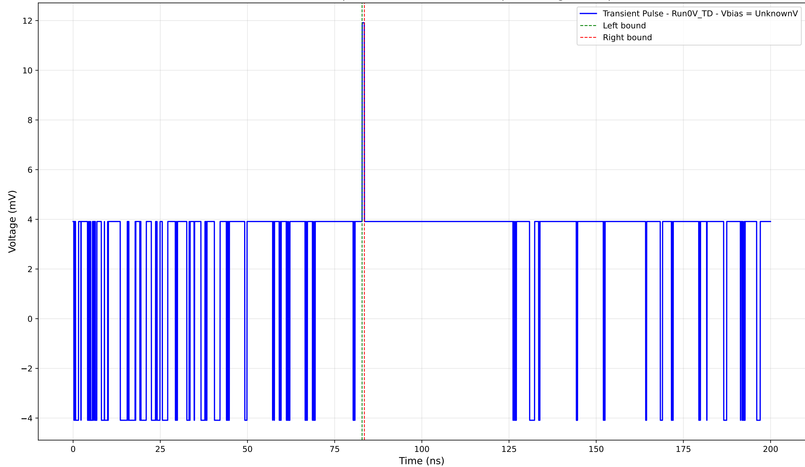
Transient Pulse - Sample: 4004 - Position: 1710.0 \mu\text{m} - Charge: 0.15 pC
