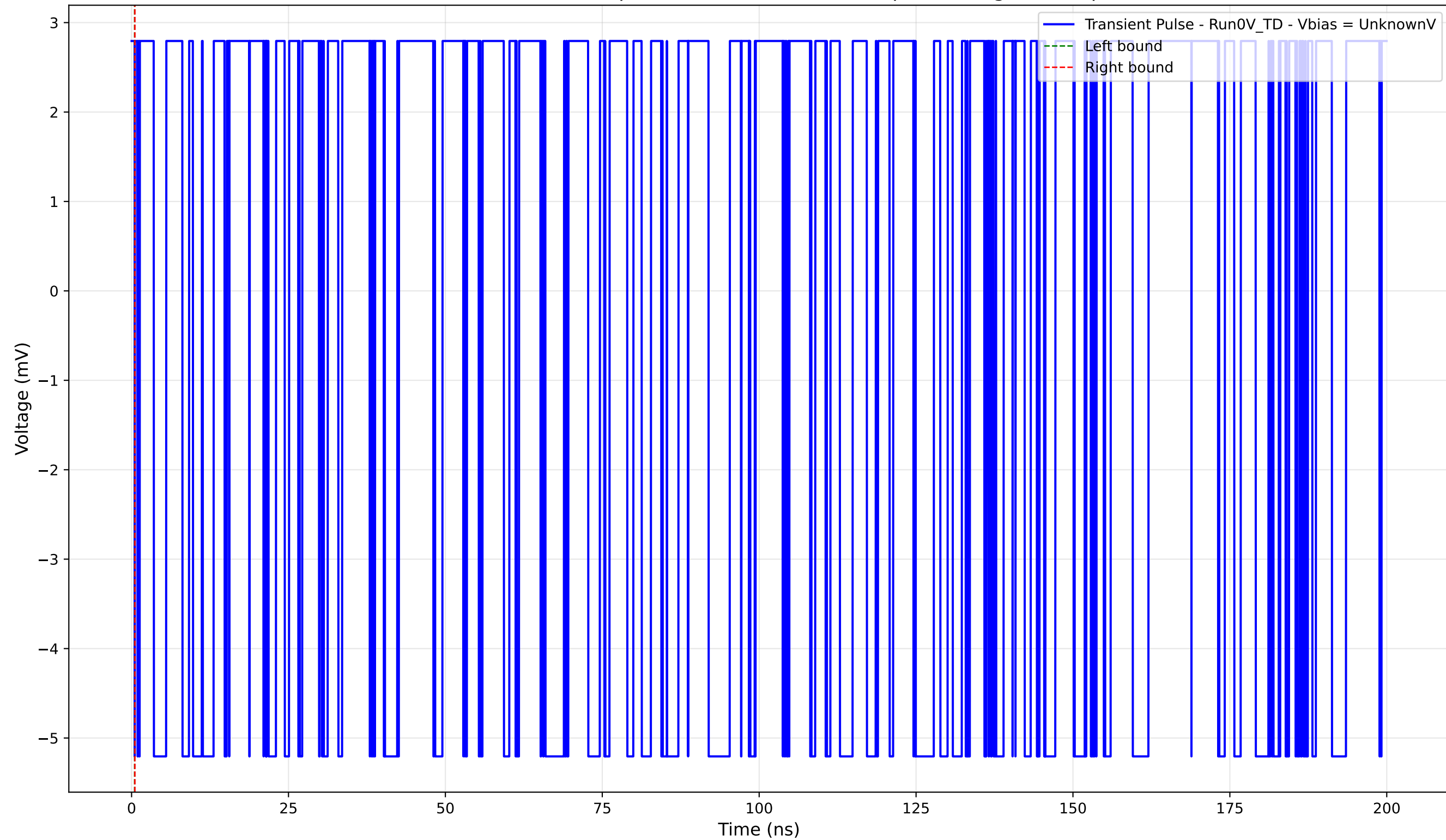
Transient Pulse - Sample: 4004 - Position: 540.0 \mu\text{m} - Charge: -0.00 pC
