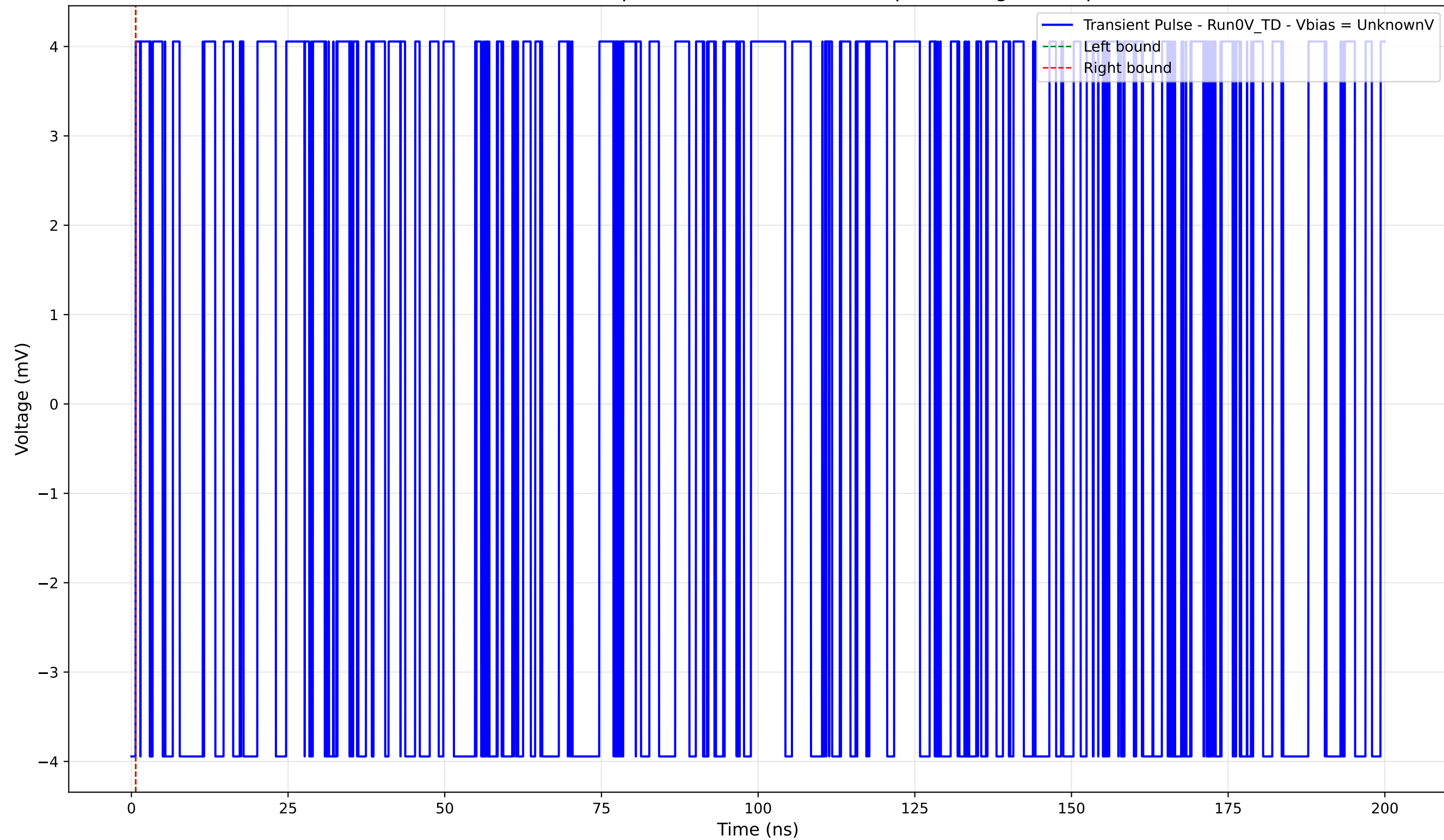
Transient Pulse - Sample: 4004 - Position: 460.0 \mu\text{m} - Charge: 0.00 pC
