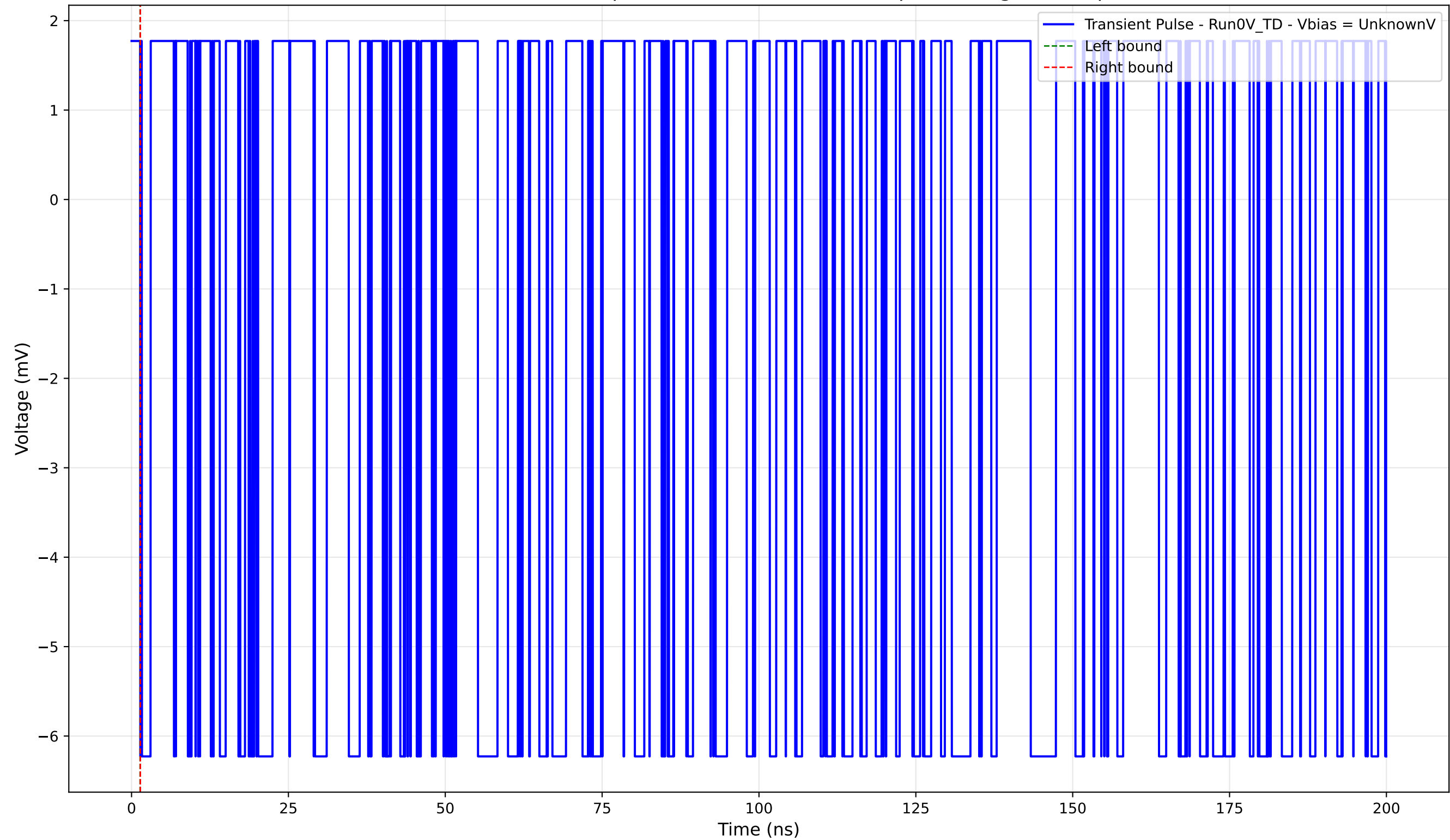
Transient Pulse - Sample: 4004 - Position: 1050.0 \mu\text{m} - Charge: -0.00 pC
