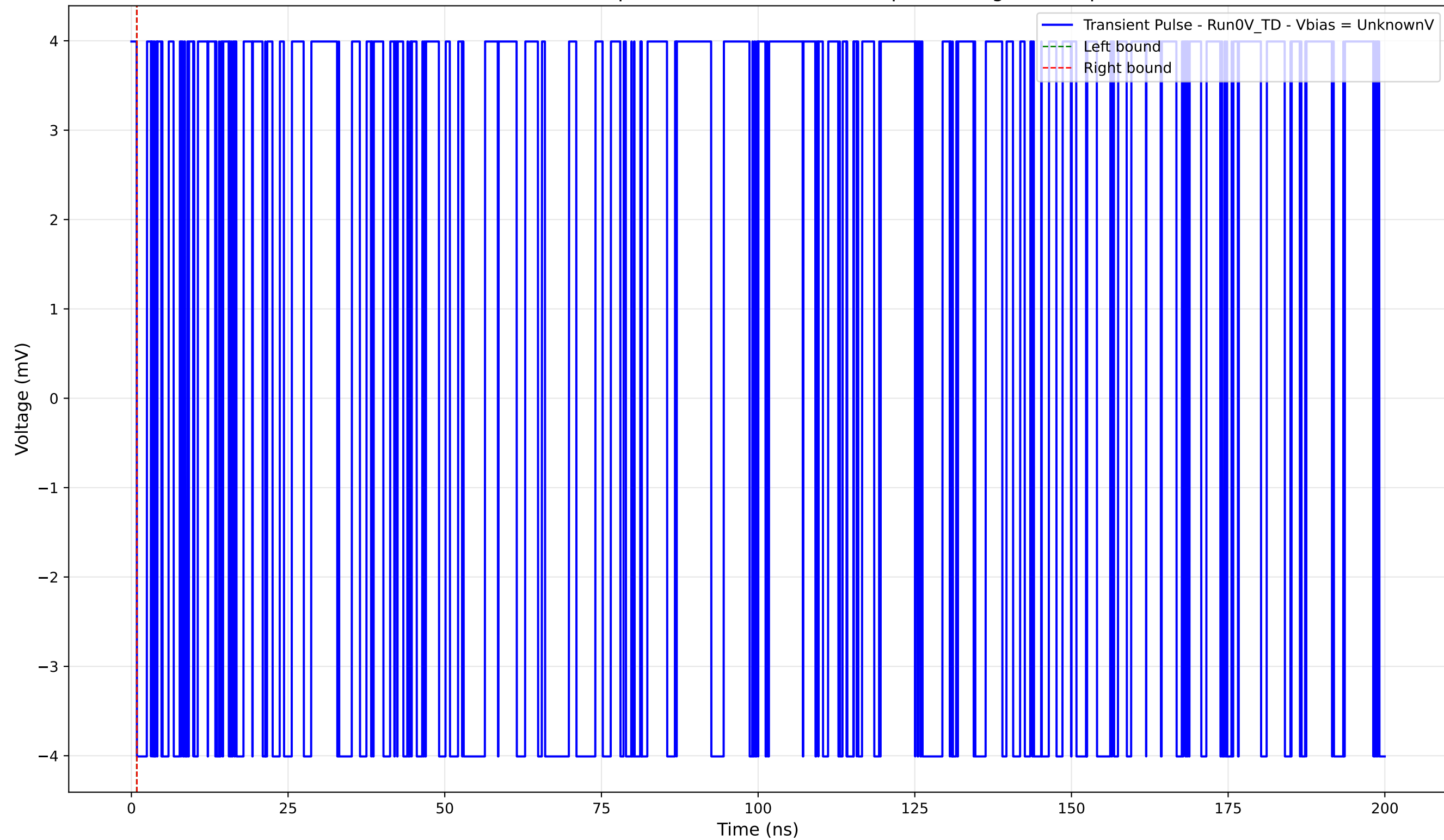
Transient Pulse - Sample: 4004 - Position: 230.0 \mu\text{m} - Charge: -0.00 pC
