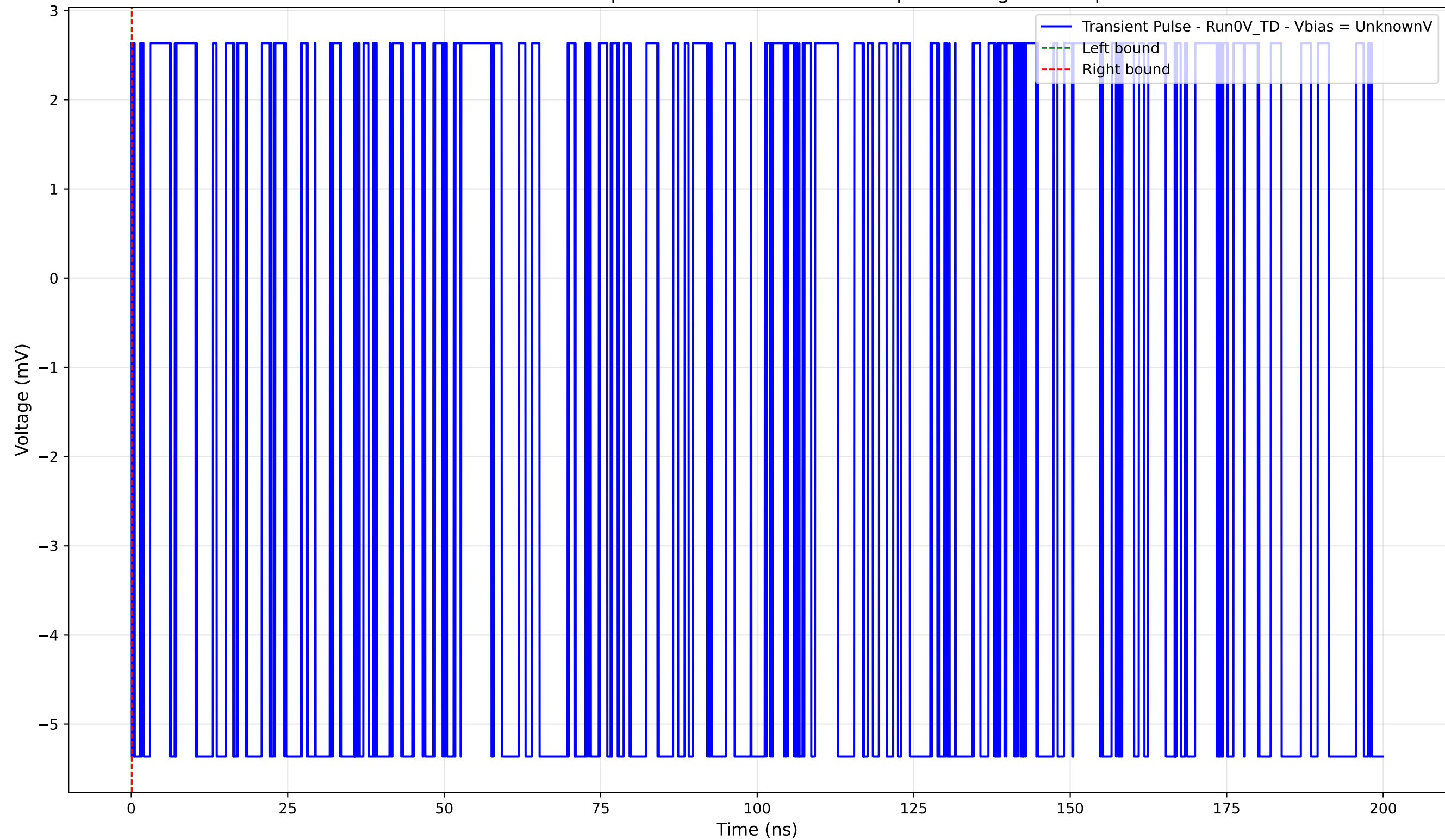
Transient Pulse - Sample: 4004 - Position: 1420.0 \mu\text{m} - Charge: -0.00 pC
