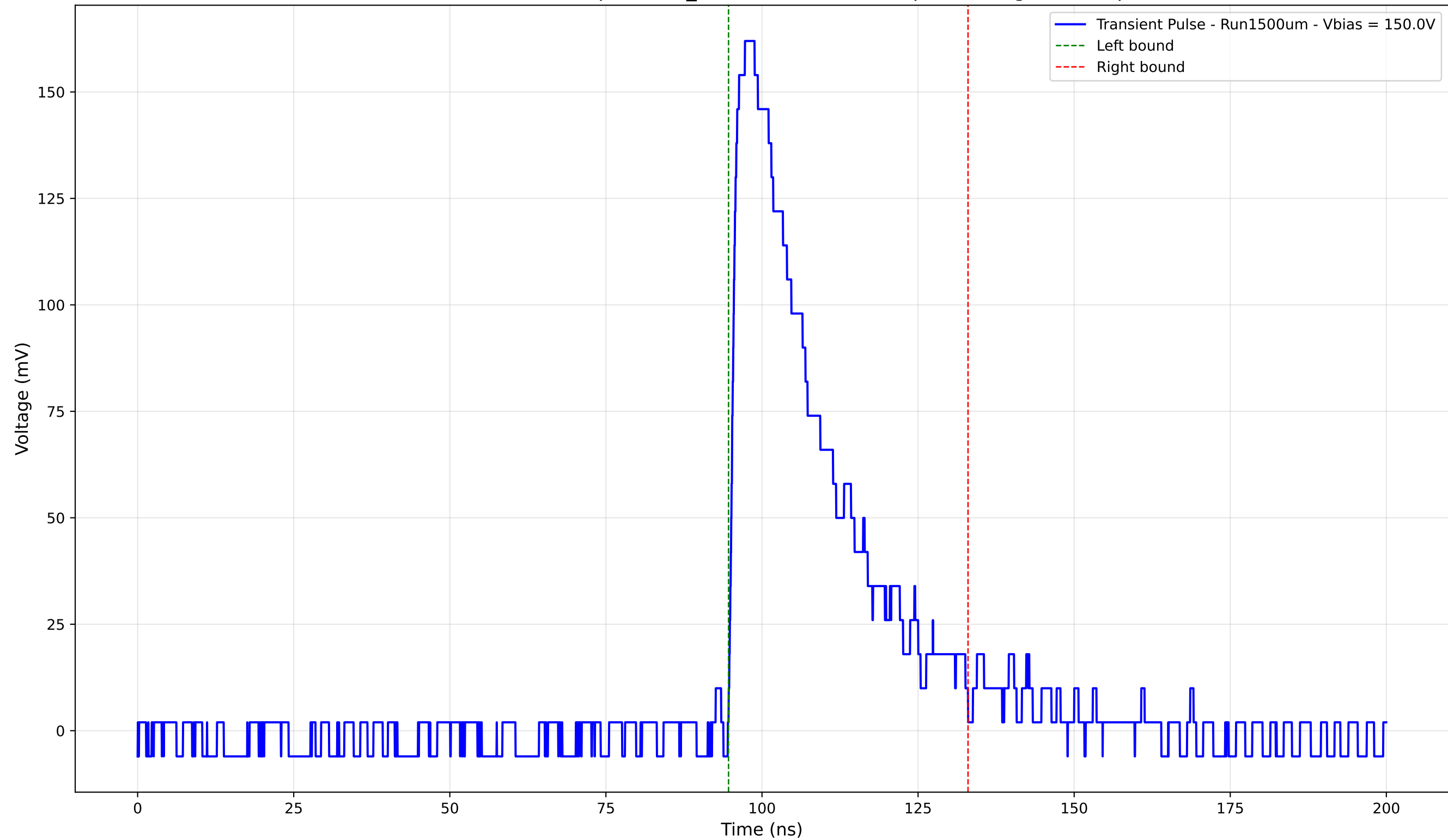
Transient Pulse - Sample: 1cm_42 - Position: 1565.0 \mu\text{m} - Charge: 49.82 pC
