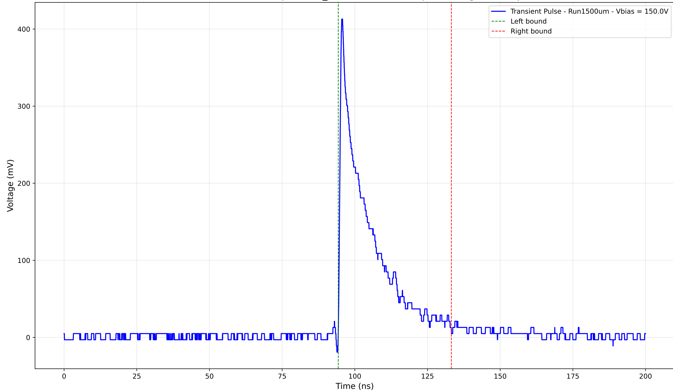
Transient Pulse - Sample: 1cm_42 - Position: 135.0 \mu\text{m} - Charge: 81.41 pC
