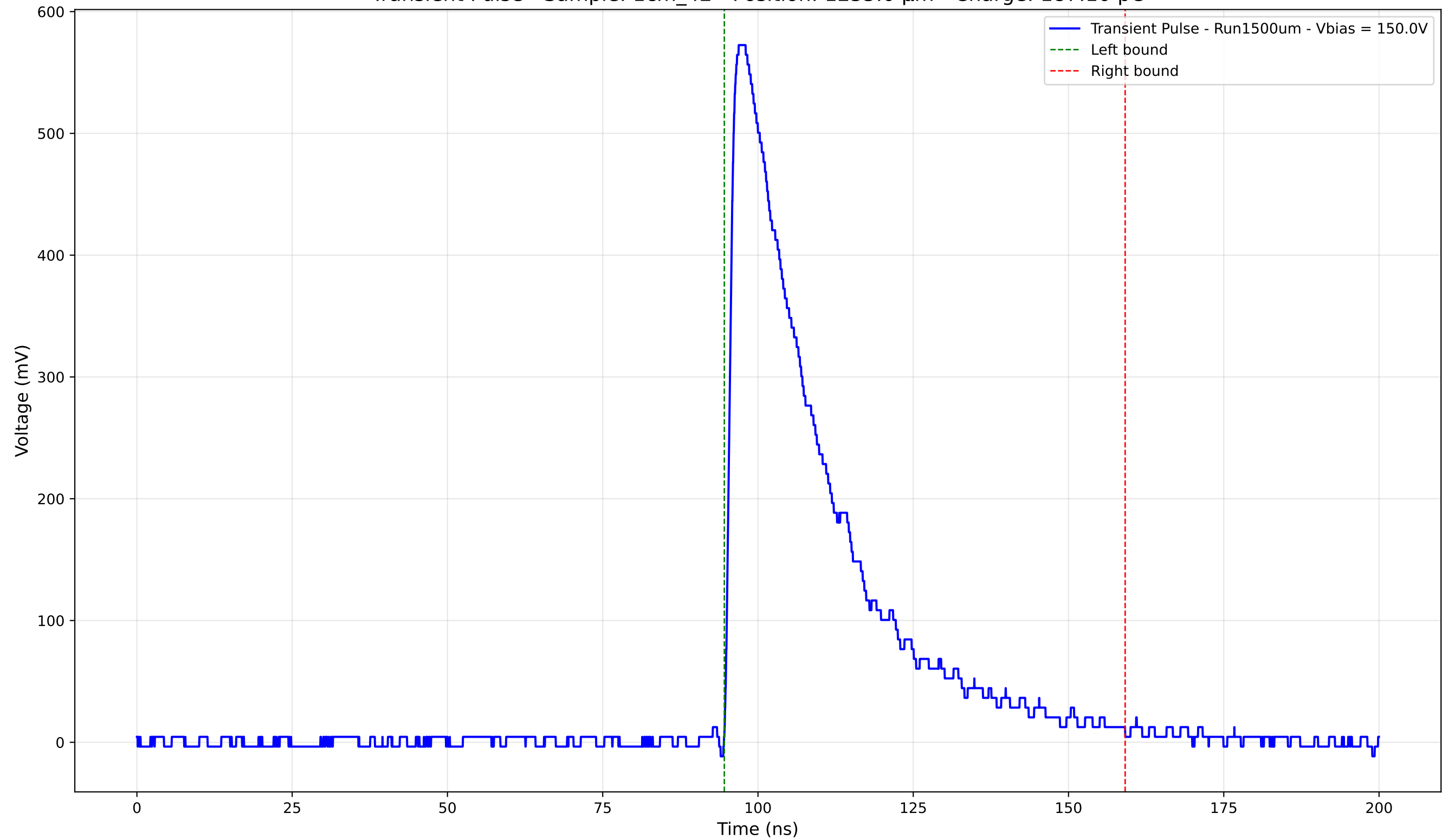
Transient Pulse - Sample: 1cm_42 - Position: 1255.0 \mu\text{m} - Charge: 187.10 pC
