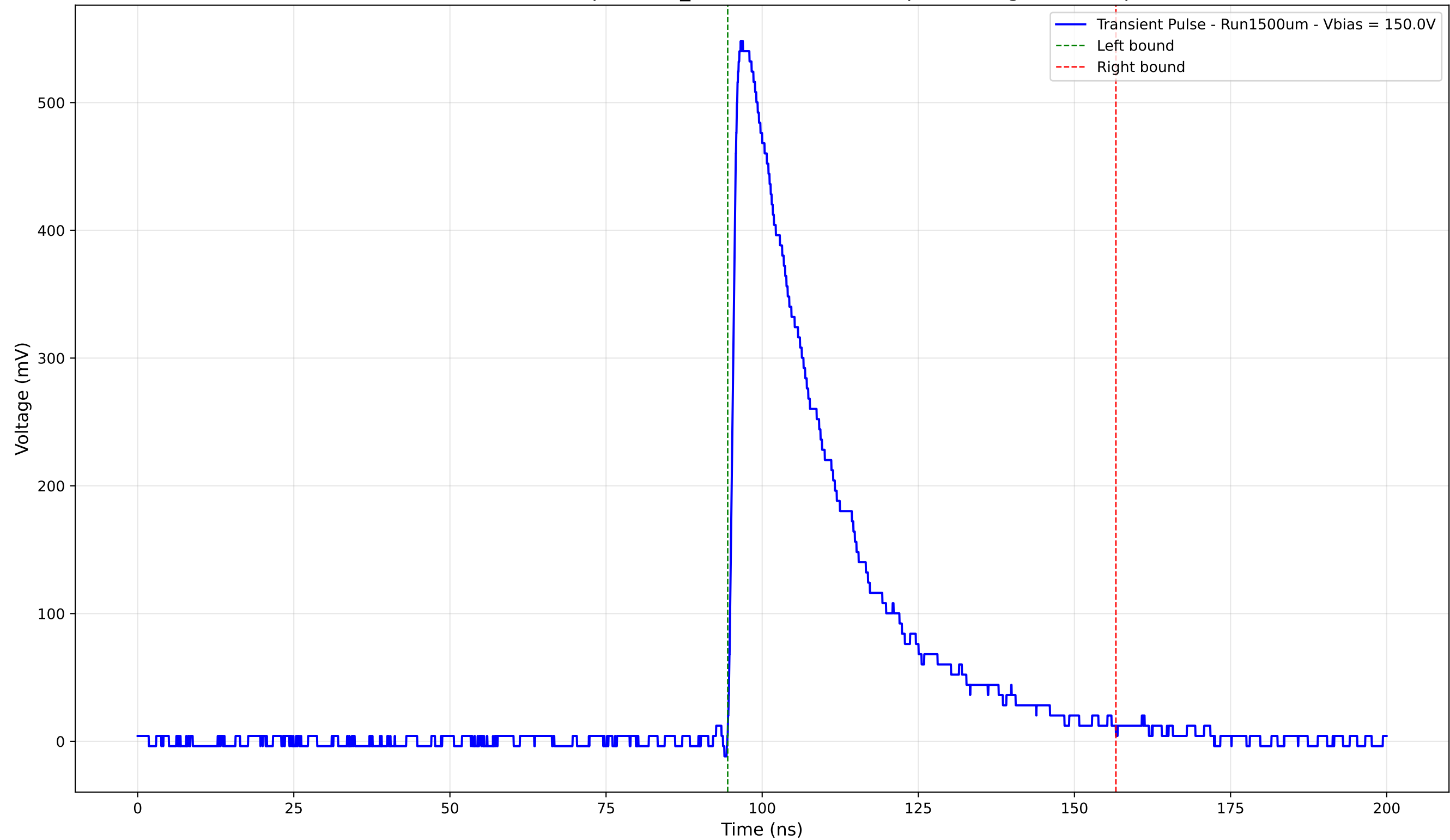
Transient Pulse - Sample: 1cm_42 - Position: 3695.0 \mu\text{m} - Charge: 180.05 pC
