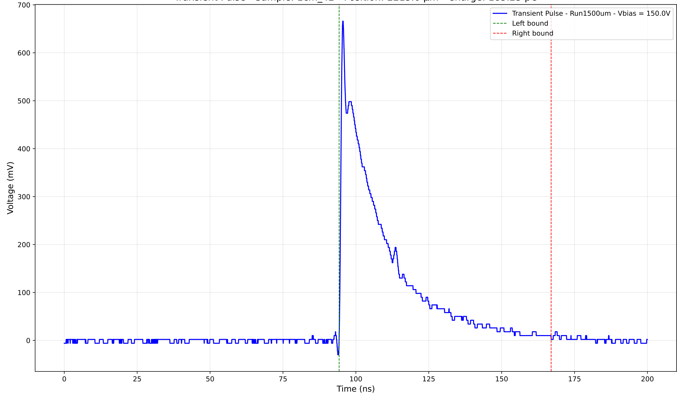
Transient Pulse - Sample: 1cm_42 - Position: 2215.0 \mu\text{m} - Charge: 183.23 pC
