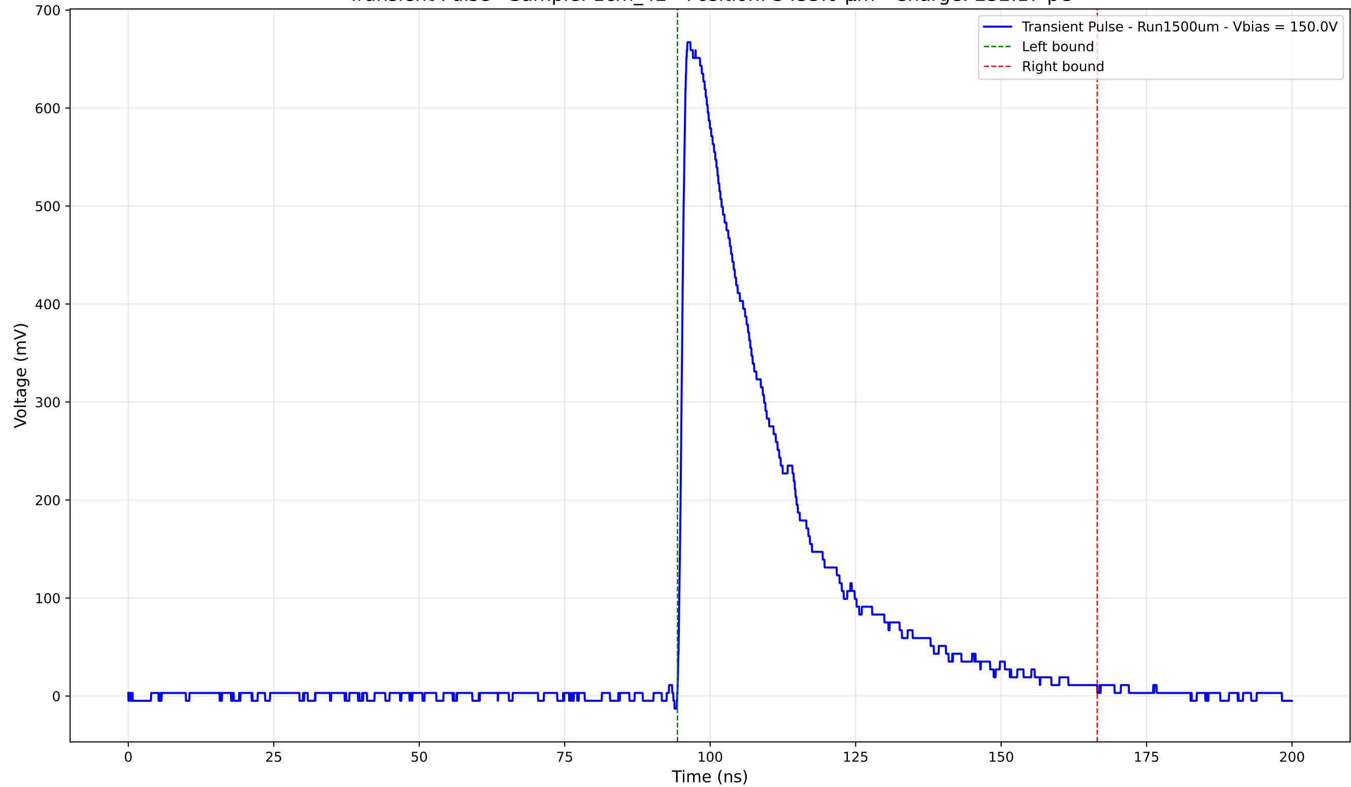
Transient Pulse - Sample: 1cm_42 - Position: 3455.0 \mu\text{m} - Charge: 232.17 pC
