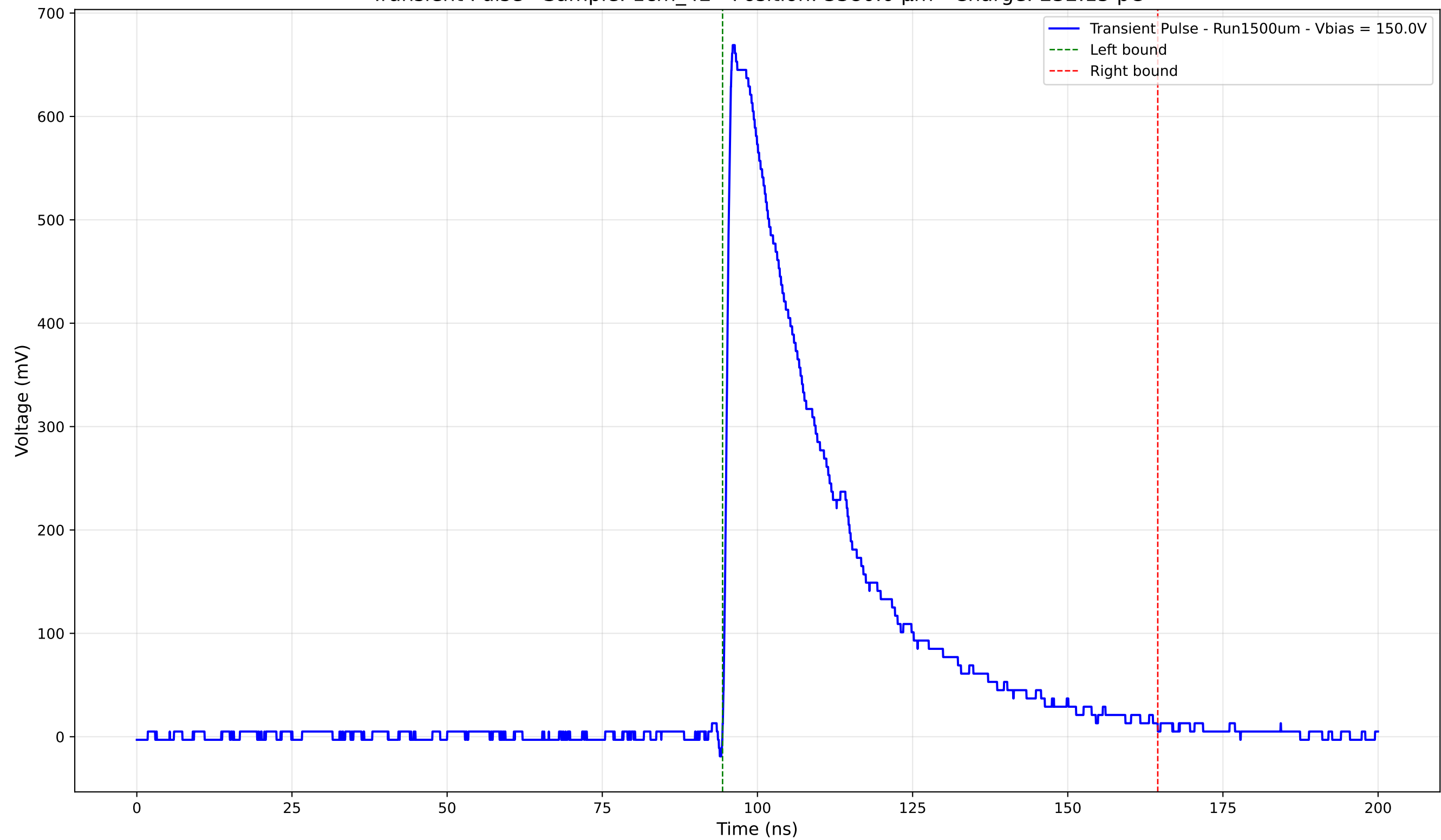
Transient Pulse - Sample: 1cm_42 - Position: 3380.0 \mu\text{m} - Charge: 232.15 pC
