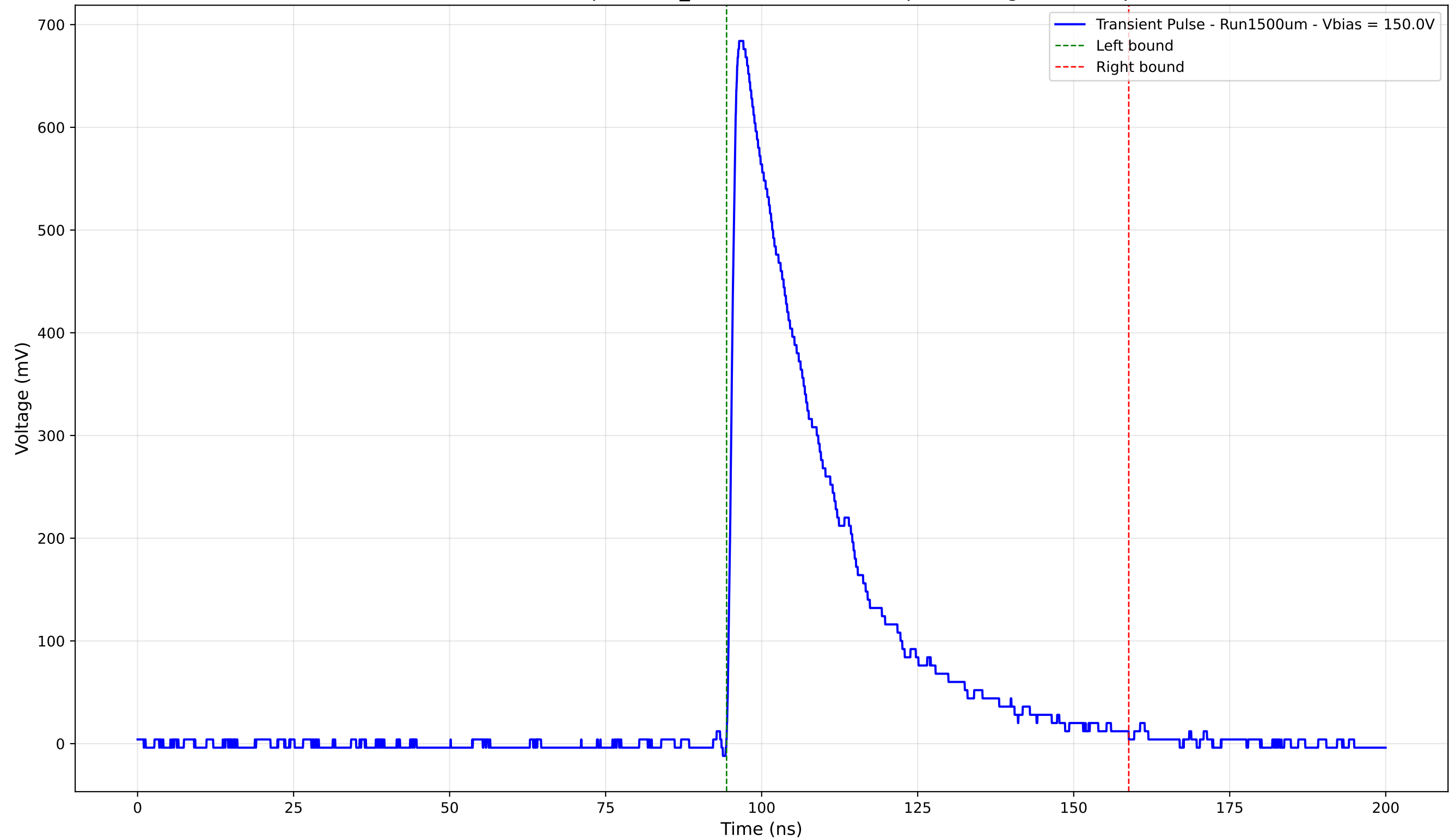
Transient Pulse - Sample: 1cm_42 - Position: 4225.0 \mu\text{m} - Charge: 214.71 pC
