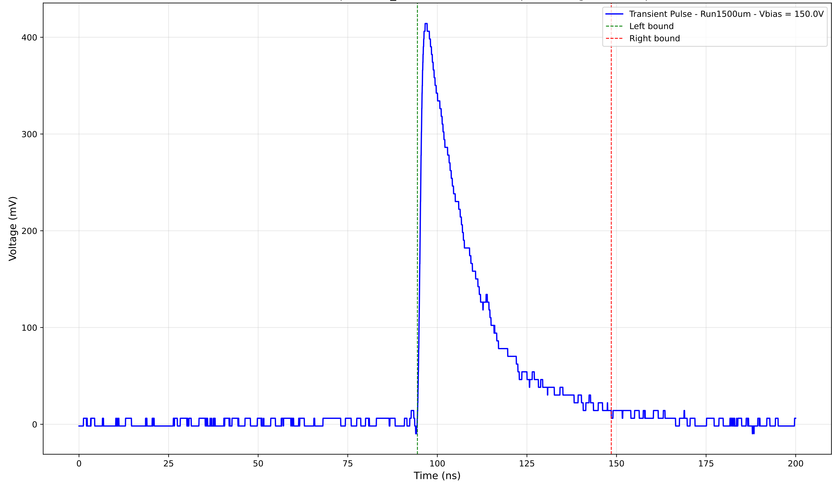
Transient Pulse - Sample: 1cm_42 - Position: 4175.0 \mu\text{m} - Charge: 127.43 pC
