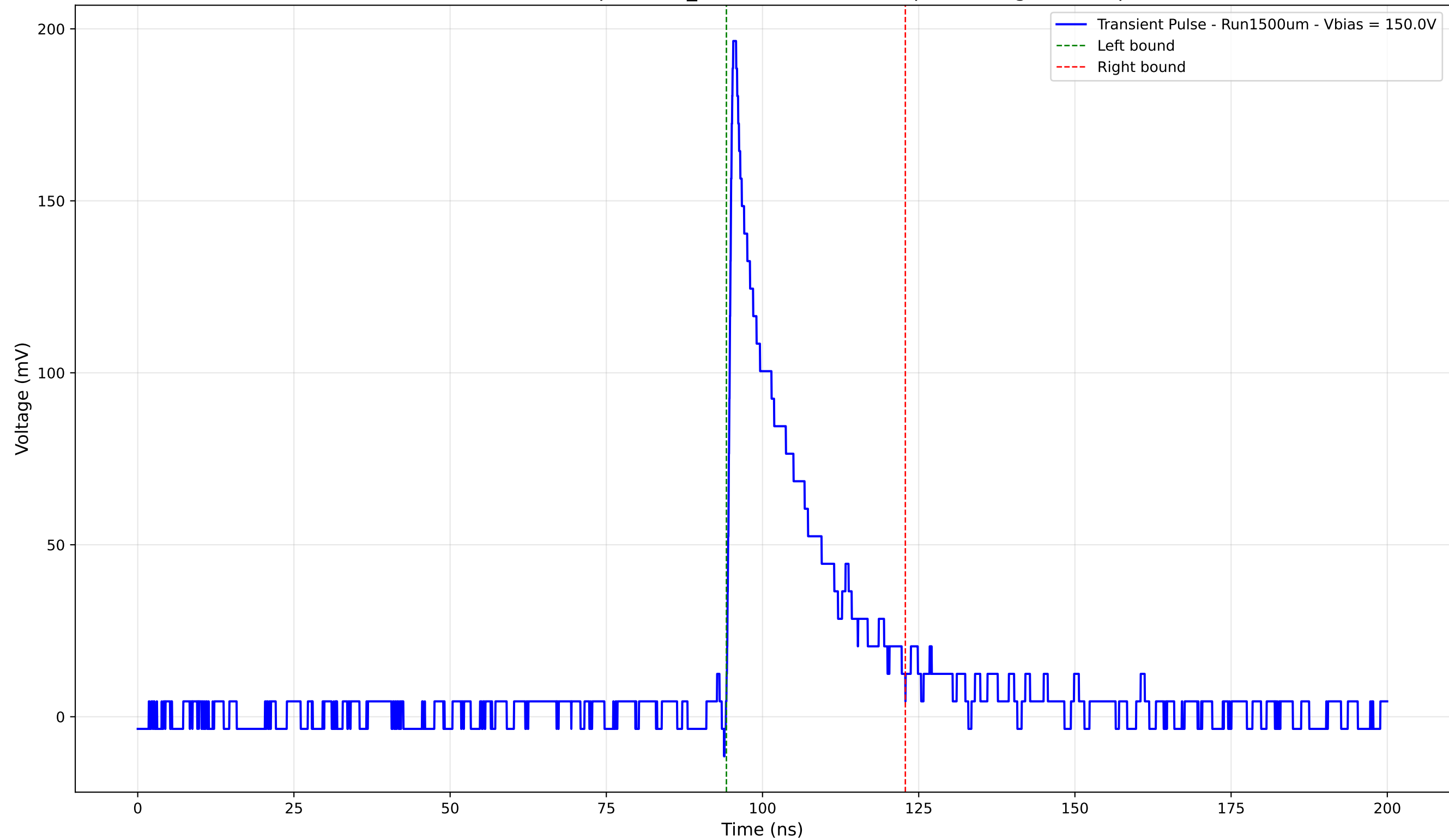
Transient Pulse - Sample: 1cm_42 - Position: 4930.0 \mu\text{m} - Charge: 37.20 pC
