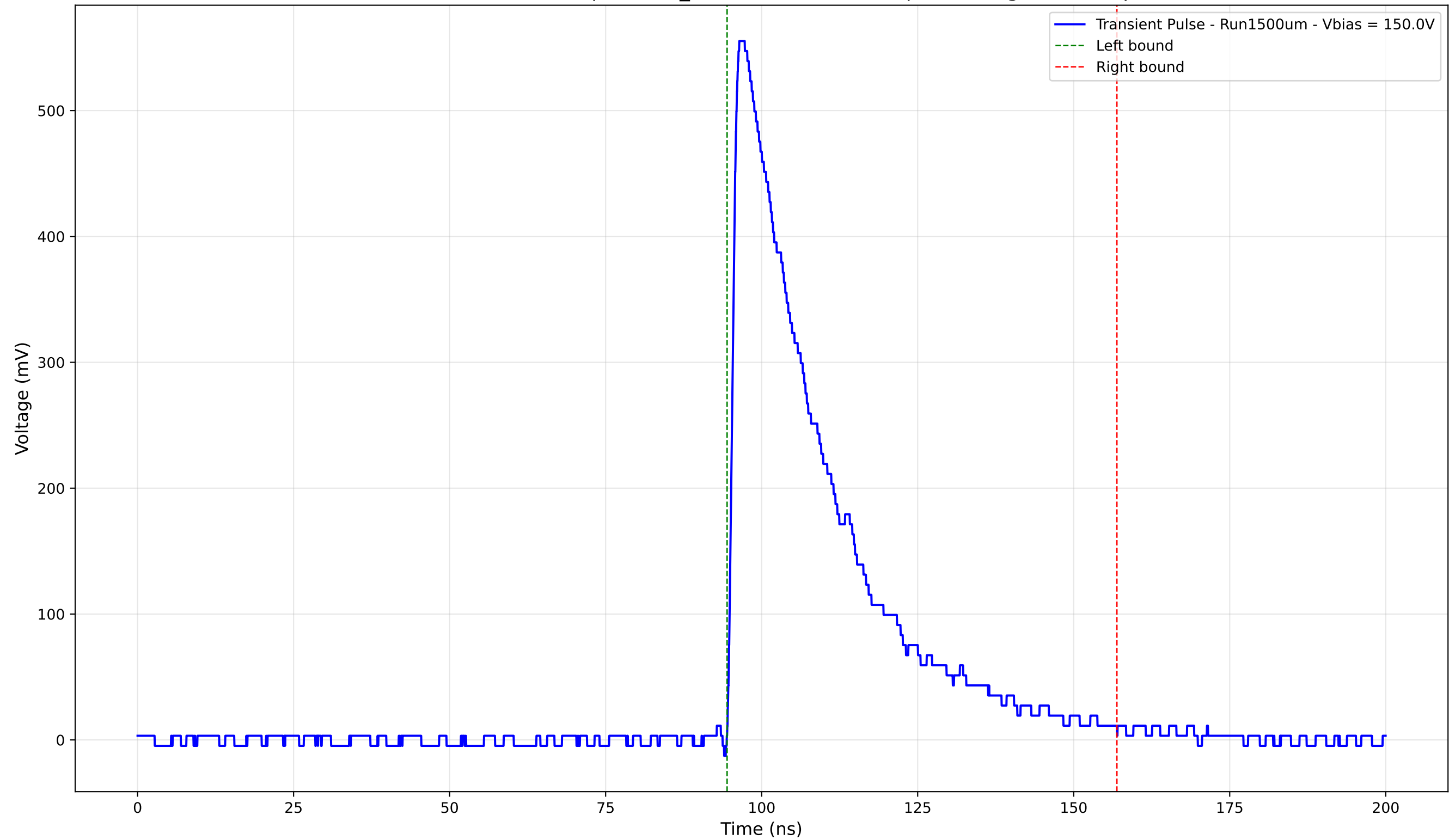
Transient Pulse - Sample: 1cm_42 - Position: 4050.0 \mu\text{m} - Charge: 175.91 pC
