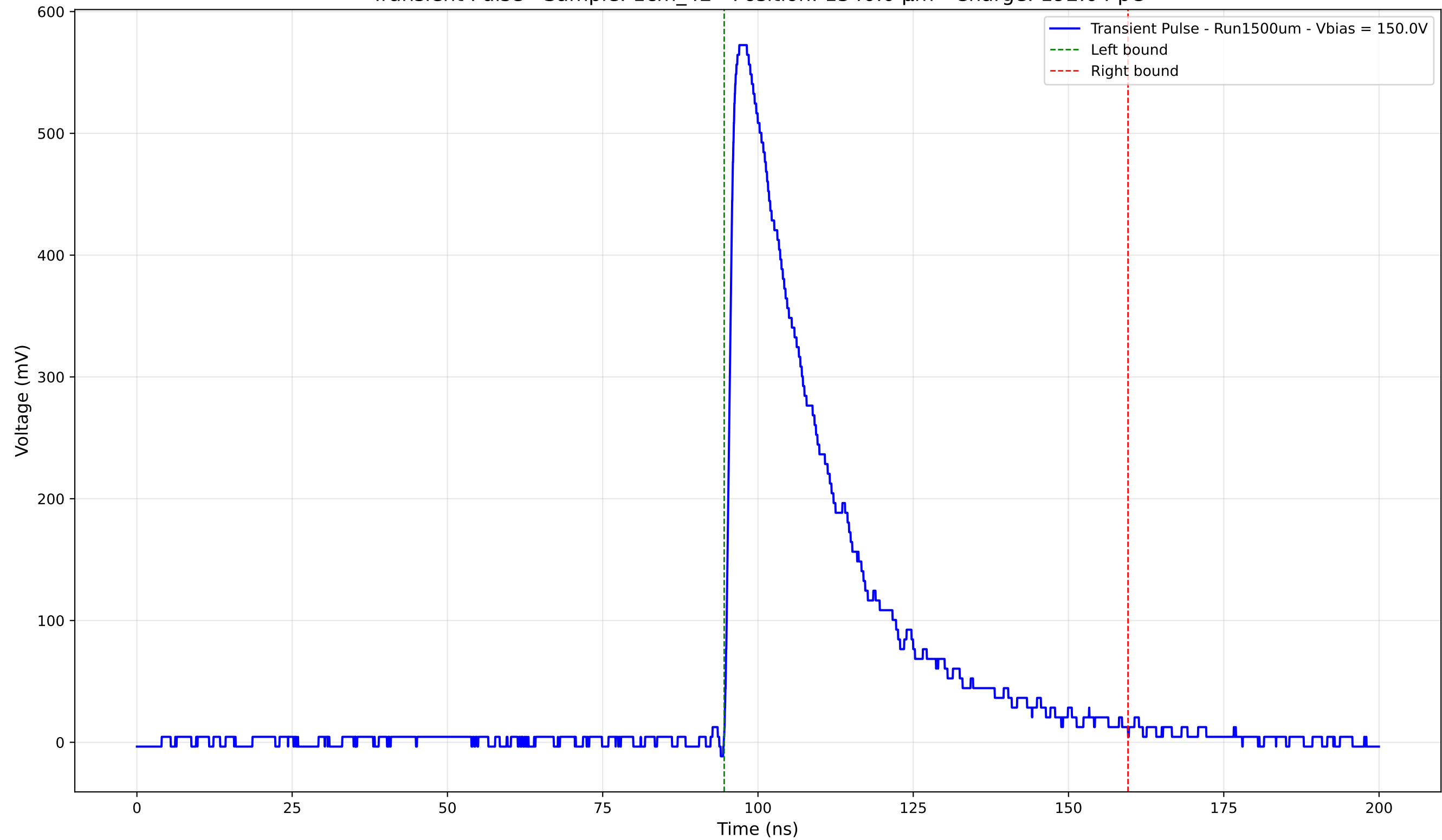
Transient Pulse - Sample: 1cm_42 - Position: 1340.0 \mu\text{m} - Charge: 192.04 pC
