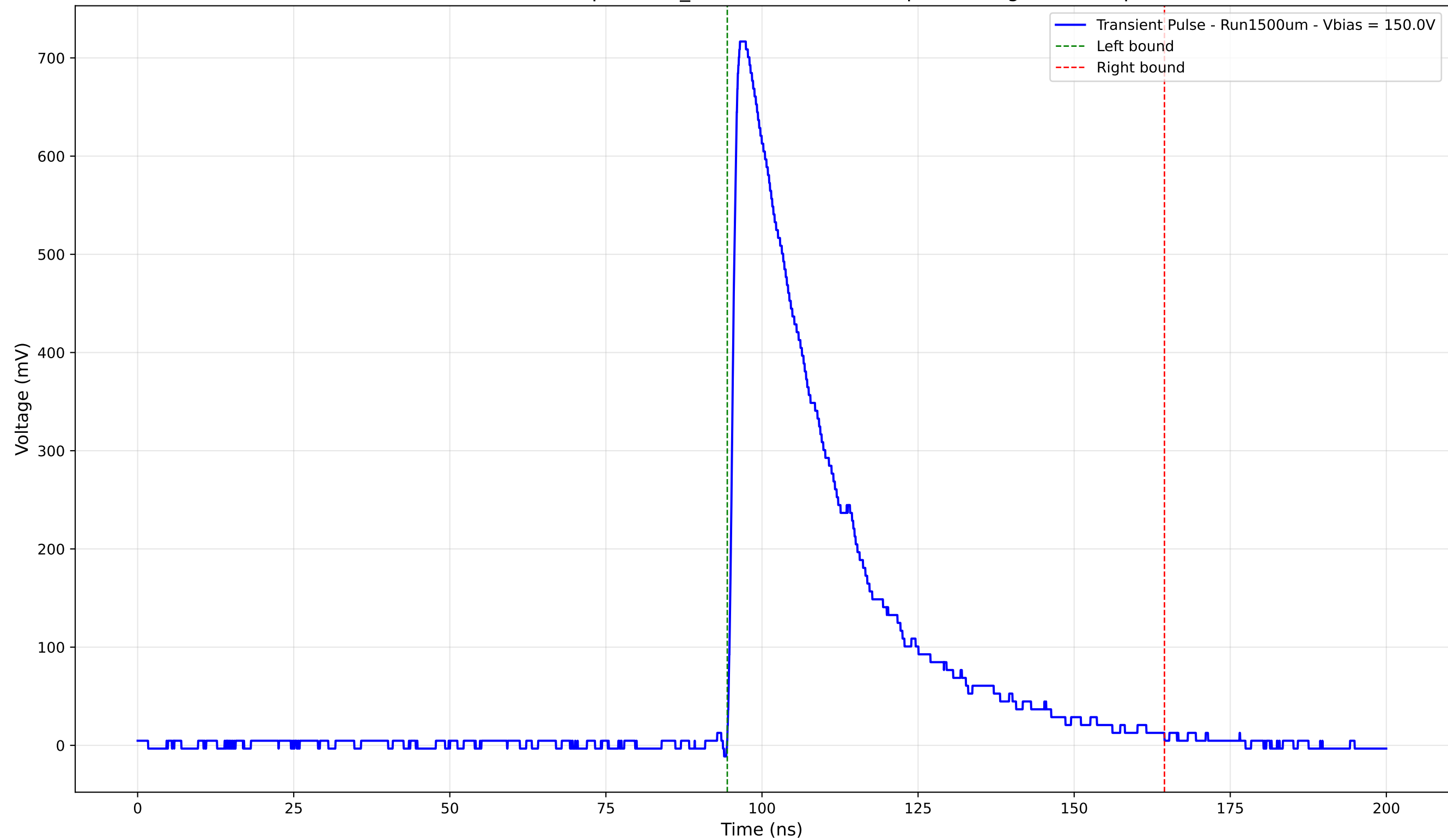
Transient Pulse - Sample: 1cm_42 - Position: 3965.0 \mu\text{m} - Charge: 240.24 pC
