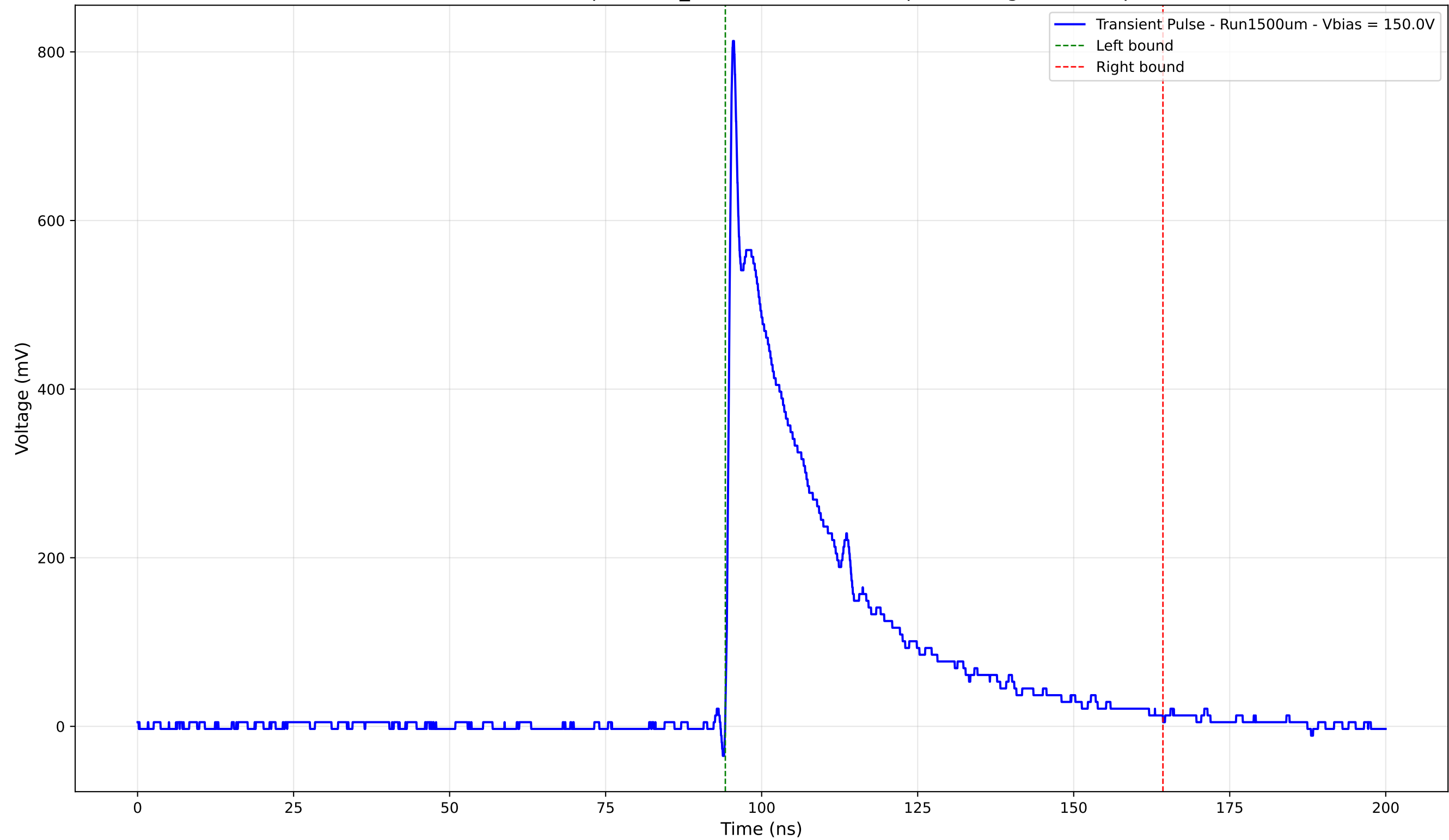
Transient Pulse - Sample: 1cm_42 - Position: 2885.0 \mu\text{m} - Charge: 214.88 pC
