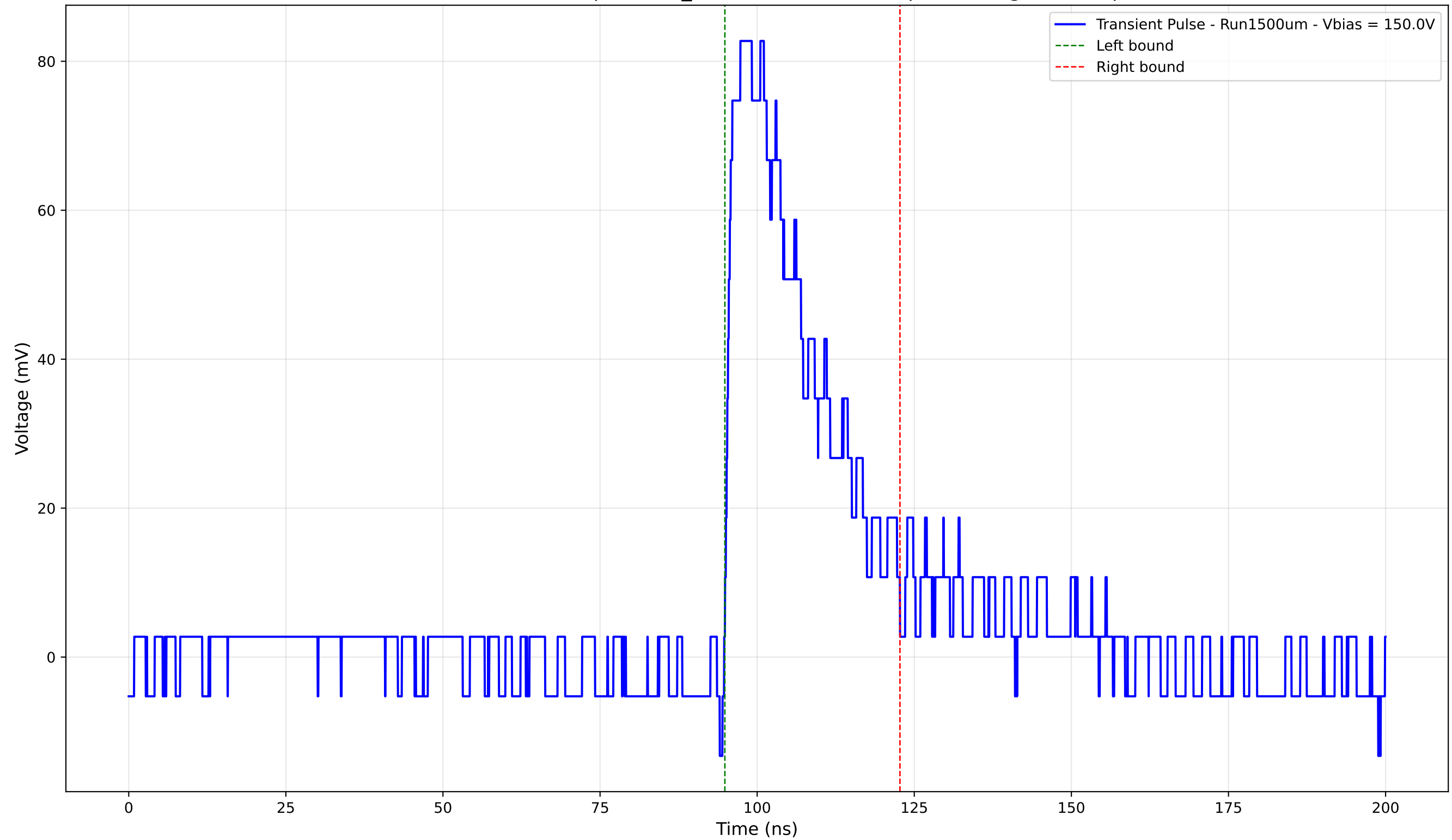
Transient Pulse - Sample: 1cm_42 - Position: 1090.0 \mu\text{m} - Charge: 24.03 pC
