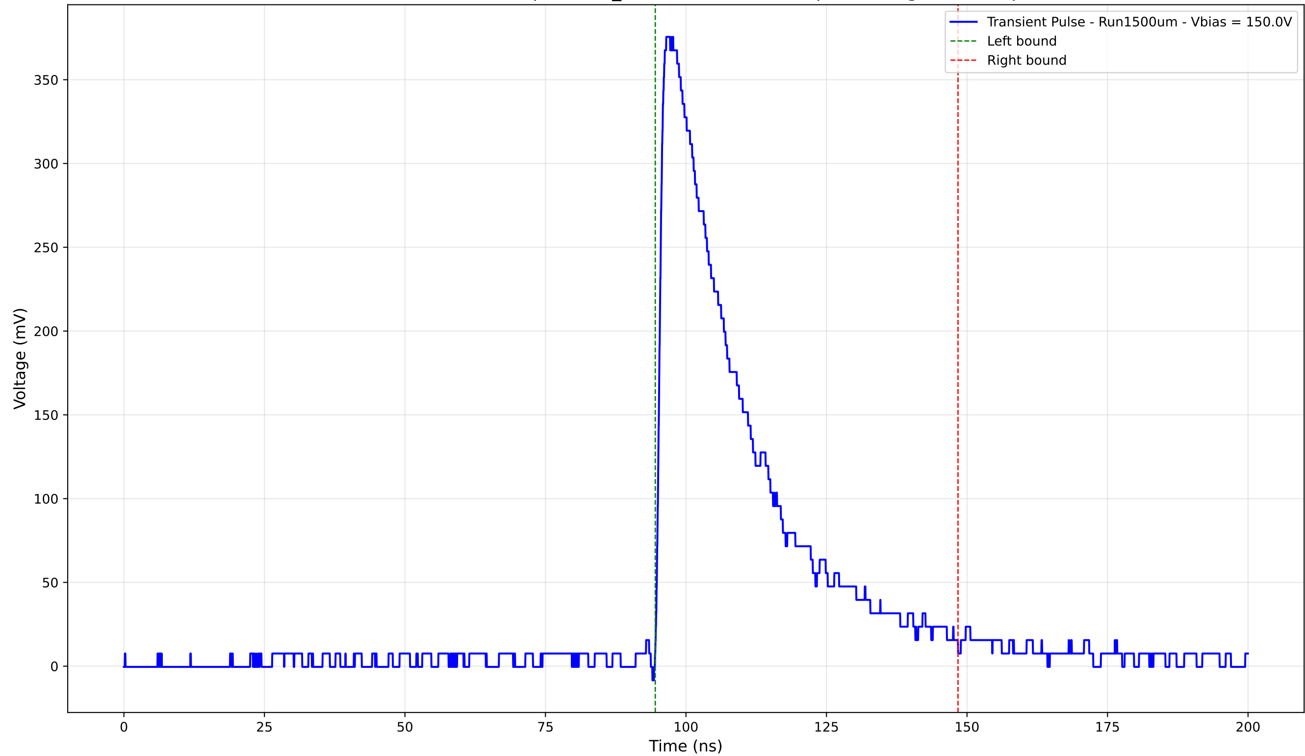
Transient Pulse - Sample: 1cm_42 - Position: 3670.0 \mu\text{m} - Charge: 123.98 pC
