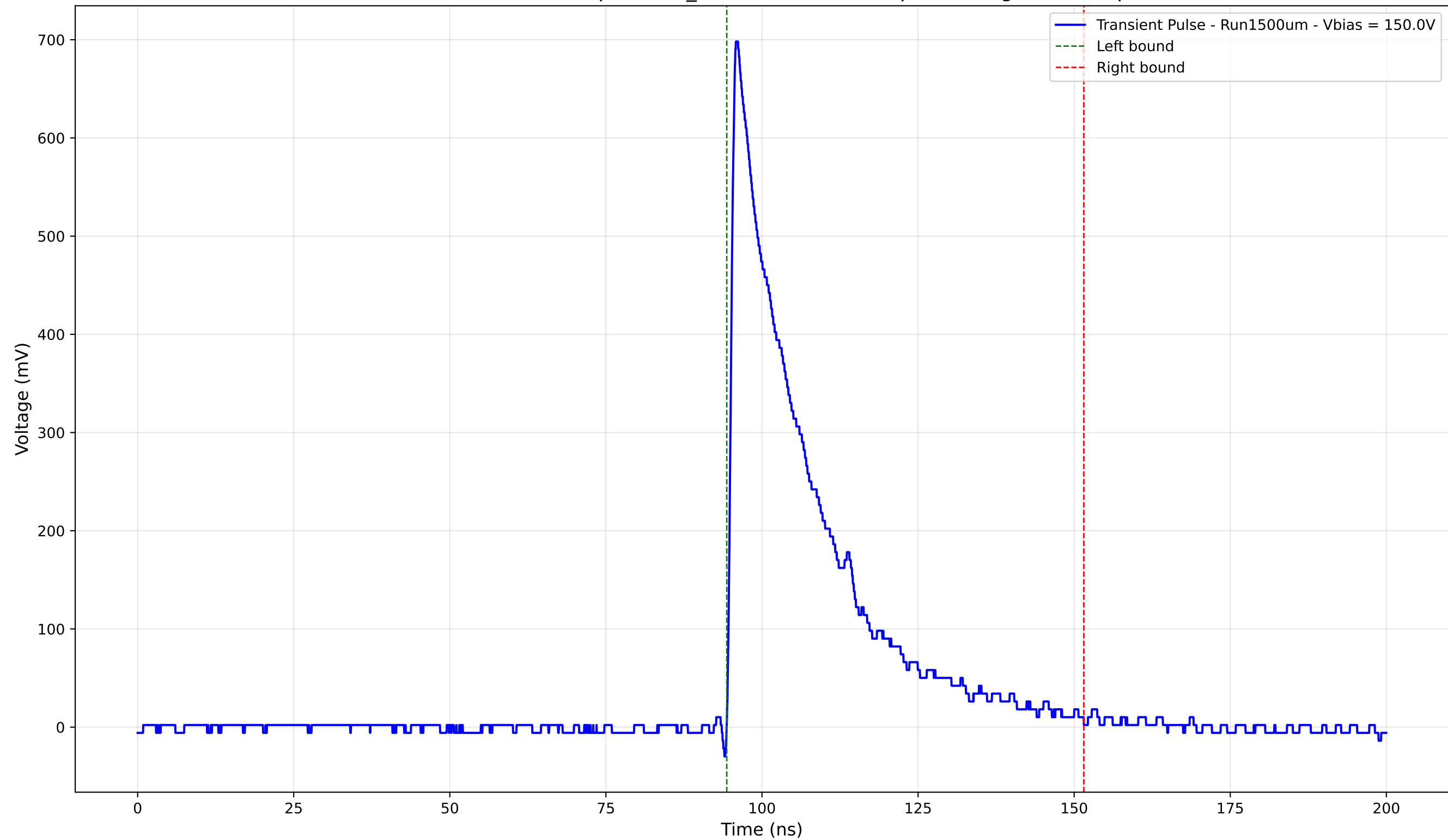
Transient Pulse - Sample: 1cm_42 - Position: 410.0 \mu\text{m} - Charge: 177.27 pC
