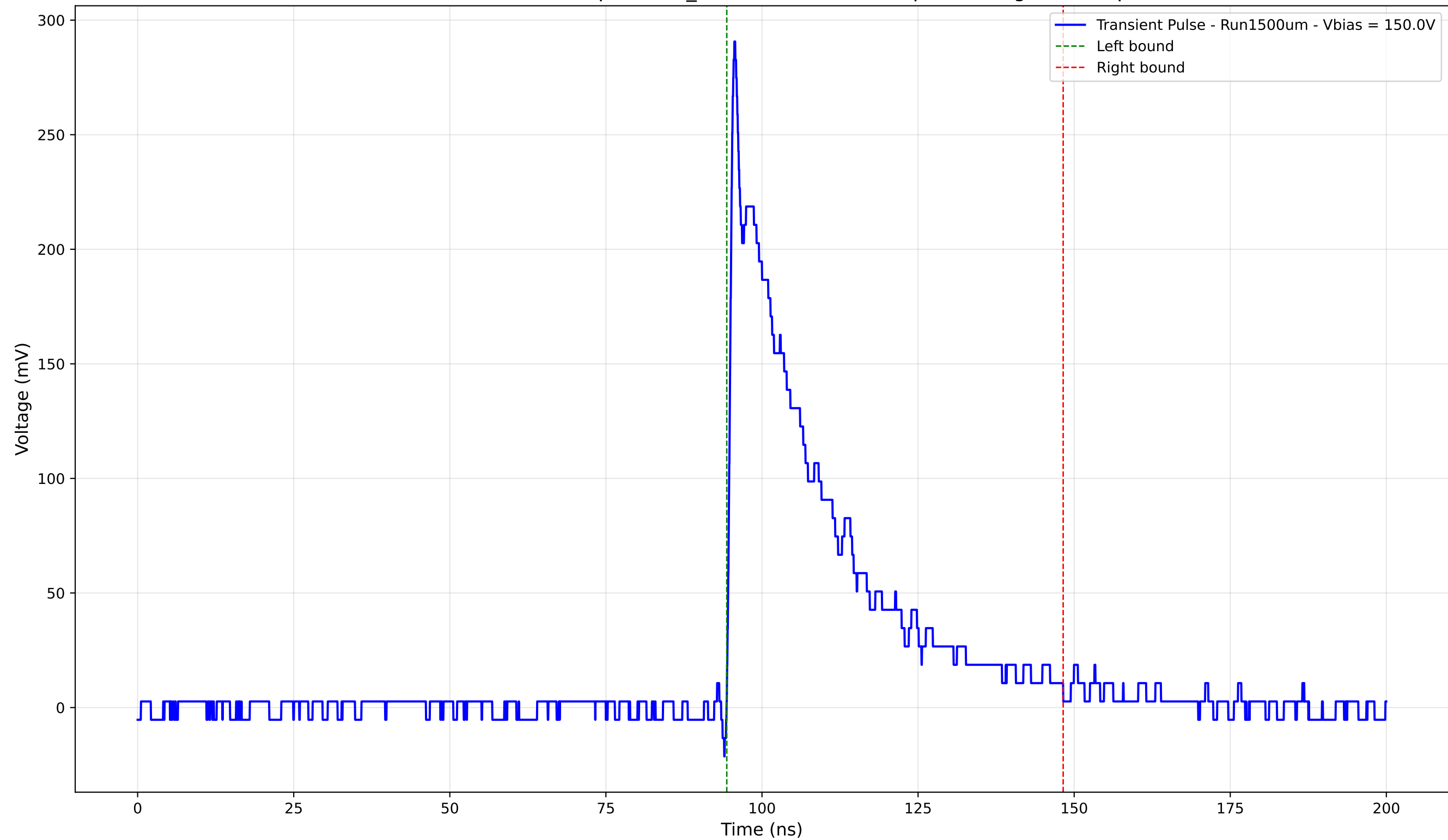
Transient Pulse - Sample: 1cm_42 - Position: 3080.0 \mu\text{m} - Charge: 76.29 pC
