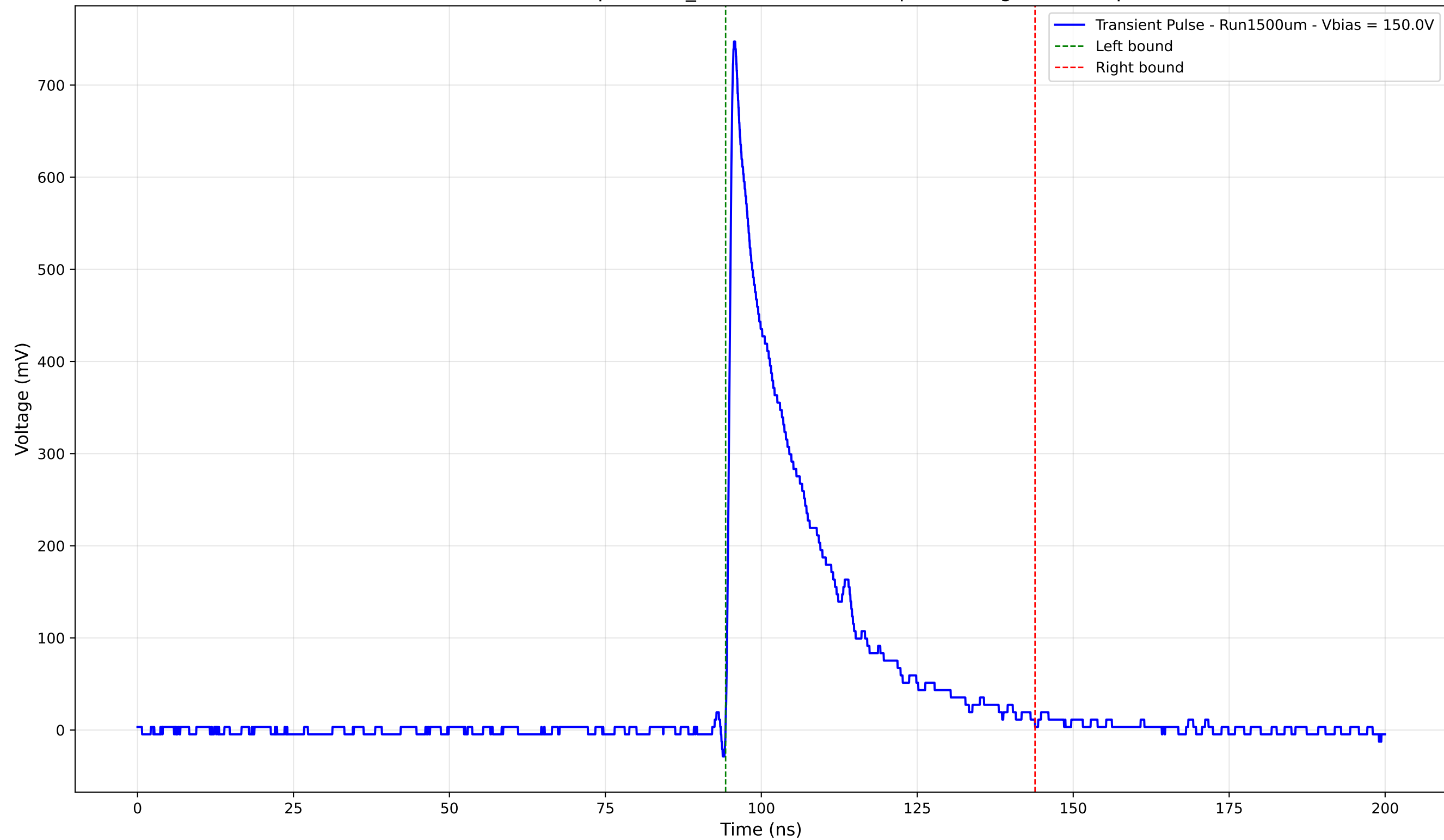
Transient Pulse - Sample: 1cm_42 - Position: 220.0 \mu\text{m} - Charge: 163.39 pC
