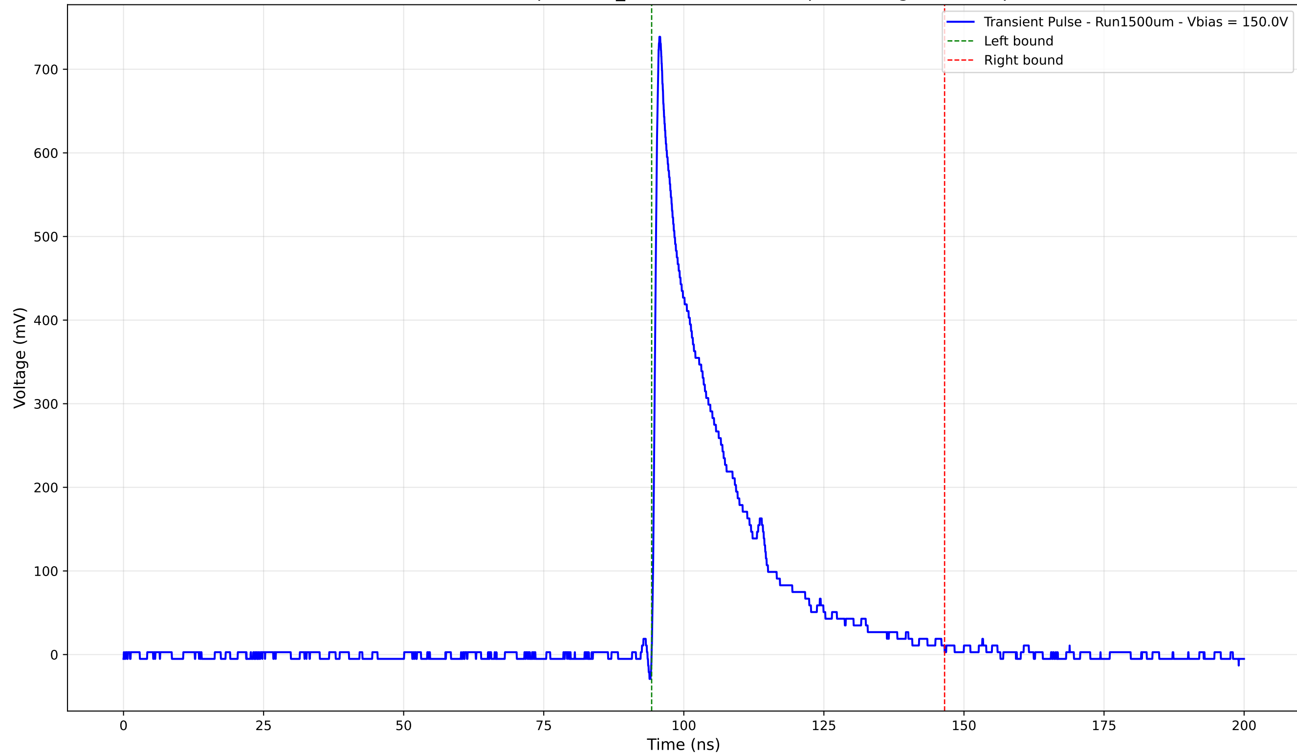
Transient Pulse - Sample: 1cm_42 - Position: 210.0 \mu\text{m} - Charge: 160.79 pC
