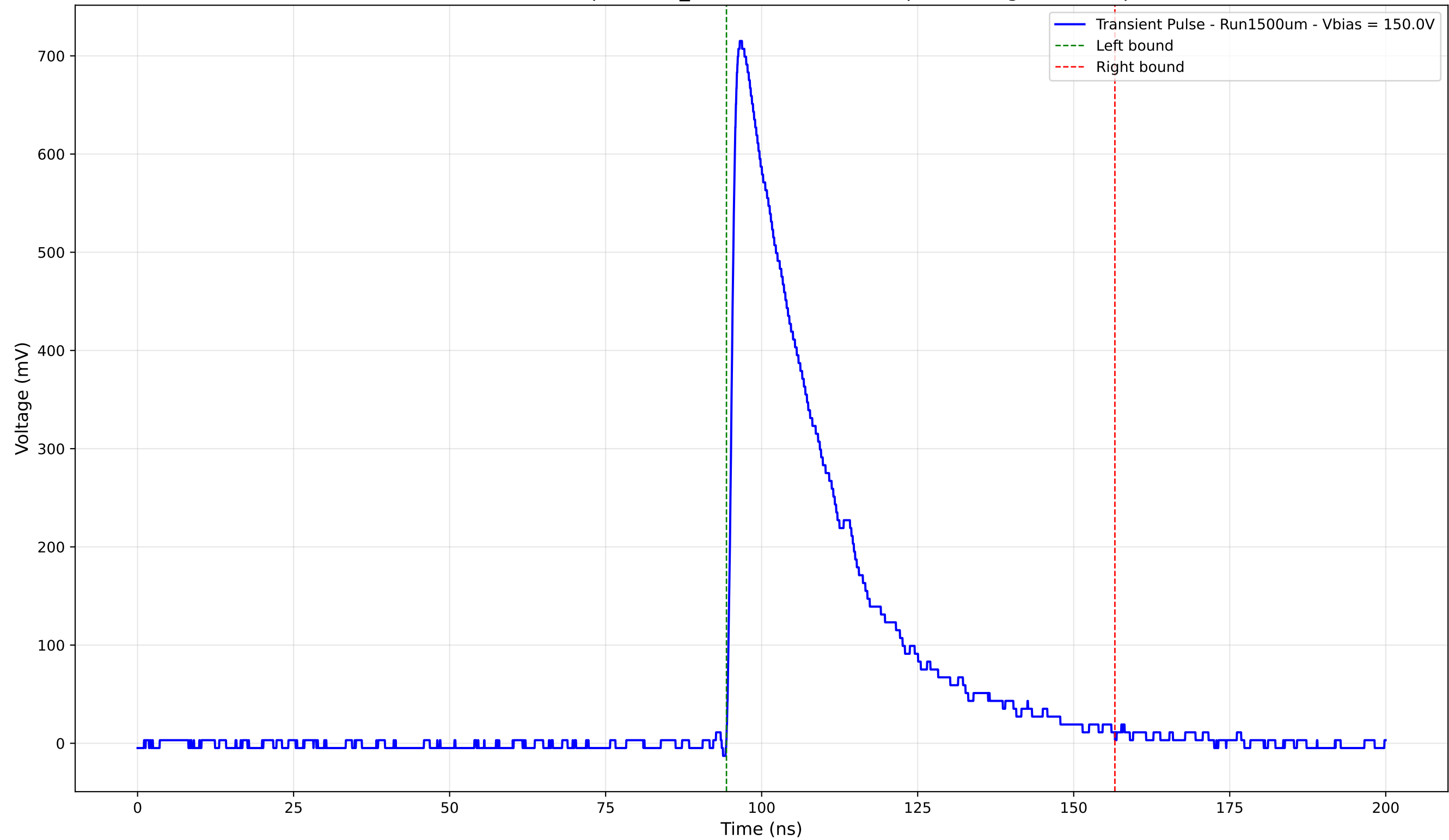
Transient Pulse - Sample: 1cm_42 - Position: 4240.0 \mu\text{m} - Charge: 223.88 pC
