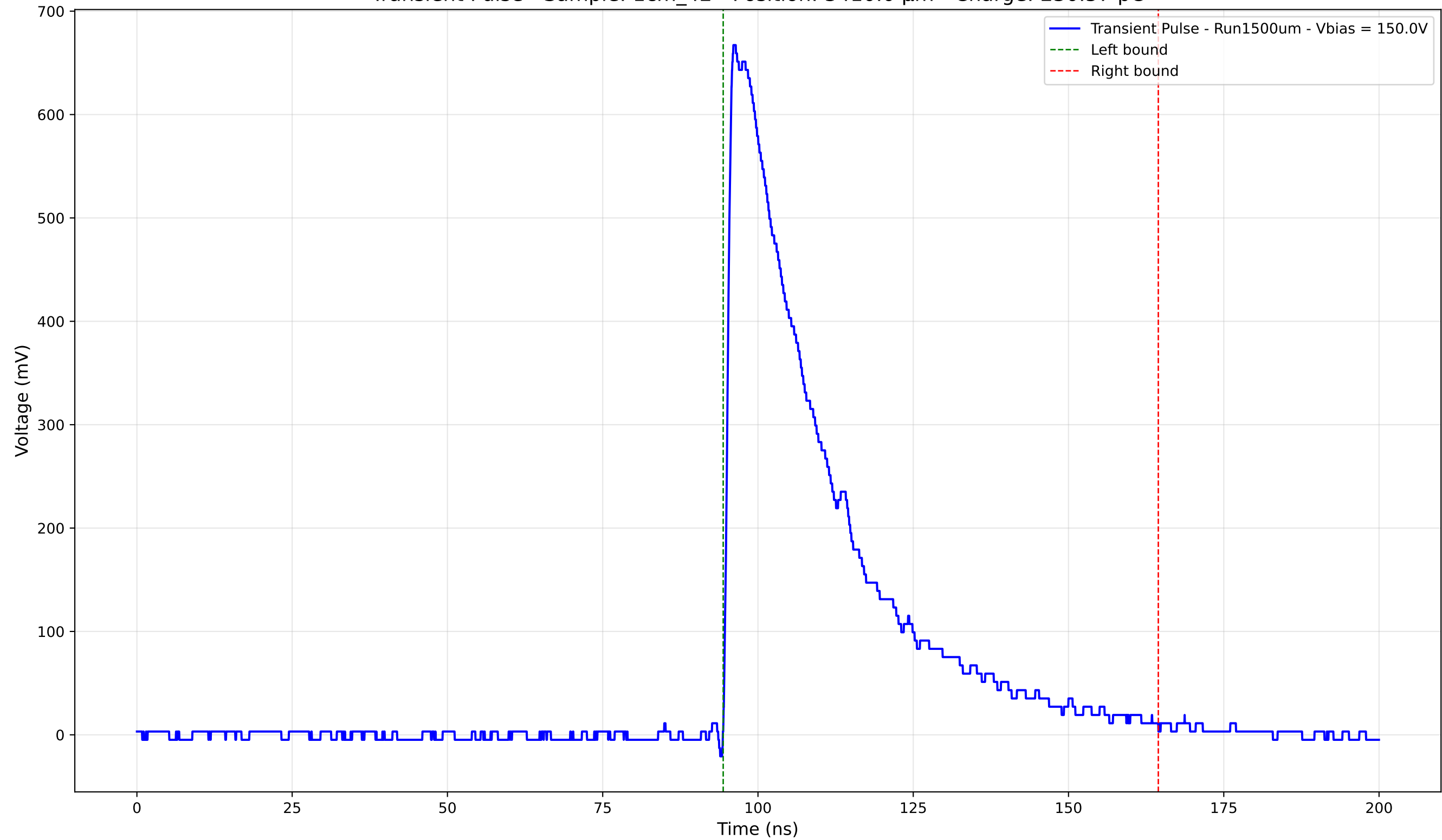
Transient Pulse - Sample: 1cm_42 - Position: 3410.0 \mu\text{m} - Charge: 230.57 pC
