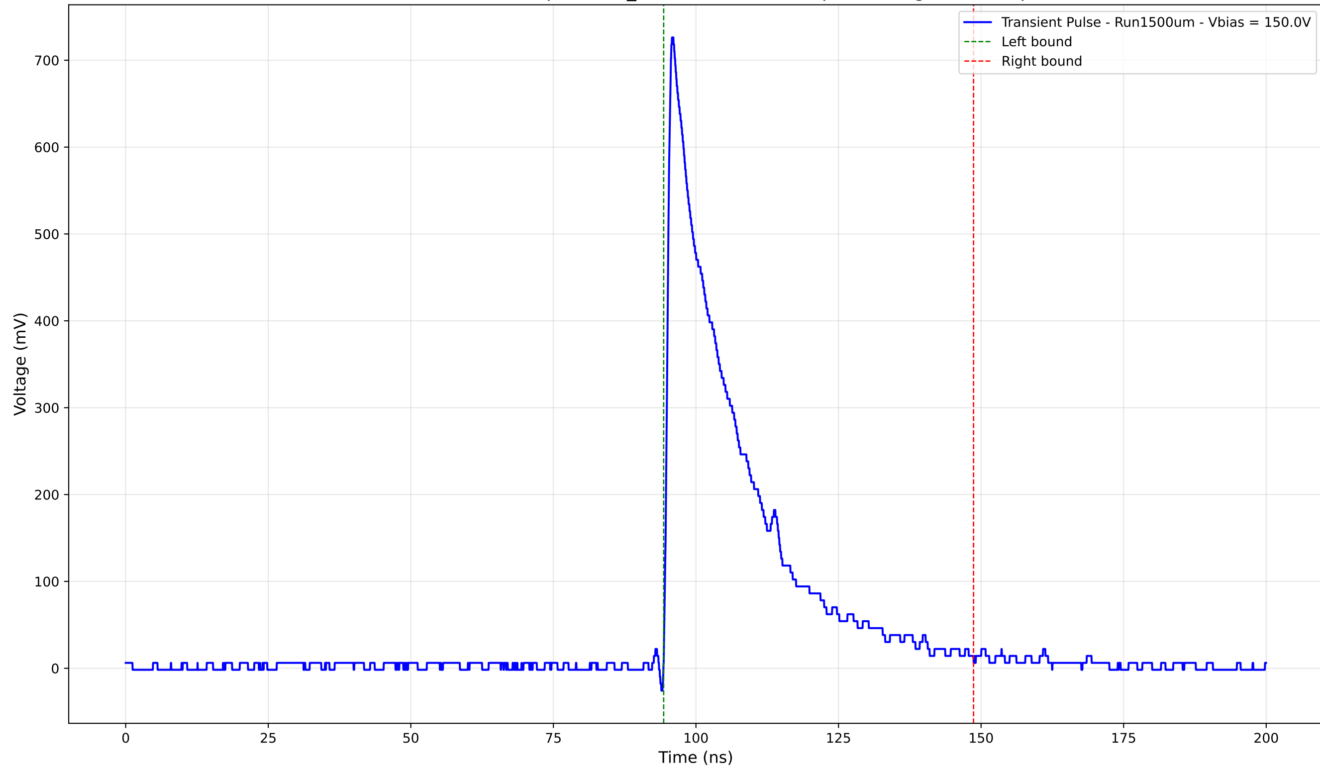
Transient Pulse - Sample: 1cm_42 - Position: 365.0 \mu\text{m} - Charge: 180.68 pC
