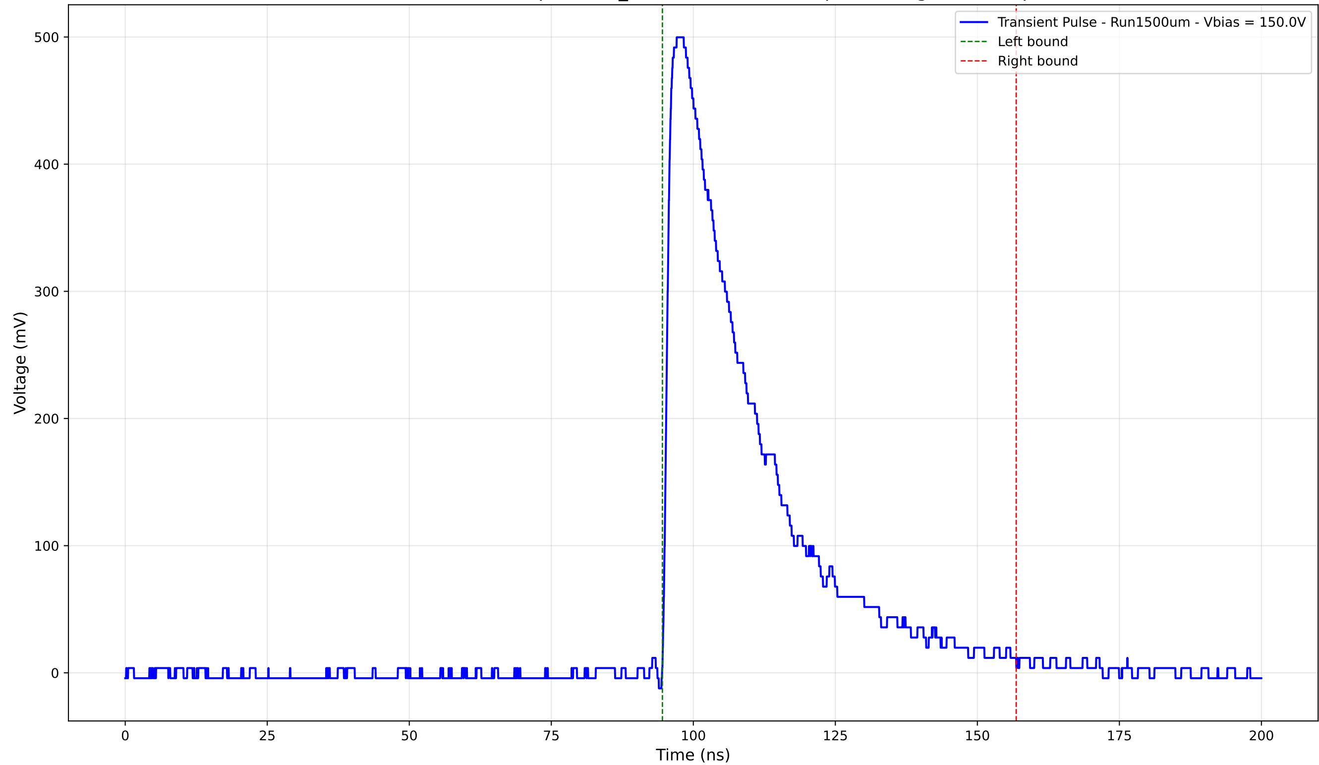
Transient Pulse - Sample: 1cm_42 - Position: 1500.0 \mu\text{m} - Charge: 168.03 pC
