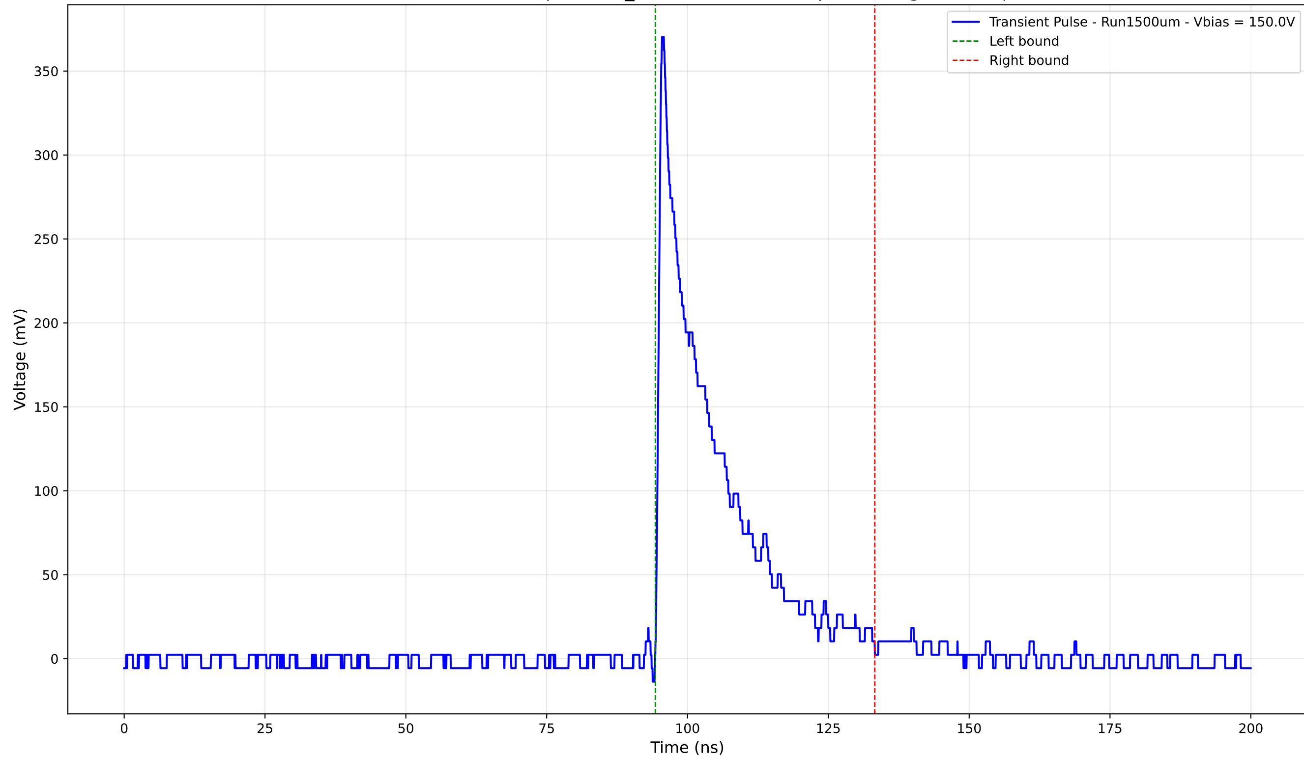
Transient Pulse - Sample: 1cm_42 - Position: 130.0 \mu\text{m} - Charge: 71.06 pC
