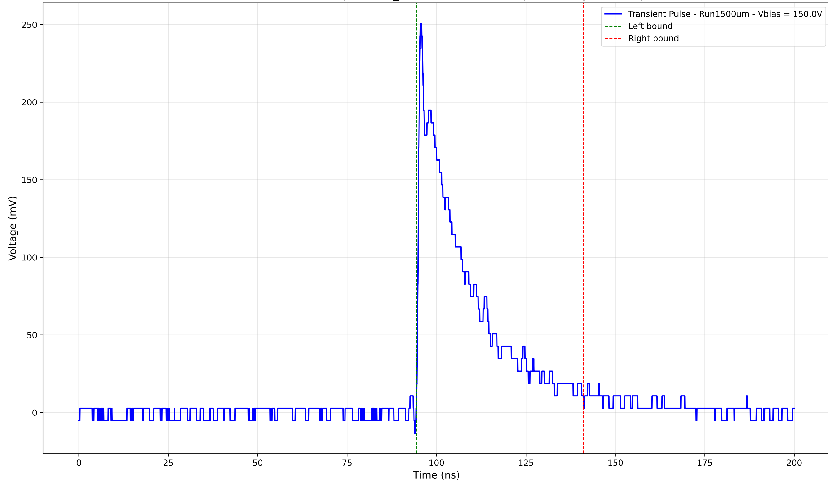
Transient Pulse - Sample: 1cm_42 - Position: 3085.0 \mu\text{m} - Charge: 65.08 pC
