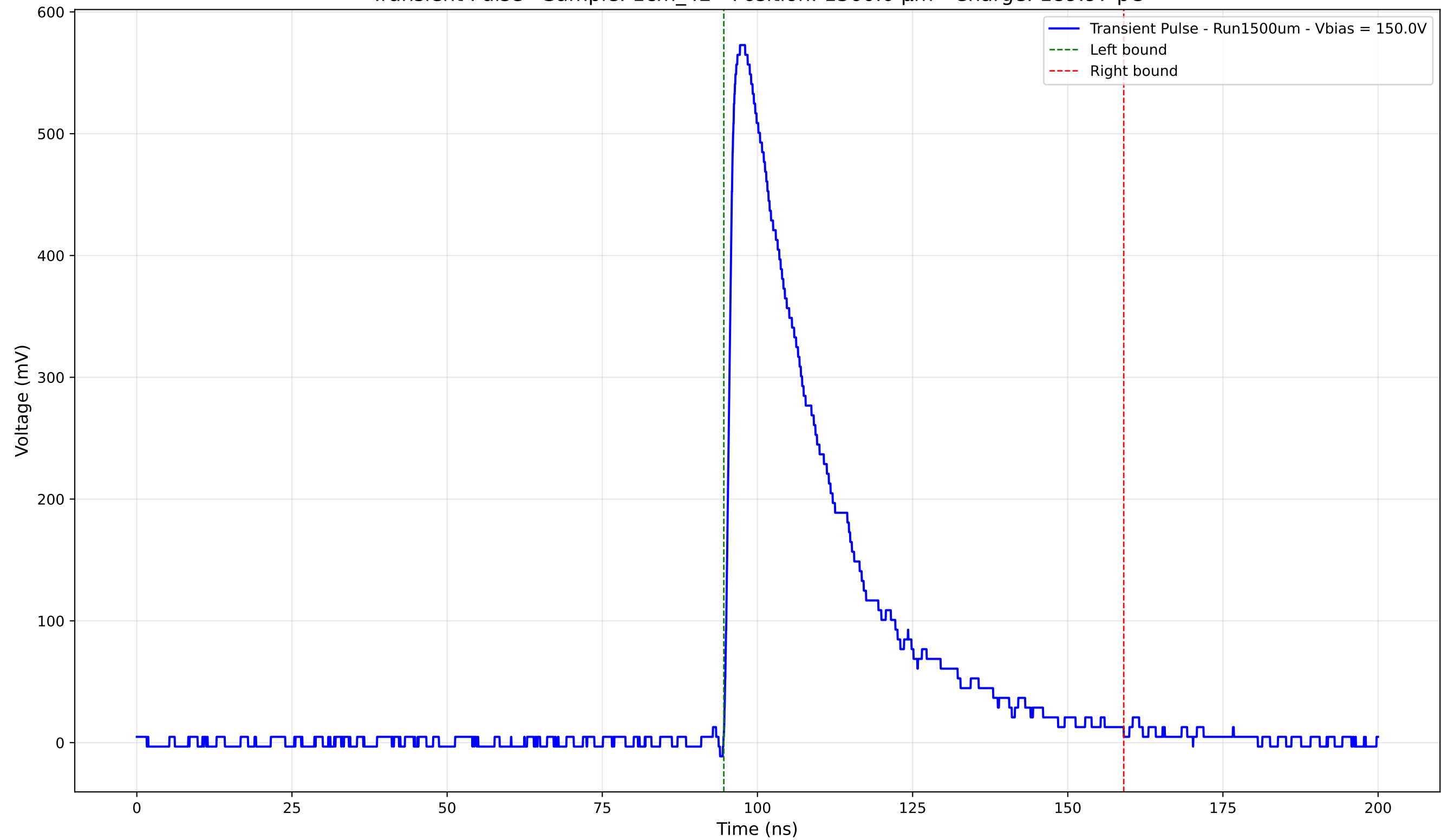
Transient Pulse - Sample: 1cm_42 - Position: 1360.0 \mu\text{m} - Charge: 189.97 pC
