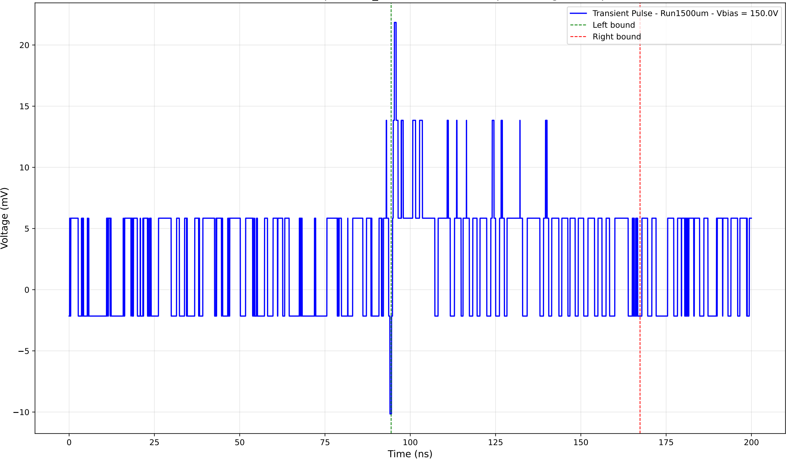
Transient Pulse - Sample: 1cm_42 - Position: 4995.0 \mu\text{m} - Charge: 5.99 pC
