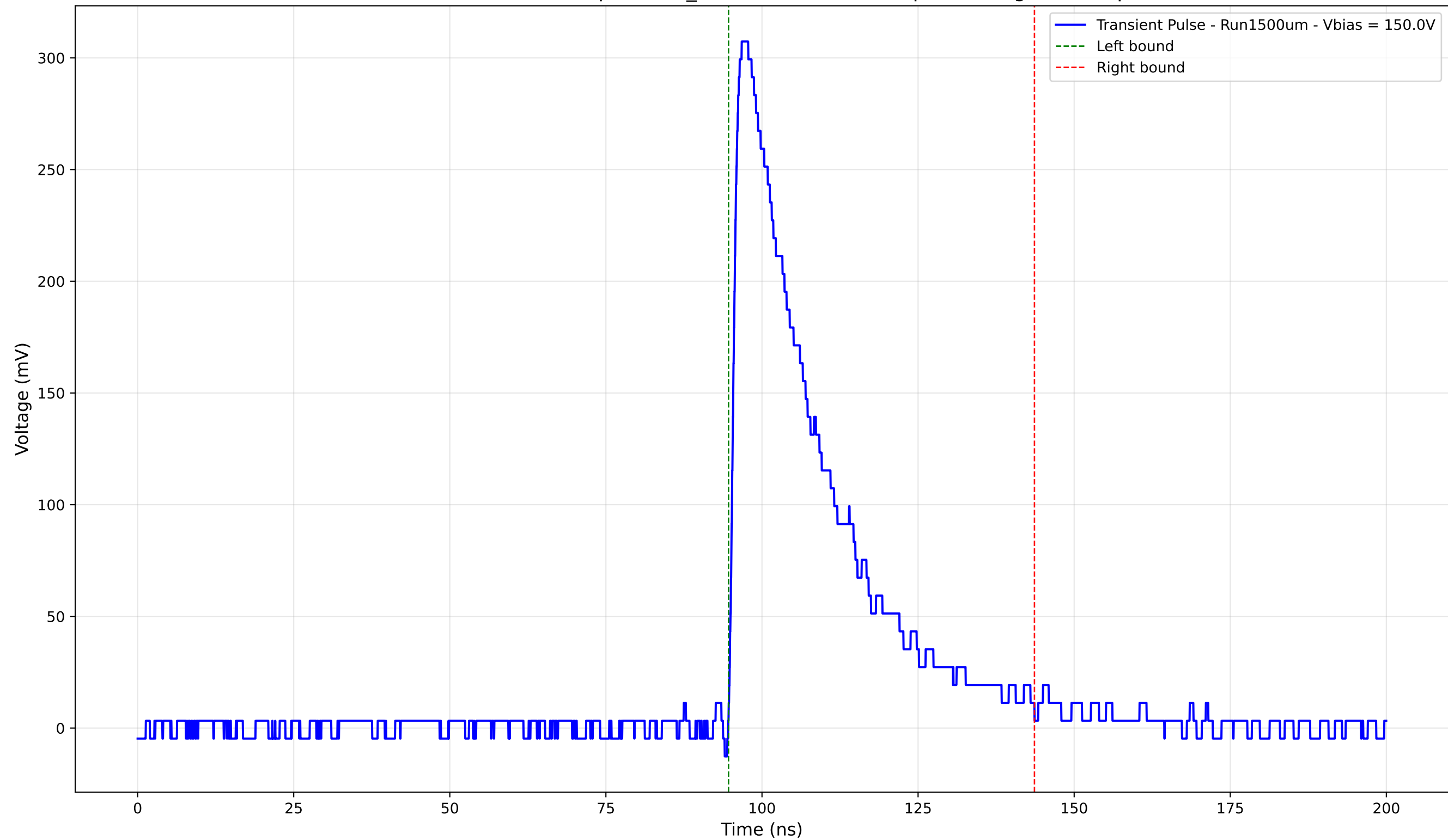
Transient Pulse - Sample: 1cm_42 - Position: 1040.0 \mu\text{m} - Charge: 91.46 pC
