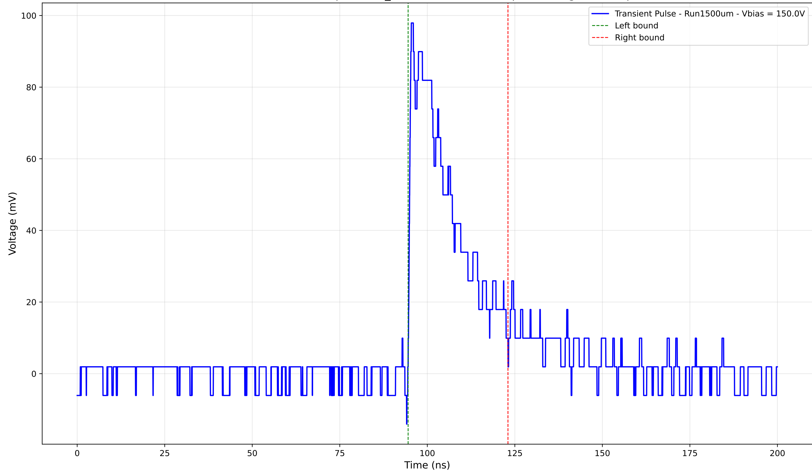
Transient Pulse - Sample: 1cm_42 - Position: 2090.0 \mu\text{m} - Charge: 26.18 pC
