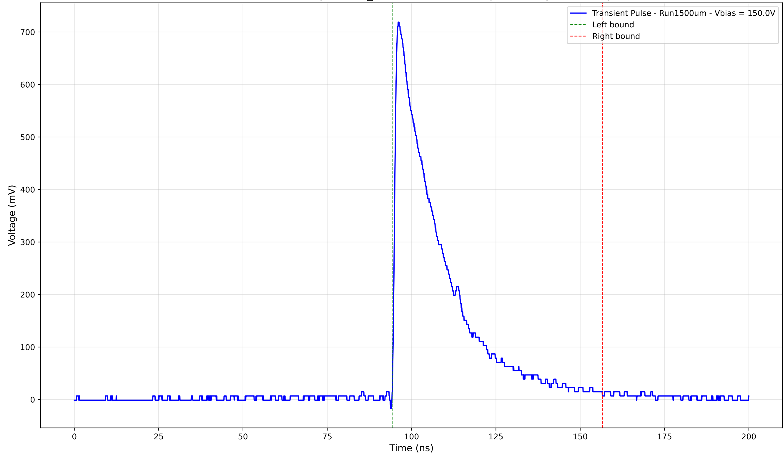
Transient Pulse - Sample: 1cm_42 - Position: 4515.0 \mu\text{m} - Charge: 211.97 pC
