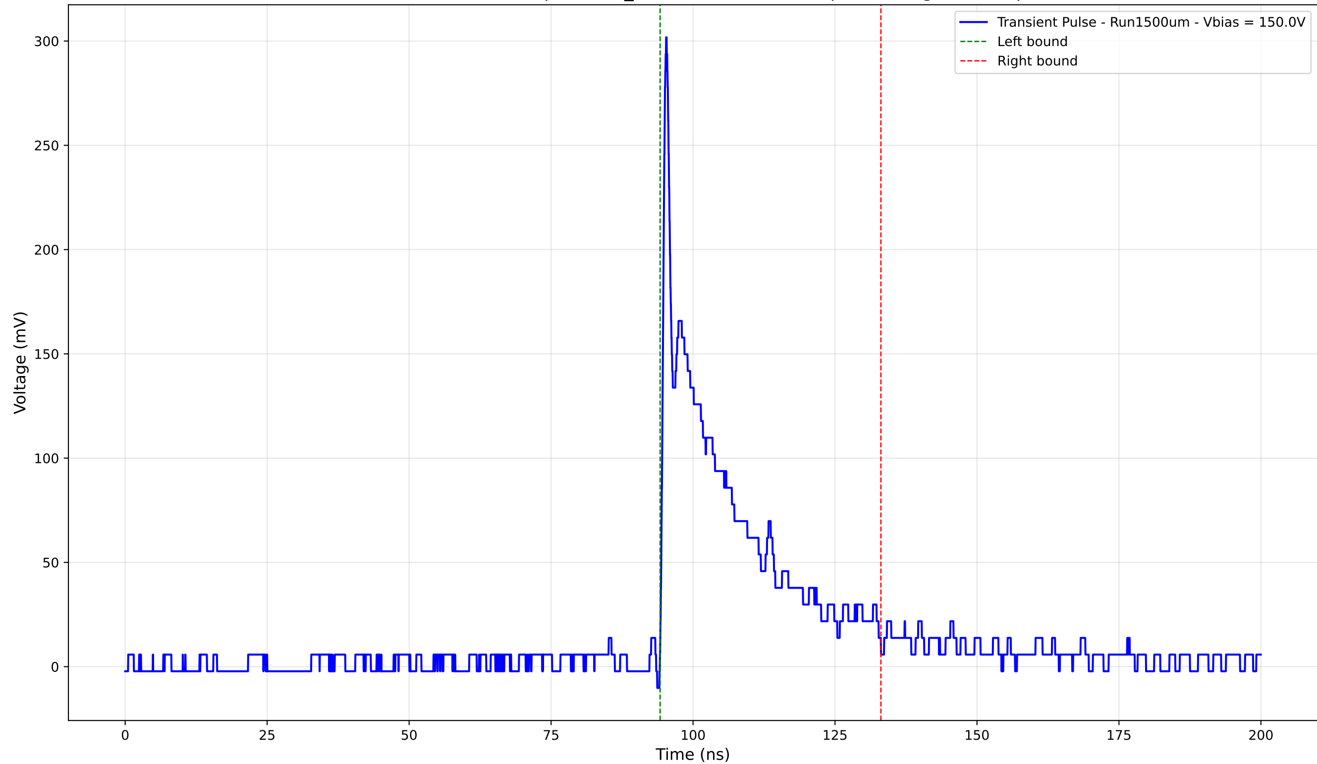
Transient Pulse - Sample: 1cm_42 - Position: 2635.0 \mu\text{m} - Charge: 54.06 pC
