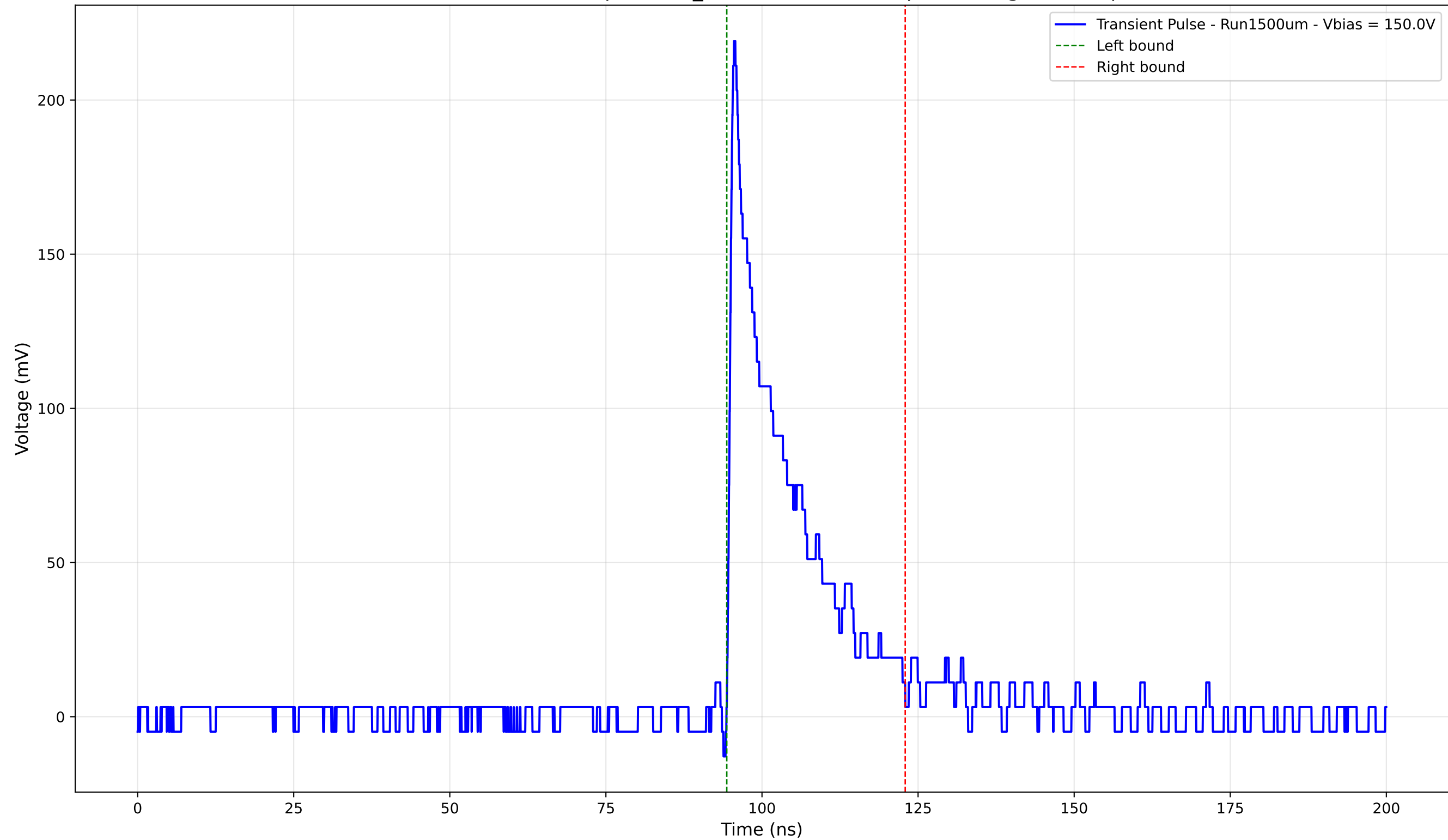
Transient Pulse - Sample: 1cm_42 - Position: 110.0 \mu\text{m} - Charge: 38.53 pC
