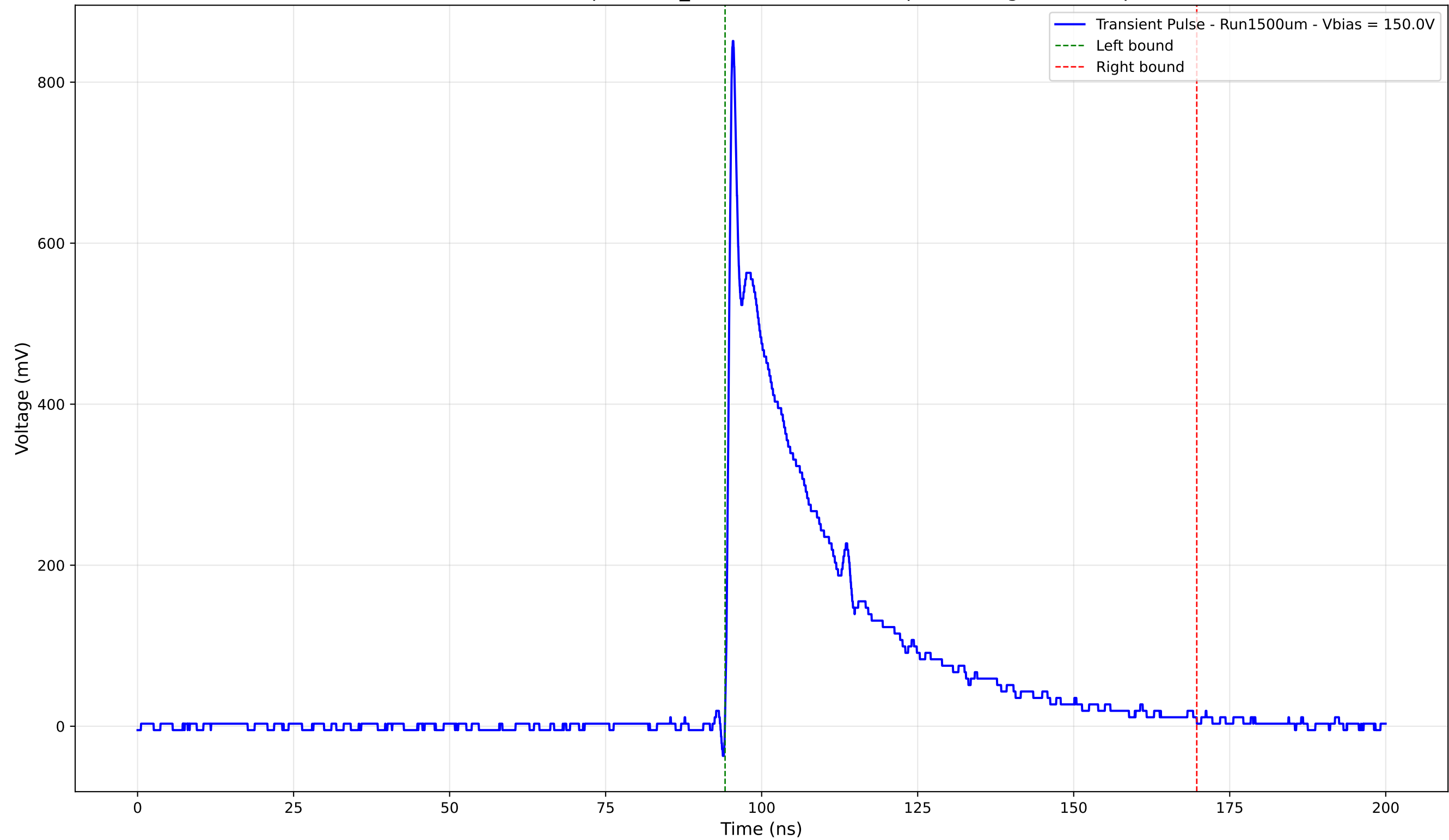
Transient Pulse - Sample: 1cm_42 - Position: 2820.0 \mu\text{m} - Charge: 213.20 pC
