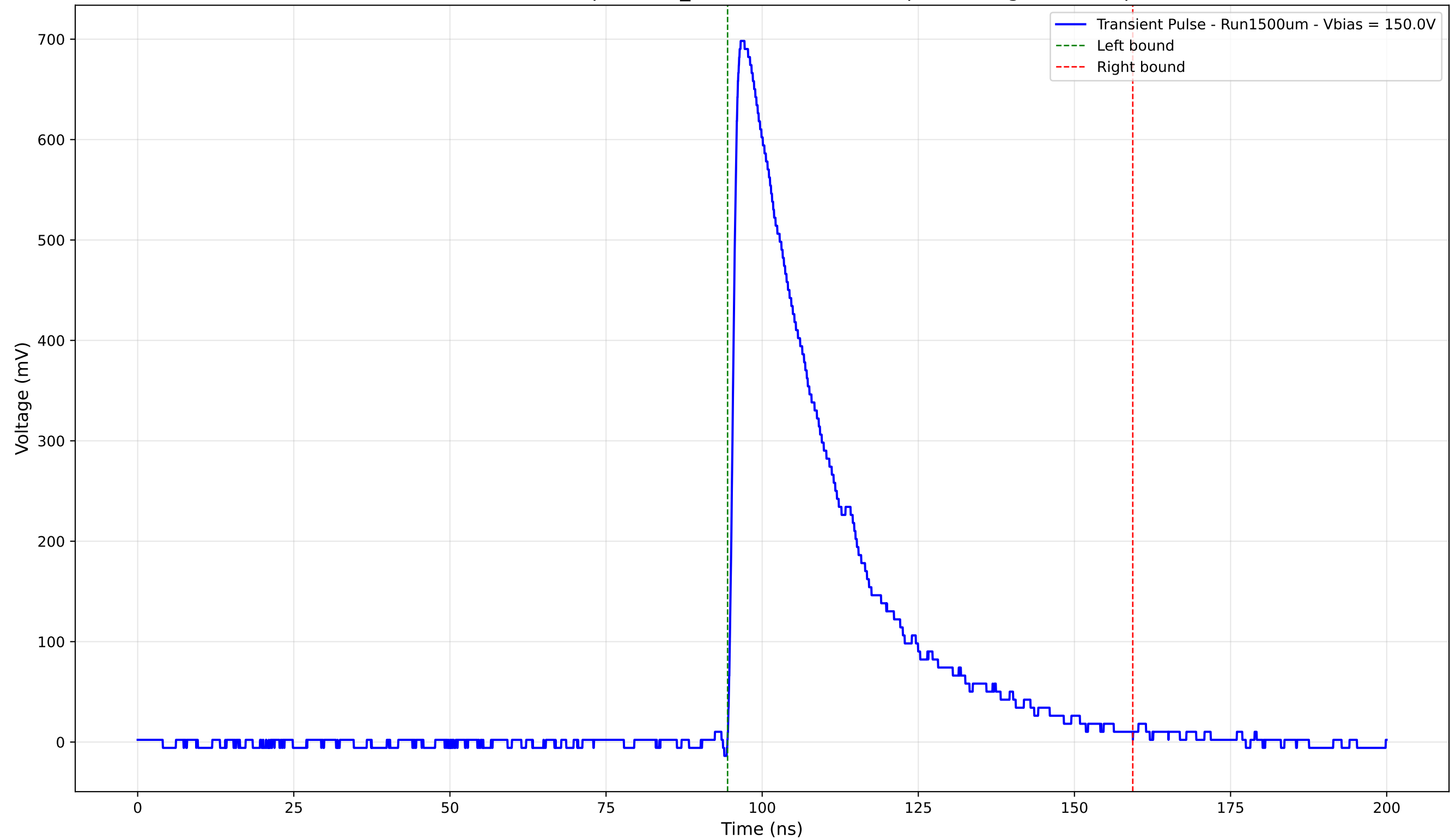
Transient Pulse - Sample: 1cm_42 - Position: 3890.0 \mu\text{m} - Charge: 229.58 pC
