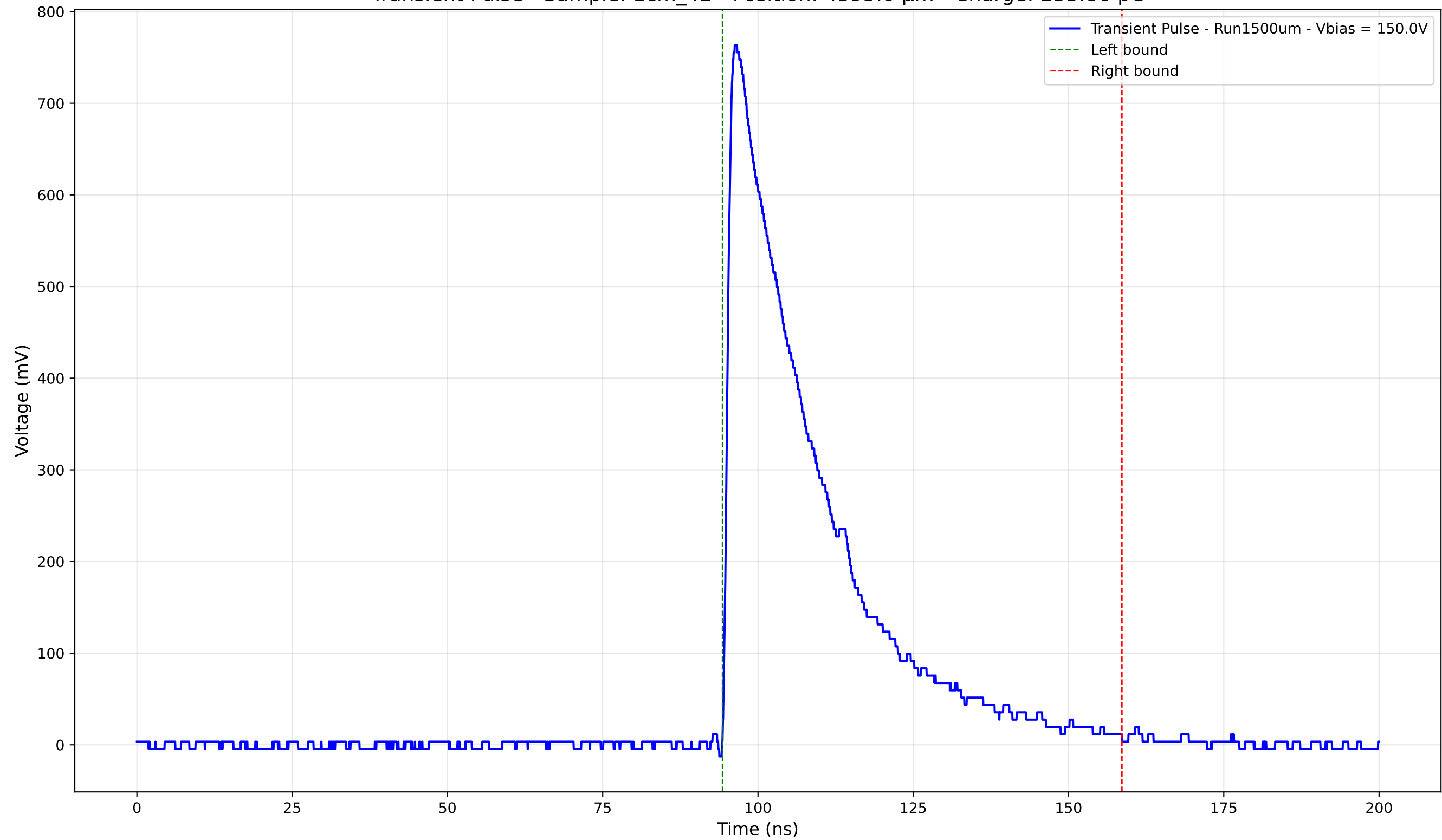
Transient Pulse - Sample: 1cm_42 - Position: 4395.0 \mu\text{m} - Charge: 233.86 pC
