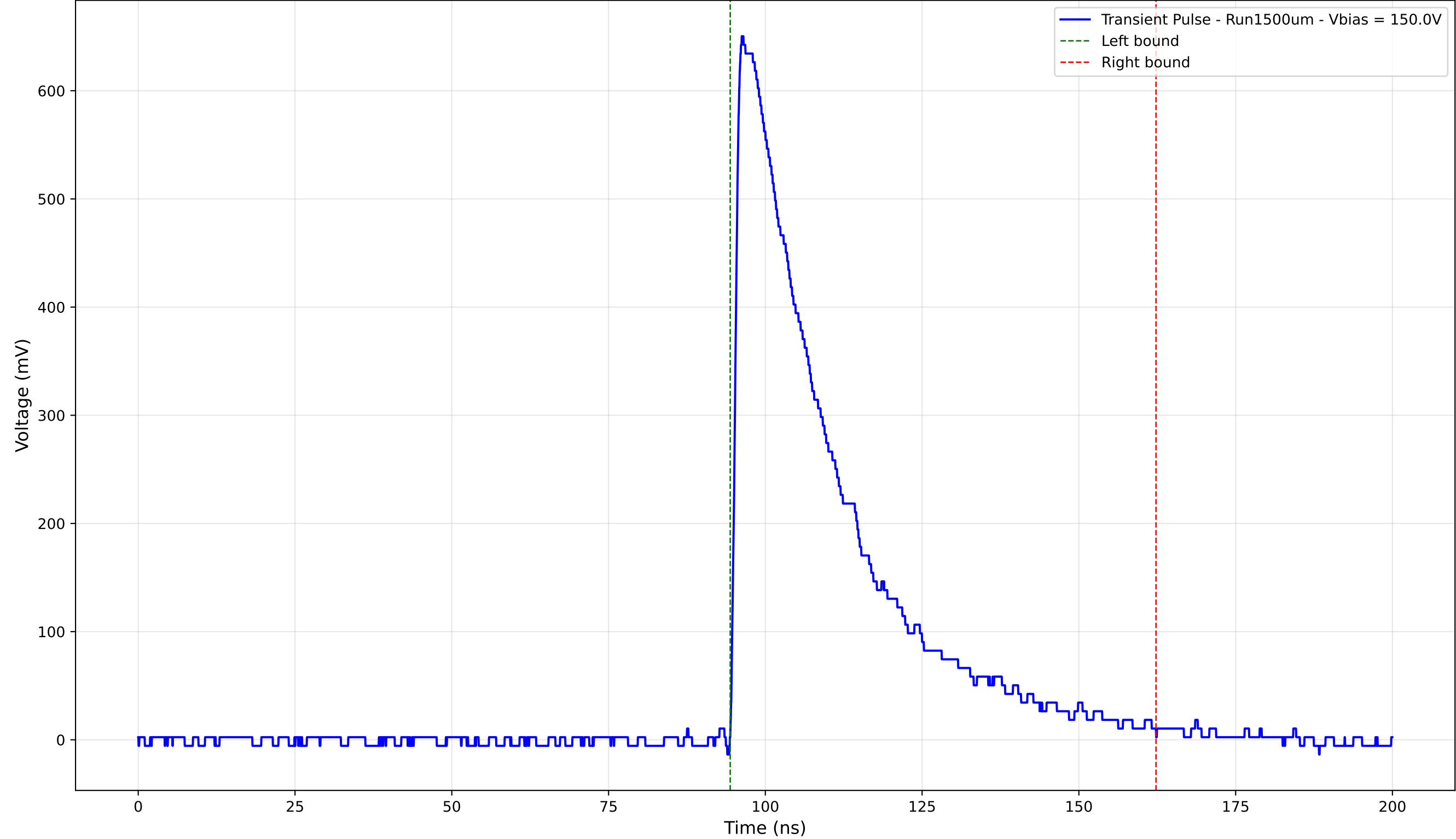
Transient Pulse - Sample: 1cm_42 - Position: 3515.0 \mu\text{m} - Charge: 220.15 pC
