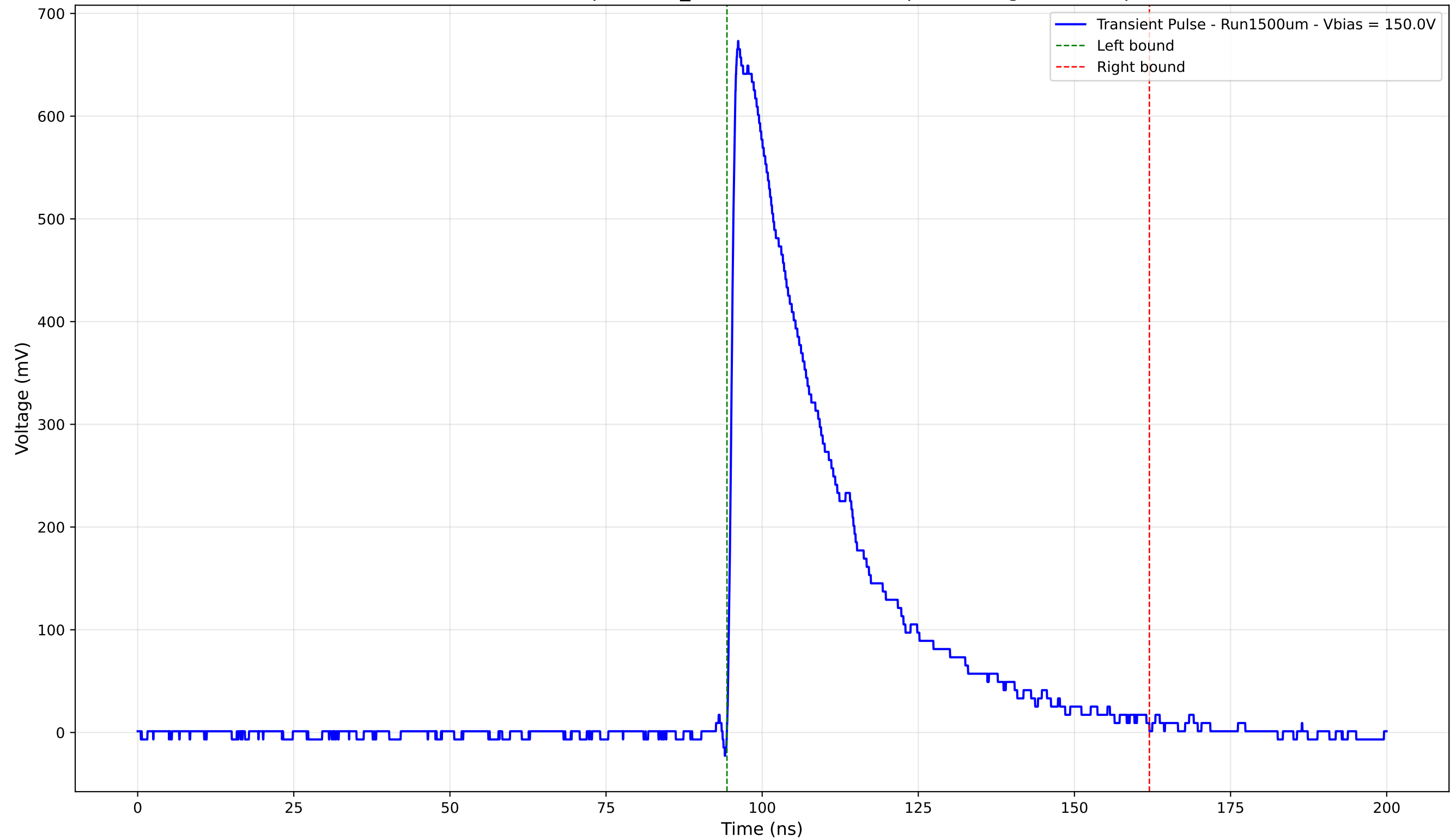
Transient Pulse - Sample: 1cm_42 - Position: 3400.0 \mu\text{m} - Charge: 226.72 pC
