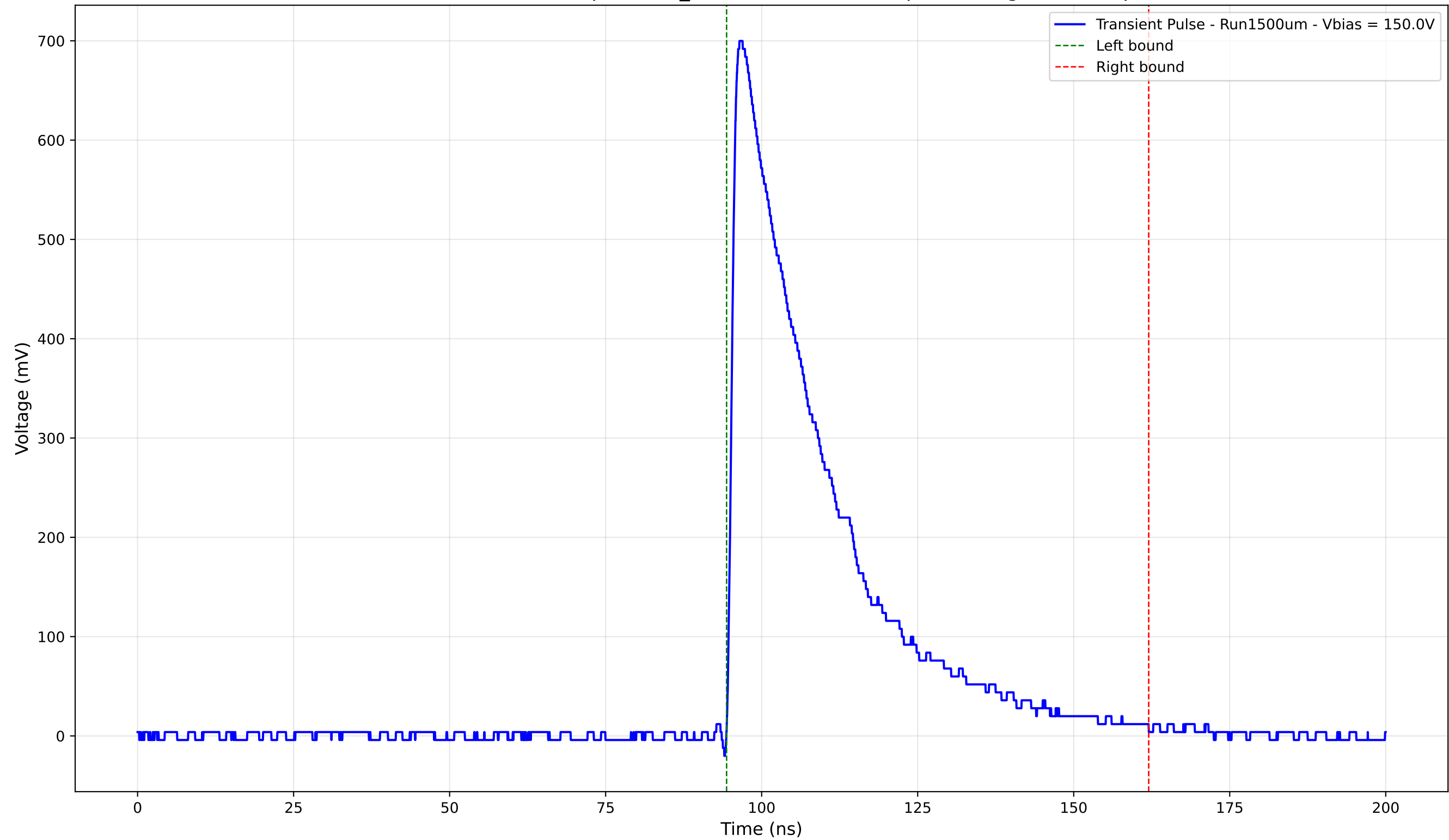
Transient Pulse - Sample: 1cm_42 - Position: 4230.0 \mu\text{m} - Charge: 220.98 pC
