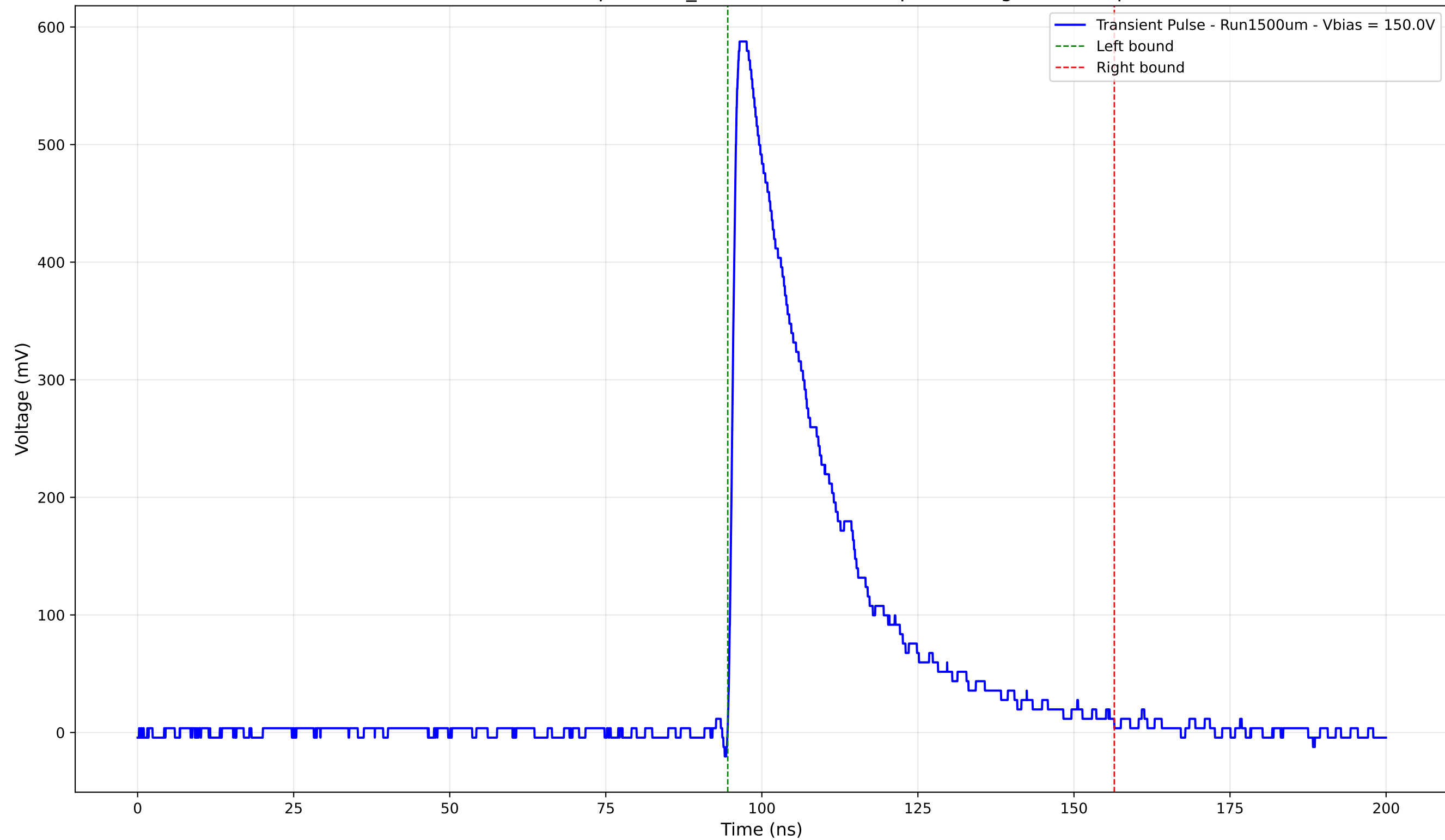
Transient Pulse - Sample: 1cm_42 - Position: 845.0 \mu\text{m} - Charge: 180.08 pC
