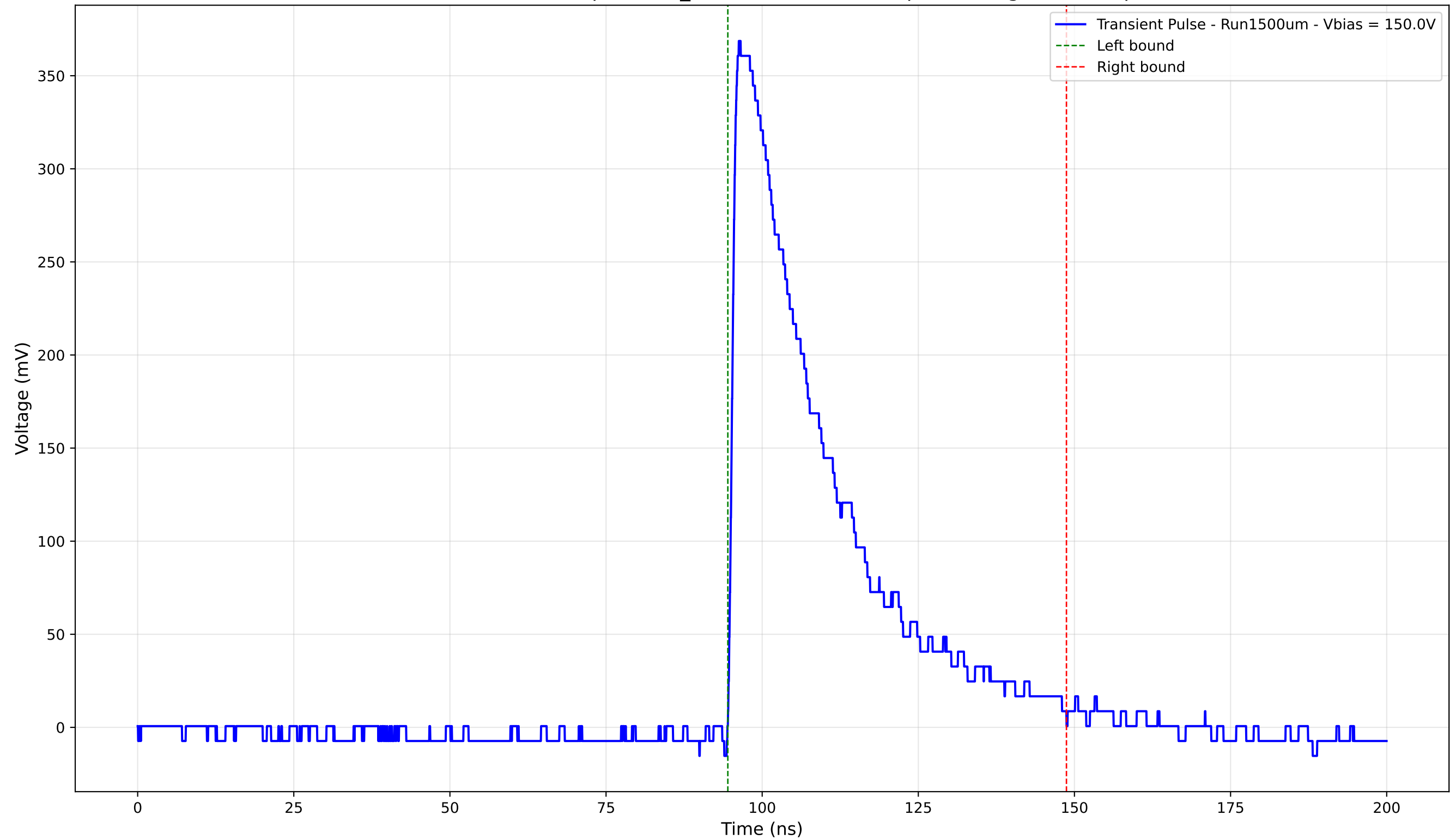
Transient Pulse - Sample: 1cm_42 - Position: 3565.0 \mu\text{m} - Charge: 118.48 pC
