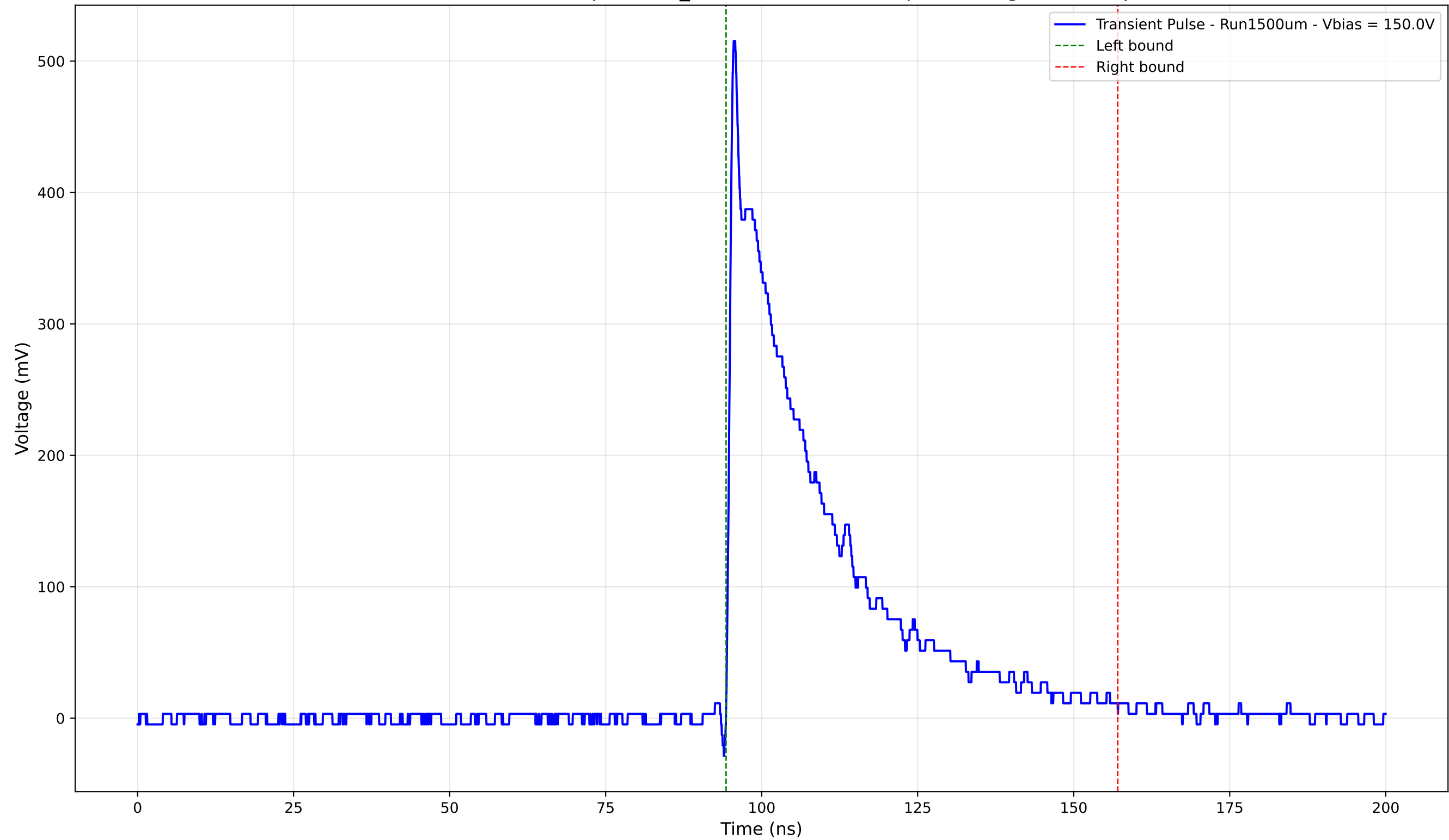
Transient Pulse - Sample: 1cm_42 - Position: 3055.0 \mu\text{m} - Charge: 139.67 pC
