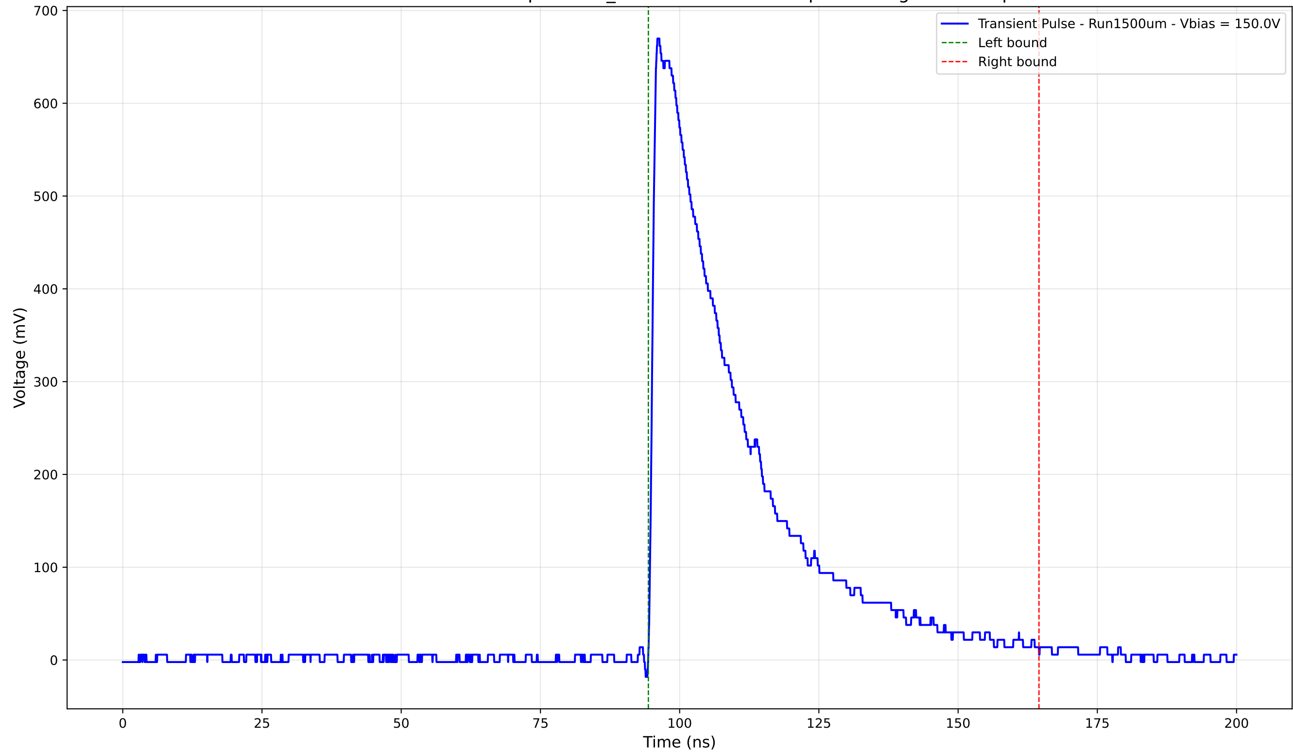
Transient Pulse - Sample: 1cm_42 - Position: 3385.0 \mu\text{m} - Charge: 232.73 pC
