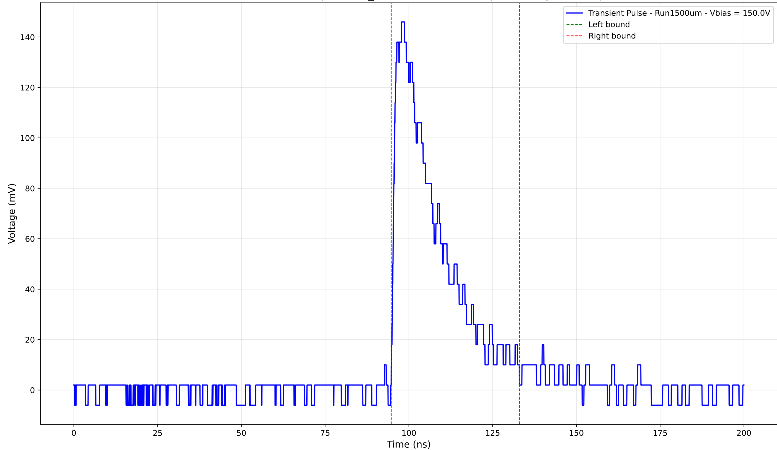
Transient Pulse - Sample: 1cm_42 - Position: 1115.0 \mu\text{m} - Charge: 42.85 pC
