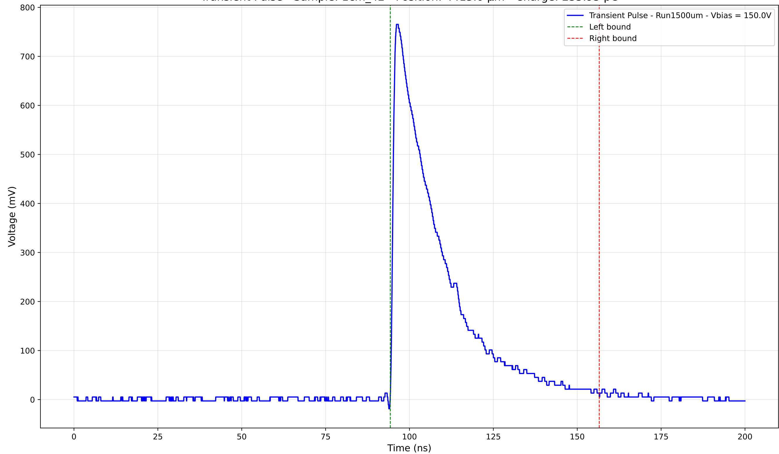
Transient Pulse - Sample: 1cm_42 - Position: 4415.0 \mu\text{m} - Charge: 235.95 pC
