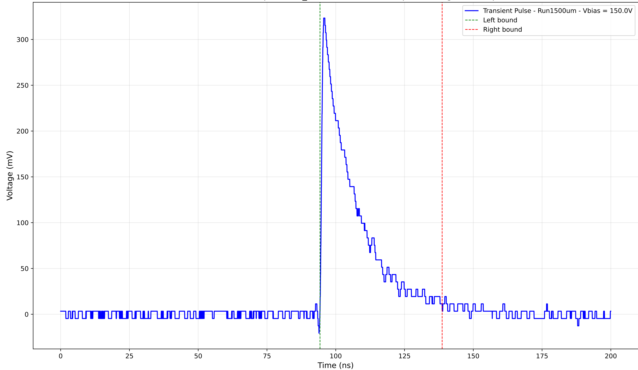
Transient Pulse - Sample: 1cm_42 - Position: 4670.0 \mu\text{m} - Charge: 80.17 pC
