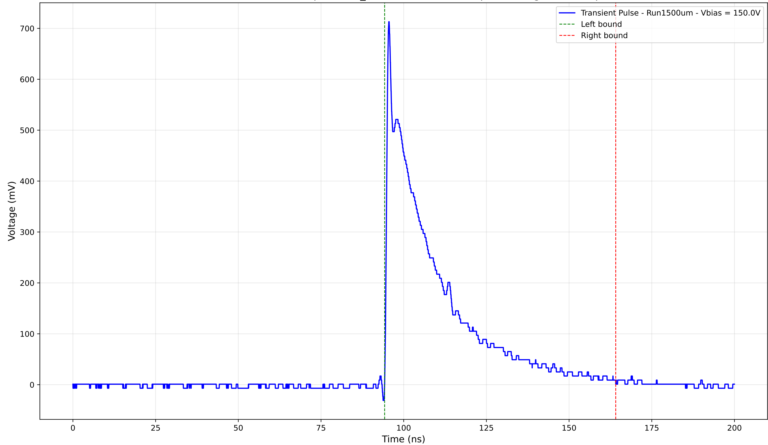
Transient Pulse - Sample: 1cm_42 - Position: 2245.0 \mu\text{m} - Charge: 192.13 pC
