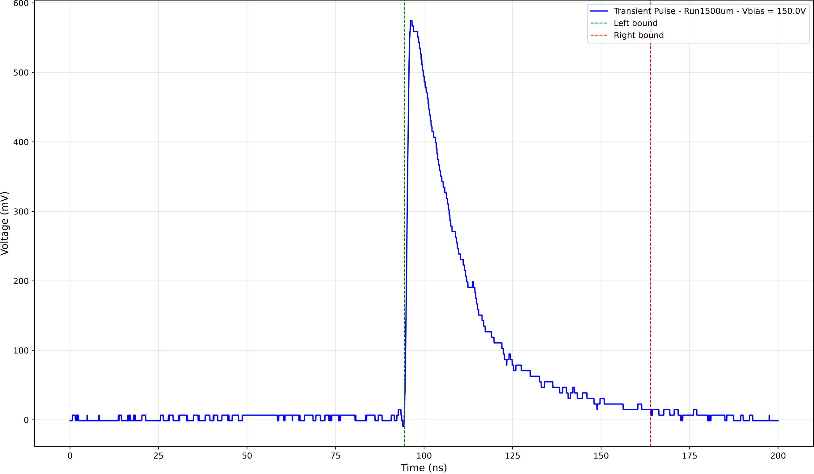
Transient Pulse - Sample: 1cm_42 - Position: 3535.0 \mu\text{m} - Charge: 196.96 pC
