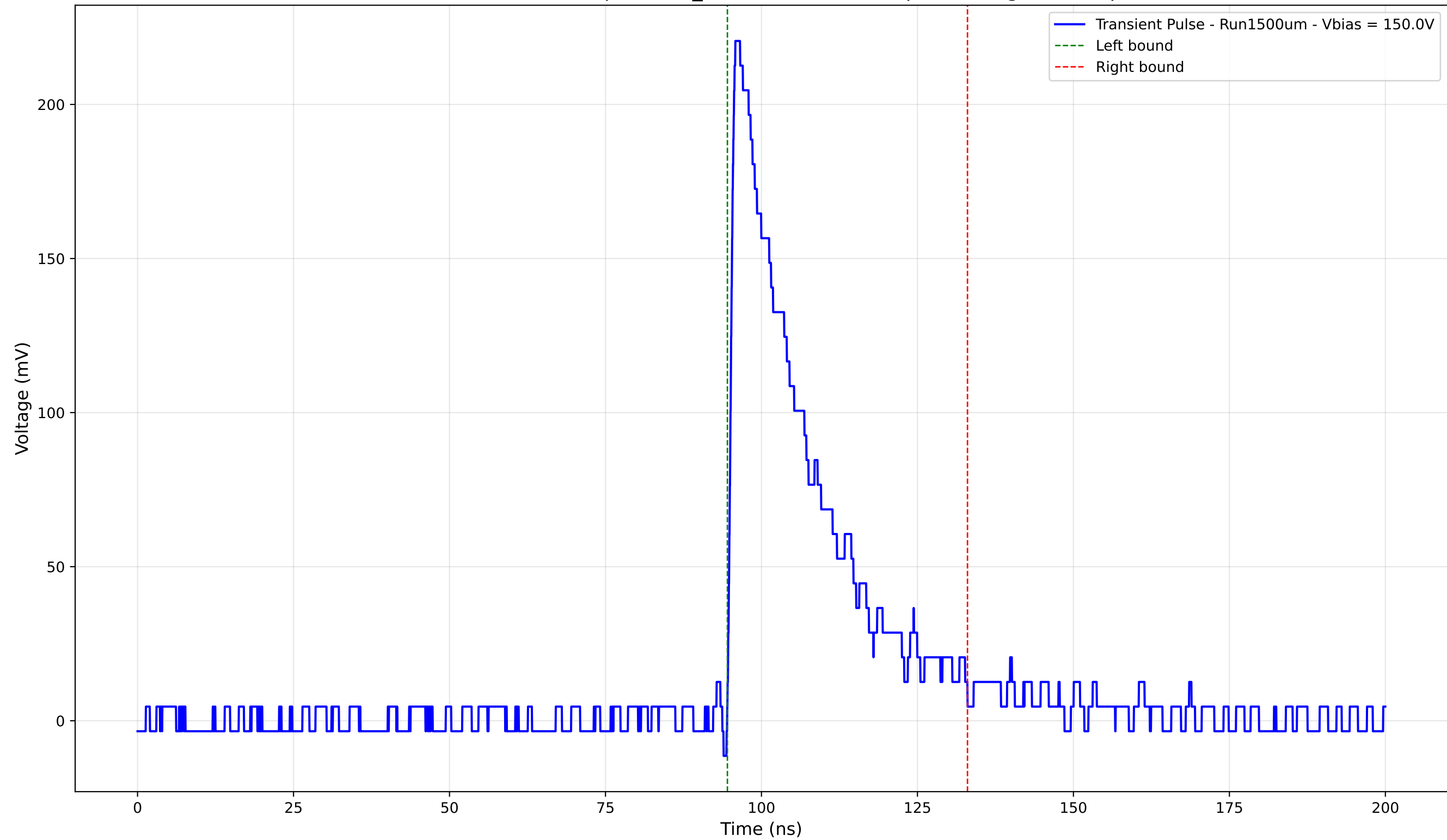
Transient Pulse - Sample: 1cm_42 - Position: 550.0 \mu\text{m} - Charge: 56.69 pC
