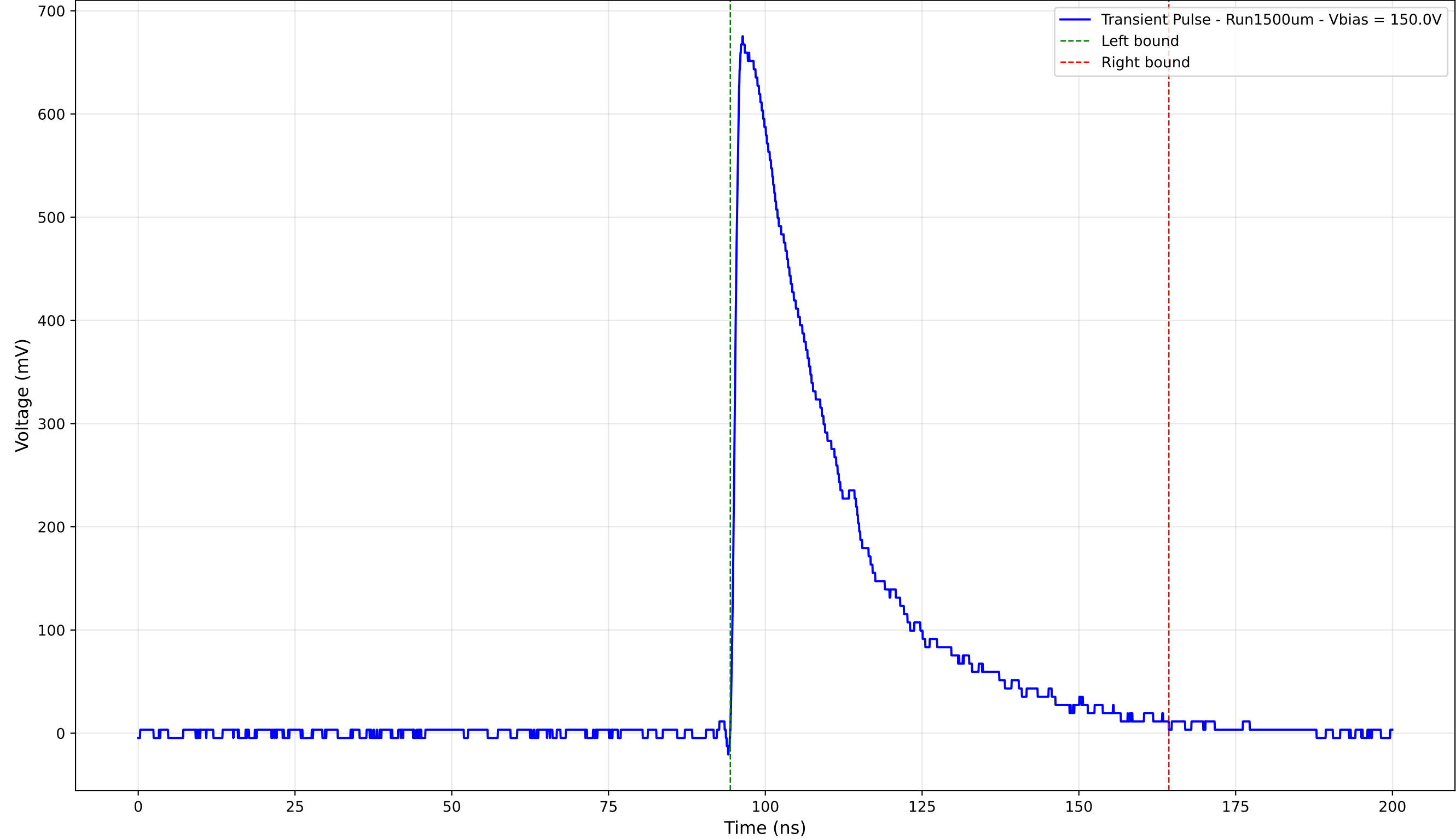
Transient Pulse - Sample: 1cm_42 - Position: 3485.0 \mu\text{m} - Charge: 230.75 pC
