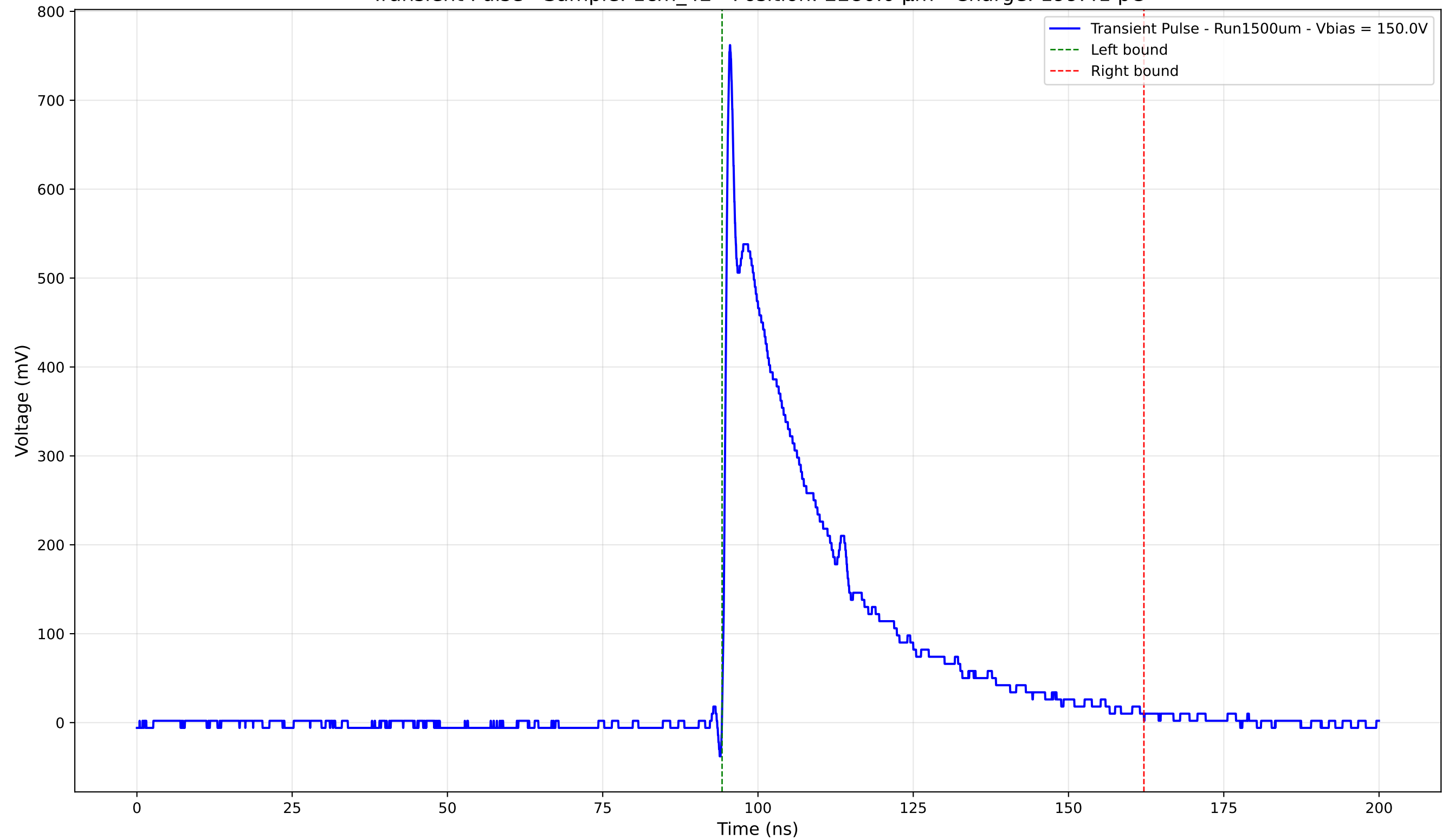
Transient Pulse - Sample: 1cm_42 - Position: 2280.0 \mu\text{m} - Charge: 199.41 pC
