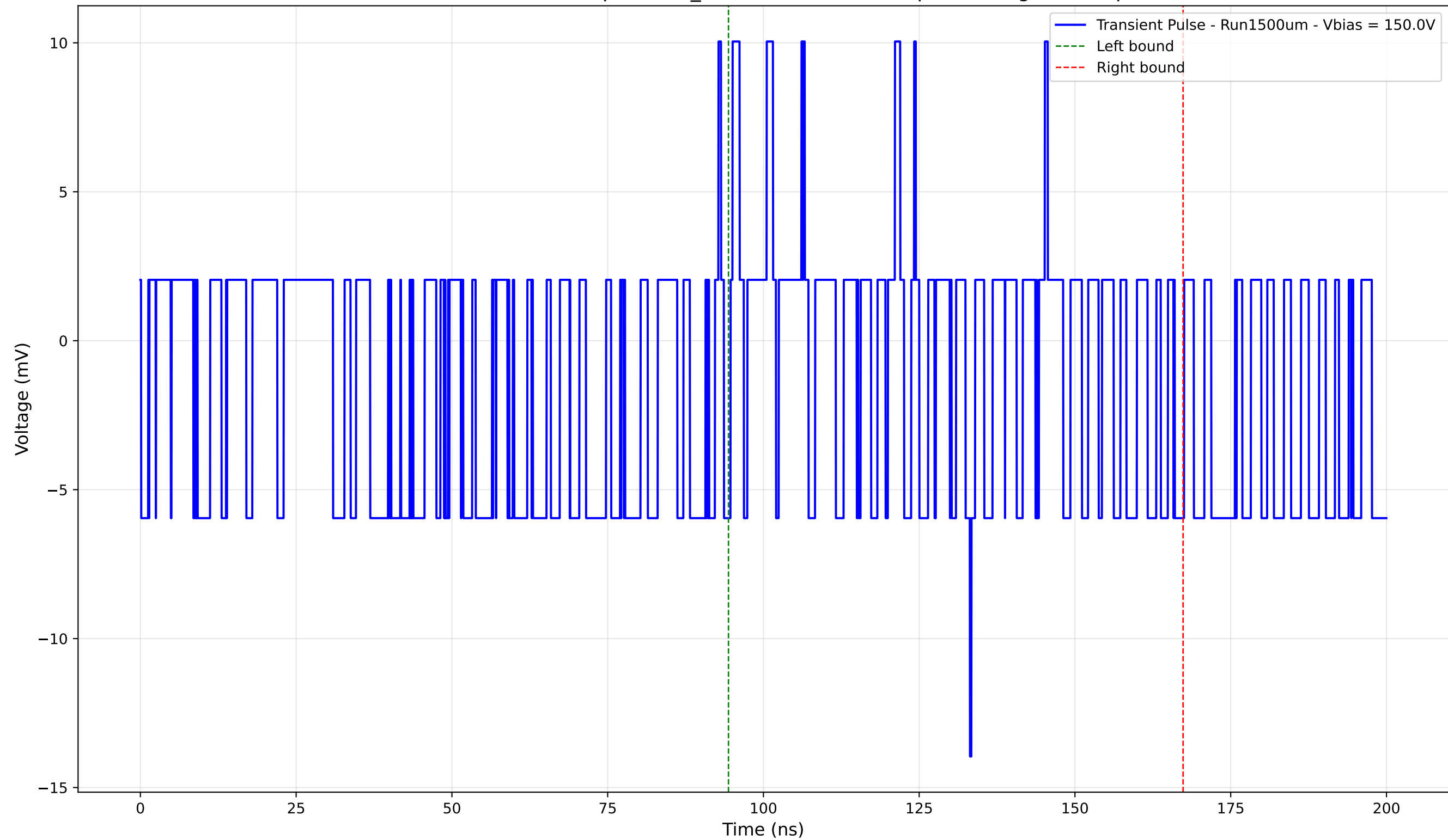
Transient Pulse - Sample: 1cm_42 - Position: 5035.0 \mu\text{m} - Charge: -0.06 pC
