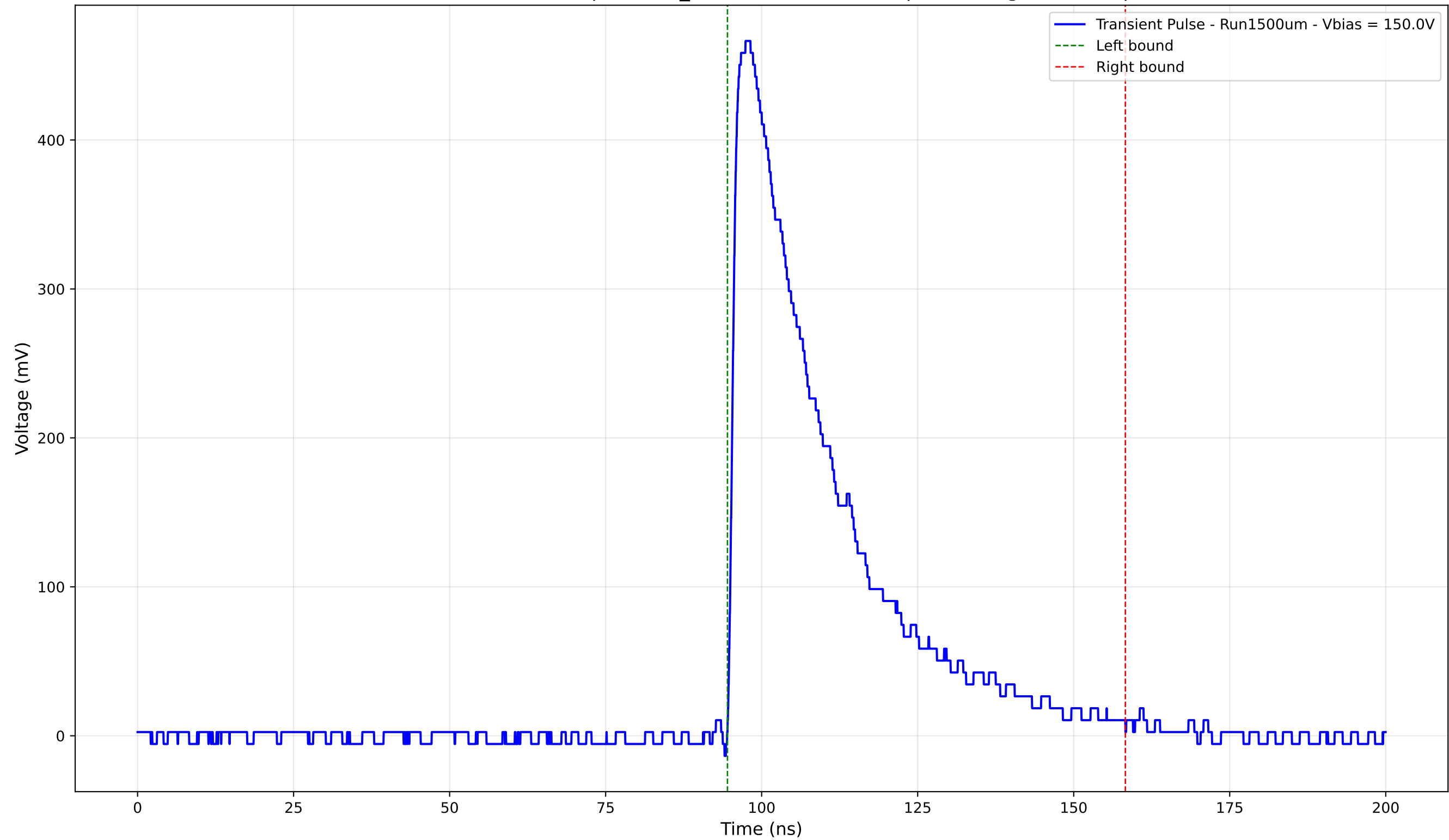
Transient Pulse - Sample: 1cm_42 - Position: 1510.0 \mu\text{m} - Charge: 156.13 pC
