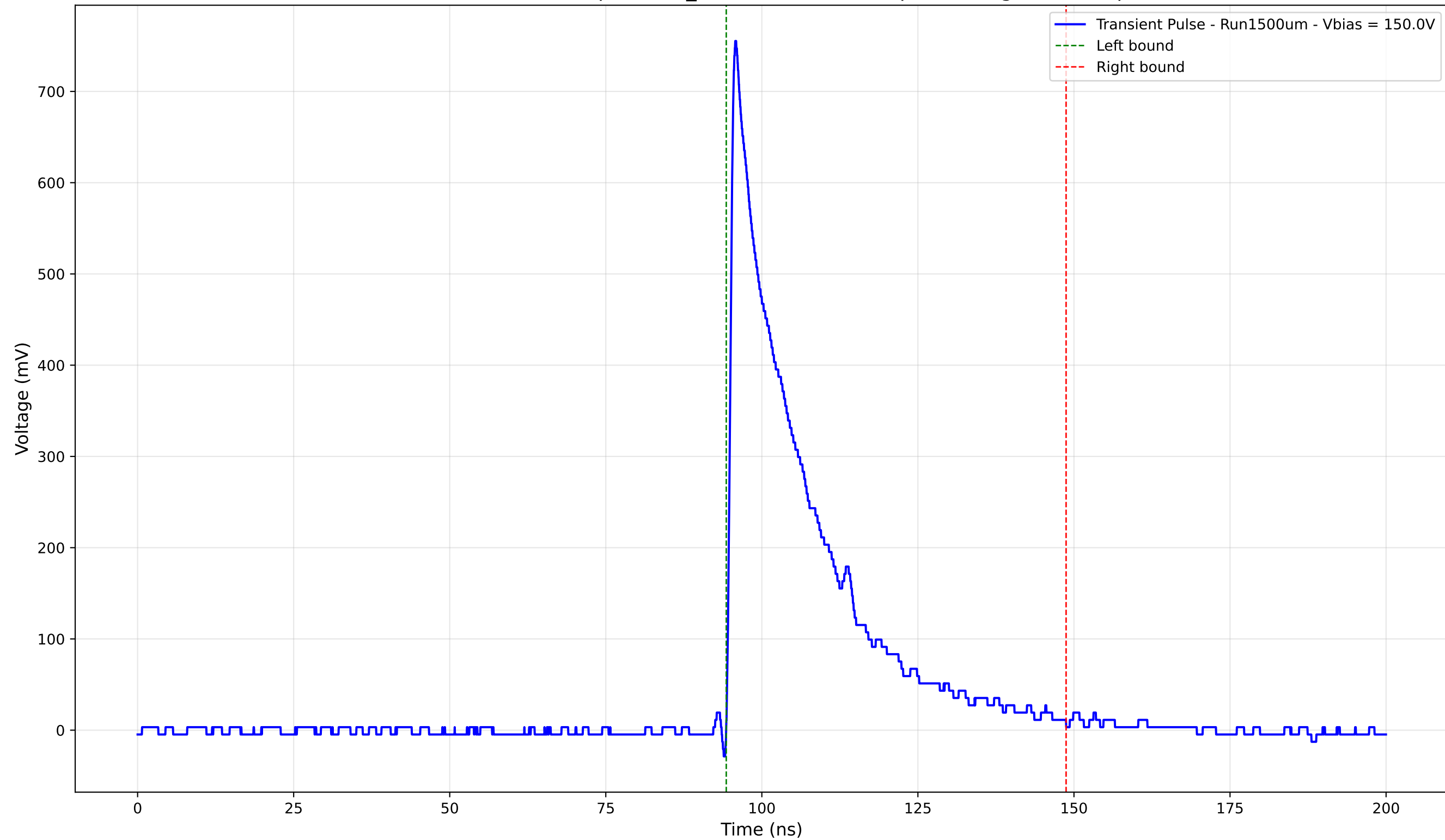
Transient Pulse - Sample: 1cm_42 - Position: 300.0 \mu\text{m} - Charge: 177.87 pC
