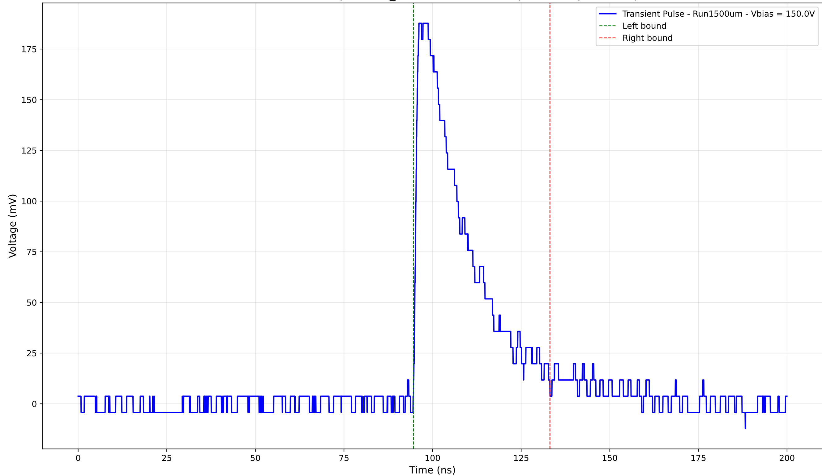
Transient Pulse - Sample: 1cm_42 - Position: 3645.0 \mu\text{m} - Charge: 58.79 pC
