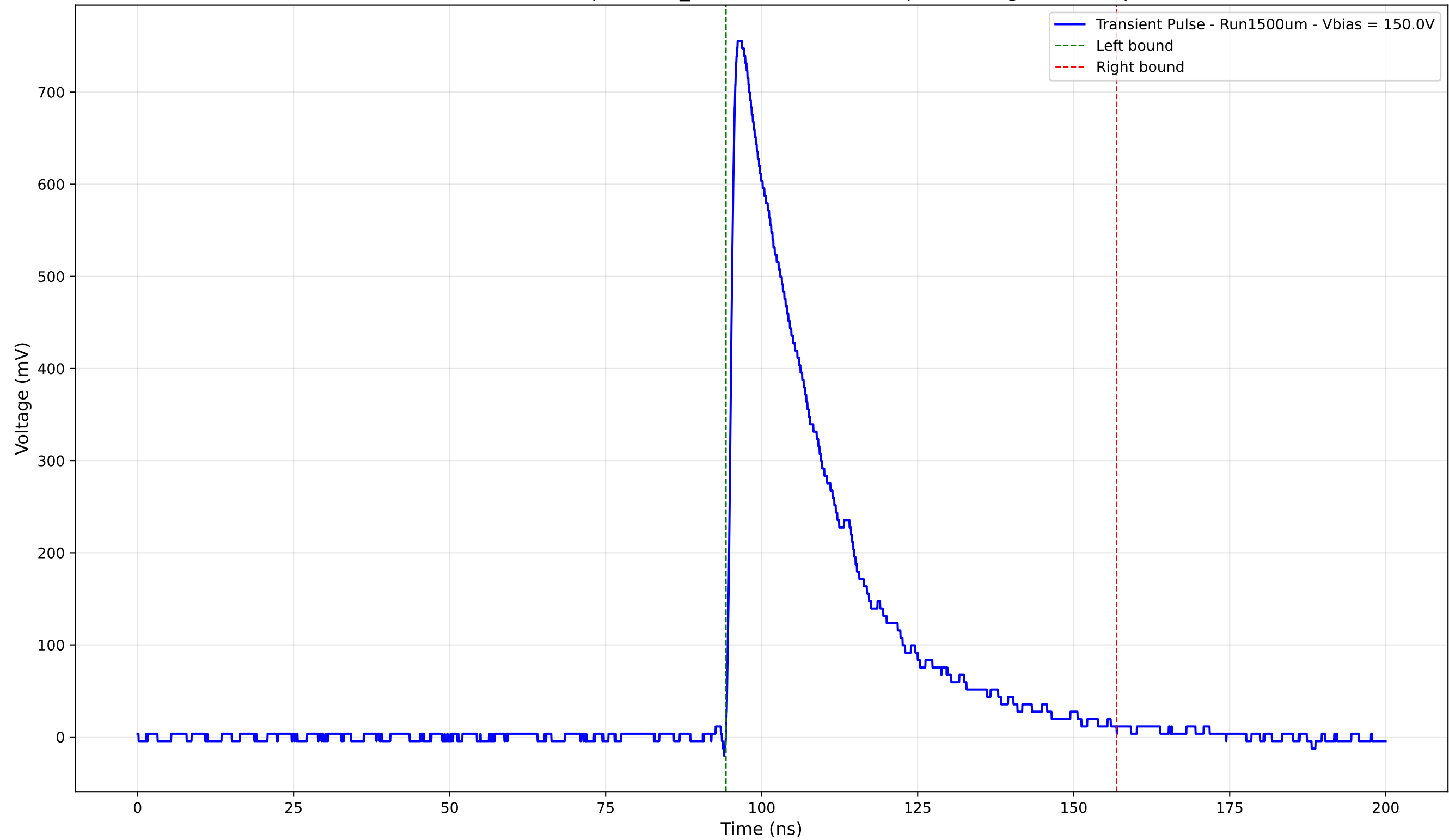
Transient Pulse - Sample: 1cm_42 - Position: 4385.0 \mu\text{m} - Charge: 233.73 pC
