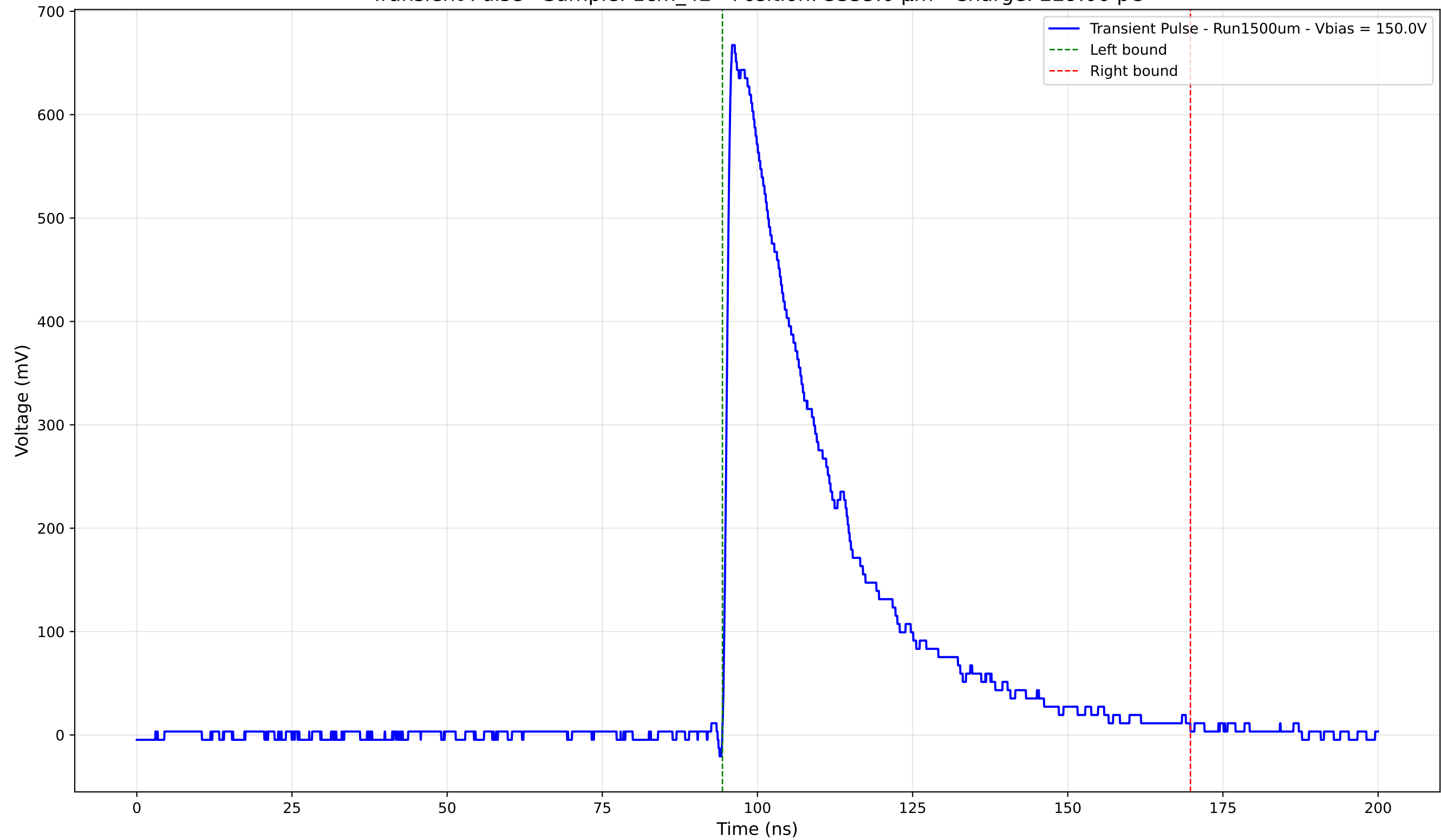
Transient Pulse - Sample: 1cm_42 - Position: 3355.0 \mu\text{m} - Charge: 229.06 pC
