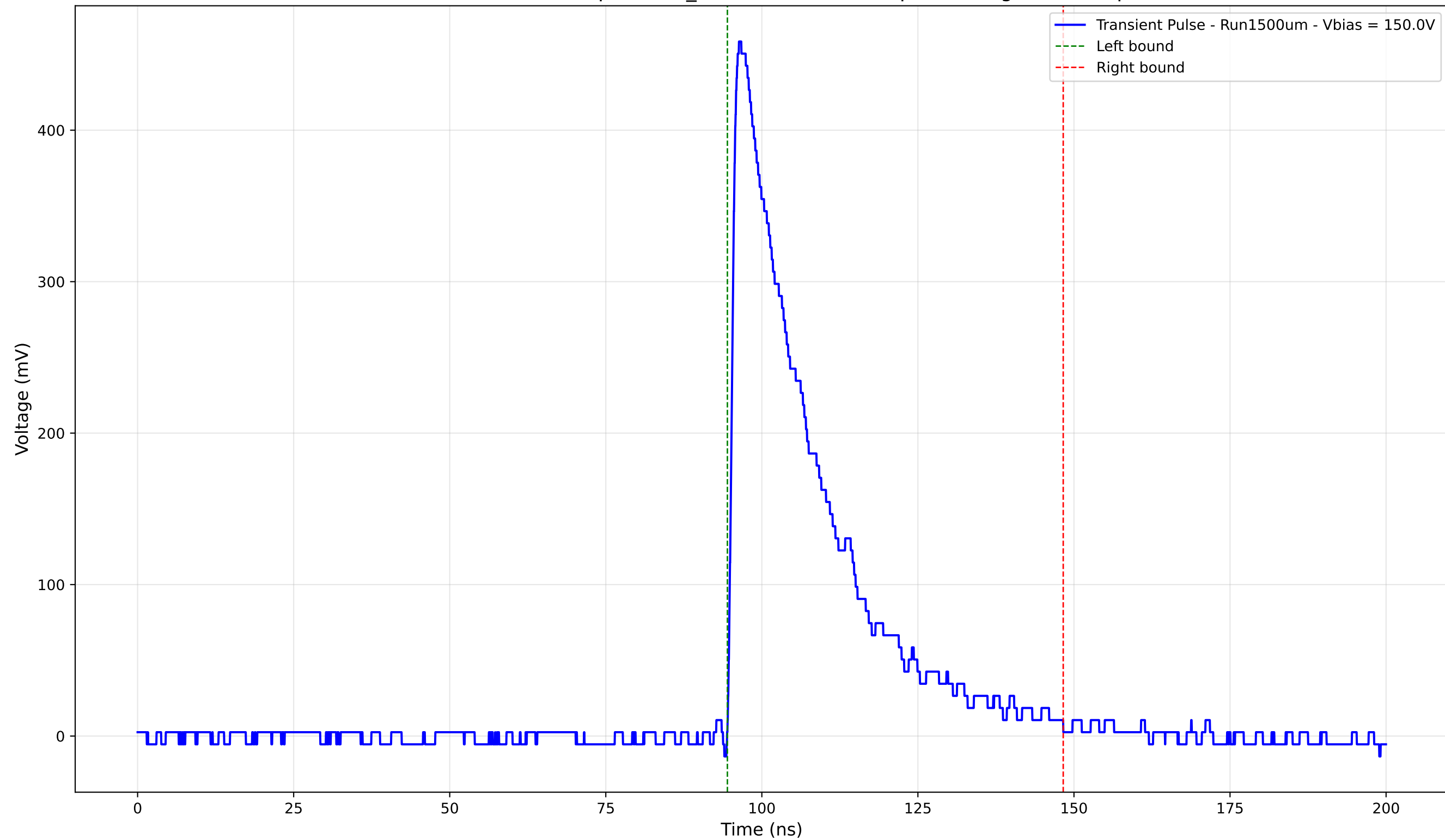
Transient Pulse - Sample: 1cm_42 - Position: 660.0 \mu\text{m} - Charge: 128.60 pC
