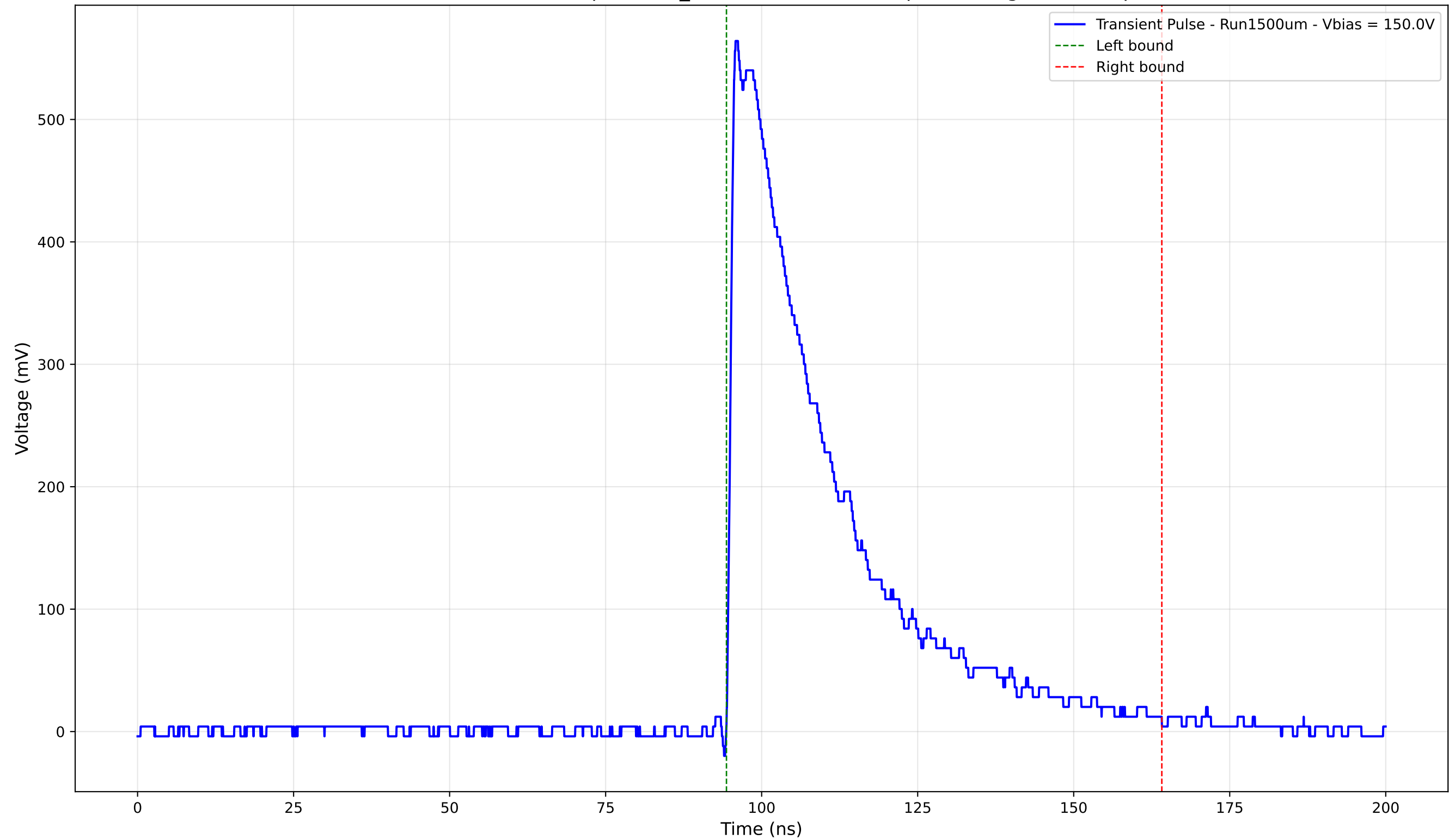
Transient Pulse - Sample: 1cm_42 - Position: 1900.0 \mu\text{m} - Charge: 195.78 pC
