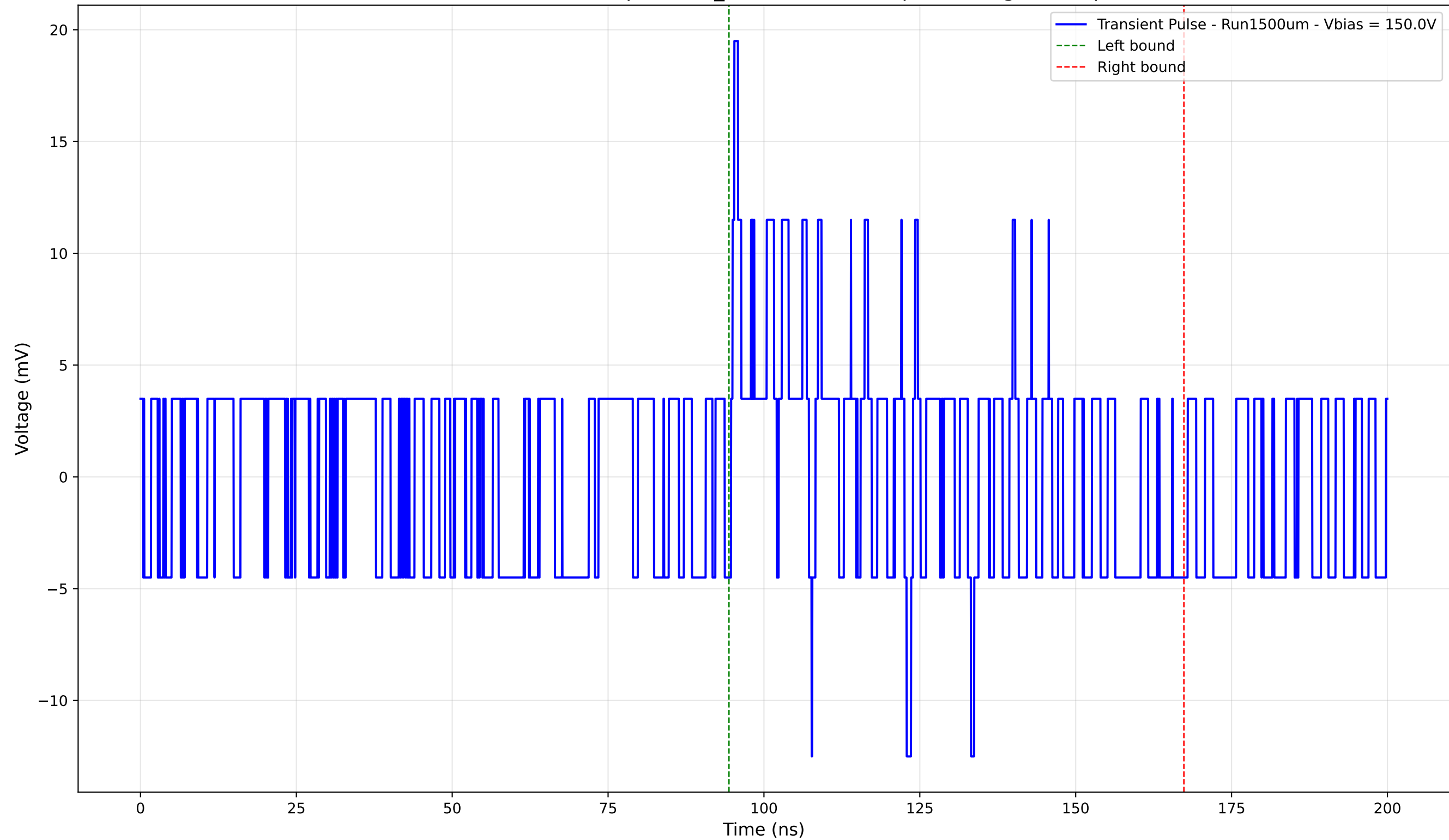
Transient Pulse - Sample: 1cm_42 - Position: 0.0 \mu\text{m} - Charge: 1.42 pC
