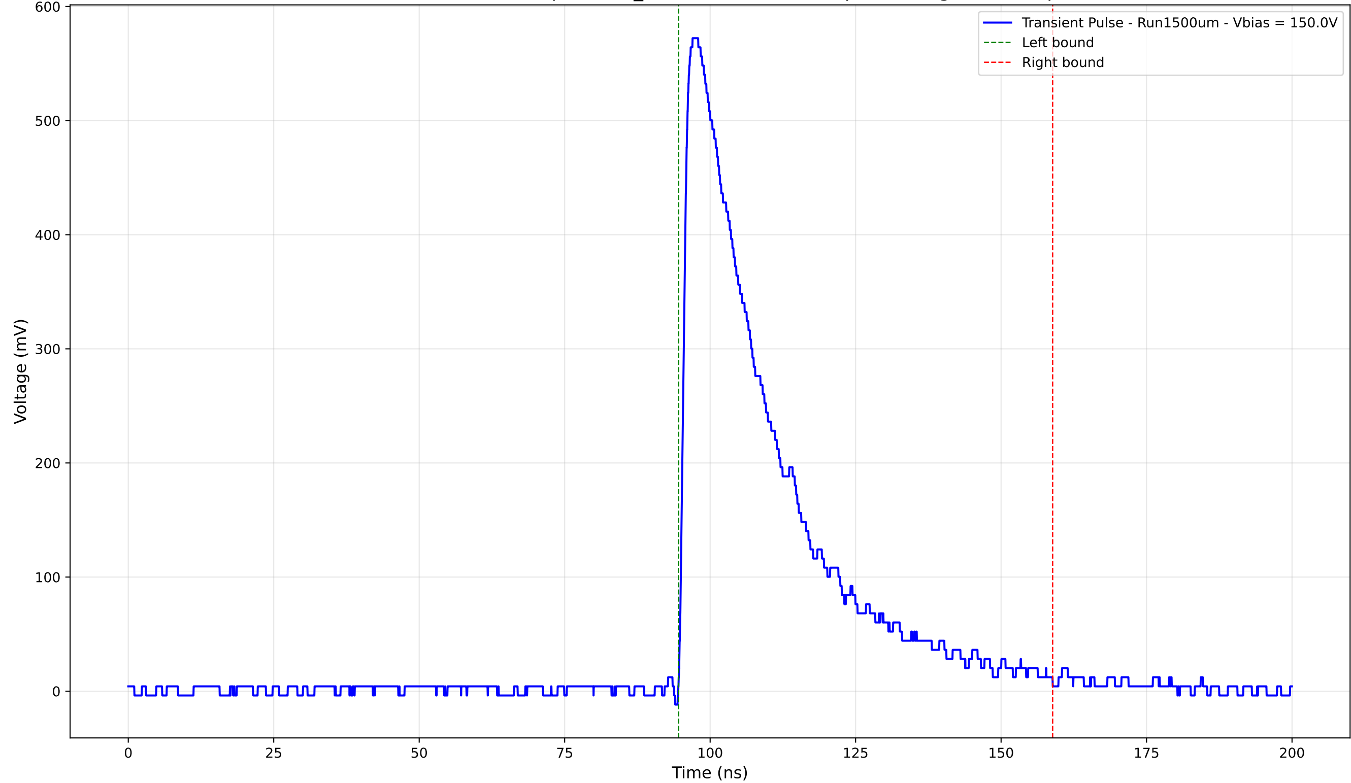
Transient Pulse - Sample: 1cm_42 - Position: 1345.0 \mu\text{m} - Charge: 190.88 pC
