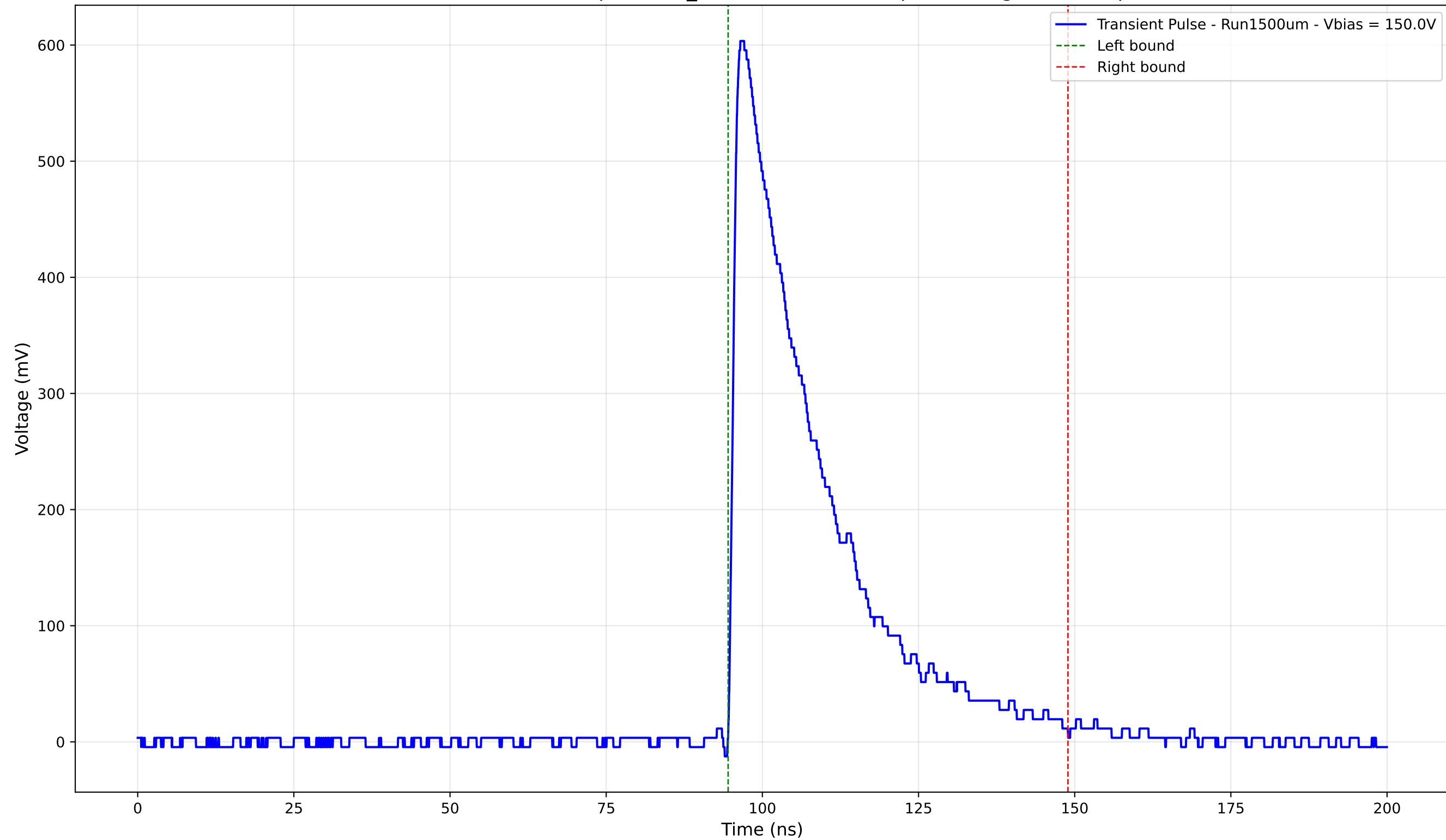
Transient Pulse - Sample: 1cm_42 - Position: 805.0 \mu\text{m} - Charge: 177.76 pC
