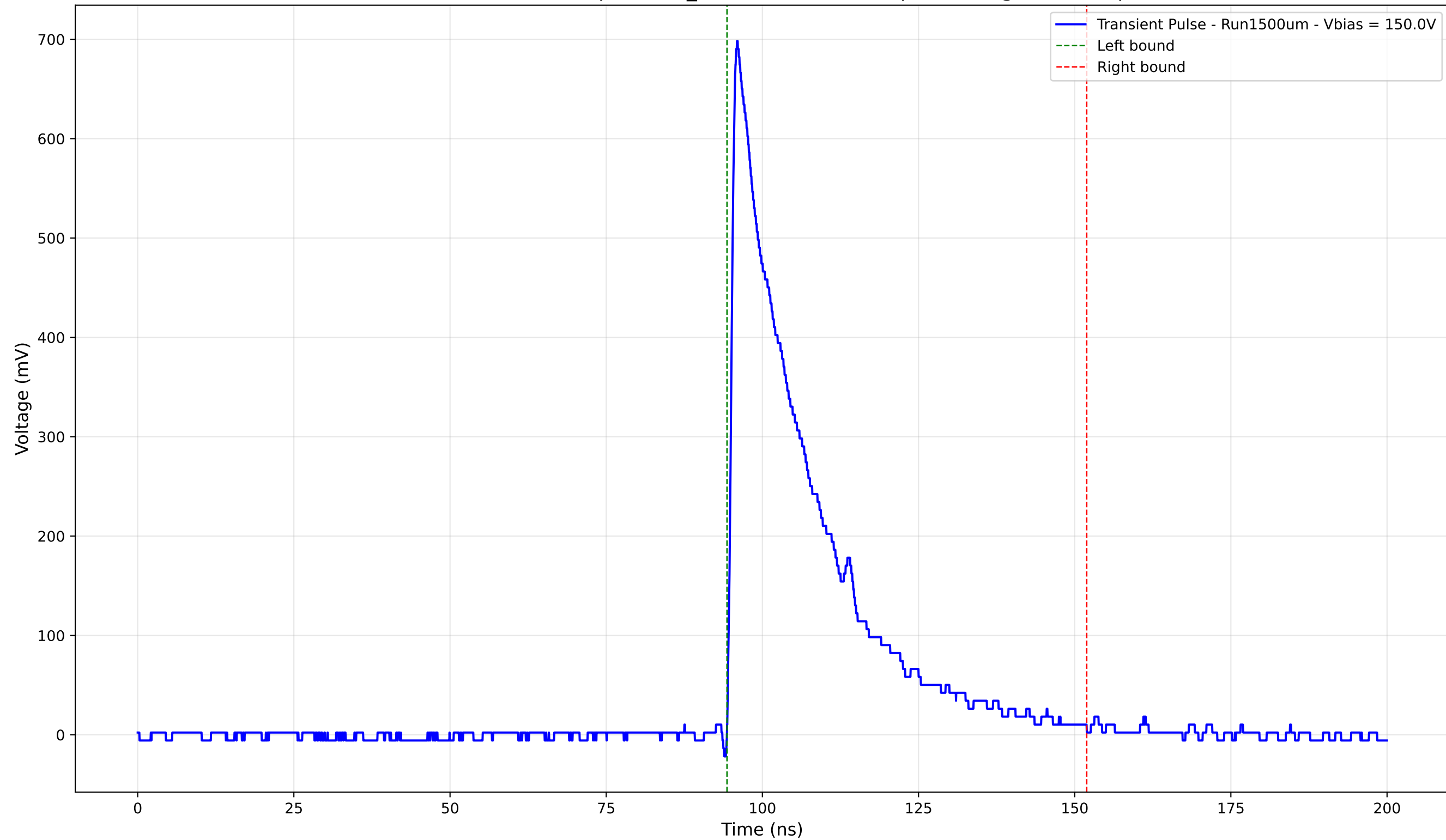
Transient Pulse - Sample: 1cm_42 - Position: 415.0 \mu\text{m} - Charge: 175.96 pC
