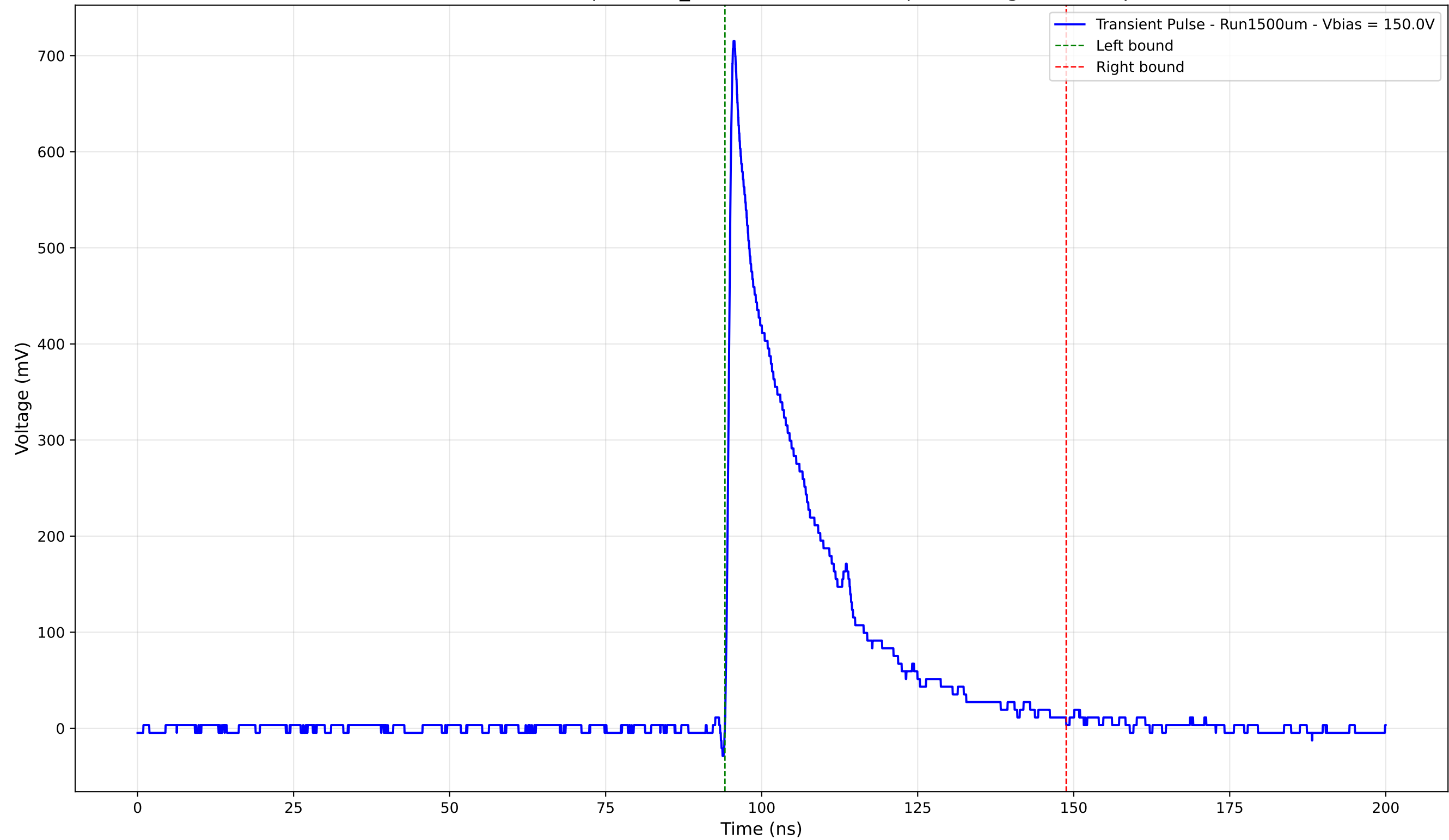
Transient Pulse - Sample: 1cm_42 - Position: 4865.0 \mu\text{m} - Charge: 164.13 pC
