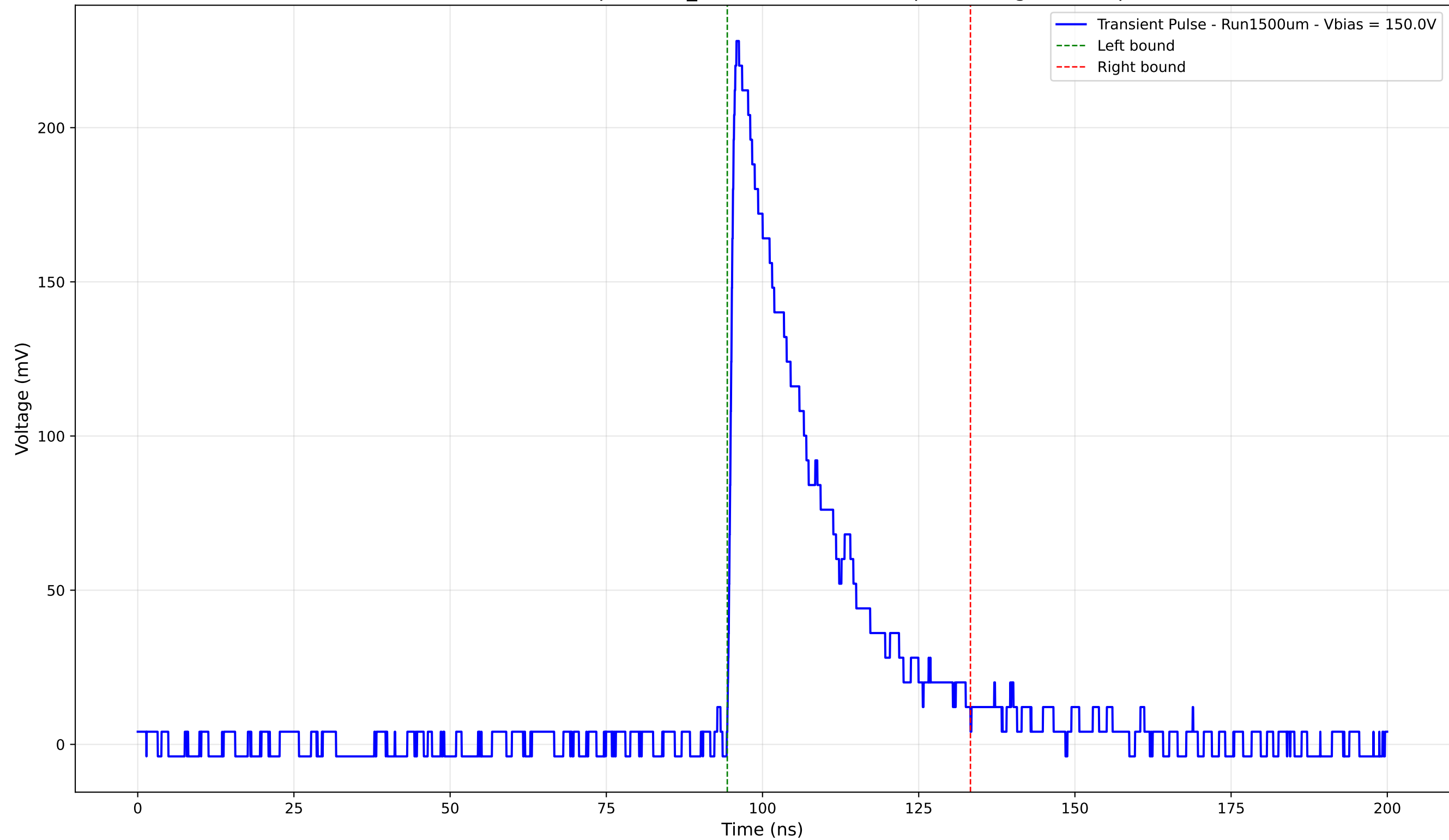
Transient Pulse - Sample: 1cm_42 - Position: 4600.0 \mu\text{m} - Charge: 60.58 pC
