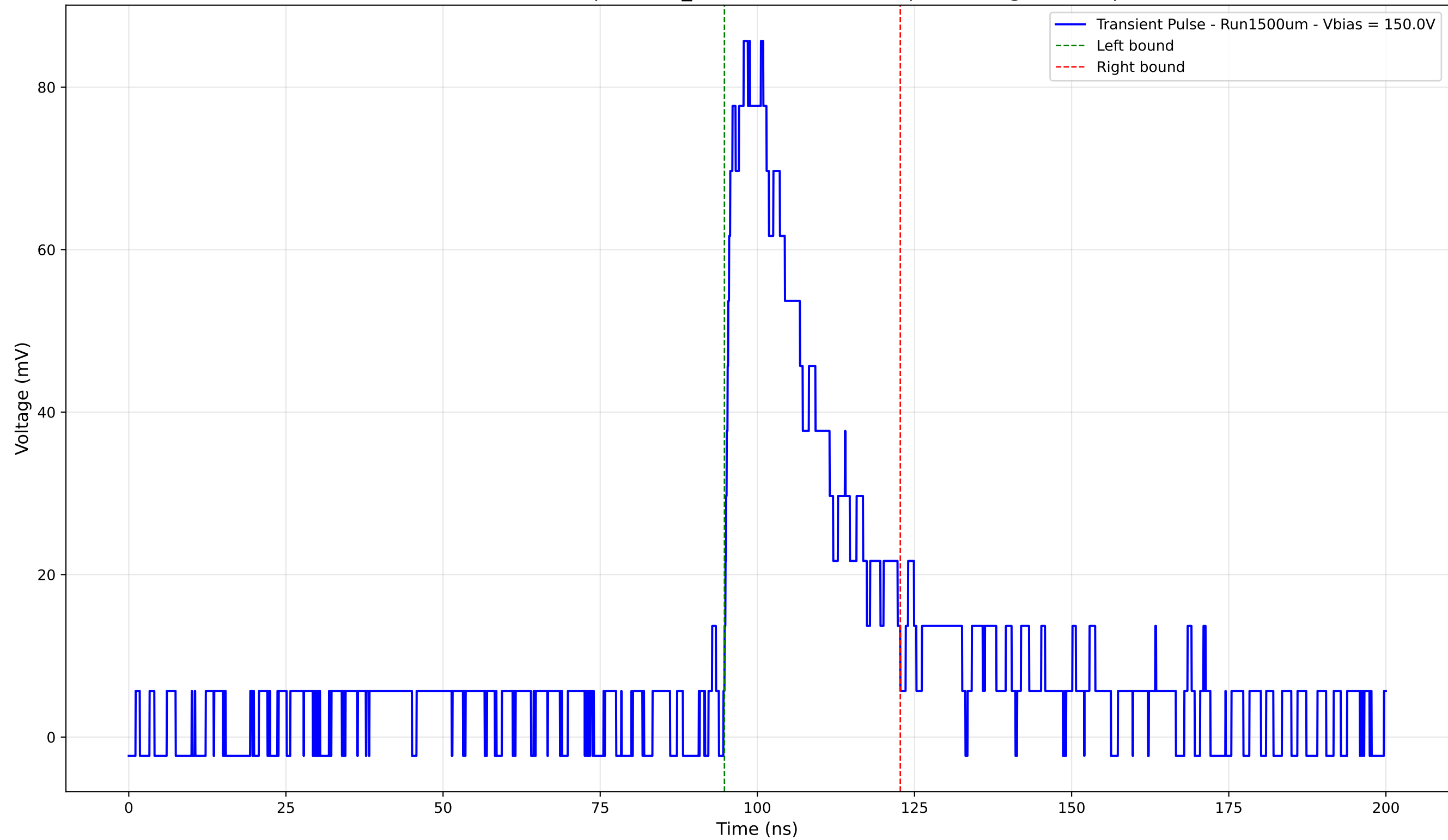
Transient Pulse - Sample: 1cm_42 - Position: 1595.0 \mu\text{m} - Charge: 25.15 pC
