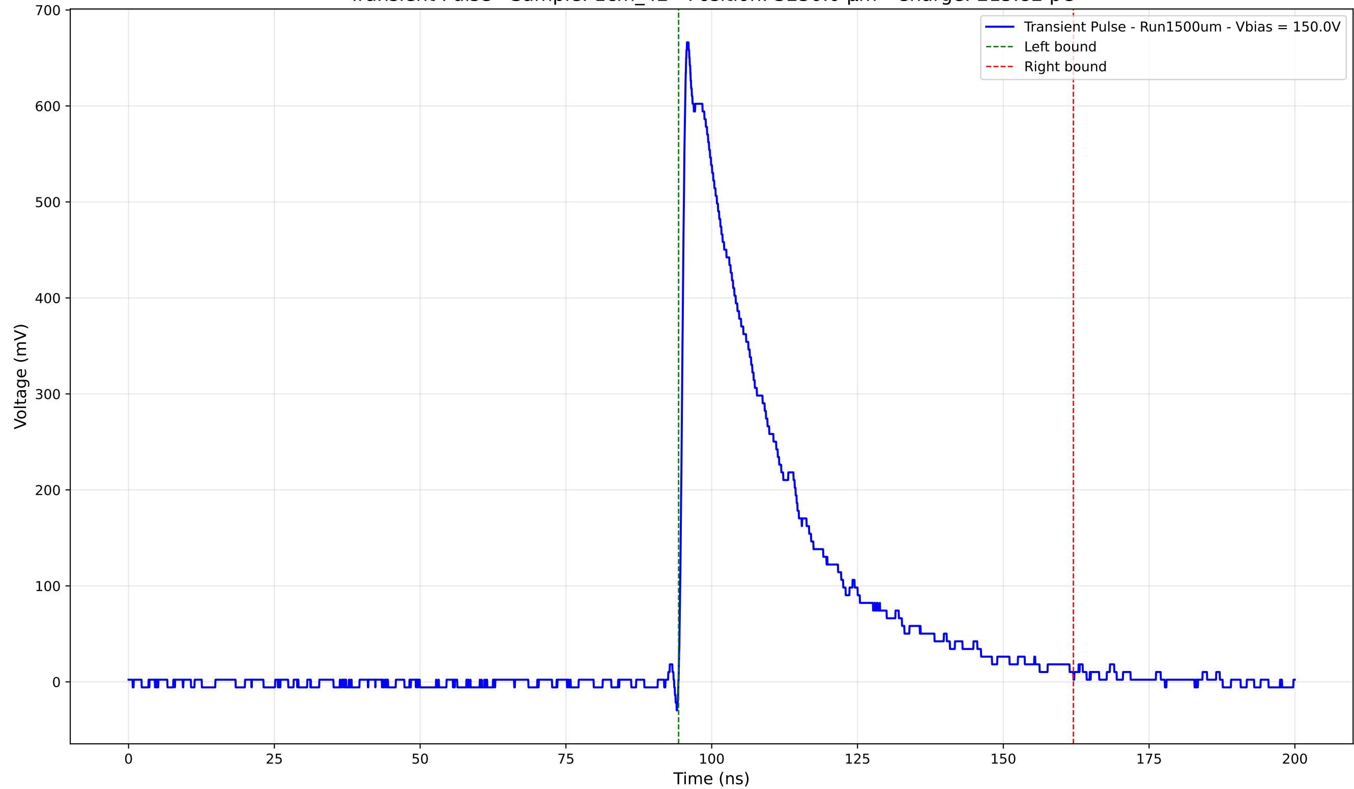
Transient Pulse - Sample: 1cm_42 - Position: 3230.0 \mu\text{m} - Charge: 215.82 pC
