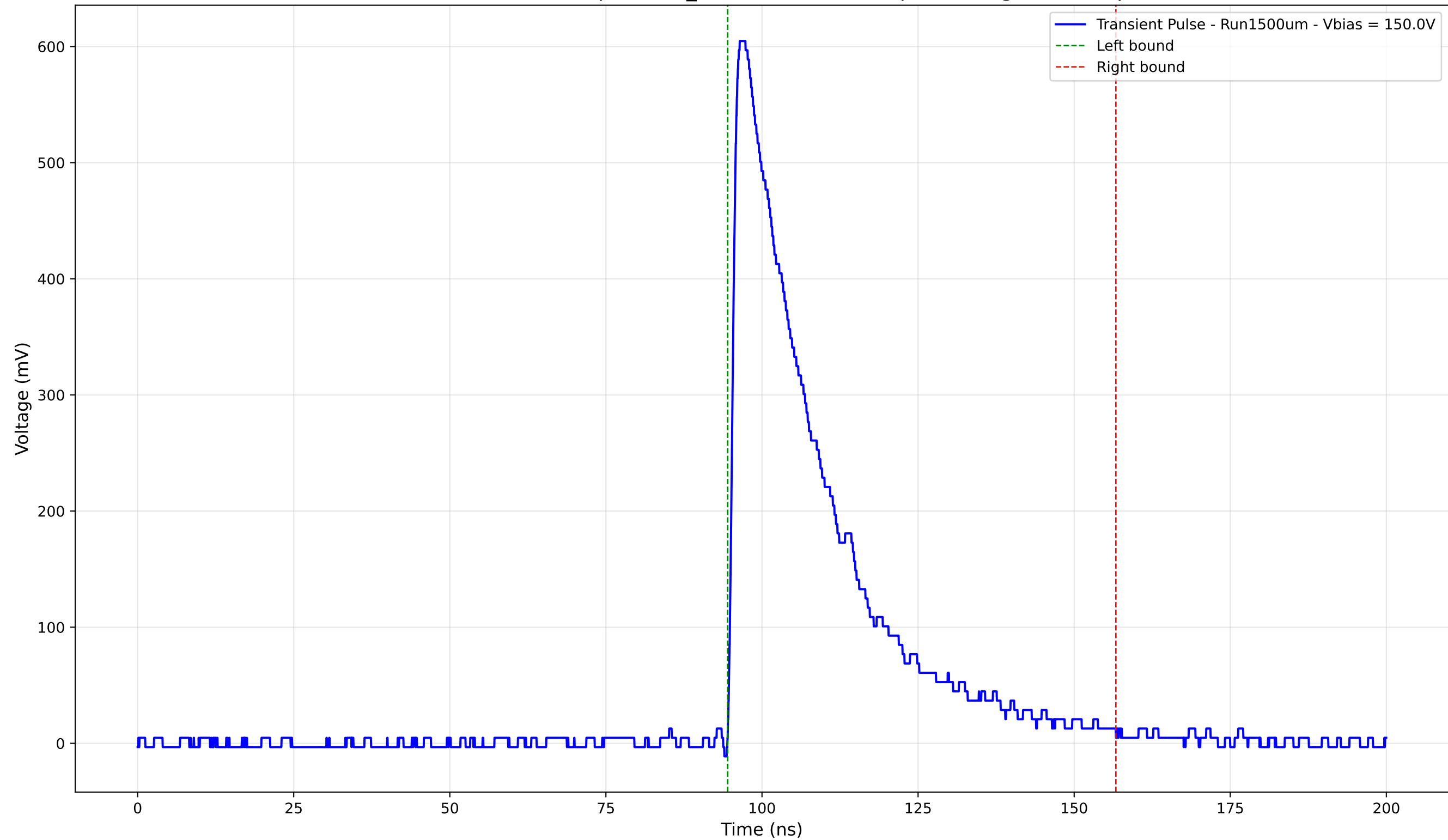
Transient Pulse - Sample: 1cm_42 - Position: 795.0 \mu\text{m} - Charge: 182.63 pC
