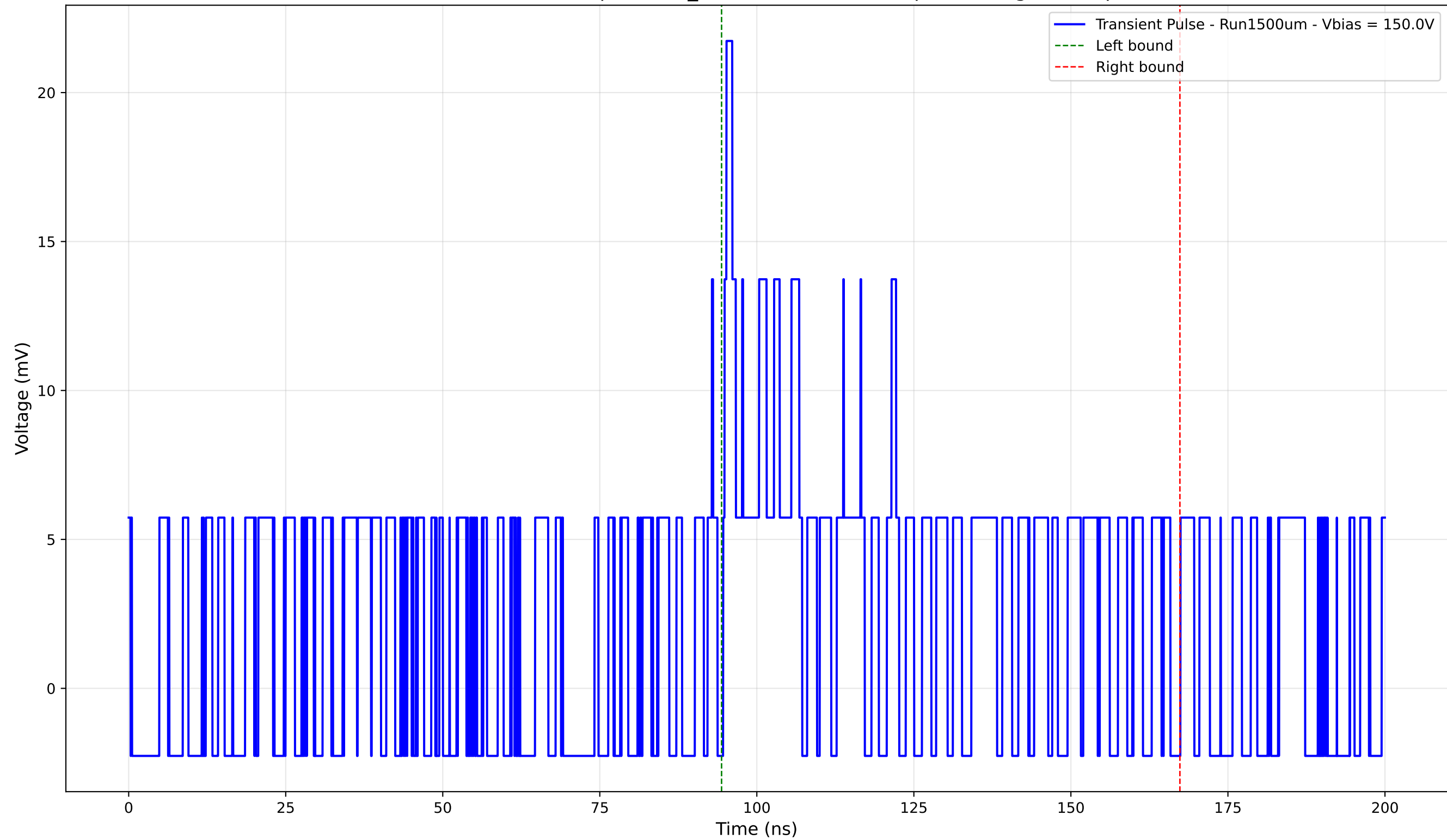
Transient Pulse - Sample: 1cm_42 - Position: 4985.0 \mu\text{m} - Charge: 6.17 pC
