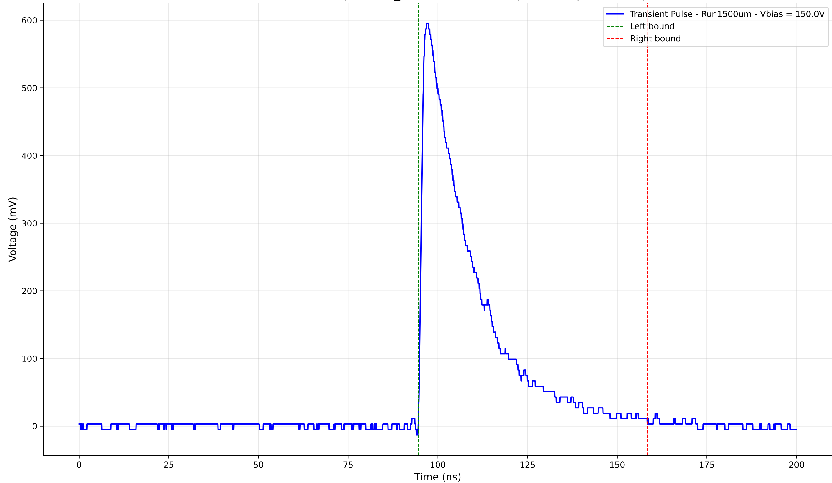
Transient Pulse - Sample: 1cm_42 - Position: 935.0 \mu\text{m} - Charge: 182.79 pC
