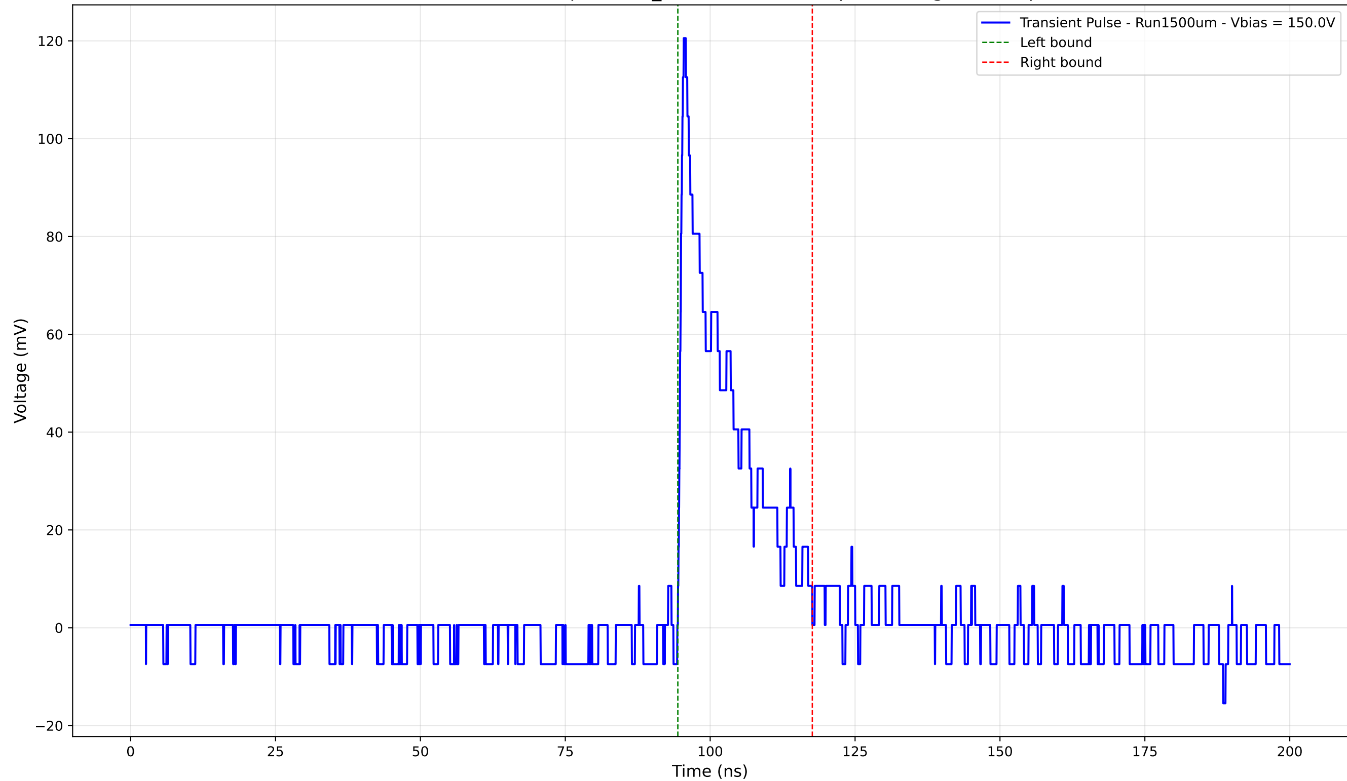
Transient Pulse - Sample: 1cm_42 - Position: 95.0 \mu\text{m} - Charge: 19.74 pC
