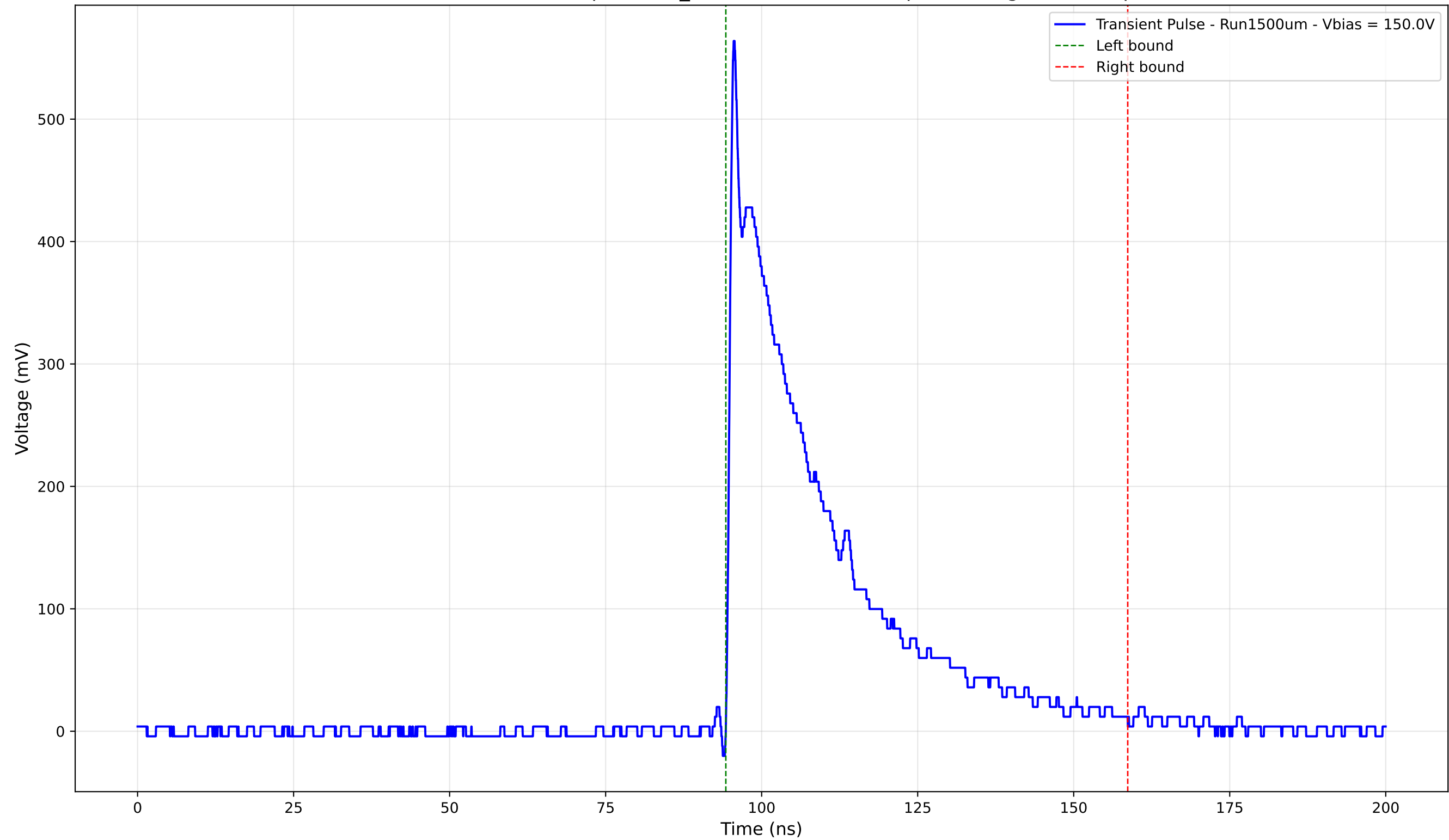
Transient Pulse - Sample: 1cm_42 - Position: 2185.0 \mu\text{m} - Charge: 156.51 pC
