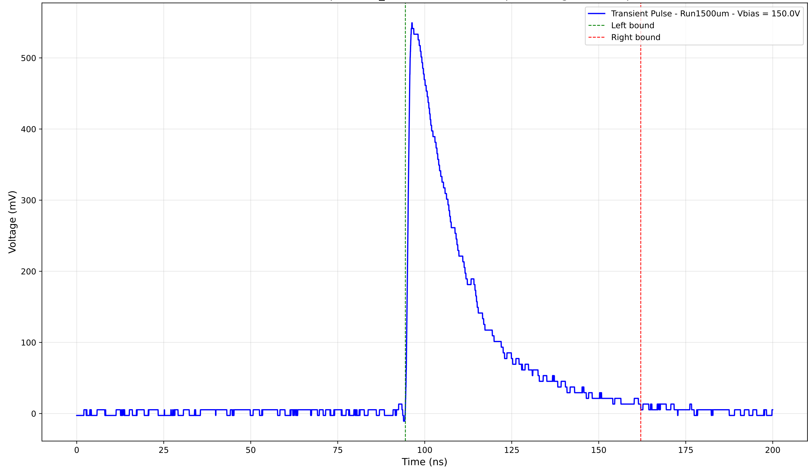
Transient Pulse - Sample: 1cm_42 - Position: 3540.0 \mu\text{m} - Charge: 185.64 pC
