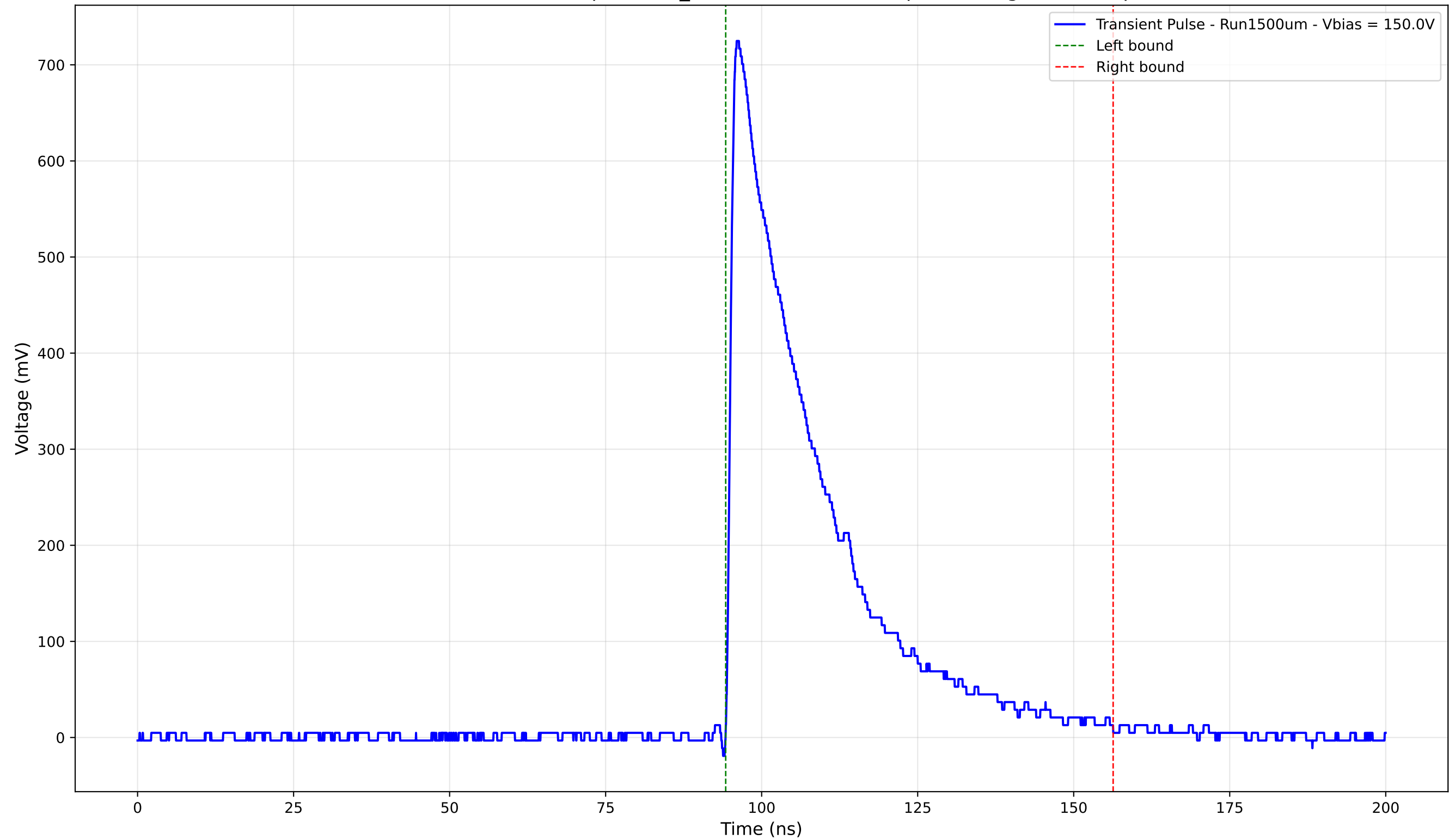
Transient Pulse - Sample: 1cm_42 - Position: 4510.0 \mu\text{m} - Charge: 213.83 pC
