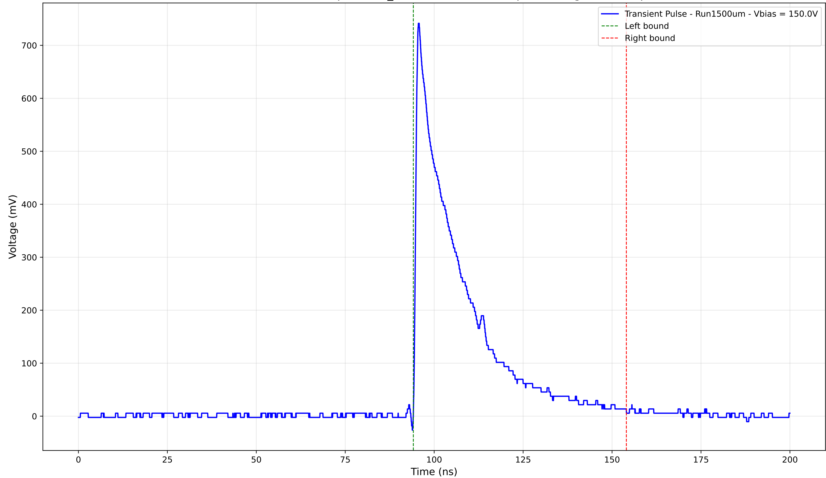
Transient Pulse - Sample: 1cm_42 - Position: 4790.0 \mu\text{m} - Charge: 188.08 pC
