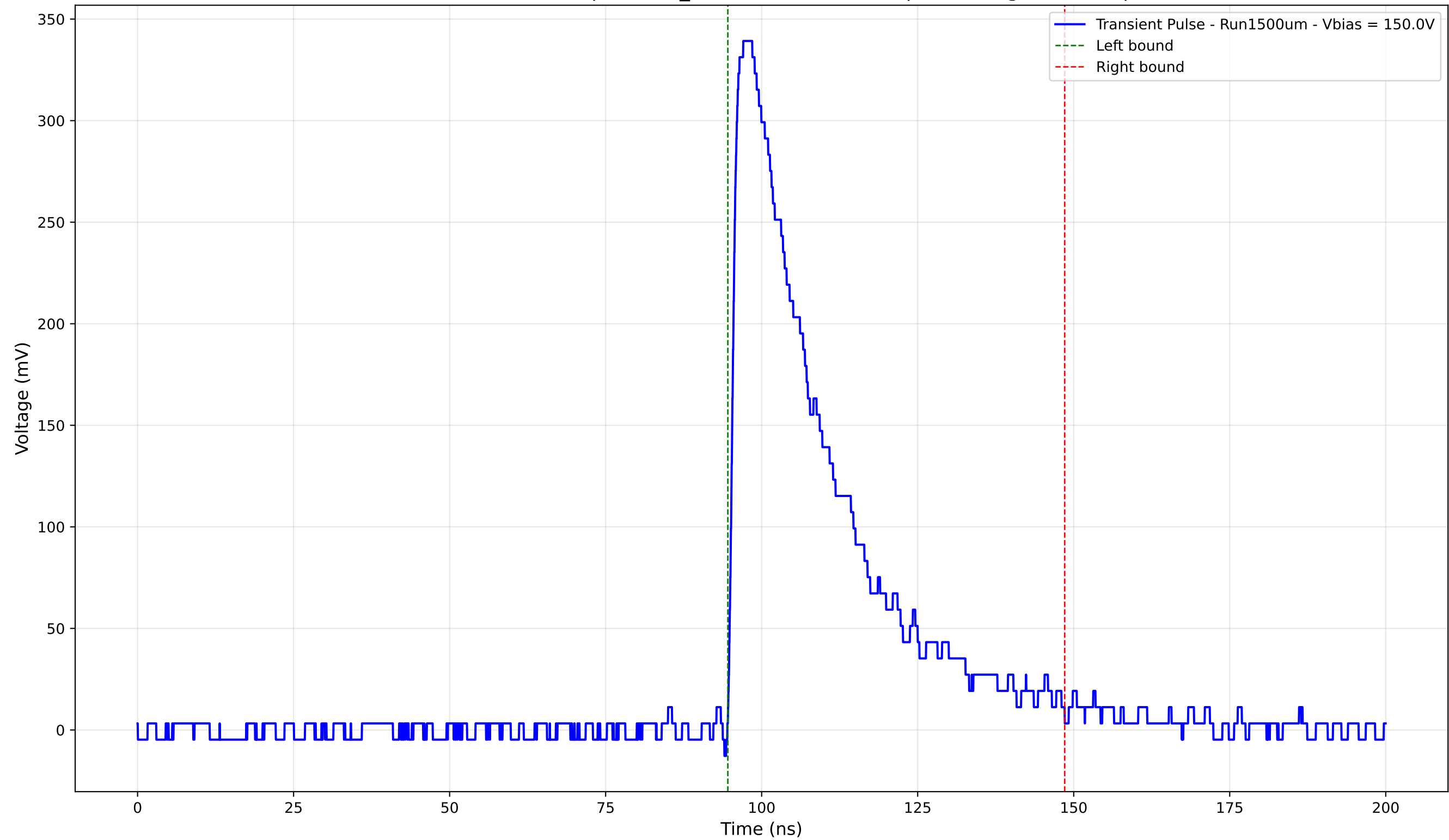
Transient Pulse - Sample: 1cm_42 - Position: 1535.0 \mu\text{m} - Charge: 111.06 pC
