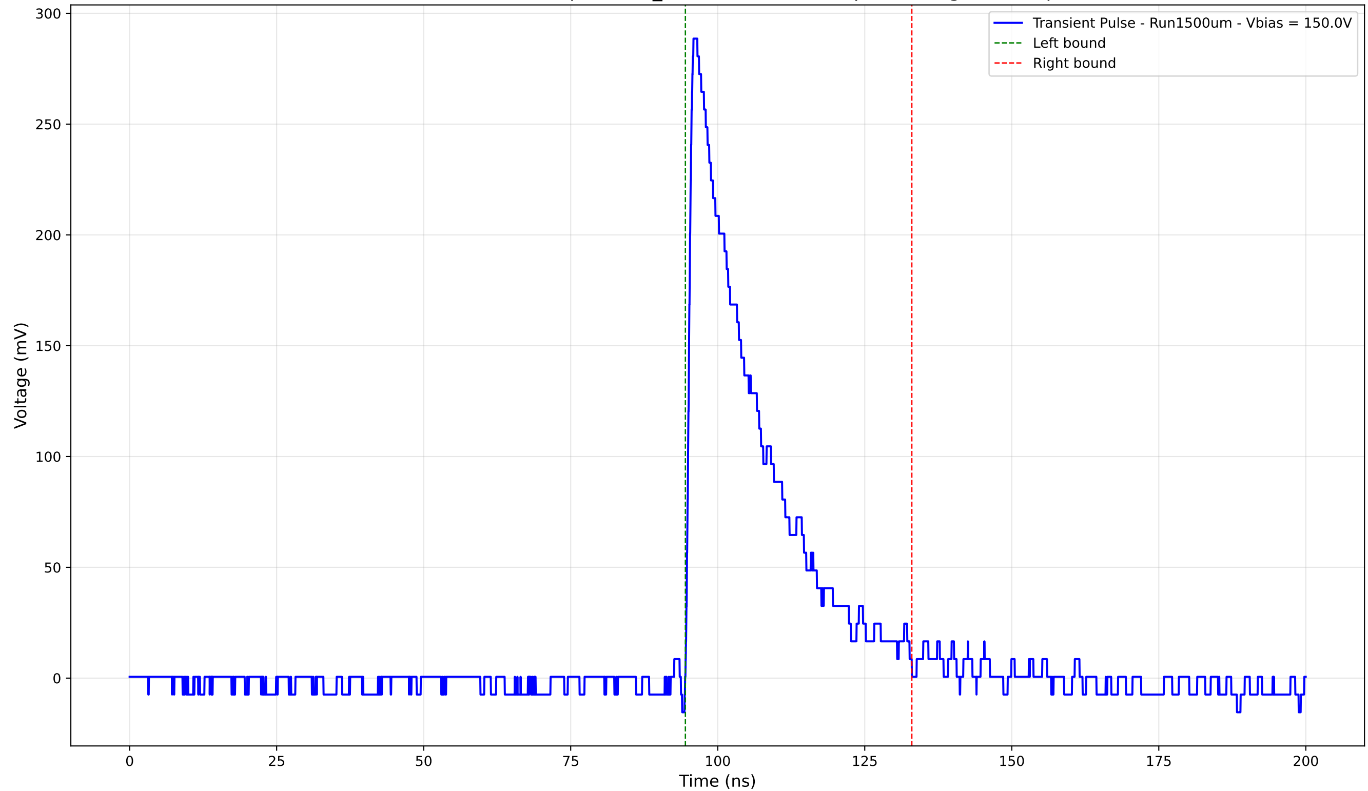
Transient Pulse - Sample: 1cm_42 - Position: 540.0 \mu\text{m} - Charge: 70.57 pC
