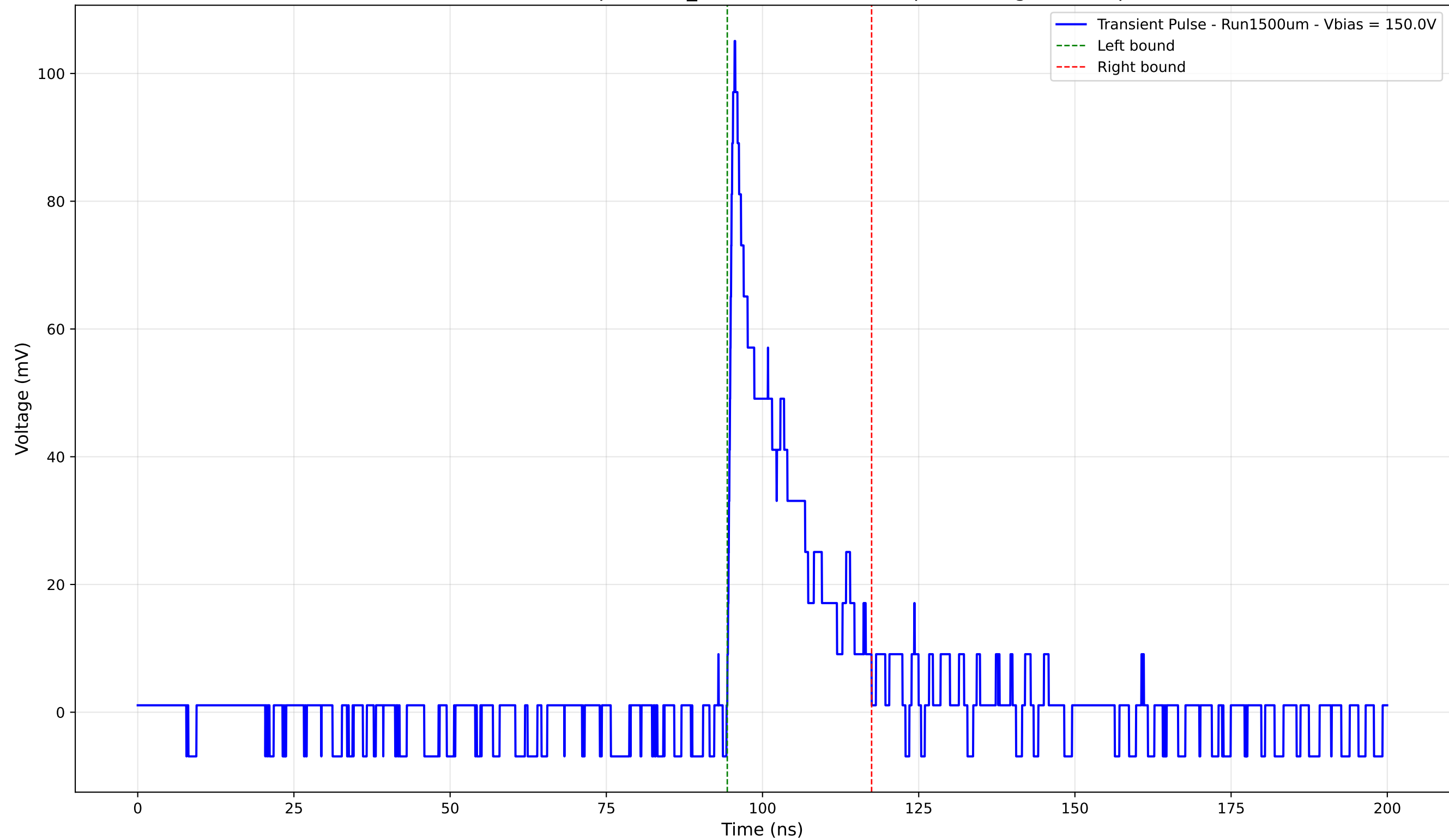
Transient Pulse - Sample: 1cm_42 - Position: 4945.0 \mu\text{m} - Charge: 16.22 pC
