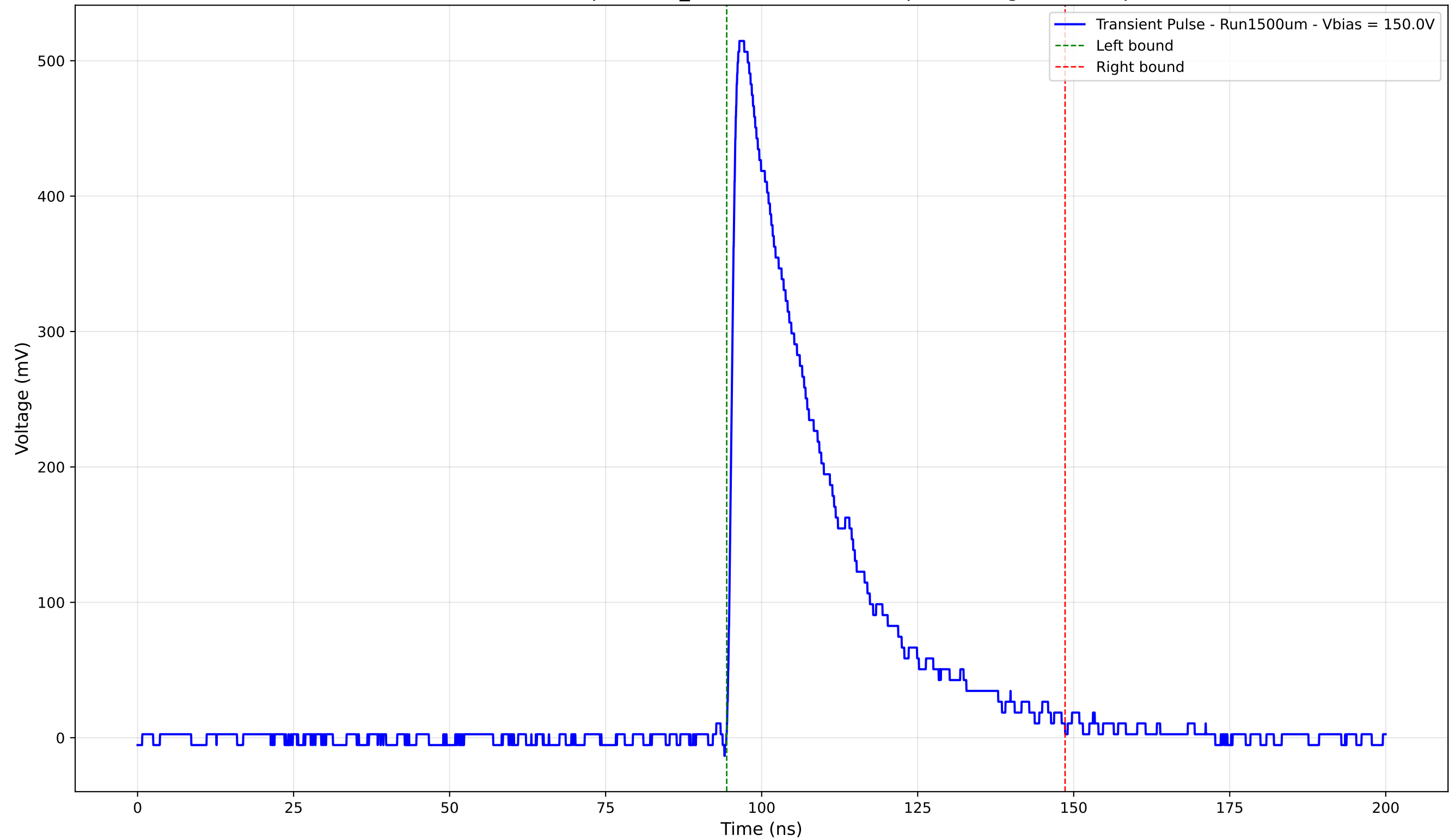
Transient Pulse - Sample: 1cm_42 - Position: 4190.0 \mu\text{m} - Charge: 157.05 pC
