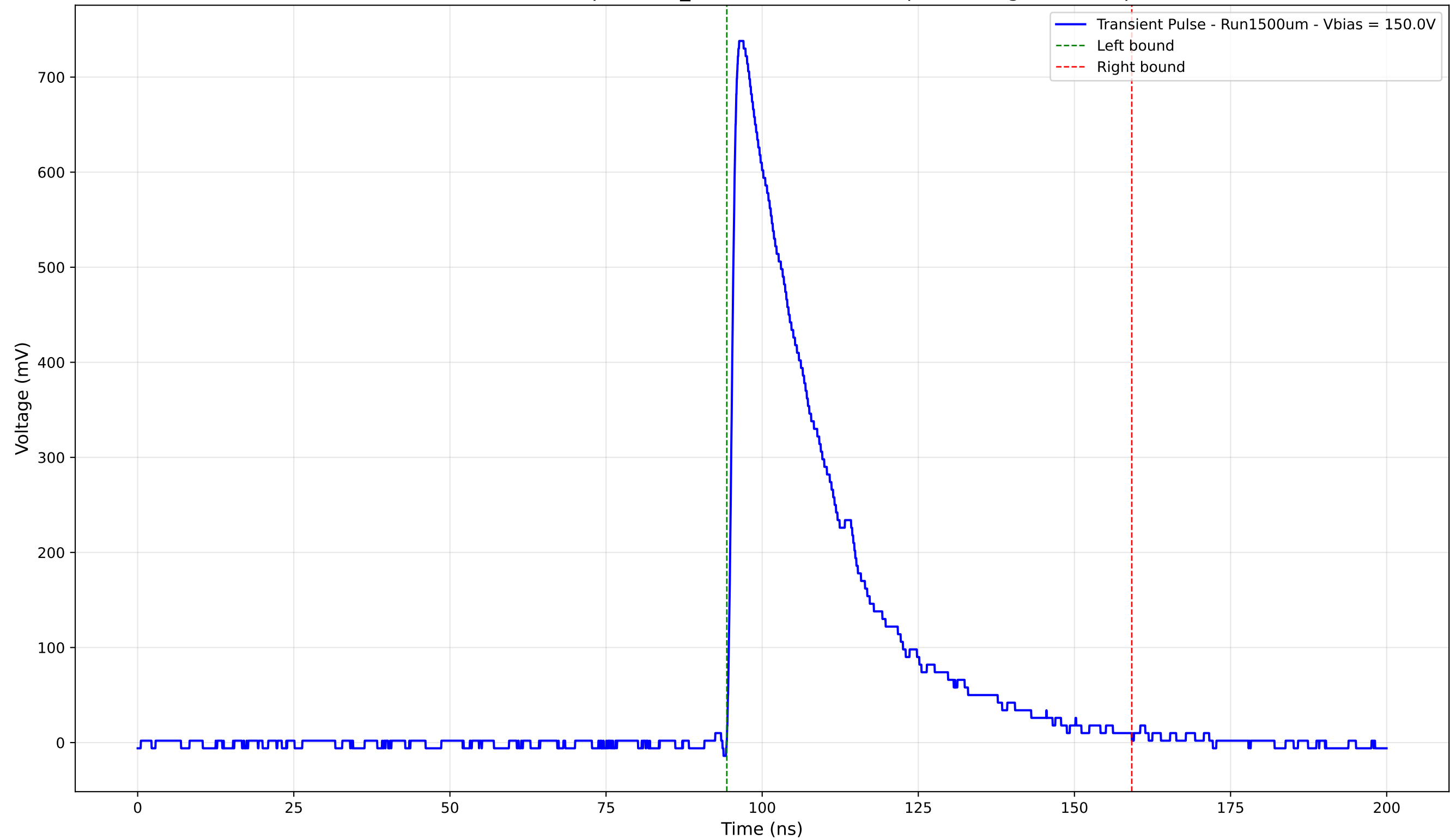
Transient Pulse - Sample: 1cm_42 - Position: 4275.0 \mu\text{m} - Charge: 230.55 pC
