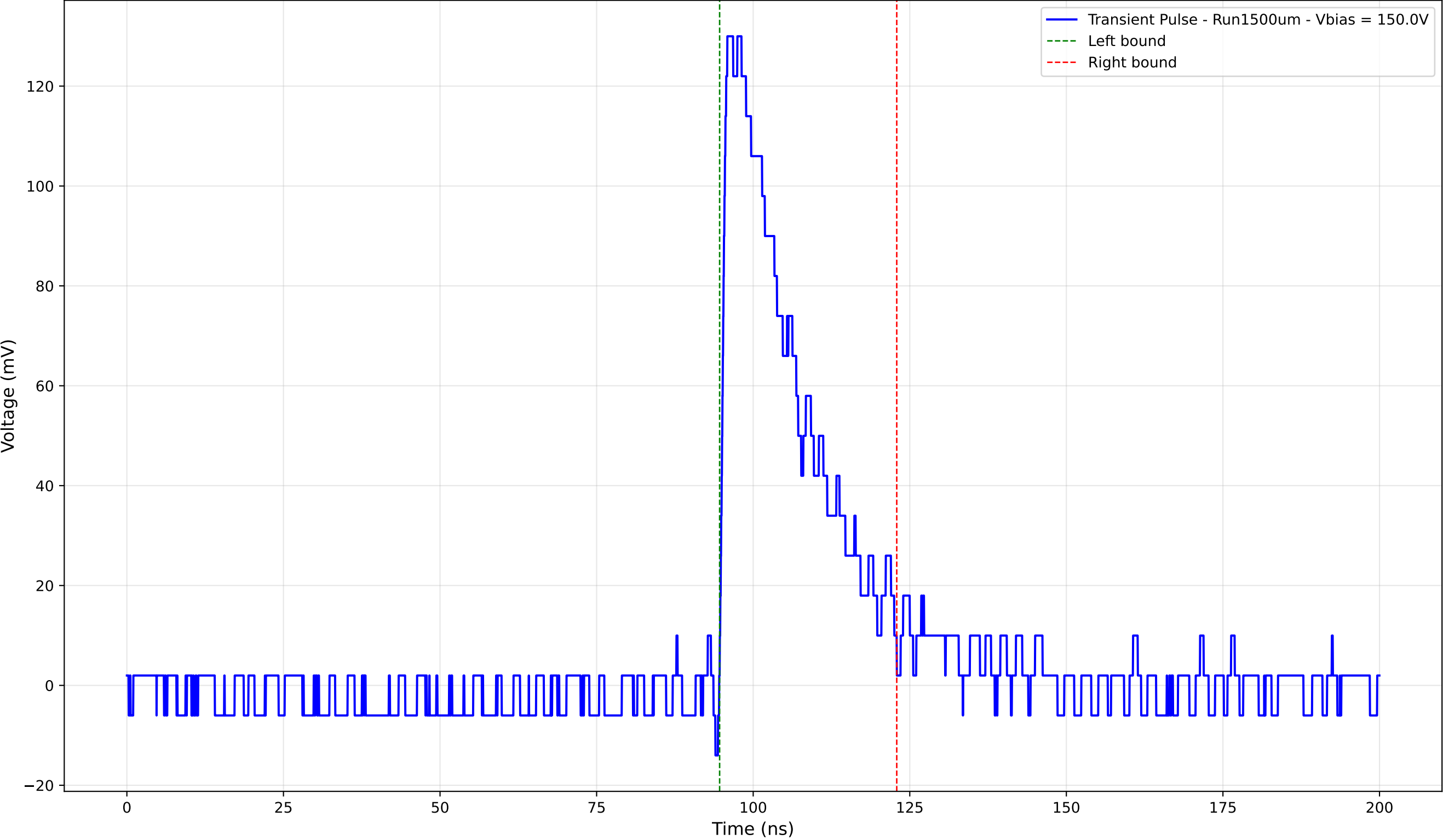
Transient Pulse - Sample: 1cm_42 - Position: 605.0 \mu\text{m} - Charge: 33.85 pC
