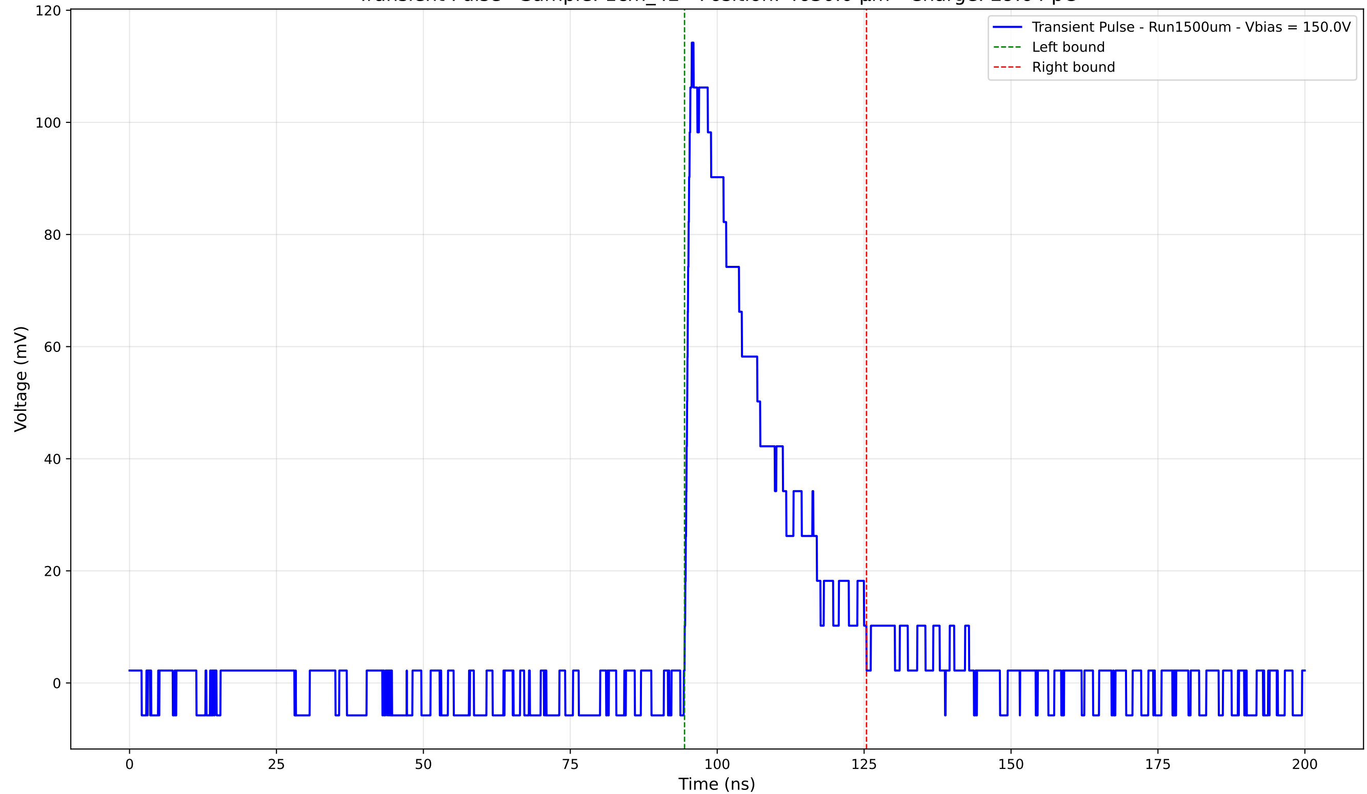
Transient Pulse - Sample: 1cm_42 - Position: 4630.0 \mu\text{m} - Charge: 29.64 pC
