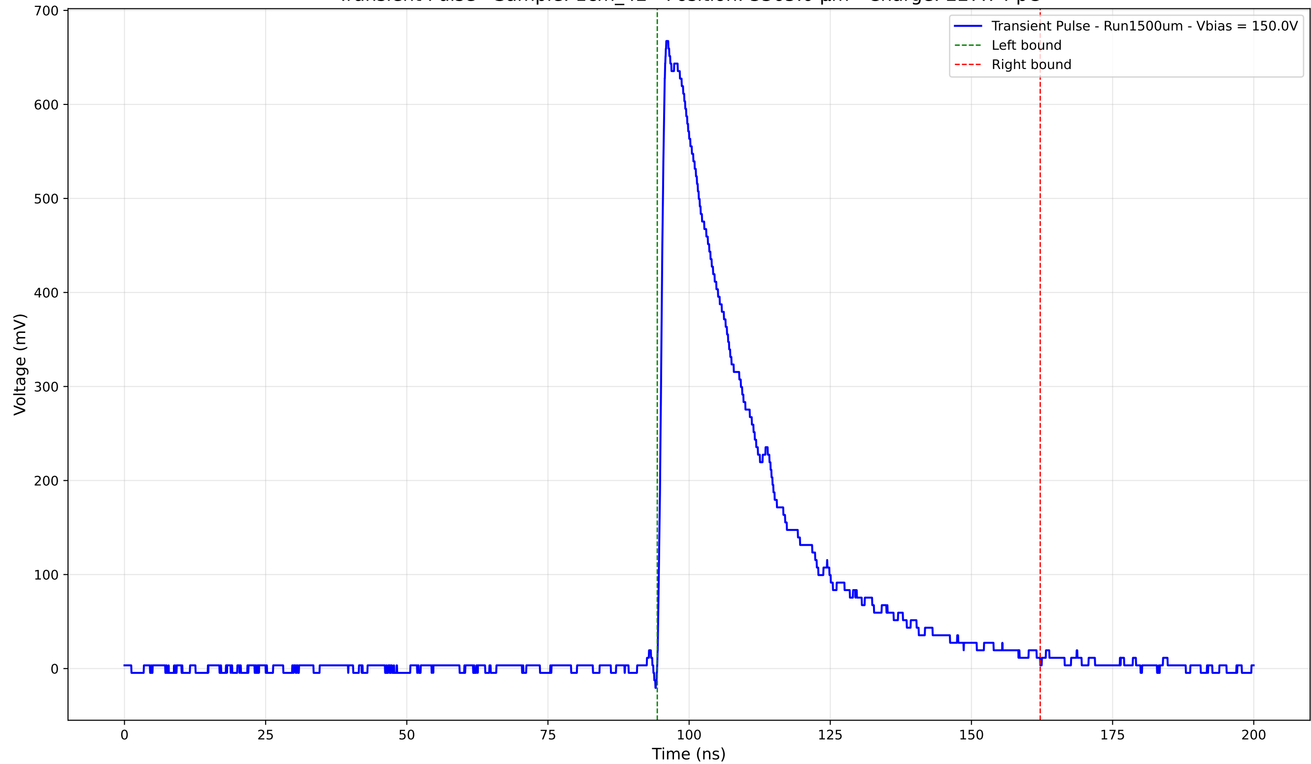
Transient Pulse - Sample: 1cm_42 - Position: 3365.0 \mu\text{m} - Charge: 227.74 pC
