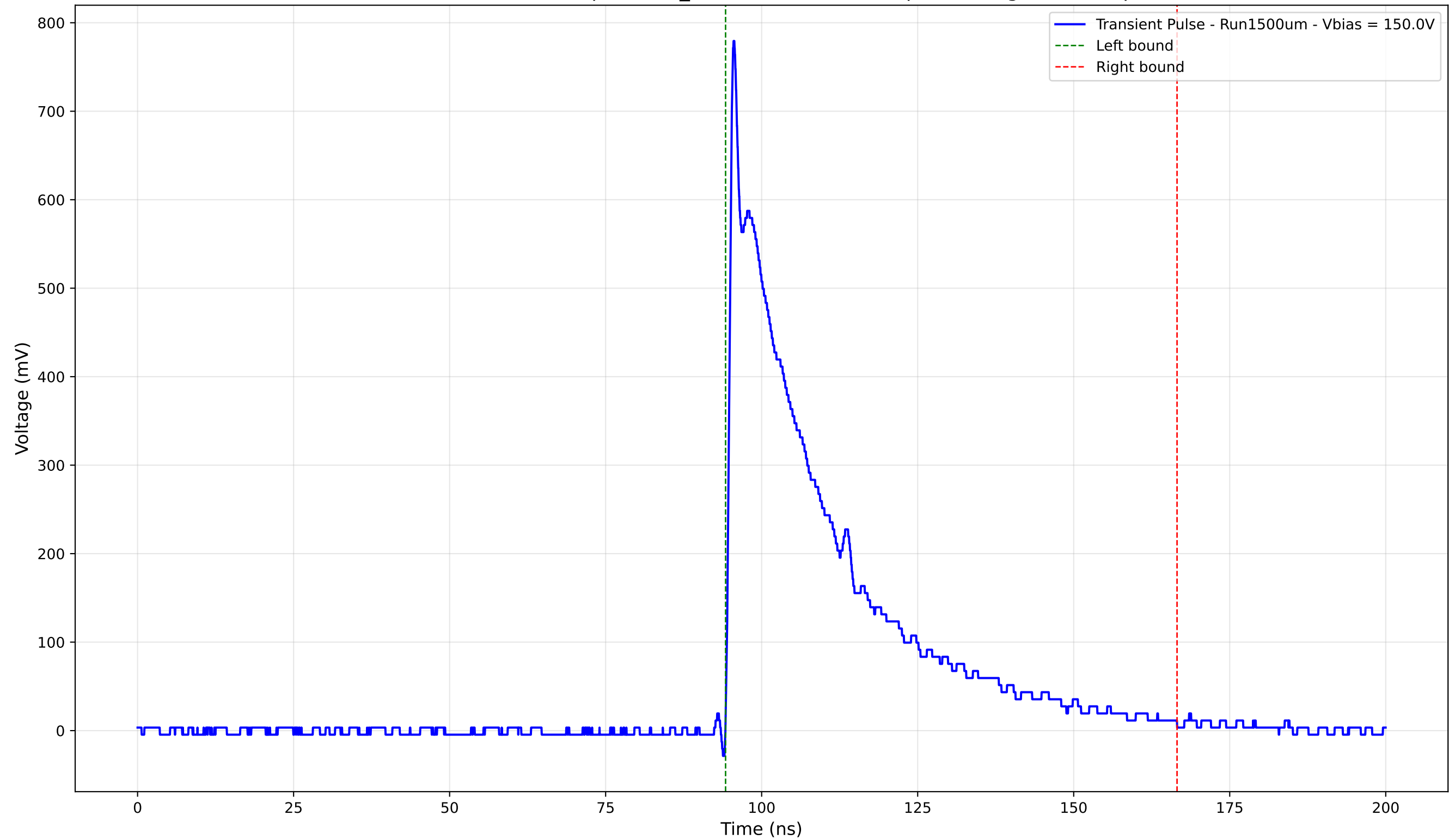
Transient Pulse - Sample: 1cm_42 - Position: 2980.0 \mu\text{m} - Charge: 218.51 pC
