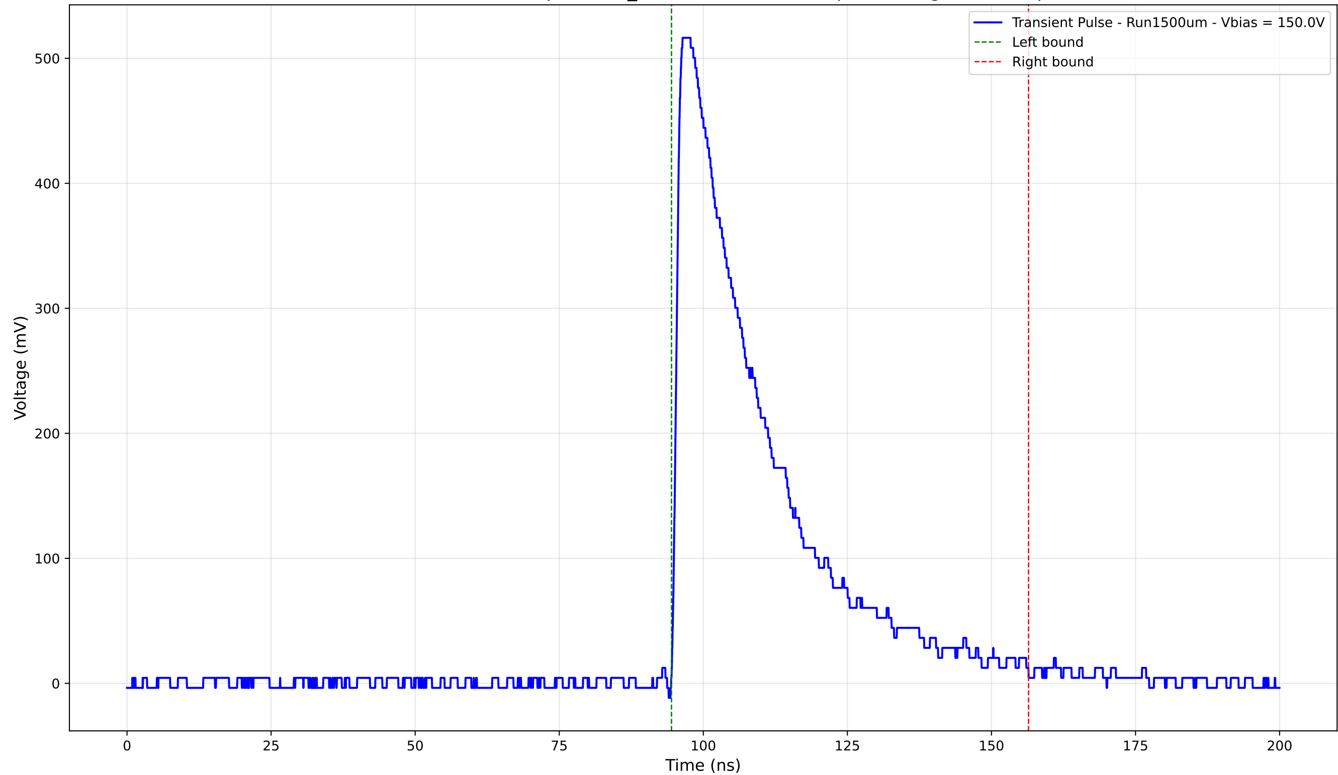
Transient Pulse - Sample: 1cm_42 - Position: 3690.0 \mu\text{m} - Charge: 171.86 pC
