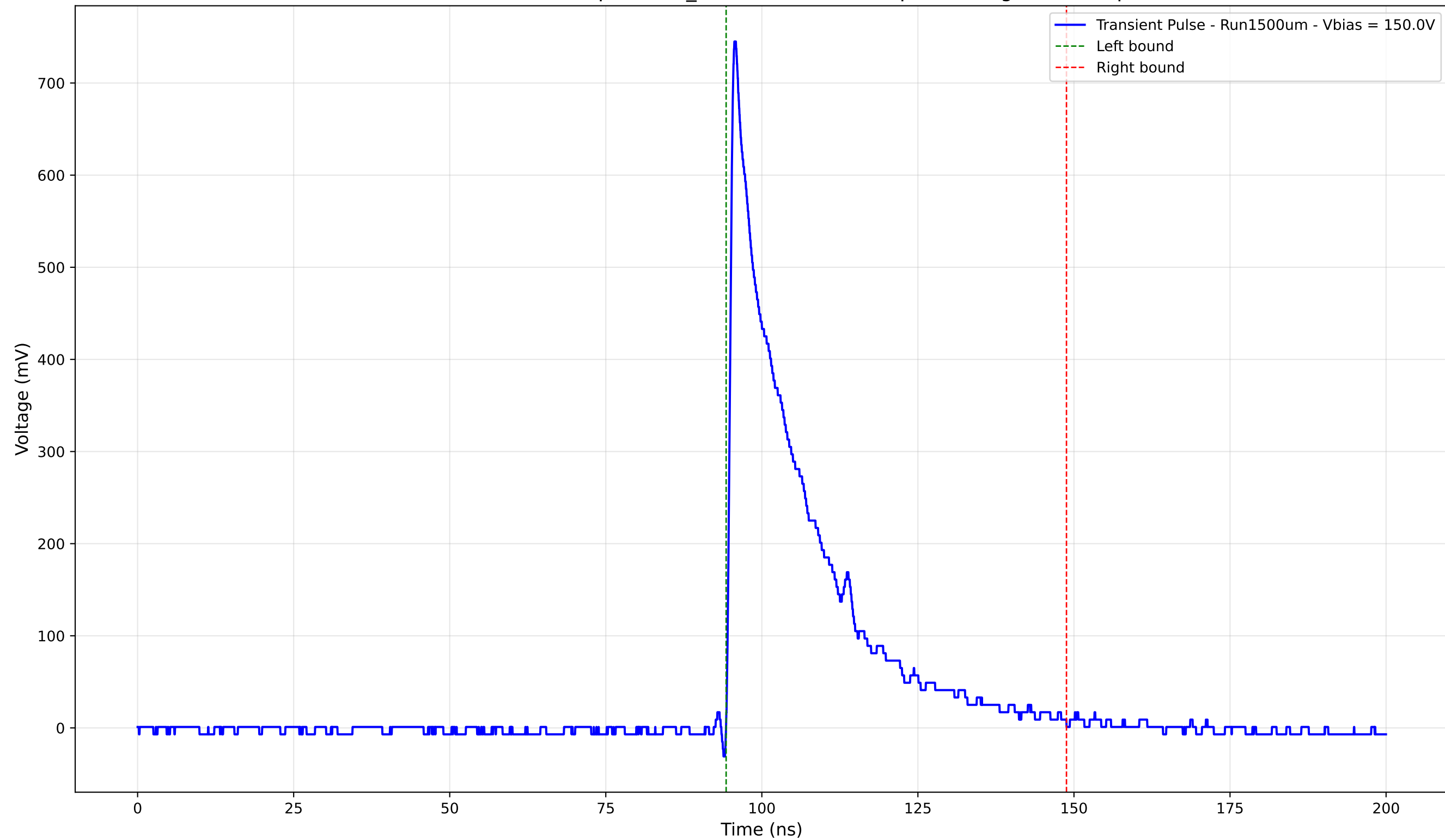
Transient Pulse - Sample: 1cm_42 - Position: 225.0 \mu\text{m} - Charge: 165.17 pC
