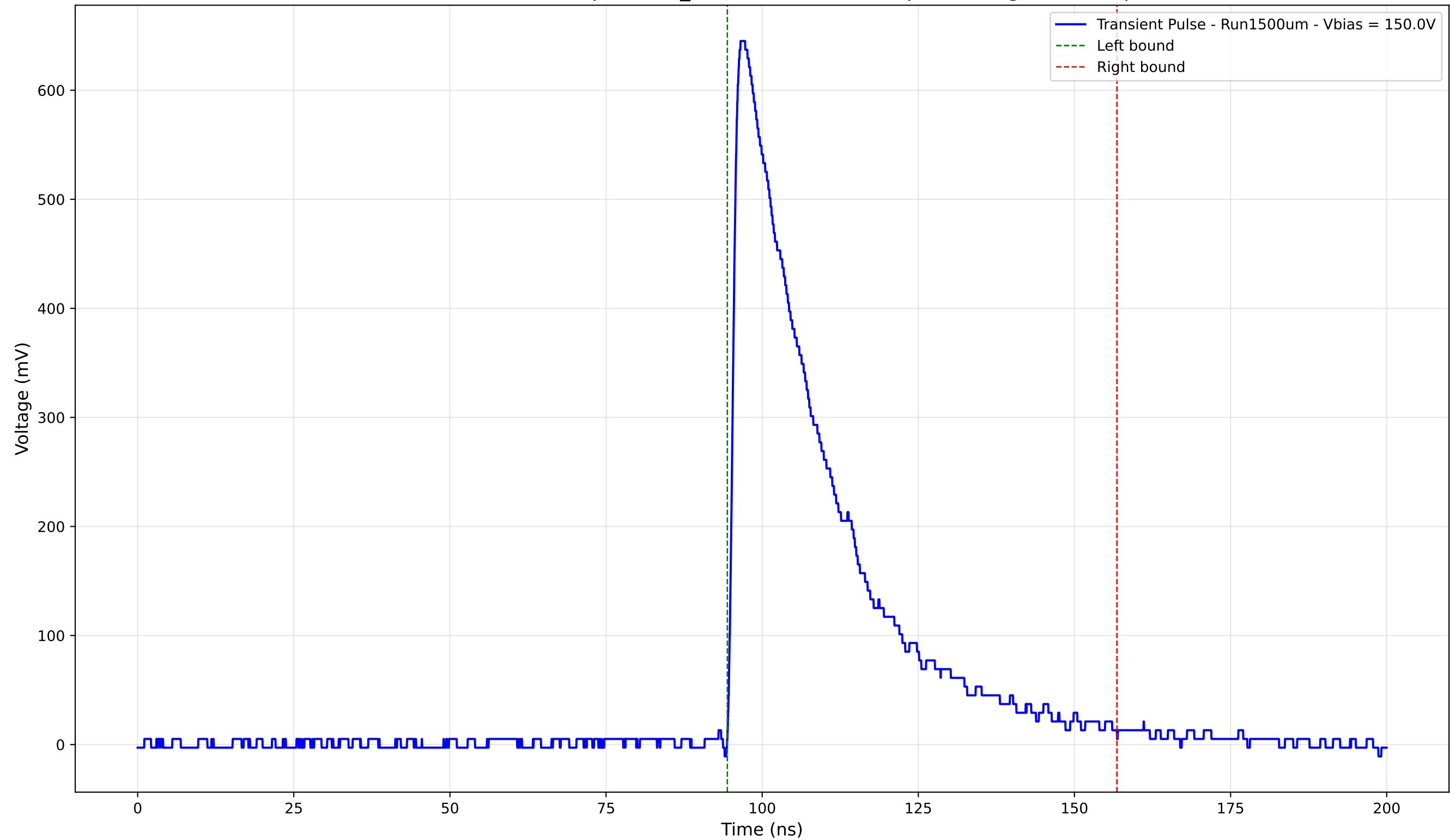
Transient Pulse - Sample: 1cm_42 - Position: 4035.0 \mu\text{m} - Charge: 206.57 pC
