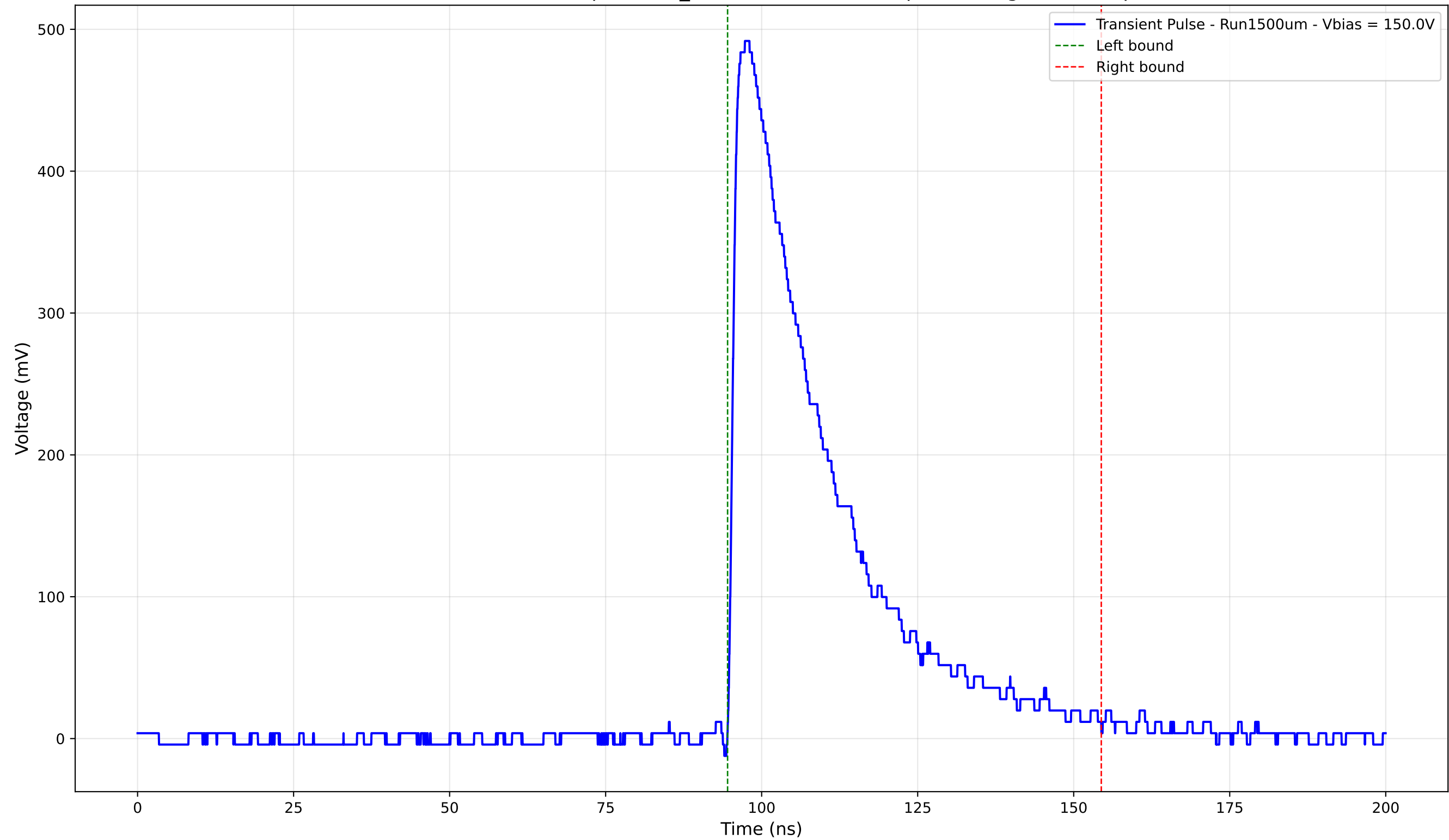
Transient Pulse - Sample: 1cm_42 - Position: 1505.0 \mu\text{m} - Charge: 162.61 pC
