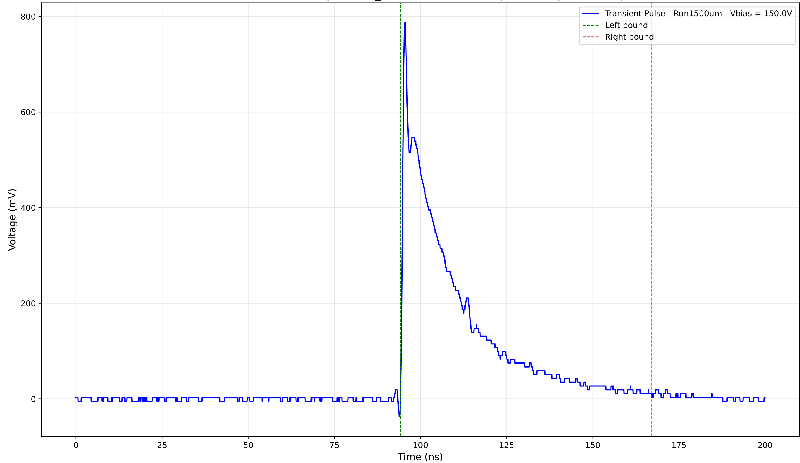
Transient Pulse - Sample: 1cm_42 - Position: 2305.0 \mu\text{m} - Charge: 205.45 pC
