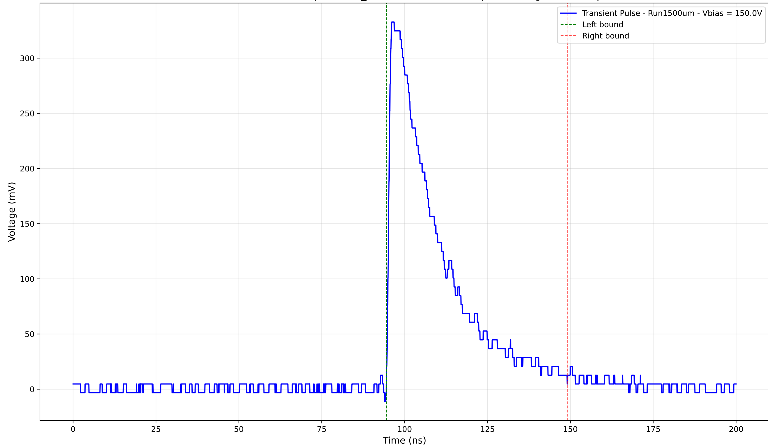
Transient Pulse - Sample: 1cm_42 - Position: 3570.0 \mu\text{m} - Charge: 109.70 pC
