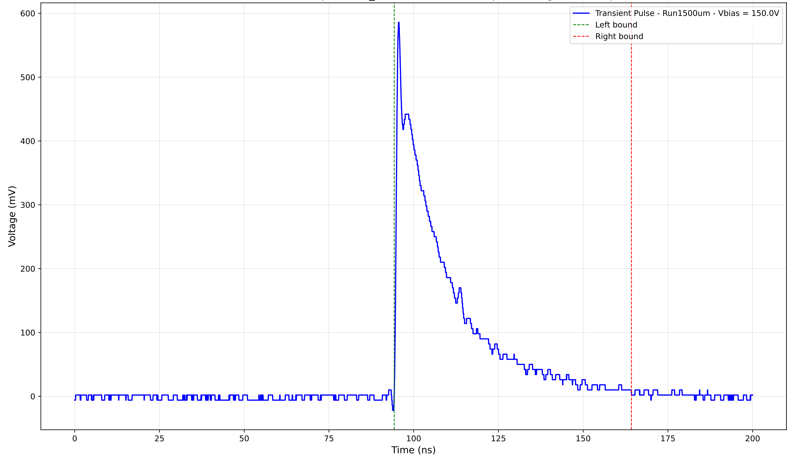
Transient Pulse - Sample: 1cm_42 - Position: 2190.0 \mu\text{m} - Charge: 162.28 pC
