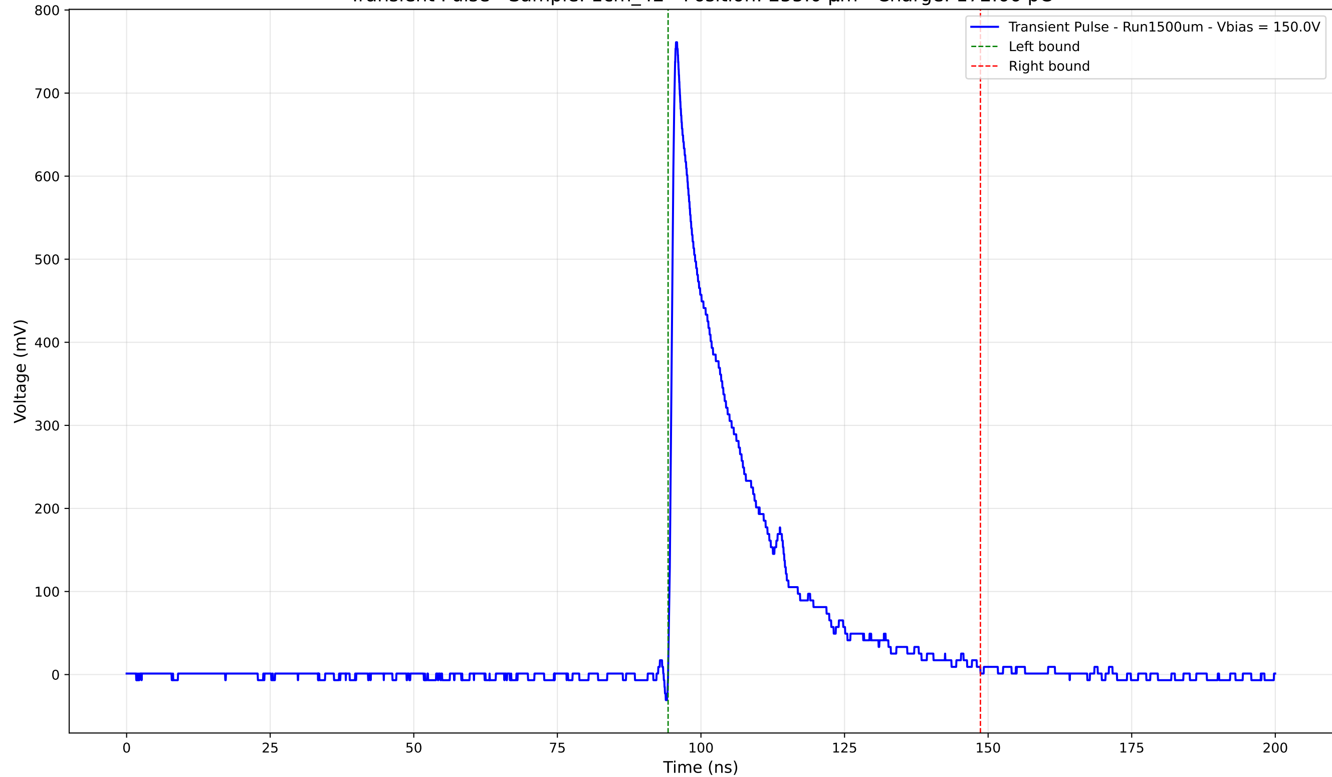
Transient Pulse - Sample: 1cm_42 - Position: 255.0 \mu\text{m} - Charge: 172.66 pC
