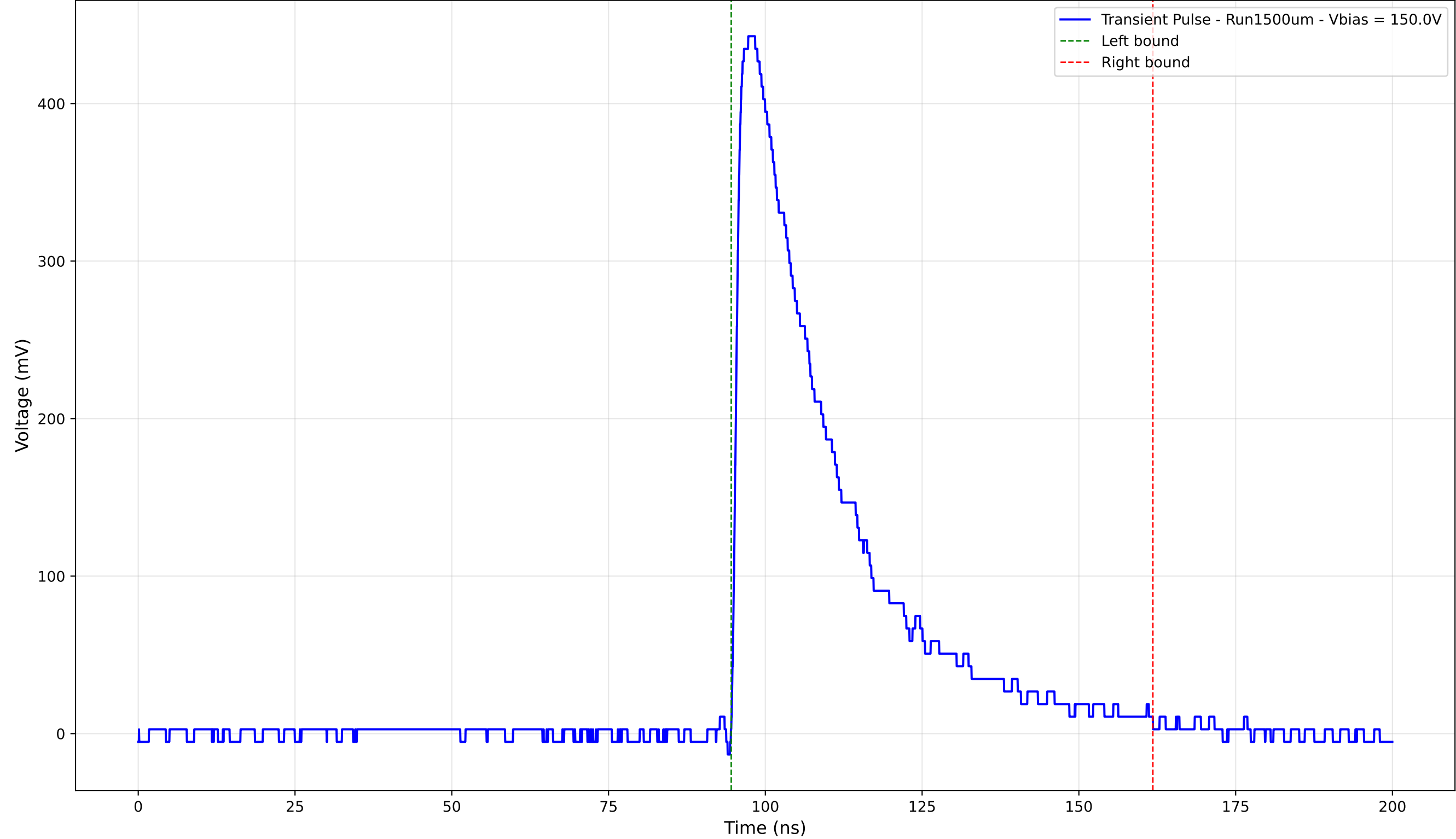
Transient Pulse - Sample: 1cm_42 - Position: 1515.0 \mu\text{m} - Charge: 149.46 pC
