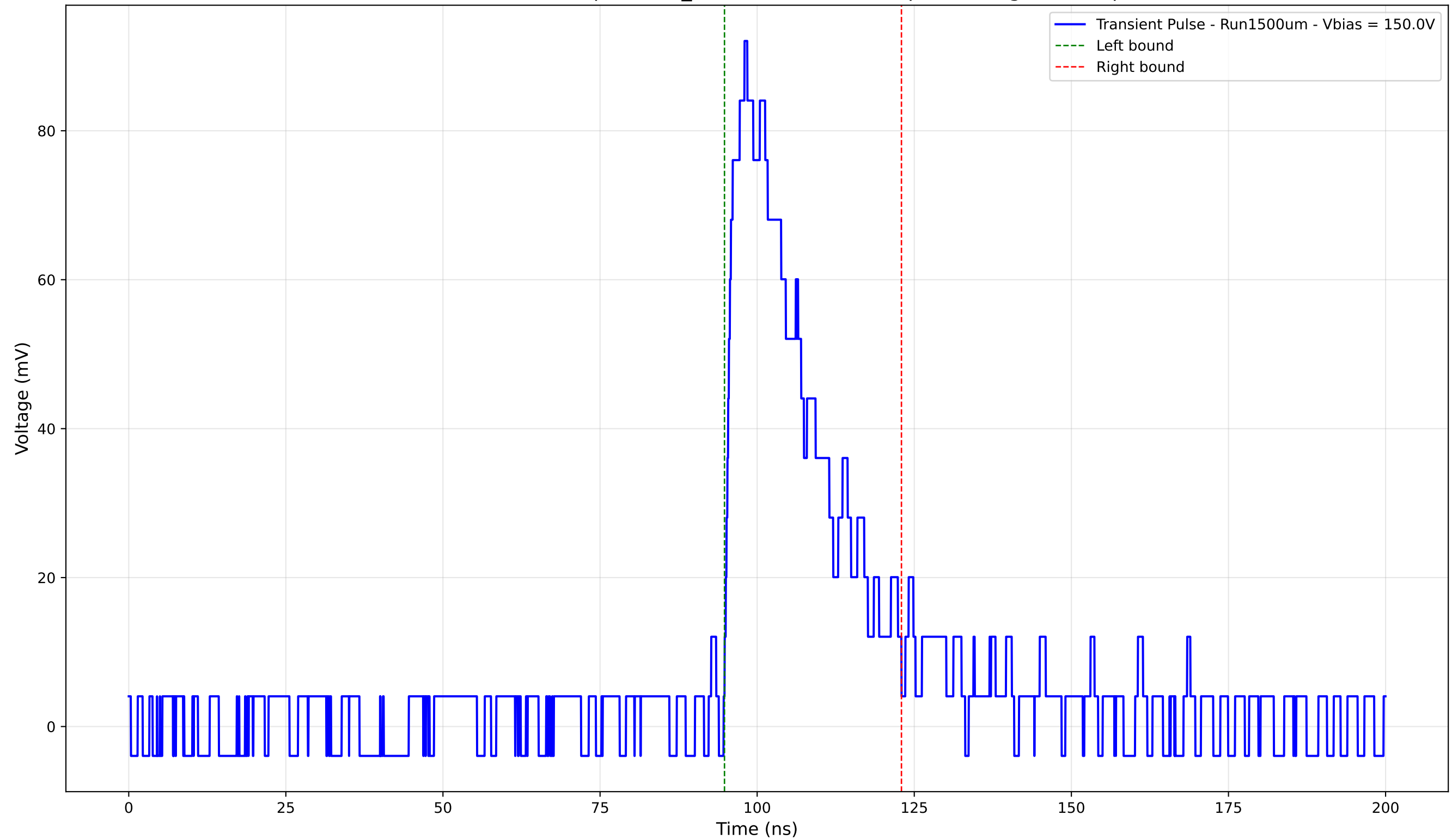
Transient Pulse - Sample: 1cm_42 - Position: 1095.0 \mu\text{m} - Charge: 24.85 pC
