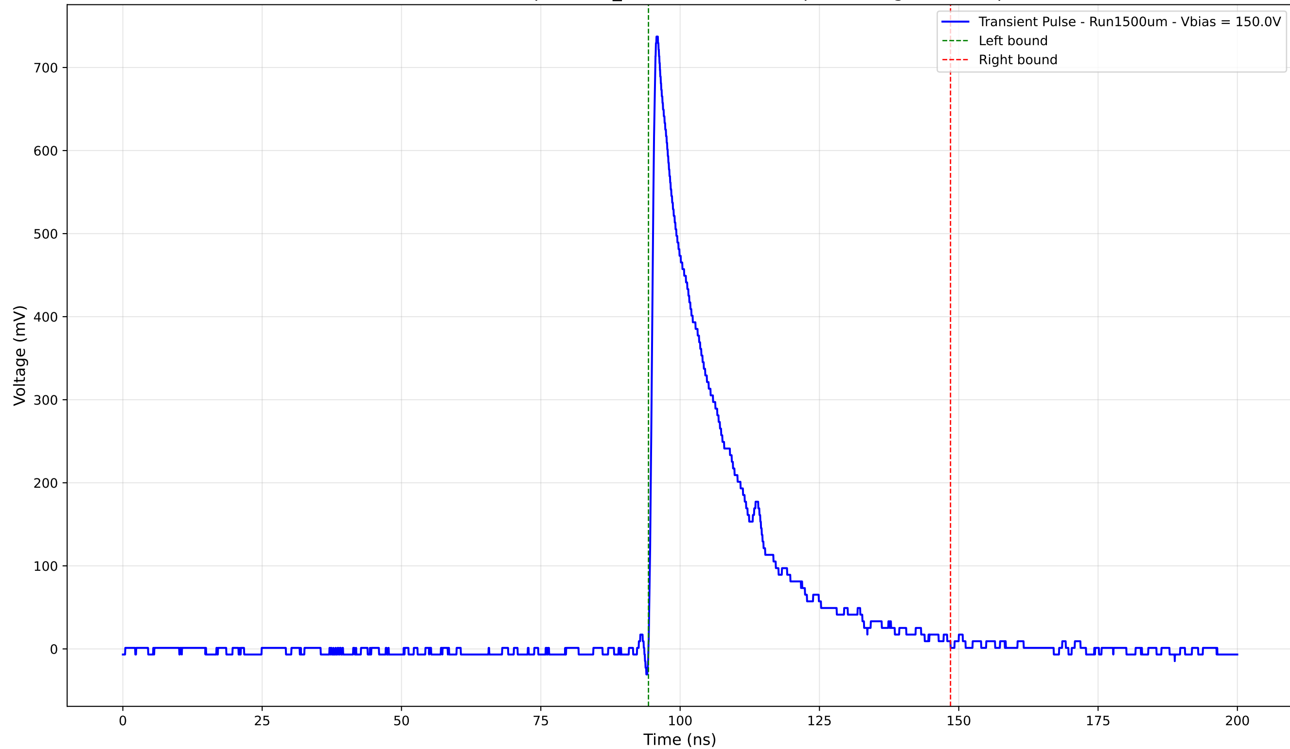
Transient Pulse - Sample: 1cm_42 - Position: 335.0 \mu\text{m} - Charge: 176.20 pC
