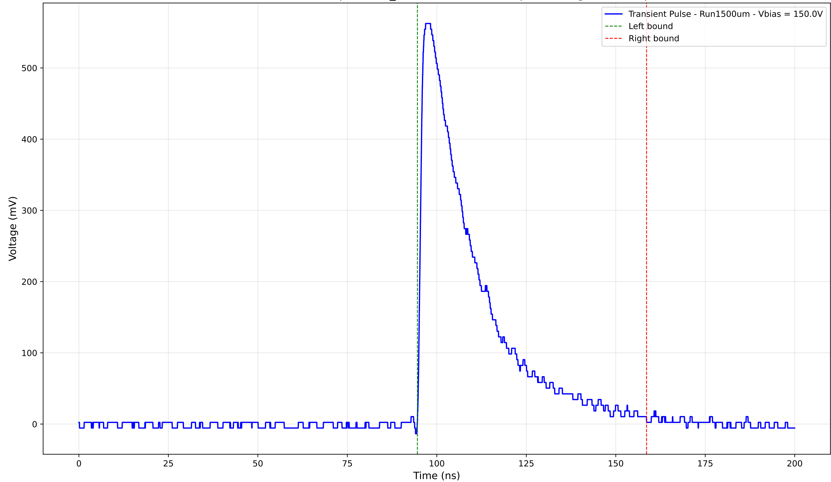
Transient Pulse - Sample: 1cm_42 - Position: 1375.0 \mu\text{m} - Charge: 187.47 pC
