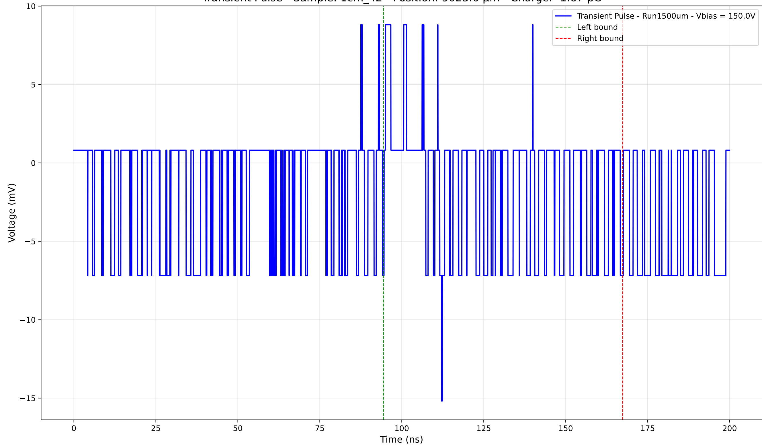
Transient Pulse - Sample: 1cm_42 - Position: 5025.0 \mu\text{m} - Charge: -1.67 pC
