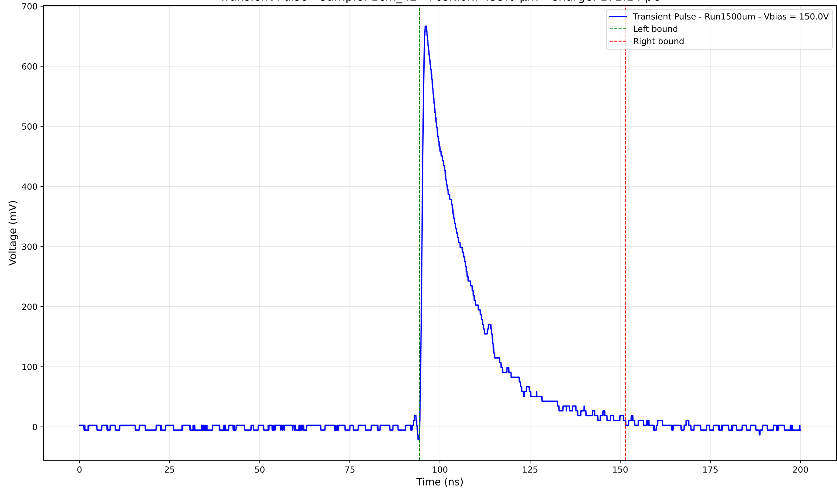
Transient Pulse - Sample: 1cm_42 - Position: 455.0 \mu\text{m} - Charge: 172.14 pC
