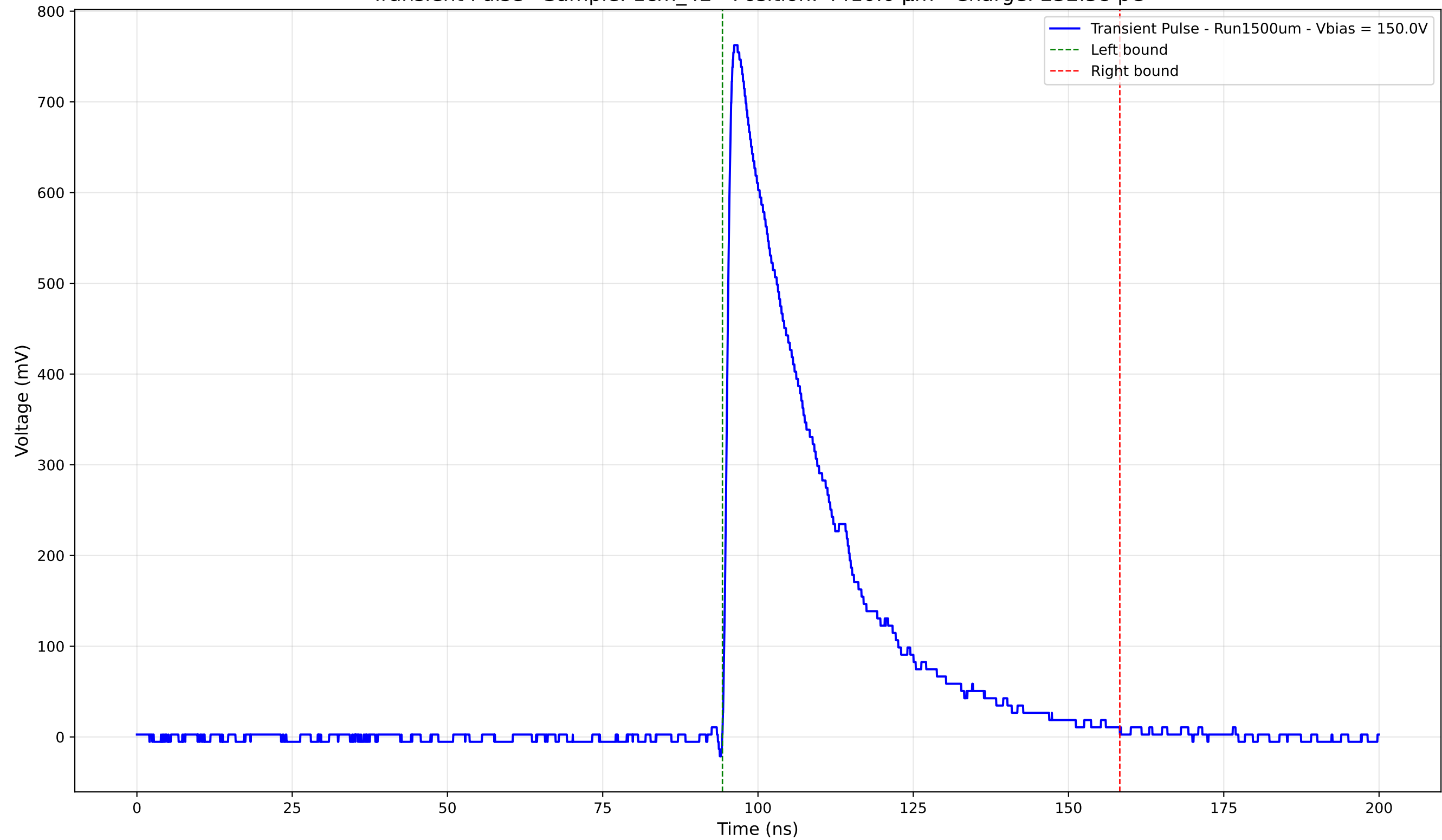
Transient Pulse - Sample: 1cm_42 - Position: 4410.0 \mu\text{m} - Charge: 232.58 pC
