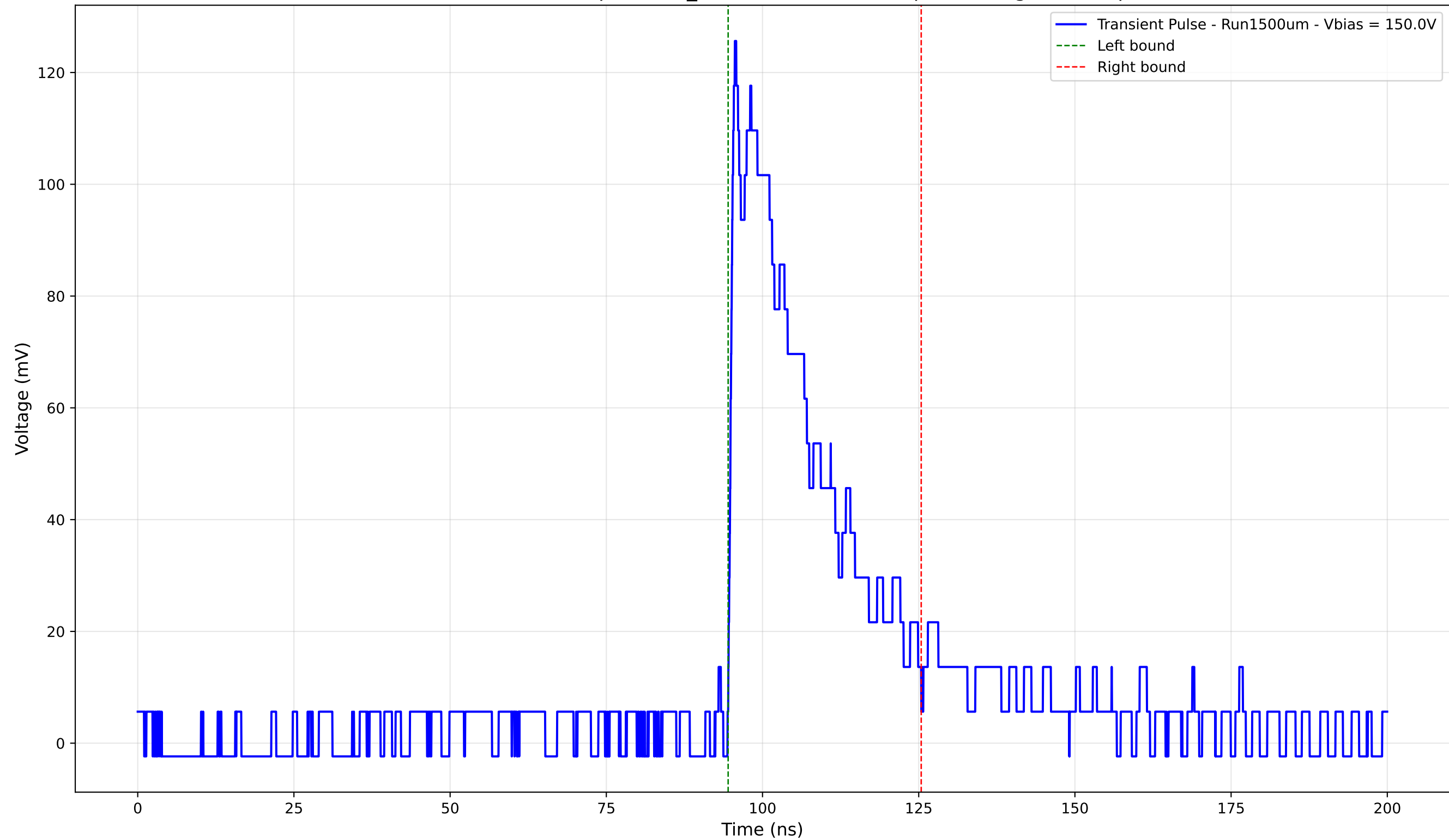
Transient Pulse - Sample: 1cm_42 - Position: 3125.0 \mu\text{m} - Charge: 34.15 pC
