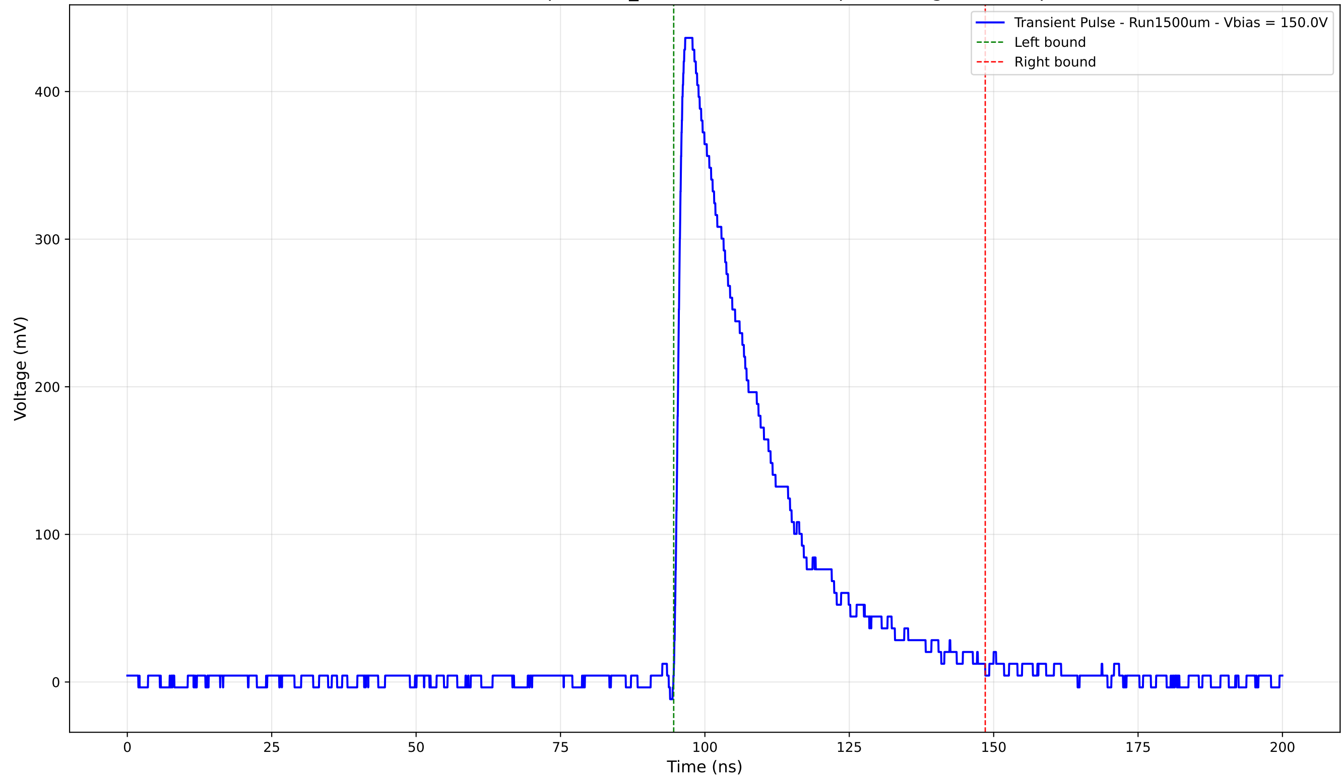
Transient Pulse - Sample: 1cm_42 - Position: 1020.0 \mu\text{m} - Charge: 133.74 pC
