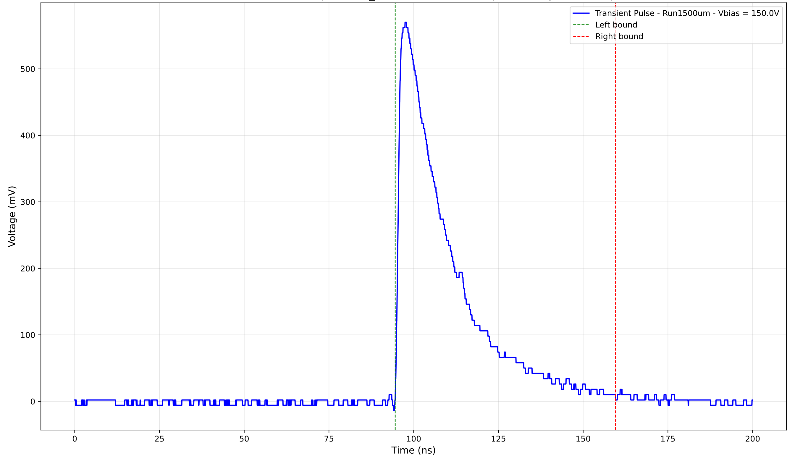
Transient Pulse - Sample: 1cm_42 - Position: 1415.0 \mu\text{m} - Charge: 188.57 pC
