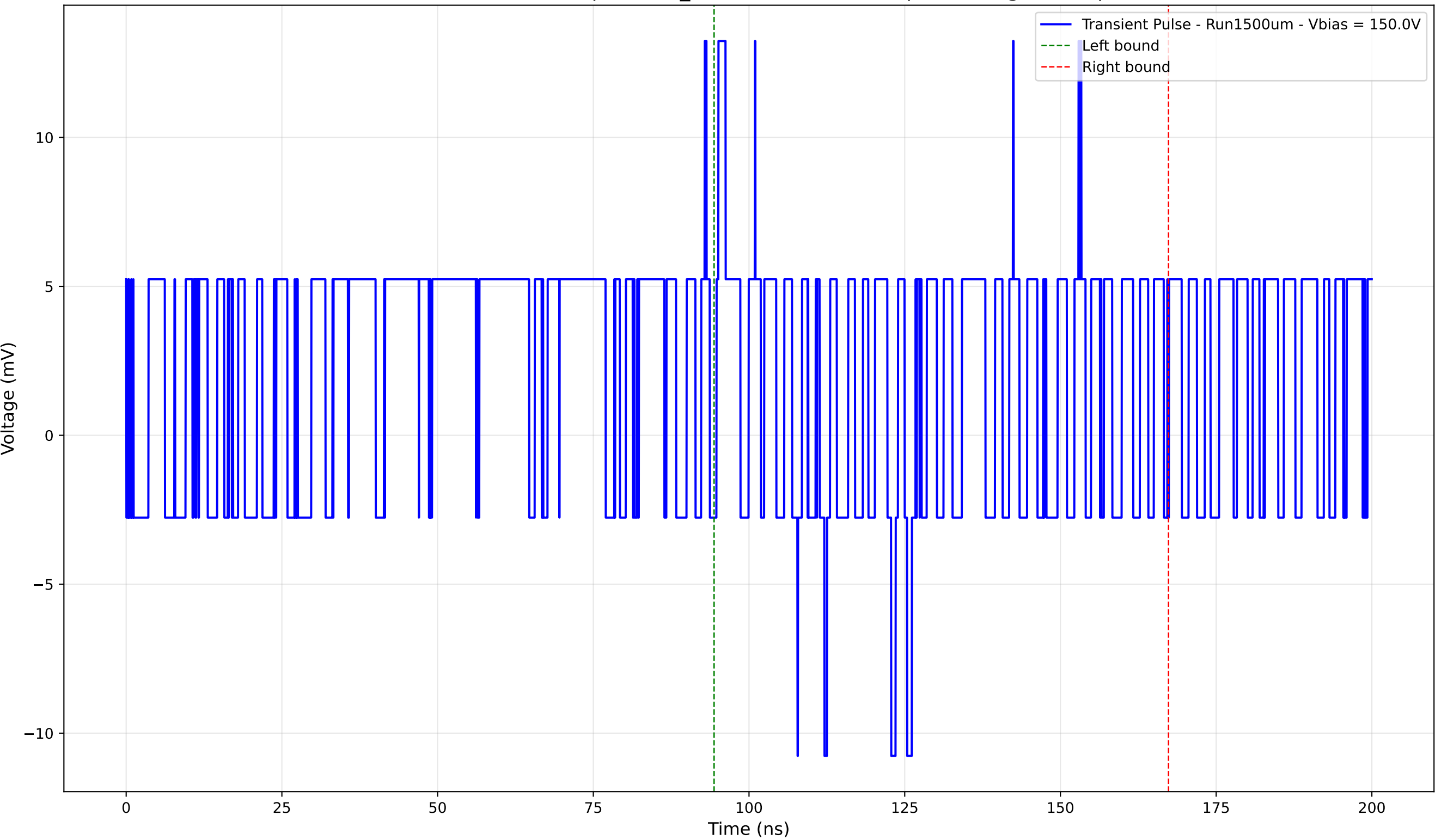
Transient Pulse - Sample: 1cm_42 - Position: 5070.0 \mu\text{m} - Charge: 2.34 pC
