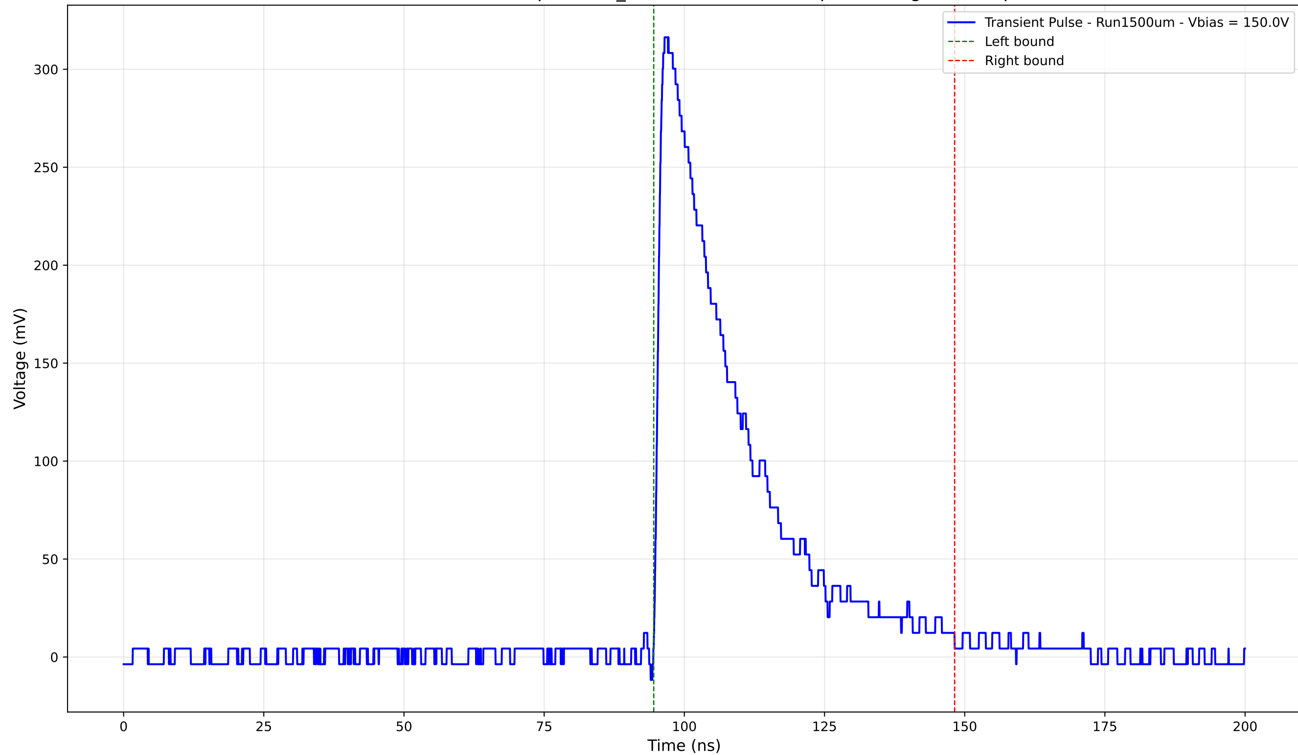
Transient Pulse - Sample: 1cm_42 - Position: 4080.0 \mu\text{m} - Charge: 97.52 pC
