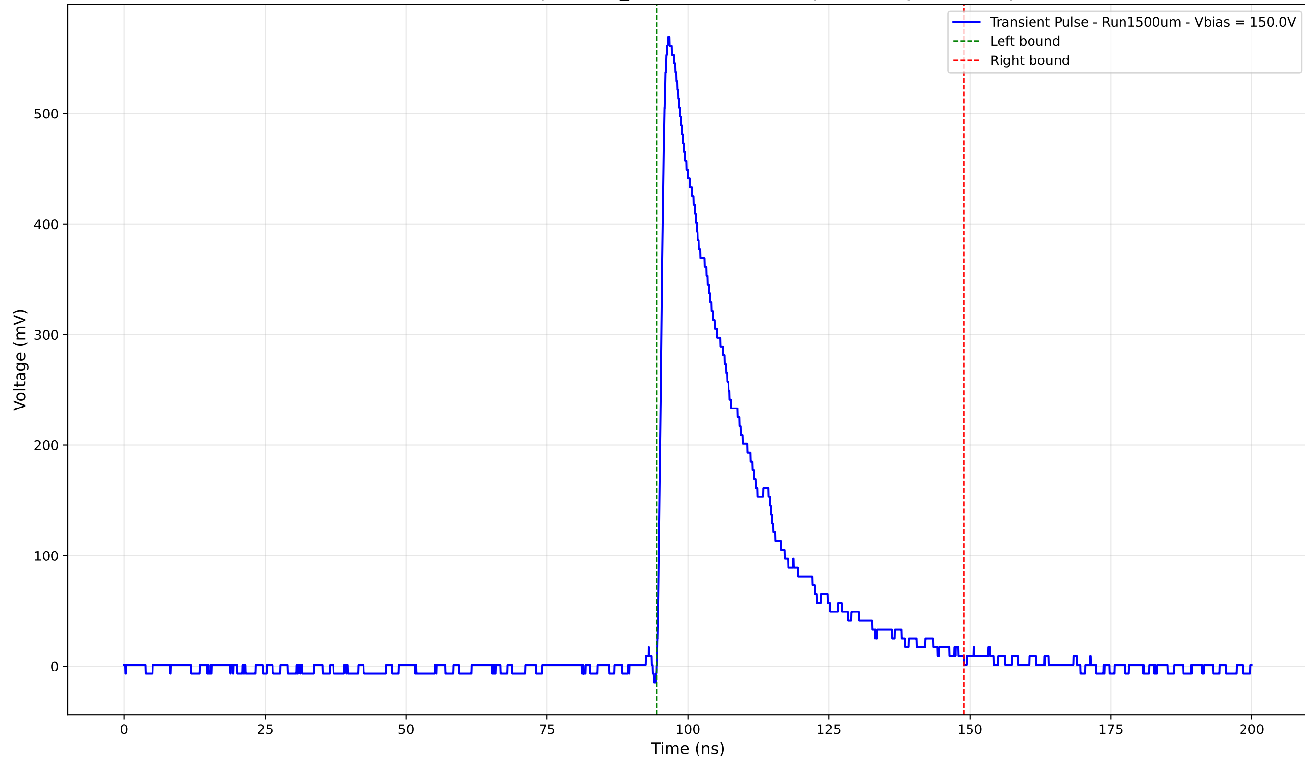
Transient Pulse - Sample: 1cm_42 - Position: 690.0 \mu\text{m} - Charge: 160.96 pC
