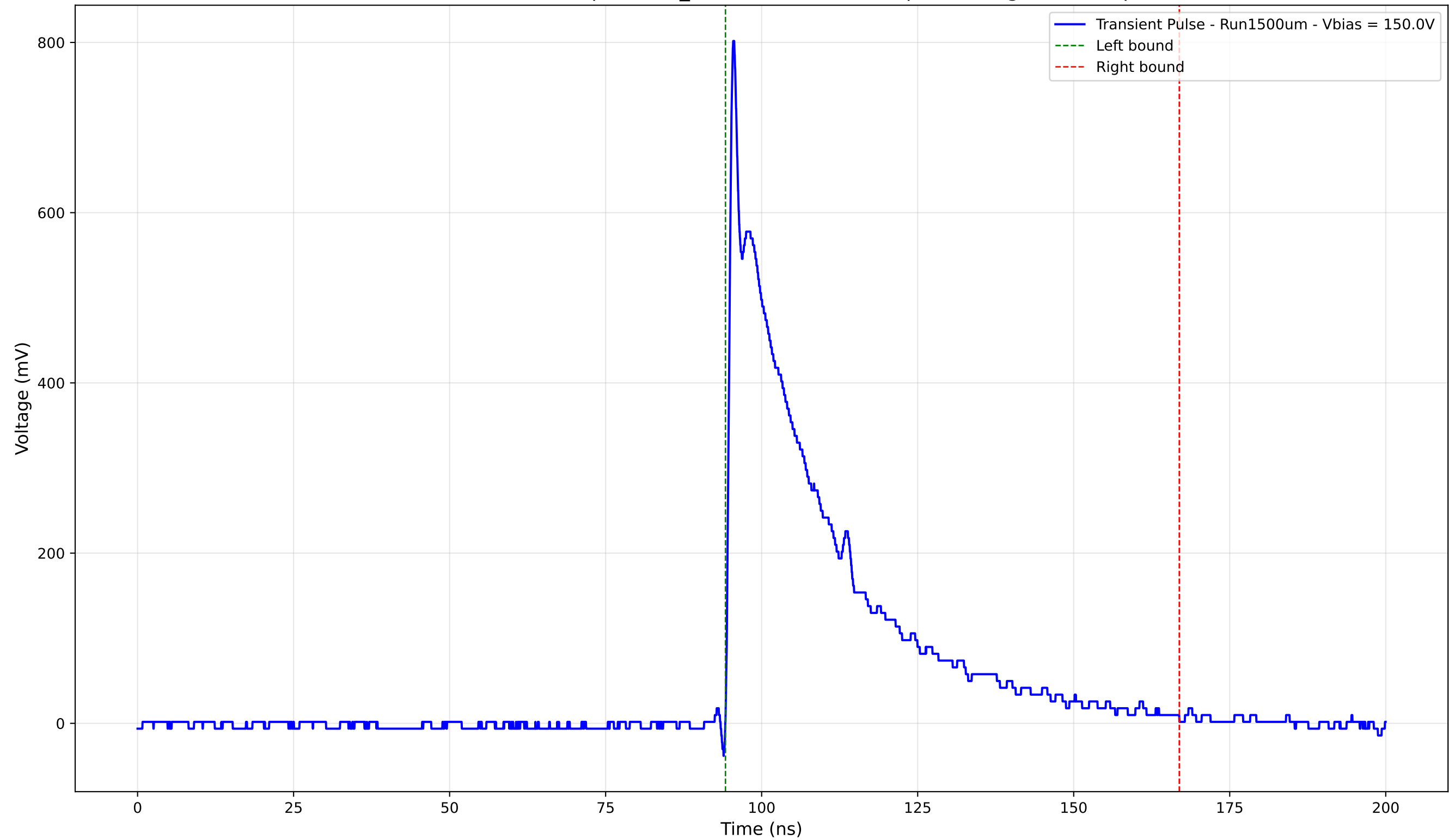
Transient Pulse - Sample: 1cm_42 - Position: 2920.0 \mu\text{m} - Charge: 213.54 pC
