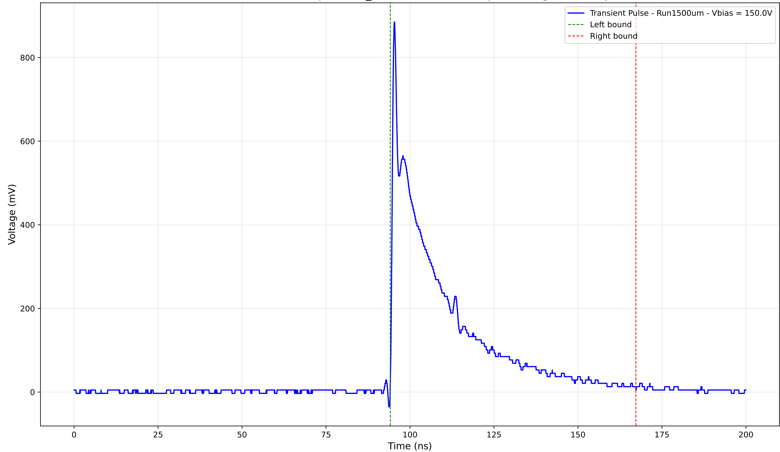
Transient Pulse - Sample: 1cm_42 - Position: 2750.0 \mu\text{m} - Charge: 214.05 pC
