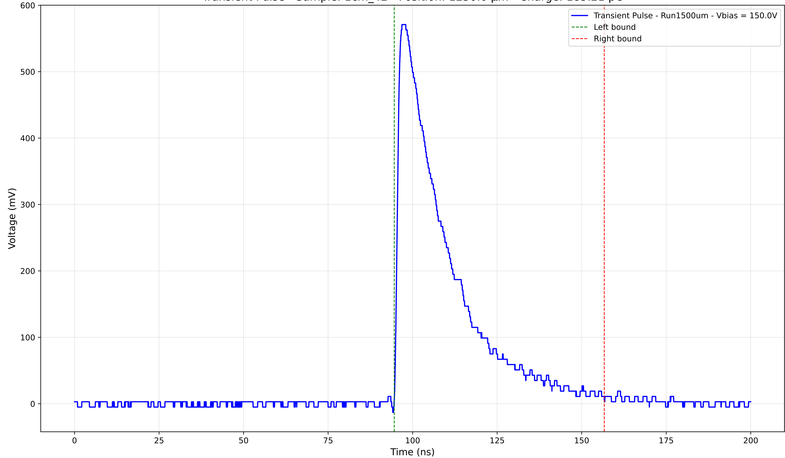
Transient Pulse - Sample: 1cm_42 - Position: 1250.0 \mu\text{m} - Charge: 185.21 pC
