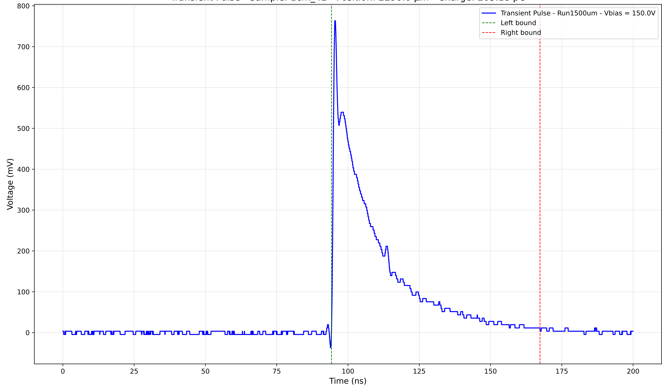
Transient Pulse - Sample: 1cm_42 - Position: 2290.0 \mu\text{m} - Charge: 203.18 pC
