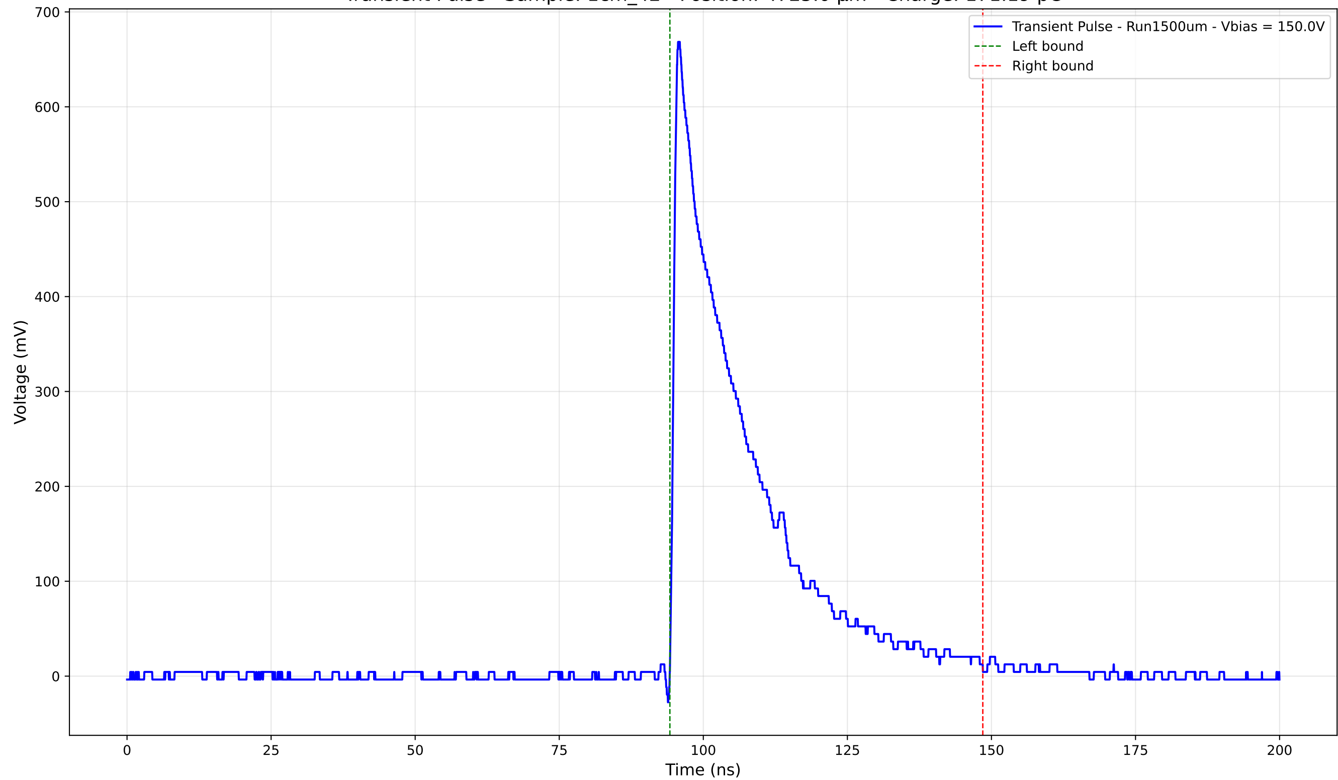
Transient Pulse - Sample: 1cm_42 - Position: 4725.0 \mu\text{m} - Charge: 171.19 pC
