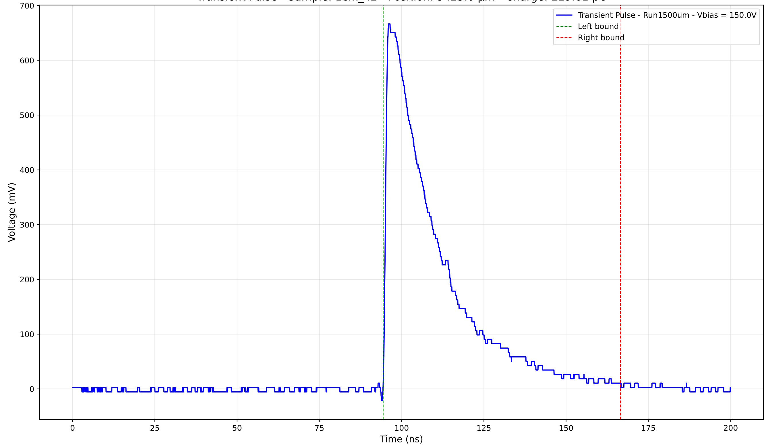
Transient Pulse - Sample: 1cm_42 - Position: 3425.0 \mu\text{m} - Charge: 229.61 pC
