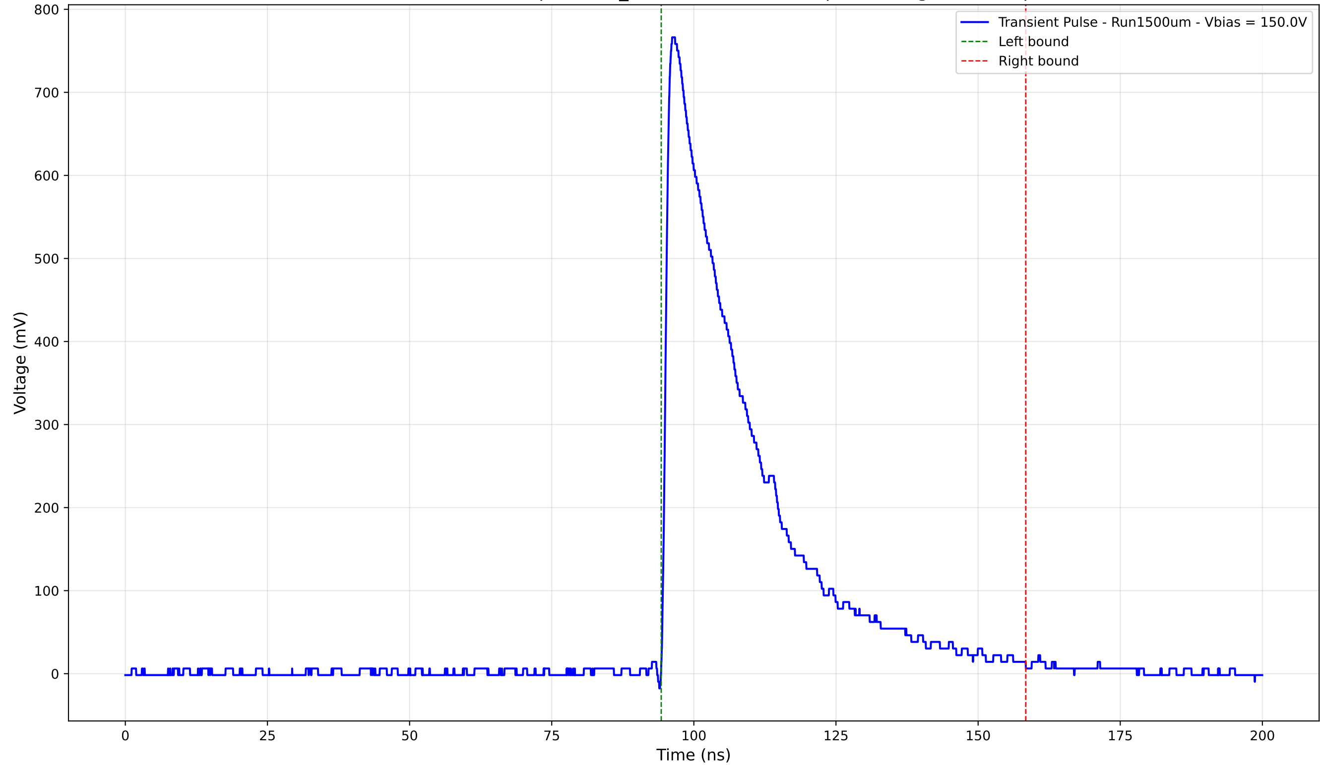
Transient Pulse - Sample: 1cm_42 - Position: 4405.0 \mu\text{m} - Charge: 237.85 pC
