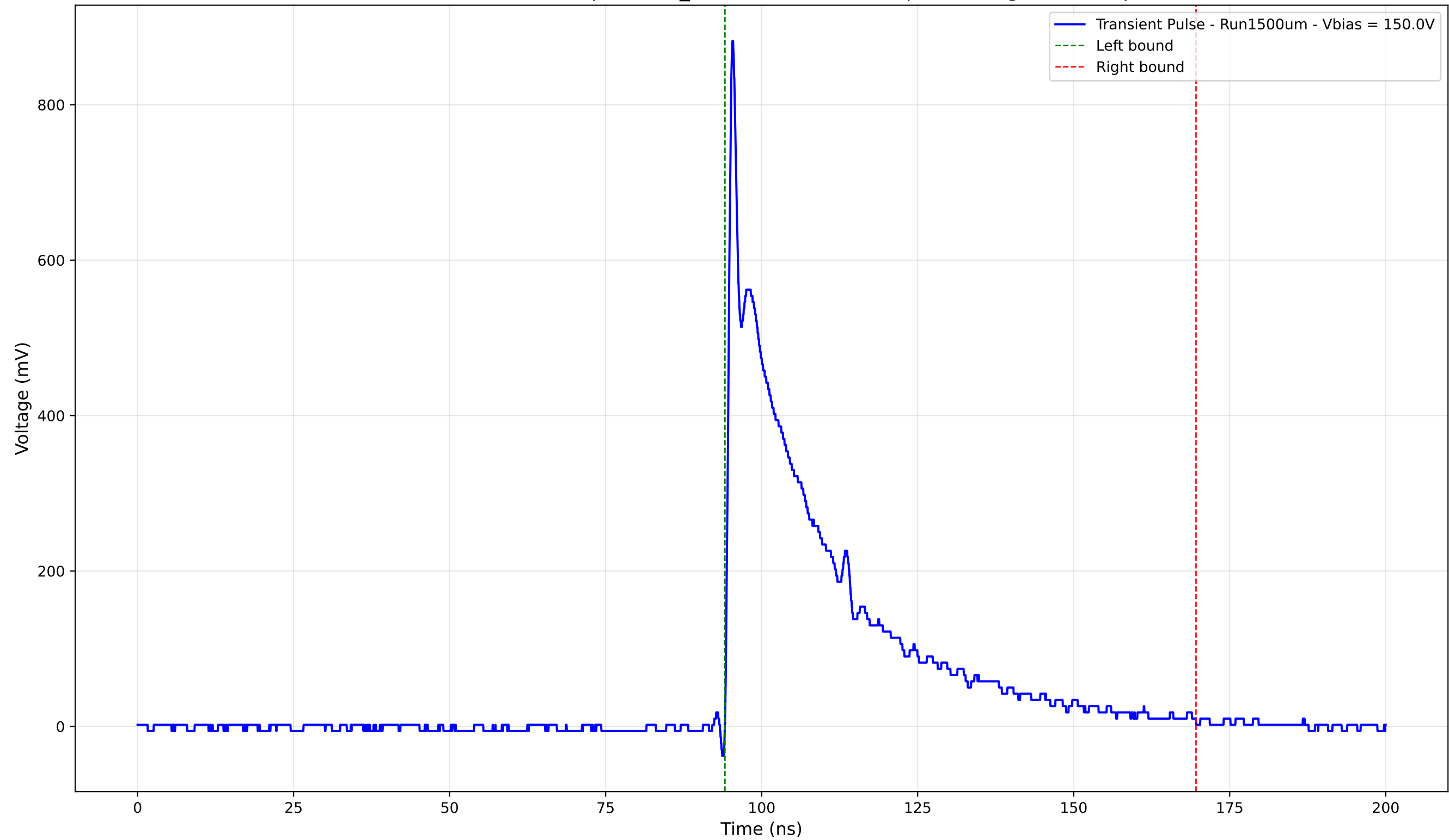
Transient Pulse - Sample: 1cm_42 - Position: 2755.0 \mu\text{m} - Charge: 211.11 pC
