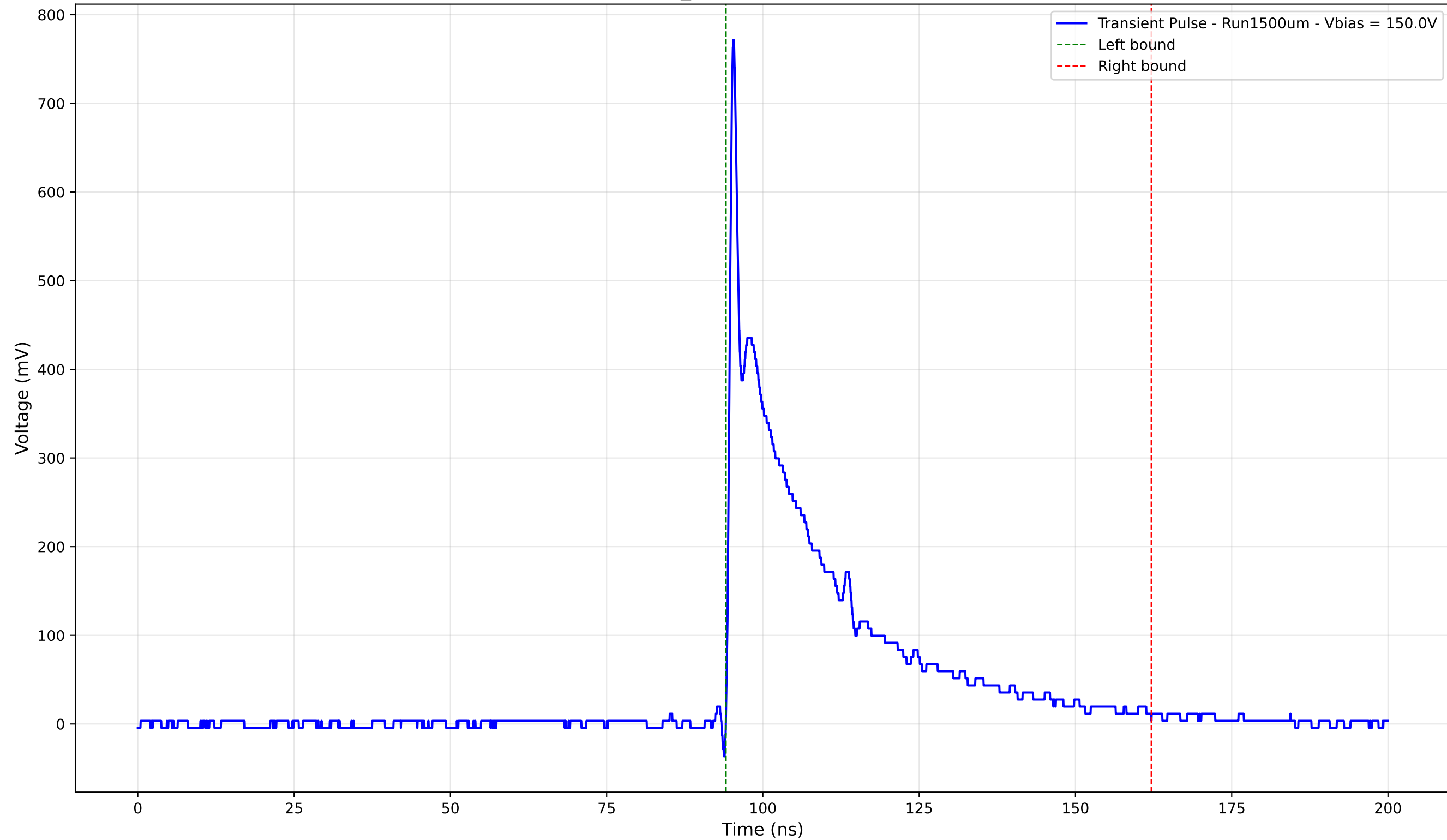
Transient Pulse - Sample: 1cm_42 - Position: 2685.0 \mu\text{m} - Charge: 162.90 pC
