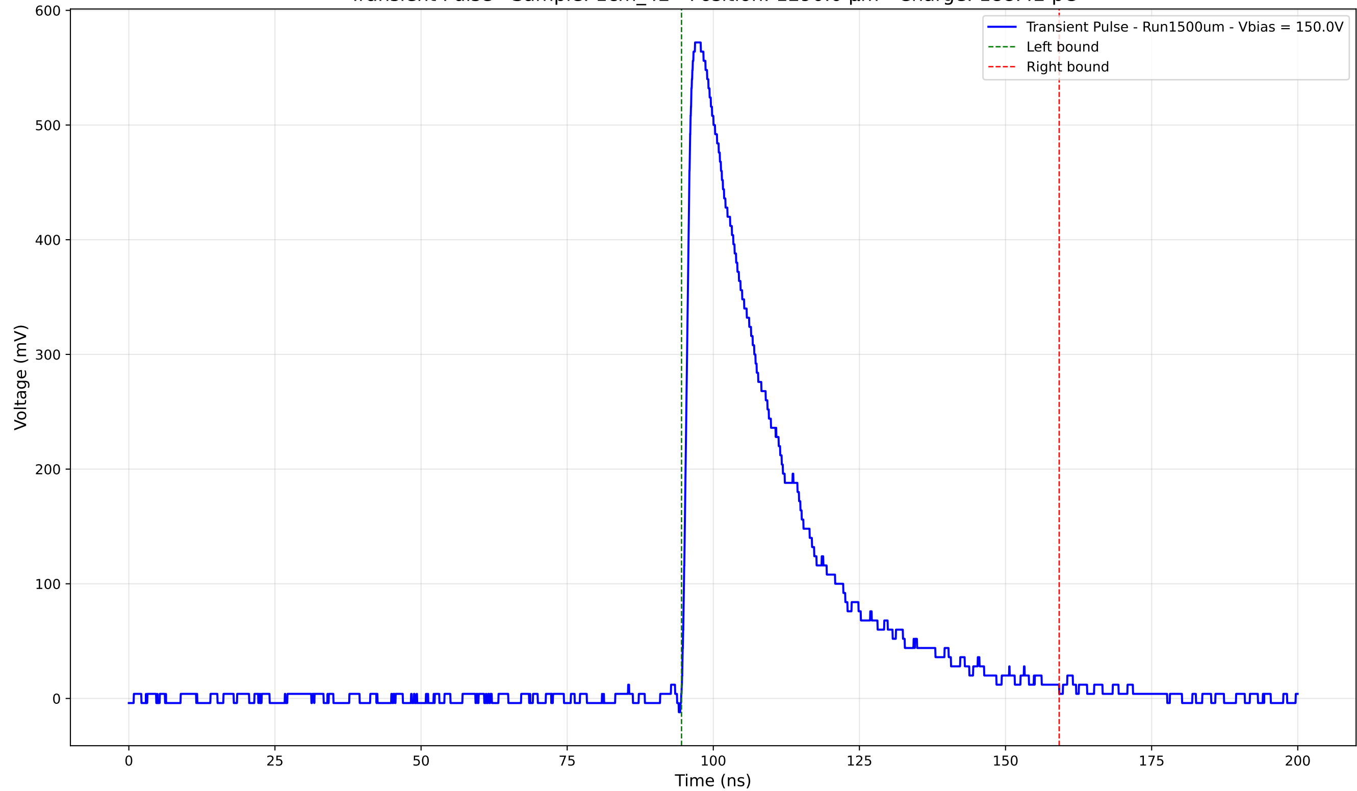
Transient Pulse - Sample: 1cm_42 - Position: 1290.0 \mu\text{m} - Charge: 188.42 pC
