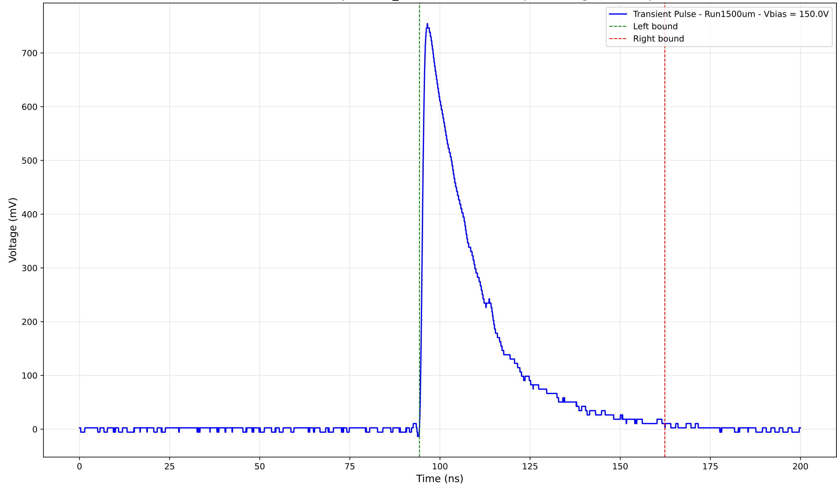
Transient Pulse - Sample: 1cm_42 - Position: 4305.0 \mu\text{m} - Charge: 235.38 pC
