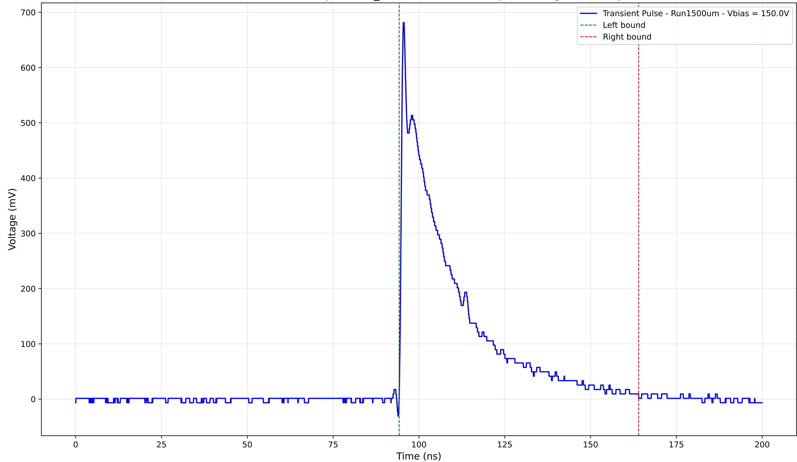
Transient Pulse - Sample: 1cm_42 - Position: 2225.0 \mu\text{m} - Charge: 186.87 pC
