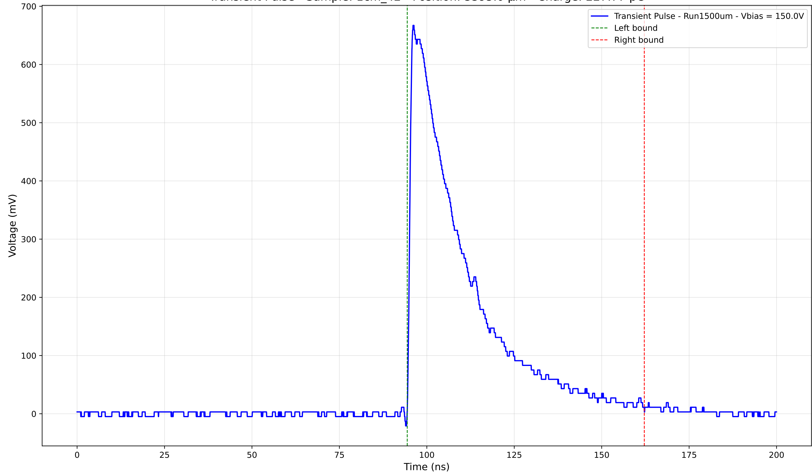
Transient Pulse - Sample: 1cm_42 - Position: 3395.0 \mu\text{m} - Charge: 227.77 pC
