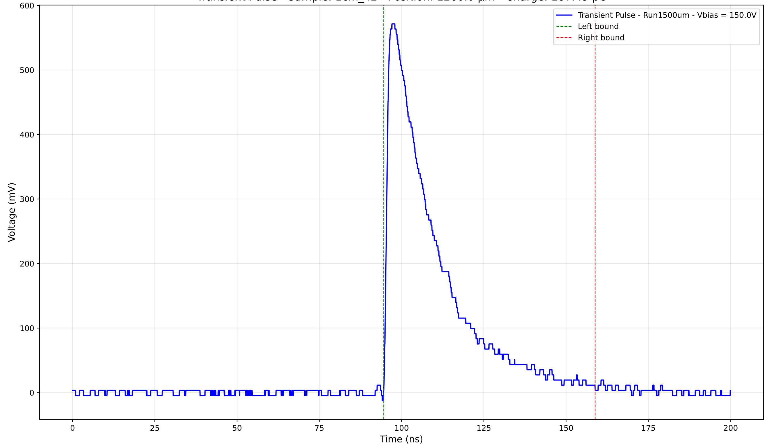
Transient Pulse - Sample: 1cm_42 - Position: 1260.0 \mu\text{m} - Charge: 187.49 pC
