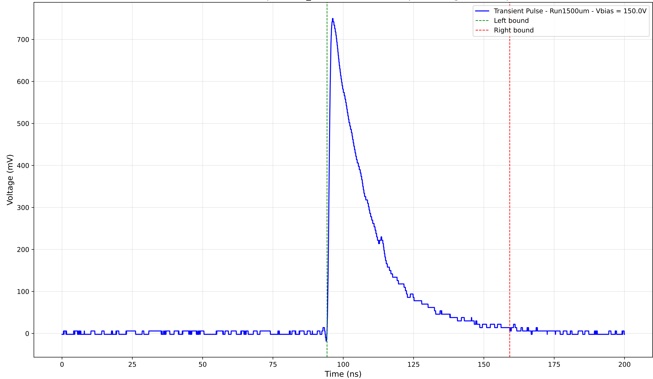
Transient Pulse - Sample: 1cm_42 - Position: 4475.0 \mu\text{m} - Charge: 225.66 pC
