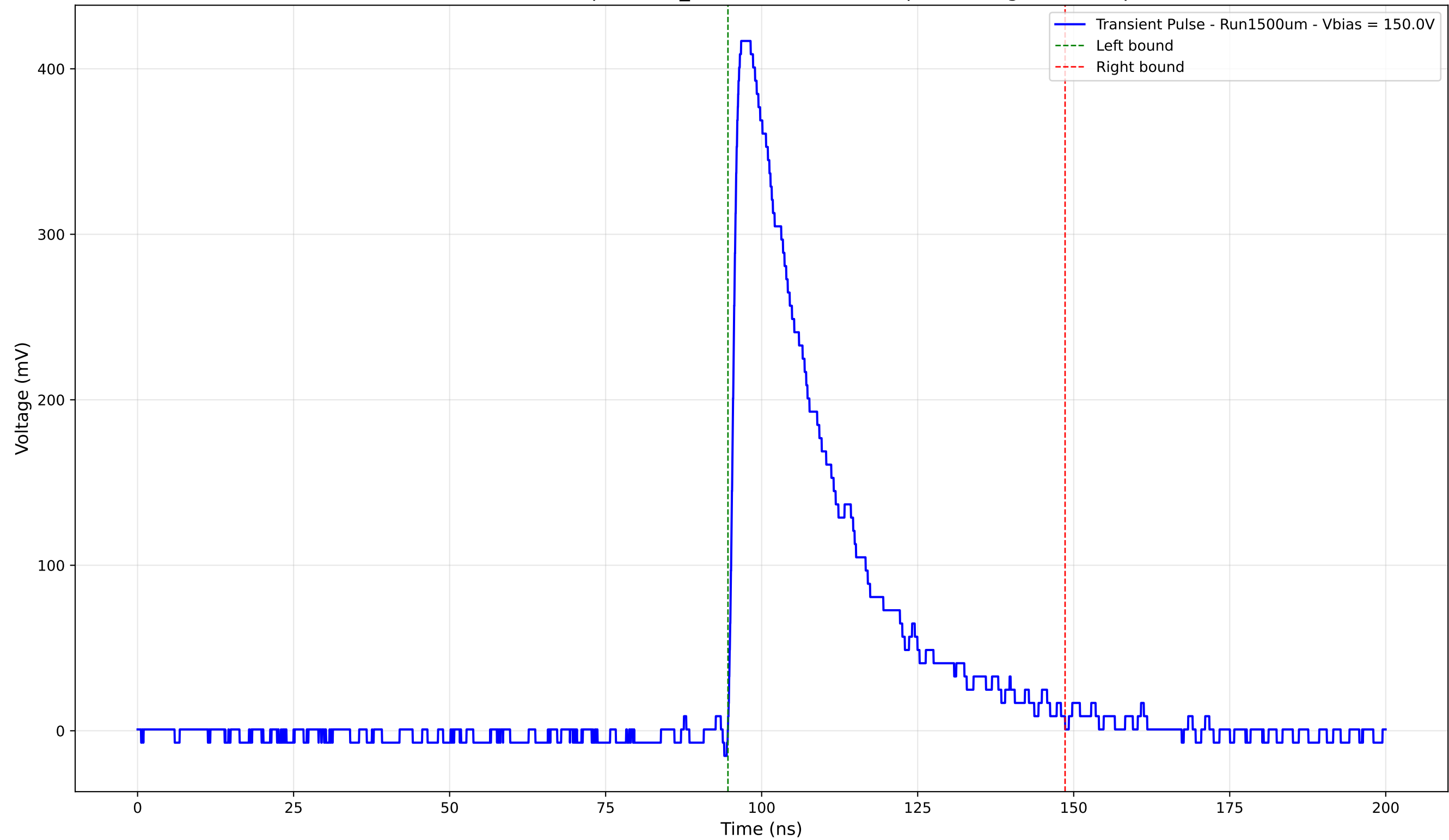
Transient Pulse - Sample: 1cm_42 - Position: 1165.0 \mu\text{m} - Charge: 131.17 pC
