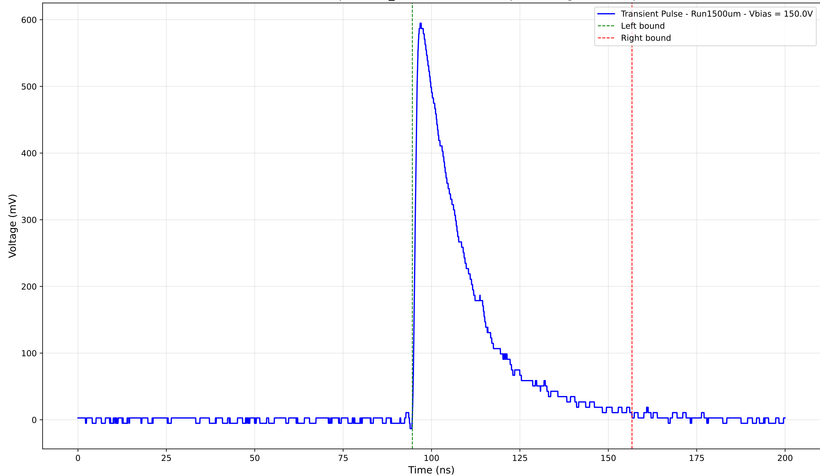
Transient Pulse - Sample: 1cm_42 - Position: 960.0 \mu\text{m} - Charge: 181.08 pC
