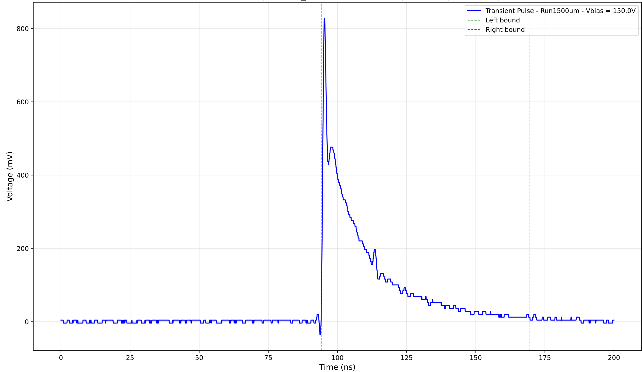
Transient Pulse - Sample: 1cm_42 - Position: 2520.0 \mu\text{m} - Charge: 183.77 pC
