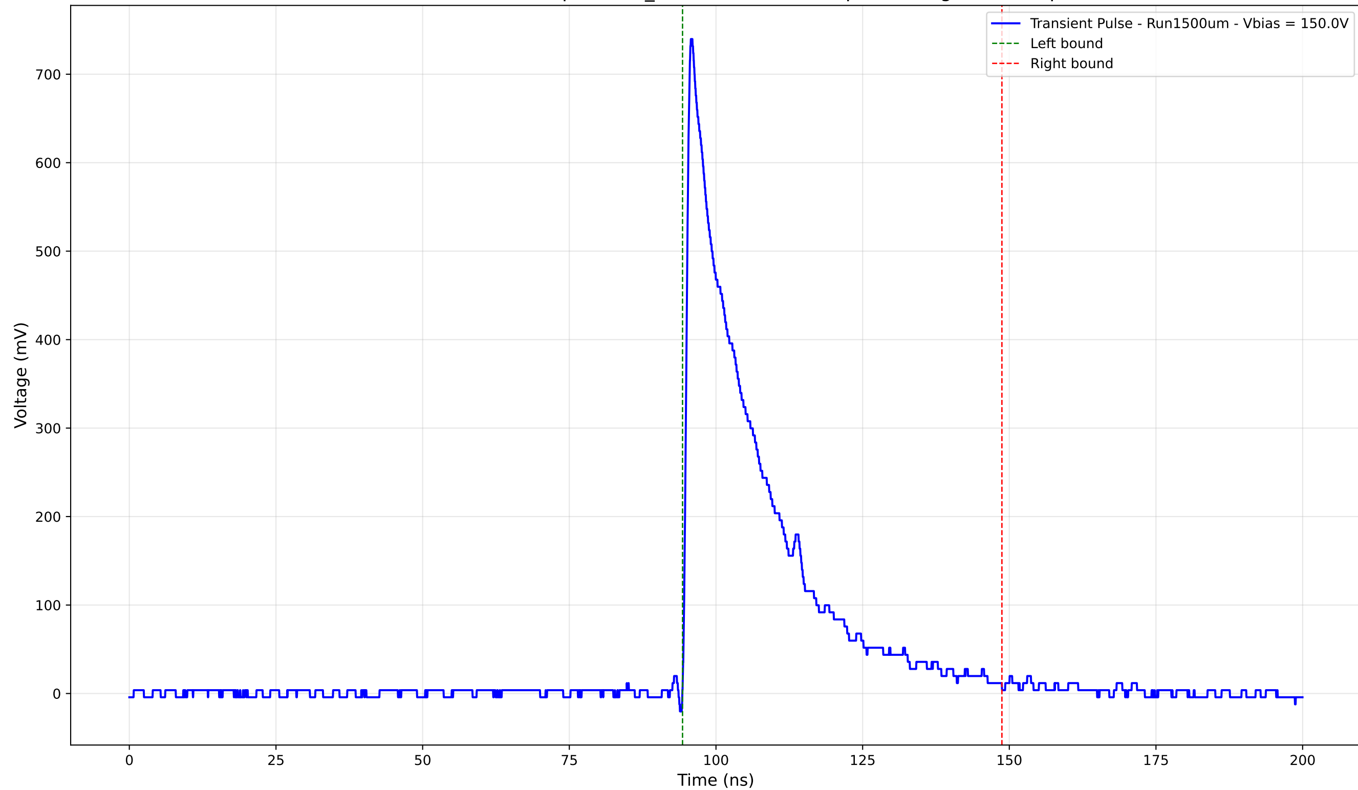
Transient Pulse - Sample: 1cm_42 - Position: 320.0 \mu\text{m} - Charge: 178.27 pC
