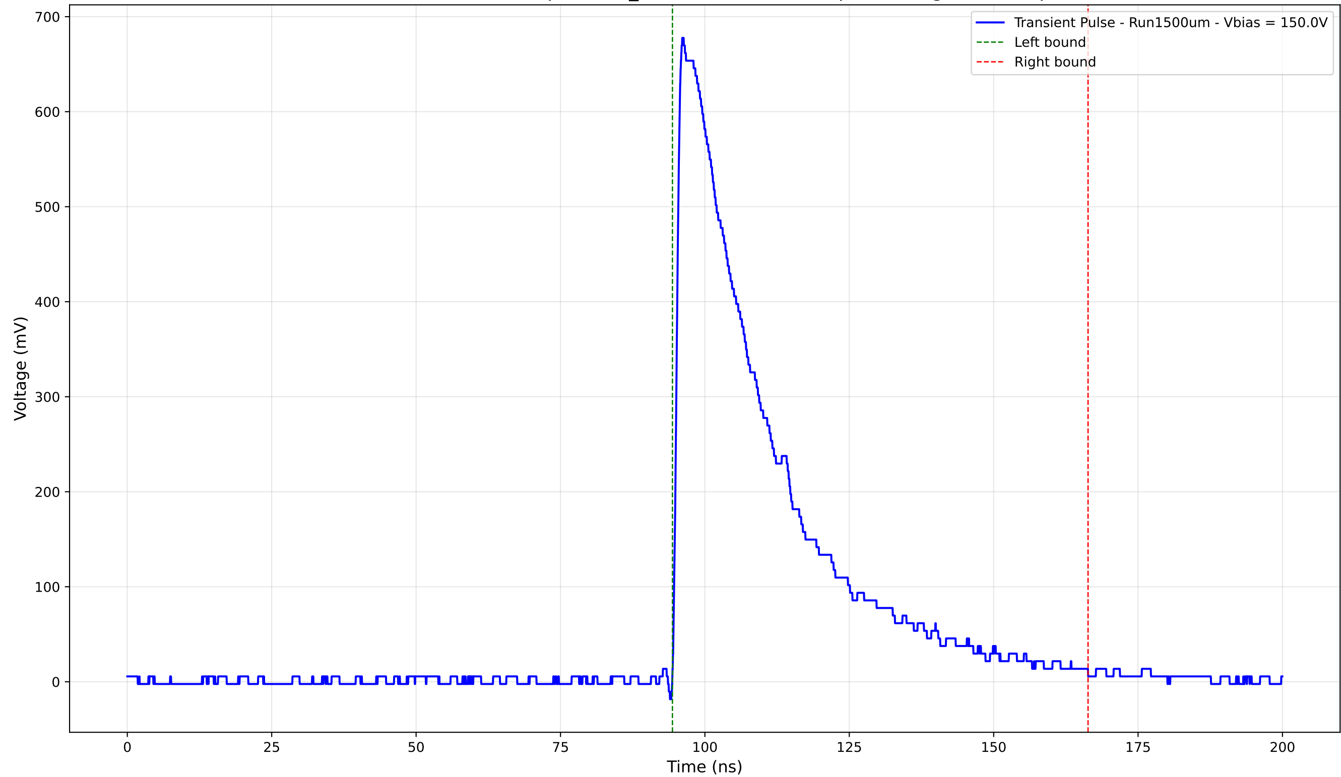
Transient Pulse - Sample: 1cm_42 - Position: 3415.0 \mu\text{m} - Charge: 234.53 pC
