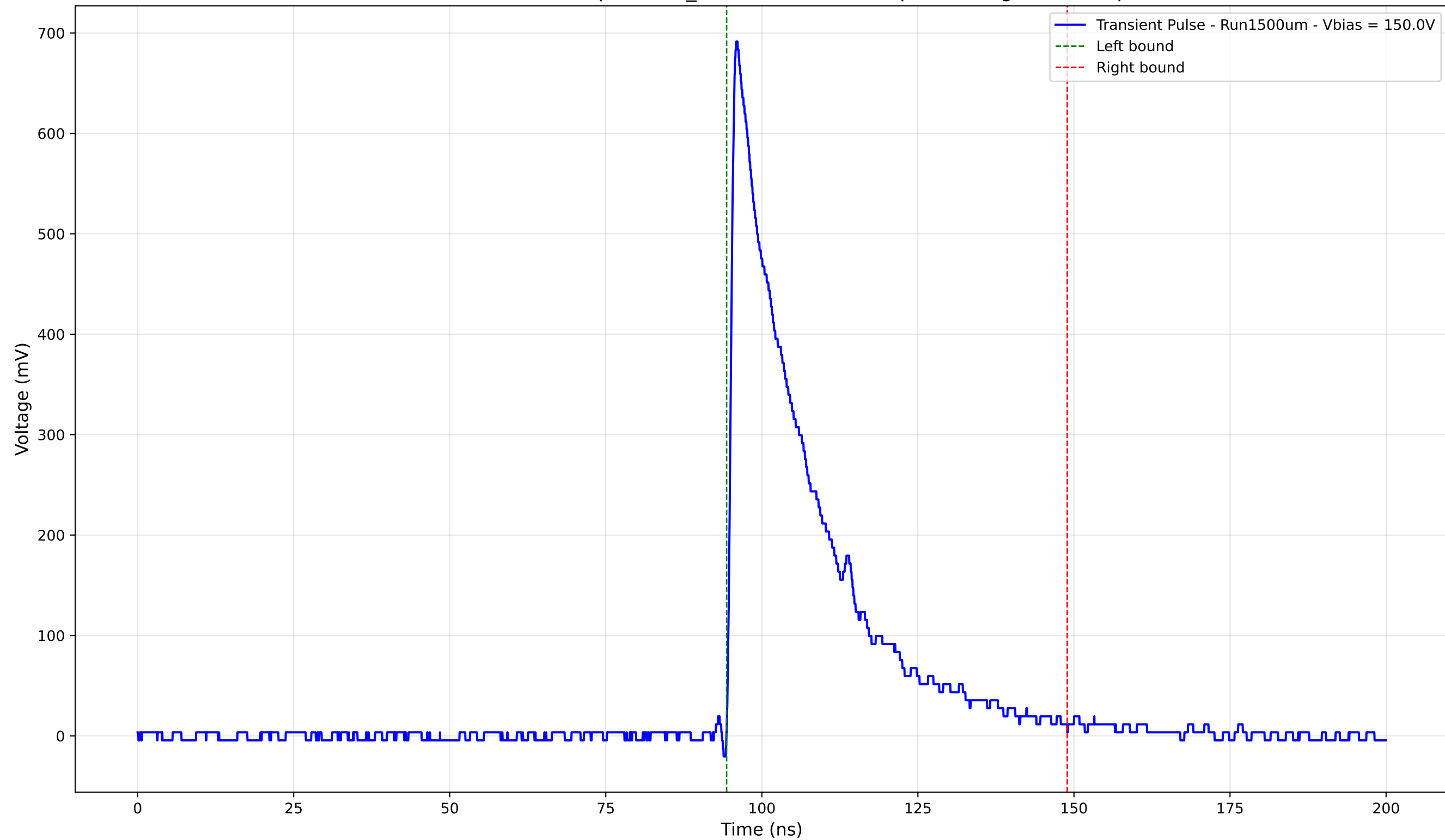
Transient Pulse - Sample: 1cm_42 - Position: 425.0 \mu\text{m} - Charge: 176.67 pC
