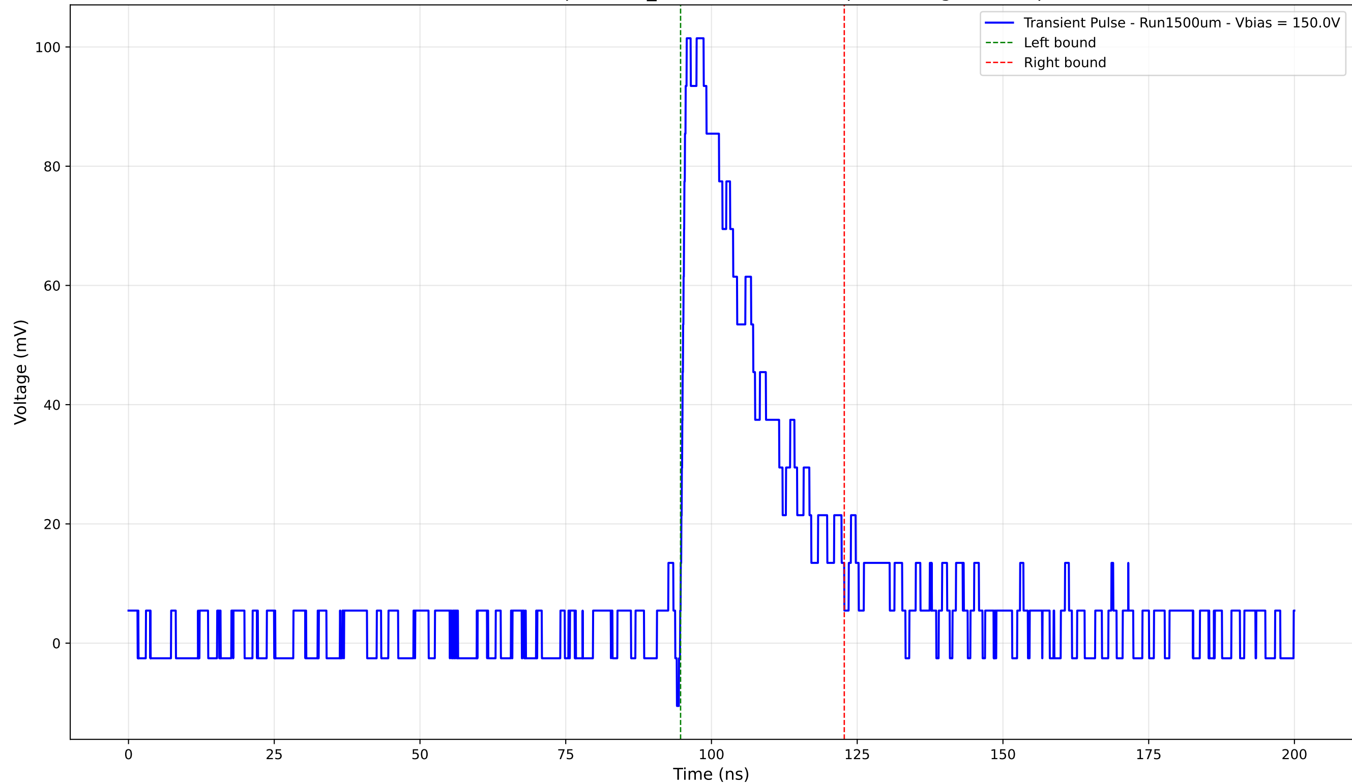
Transient Pulse - Sample: 1cm_42 -Position: 595.0 \mu\text{m} - Charge: 27.63 pC
