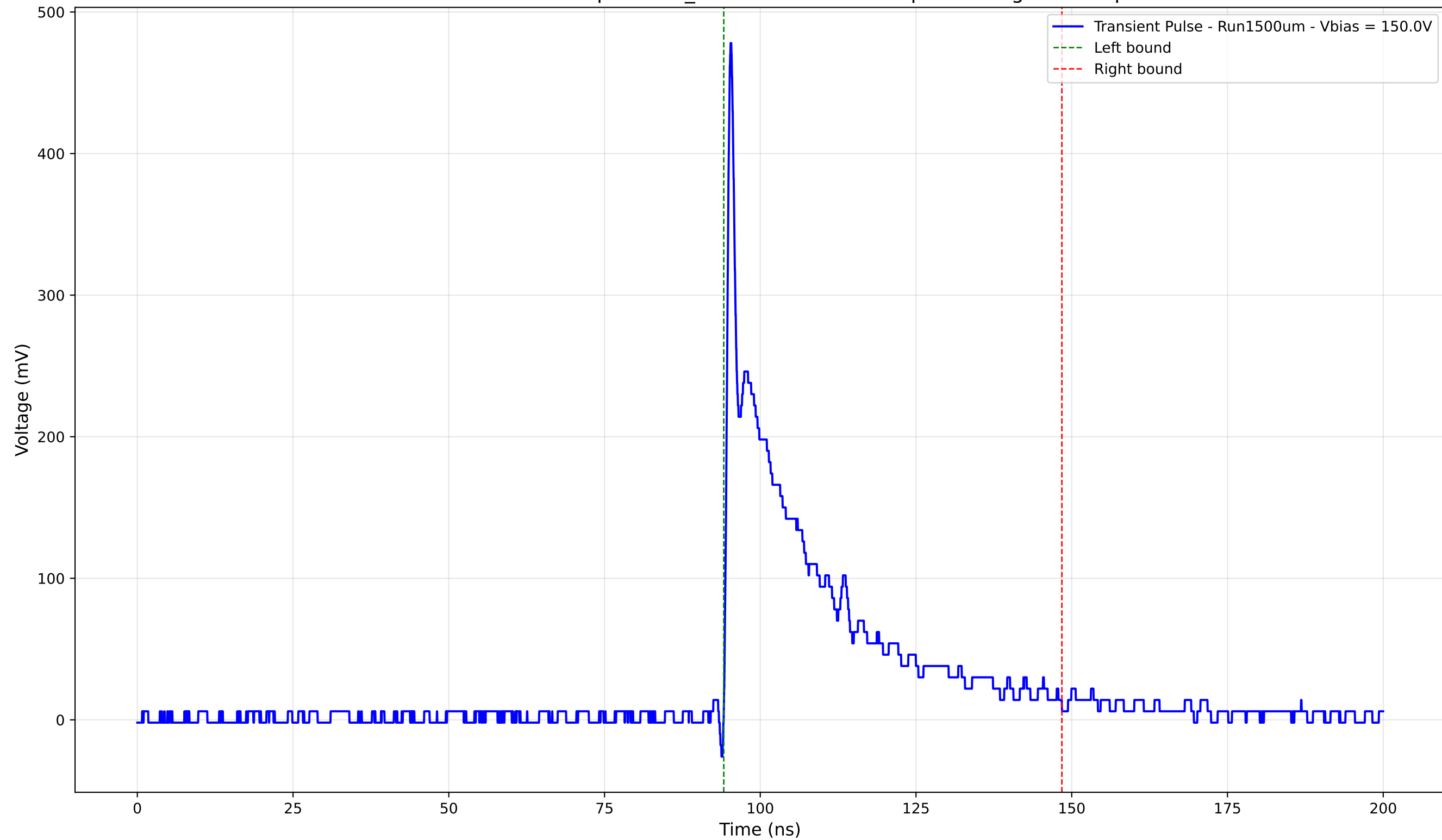
Transient Pulse - Sample: 1cm_42 - Position: 2565.0 \mu\text{m} - Charge: 90.34 pC
