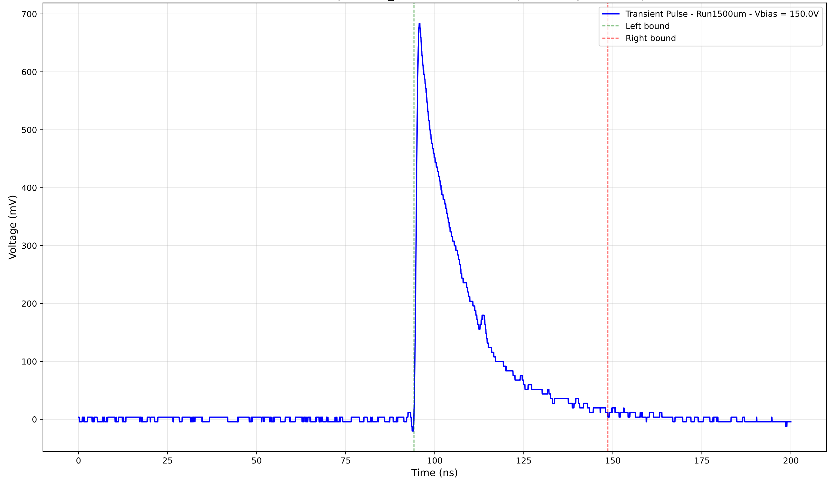
Transient Pulse - Sample: 1cm_42 - Position: 4730.0 \mu\text{m} - Charge: 174.94 pC
