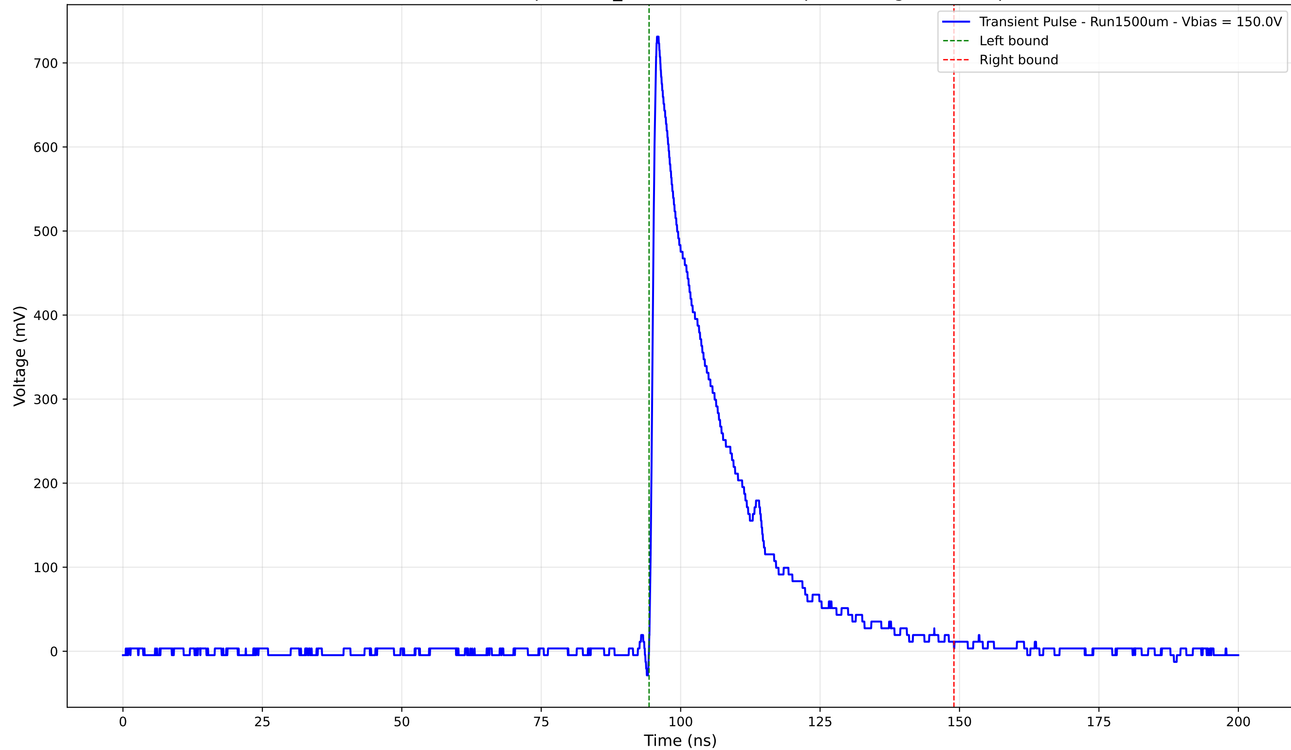
Transient Pulse - Sample: 1cm_42 - Position: 355.0 \mu\text{m} - Charge: 178.61 pC
