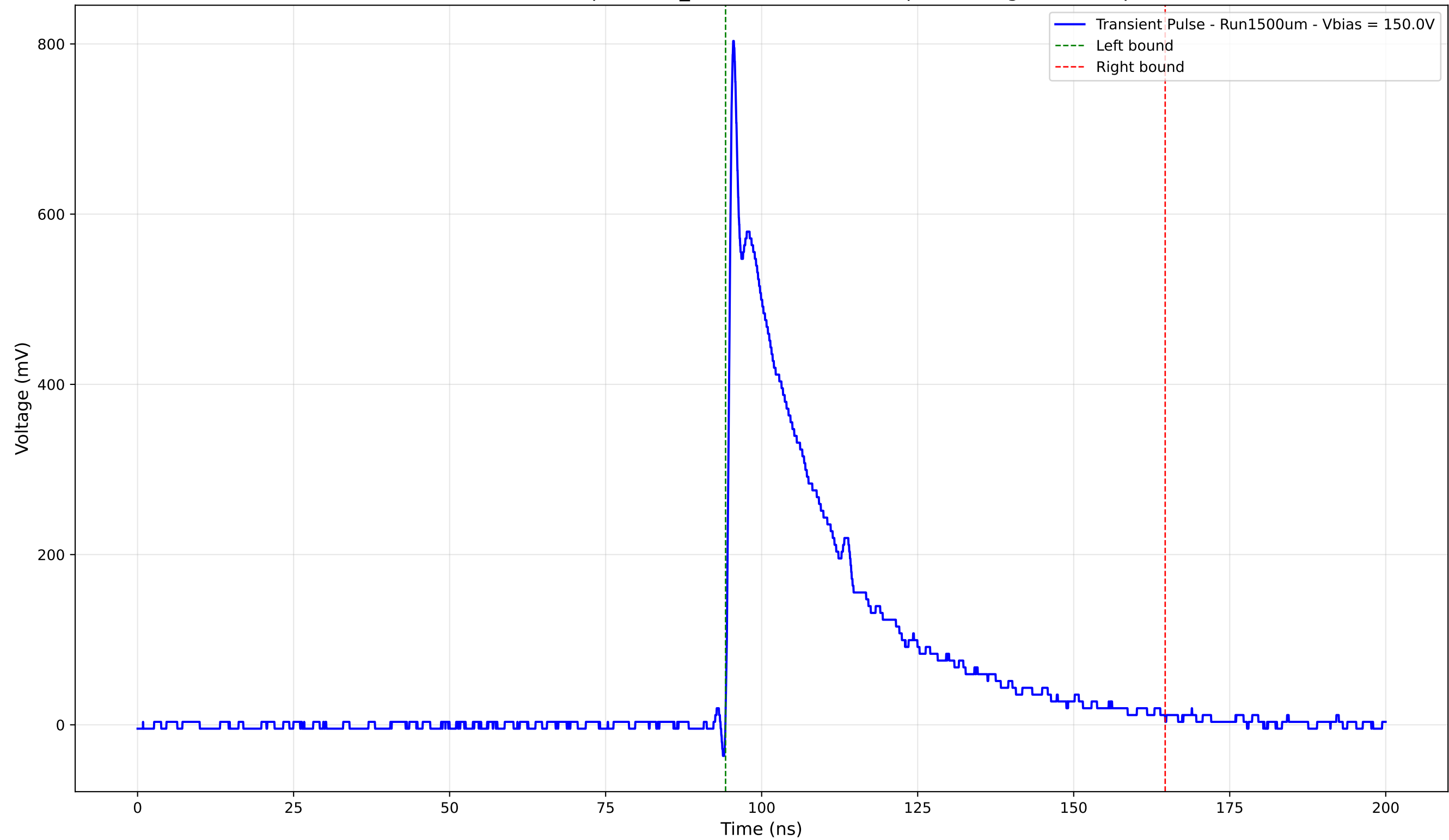
Transient Pulse - Sample: 1cm_42 - Position: 2925.0 \mu\text{m} - Charge: 214.28 pC
