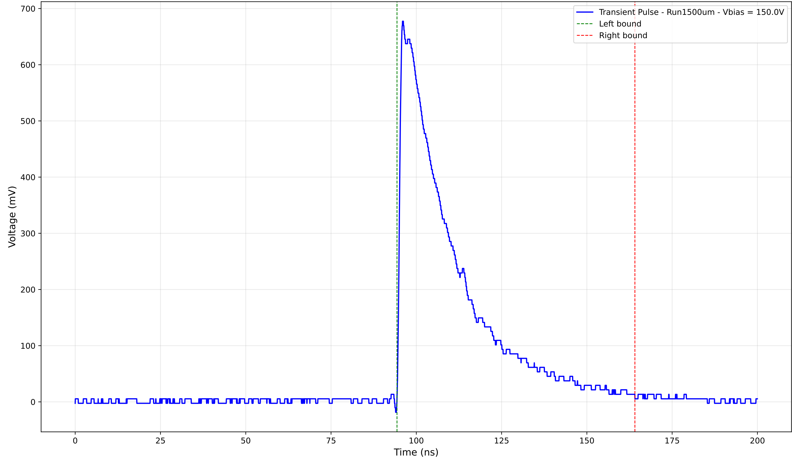
Transient Pulse - Sample: 1cm_42 - Position: 3340.0 \mu\text{m} - Charge: 231.84 pC
