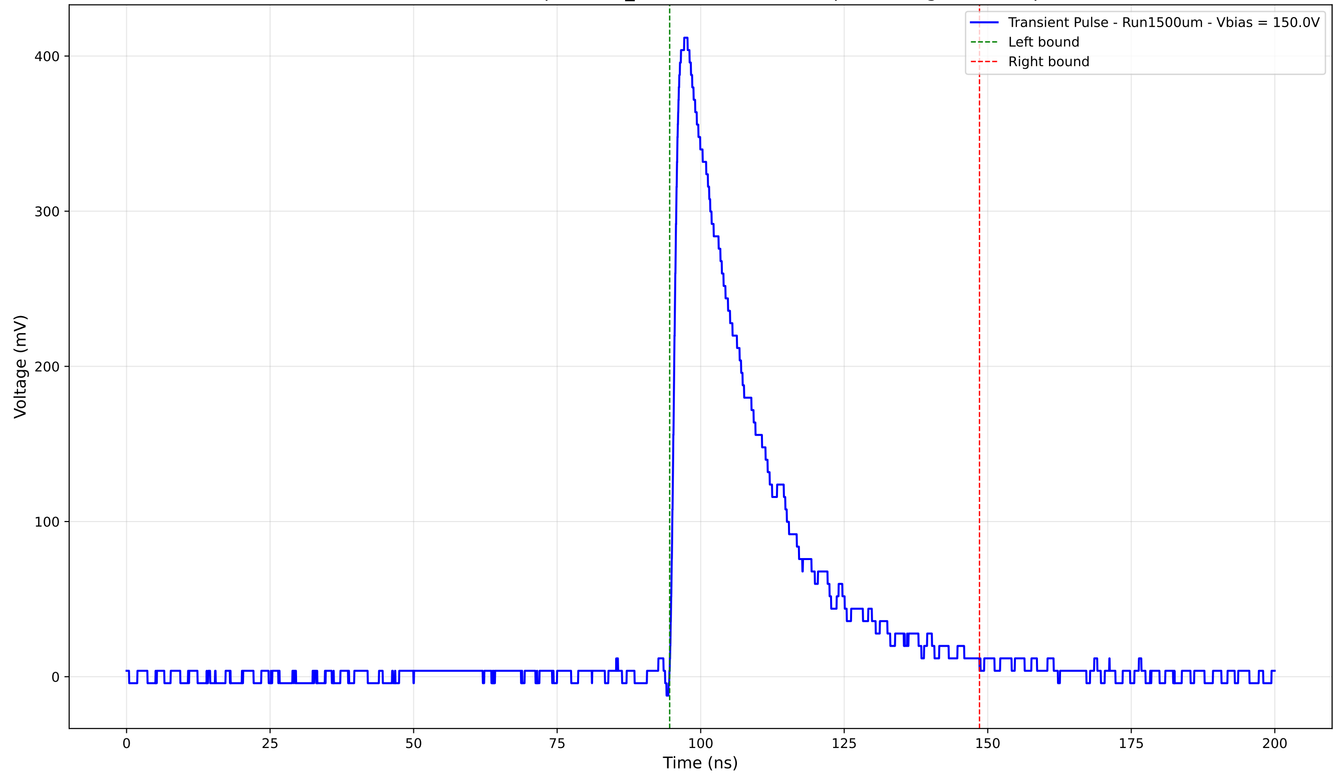
Transient Pulse - Sample: 1cm_42 - Position: 1025.0 \mu\text{m} - Charge: 122.75 pC
