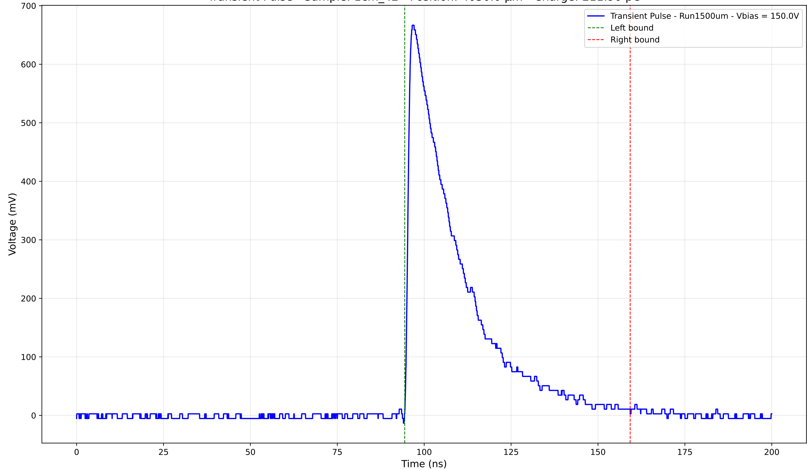
Transient Pulse - Sample: 1cm_42 - Position: 4030.0 \mu\text{m} - Charge: 211.90 pC
