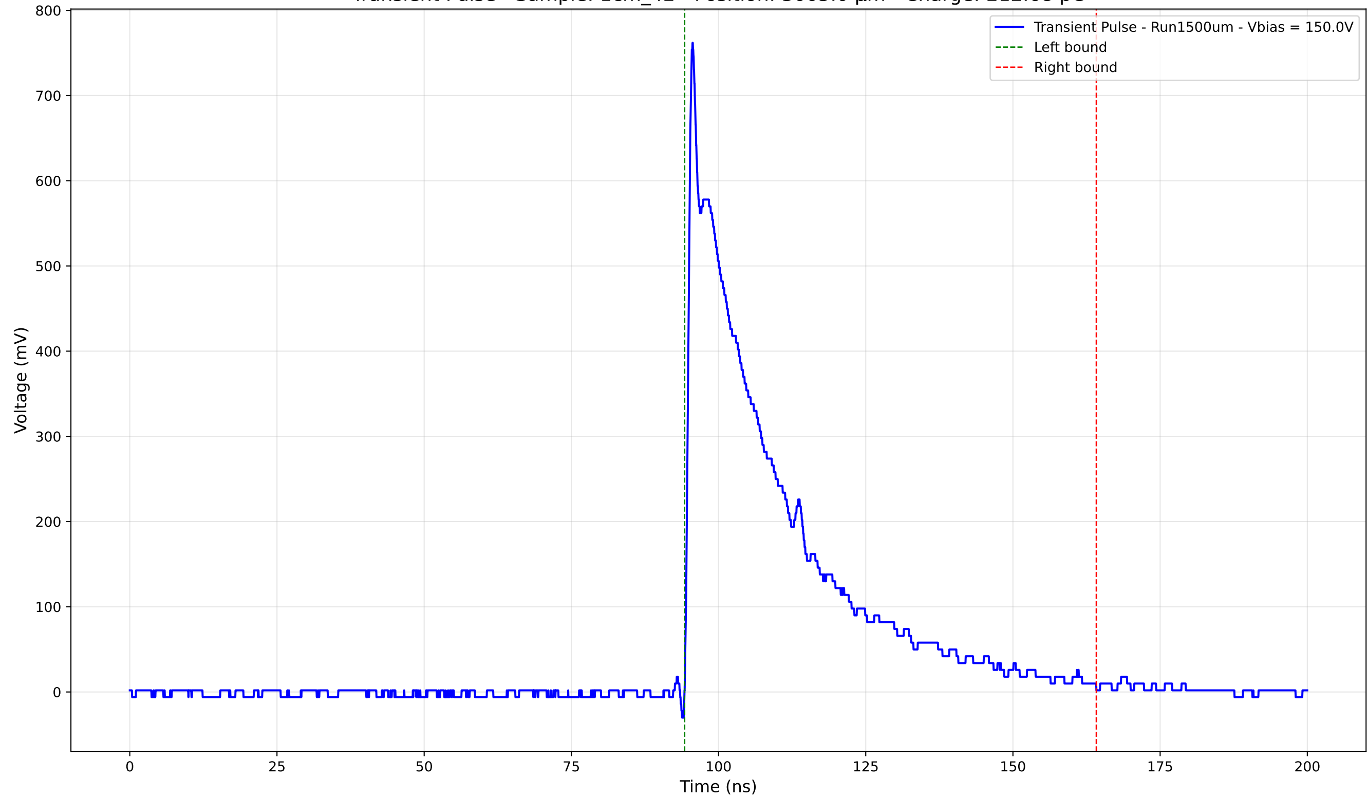
Transient Pulse - Sample: 1cm_42 - Position: 3005.0 \mu\text{m} - Charge: 212.68 pC
