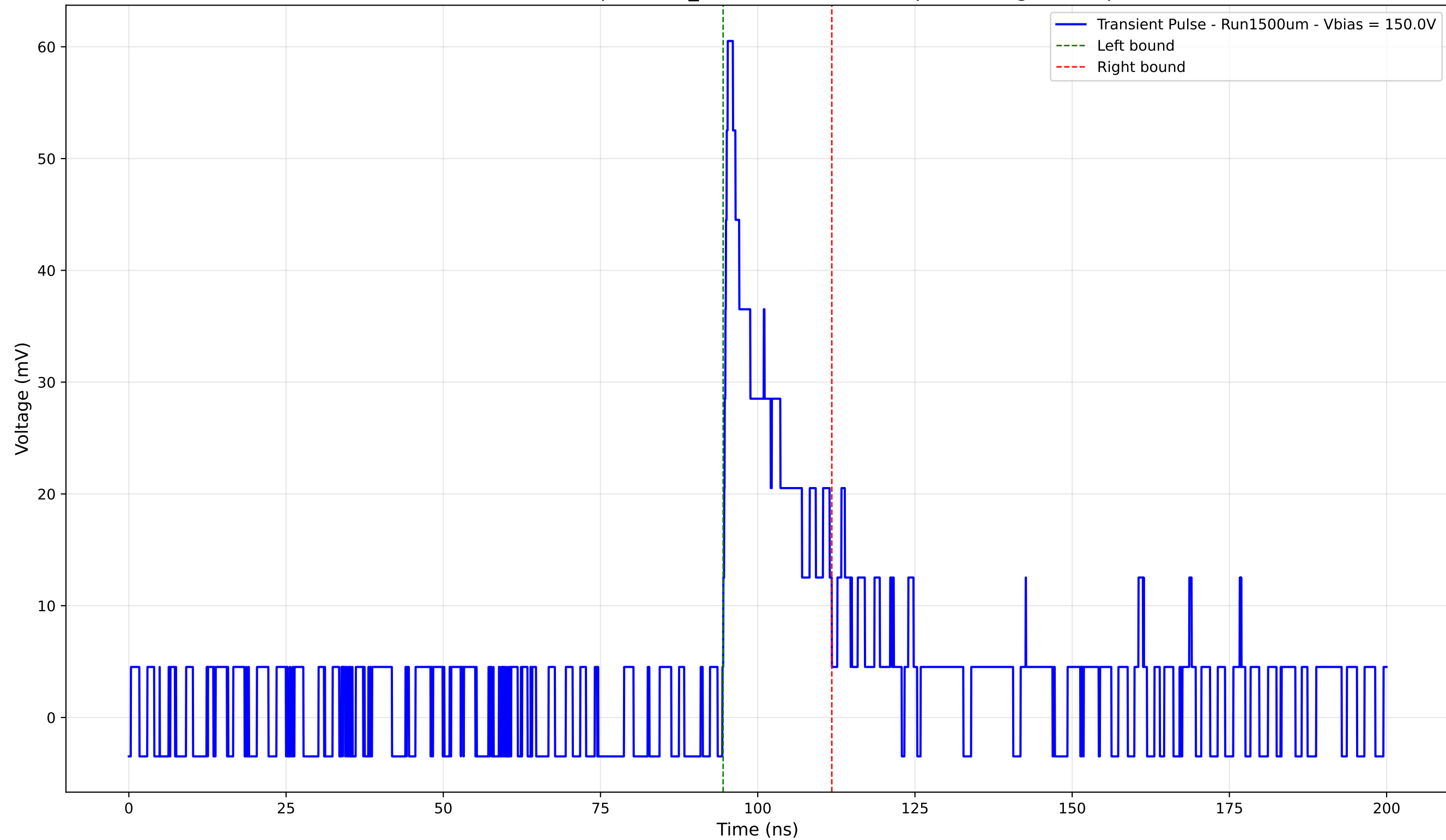
Transient Pulse - Sample: 1cm_42 - Position: 4955.0 \mu\text{m} - Charge: 9.37 pC
