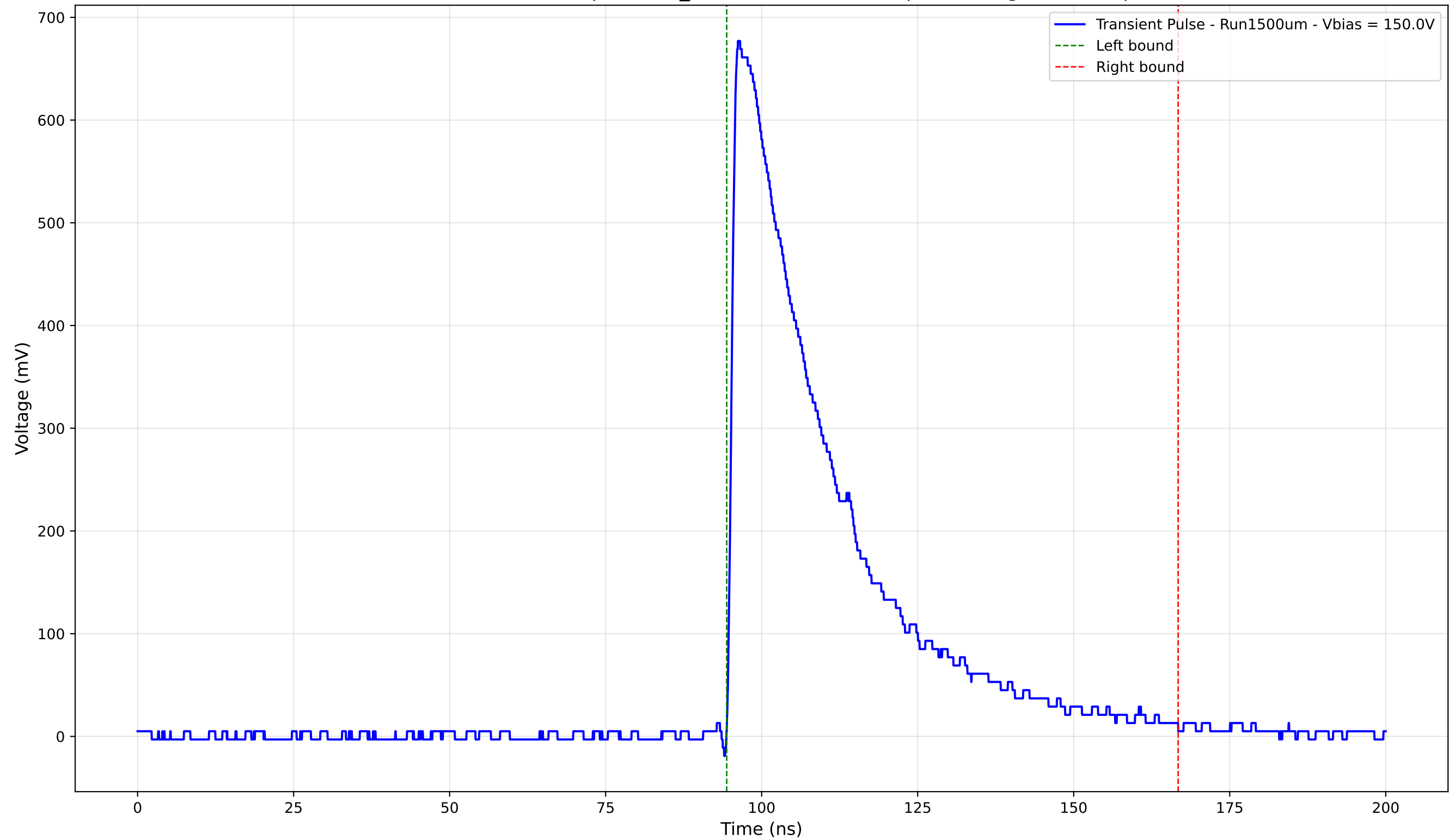
Transient Pulse - Sample: 1cm_42 - Position: 3495.0 \mu\text{m} - Charge: 233.15 pC
