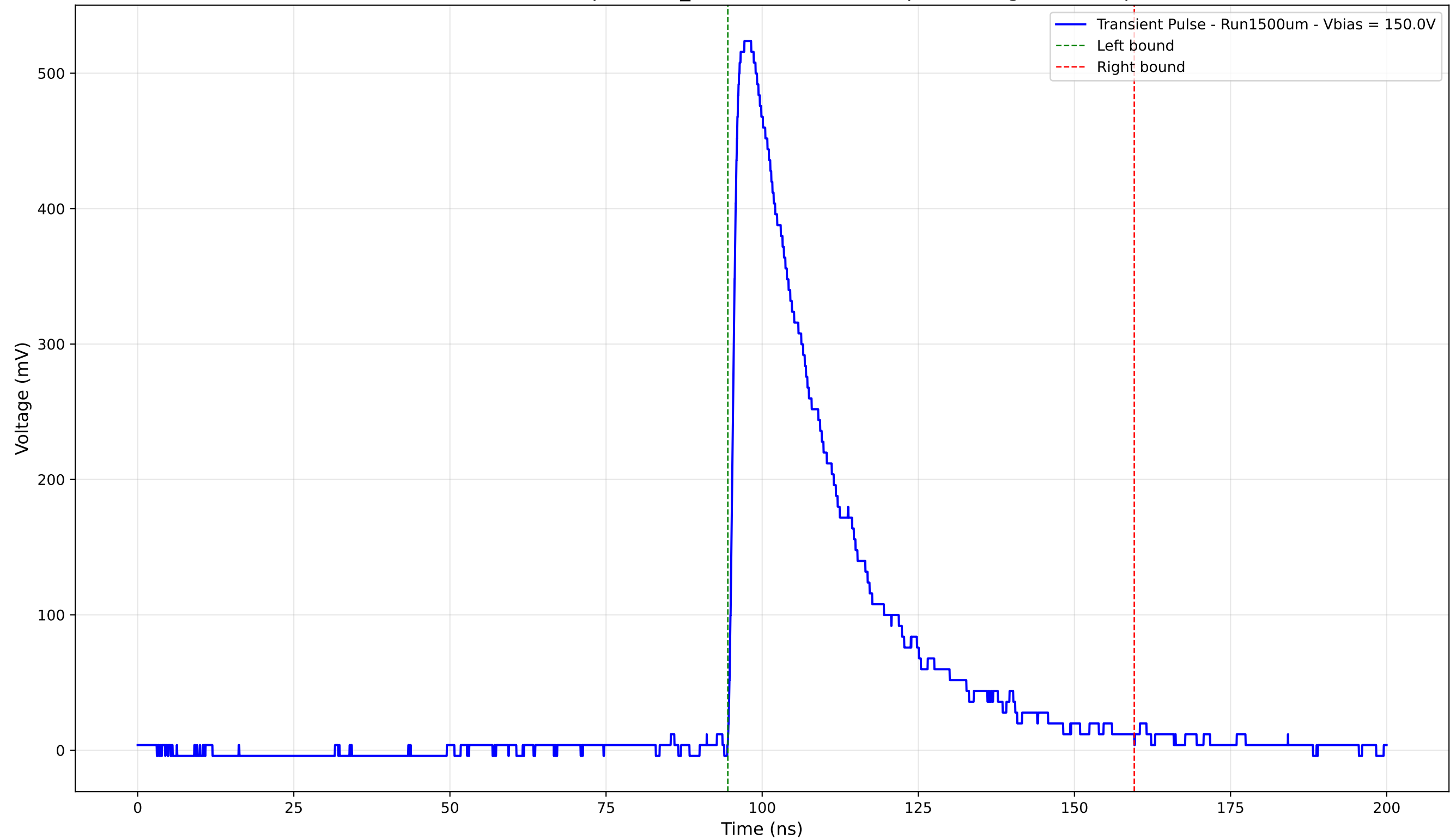
Transient Pulse - Sample: 1cm_42 - Position: 1490.0 \mu\text{m} - Charge: 175.49 pC
