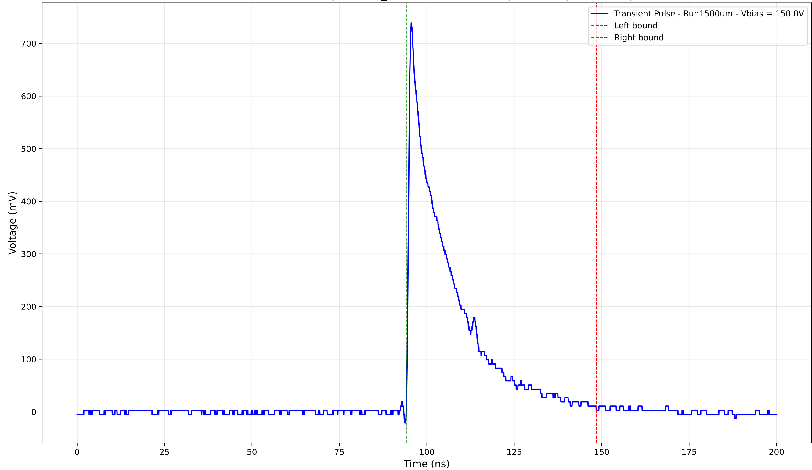
Transient Pulse - Sample: 1cm_42 - Position: 4850.0 \mu\text{m} - Charge: 171.55 pC
