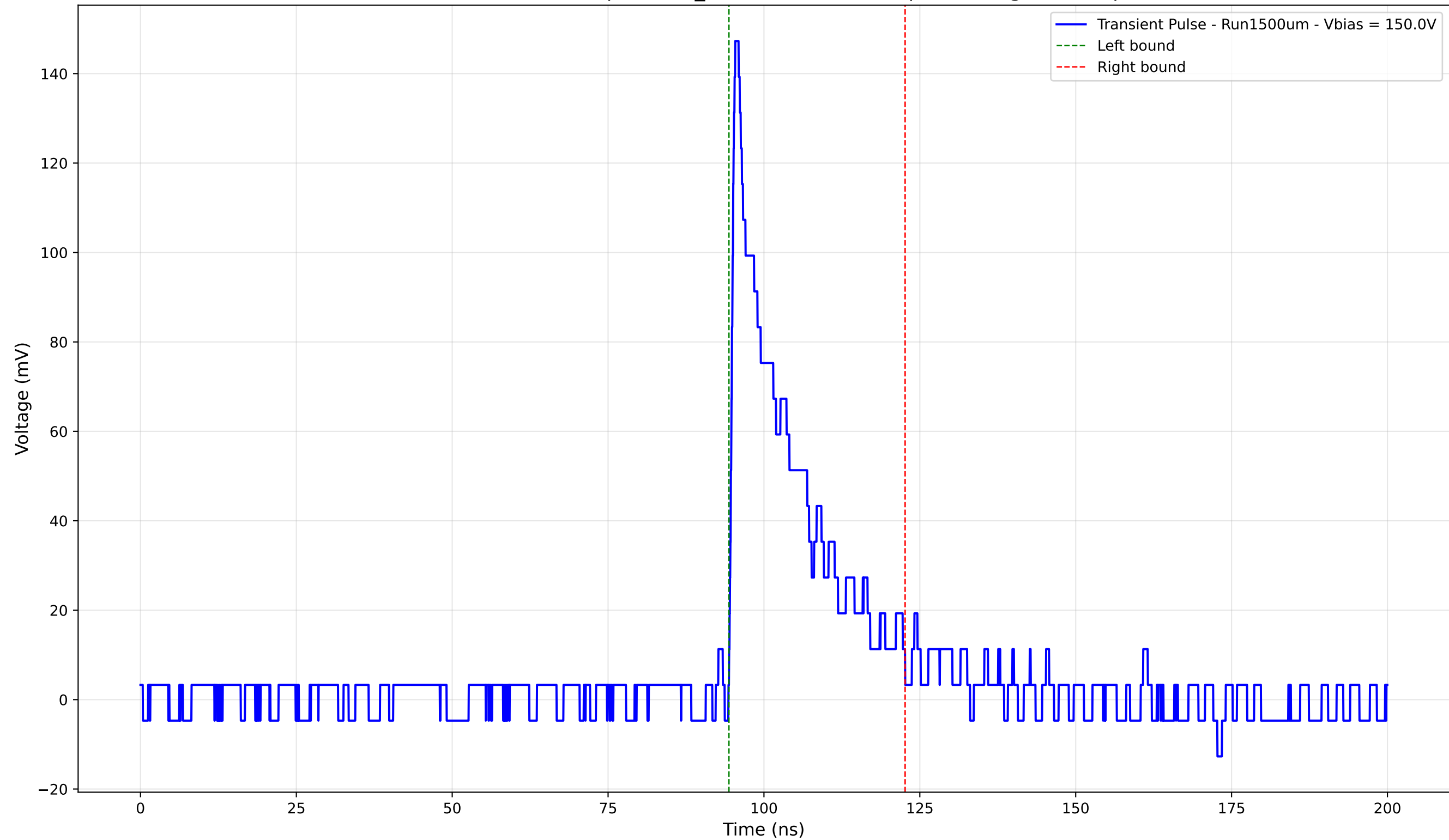
Transient Pulse - Sample: 1cm_42 - Position: 100.0 \mu\text{m} - Charge: 26.98 pC
