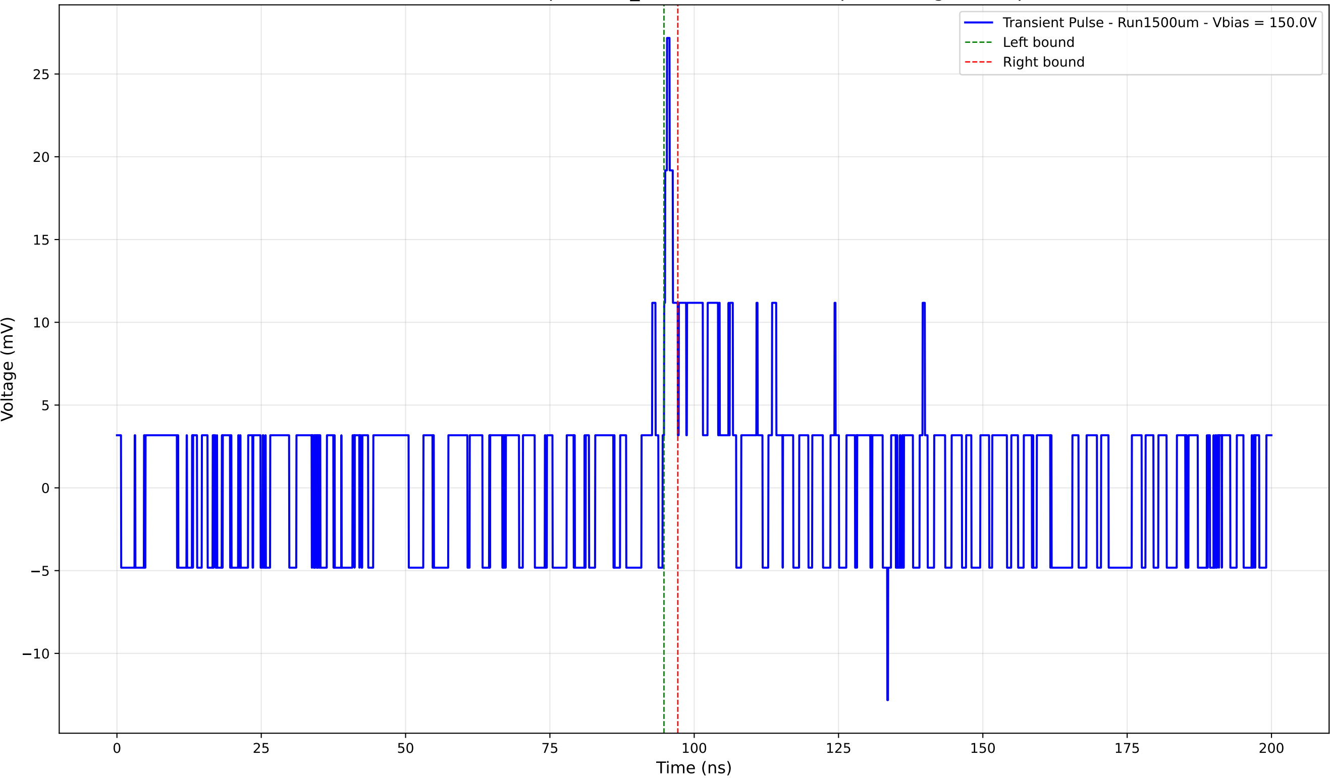
Transient Pulse - Sample: 1cm_42 - Position: 4980.0 \mu\text{m} - Charge: 0.82 pC
