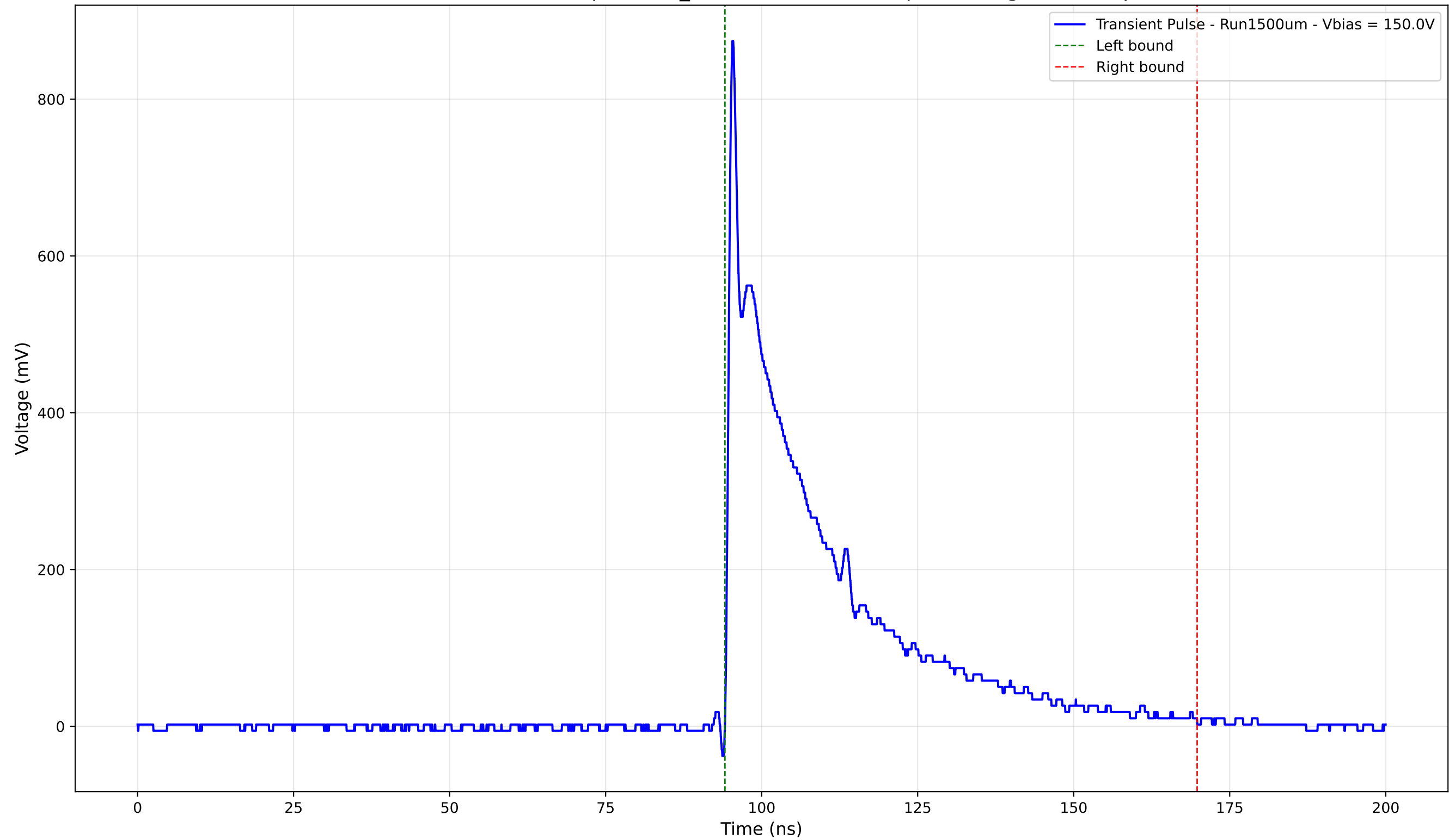
Transient Pulse - Sample: 1cm_42 - Position: 2780.0 \mu\text{m} - Charge: 213.96 pC
