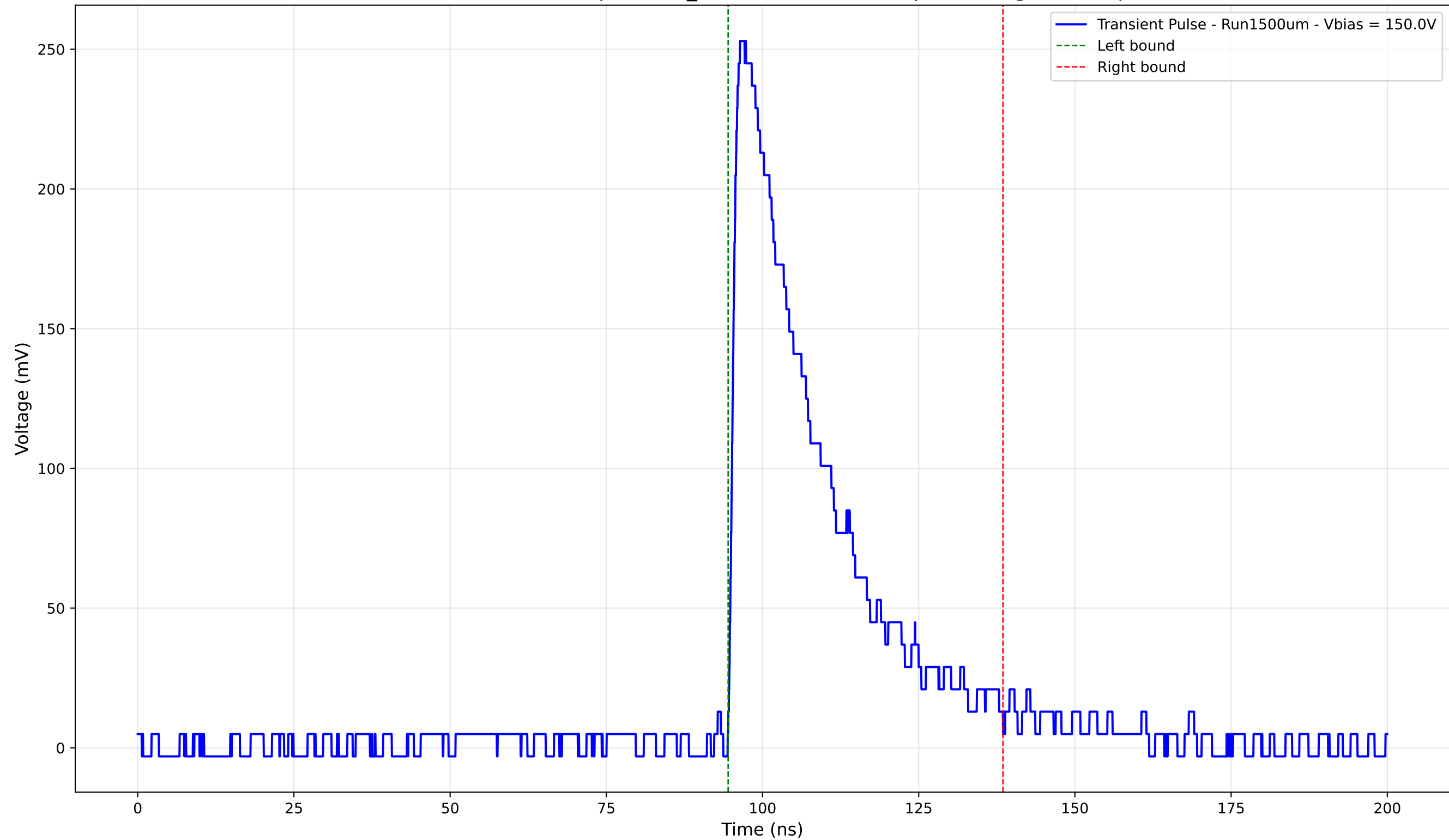
Transient Pulse - Sample: 1cm_42 - Position: 4155.0 \mu\text{m} - Charge: 76.01 pC
