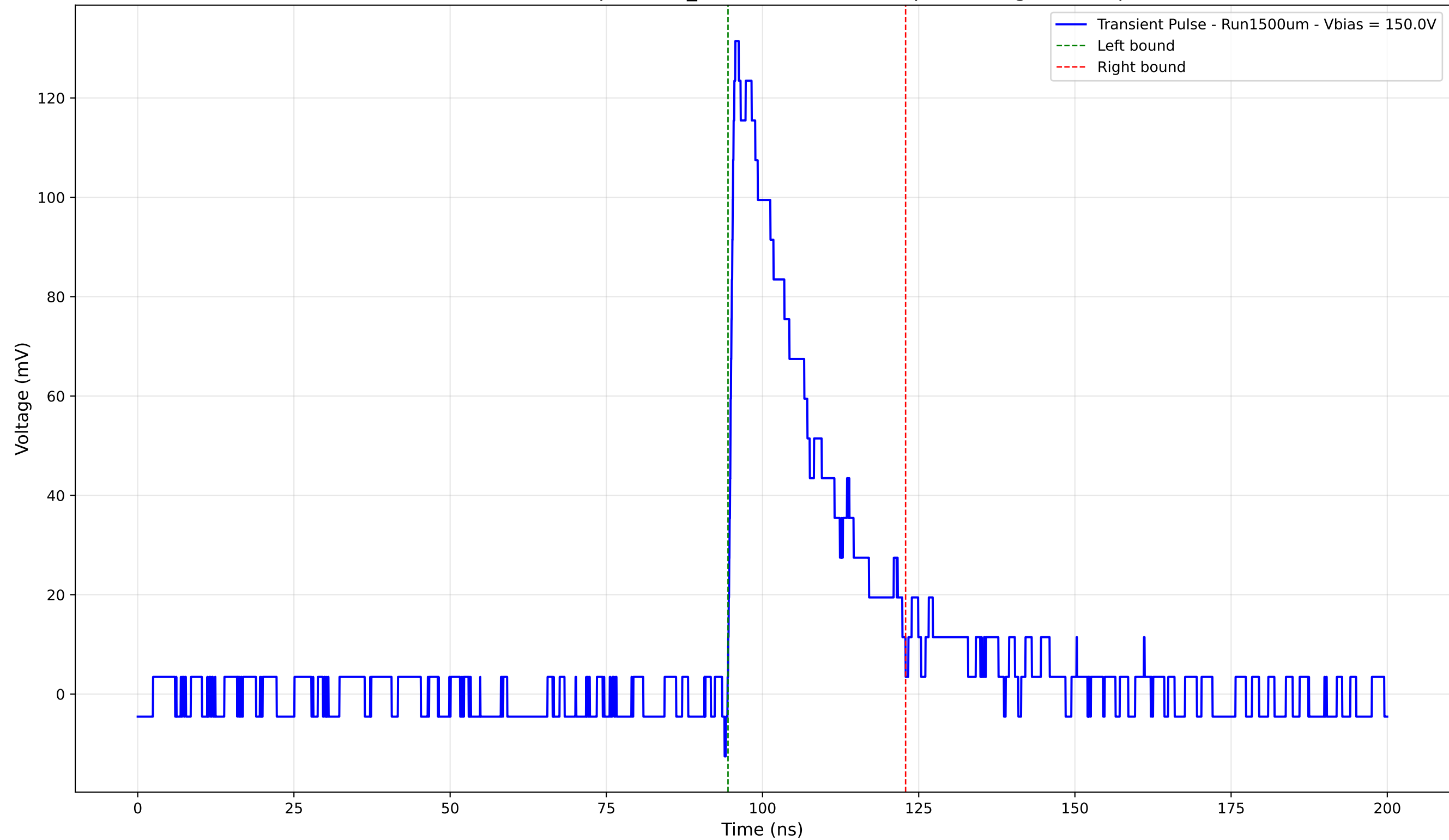
Transient Pulse - Sample: 1cm_42 - Position: 4620.0 \mu\text{m} - Charge: 32.99 pC
