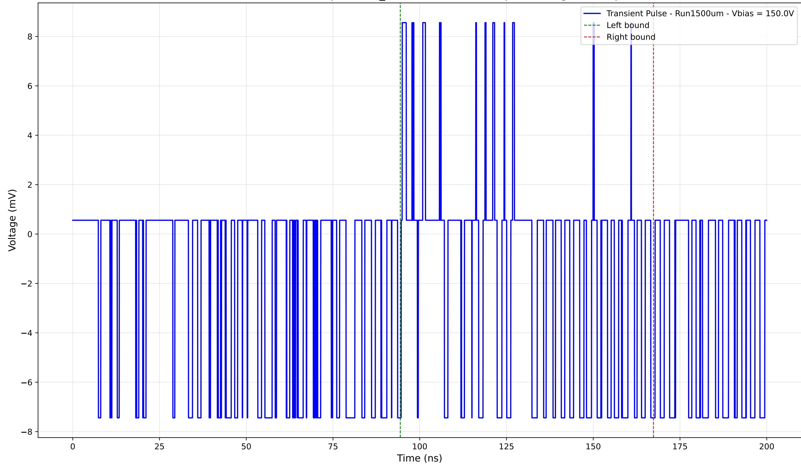
Transient Pulse - Sample: 1cm_42 - Position: 5030.0 \mu\text{m} - Charge: -2.00 pC
