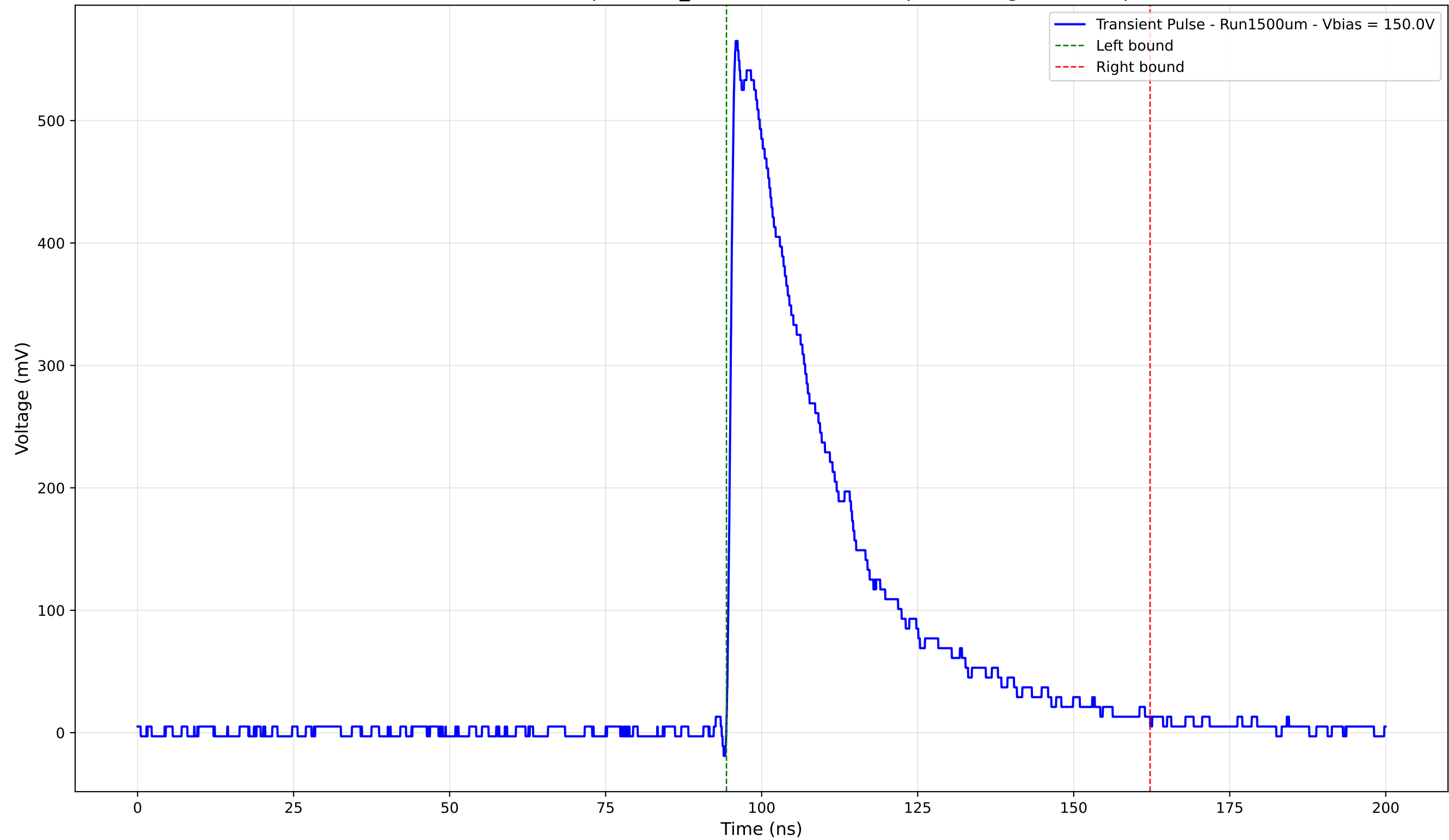
Transient Pulse - Sample: 1cm_42 - Position: 1905.0 \mu\text{m} - Charge: 194.43 pC
