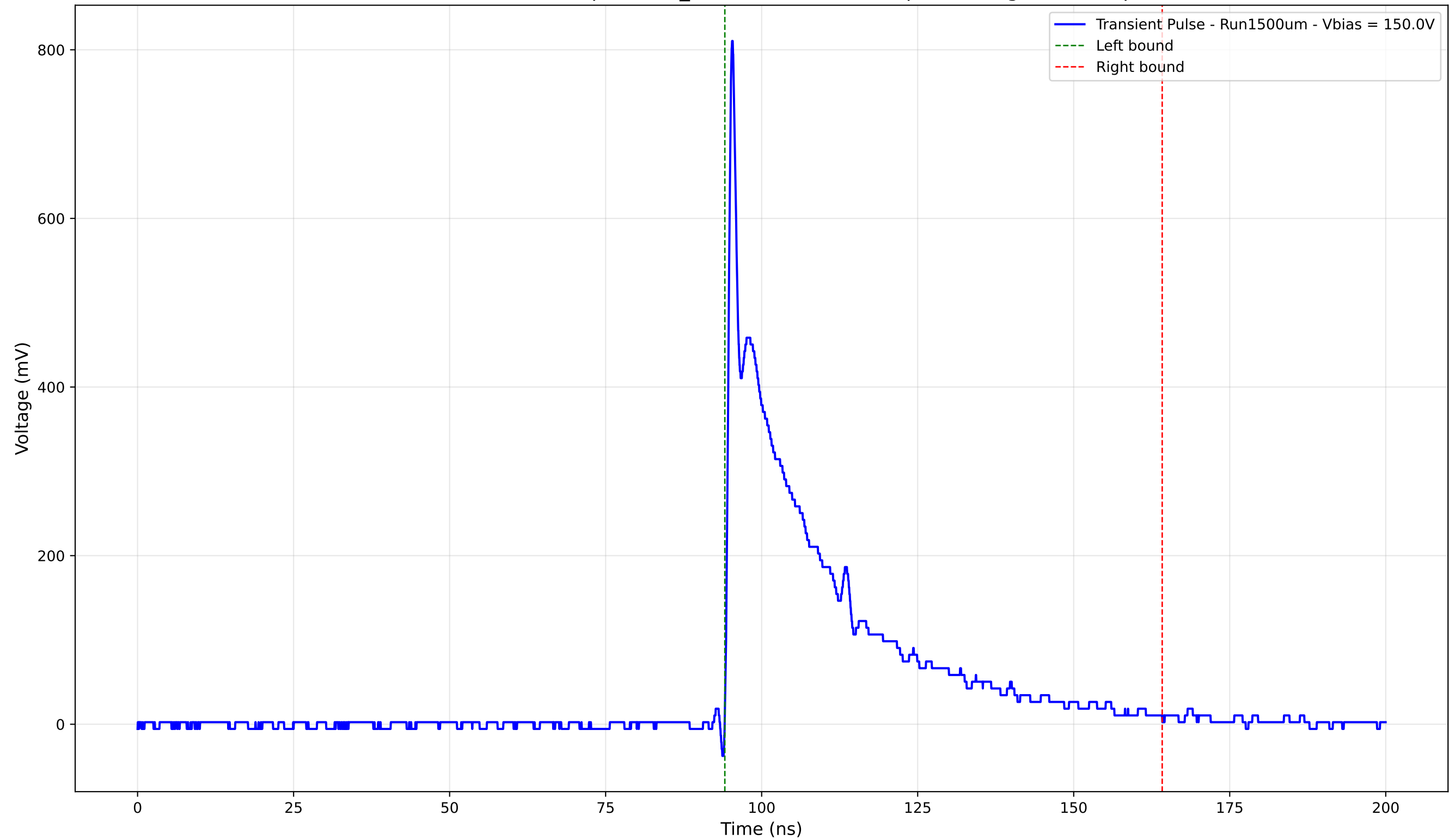
Transient Pulse - Sample: 1cm_42 - Position: 2525.0 \mu\text{m} - Charge: 172.99 pC
