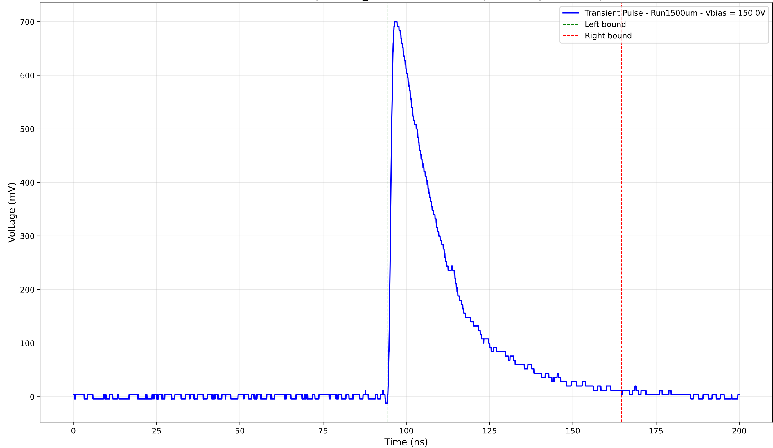
Transient Pulse - Sample: 1cm_42 - Position: 3760.0 \mu\text{m} - Charge: 237.04 pC
