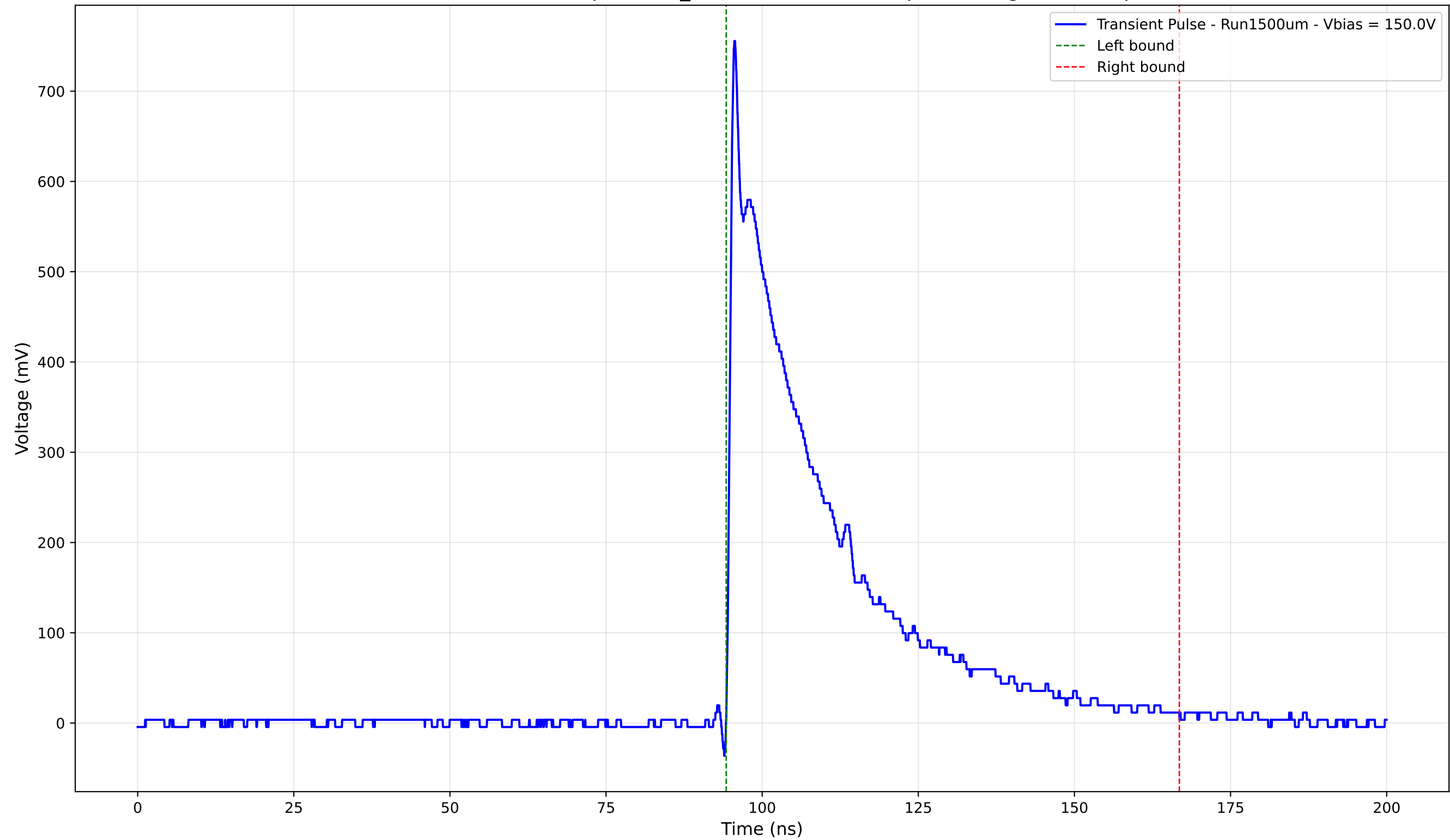
Transient Pulse - Sample: 1cm_42 - Position: 3010.0 \mu\text{m} - Charge: 214.40 pC
