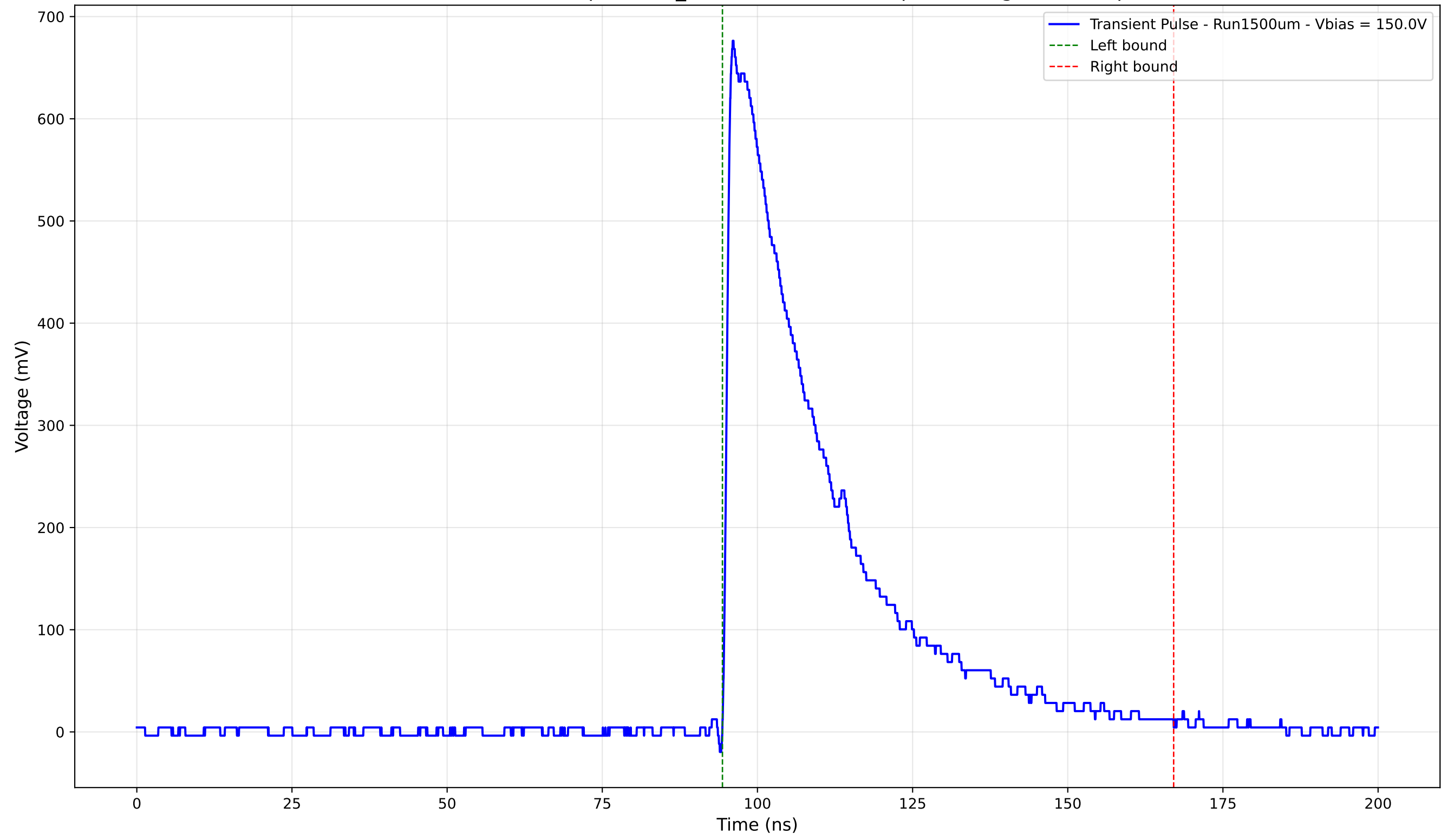
Transient Pulse - Sample: 1cm_42 - Position: 3345.0 \mu\text{m} - Charge: 229.85 pC
