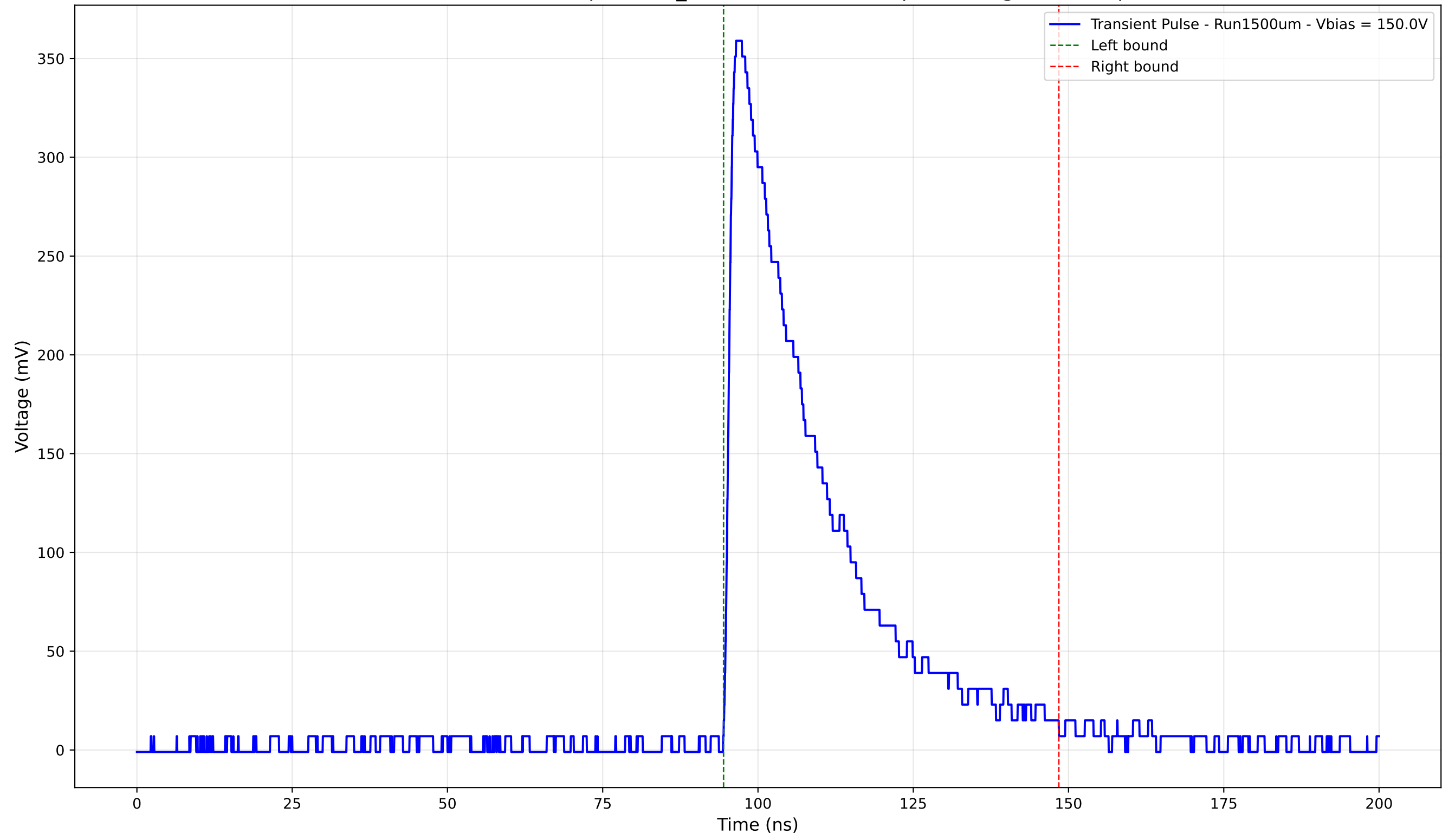
Transient Pulse - Sample: 1cm_42 - Position: 4075.0 \mu\text{m} - Charge: 113.18 pC
