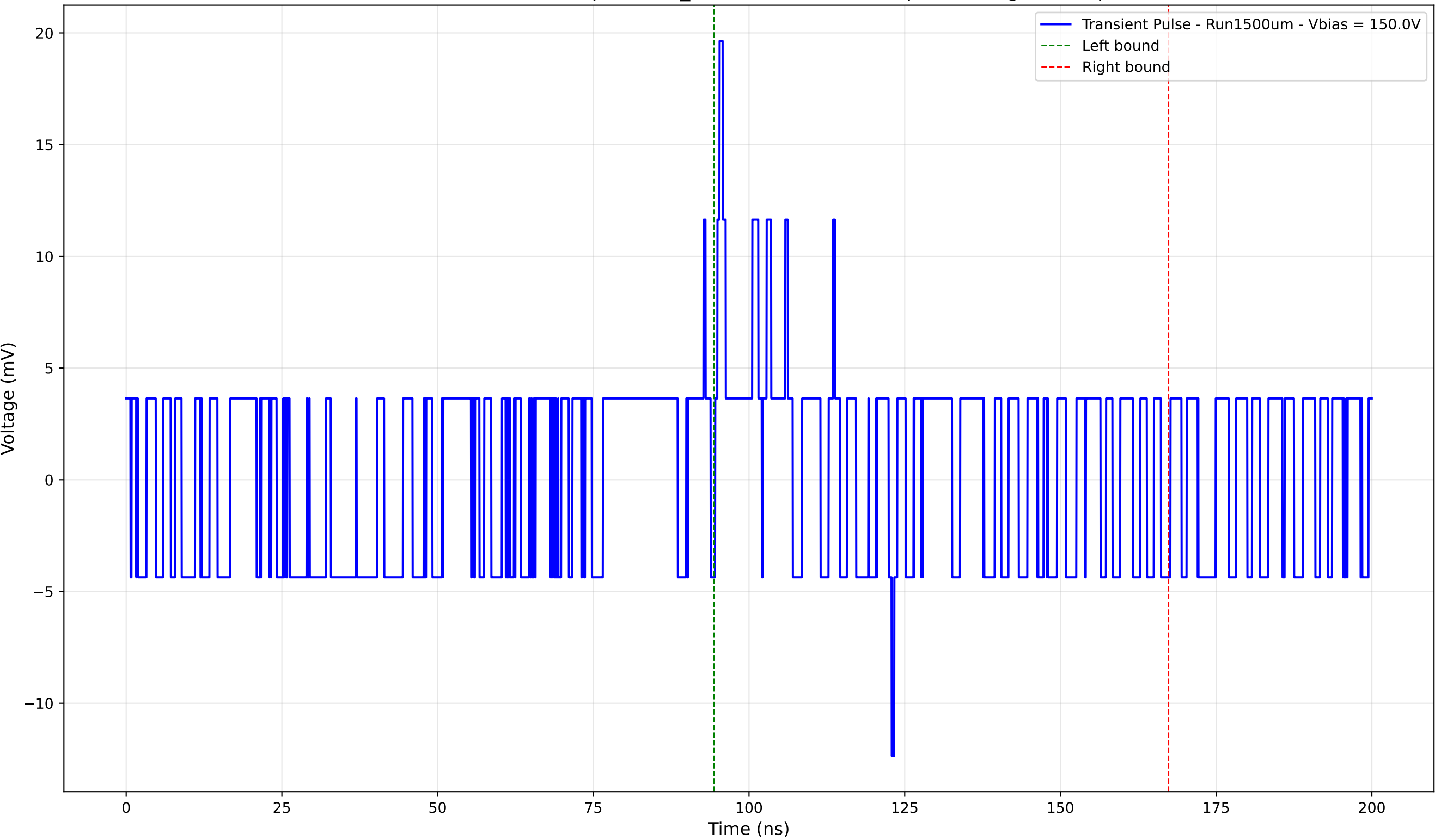
Transient Pulse - Sample: 1cm_42 - Position: 5020.0 \mu\text{m} - Charge: 1.84 pC
