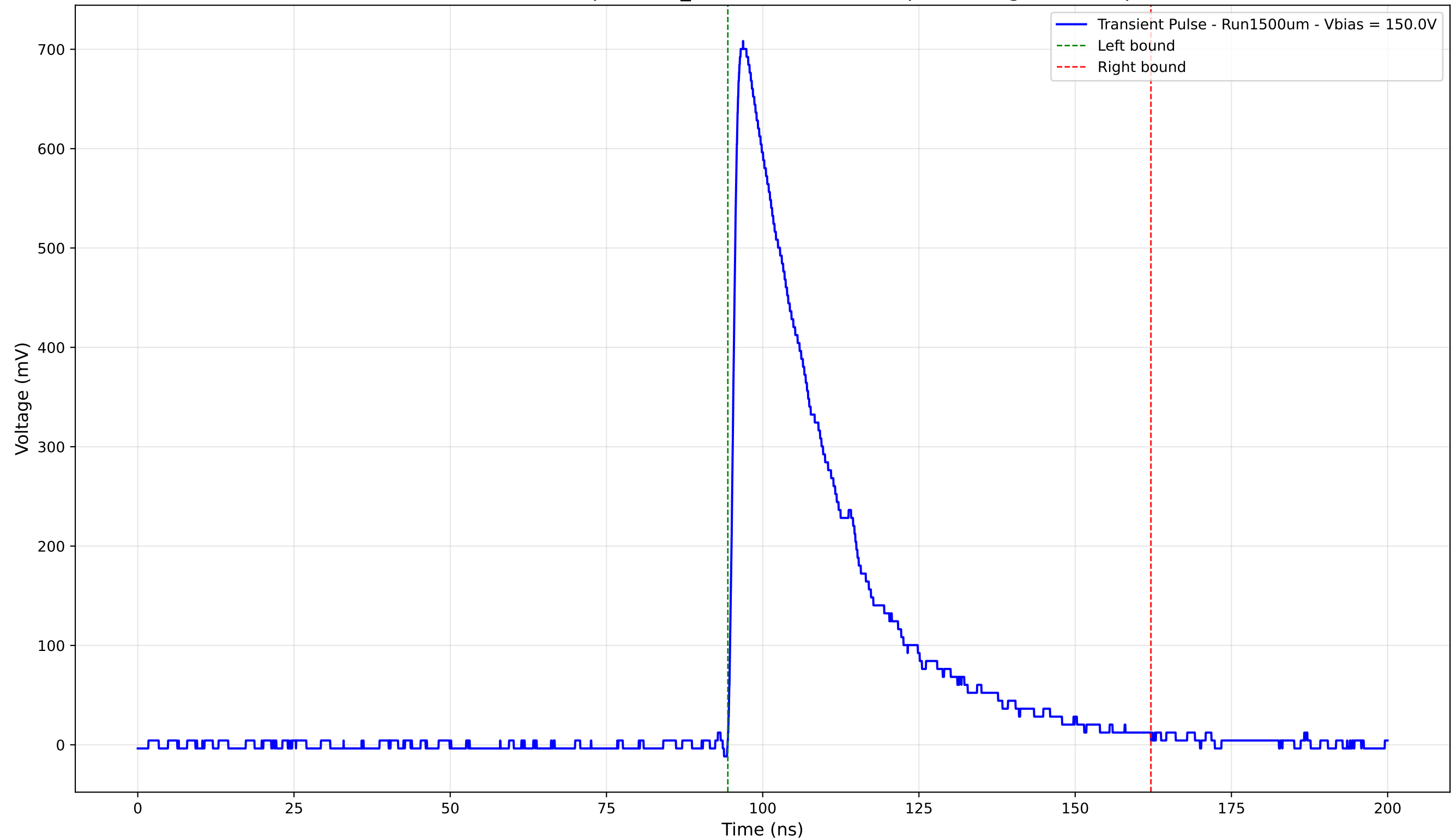
Transient Pulse - Sample: 1cm_42 - Position: 4015.0 \mu\text{m} - Charge: 228.13 pC
