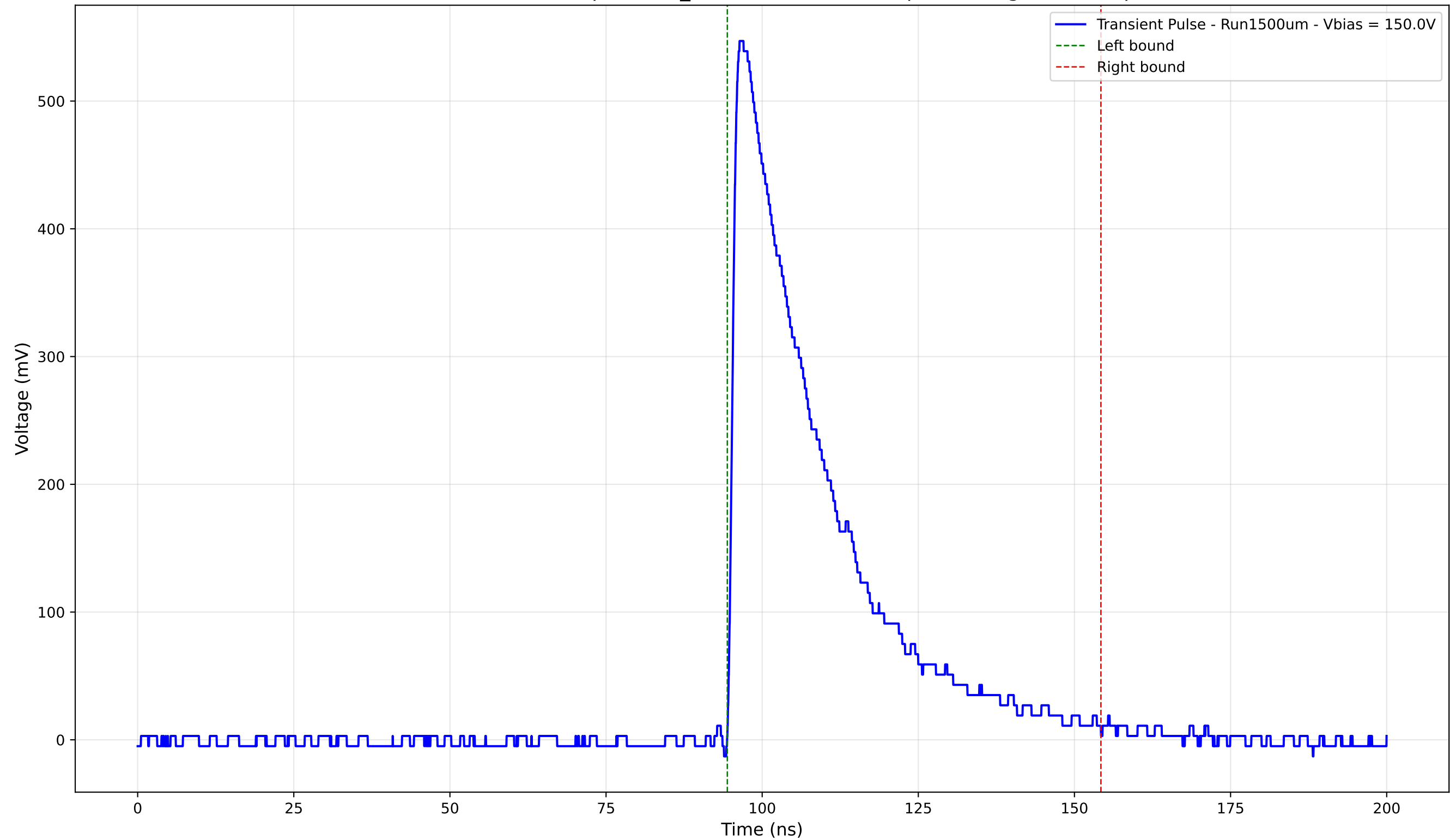
Transient Pulse - Sample: 1cm_42 - Position: 4195.0 \mu\text{m} - Charge: 168.63 pC
