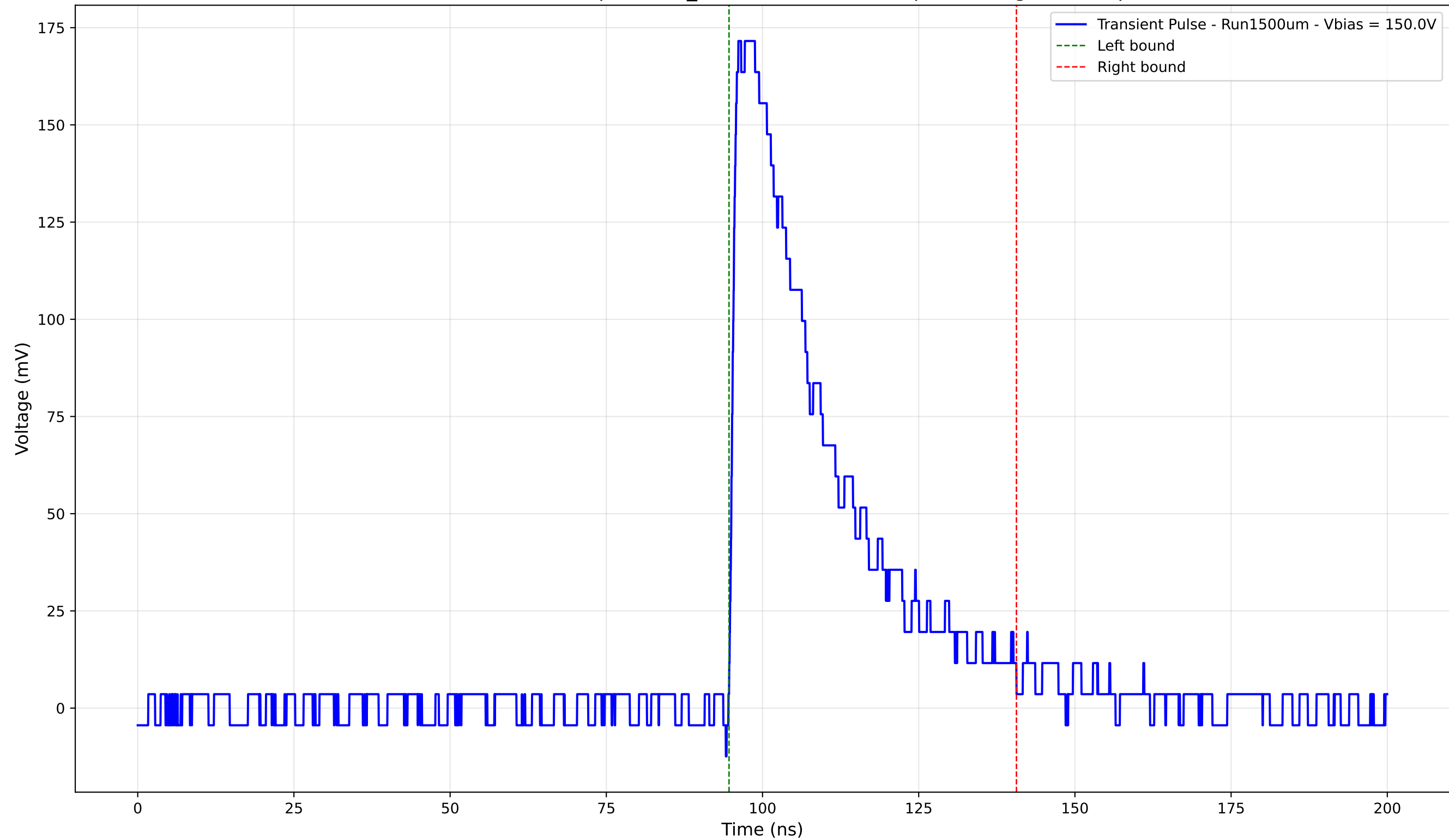
Transient Pulse - Sample: 1cm_42 - Position: 3595.0 \mu\text{m} - Charge: 56.31 pC
