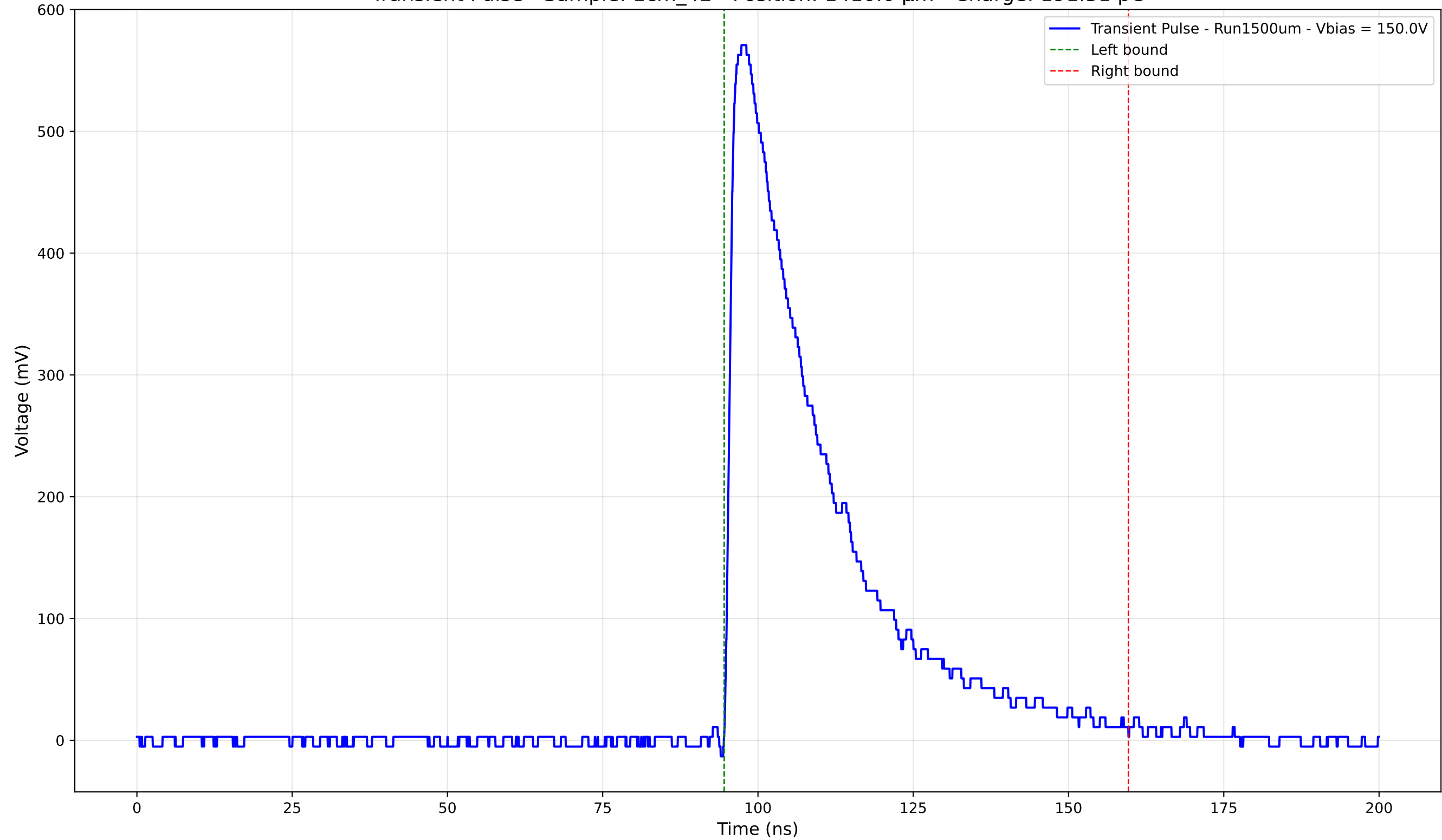
Transient Pulse - Sample: 1cm_42 - Position: 1410.0 \mu\text{m} - Charge: 191.31 pC
