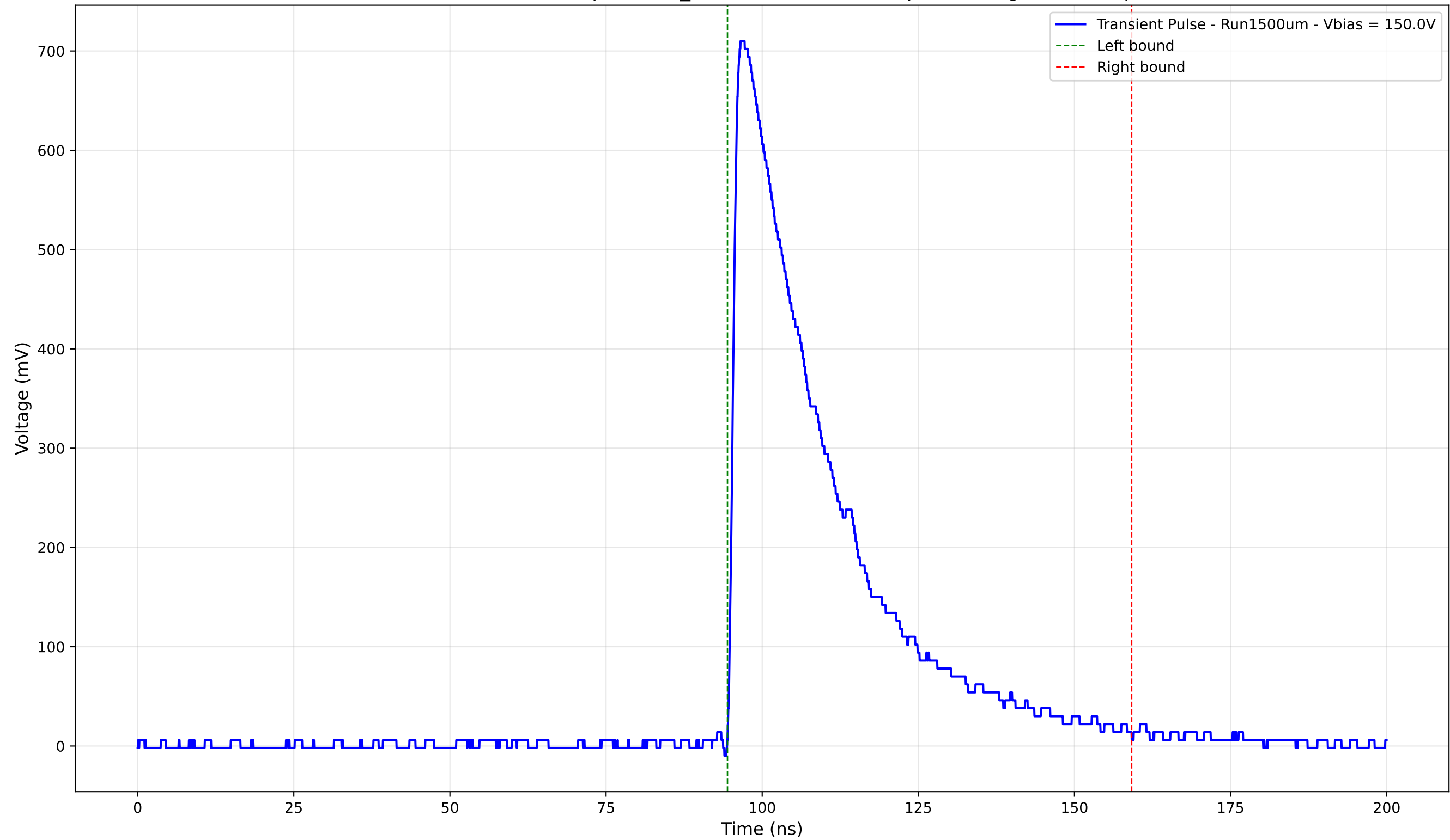
Transient Pulse - Sample: 1cm_42 - Position: 3925.0 \mu\text{m} - Charge: 235.63 pC
