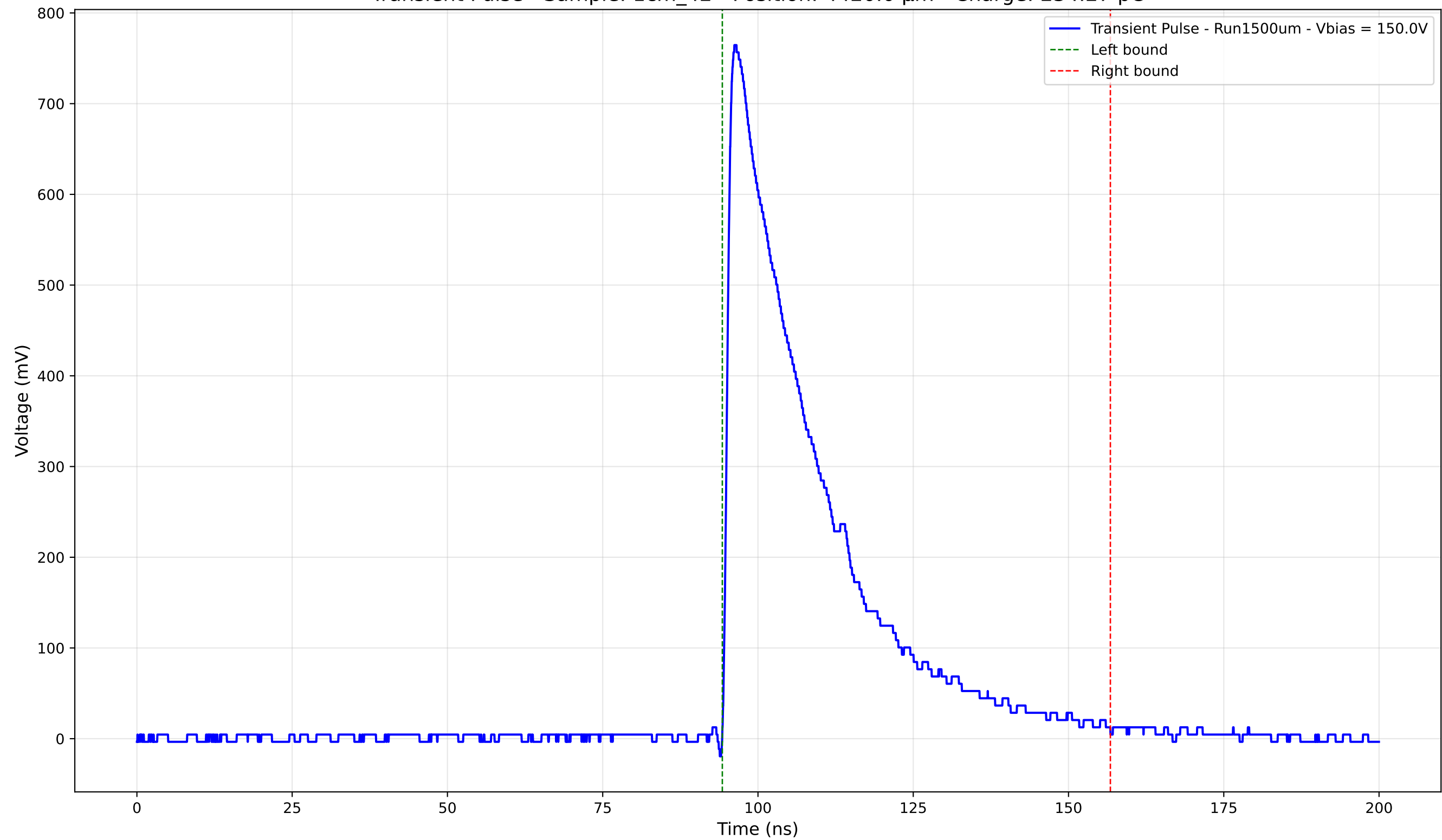
Transient Pulse - Sample: 1cm_42 - Position: 4420.0 \mu\text{m} - Charge: 234.27 pC
