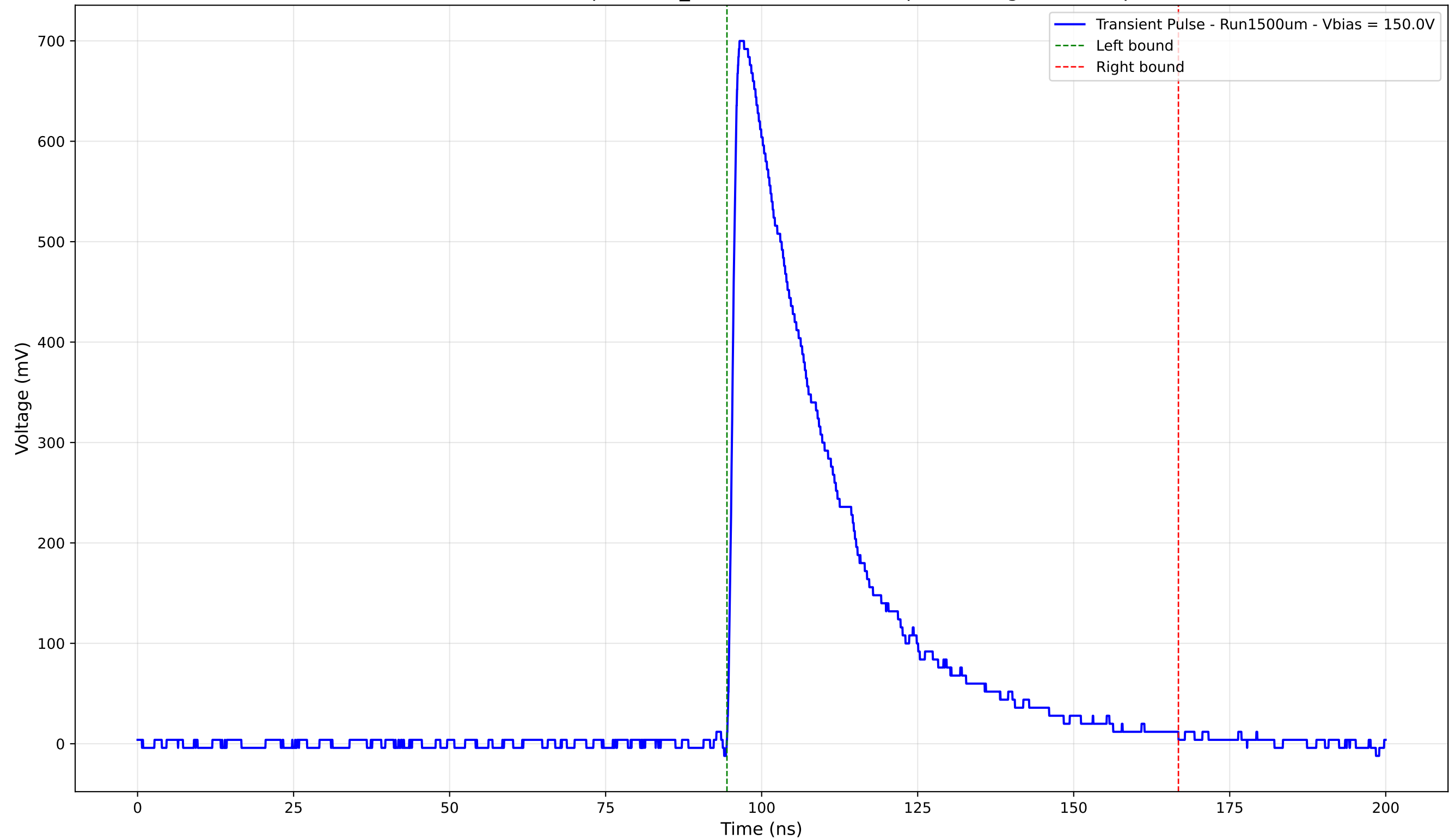
Transient Pulse - Sample: 1cm_42 - Position: 3825.0 \mu\text{m} - Charge: 235.93 pC
