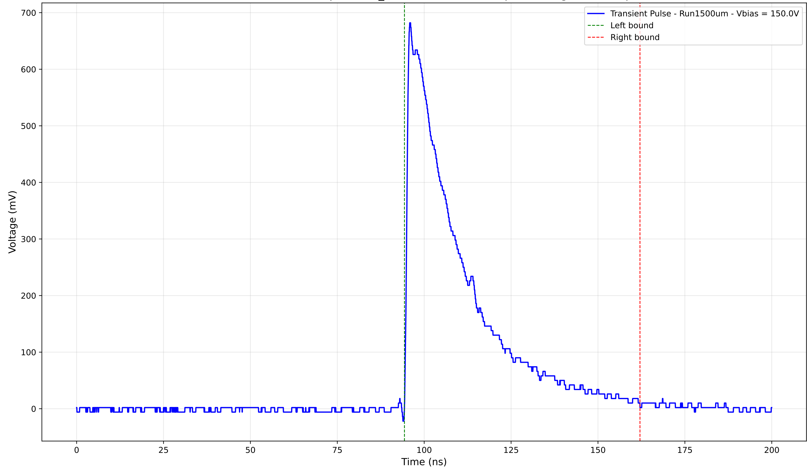
Transient Pulse - Sample: 1cm_42 - Position: 3275.0 \mu\text{m} - Charge: 226.43 pC
