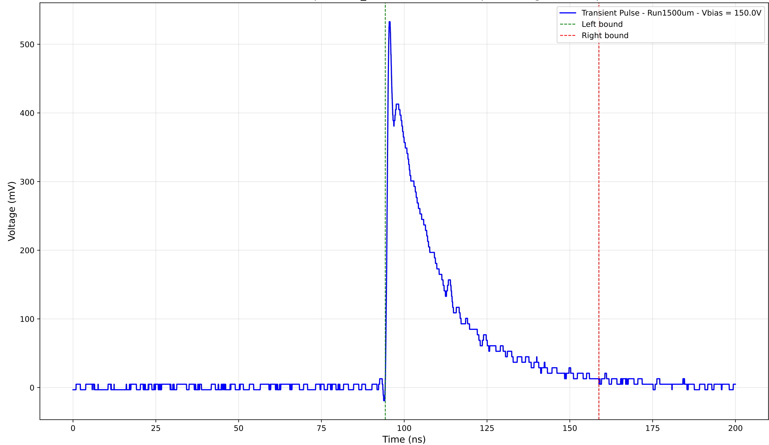
Transient Pulse - Sample: 1cm_42 - Position: 2180.0 \mu\text{m} - Charge: 150.48 pC
