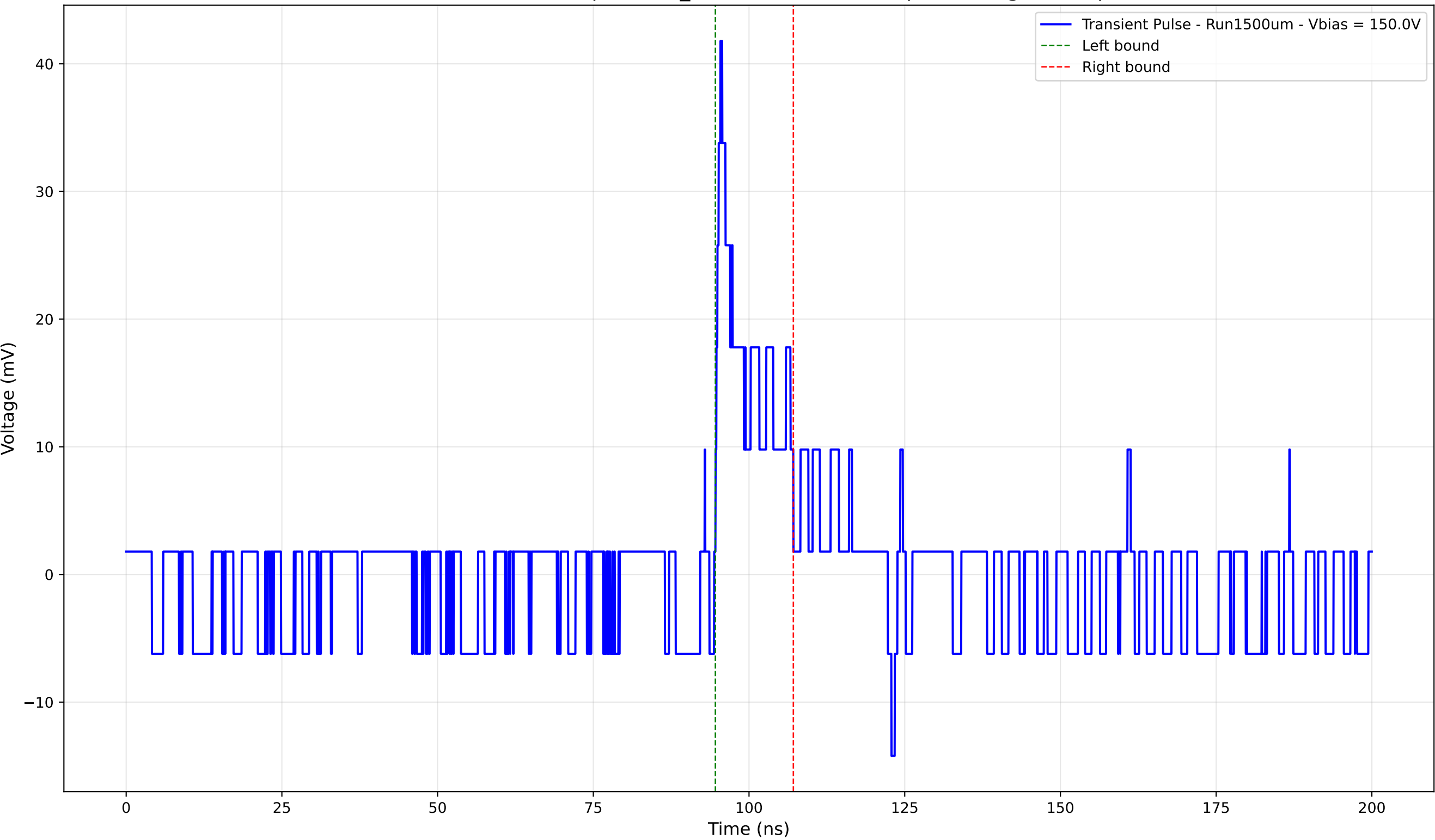
Transient Pulse - Sample: 1cm_42 - Position: 4965.0 \mu\text{m} - Charge: 4.24 pC
