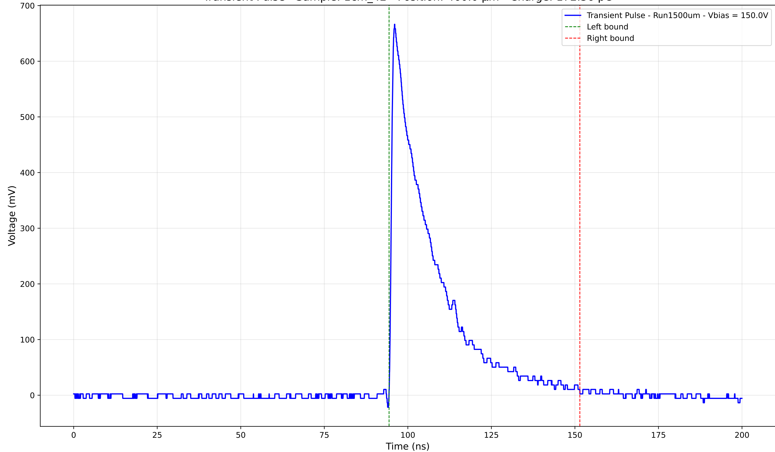
Transient Pulse - Sample: 1cm_42 - Position: 460.0 \mu\text{m} - Charge: 172.36 pC
