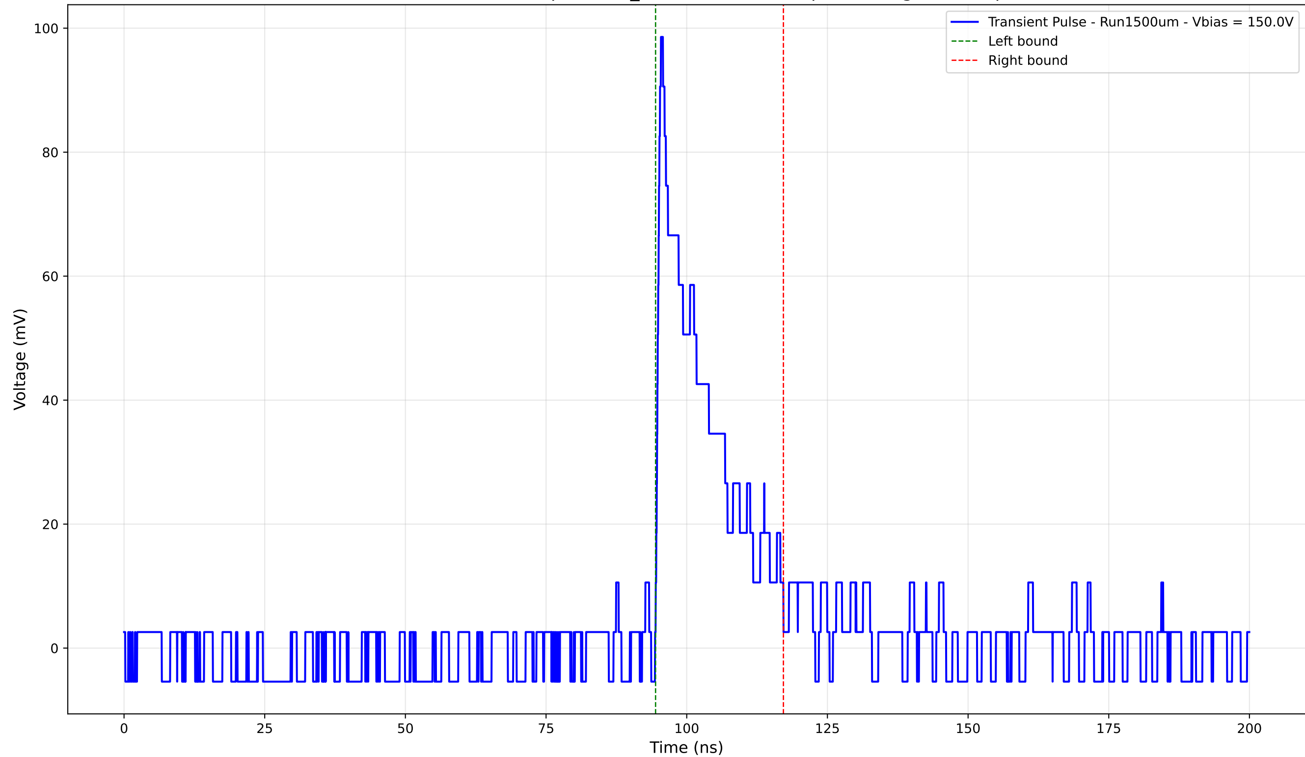
Transient Pulse - Sample: 1cm_42 - Position: 90.0 \mu\text{m} - Charge: 16.77 pC
