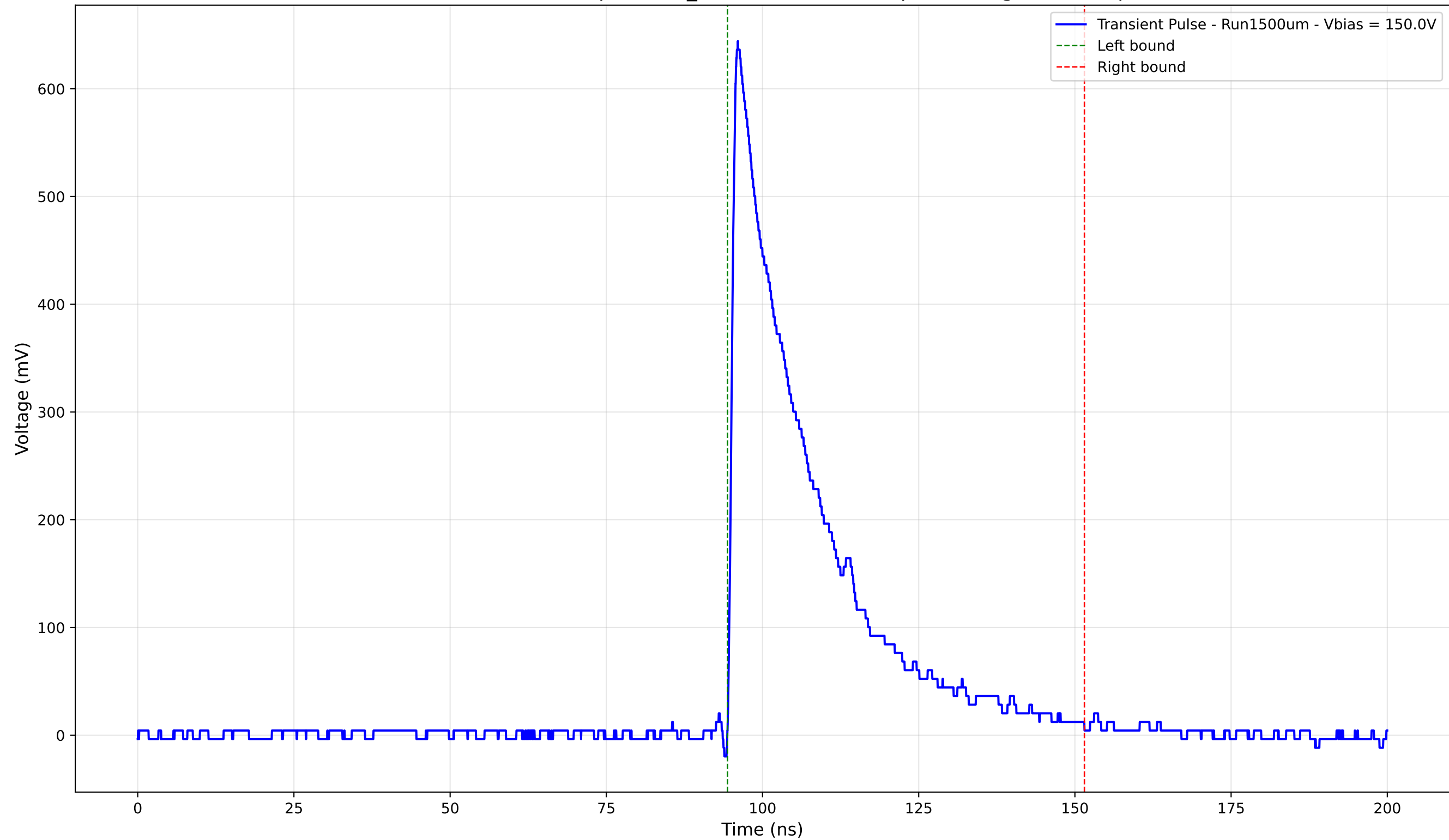
Transient Pulse - Sample: 1cm_42 - Position: 475.0 \mu\text{m} - Charge: 167.51 pC
