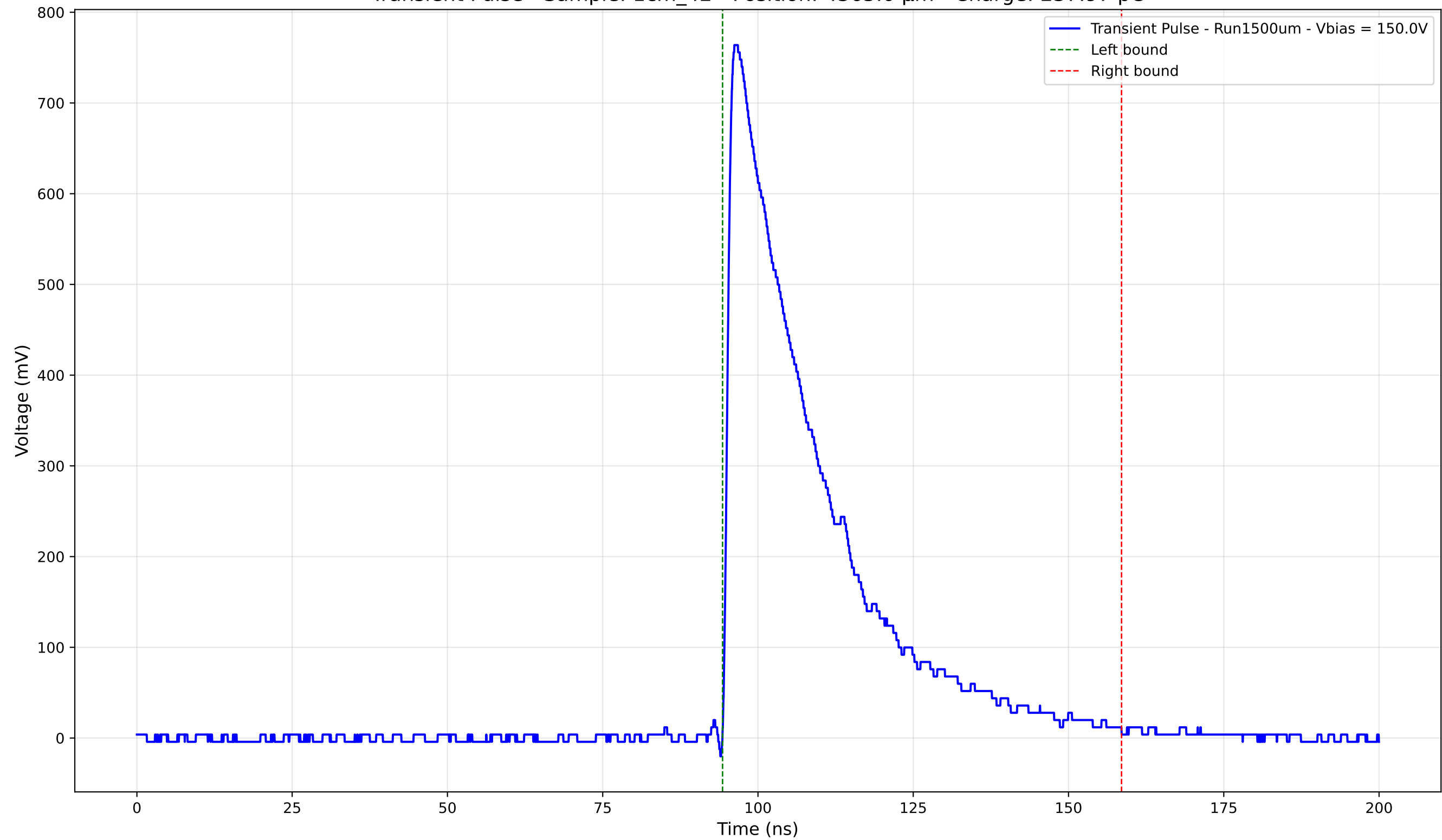
Transient Pulse - Sample: 1cm_42 - Position: 4365.0 \mu\text{m} - Charge: 237.97 pC
