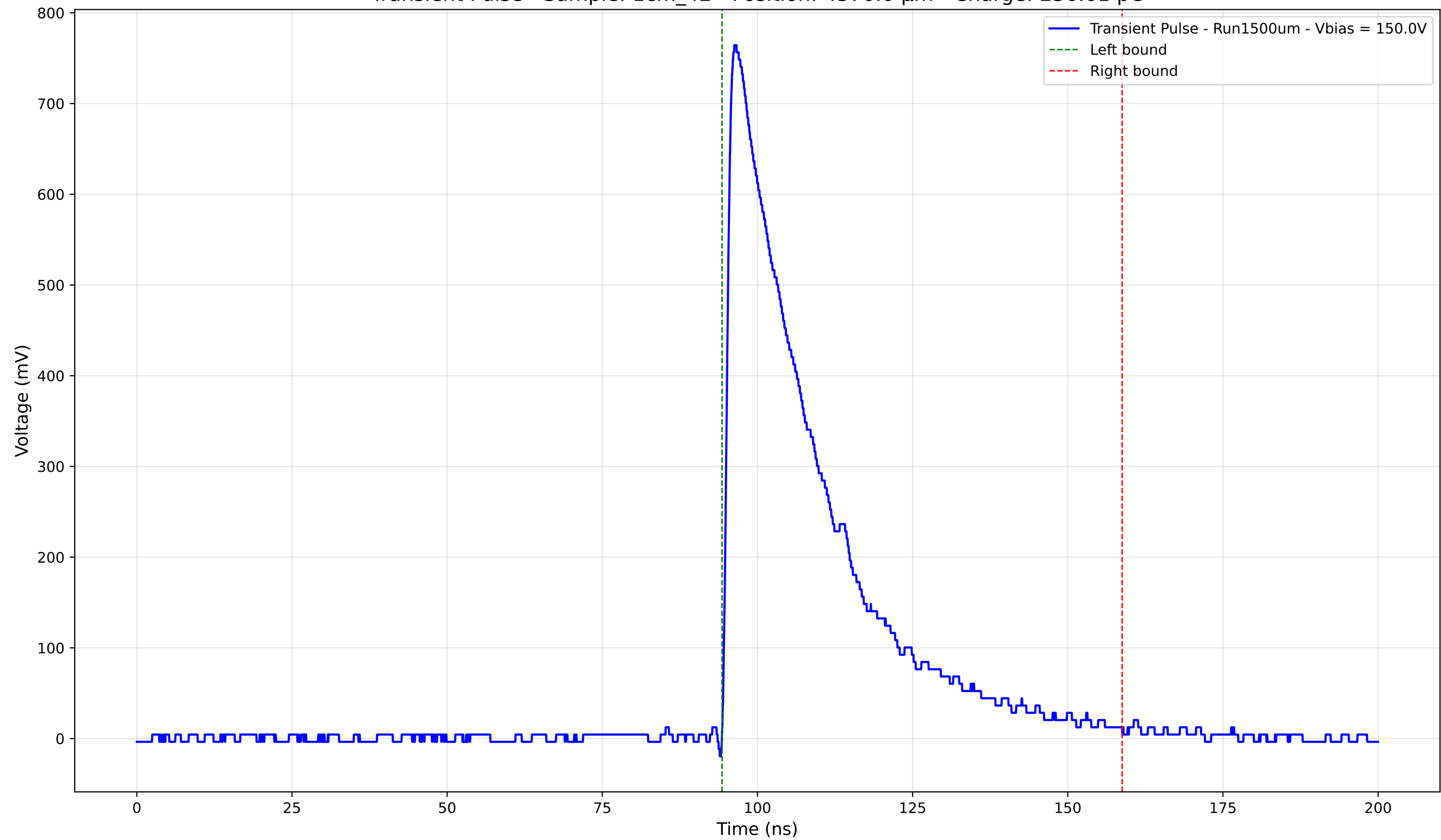
Transient Pulse - Sample: 1cm_42 - Position: 4370.0 \mu\text{m} - Charge: 236.61 pC
