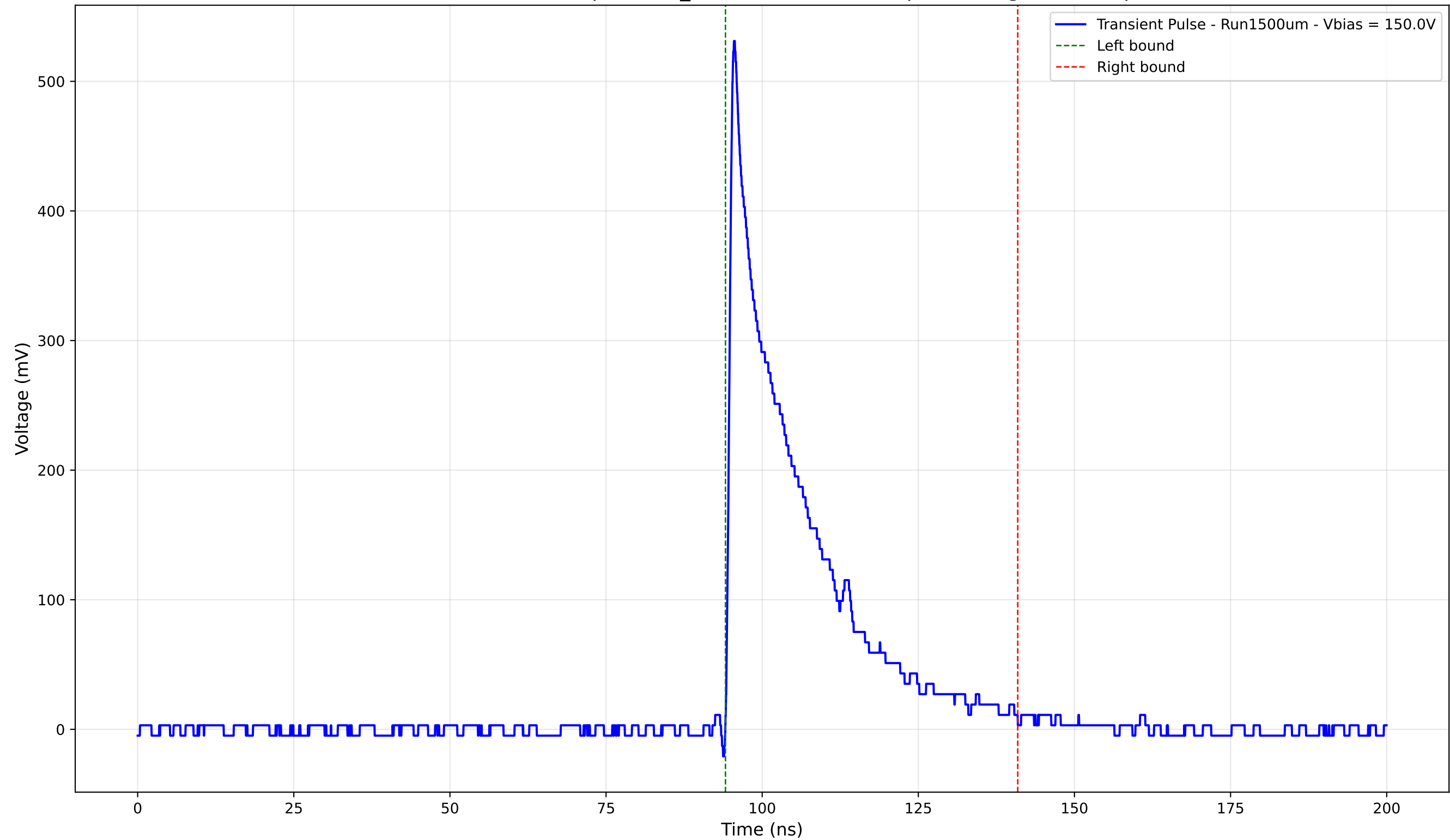
Transient Pulse - Sample: 1cm_42 - Position: 4895.0 \mu\text{m} - Charge: 112.92 pC
