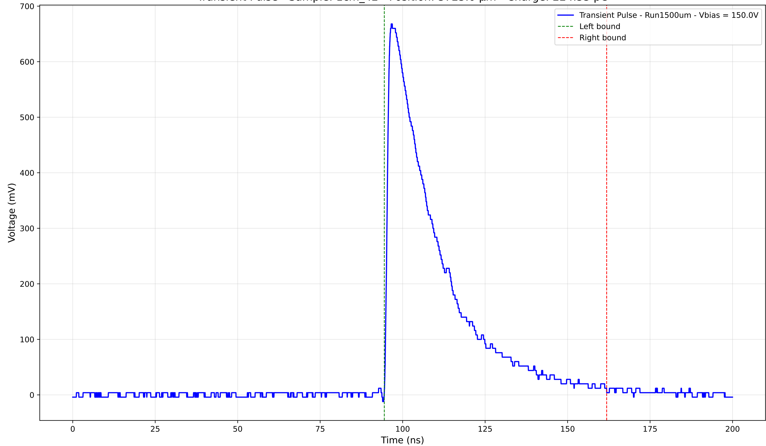
Transient Pulse - Sample: 1cm_42 - Position: 3725.0 \mu\text{m} - Charge: 224.53 pC
