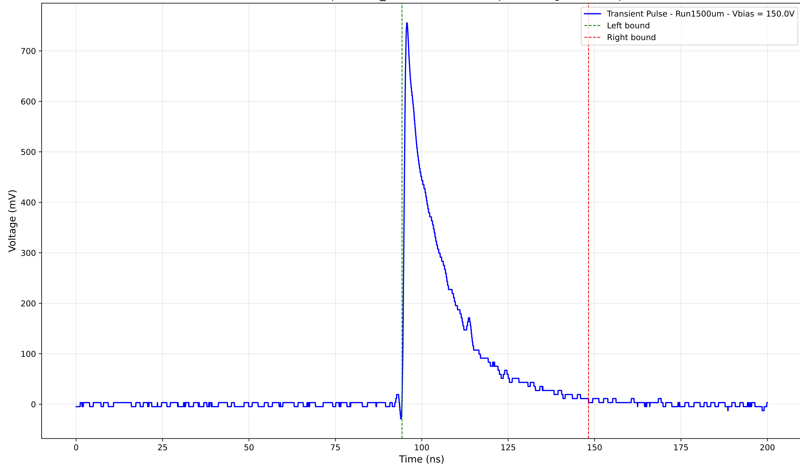
Transient Pulse - Sample: 1cm_42 - Position: 235.0 \mu\text{m} - Charge: 169.28 pC
