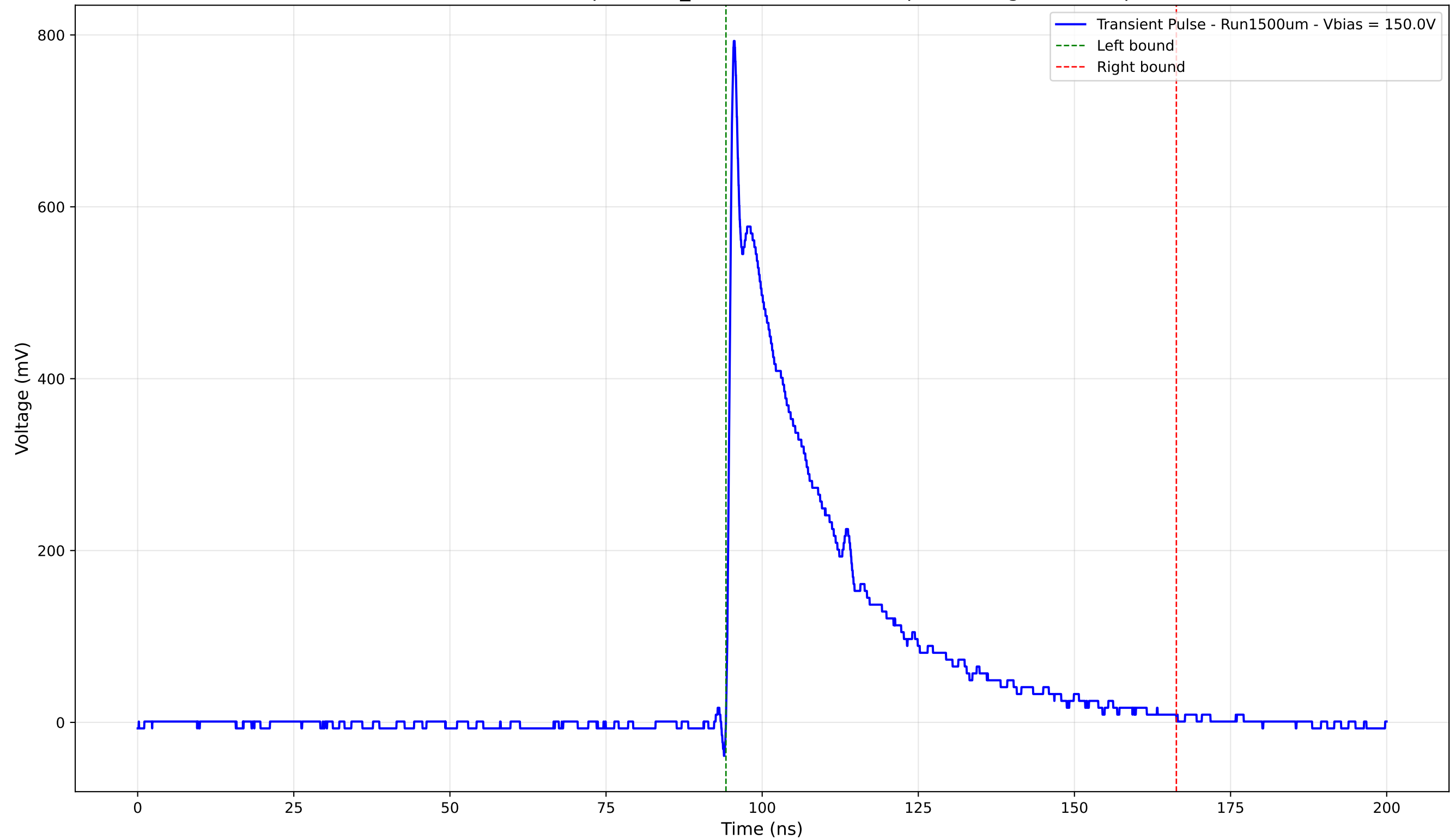
Transient Pulse - Sample: 1cm_42 - Position: 2935.0 \mu\text{m} - Charge: 212.28 pC
