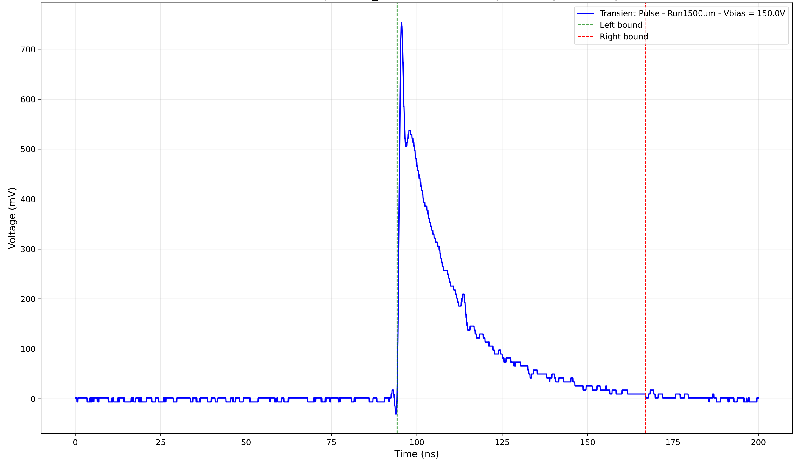
Transient Pulse - Sample: 1cm_42 - Position: 2275.0 \mu\text{m} - Charge: 199.30 pC
