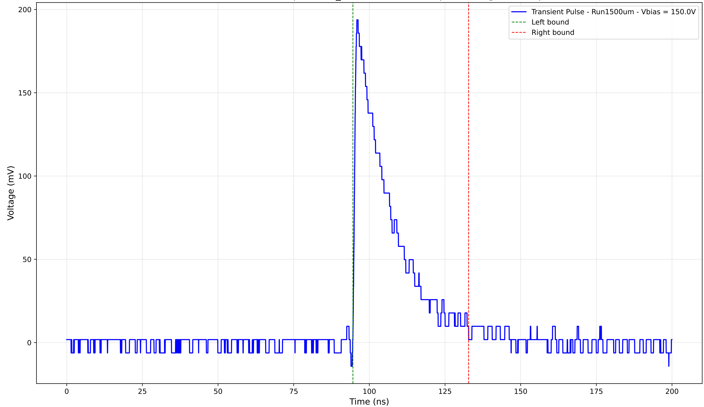
Transient Pulse - Sample: 1cm_42 -Position: 555.0 \mu\text{m} - Charge: 48.06 pC
