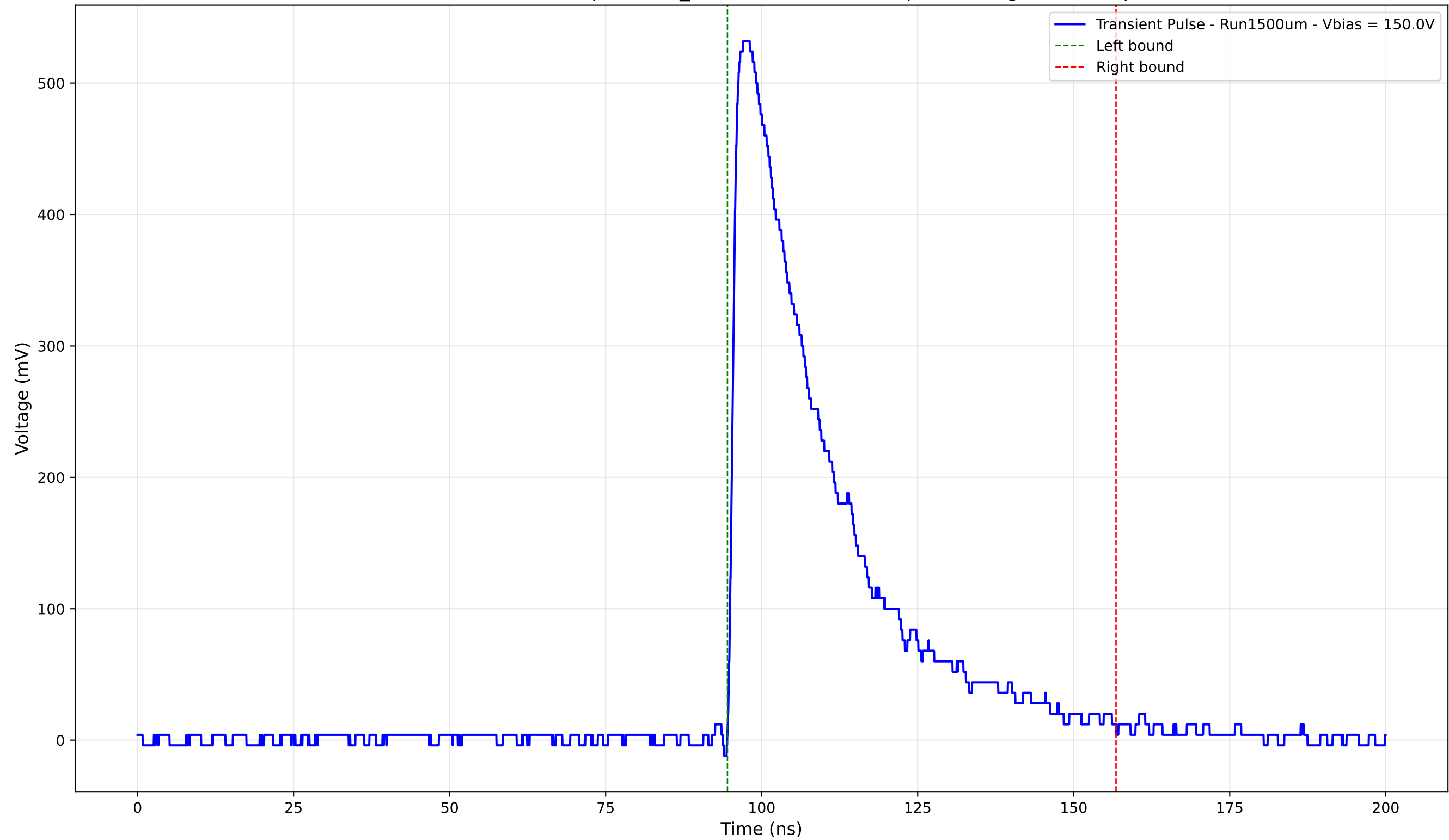
Transient Pulse - Sample: 1cm_42 - Position: 1485.0 \mu\text{m} - Charge: 178.60 pC
