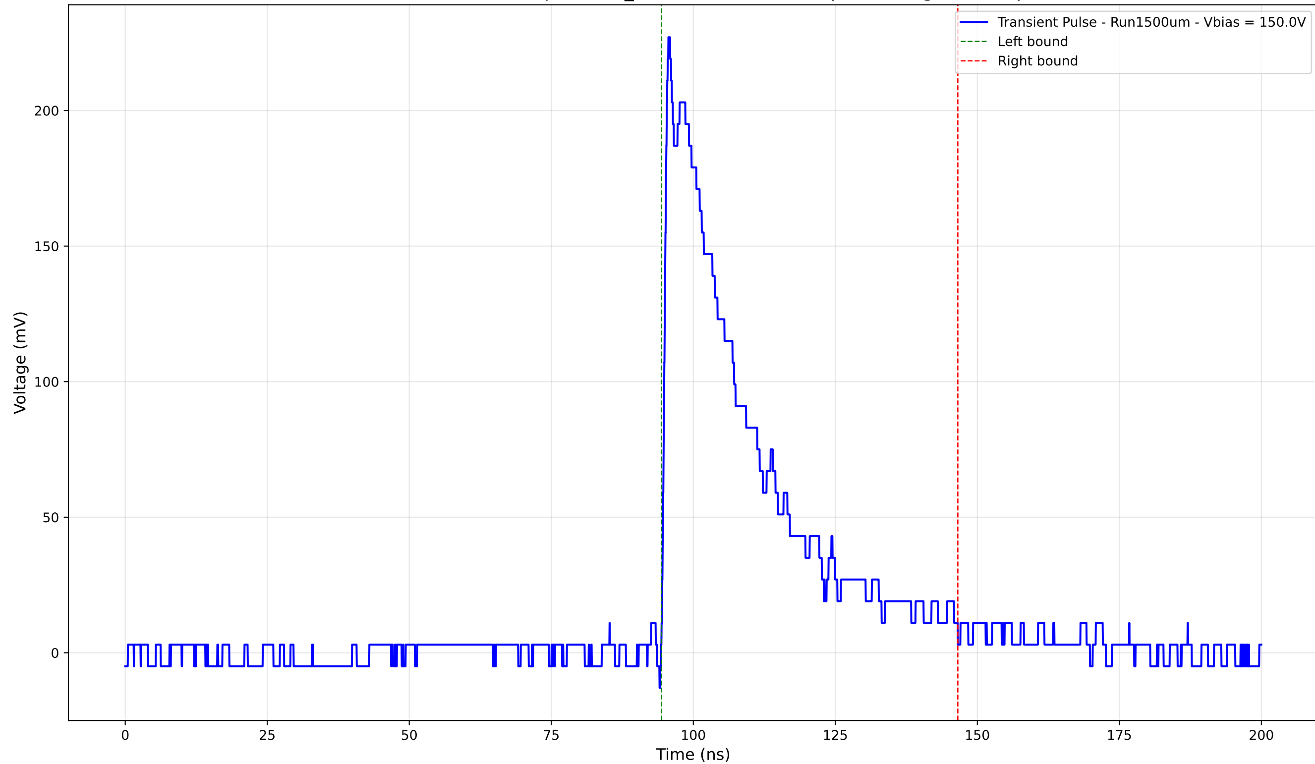
Transient Pulse - Sample: 1cm_42 - Position: 2060.0 \mu\text{m} - Charge: 69.01 pC
