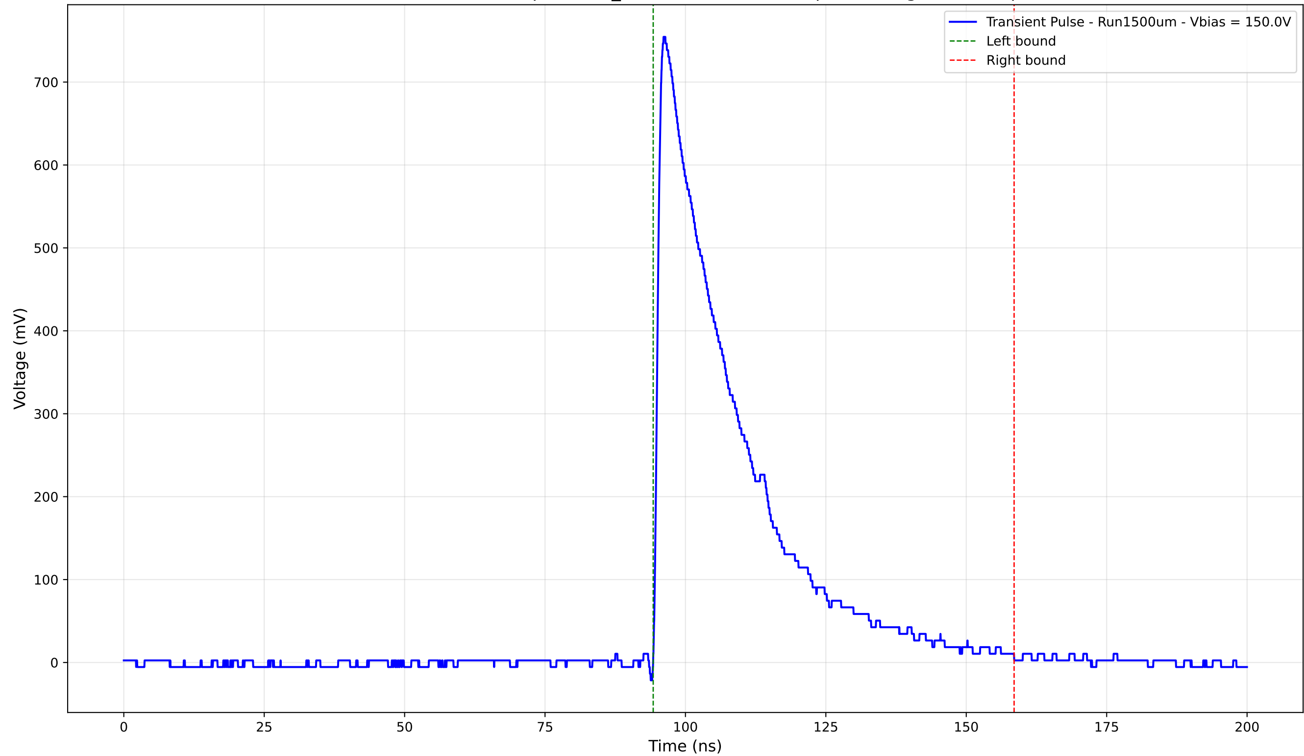
Transient Pulse - Sample: 1cm_42 - Position: 4460.0 \mu\text{m} - Charge: 224.76 pC
