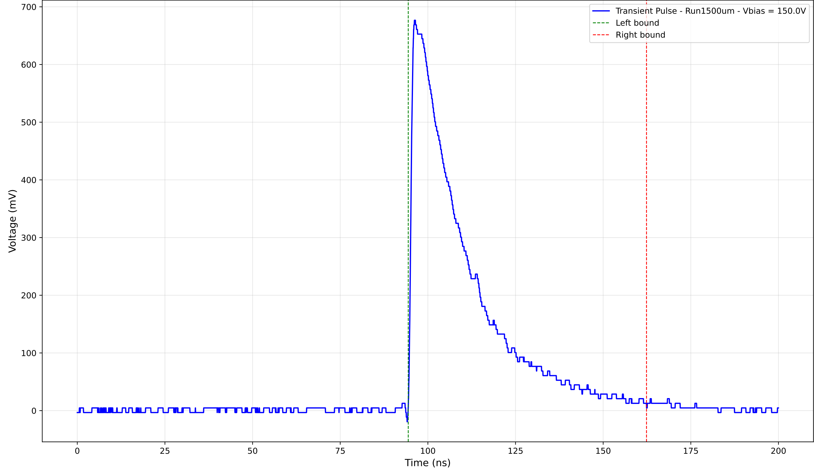
Transient Pulse - Sample: 1cm_42 - Position: 3445.0 \mu\text{m} - Charge: 231.93 pC
