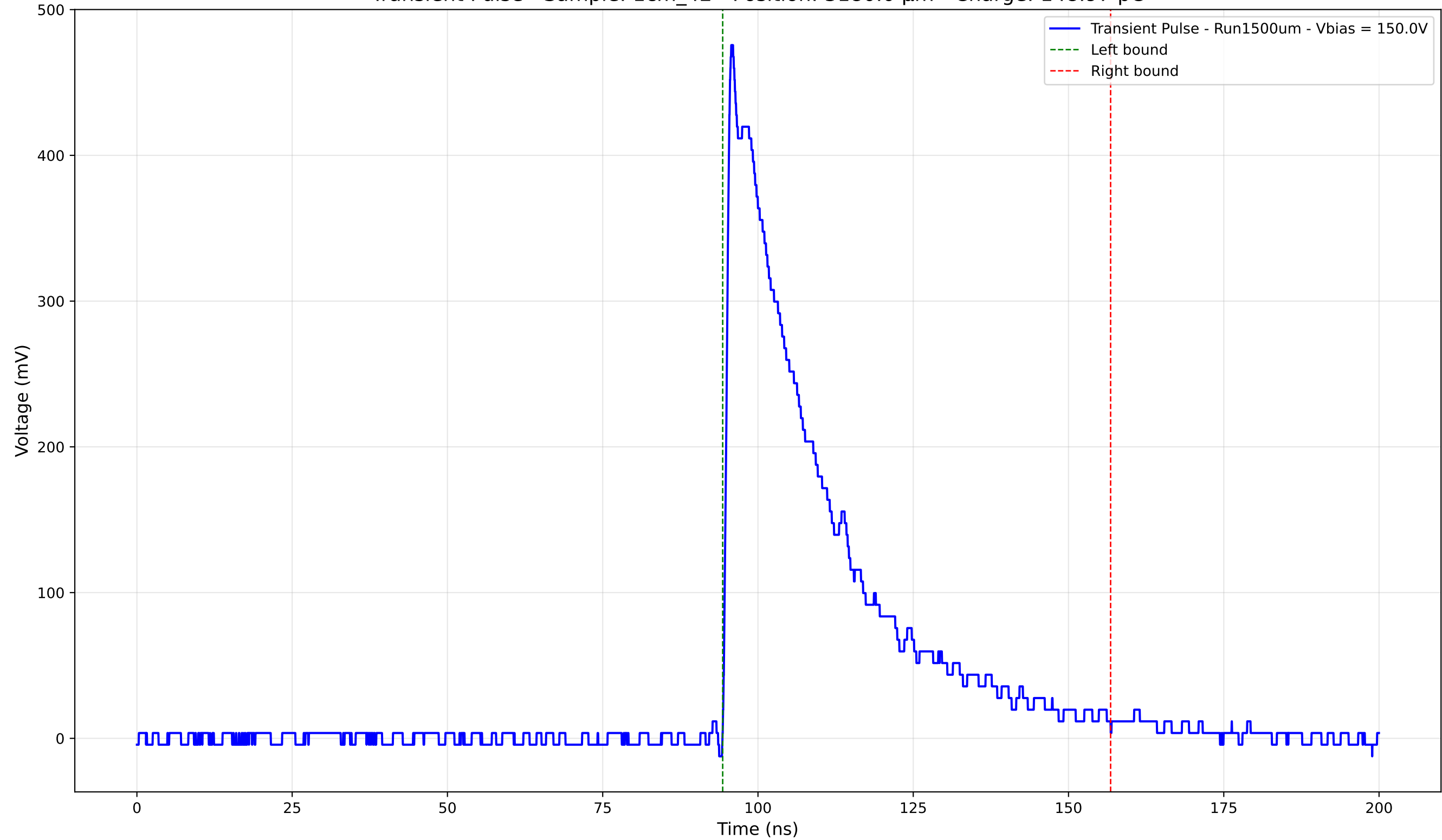
Transient Pulse - Sample: 1cm_42 - Position: 3180.0 \mu\text{m} - Charge: 148.97 pC
