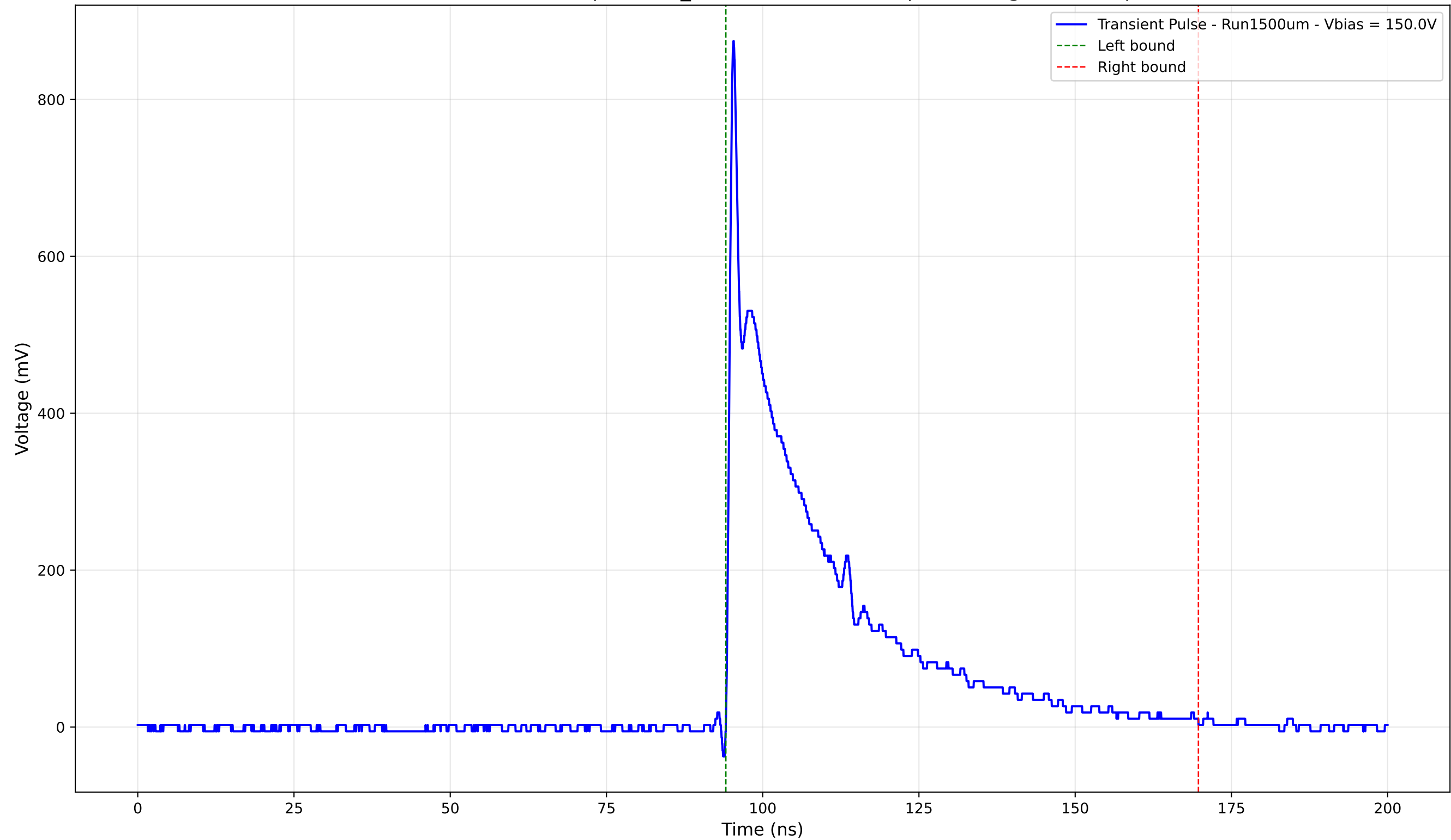
Transient Pulse - Sample: 1cm_42 - Position: 2485.0 \mu\text{m} - Charge: 202.04 pC
