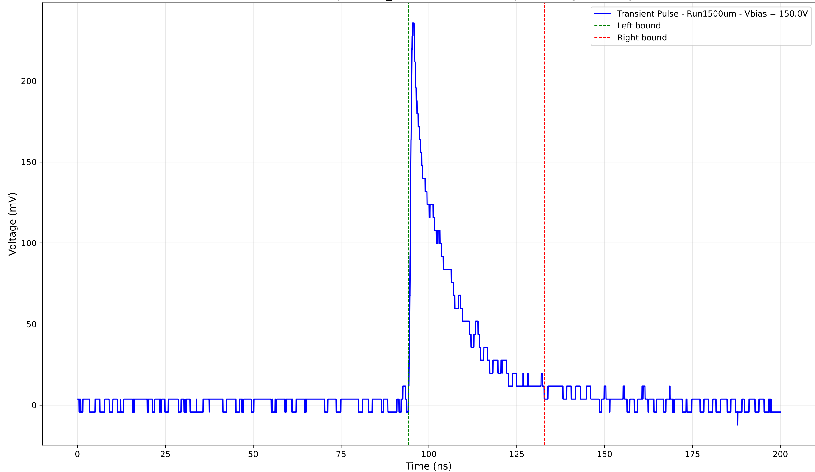
Transient Pulse - Sample: 1cm_42 - Position: 4925.0 \mu\text{m} - Charge: 46.68 pC
