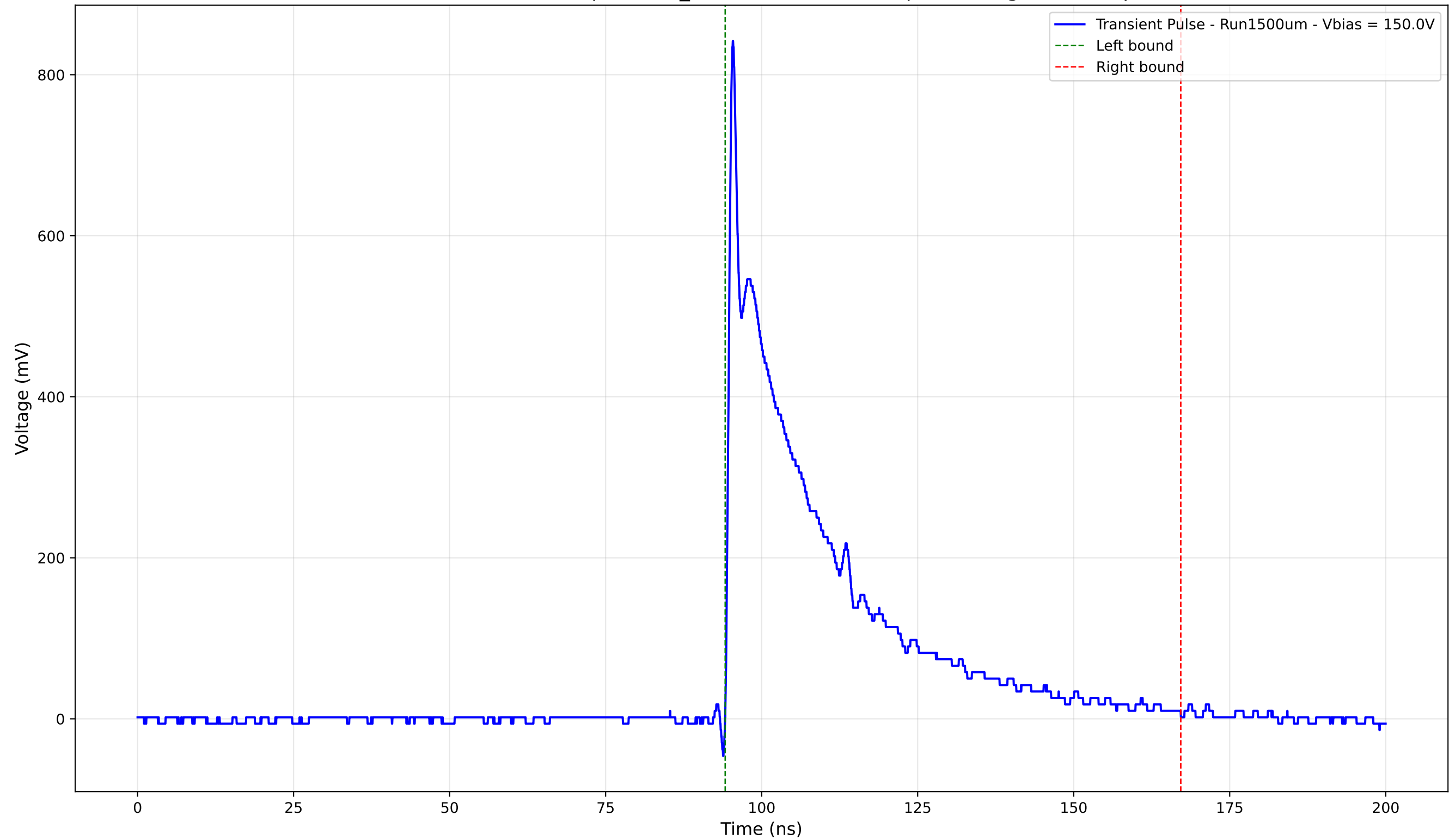
Transient Pulse - Sample: 1cm_42 - Position: 2400.0 \mu\text{m} - Charge: 203.97 pC
