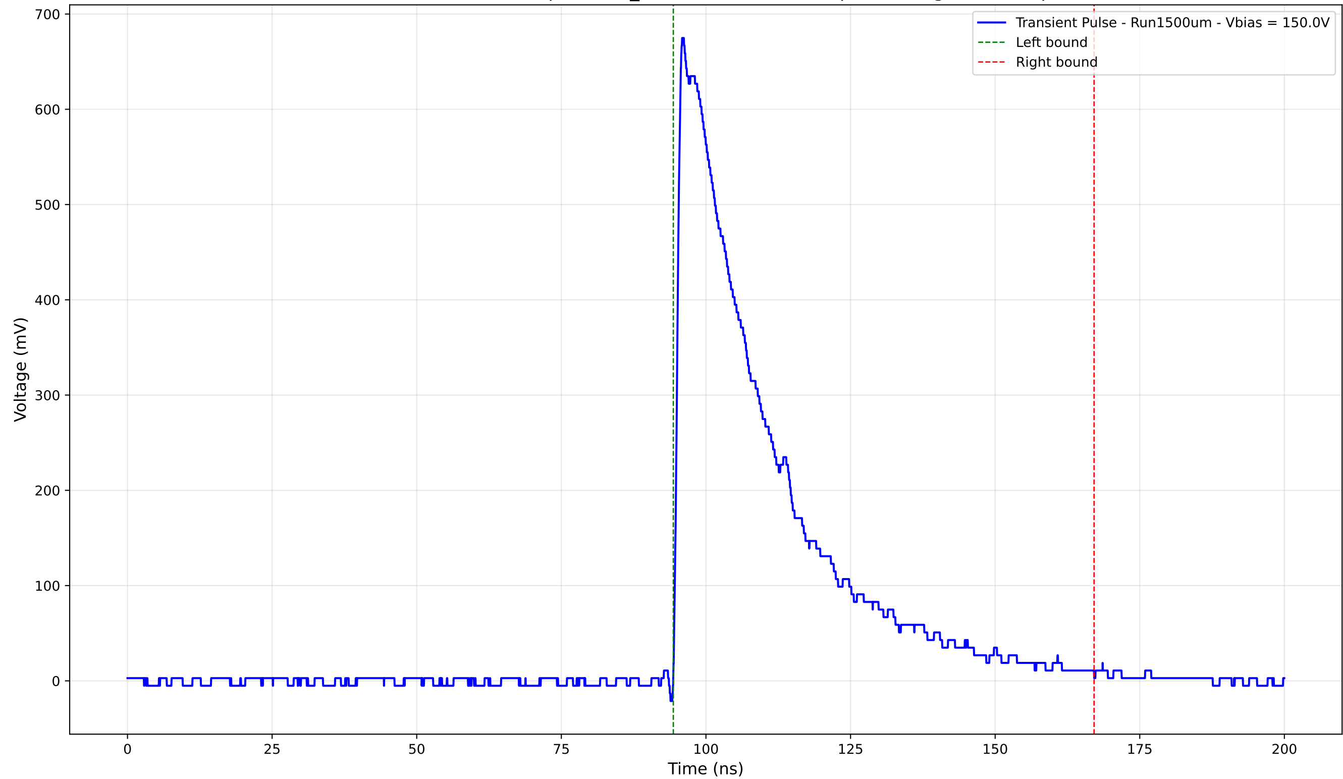
Transient Pulse - Sample: 1cm_42 - Position: 3305.0 \mu\text{m} - Charge: 227.29 pC
