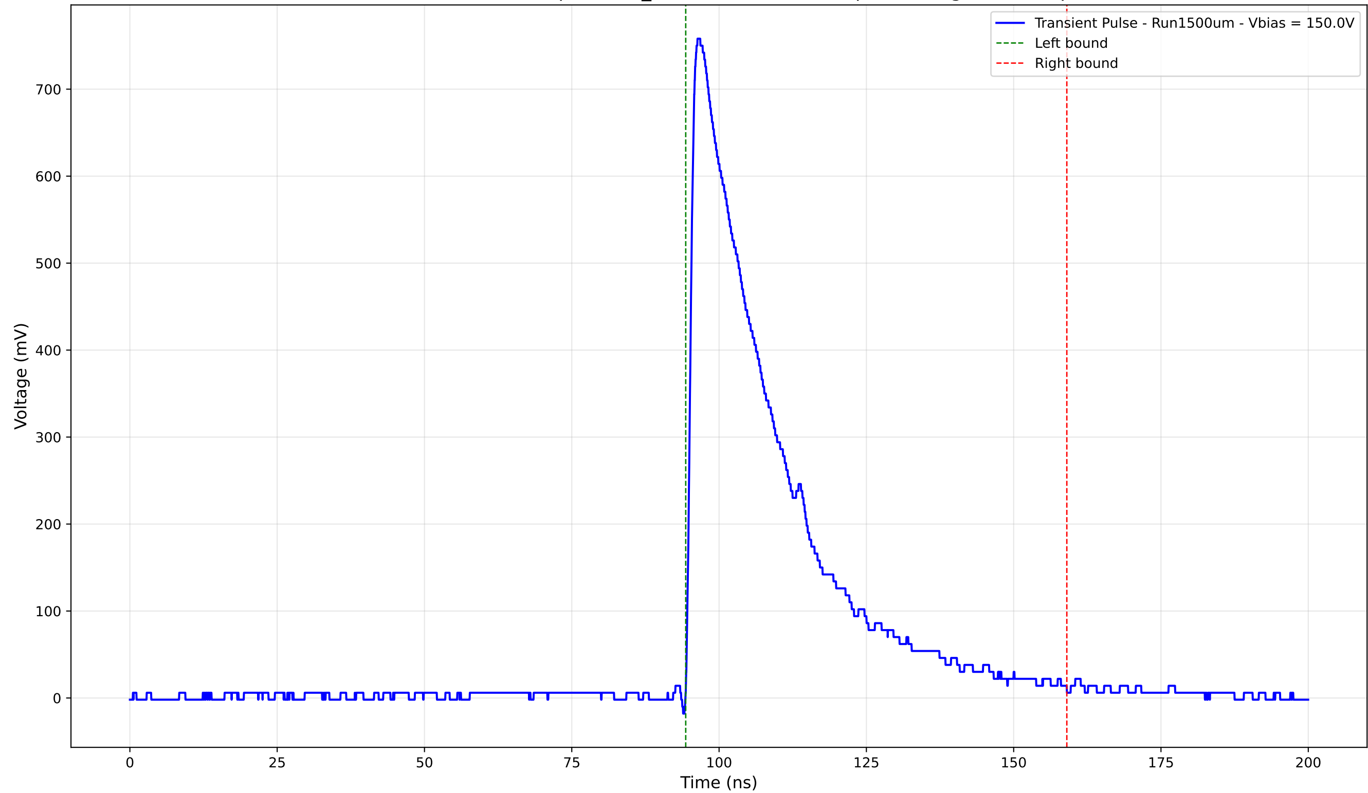
Transient Pulse - Sample: 1cm_42 - Position: 4330.0 \mu\text{m} - Charge: 237.63 pC
