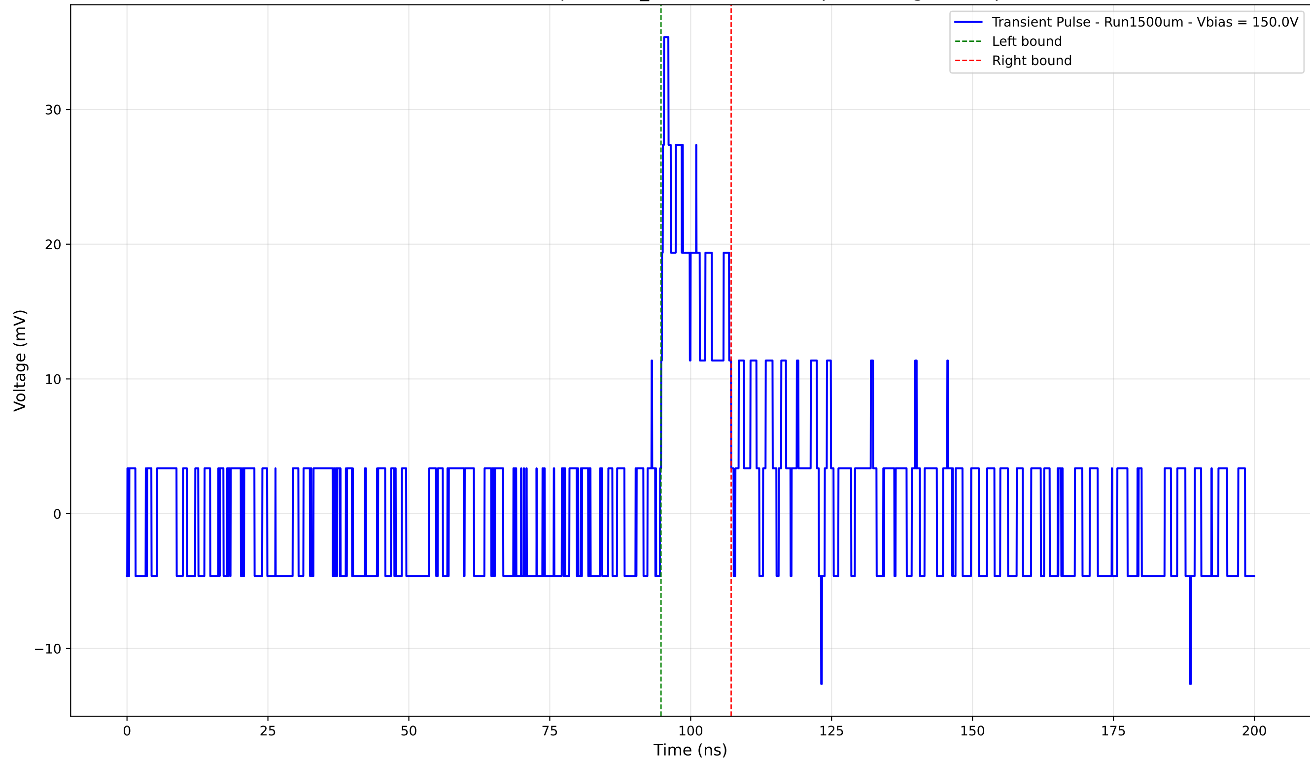
Transient Pulse - Sample: 1cm_42 - Position: 60.0 \mu\text{m} - Charge: 4.77 pC
