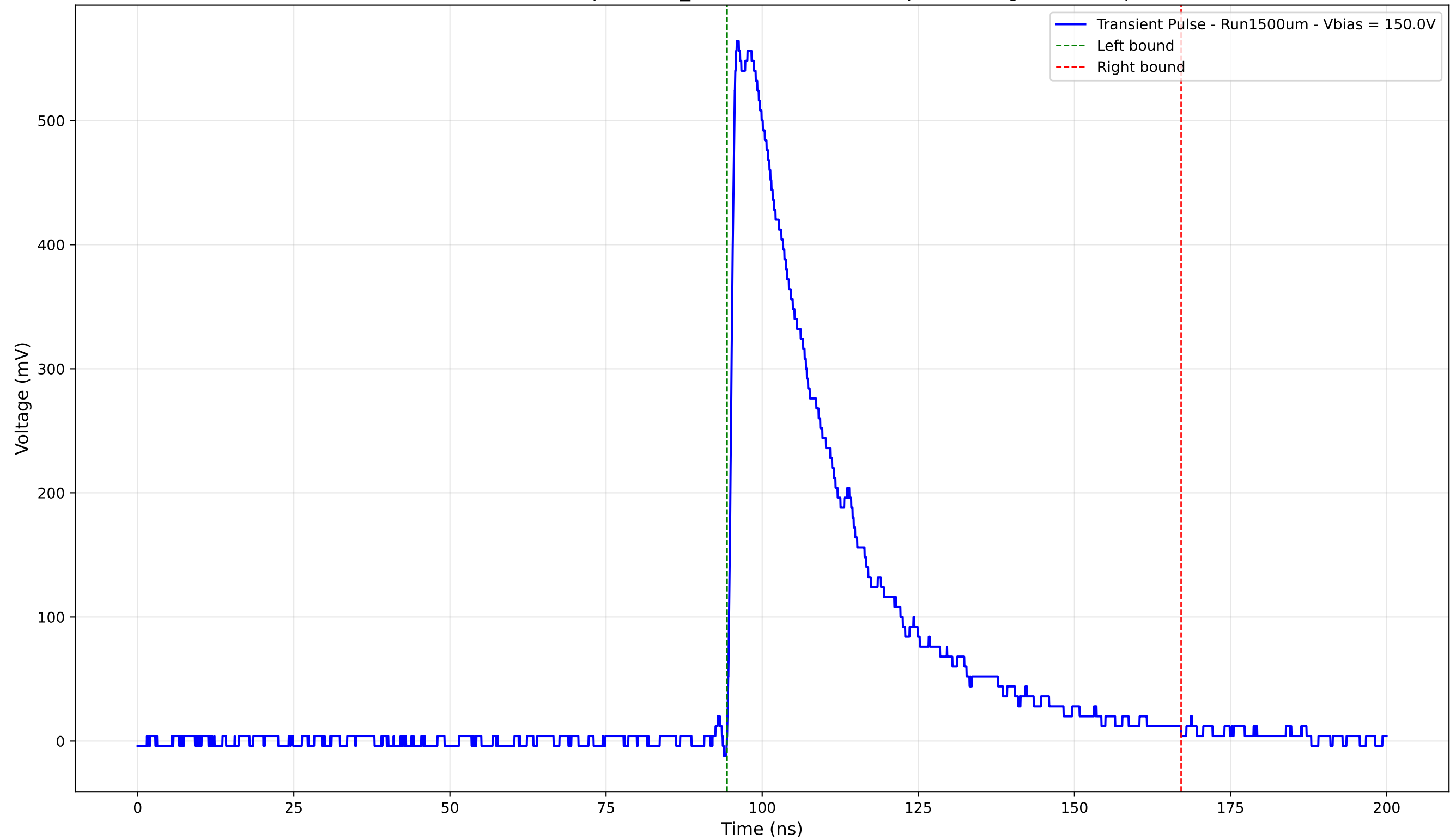
Transient Pulse - Sample: 1cm_42 - Position: 1855.0 \mu\text{m} - Charge: 199.30 pC
