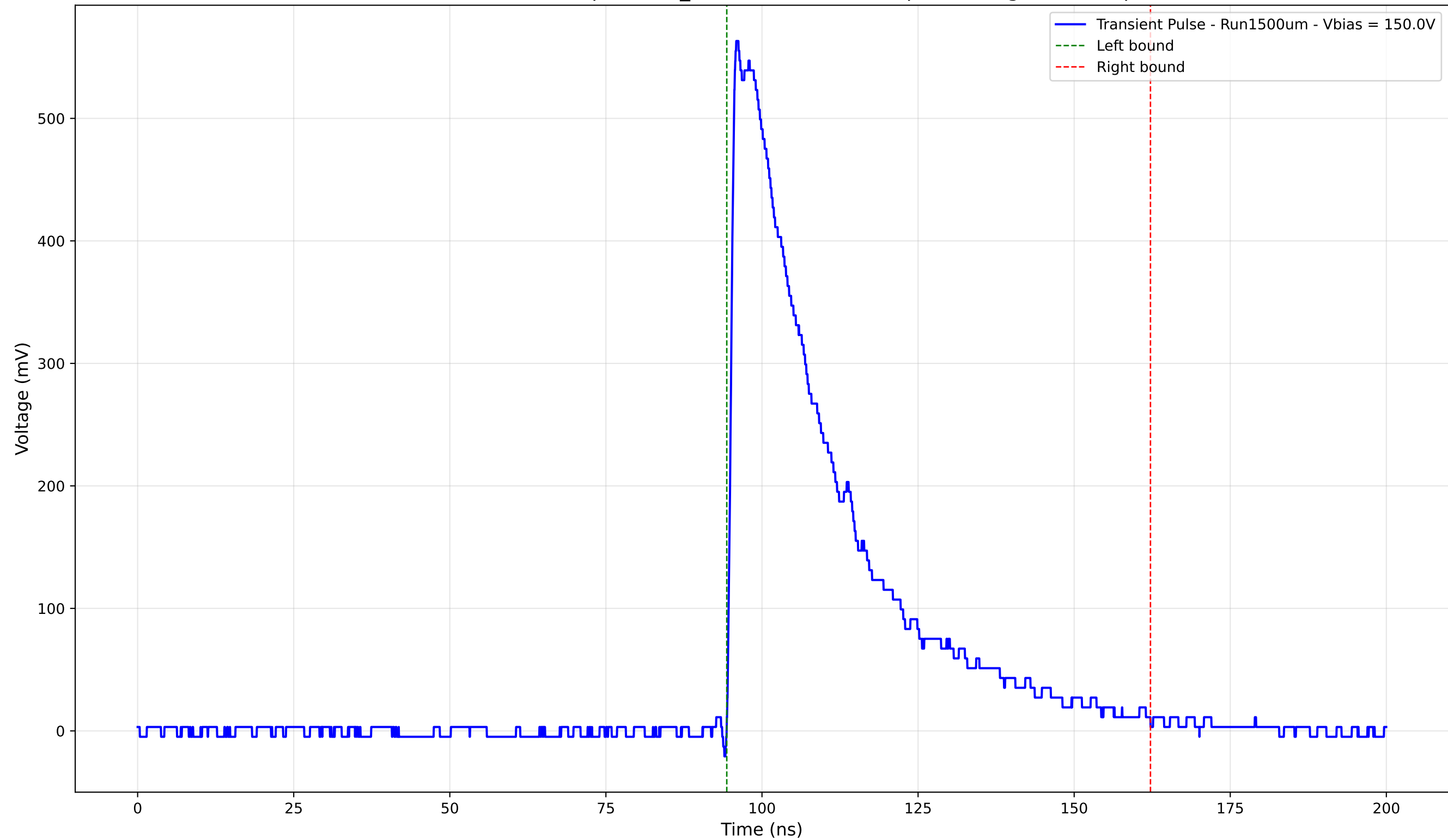
Transient Pulse - Sample: 1cm_42 - Position: 1880.0 \mu\text{m} - Charge: 195.60 pC
