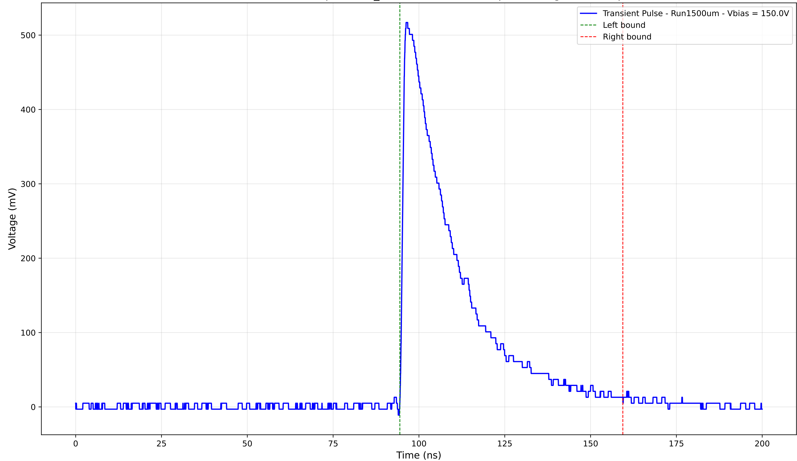
Transient Pulse - Sample: 1cm_42 - Position: 3545.0 \mu\text{m} - Charge: 172.81 pC
