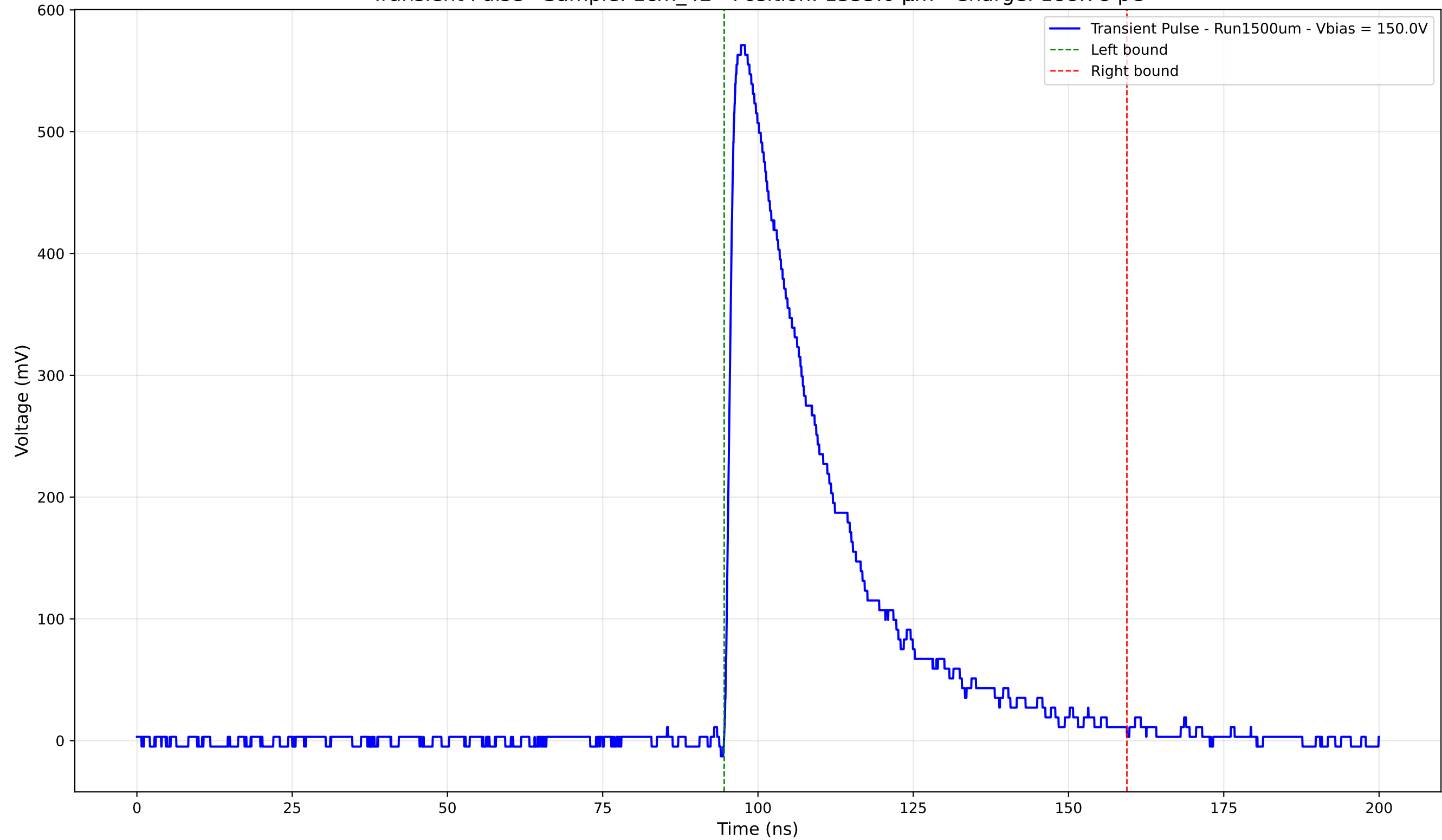
Transient Pulse - Sample: 1cm_42 - Position: 1355.0 \mu\text{m} - Charge: 188.78 pC
