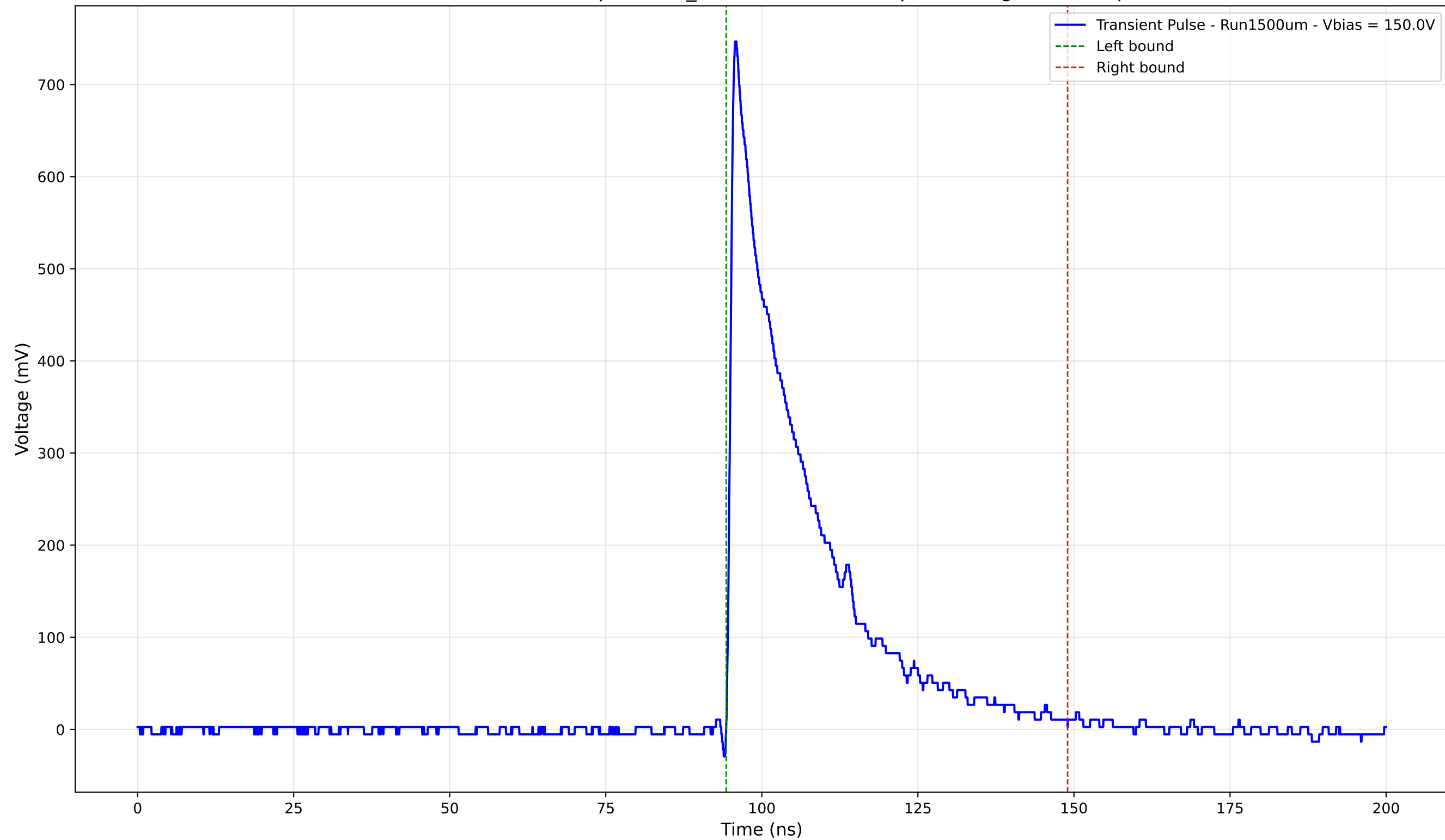
Transient Pulse - Sample: 1cm_42 - Position: 315.0 \mu\text{m} - Charge: 177.64 pC
