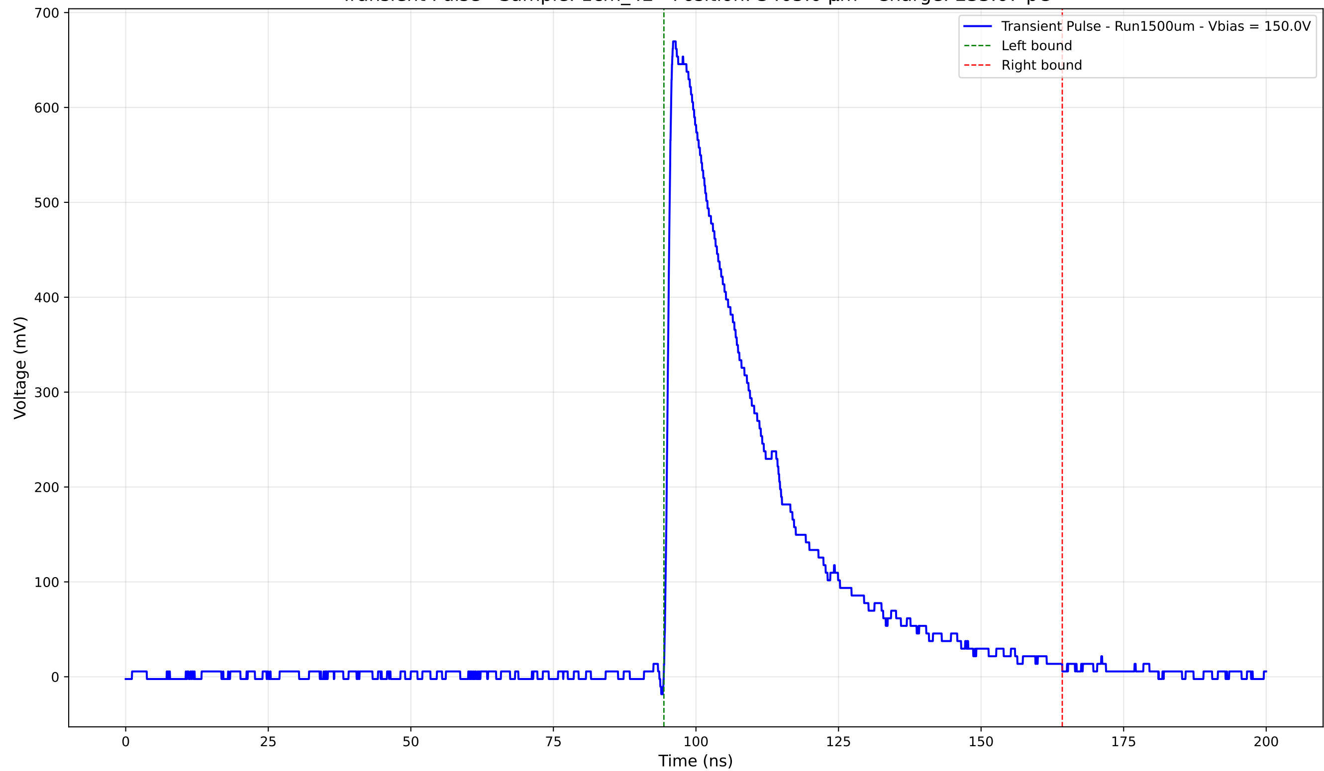
Transient Pulse - Sample: 1cm_42 - Position: 3405.0 \mu\text{m} - Charge: 233.67 pC
