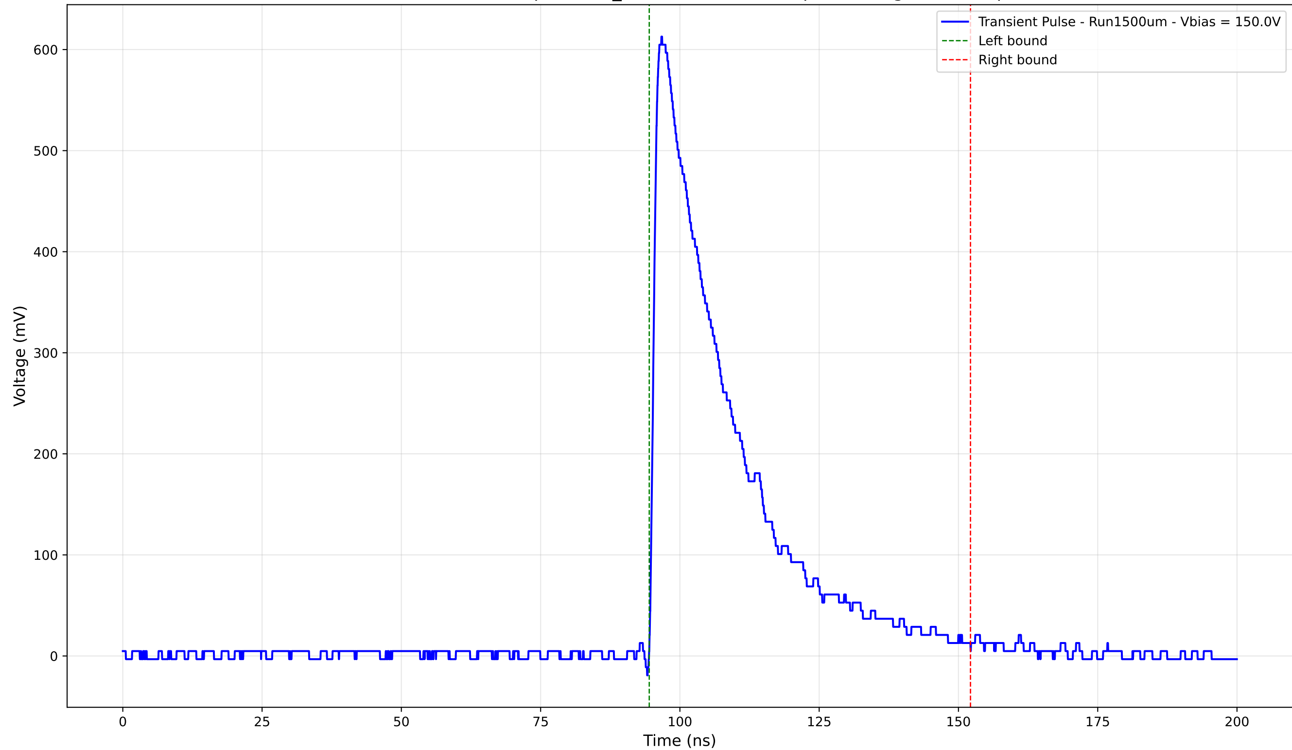
Transient Pulse - Sample: 1cm_42 - Position: 760.0 \mu\text{m} - Charge: 181.01 pC
