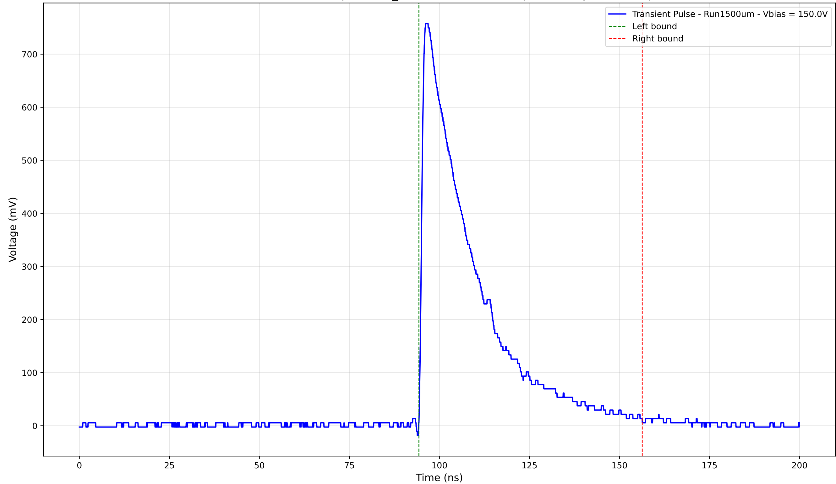
Transient Pulse - Sample: 1cm_42 - Position: 4390.0 \mu\text{m} - Charge: 235.80 pC
