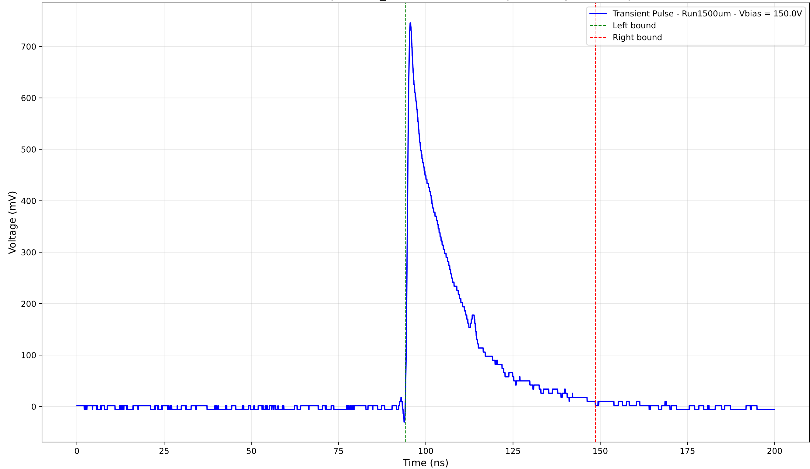
Transient Pulse - Sample: 1cm_42 - Position: 4845.0 \mu\text{m} - Charge: 174.07 pC
