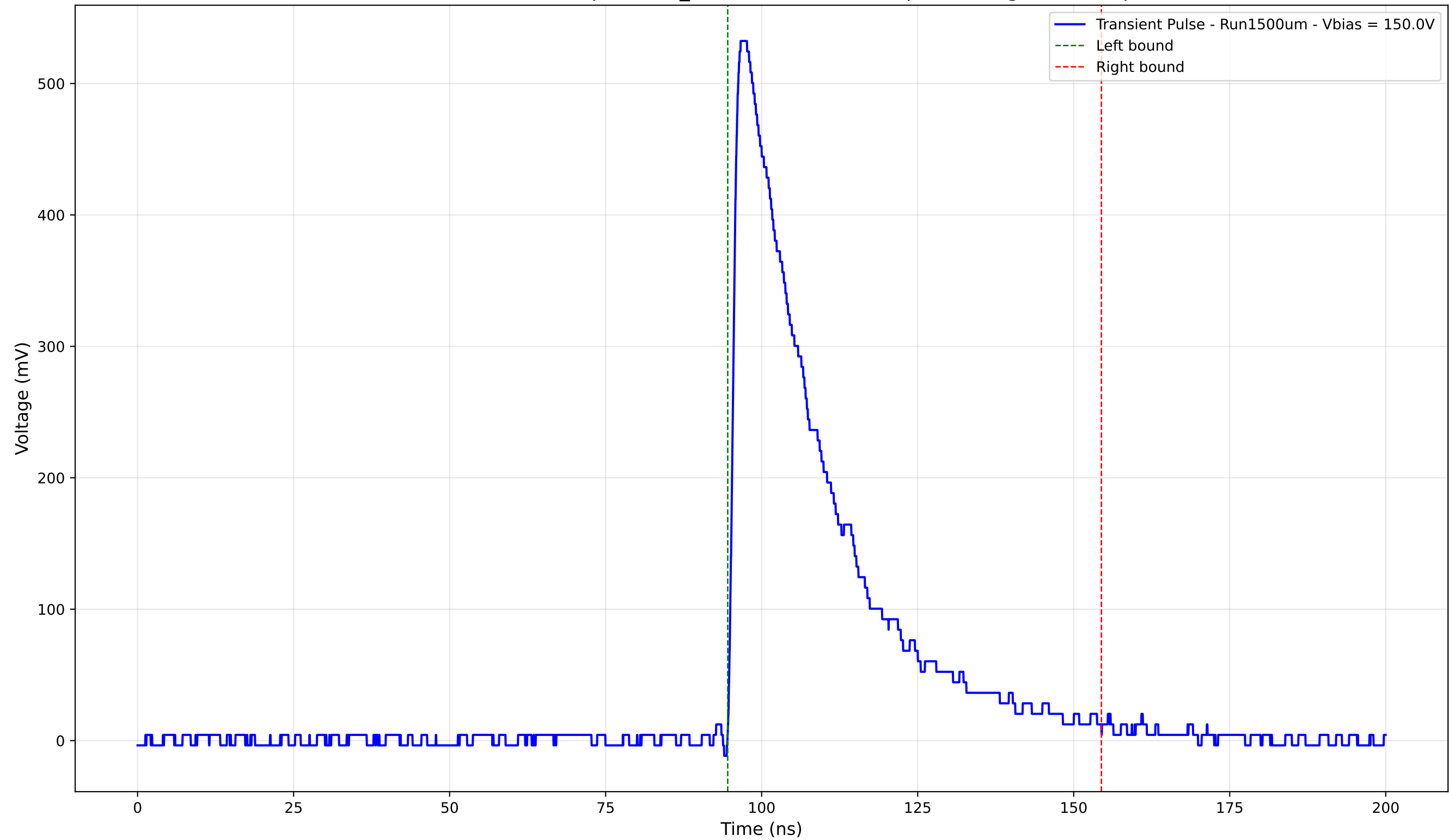
Transient Pulse - Sample: 1cm_42 - Position: 1000.0 \mu\text{m} - Charge: 165.56 pC
