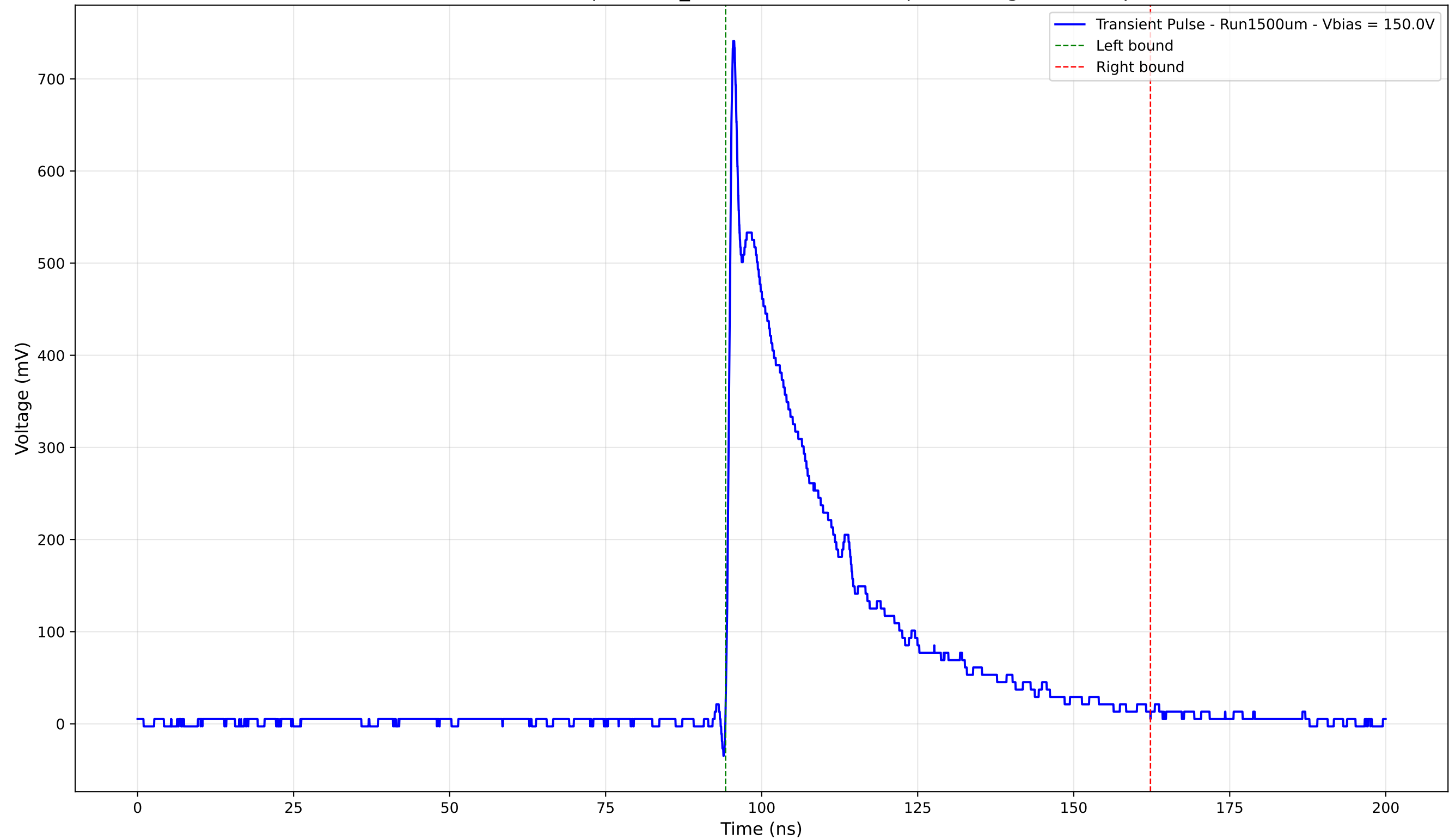
Transient Pulse - Sample: 1cm_42 - Position: 2265.0 \mu\text{m} - Charge: 201.11 pC
