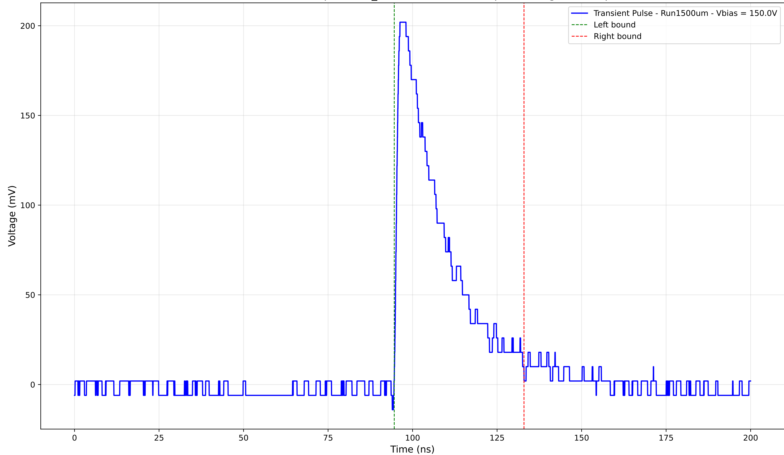
Transient Pulse - Sample: 1cm_42 - Position: 4095.0 \mu\text{m} - Charge: 59.07 pC
