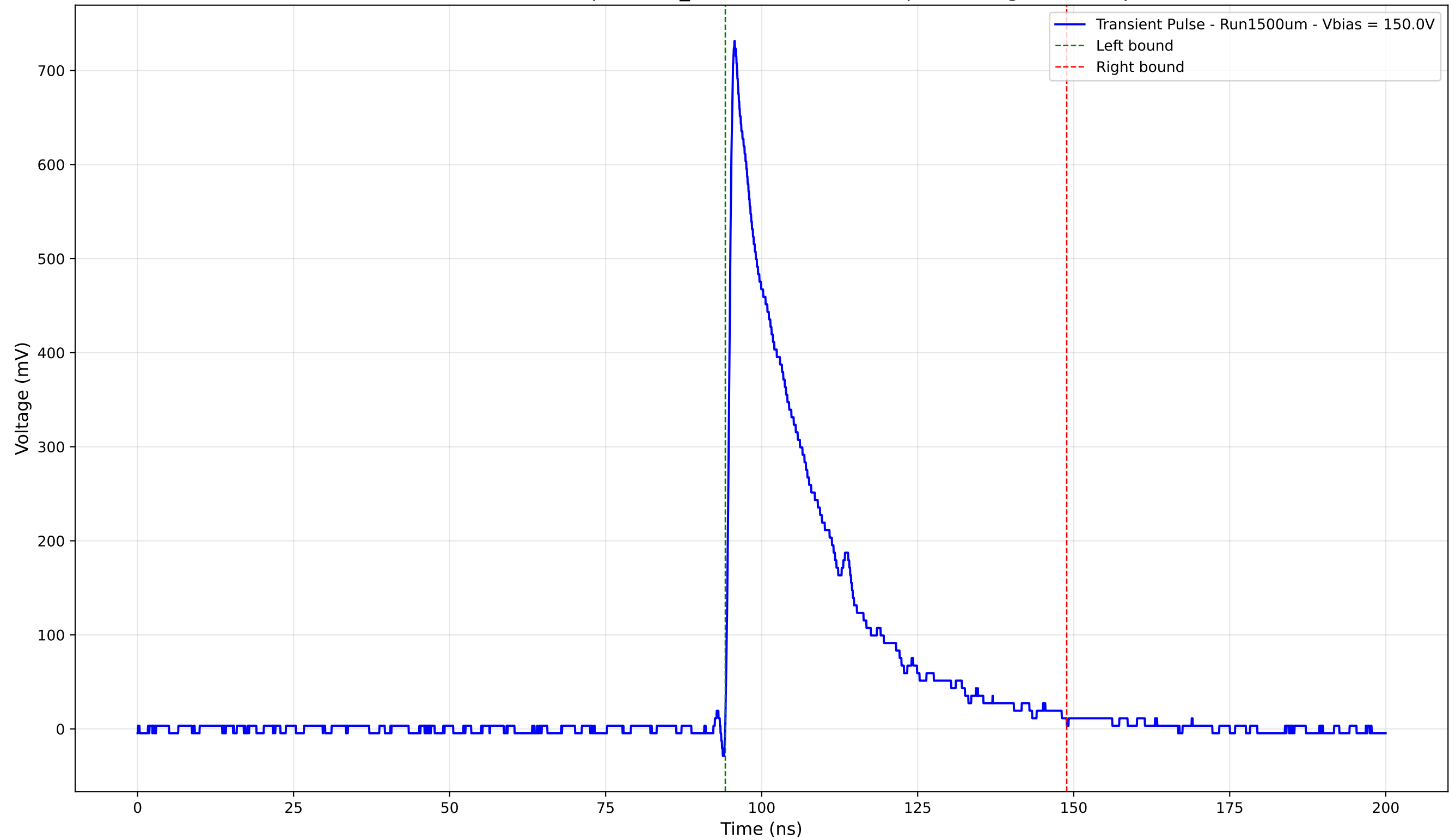
Transient Pulse - Sample: 1cm_42 - Position: 4765.0 \mu\text{m} - Charge: 182.31 pC
