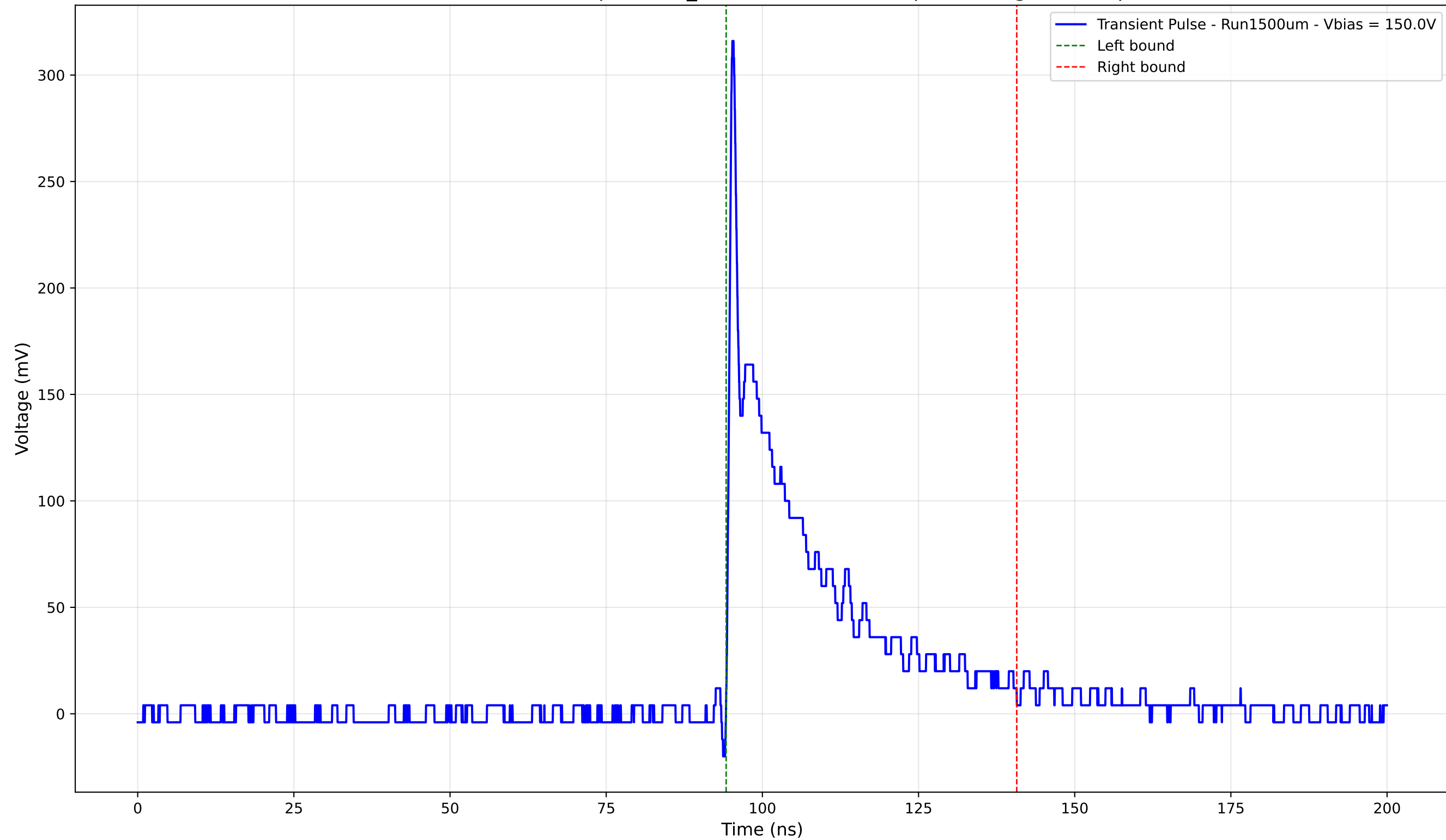
Transient Pulse - Sample: 1cm_42 - Position: 2580.0 \mu\text{m} - Charge: 57.84 pC
