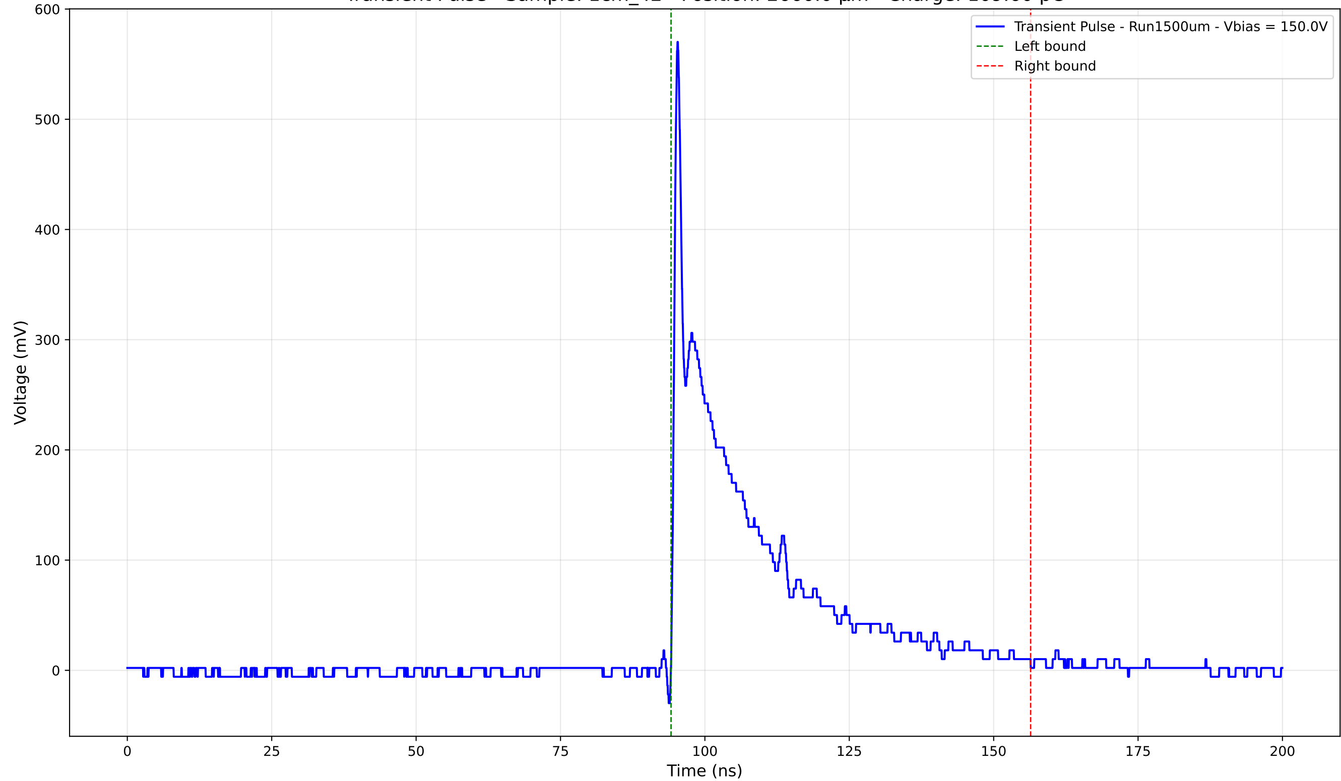
Transient Pulse - Sample: 1cm_42 - Position: 2660.0 \mu\text{m} - Charge: 109.60 pC
