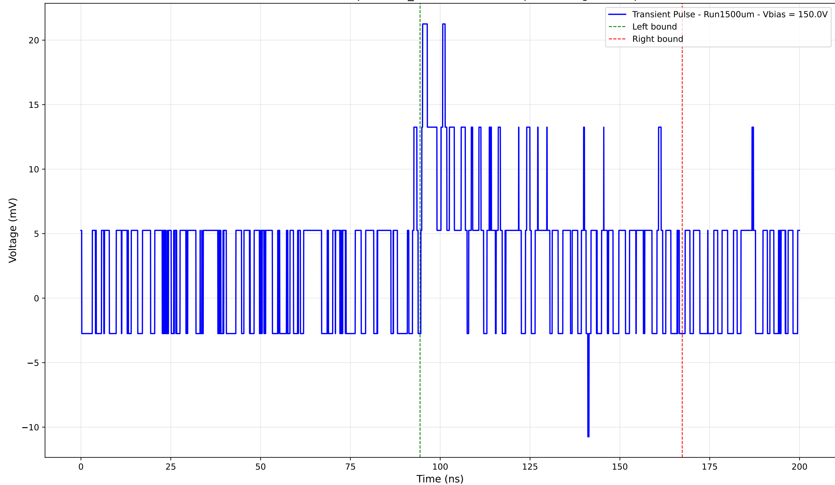
Transient Pulse - Sample: 1cm_42 - Position: 25.0 \mu\text{m} - Charge: 6.85 pC
