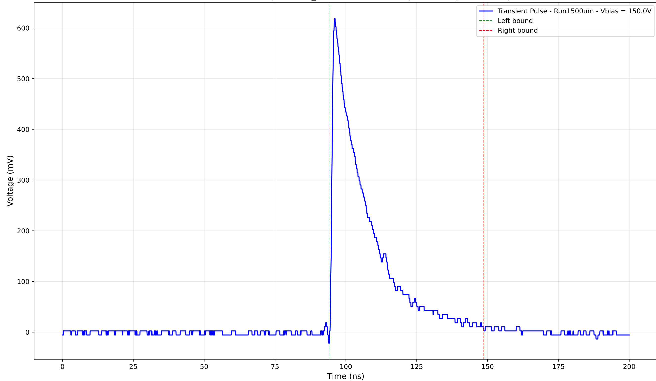
Transient Pulse - Sample: 1cm_42 - Position: 485.0 \mu\text{m} - Charge: 159.02 pC
