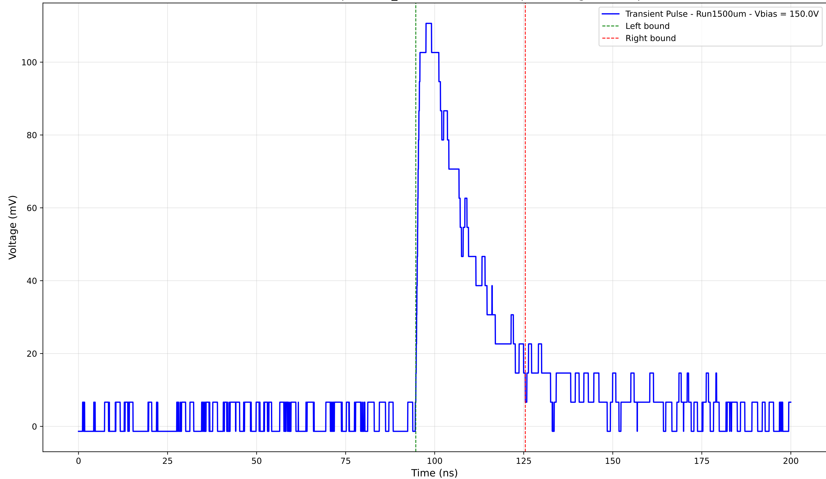
Transient Pulse - Sample: 1cm_42 - Position: 3620.0 \mu\text{m} - Charge: 33.89 pC
