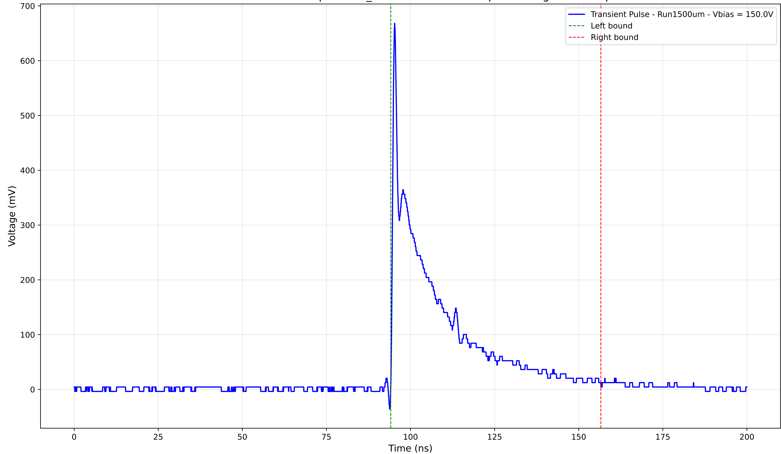
Transient Pulse - Sample: 1cm_42 - Position: 2670.0 \mu\text{m} - Charge: 133.26 pC
