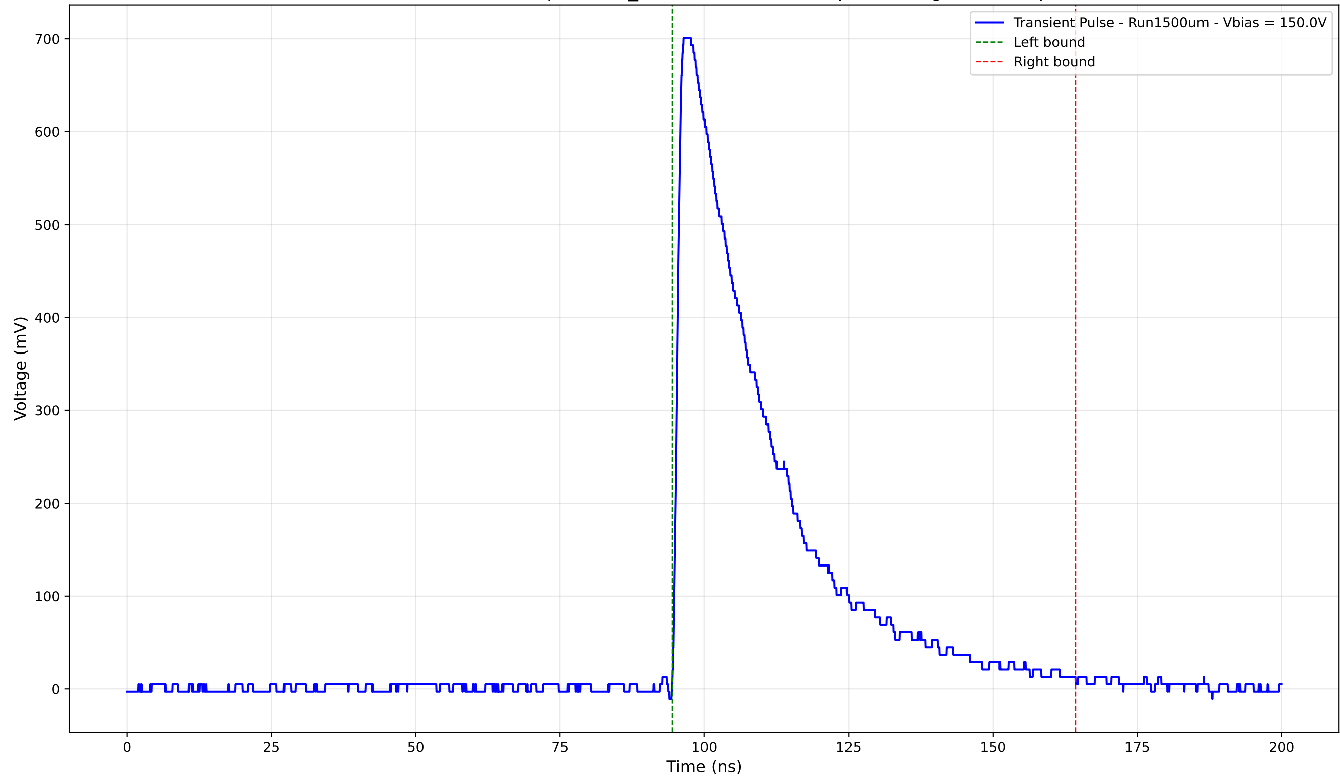
Transient Pulse - Sample: 1cm_42 - Position: 3780.0 \mu\text{m} - Charge: 238.76 pC
