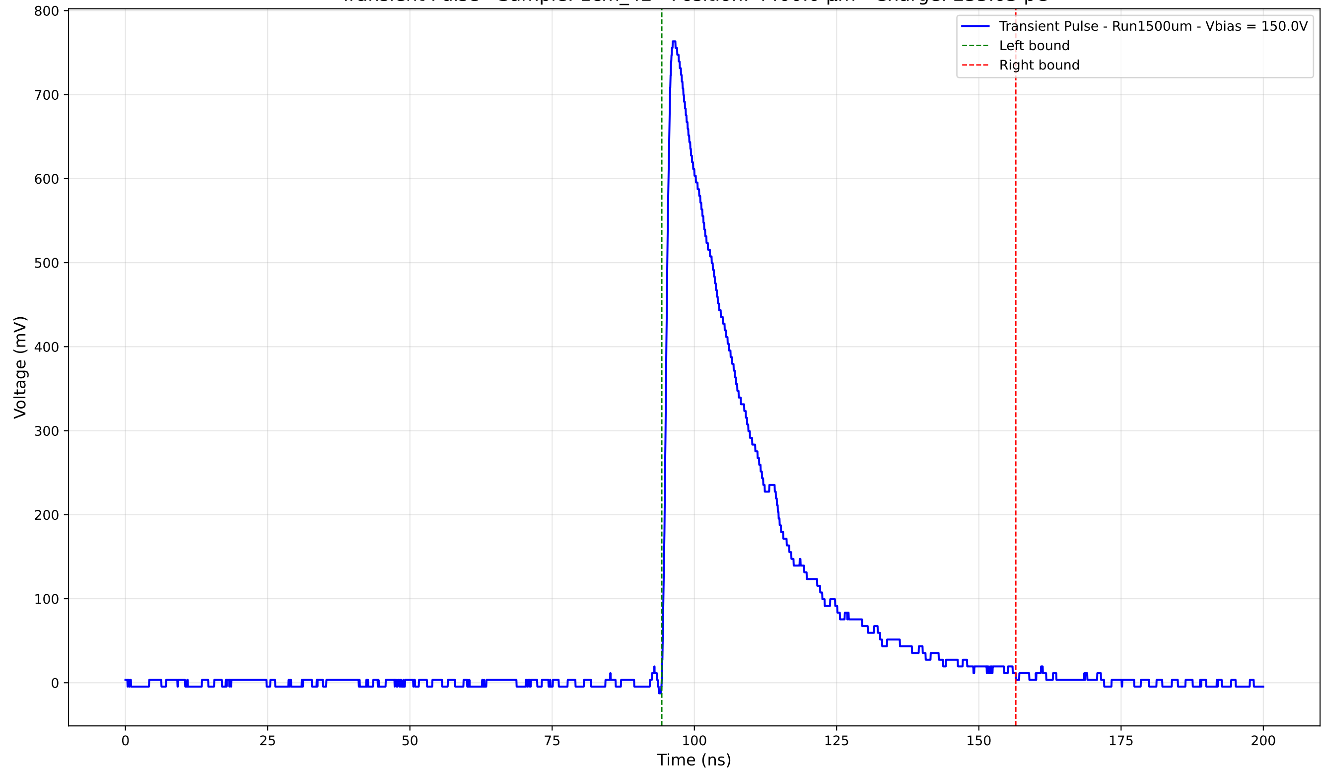
Transient Pulse - Sample: 1cm_42 - Position: 4400.0 \mu\text{m} - Charge: 233.03 pC
