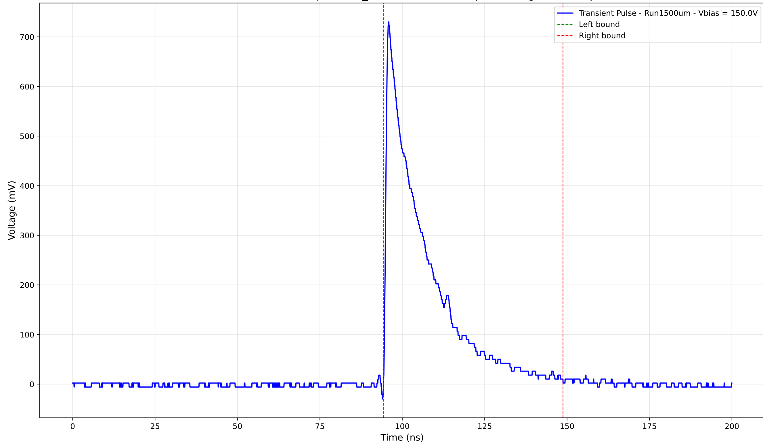
Transient Pulse - Sample: 1cm_42 - Position: 360.0 \mu\text{m} - Charge: 176.70 pC
