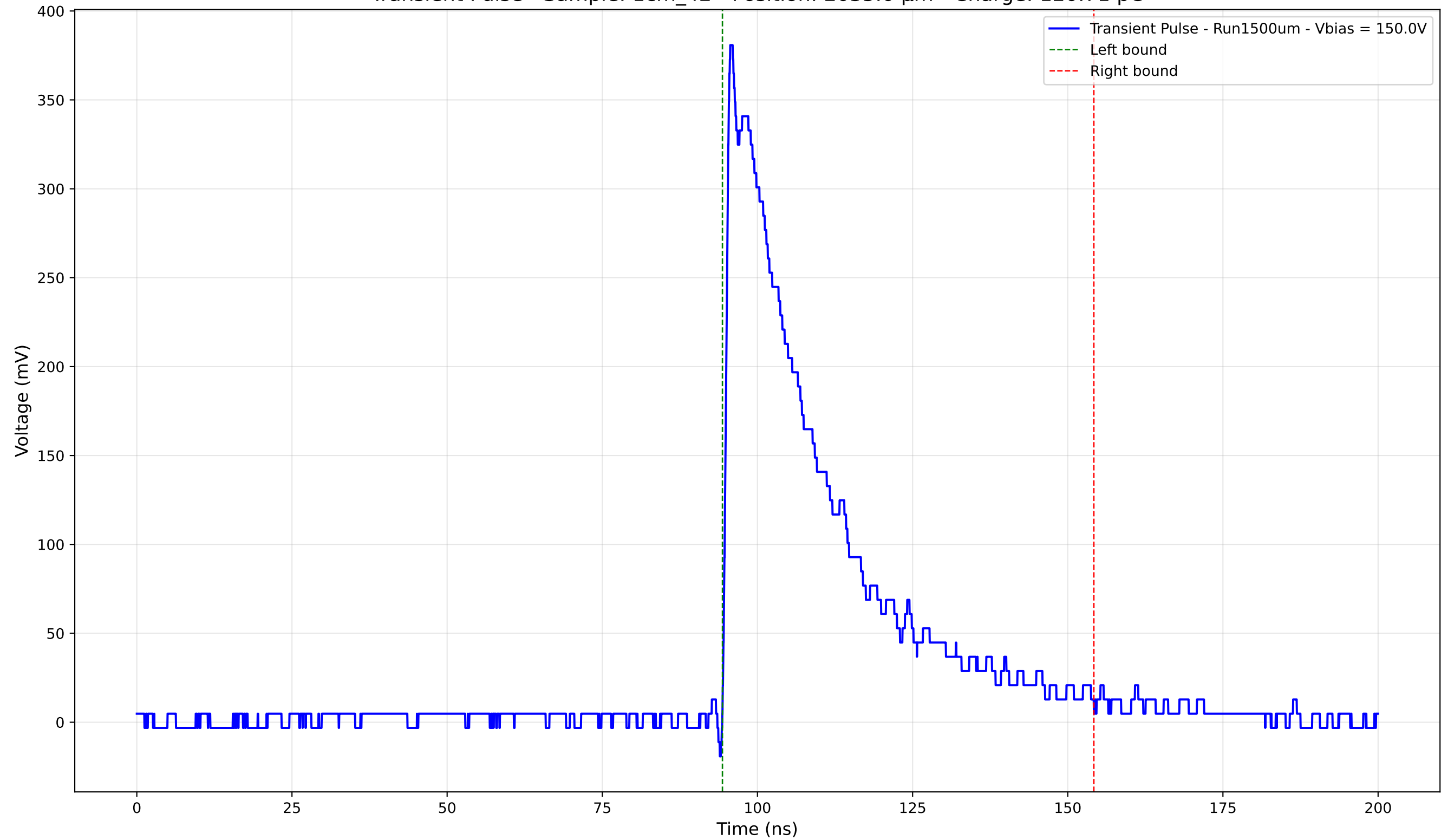
Transient Pulse - Sample: 1cm_42 - Position: 2035.0 \mu\text{m} - Charge: 120.71 pC
