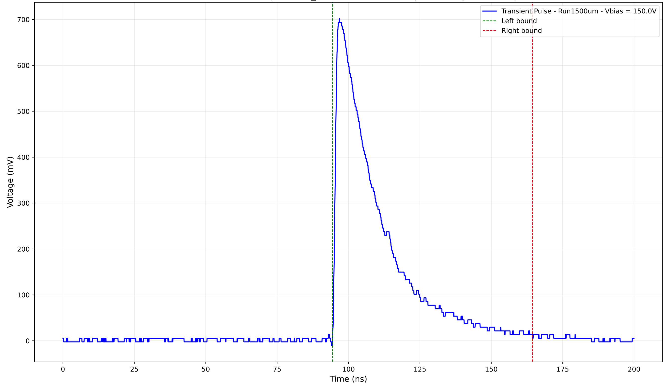
Transient Pulse - Sample: 1cm_42 - Position: 3875.0 \mu\text{m} - Charge: 235.37 pC
