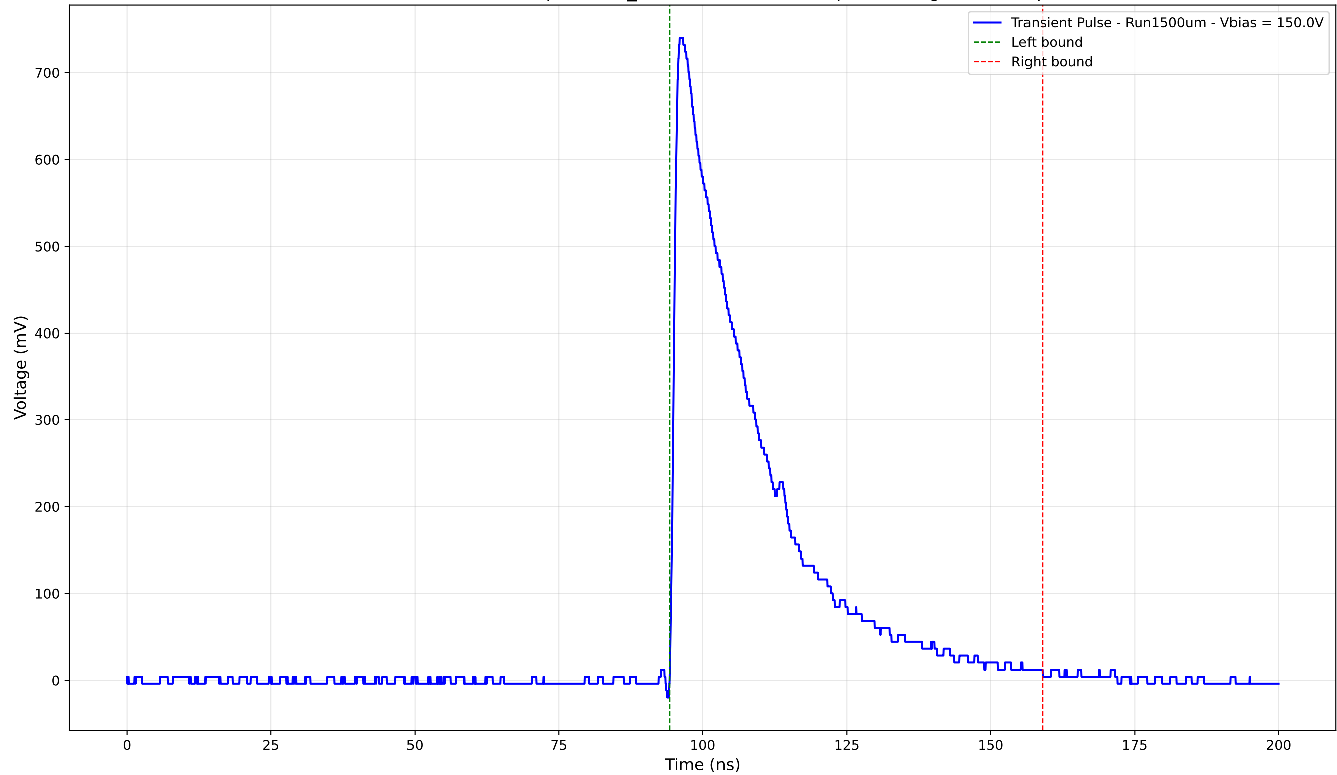
Transient Pulse - Sample: 1cm_42 - Position: 4470.0 \mu\text{m} - Charge: 223.83 pC
