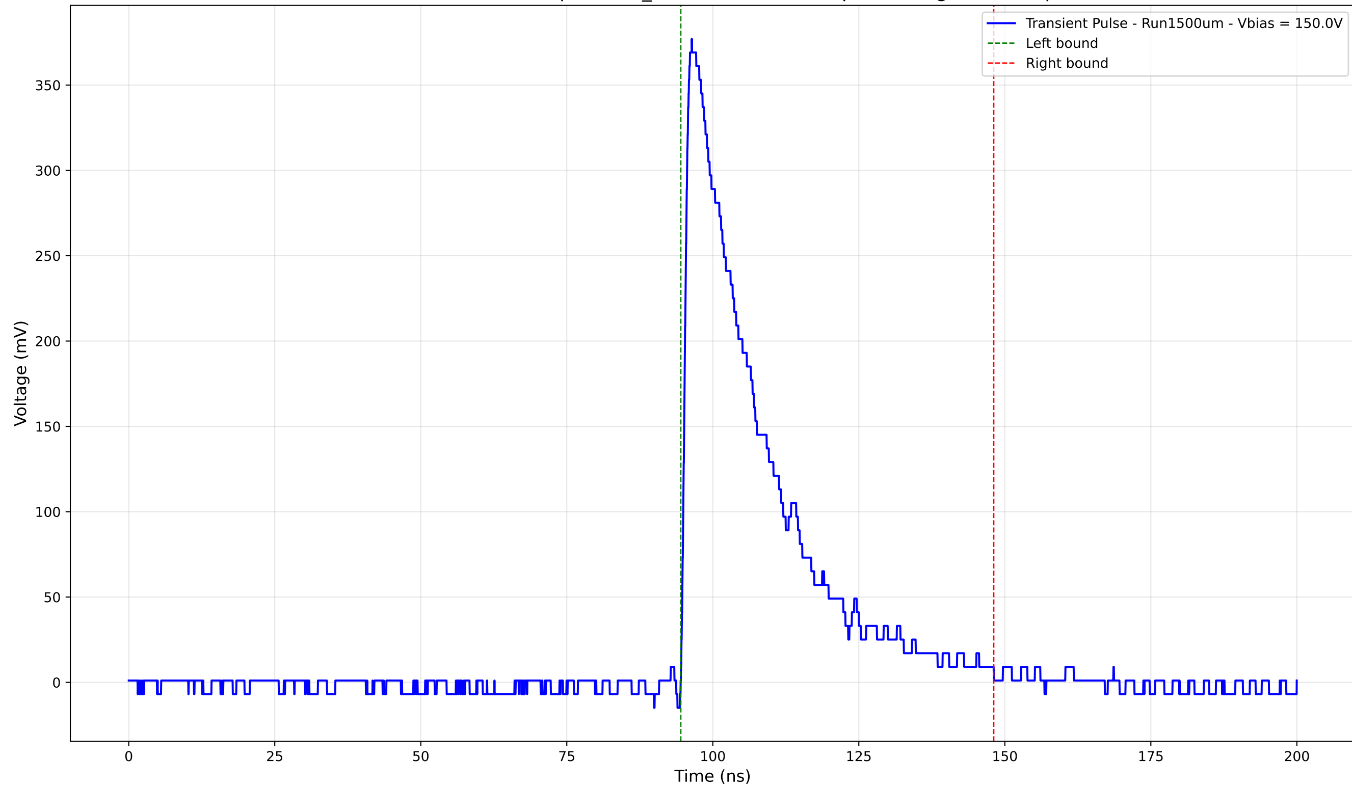
Transient Pulse - Sample: 1cm_42 - Position: 645.0 \mu\text{m} - Charge: 103.56 pC
