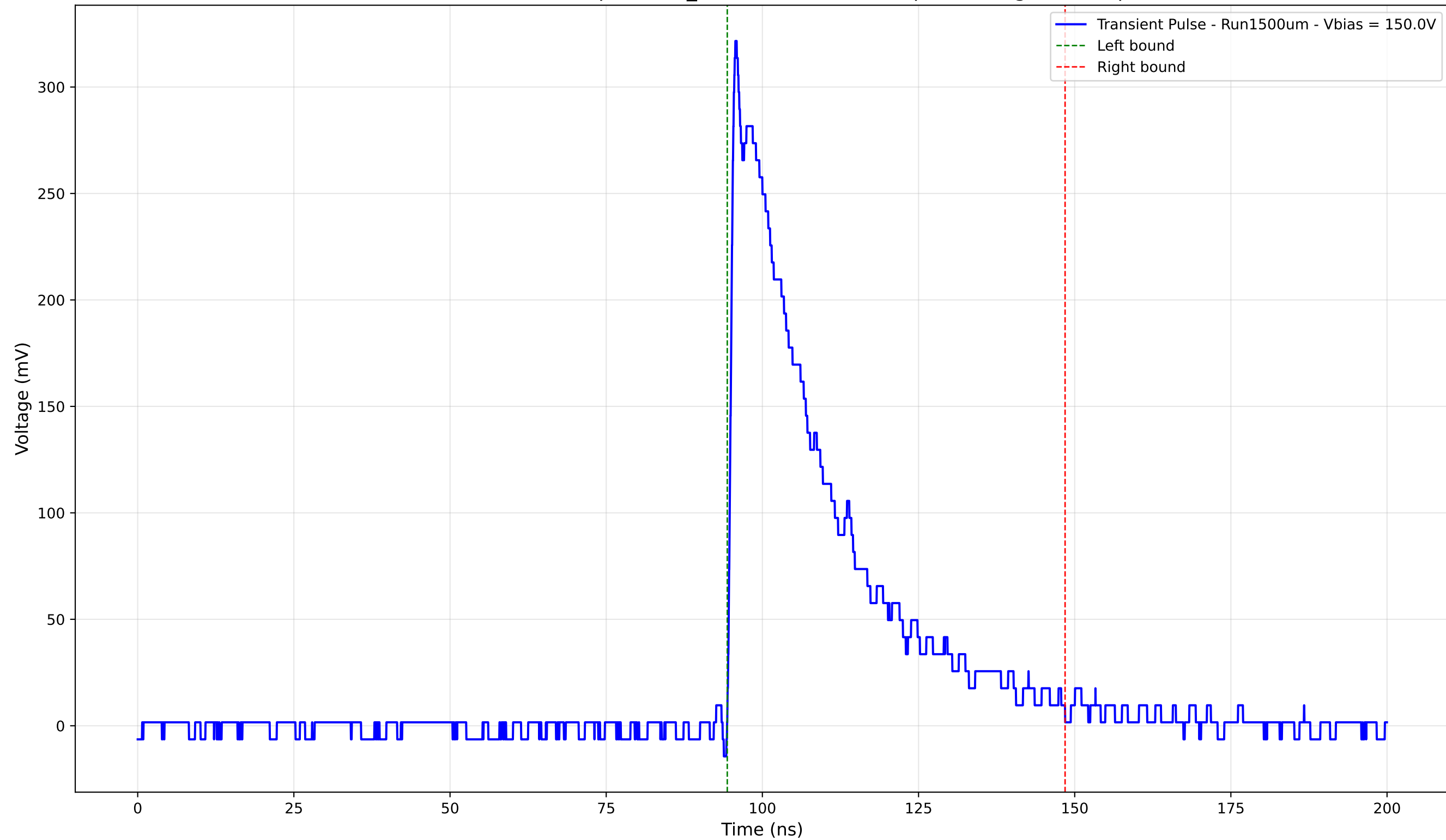
Transient Pulse - Sample: 1cm_42 - Position: 2045.0 \mu\text{m} - Charge: 96.36 pC
