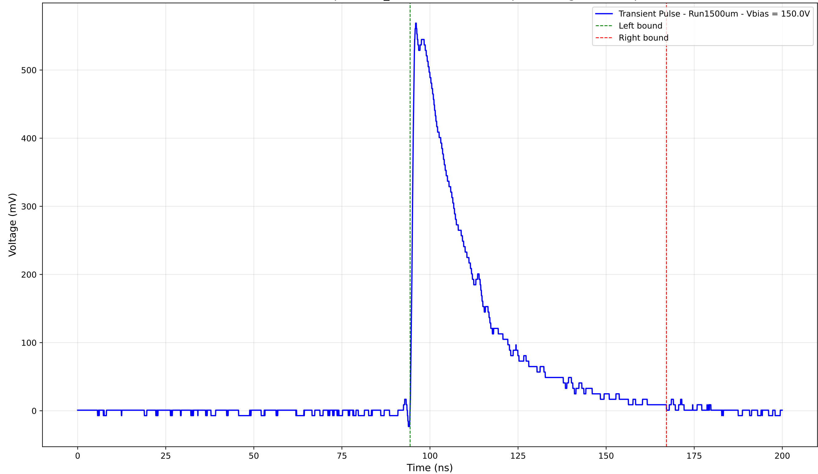
Transient Pulse - Sample: 1cm_42 - Position: 1895.0 \mu\text{m} - Charge: 193.63 pC
