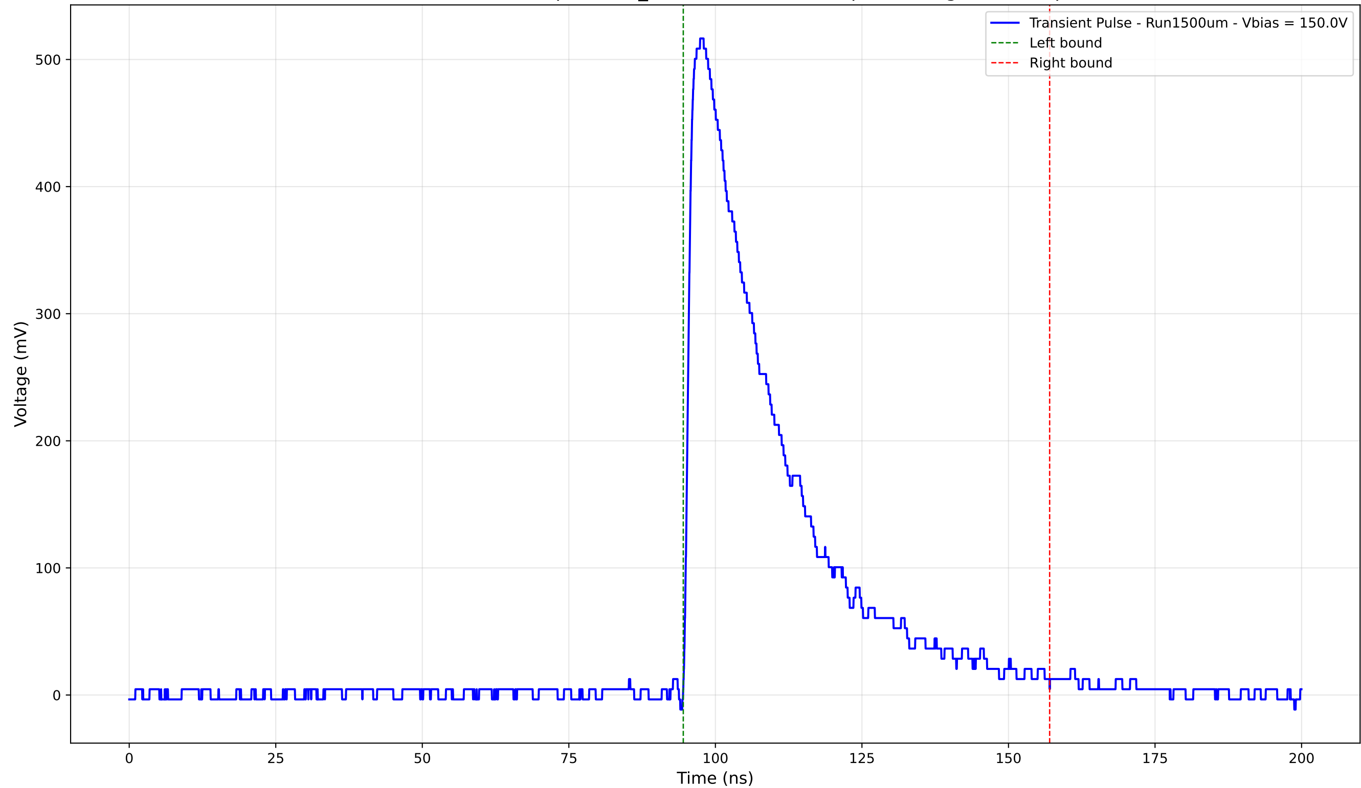
Transient Pulse - Sample: 1cm_42 - Position: 1495.0 \mu\text{m} - Charge: 172.77 pC
