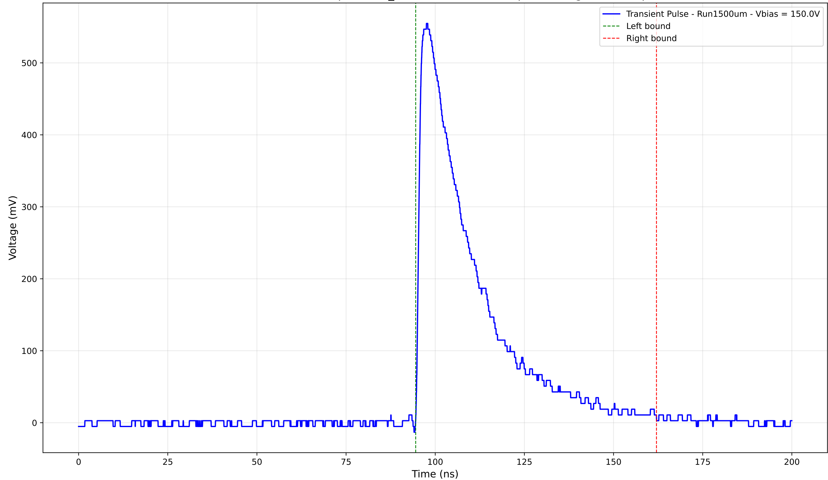
Transient Pulse - Sample: 1cm_42 - Position: 1460.0 \mu\text{m} - Charge: 185.24 pC
