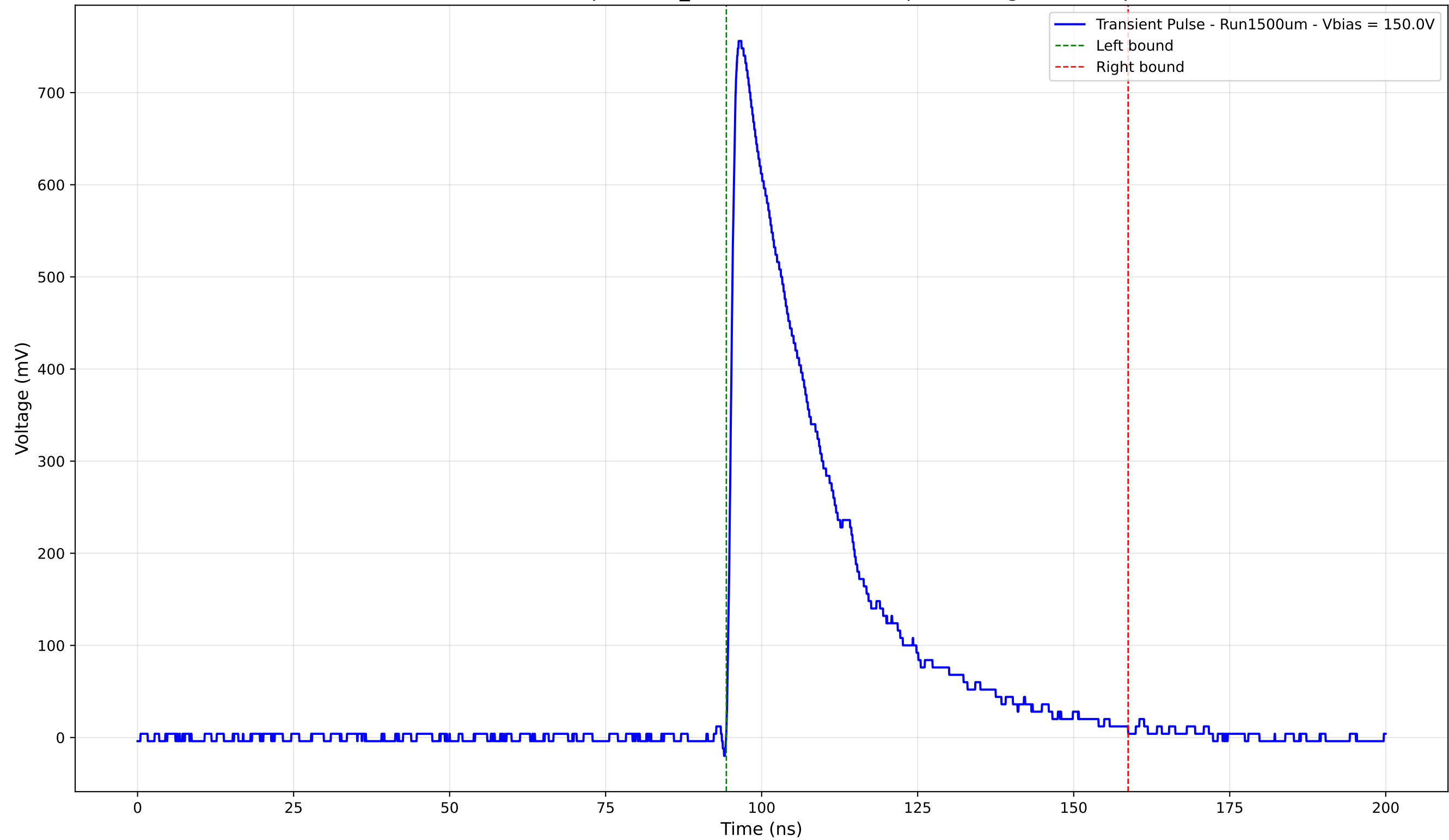
Transient Pulse - Sample: 1cm_42 - Position: 4320.0 \mu\text{m} - Charge: 236.07 pC
