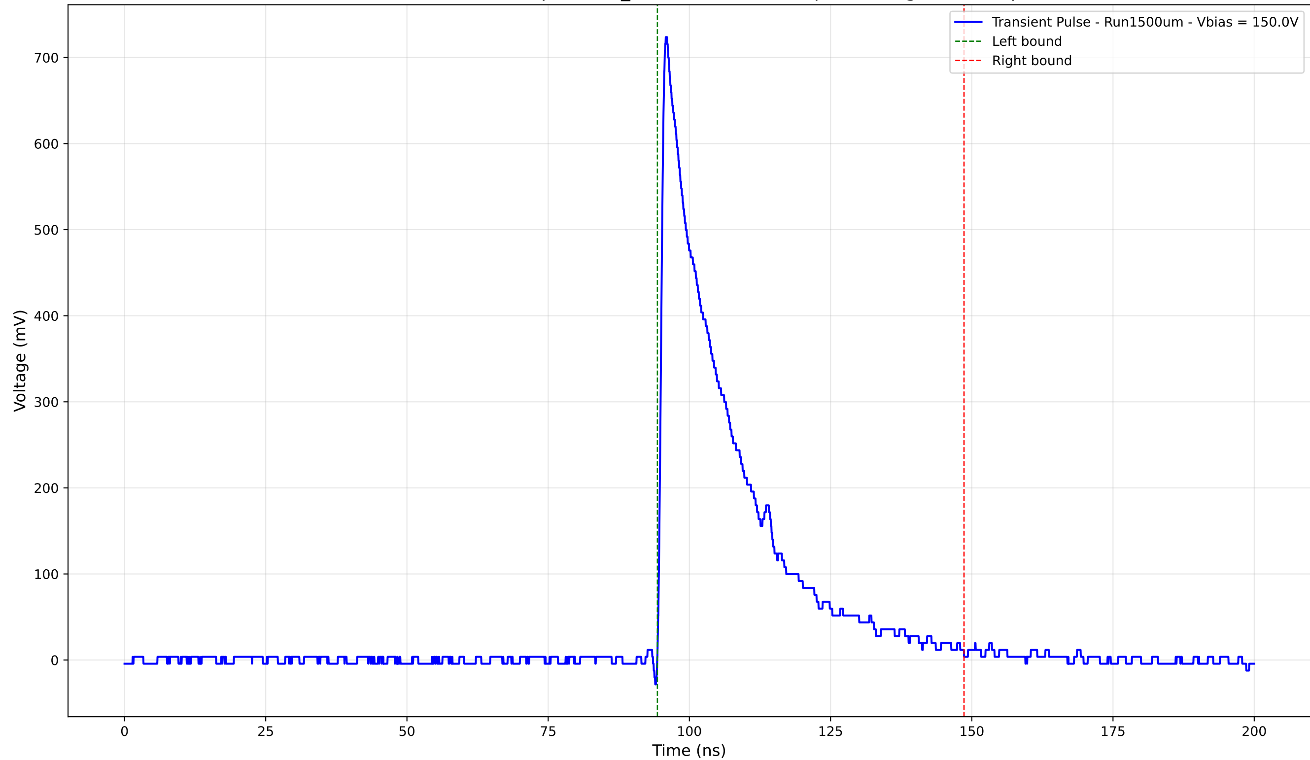
Transient Pulse - Sample: 1cm_42 - Position: 375.0 \mu\text{m} - Charge: 179.74 pC
