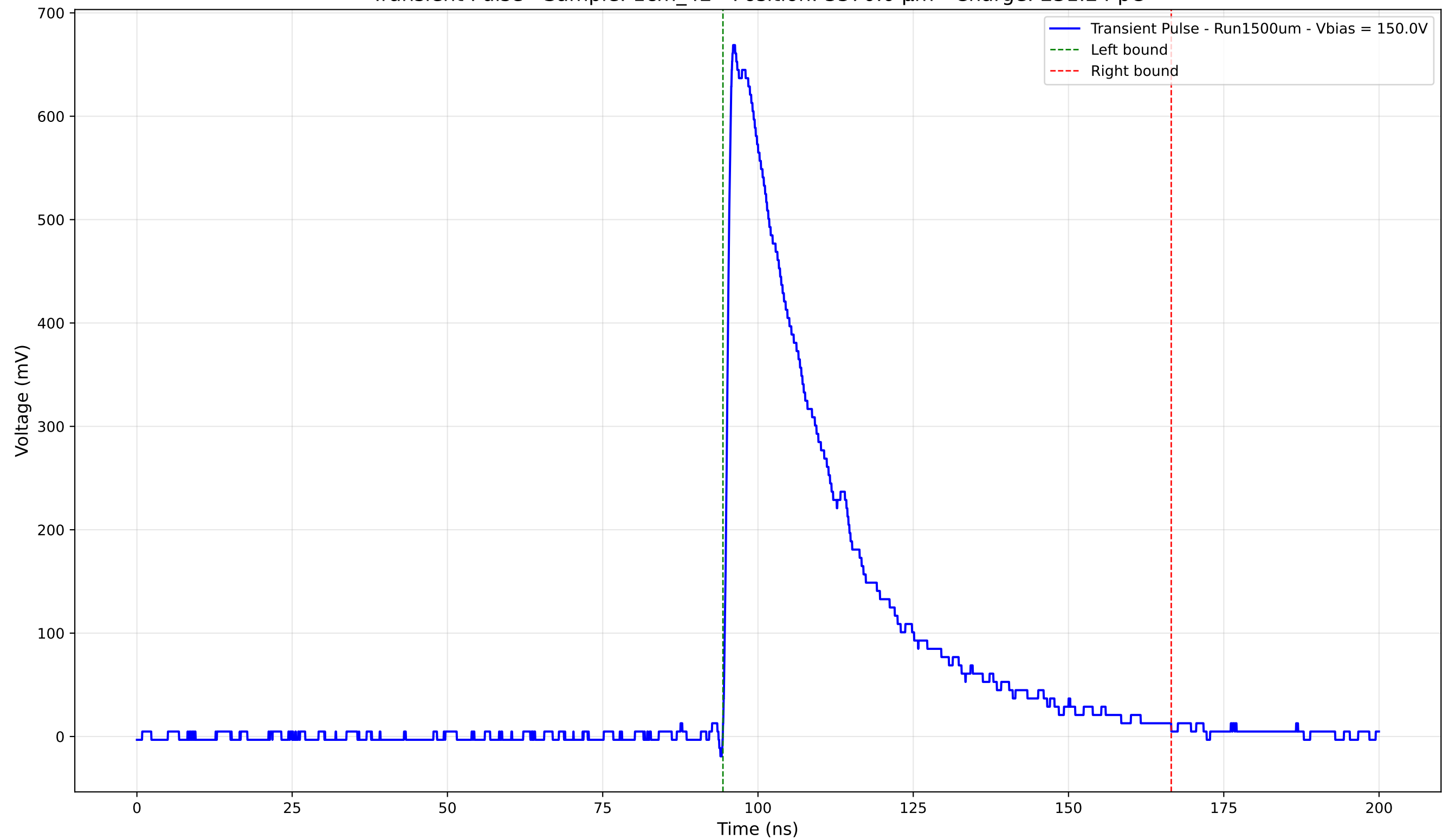
Transient Pulse - Sample: 1cm_42 - Position: 3370.0 \mu\text{m} - Charge: 231.24 pC
