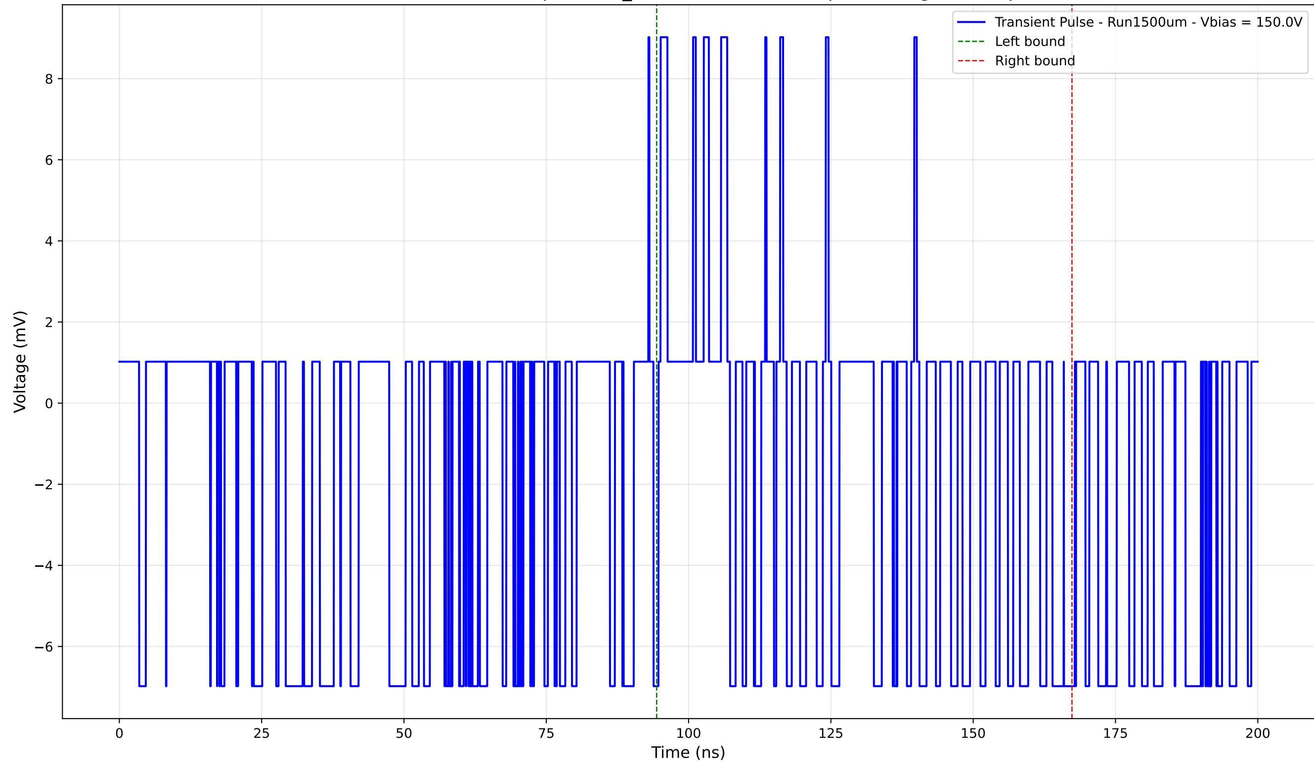
Transient Pulse - Sample: 1cm_42 - Position: 5050.0 \mu\text{m} - Charge: -1.44 pC
