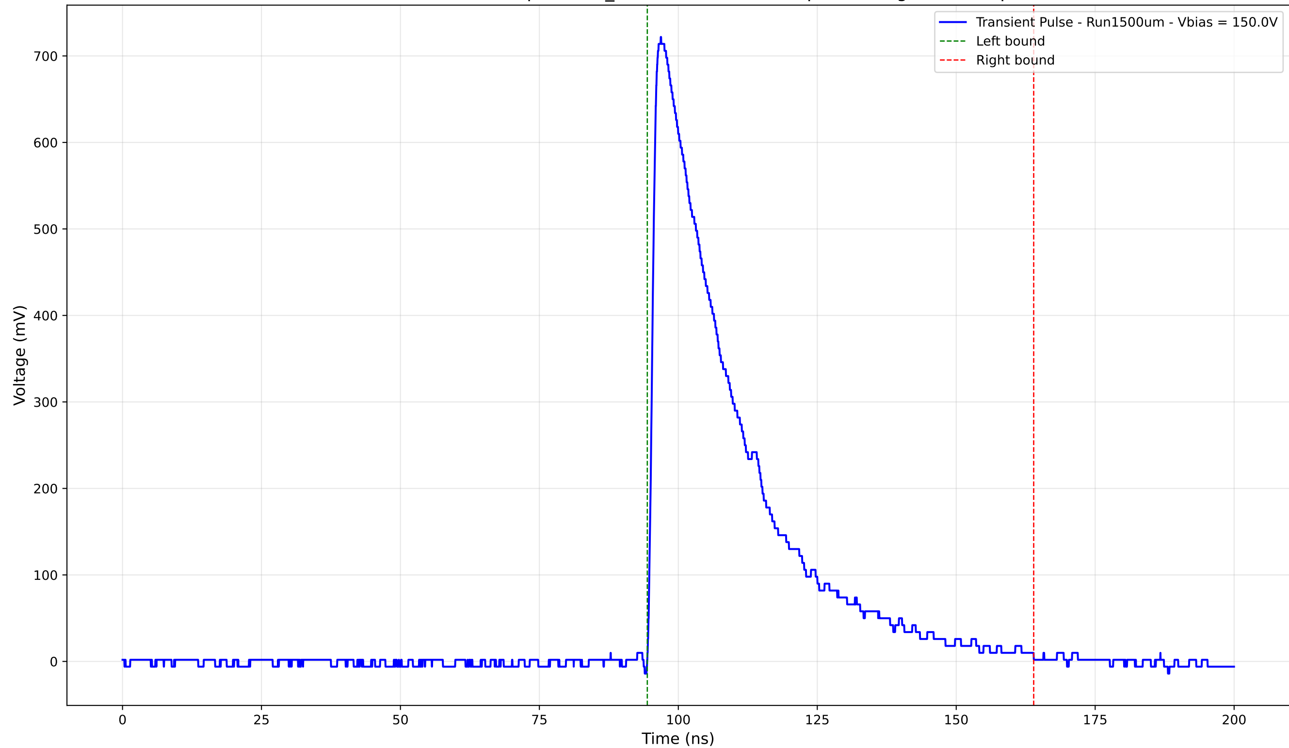
Transient Pulse - Sample: 1cm_42 - Position: 3980.0 \mu\text{m} - Charge: 234.91 pC
