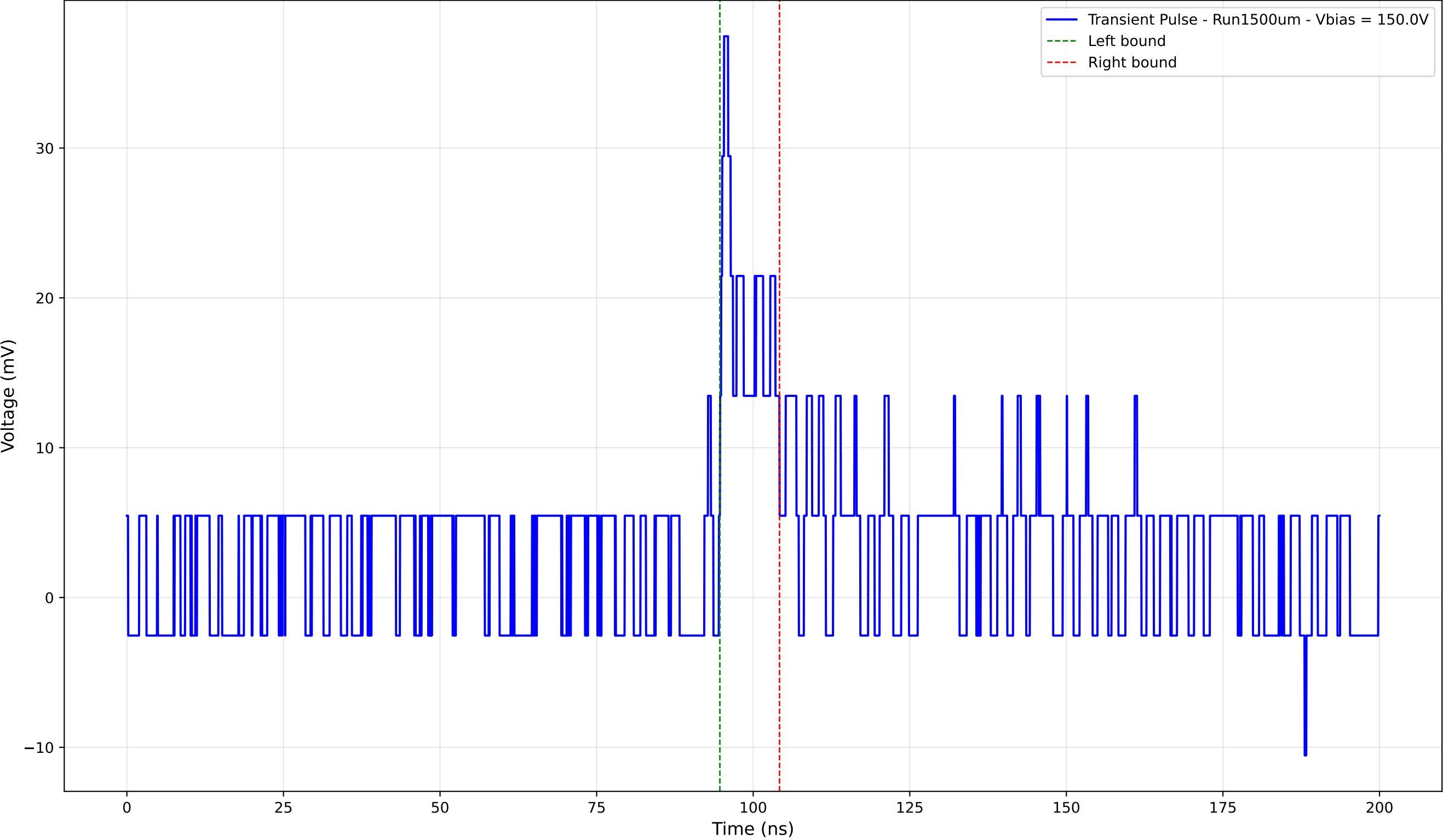
Transient Pulse - Sample: 1cm_42 - Position: 4970.0 \mu\text{m} - Charge: 3.70 pC
