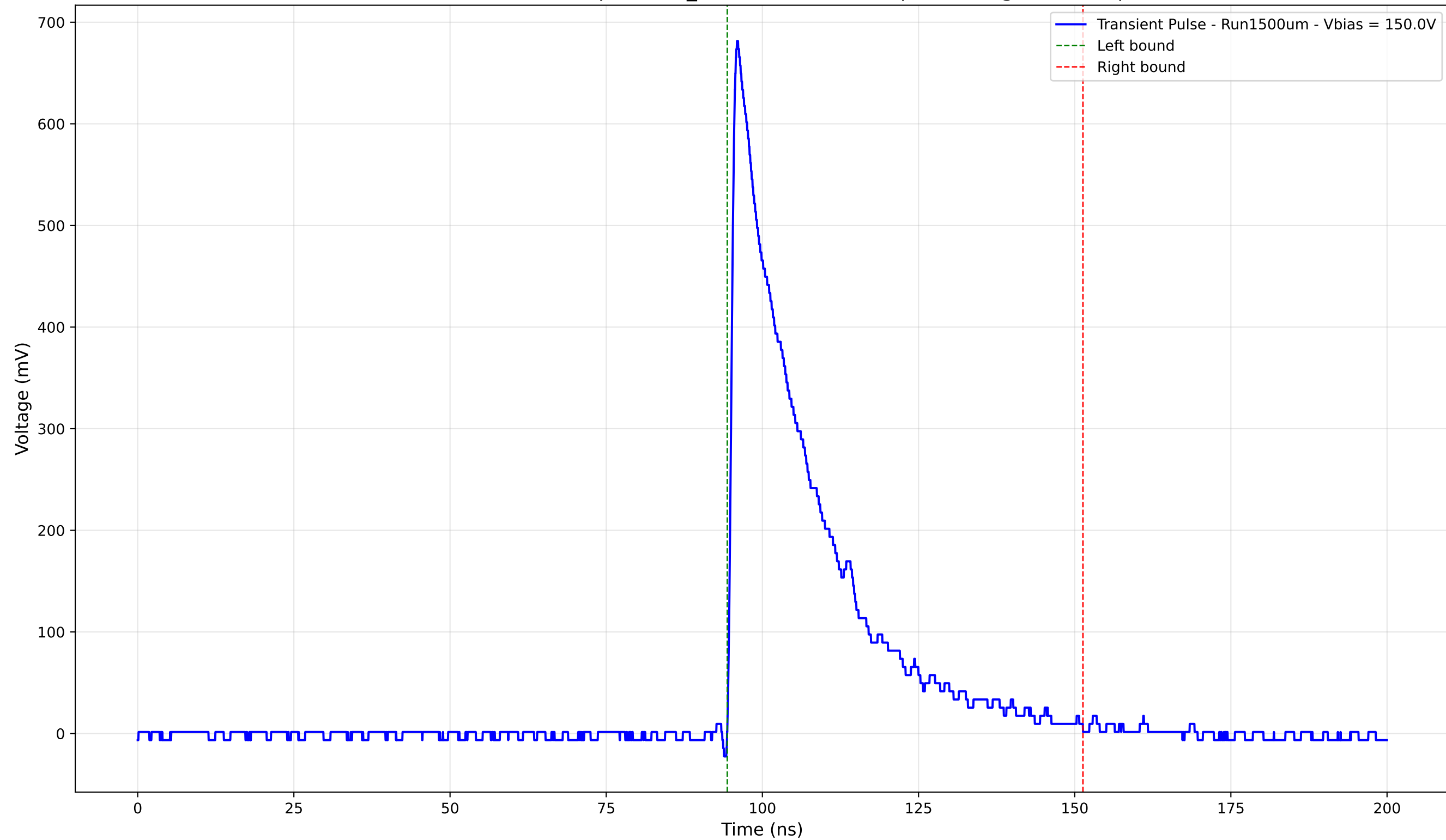
Transient Pulse - Sample: 1cm_42 - Position: 440.0 \mu\text{m} - Charge: 172.57 pC
