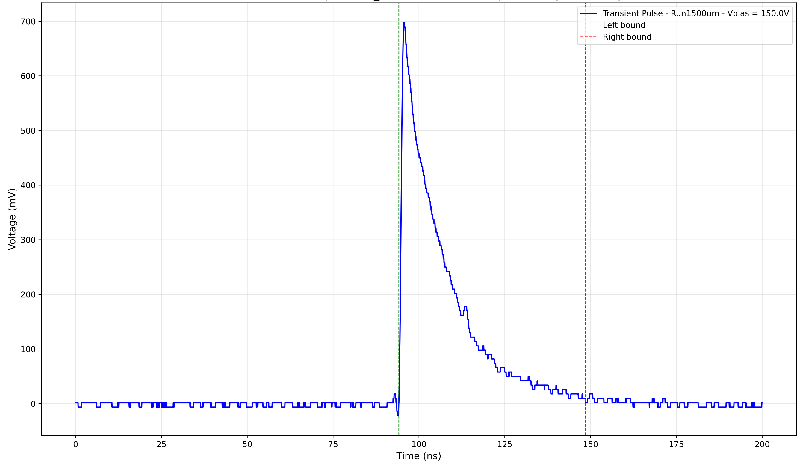
Transient Pulse - Sample: 1cm_42 - Position: 4740.0 \mu\text{m} - Charge: 175.16 pC
