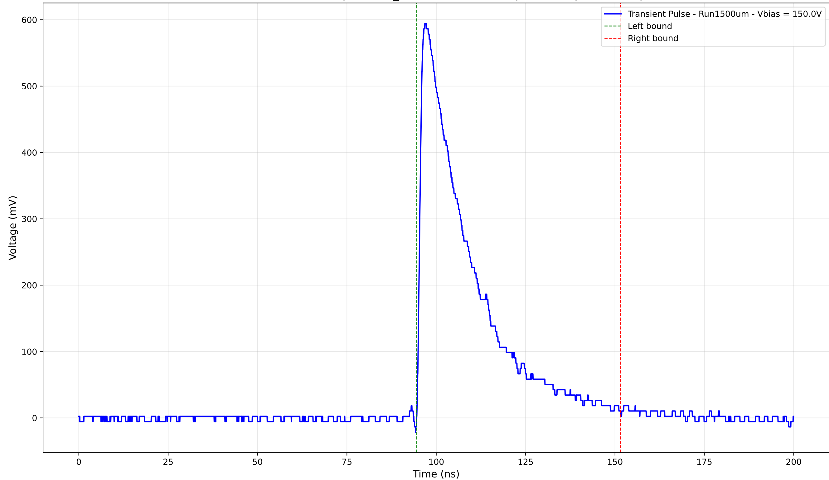
Transient Pulse - Sample: 1cm_42 - Position: 940.0 \mu\text{m} - Charge: 181.03 pC
