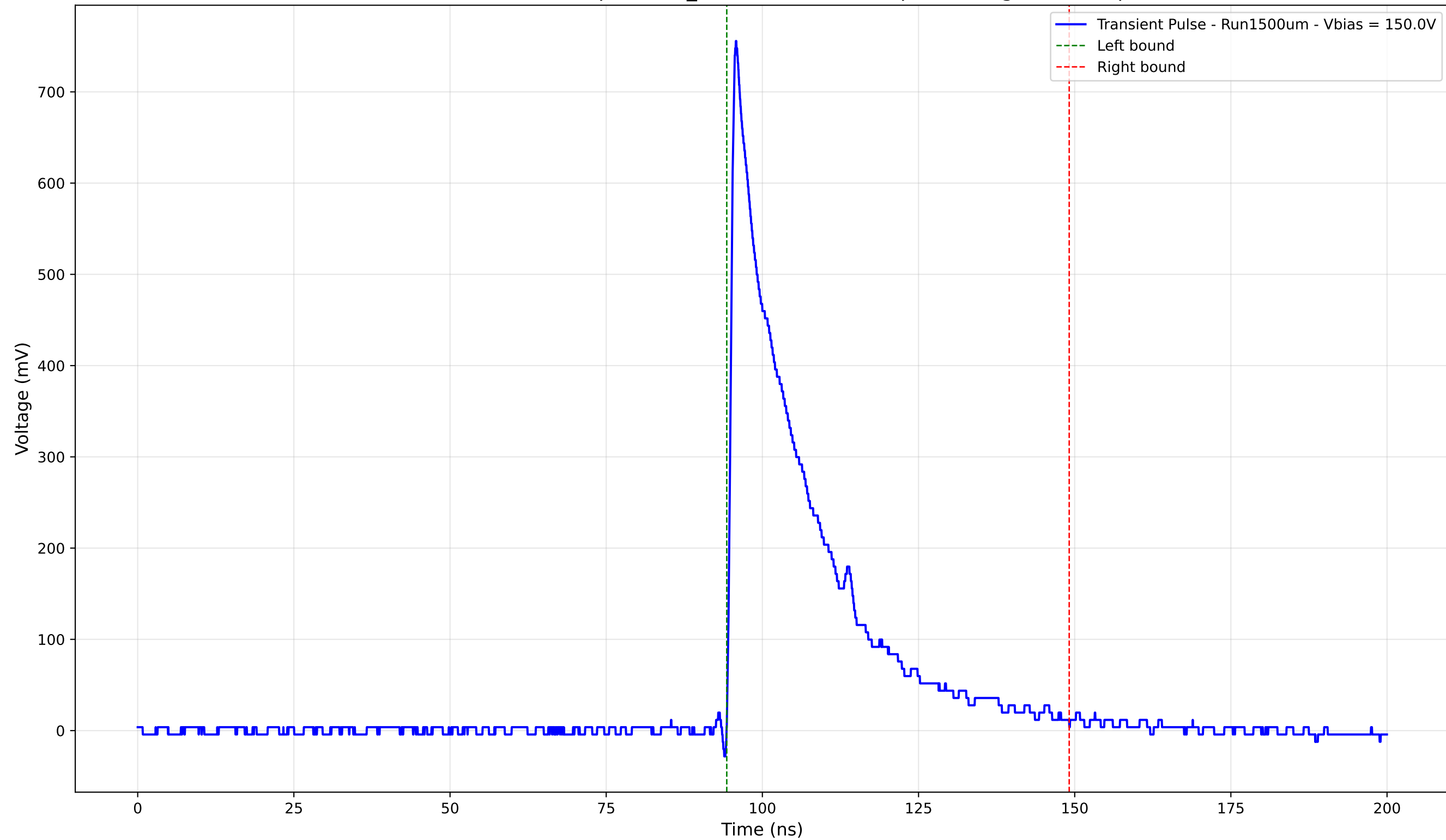
Transient Pulse - Sample: 1cm_42 - Position: 285.0 \mu\text{m} - Charge: 177.17 pC
