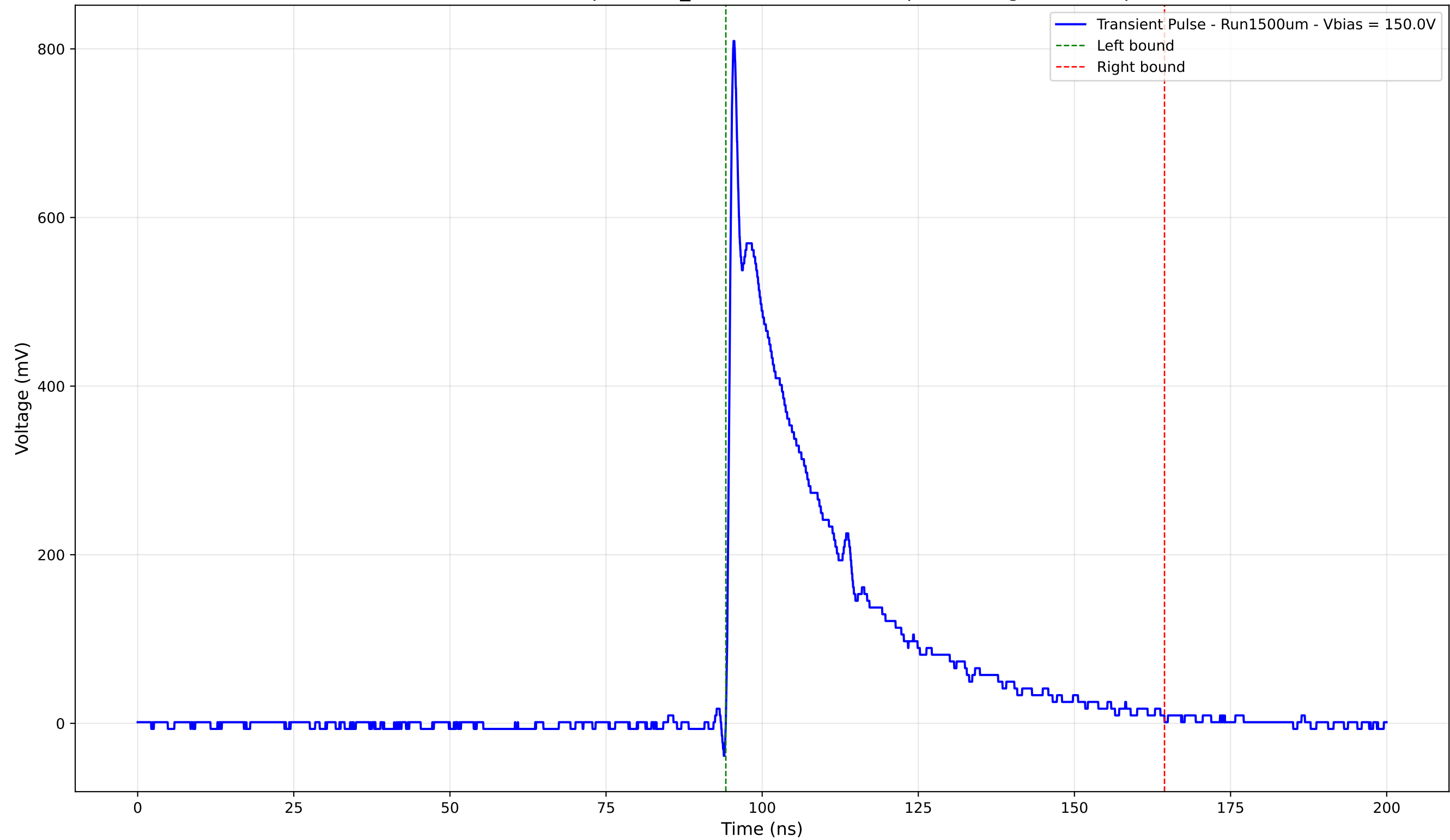
Transient Pulse - Sample: 1cm_42 - Position: 2900.0 \mu\text{m} - Charge: 212.17 pC
