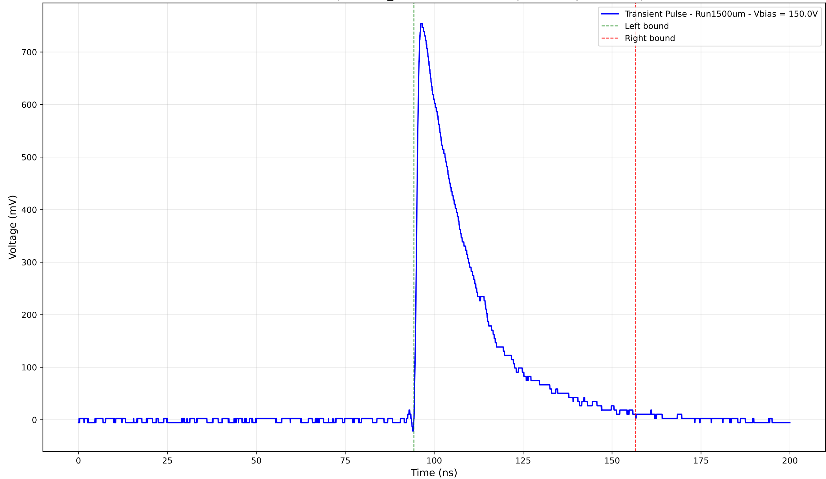
Transient Pulse - Sample: 1cm_42 - Position: 4345.0 \mu\text{m} - Charge: 233.49 pC
