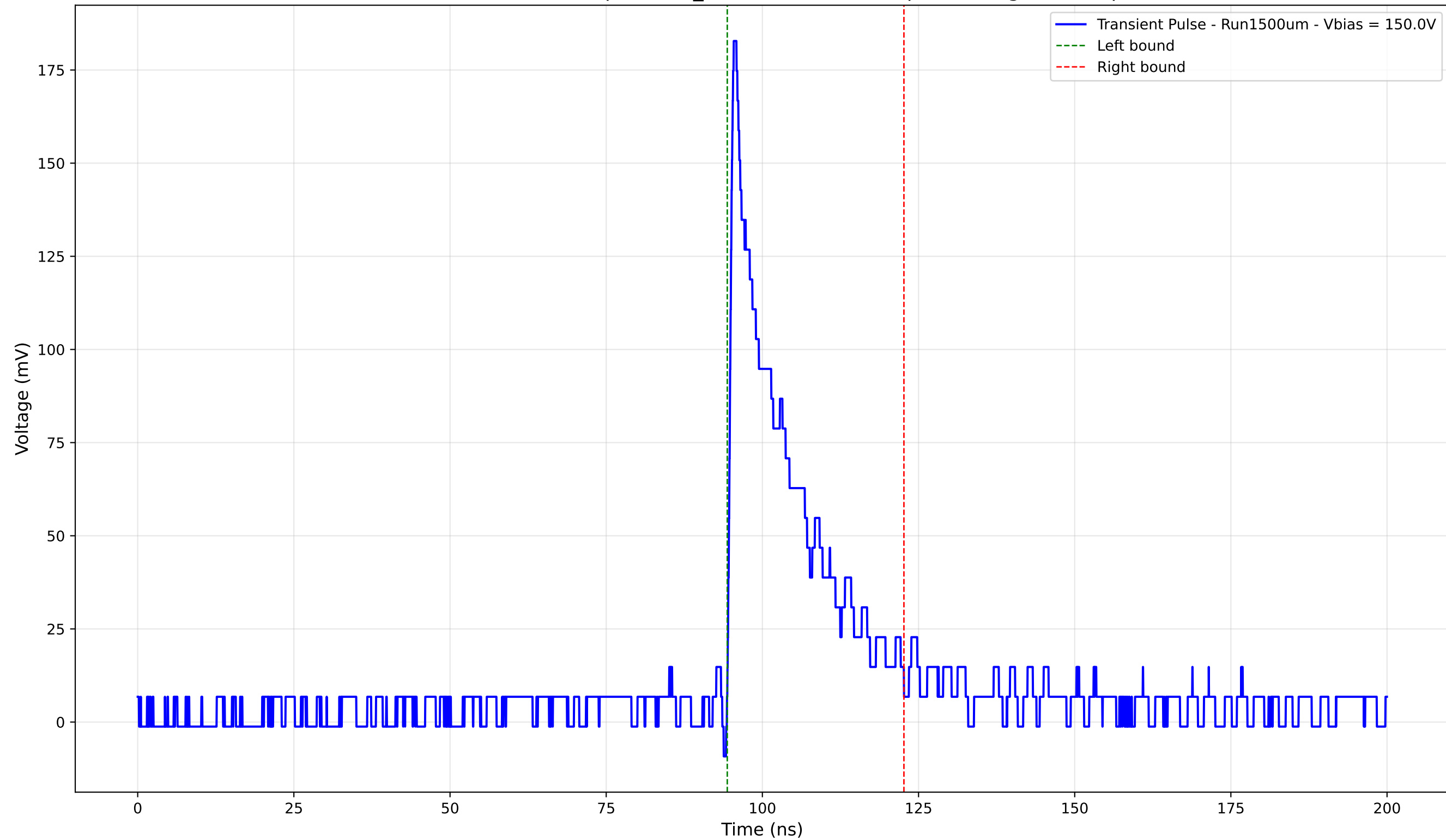
Transient Pulse - Sample: 1cm_42 -Position: 105.0 \mu\text{m} - Charge: 33.94 pC
