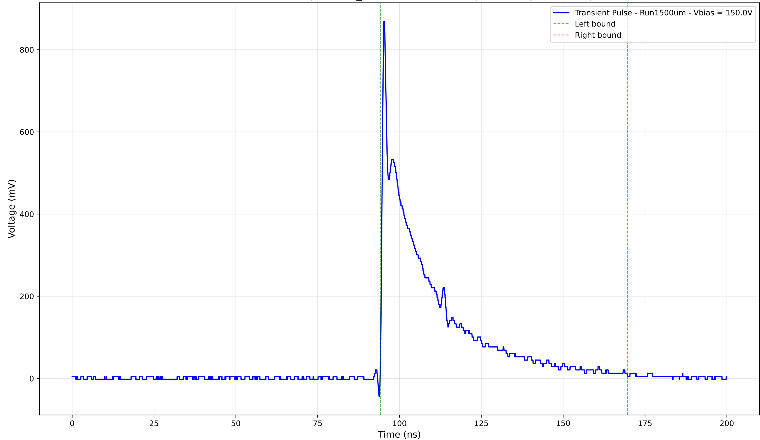
Transient Pulse - Sample: 1cm_42 - Position: 2715.0 \mu\text{m} - Charge: 202.96 pC
