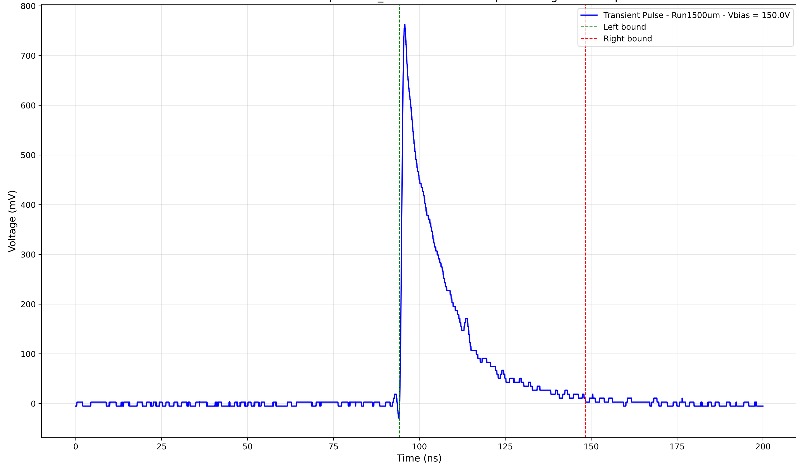
Transient Pulse - Sample: 1cm_42 - Position: 240.0 \mu\text{m} - Charge: 170.70 pC
