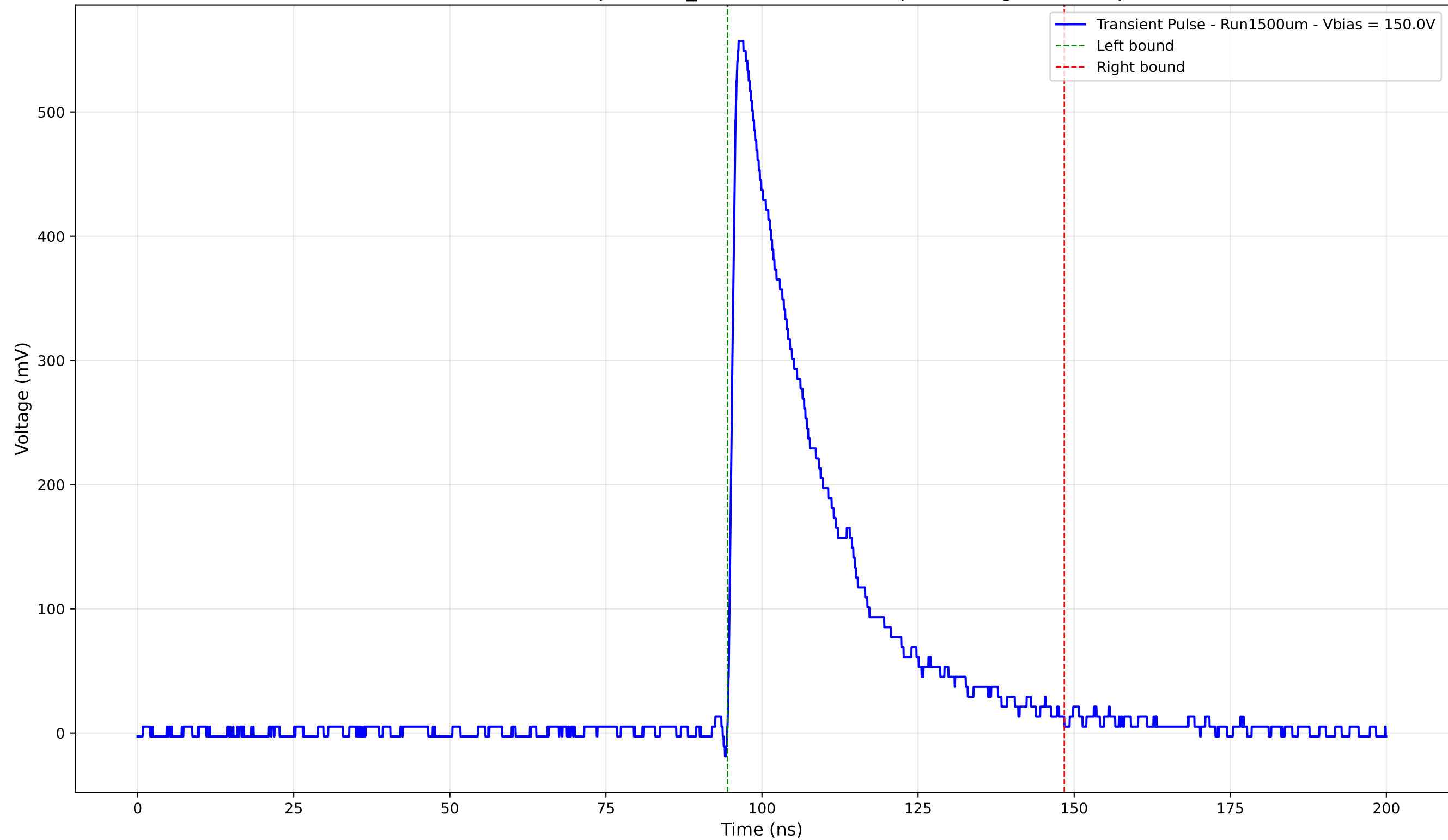
Transient Pulse - Sample: 1cm_42 - Position: 685.0 \mu\text{m} - Charge: 161.16 pC
