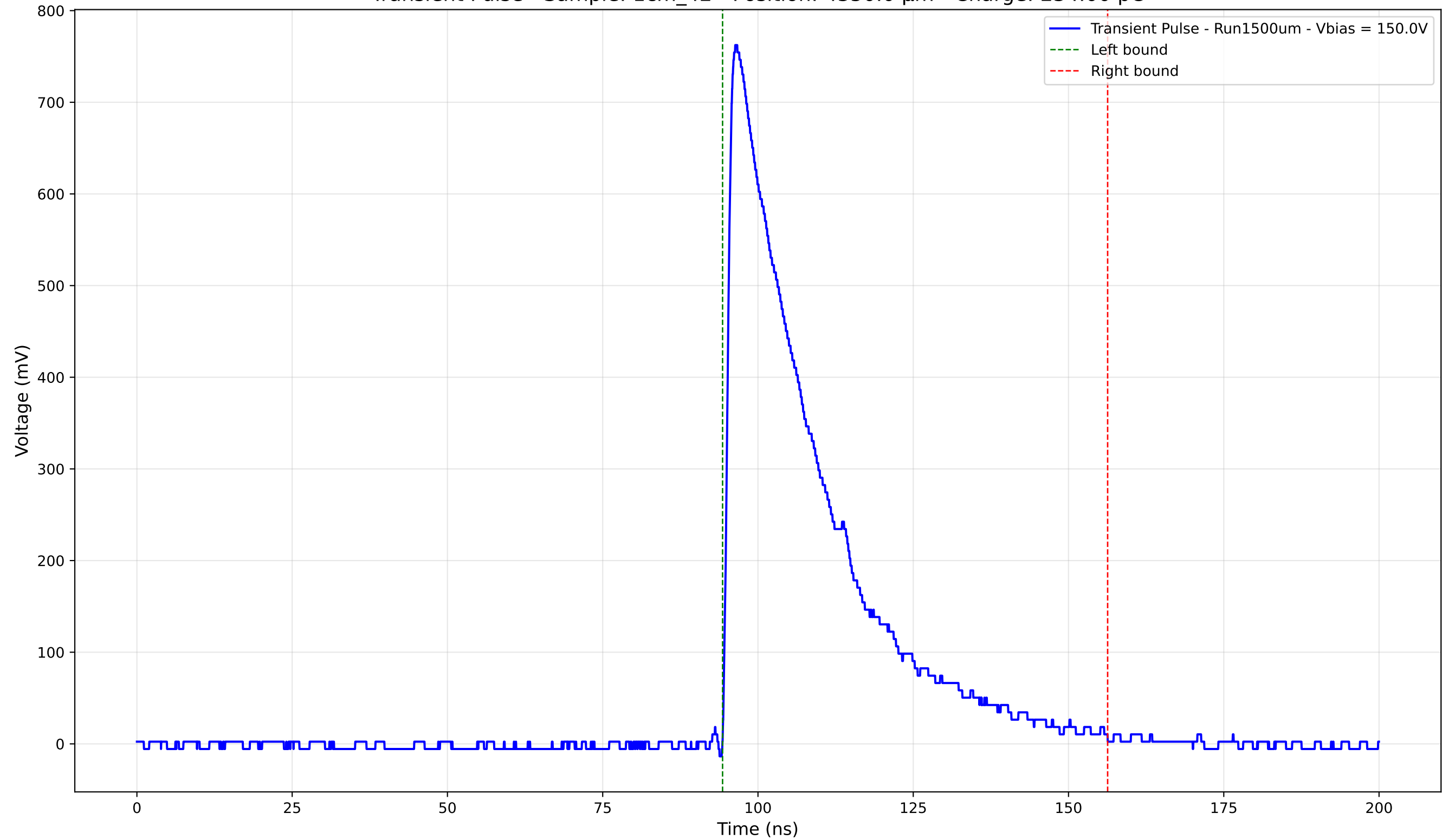
Transient Pulse - Sample: 1cm_42 - Position: 4350.0 \mu\text{m} - Charge: 234.00 pC
