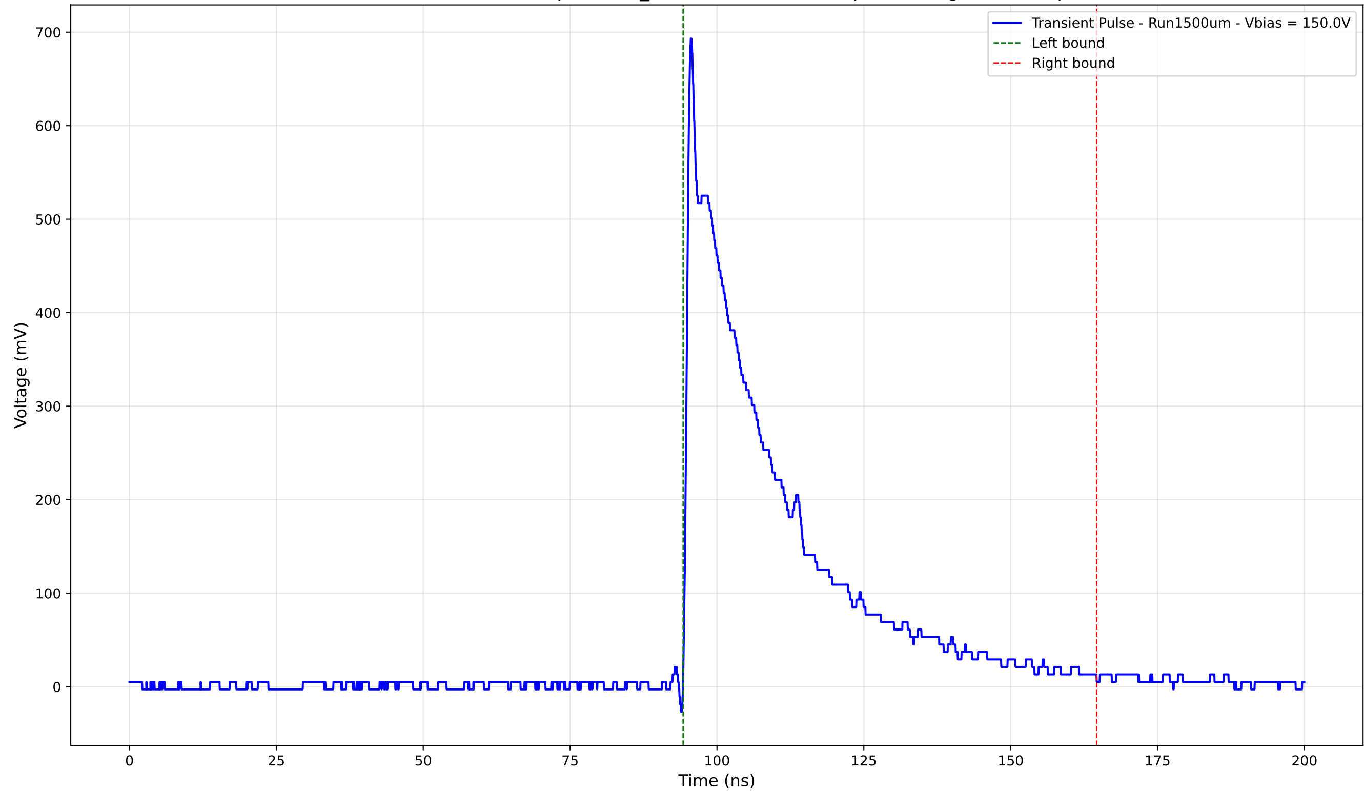
Transient Pulse - Sample: 1cm_42 - Position: 3030.0 \mu\text{m} - Charge: 195.57 pC
