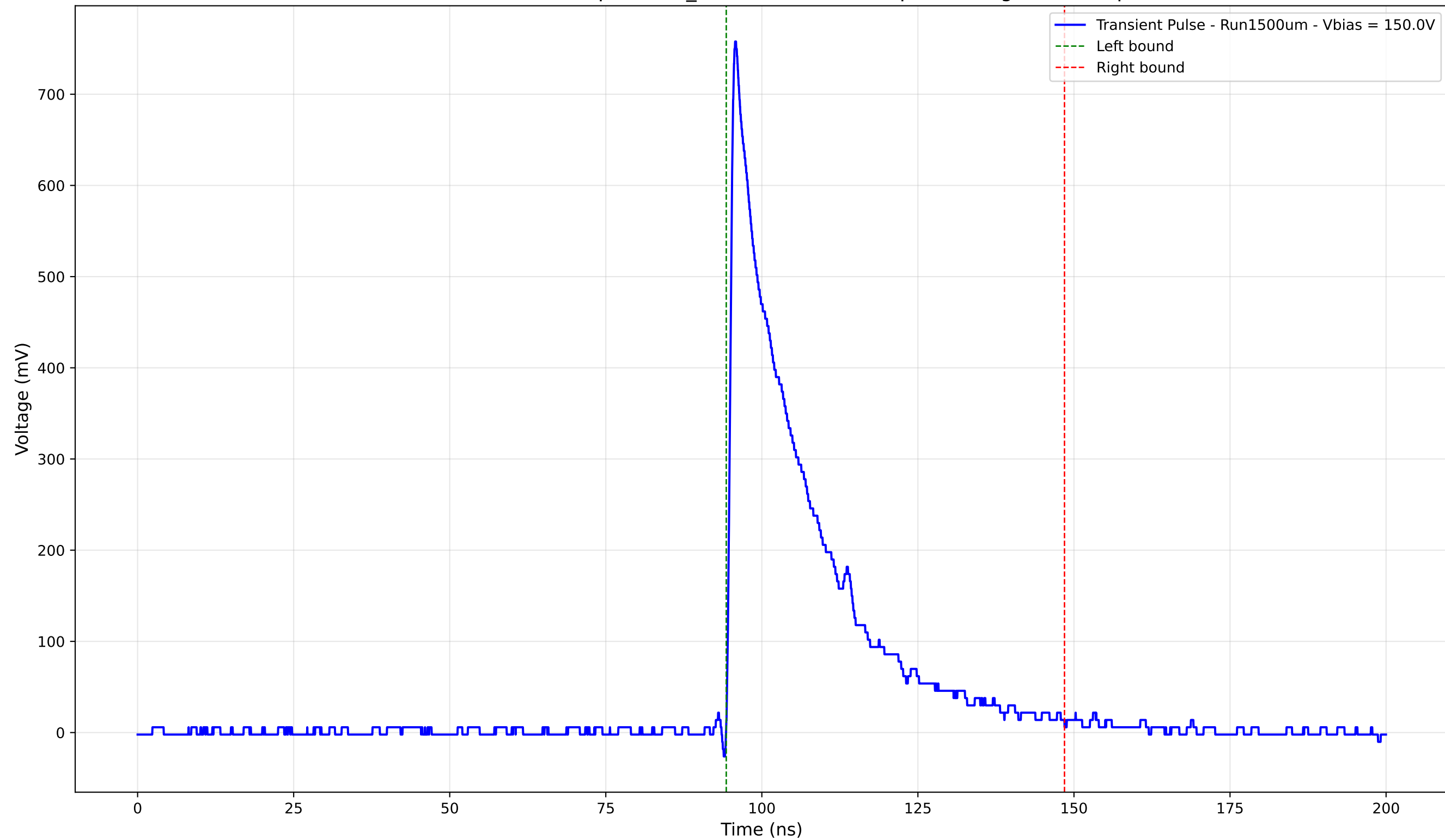
Transient Pulse - Sample: 1cm_42 - Position: 290.0 \mu\text{m} - Charge: 178.41 pC
