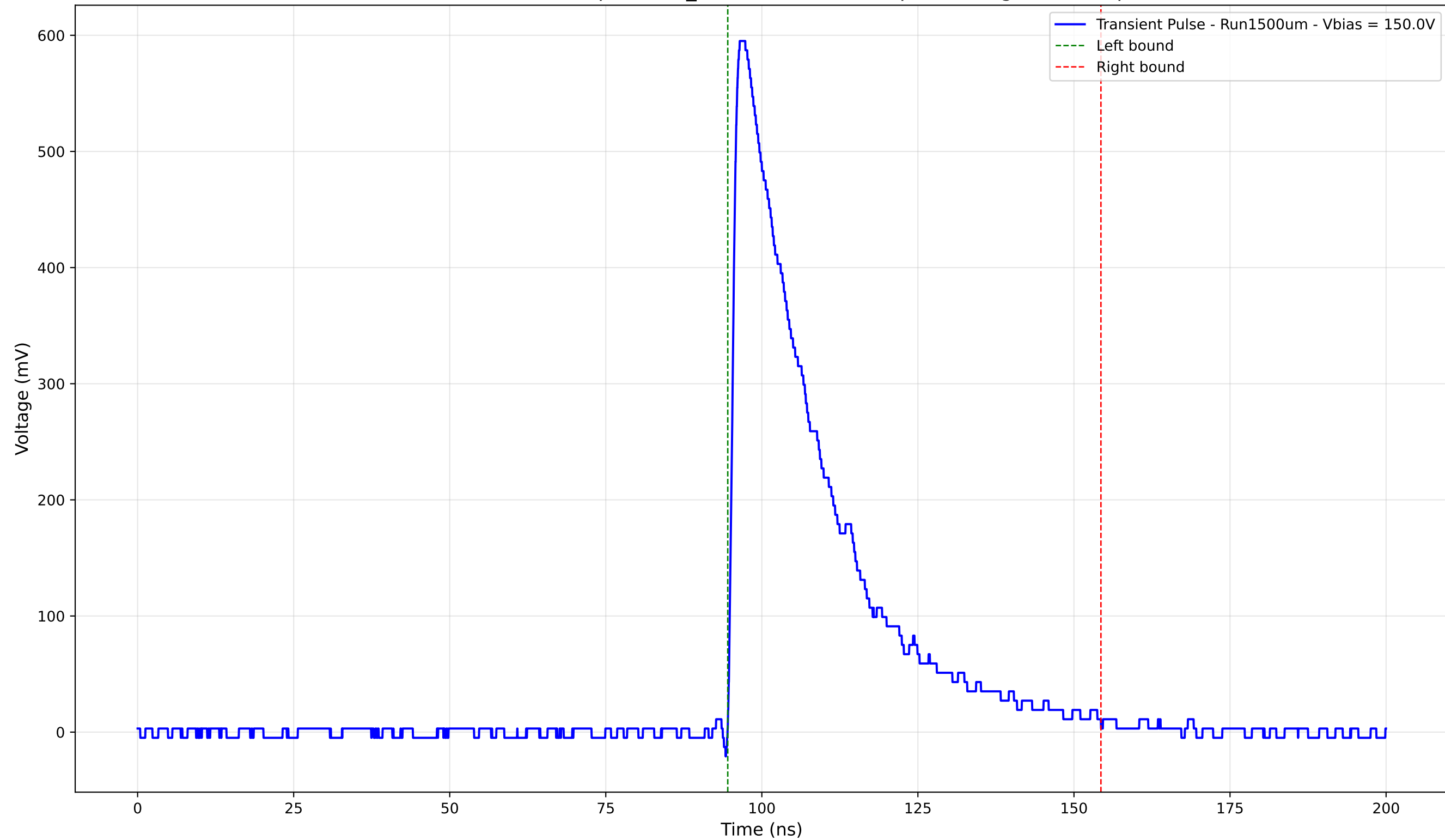
Transient Pulse - Sample: 1cm_42 - Position: 820.0 \mu\text{m} - Charge: 178.56 pC
