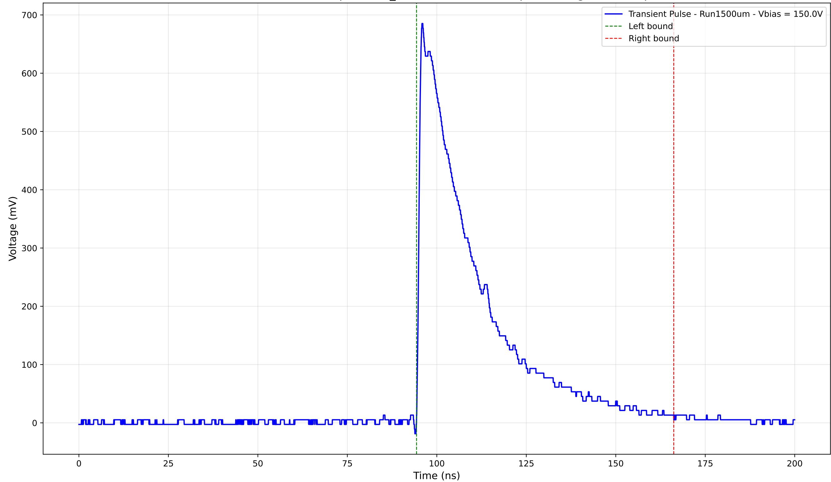
Transient Pulse - Sample: 1cm_42 - Position: 3280.0 \mu\text{m} - Charge: 231.96 pC
