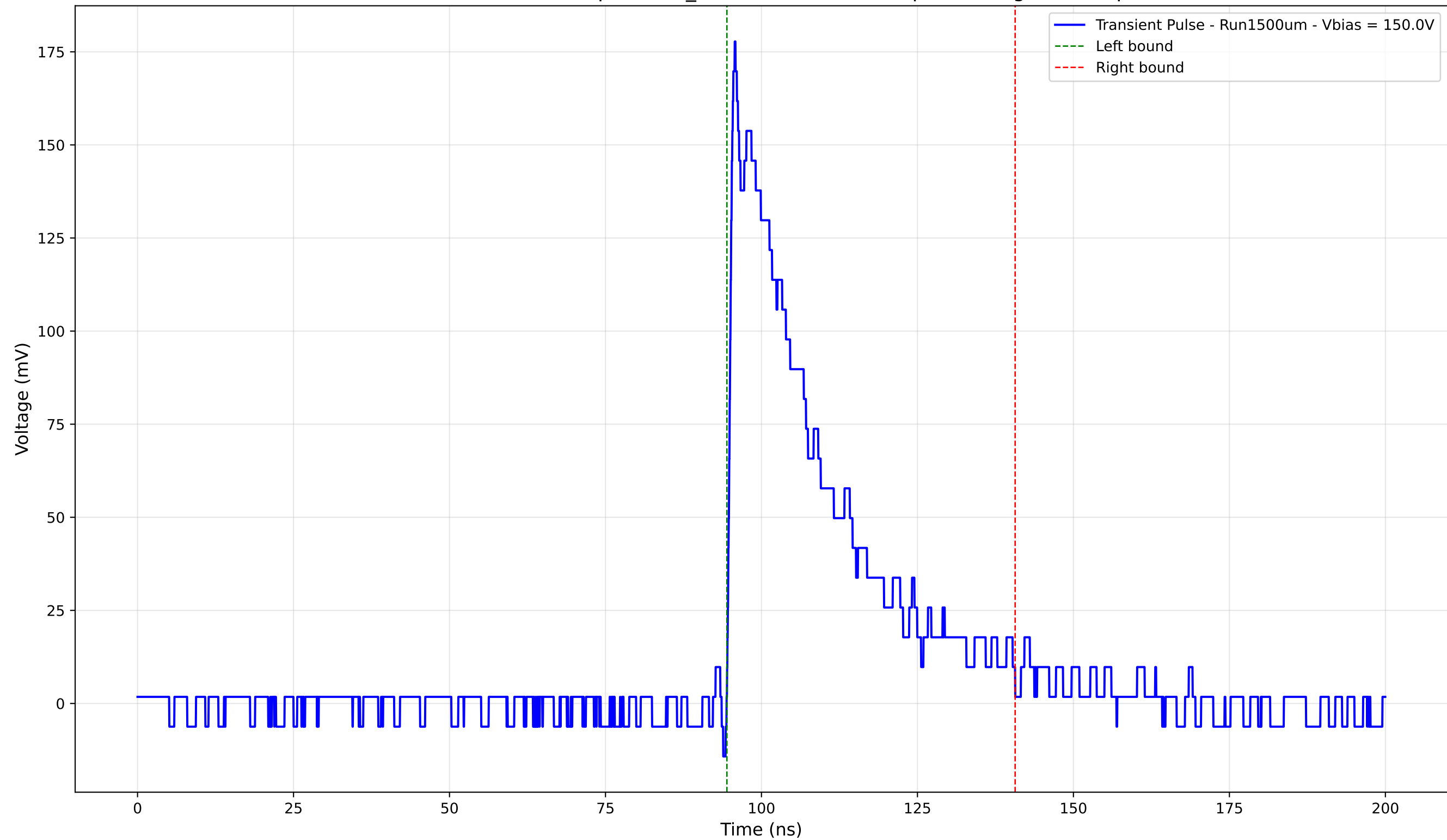
Transient Pulse - Sample: 1cm_42 - Position: 2070.0 \mu\text{m} - Charge: 50.71 pC
