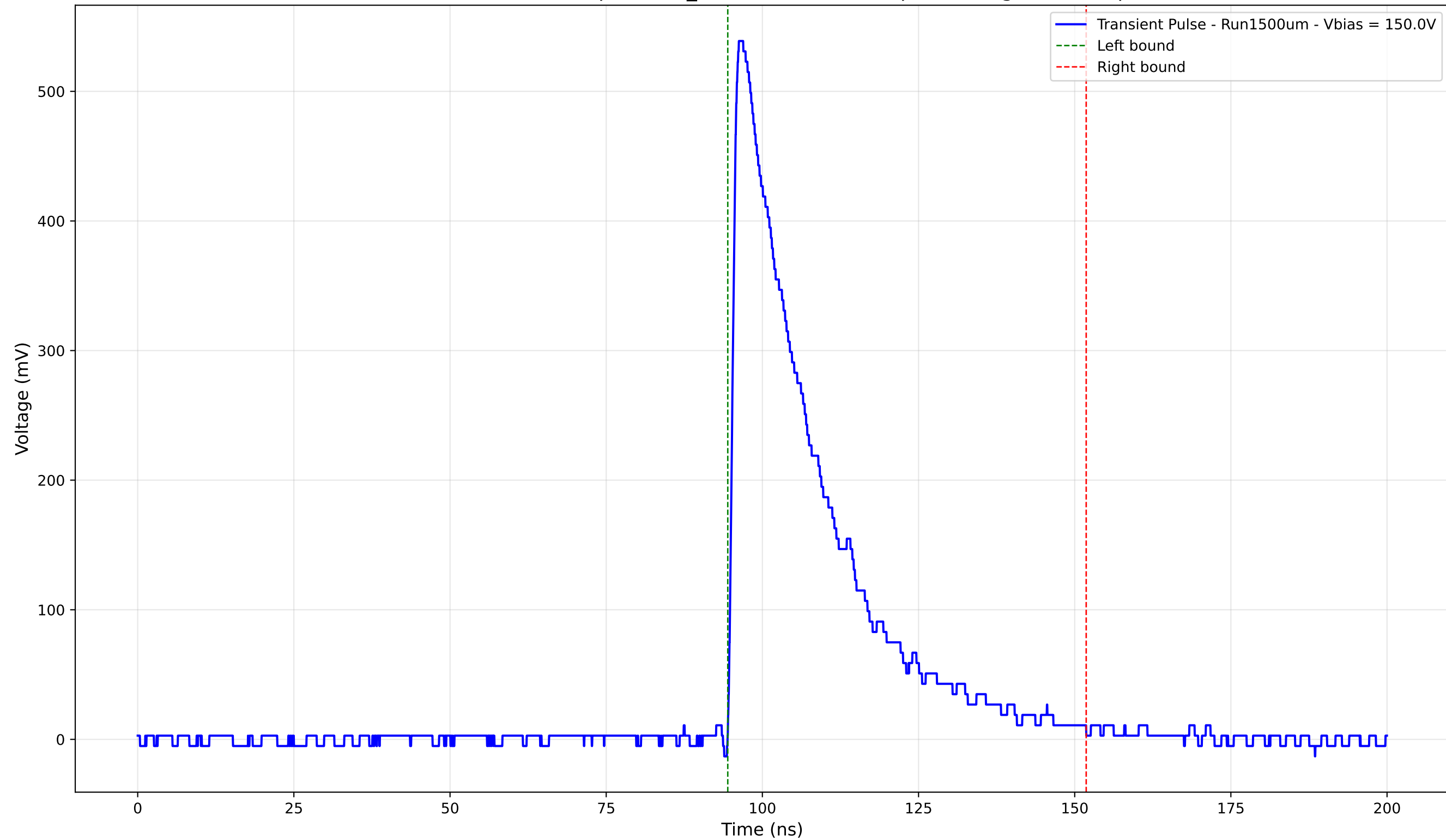
Transient Pulse - Sample: 1cm_42 - Position: 680.0 \mu\text{m} - Charge: 153.78 pC
