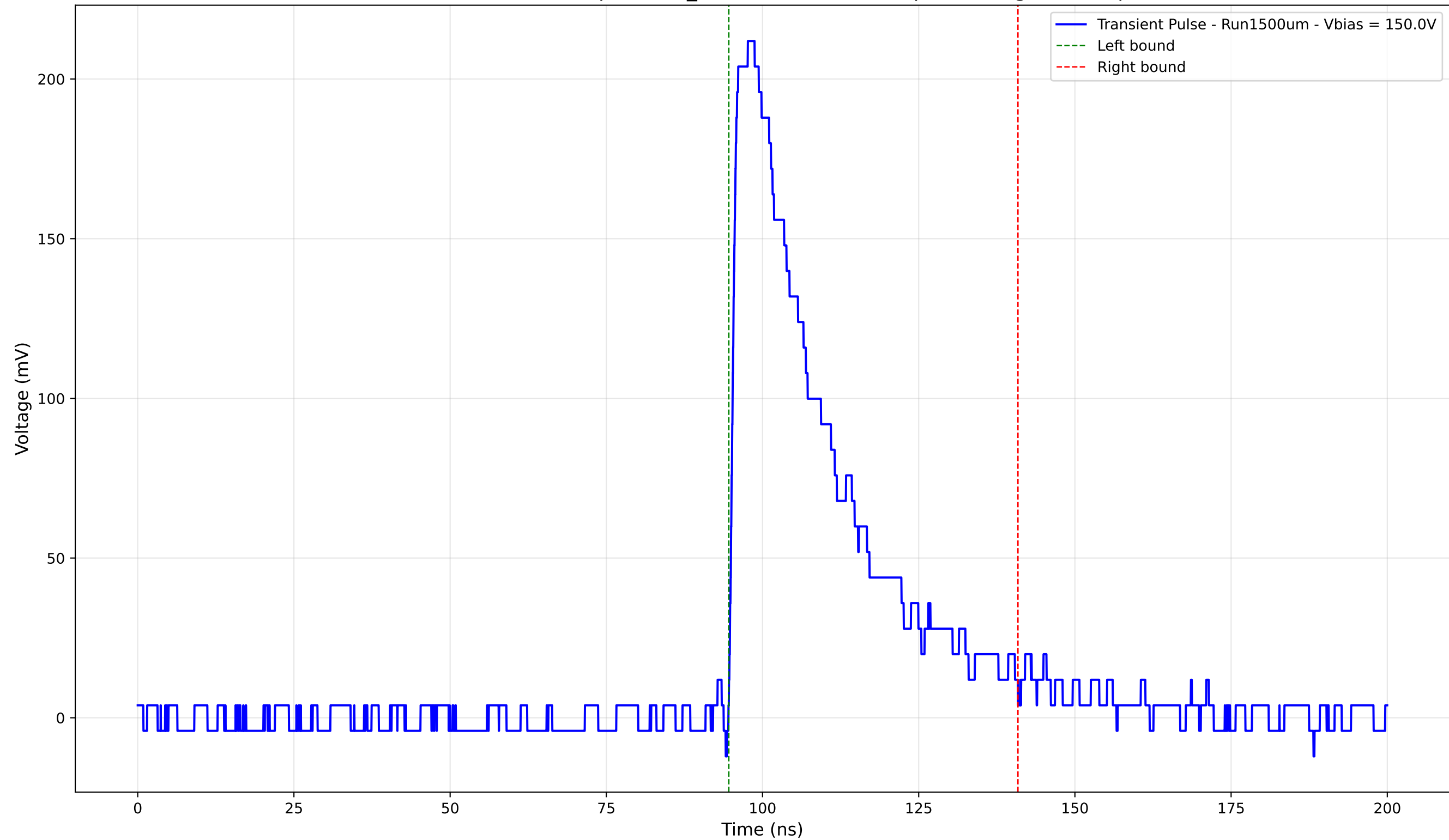
Transient Pulse - Sample: 1cm_42 - Position: 1635.0 \mu\text{m} - Charge: 69.47 pC
