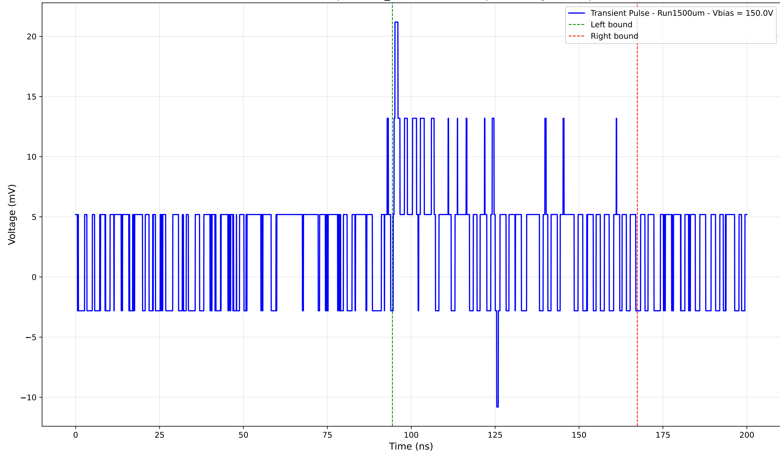
Transient Pulse - Sample: 1cm_42 - Position: 5.0 \mu\text{m} - Charge: 5.53 pC
