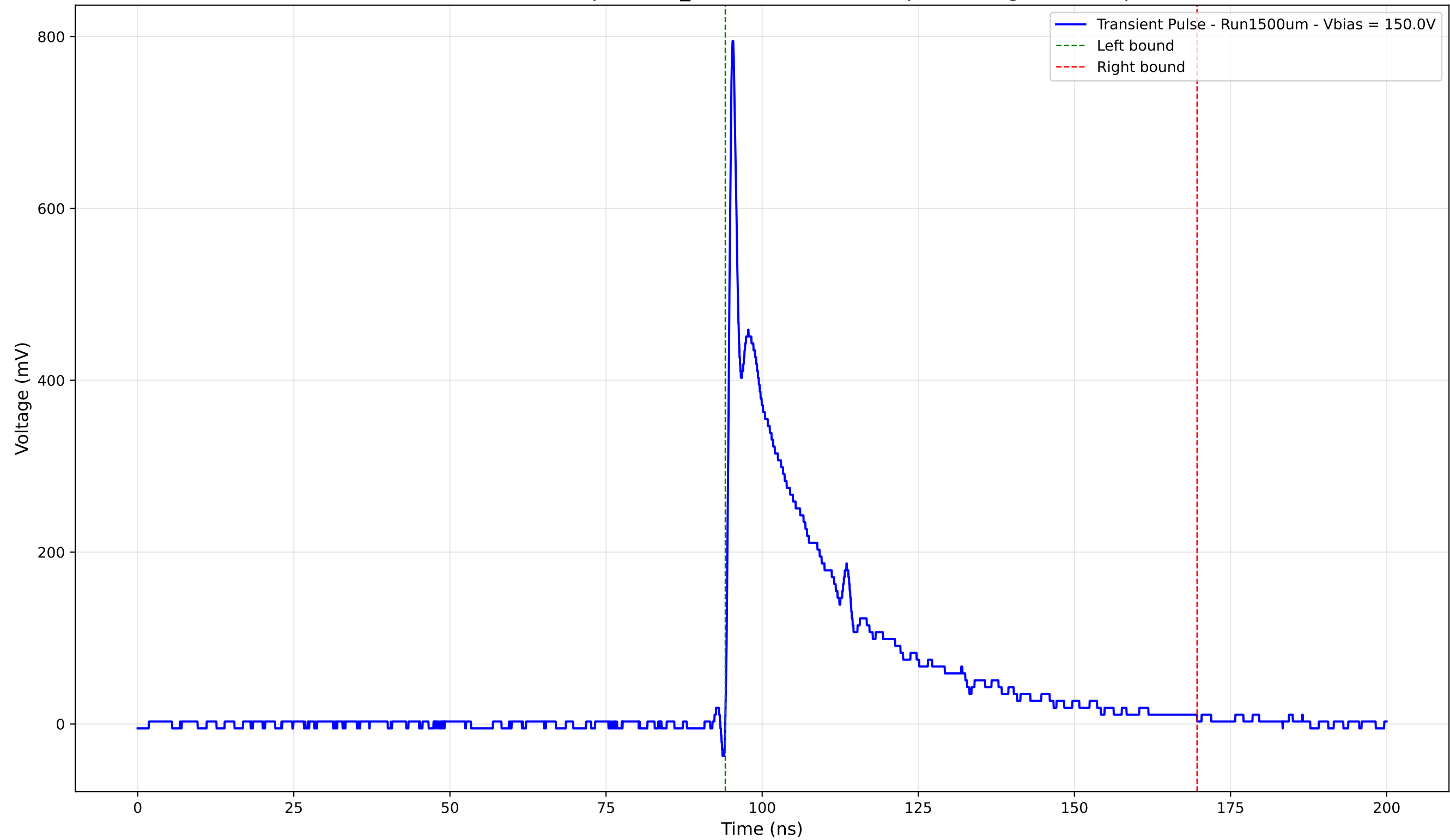
Transient Pulse - Sample: 1cm_42 - Position: 2690.0 \mu\text{m} - Charge: 171.16 pC
