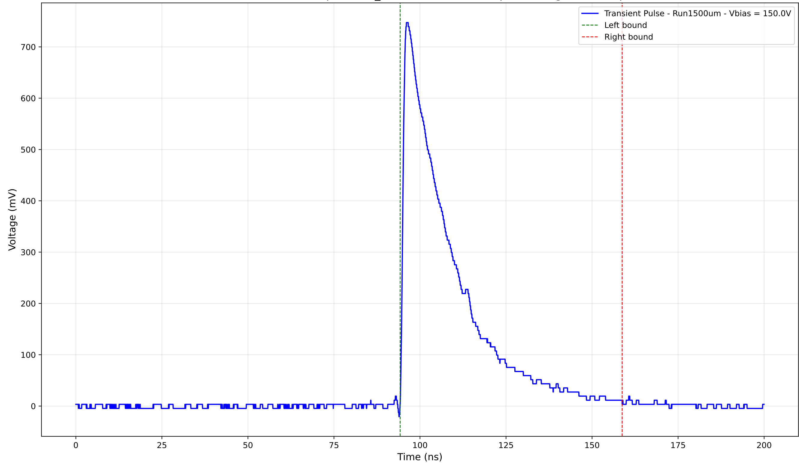
Transient Pulse - Sample: 1cm_42 - Position: 4465.0 \mu\text{m} - Charge: 224.86 pC
