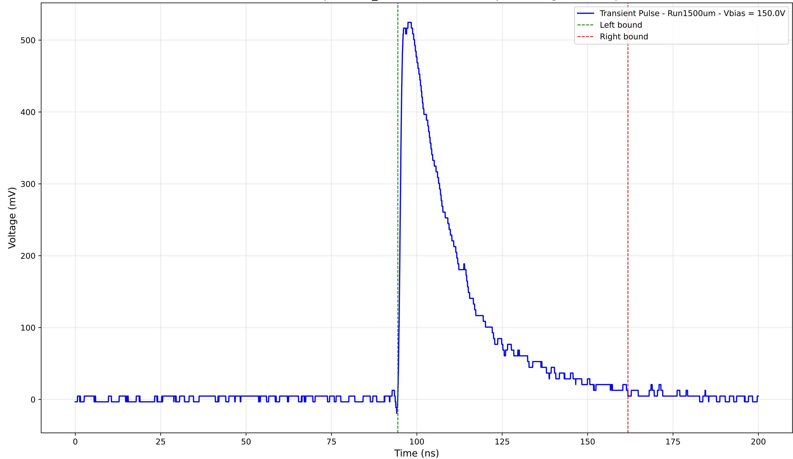
Transient Pulse - Sample: 1cm_42 - Position: 1750.0 \mu\text{m} - Charge: 184.95 pC
