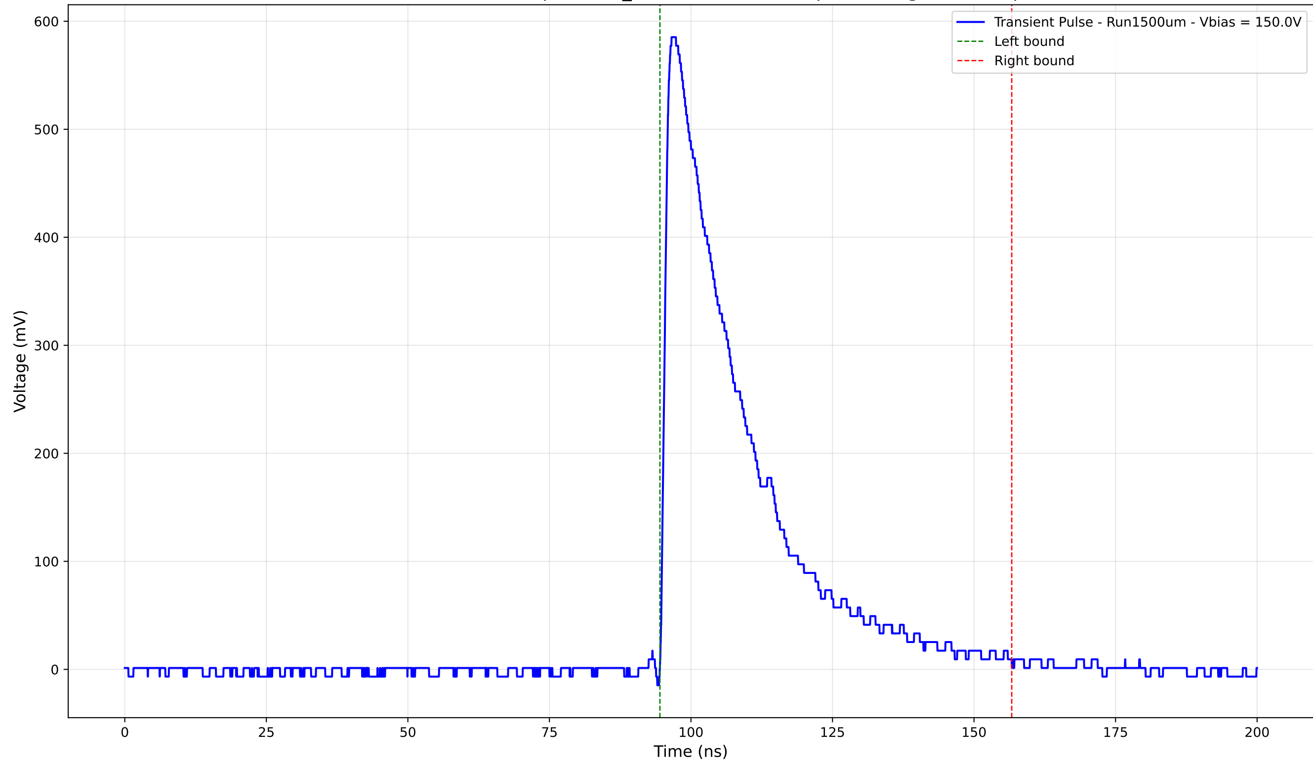
Transient Pulse - Sample: 1cm_42 - Position: 870.0 \mu\text{m} - Charge: 176.68 pC
