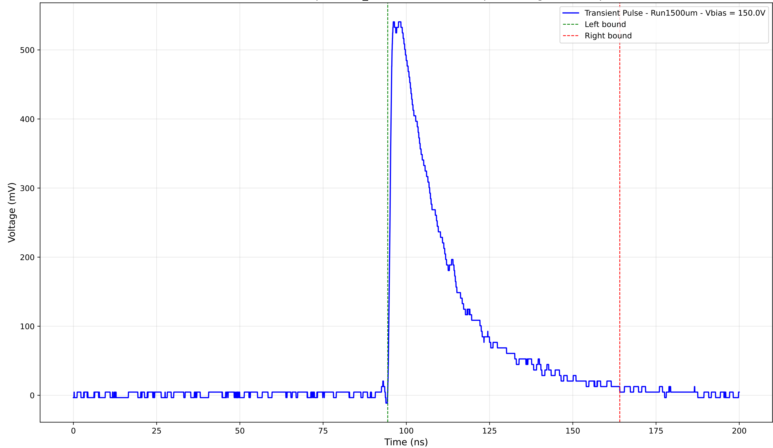
Transient Pulse - Sample: 1cm_42 - Position: 1785.0 \mu\text{m} - Charge: 192.10 pC
