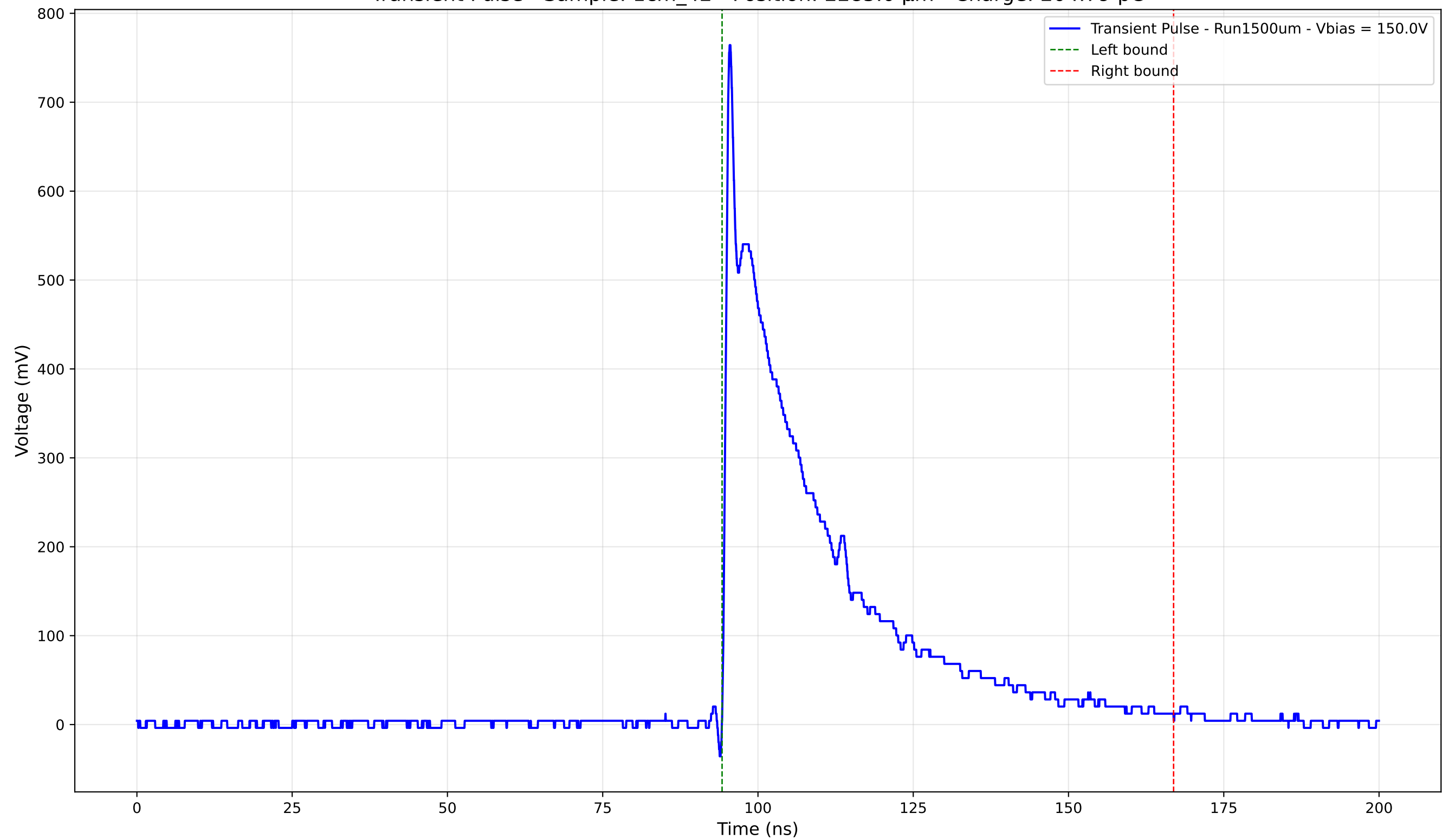
Transient Pulse - Sample: 1cm_42 - Position: 2285.0 \mu\text{m} - Charge: 204.79 pC
