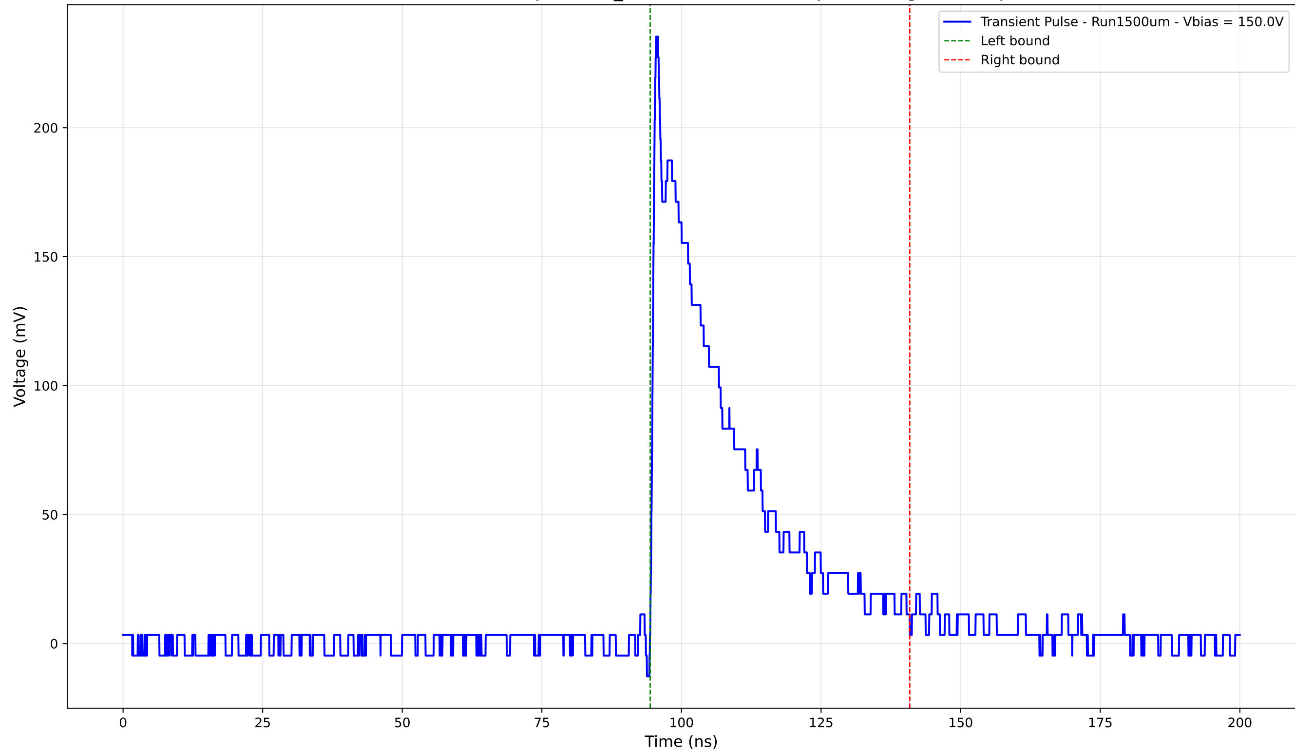
Transient Pulse - Sample: 1cm_42 - Position: 2135.0 \mu\text{m} - Charge: 62.69 pC
