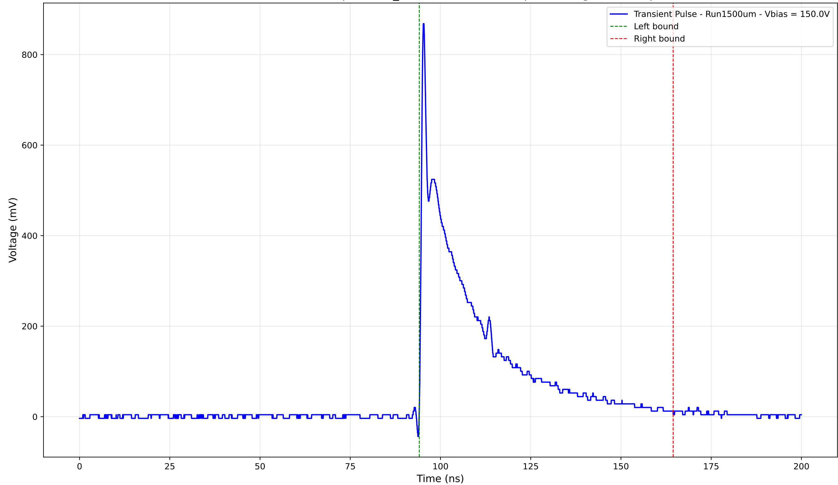
Transient Pulse - Sample: 1cm_42 - Position: 2495.0 \mu\text{m} - Charge: 200.67 pC
