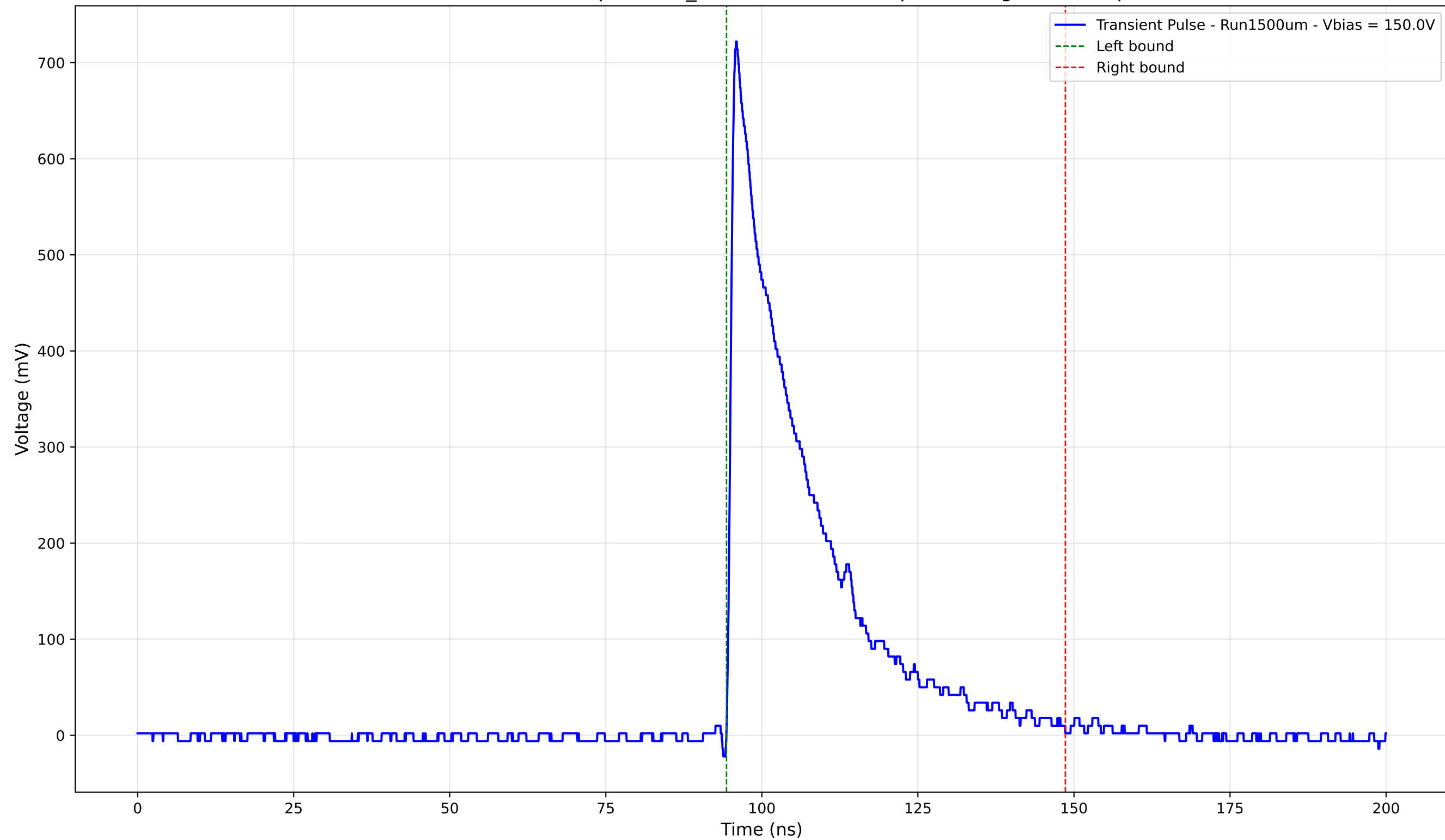
Transient Pulse - Sample: 1cm_42 - Position: 385.0 \mu\text{m} - Charge: 177.63 pC
