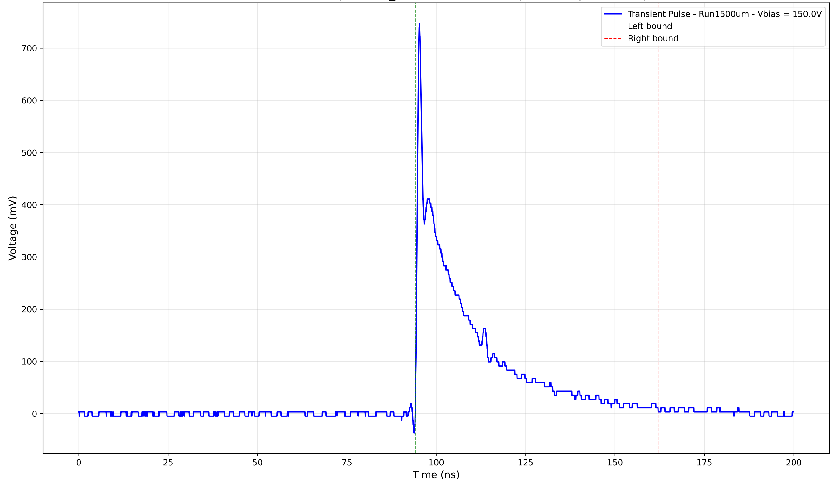
Transient Pulse - Sample: 1cm_42 - Position: 2680.0 \mu\text{m} - Charge: 154.04 pC
