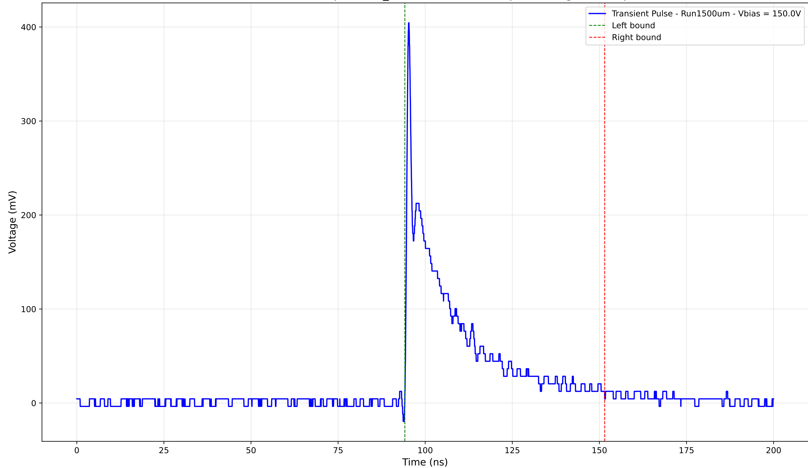
Transient Pulse - Sample: 1cm_42 - Position: 2645.0 \mu\text{m} - Charge: 77.64 pC
