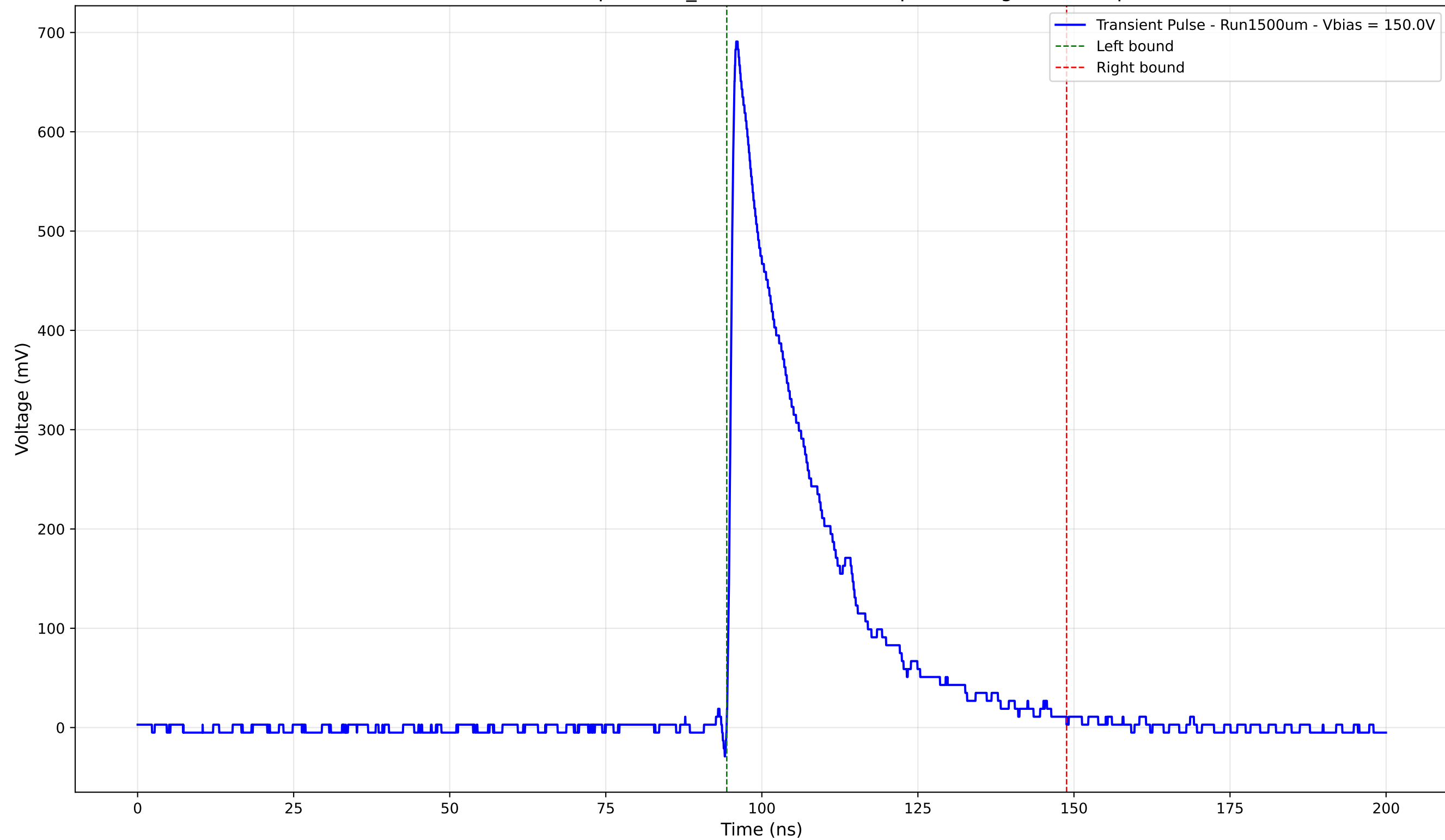
Transient Pulse - Sample: 1cm_42 - Position: 435.0 \mu\text{m} - Charge: 174.49 pC
