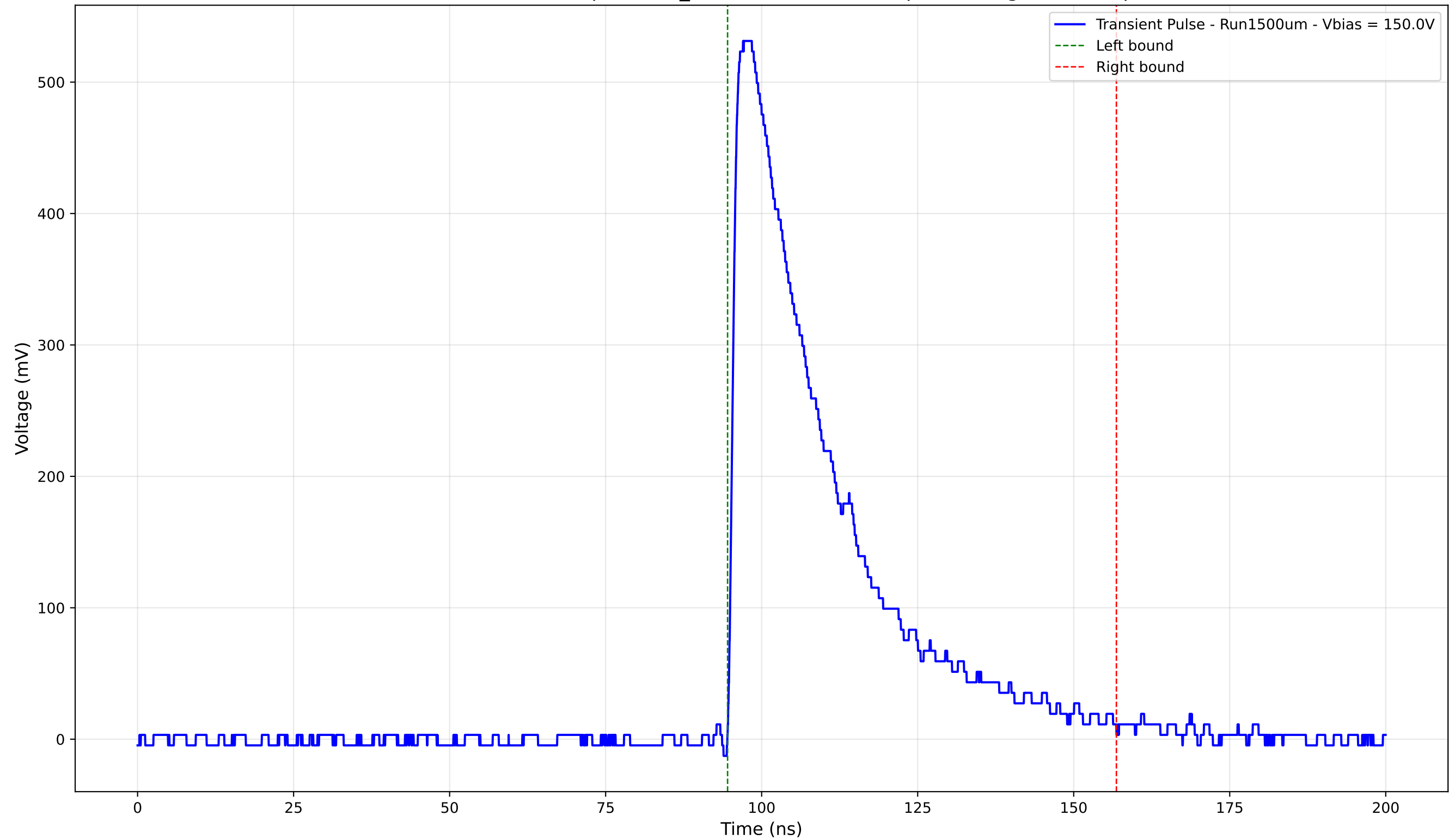
Transient Pulse - Sample: 1cm_42 - Position: 1480.0 \mu\text{m} - Charge: 179.30 pC
