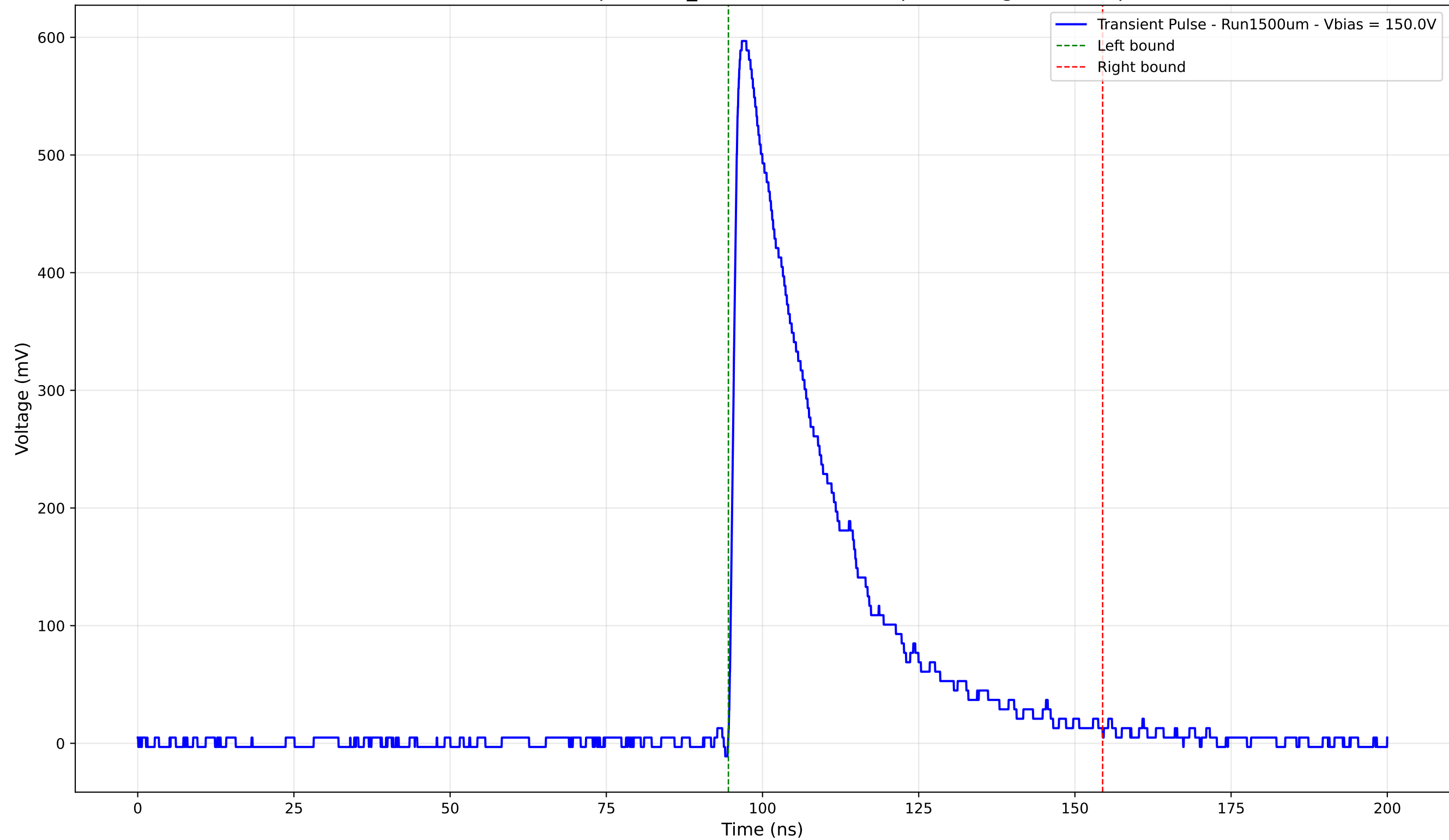
Transient Pulse - Sample: 1cm_42 - Position: 915.0 \mu\text{m} - Charge: 183.05 pC
