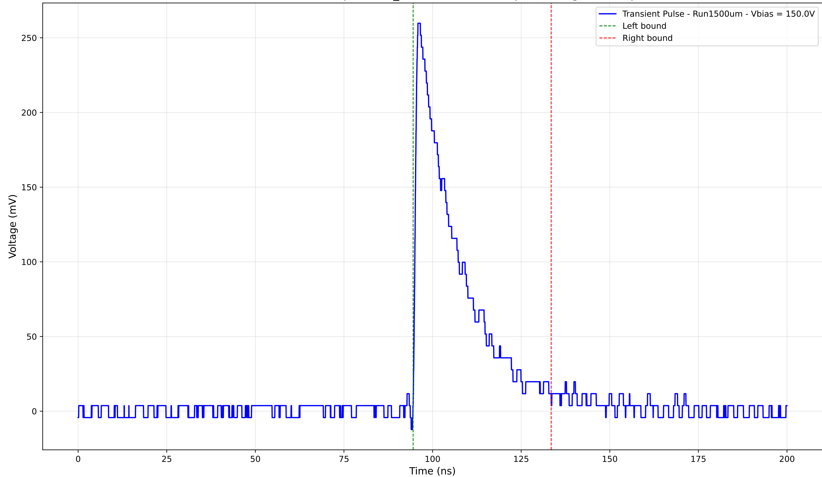
Transient Pulse - Sample: 1cm_42 -Position: 545.0 \mu\text{m} - Charge: 65.37 pC
