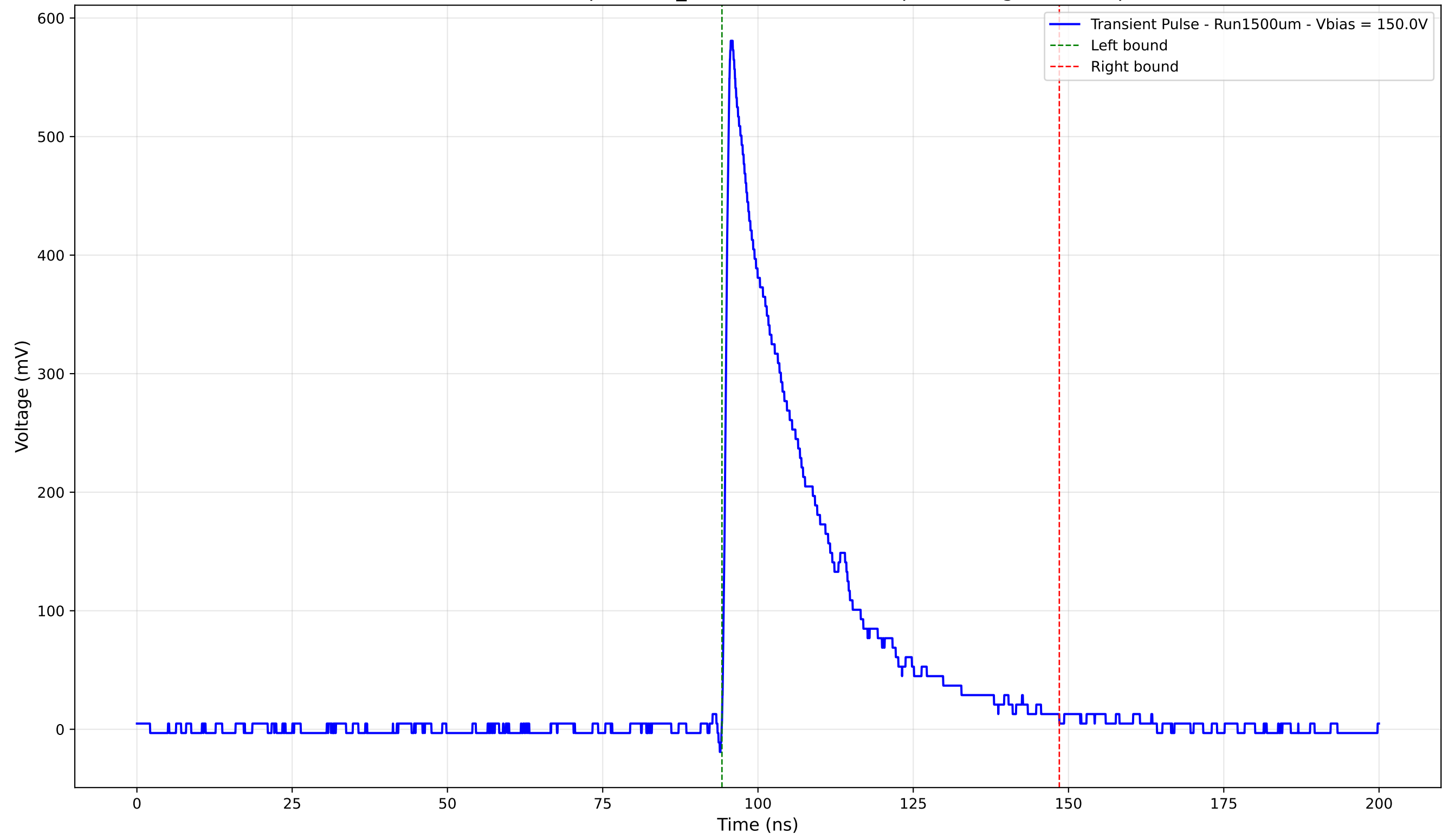
Transient Pulse - Sample: 1cm_42 - Position: 4705.0 \mu\text{m} - Charge: 148.64 pC
