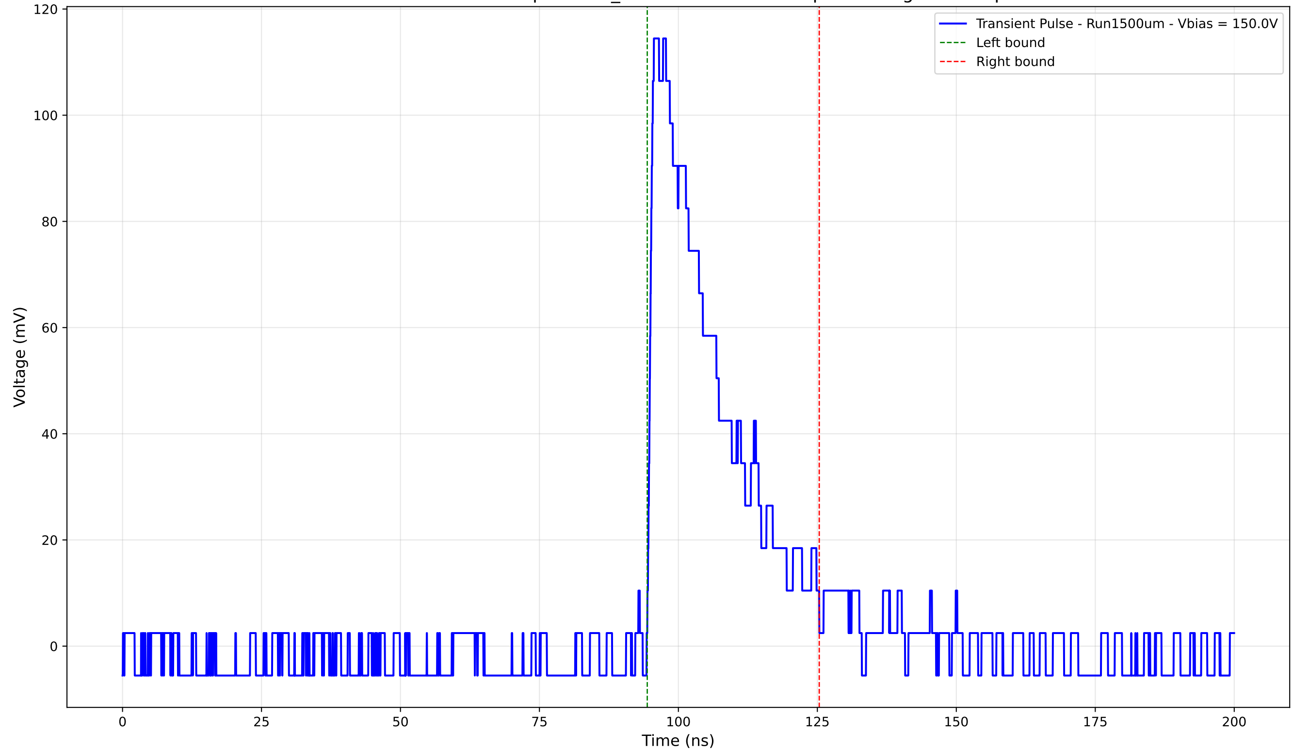
Transient Pulse - Sample: 1cm_42 - Position: 4625.0 \mu\text{m} - Charge: 29.97 pC
