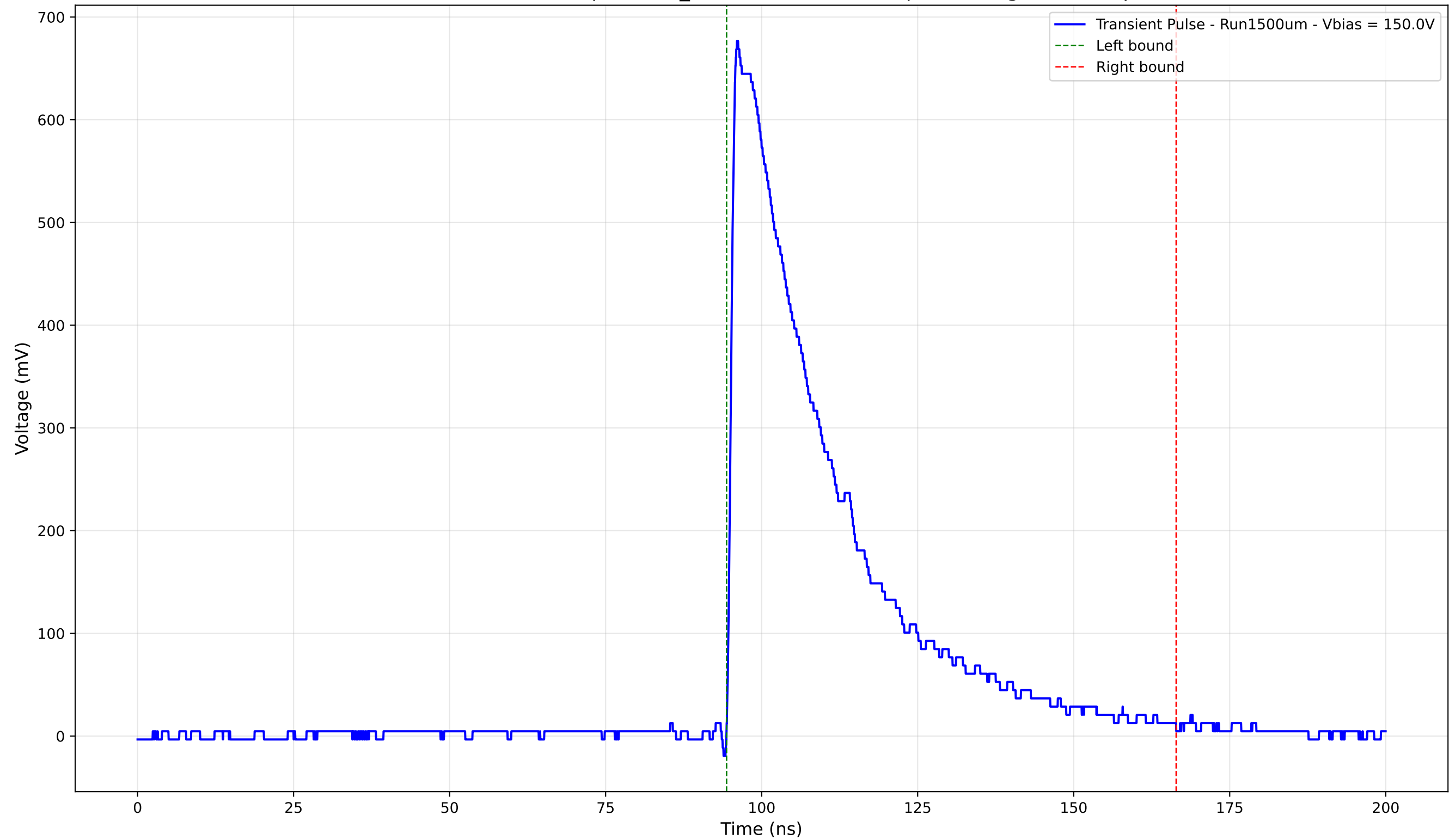
Transient Pulse - Sample: 1cm_42 - Position: 3375.0 \mu\text{m} - Charge: 232.36 pC
