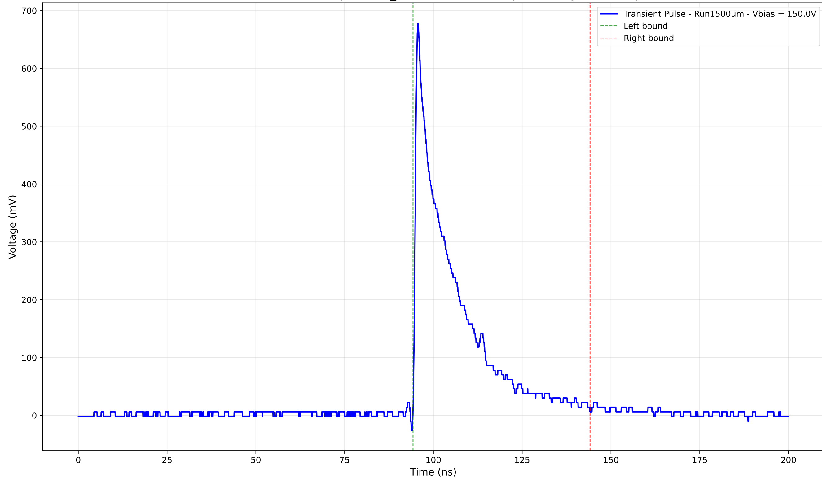
Transient Pulse - Sample: 1cm_42 - Position: 180.0 \mu\text{m} - Charge: 143.18 pC
