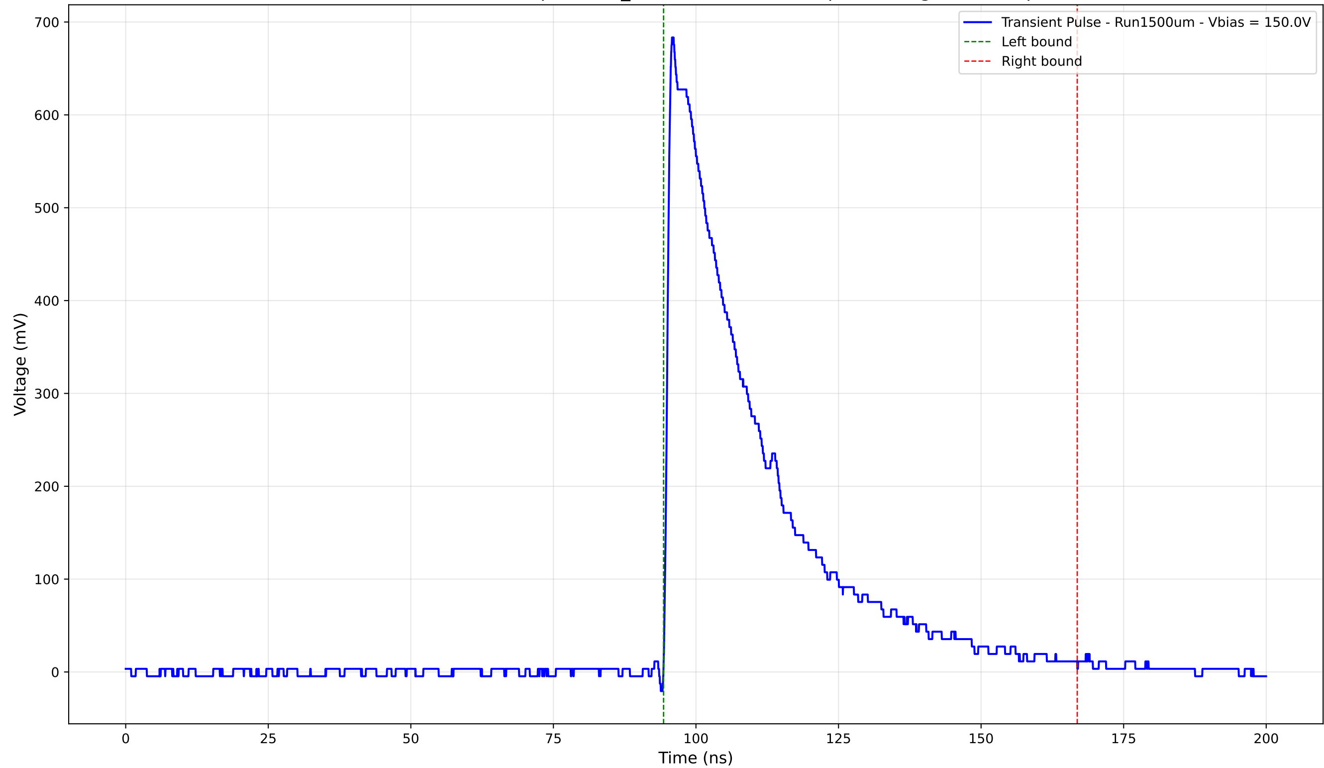
Transient Pulse - Sample: 1cm_42 - Position: 3255.0 \mu\text{m} - Charge: 228.58 pC
