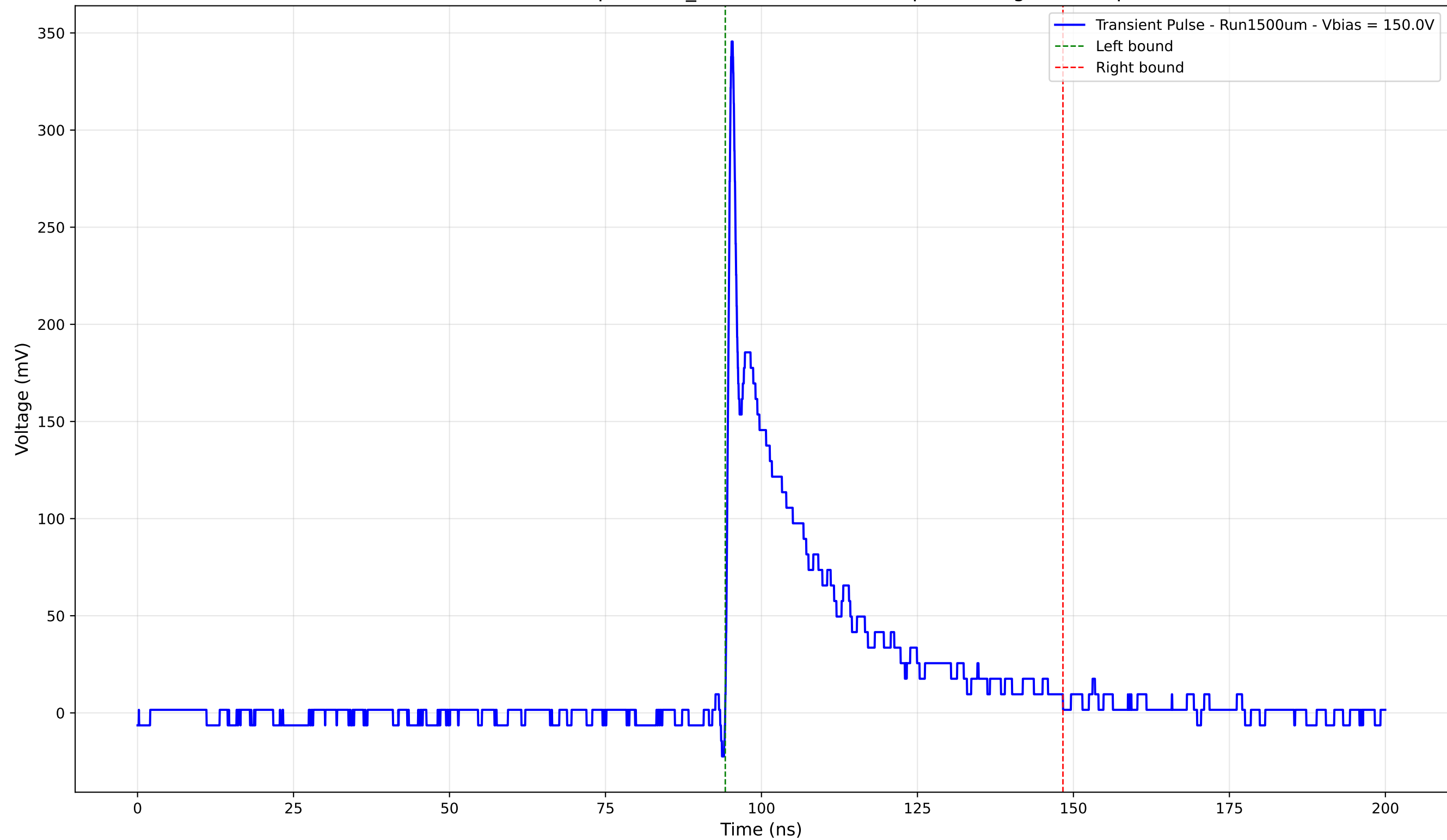
Transient Pulse - Sample: 1cm_42 - Position: 2640.0 \mu\text{m} - Charge: 63.93 pC
