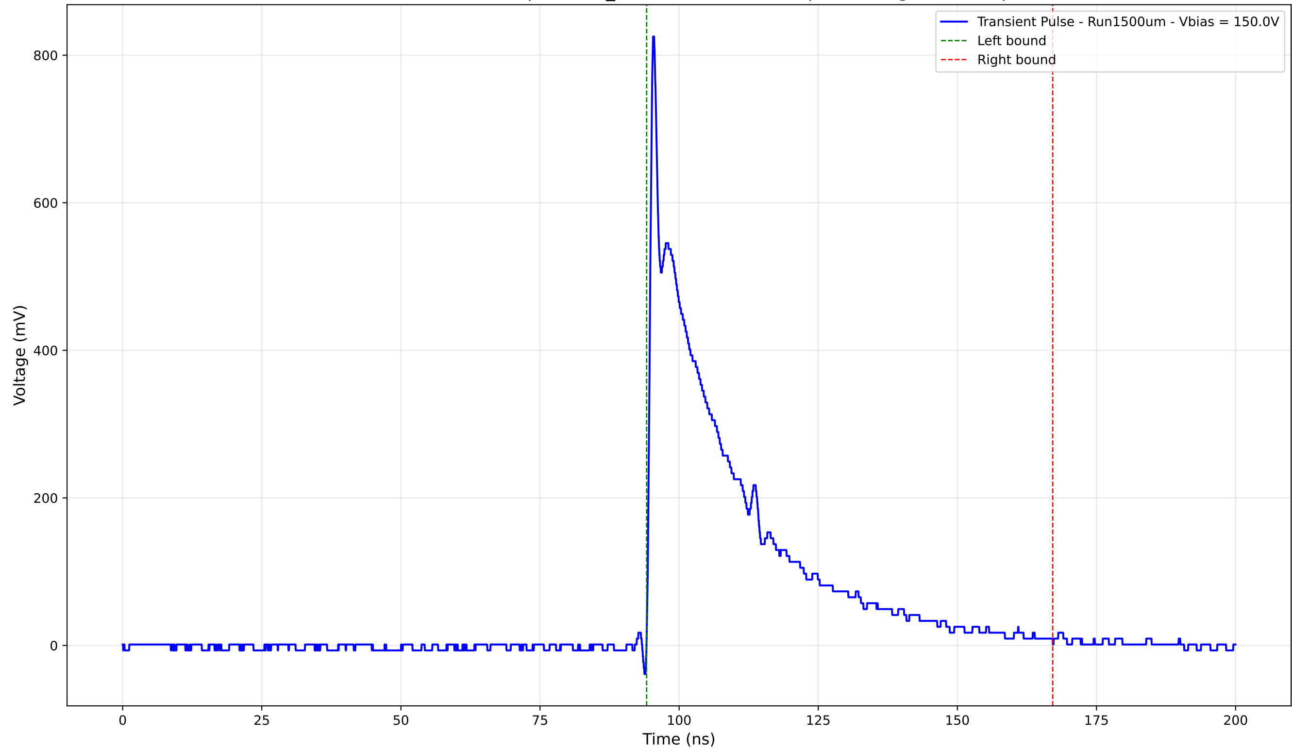
Transient Pulse - Sample: 1cm_42 - Position: 2380.0 \mu\text{m} - Charge: 203.35 pC
