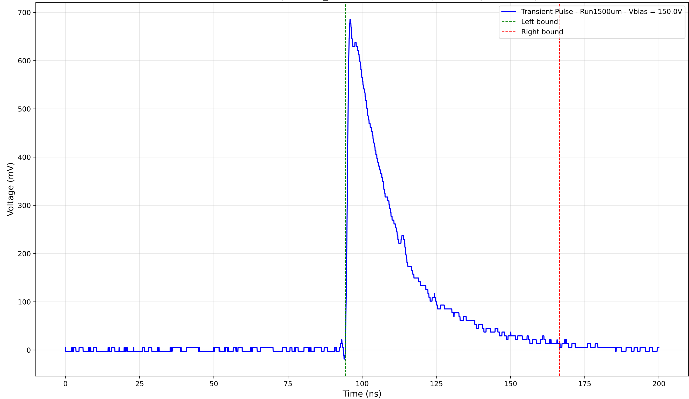
Transient Pulse - Sample: 1cm_42 - Position: 3285.0 \mu\text{m} - Charge: 231.57 pC
