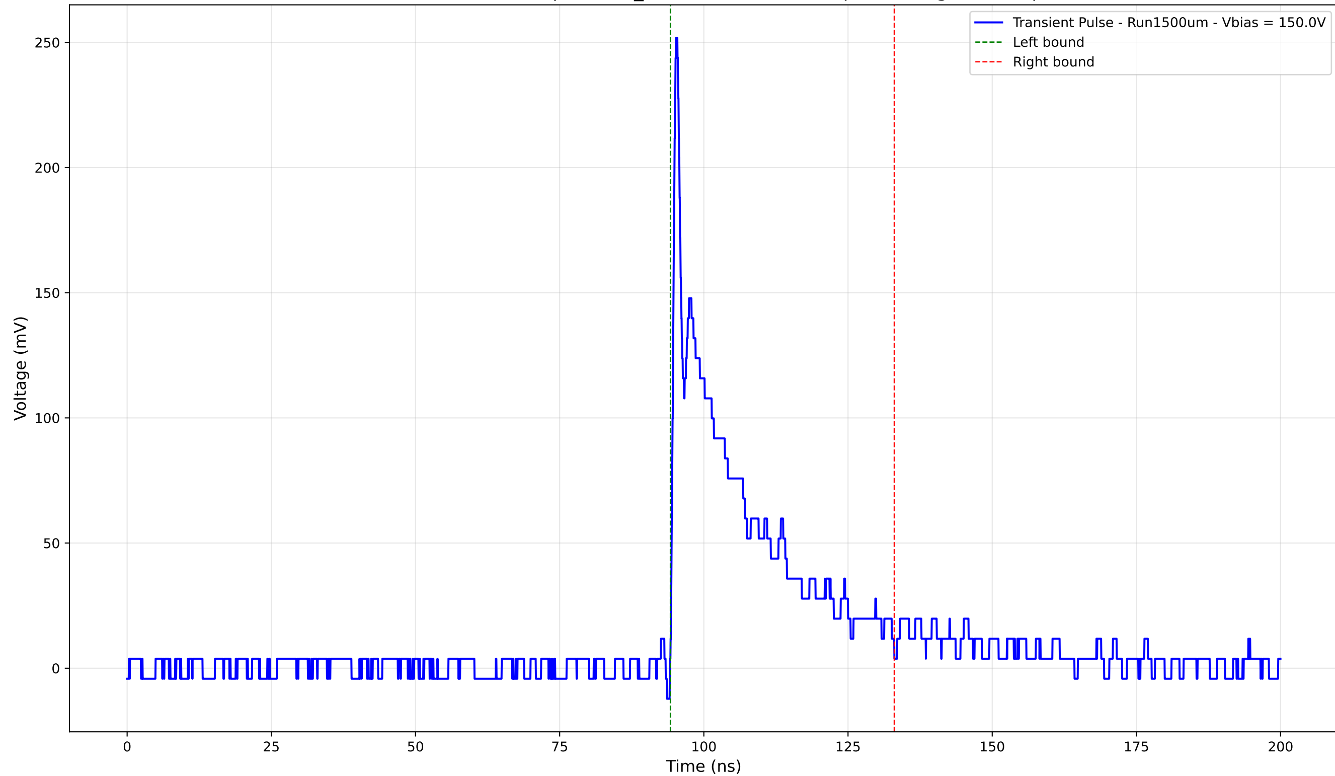
Transient Pulse - Sample: 1cm_42 - Position: 2630.0 \mu\text{m} - Charge: 46.00 pC
