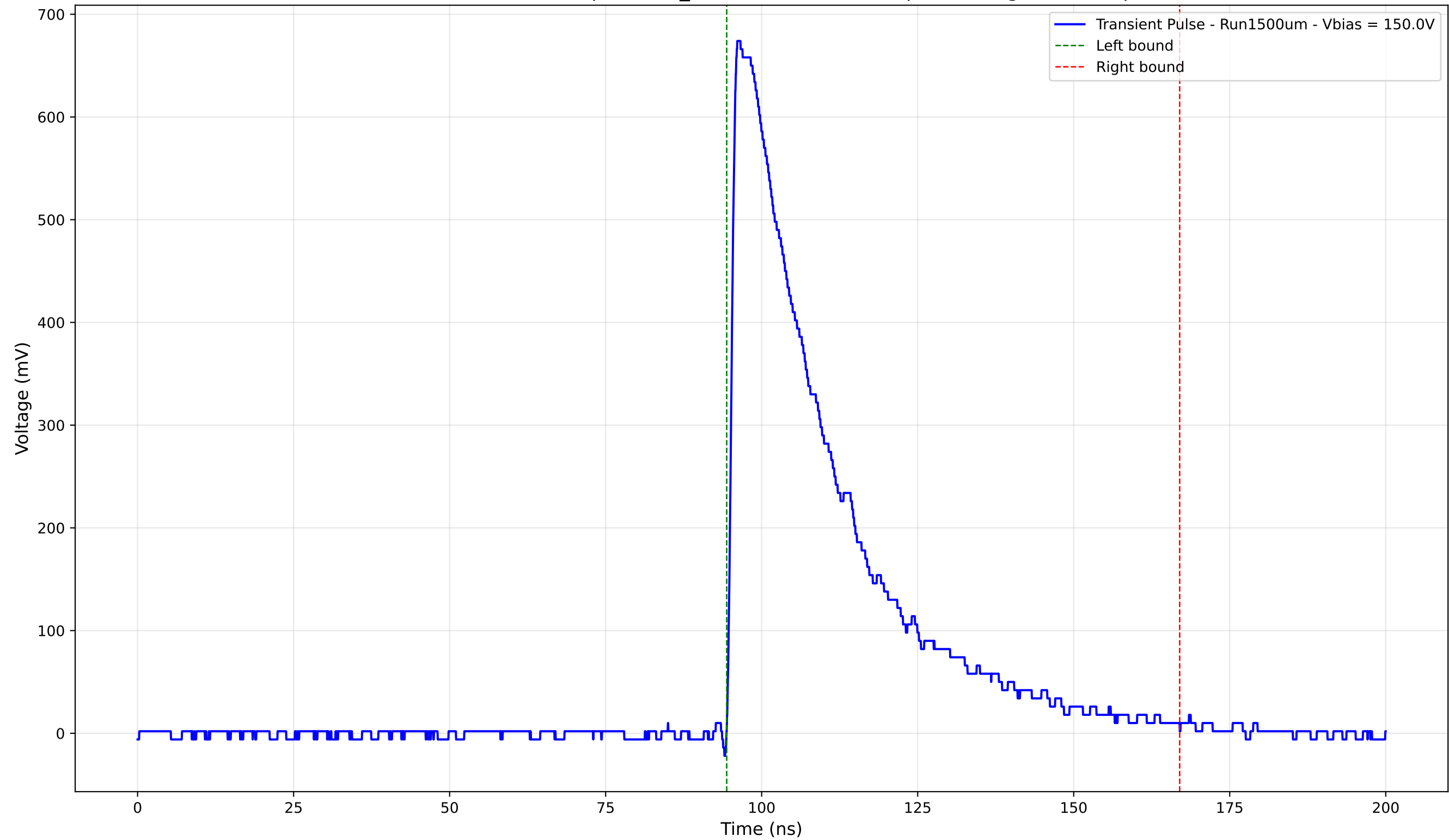
Transient Pulse - Sample: 1cm_42 - Position: 3470.0 \mu\text{m} - Charge: 233.03 pC
