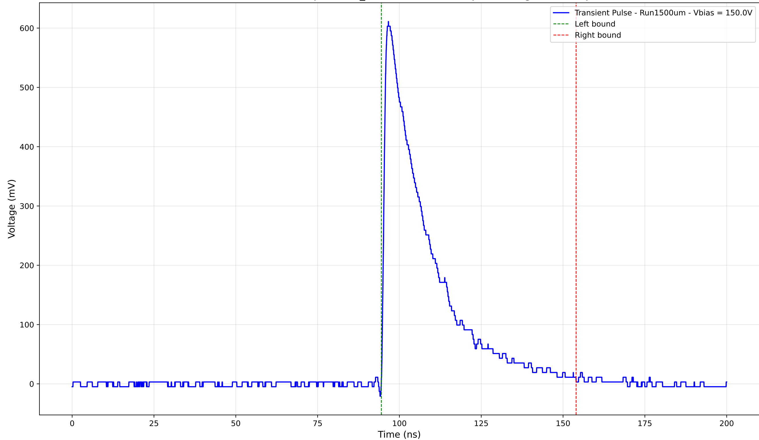
Transient Pulse - Sample: 1cm_42 - Position: 735.0 \mu\text{m} - Charge: 177.55 pC
