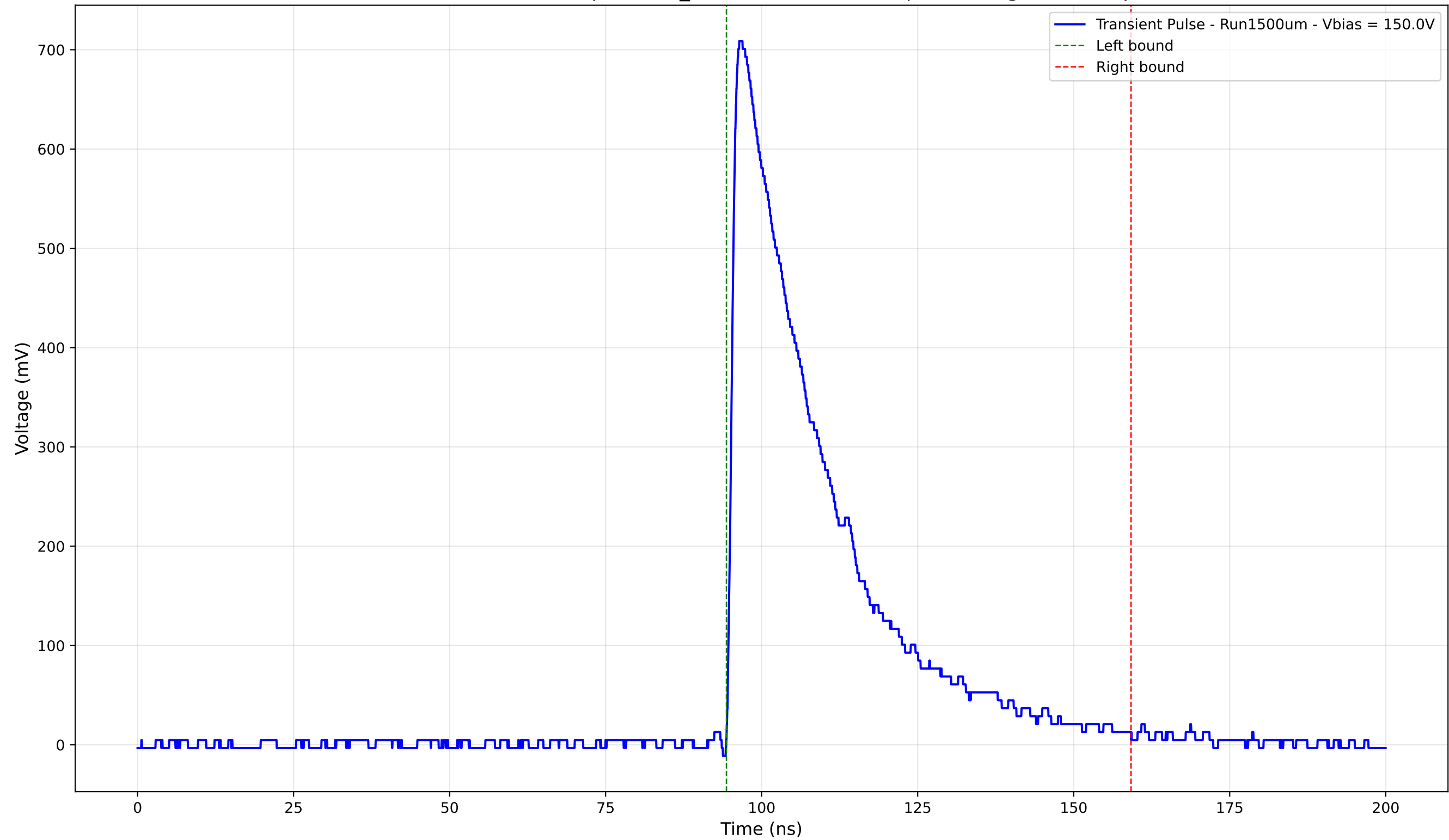
Transient Pulse - Sample: 1cm_42 - Position: 4235.0 \mu\text{m} - Charge: 224.46 pC
