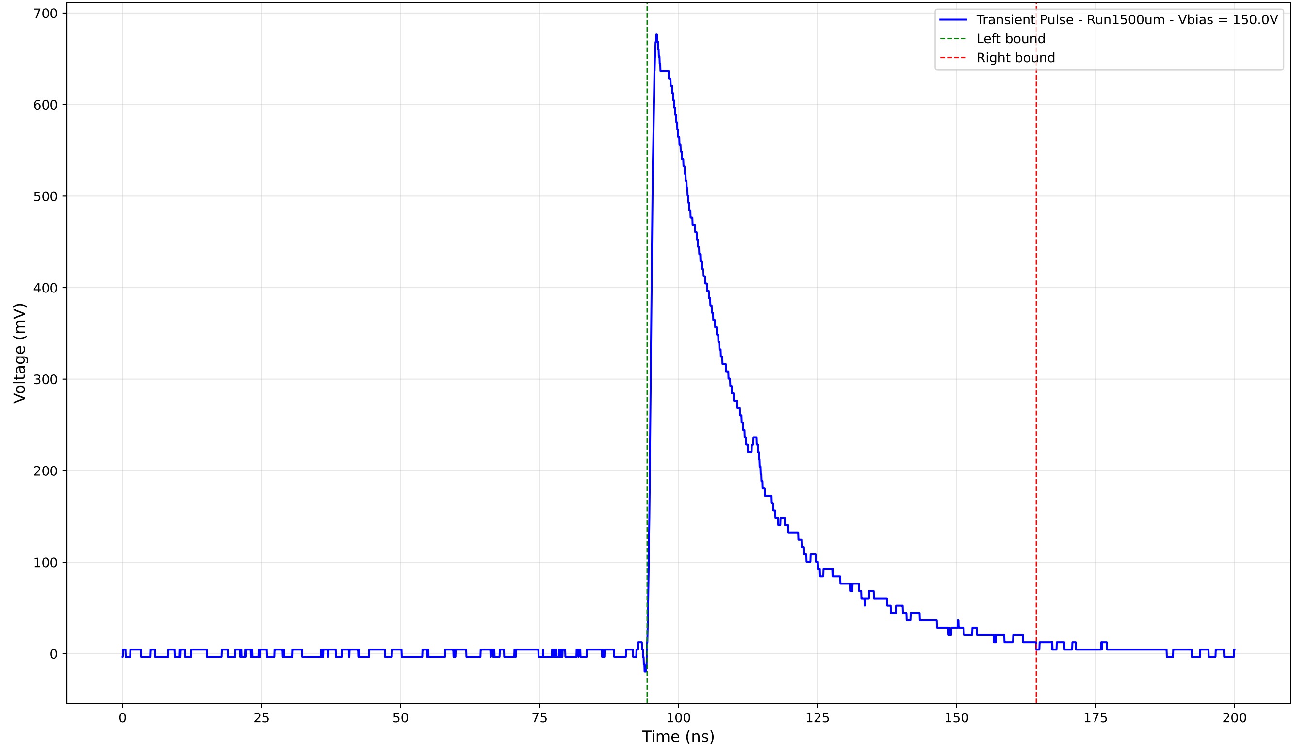
Transient Pulse - Sample: 1cm_42 - Position: 3325.0 \mu\text{m} - Charge: 229.30 pC
