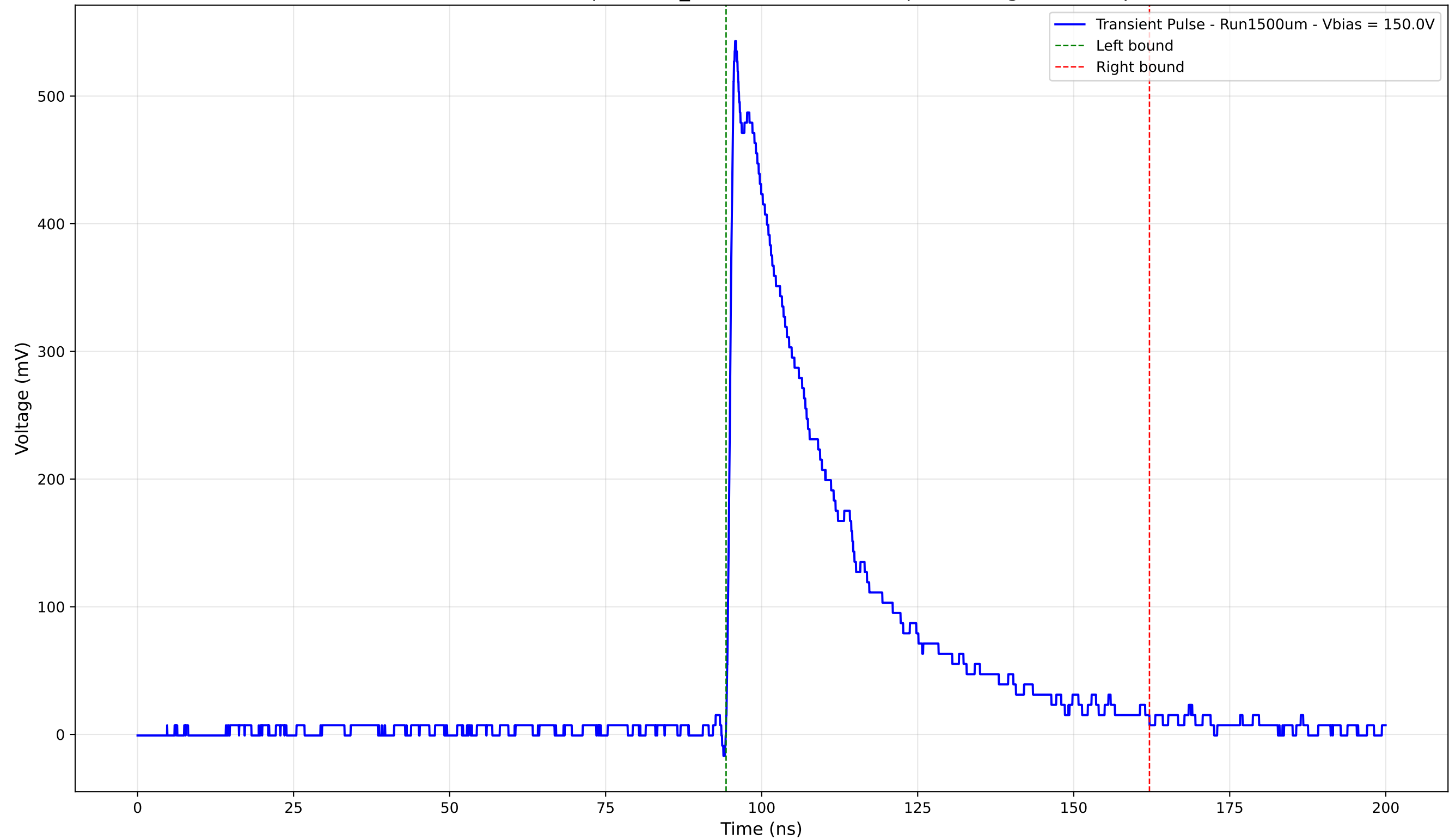
Transient Pulse - Sample: 1cm_42 - Position: 3190.0 \mu\text{m} - Charge: 176.08 pC
