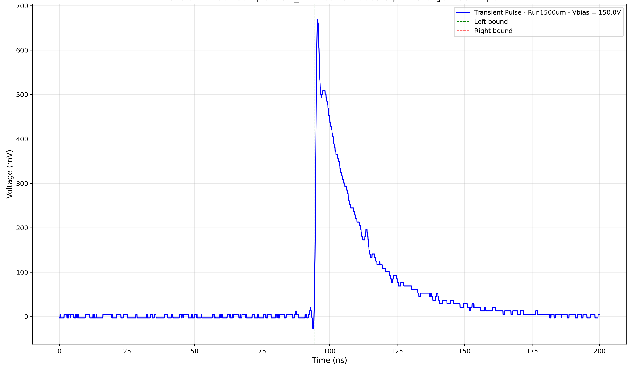
Transient Pulse - Sample: 1cm_42 - Position: 3035.0 \mu\text{m} - Charge: 188.14 pC
