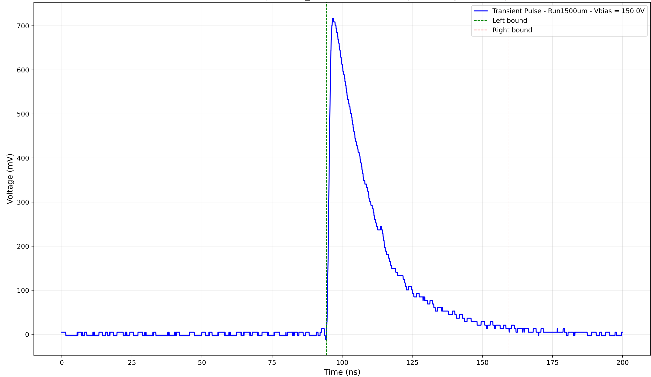
Transient Pulse - Sample: 1cm_42 - Position: 3935.0 \mu\text{m} - Charge: 236.58 pC
