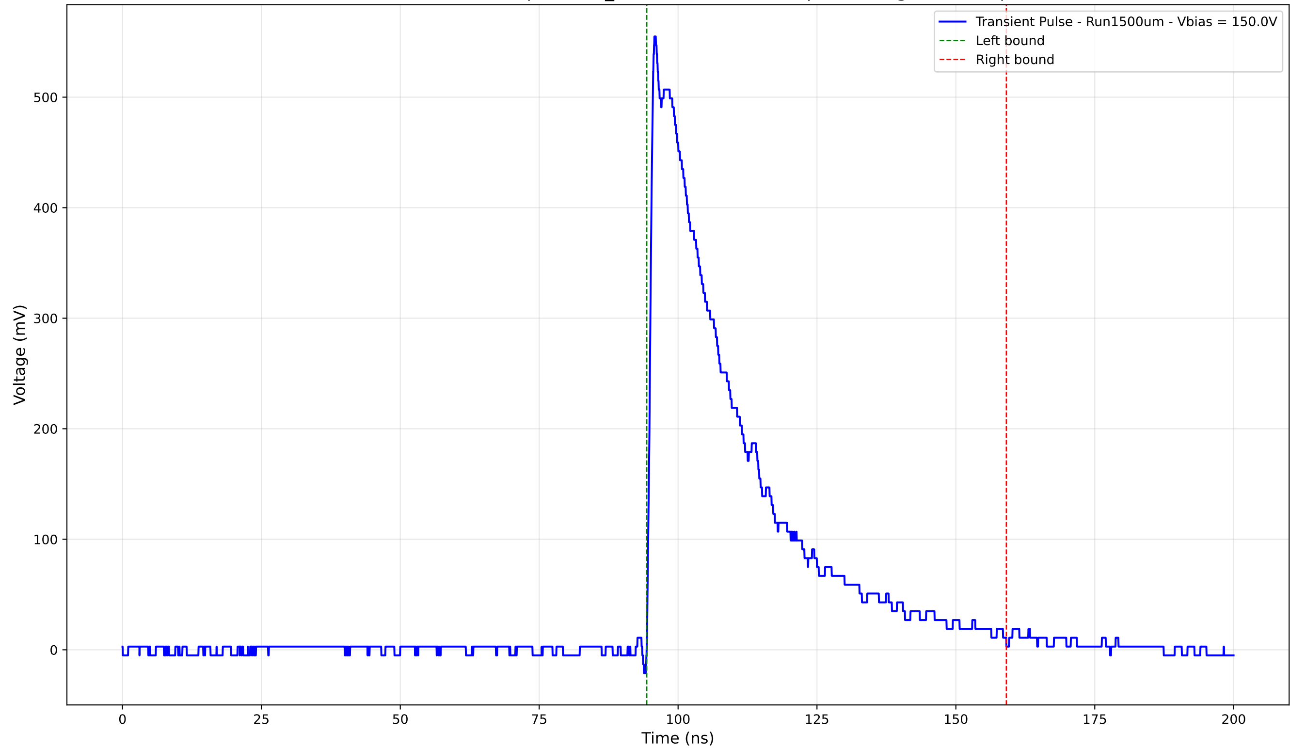
Transient Pulse - Sample: 1cm_42 - Position: 1975.0 \mu\text{m} - Charge: 182.87 pC
