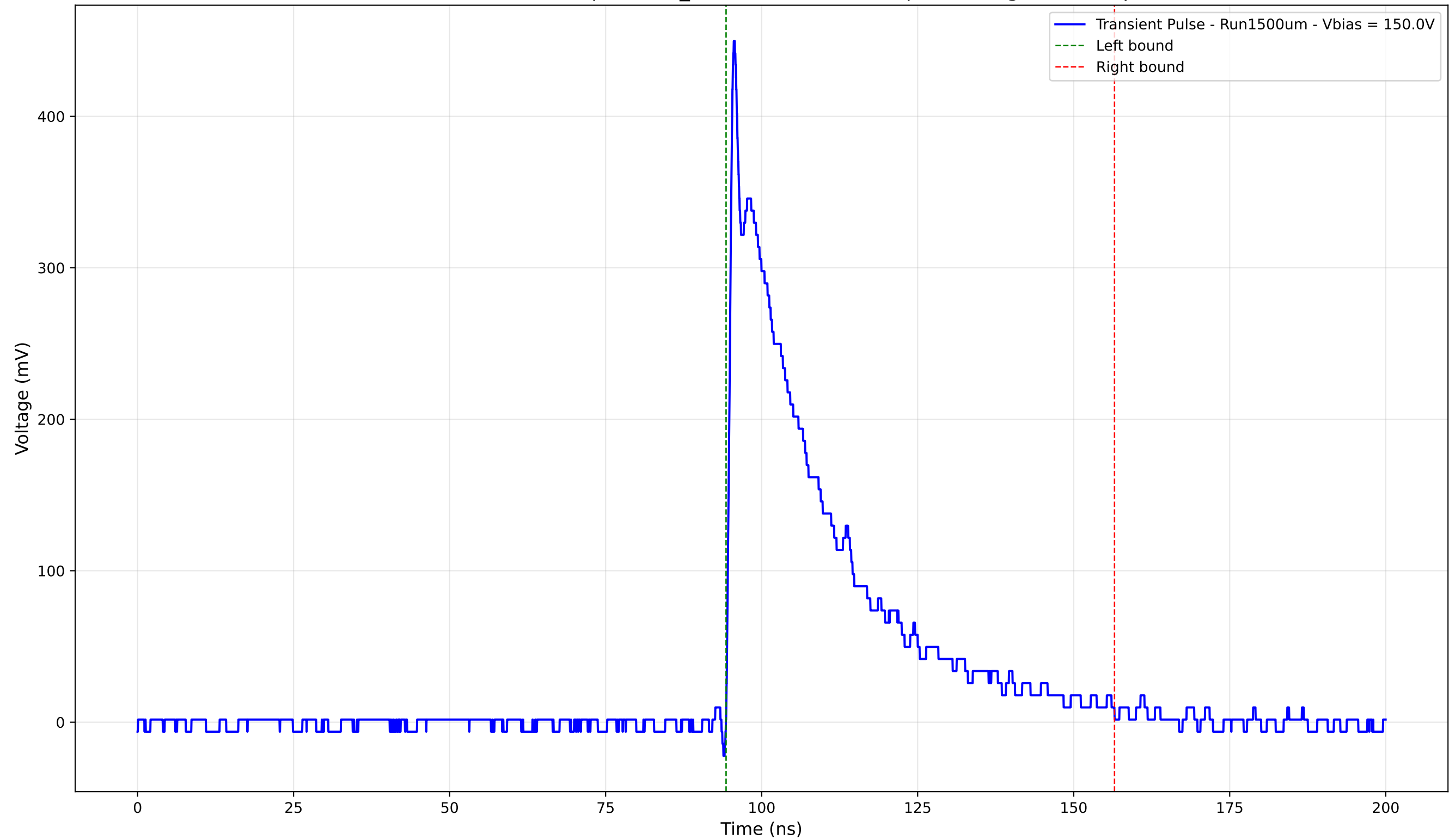
Transient Pulse - Sample: 1cm_42 - Position: 2165.0 \mu\text{m} - Charge: 122.56 pC
