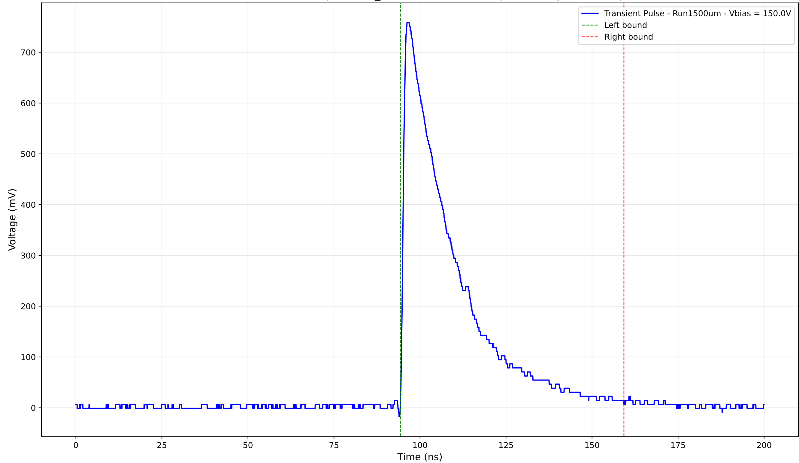
Transient Pulse - Sample: 1cm_42 - Position: 4360.0 \mu\text{m} - Charge: 238.00 pC
