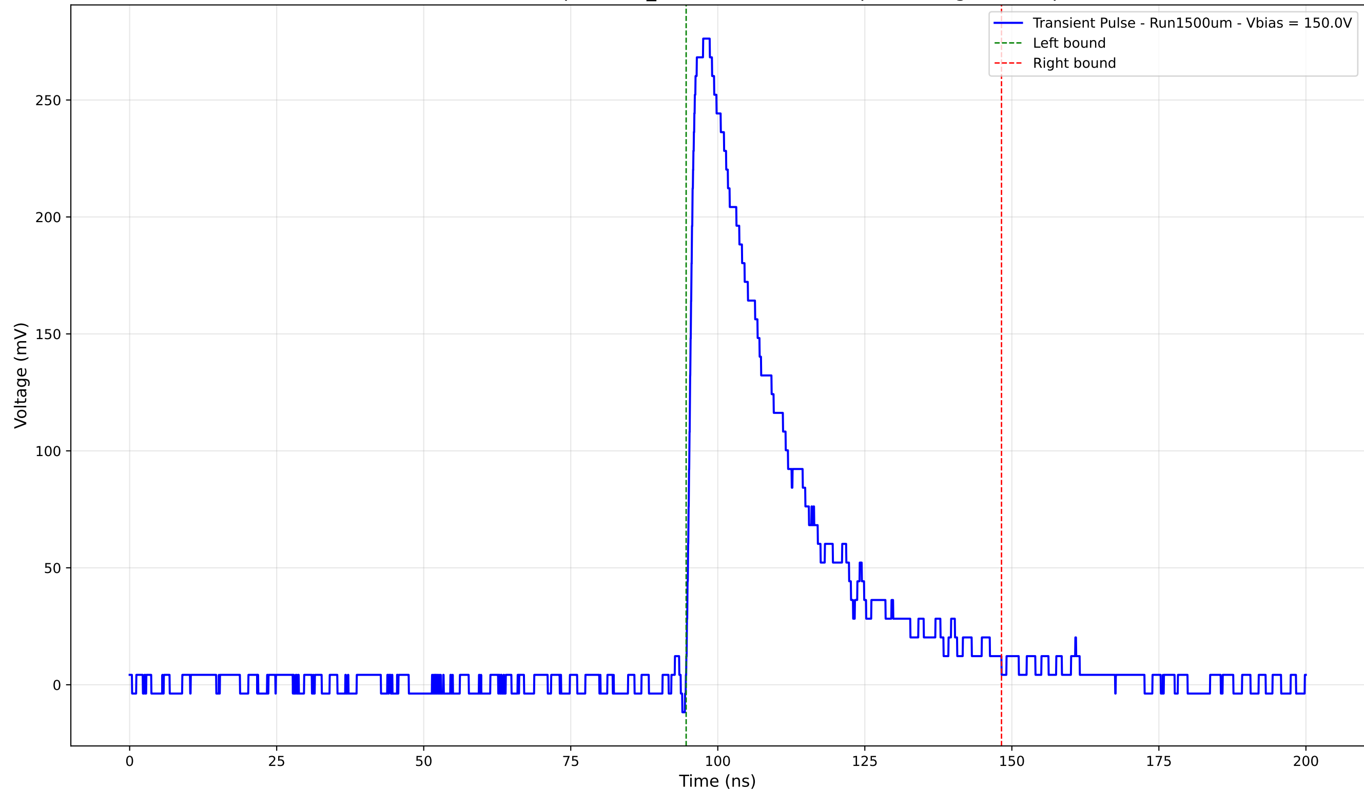
Transient Pulse - Sample: 1cm_42 - Position: 1545.0 \mu\text{m} - Charge: 91.21 pC
