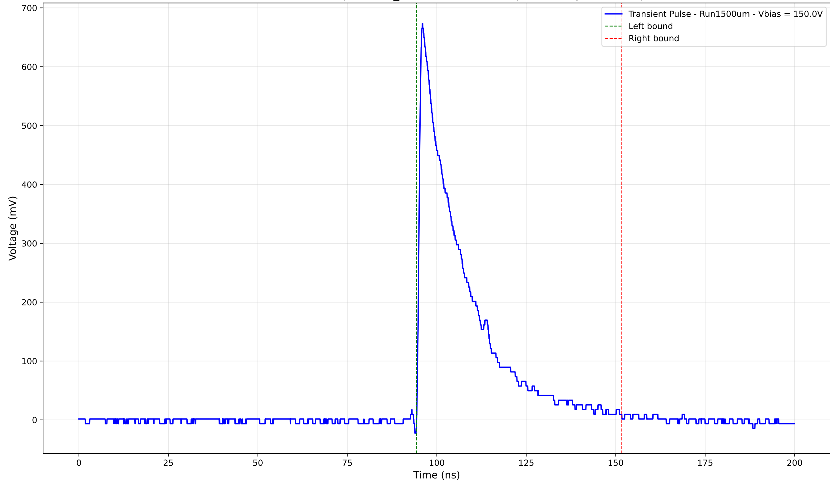
Transient Pulse - Sample: 1cm_42 - Position: 445.0 \mu\text{m} - Charge: 171.78 pC
