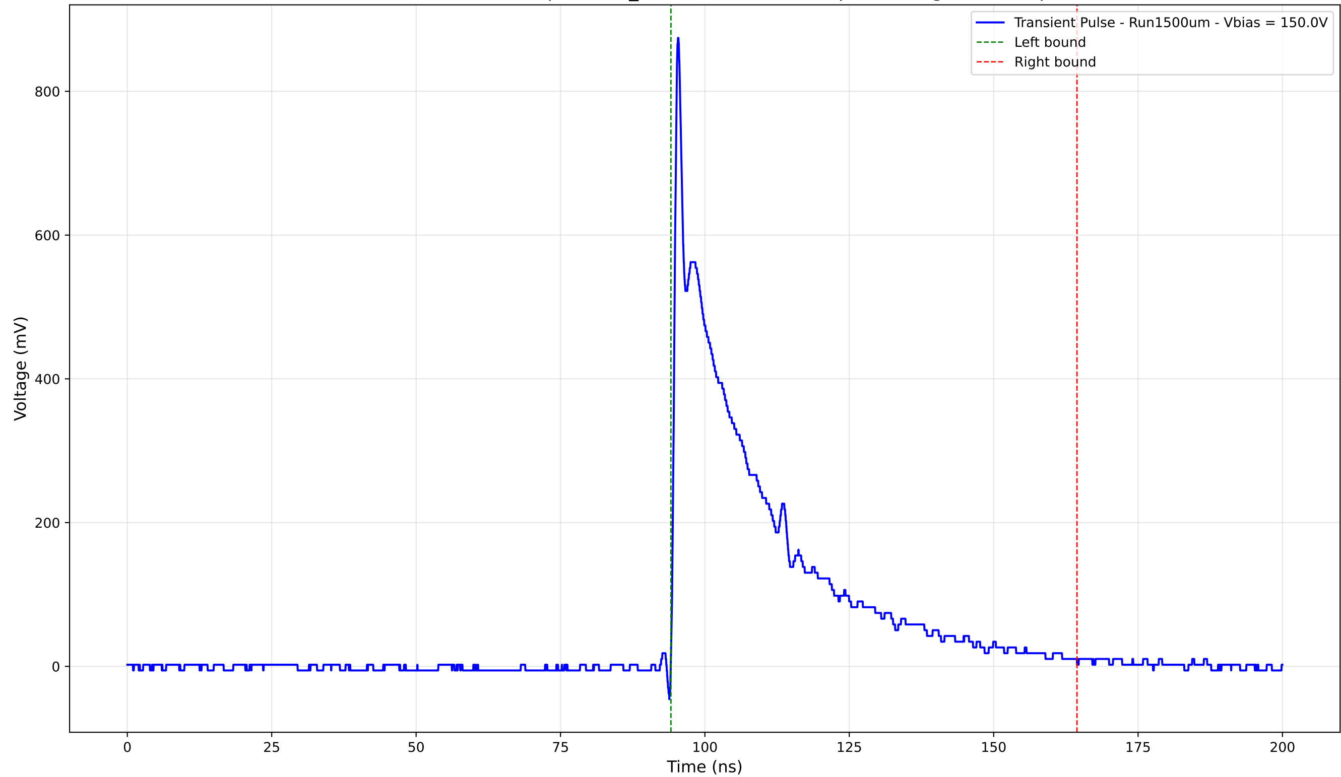
Transient Pulse - Sample: 1cm_42 - Position: 2775.0 \mu\text{m} - Charge: 210.89 pC
