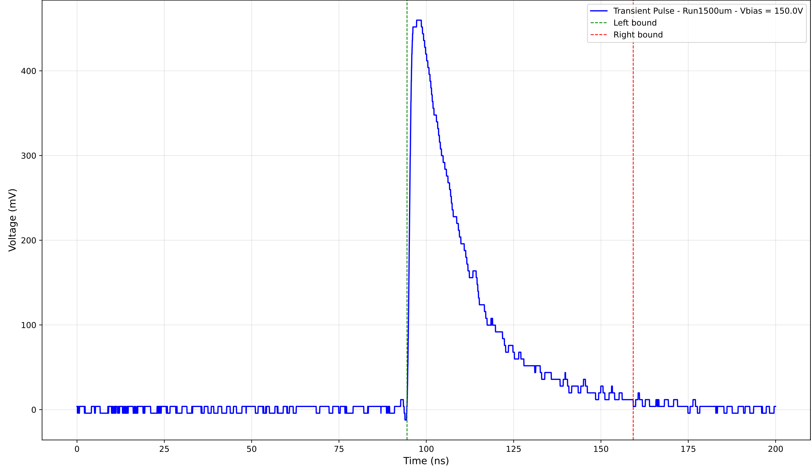
Transient Pulse - Sample: 1cm_42 - Position: 1695.0 \mu\text{m} - Charge: 160.00 pC
