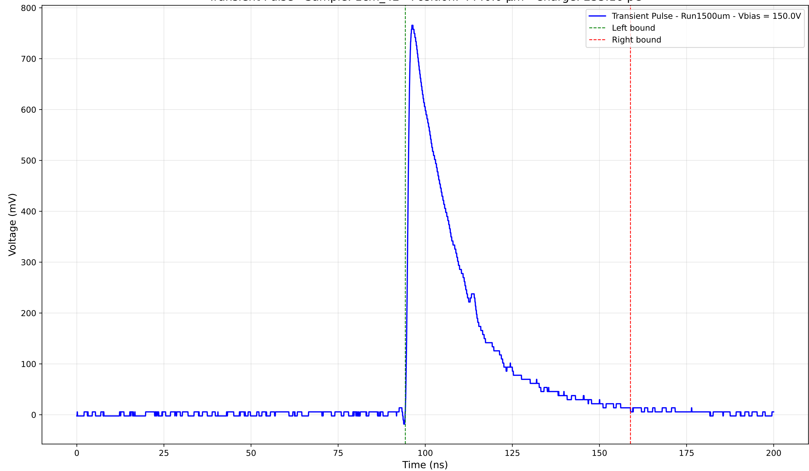
Transient Pulse - Sample: 1cm_42 - Position: 4440.0 \mu\text{m} - Charge: 233.16 pC
