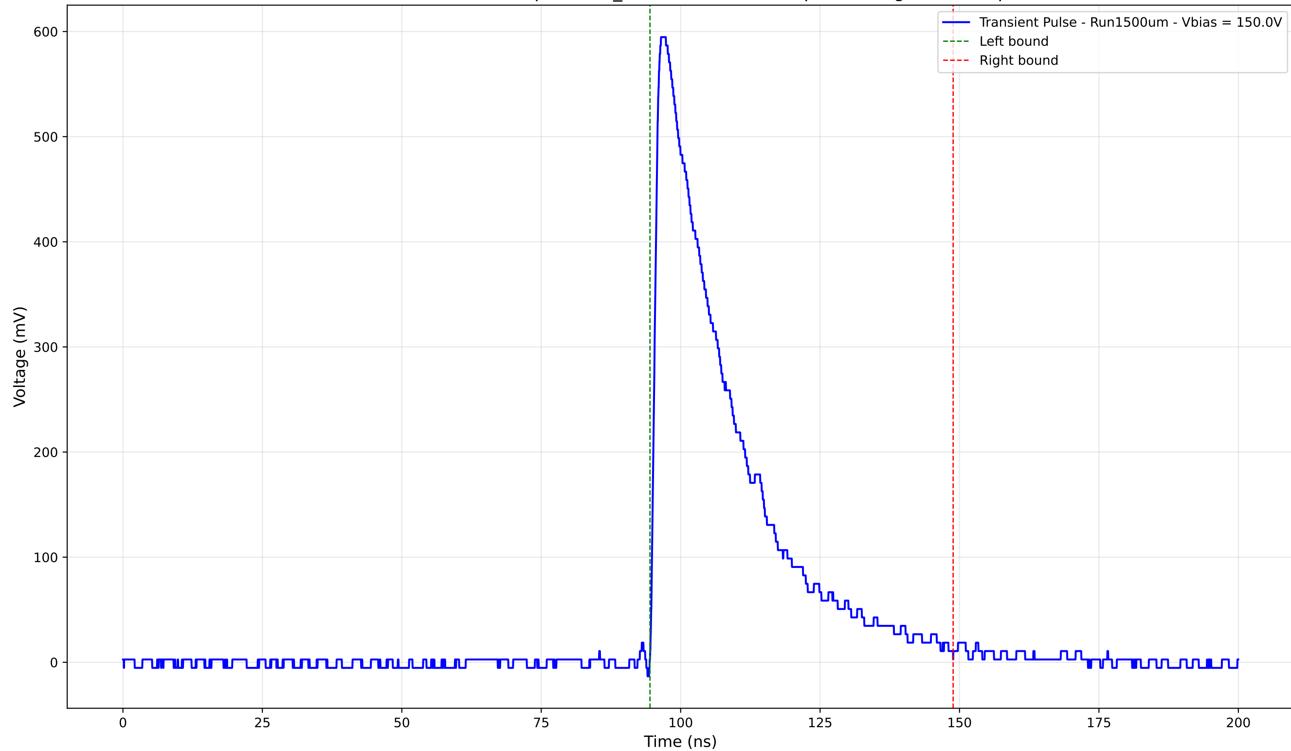
Transient Pulse - Sample: 1cm_42 - Position: 840.0 \mu\text{m} - Charge: 176.80 pC
