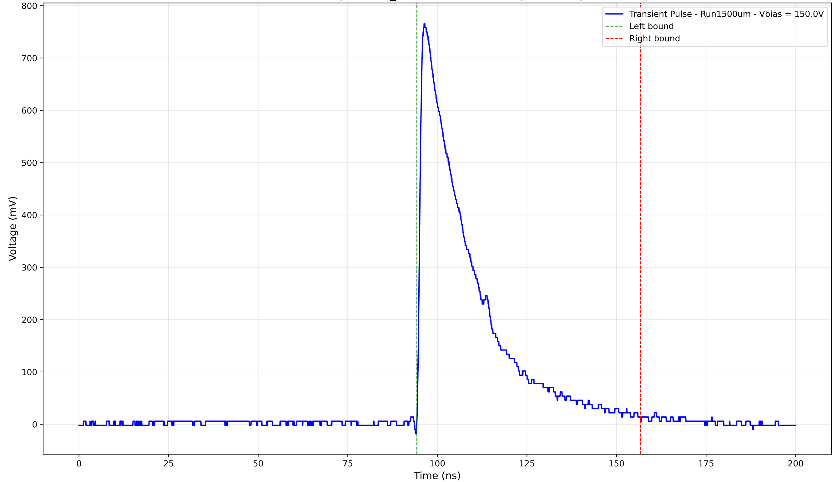
Transient Pulse - Sample: 1cm_42 - Position: 4375.0 \mu\text{m} - Charge: 238.02 pC
