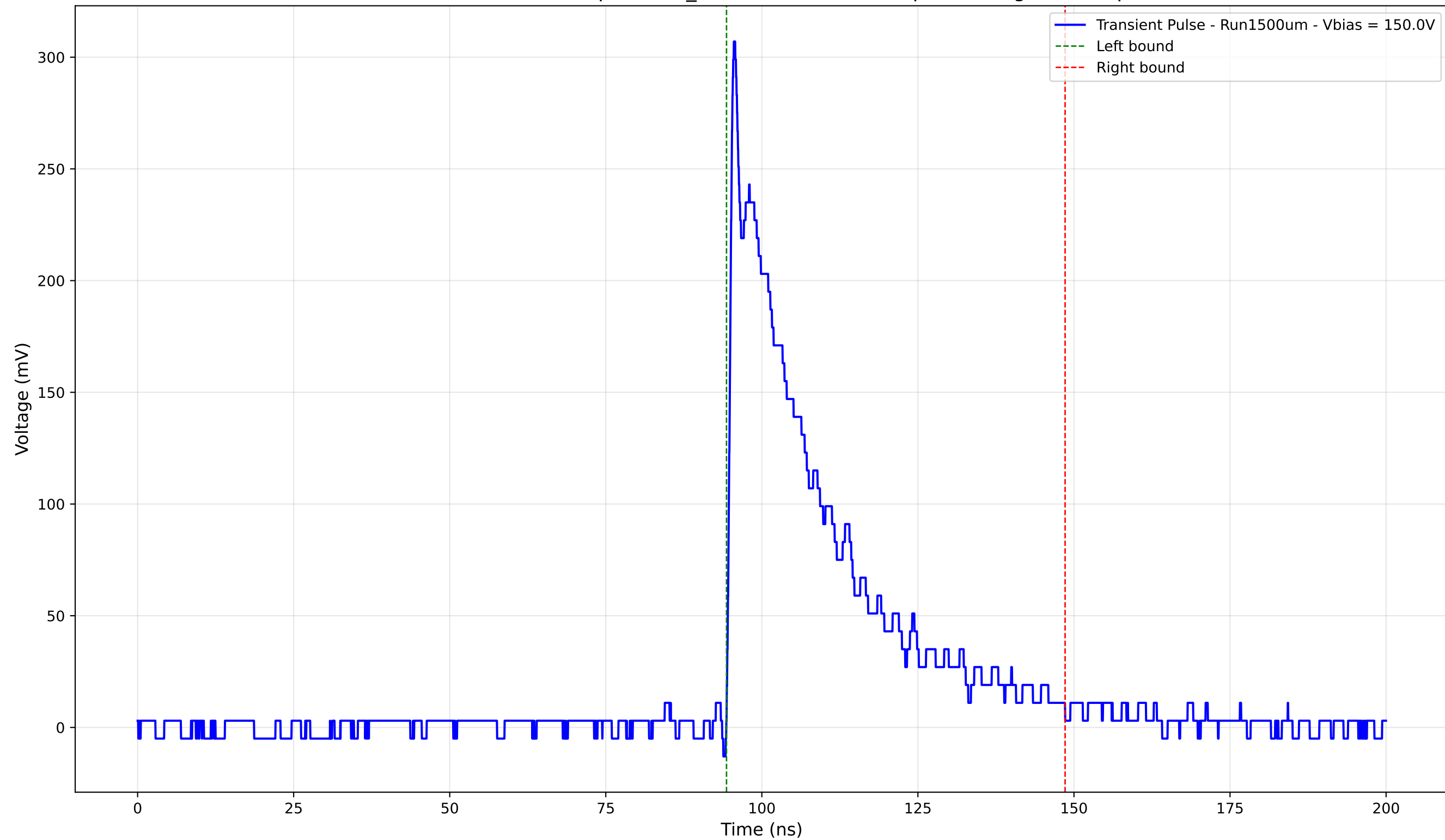
Transient Pulse - Sample: 1cm_42 - Position: 2145.0 \mu\text{m} - Charge: 82.99 pC
