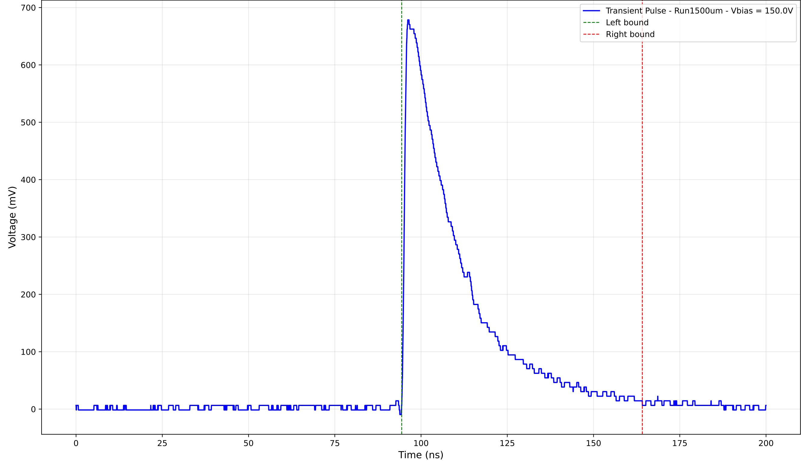
Transient Pulse - Sample: 1cm_42 - Position: 3480.0 \mu\text{m} - Charge: 235.48 pC
