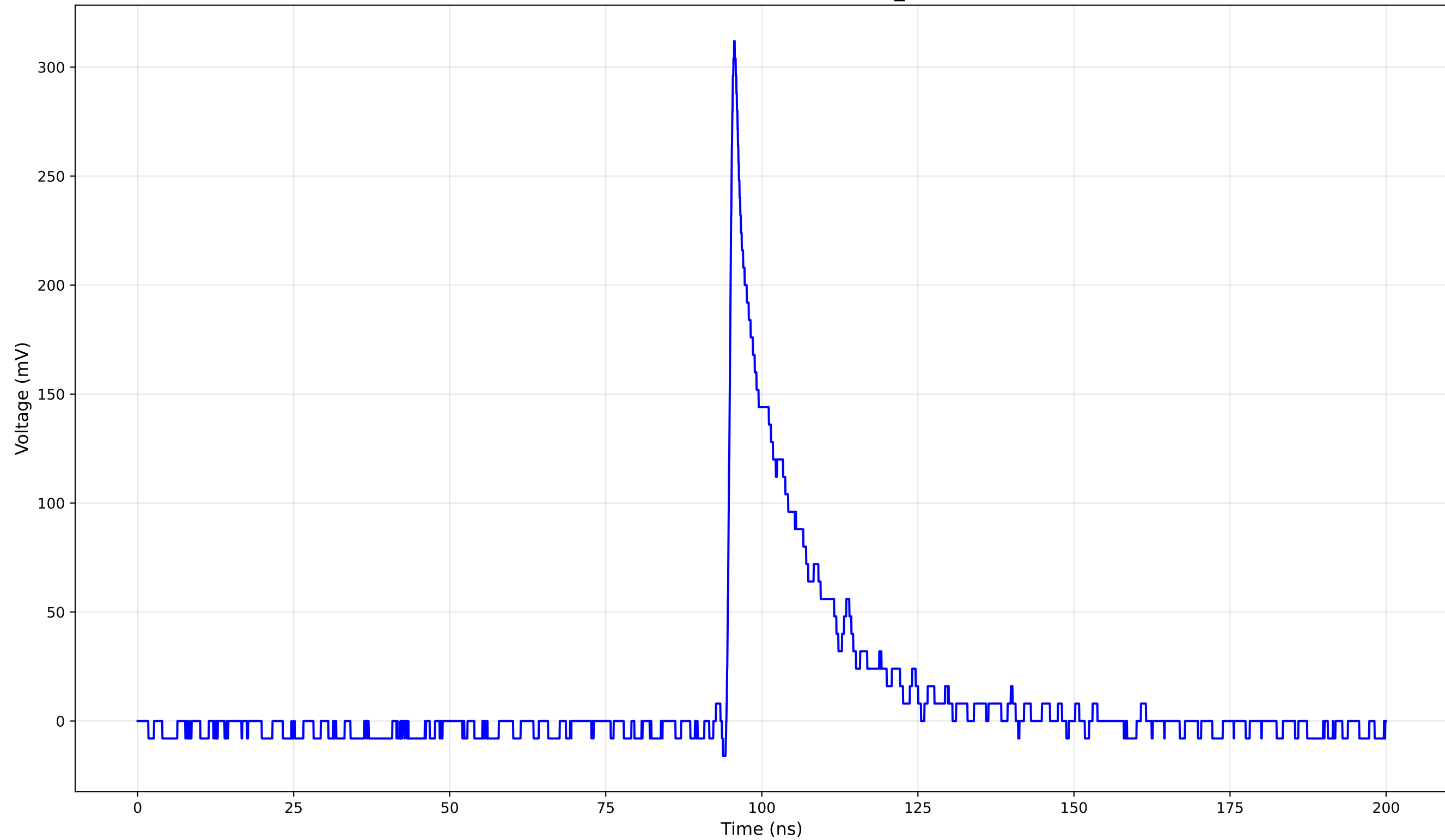
TCT Pulse Waveform - Run 155um: 1cm_42 (150.0 V)
