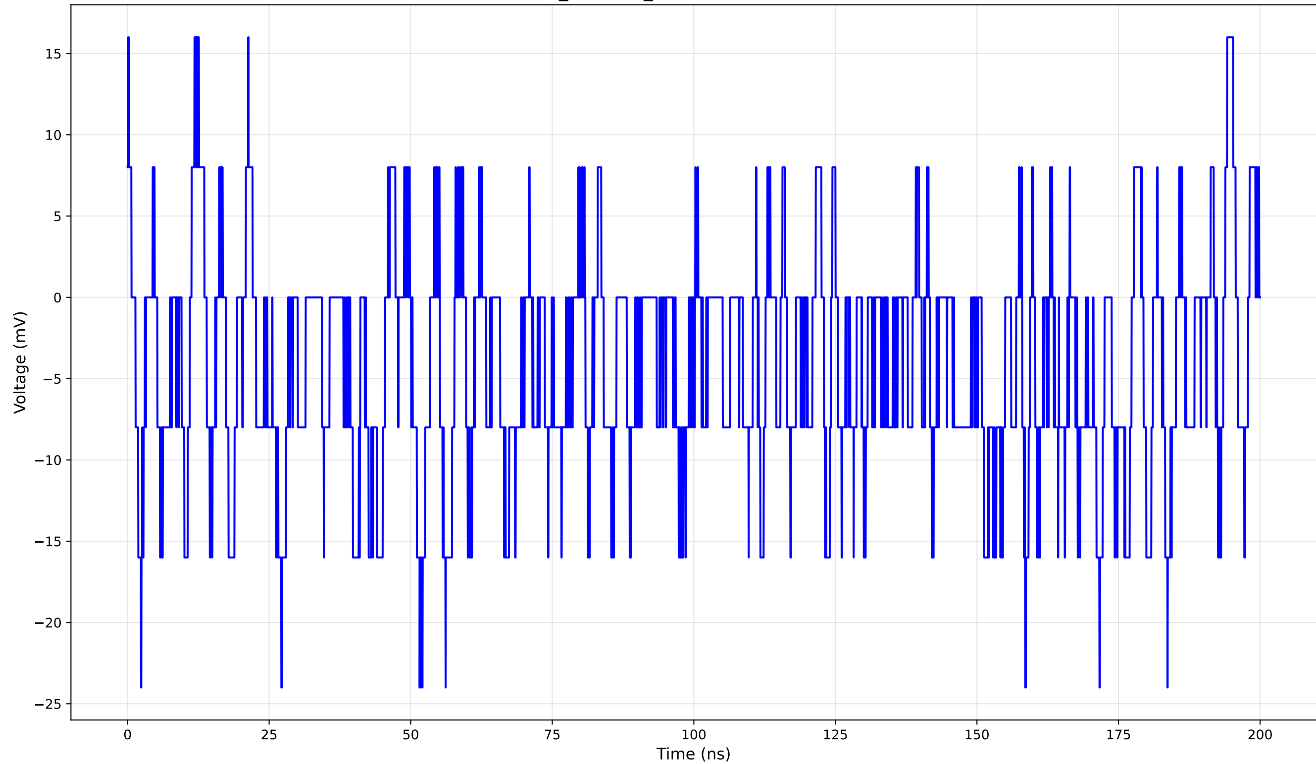
TCT Pulse Waveform - Run 1_10: 1cm_42-Position1 (10.0 V) - Rise Time: 0.00 ns (N/A)
