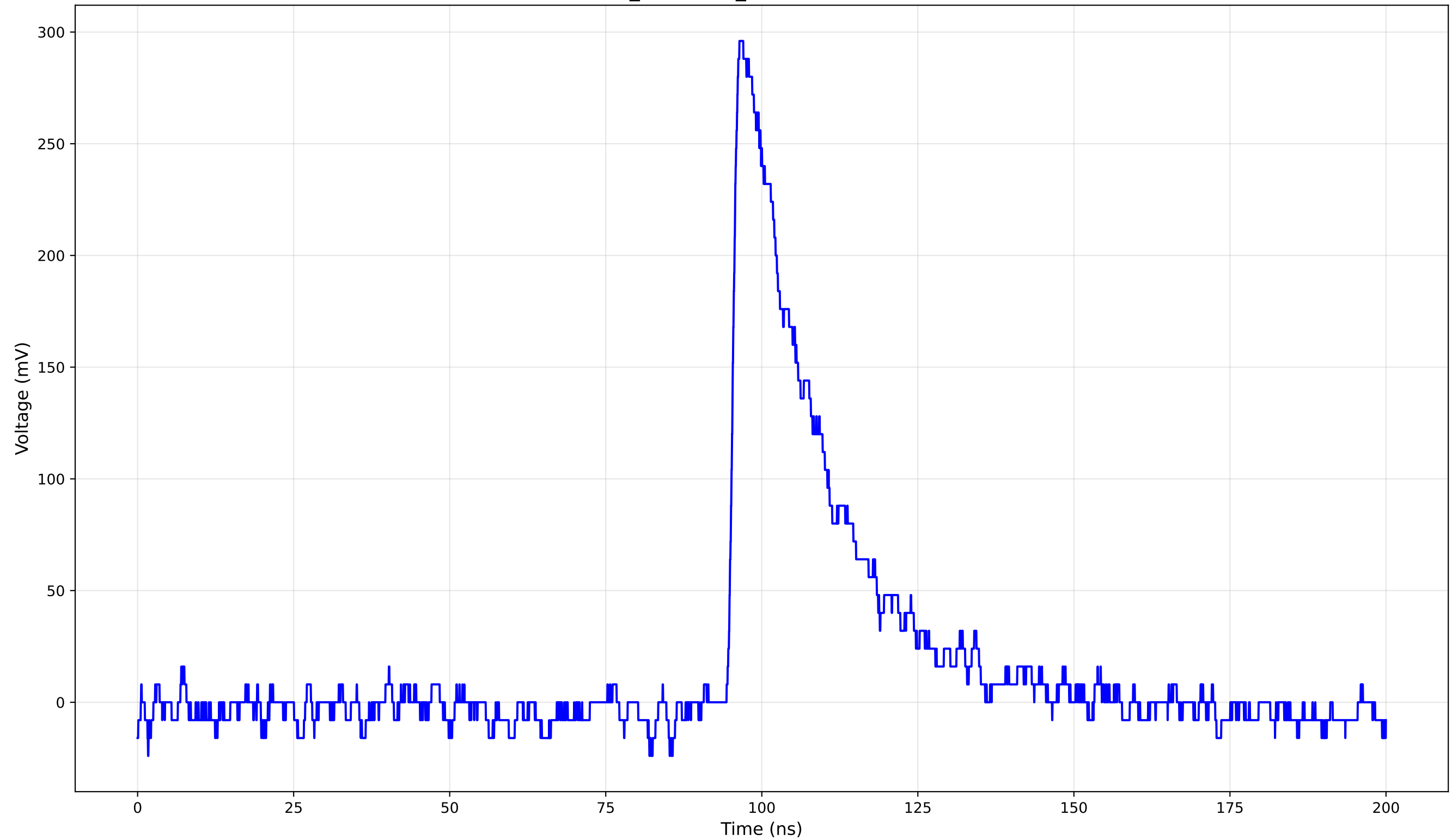
TCT Pulse Waveform - Run 1_100: 1cm_42-Position1 (100.0 V) - Rise Time: 1.35 ns
