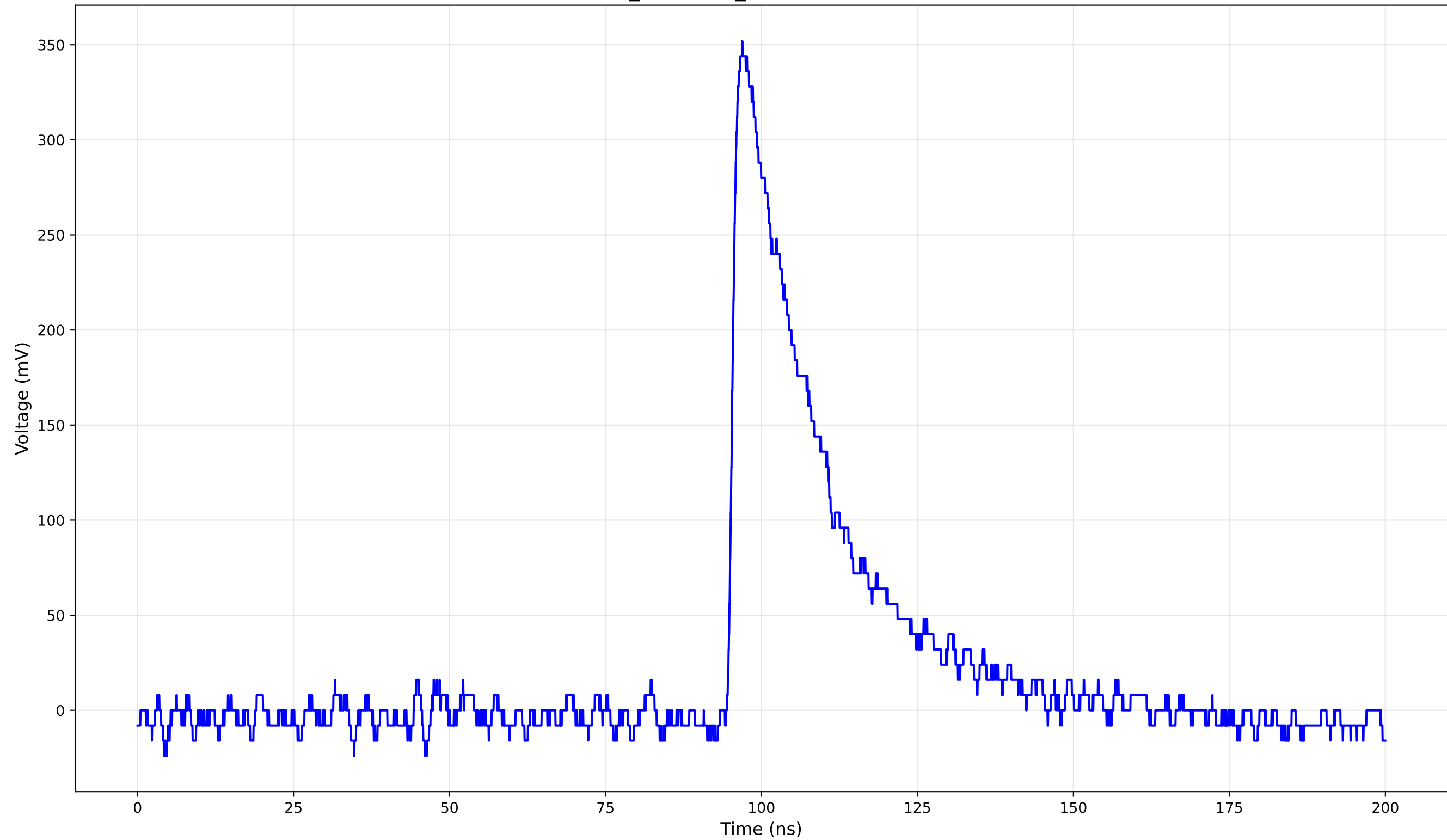
TCT Pulse Waveform - Run 1_110: 1cm_42-Position1 (110.0 V) - Rise Time: 1.40 ns
