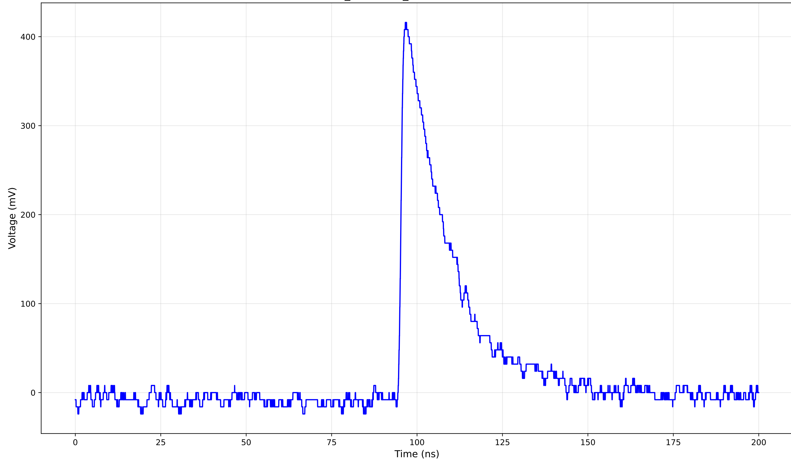
TCT Pulse Waveform - Run 1_120: 1cm_42-Position1 (120.0 V) - Rise Time: 1.27 ns
