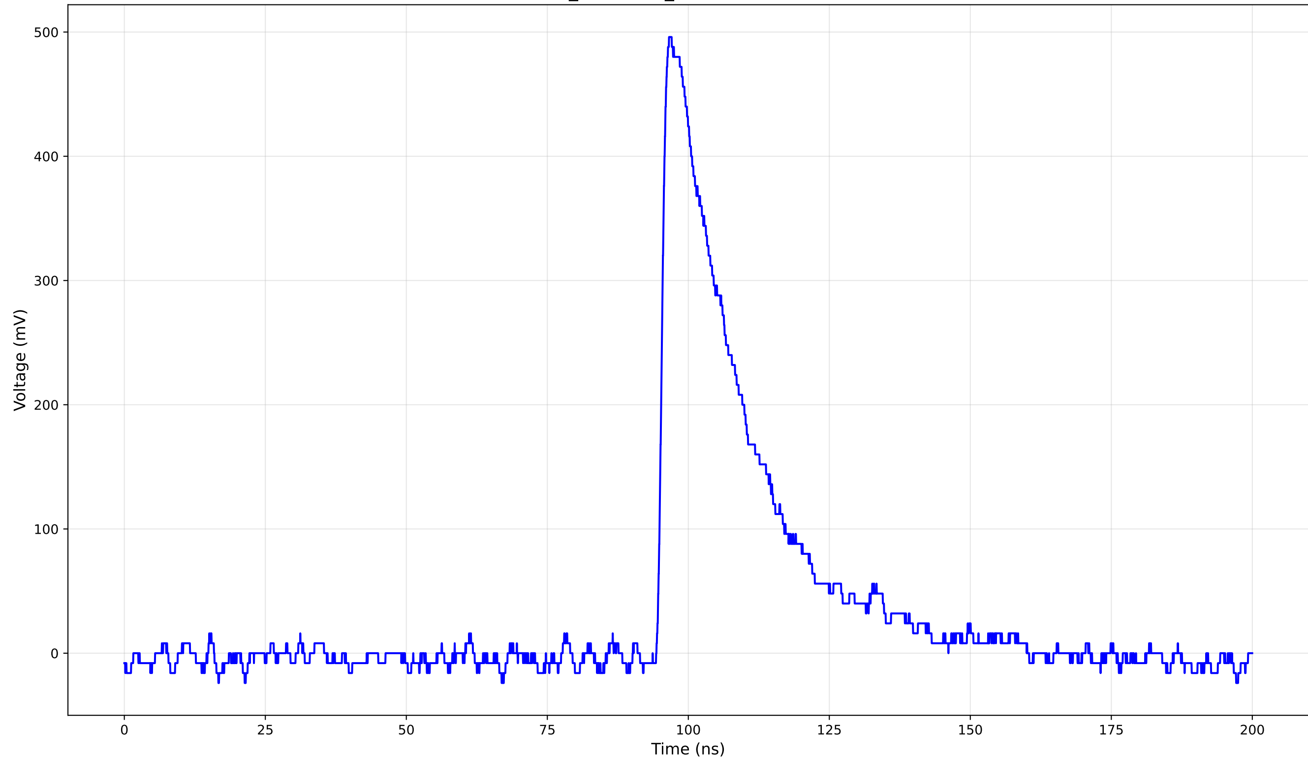
TCT Pulse Waveform - Run 1_130: 1cm_42-Position1 (130.0 V) - Rise Time: 1.37 ns
