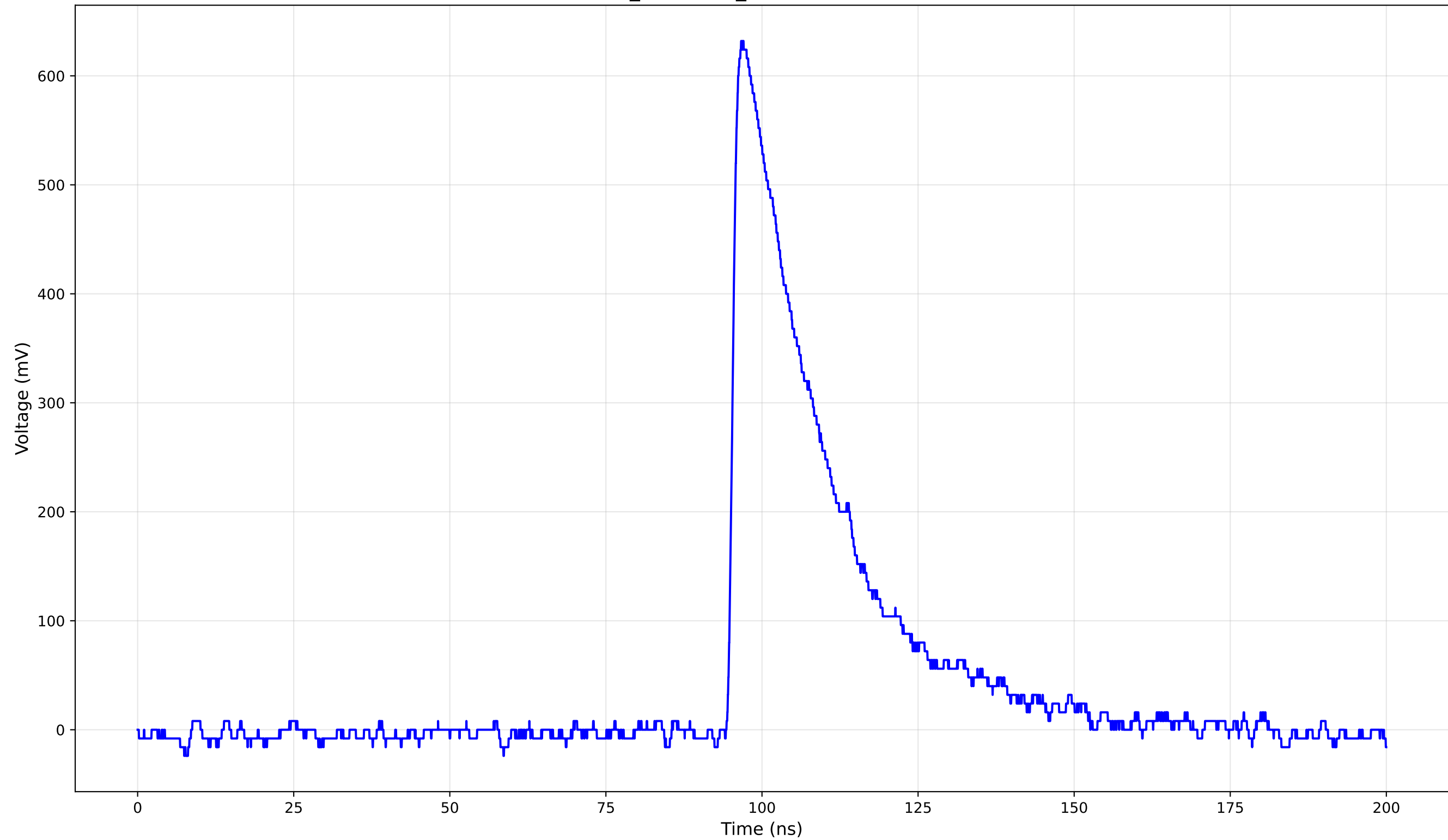
TCT Pulse Waveform - Run 1_140: 1cm_42-Position1 (140.0 V) - Rise Time: 1.40 ns
