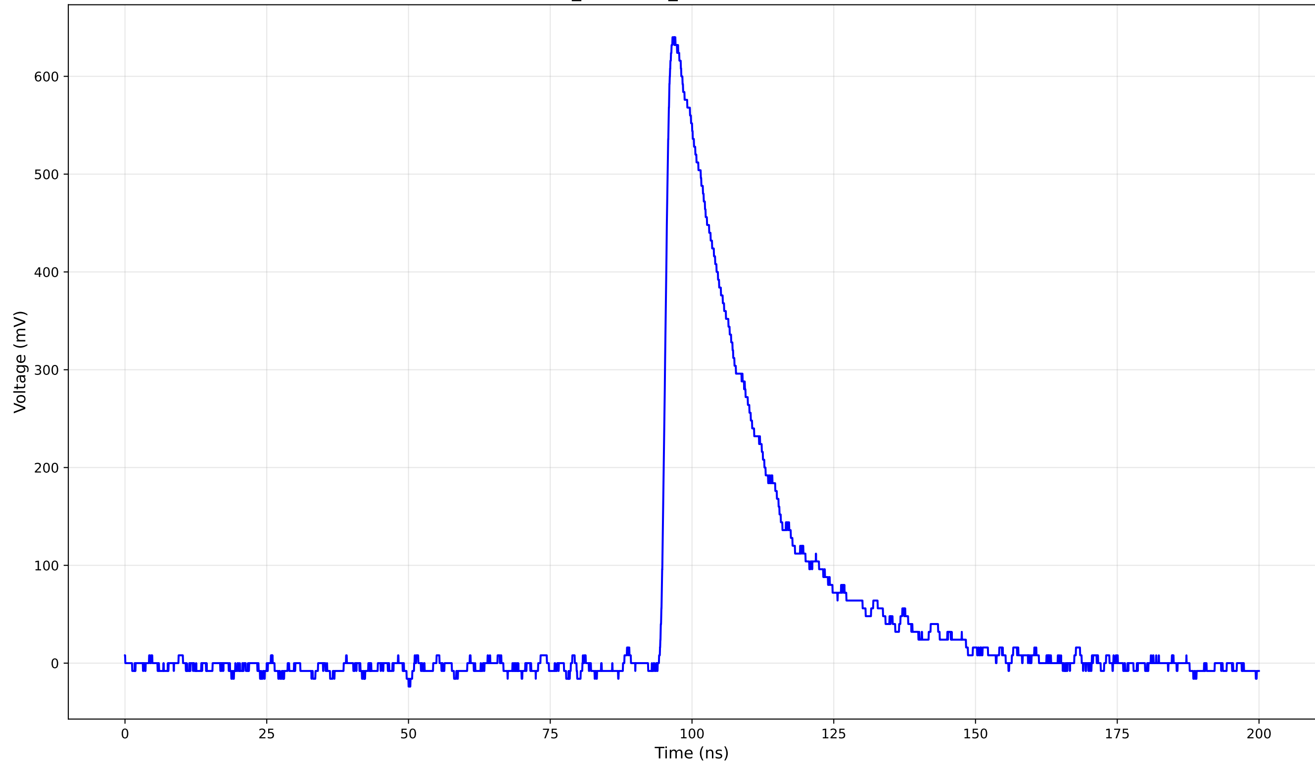
TCT Pulse Waveform - Run 1_141: 1cm_42-Position1 (141.0 V) - Rise Time: 1.32 ns
