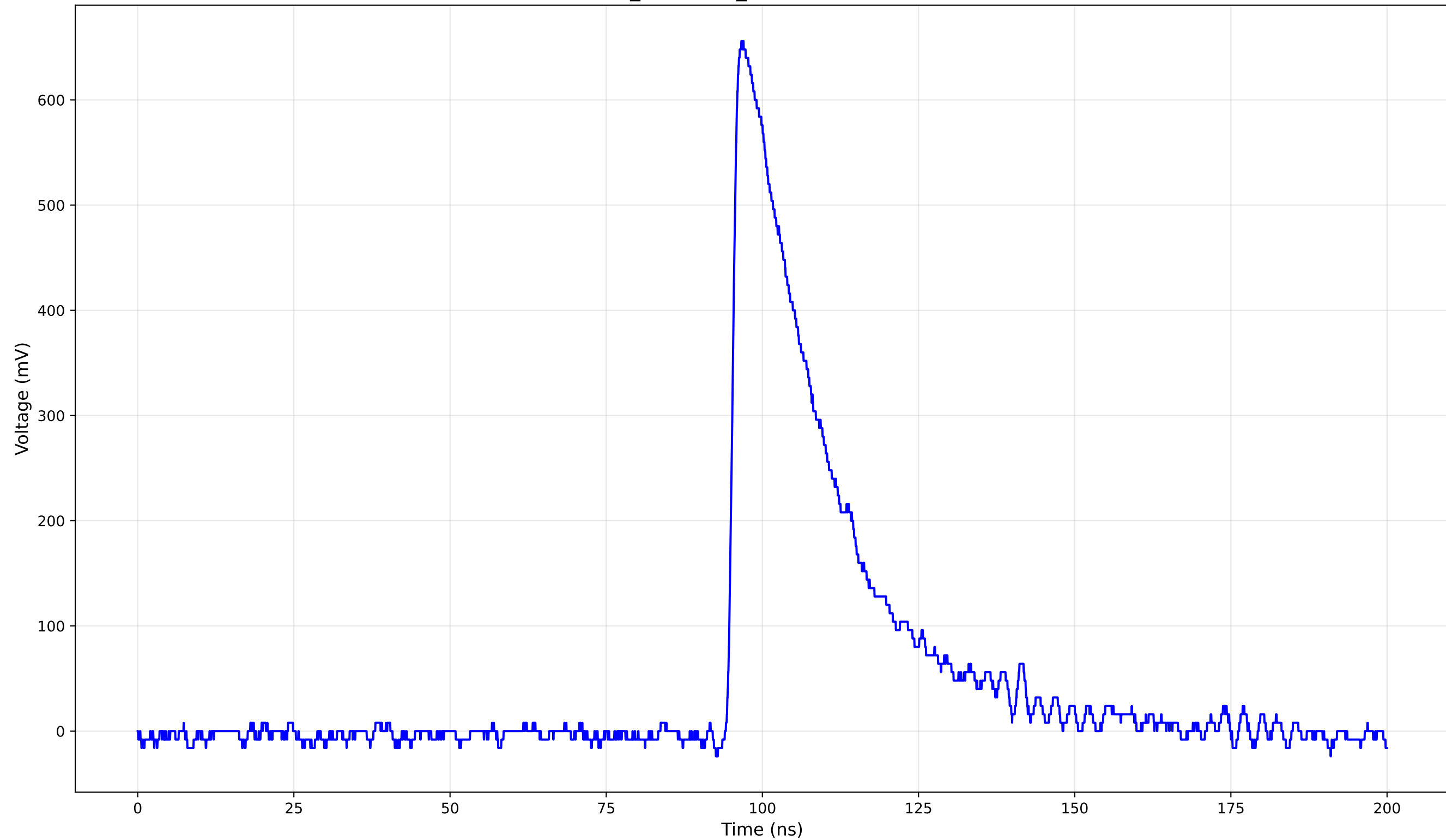
TCT Pulse Waveform - Run 1_142: 1cm_42-Position1 (142.0 V) - Rise Time: 1.35 ns
