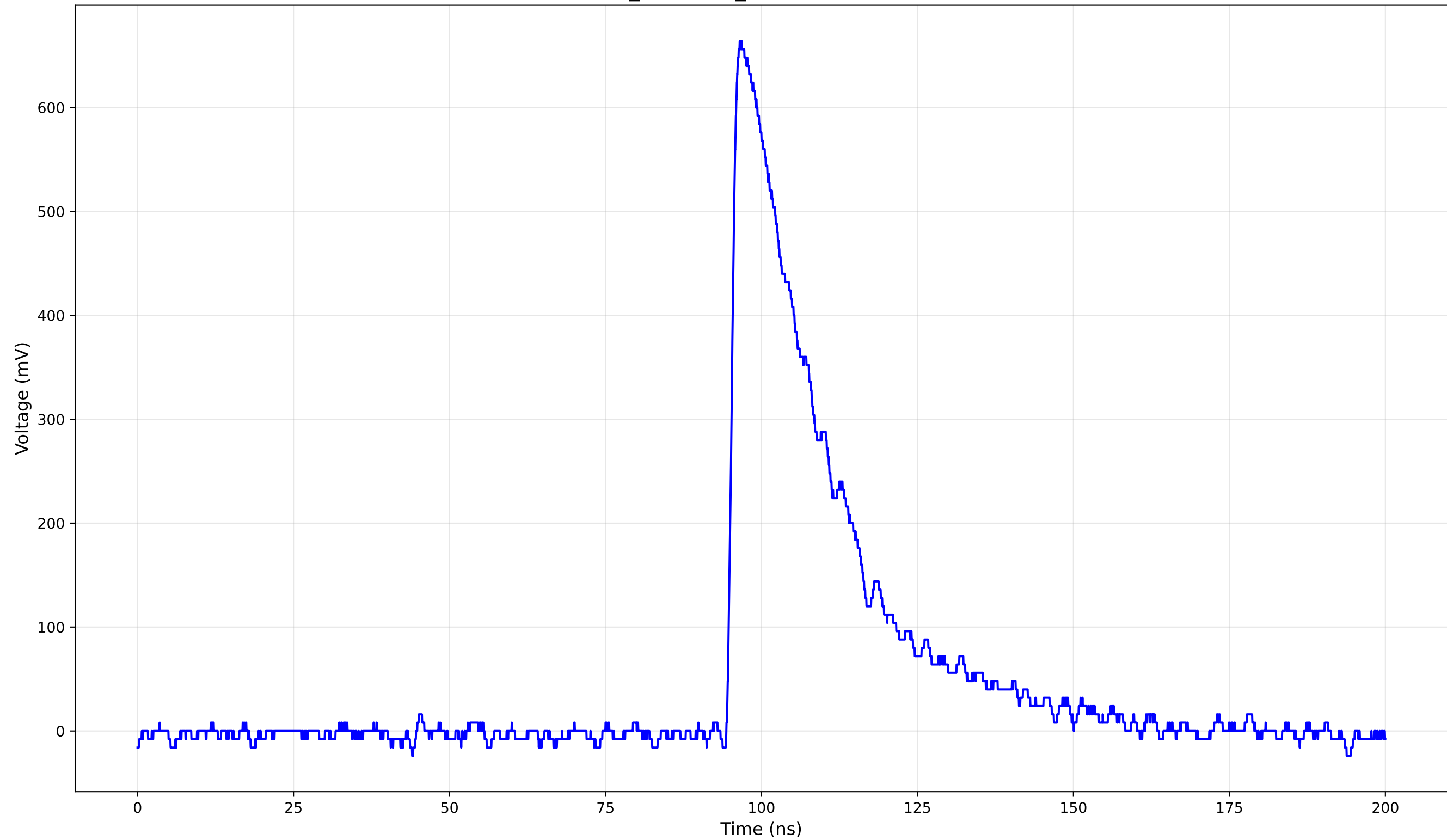
TCT Pulse Waveform - Run 1_143: 1cm_42-Position1 (143.0 V) - Rise Time: 1.28 ns
