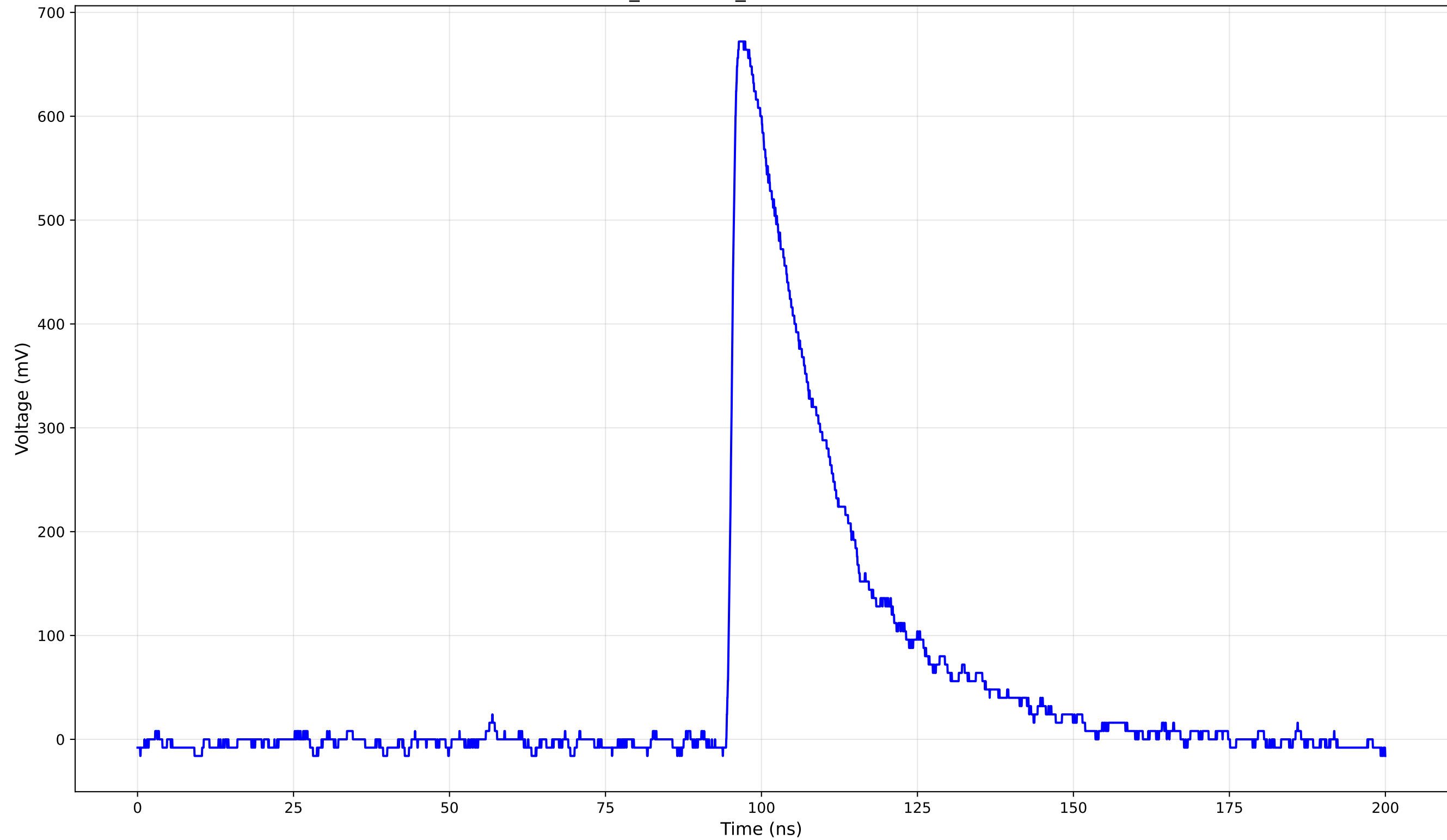
TCT Pulse Waveform - Run 1_144: 1cm_42-Position1 (144.0 V) - Rise Time: 1.22 ns
