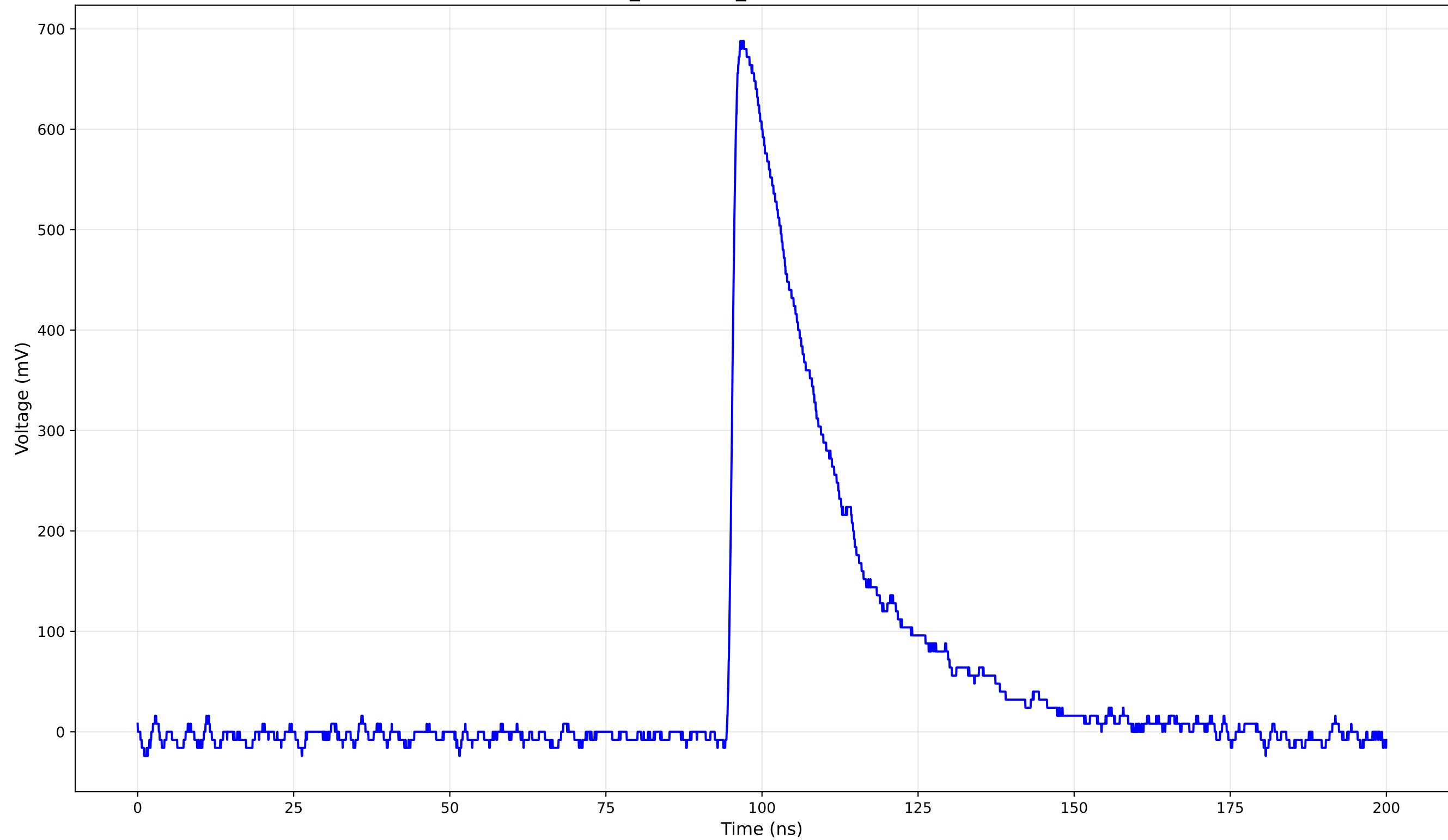
TCT Pulse Waveform - Run 1_145: 1cm_42-Position1 (145.0 V) - Rise Time: 1.28 ns
