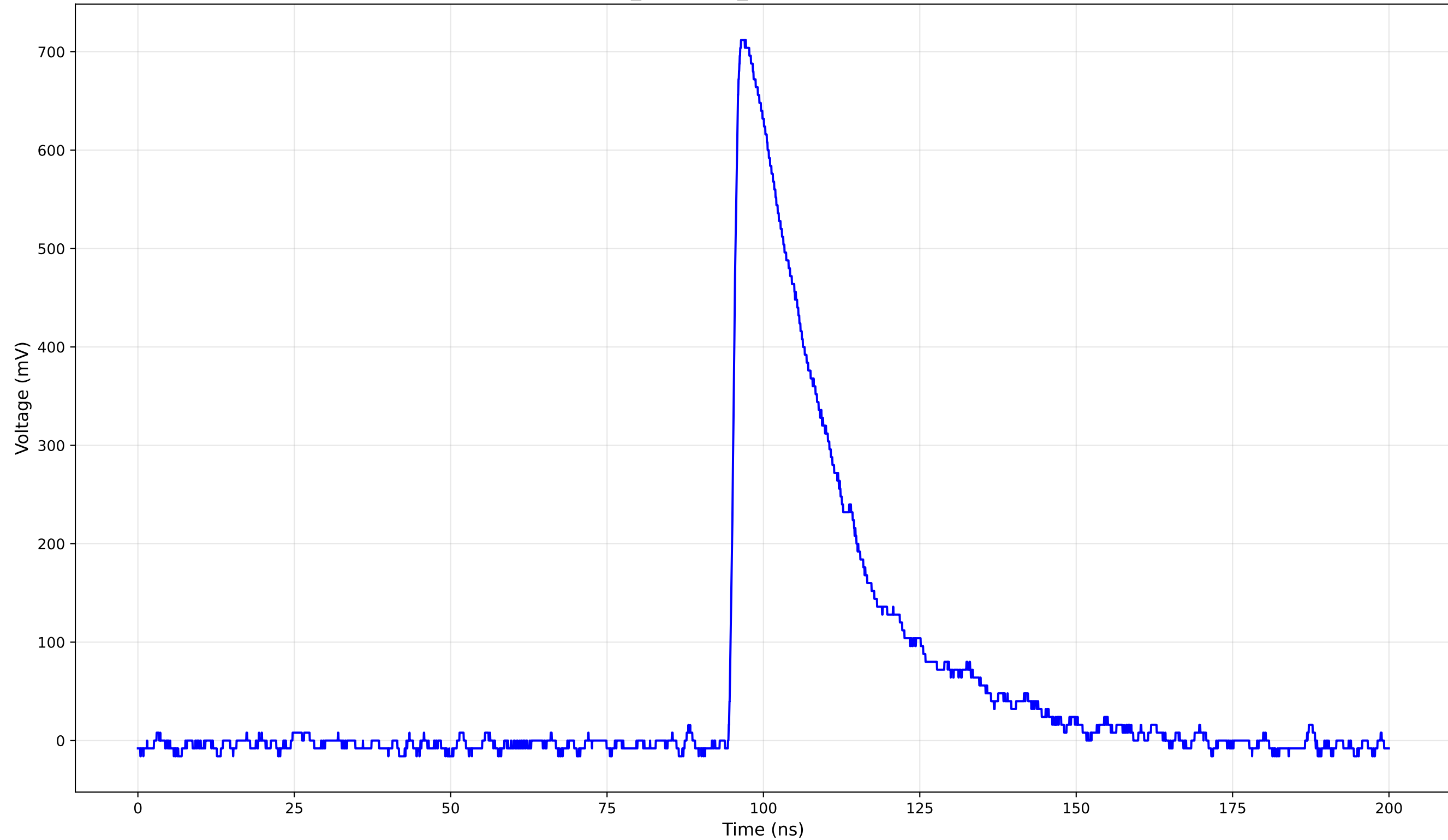
TCT Pulse Waveform - Run 1_146: 1cm_42-Position1 (146.0 V) - Rise Time: 1.21 ns
