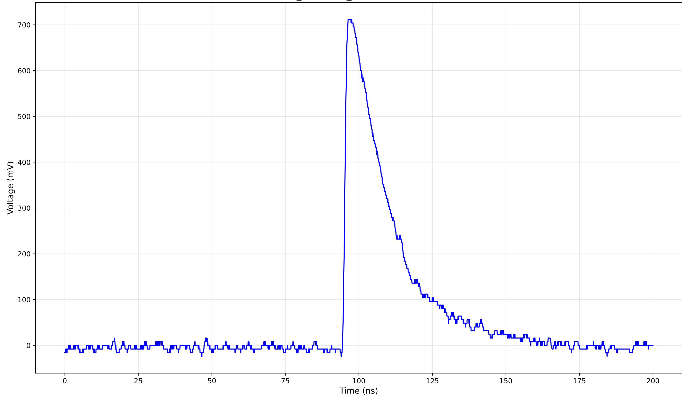
TCT Pulse Waveform - Run 1_147: 1cm_42-Position1 (147.0 V) - Rise Time: 1.22 ns
