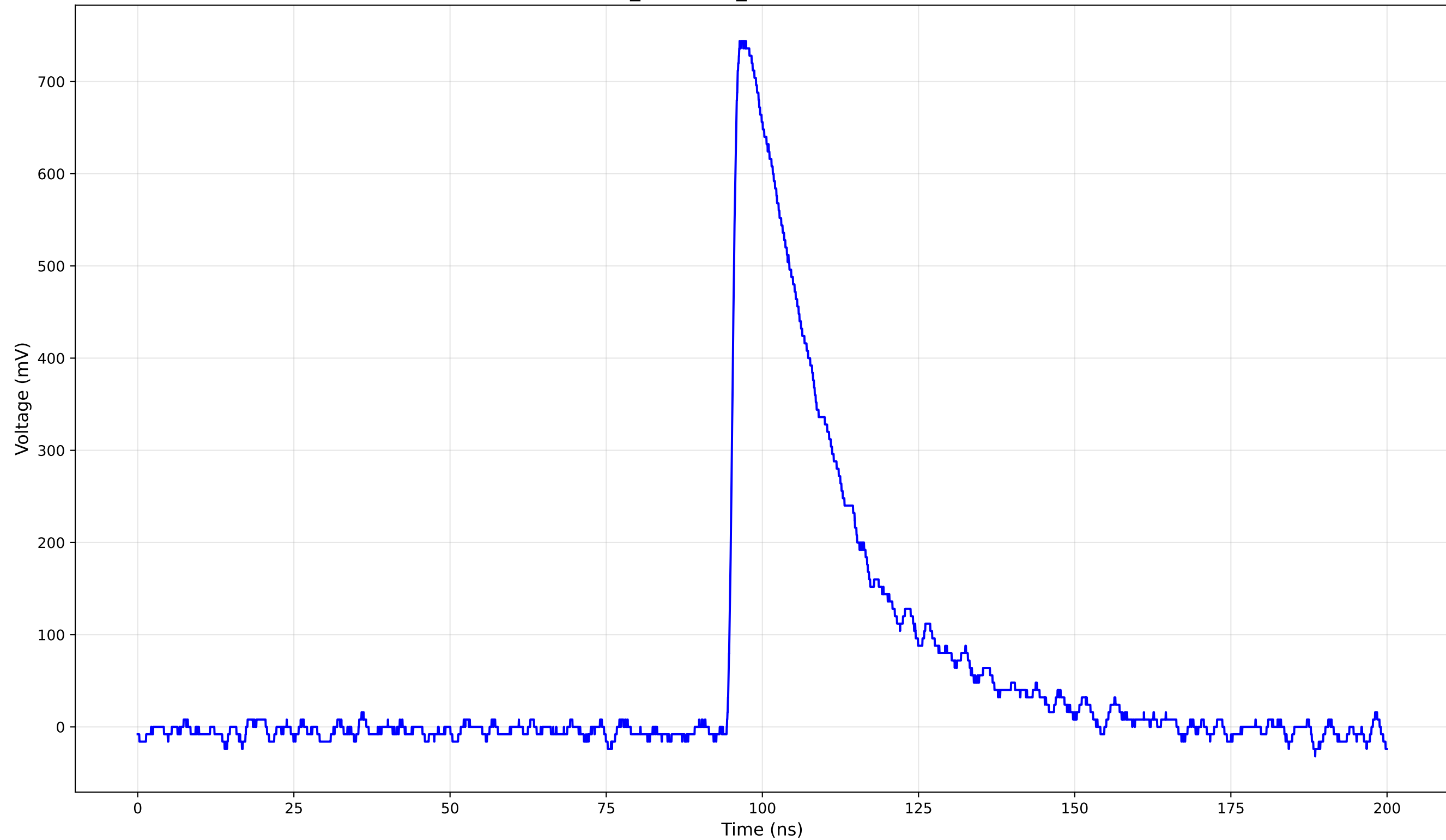
TCT Pulse Waveform - Run 1_148: 1cm_42-Position1 (148.0 V) - Rise Time: 1.22 ns
