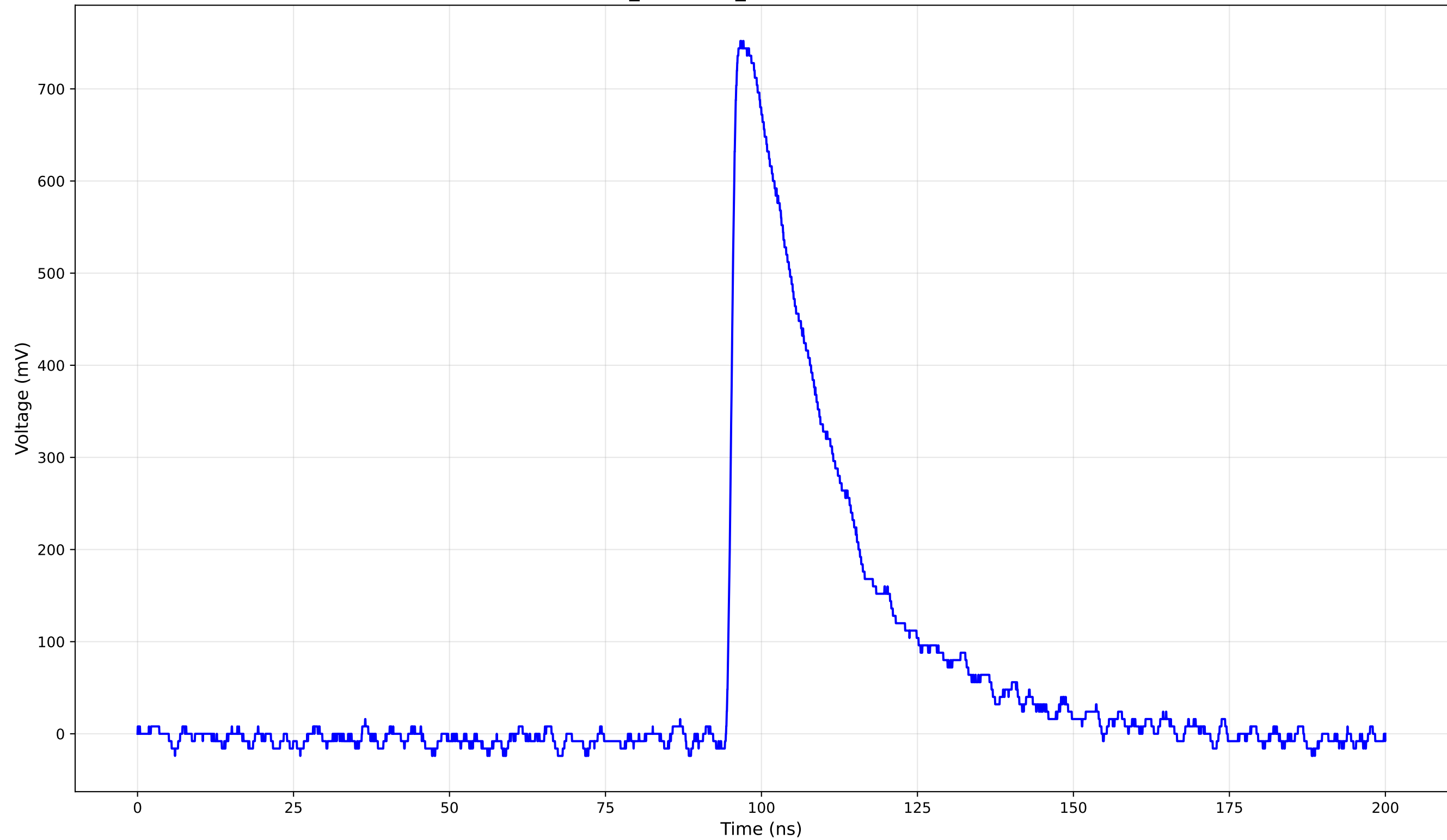
TCT Pulse Waveform - Run 1_149: 1cm_42-Position1 (149.0 V) - Rise Time: 1.23 ns
