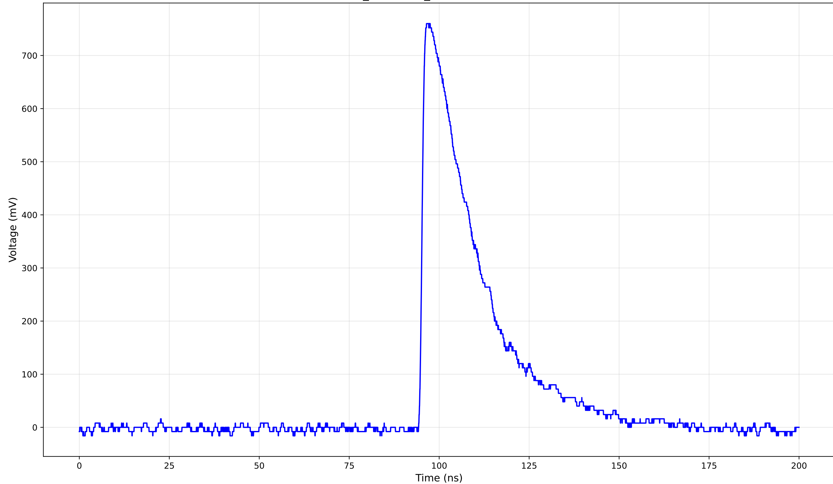
TCT Pulse Waveform - Run 1_150: 1cm_42-Position1 (150.0 V) - Rise Time: 1.23 ns
