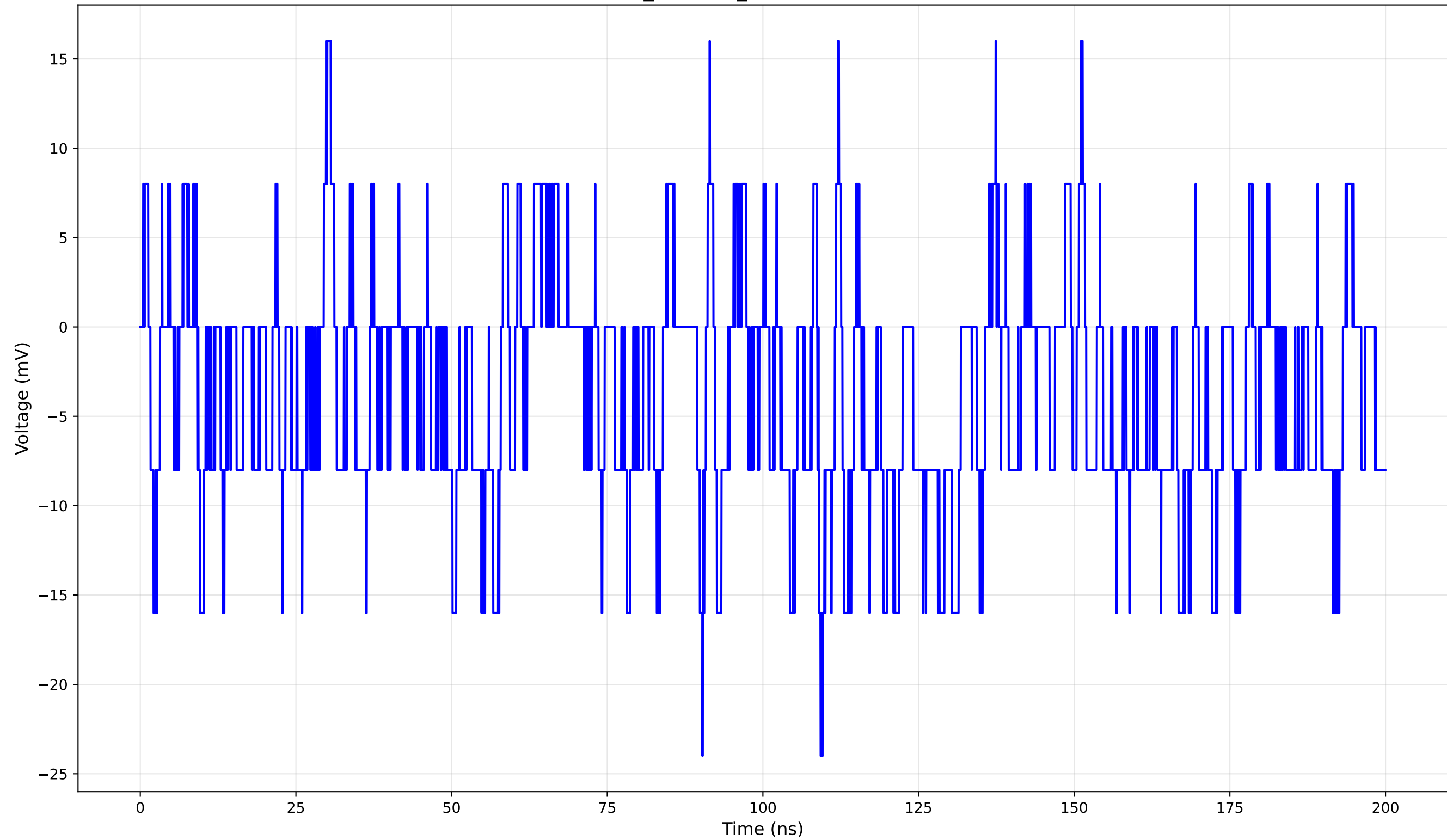
TCT Pulse Waveform - Run 1_20: 1cm_42-Position1 (20.0 V) - Rise Time: 0.86 ns
