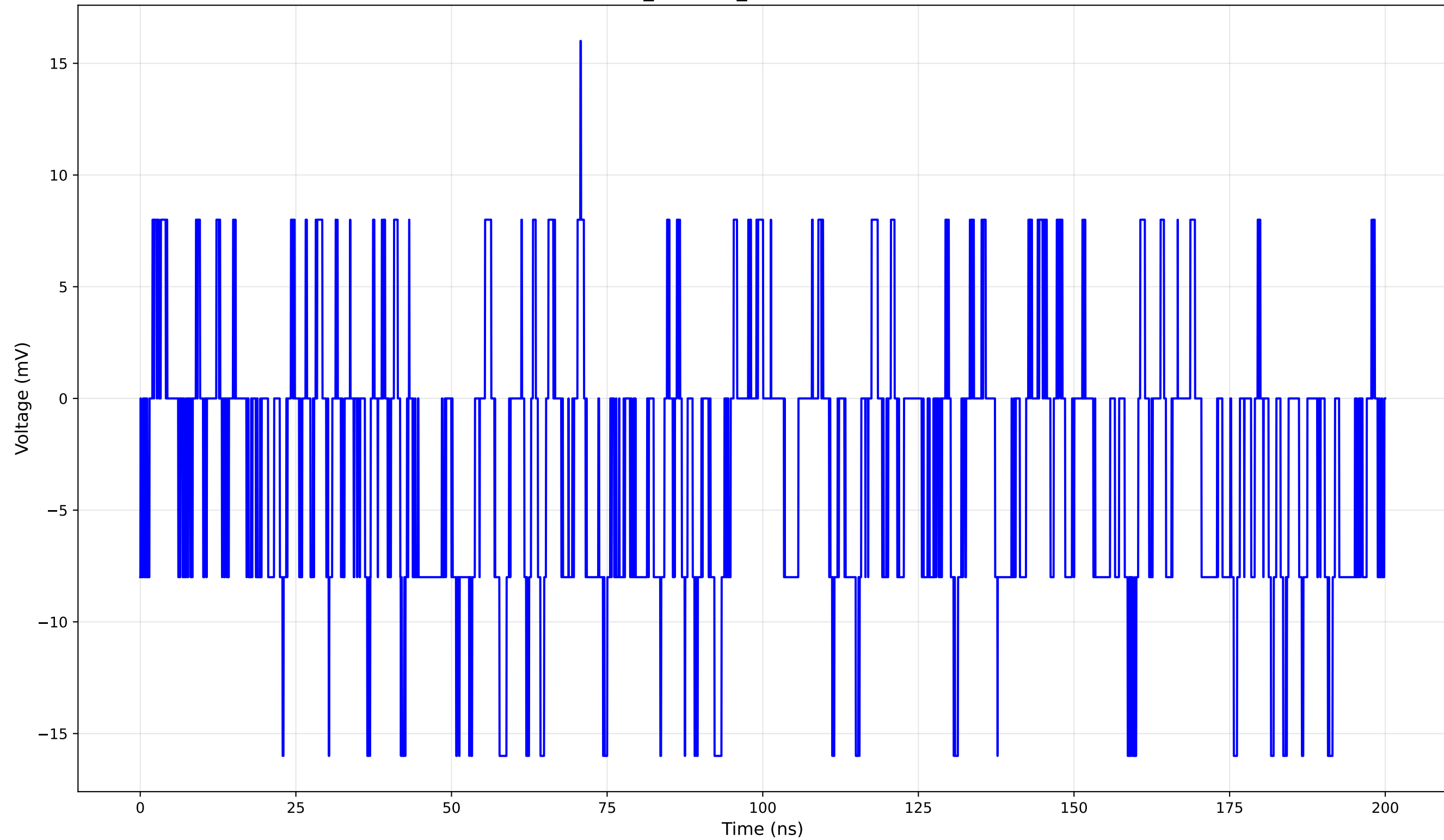
TCT Pulse Waveform - Run 1_30: 1cm_42-Position1 (30.0 V) - Rise Time: 0.46 ns
