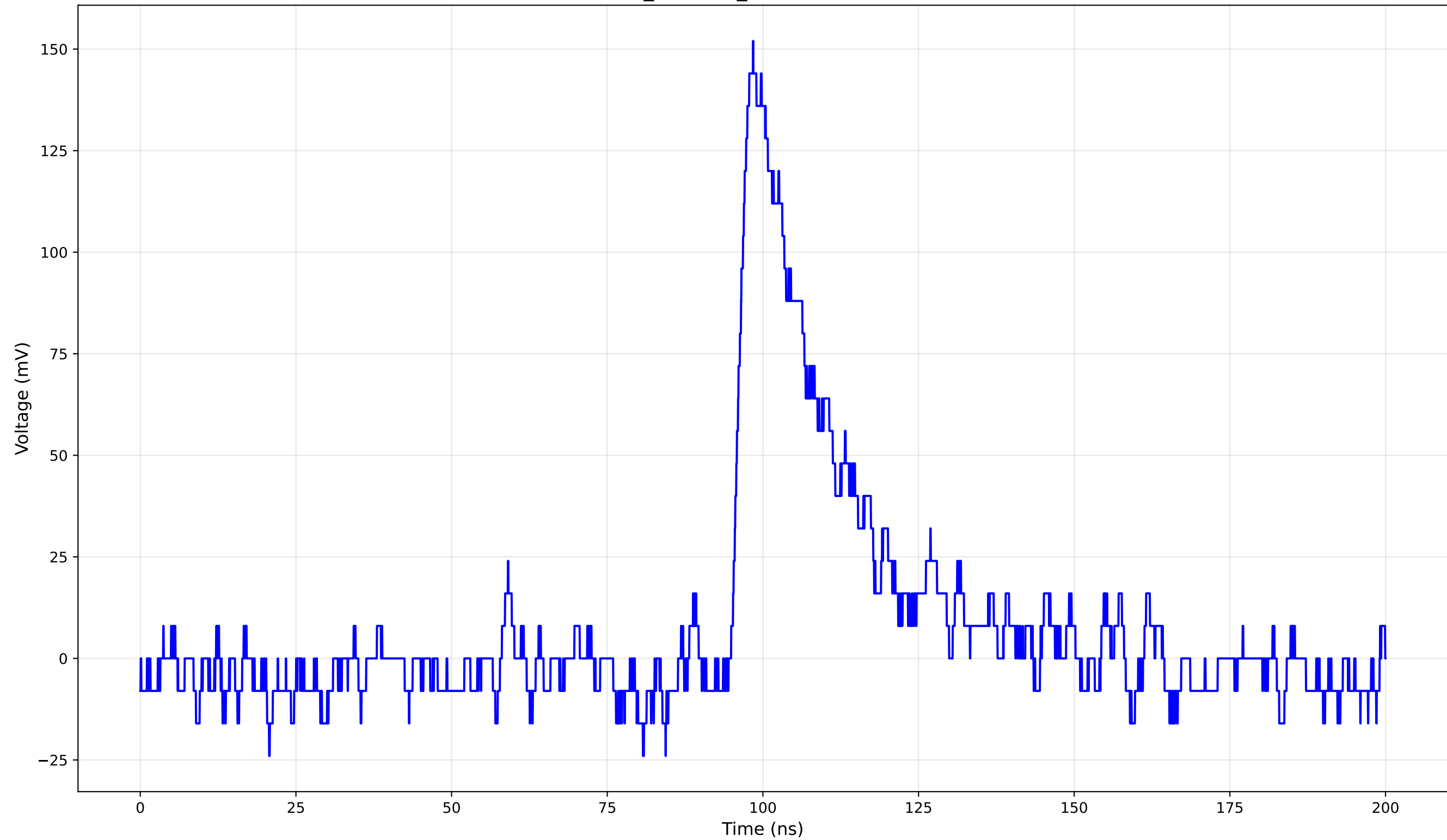
TCT Pulse Waveform - Run 1_40: 1cm_42-Position1 (40.0 V) - Rise Time: 2.61 ns
