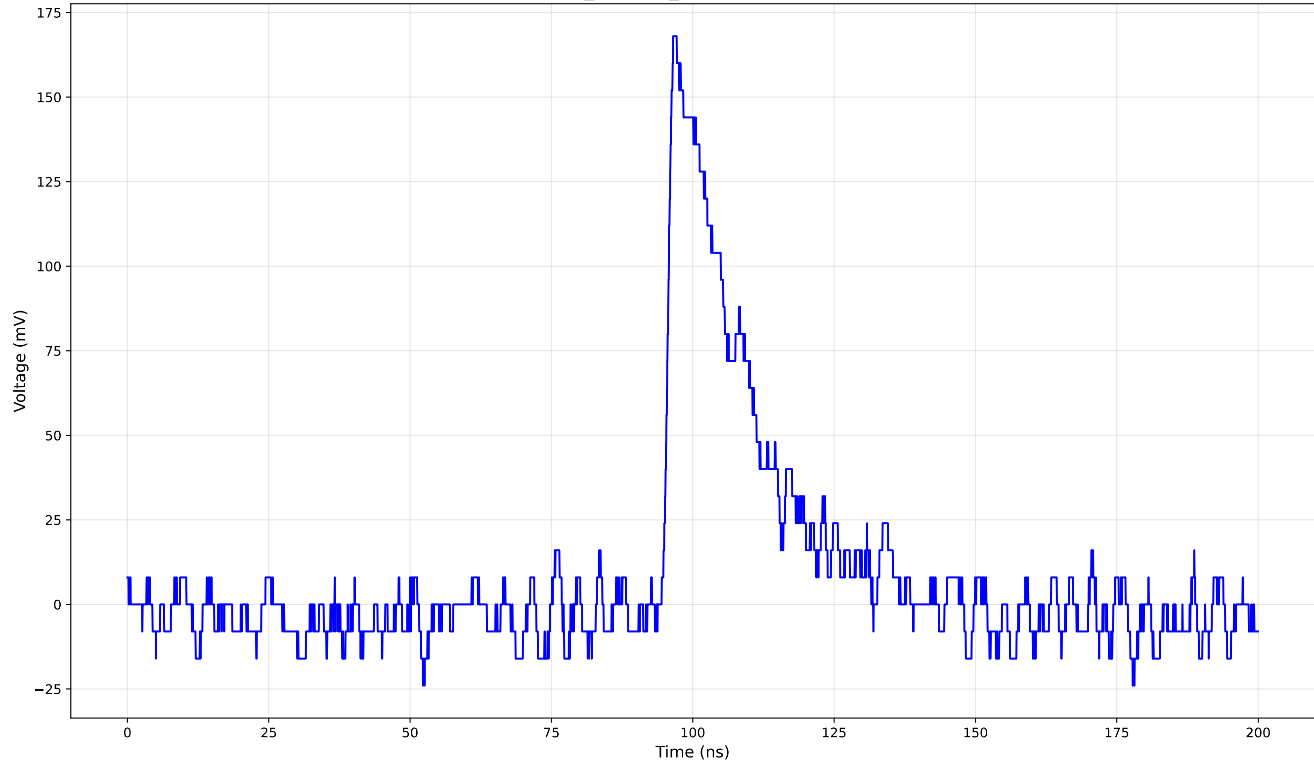
TCT Pulse Waveform - Run 1_50: 1cm_42-Position1 (50.0 V) - Rise Time: 1.30 ns
