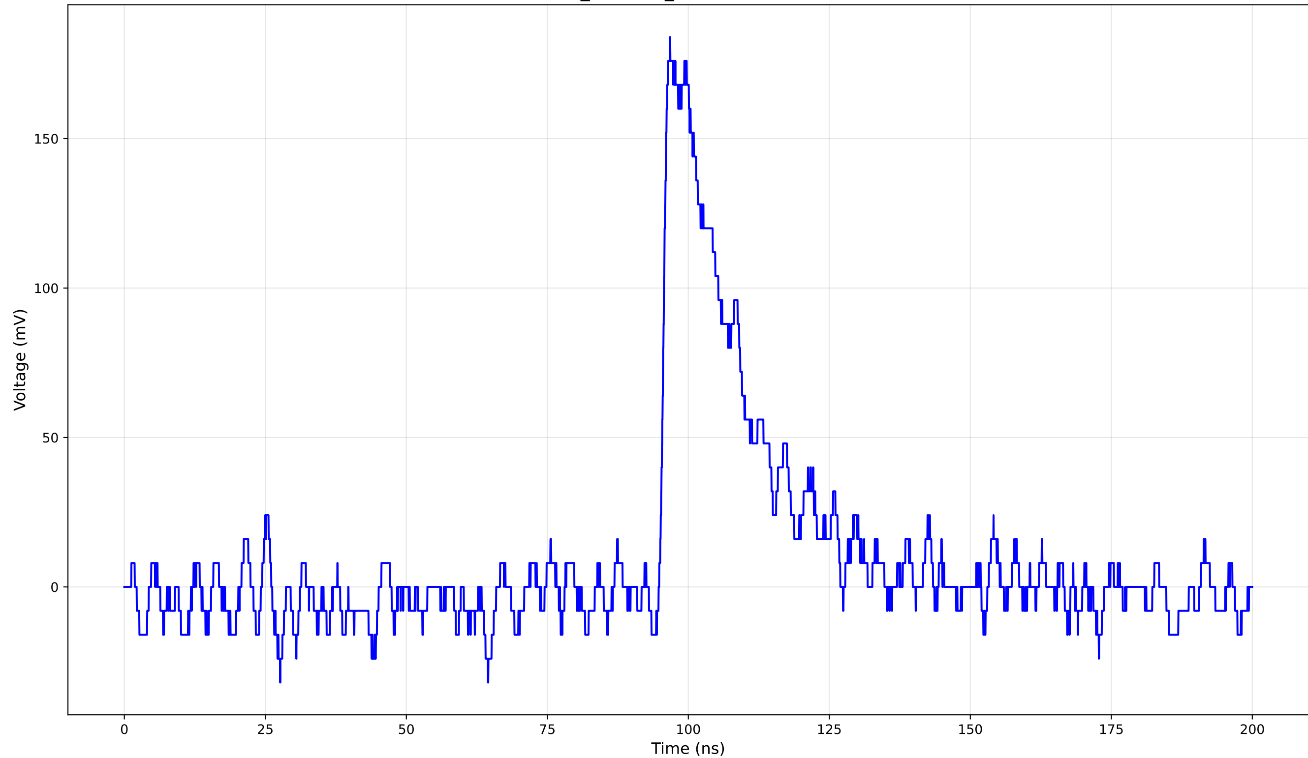
TCT Pulse Waveform - Run 1_60: 1cm_42-Position1 (60.0 V) - Rise Time: 1.22 ns
