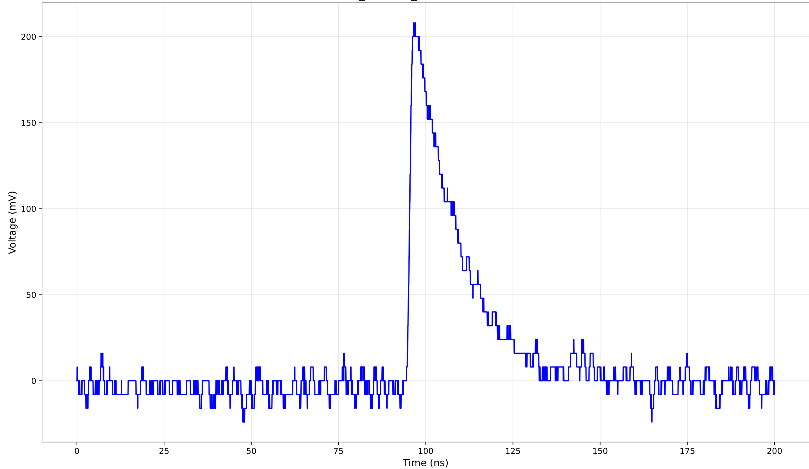
TCT Pulse Waveform - Run 1_70: 1cm_42-Position1 (70.0 V) - Rise Time: 1.29 ns
